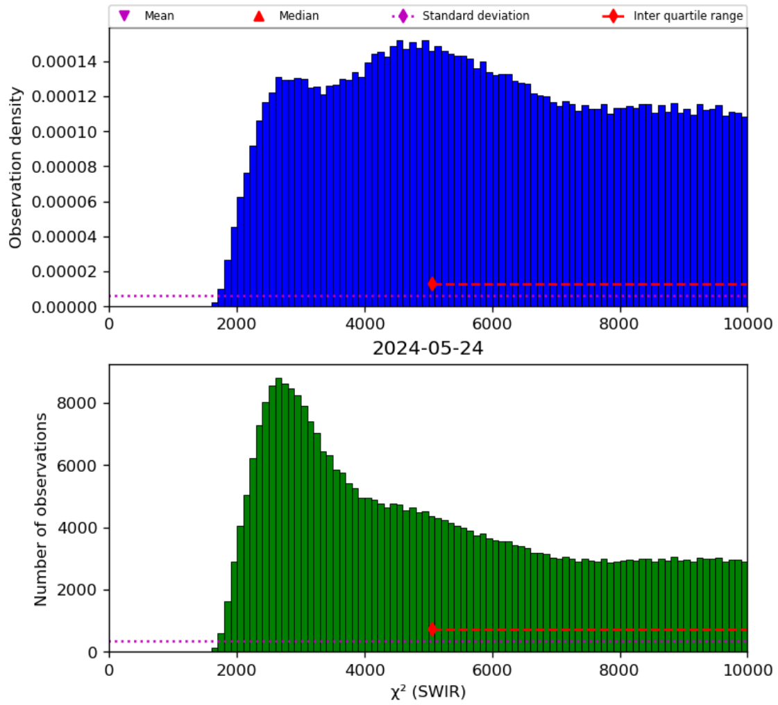
Figure 28: Histogram of “ \chi^2 (SWIR)” for 2024-05-23 to 2024-05-25
