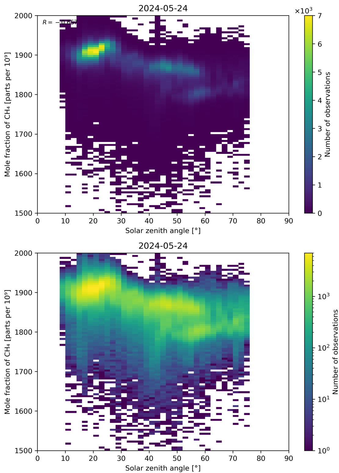
Figure 99: Scatter density plot of “Solar zenith angle” against “Mole fraction of CH 4 ” for 2024-05-23 to 2024-05-25.
