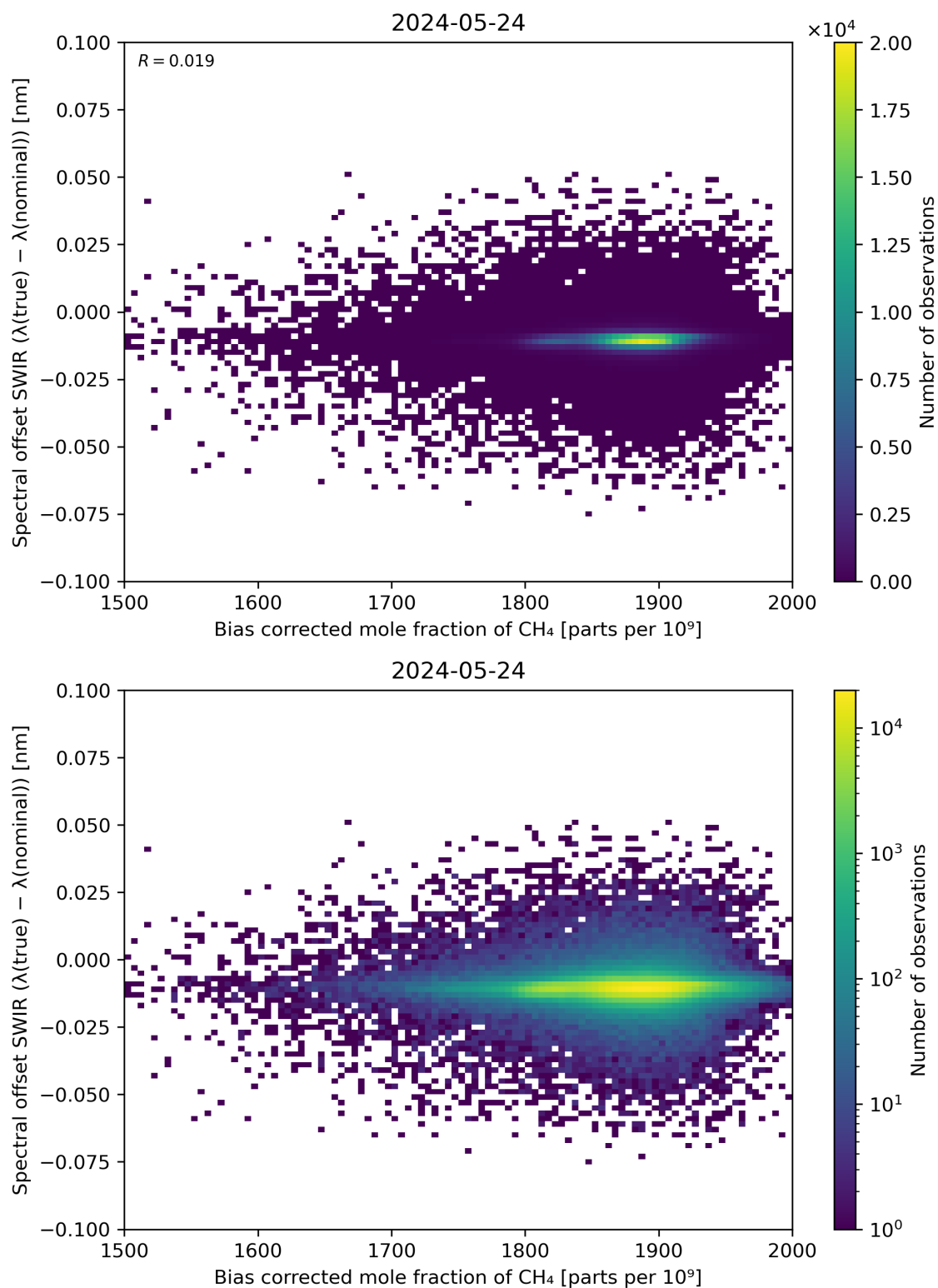
Figure 69: Scatter density plot of “Bias corrected mole fraction of \text{CH}_4 ” against “Spectral offset SWIR ( \lambda(\text{true}) - \lambda(\text{nominal}) )” for 2024-05-23 to 2024-05-25.
