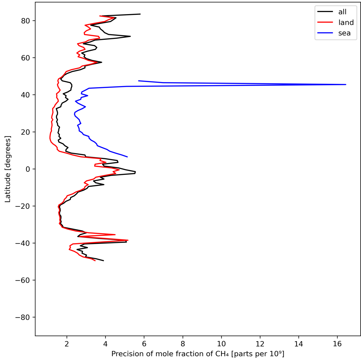
Figure 13: Zonal average of “Precision of mole fraction of CH 4 ” for 2024-05-23 to 2024-05-25.
