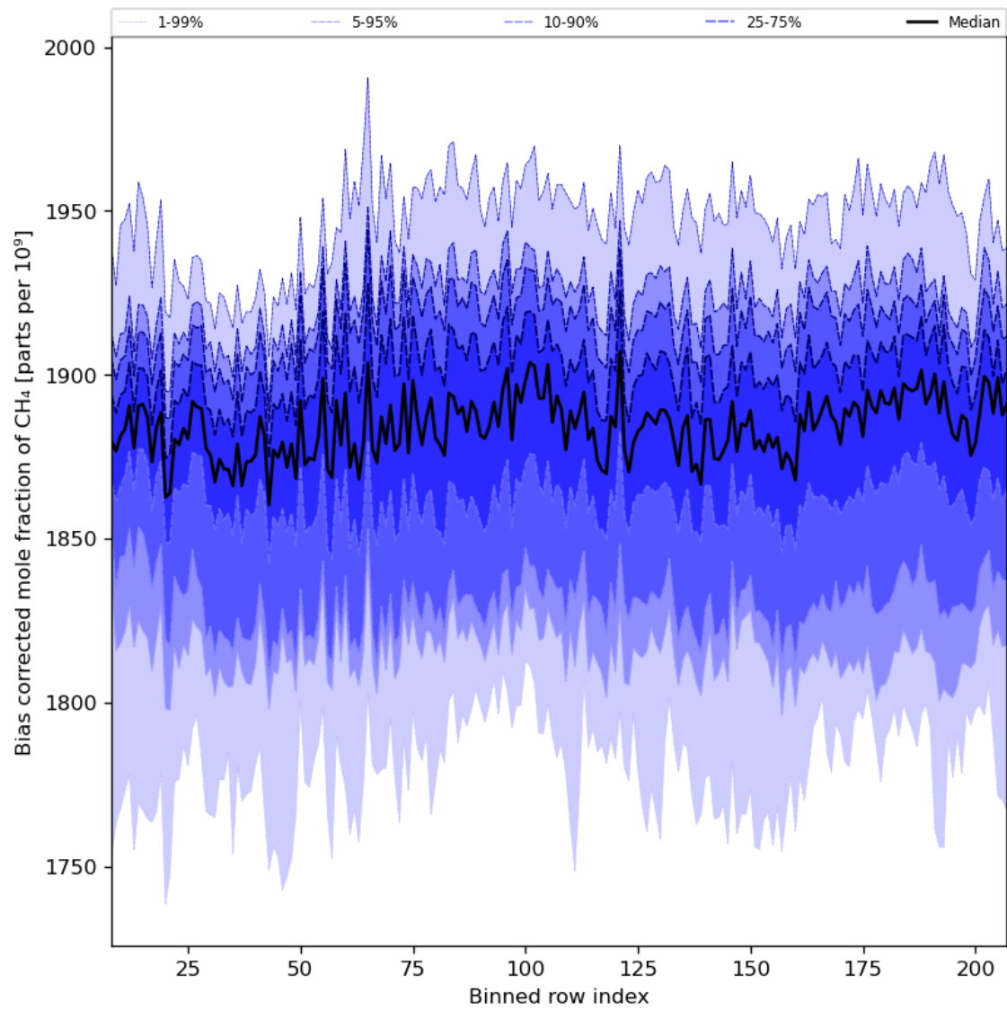
Figure 36: Along track statistics of “Bias corrected mole fraction of CH 4 ” for 2024-05-23 to 2024-05-25
