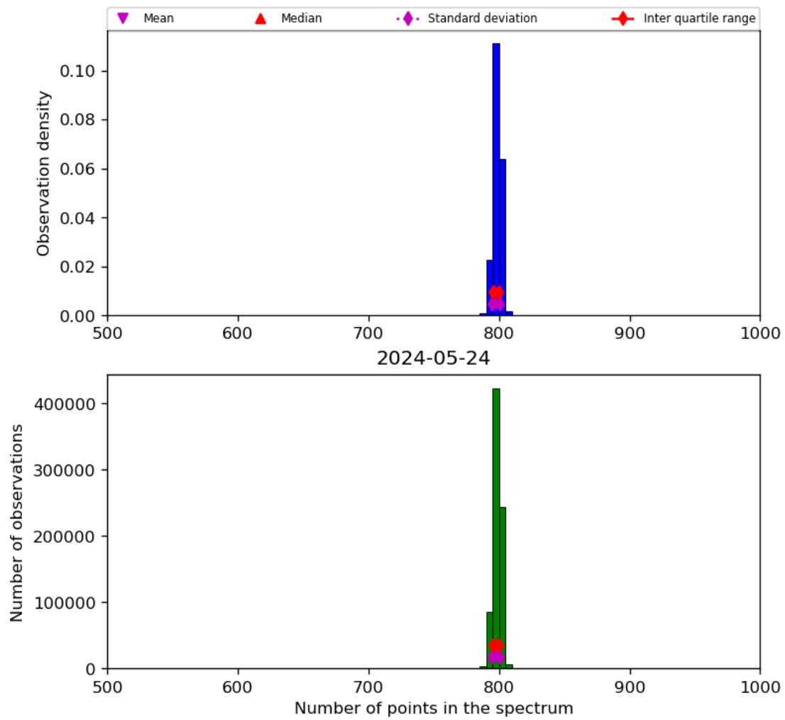
Figure 26: Histogram of “Number of points in the spectrum” for 2024-05-23 to 2024-05-25
