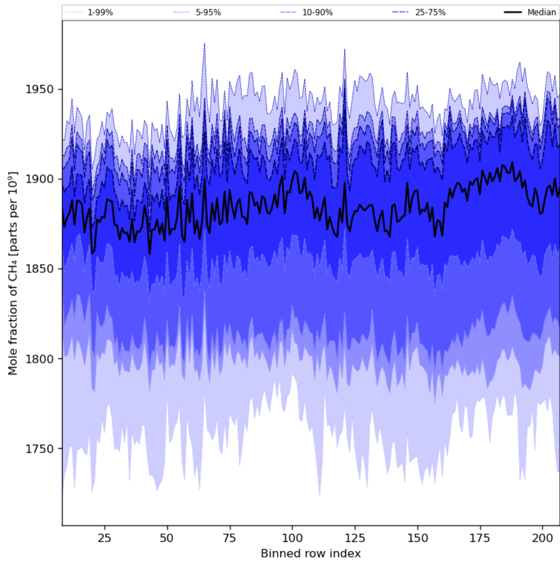
Figure 34: Along track statistics of “Mole fraction of CH 4 ” for 2024-05-23 to 2024-05-25
