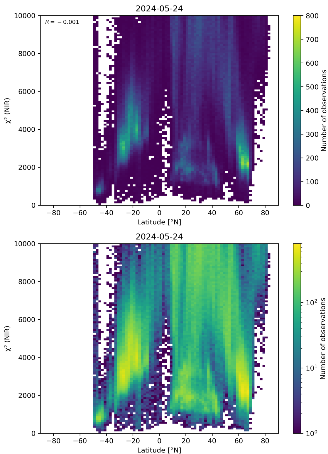
Figure 53: Scatter density plot of “Latitude” against “ \chi^2 (NIR)” for 2024-05-23 to 2024-05-25.
