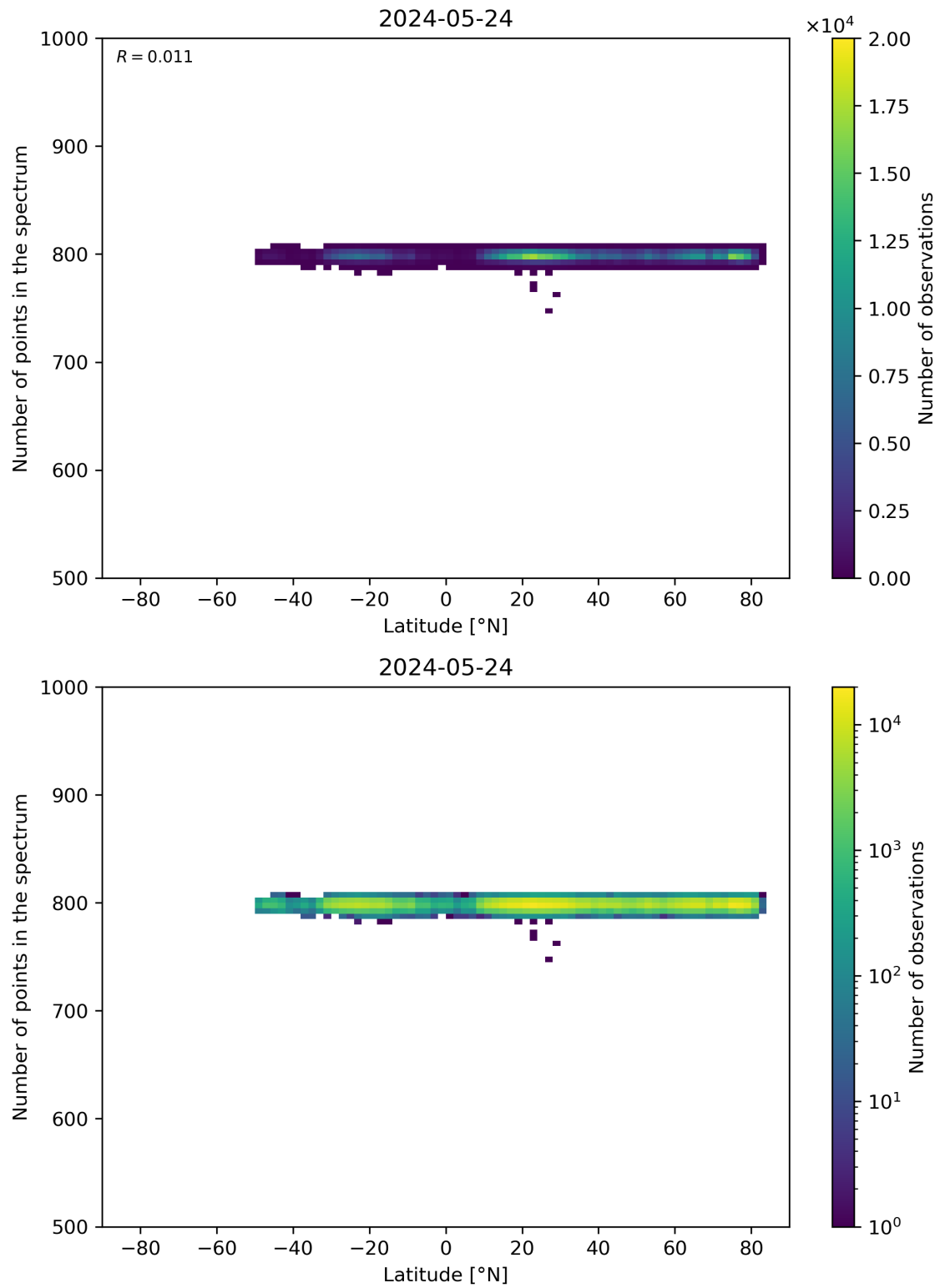
Figure 61: Scatter density plot of “Latitude” against “Number of points in the spectrum” for 2024-05-23 to 2024-05-25.
