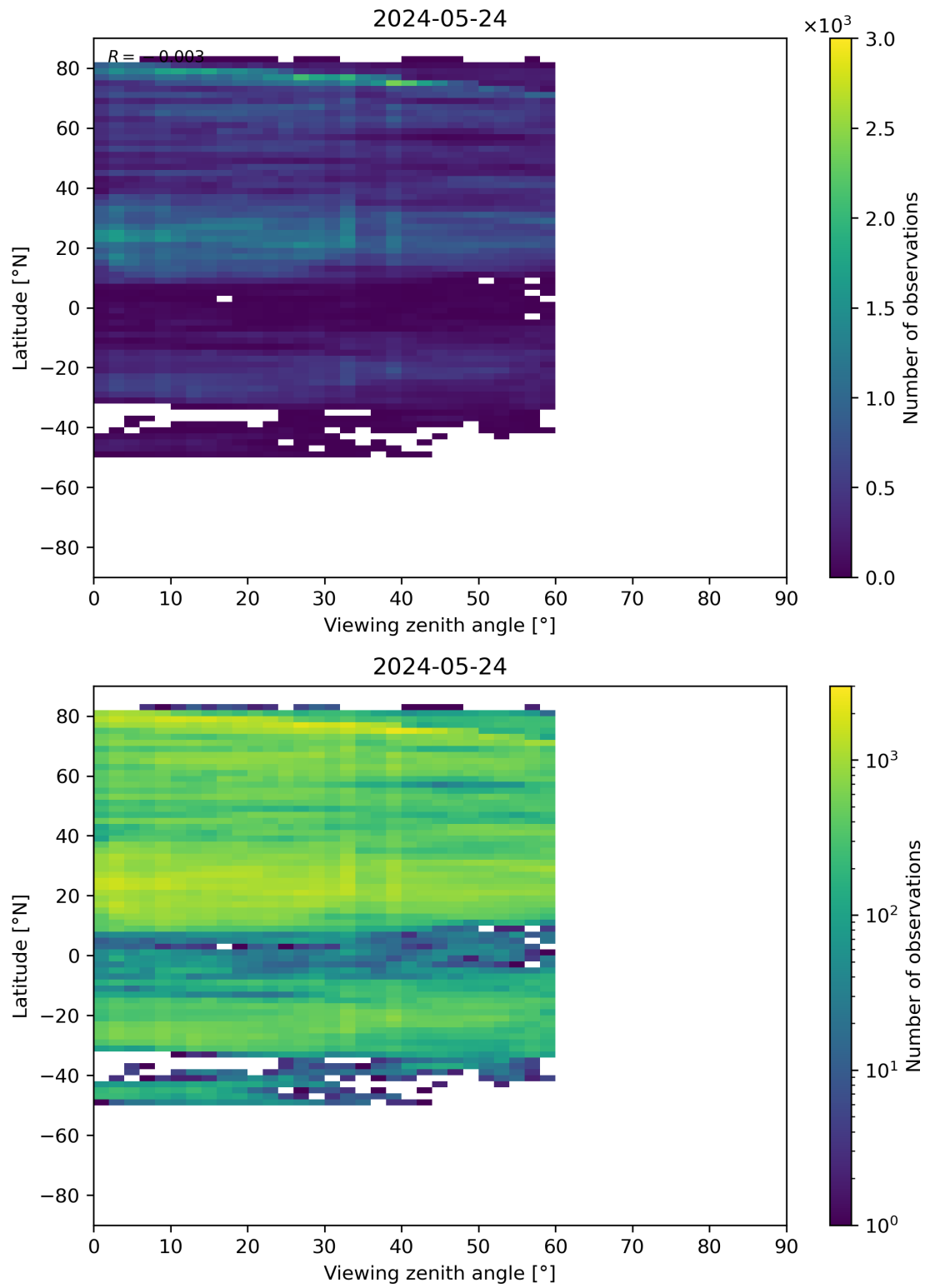
Figure 109: Scatter density plot of “Viewing zenith angle” against “Latitude” for 2024-05-23 to 2024-05-25.
