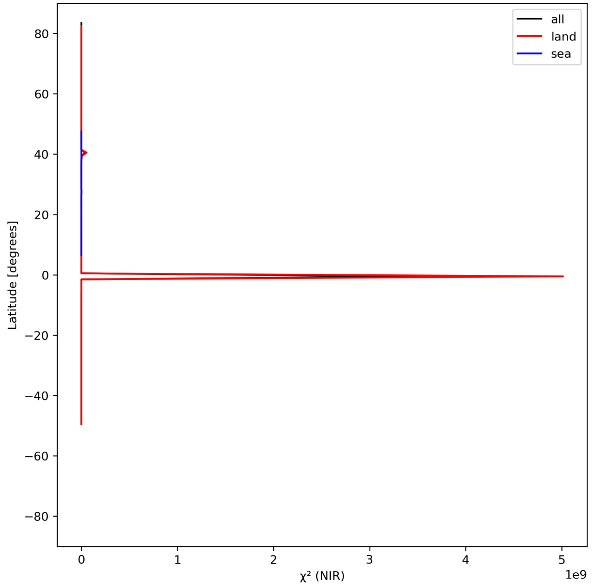
Figure 18: Zonal average of “ \chi^2 (NIR)” for 2024-05-23 to 2024-05-25.
