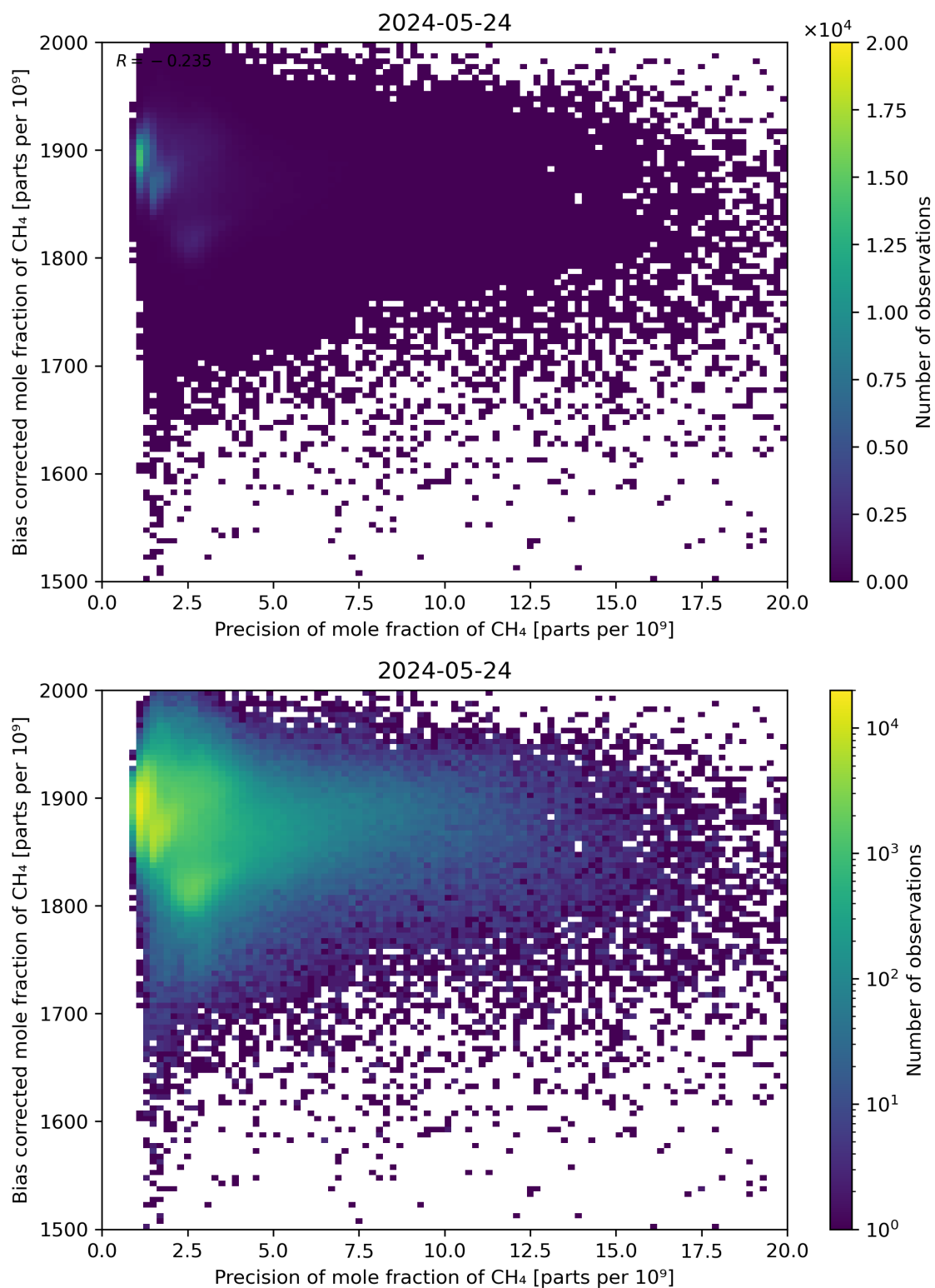
Figure 82: Scatter density plot of “Precision of mole fraction of CH 4 ” against “Bias corrected mole fraction of CH 4 ” for 2024-05-23 to 2024-05-25.
