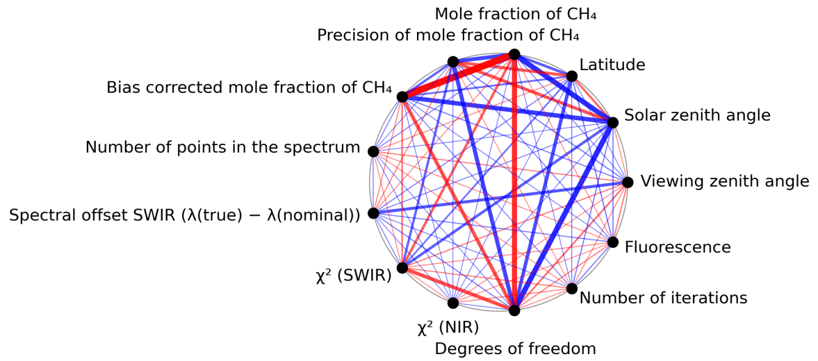
Figure 1: Map of correlation graph for 2024-05-23 to 2024-05-25.
