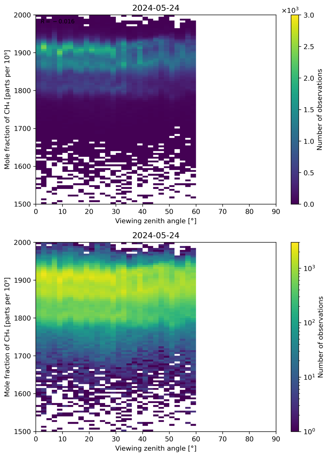
Figure 110: Scatter density plot of “Viewing zenith angle” against “Mole fraction of CH 4 ” for 2024-05-23 to 2024-05-25.
