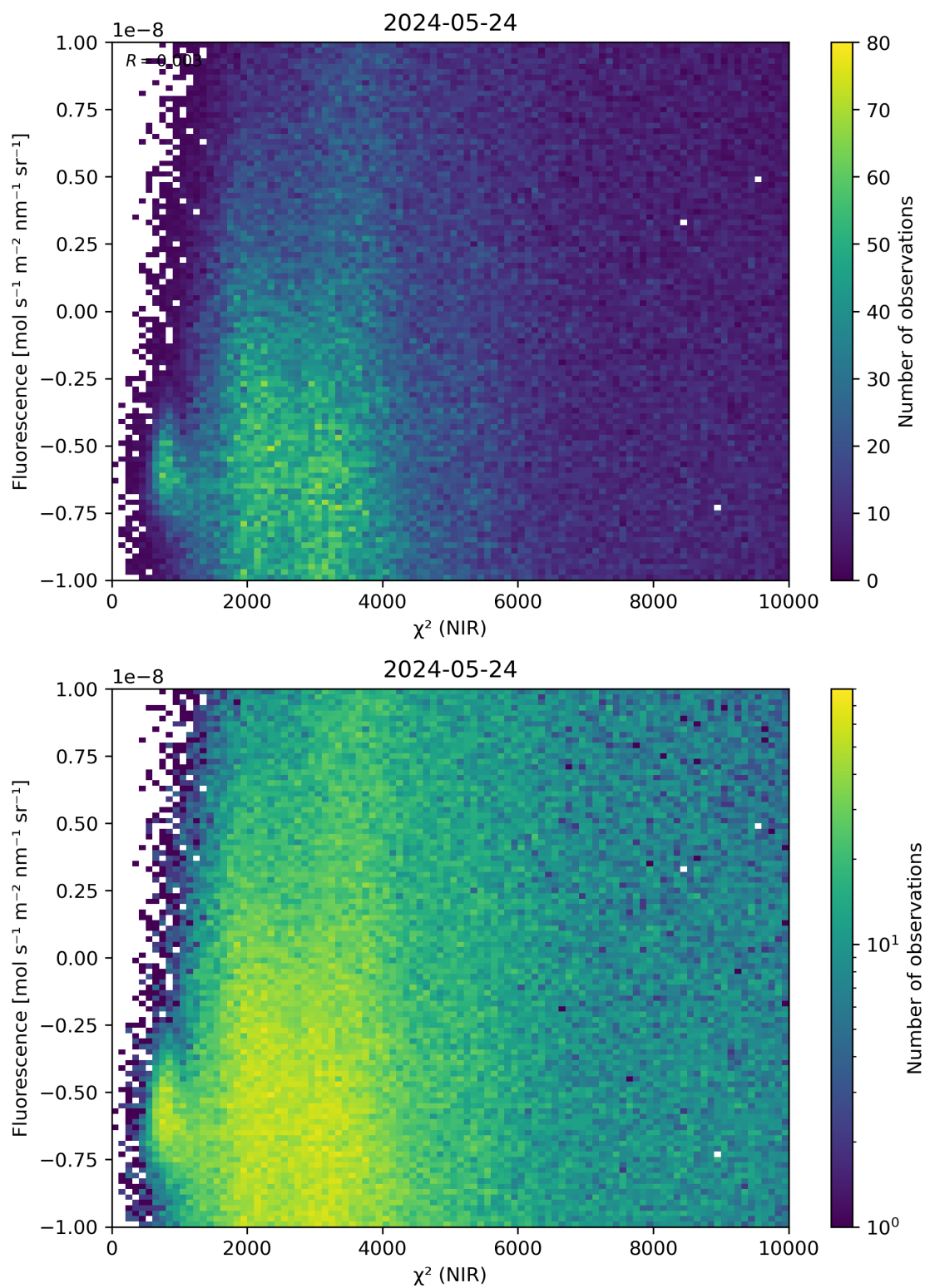
Figure 45: Scatter density plot of “ \chi^2 (NIR)” against “Fluorescence” for 2024-05-23 to 2024-05-25.
