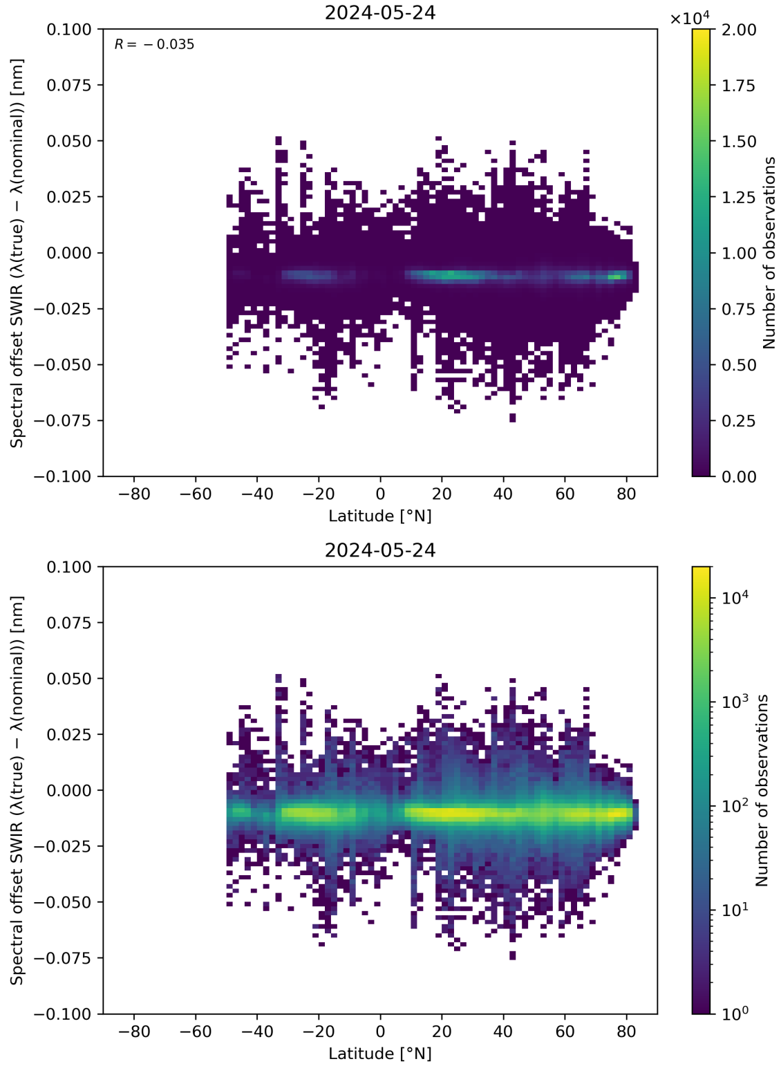
Figure 62: Scatter density plot of “Latitude” against “Spectral offset SWIR ( \lambda(\text{true}) - \lambda(\text{nominal}) )” for 2024-05-23 to 2024-05-25.
