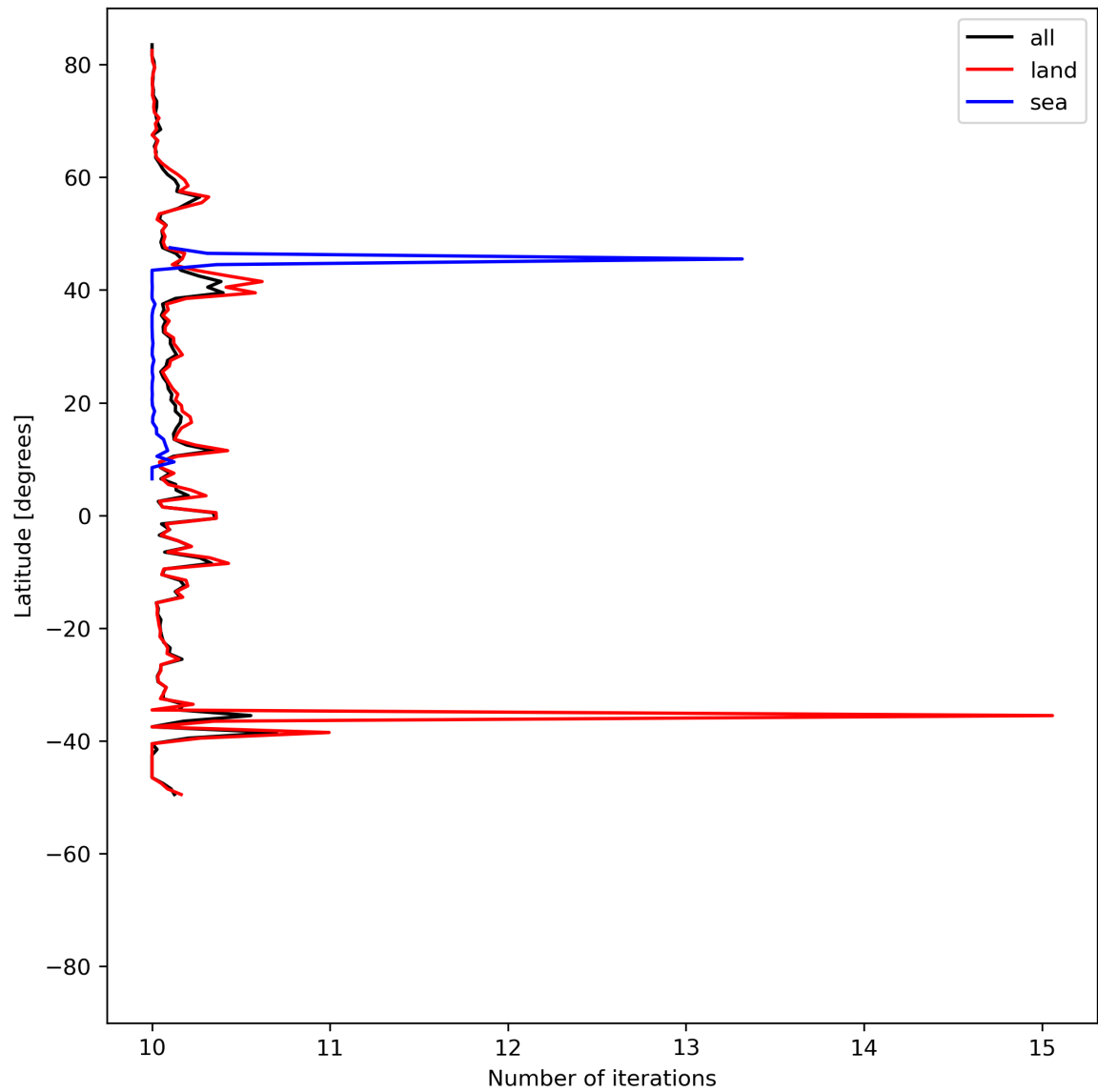
Figure 20: Zonal average of “Number of iterations” for 2024-05-23 to 2024-05-25.
