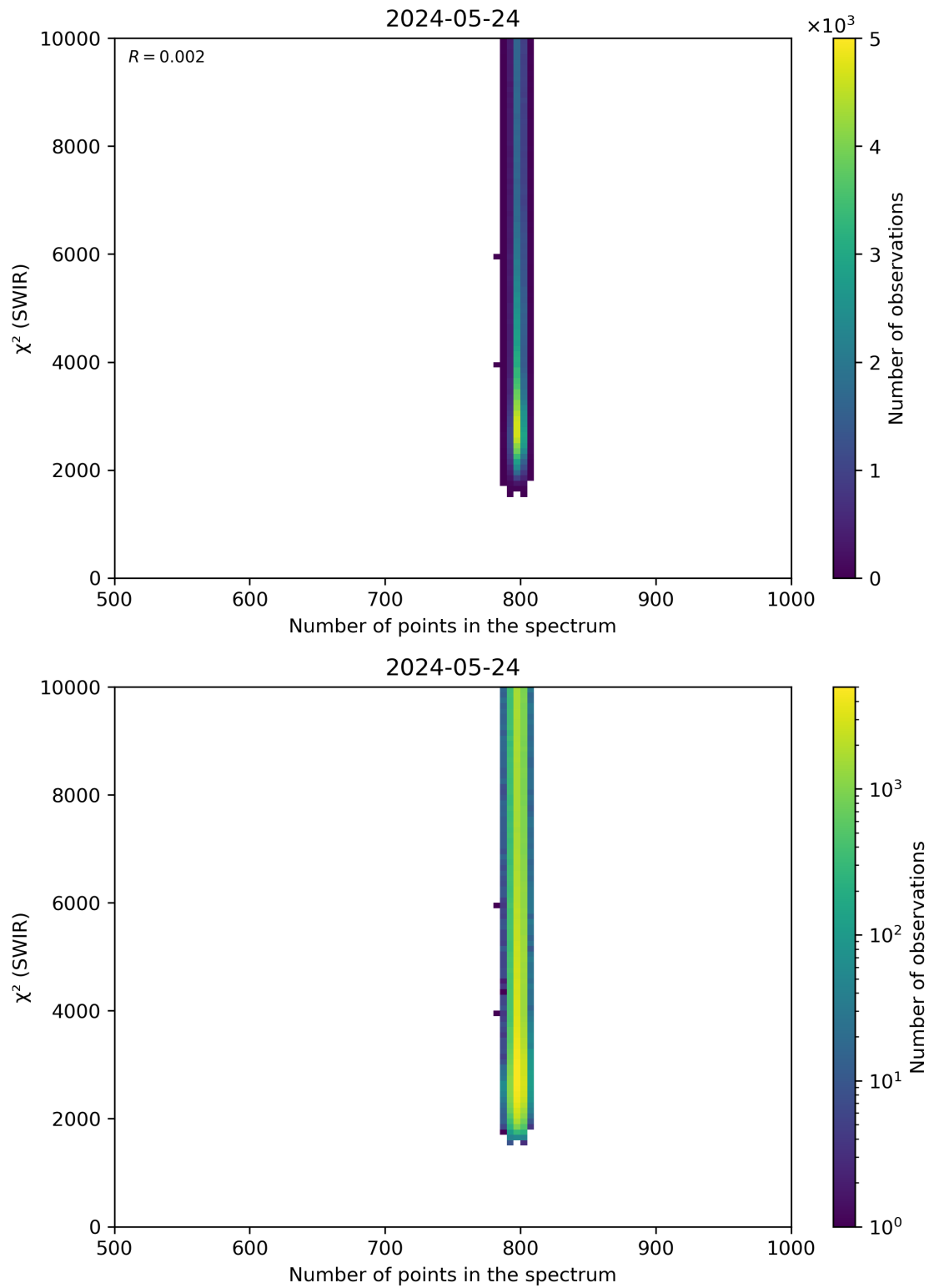
Figure 89: Scatter density plot of “Number of points in the spectrum” against “ \chi^2 (SWIR)” for 2024-05-23 to 2024-05-25.
