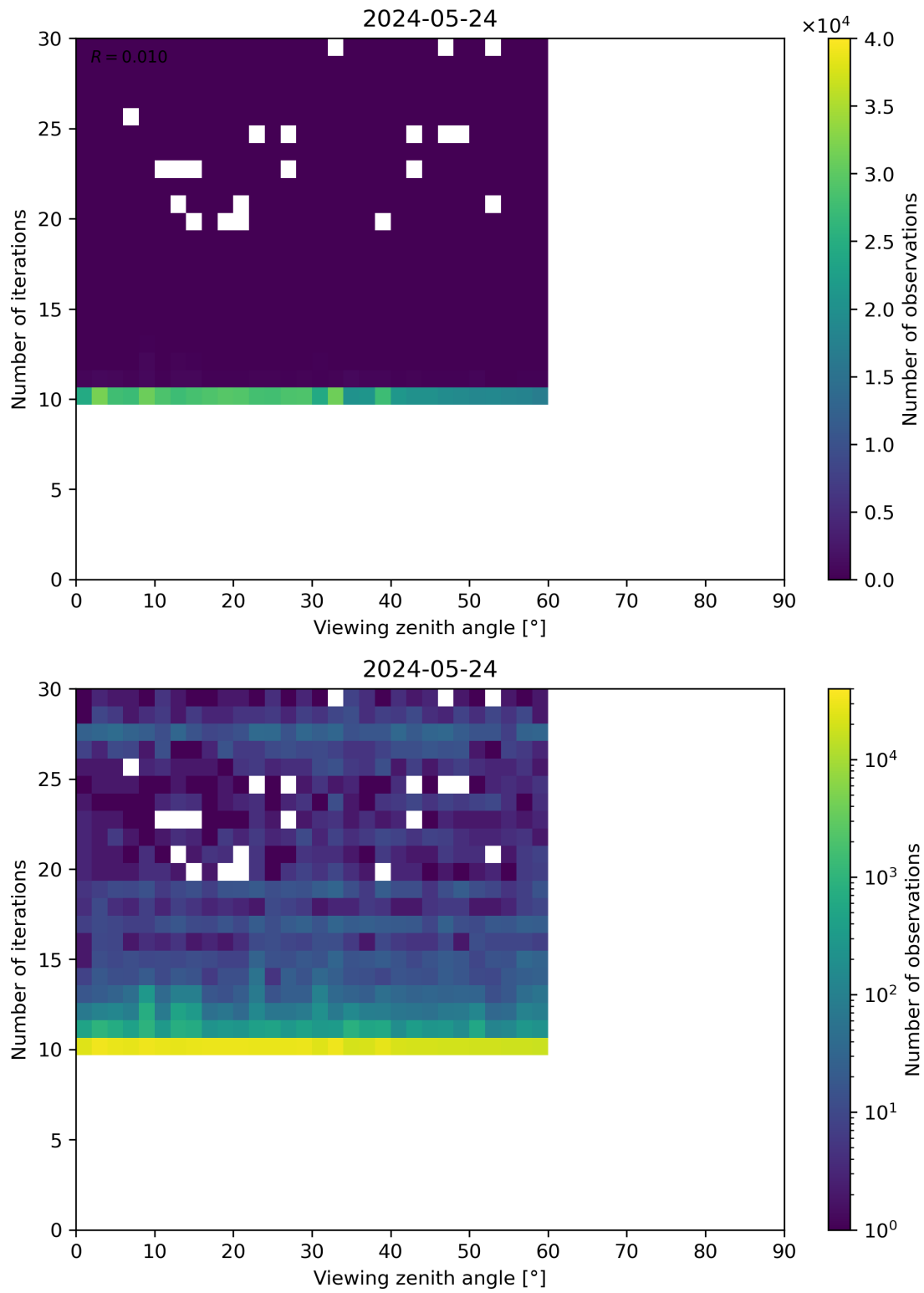
Figure 113: Scatter density plot of “Viewing zenith angle” against “Number of iterations” for 2024-05-23 to 2024-05-25.
