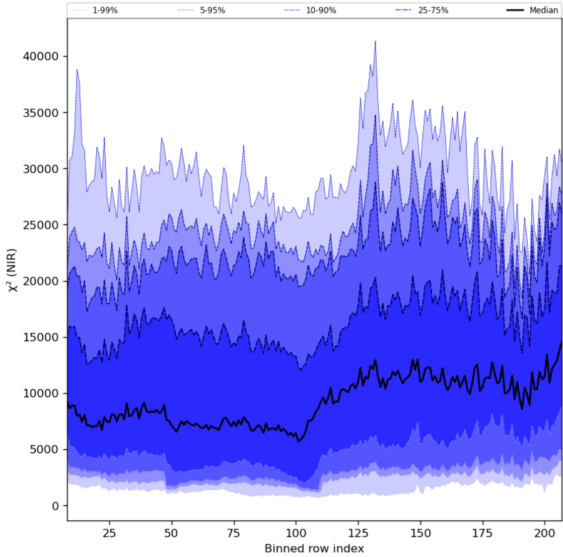
Figure 40: Along track statistics of “ \chi^2 (NIR)” for 2024-05-23 to 2024-05-25
