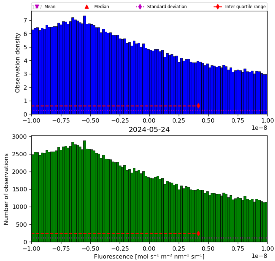
Figure 32: Histogram of “Fluorescence” for 2024-05-23 to 2024-05-25
