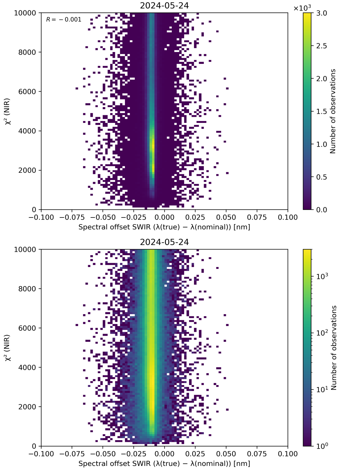
Figure 117: Scatter density plot of “Spectral offset SWIR ( \lambda(\text{true}) - \lambda(\text{nominal}) )” against “ \chi^2 (NIR)” for 2024-05-23 to 2024-05-25.
