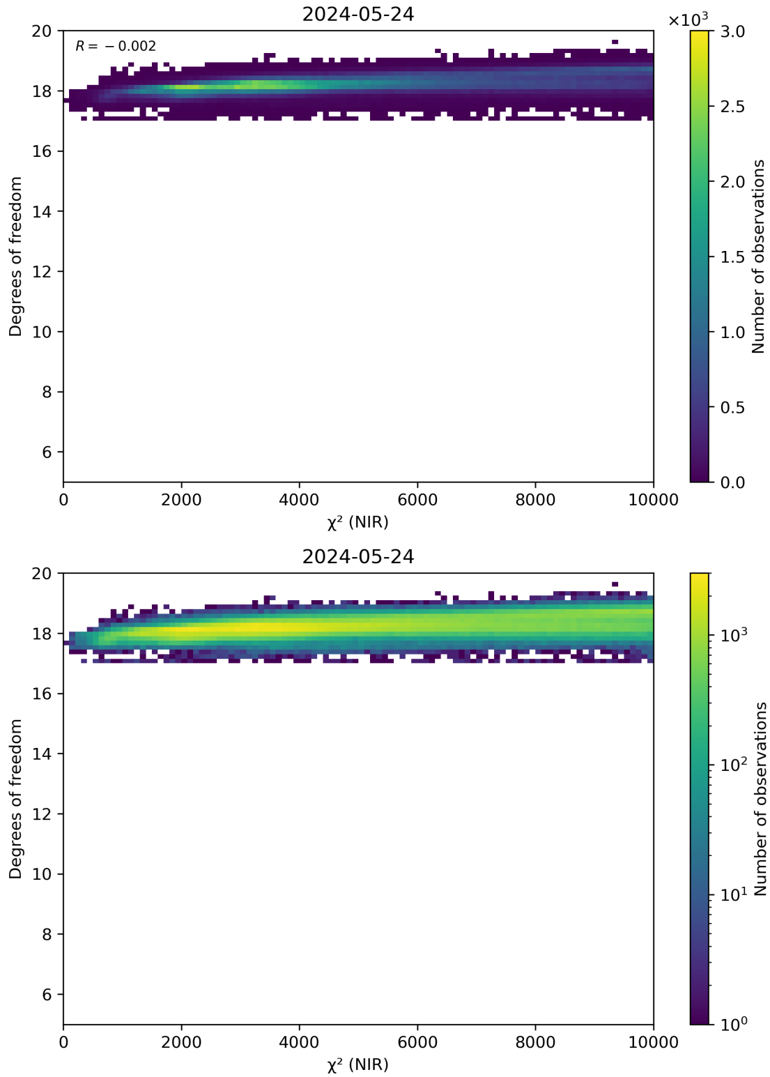
Figure 44: Scatter density plot of “ \chi^2 (NIR)” against “Degrees of freedom” for 2024-05-23 to 2024-05-25.
