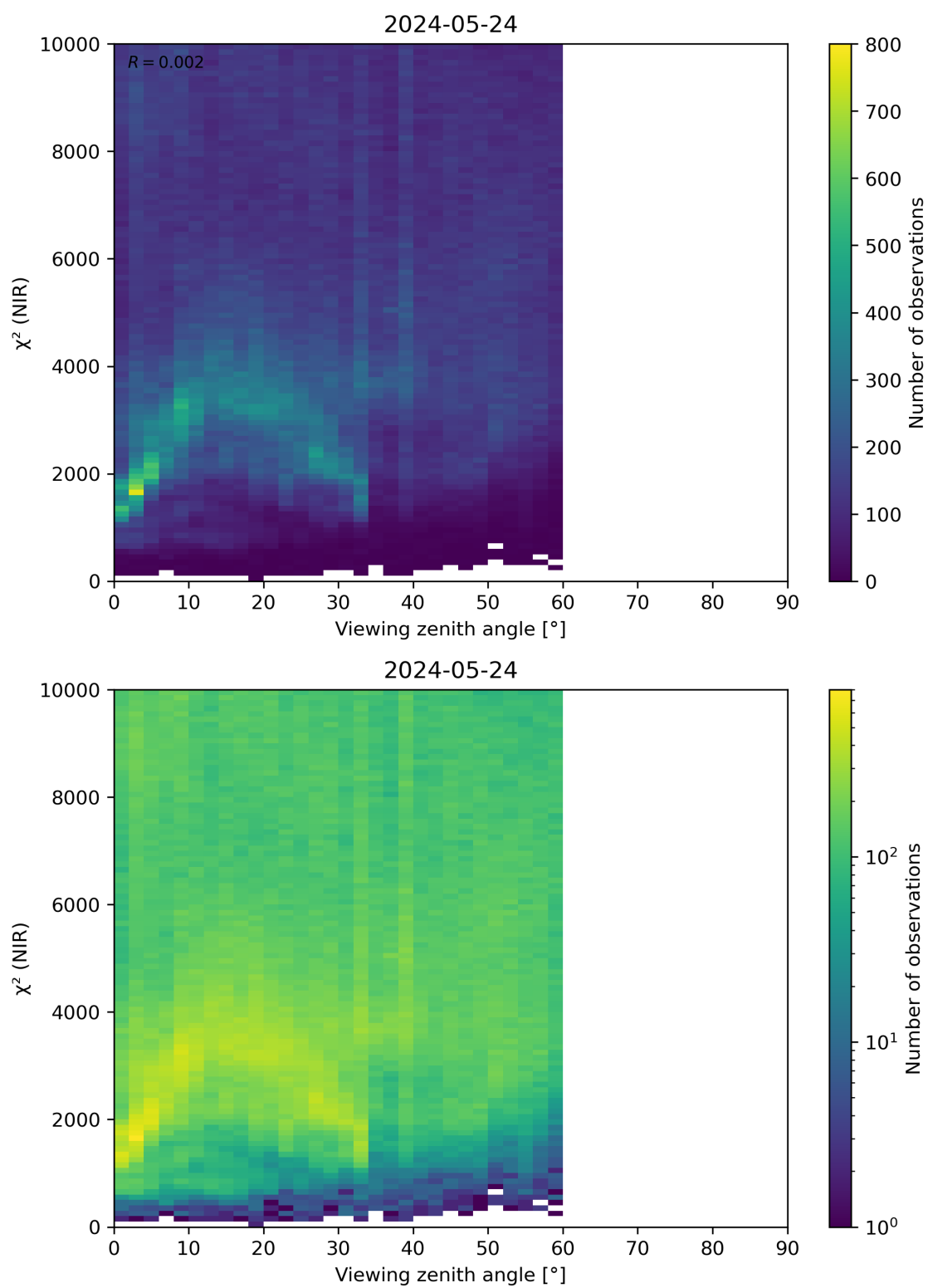
Figure 105: Scatter density plot of “Viewing zenith angle” against “ \chi^2 (NIR)” for 2024-05-23 to 2024-05-25.
