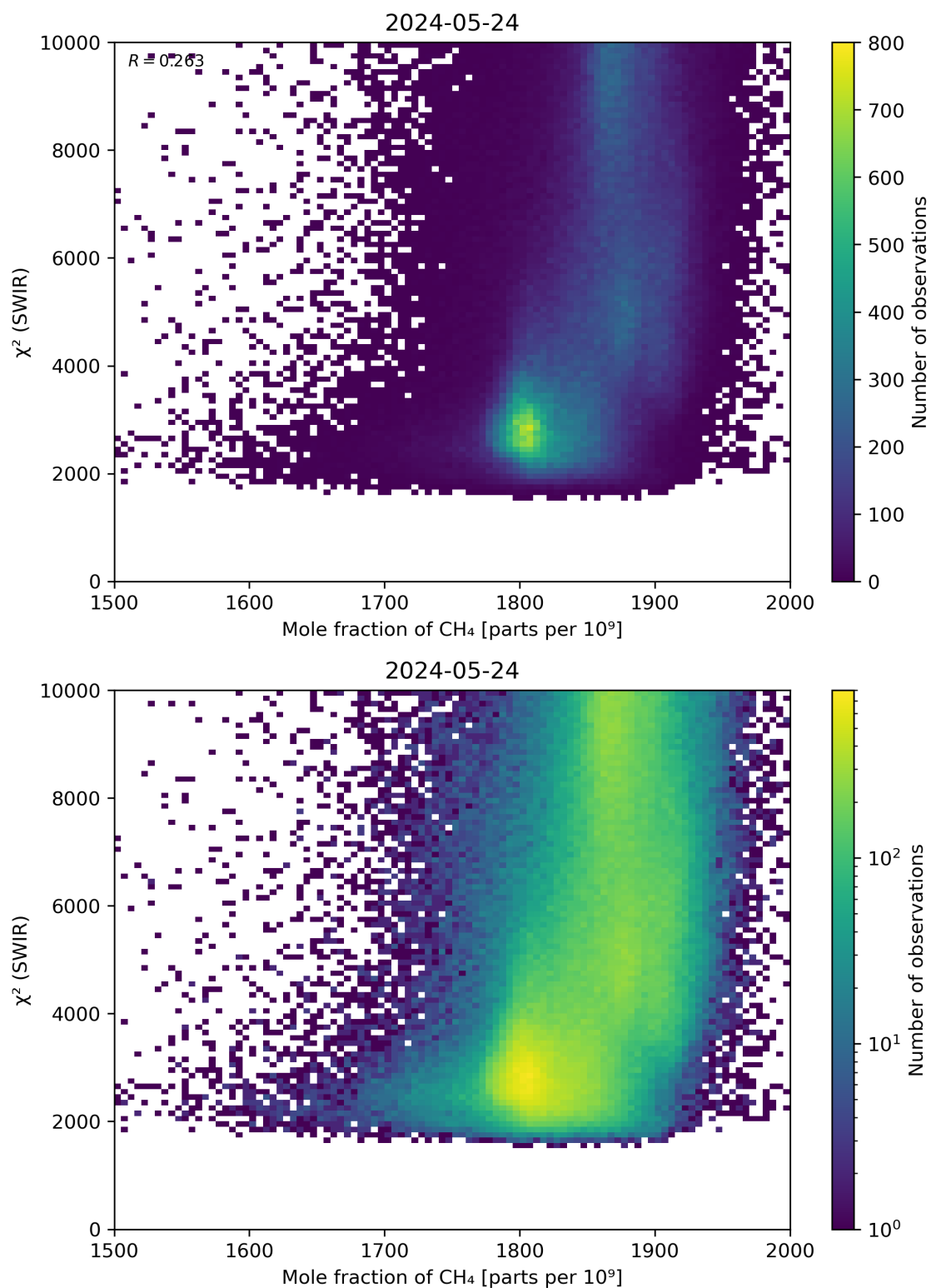
Figure 71: Scatter density plot of “Mole fraction of \text{CH}_4 ” against “ \chi^2 (SWIR)” for 2024-05-23 to 2024-05-25.
