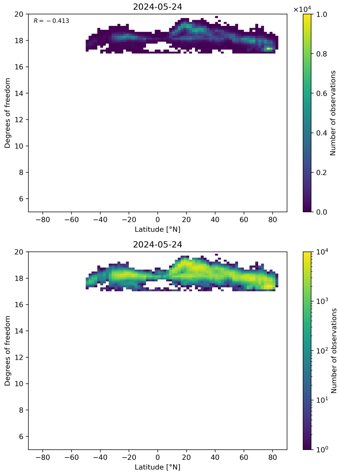
Figure 55: Scatter density plot of “Latitude” against “Degrees of freedom” for 2024-05-23 to 2024-05-25.
