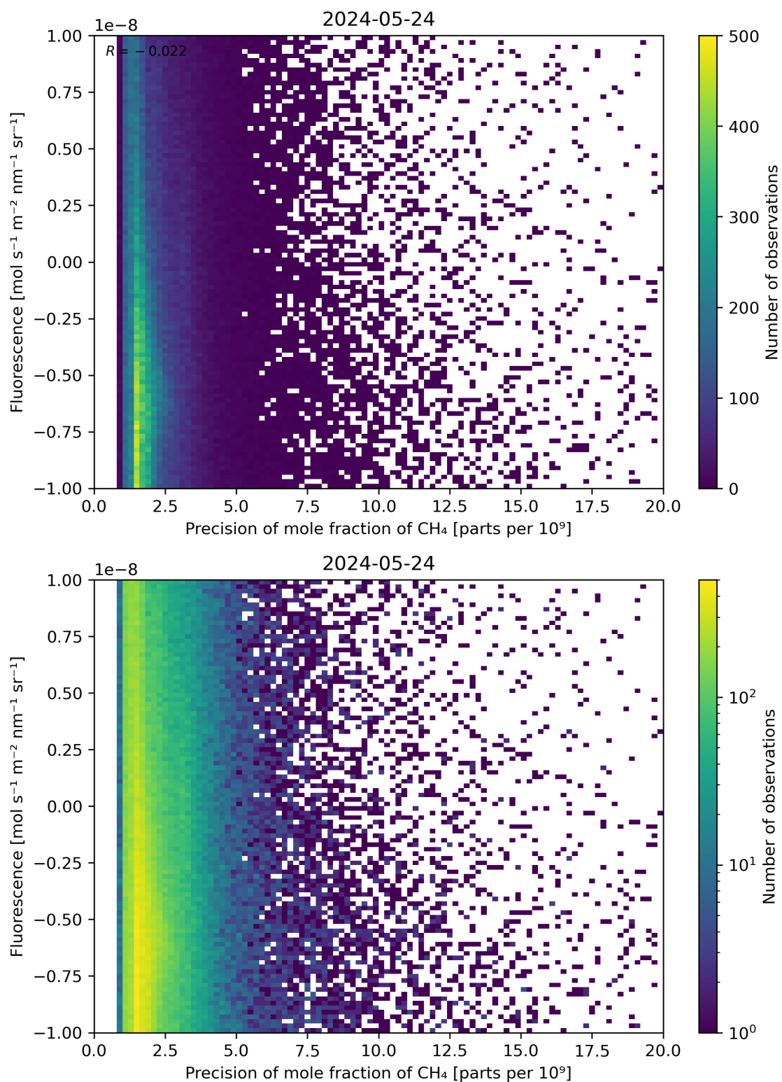
Figure 81: Scatter density plot of “Precision of mole fraction of \text{CH}_4 ” against “Fluorescence” for 2024-05-23 to 2024-05-25.
