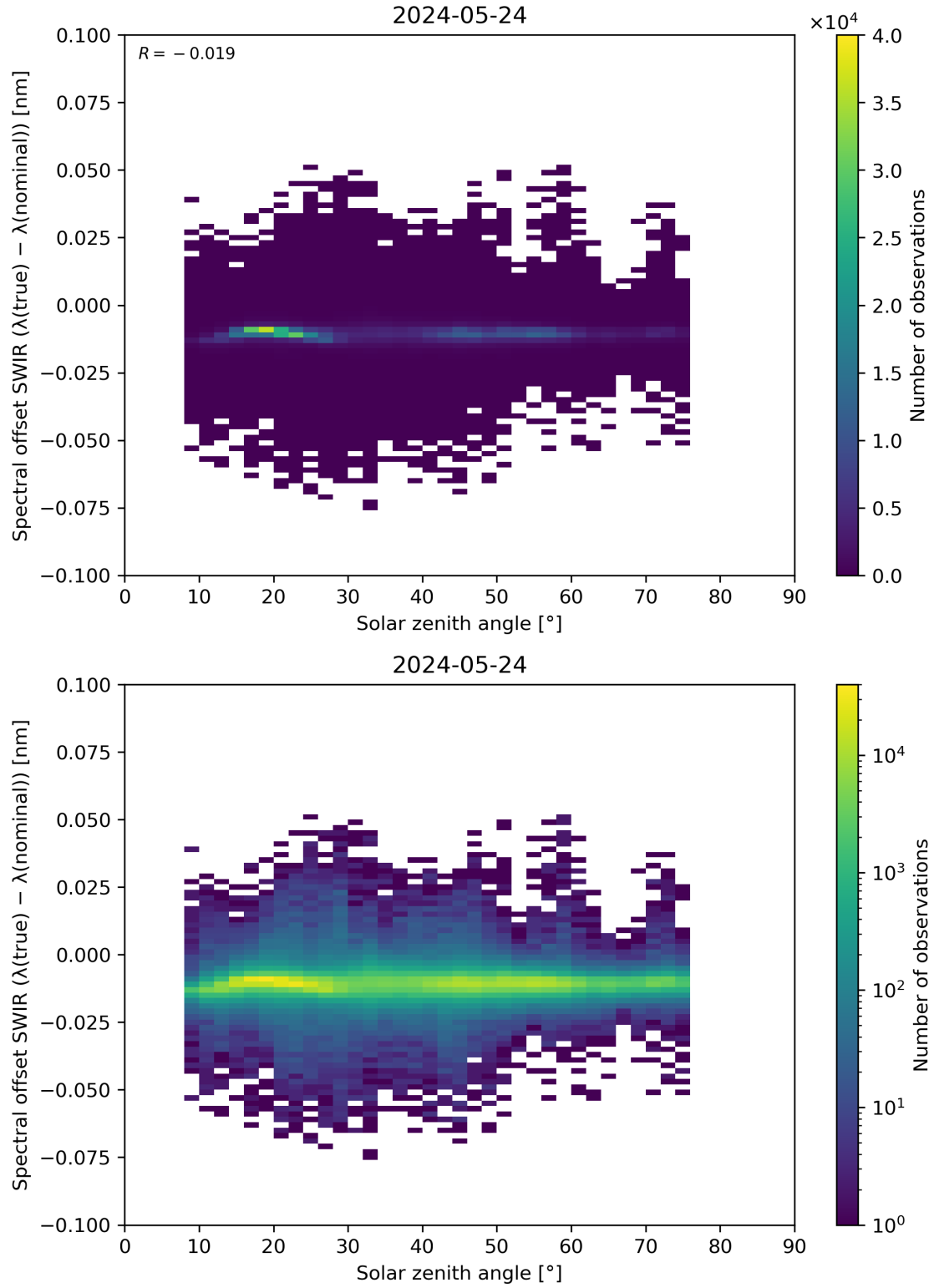
Figure 104: Scatter density plot of “Solar zenith angle” against “Spectral offset SWIR ( \lambda(\text{true}) - \lambda(\text{nominal}) )” for 2024-05-23 to 2024-05-25.
