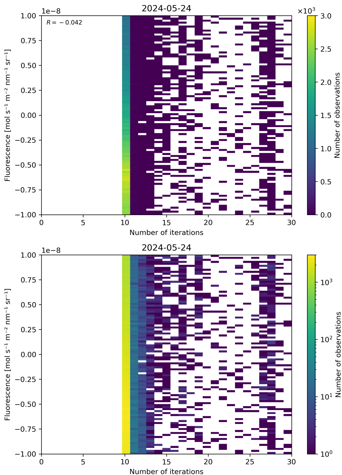
Figure 87: Scatter density plot of “Number of iterations” against “Fluorescence” for 2024-05-23 to 2024-05-25.
