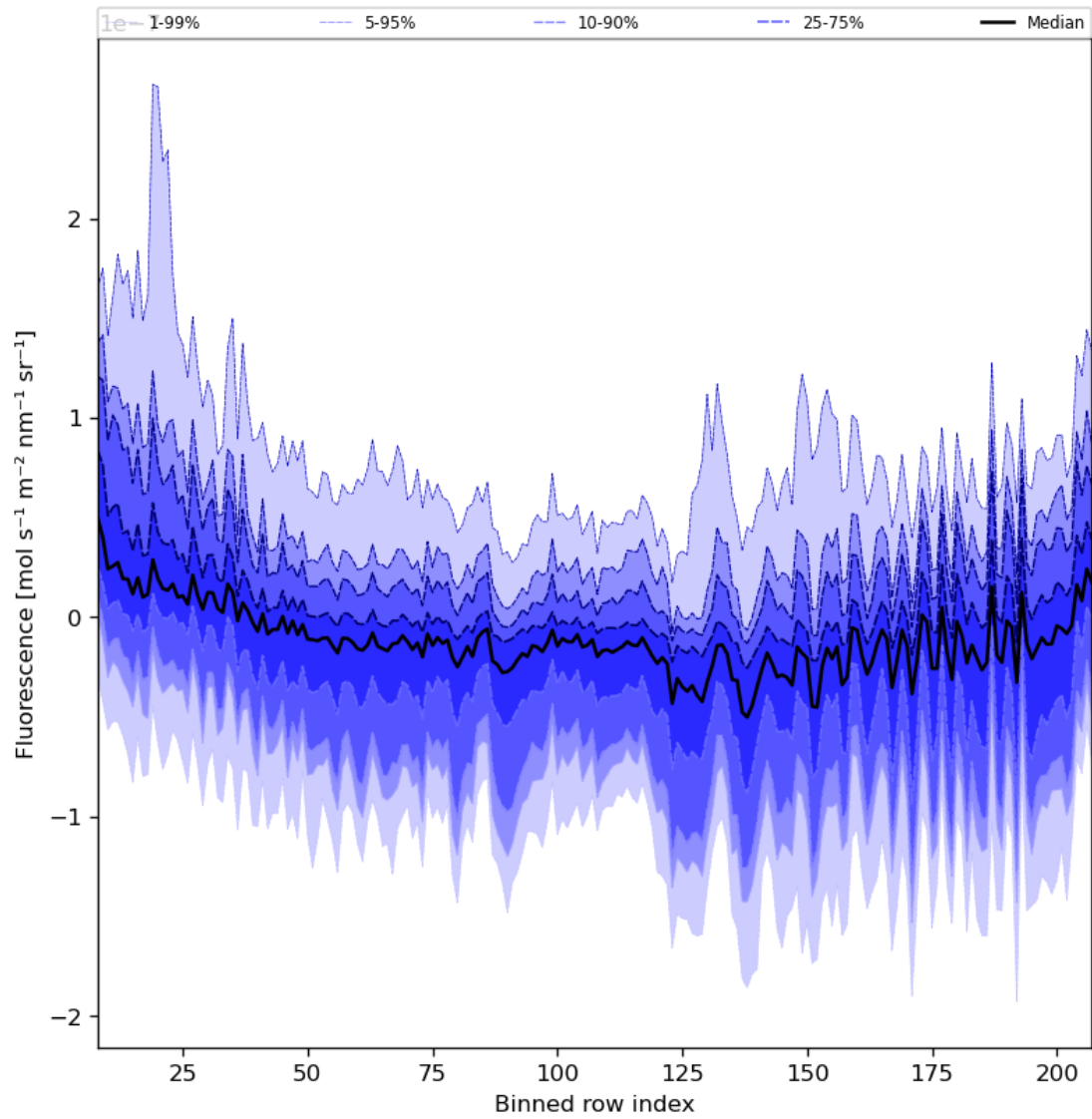
Figure 43: Along track statistics of “Fluorescence” for 2024-05-23 to 2024-05-25
