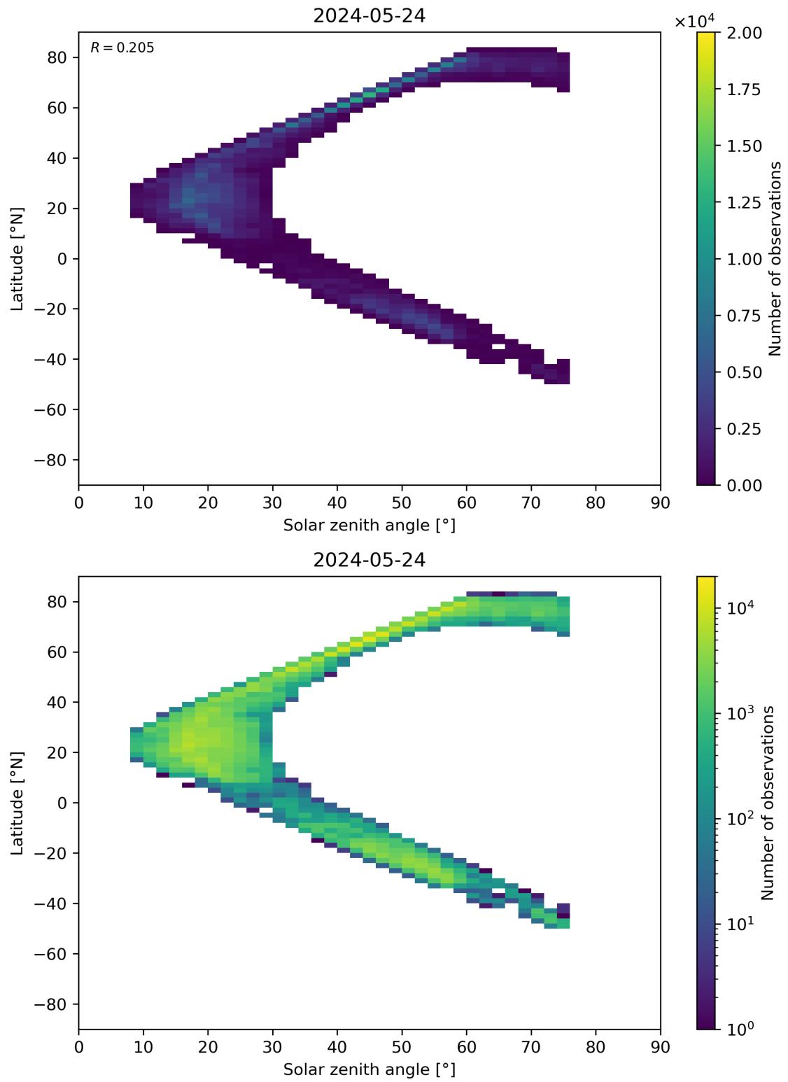
Figure 98: Scatter density plot of “Solar zenith angle” against “Latitude” for 2024-05-23 to 2024-05-25.
