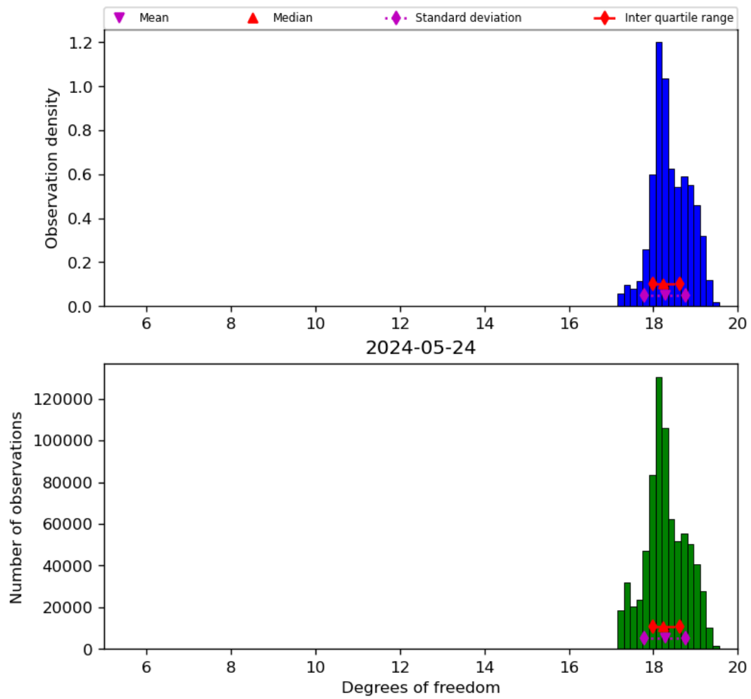
Figure 30: Histogram of “Degrees of freedom” for 2024-05-23 to 2024-05-25
