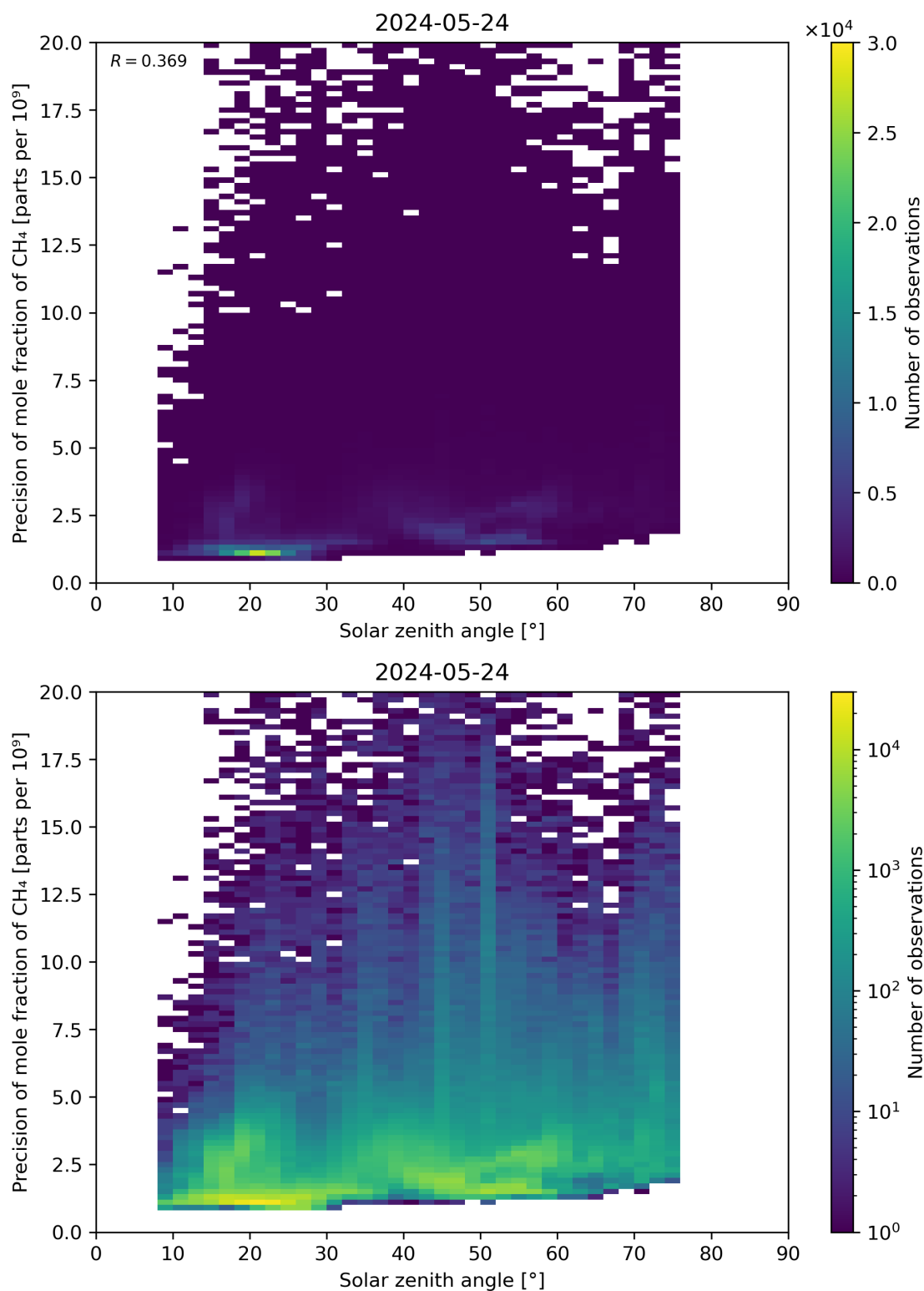
Figure 101: Scatter density plot of “Solar zenith angle” against “Precision of mole fraction of CH 4 ” for 2024-05-23 to 2024-05-25.
