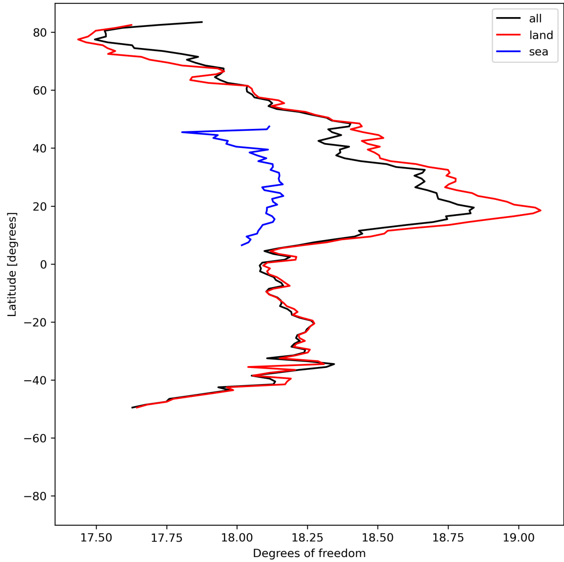
Figure 19: Zonal average of “Degrees of freedom” for 2024-05-23 to 2024-05-25.
