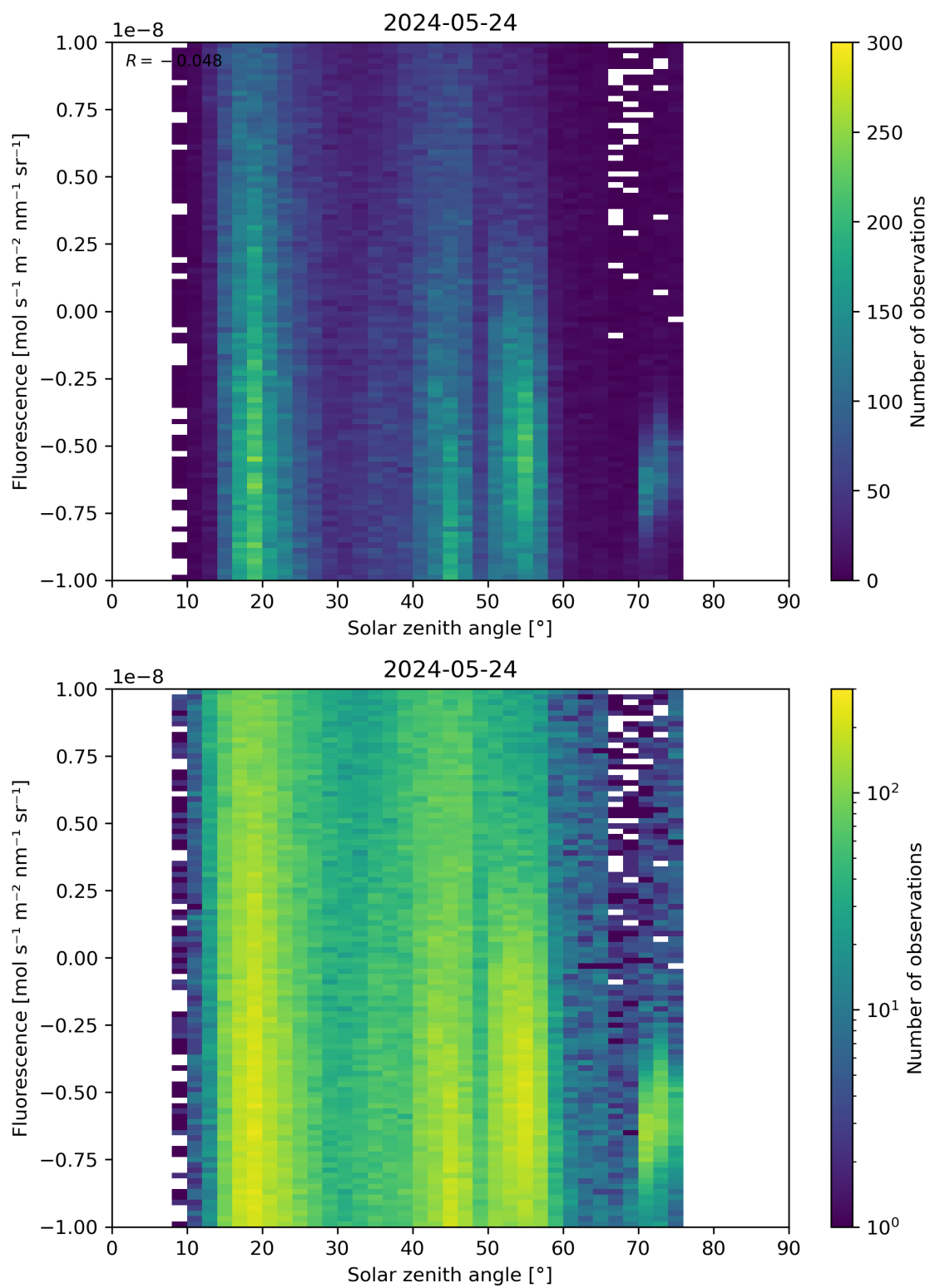
Figure 97: Scatter density plot of “Solar zenith angle” against “Fluorescence” for 2024-05-23 to 2024-05-25.
