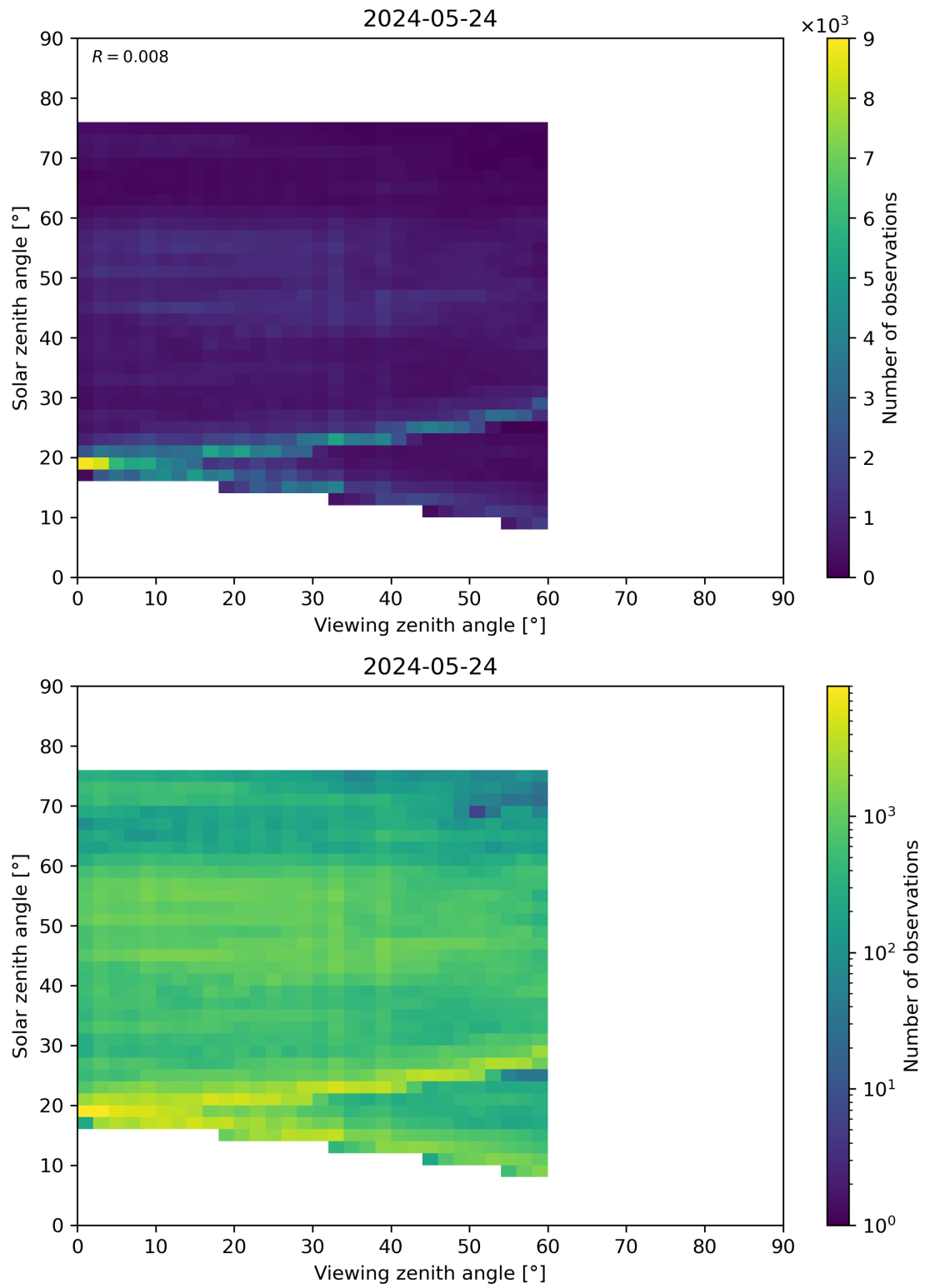
Figure 115: Scatter density plot of “Viewing zenith angle” against “Solar zenith angle” for 2024-05-23 to 2024-05-25.
