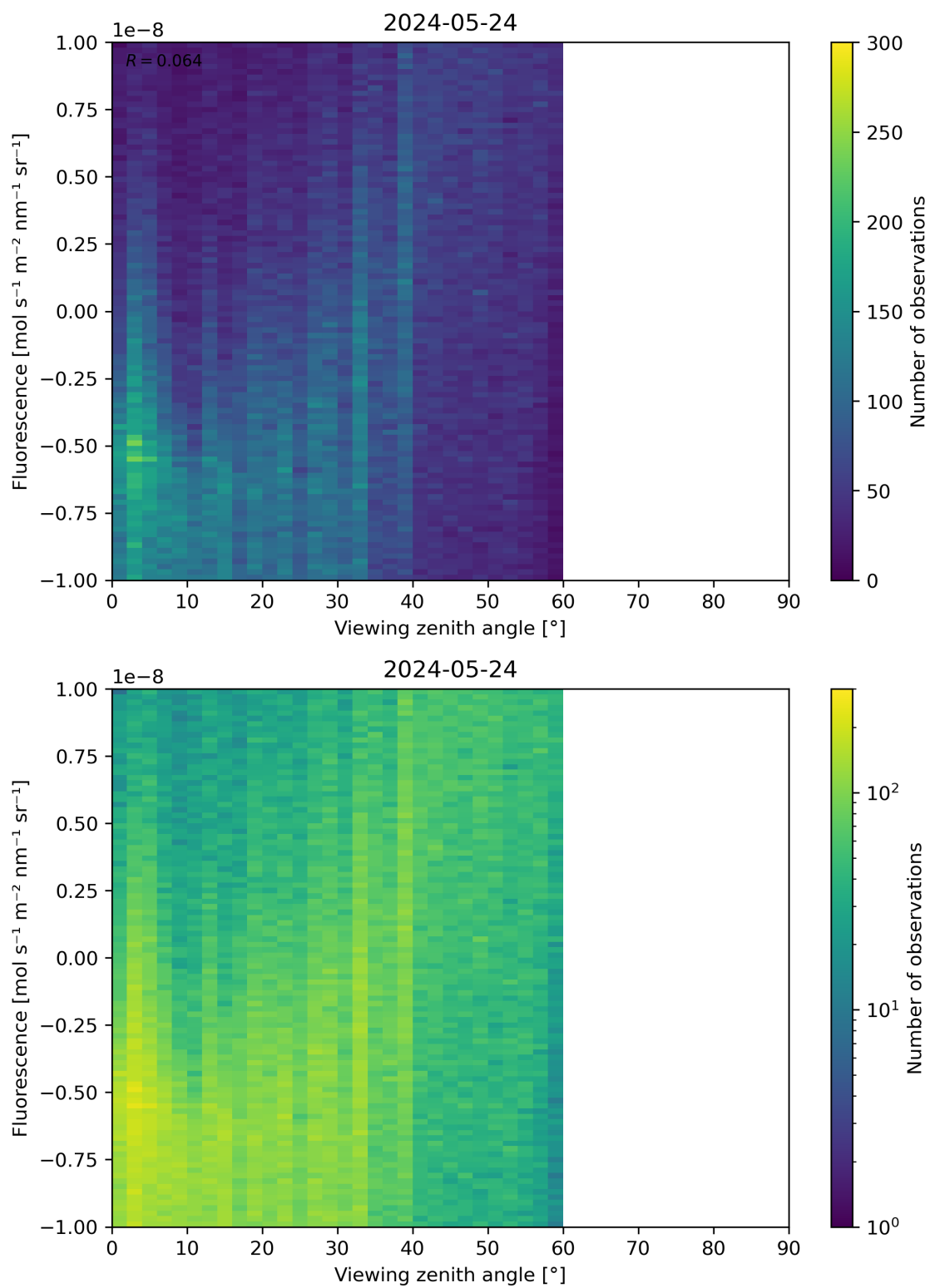
Figure 108: Scatter density plot of “Viewing zenith angle” against “Fluorescence” for 2024-05-23 to 2024-05-25.
