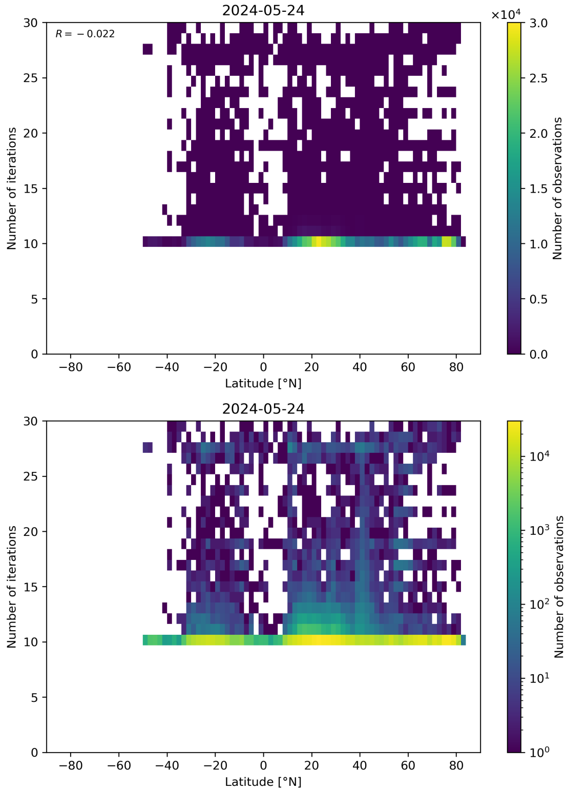
Figure 60: Scatter density plot of “Latitude” against “Number of iterations” for 2024-05-23 to 2024-05-25.
