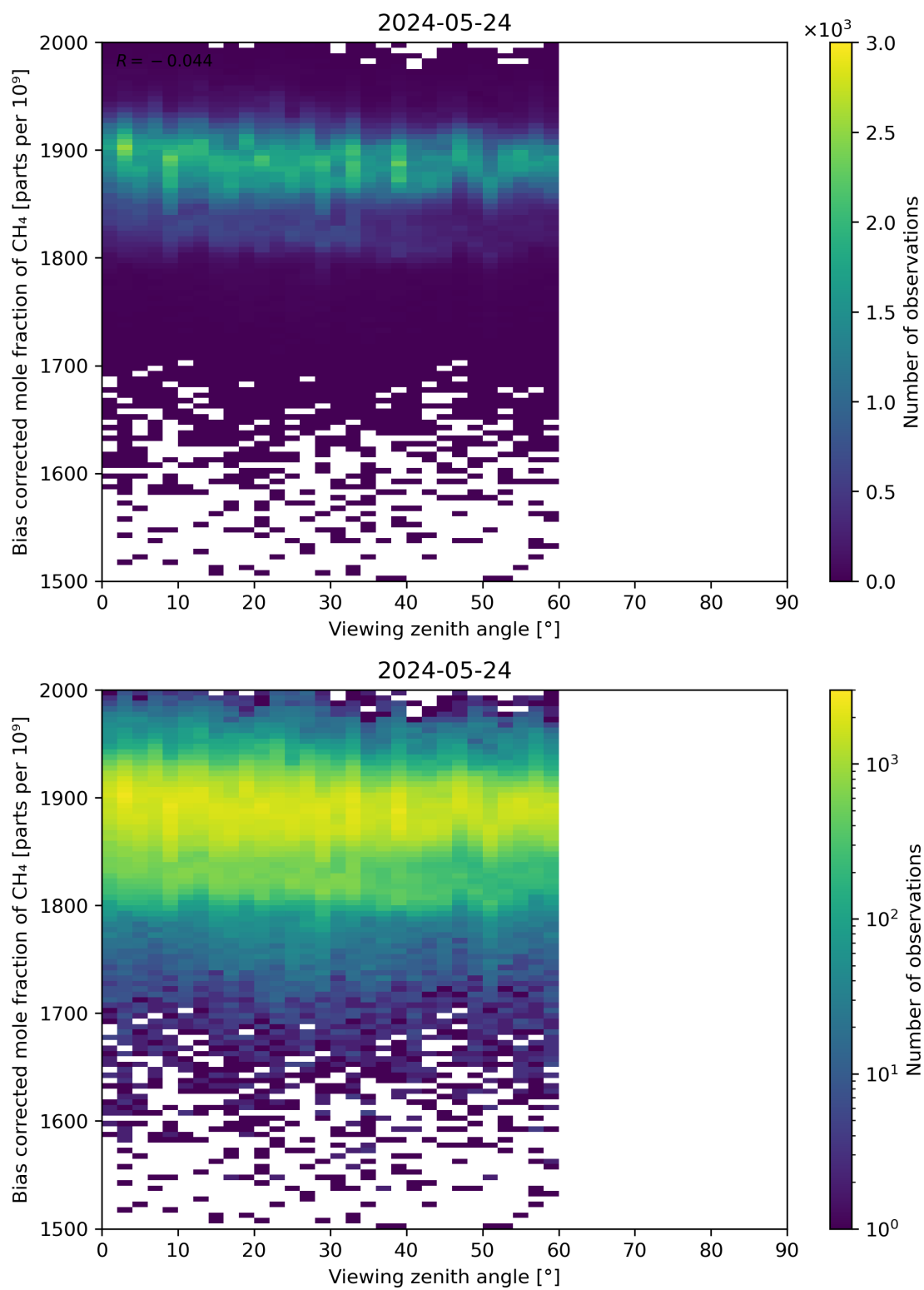
Figure 111: Scatter density plot of “Viewing zenith angle” against “Bias corrected mole fraction of CH 4 ” for 2024-05-23 to 2024-05-25.
