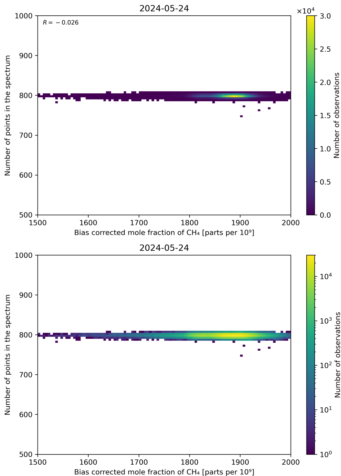
Figure 68: Scatter density plot of “Bias corrected mole fraction of CH 4 ” against “Number of points in the spectrum” for 2024-05-23 to 2024-05-25.
