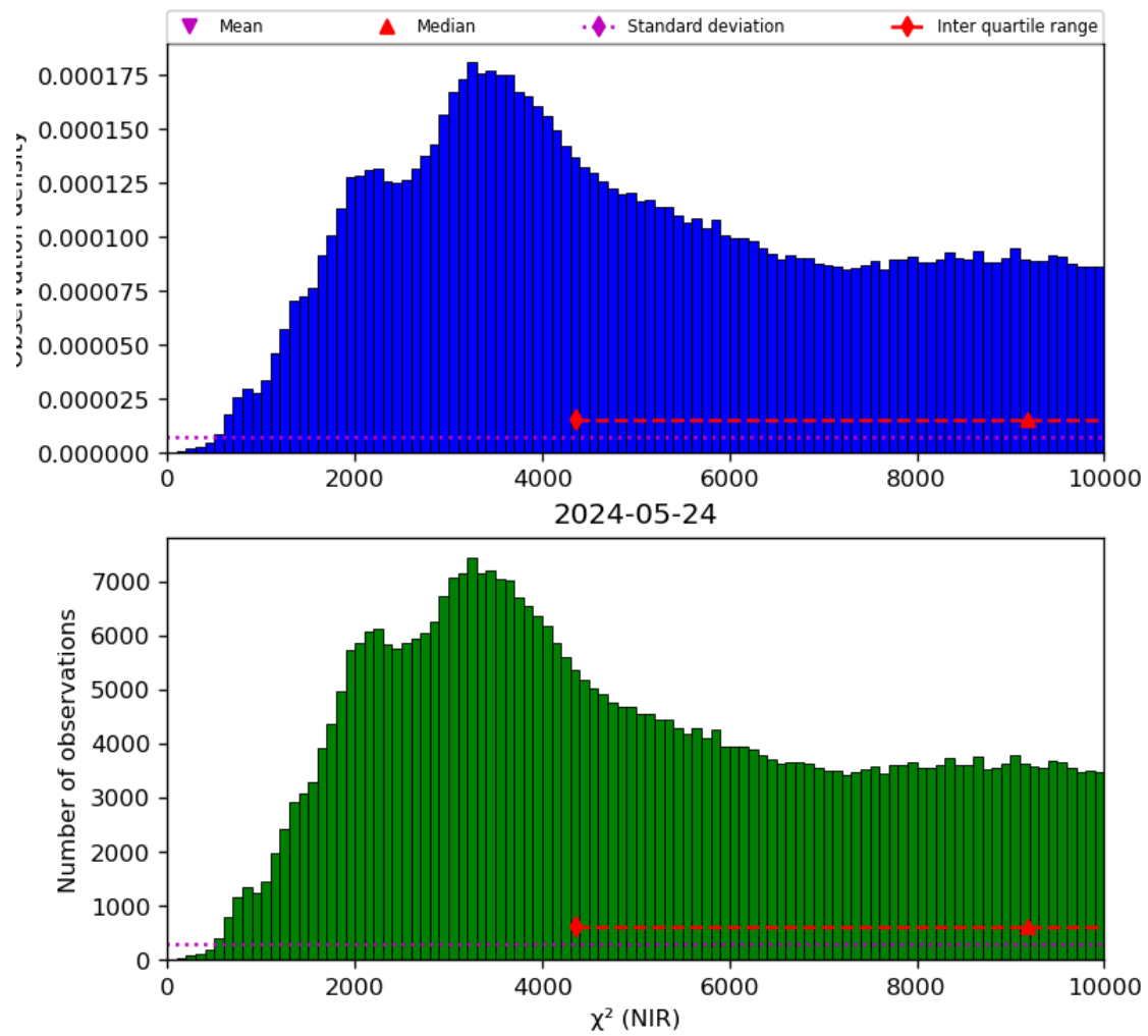
Figure 29: Histogram of “ \chi^2 (NIR)” for 2024-05-23 to 2024-05-25
