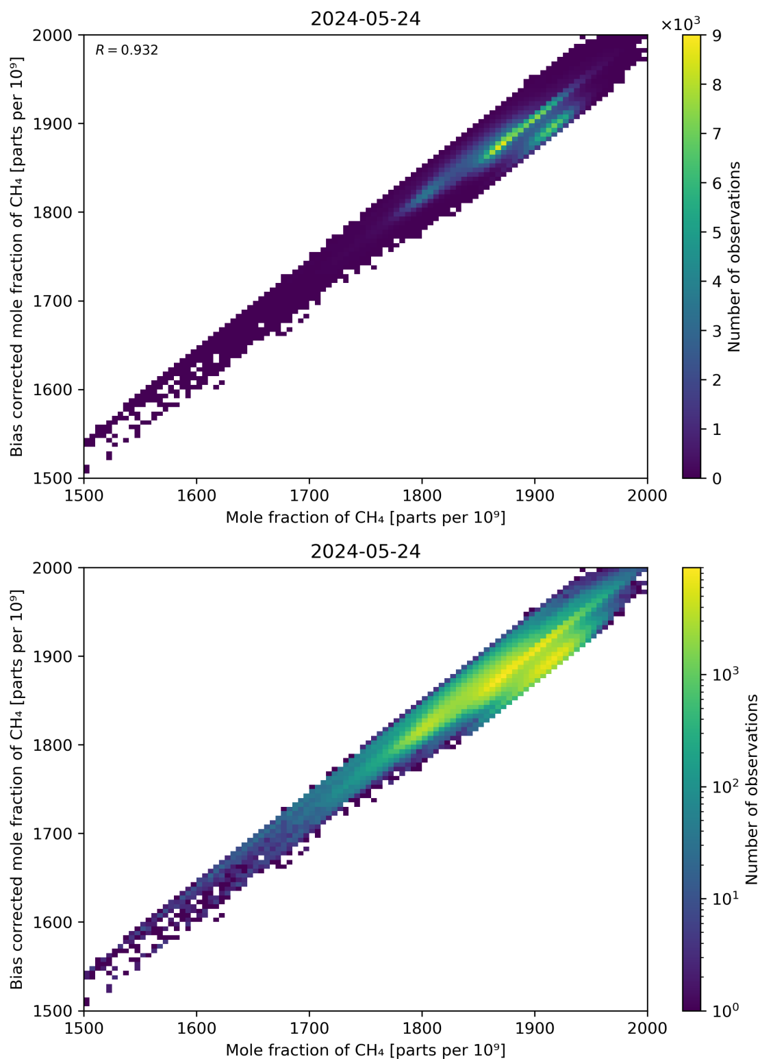
Figure 74: Scatter density plot of “Mole fraction of CH 4 ” against “Bias corrected mole fraction of CH 4 ” for 2024-05-23 to 2024-05-25.
