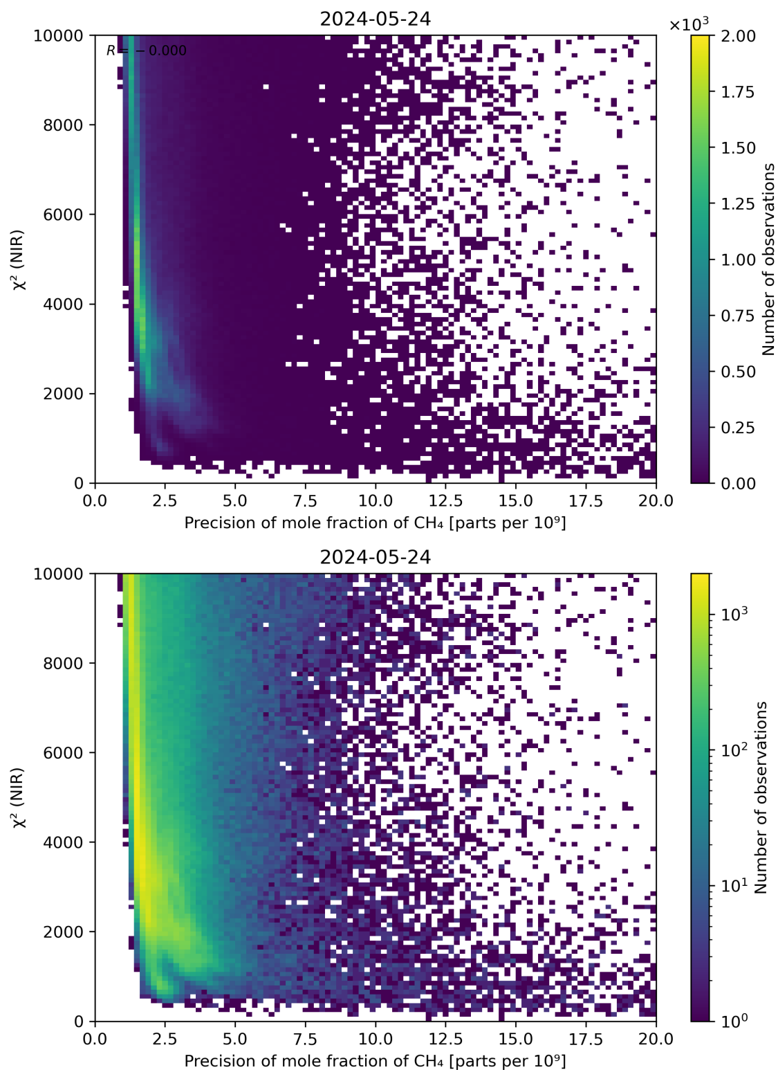
Figure 78: Scatter density plot of “Precision of mole fraction of \text{CH}_4 ” against “ \chi^2 (NIR)” for 2024-05-23 to 2024-05-25.
