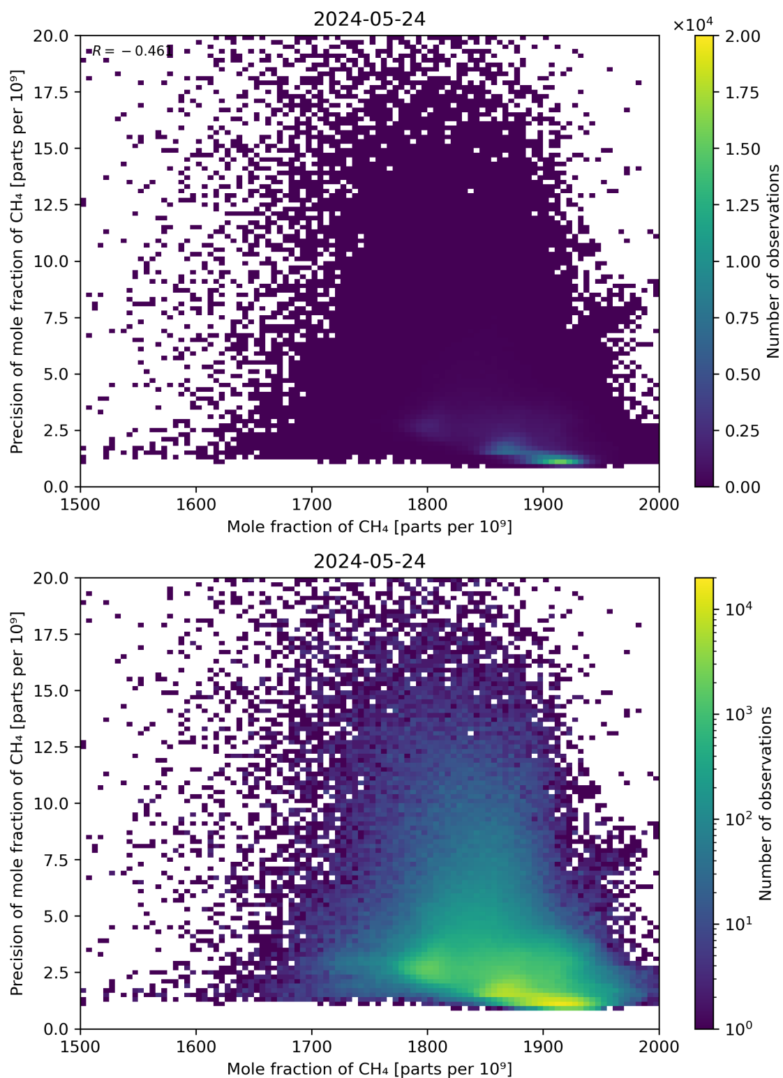
Figure 75: Scatter density plot of “Mole fraction of CH 4 ” against “Precision of mole fraction of CH 4 ” for 2024-05-23 to 2024-05-25.
