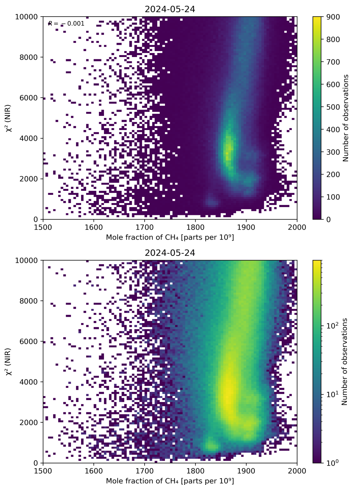
Figure 70: Scatter density plot of “Mole fraction of \text{CH}_4 ” against “ \chi^2 (NIR)” for 2024-05-23 to 2024-05-25.
