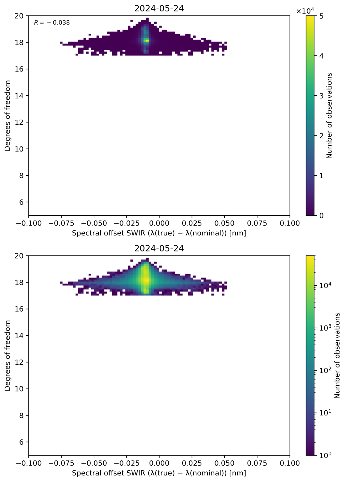
Figure 119: Scatter density plot of “Spectral offset SWIR ( \lambda(\text{true}) - \lambda(\text{nominal}) )” against “Degrees of freedom” for 2024-05-23 to 2024-05-25.
