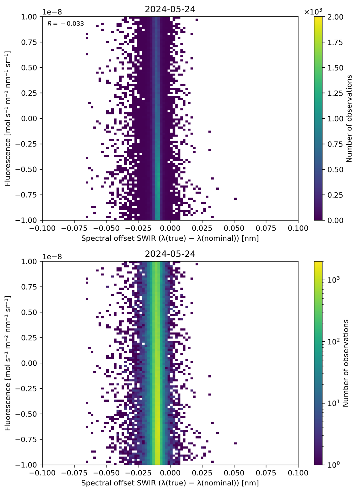
Figure 120: Scatter density plot of “Spectral offset SWIR ( \lambda(\text{true}) - \lambda(\text{nominal}) )” against “Fluorescence” for 2024-05-23 to 2024-05-25.
