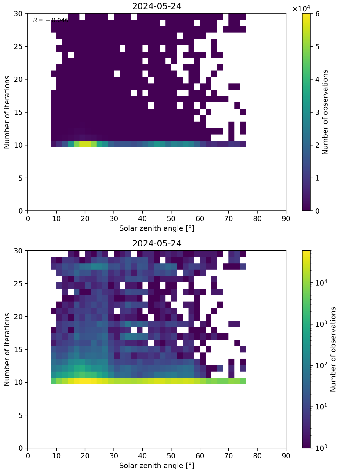
Figure 102: Scatter density plot of “Solar zenith angle” against “Number of iterations” for 2024-05-23 to 2024-05-25.
