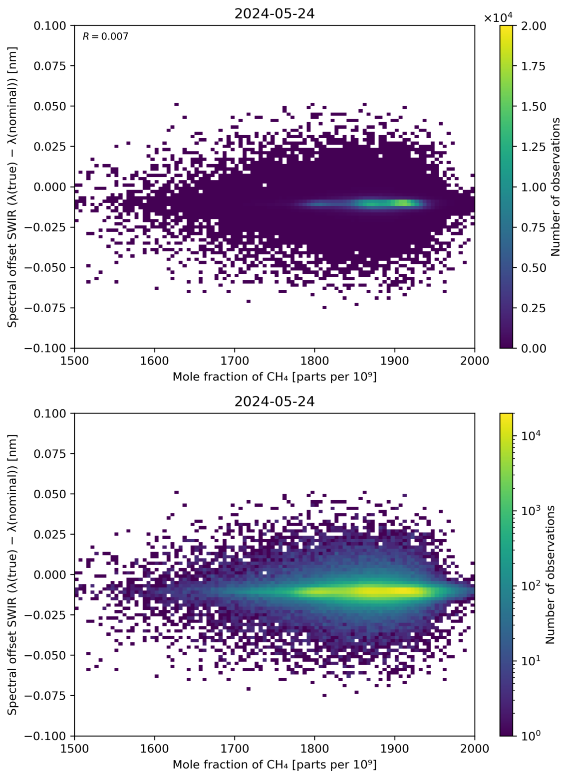
Figure 86: Scatter density plot of “Mole fraction of CH 4 ” against “Spectral offset SWIR ( \lambda(\text{true}) - \lambda(\text{nominal}) )” for 2024-05-23 to 2024-05-25.
