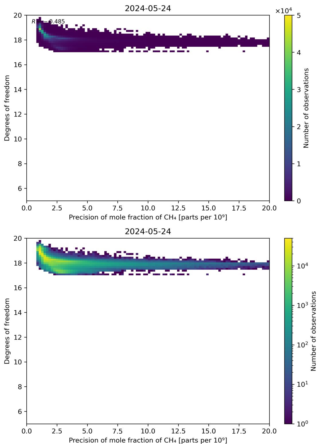
Figure 80: Scatter density plot of “Precision of mole fraction of CH 4 ” against “Degrees of freedom” for 2024-05-23 to 2024-05-25.
