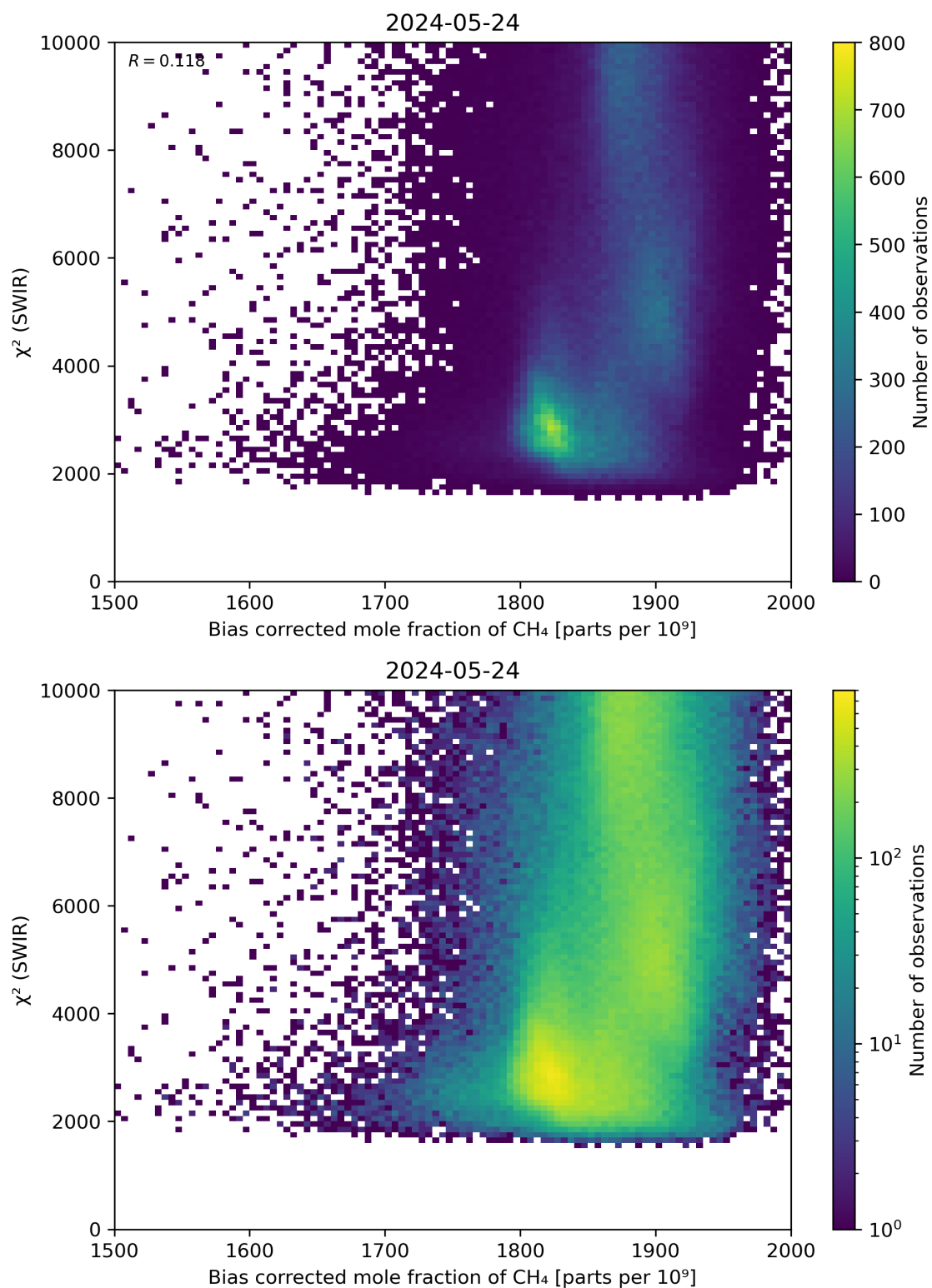
Figure 64: Scatter density plot of “Bias corrected mole fraction of \text{CH}_4 ” against “ \chi^2 (SWIR)” for 2024-05-23 to 2024-05-25.
