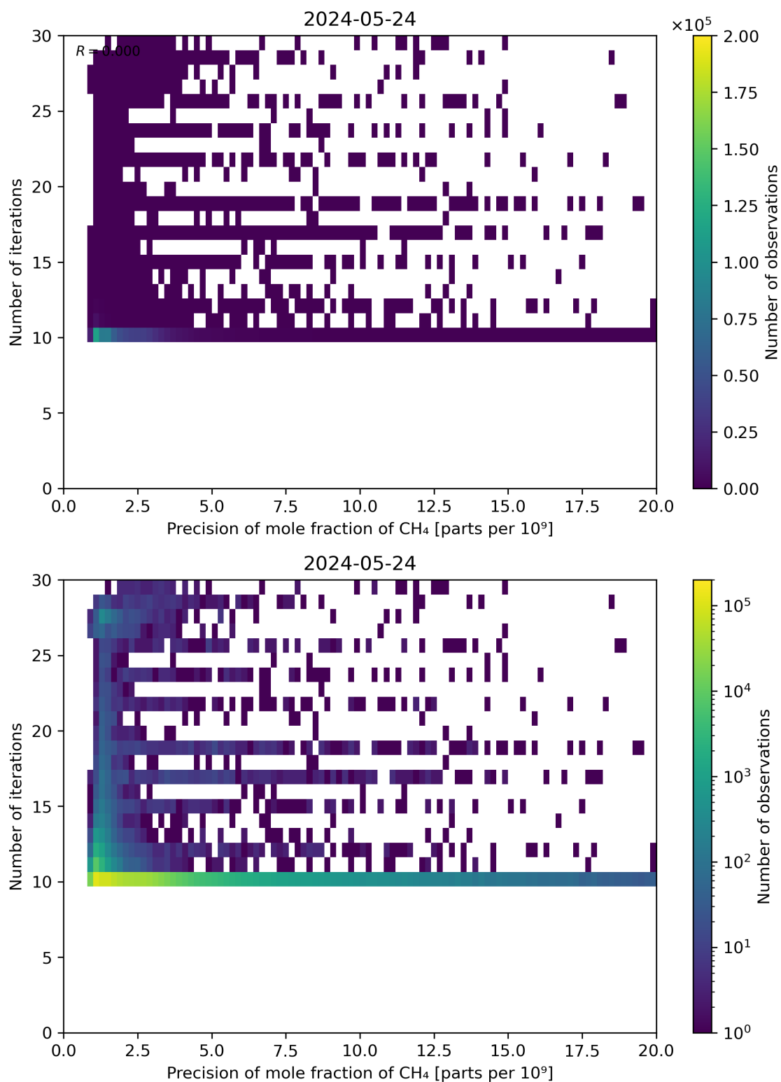
Figure 83: Scatter density plot of “Precision of mole fraction of CH 4 ” against “Number of iterations” for 2024-05-23 to 2024-05-25.
