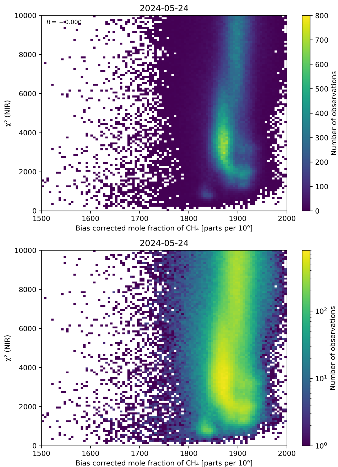
Figure 63: Scatter density plot of “Bias corrected mole fraction of CH 4 ” against “ \chi^2 (NIR)” for 2024-05-23 to 2024-05-25.
