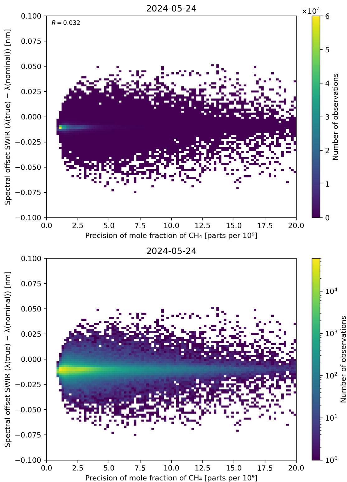
Figure 85: Scatter density plot of “Precision of mole fraction of CH 4 ” against “Spectral offset SWIR ( \lambda(\text{true}) - \lambda(\text{nominal}) )” for 2024-05-23 to 2024-05-25.
