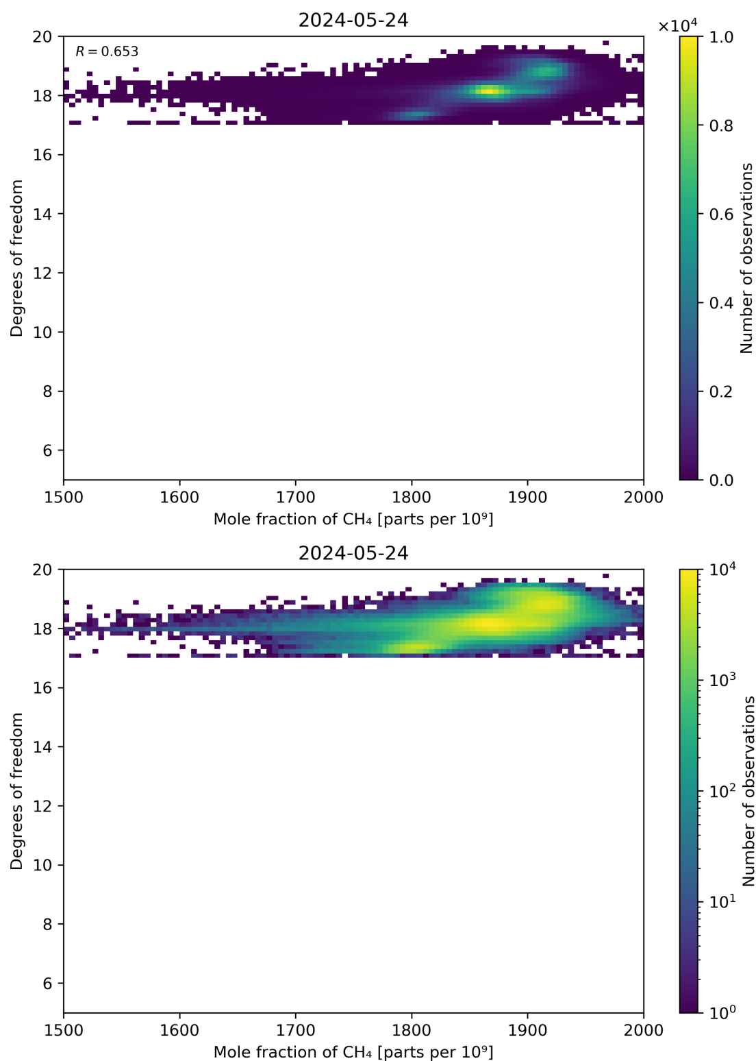
Figure 72: Scatter density plot of “Mole fraction of CH 4 ” against “Degrees of freedom” for 2024-05-23 to 2024-05-25.
