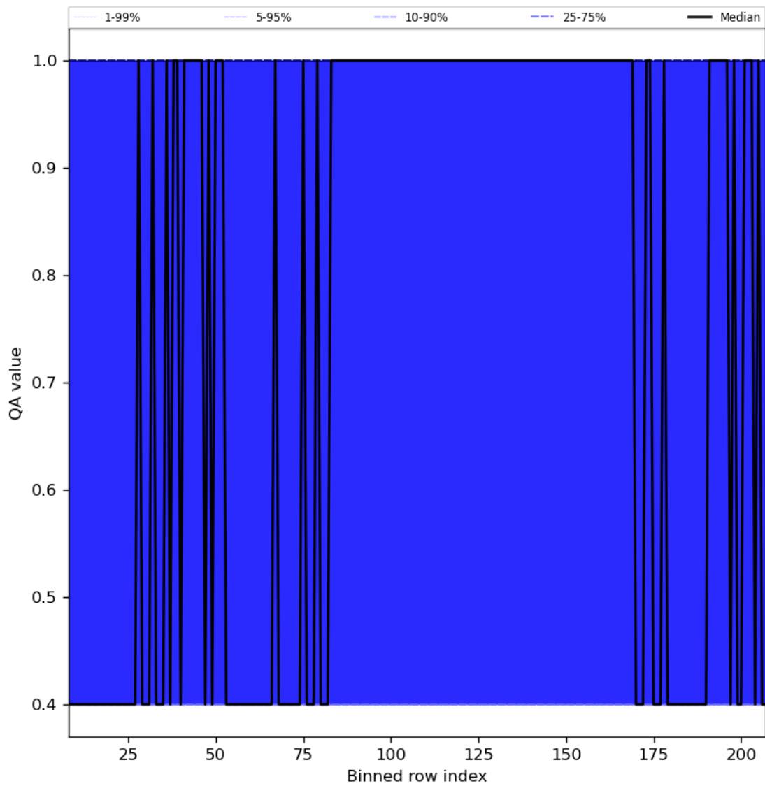
Figure 33: Along track statistics of “QA value” for 2024-05-23 to 2024-05-25
