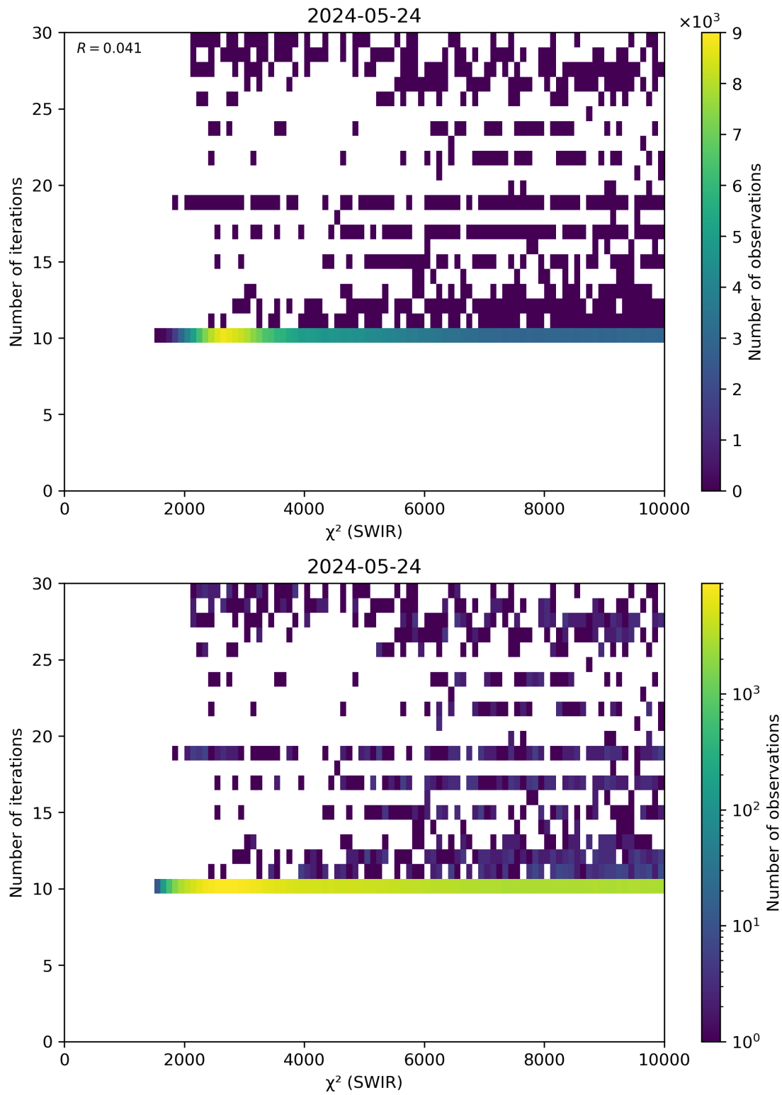
Figure 50: Scatter density plot of “ \chi^2 (SWIR)” against “Number of iterations” for 2024-05-23 to 2024-05-25.
