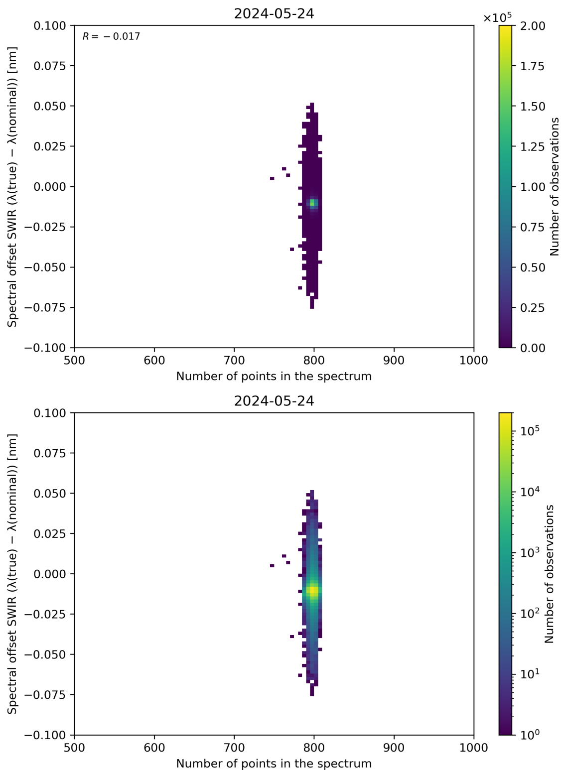
Figure 93: Scatter density plot of “Number of points in the spectrum” against “Spectral offset SWIR ( \lambda(\text{true}) - \lambda(\text{nominal}) )” for 2024-05-23 to 2024-05-25.
