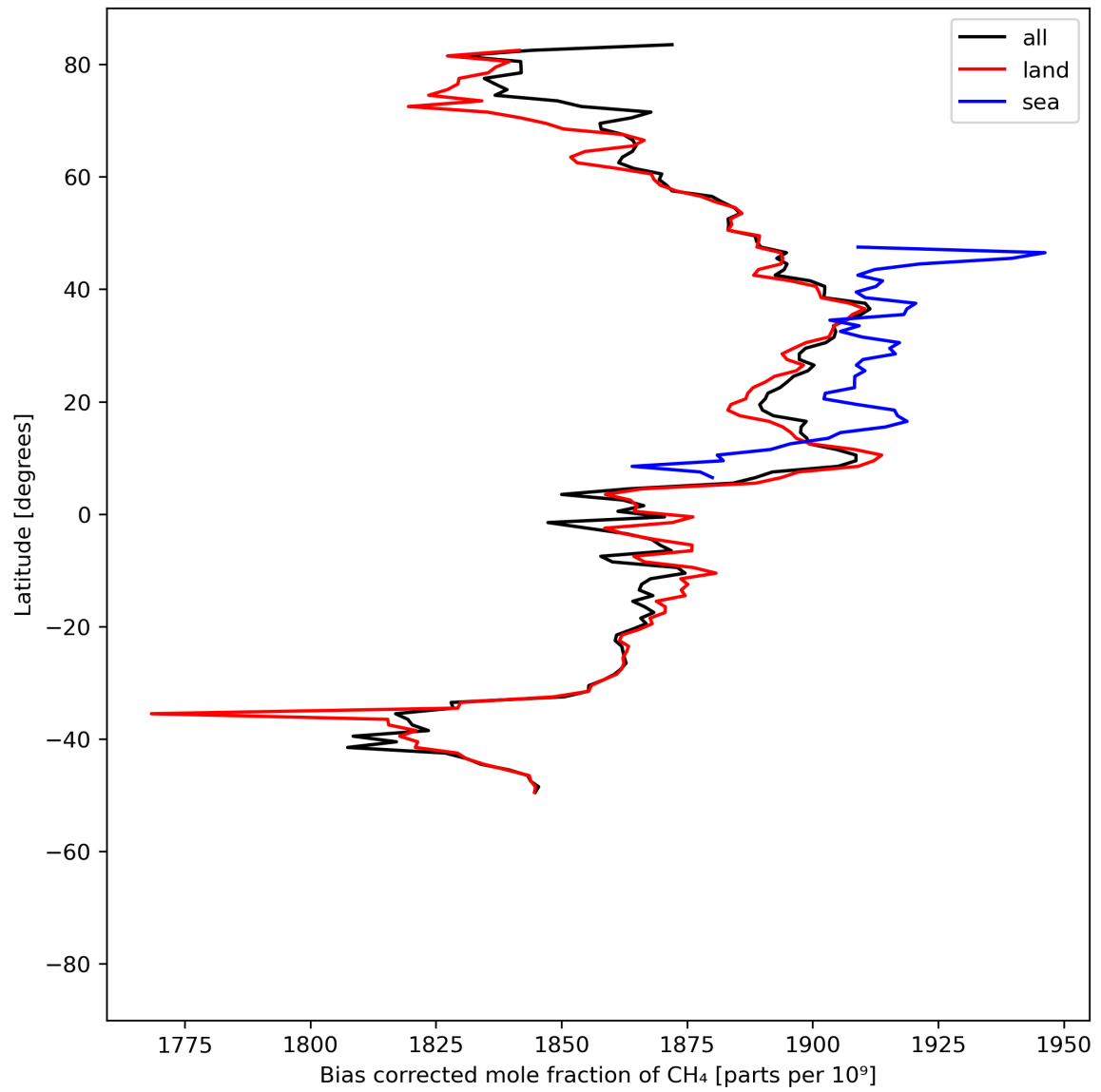
Figure 14: Zonal average of “Bias corrected mole fraction of CH 4 ” for 2024-05-23 to 2024-05-25.
