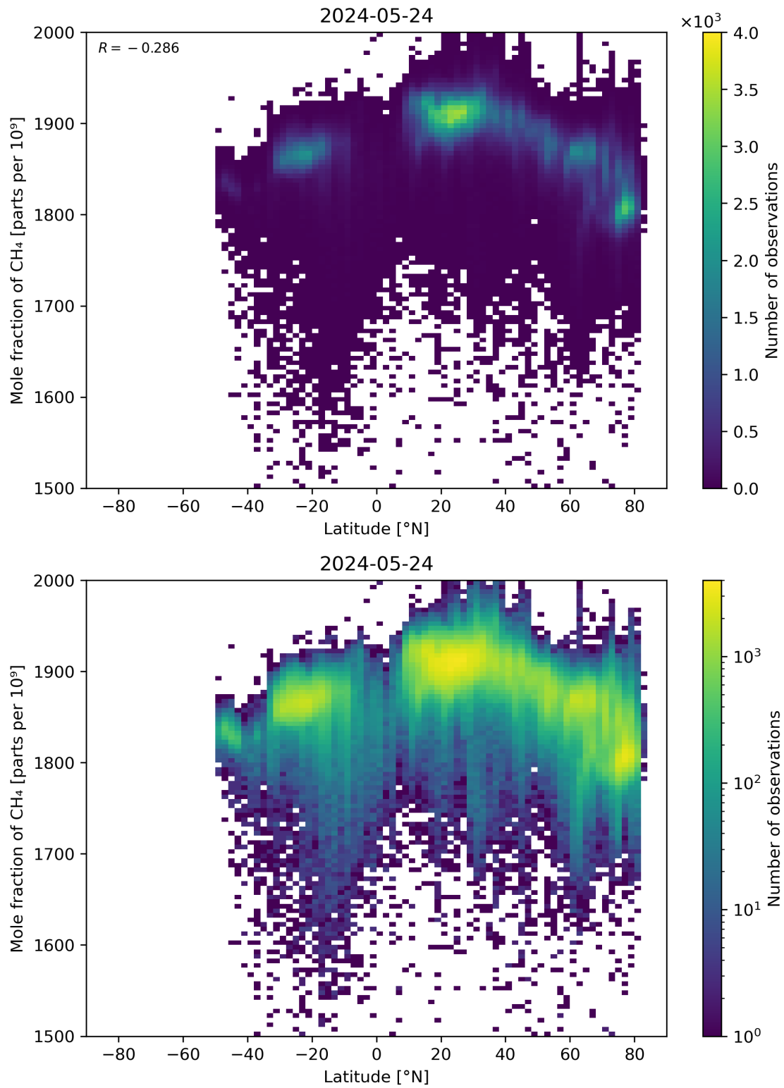
Figure 57: Scatter density plot of “Latitude” against “Mole fraction of CH 4 ” for 2024-05-23 to 2024-05-25.
