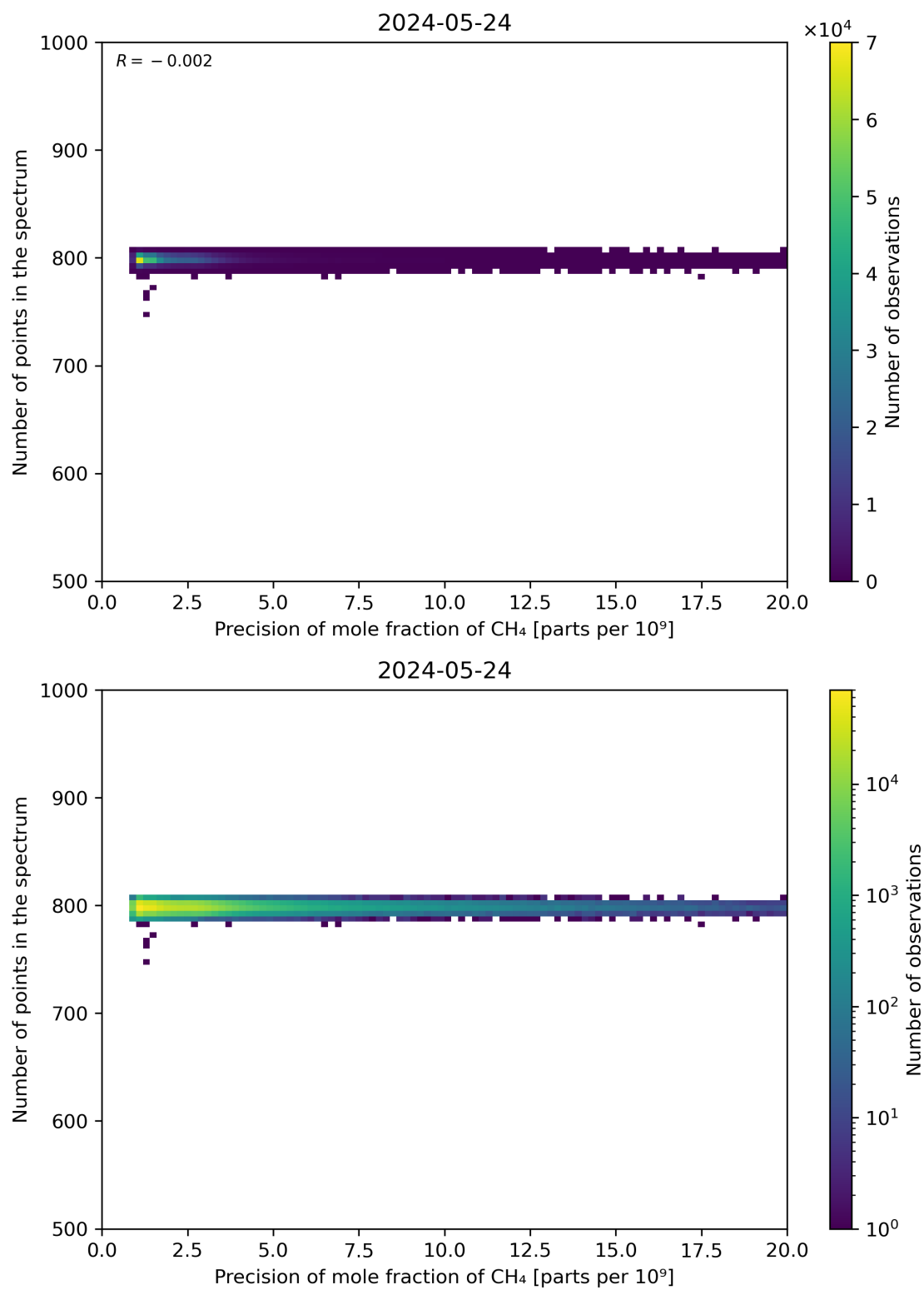
Figure 84: Scatter density plot of “Precision of mole fraction of CH 4 ” against “Number of points in the spectrum” for 2024-05-23 to 2024-05-25.
