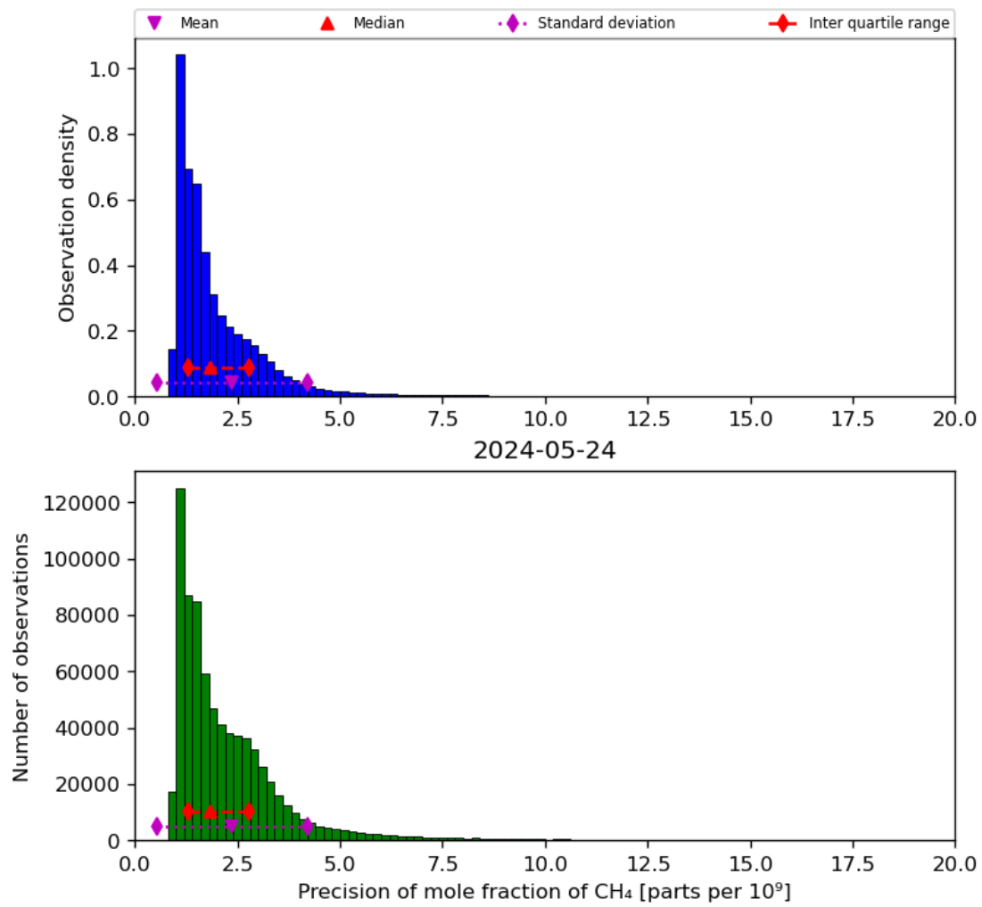
Figure 24: Histogram of “Precision of mole fraction of CH 4 ” for 2024-05-23 to 2024-05-25
