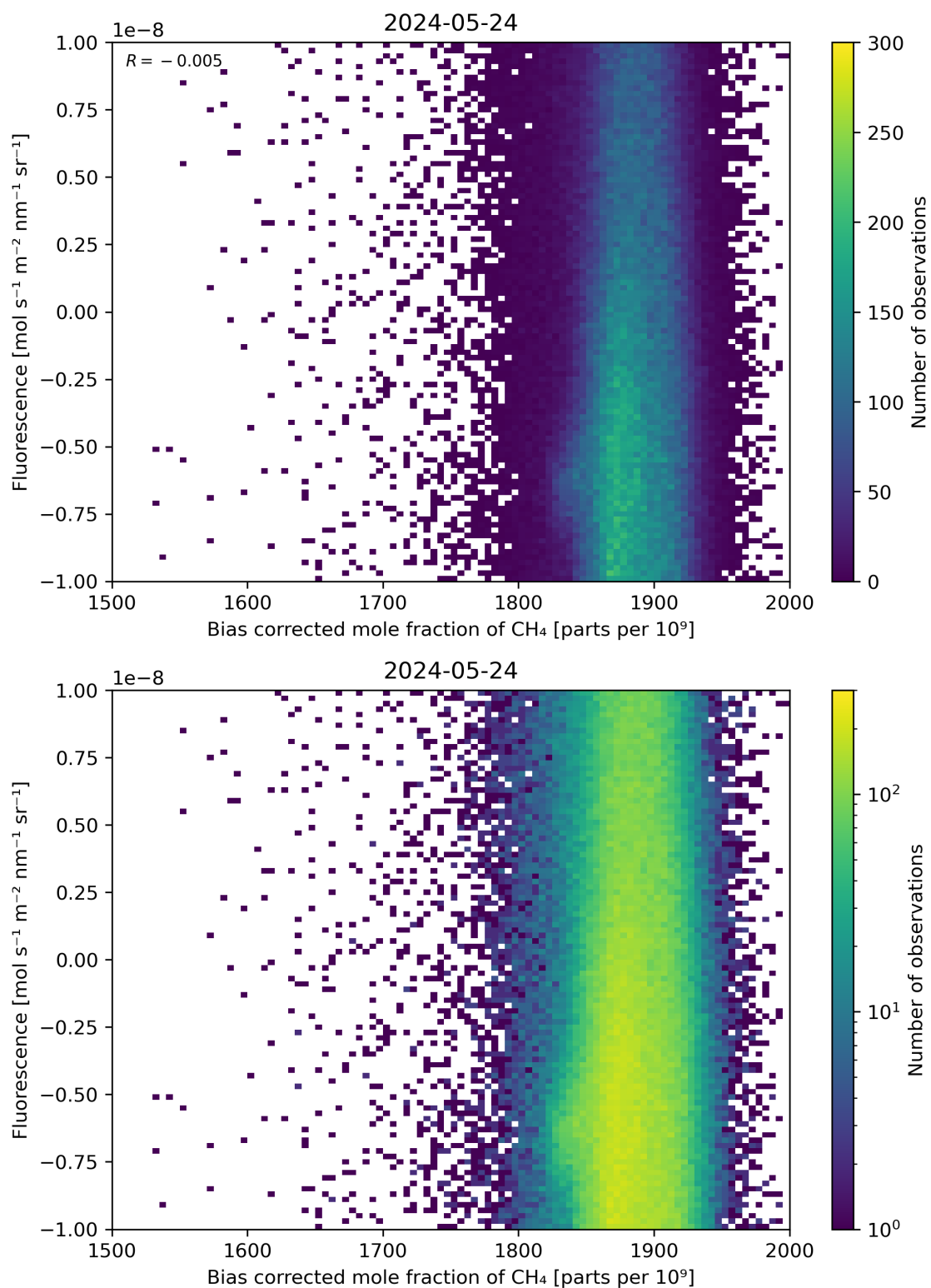
Figure 66: Scatter density plot of “Bias corrected mole fraction of \text{CH}_4 ” against “Fluorescence” for 2024-05-23 to 2024-05-25.
