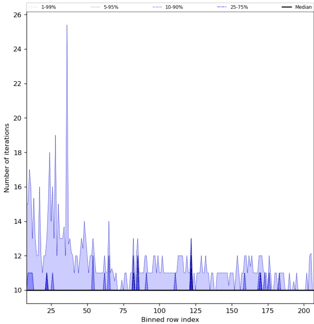
Figure 42: Along track statistics of “Number of iterations” for 2024-05-23 to 2024-05-25
