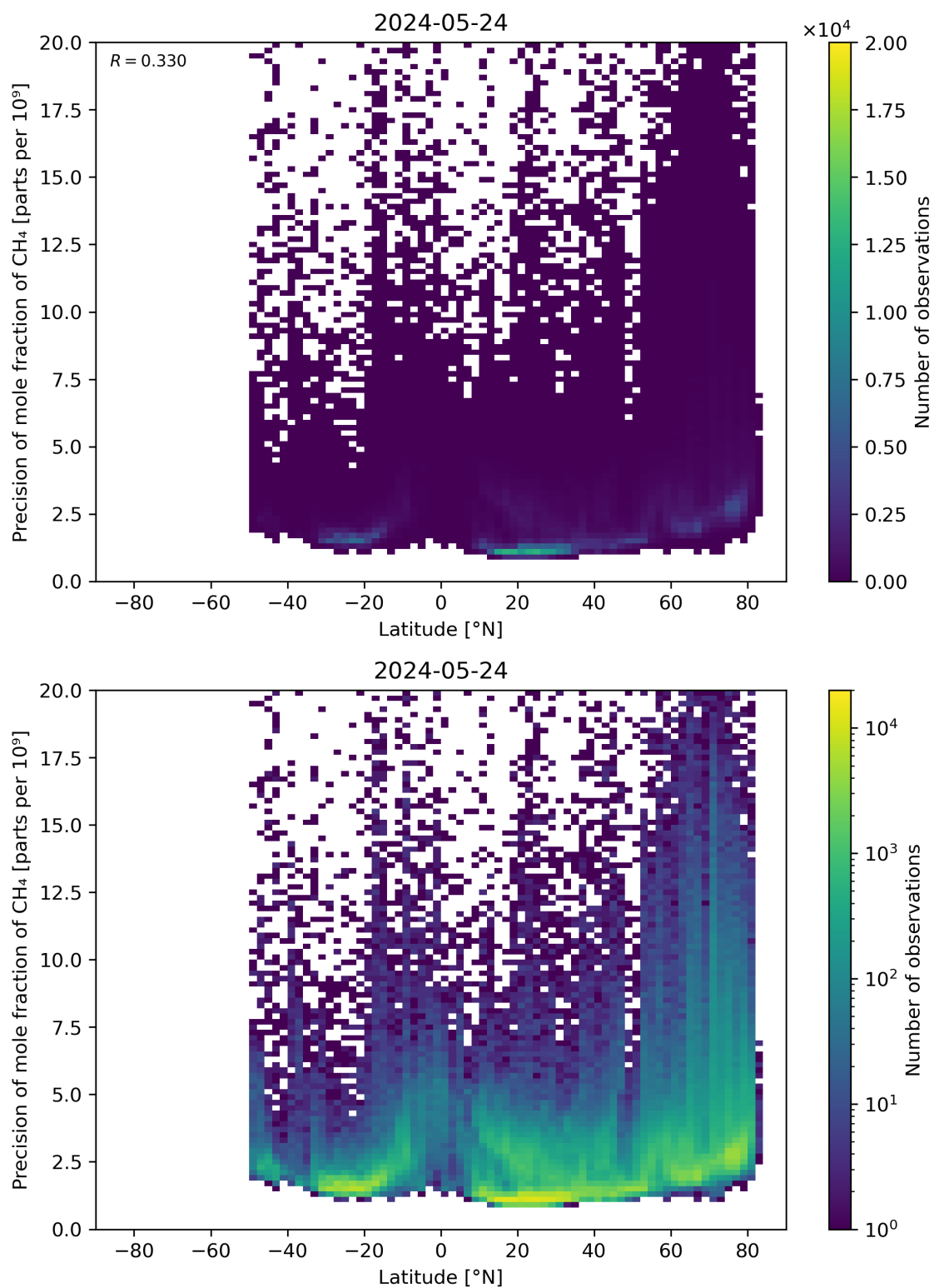
Figure 59: Scatter density plot of “Latitude” against “Precision of mole fraction of \text{CH}_4 ” for 2024-05-23 to 2024-05-25.
