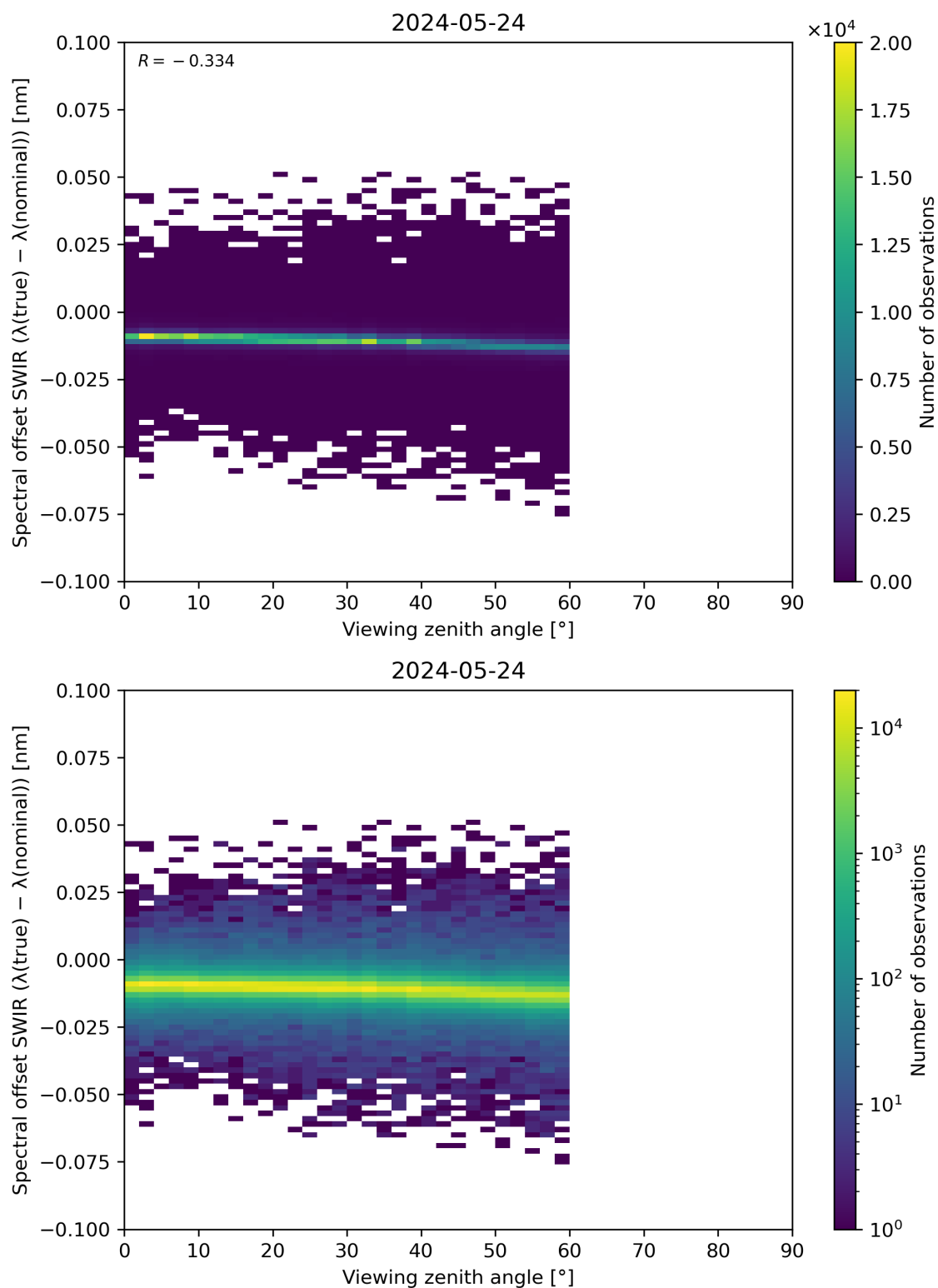
Figure 116: Scatter density plot of “Viewing zenith angle” against “Spectral offset SWIR ( \lambda(\text{true}) - \lambda(\text{nominal}) )” for 2024-05-23 to 2024-05-25.
