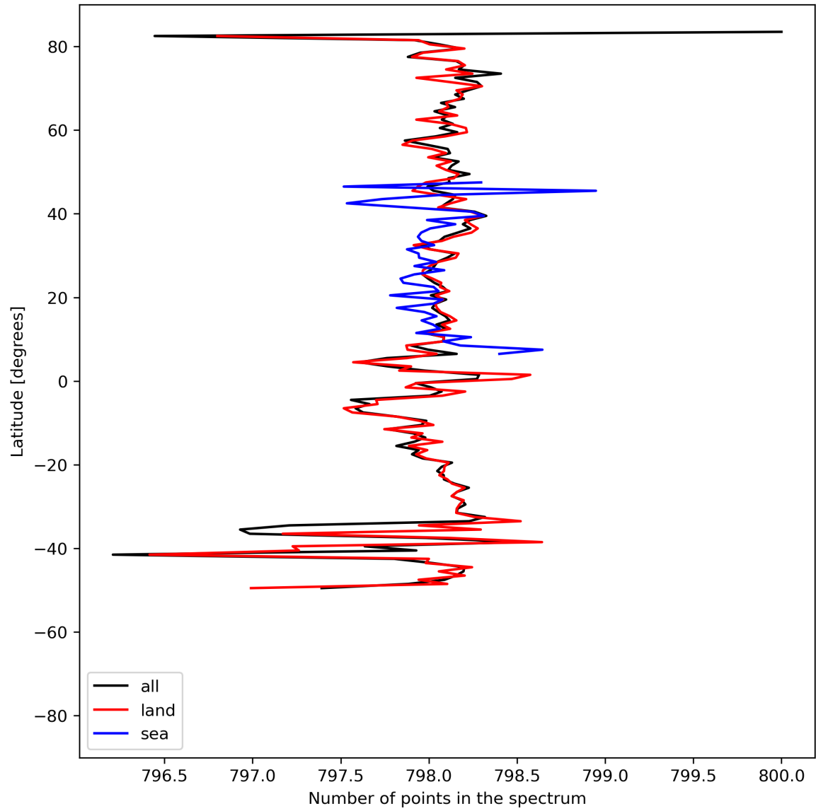
Figure 15: Zonal average of “Number of points in the spectrum” for 2024-05-23 to 2024-05-25.
