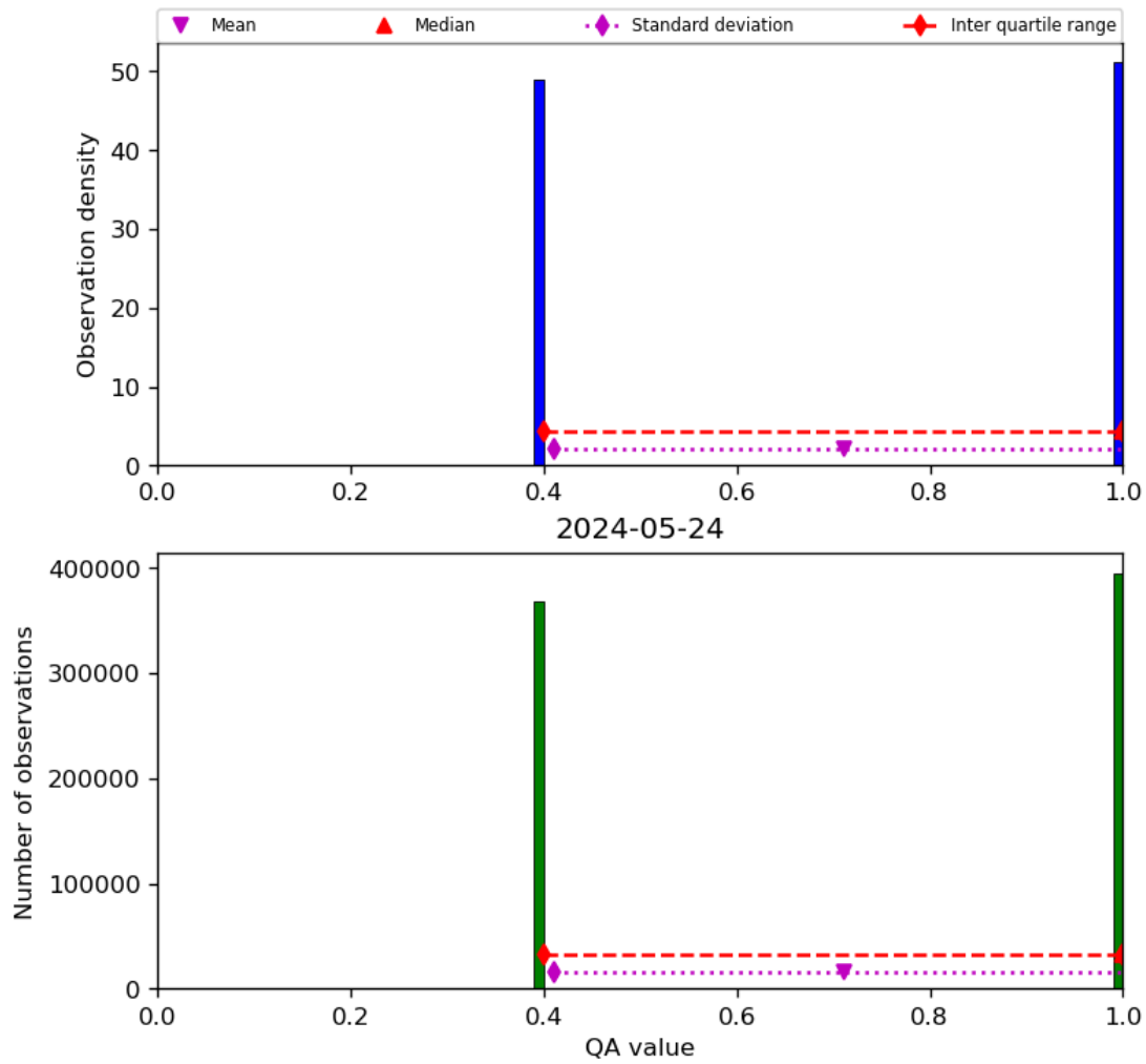
Figure 22: Histogram of “QA value” for 2024-05-23 to 2024-05-25
