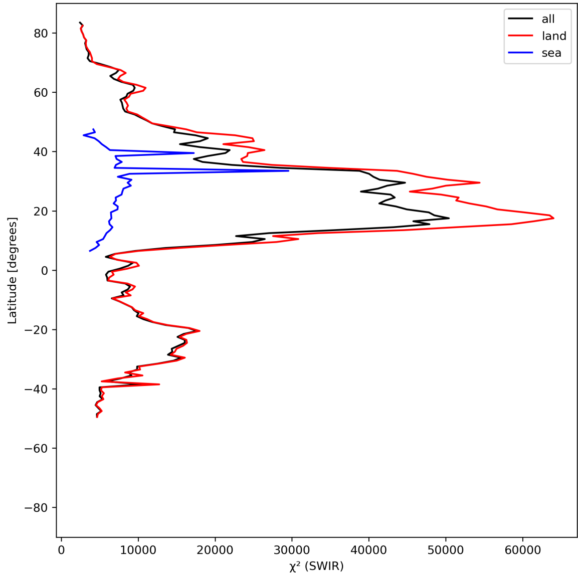
Figure 17: Zonal average of “ \chi^2 (SWIR)” for 2024-05-23 to 2024-05-25.
