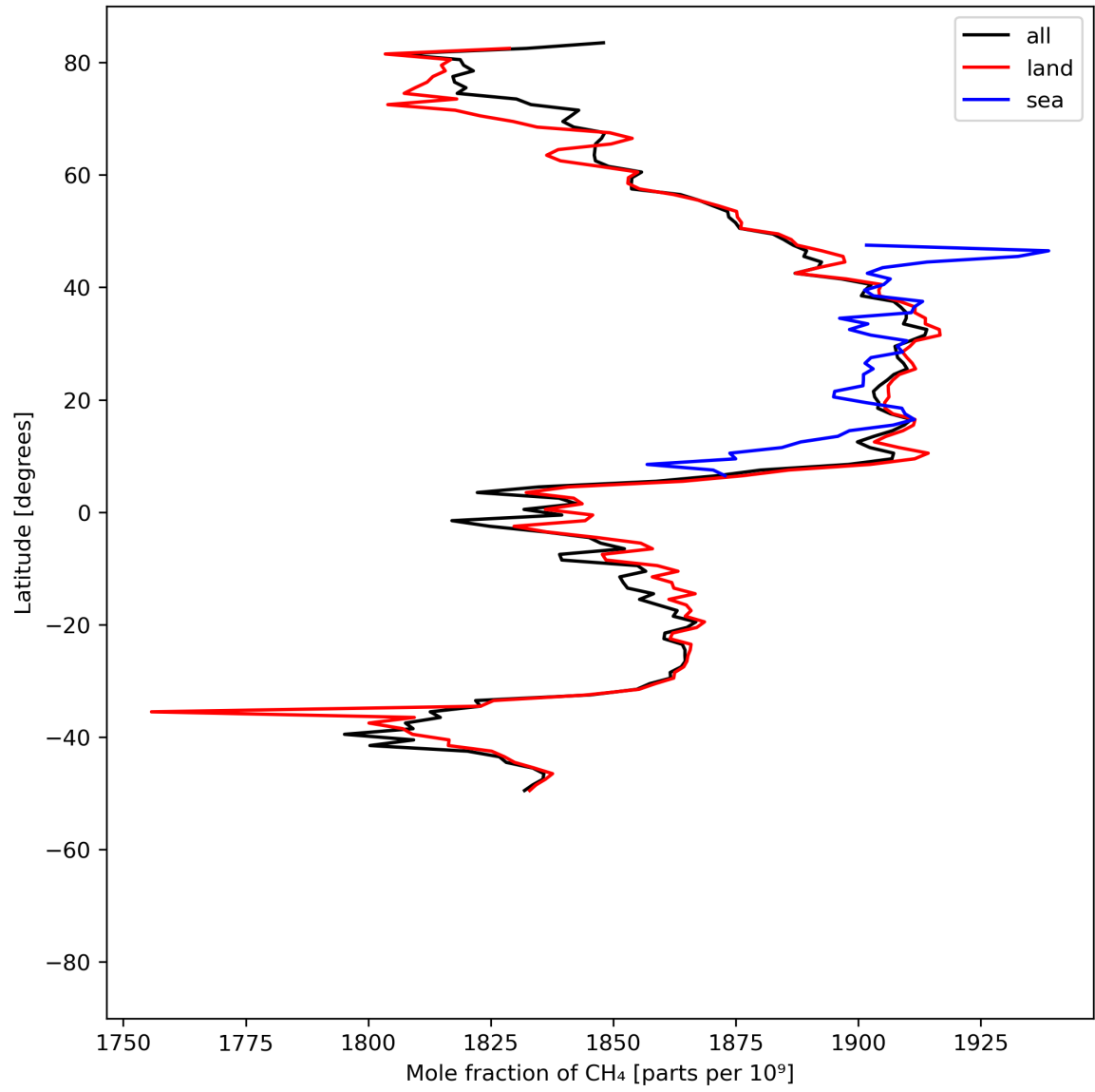
Figure 12: Zonal average of “Mole fraction of CH 4 ” for 2024-05-23 to 2024-05-25.
