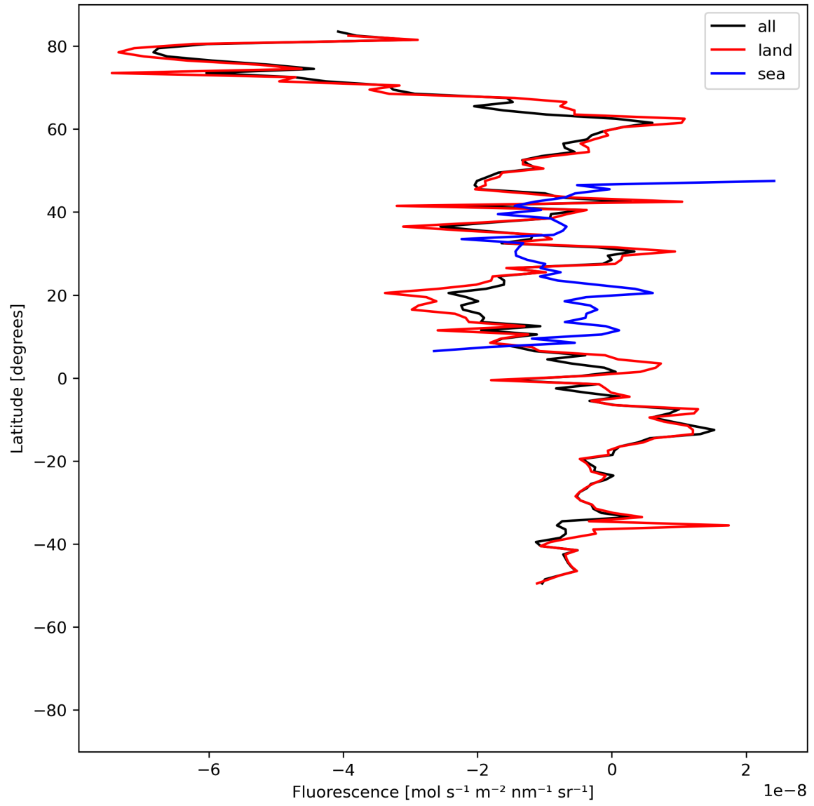
Figure 21: Zonal average of “Fluorescence” for 2024-05-23 to 2024-05-25.
