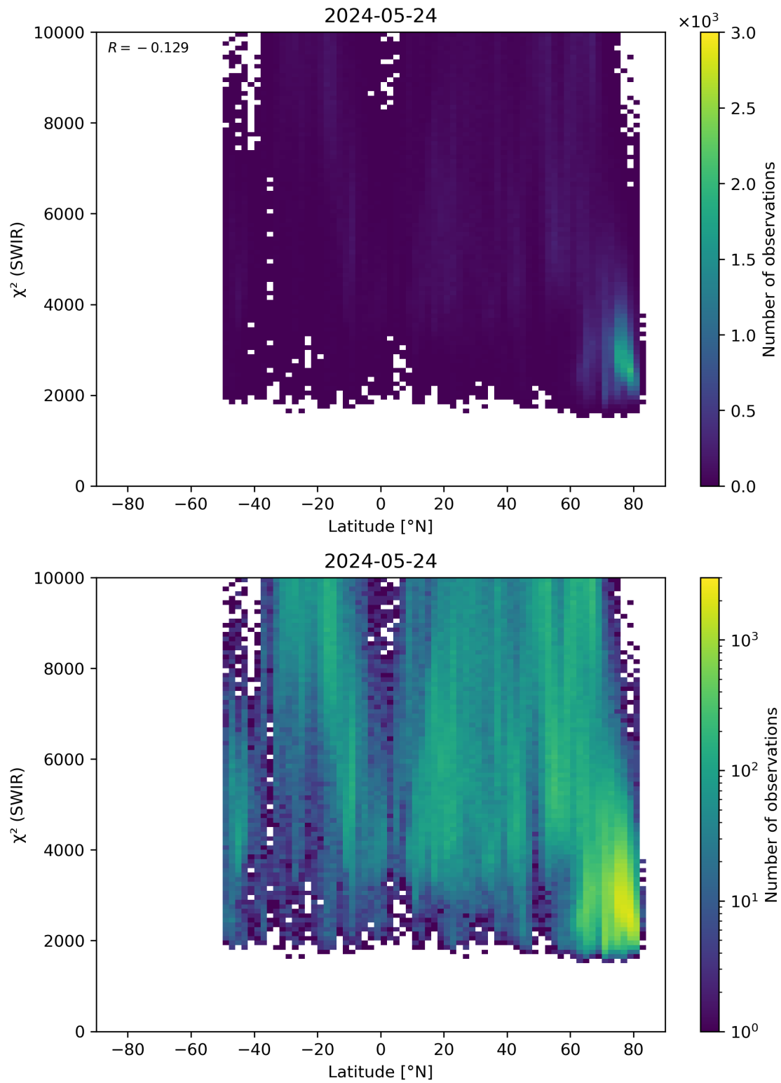
Figure 54: Scatter density plot of “Latitude” against “ \chi^2 (SWIR)” for 2024-05-23 to 2024-05-25.
