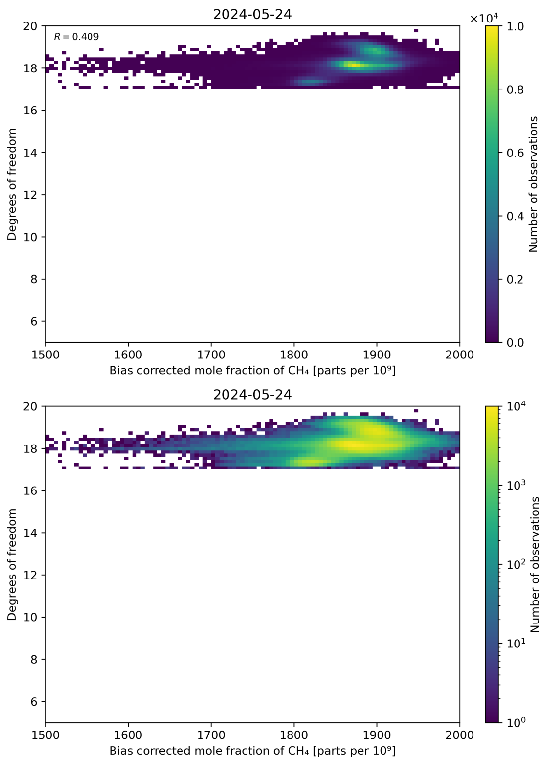
Figure 65: Scatter density plot of “Bias corrected mole fraction of CH 4 ” against “Degrees of freedom” for 2024-05-23 to 2024-05-25.
