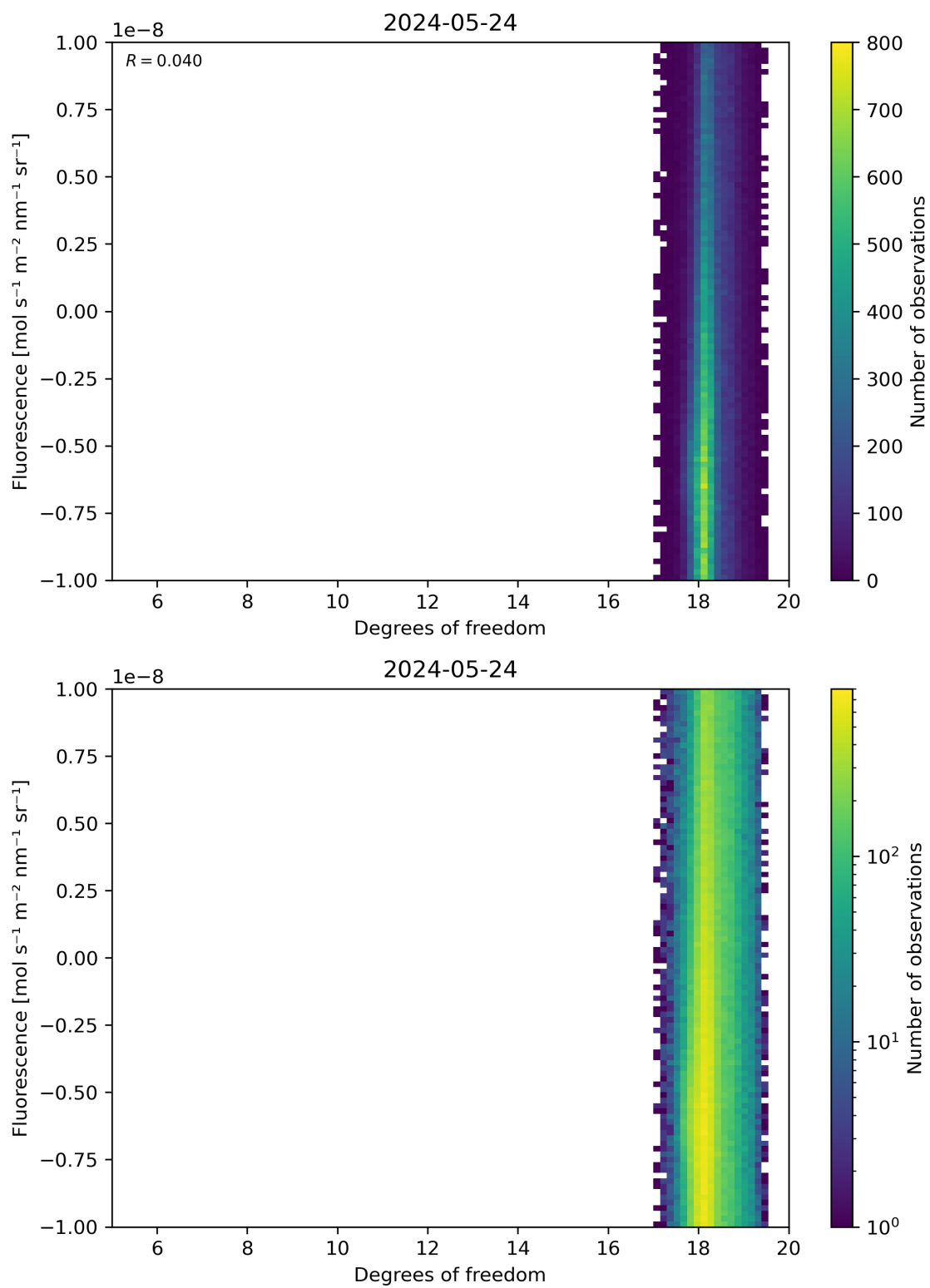
Figure 51: Scatter density plot of “Degrees of freedom” against “Fluorescence” for 2024-05-23 to 2024-05-25.
