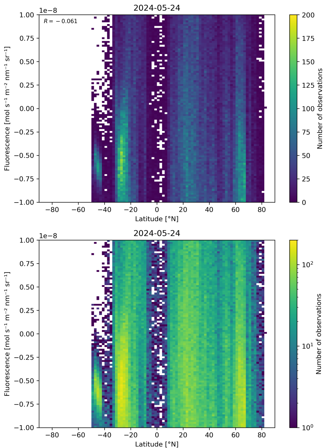
Figure 56: Scatter density plot of “Latitude” against “Fluorescence” for 2024-05-23 to 2024-05-25.
