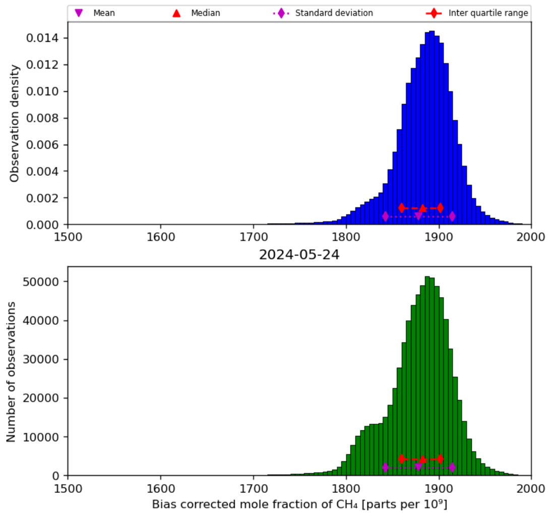
Figure 25: Histogram of “Bias corrected mole fraction of CH 4 ” for 2024-05-23 to 2024-05-25
