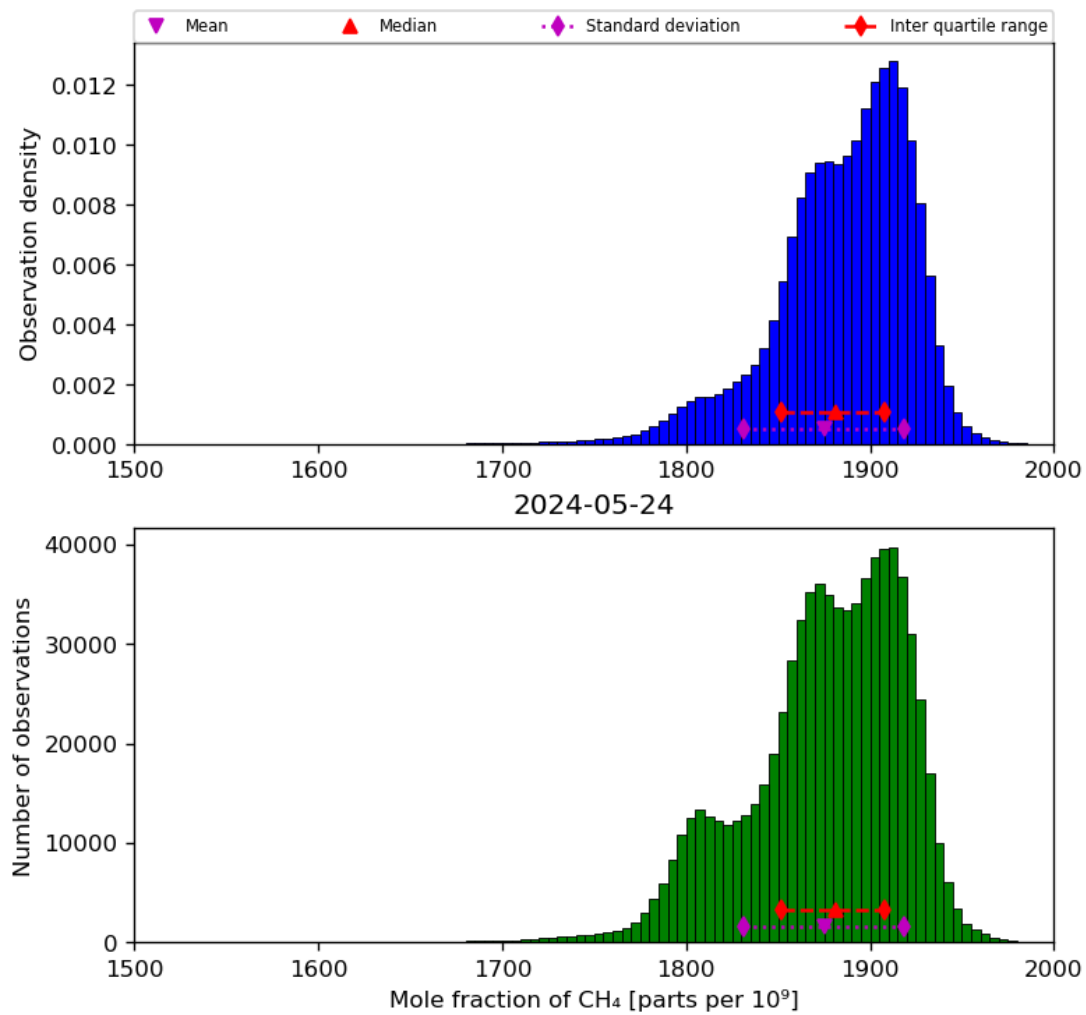
Figure 23: Histogram of “Mole fraction of CH 4 ” for 2024-05-23 to 2024-05-25
