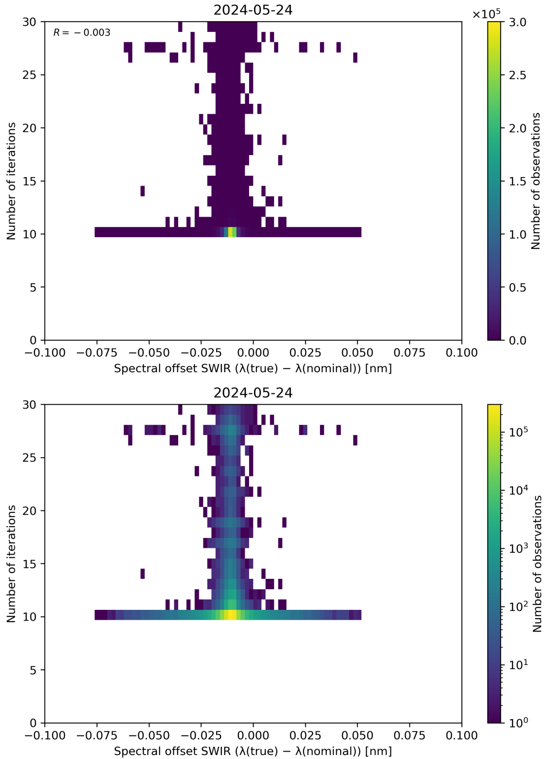
Figure 121: Scatter density plot of “Spectral offset SWIR ( \lambda(\text{true}) - \lambda(\text{nominal}) )” against “Number of iterations” for 2024-05-23 to 2024-05-25.
