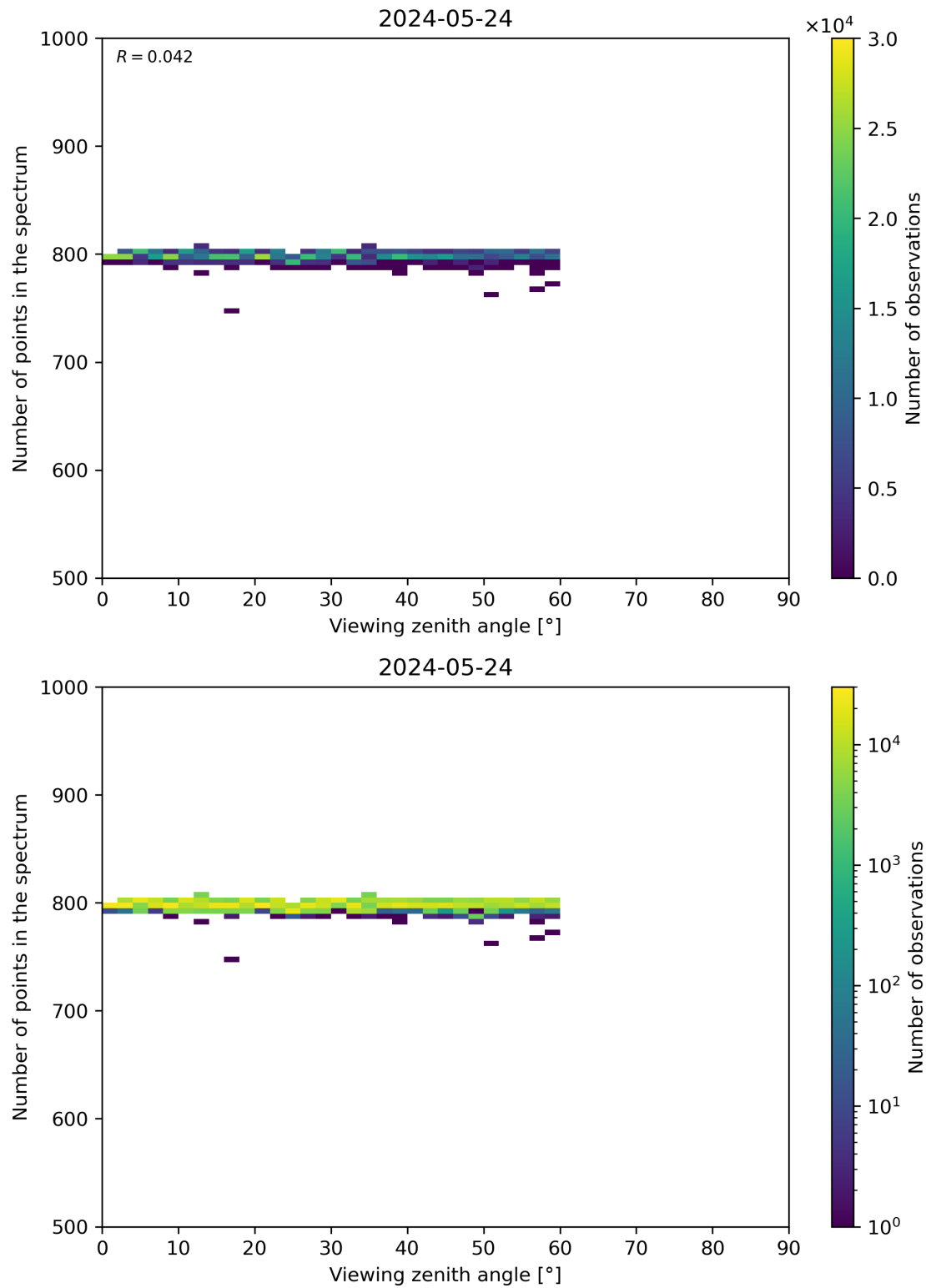
Figure 114: Scatter density plot of “Viewing zenith angle” against “Number of points in the spectrum” for 2024-05-23 to 2024-05-25.
