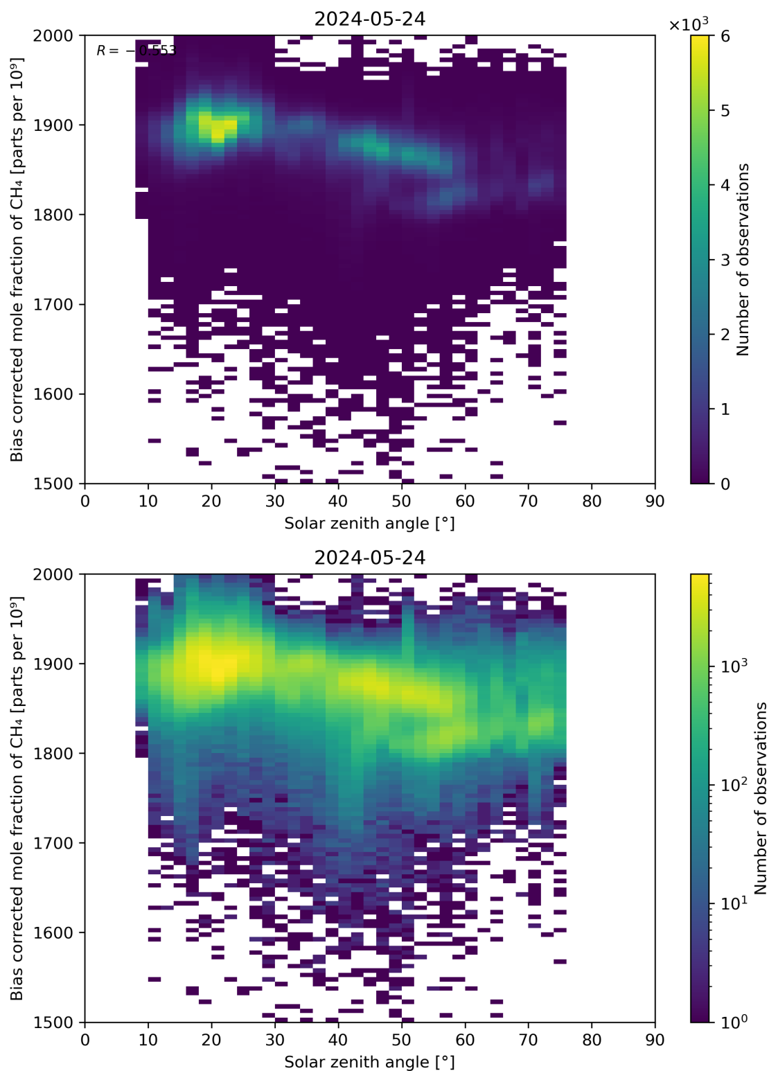
Figure 100: Scatter density plot of “Solar zenith angle” against “Bias corrected mole fraction of CH 4 ” for 2024-05-23 to 2024-05-25.
