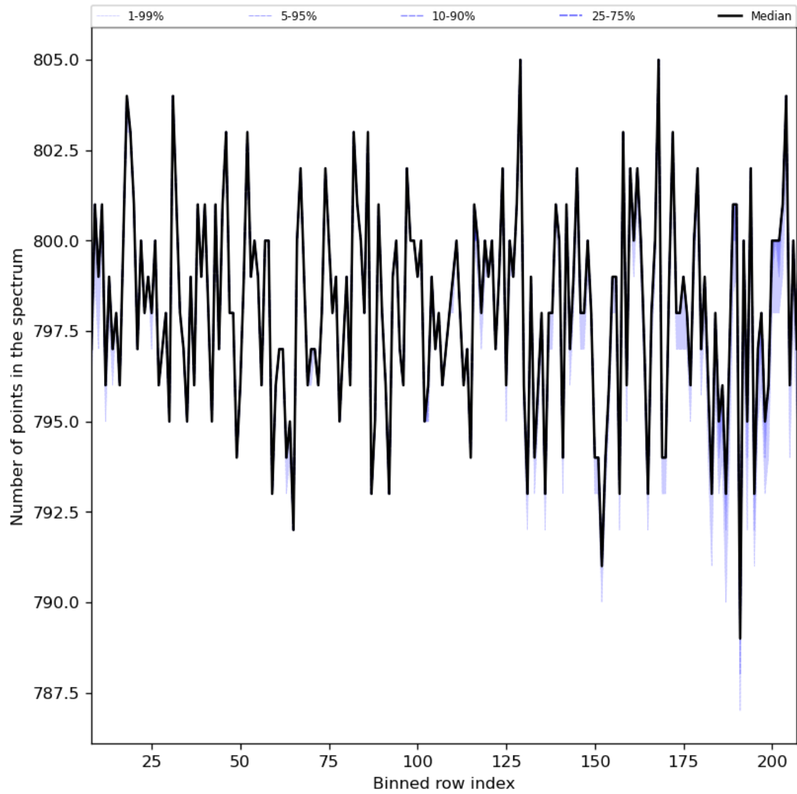
Figure 37: Along track statistics of “Number of points in the spectrum” for 2024-05-23 to 2024-05-25
