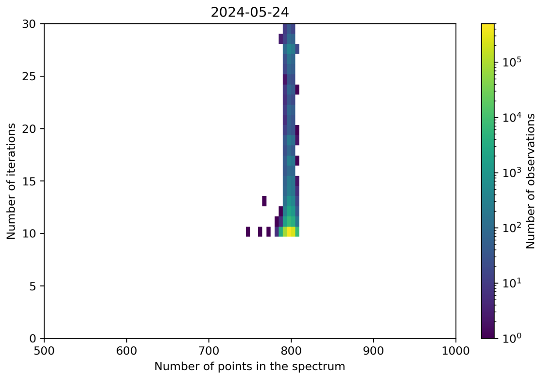
Figure 92: Scatter density plot of “Number of points in the spectrum” against “Number of iterations” for 2024-05-23 to 2024-05-25.
