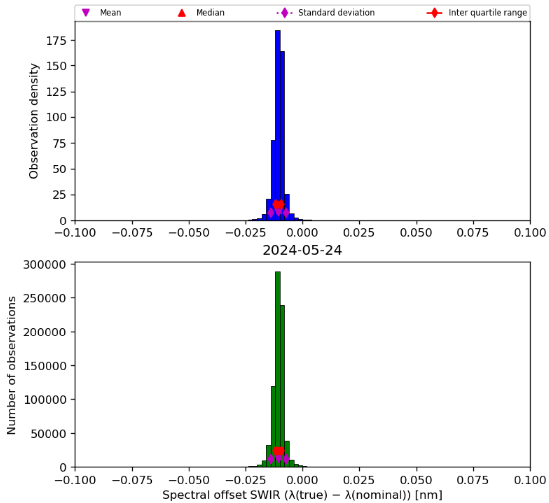
Figure 27: Histogram of “Spectral offset SWIR ( \lambda(\text{true}) - \lambda(\text{nominal}) )” for 2024-05-23 to 2024-05-25
