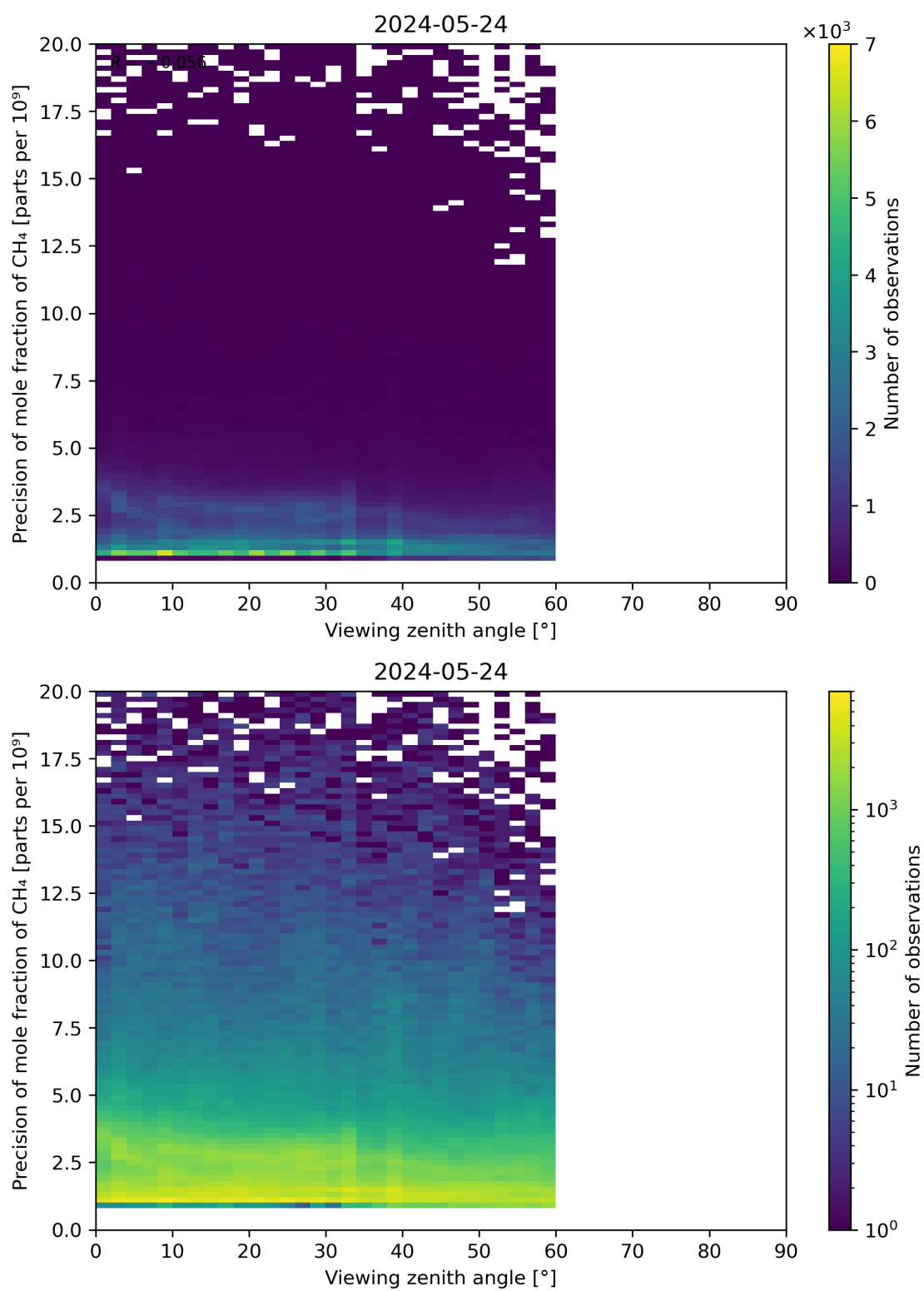
Figure 112: Scatter density plot of “Viewing zenith angle” against “Precision of mole fraction of CH 4 ” for 2024-05-23 to 2024-05-25.
