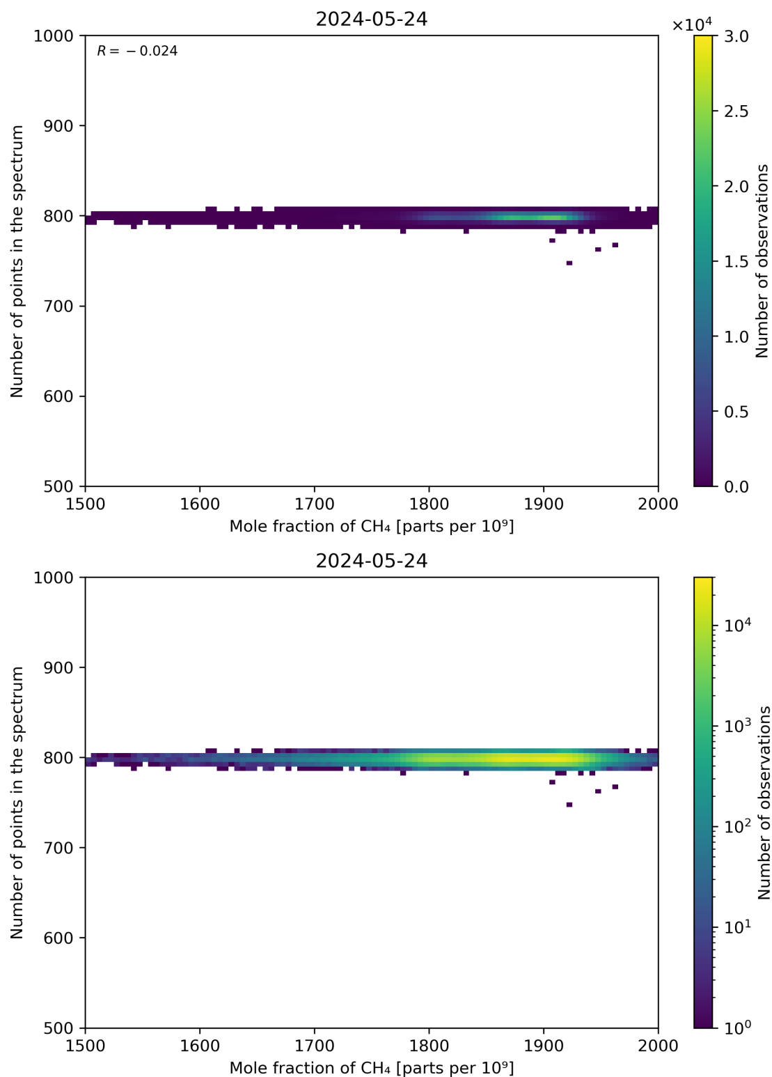
Figure 77: Scatter density plot of “Mole fraction of CH 4 ” against “Number of points in the spectrum” for 2024-05-23 to 2024-05-25.
