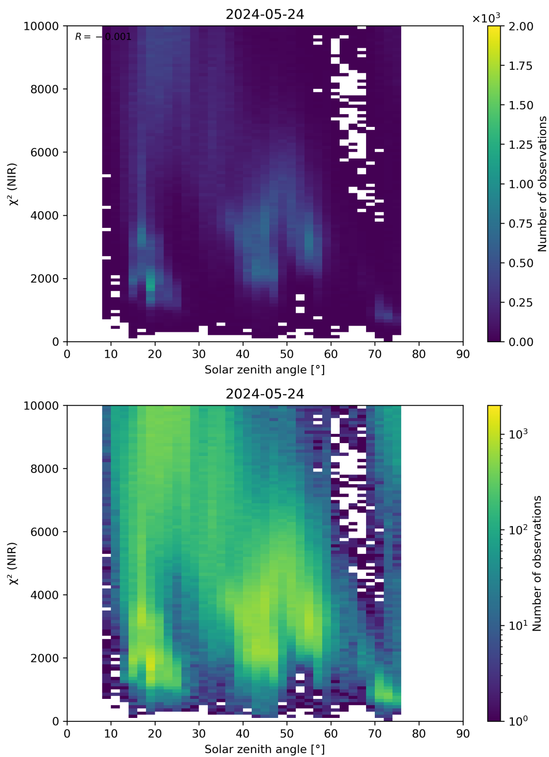
Figure 94: Scatter density plot of “Solar zenith angle” against “ \chi^2 (NIR)” for 2024-05-23 to 2024-05-25.
