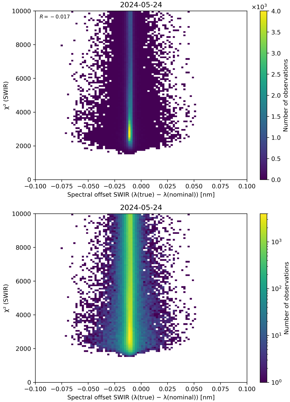
Figure 118: Scatter density plot of “Spectral offset SWIR ( \lambda(\text{true}) - \lambda(\text{nominal}) )” against “ \chi^2 (SWIR)” for 2024-05-23 to 2024-05-25.
