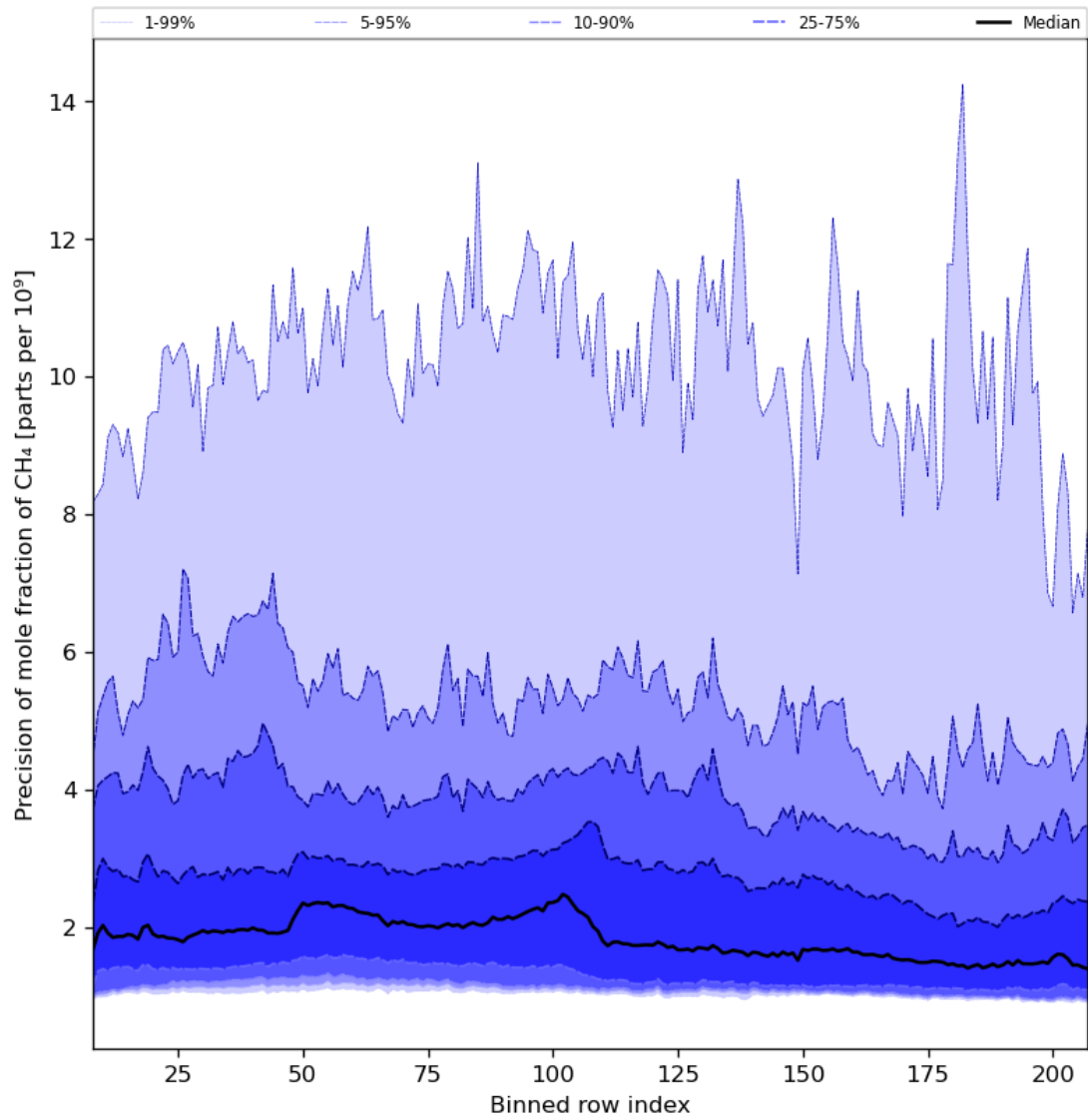
Figure 35: Along track statistics of “Precision of mole fraction of CH 4 ” for 2024-05-23 to 2024-05-25
