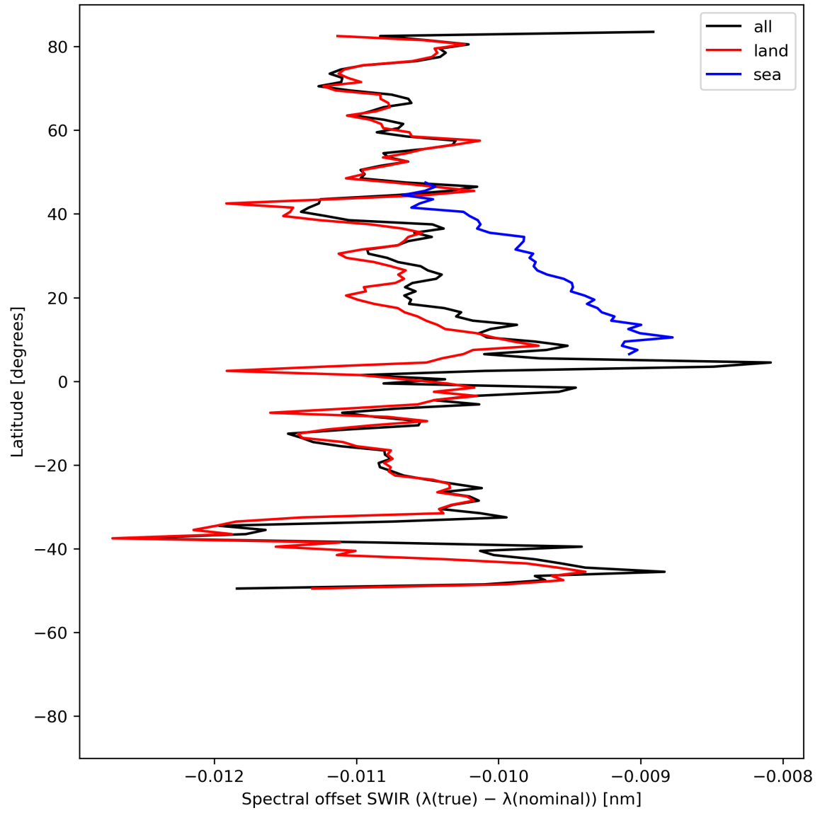
Figure 16: Zonal average of “Spectral offset SWIR ( \lambda(\text{true}) - \lambda(\text{nominal}) )” for 2024-05-23 to 2024-05-25.
