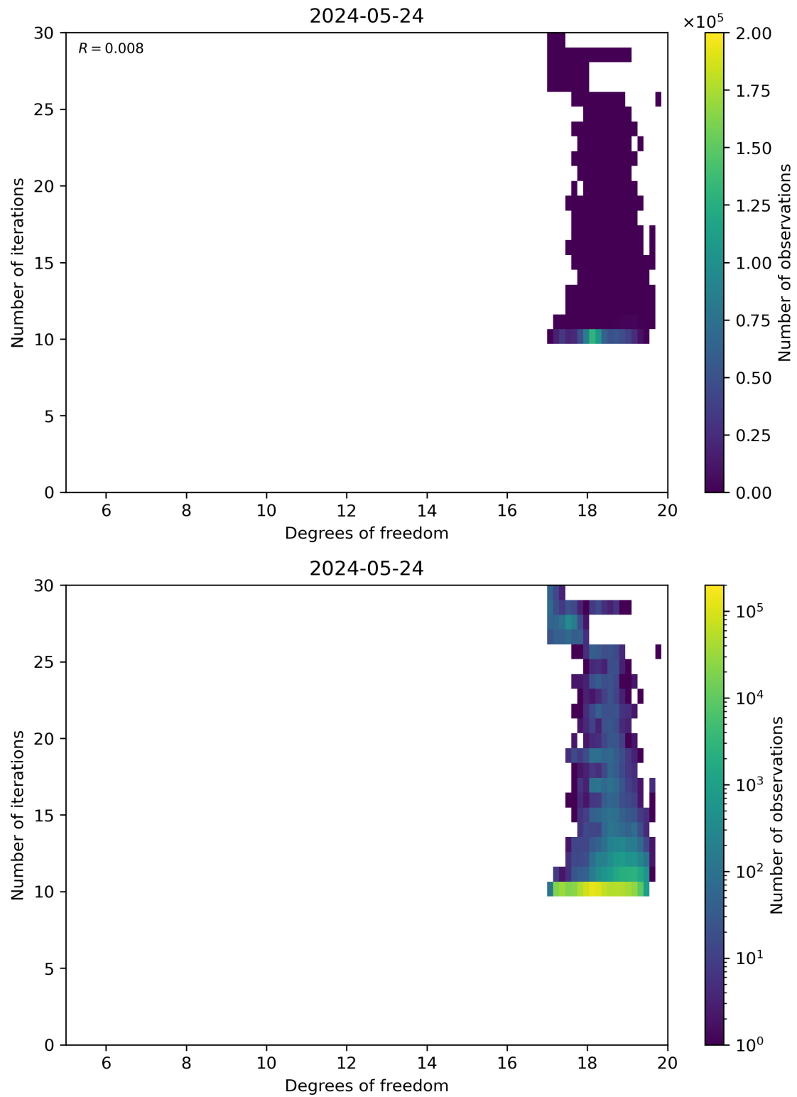
Figure 52: Scatter density plot of “Degrees of freedom” against “Number of iterations” for 2024-05-23 to 2024-05-25.
