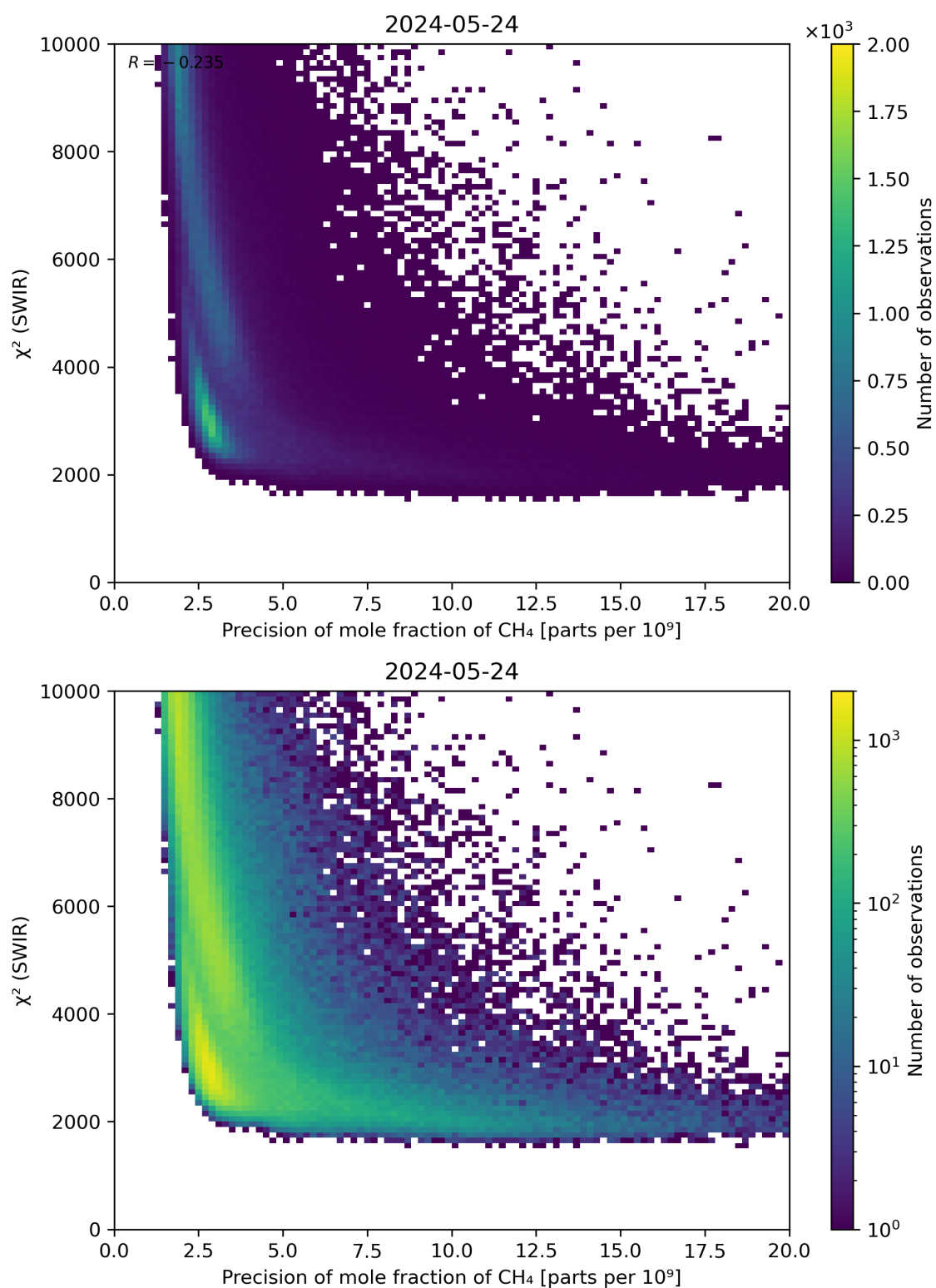
Figure 79: Scatter density plot of “Precision of mole fraction of \text{CH}_4 ” against “ \chi^2 (SWIR)” for 2024-05-23 to 2024-05-25.
