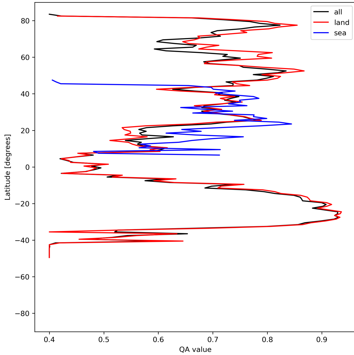
Figure 11: Zonal average of “QA value” for 2024-05-23 to 2024-05-25.
