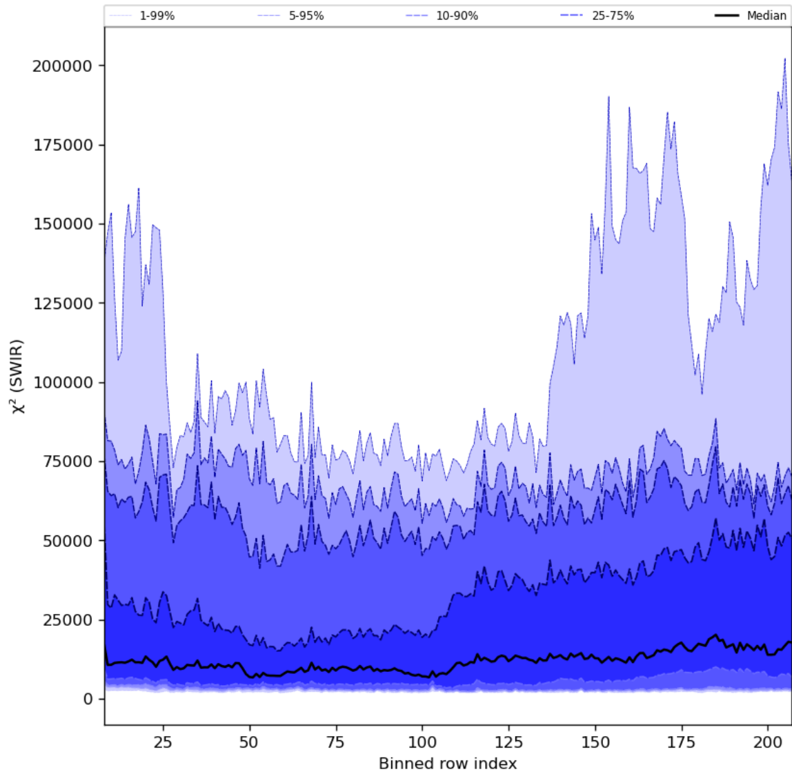
Figure 39: Along track statistics of “ \chi^2 (SWIR)” for 2024-05-23 to 2024-05-25
