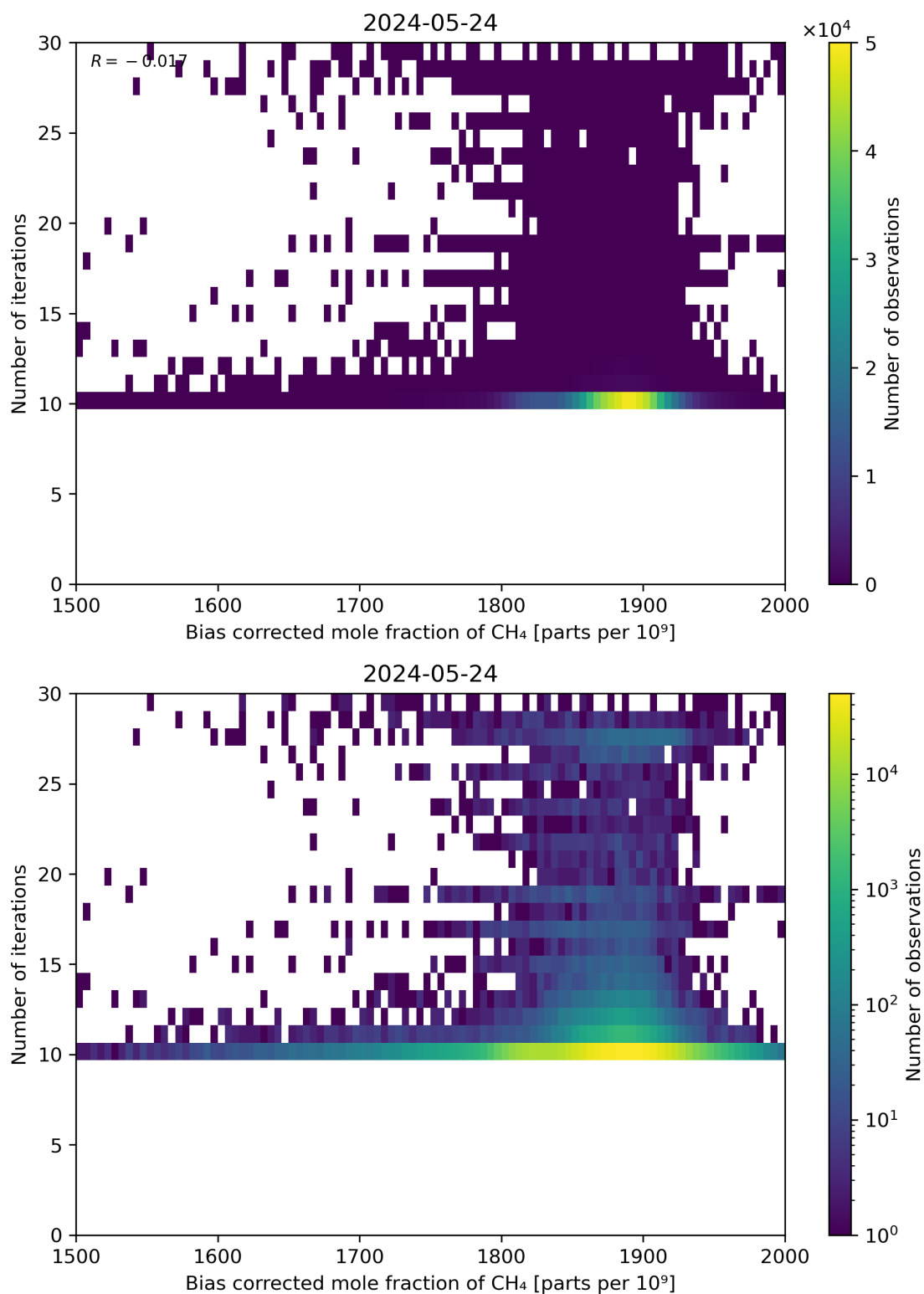
Figure 67: Scatter density plot of “Bias corrected mole fraction of CH 4 ” against “Number of iterations” for 2024-05-23 to 2024-05-25.
