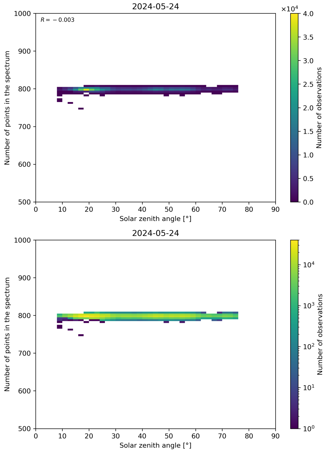
Figure 103: Scatter density plot of “Solar zenith angle” against “Number of points in the spectrum” for 2024-05-23 to 2024-05-25.
