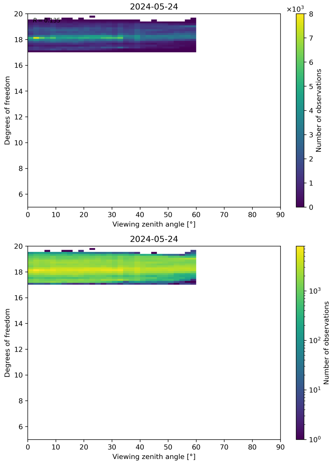
Figure 107: Scatter density plot of “Viewing zenith angle” against “Degrees of freedom” for 2024-05-23 to 2024-05-25.
