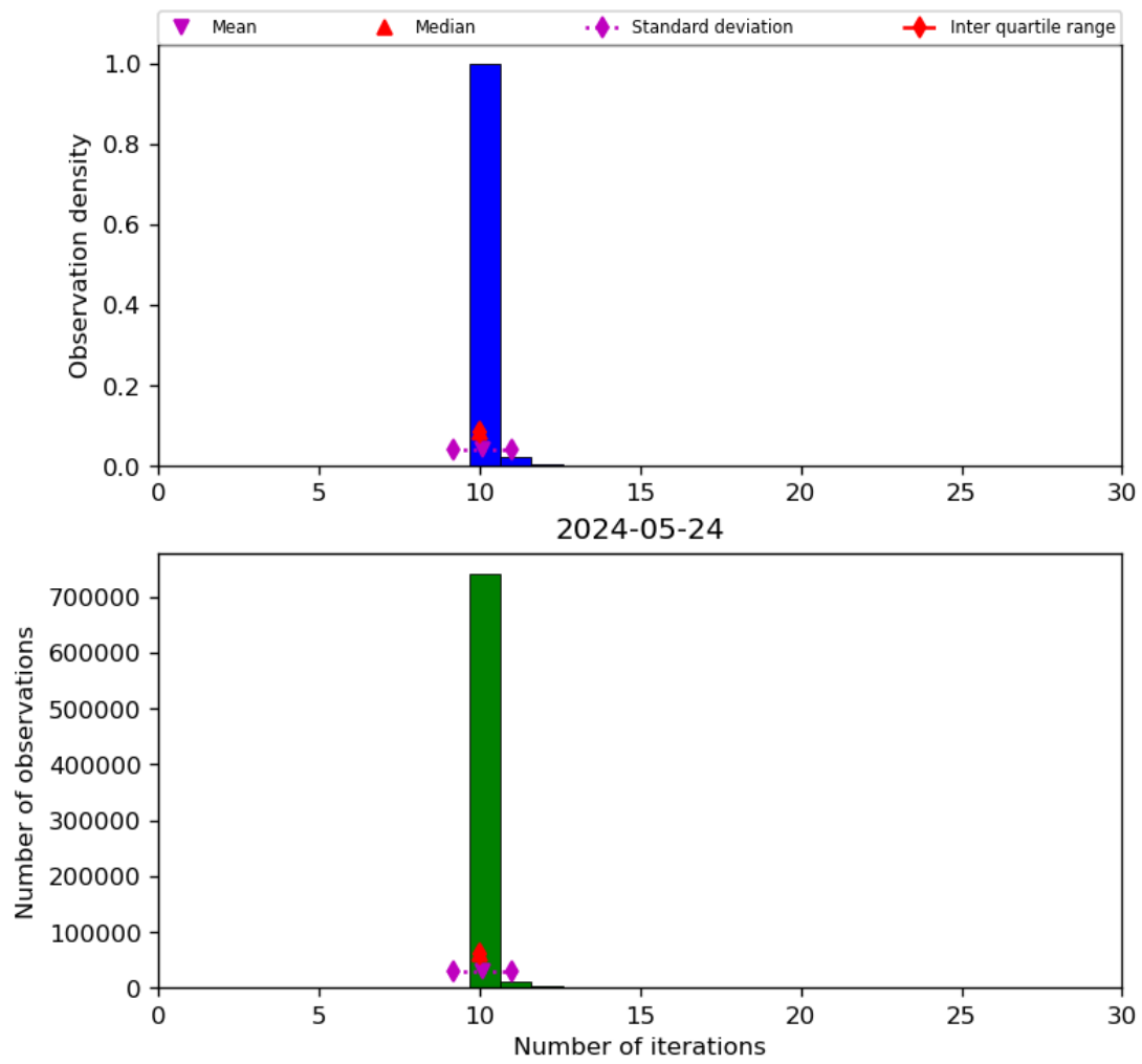
Figure 31: Histogram of “Number of iterations” for 2024-05-23 to 2024-05-25
