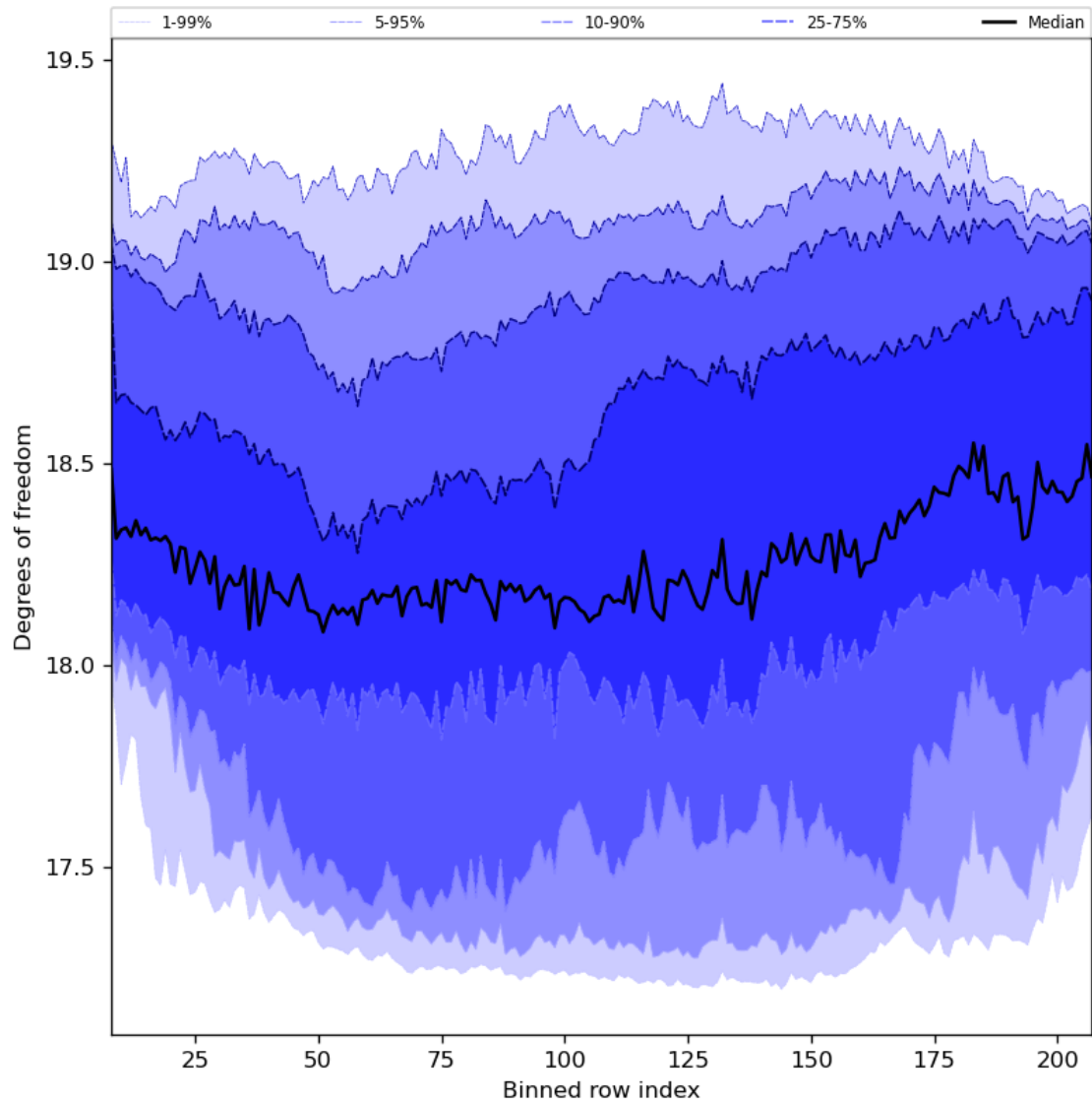
Figure 41: Along track statistics of “Degrees of freedom” for 2024-05-23 to 2024-05-25
