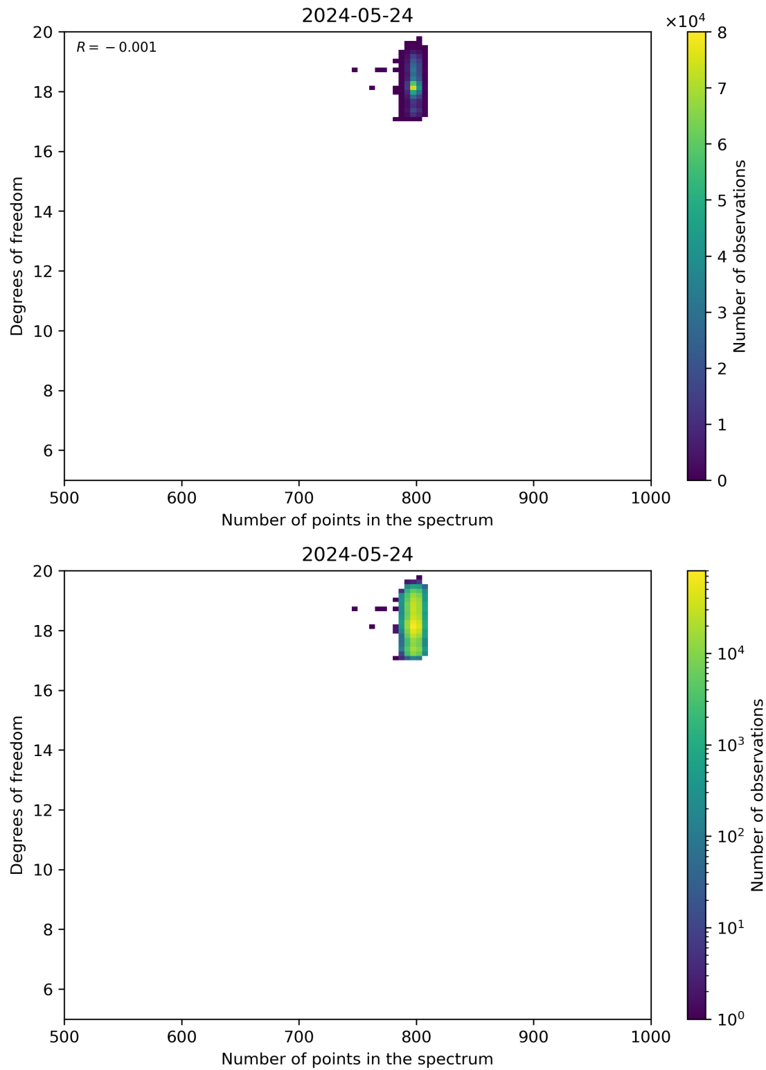
Figure 90: Scatter density plot of “Number of points in the spectrum” against “Degrees of freedom” for 2024-05-23 to 2024-05-25.
