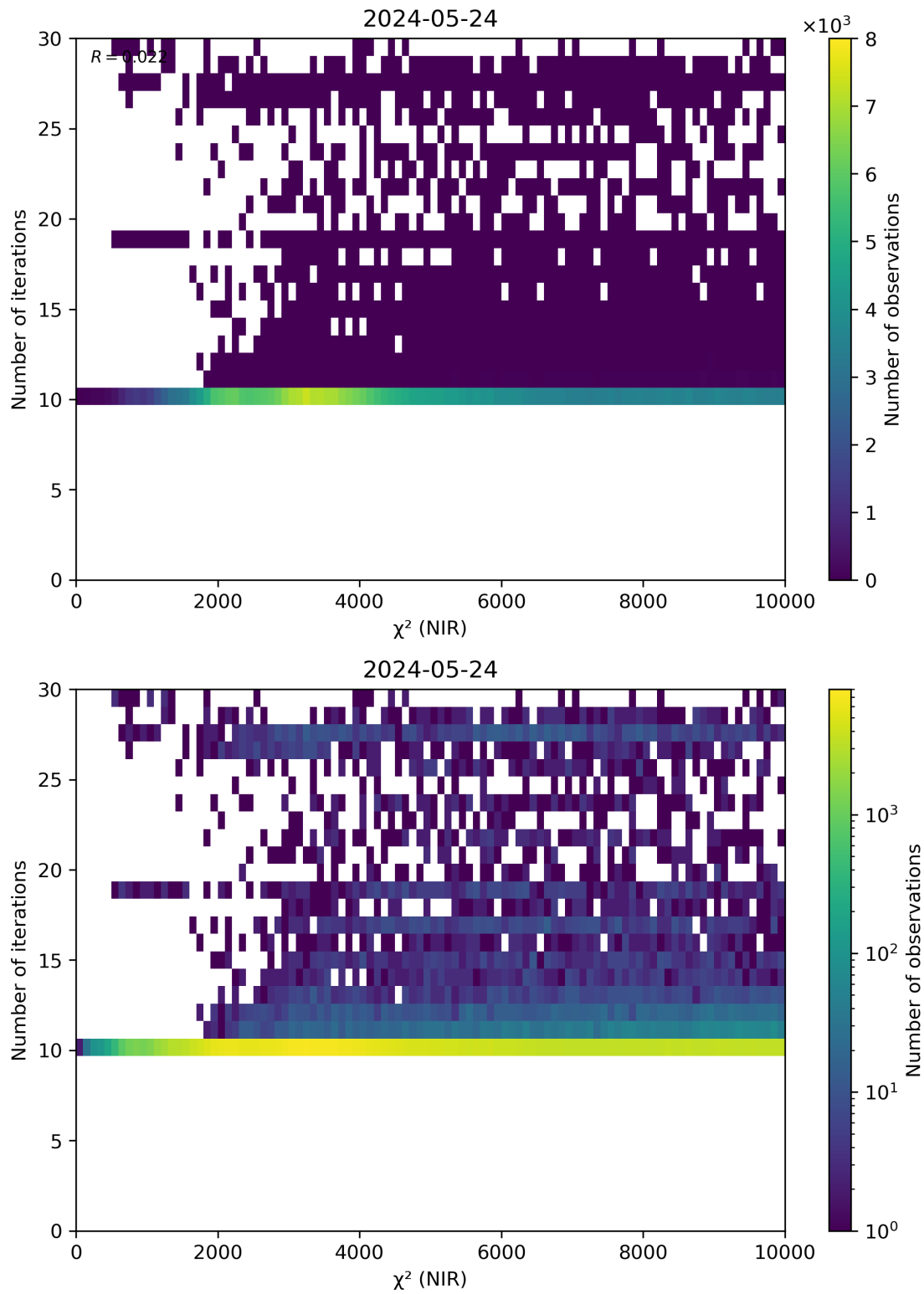
Figure 46: Scatter density plot of “ \chi^2 (NIR)” against “Number of iterations” for 2024-05-23 to 2024-05-25.
