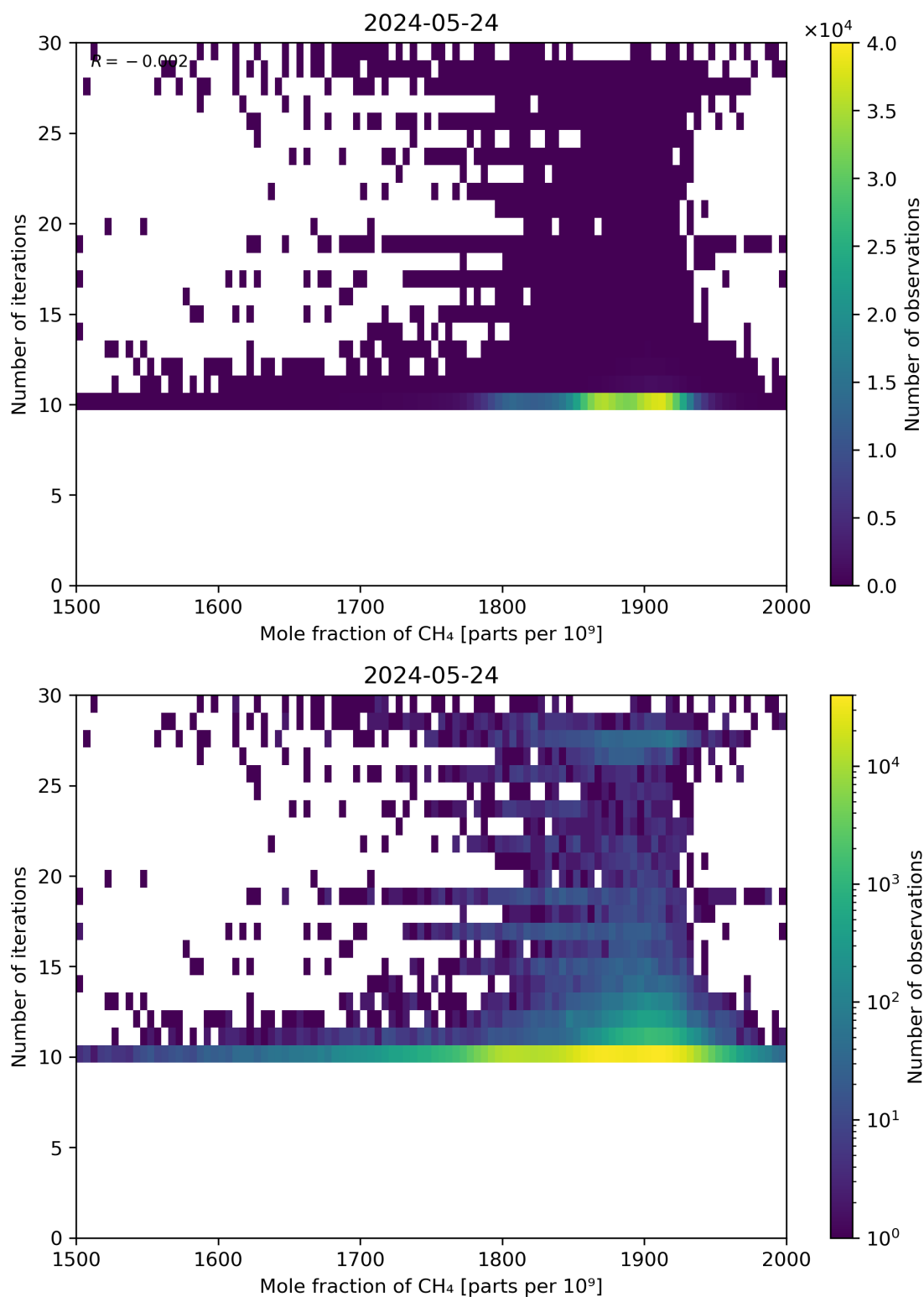
Figure 76: Scatter density plot of “Mole fraction of CH 4 ” against “Number of iterations” for 2024-05-23 to 2024-05-25.
