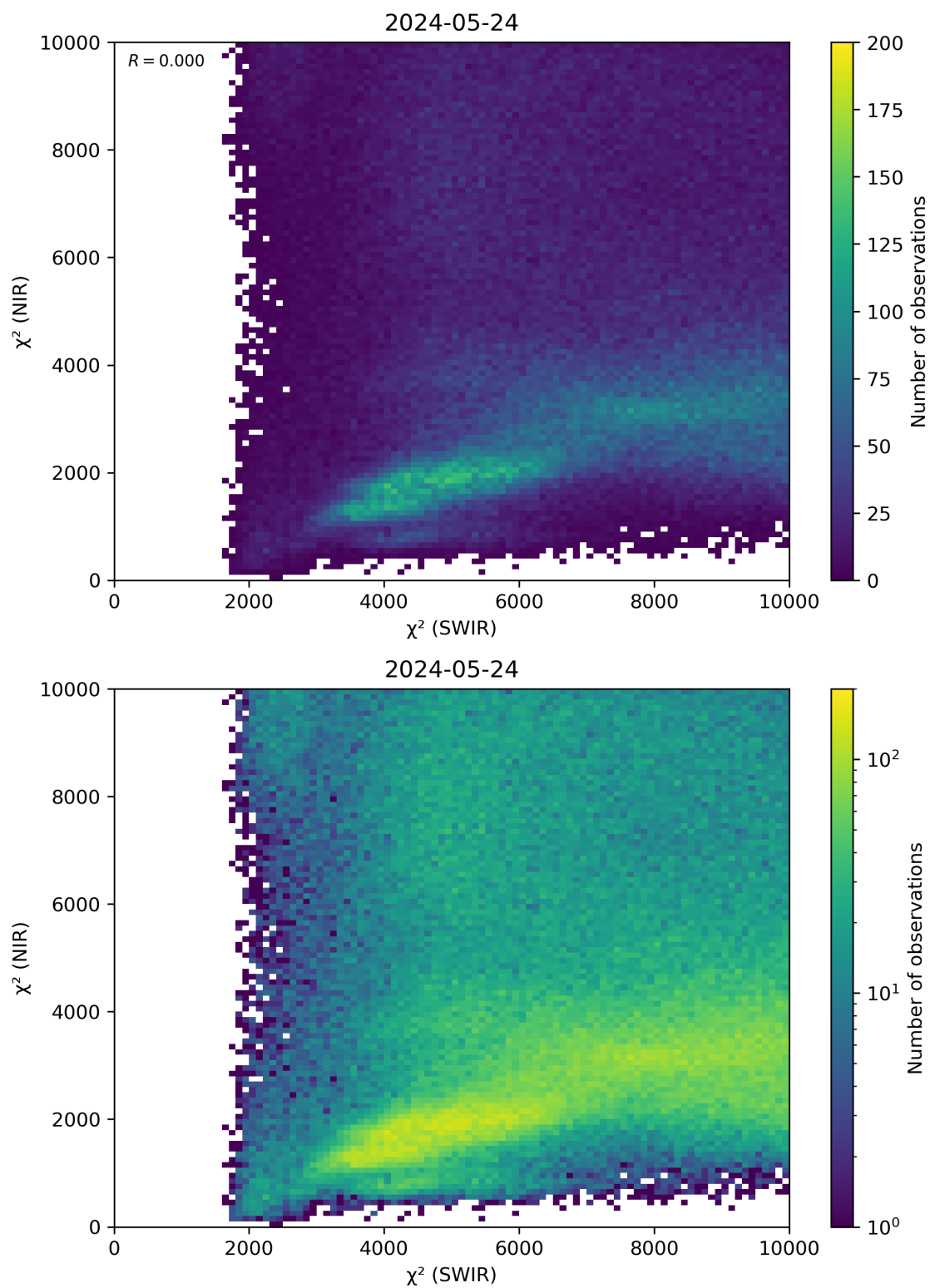
Figure 47: Scatter density plot of “ \chi^2 (SWIR)” against “ \chi^2 (NIR)” for 2024-05-23 to 2024-05-25.
