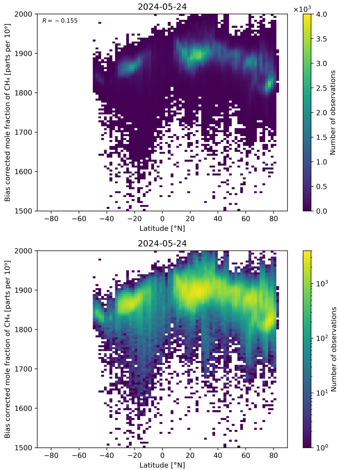
Figure 58: Scatter density plot of “Latitude” against “Bias corrected mole fraction of \text{CH}_4 ” for 2024-05-23 to 2024-05-25.
