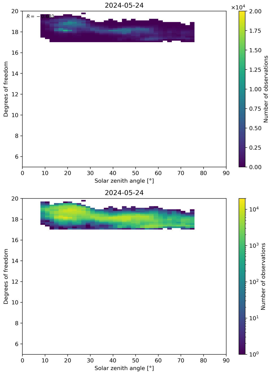
Figure 96: Scatter density plot of “Solar zenith angle” against “Degrees of freedom” for 2024-05-23 to 2024-05-25.
