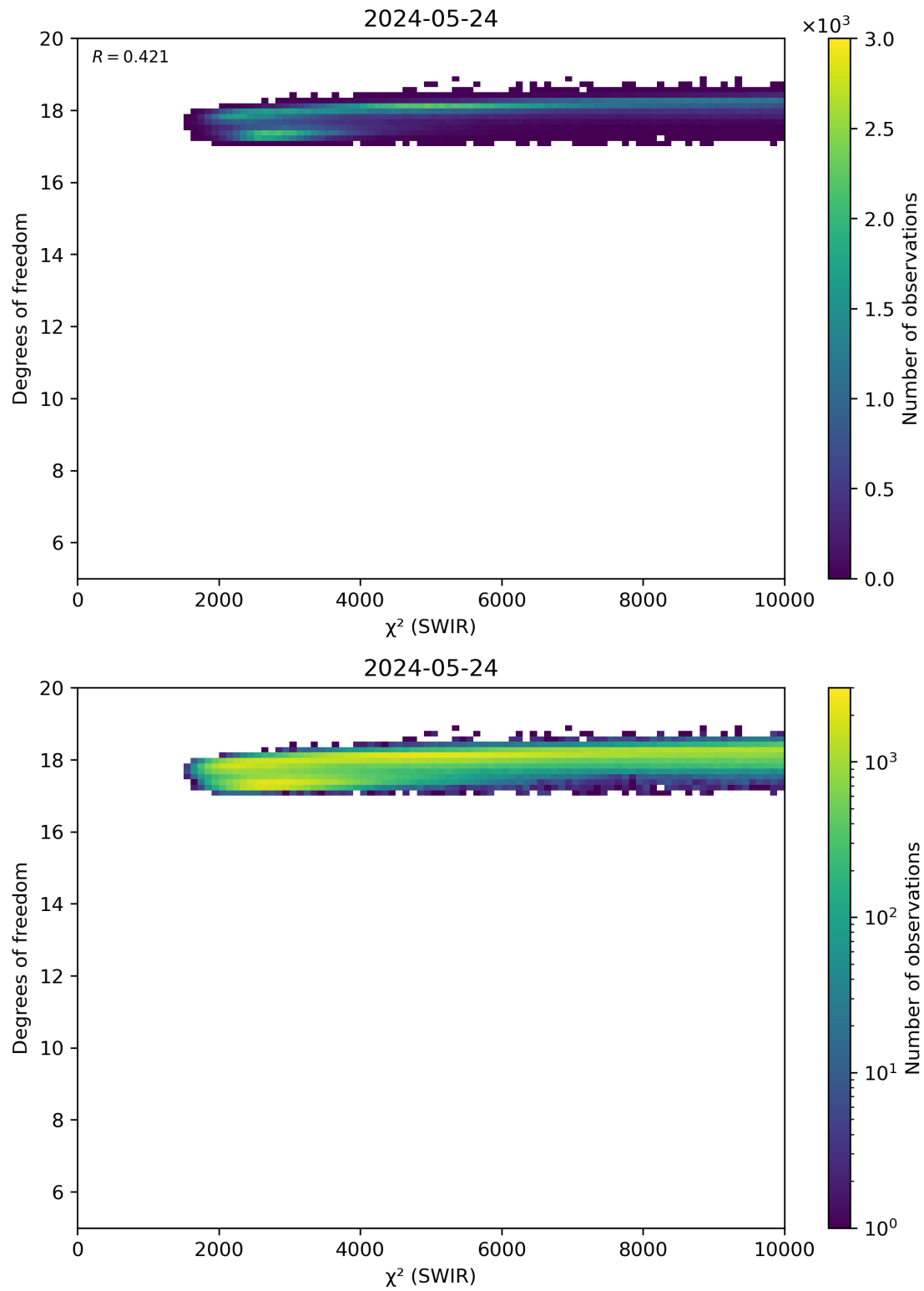
Figure 48: Scatter density plot of " \chi^2 (SWIR)" against "Degrees of freedom" for 2024-05-23 to 2024-05-25.
