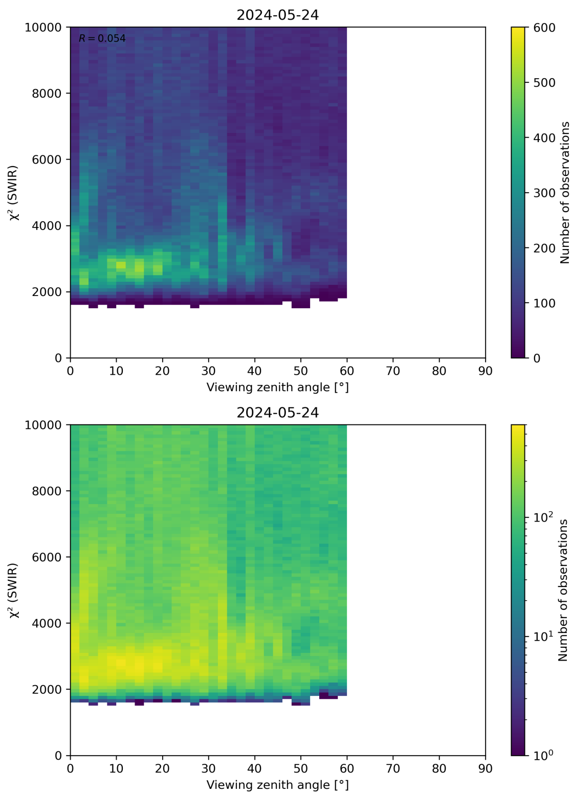
Figure 106: Scatter density plot of “Viewing zenith angle” against “ \chi^2 (SWIR)” for 2024-05-23 to 2024-05-25.
