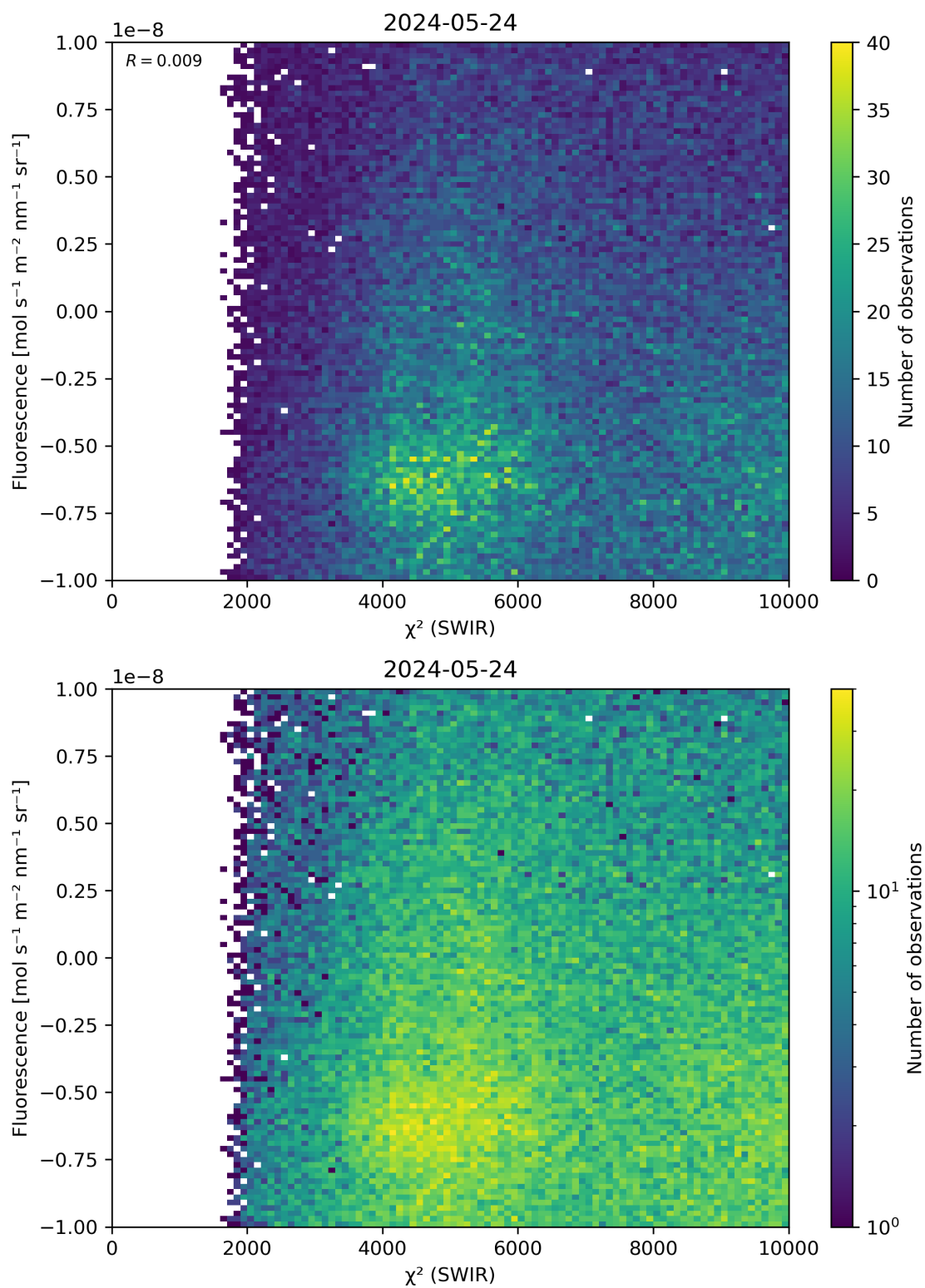
Figure 49: Scatter density plot of “ \chi^2 (SWIR)” against “Fluorescence” for 2024-05-23 to 2024-05-25.
