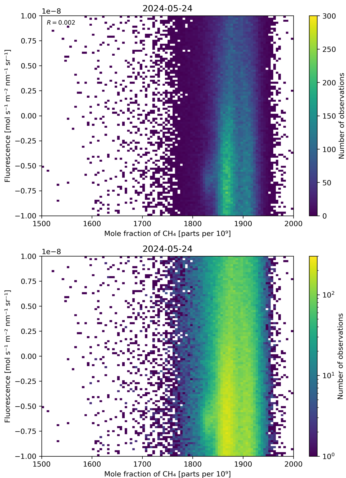
Figure 73: Scatter density plot of “Mole fraction of \text{CH}_4 ” against “Fluorescence” for 2024-05-23 to 2024-05-25.
