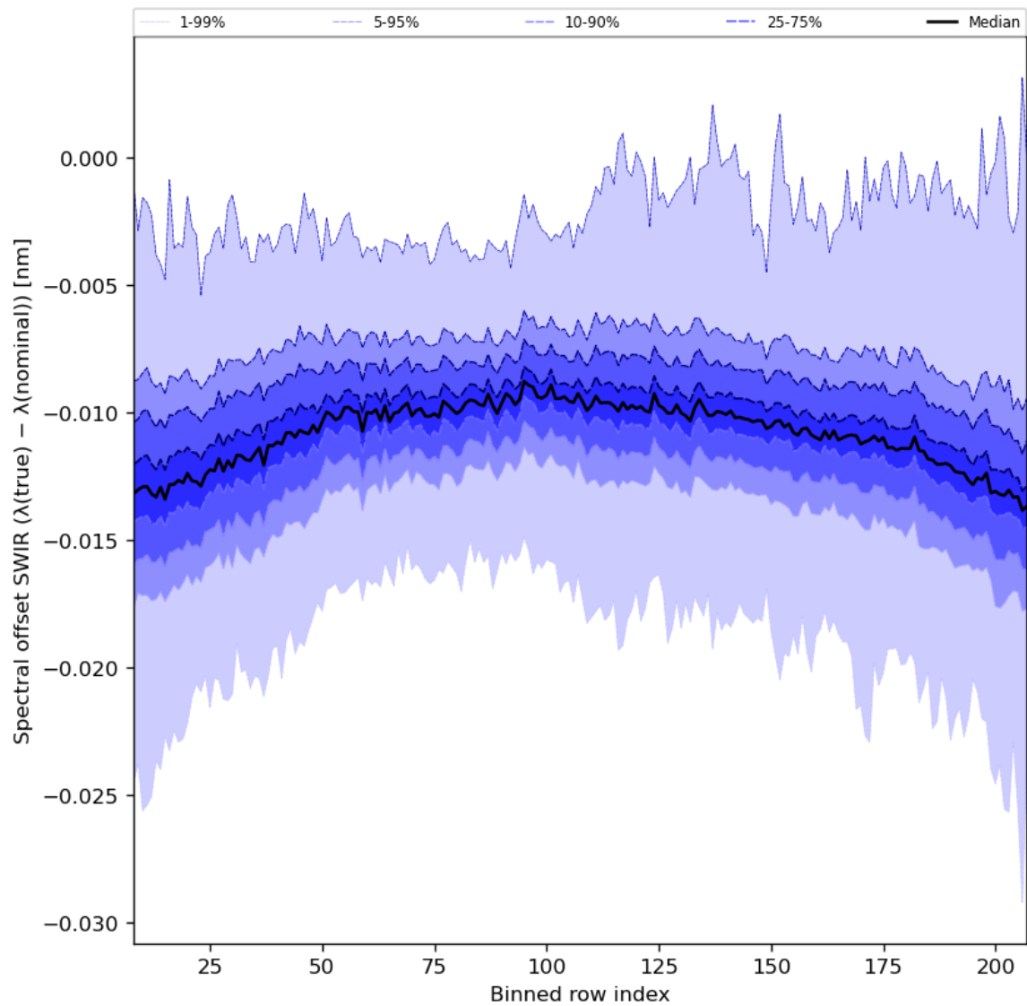
Figure 38: Along track statistics of “Spectral offset SWIR ( \lambda(\text{true}) - \lambda(\text{nominal}) )” for 2024-05-23 to 2024-05-25
