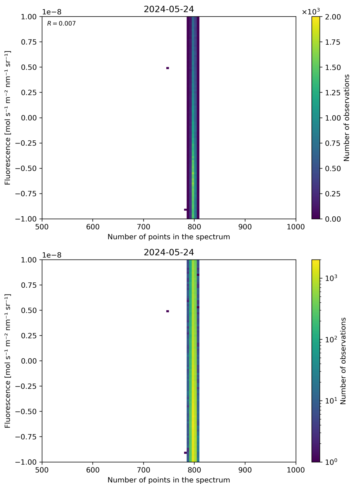
Figure 91: Scatter density plot of “Number of points in the spectrum” against “Fluorescence” for 2024-05-23 to 2024-05-25.
