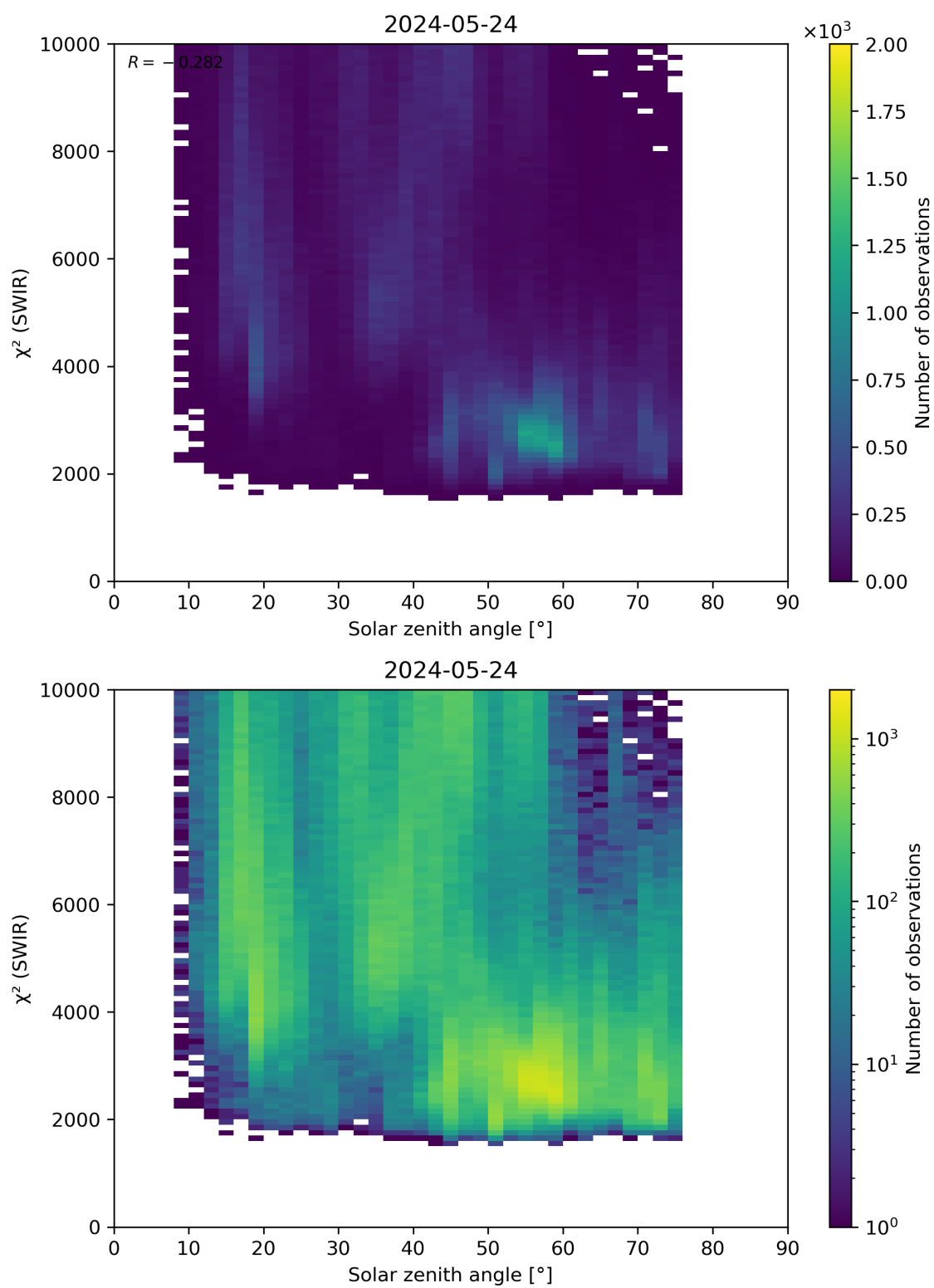
Figure 95: Scatter density plot of “Solar zenith angle” against “ \chi^2 (SWIR)” for 2024-05-23 to 2024-05-25.
