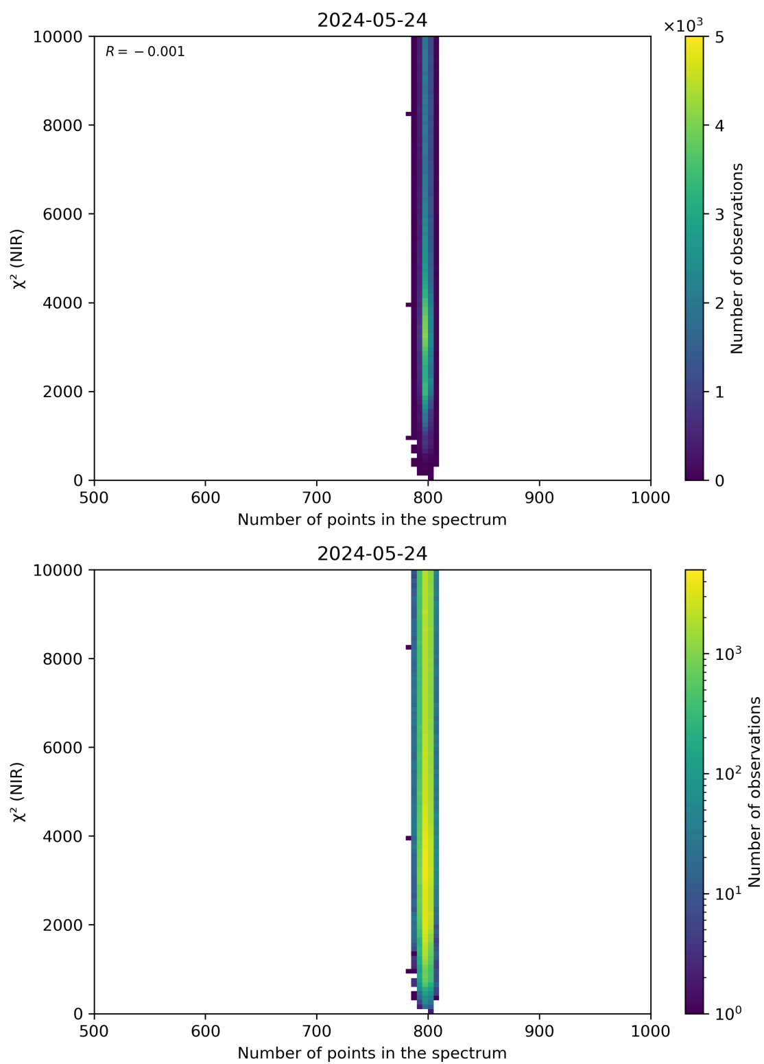
Figure 88: Scatter density plot of “Number of points in the spectrum” against “ \chi^2 (NIR)” for 2024-05-23 to 2024-05-25.
