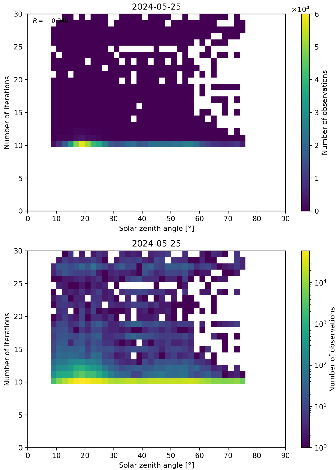
Figure 102: Scatter density plot of “Solar zenith angle” against “Number of iterations” for 2024-05-24 to 2024-05-26.
