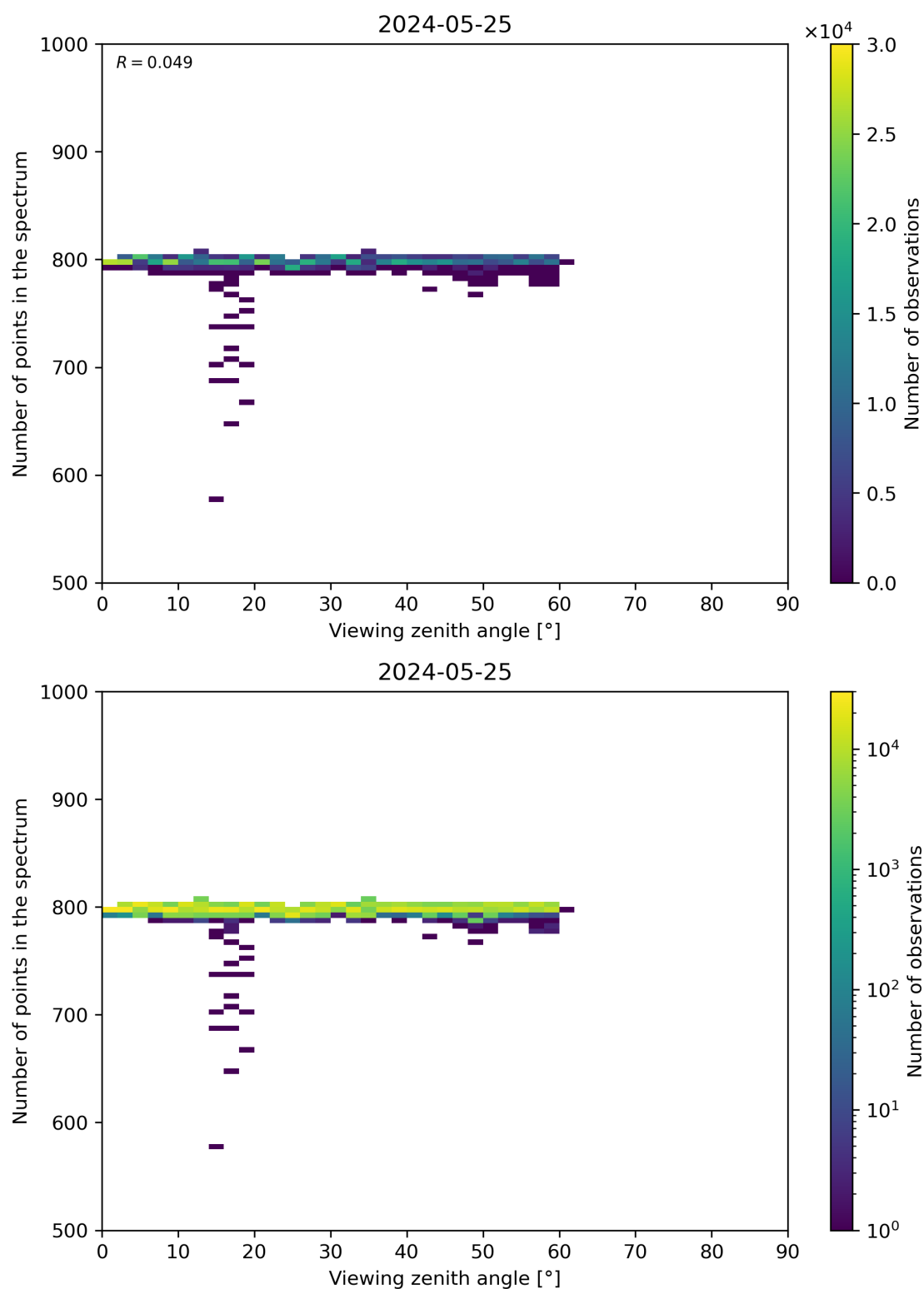
Figure 114: Scatter density plot of “Viewing zenith angle” against “Number of points in the spectrum” for 2024-05-24 to 2024-05-26.
