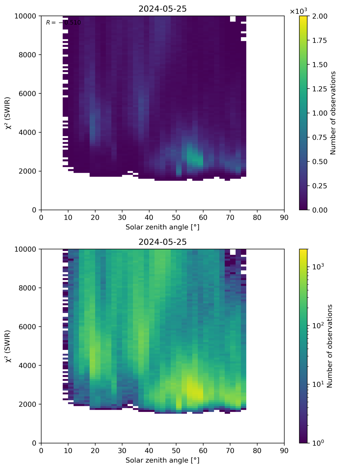
Figure 95: Scatter density plot of “Solar zenith angle” against “ \chi^2 (SWIR)” for 2024-05-24 to 2024-05-26.
