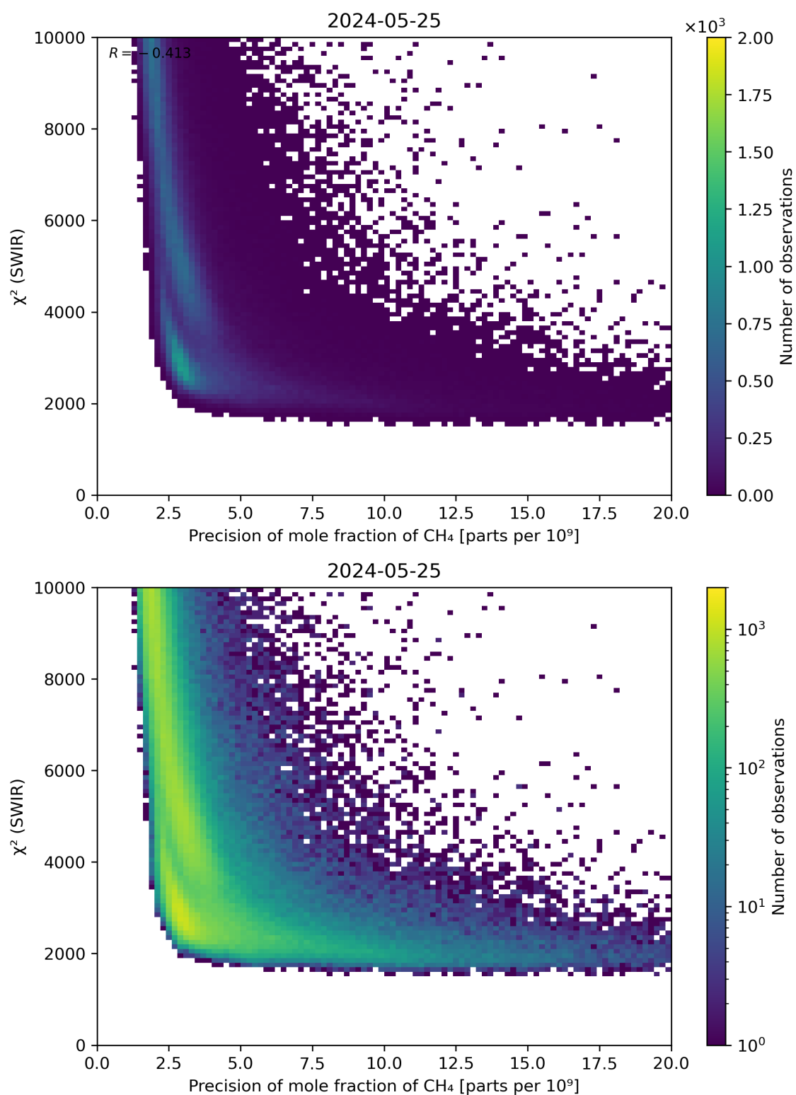
Figure 79: Scatter density plot of “Precision of mole fraction of \text{CH}_4 ” against “ \chi^2 (SWIR)” for 2024-05-24 to 2024-05-26.
