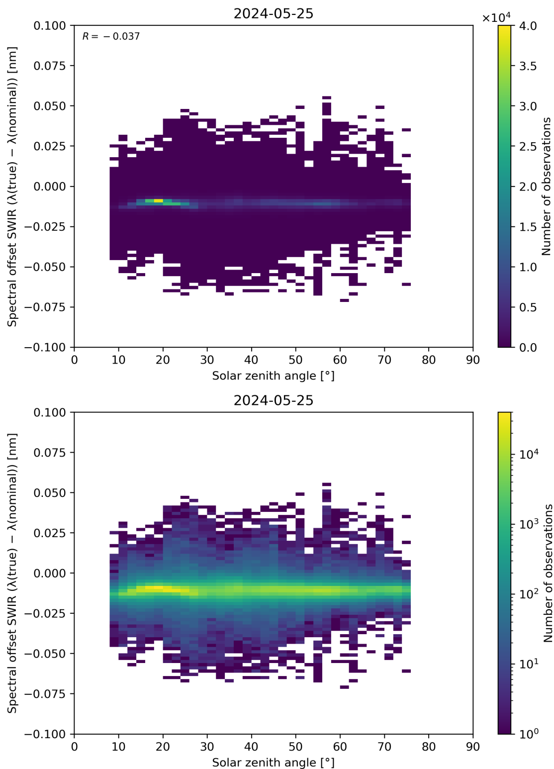
Figure 104: Scatter density plot of “Solar zenith angle” against “Spectral offset SWIR ( \lambda(\text{true}) - \lambda(\text{nominal}) )” for 2024-05-24 to 2024-05-26.
