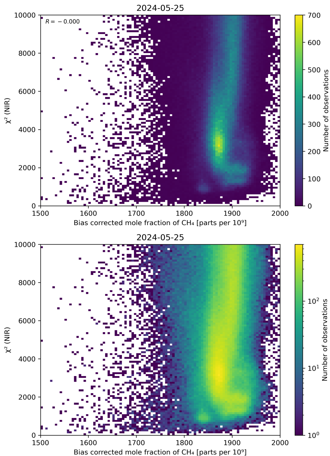
Figure 63: Scatter density plot of “Bias corrected mole fraction of CH 4 ” against “ \chi^2 (NIR)” for 2024-05-24 to 2024-05-26.
