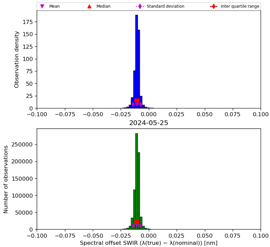
Figure 27: Histogram of “Spectral offset SWIR ( \lambda(\text{true}) - \lambda(\text{nominal}) )” for 2024-05-24 to 2024-05-26
