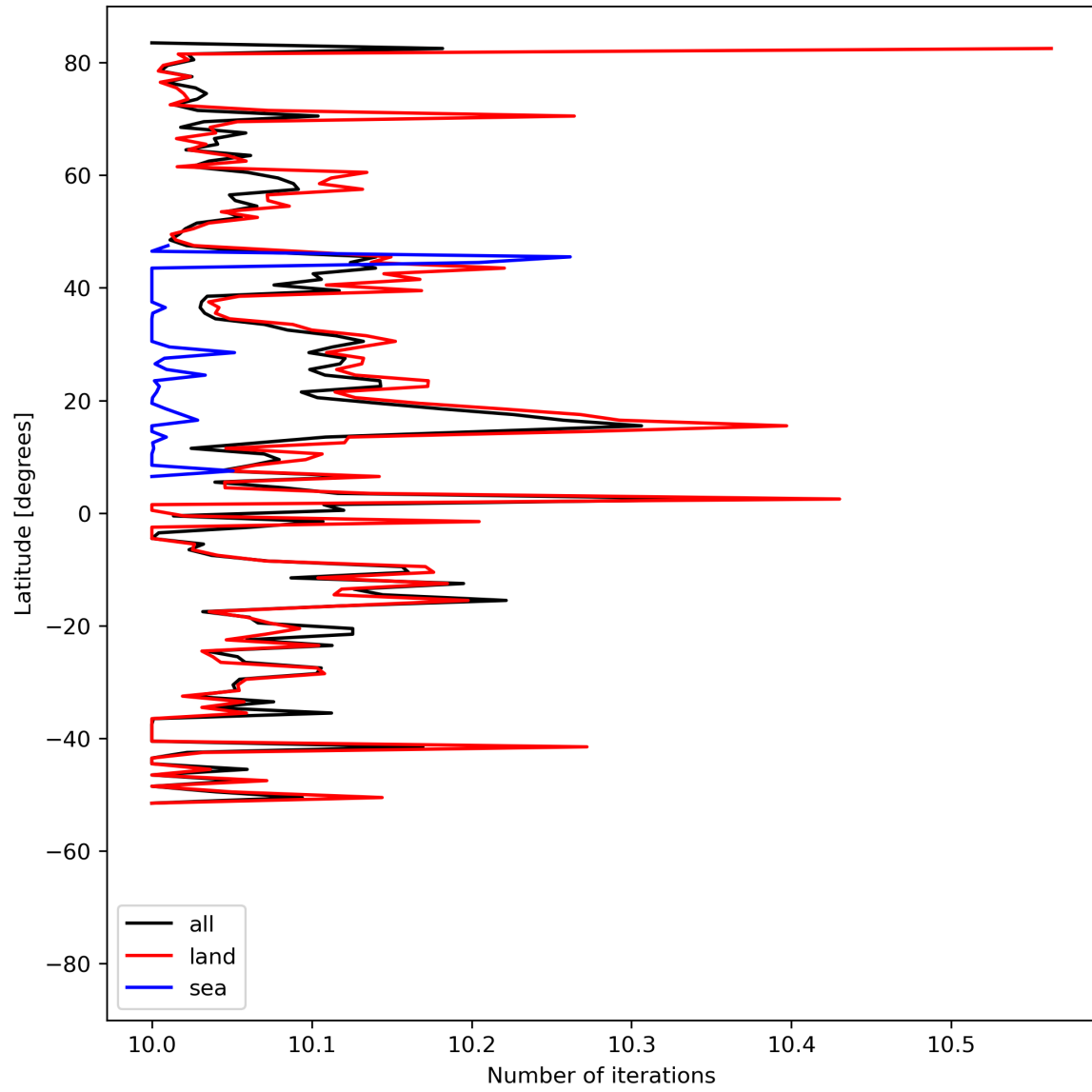
Figure 20: Zonal average of “Number of iterations” for 2024-05-24 to 2024-05-26.
