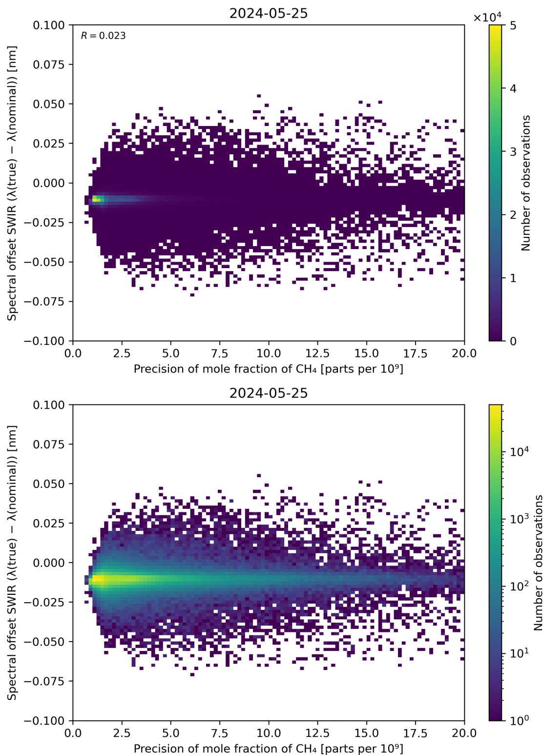
Figure 85: Scatter density plot of “Precision of mole fraction of \text{CH}_4 ” against “Spectral offset SWIR ( \lambda(\text{true}) - \lambda(\text{nominal}) )” for 2024-05-24 to 2024-05-26.
