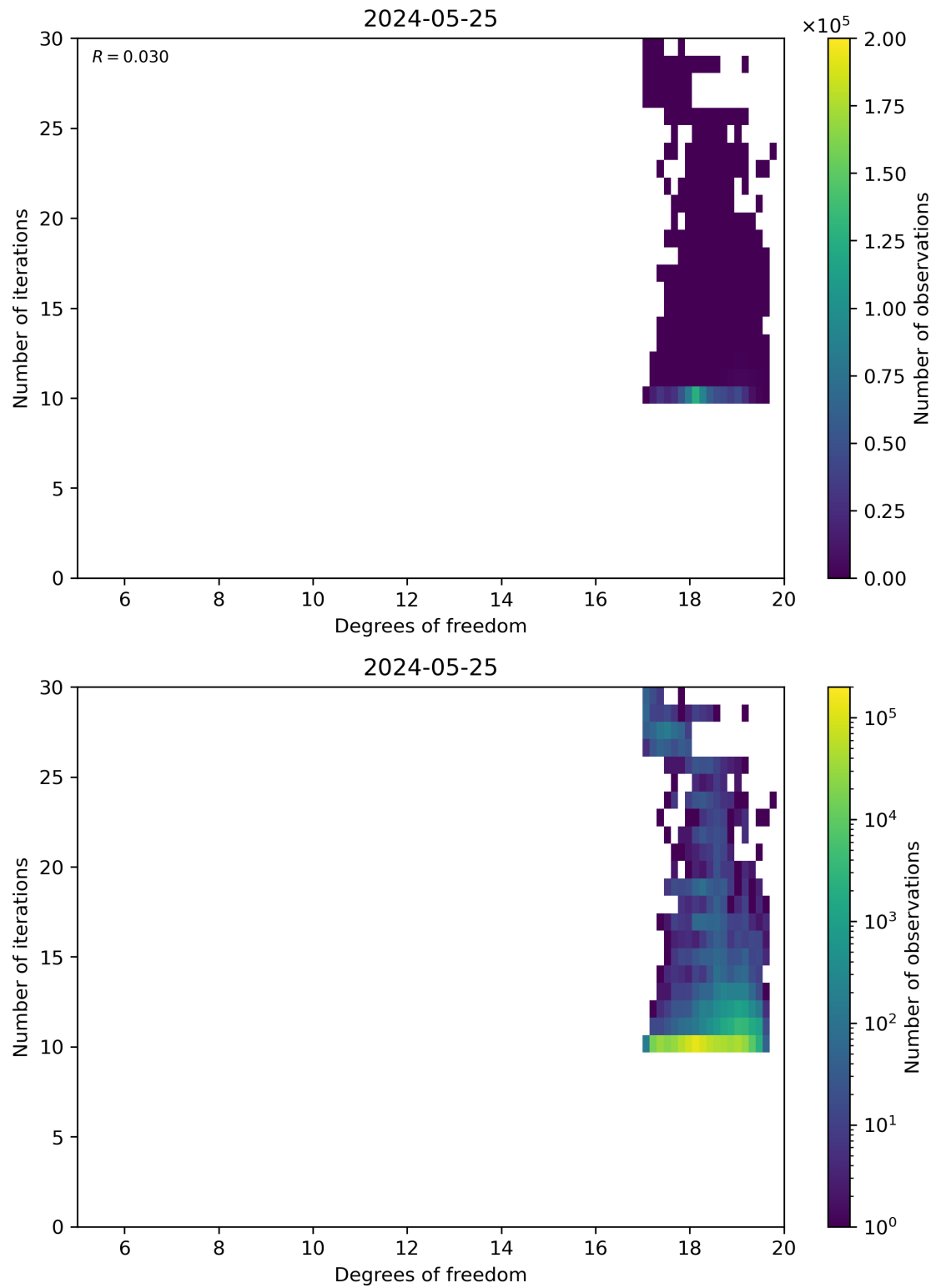
Figure 52: Scatter density plot of “Degrees of freedom” against “Number of iterations” for 2024-05-24 to 2024-05-26.
