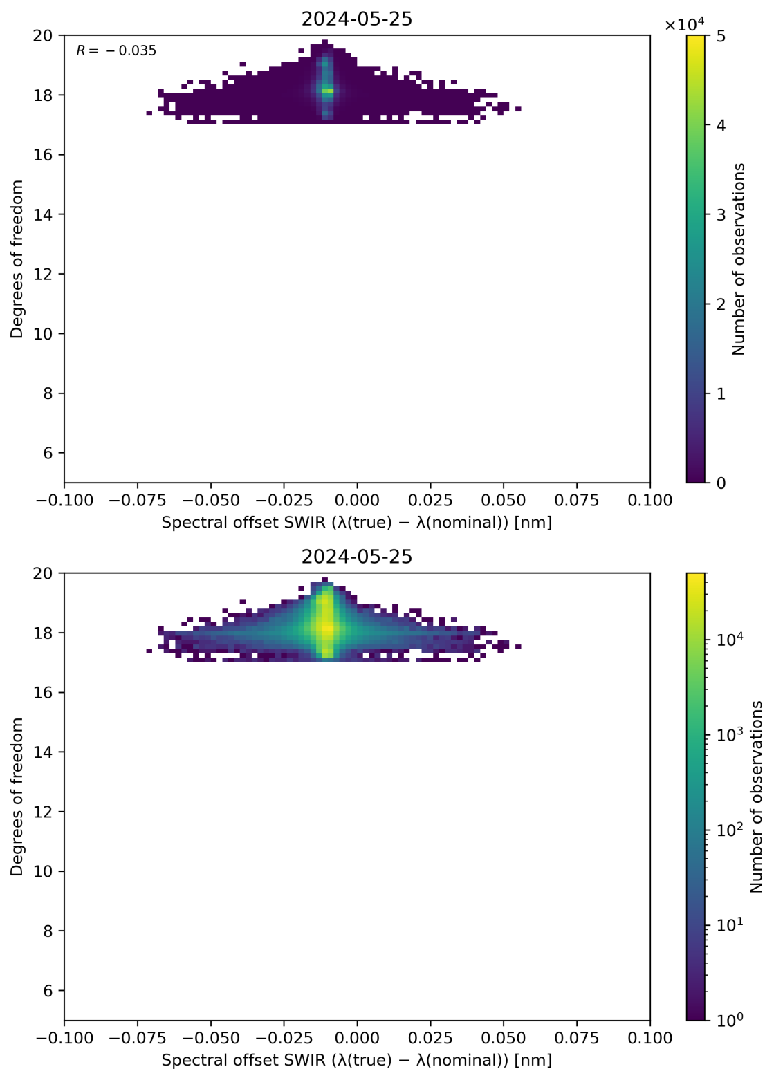
Figure 119: Scatter density plot of “Spectral offset SWIR ( \lambda(\text{true}) - \lambda(\text{nominal}) )” against “Degrees of freedom” for 2024-05-24 to 2024-05-26.
