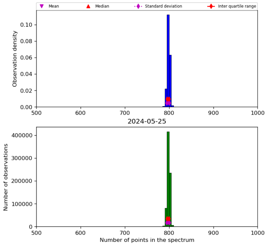
Figure 26: Histogram of “Number of points in the spectrum” for 2024-05-24 to 2024-05-26
