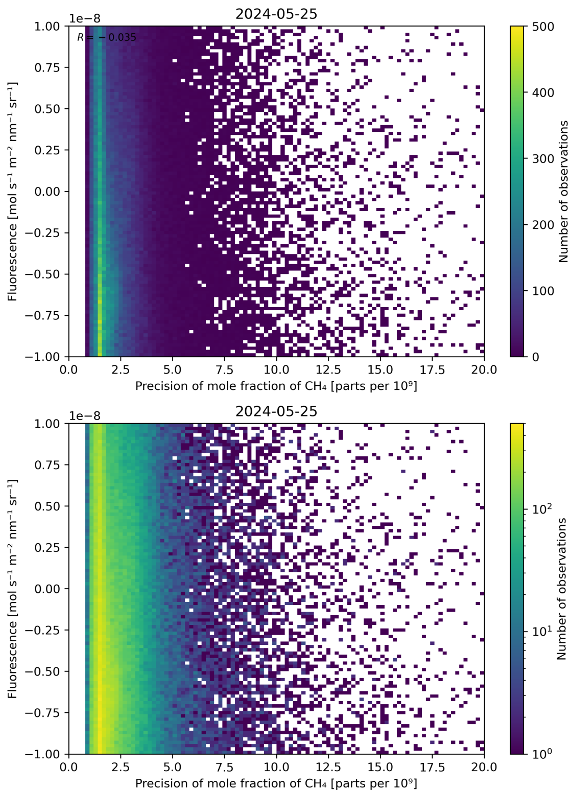
Figure 81: Scatter density plot of “Precision of mole fraction of CH 4 ” against “Fluorescence” for 2024-05-24 to 2024-05-26.
