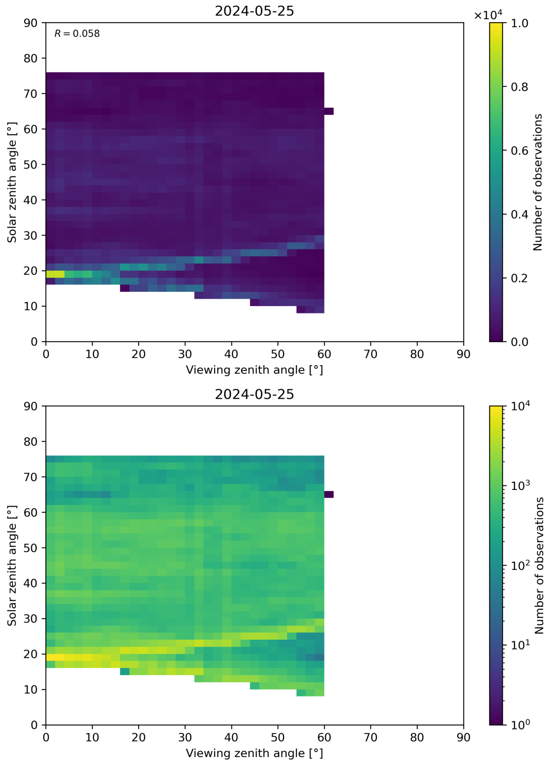
Figure 115: Scatter density plot of “Viewing zenith angle” against “Solar zenith angle” for 2024-05-24 to 2024-05-26.
