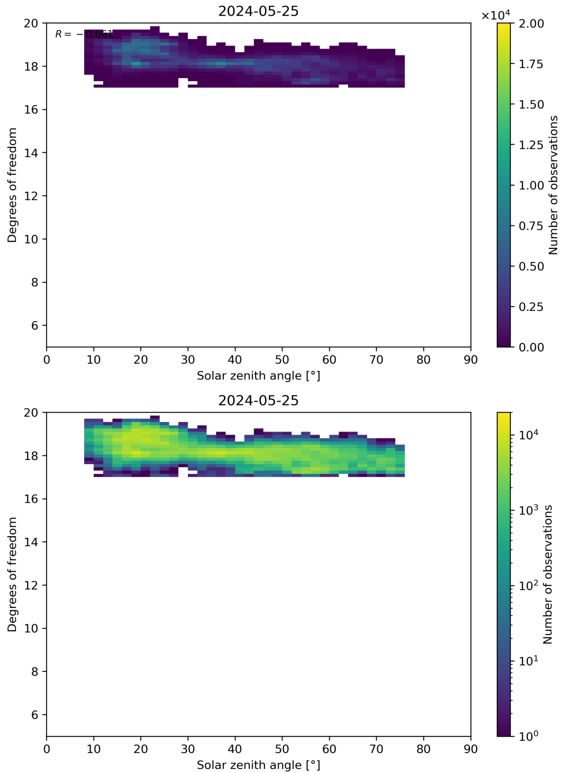
Figure 96: Scatter density plot of “Solar zenith angle” against “Degrees of freedom” for 2024-05-24 to 2024-05-26.
