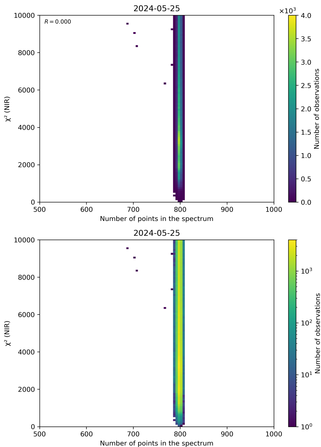
Figure 88: Scatter density plot of “Number of points in the spectrum” against “ \chi^2 (NIR)” for 2024-05-24 to 2024-05-26.
