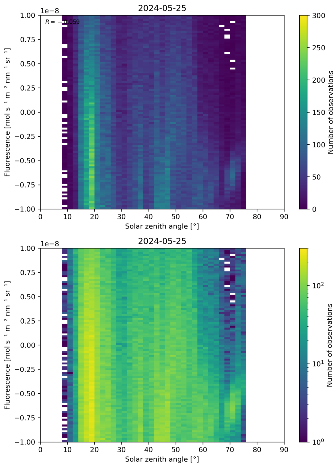
Figure 97: Scatter density plot of “Solar zenith angle” against “Fluorescence” for 2024-05-24 to 2024-05-26.
