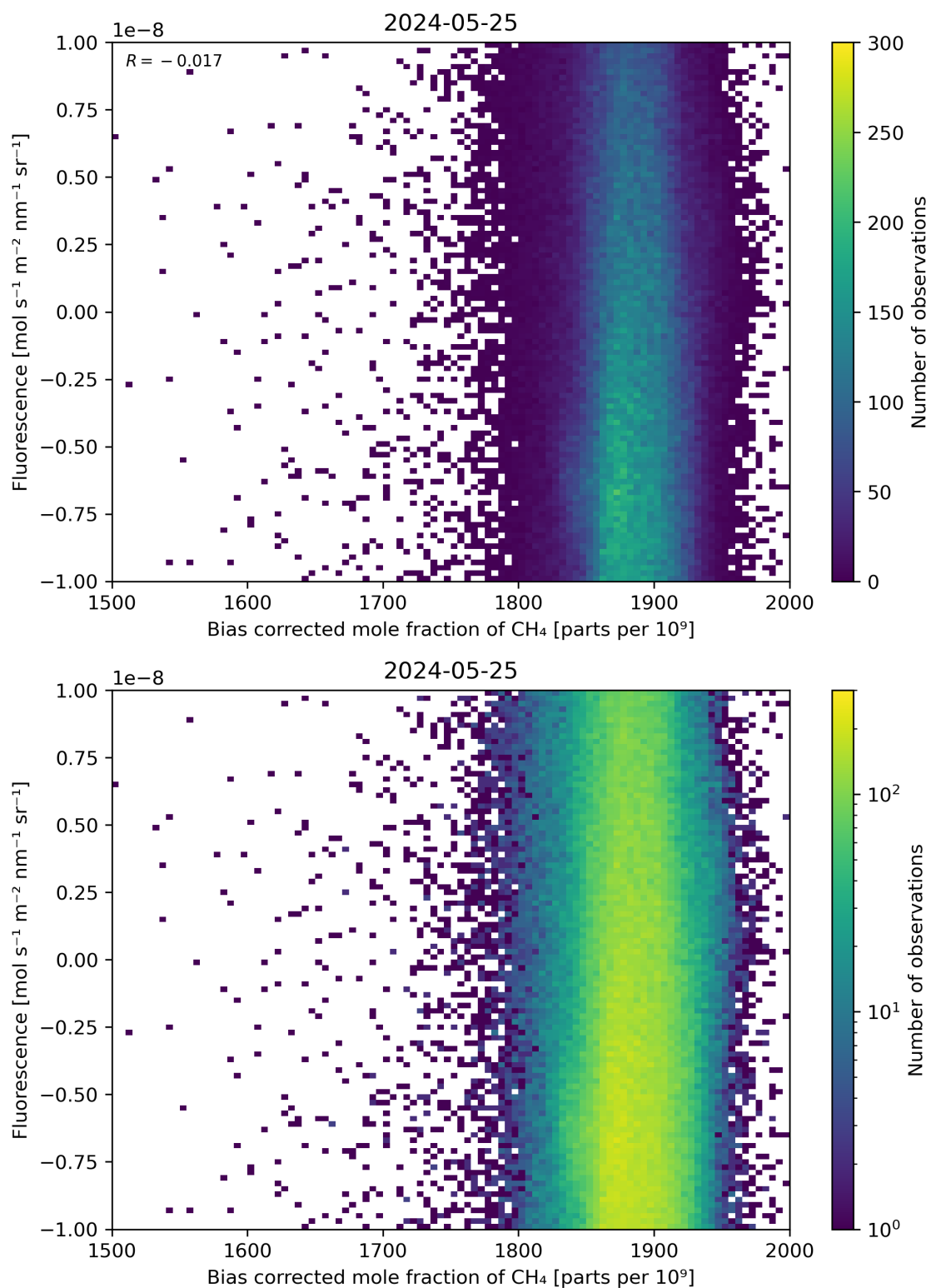
Figure 66: Scatter density plot of “Bias corrected mole fraction of \text{CH}_4 ” against “Fluorescence” for 2024-05-24 to 2024-05-26.
