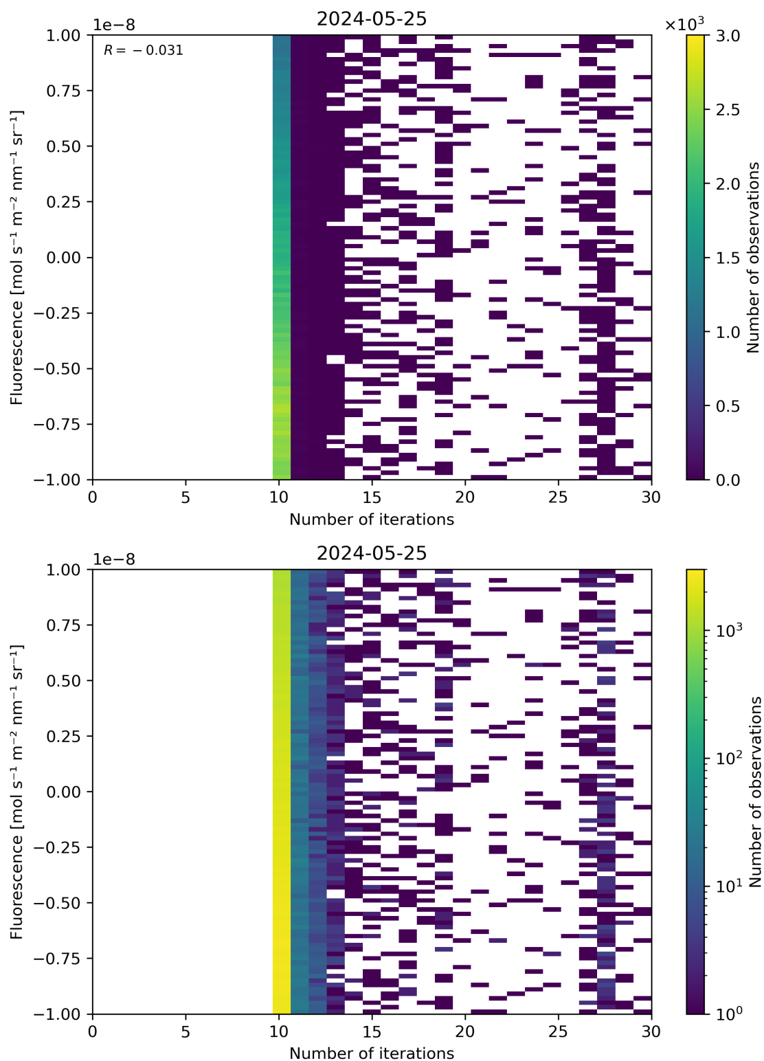
Figure 87: Scatter density plot of “Number of iterations” against “Fluorescence” for 2024-05-24 to 2024-05-26.
