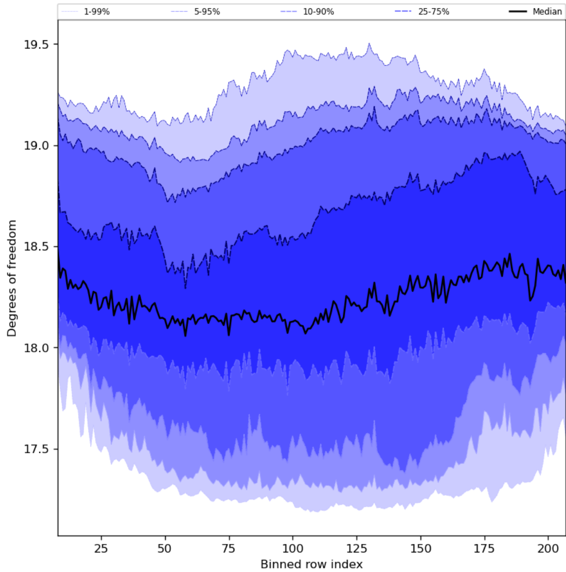
Figure 41: Along track statistics of “Degrees of freedom” for 2024-05-24 to 2024-05-26
