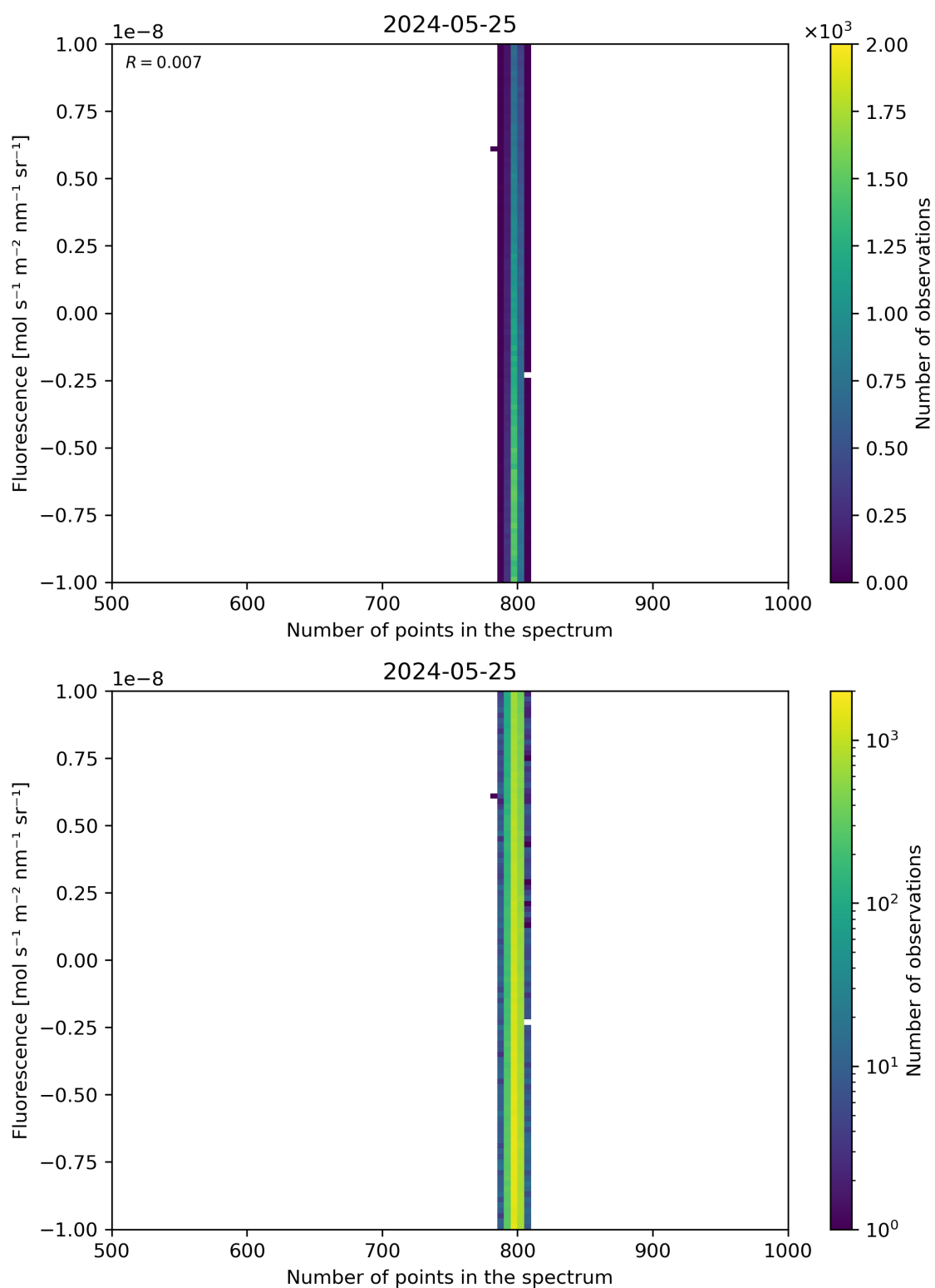
Figure 91: Scatter density plot of “Number of points in the spectrum” against “Fluorescence” for 2024-05-24 to 2024-05-26.
