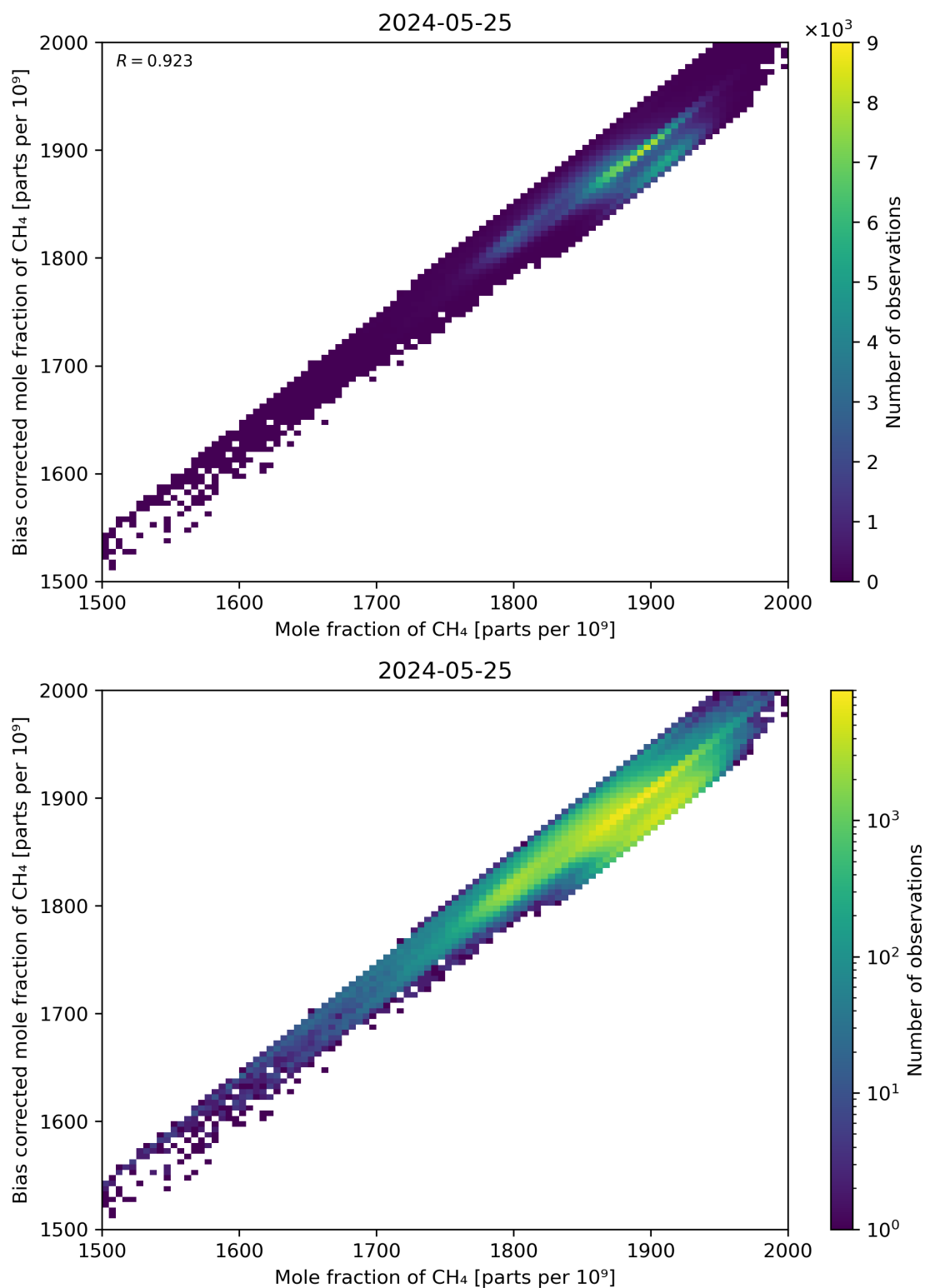
Figure 74: Scatter density plot of “Mole fraction of CH 4 ” against “Bias corrected mole fraction of CH 4 ” for 2024-05-24 to 2024-05-26.
