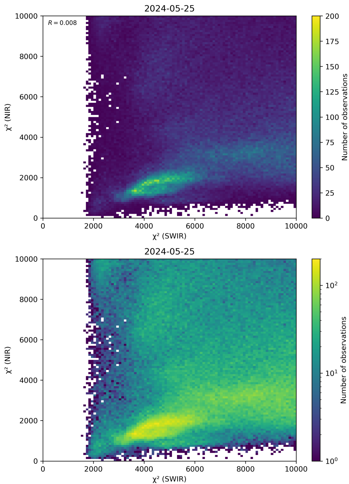
Figure 47: Scatter density plot of “ \chi^2 (SWIR)” against “ \chi^2 (NIR)” for 2024-05-24 to 2024-05-26.
