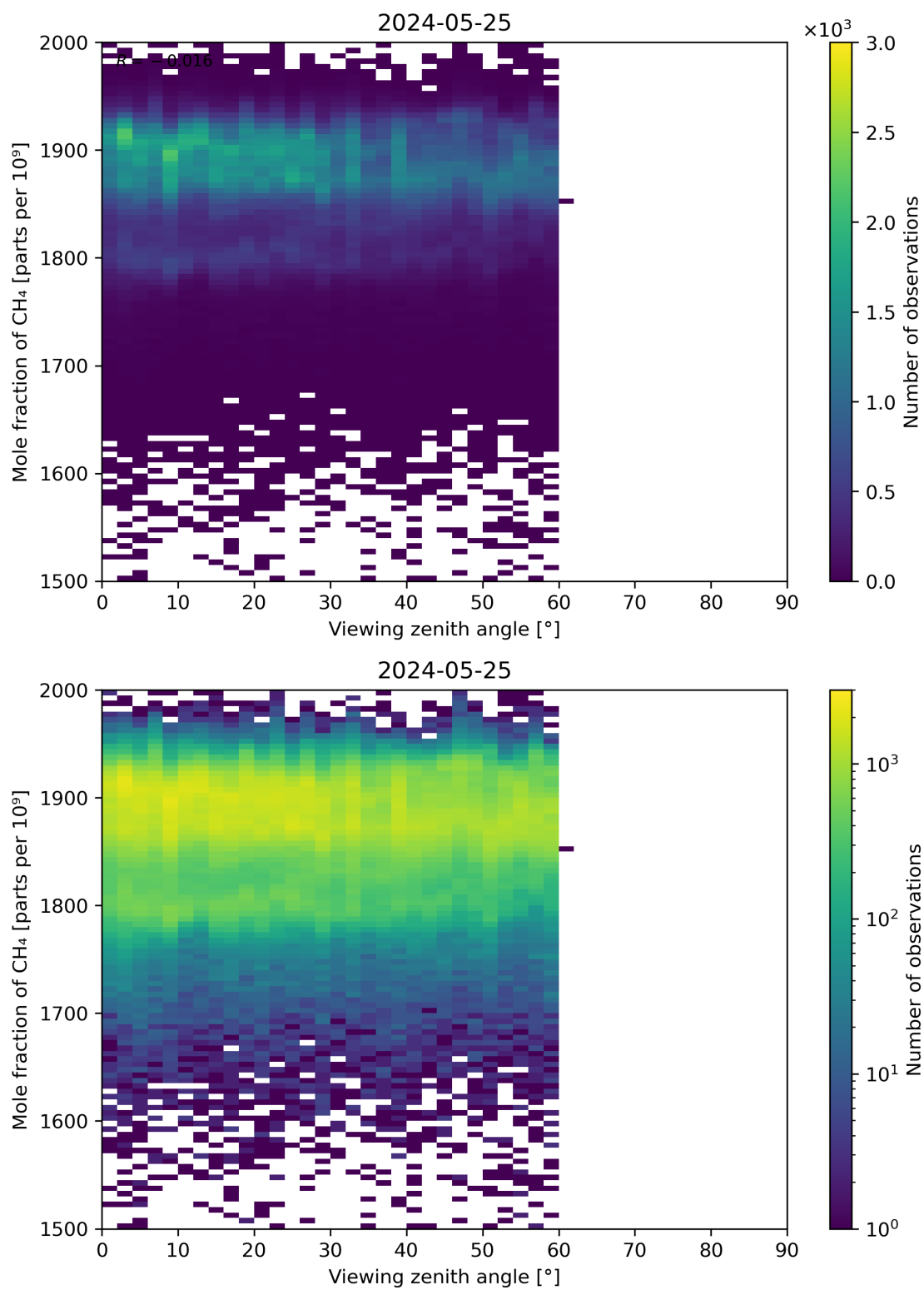
Figure 110: Scatter density plot of “Viewing zenith angle” against “Mole fraction of CH 4 ” for 2024-05-24 to 2024-05-26.
