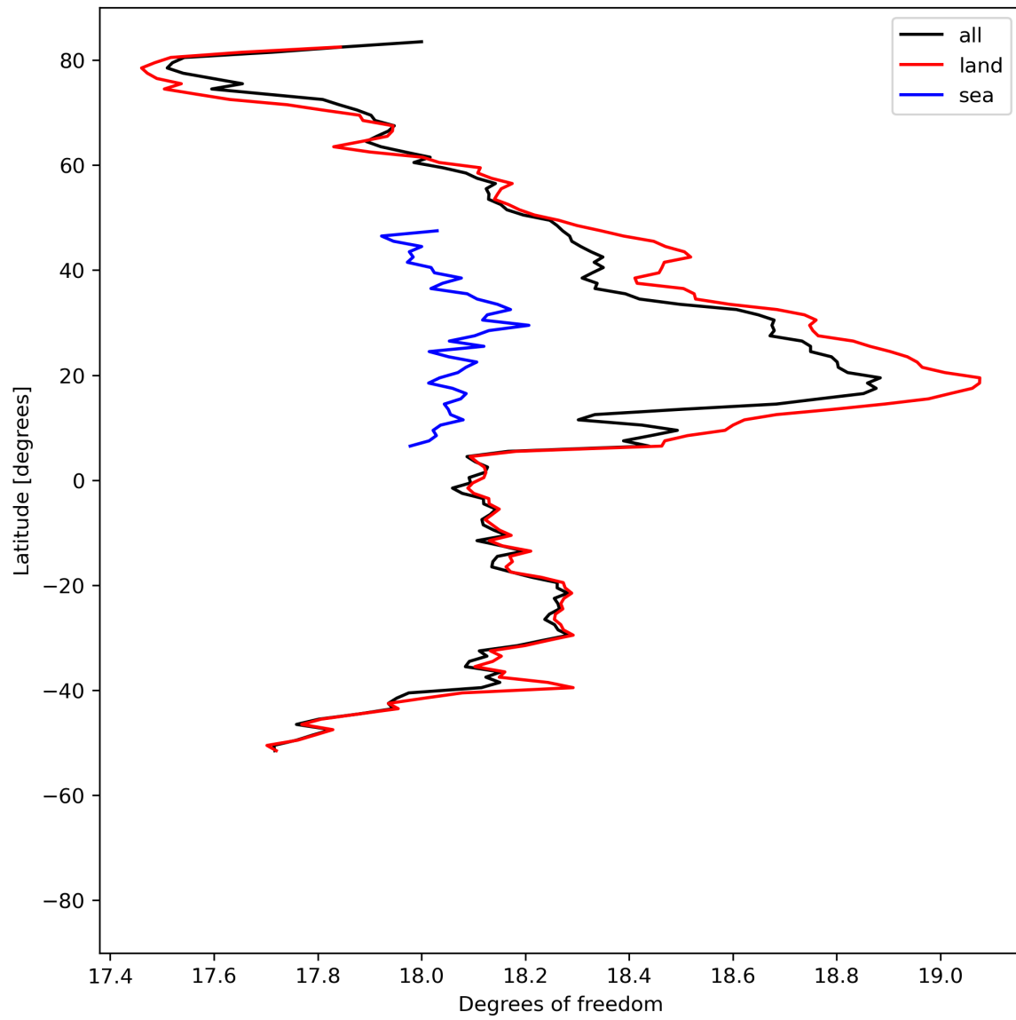
Figure 19: Zonal average of “Degrees of freedom” for 2024-05-24 to 2024-05-26.
