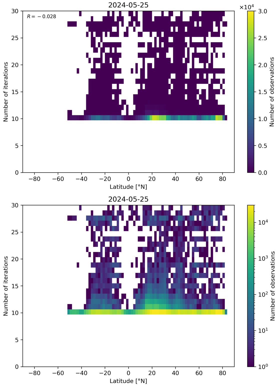
Figure 60: Scatter density plot of “Latitude” against “Number of iterations” for 2024-05-24 to 2024-05-26.
