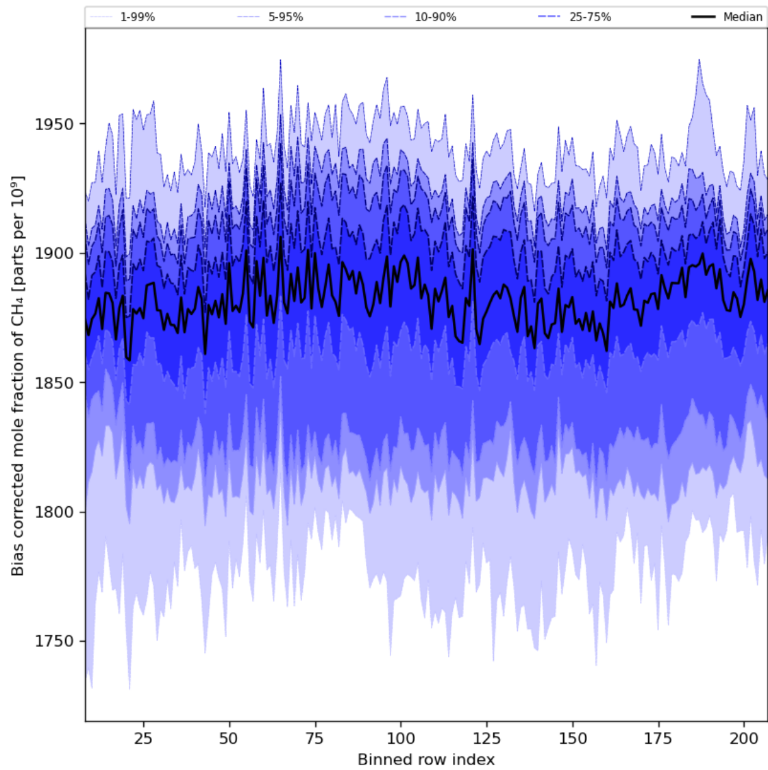
Figure 36: Along track statistics of “Bias corrected mole fraction of CH 4 ” for 2024-05-24 to 2024-05-26
