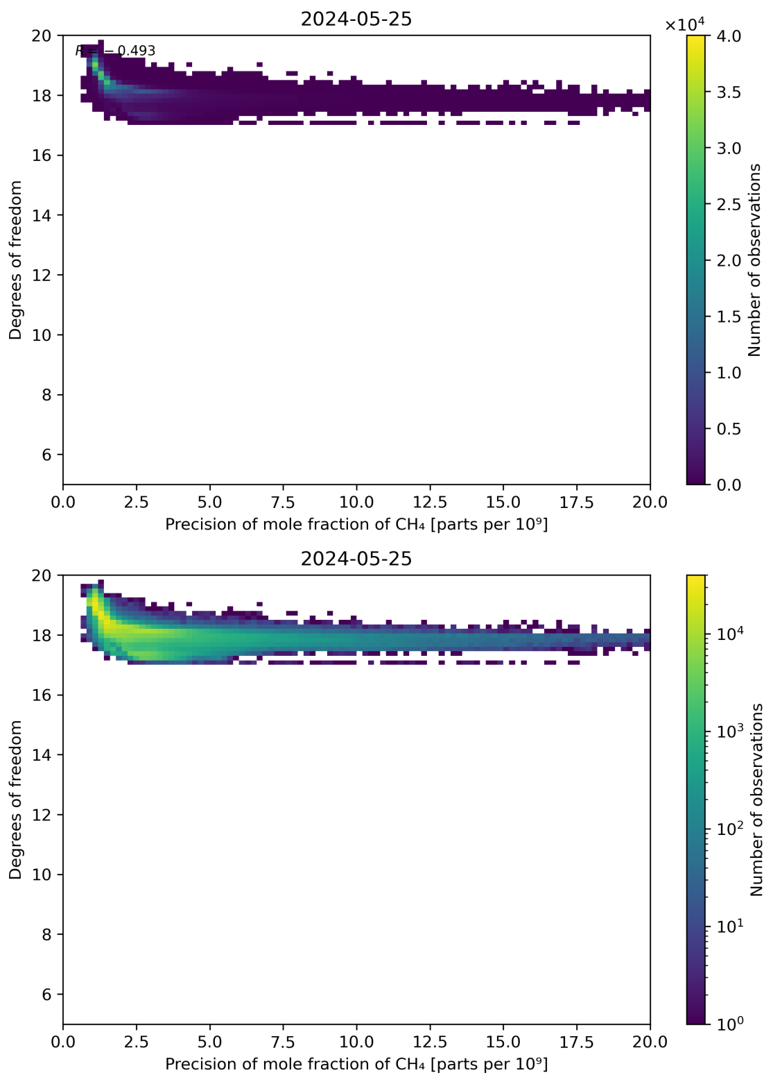
Figure 80: Scatter density plot of “Precision of mole fraction of CH 4 ” against “Degrees of freedom” for 2024-05-24 to 2024-05-26.
