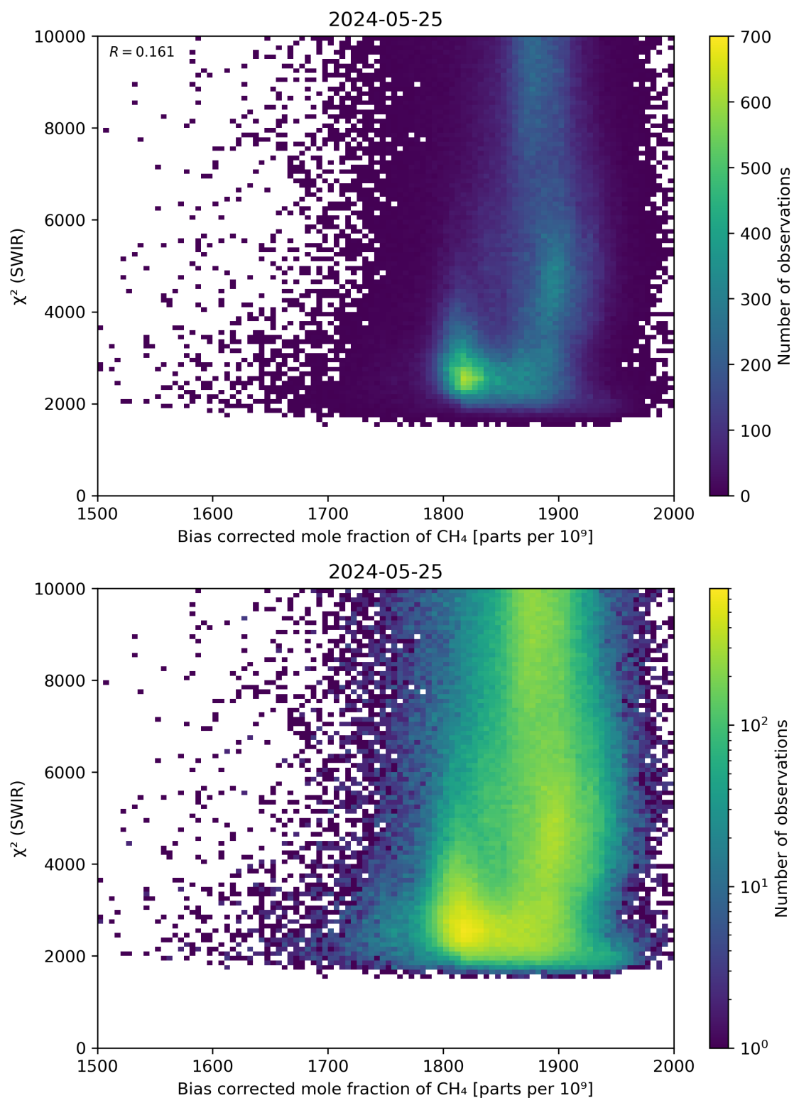
Figure 64: Scatter density plot of “Bias corrected mole fraction of \text{CH}_4 ” against “ \chi^2 (SWIR)” for 2024-05-24 to 2024-05-26.
