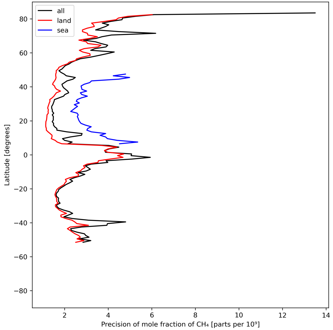
Figure 13: Zonal average of “Precision of mole fraction of CH 4 ” for 2024-05-24 to 2024-05-26.
