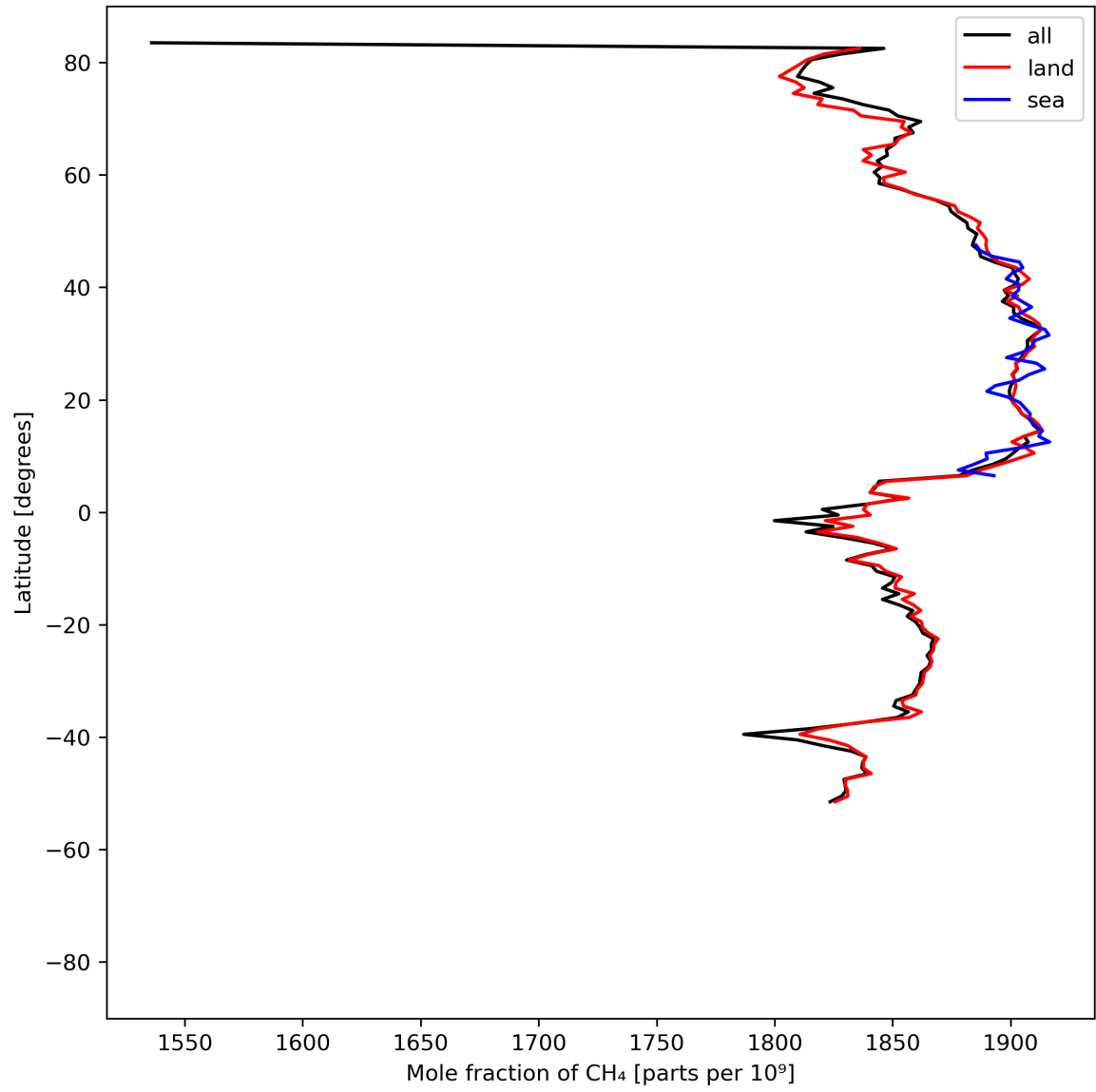
Figure 12: Zonal average of “Mole fraction of \text{CH}_4 ” for 2024-05-24 to 2024-05-26.
