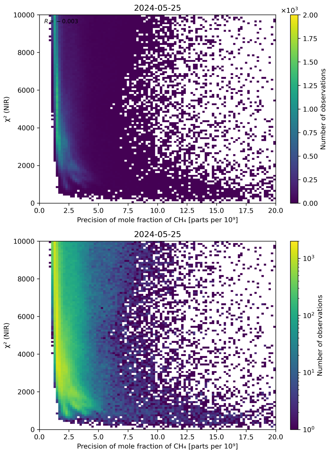
Figure 78: Scatter density plot of “Precision of mole fraction of CH 4 ” against “ \chi^2 (NIR)” for 2024-05-24 to 2024-05-26.
