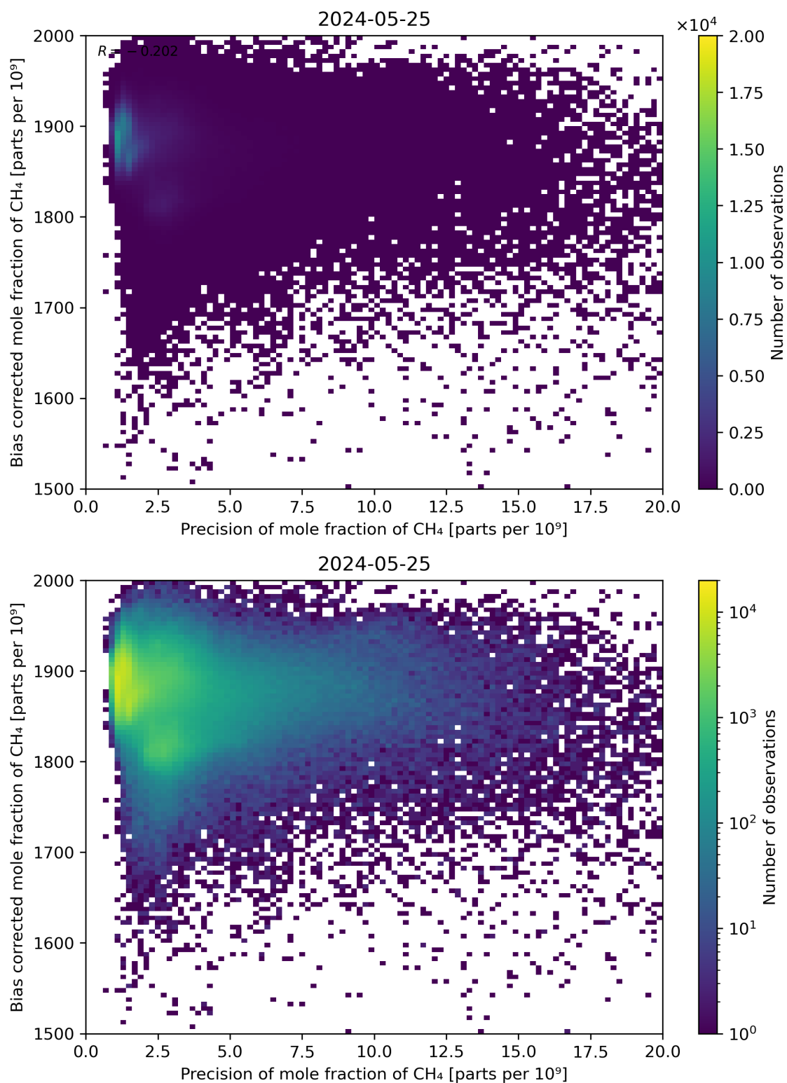
Figure 82: Scatter density plot of “Precision of mole fraction of CH 4 ” against “Bias corrected mole fraction of CH 4 ” for 2024-05-24 to 2024-05-26.
