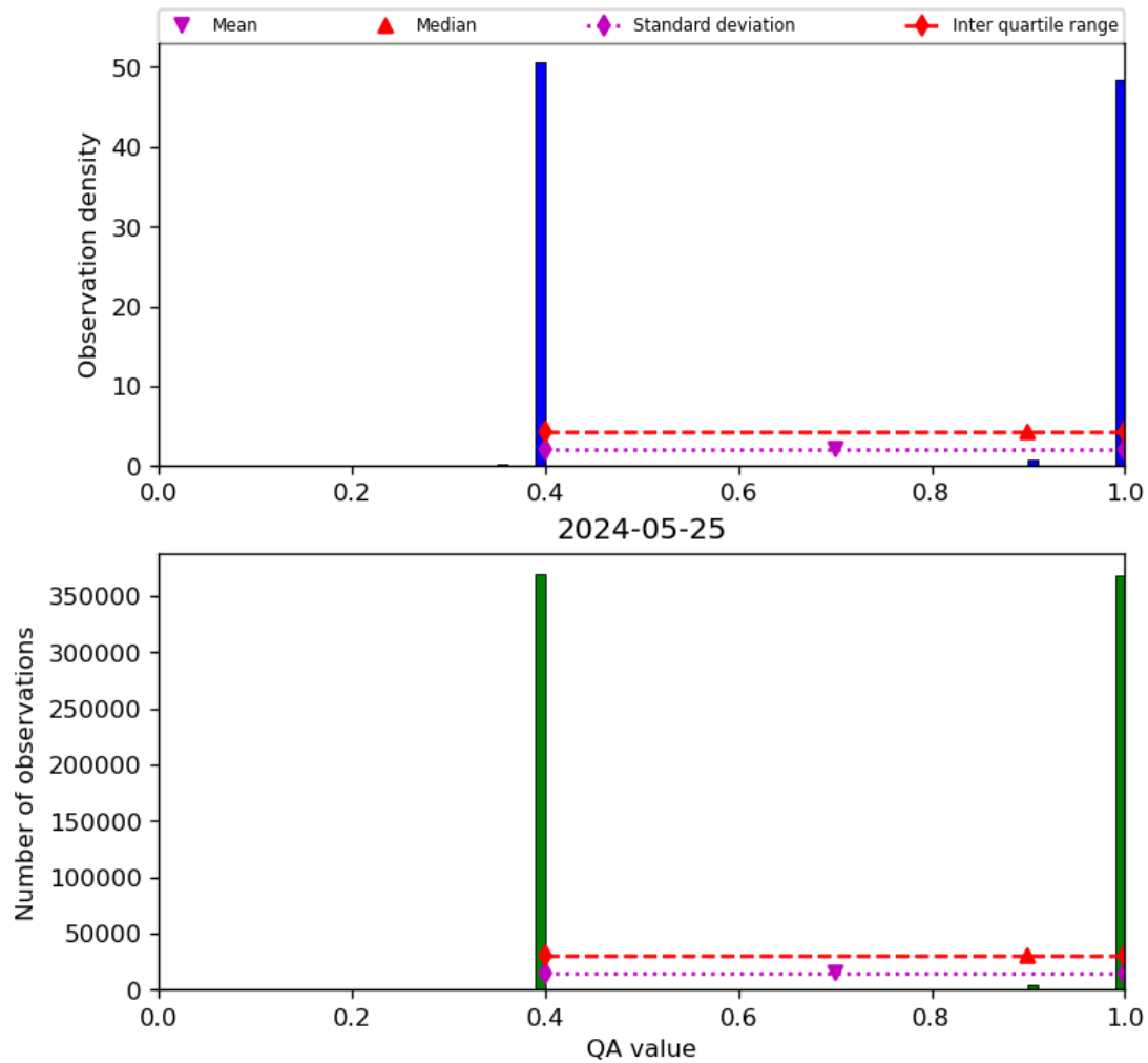
Figure 22: Histogram of "QA value" for 2024-05-24 to 2024-05-26
