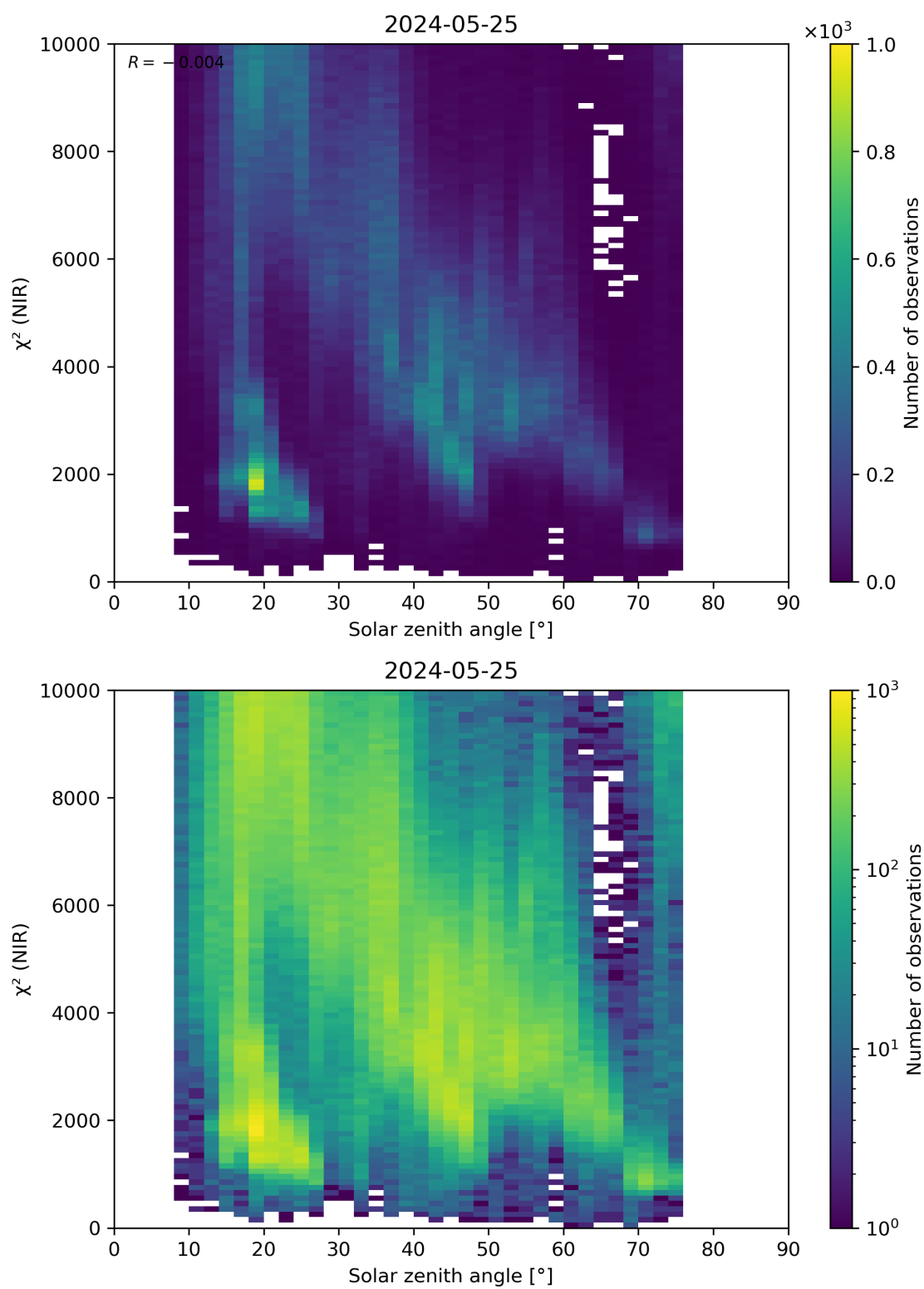
Figure 94: Scatter density plot of “Solar zenith angle” against “ \chi^2 (NIR)” for 2024-05-24 to 2024-05-26.
