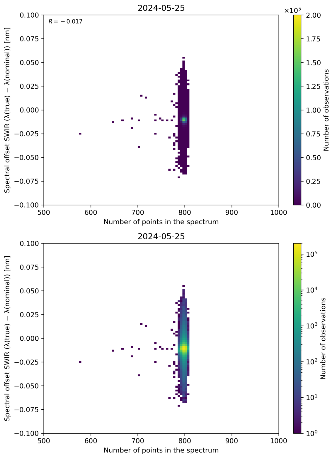
Figure 93: Scatter density plot of “Number of points in the spectrum” against “Spectral offset SWIR ( \lambda(\text{true}) - \lambda(\text{nominal}) )” for 2024-05-24 to 2024-05-26.
