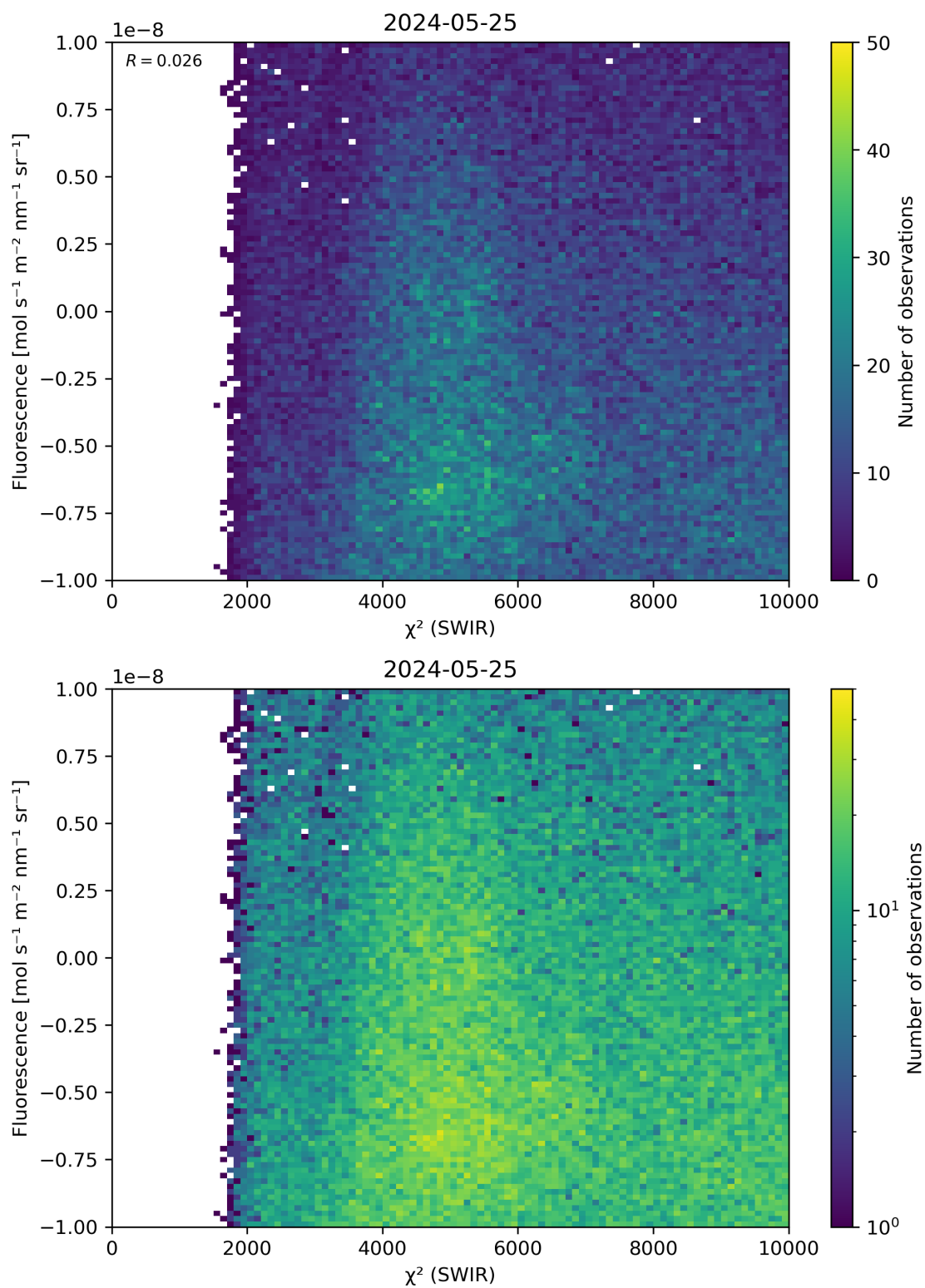
Figure 49: Scatter density plot of “ \chi^2 (SWIR)” against “Fluorescence” for 2024-05-24 to 2024-05-26.
