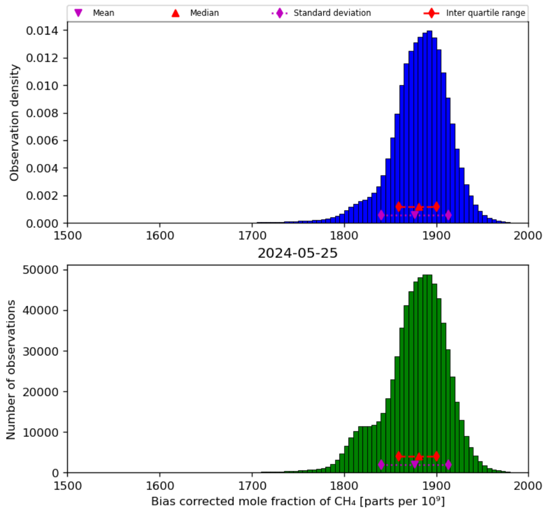
Figure 25: Histogram of “Bias corrected mole fraction of CH 4 ” for 2024-05-24 to 2024-05-26
