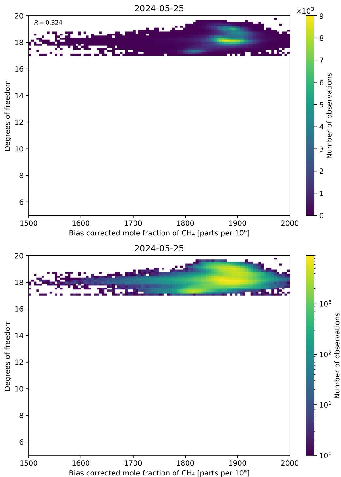
Figure 65: Scatter density plot of “Bias corrected mole fraction of CH 4 ” against “Degrees of freedom” for 2024-05-24 to 2024-05-26.
