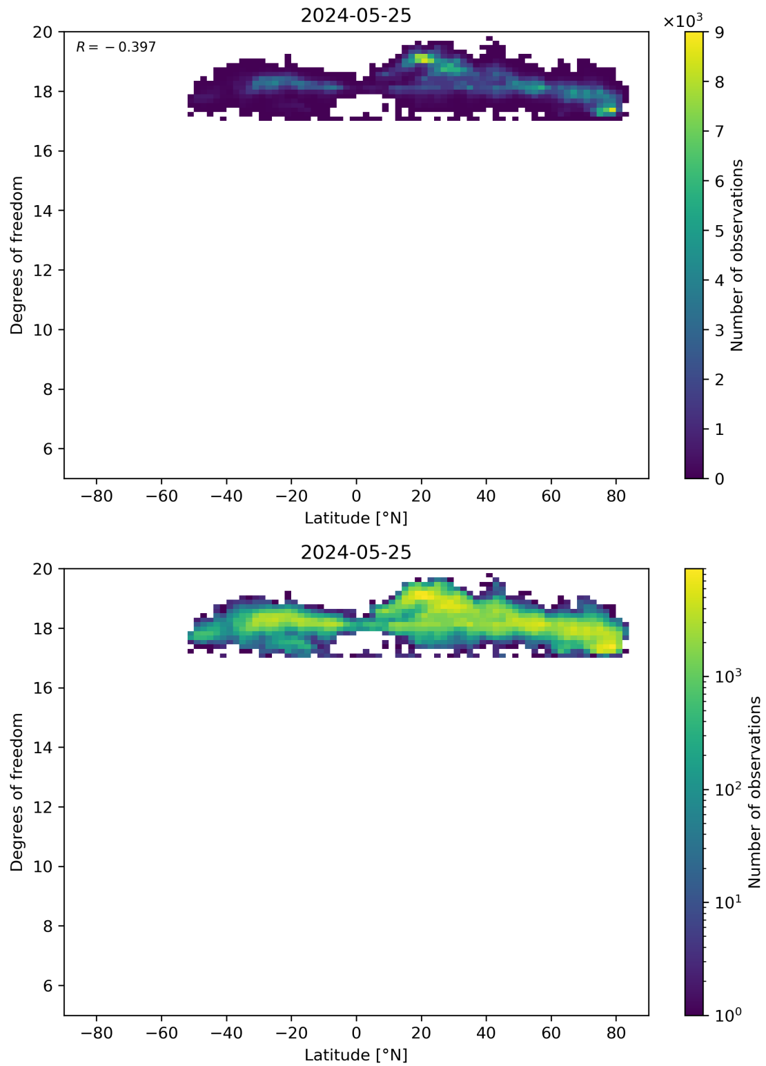
Figure 55: Scatter density plot of “Latitude” against “Degrees of freedom” for 2024-05-24 to 2024-05-26.
