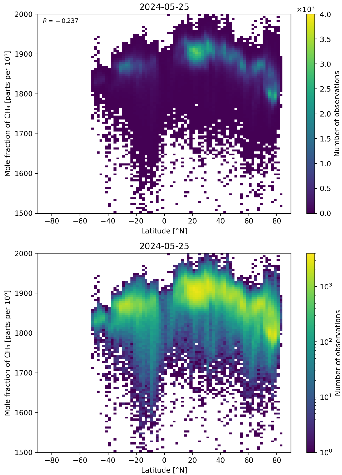
Figure 57: Scatter density plot of “Latitude” against “Mole fraction of CH 4 ” for 2024-05-24 to 2024-05-26.
