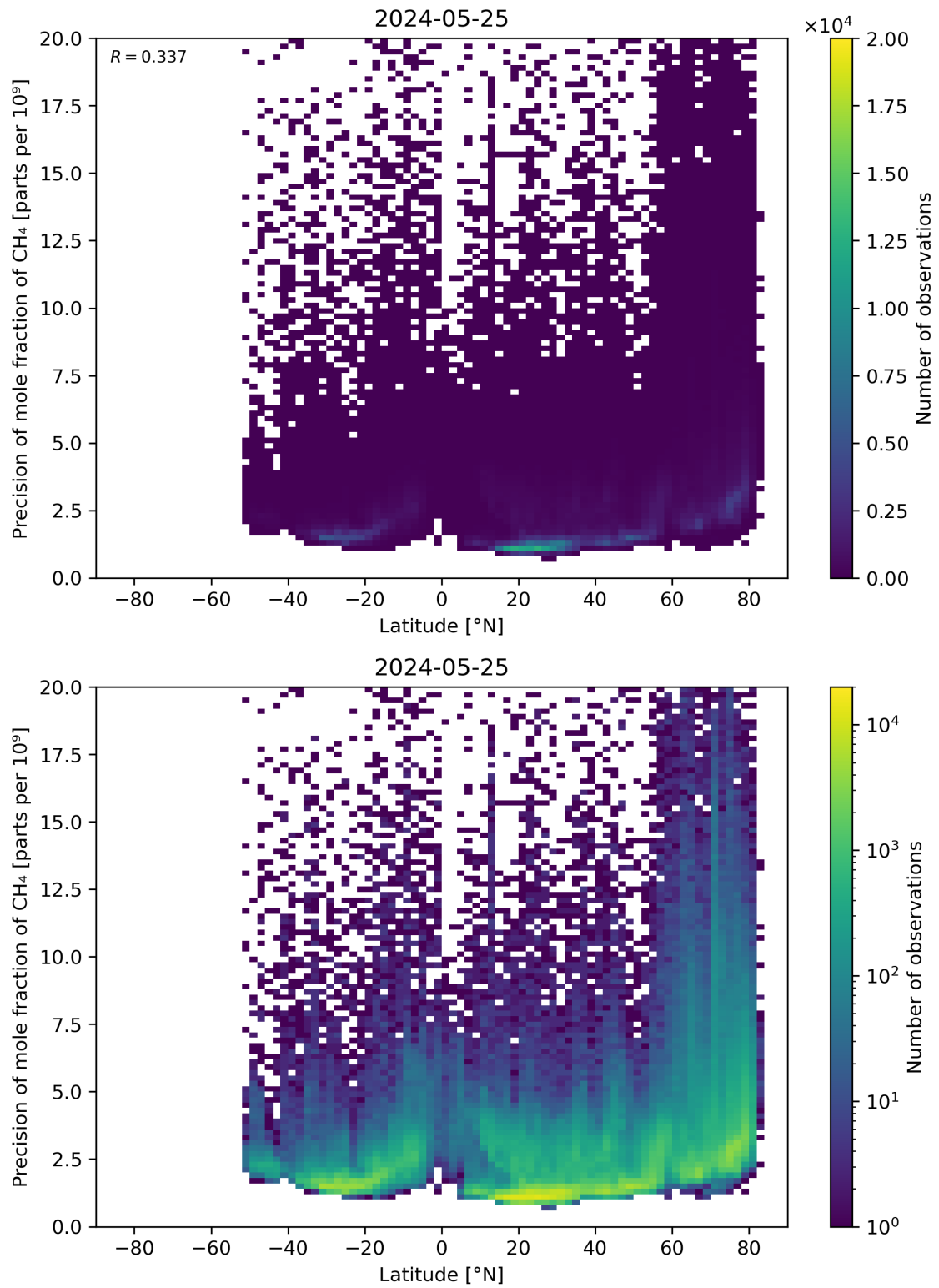
Figure 59: Scatter density plot of “Latitude” against “Precision of mole fraction of \text{CH}_4 ” for 2024-05-24 to 2024-05-26.
