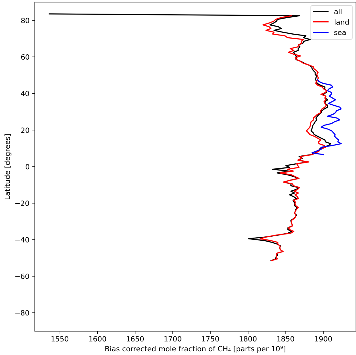
Figure 14: Zonal average of “Bias corrected mole fraction of \text{CH}_4 ” for 2024-05-24 to 2024-05-26.
