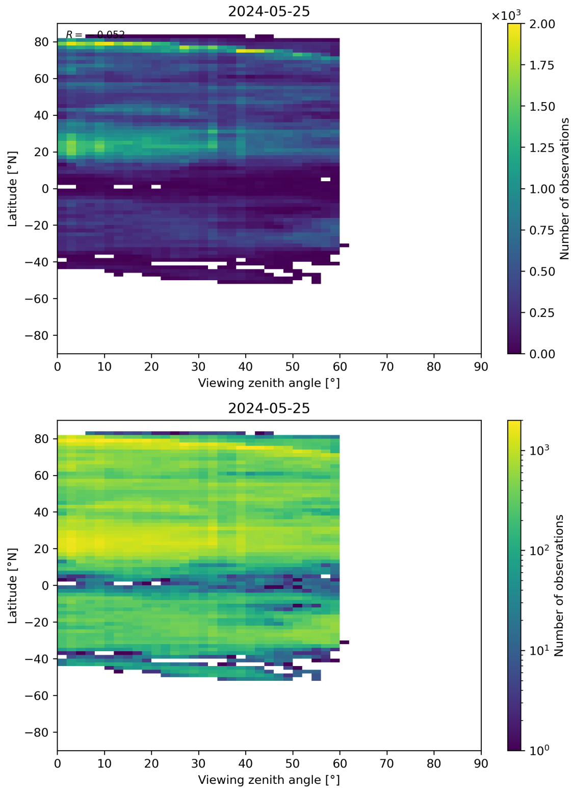
Figure 109: Scatter density plot of “Viewing zenith angle” against “Latitude” for 2024-05-24 to 2024-05-26.
