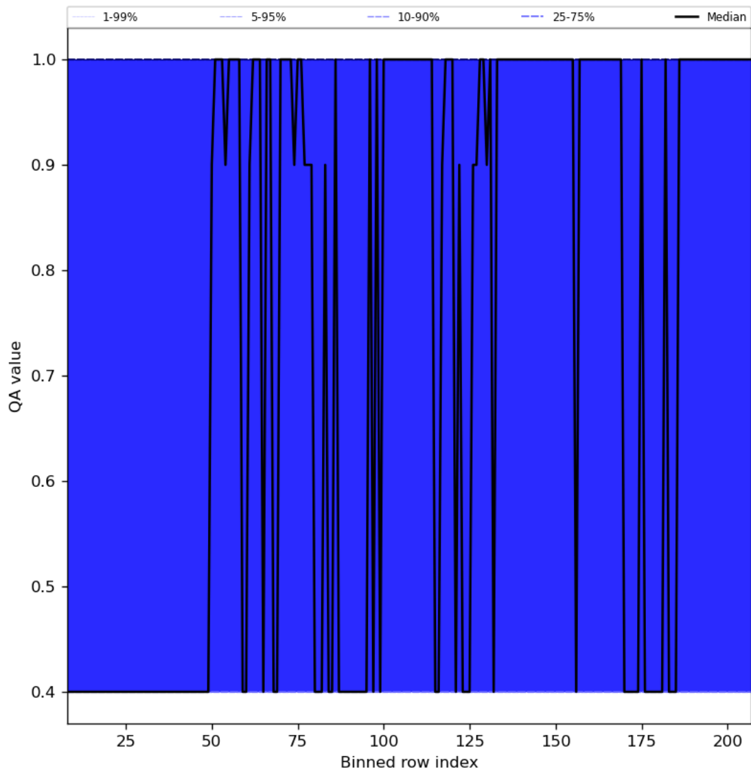
Figure 33: Along track statistics of “QA value” for 2024-05-24 to 2024-05-26
