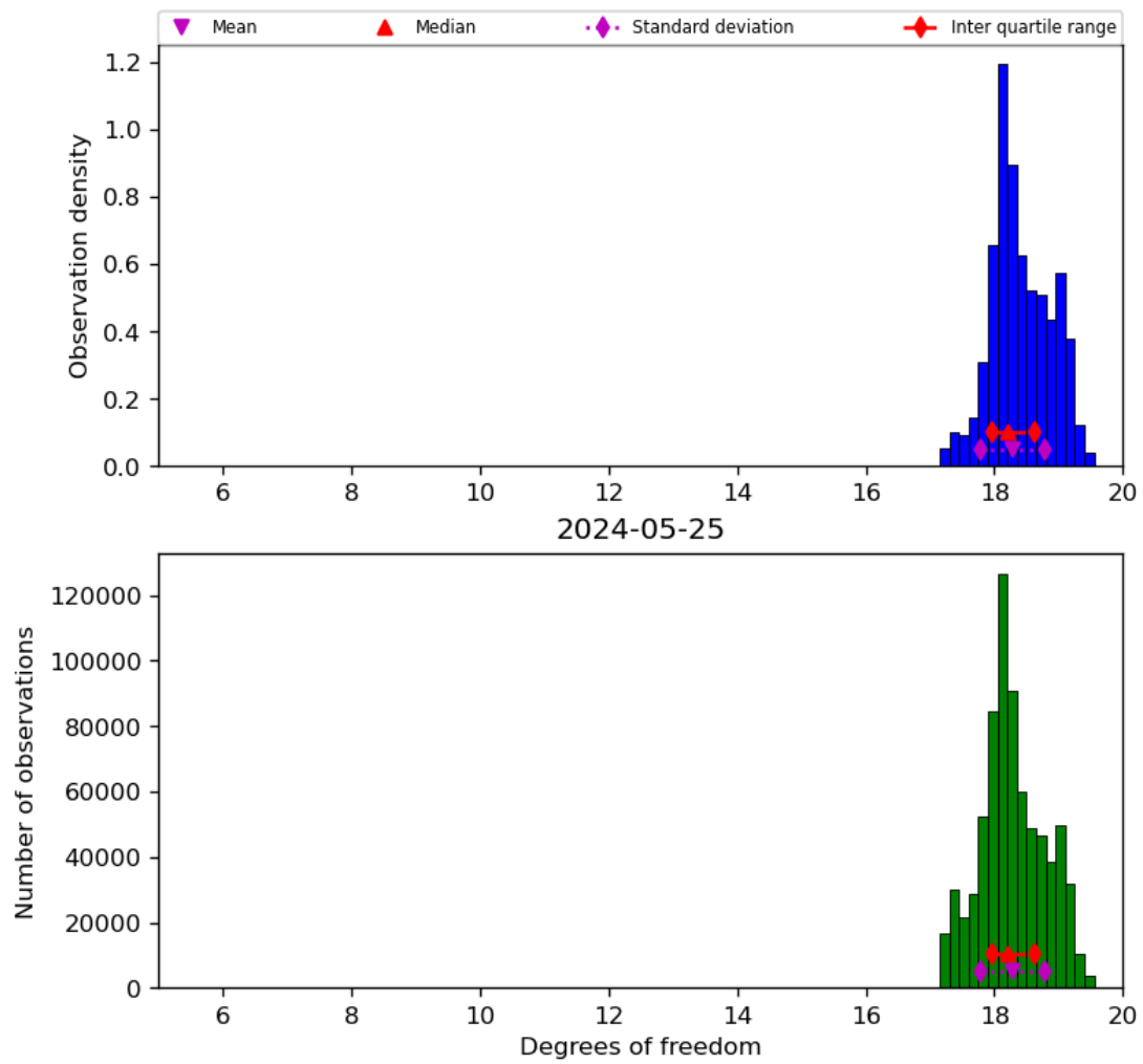
Figure 30: Histogram of “Degrees of freedom” for 2024-05-24 to 2024-05-26
