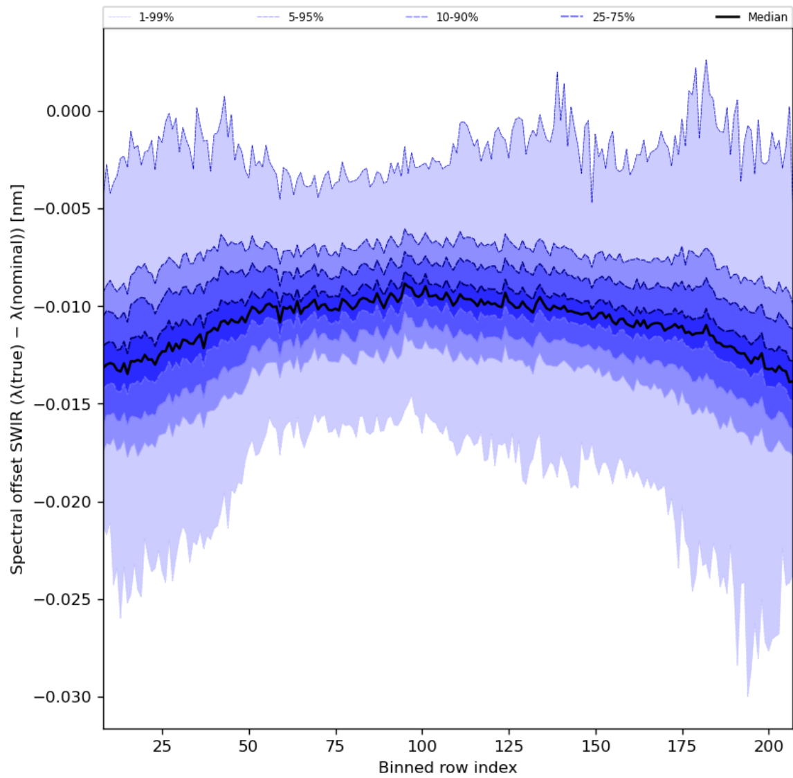
Figure 38: Along track statistics of “Spectral offset SWIR ( \lambda(\text{true}) - \lambda(\text{nominal}) )” for 2024-05-24 to 2024-05-26
