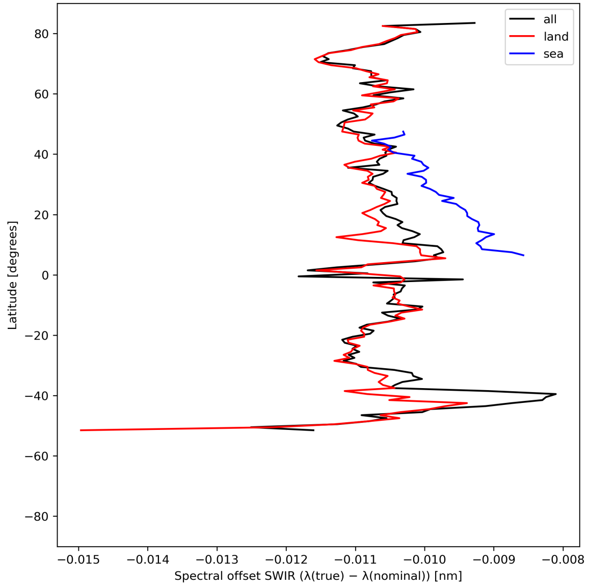
Figure 16: Zonal average of “Spectral offset SWIR ( \lambda(\text{true}) - \lambda(\text{nominal}) )” for 2024-05-24 to 2024-05-26.
