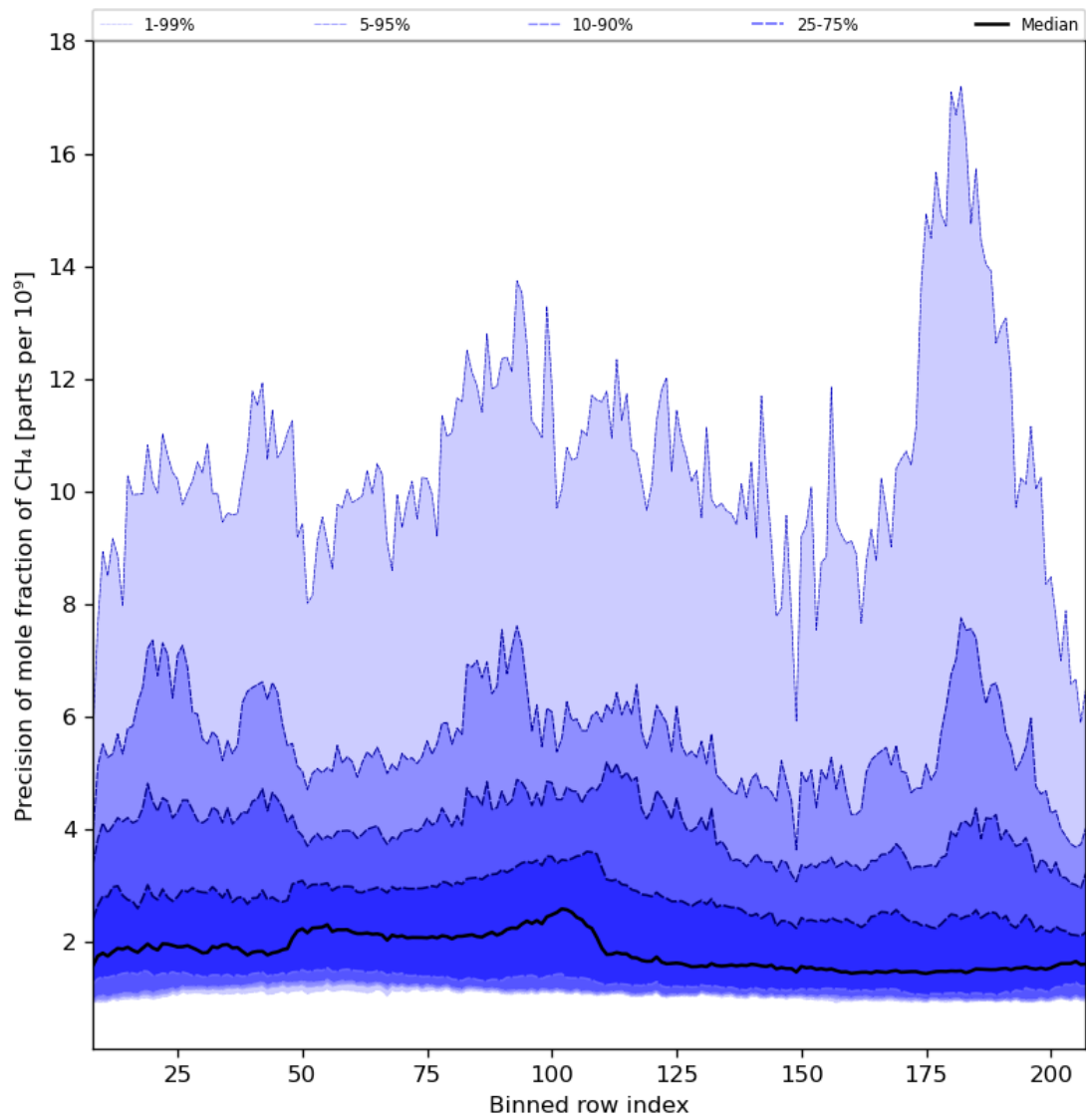
Figure 35: Along track statistics of “Precision of mole fraction of CH 4 ” for 2024-05-24 to 2024-05-26
