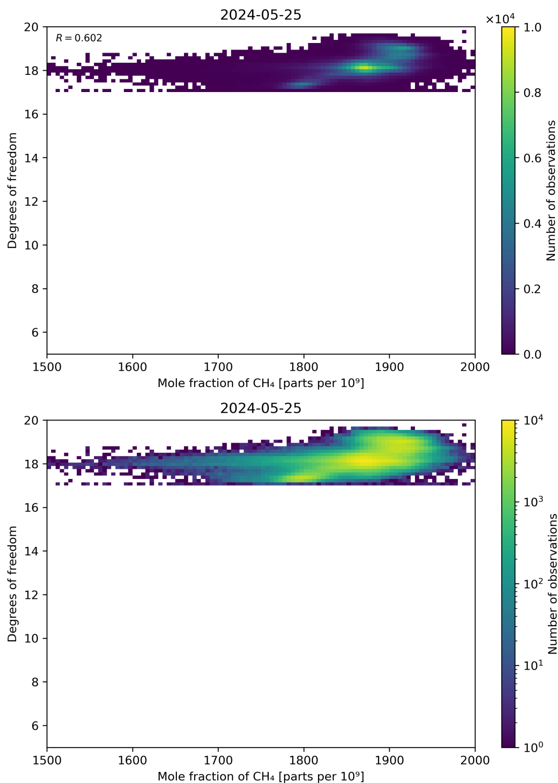
Figure 72: Scatter density plot of “Mole fraction of CH 4 ” against “Degrees of freedom” for 2024-05-24 to 2024-05-26.
