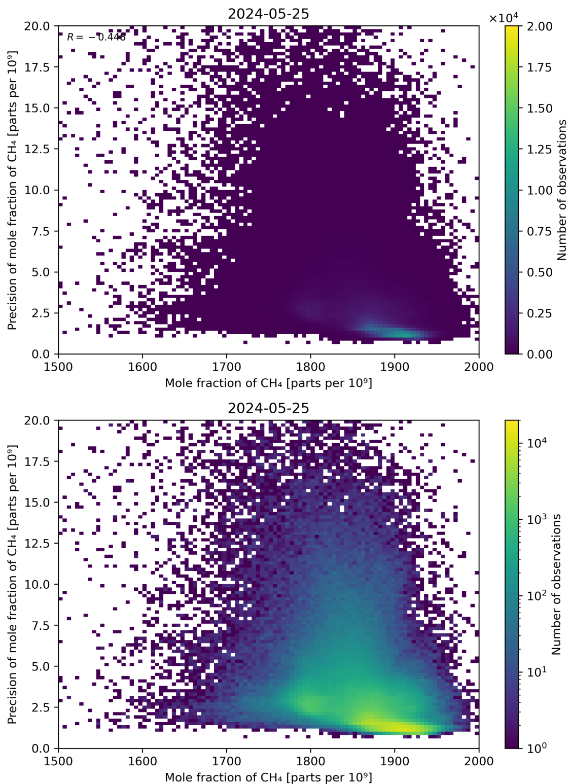
Figure 75: Scatter density plot of “Mole fraction of CH 4 ” against “Precision of mole fraction of CH 4 ” for 2024-05-24 to 2024-05-26.
