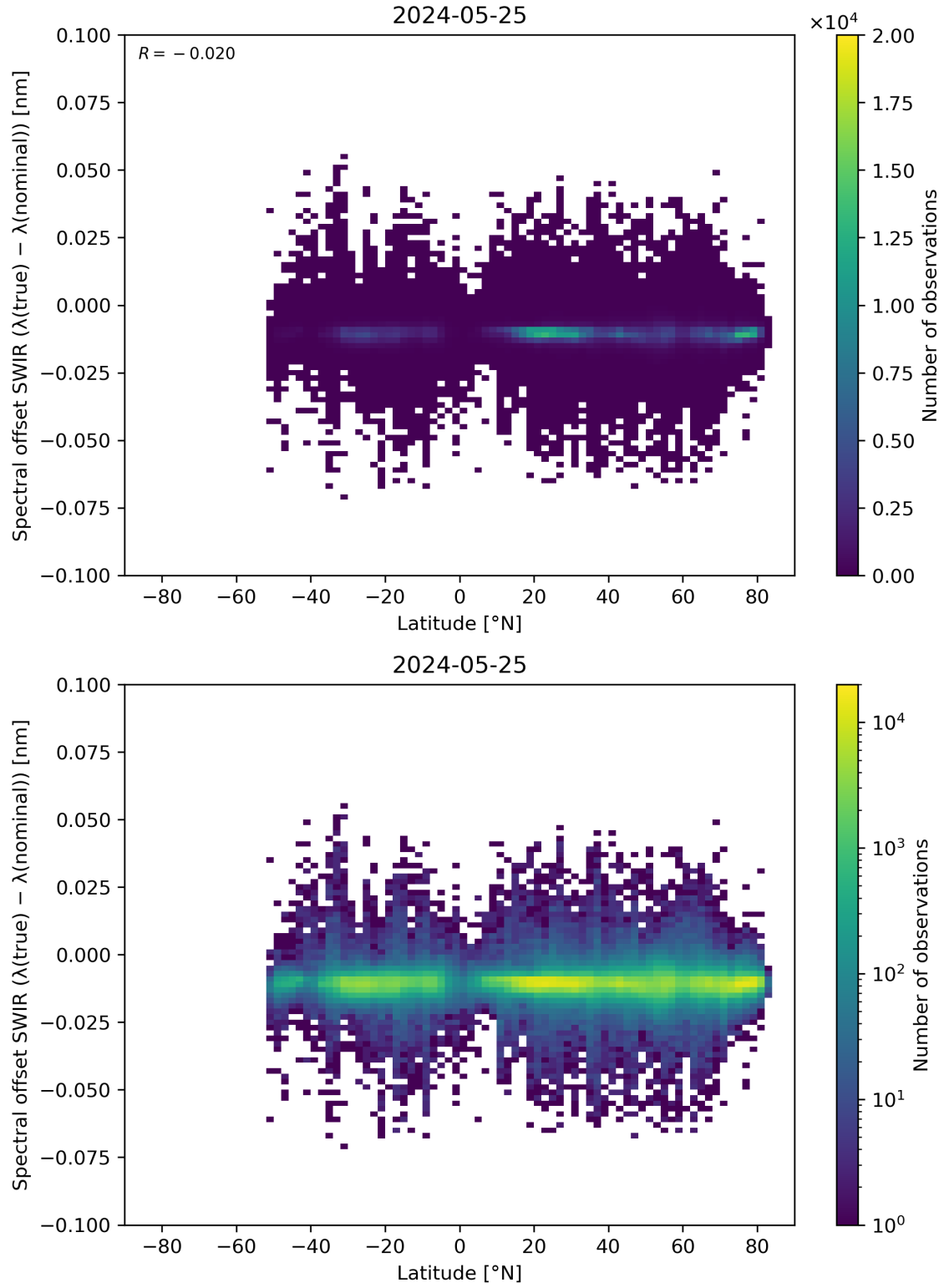
Figure 62: Scatter density plot of “Latitude” against “Spectral offset SWIR ( \lambda(\text{true}) - \lambda(\text{nominal}) )” for 2024-05-24 to 2024-05-26.
