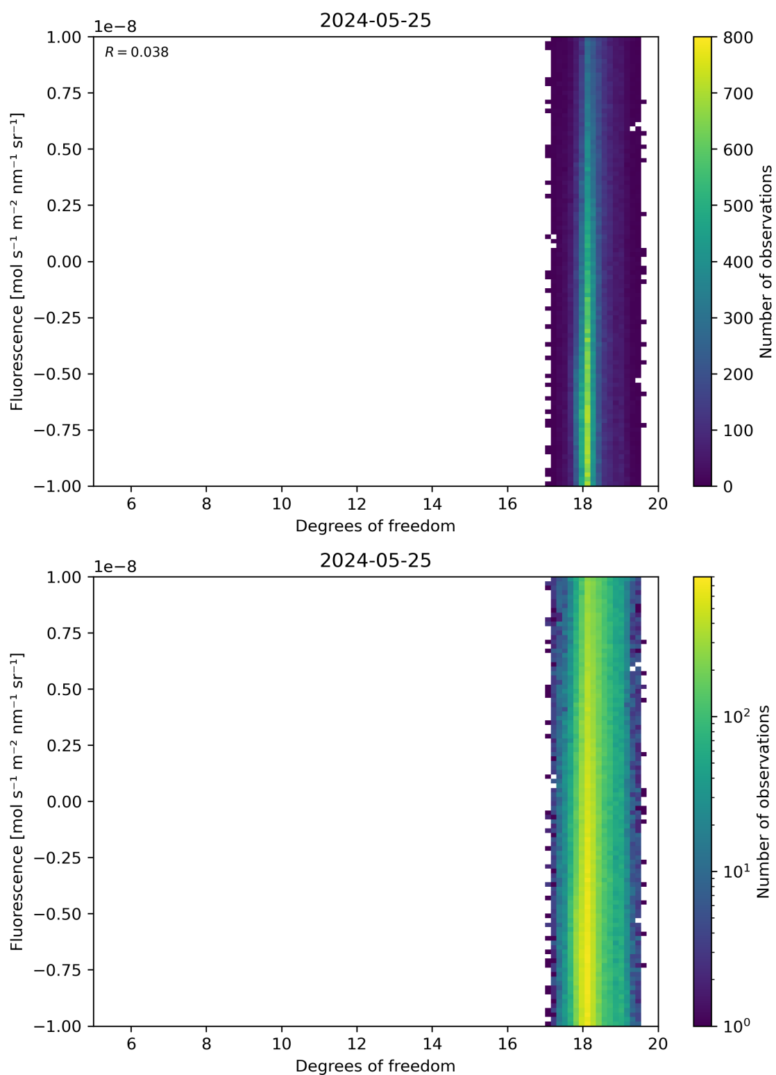
Figure 51: Scatter density plot of “Degrees of freedom” against “Fluorescence” for 2024-05-24 to 2024-05-26.
