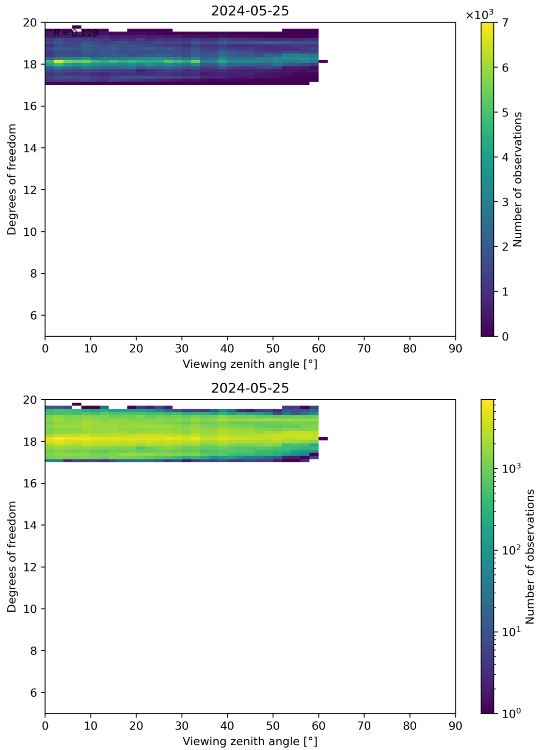
Figure 107: Scatter density plot of “Viewing zenith angle” against “Degrees of freedom” for 2024-05-24 to 2024-05-26.
