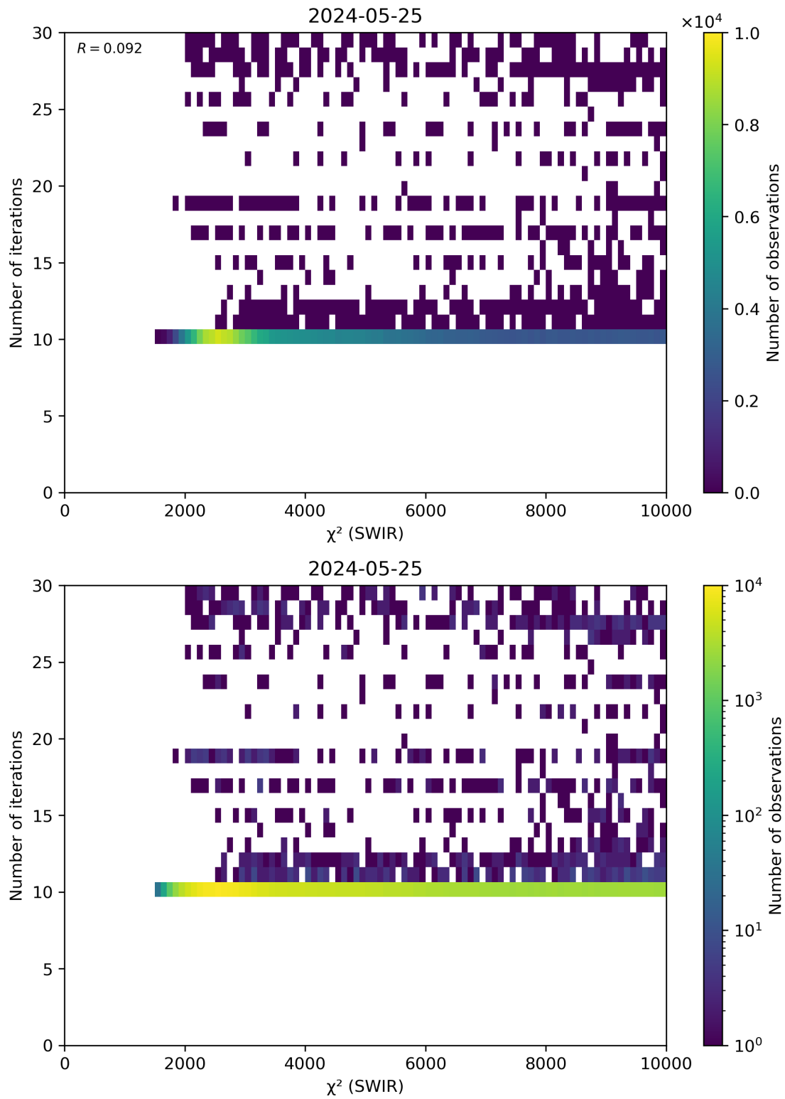
Figure 50: Scatter density plot of “ \chi^2 (SWIR)” against “Number of iterations” for 2024-05-24 to 2024-05-26.
