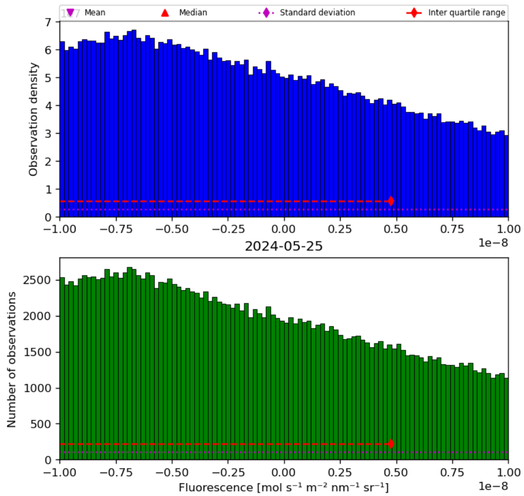
Figure 32: Histogram of “Fluorescence” for 2024-05-24 to 2024-05-26
