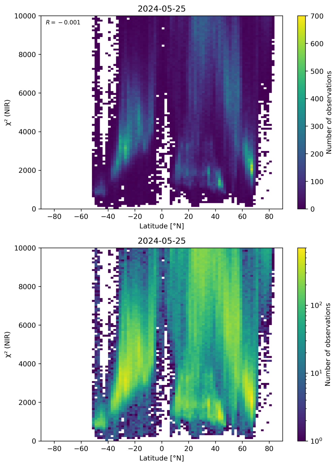
Figure 53: Scatter density plot of “Latitude” against “ \chi^2 (NIR)” for 2024-05-24 to 2024-05-26.
