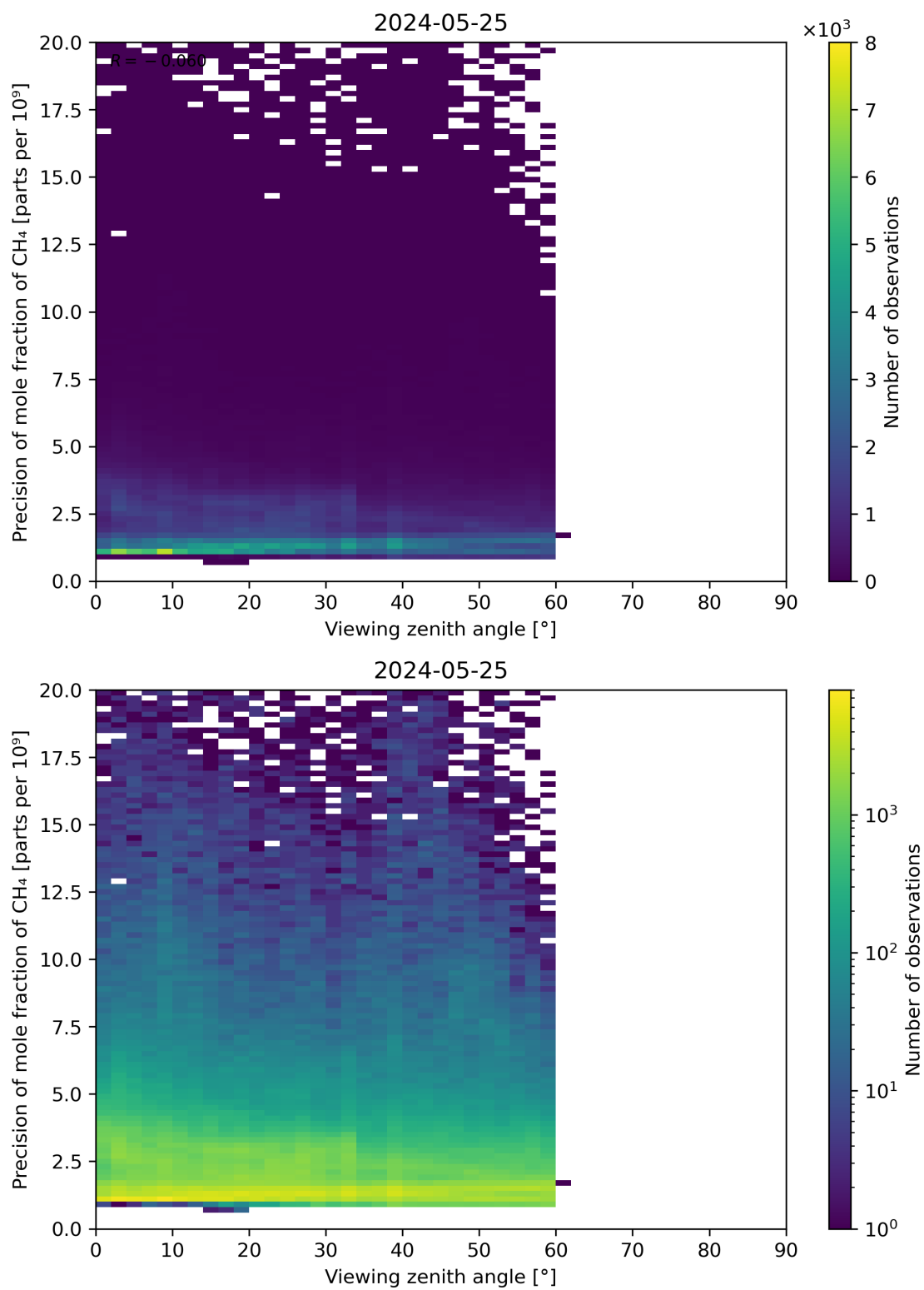
Figure 112: Scatter density plot of “Viewing zenith angle” against “Precision of mole fraction of CH 4 ” for 2024-05-24 to 2024-05-26.
