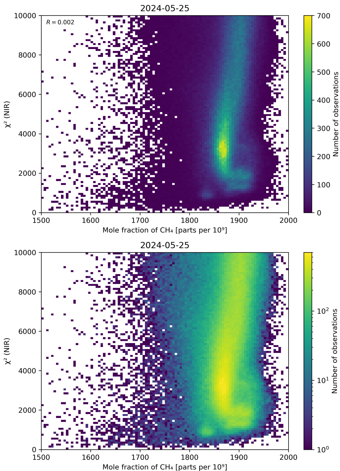
Figure 70: Scatter density plot of “Mole fraction of CH 4 ” against “ \chi^2 (NIR)” for 2024-05-24 to 2024-05-26.
