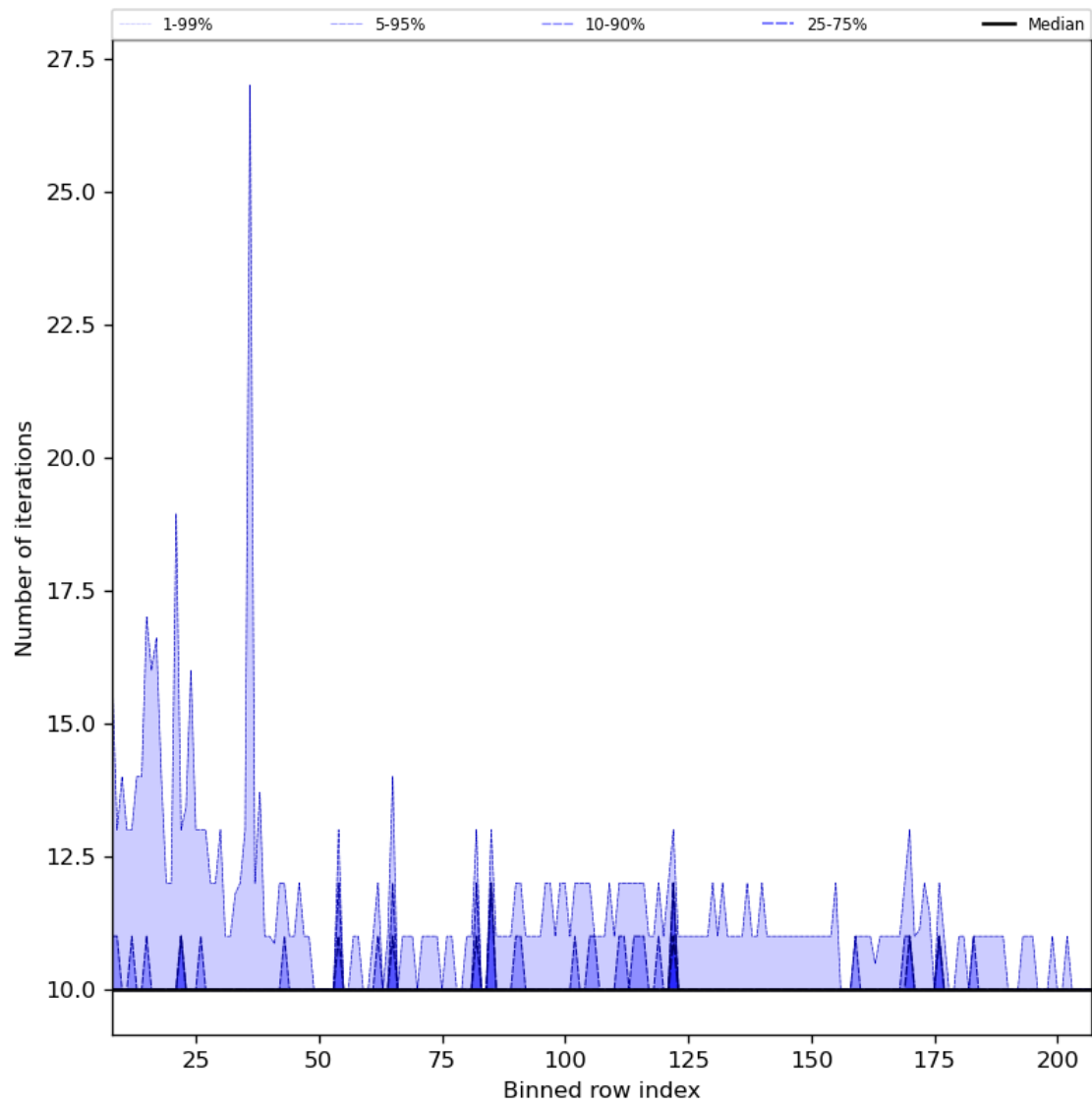
Figure 42: Along track statistics of “Number of iterations” for 2024-05-24 to 2024-05-26
