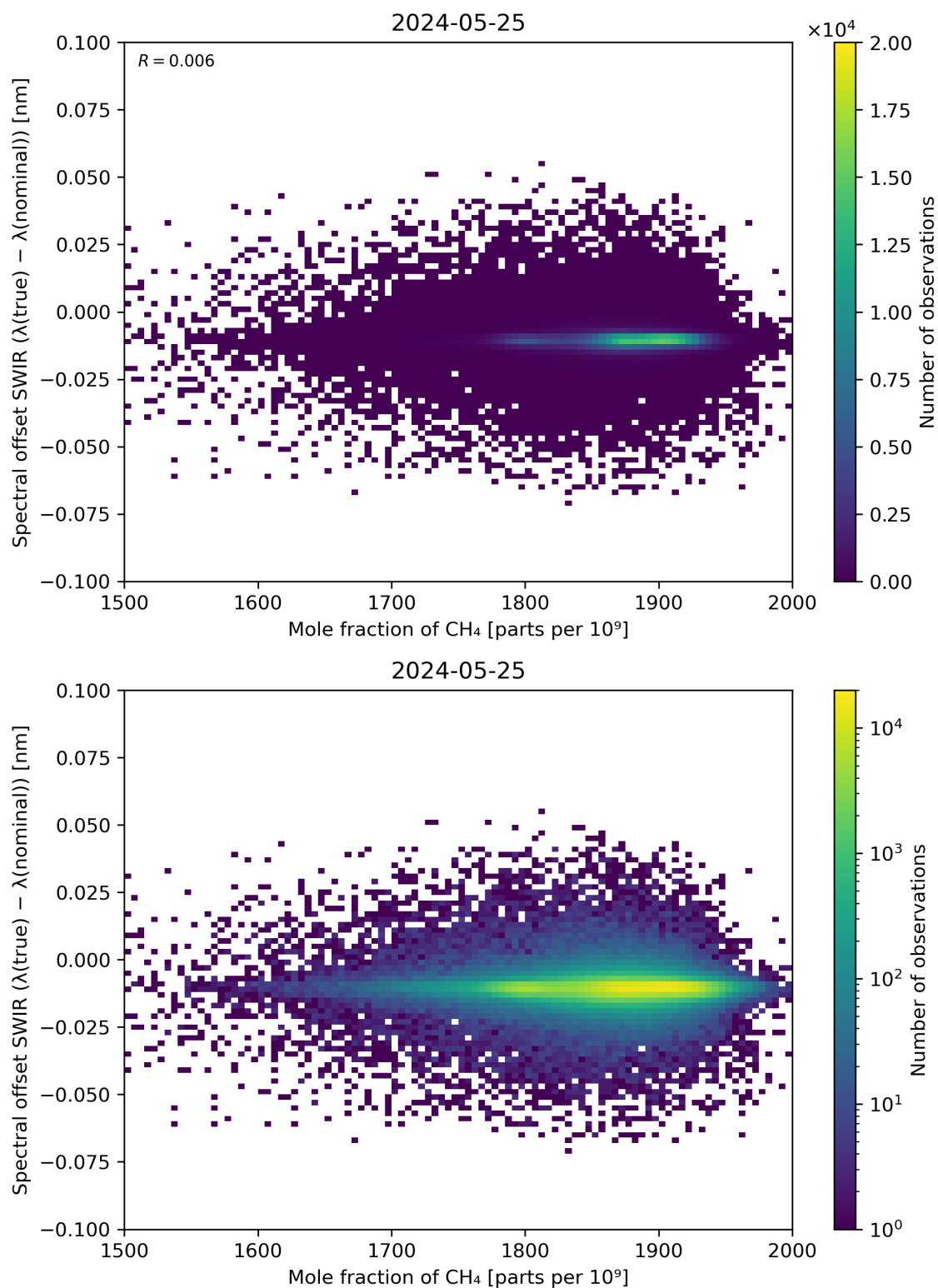
Figure 86: Scatter density plot of “Mole fraction of CH 4 ” against “Spectral offset SWIR ( \lambda(\text{true}) - \lambda(\text{nominal}) )” for 2024-05-24 to 2024-05-26.
