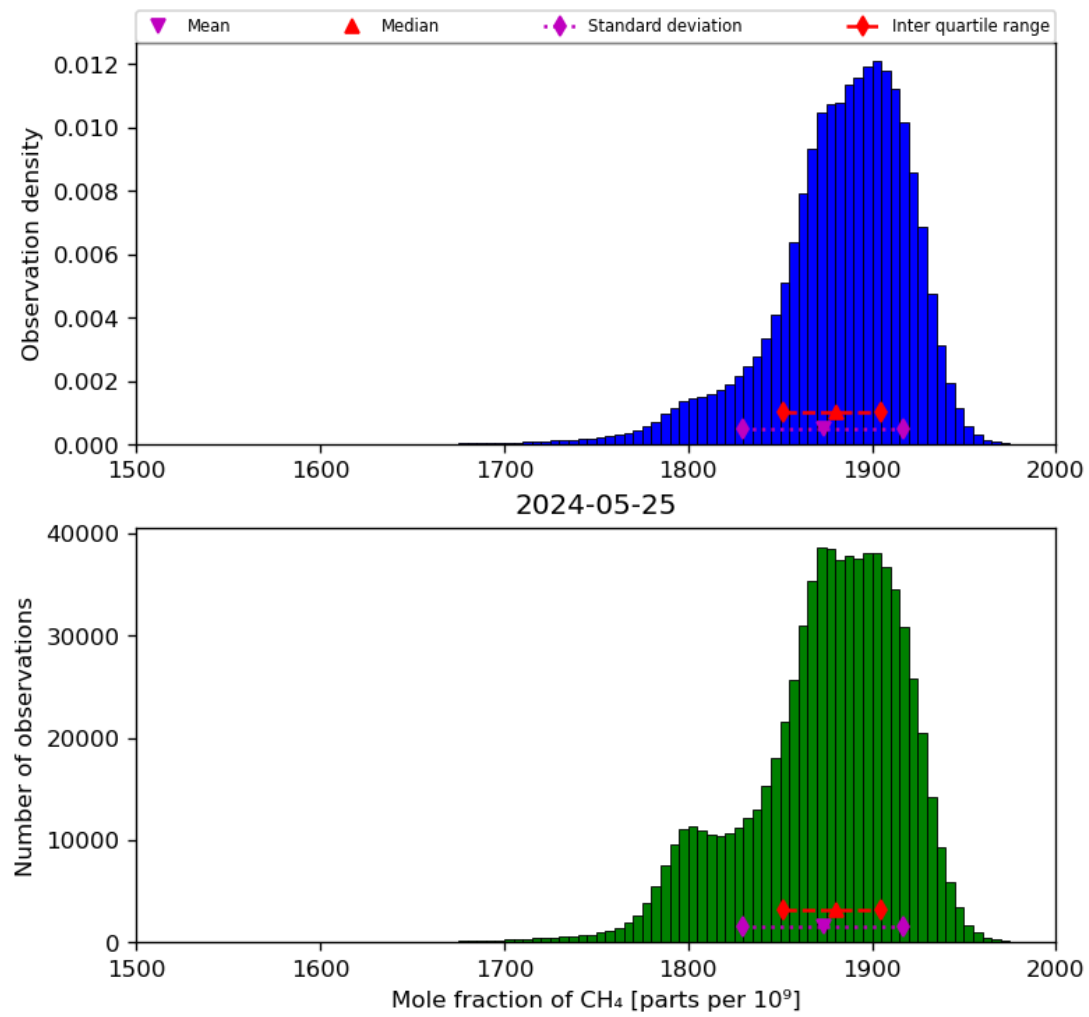
Figure 23: Histogram of “Mole fraction of CH 4 ” for 2024-05-24 to 2024-05-26
