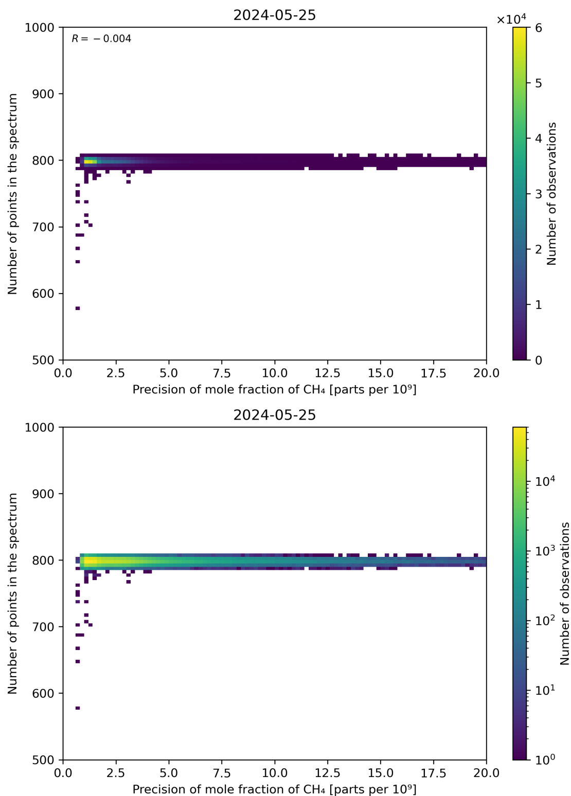
Figure 84: Scatter density plot of “Precision of mole fraction of CH 4 ” against “Number of points in the spectrum” for 2024-05-24 to 2024-05-26.
