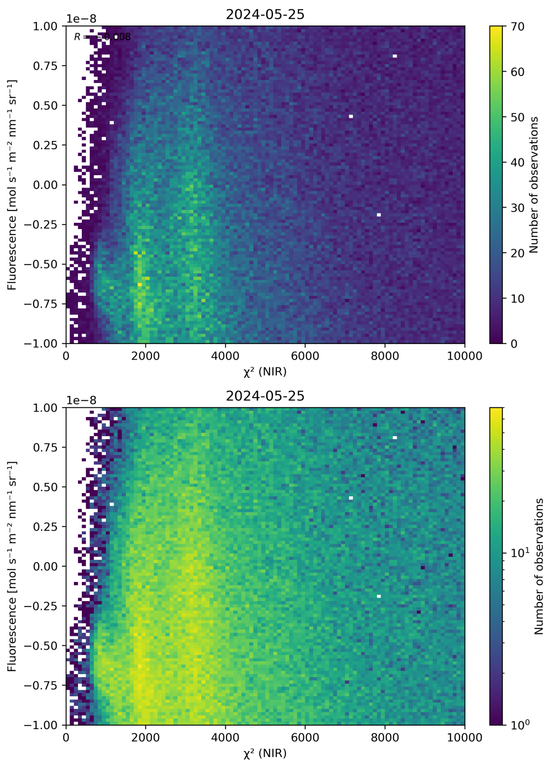
Figure 45: Scatter density plot of “ \chi^2 (NIR)” against “Fluorescence” for 2024-05-24 to 2024-05-26.
