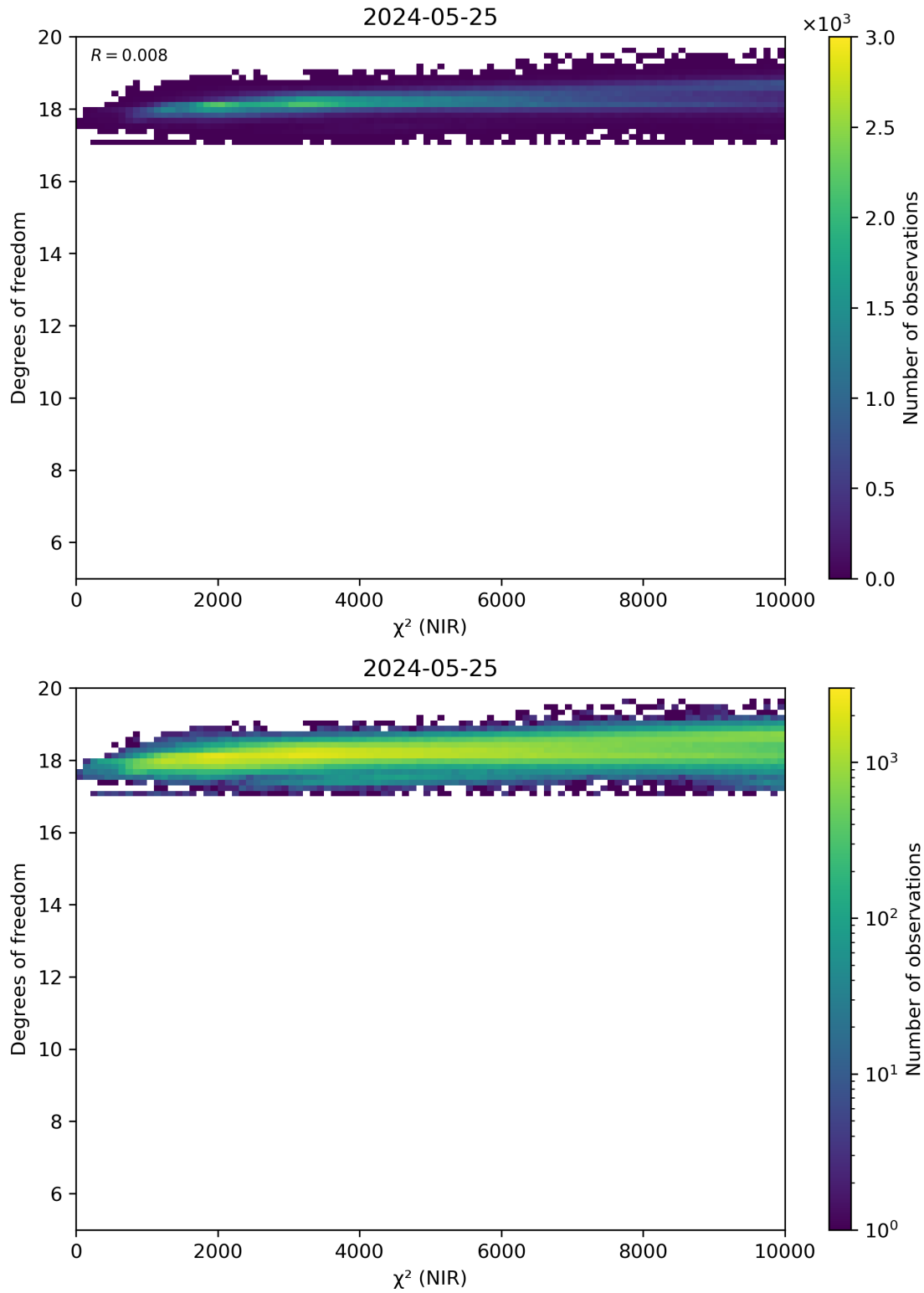
Figure 44: Scatter density plot of “ \chi^2 (NIR)” against “Degrees of freedom” for 2024-05-24 to 2024-05-26.
