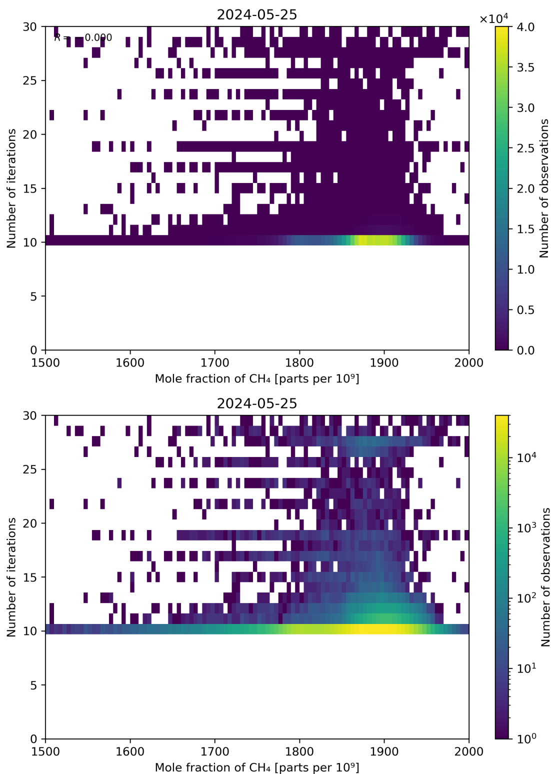
Figure 76: Scatter density plot of “Mole fraction of CH 4 ” against “Number of iterations” for 2024-05-24 to 2024-05-26.
