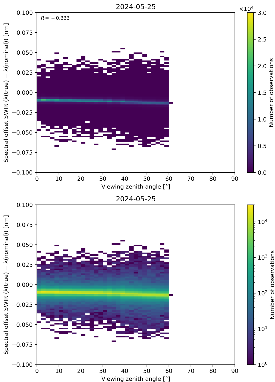
Figure 116: Scatter density plot of “Viewing zenith angle” against “Spectral offset SWIR ( \lambda(\text{true}) - \lambda(\text{nominal}) )” for 2024-05-24 to 2024-05-26.
