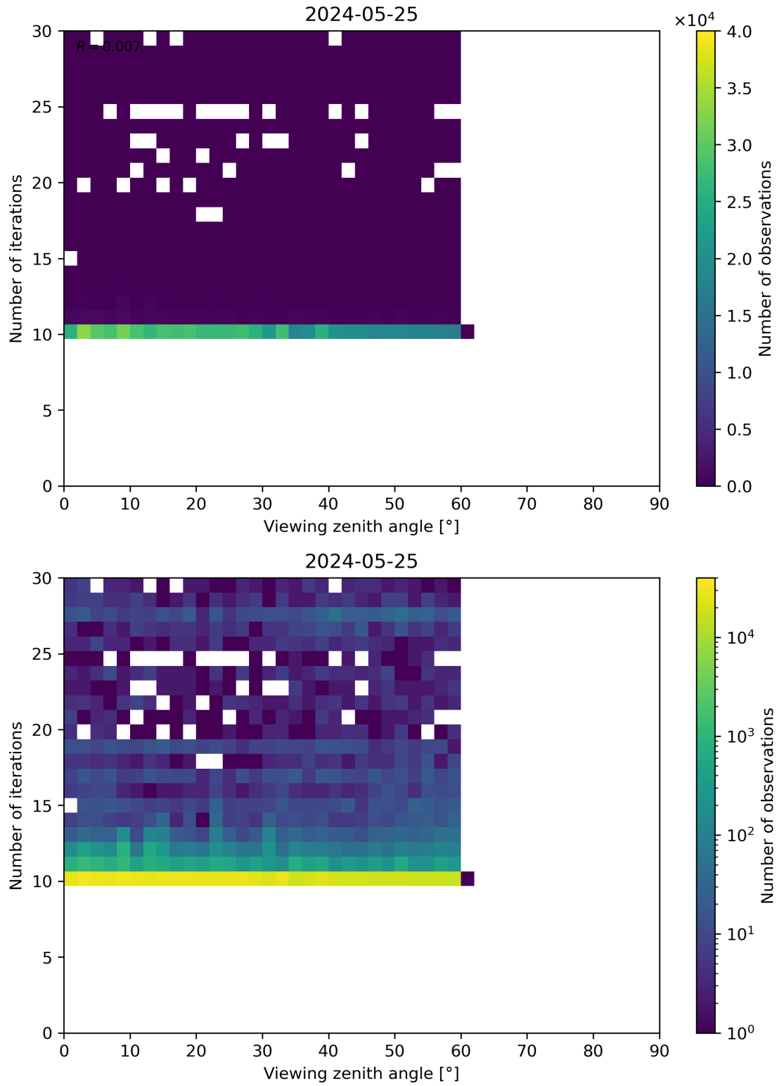
Figure 113: Scatter density plot of “Viewing zenith angle” against “Number of iterations” for 2024-05-24 to 2024-05-26.
