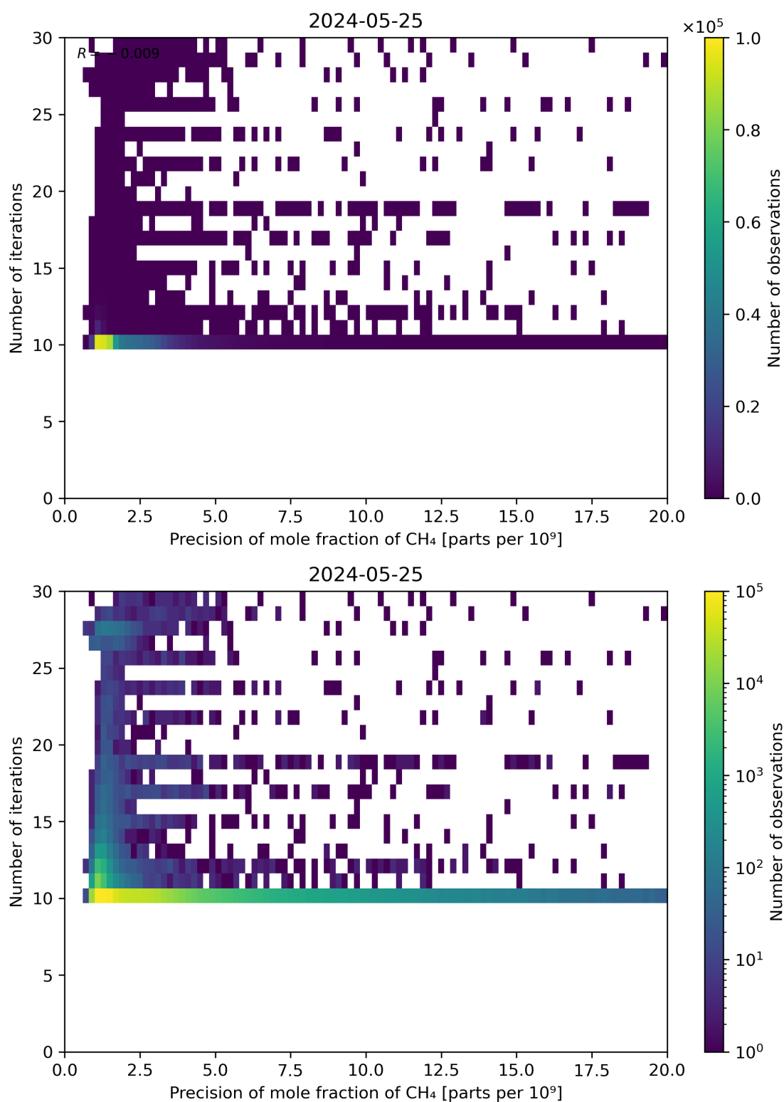
Figure 83: Scatter density plot of “Precision of mole fraction of CH 4 ” against “Number of iterations” for 2024-05-24 to 2024-05-26.
