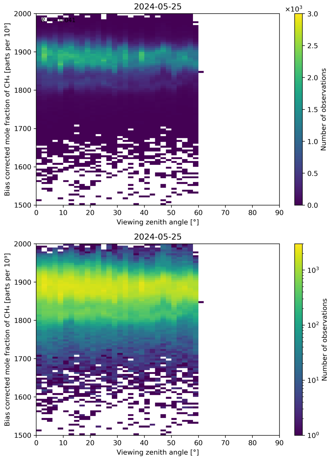
Figure 111: Scatter density plot of “Viewing zenith angle” against “Bias corrected mole fraction of CH 4 ” for 2024-05-24 to 2024-05-26.
