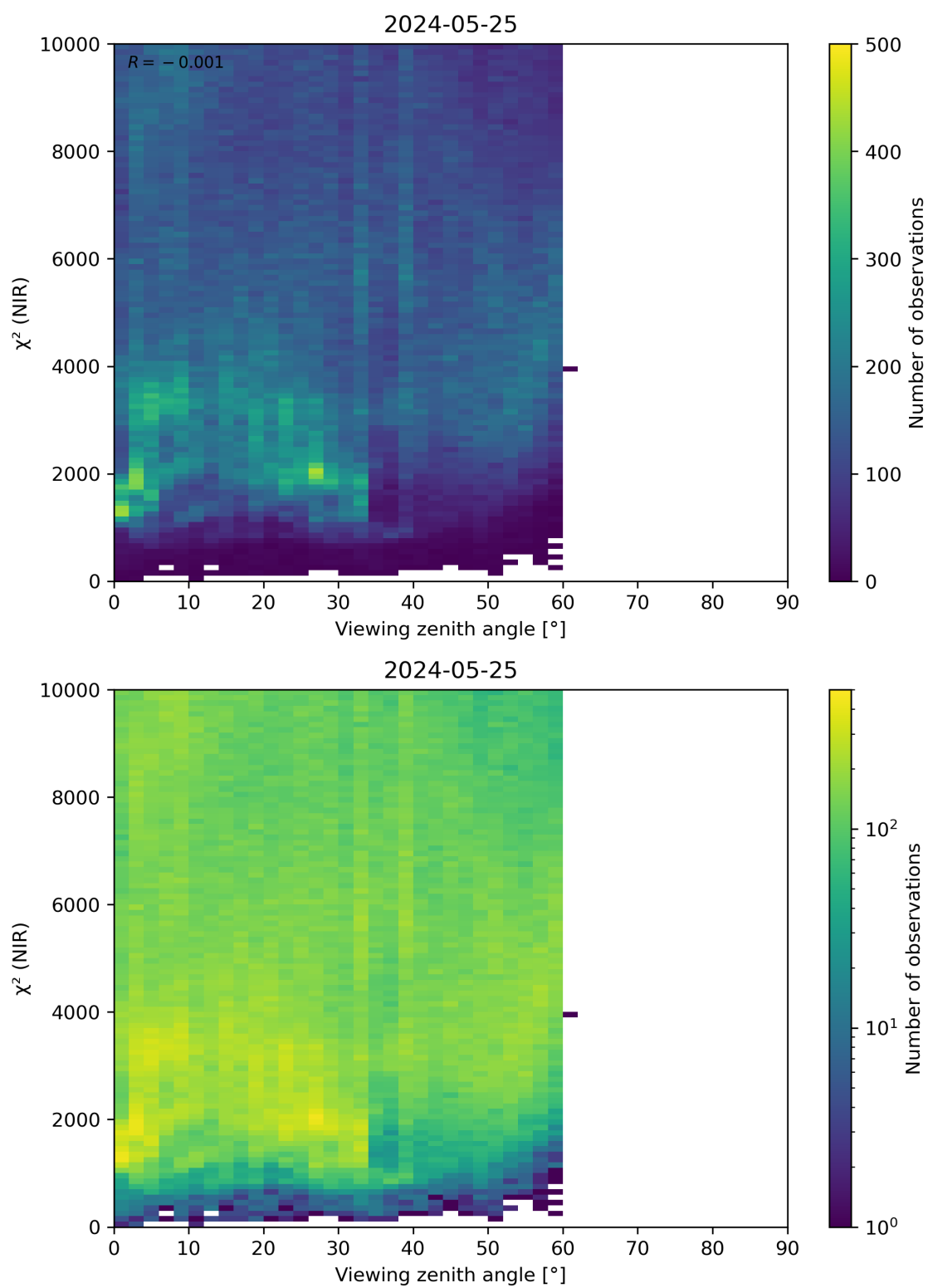
Figure 105: Scatter density plot of “Viewing zenith angle” against “ \chi^2 (NIR)” for 2024-05-24 to 2024-05-26.
