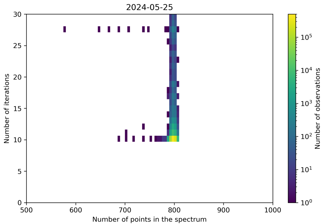
Figure 92: Scatter density plot of “Number of points in the spectrum” against “Number of iterations” for 2024-05-24 to 2024-05-26.
