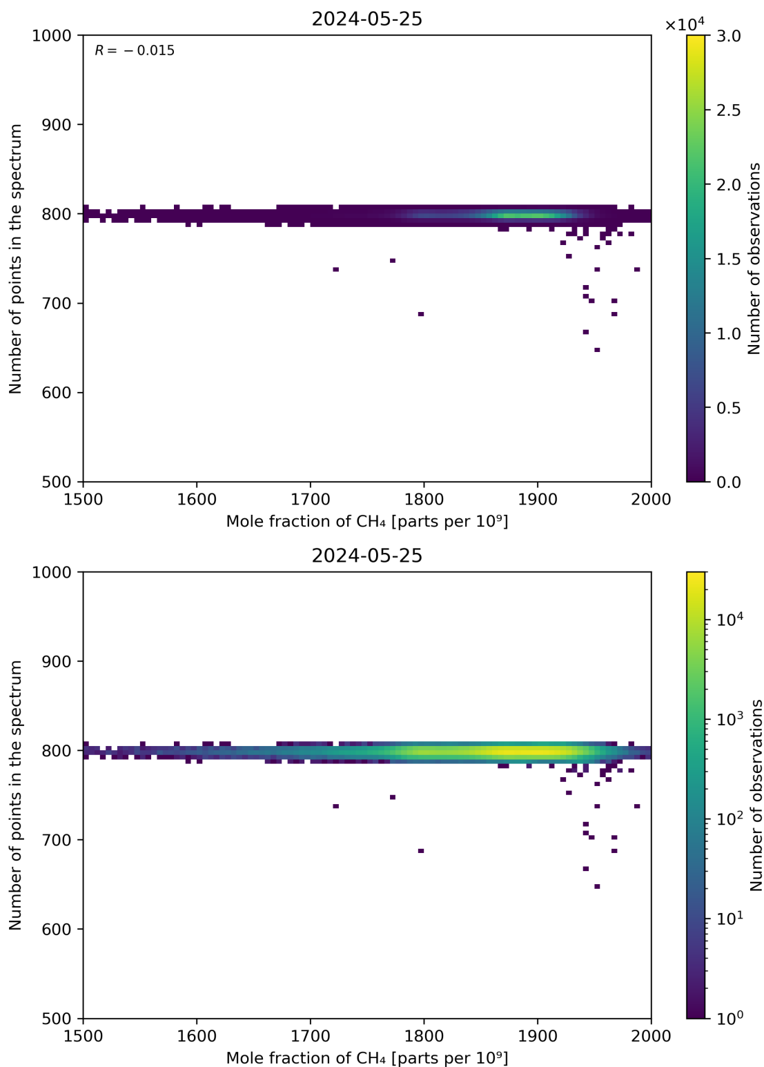
Figure 77: Scatter density plot of “Mole fraction of CH 4 ” against “Number of points in the spectrum” for 2024-05-24 to 2024-05-26.
