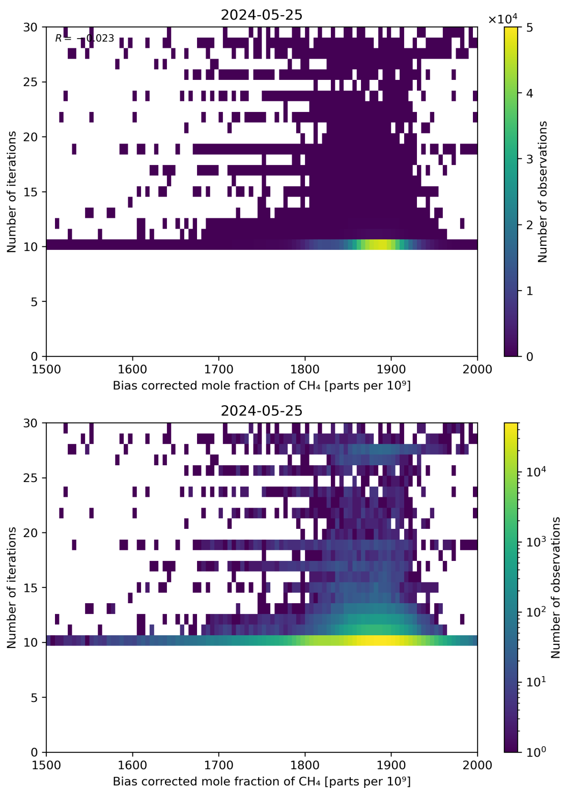
Figure 67: Scatter density plot of “Bias corrected mole fraction of CH 4 ” against “Number of iterations” for 2024-05-24 to 2024-05-26.
