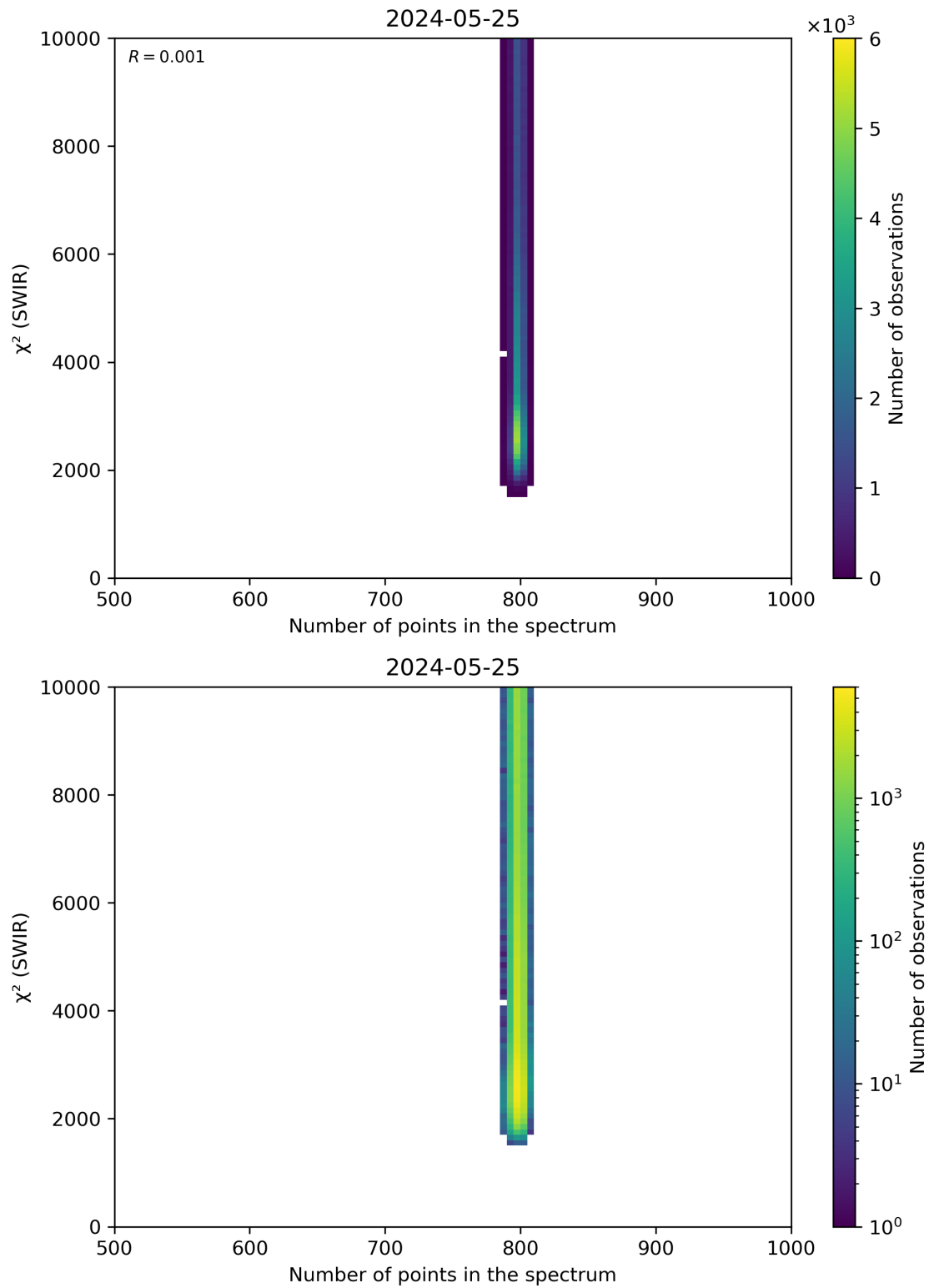
Figure 89: Scatter density plot of “Number of points in the spectrum” against “ \chi^2 (SWIR)” for 2024-05-24 to 2024-05-26.
