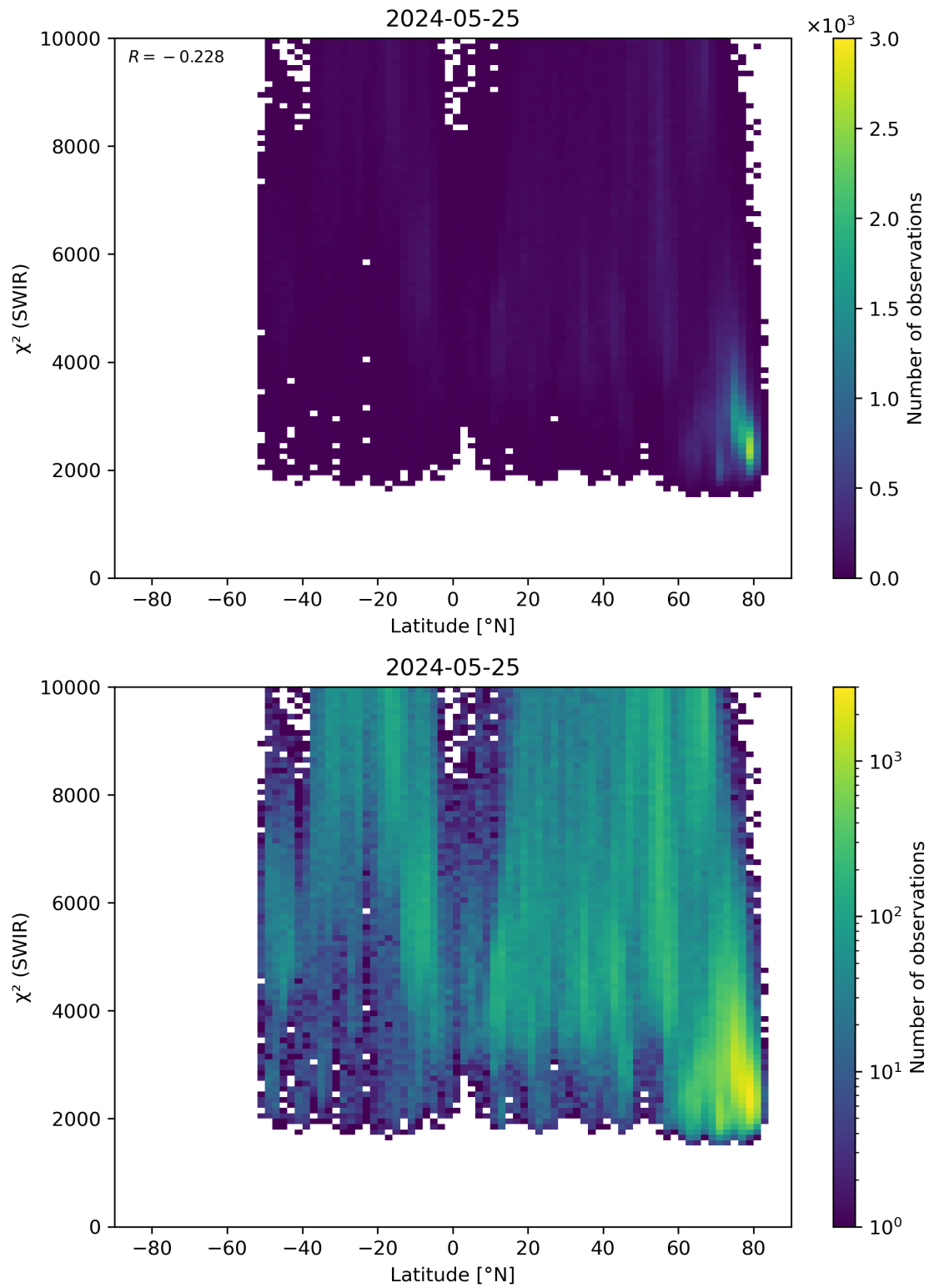
Figure 54: Scatter density plot of “Latitude” against “ \chi^2 (SWIR)” for 2024-05-24 to 2024-05-26.
