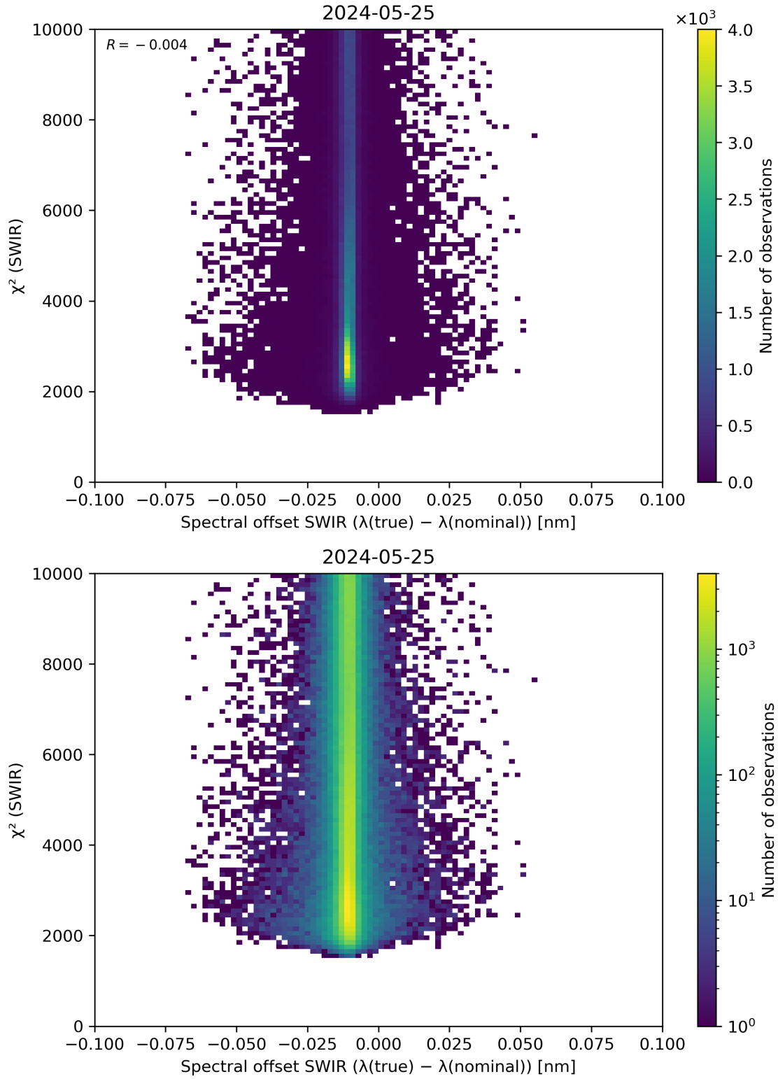
Figure 118: Scatter density plot of “Spectral offset SWIR ( \lambda(\text{true}) - \lambda(\text{nominal}) )” against “ \chi^2 (SWIR)” for 2024-05-24 to 2024-05-26.
