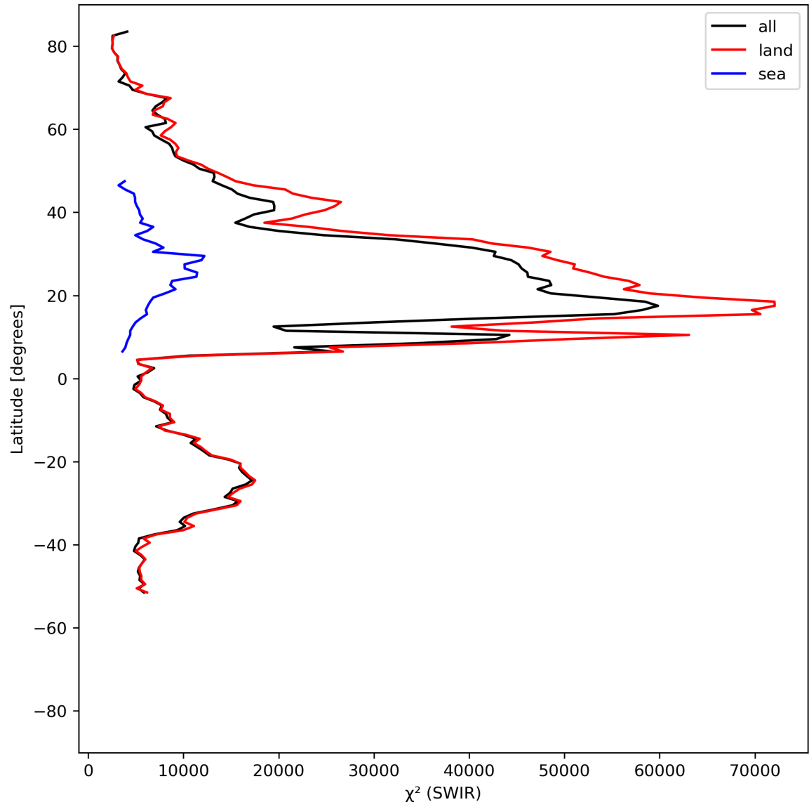
Figure 17: Zonal average of “ \chi^2 (SWIR)” for 2024-05-24 to 2024-05-26.
