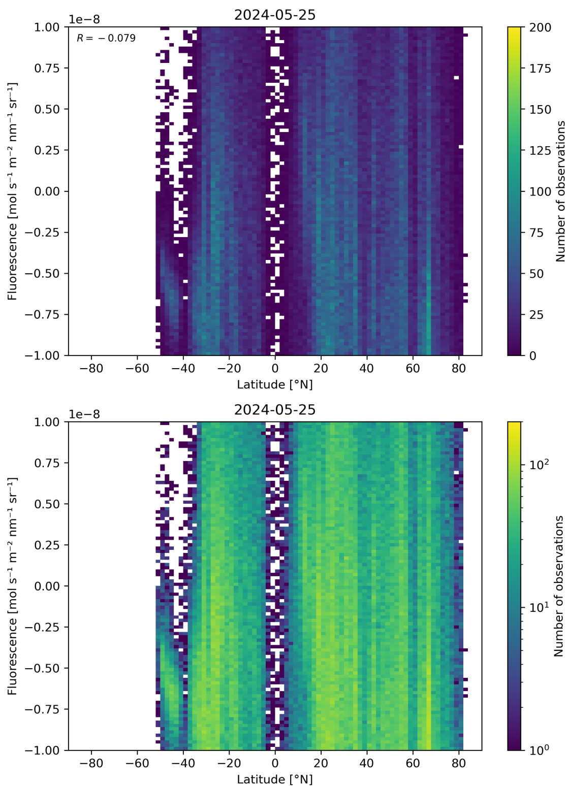
Figure 56: Scatter density plot of “Latitude” against “Fluorescence” for 2024-05-24 to 2024-05-26.
