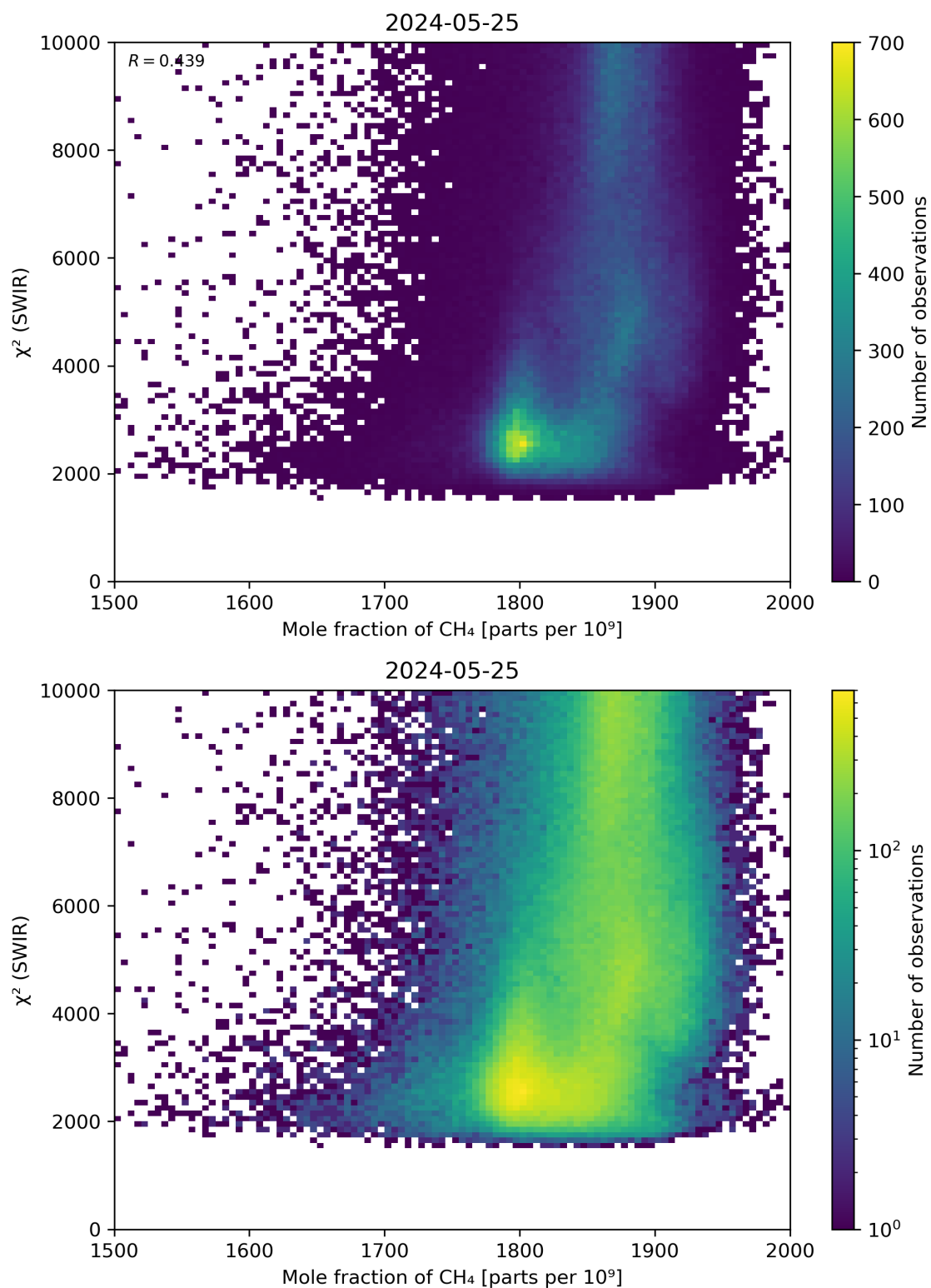
Figure 71: Scatter density plot of “Mole fraction of \text{CH}_4 ” against “ \chi^2 (SWIR)” for 2024-05-24 to 2024-05-26.
