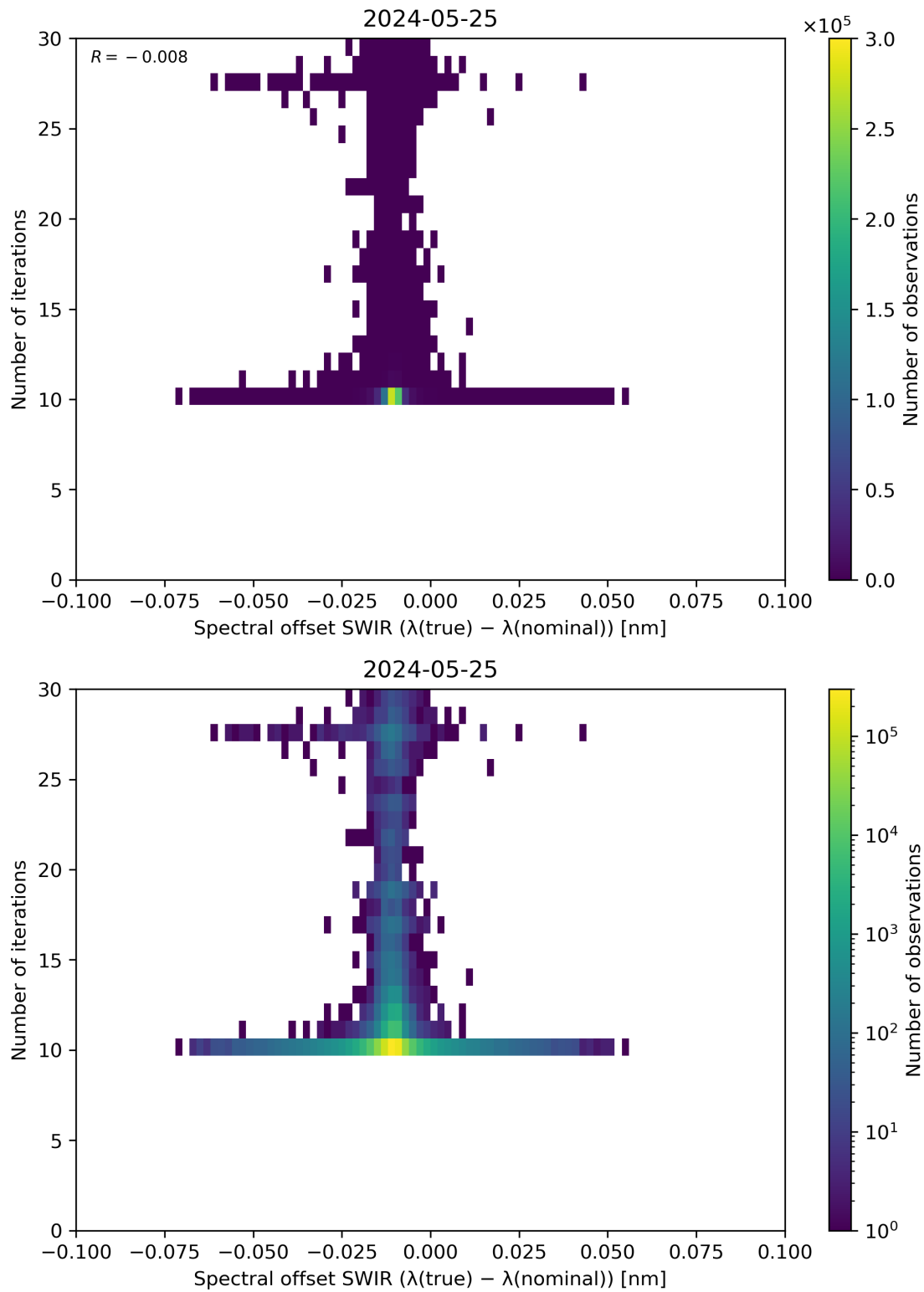
Figure 121: Scatter density plot of “Spectral offset SWIR ( \lambda(\text{true}) - \lambda(\text{nominal}) )” against “Number of iterations” for 2024-05-24 to 2024-05-26.
