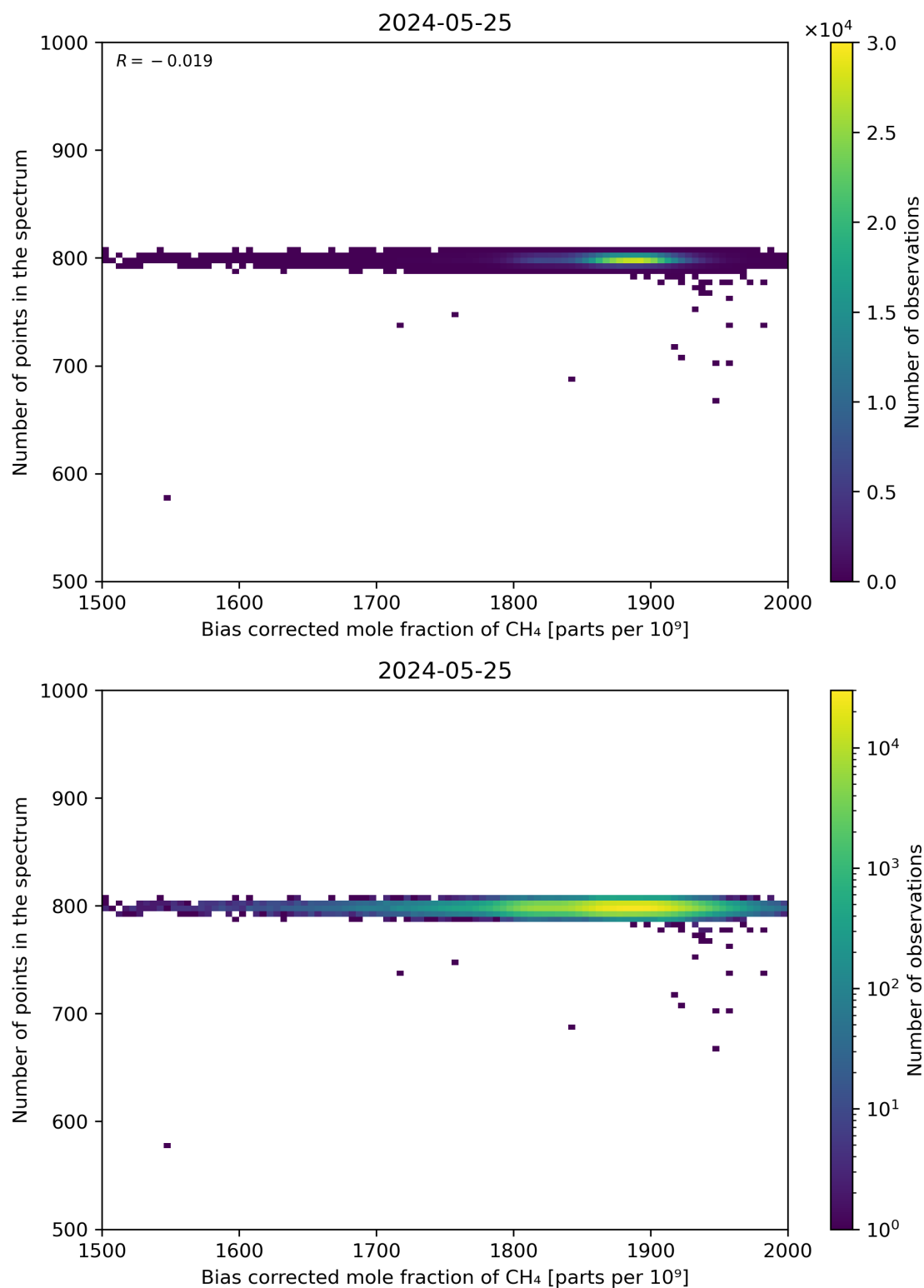
Figure 68: Scatter density plot of “Bias corrected mole fraction of CH 4 ” against “Number of points in the spectrum” for 2024-05-24 to 2024-05-26.
