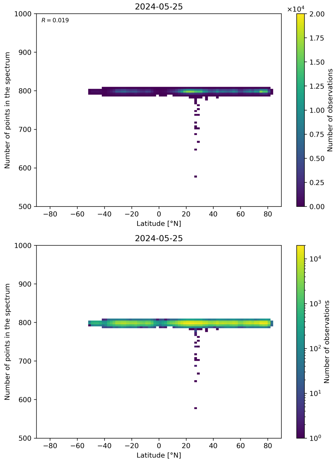
Figure 61: Scatter density plot of “Latitude” against “Number of points in the spectrum” for 2024-05-24 to 2024-05-26.
