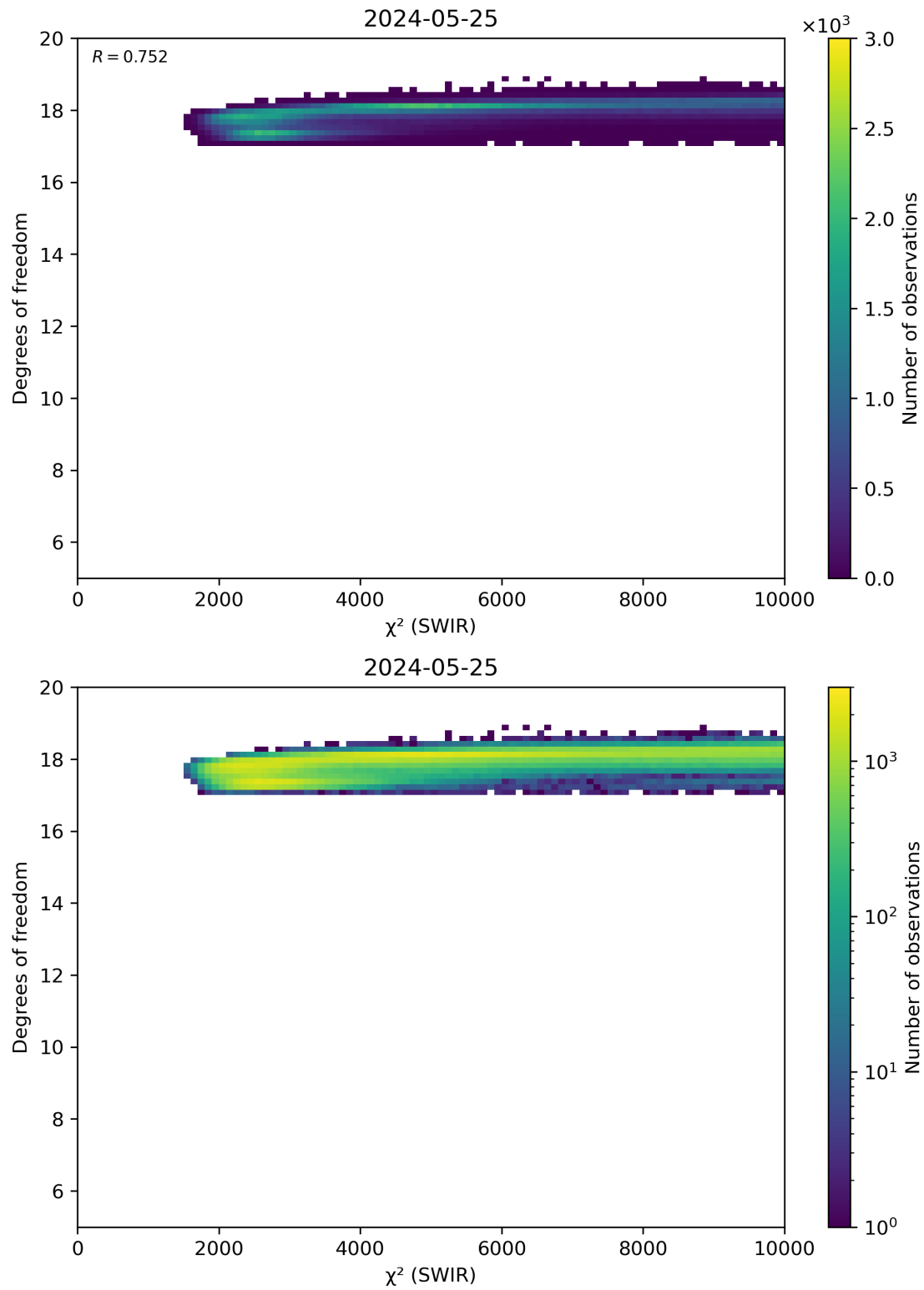
Figure 48: Scatter density plot of “ \chi^2 (SWIR)” against “Degrees of freedom” for 2024-05-24 to 2024-05-26.
