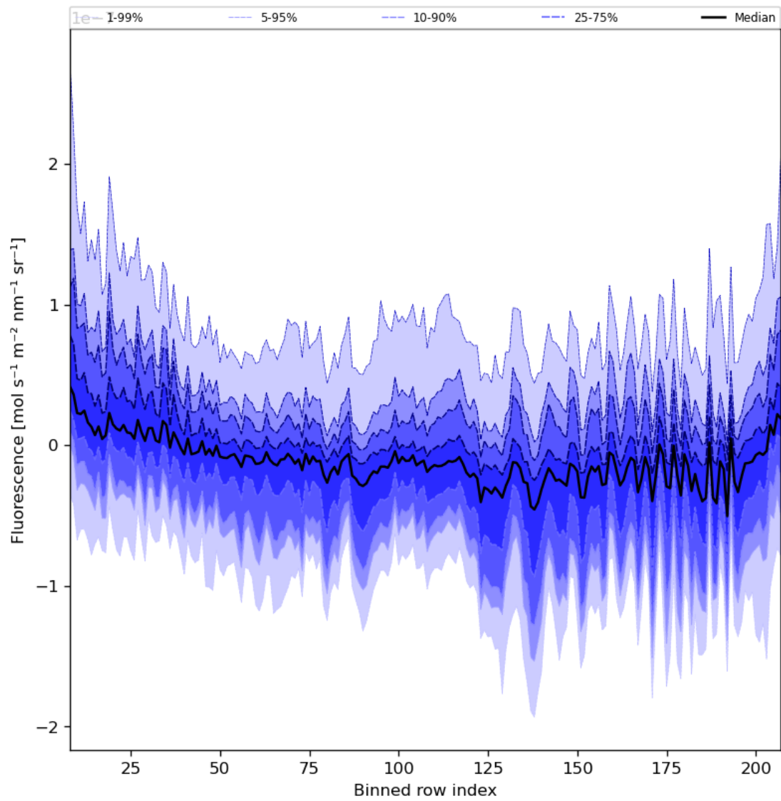
Figure 43: Along track statistics of “Fluorescence” for 2024-05-24 to 2024-05-26
