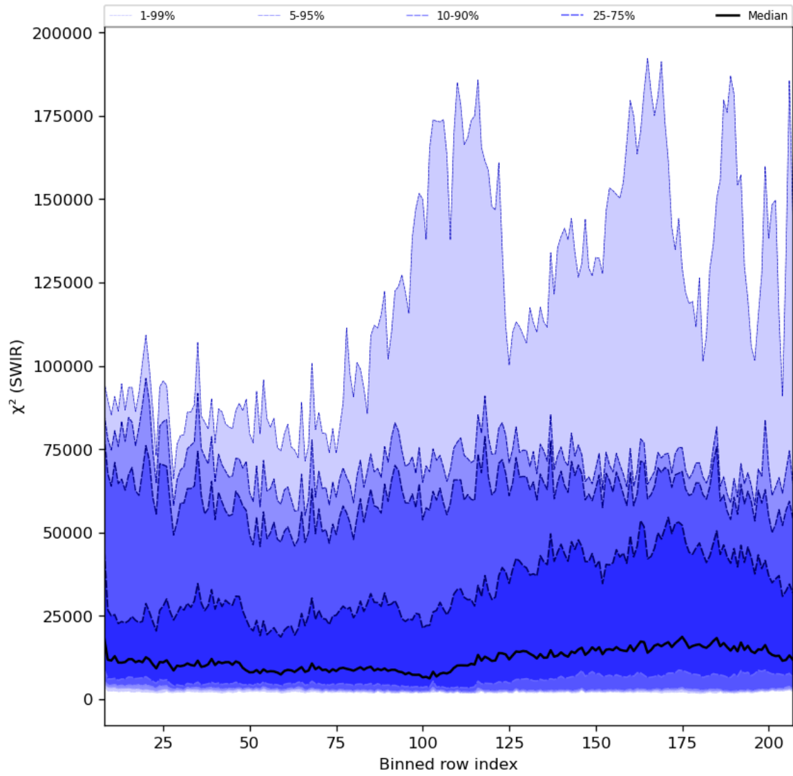
Figure 39: Along track statistics of " \chi^2 (SWIR)" for 2024-05-24 to 2024-05-26
