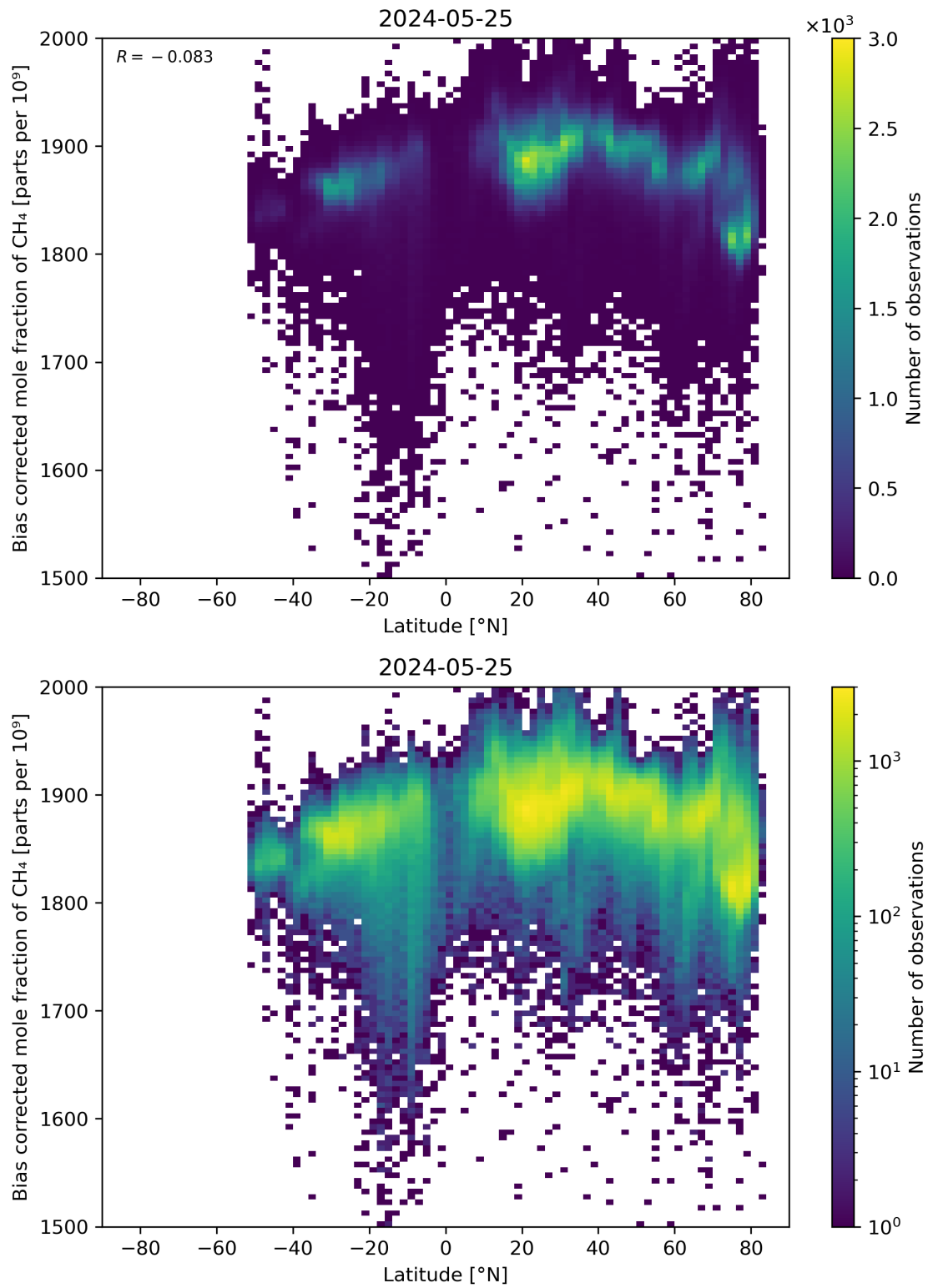
Figure 58: Scatter density plot of “Latitude” against “Bias corrected mole fraction of \text{CH}_4 ” for 2024-05-24 to 2024-05-26.
