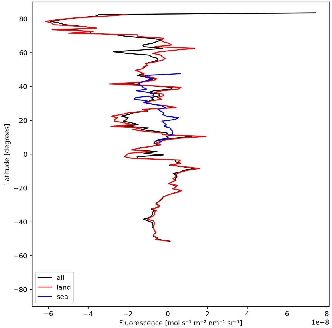
Figure 21: Zonal average of “Fluorescence” for 2024-05-24 to 2024-05-26.
