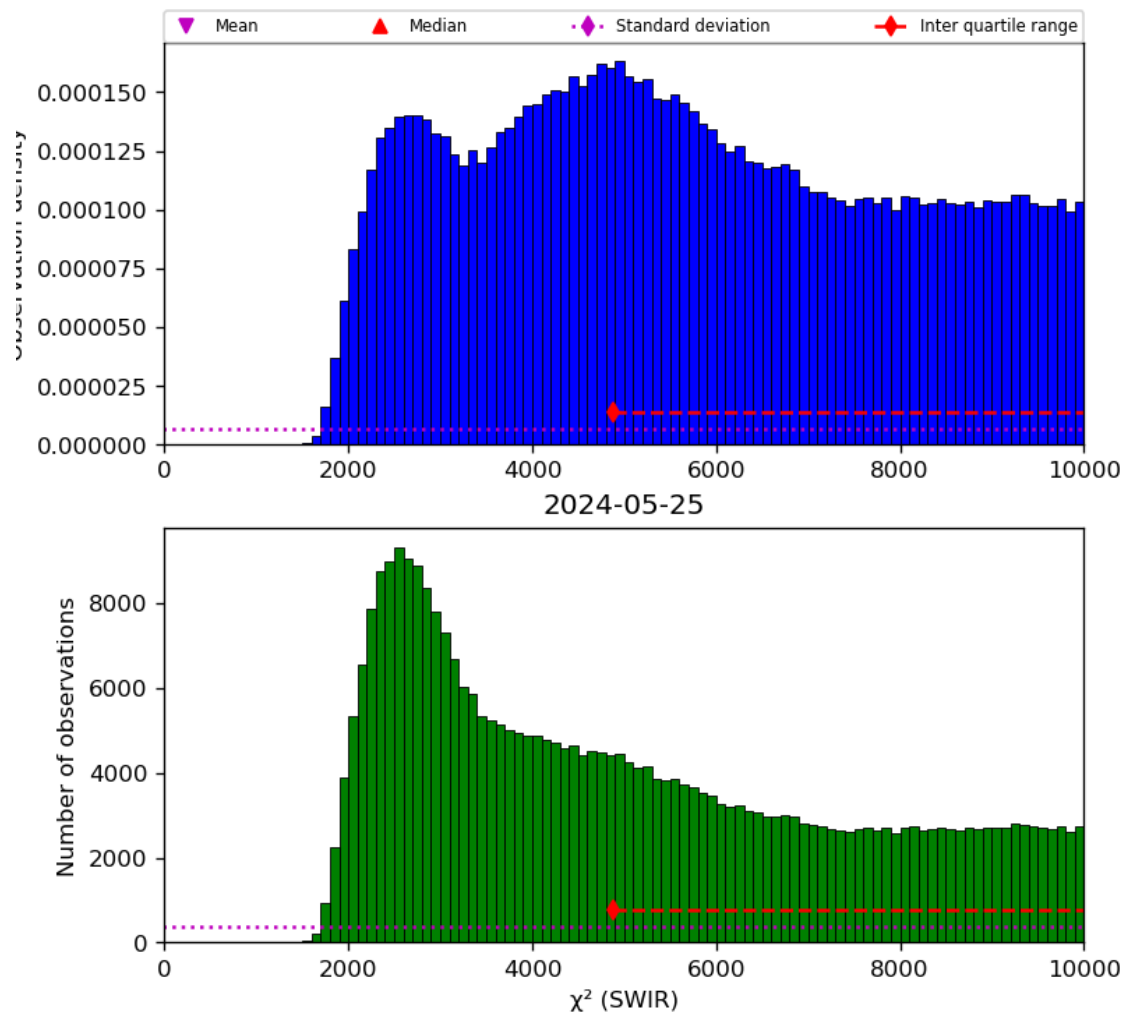
Figure 28: Histogram of “ \chi^2 (SWIR)” for 2024-05-24 to 2024-05-26
