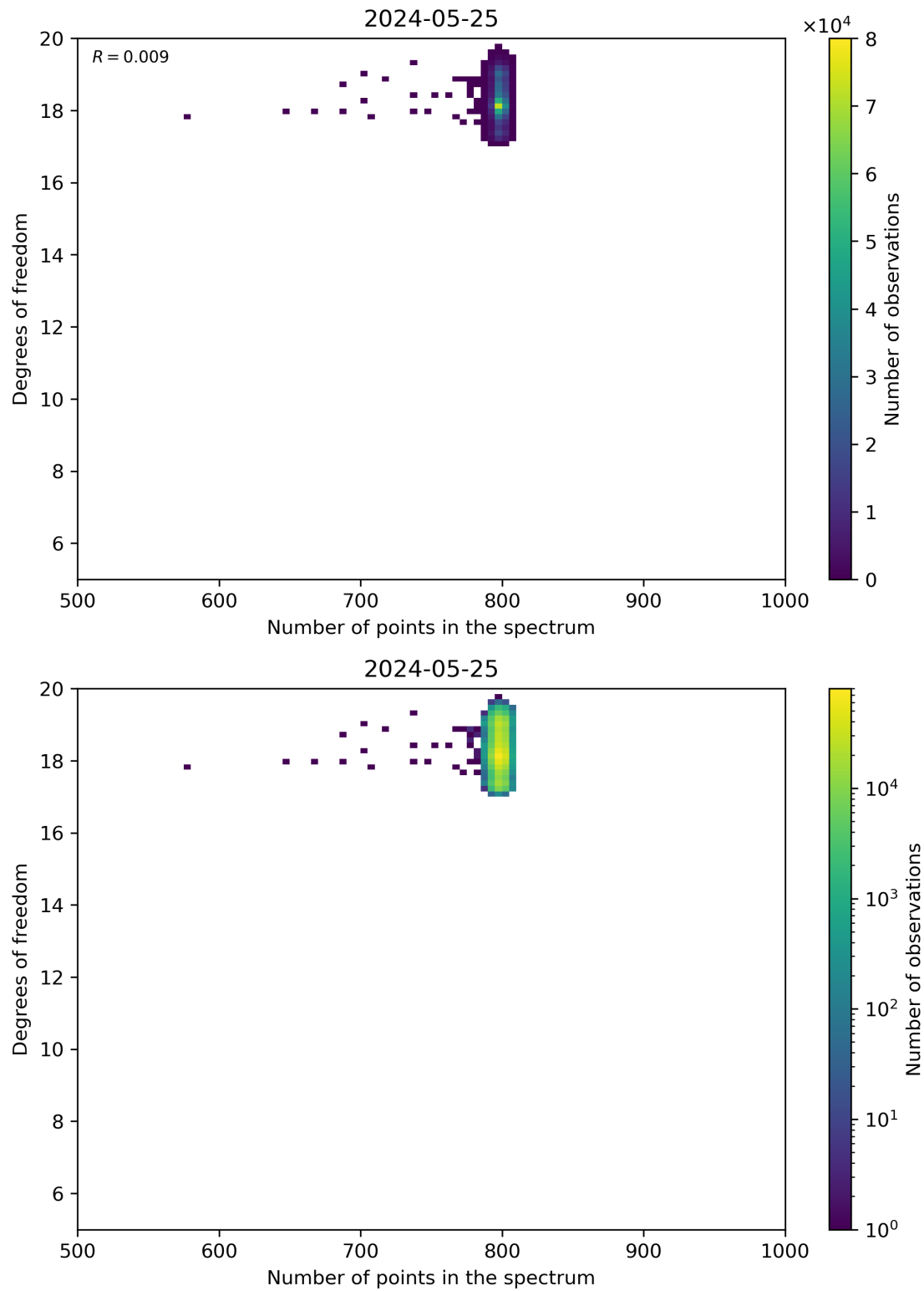
Figure 90: Scatter density plot of “Number of points in the spectrum” against “Degrees of freedom” for 2024-05-24 to 2024-05-26.
