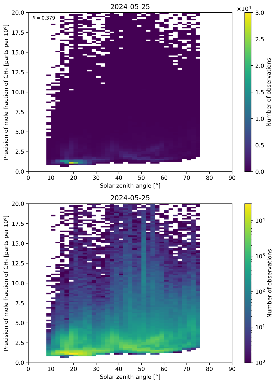
Figure 101: Scatter density plot of “Solar zenith angle” against “Precision of mole fraction of CH 4 ” for 2024-05-24 to 2024-05-26.
