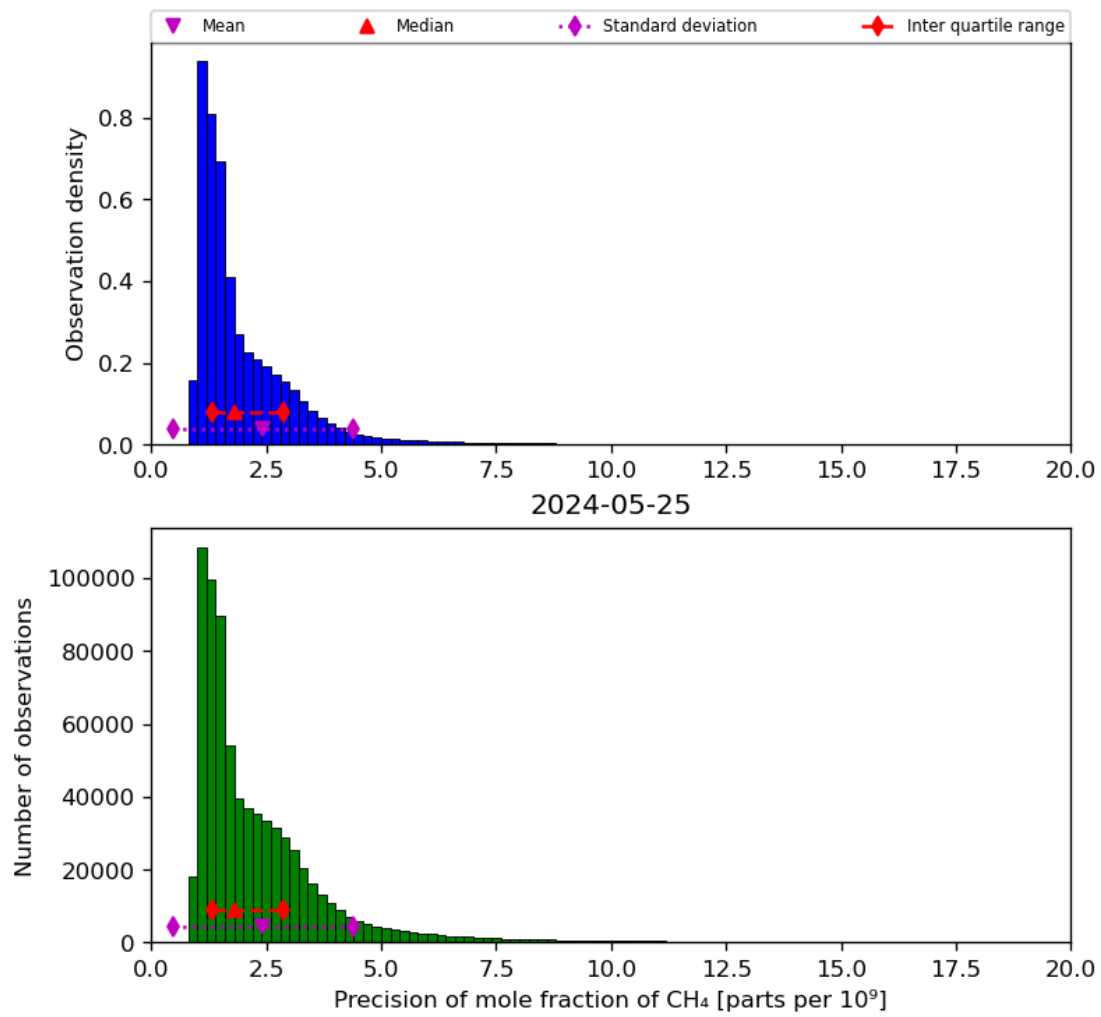
Figure 24: Histogram of “Precision of mole fraction of CH 4 ” for 2024-05-24 to 2024-05-26
