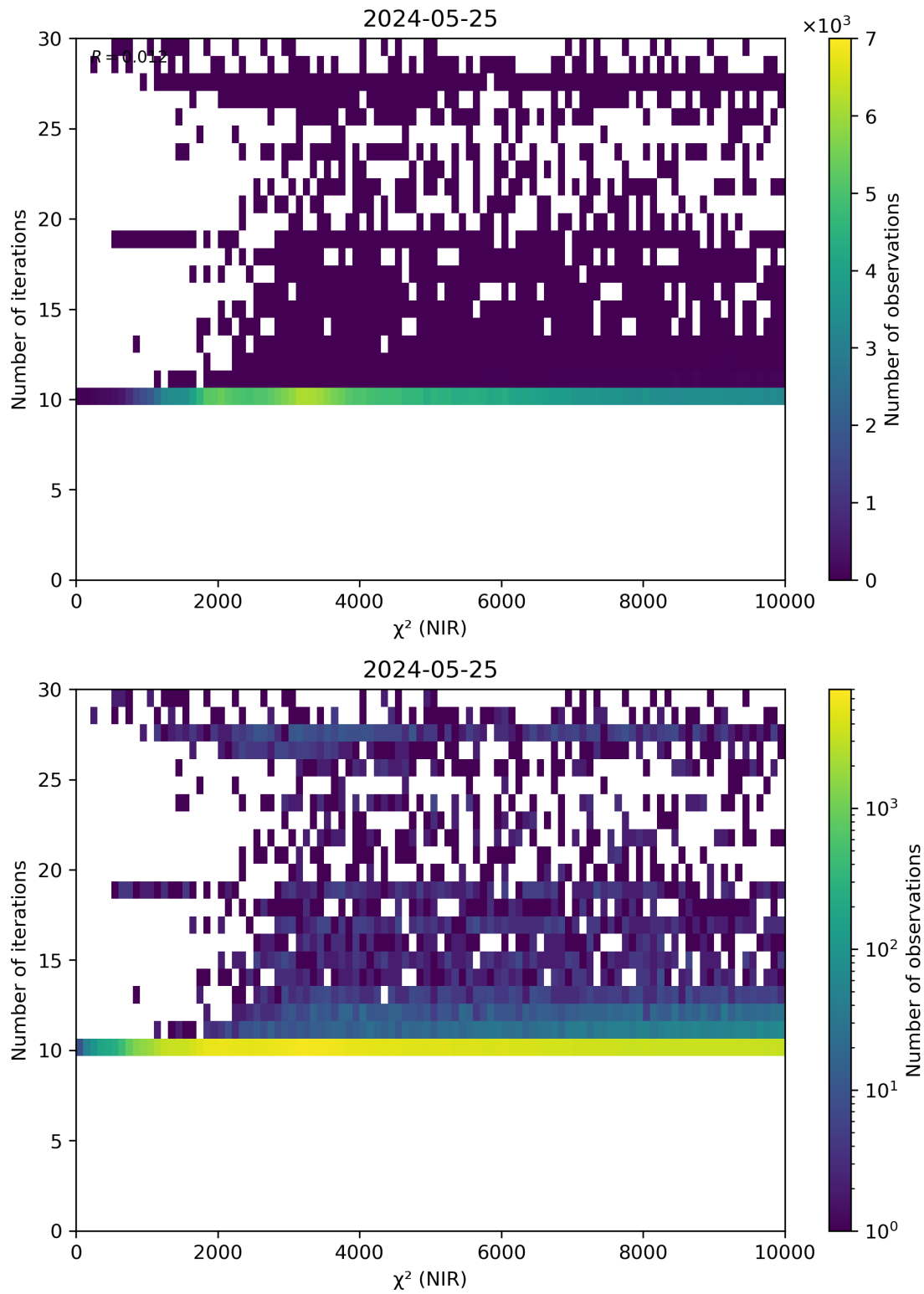
Figure 46: Scatter density plot of “ \chi^2 (NIR)” against “Number of iterations” for 2024-05-24 to 2024-05-26.
