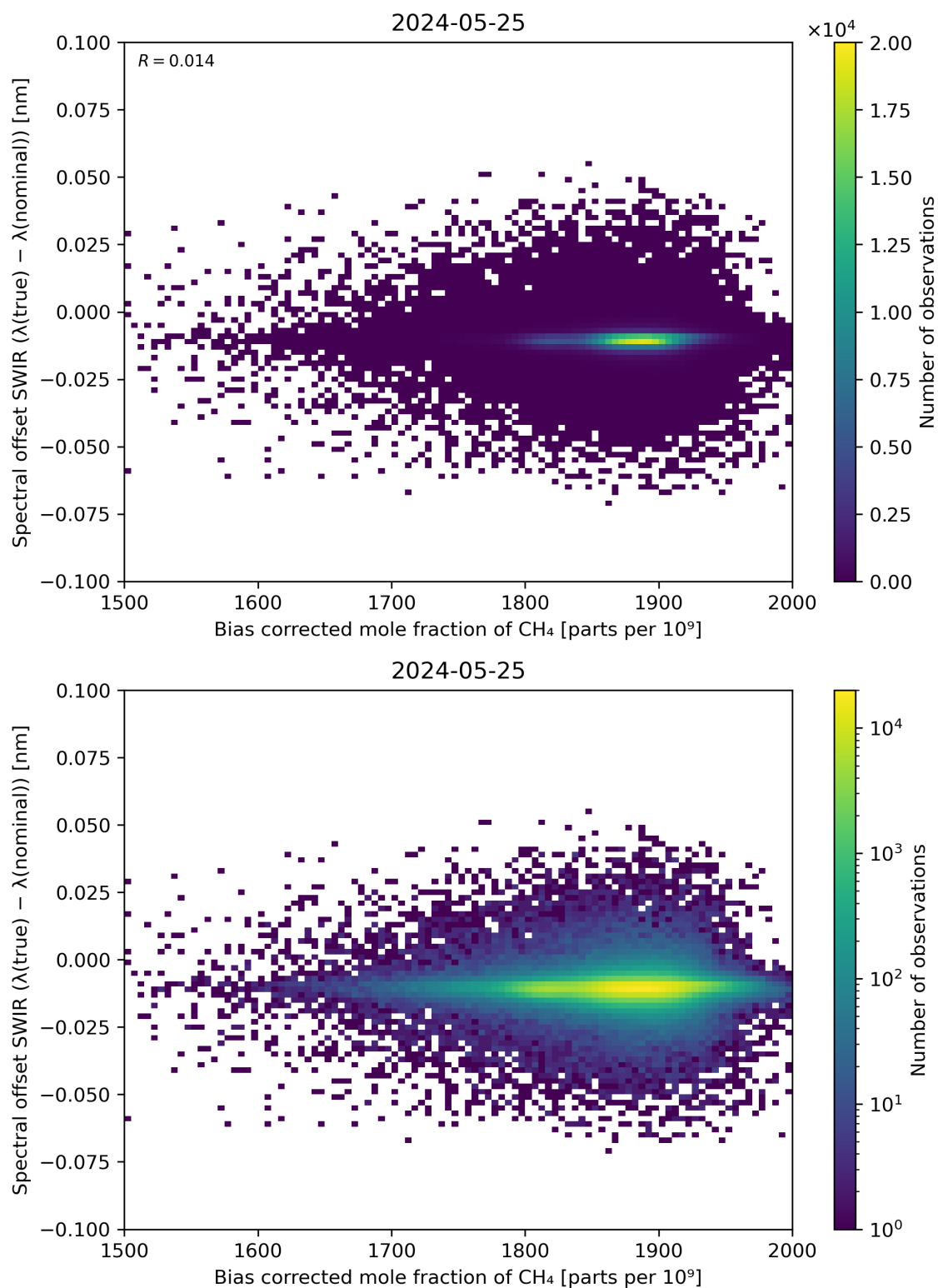
Figure 69: Scatter density plot of “Bias corrected mole fraction of \text{CH}_4 ” against “Spectral offset SWIR ( \lambda(\text{true}) - \lambda(\text{nominal}) )” for 2024-05-24 to 2024-05-26.
