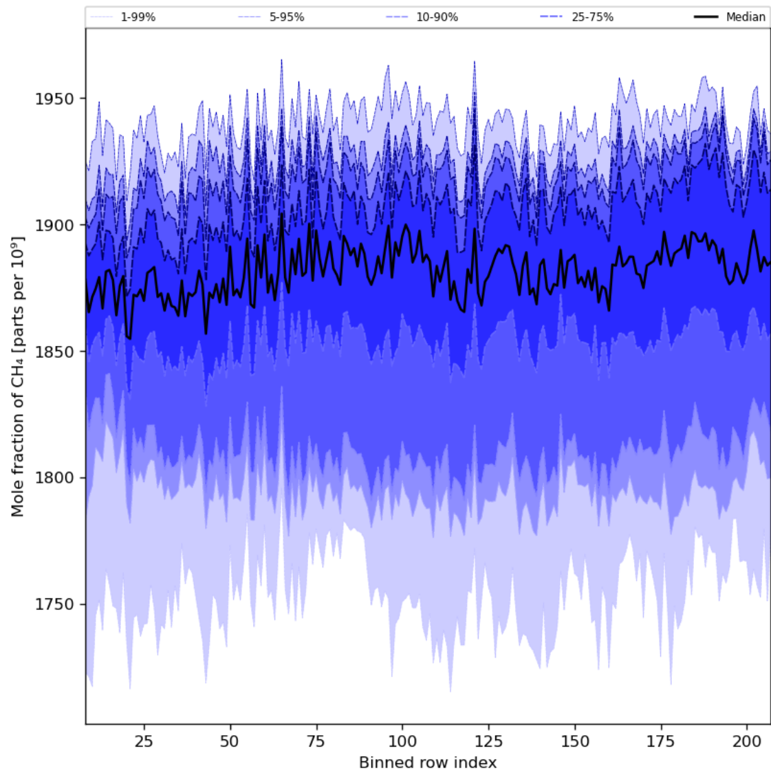
Figure 34: Along track statistics of “Mole fraction of CH 4 ” for 2024-05-24 to 2024-05-26
