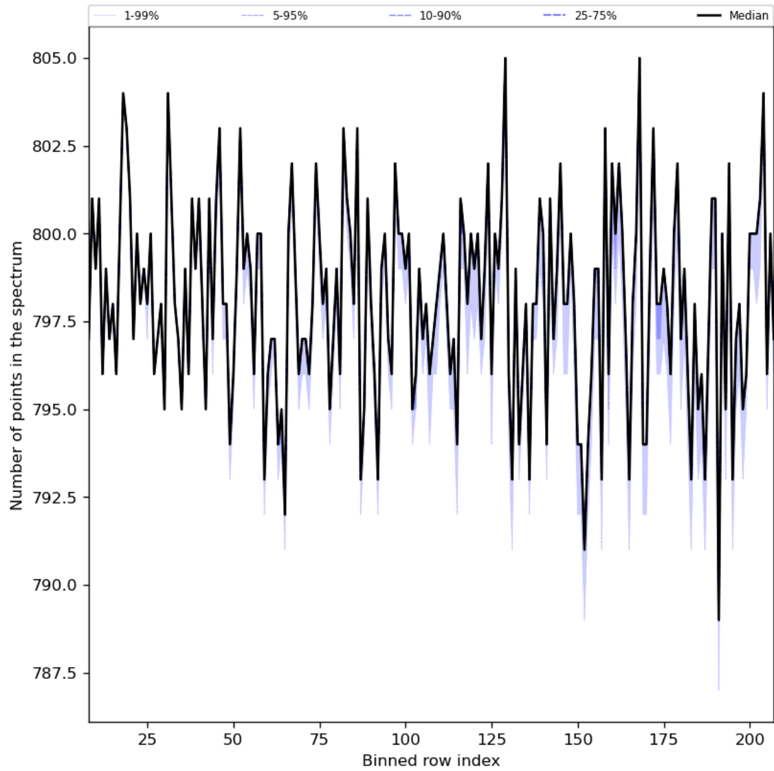
Figure 37: Along track statistics of “Number of points in the spectrum” for 2024-05-24 to 2024-05-26
