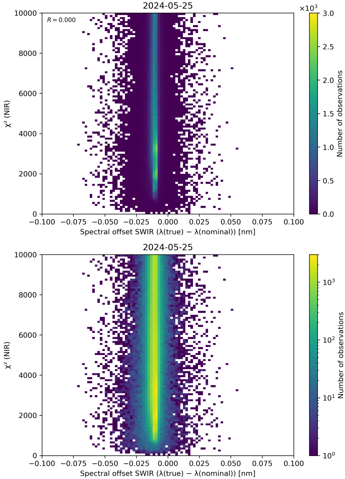
Figure 117: Scatter density plot of “Spectral offset SWIR ( \lambda(\text{true}) - \lambda(\text{nominal}) )” against “ \chi^2 (NIR)” for 2024-05-24 to 2024-05-26.
