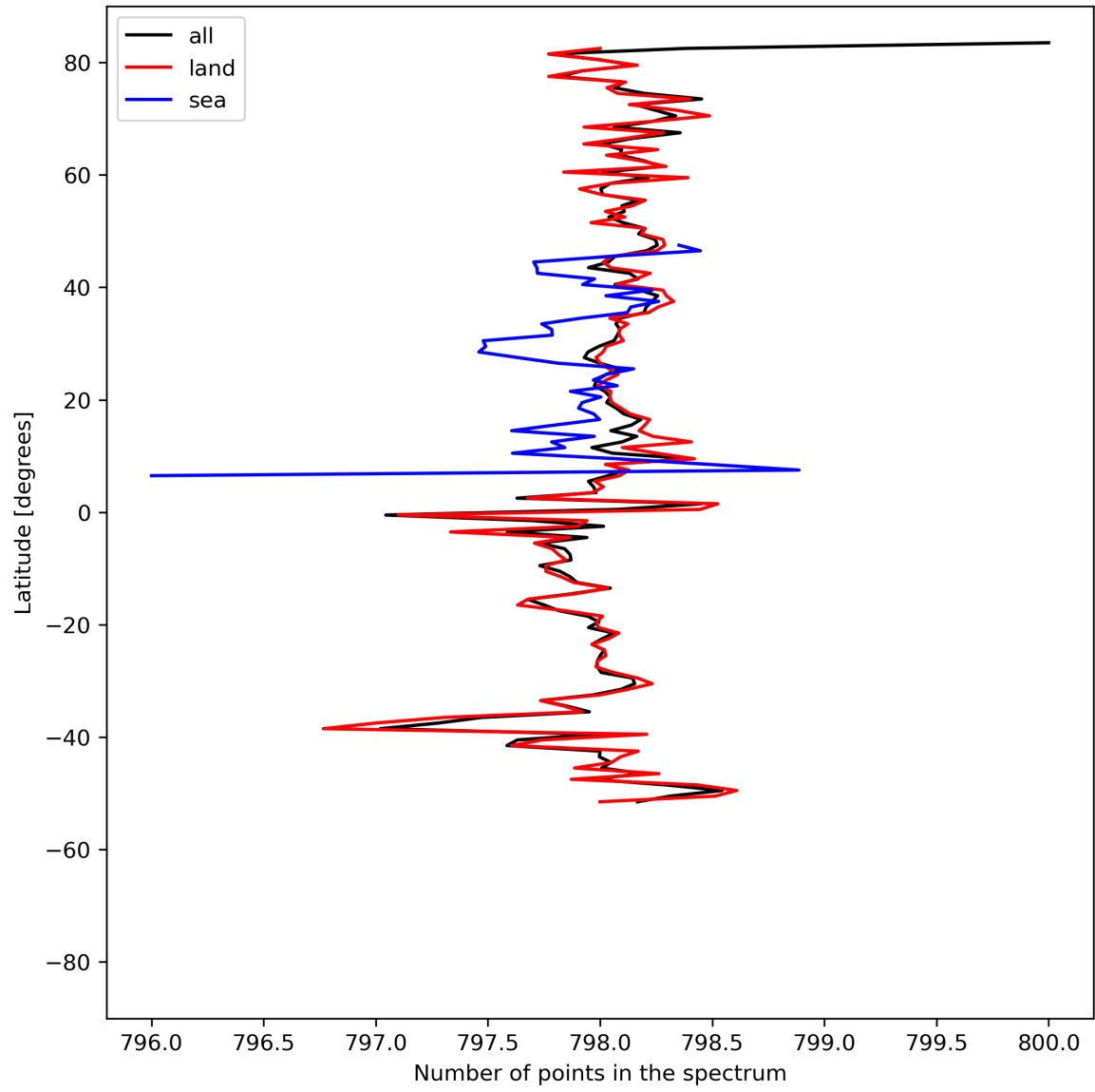
Figure 15: Zonal average of “Number of points in the spectrum” for 2024-05-24 to 2024-05-26.
