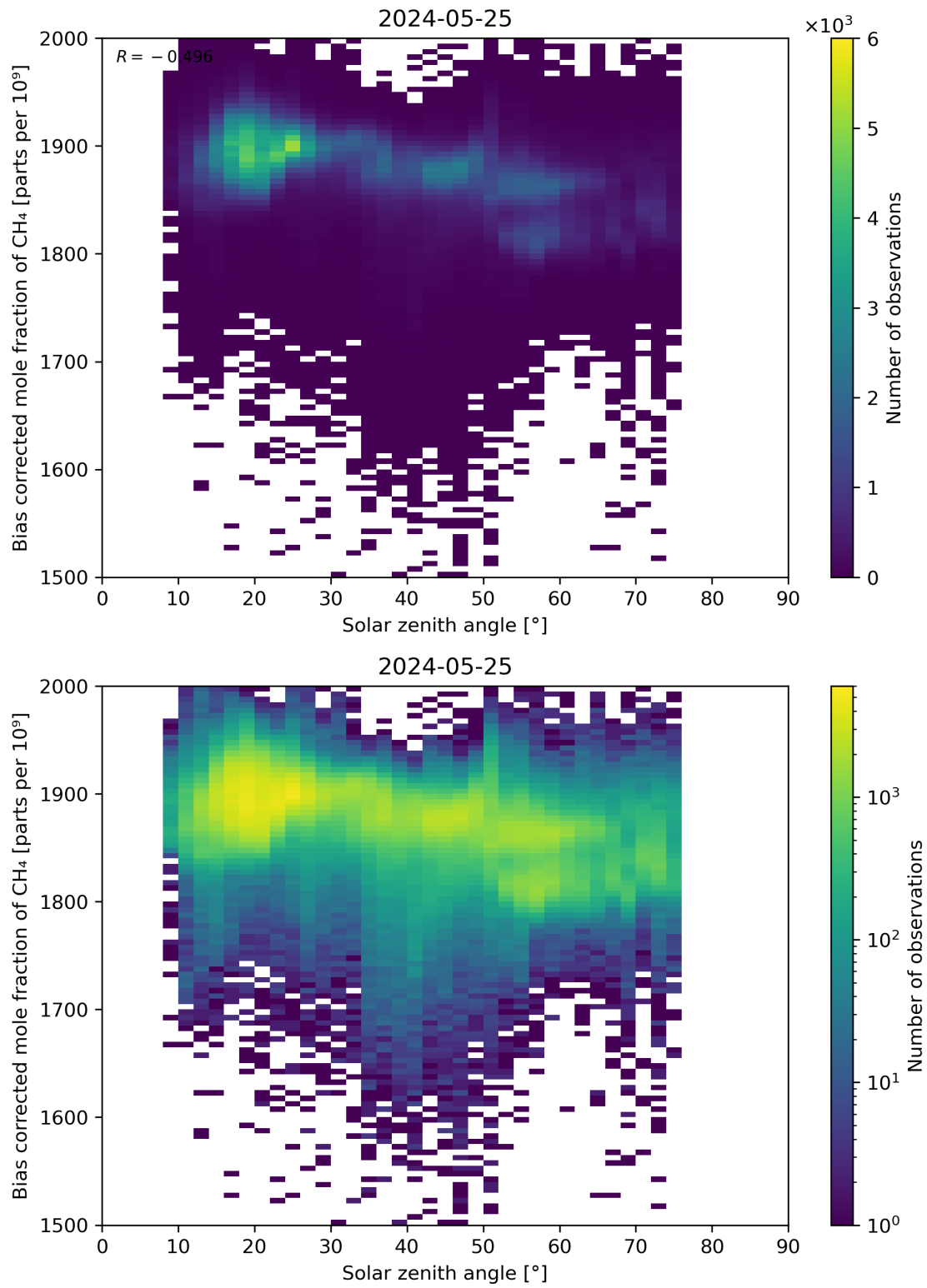
Figure 100: Scatter density plot of “Solar zenith angle” against “Bias corrected mole fraction of \text{CH}_4 ” for 2024-05-24 to 2024-05-26.
