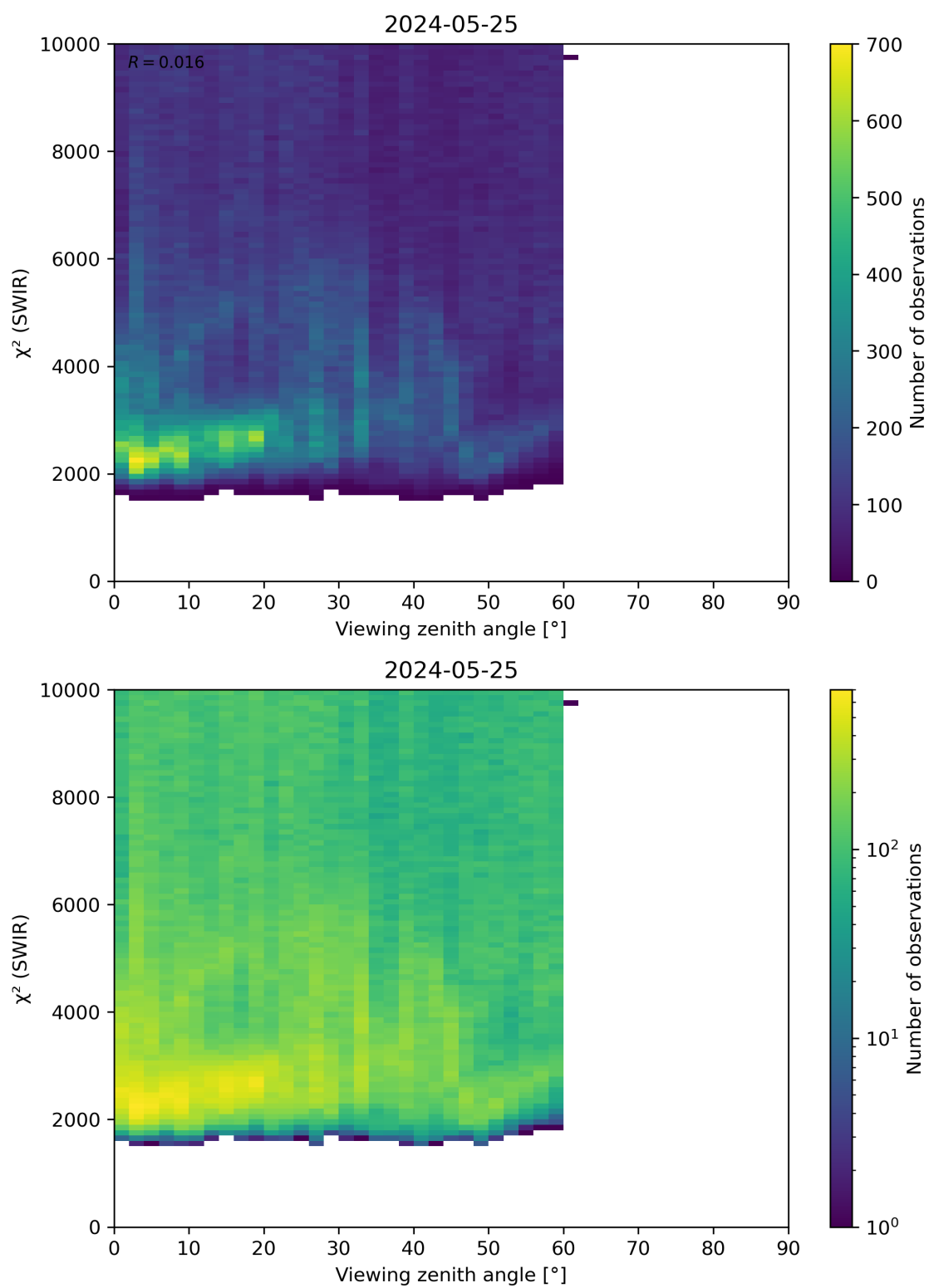
Figure 106: Scatter density plot of “Viewing zenith angle” against “ \chi^2 (SWIR)” for 2024-05-24 to 2024-05-26.
