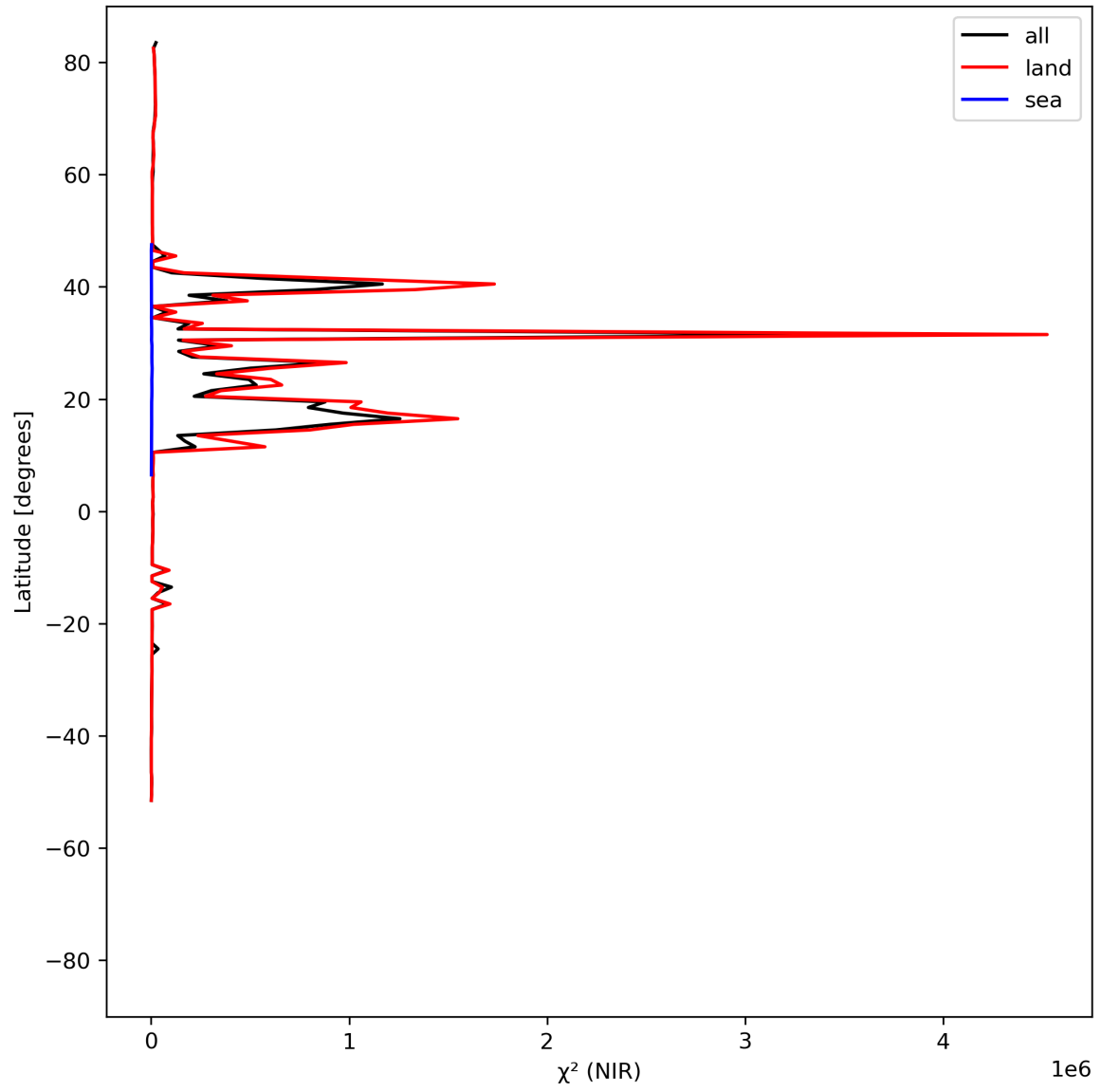
Figure 18: Zonal average of “ \chi^2 (NIR)” for 2024-05-24 to 2024-05-26.
