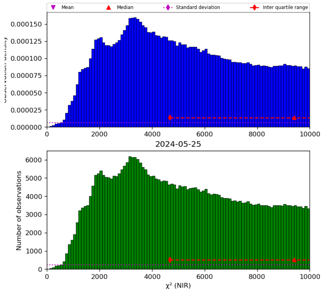
Figure 29: Histogram of “ \chi^2 (NIR)” for 2024-05-24 to 2024-05-26
