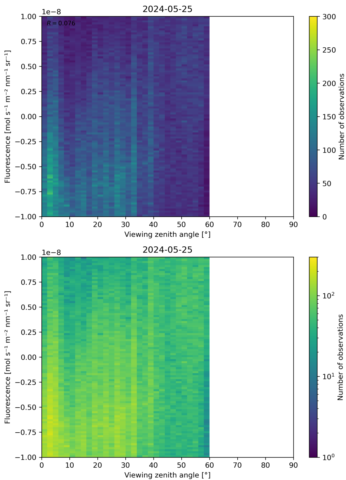
Figure 108: Scatter density plot of “Viewing zenith angle” against “Fluorescence” for 2024-05-24 to 2024-05-26.
