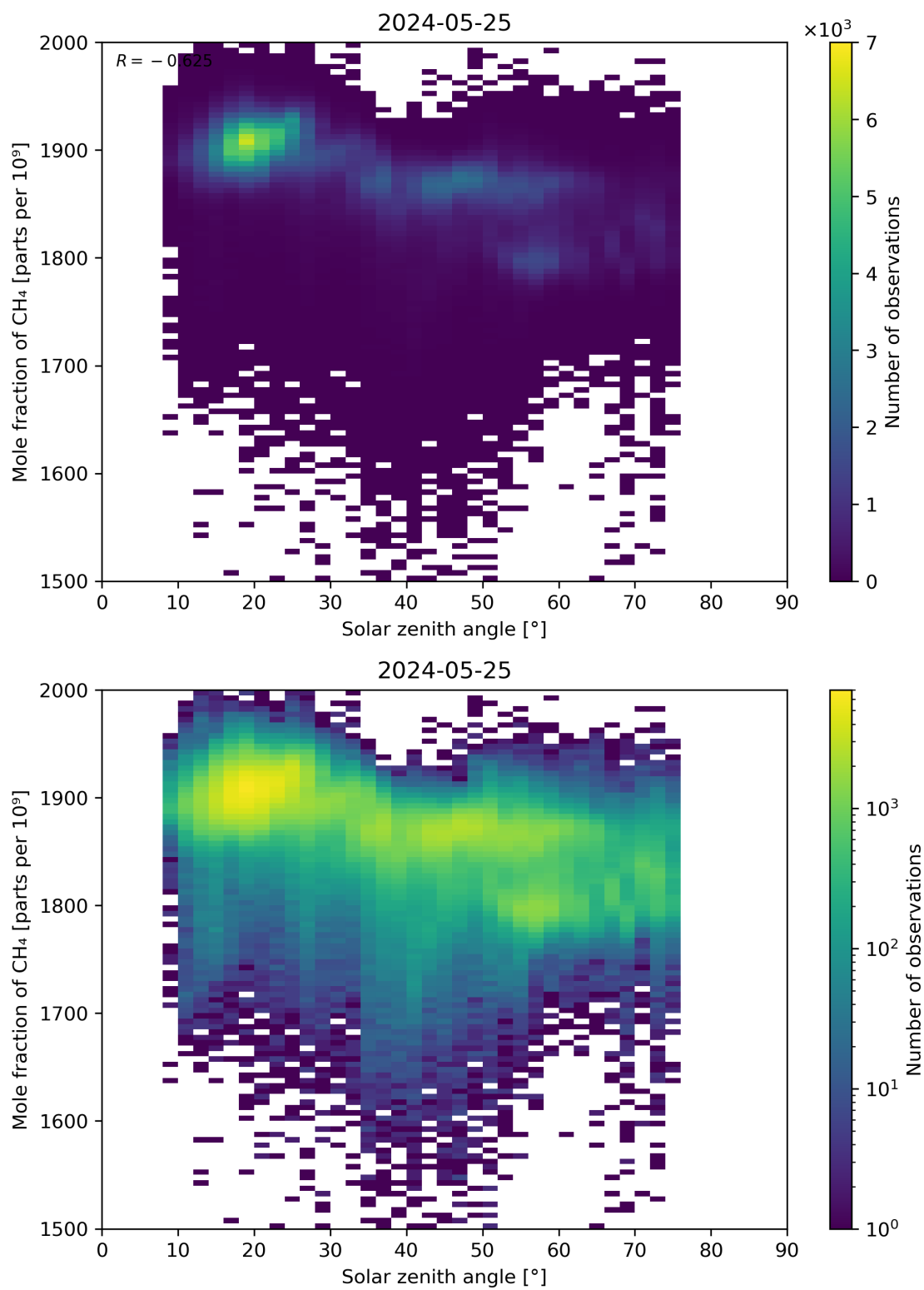
Figure 99: Scatter density plot of “Solar zenith angle” against “Mole fraction of CH 4 ” for 2024-05-24 to 2024-05-26.
