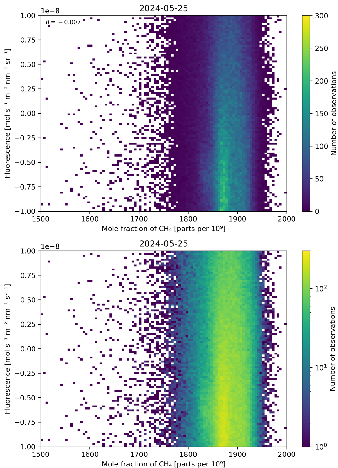
Figure 73: Scatter density plot of “Mole fraction of \text{CH}_4 ” against “Fluorescence” for 2024-05-24 to 2024-05-26.
