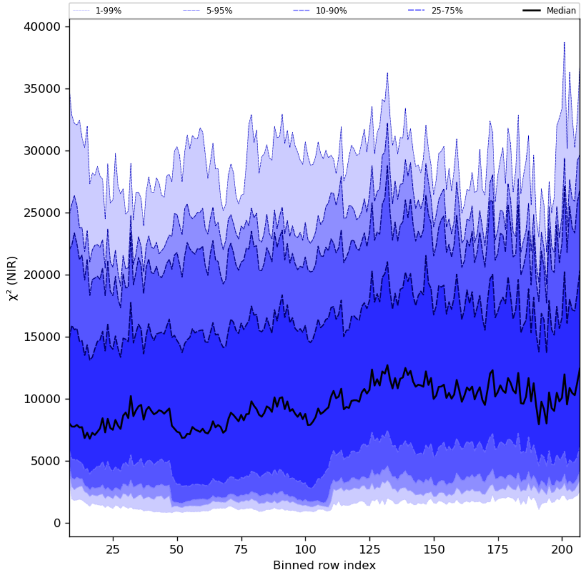
Figure 40: Along track statistics of " \chi^2 (NIR)" for 2024-05-24 to 2024-05-26
