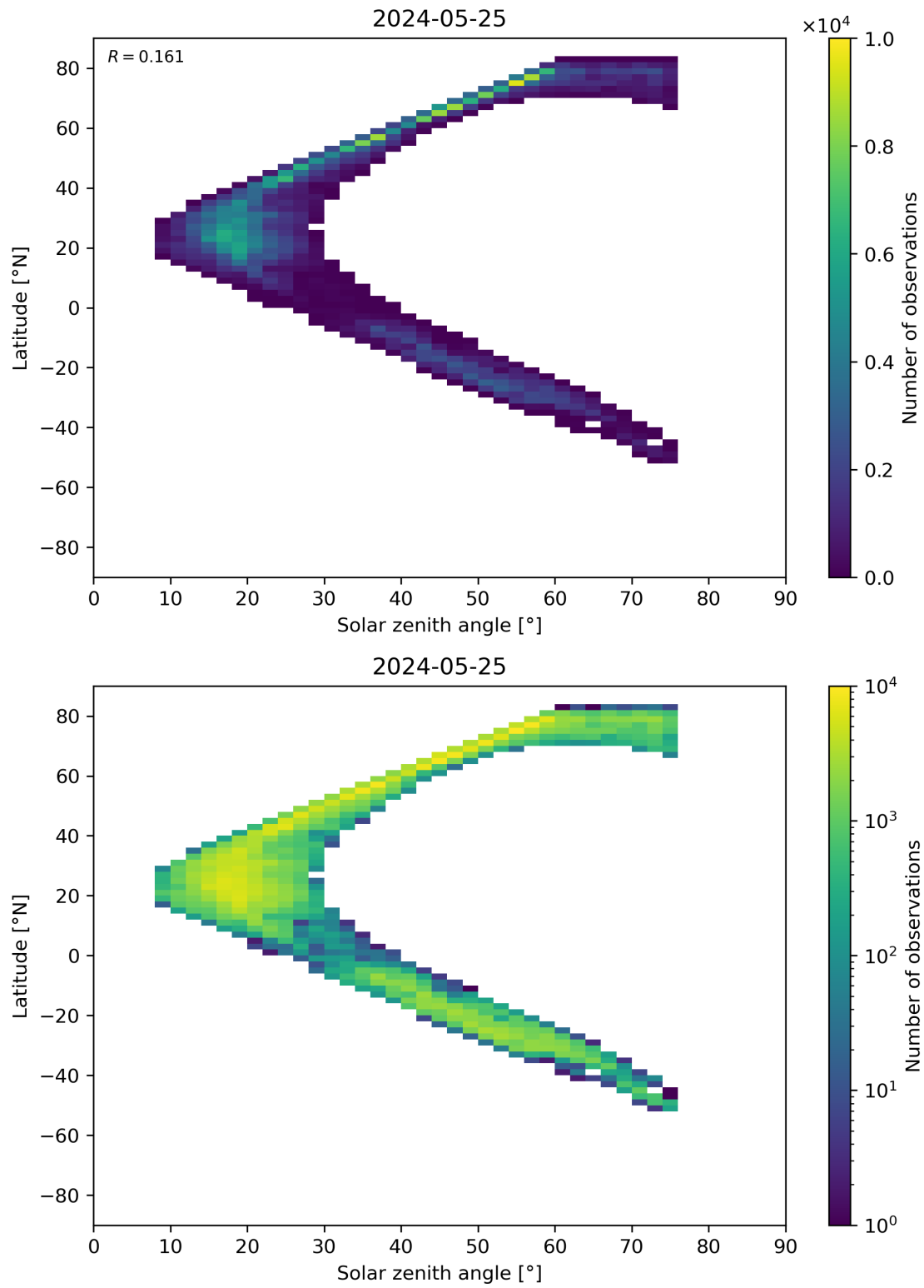
Figure 98: Scatter density plot of “Solar zenith angle” against “Latitude” for 2024-05-24 to 2024-05-26.
