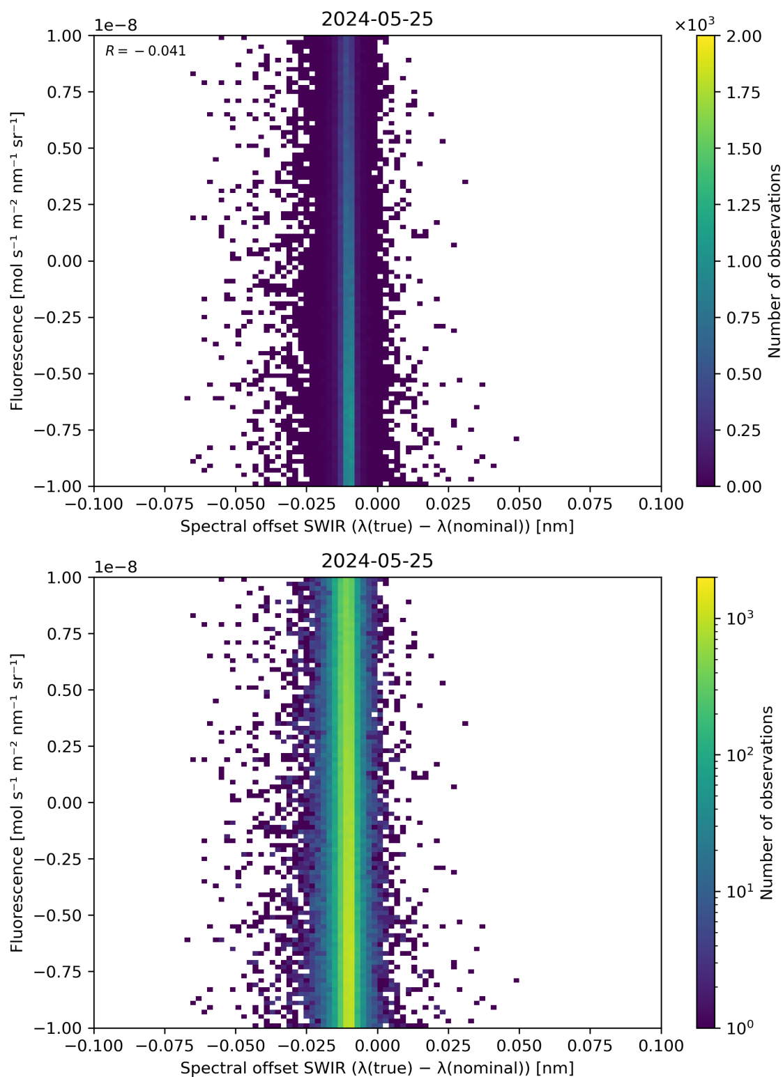
Figure 120: Scatter density plot of “Spectral offset SWIR ( \lambda(\text{true}) - \lambda(\text{nominal}) )” against “Fluorescence” for 2024-05-24 to 2024-05-26.
