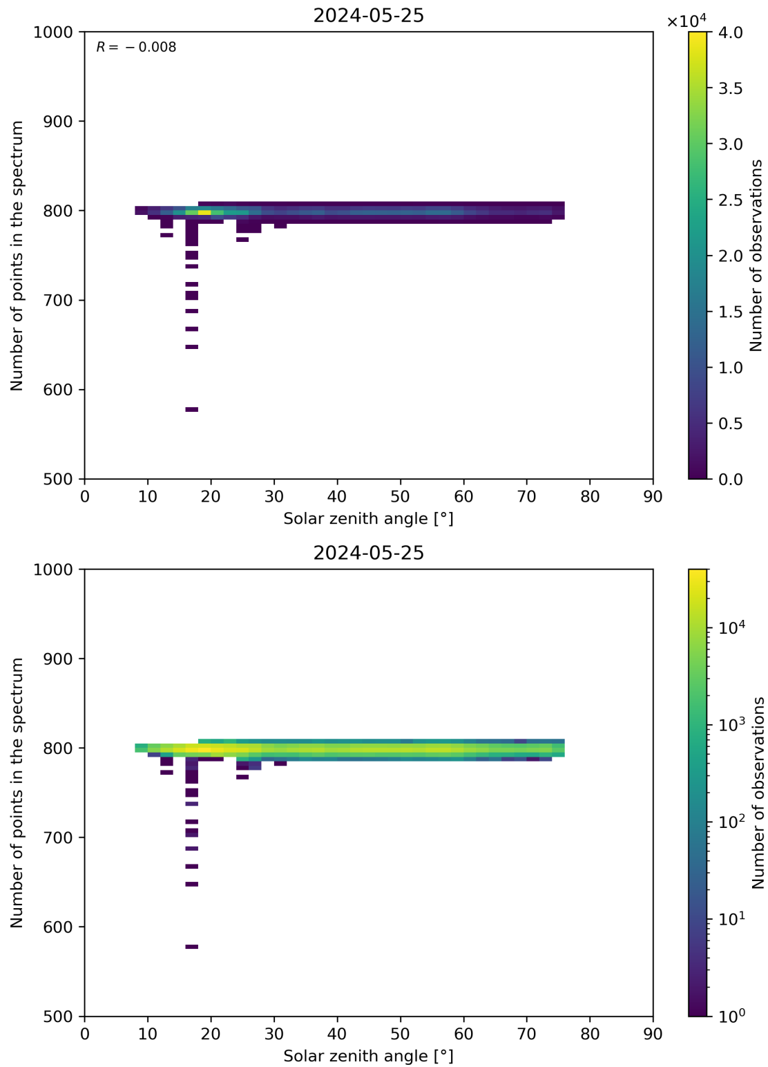
Figure 103: Scatter density plot of “Solar zenith angle” against “Number of points in the spectrum” for 2024-05-24 to 2024-05-26.
