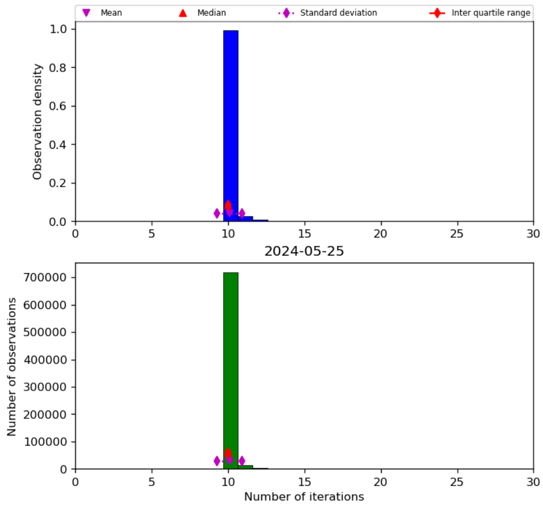
Figure 31: Histogram of “Number of iterations” for 2024-05-24 to 2024-05-26
