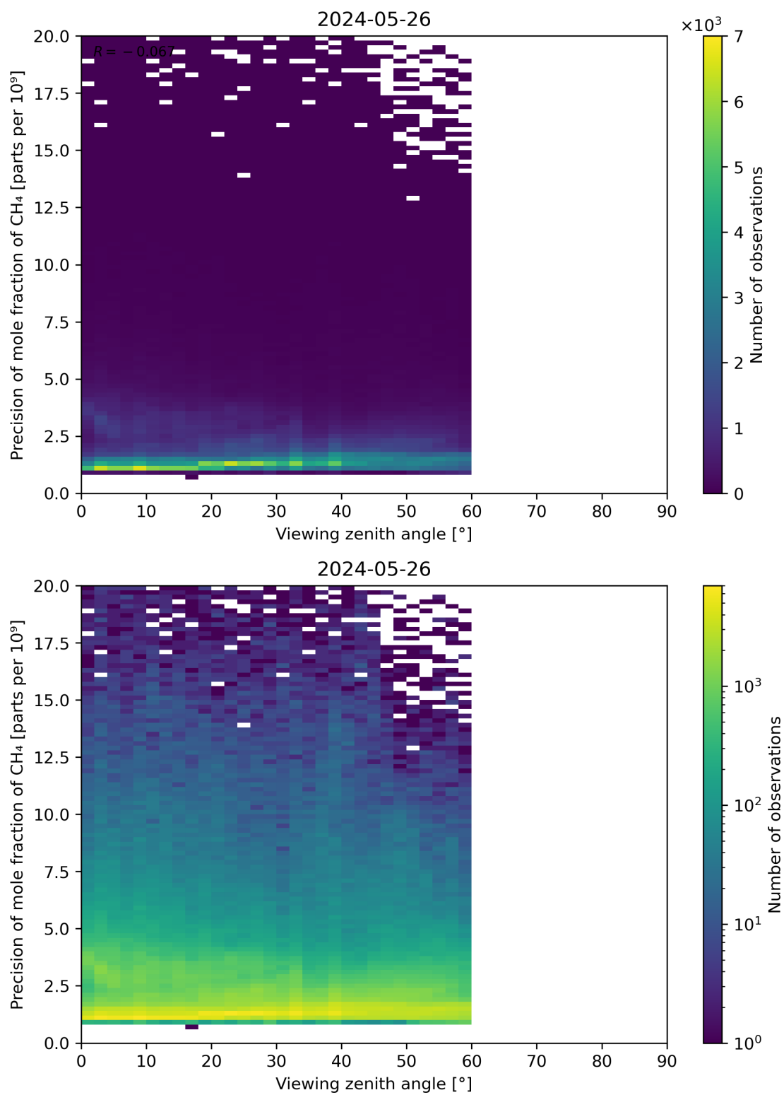
Figure 112: Scatter density plot of “Viewing zenith angle” against “Precision of mole fraction of CH 4 ” for 2024-05-25 to 2024-05-27.
