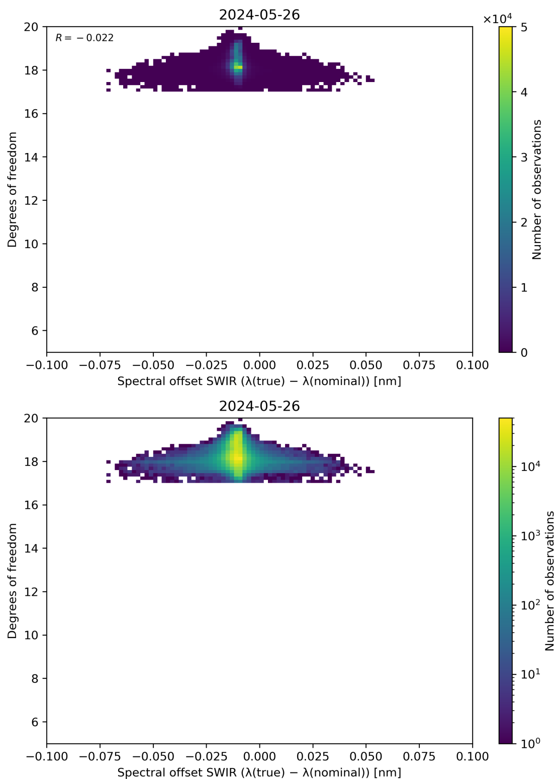
Figure 119: Scatter density plot of “Spectral offset SWIR ( \lambda(\text{true}) - \lambda(\text{nominal}) )” against “Degrees of freedom” for 2024-05-25 to 2024-05-27.
