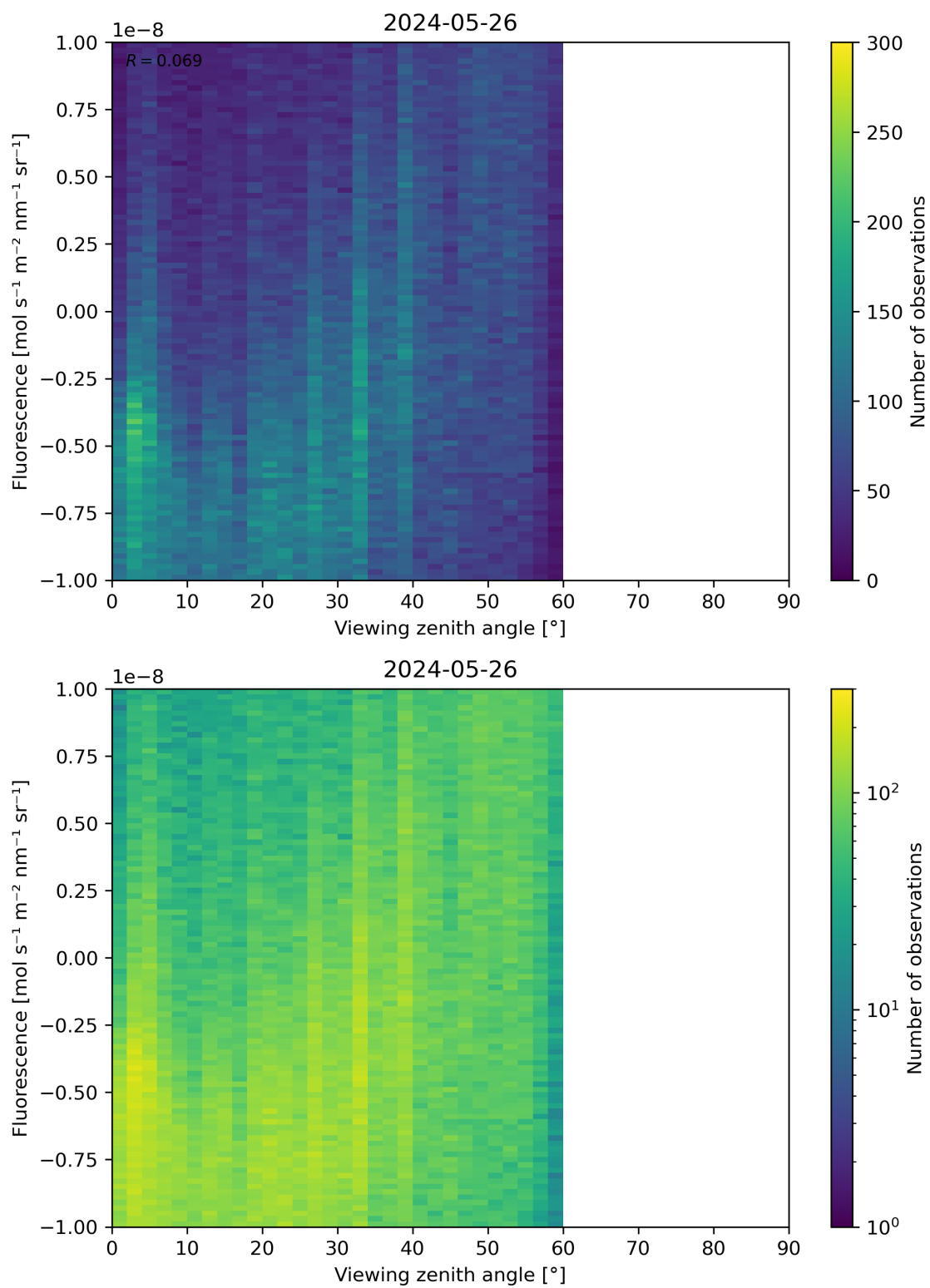
Figure 108: Scatter density plot of “Viewing zenith angle” against “Fluorescence” for 2024-05-25 to 2024-05-27.
