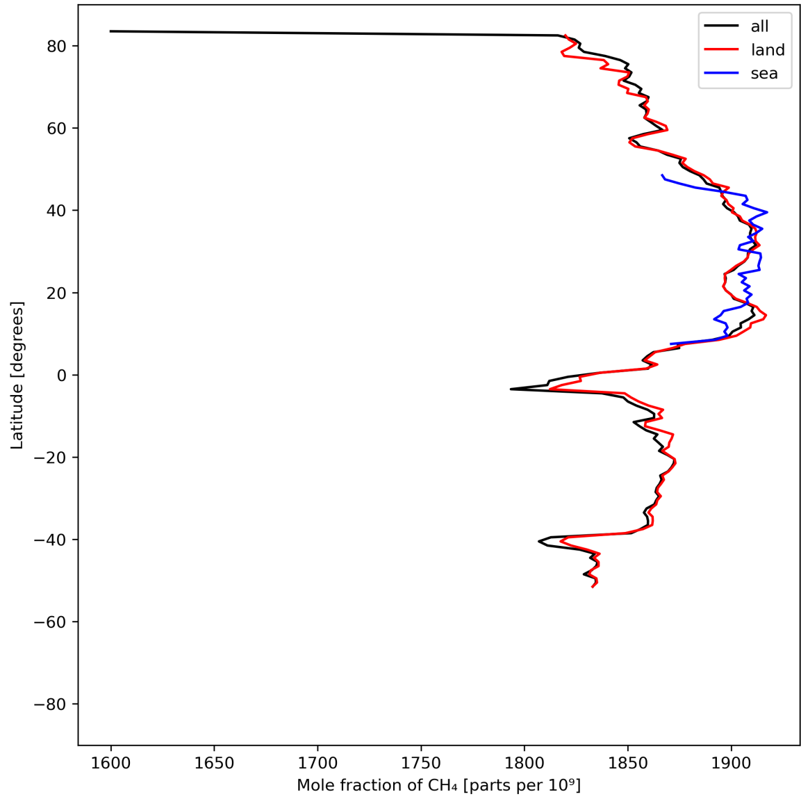
Figure 12: Zonal average of “Mole fraction of \text{CH}_4 ” for 2024-05-25 to 2024-05-27.
