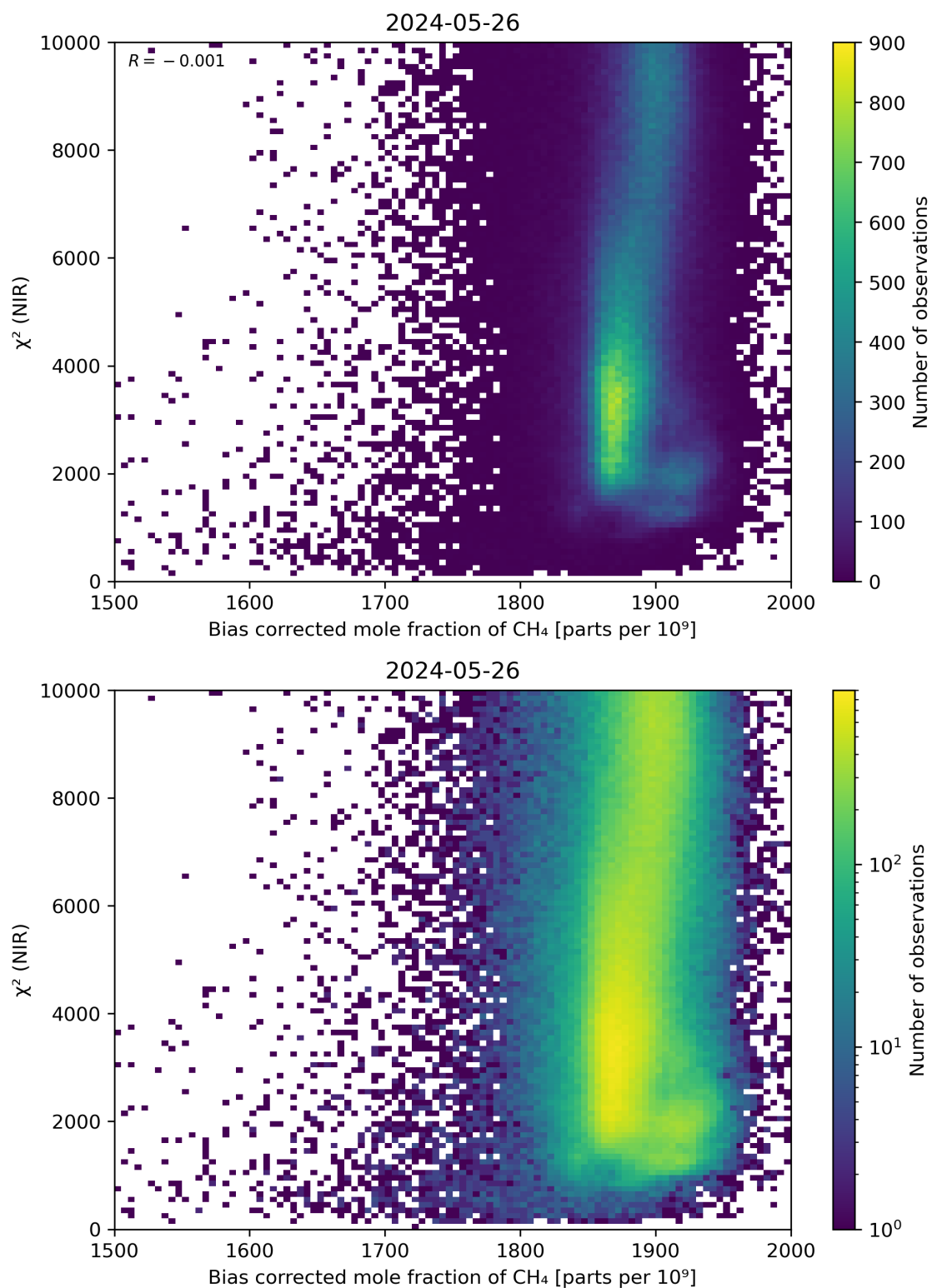
Figure 63: Scatter density plot of “Bias corrected mole fraction of CH 4 ” against “ \chi^2 (NIR)” for 2024-05-25 to 2024-05-27.
