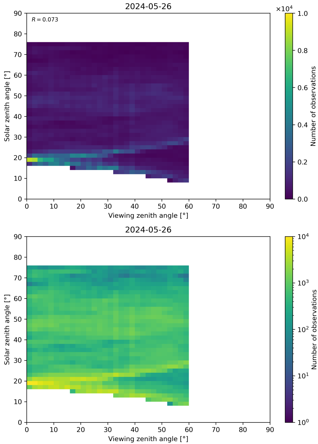
Figure 115: Scatter density plot of “Viewing zenith angle” against “Solar zenith angle” for 2024-05-25 to 2024-05-27.
