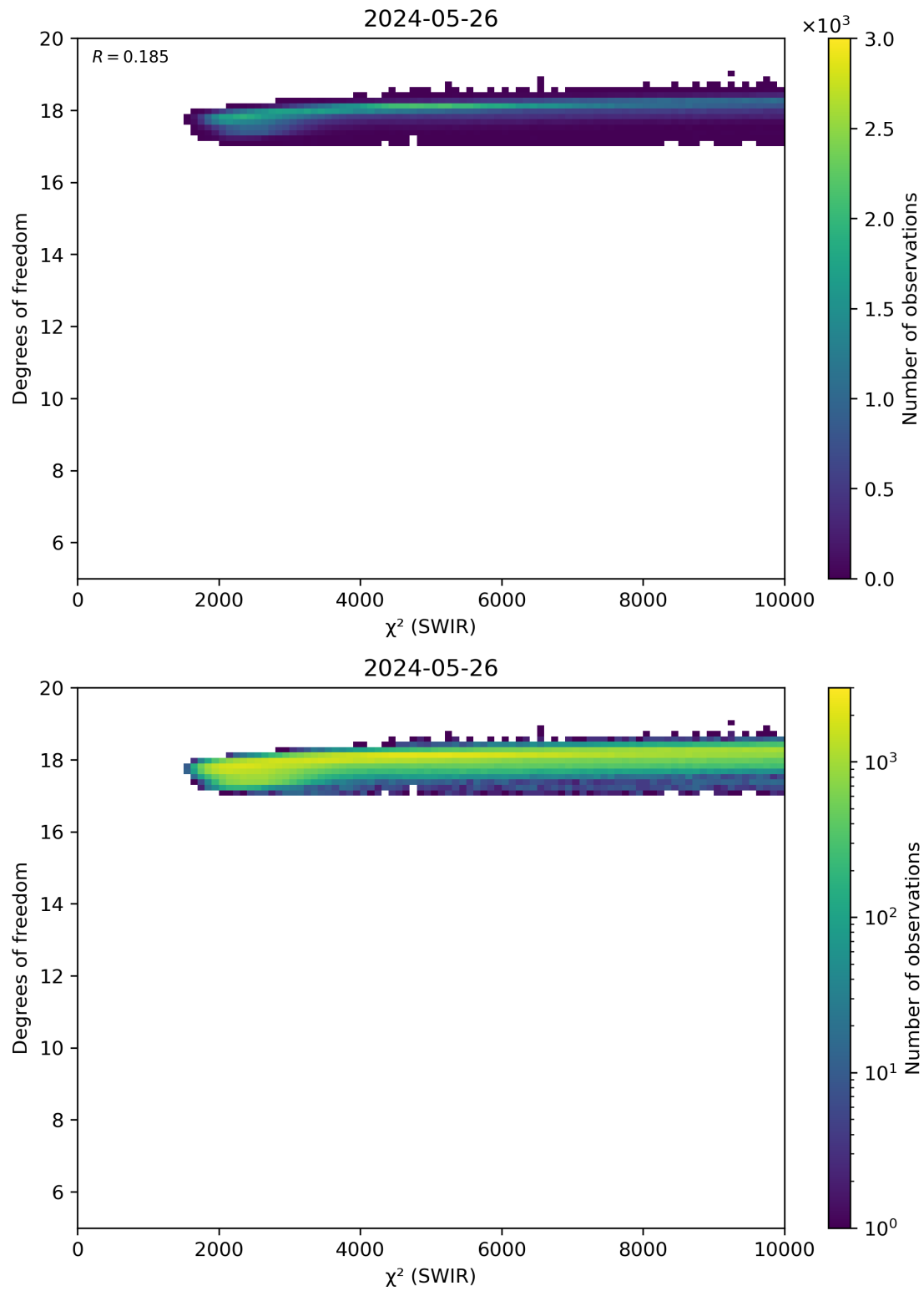
Figure 48: Scatter density plot of “ \chi^2 (SWIR)” against “Degrees of freedom” for 2024-05-25 to 2024-05-27.
