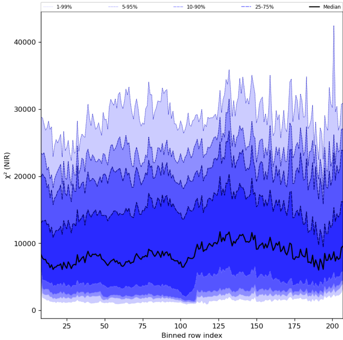
Figure 40: Along track statistics of “ \chi^2 (NIR)” for 2024-05-25 to 2024-05-27
