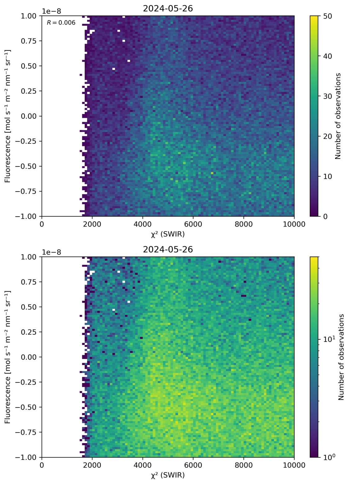
Figure 49: Scatter density plot of “ \chi^2 (SWIR)” against “Fluorescence” for 2024-05-25 to 2024-05-27.
