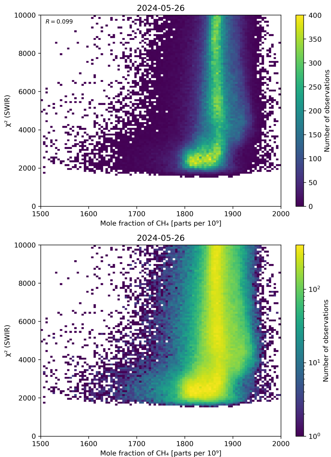
Figure 71: Scatter density plot of “Mole fraction of \text{CH}_4 ” against “ \chi^2 (SWIR)” for 2024-05-25 to 2024-05-27.
