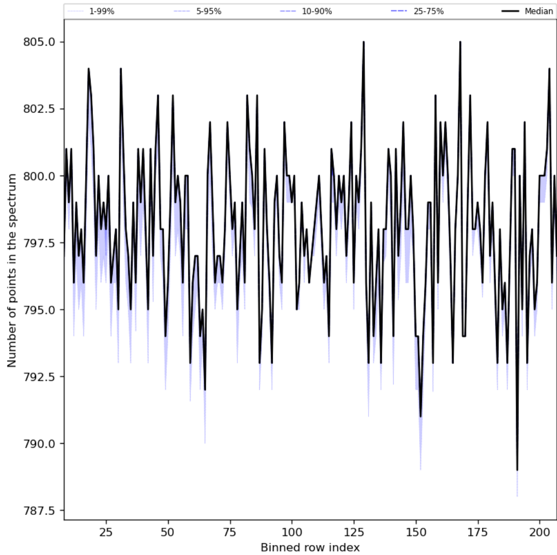
Figure 37: Along track statistics of “Number of points in the spectrum” for 2024-05-25 to 2024-05-27
