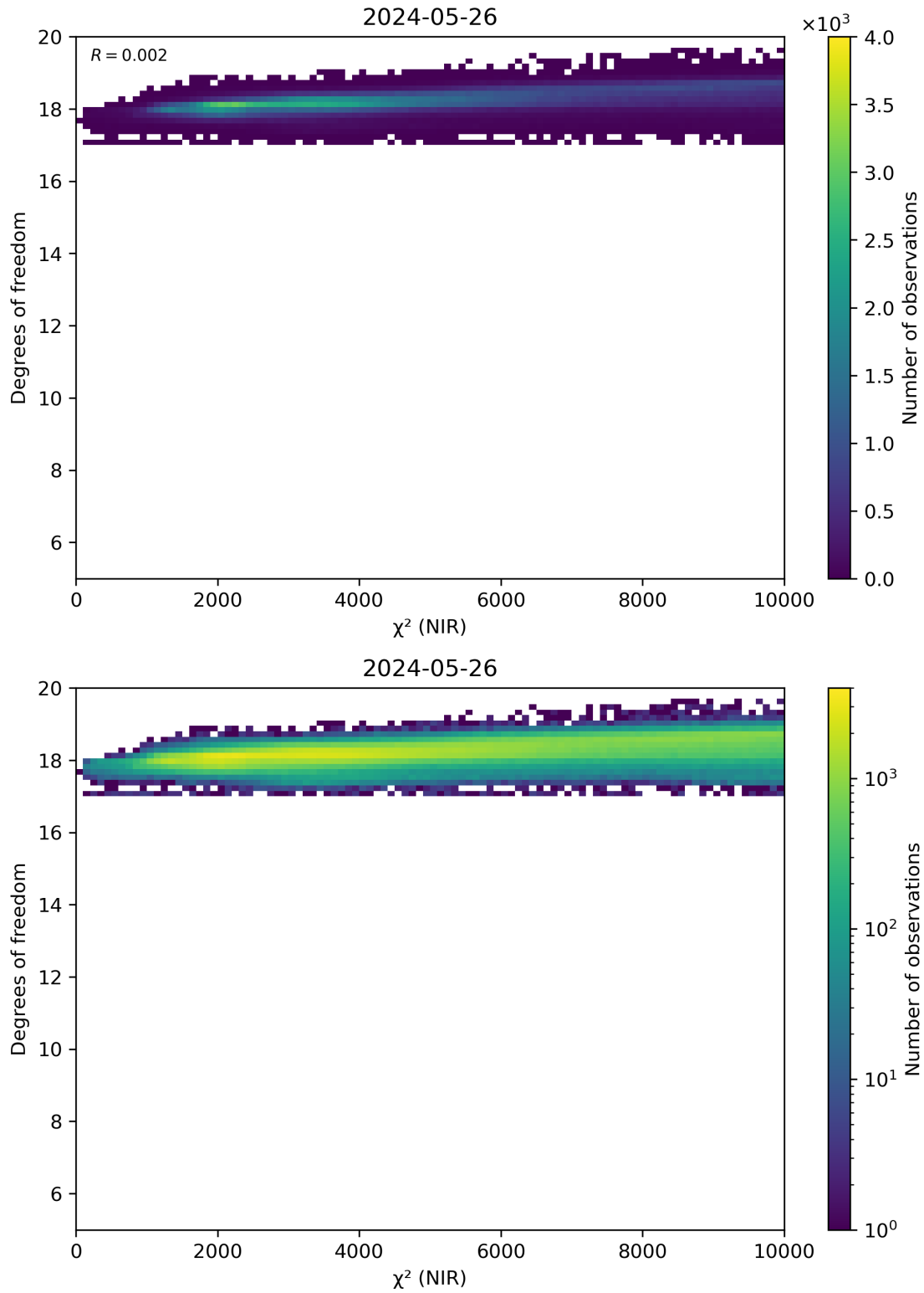
Figure 44: Scatter density plot of “ \chi^2 (NIR)” against “Degrees of freedom” for 2024-05-25 to 2024-05-27.
