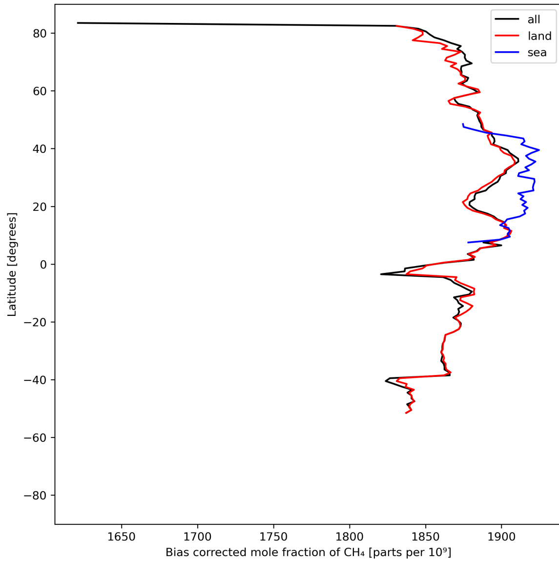
Figure 14: Zonal average of “Bias corrected mole fraction of \text{CH}_4 ” for 2024-05-25 to 2024-05-27.
