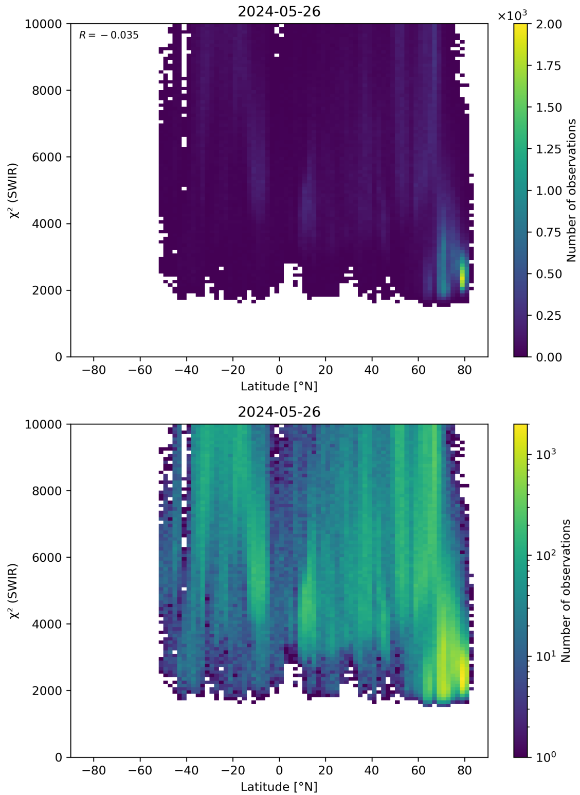
Figure 54: Scatter density plot of “Latitude” against “ \chi^2 (SWIR)” for 2024-05-25 to 2024-05-27.
