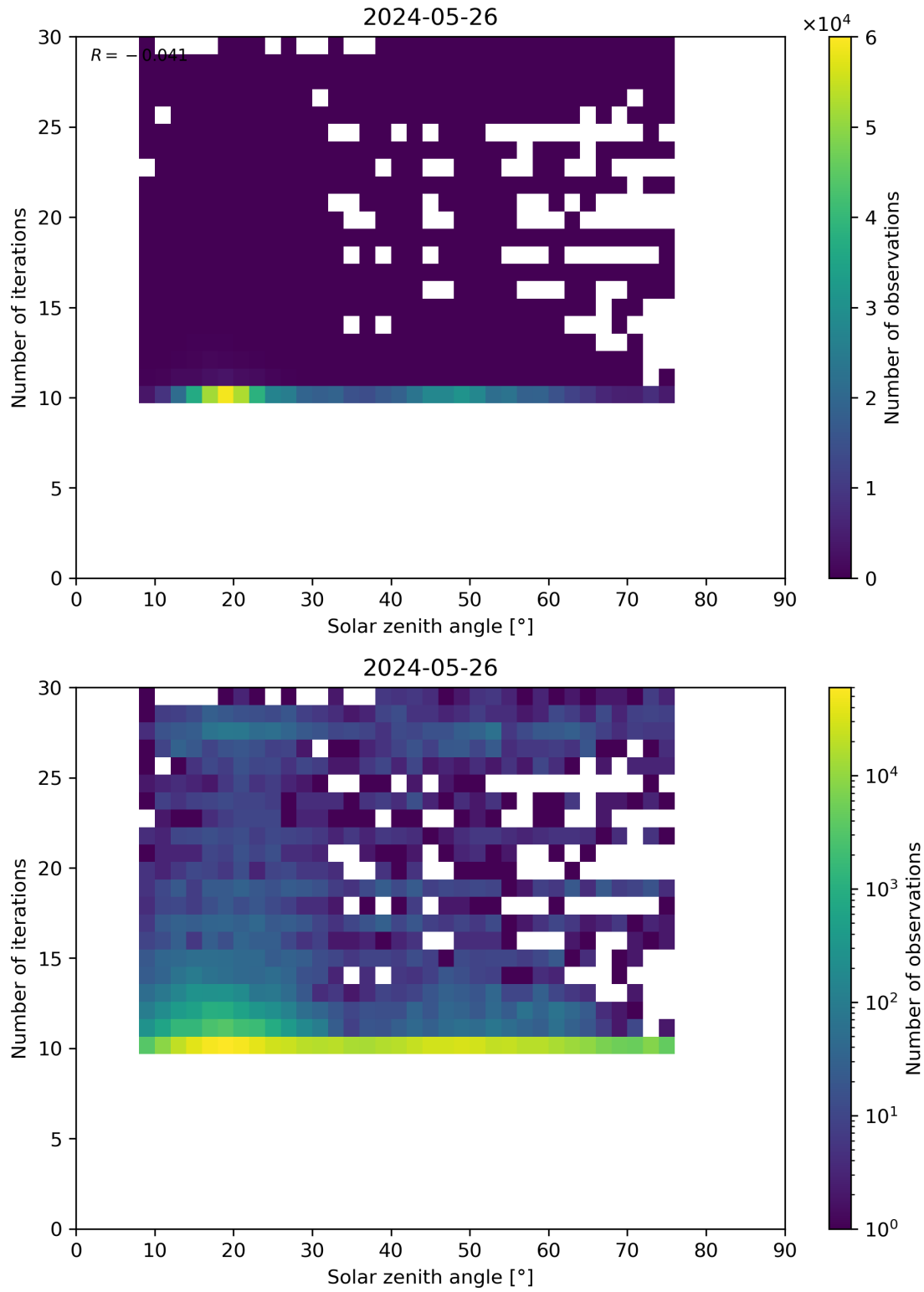
Figure 102: Scatter density plot of “Solar zenith angle” against “Number of iterations” for 2024-05-25 to 2024-05-27.
