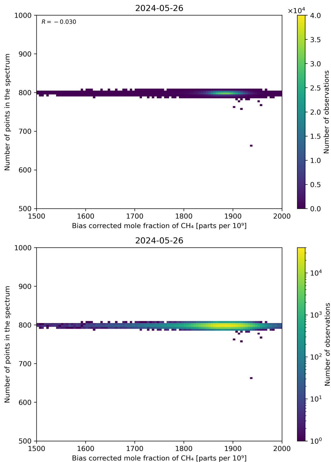
Figure 68: Scatter density plot of “Bias corrected mole fraction of CH 4 ” against “Number of points in the spectrum” for 2024-05-25 to 2024-05-27.
