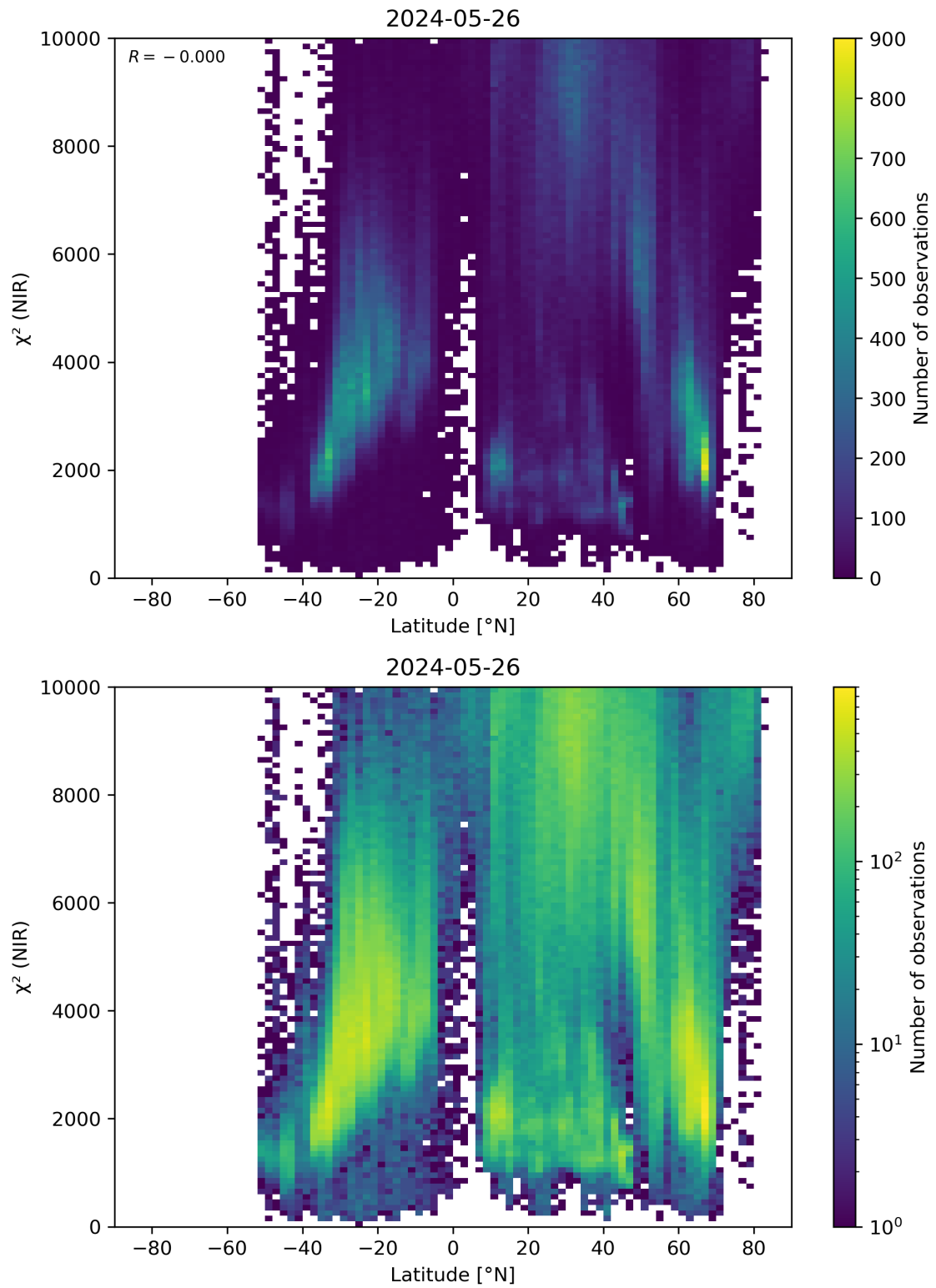
Figure 53: Scatter density plot of “Latitude” against “ \chi^2 (NIR)” for 2024-05-25 to 2024-05-27.
