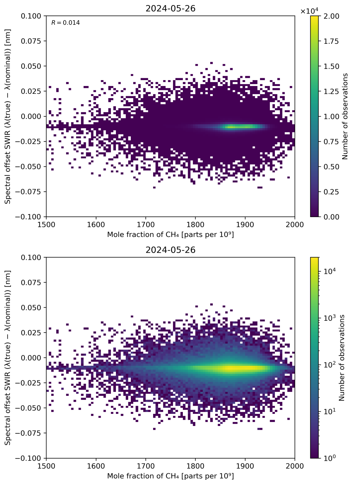
Figure 86: Scatter density plot of “Mole fraction of CH 4 ” against “Spectral offset SWIR ( \lambda(\text{true}) - \lambda(\text{nominal}) )” for 2024-05-25 to 2024-05-27.
