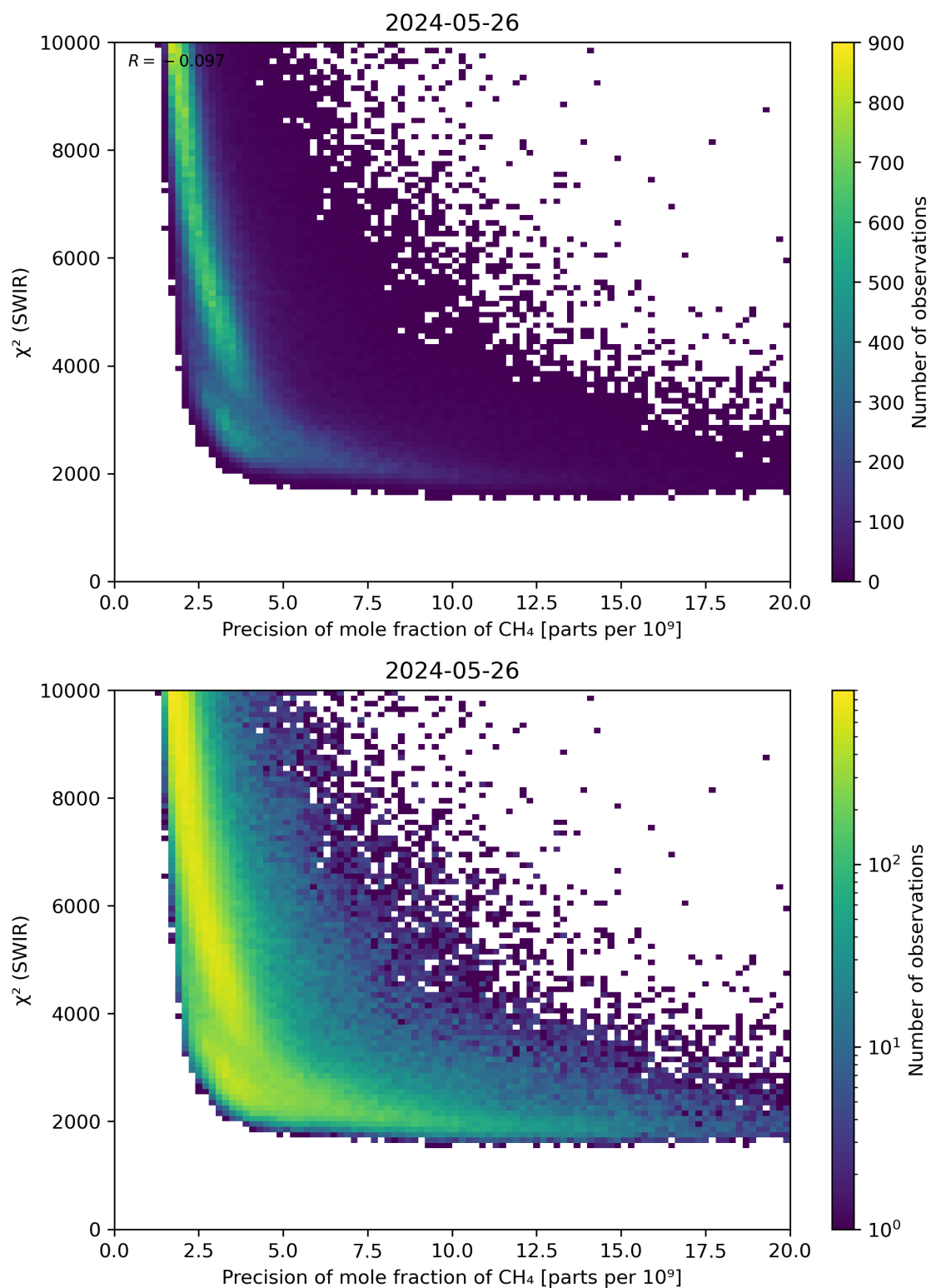
Figure 79: Scatter density plot of “Precision of mole fraction of CH 4 ” against “ \chi^2 (SWIR)” for 2024-05-25 to 2024-05-27.
