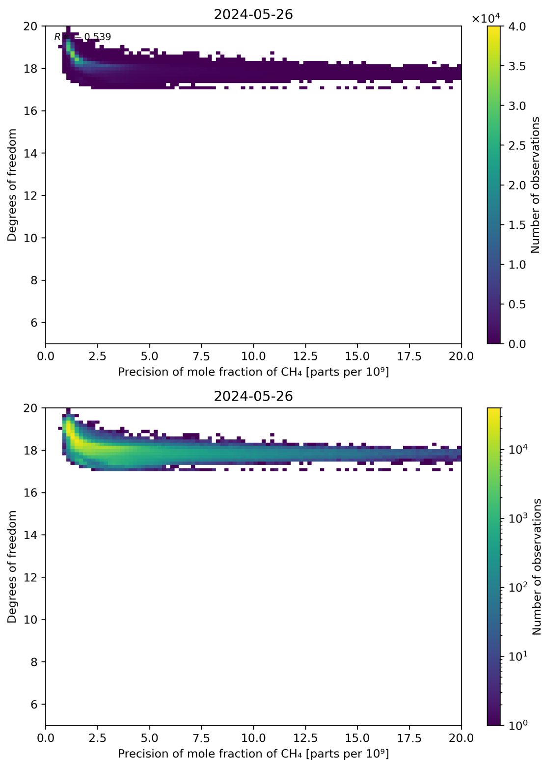
Figure 80: Scatter density plot of “Precision of mole fraction of CH 4 ” against “Degrees of freedom” for 2024-05-25 to 2024-05-27.
