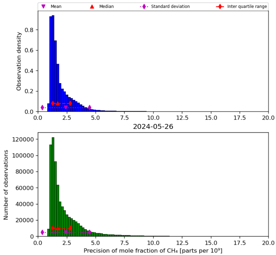
Figure 24: Histogram of “Precision of mole fraction of CH 4 ” for 2024-05-25 to 2024-05-27
