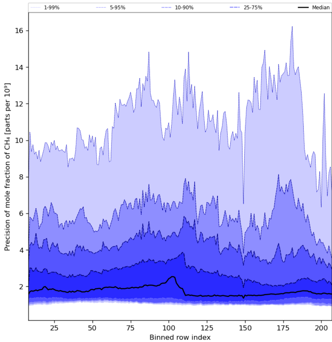
Figure 35: Along track statistics of “Precision of mole fraction of CH 4 ” for 2024-05-25 to 2024-05-27
