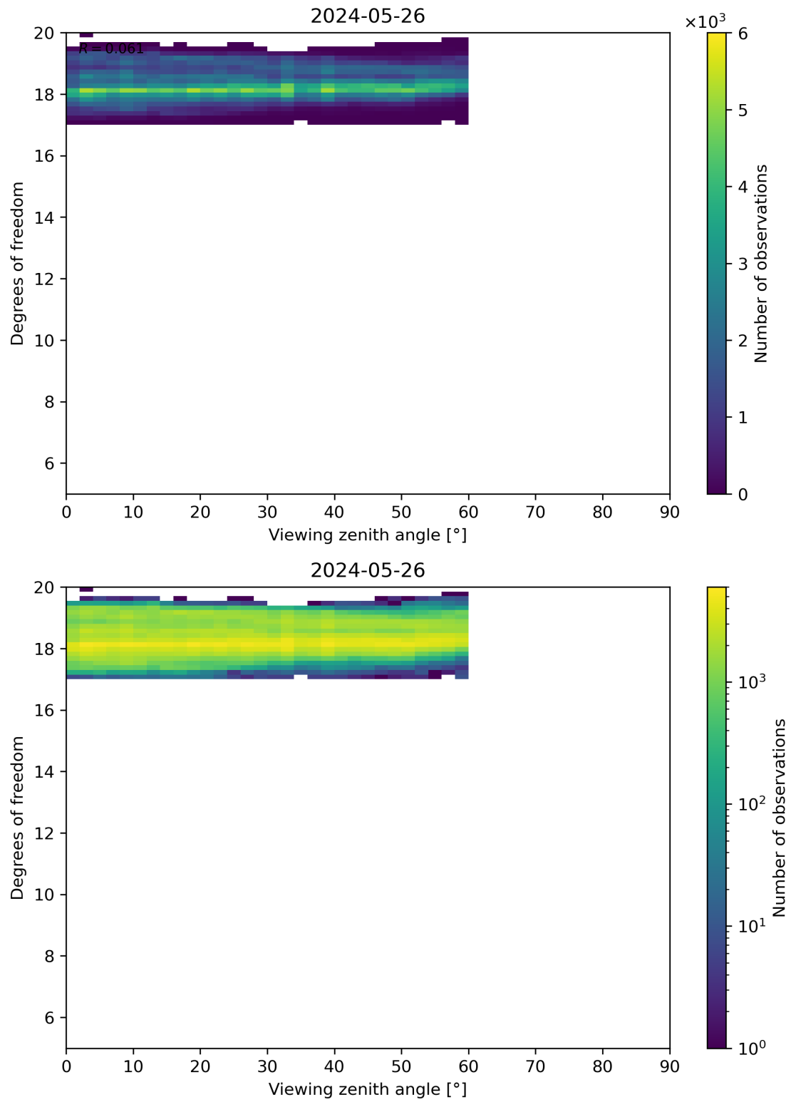
Figure 107: Scatter density plot of “Viewing zenith angle” against “Degrees of freedom” for 2024-05-25 to 2024-05-27.
