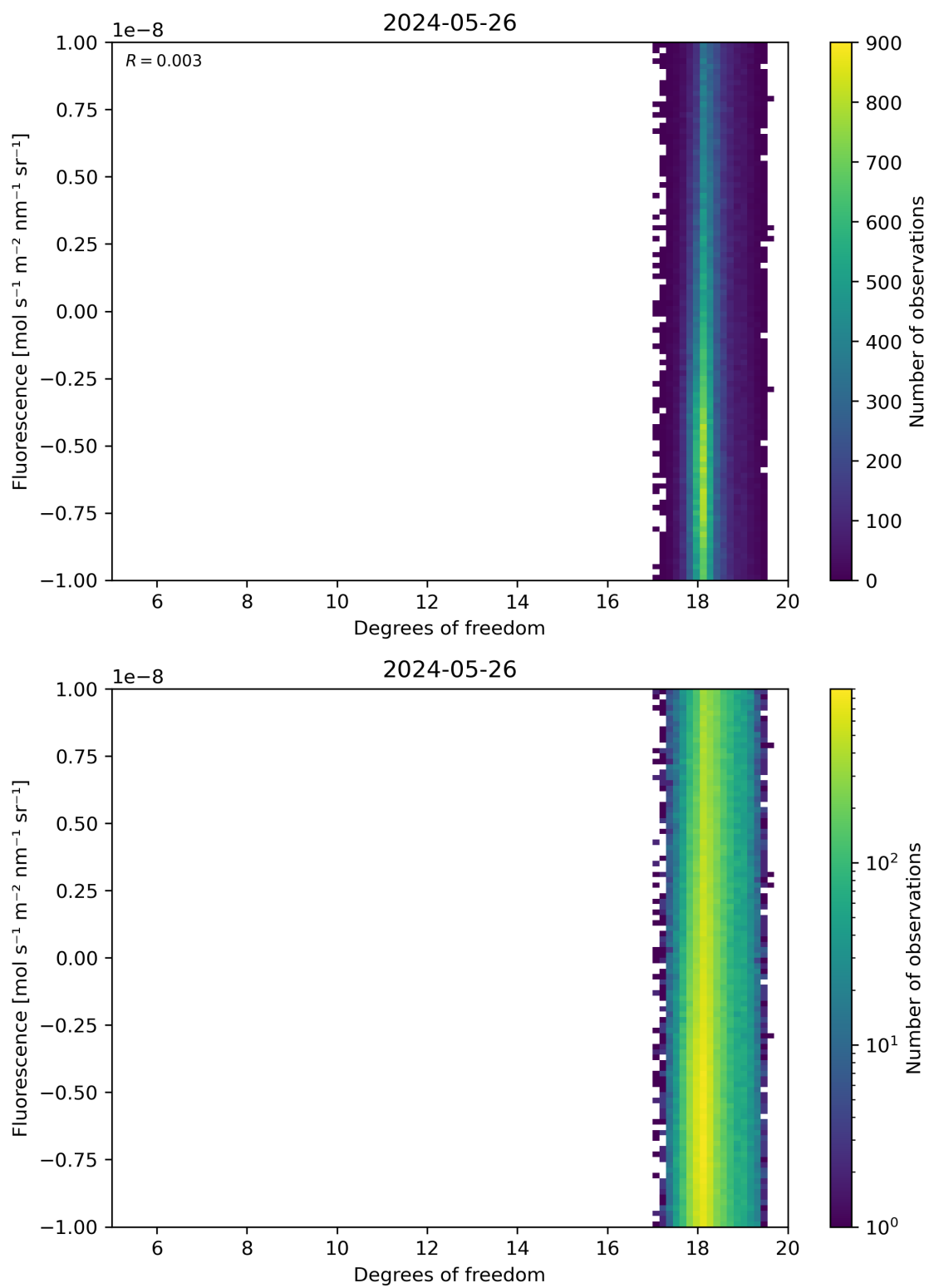
Figure 51: Scatter density plot of “Degrees of freedom” against “Fluorescence” for 2024-05-25 to 2024-05-27.
