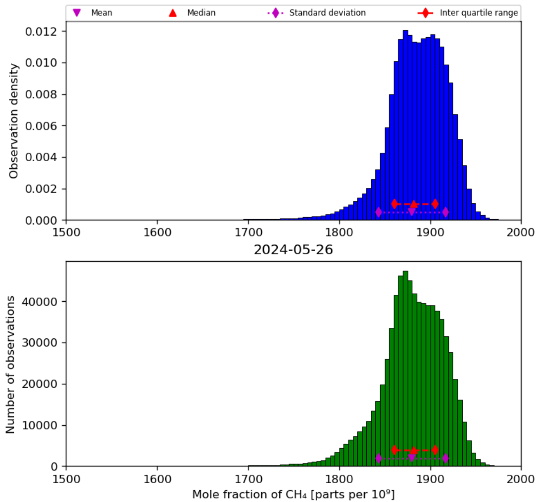
Figure 23: Histogram of “Mole fraction of CH 4 ” for 2024-05-25 to 2024-05-27
