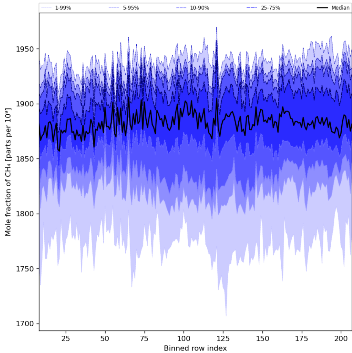
Figure 34: Along track statistics of “Mole fraction of CH 4 ” for 2024-05-25 to 2024-05-27
