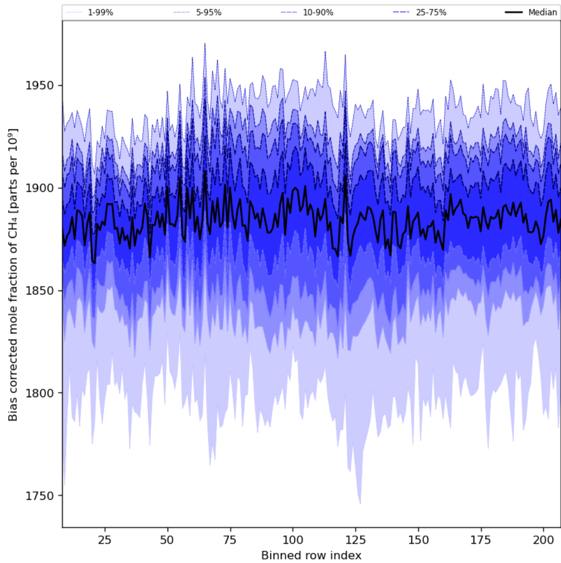
Figure 36: Along track statistics of “Bias corrected mole fraction of CH 4 ” for 2024-05-25 to 2024-05-27
