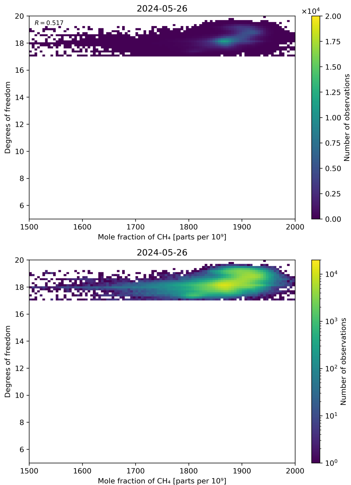
Figure 72: Scatter density plot of “Mole fraction of CH 4 ” against “Degrees of freedom” for 2024-05-25 to 2024-05-27.
