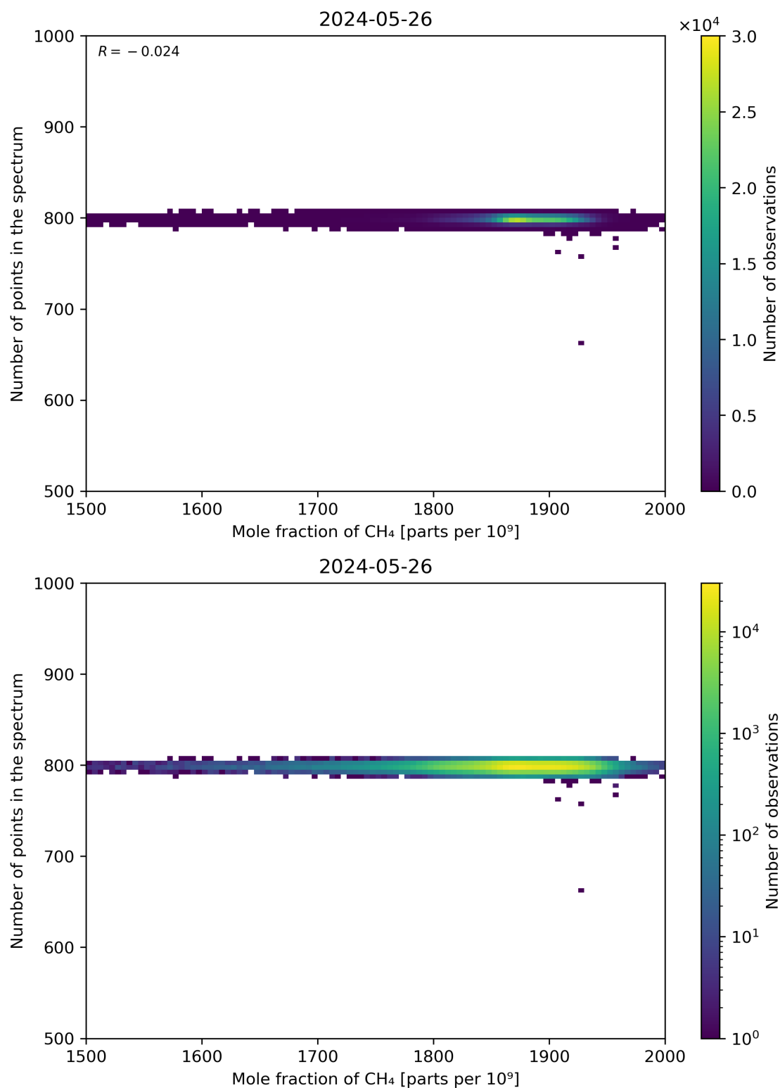
Figure 77: Scatter density plot of “Mole fraction of CH 4 ” against “Number of points in the spectrum” for 2024-05-25 to 2024-05-27.
