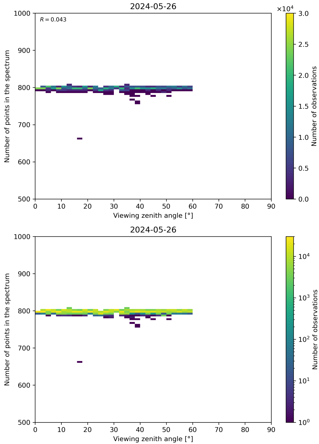
Figure 114: Scatter density plot of “Viewing zenith angle” against “Number of points in the spectrum” for 2024-05-25 to 2024-05-27.
