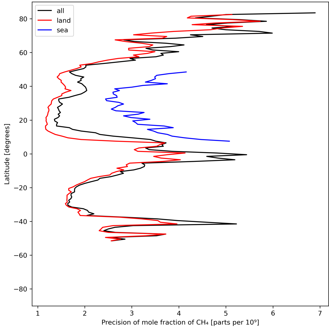
Figure 13: Zonal average of “Precision of mole fraction of CH 4 ” for 2024-05-25 to 2024-05-27.
