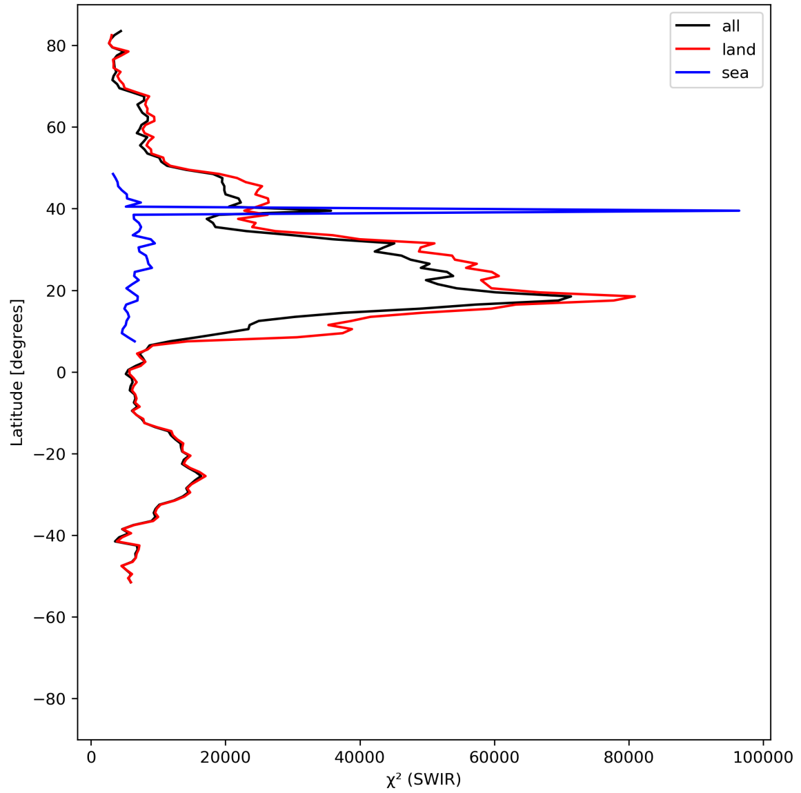
Figure 17: Zonal average of “ \chi^2 (SWIR)” for 2024-05-25 to 2024-05-27.
