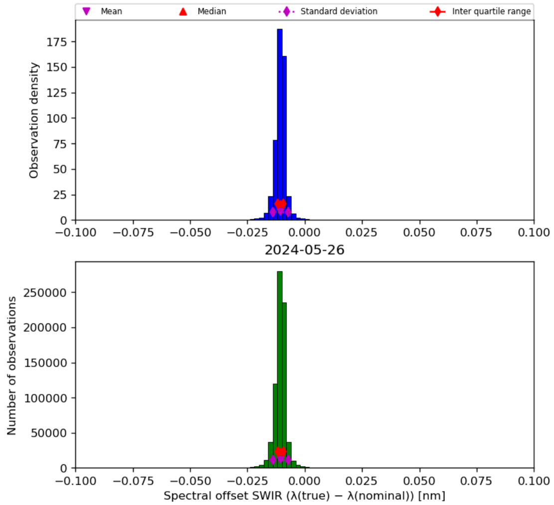
Figure 27: Histogram of “Spectral offset SWIR ( \lambda(\text{true}) - \lambda(\text{nominal}) )” for 2024-05-25 to 2024-05-27
