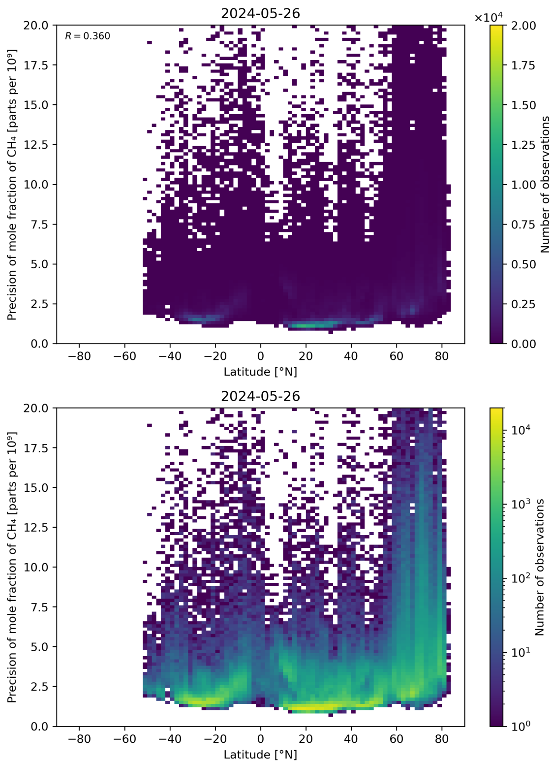
Figure 59: Scatter density plot of “Latitude” against “Precision of mole fraction of \text{CH}_4 ” for 2024-05-25 to 2024-05-27.
