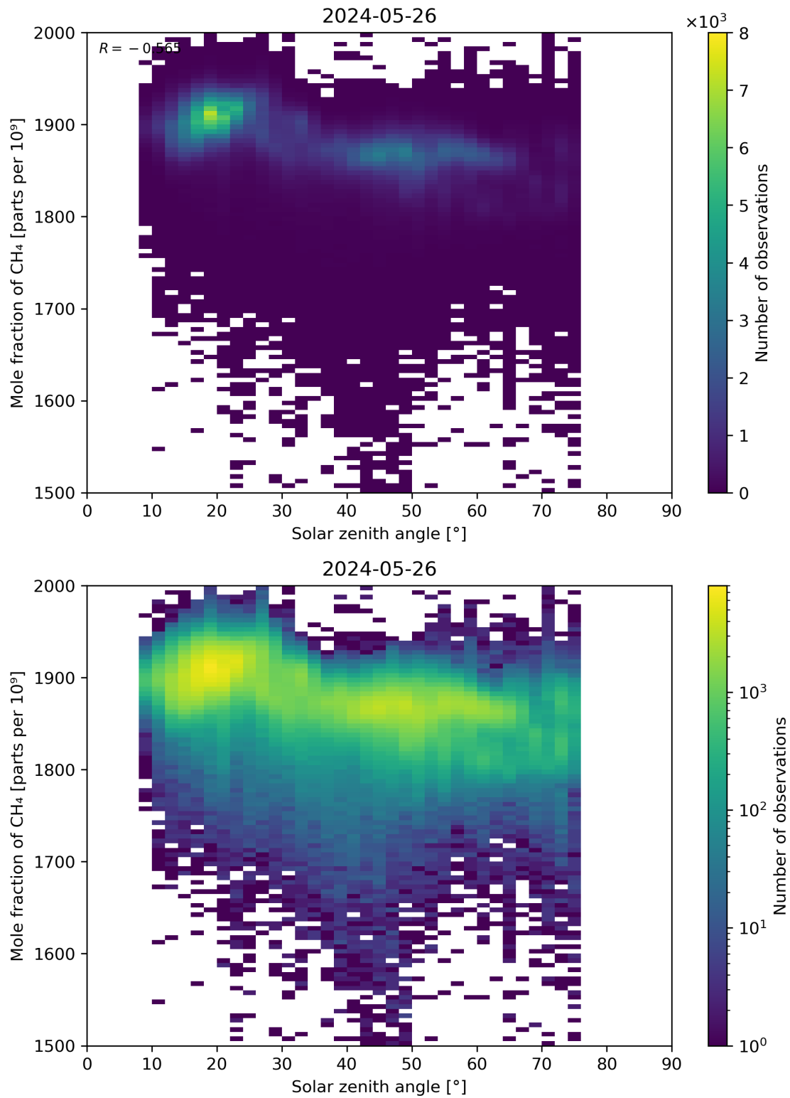
Figure 99: Scatter density plot of “Solar zenith angle” against “Mole fraction of \text{CH}_4 ” for 2024-05-25 to 2024-05-27.
