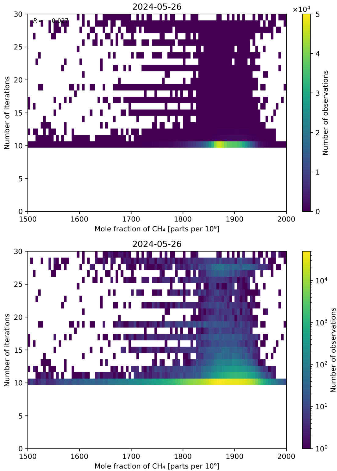
Figure 76: Scatter density plot of “Mole fraction of CH 4 ” against “Number of iterations” for 2024-05-25 to 2024-05-27.
