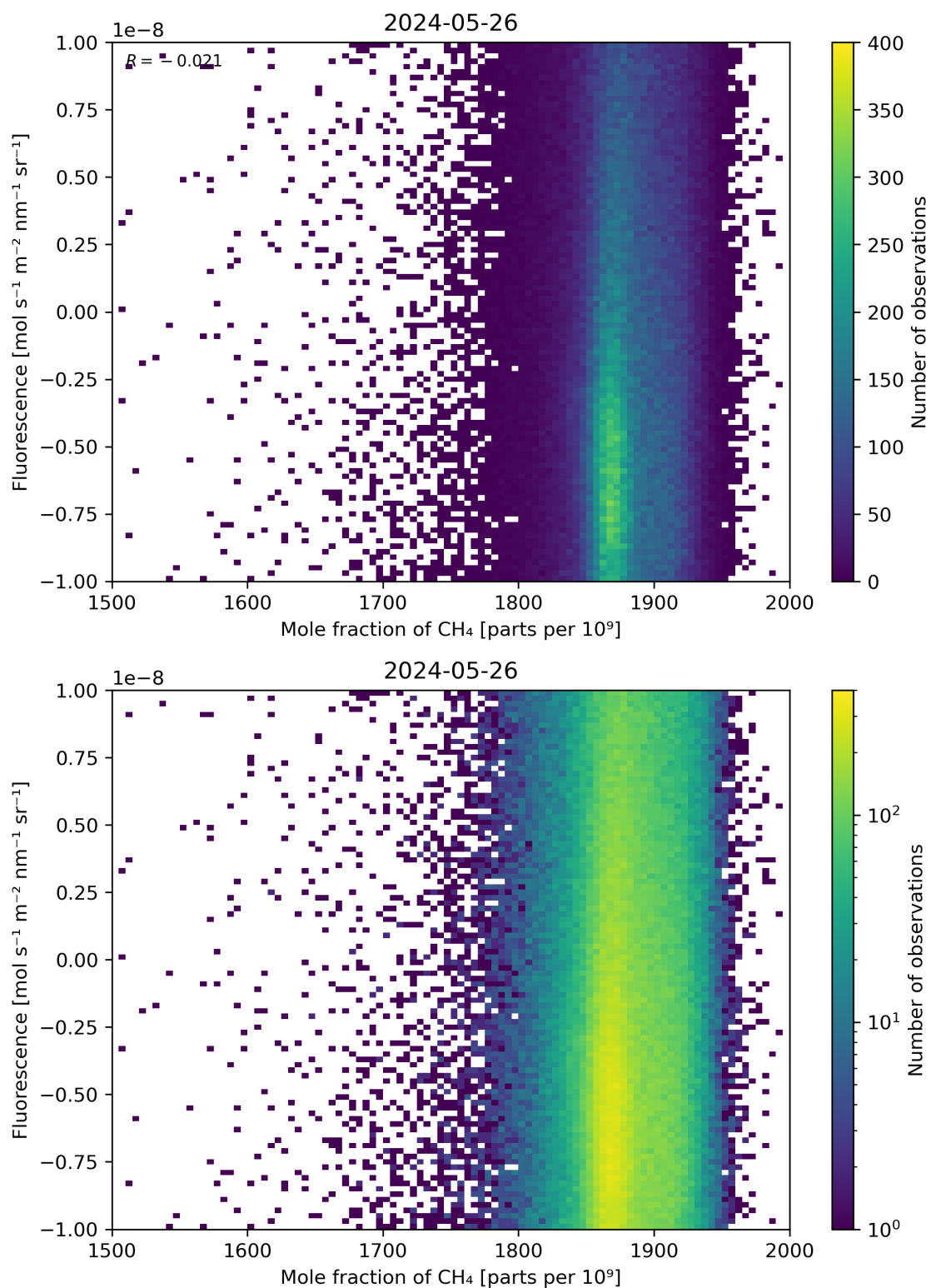
Figure 73: Scatter density plot of “Mole fraction of \text{CH}_4 ” against “Fluorescence” for 2024-05-25 to 2024-05-27.
