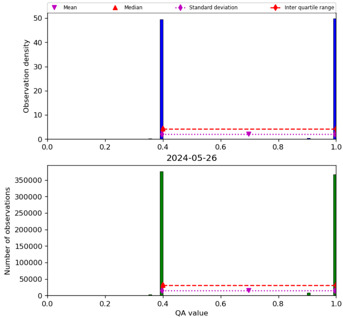
Figure 22: Histogram of “QA value” for 2024-05-25 to 2024-05-27
