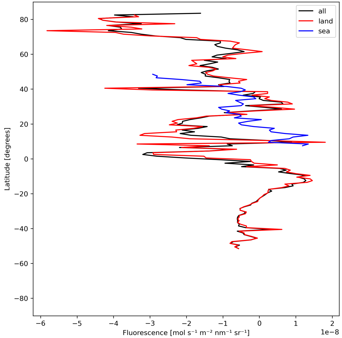
Figure 21: Zonal average of “Fluorescence” for 2024-05-25 to 2024-05-27.
