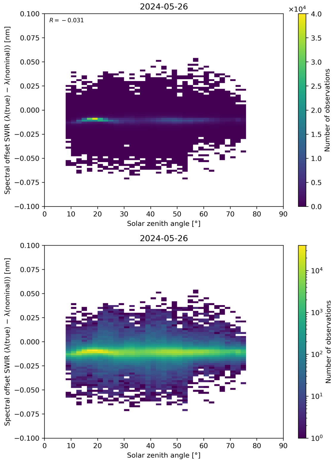
Figure 104: Scatter density plot of “Solar zenith angle” against “Spectral offset SWIR ( \lambda(\text{true}) - \lambda(\text{nominal}) )” for 2024-05-25 to 2024-05-27.
