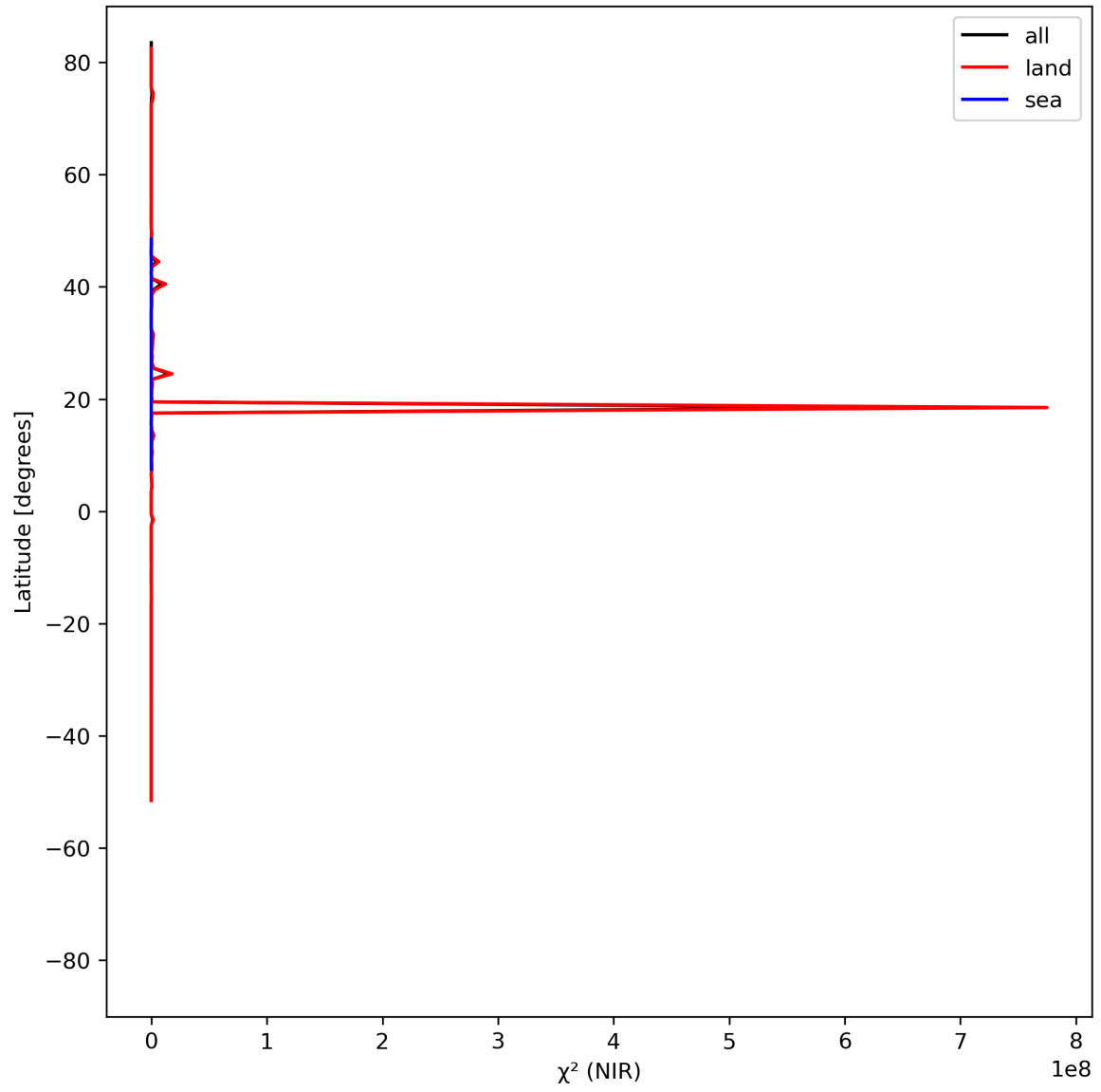
Figure 18: Zonal average of “ \chi^2 (NIR)” for 2024-05-25 to 2024-05-27.
