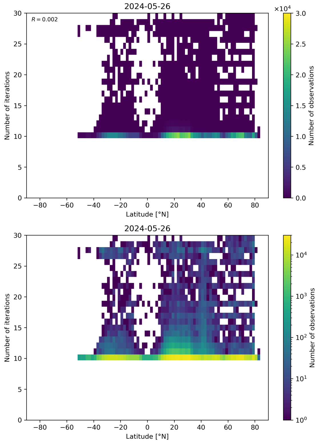
Figure 60: Scatter density plot of “Latitude” against “Number of iterations” for 2024-05-25 to 2024-05-27.
