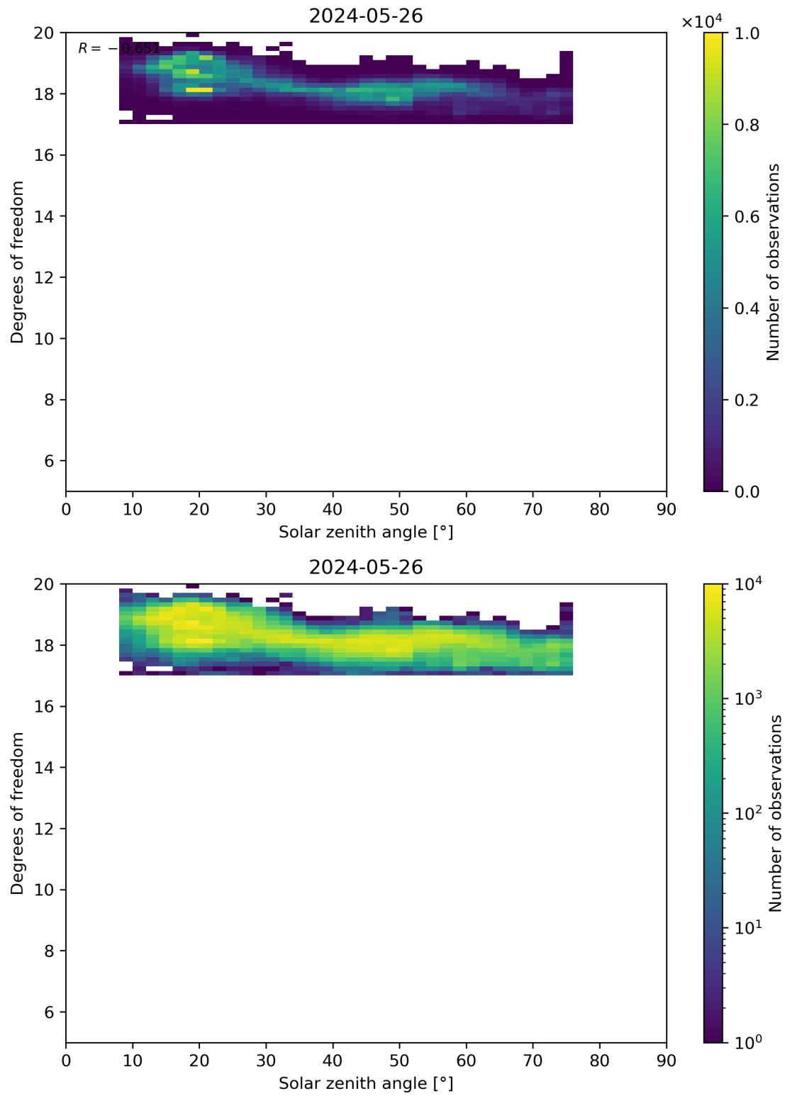
Figure 96: Scatter density plot of “Solar zenith angle” against “Degrees of freedom” for 2024-05-25 to 2024-05-27.
