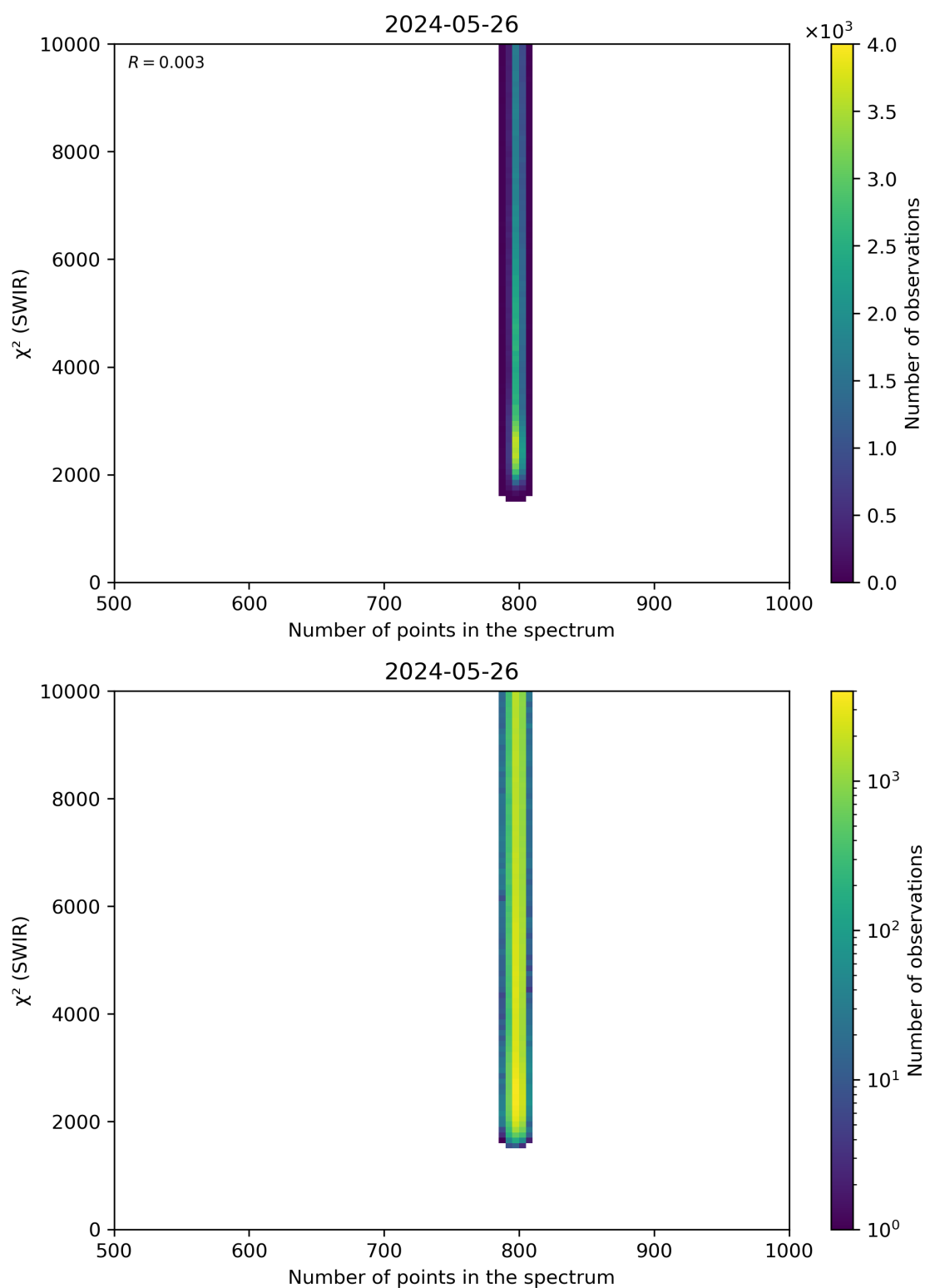
Figure 89: Scatter density plot of “Number of points in the spectrum” against “ \chi^2 (SWIR)” for 2024-05-25 to 2024-05-27.
