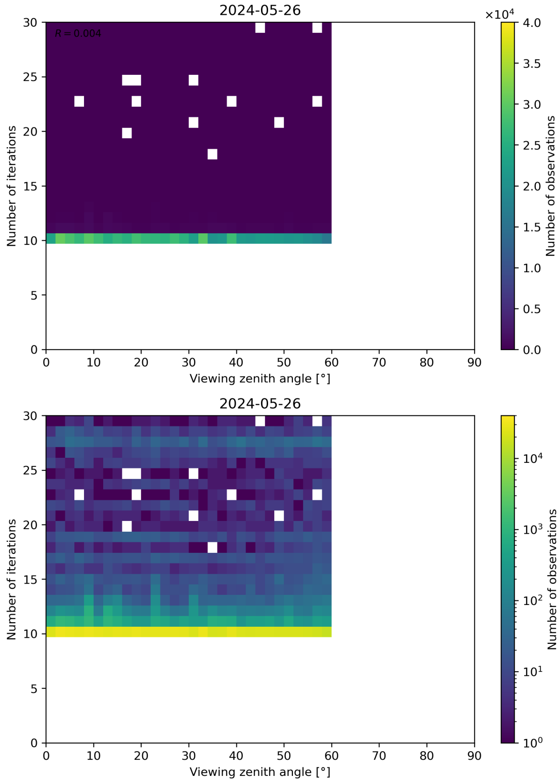
Figure 113: Scatter density plot of “Viewing zenith angle” against “Number of iterations” for 2024-05-25 to 2024-05-27.
