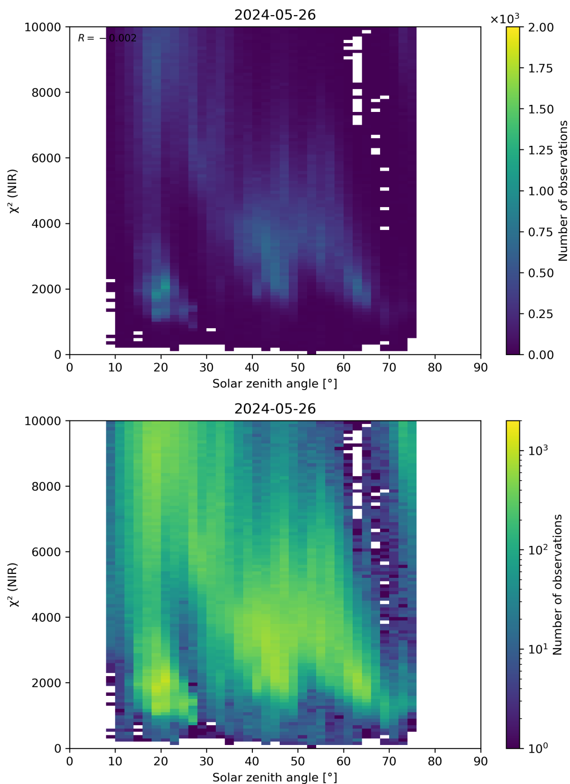
Figure 94: Scatter density plot of “Solar zenith angle” against “ \chi^2 (NIR)” for 2024-05-25 to 2024-05-27.
