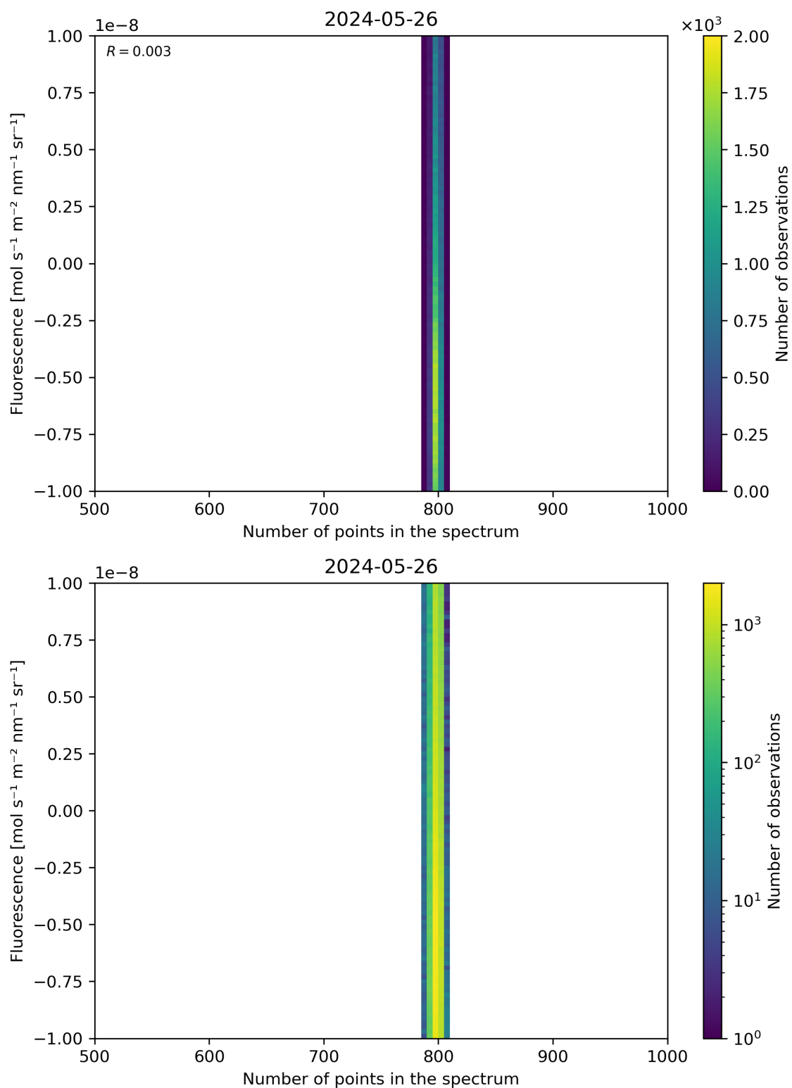
Figure 91: Scatter density plot of “Number of points in the spectrum” against “Fluorescence” for 2024-05-25 to 2024-05-27.
