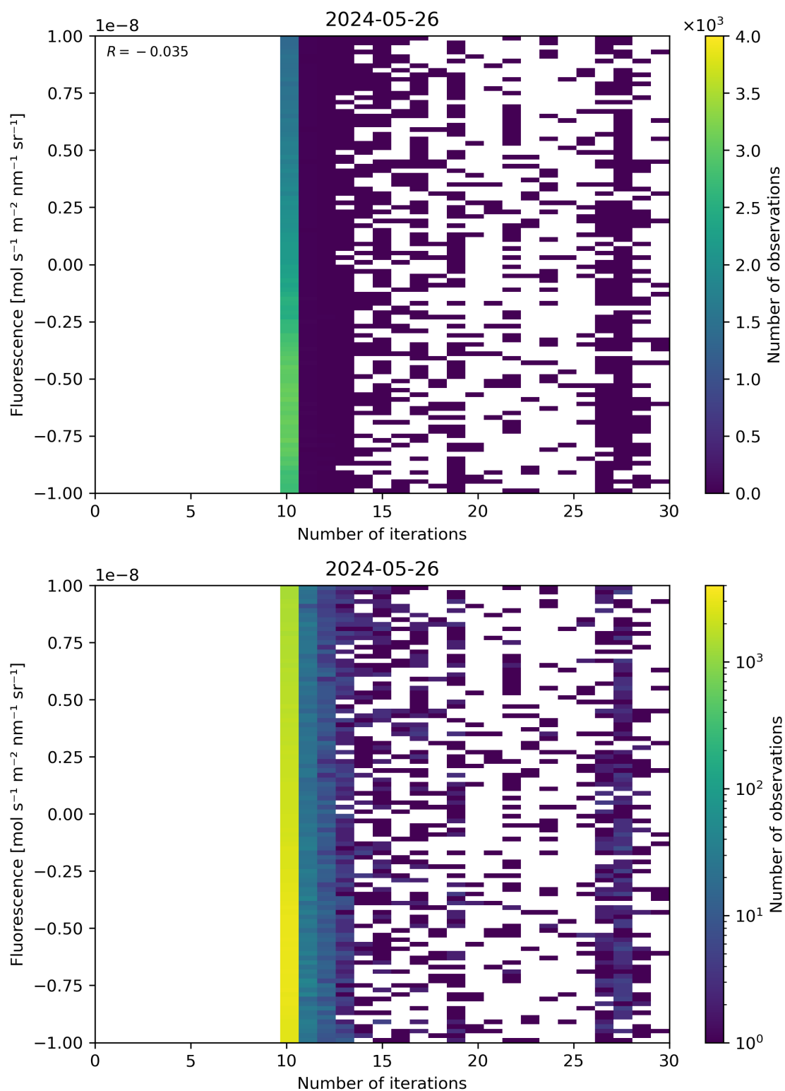
Figure 87: Scatter density plot of “Number of iterations” against “Fluorescence” for 2024-05-25 to 2024-05-27.
