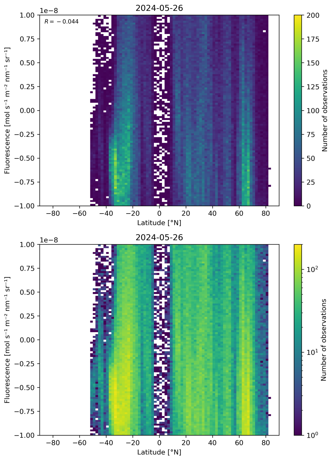
Figure 56: Scatter density plot of “Latitude” against “Fluorescence” for 2024-05-25 to 2024-05-27.
