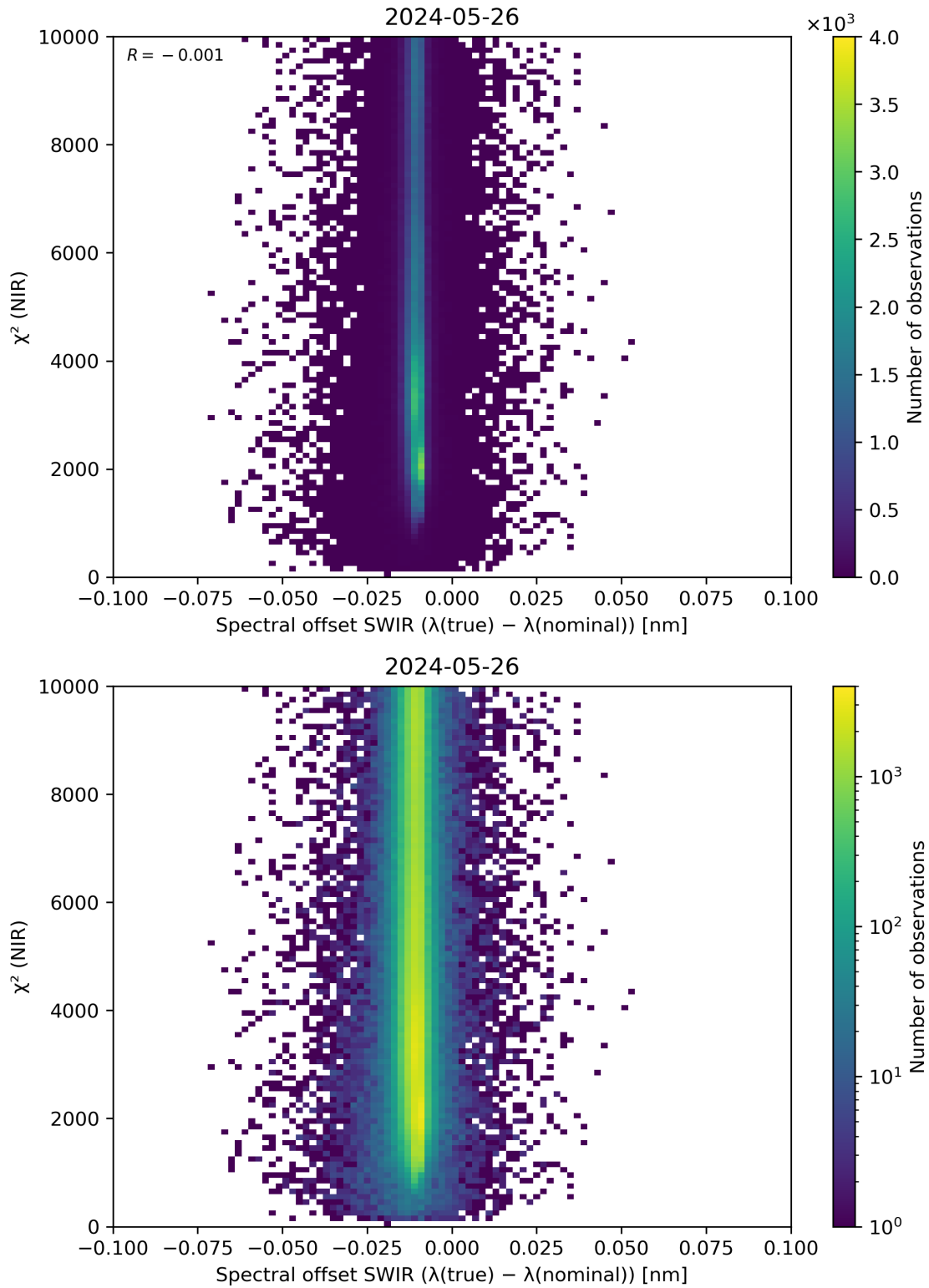
Figure 117: Scatter density plot of “Spectral offset SWIR ( \lambda(\text{true}) - \lambda(\text{nominal}) )” against “ \chi^2 (NIR)” for 2024-05-25 to 2024-05-27.
