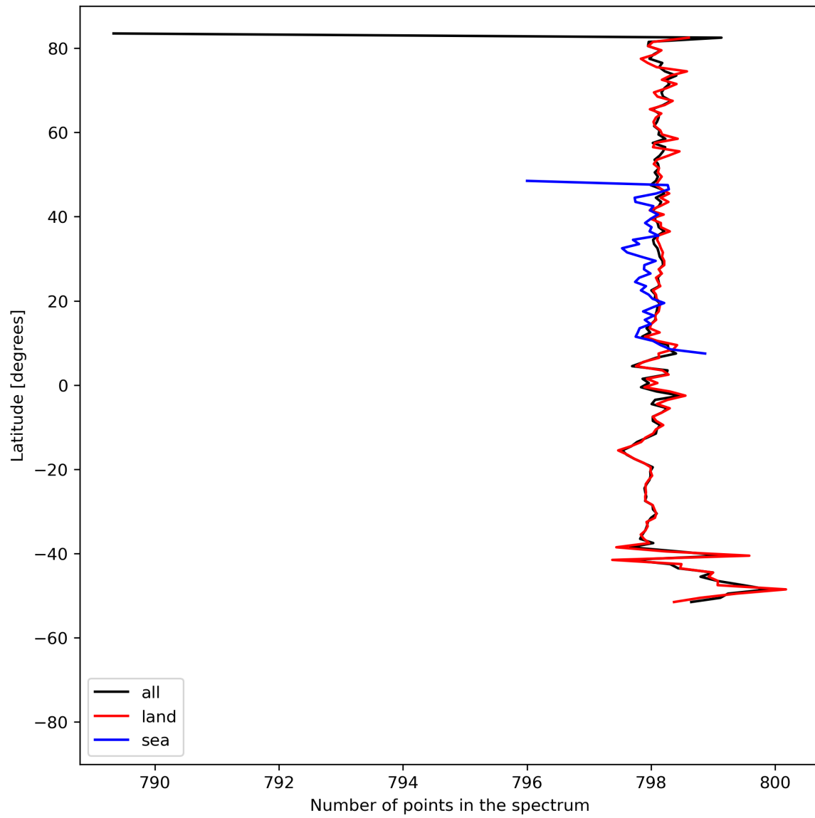
Figure 15: Zonal average of “Number of points in the spectrum” for 2024-05-25 to 2024-05-27.
