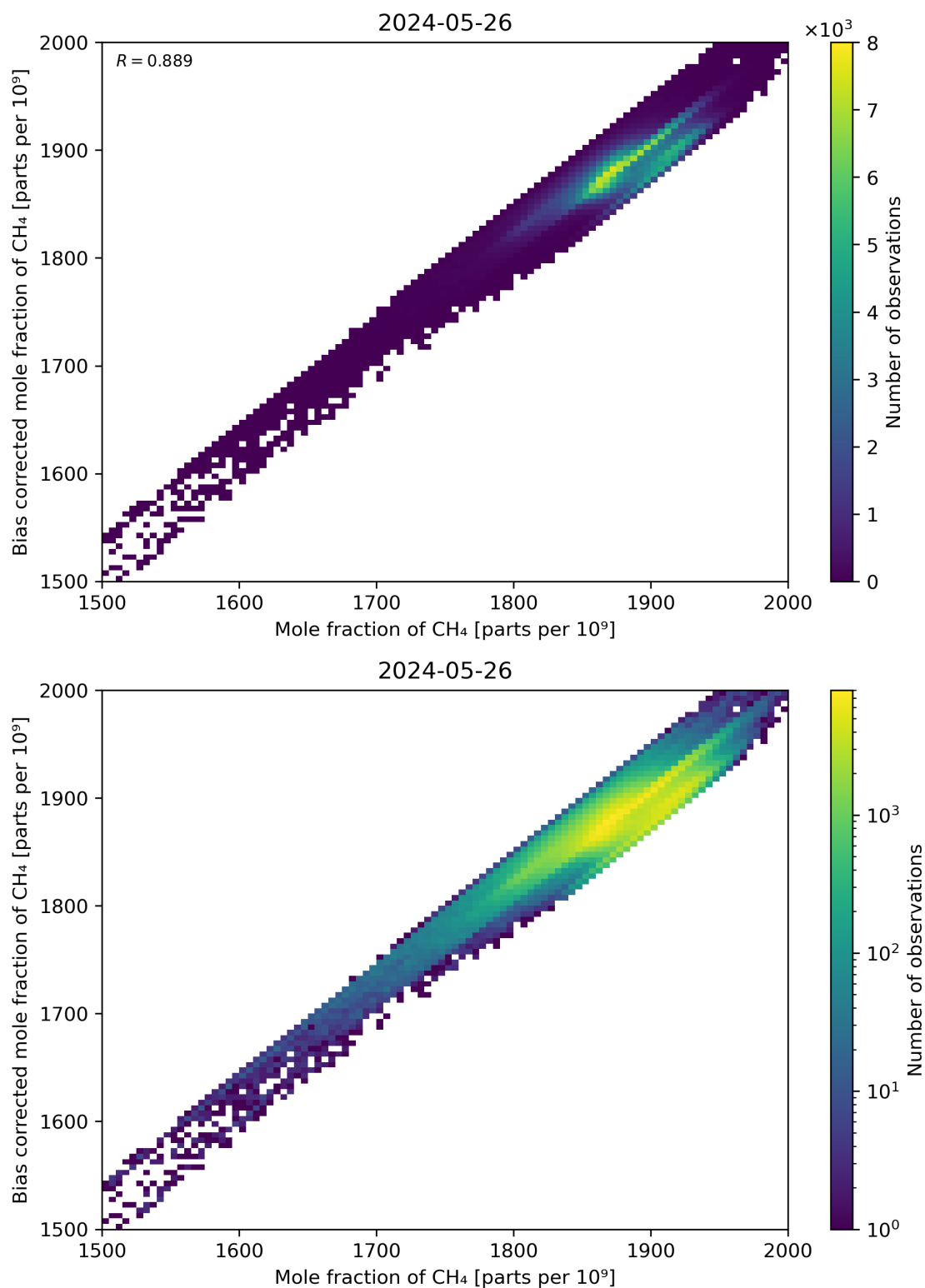
Figure 74: Scatter density plot of “Mole fraction of CH 4 ” against “Bias corrected mole fraction of CH 4 ” for 2024-05-25 to 2024-05-27.
