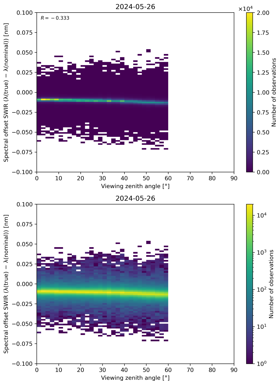
Figure 116: Scatter density plot of “Viewing zenith angle” against “Spectral offset SWIR ( \lambda(\text{true}) - \lambda(\text{nominal}) )” for 2024-05-25 to 2024-05-27.
