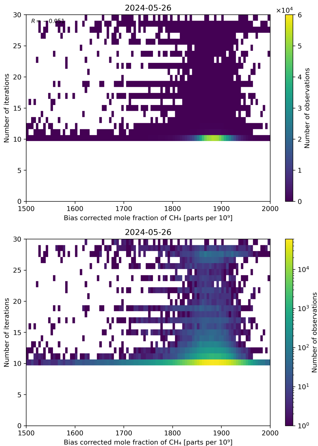
Figure 67: Scatter density plot of “Bias corrected mole fraction of \text{CH}_4 ” against “Number of iterations” for 2024-05-25 to 2024-05-27.
