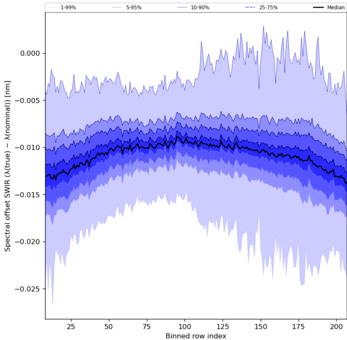
Figure 38: Along track statistics of “Spectral offset SWIR ( \lambda(\text{true}) - \lambda(\text{nominal}) )” for 2024-05-25 to 2024-05-27
