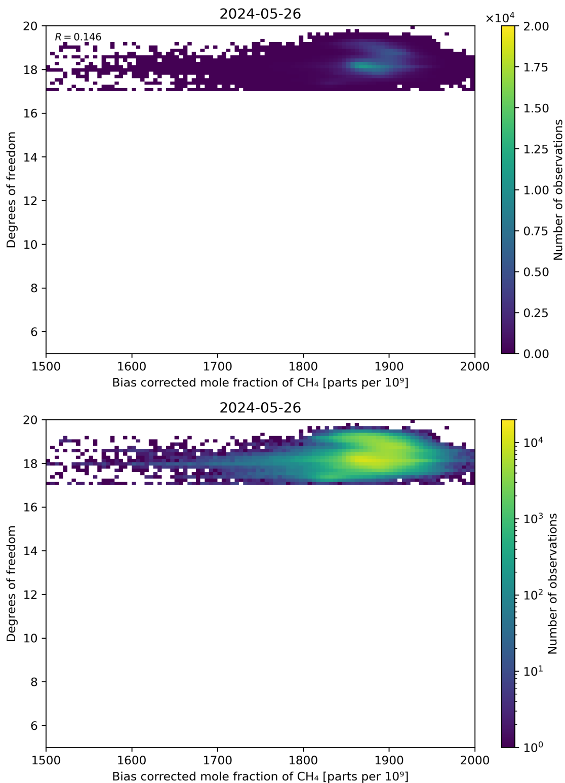
Figure 65: Scatter density plot of “Bias corrected mole fraction of CH 4 ” against “Degrees of freedom” for 2024-05-25 to 2024-05-27.
