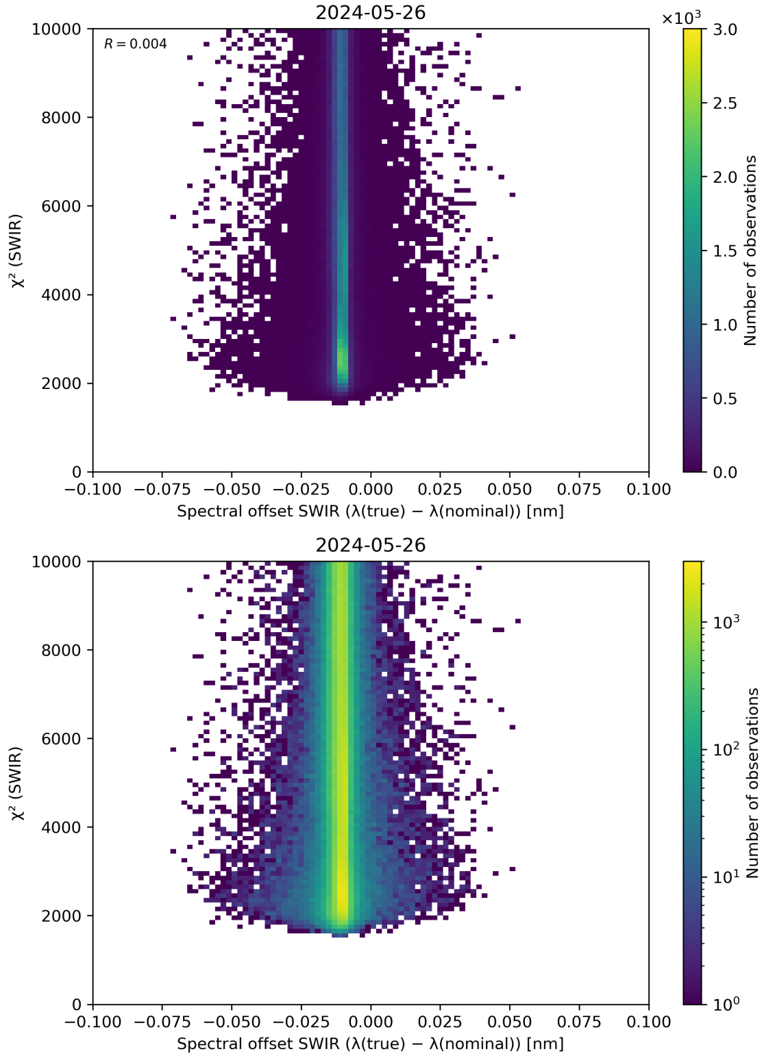
Figure 118: Scatter density plot of “Spectral offset SWIR ( \lambda(\text{true}) - \lambda(\text{nominal}) )” against “ \chi^2 (SWIR)” for 2024-05-25 to 2024-05-27.
