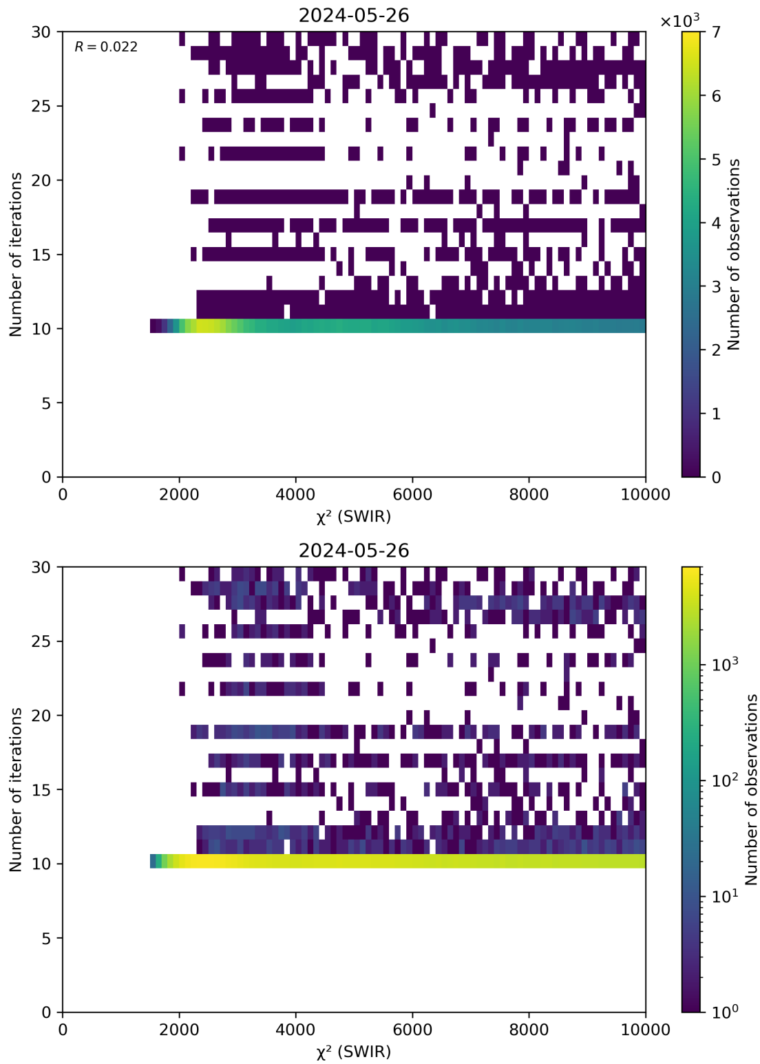
Figure 50: Scatter density plot of “ \chi^2 (SWIR)” against “Number of iterations” for 2024-05-25 to 2024-05-27.
