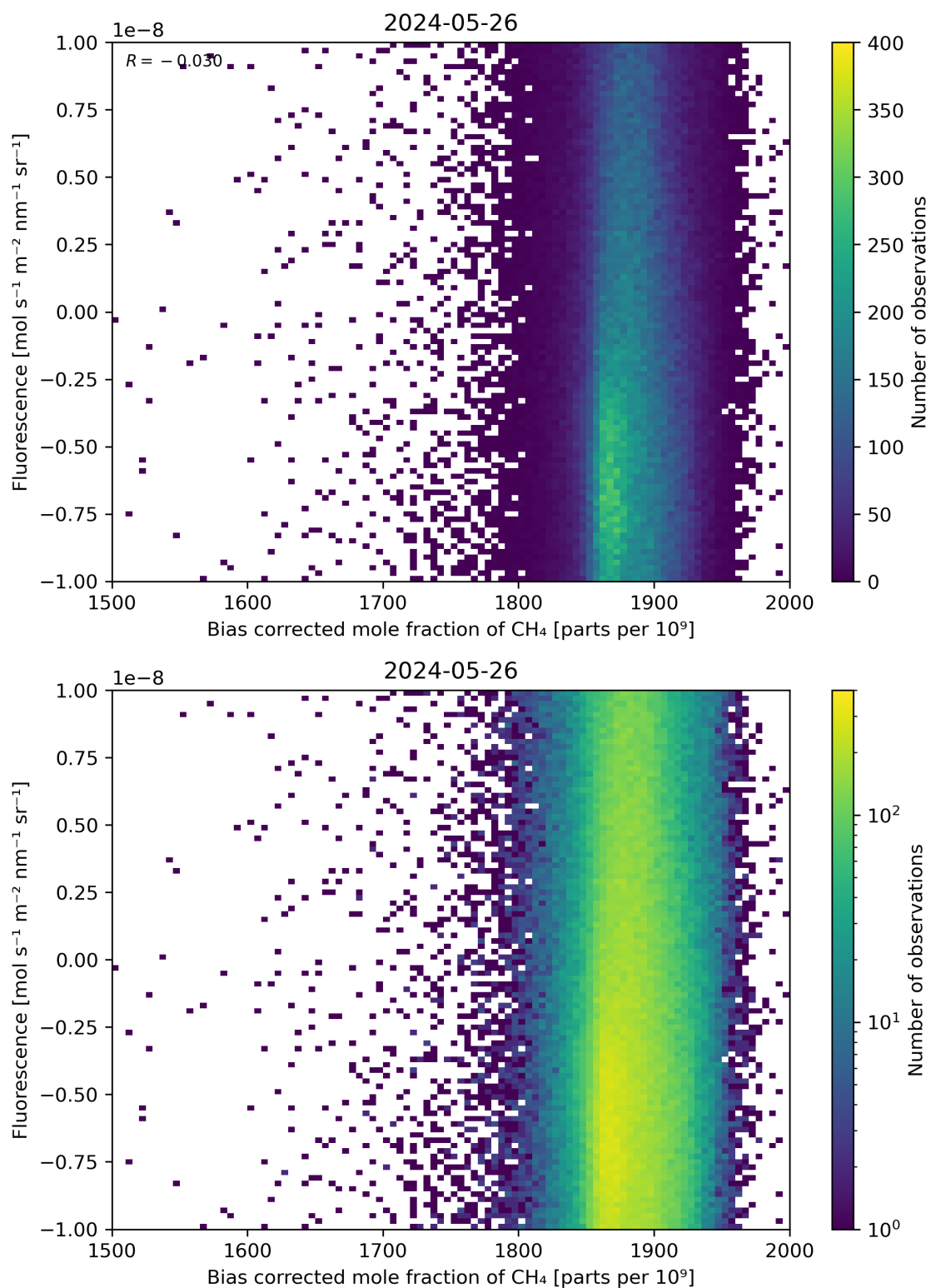
Figure 66: Scatter density plot of “Bias corrected mole fraction of \text{CH}_4 ” against “Fluorescence” for 2024-05-25 to 2024-05-27.
