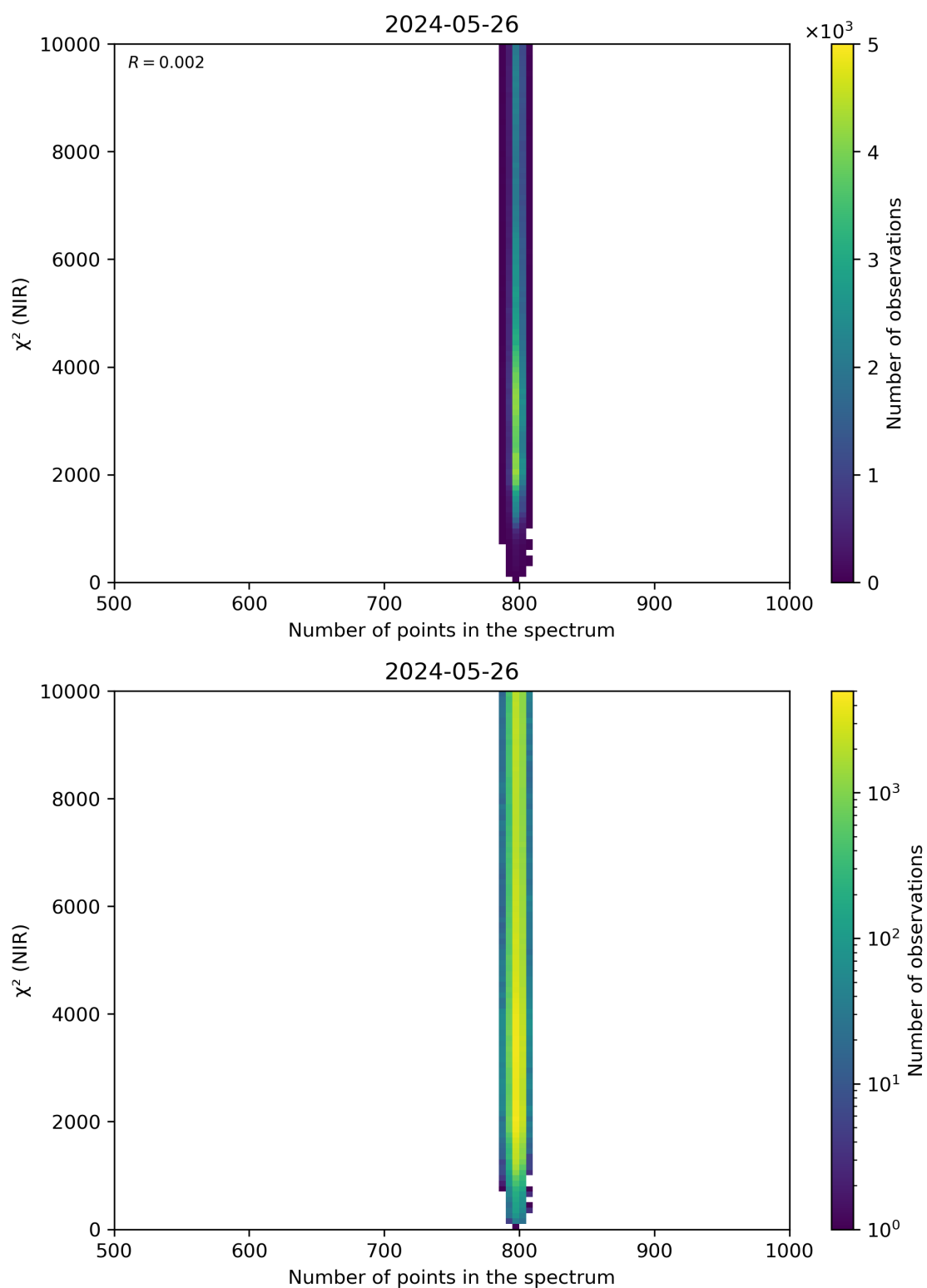
Figure 88: Scatter density plot of “Number of points in the spectrum” against “ \chi^2 (NIR)” for 2024-05-25 to 2024-05-27.
