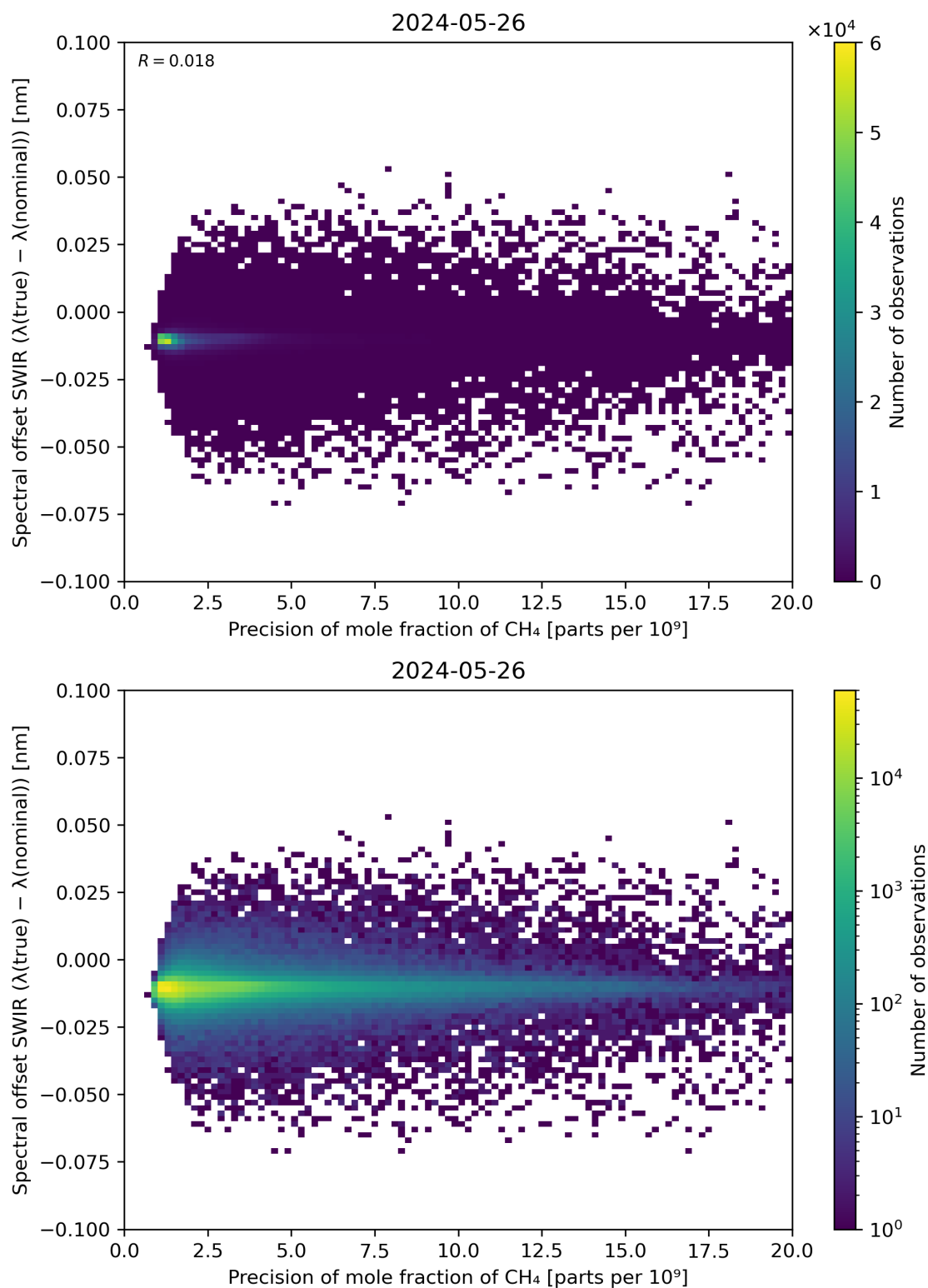
Figure 85: Scatter density plot of “Precision of mole fraction of \text{CH}_4 ” against “Spectral offset SWIR ( \lambda(\text{true}) - \lambda(\text{nominal}) )” for 2024-05-25 to 2024-05-27.
