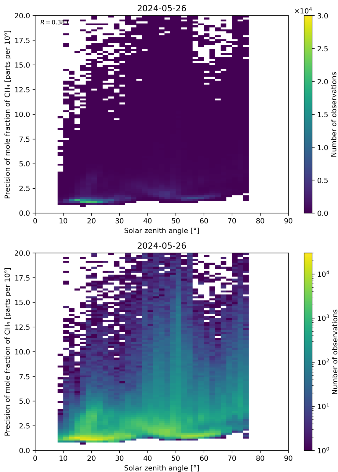
Figure 101: Scatter density plot of “Solar zenith angle” against “Precision of mole fraction of CH 4 ” for 2024-05-25 to 2024-05-27.
