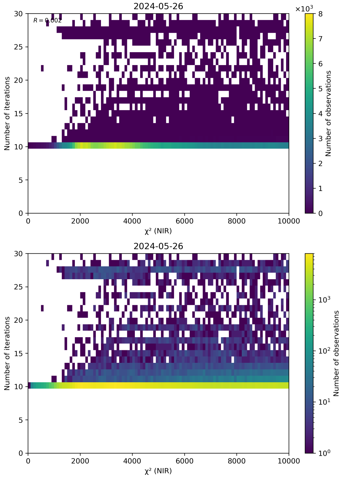
Figure 46: Scatter density plot of “ \chi^2 (NIR)” against “Number of iterations” for 2024-05-25 to 2024-05-27.
