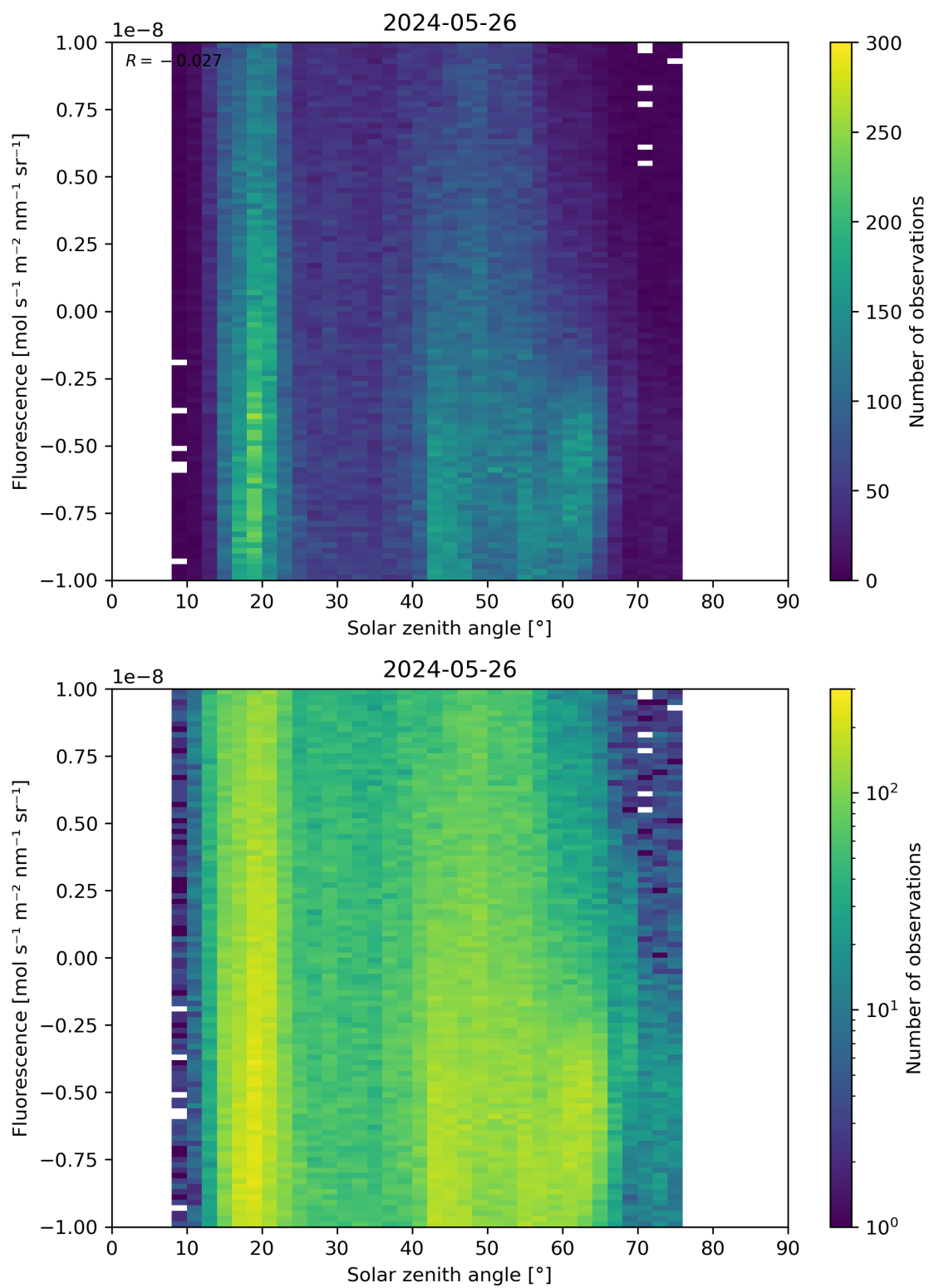
Figure 97: Scatter density plot of “Solar zenith angle” against “Fluorescence” for 2024-05-25 to 2024-05-27.
