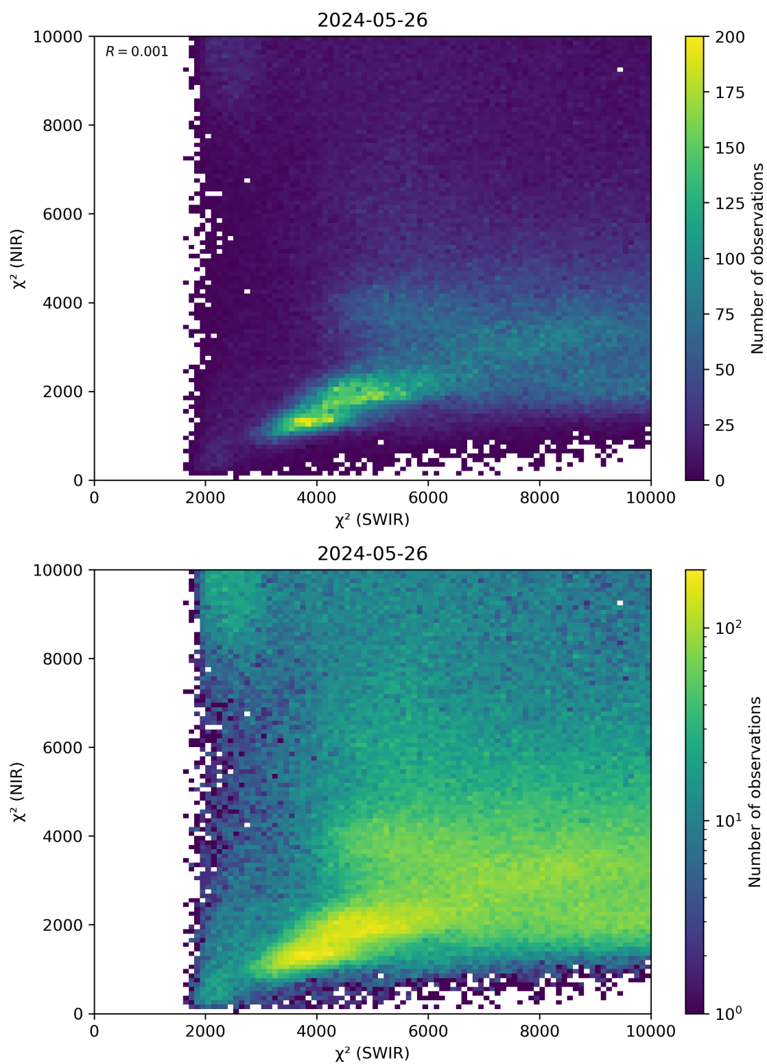
Figure 47: Scatter density plot of “ \chi^2 (SWIR)” against “ \chi^2 (NIR)” for 2024-05-25 to 2024-05-27.
