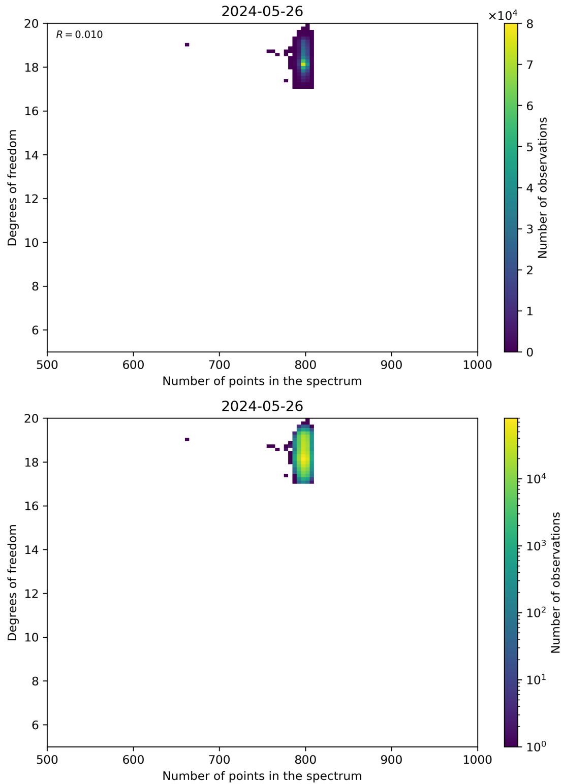
Figure 90: Scatter density plot of “Number of points in the spectrum” against “Degrees of freedom” for 2024-05-25 to 2024-05-27.
