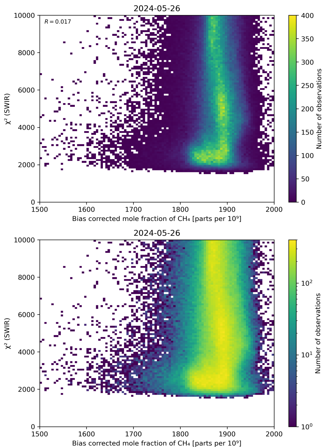
Figure 64: Scatter density plot of “Bias corrected mole fraction of \text{CH}_4 ” against “ \chi^2 (SWIR)” for 2024-05-25 to 2024-05-27.
