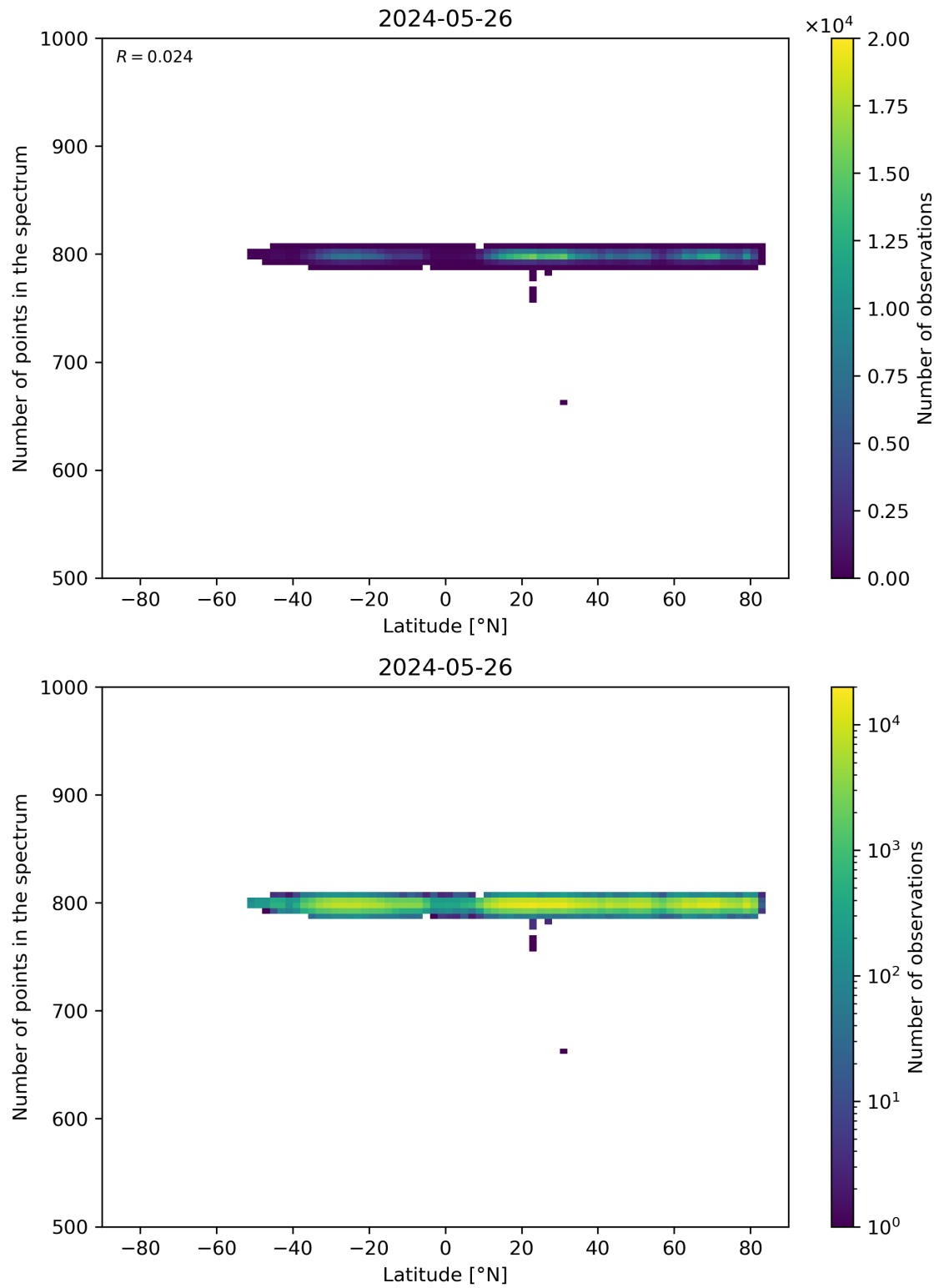
Figure 61: Scatter density plot of “Latitude” against “Number of points in the spectrum” for 2024-05-25 to 2024-05-27.
