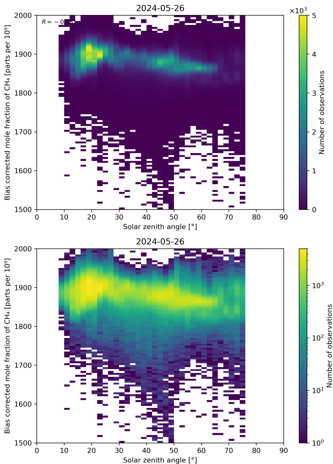
Figure 100: Scatter density plot of “Solar zenith angle” against “Bias corrected mole fraction of \text{CH}_4 ” for 2024-05-25 to 2024-05-27.
