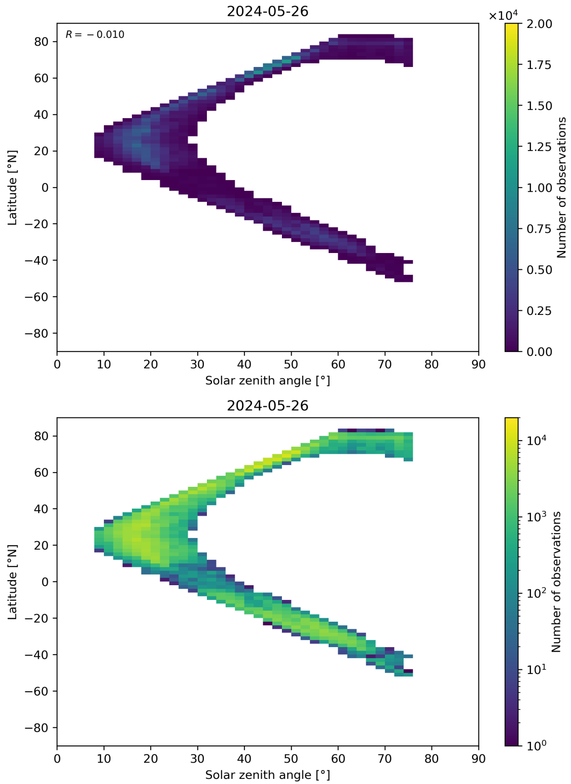
Figure 98: Scatter density plot of “Solar zenith angle” against “Latitude” for 2024-05-25 to 2024-05-27.
