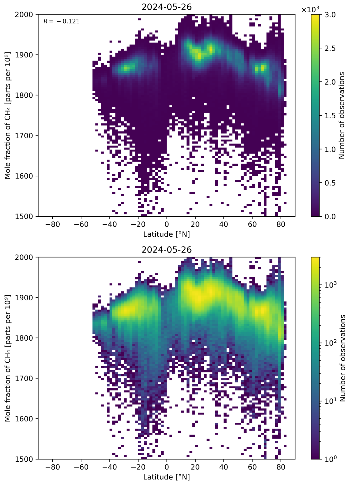
Figure 57: Scatter density plot of “Latitude” against “Mole fraction of CH 4 ” for 2024-05-25 to 2024-05-27.
