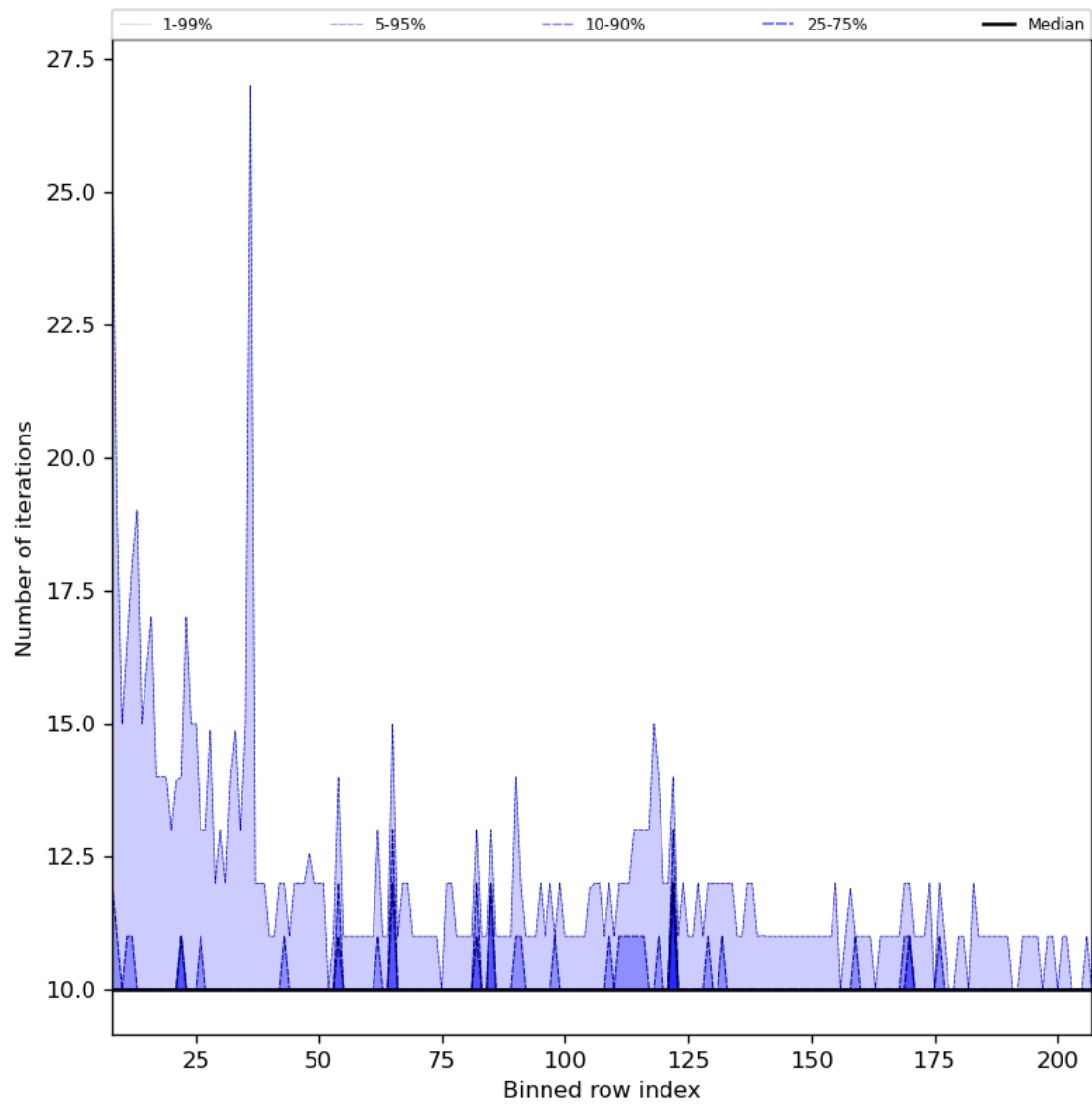
Figure 42: Along track statistics of “Number of iterations” for 2024-05-25 to 2024-05-27
