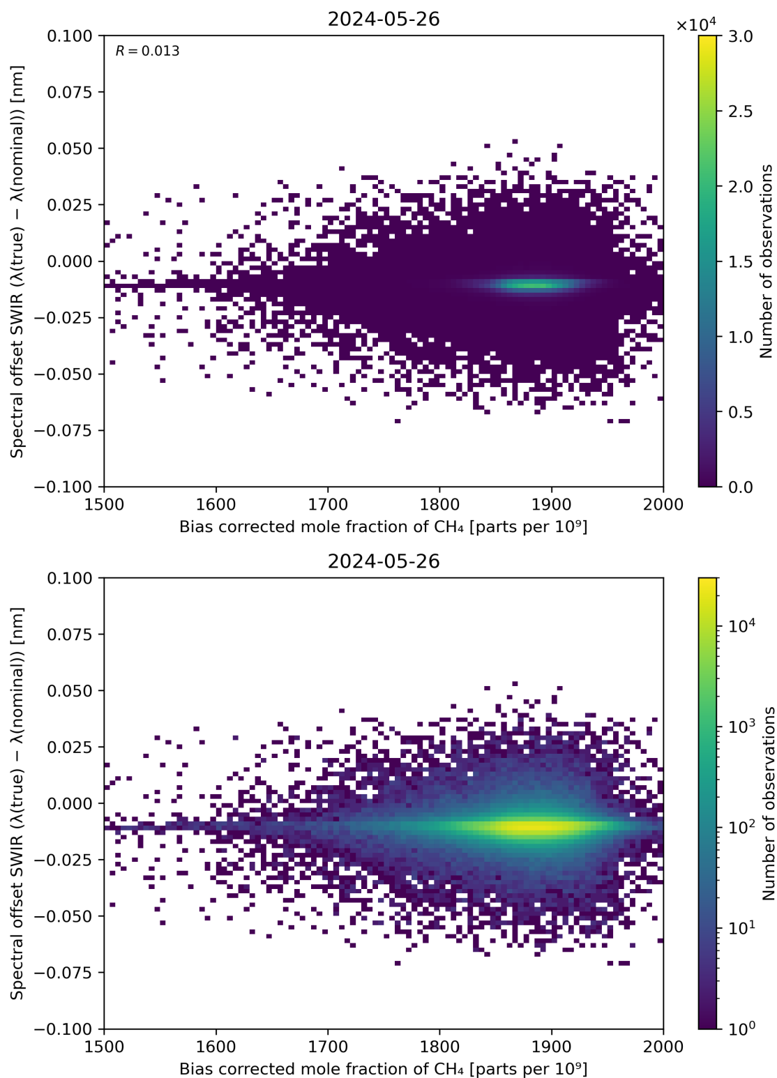
Figure 69: Scatter density plot of “Bias corrected mole fraction of \text{CH}_4 ” against “Spectral offset SWIR ( \lambda(\text{true}) - \lambda(\text{nominal}) )” for 2024-05-25 to 2024-05-27.
