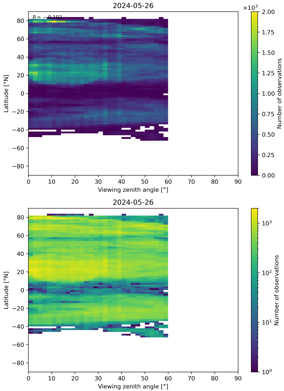
Figure 109: Scatter density plot of “Viewing zenith angle” against “Latitude” for 2024-05-25 to 2024-05-27.
