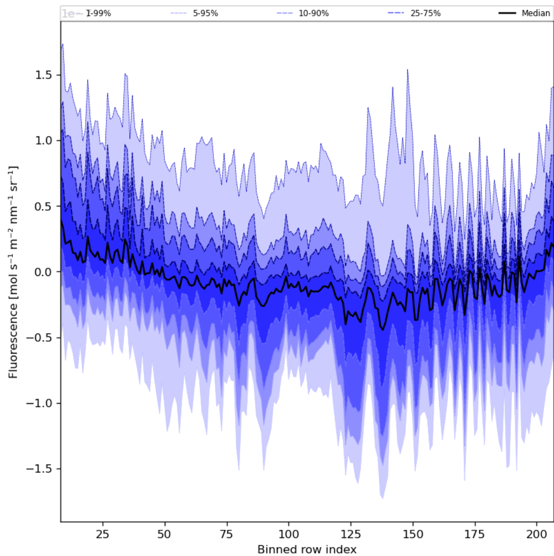
Figure 43: Along track statistics of “Fluorescence” for 2024-05-25 to 2024-05-27
