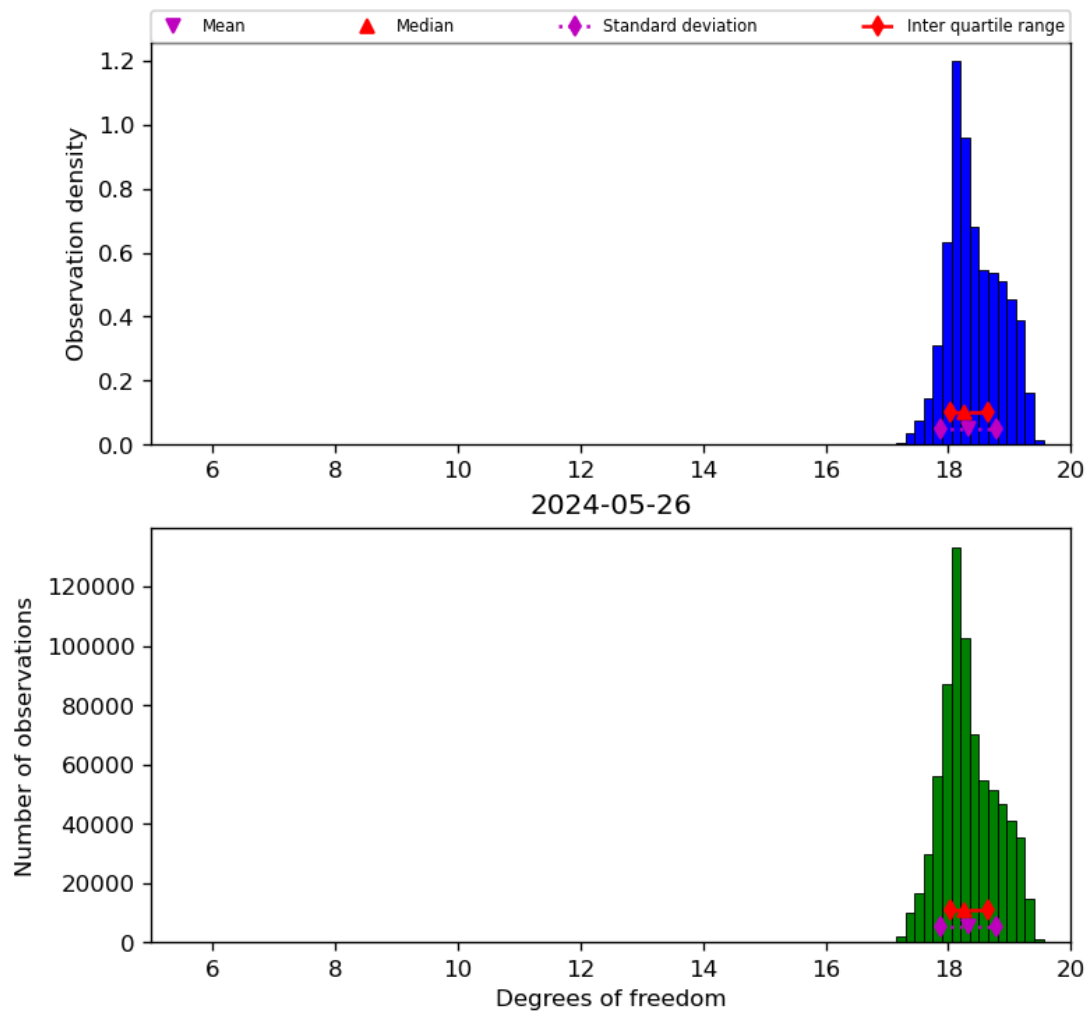
Figure 30: Histogram of “Degrees of freedom” for 2024-05-25 to 2024-05-27
