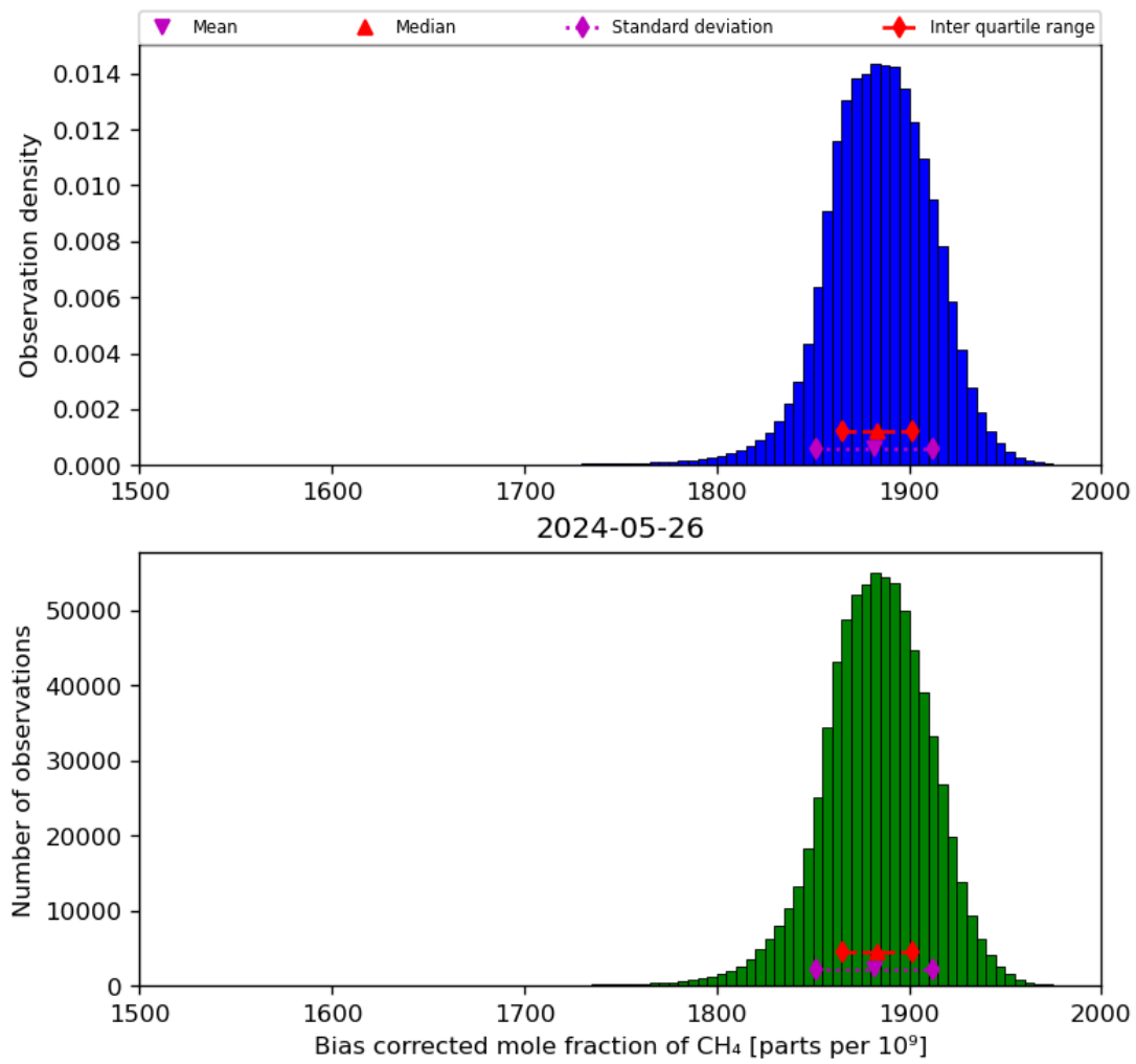
Figure 25: Histogram of “Bias corrected mole fraction of CH 4 ” for 2024-05-25 to 2024-05-27
