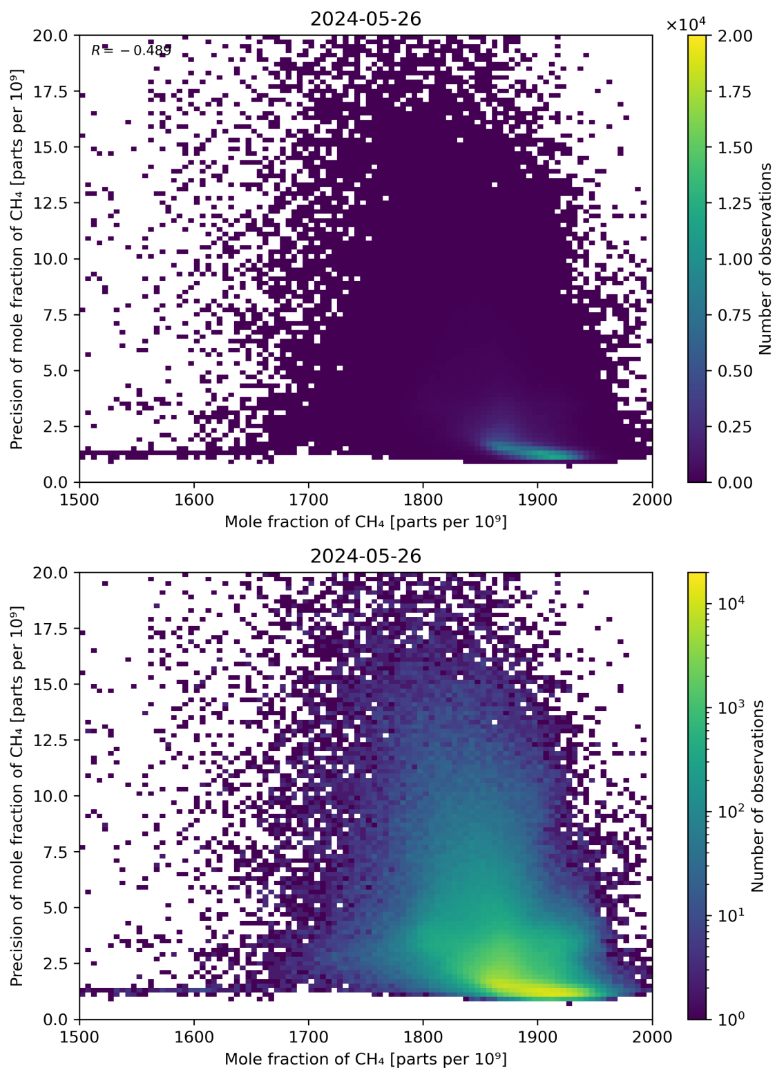
Figure 75: Scatter density plot of “Mole fraction of CH 4 ” against “Precision of mole fraction of CH 4 ” for 2024-05-25 to 2024-05-27.
