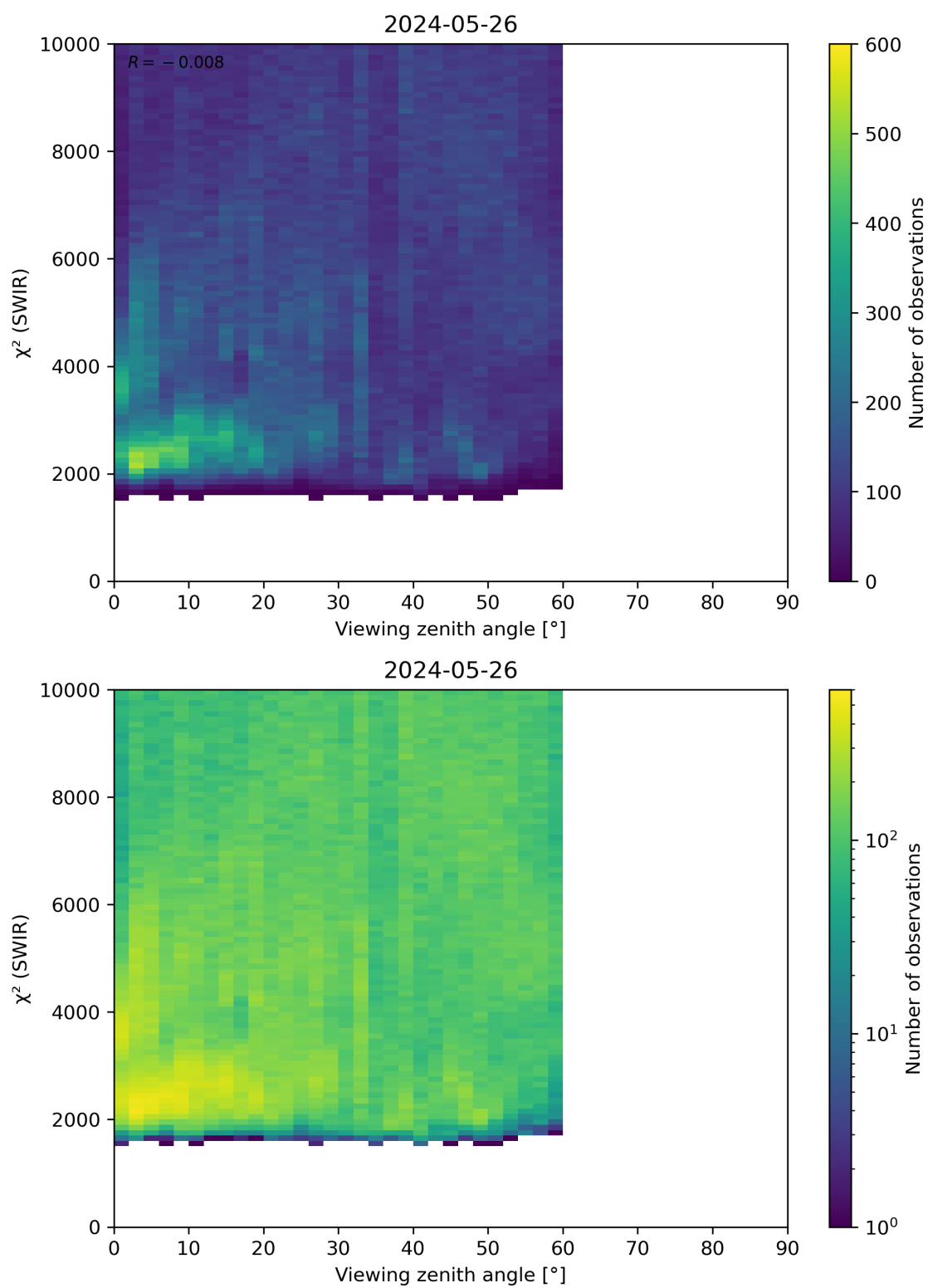
Figure 106: Scatter density plot of “Viewing zenith angle” against “ \chi^2 (SWIR)” for 2024-05-25 to 2024-05-27.
