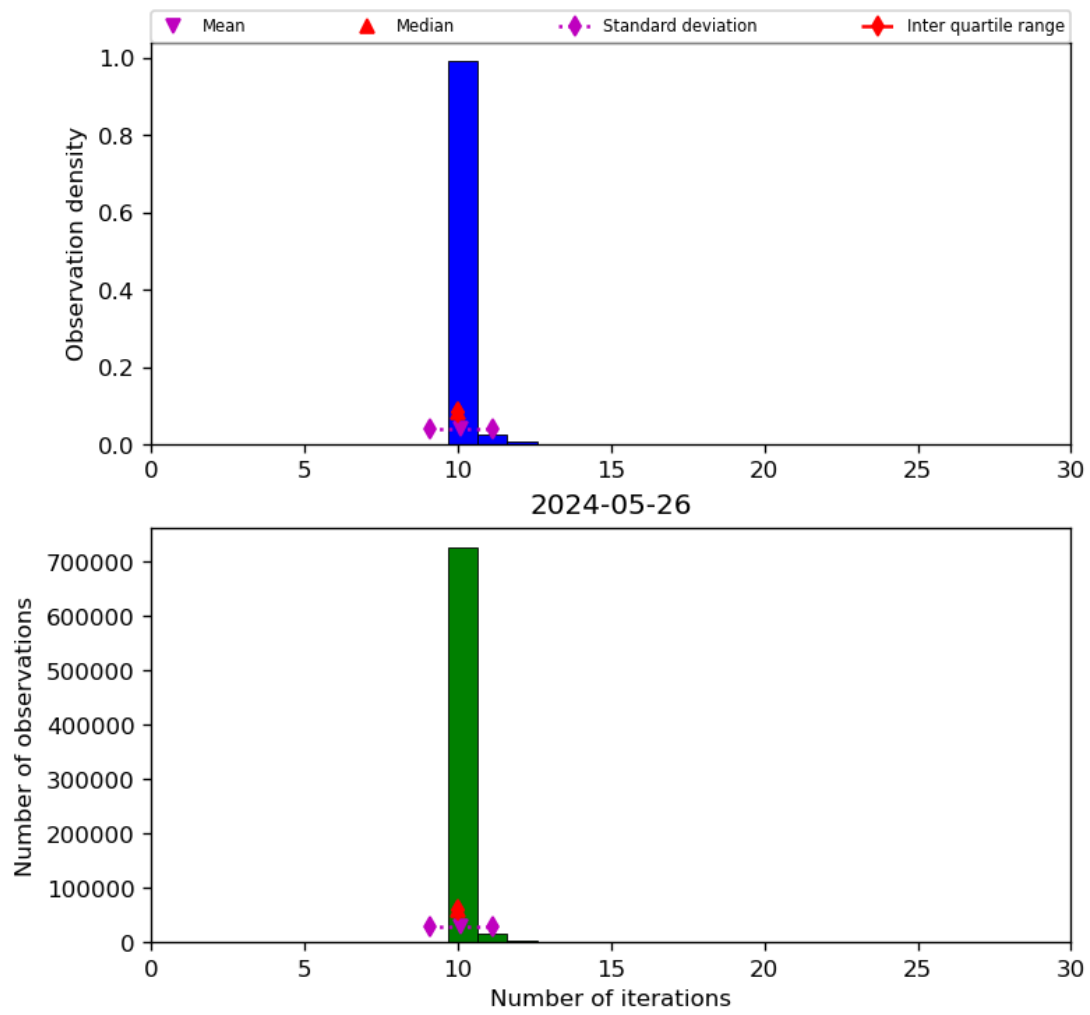
Figure 31: Histogram of “Number of iterations” for 2024-05-25 to 2024-05-27
