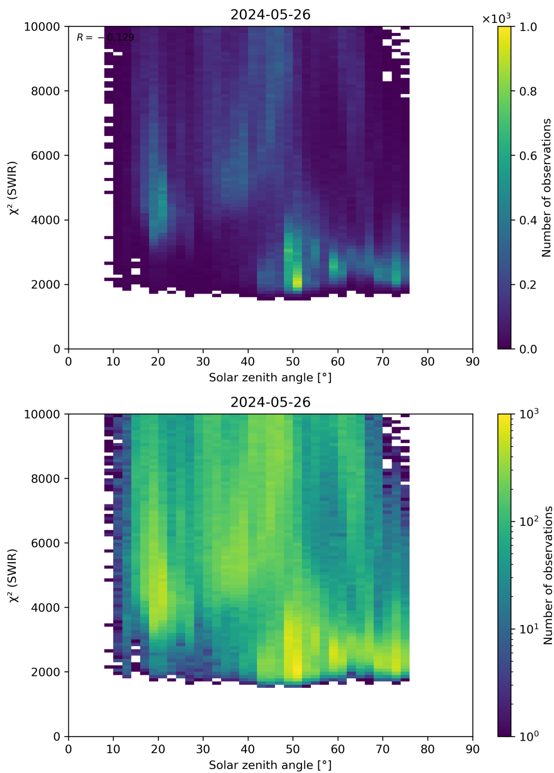
Figure 95: Scatter density plot of “Solar zenith angle” against “ \chi^2 (SWIR)” for 2024-05-25 to 2024-05-27.
