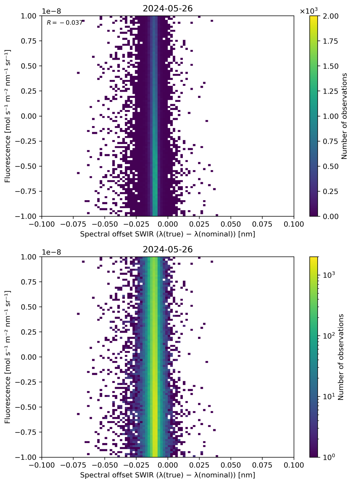
Figure 120: Scatter density plot of “Spectral offset SWIR ( \lambda(\text{true}) - \lambda(\text{nominal}) )” against “Fluorescence” for 2024-05-25 to 2024-05-27.
