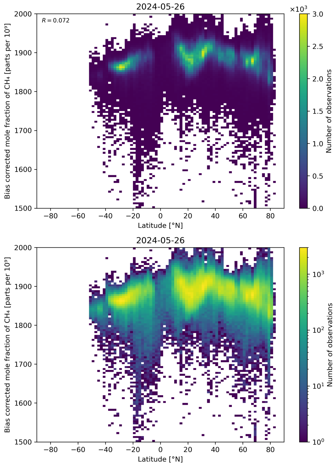
Figure 58: Scatter density plot of “Latitude” against “Bias corrected mole fraction of CH 4 ” for 2024-05-25 to 2024-05-27.
