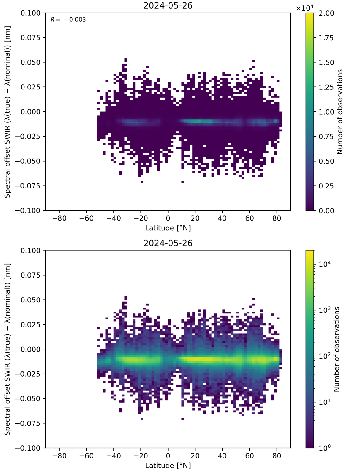
Figure 62: Scatter density plot of “Latitude” against “Spectral offset SWIR ( \lambda(\text{true}) - \lambda(\text{nominal}) )” for 2024-05-25 to 2024-05-27.
