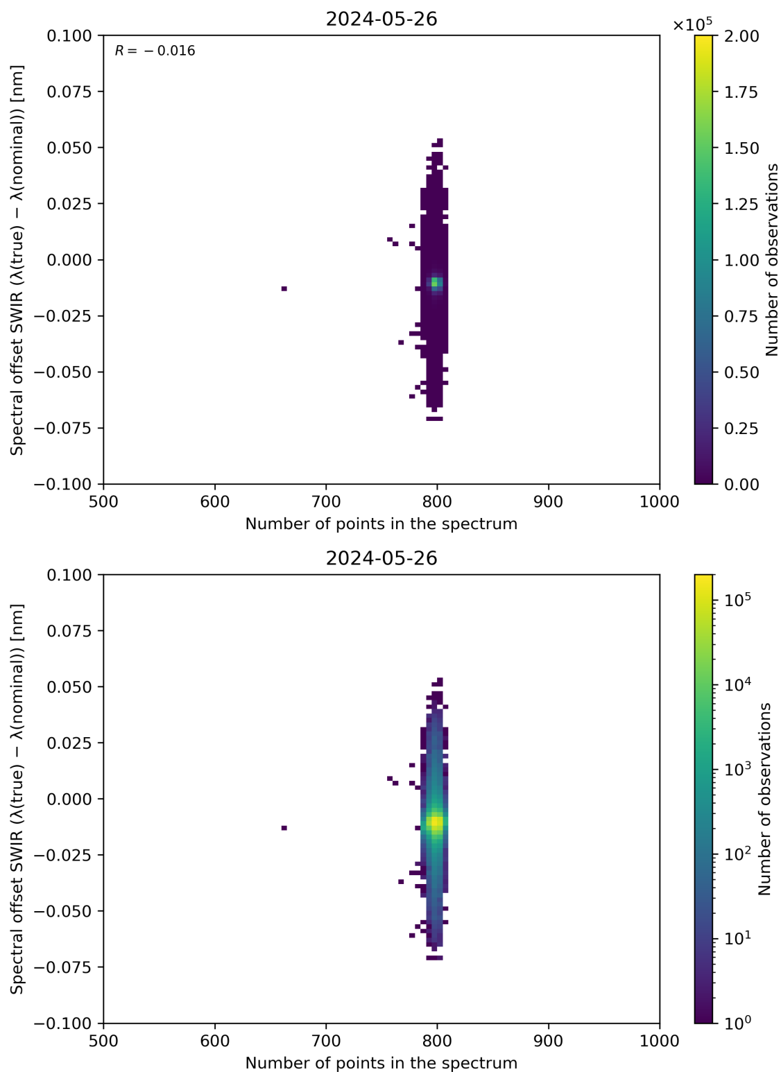
Figure 93: Scatter density plot of “Number of points in the spectrum” against “Spectral offset SWIR ( \lambda(\text{true}) - \lambda(\text{nominal}) )” for 2024-05-25 to 2024-05-27.
