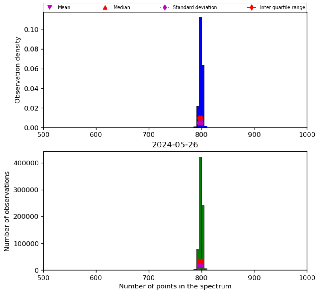
Figure 26: Histogram of “Number of points in the spectrum” for 2024-05-25 to 2024-05-27
