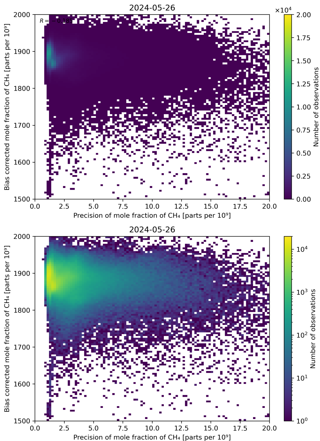
Figure 82: Scatter density plot of “Precision of mole fraction of \text{CH}_4 ” against “Bias corrected mole fraction of \text{CH}_4 ” for 2024-05-25 to 2024-05-27.
