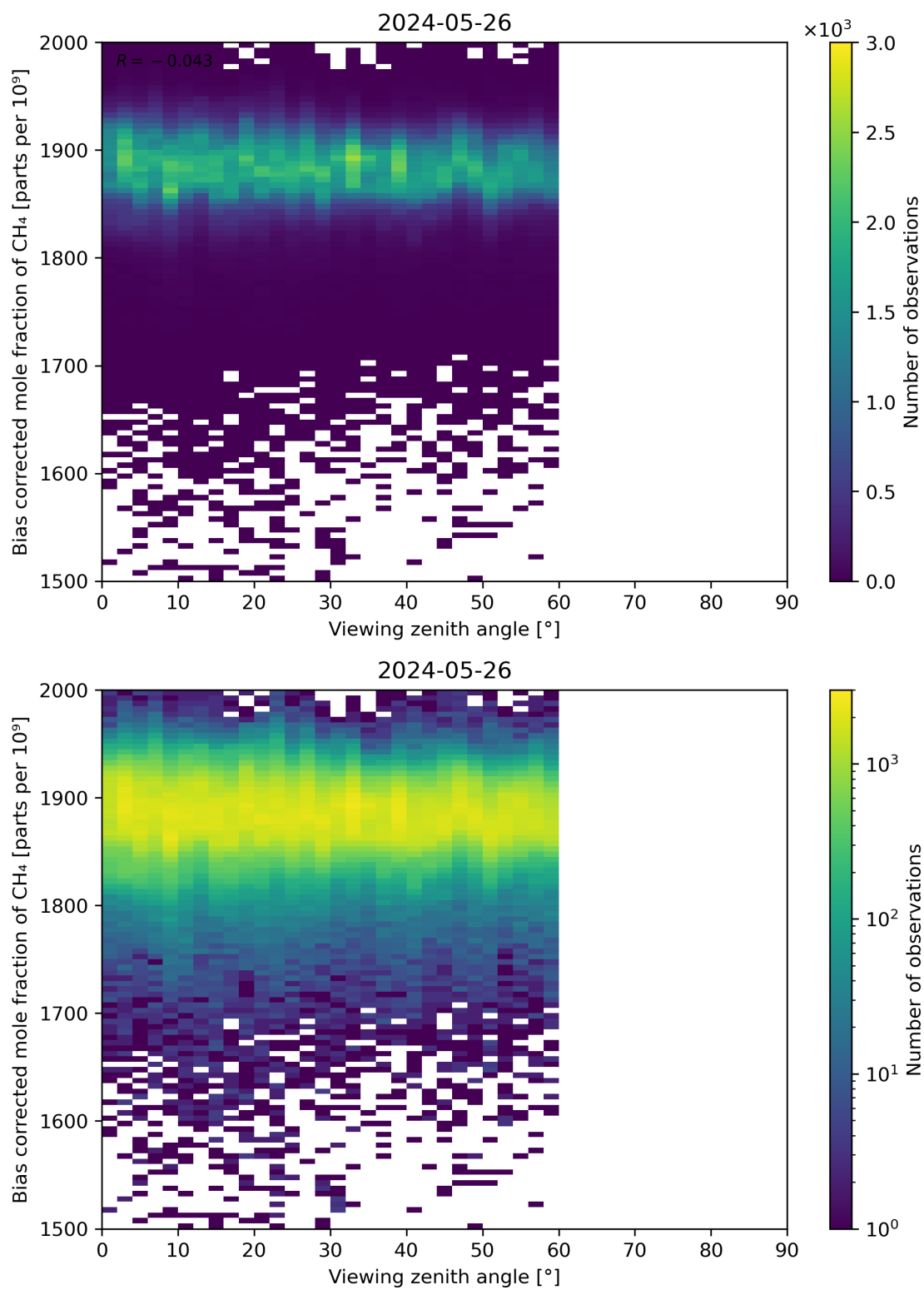
Figure 111: Scatter density plot of “Viewing zenith angle” against “Bias corrected mole fraction of CH 4 ” for 2024-05-25 to 2024-05-27.
