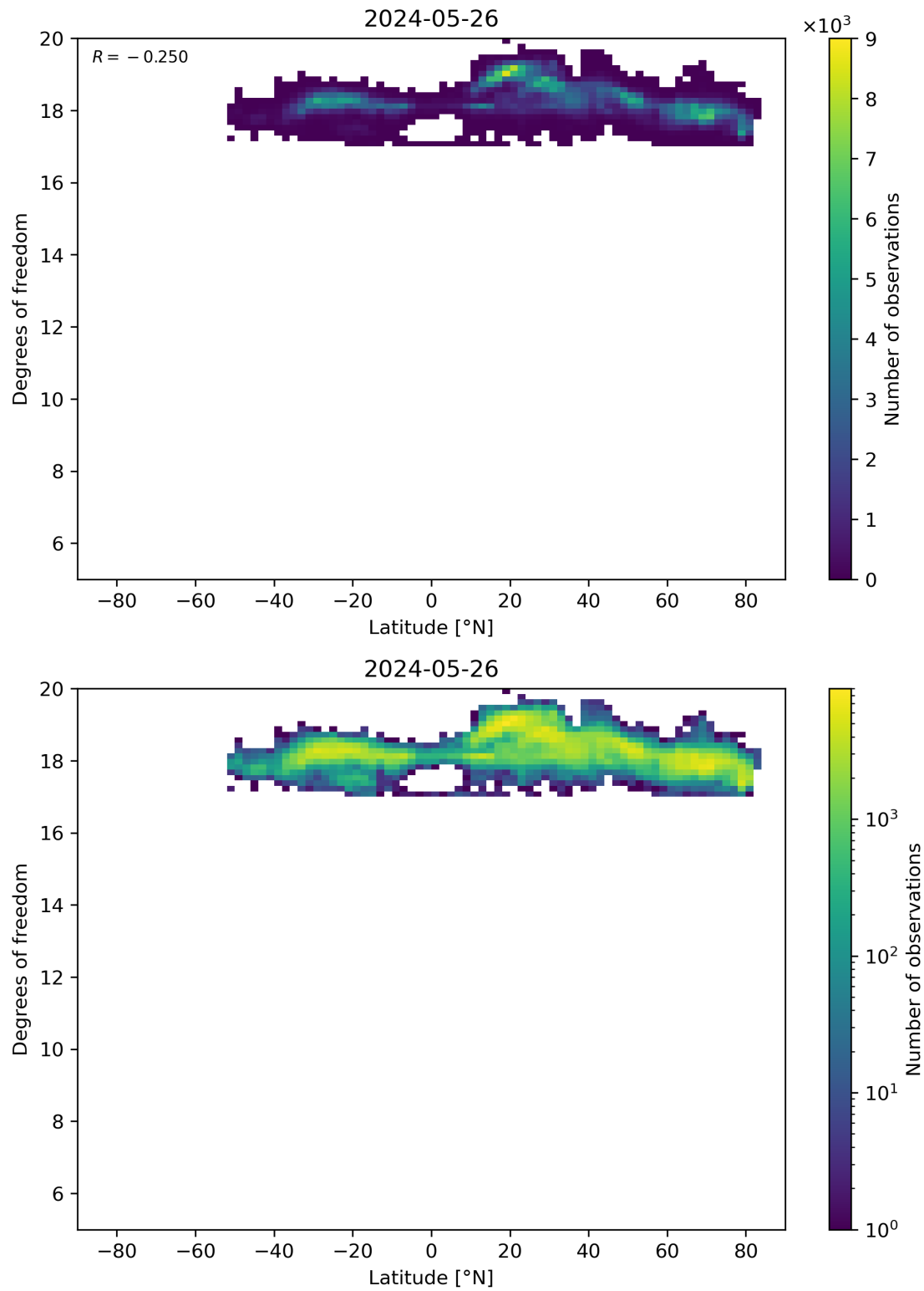
Figure 55: Scatter density plot of “Latitude” against “Degrees of freedom” for 2024-05-25 to 2024-05-27.
