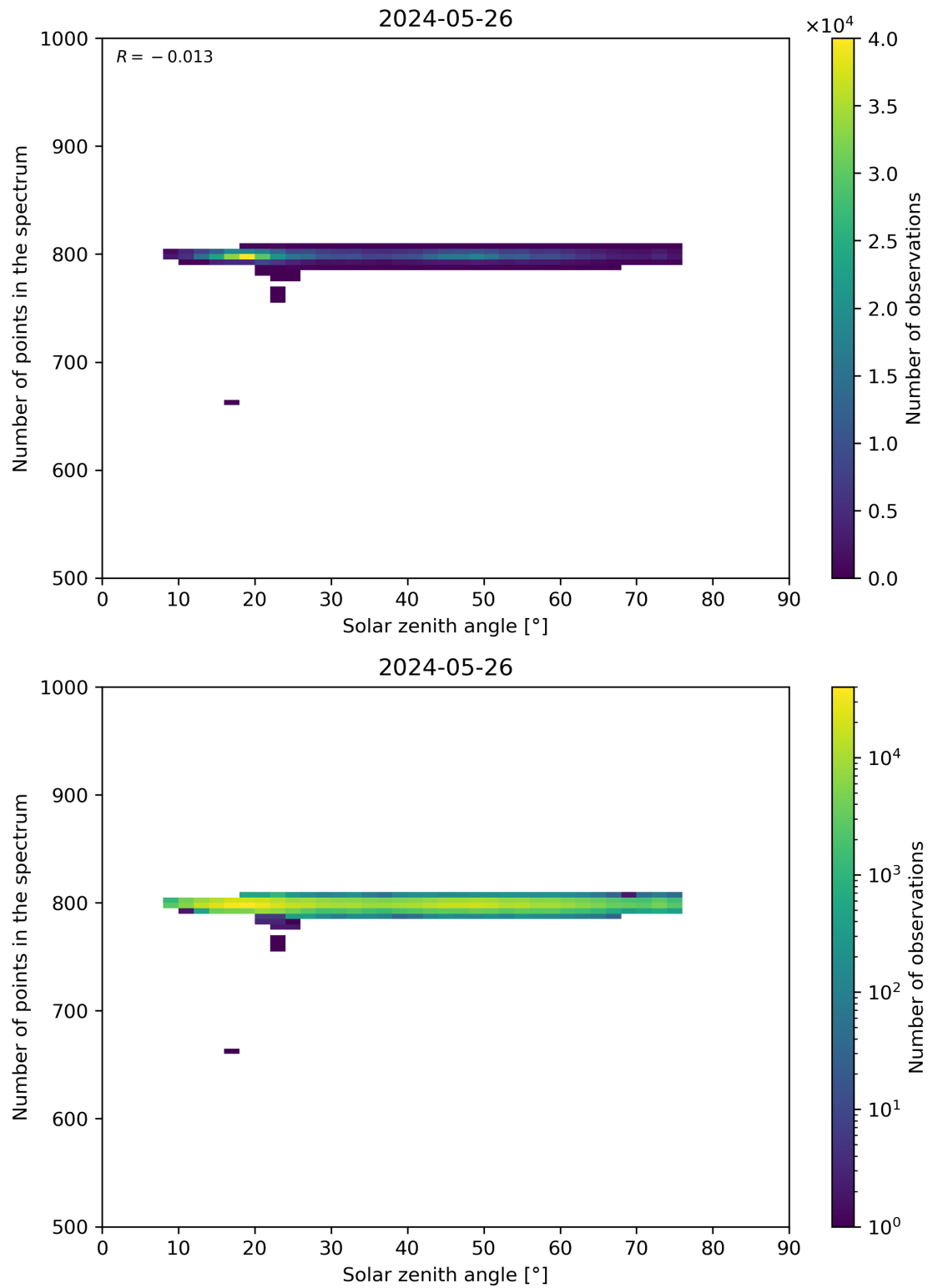
Figure 103: Scatter density plot of “Solar zenith angle” against “Number of points in the spectrum” for 2024-05-25 to 2024-05-27.
