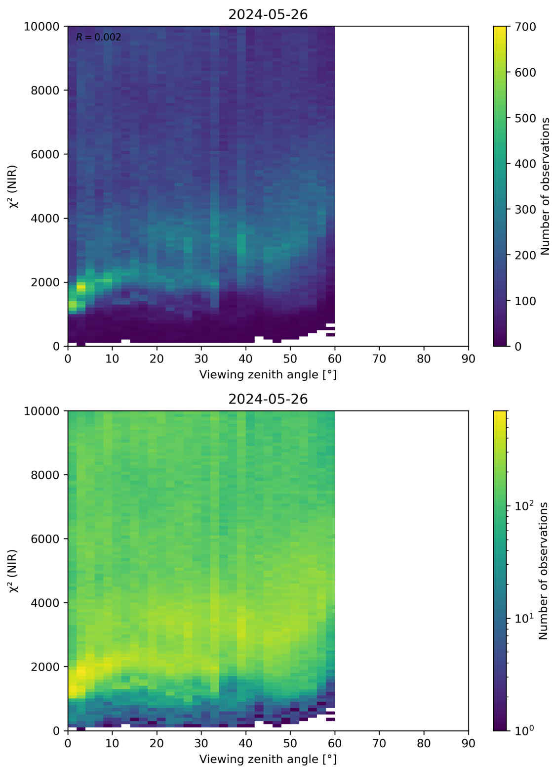
Figure 105: Scatter density plot of “Viewing zenith angle” against “ \chi^2 (NIR)” for 2024-05-25 to 2024-05-27.
