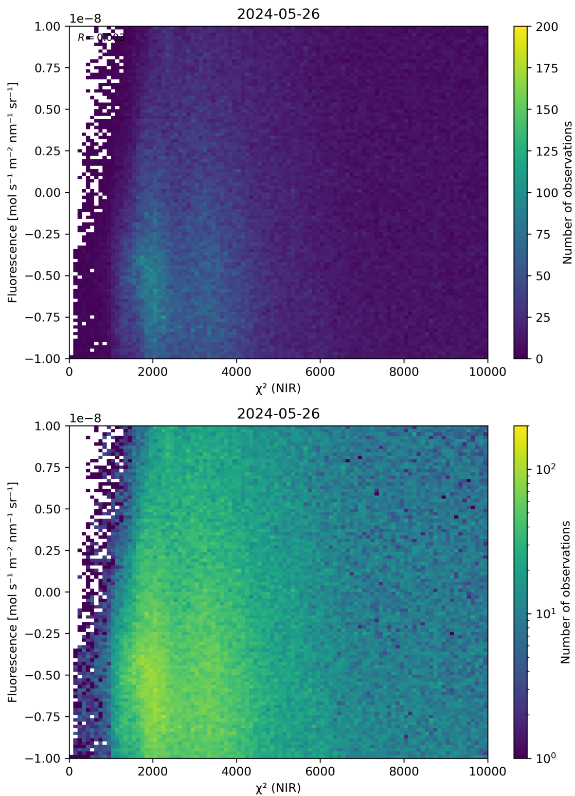
Figure 45: Scatter density plot of “ \chi^2 (NIR)” against “Fluorescence” for 2024-05-25 to 2024-05-27.
