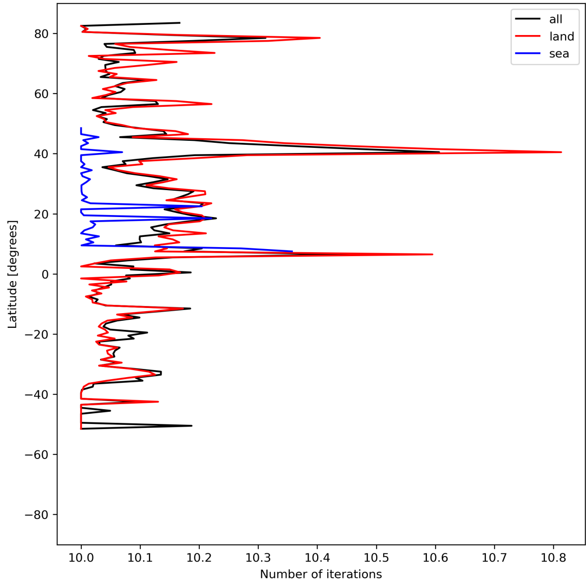
Figure 20: Zonal average of “Number of iterations” for 2024-05-25 to 2024-05-27.
