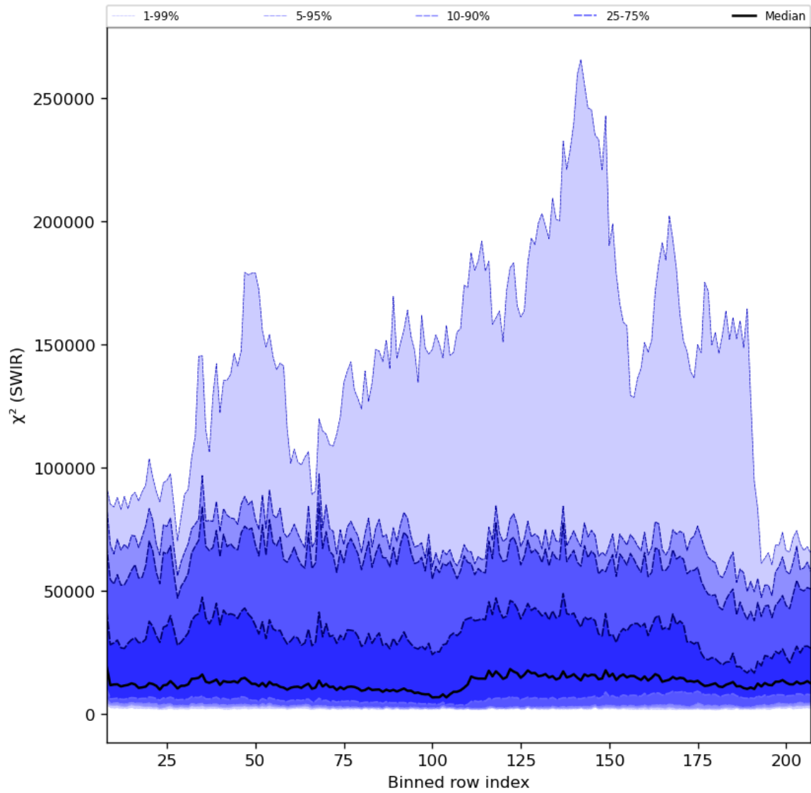
Figure 39: Along track statistics of “ \chi^2 (SWIR)” for 2024-05-25 to 2024-05-27
