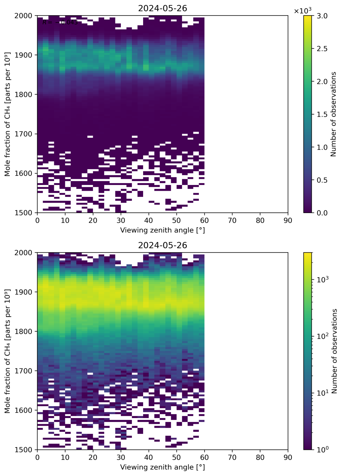
Figure 110: Scatter density plot of “Viewing zenith angle” against “Mole fraction of CH 4 ” for 2024-05-25 to 2024-05-27.
