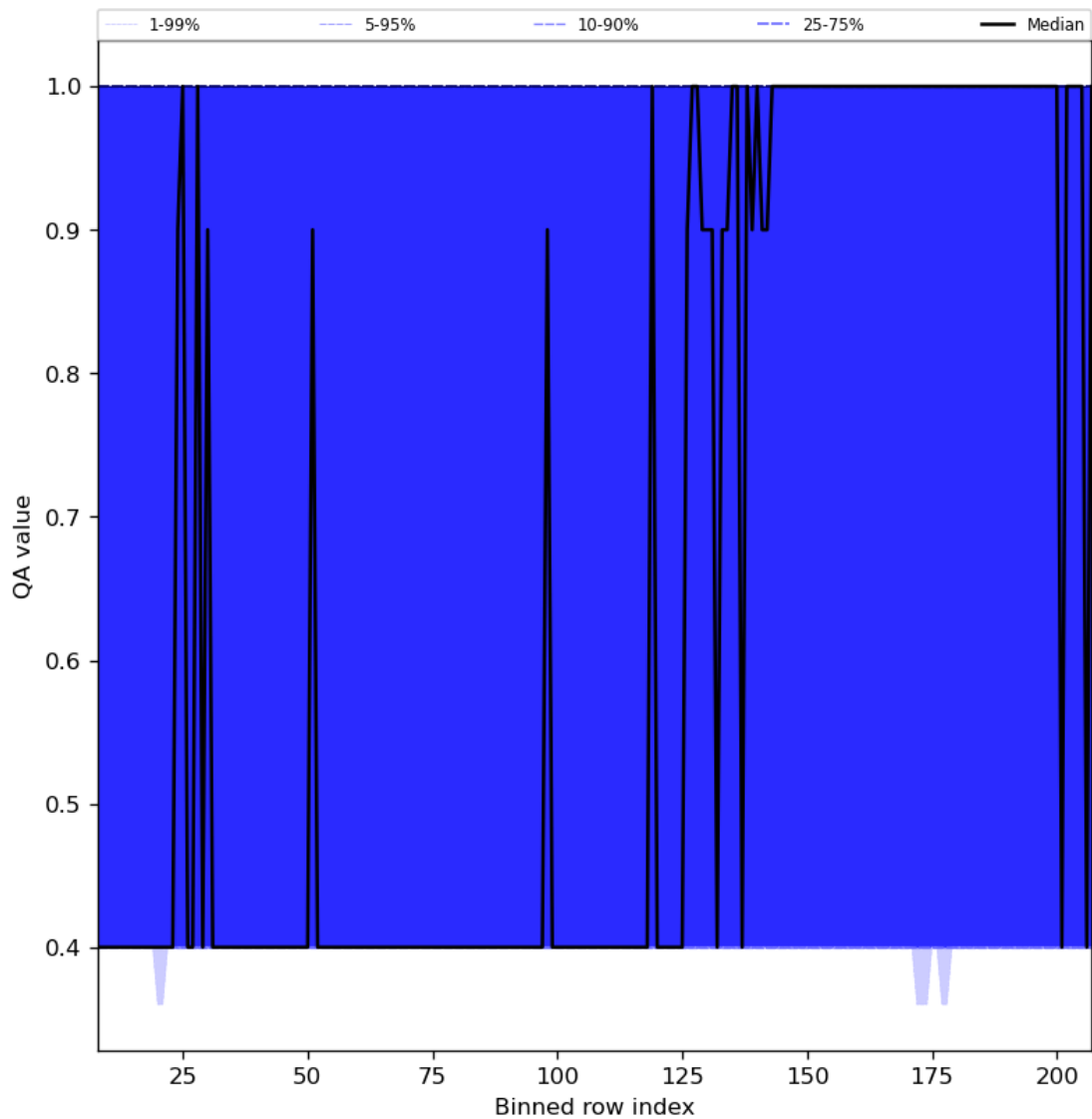
Figure 33: Along track statistics of “QA value” for 2024-05-25 to 2024-05-27
