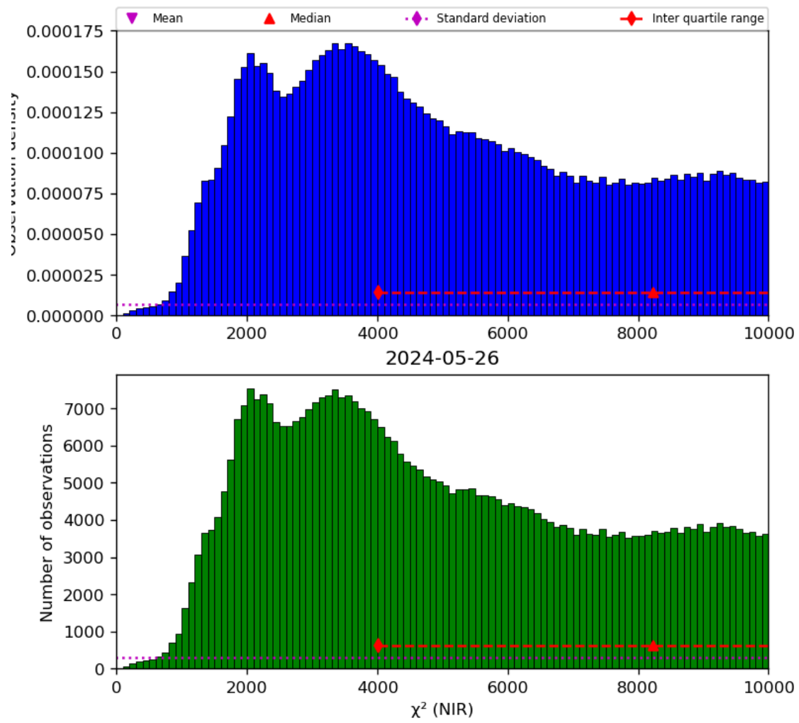
Figure 29: Histogram of “ \chi^2 (NIR)” for 2024-05-25 to 2024-05-27
