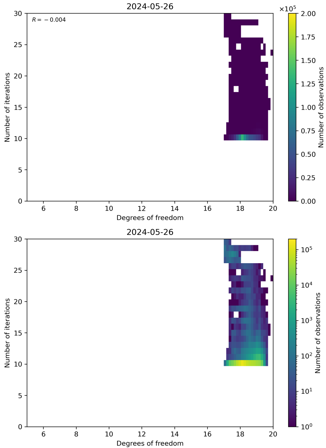
Figure 52: Scatter density plot of “Degrees of freedom” against “Number of iterations” for 2024-05-25 to 2024-05-27.
