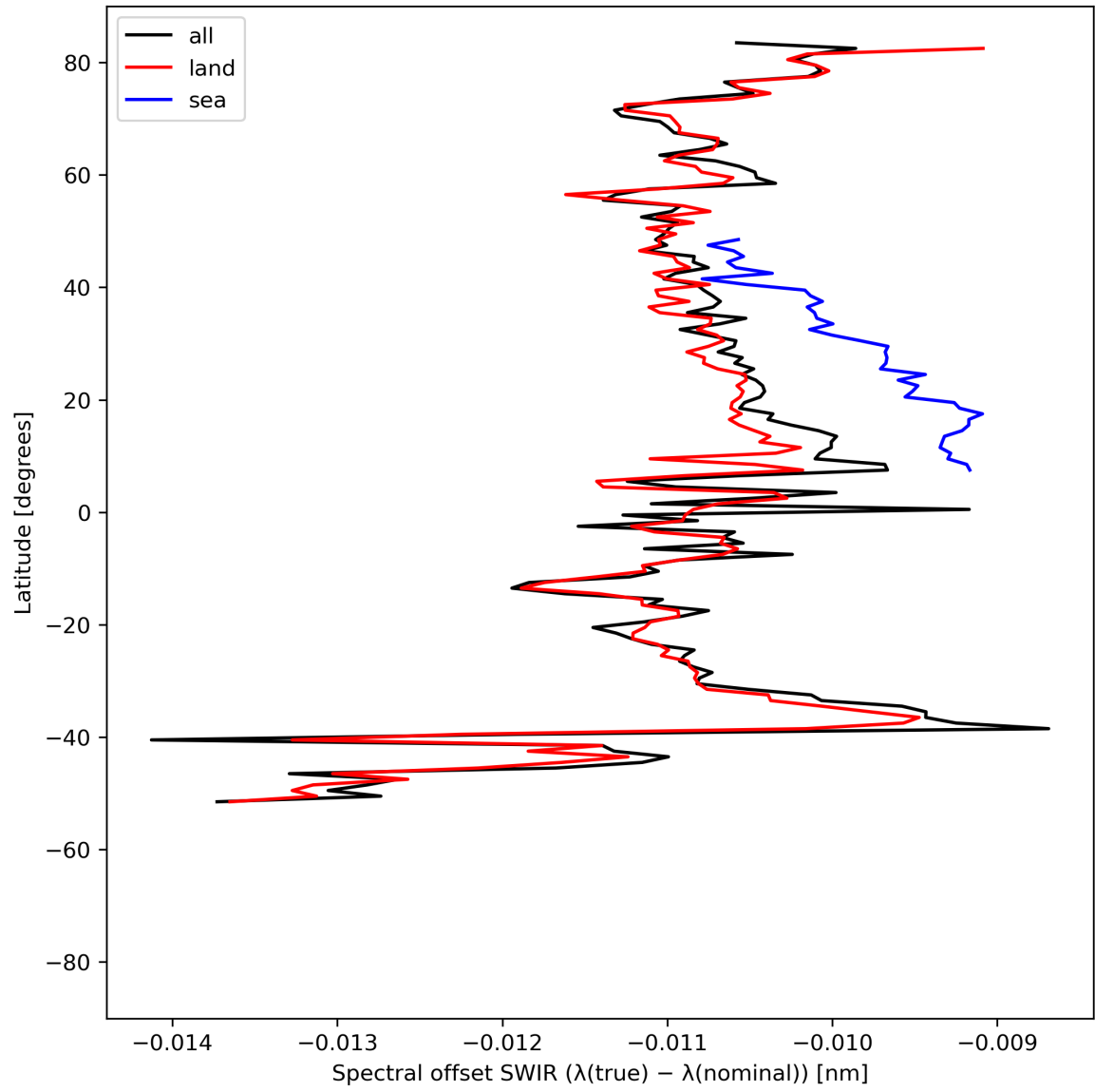
Figure 16: Zonal average of “Spectral offset SWIR ( \lambda(\text{true}) - \lambda(\text{nominal}) )” for 2024-05-25 to 2024-05-27.
