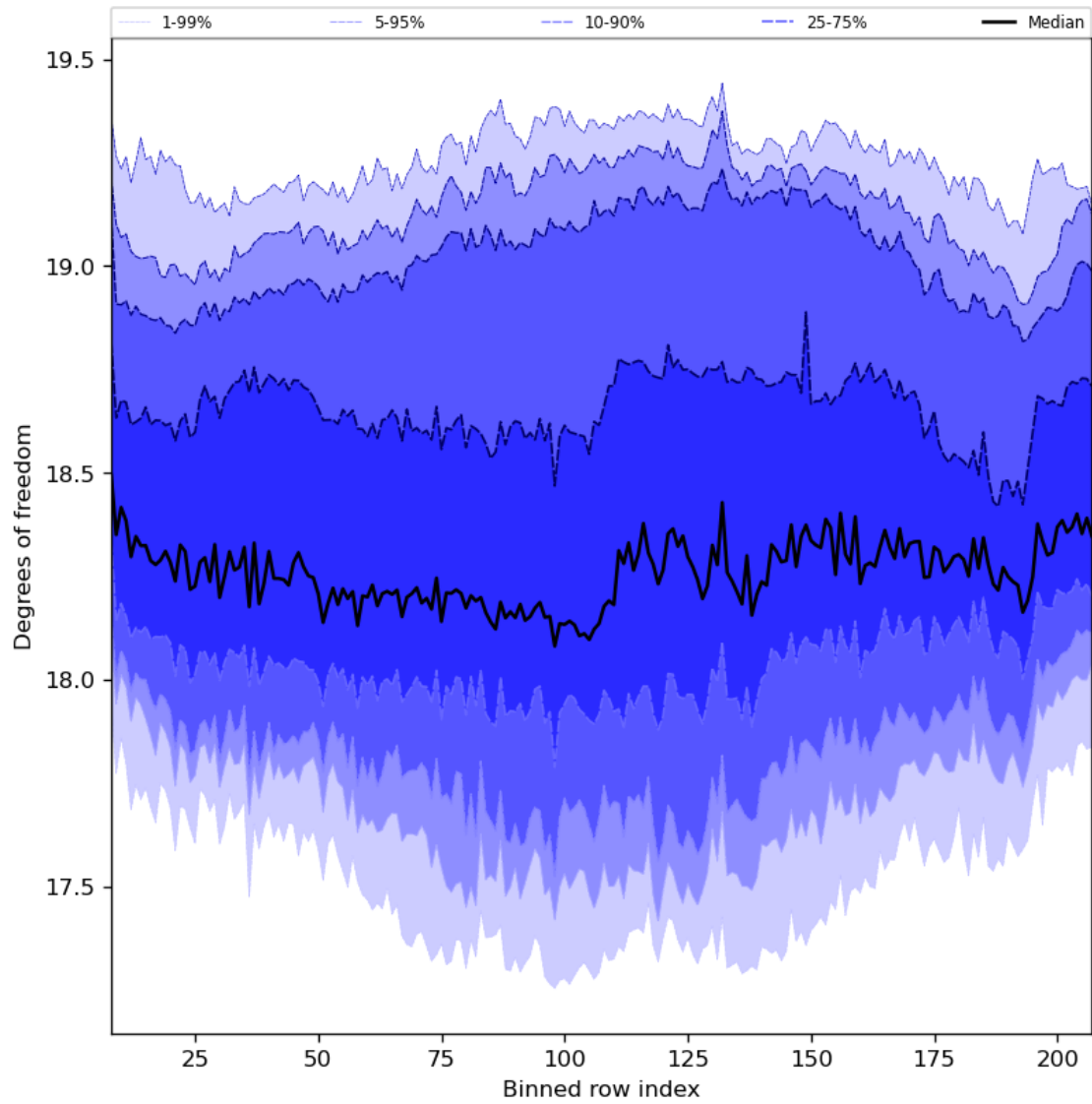
Figure 41: Along track statistics of “Degrees of freedom” for 2024-05-25 to 2024-05-27
