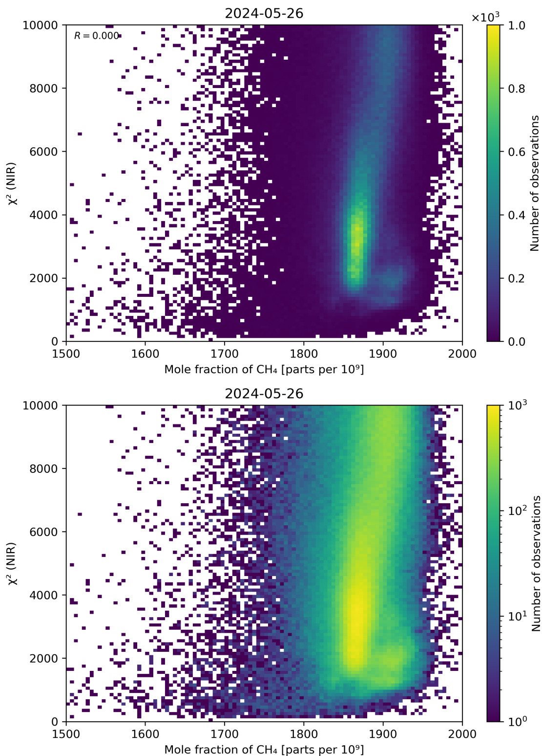
Figure 70: Scatter density plot of “Mole fraction of CH 4 ” against “ \chi^2 (NIR)” for 2024-05-25 to 2024-05-27.
