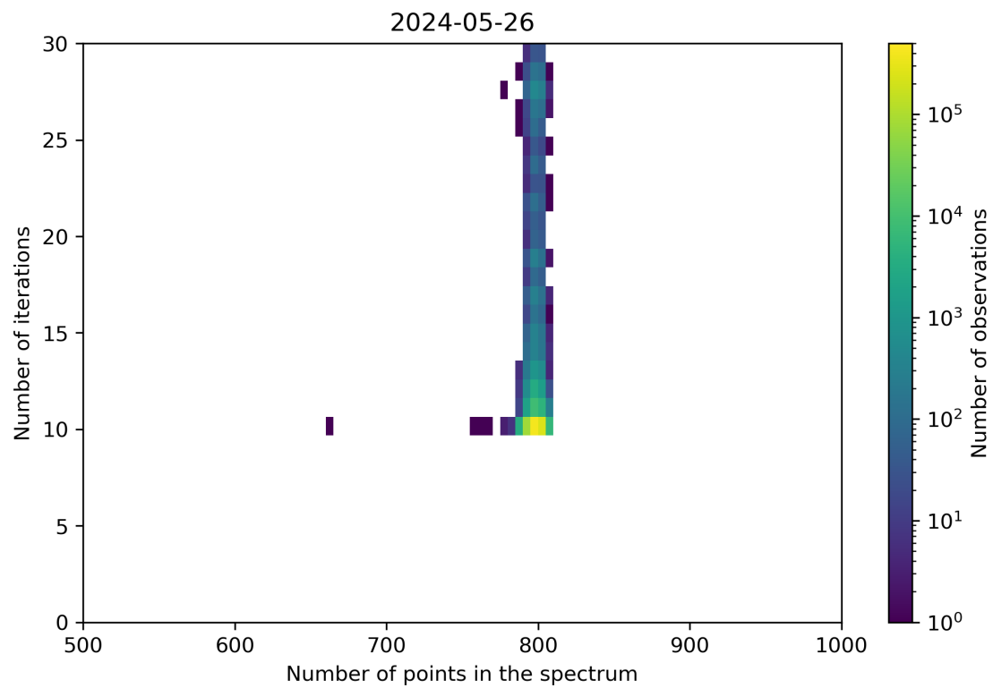
Figure 92: Scatter density plot of “Number of points in the spectrum” against “Number of iterations” for 2024-05-25 to 2024-05-27.
