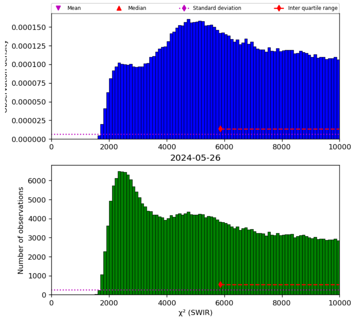
Figure 28: Histogram of “ \chi^2 (SWIR)” for 2024-05-25 to 2024-05-27
