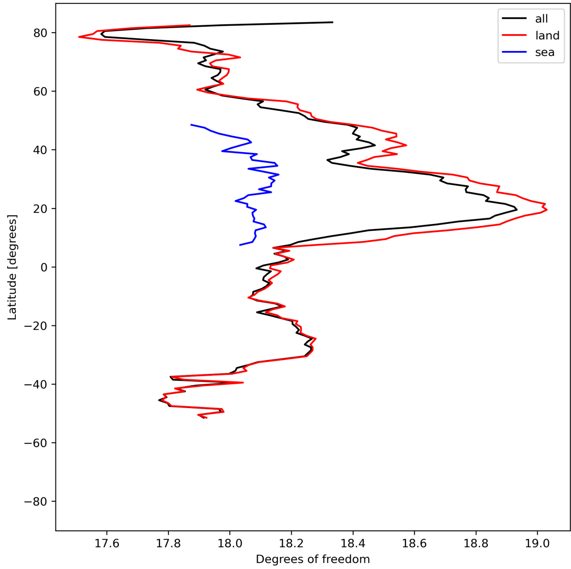
Figure 19: Zonal average of “Degrees of freedom” for 2024-05-25 to 2024-05-27.
