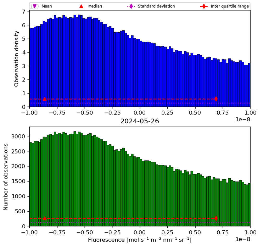
Figure 32: Histogram of “Fluorescence” for 2024-05-25 to 2024-05-27
