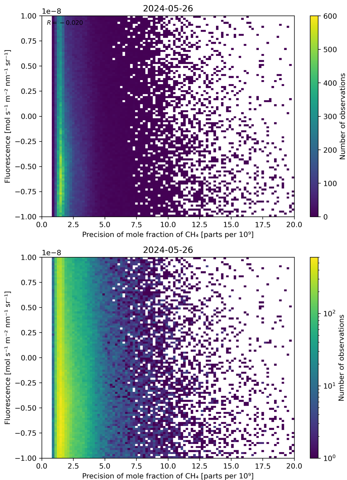
Figure 81: Scatter density plot of “Precision of mole fraction of CH 4 ” against “Fluorescence” for 2024-05-25 to 2024-05-27.
