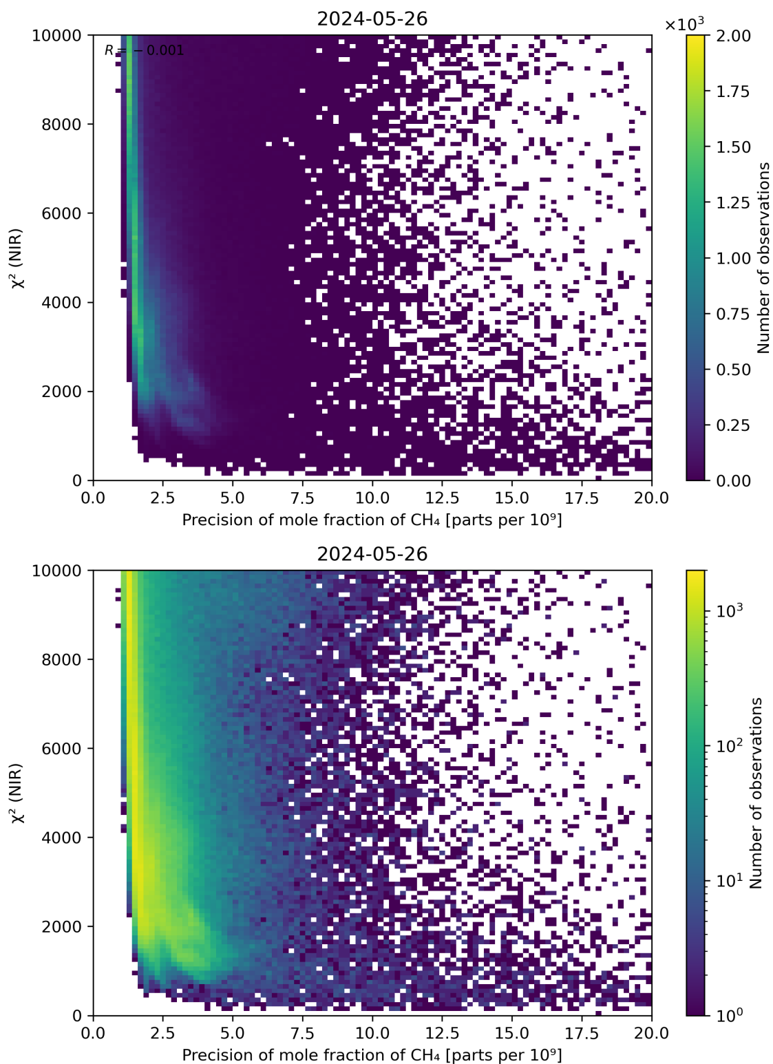
Figure 78: Scatter density plot of “Precision of mole fraction of CH 4 ” against “ \chi^2 (NIR)” for 2024-05-25 to 2024-05-27.
