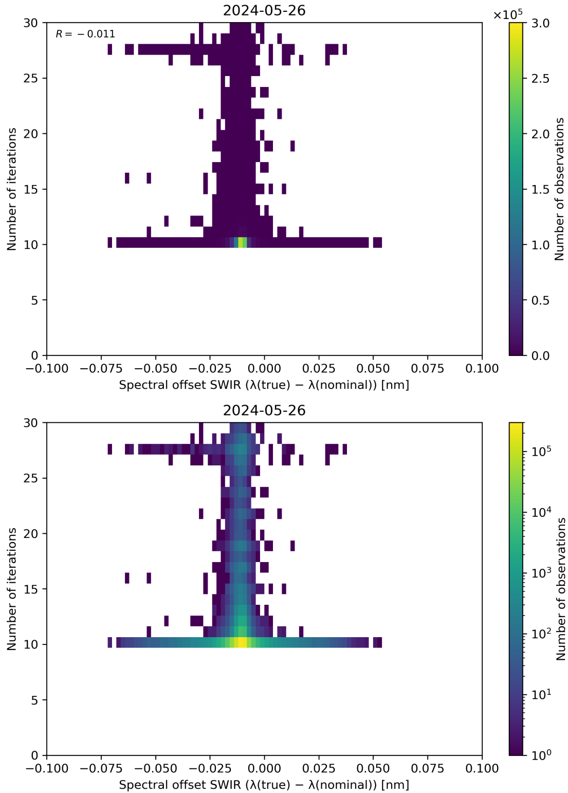
Figure 121: Scatter density plot of “Spectral offset SWIR ( \lambda(\text{true}) - \lambda(\text{nominal}) )” against “Number of iterations” for 2024-05-25 to 2024-05-27.
