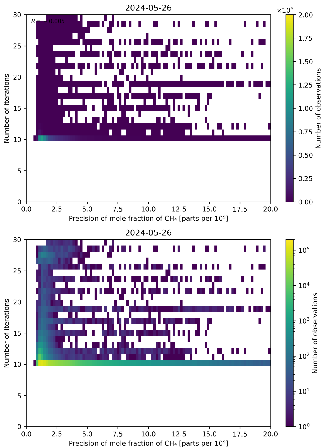
Figure 83: Scatter density plot of “Precision of mole fraction of CH 4 ” against “Number of iterations” for 2024-05-25 to 2024-05-27.
