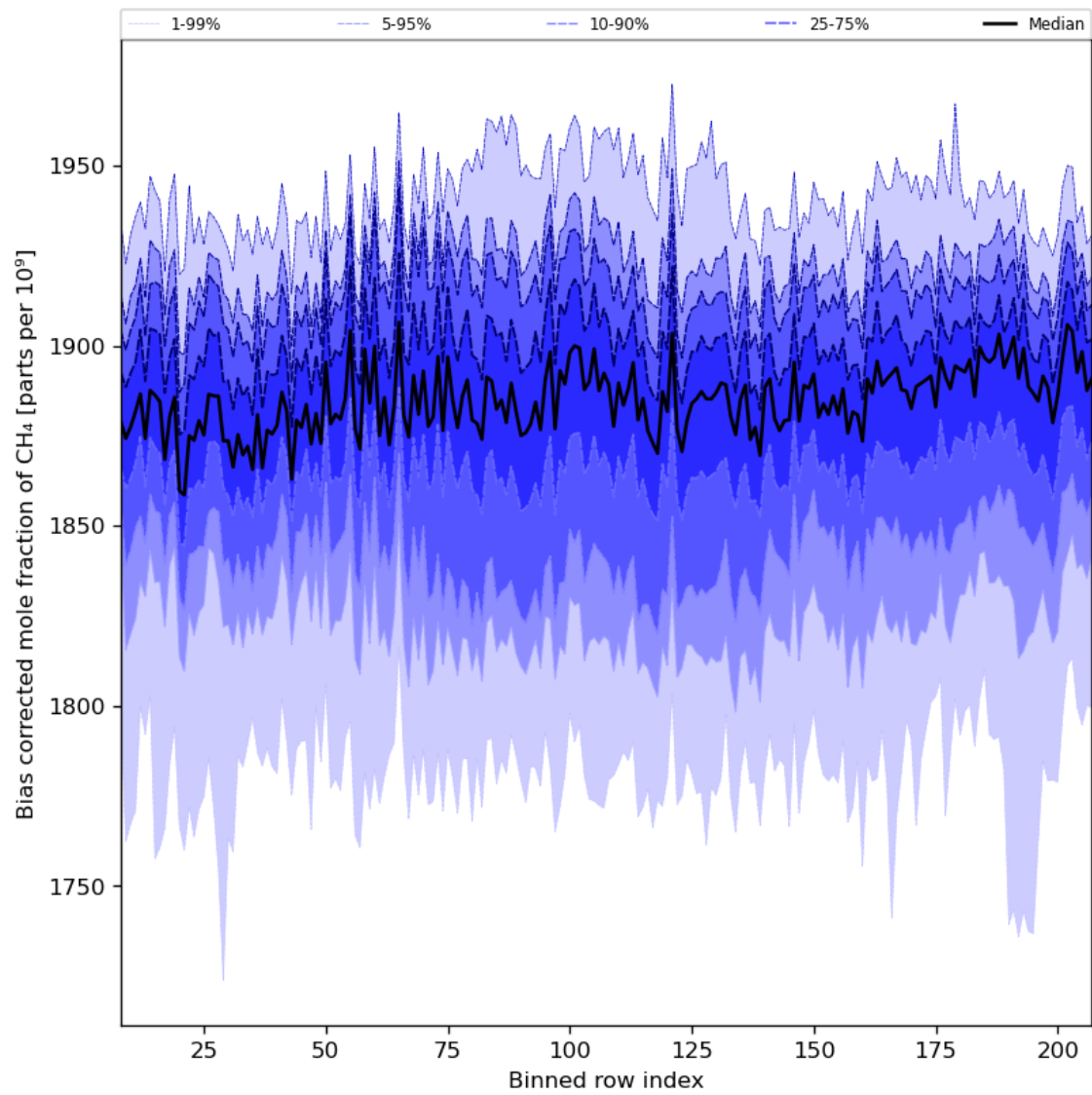
Figure 36: Along track statistics of “Bias corrected mole fraction of CH 4 ” for 2024-05-28 to 2024-05-29
