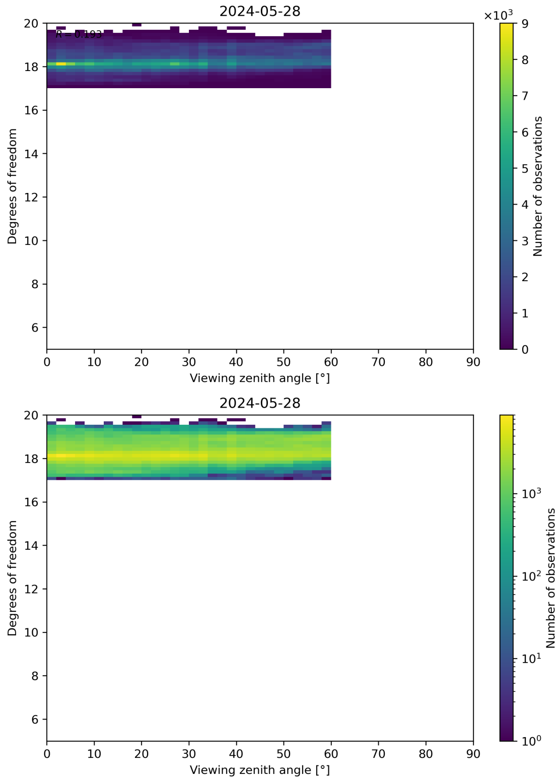
Figure 107: Scatter density plot of “Viewing zenith angle” against “Degrees of freedom” for 2024-05-28 to 2024-05-29.
