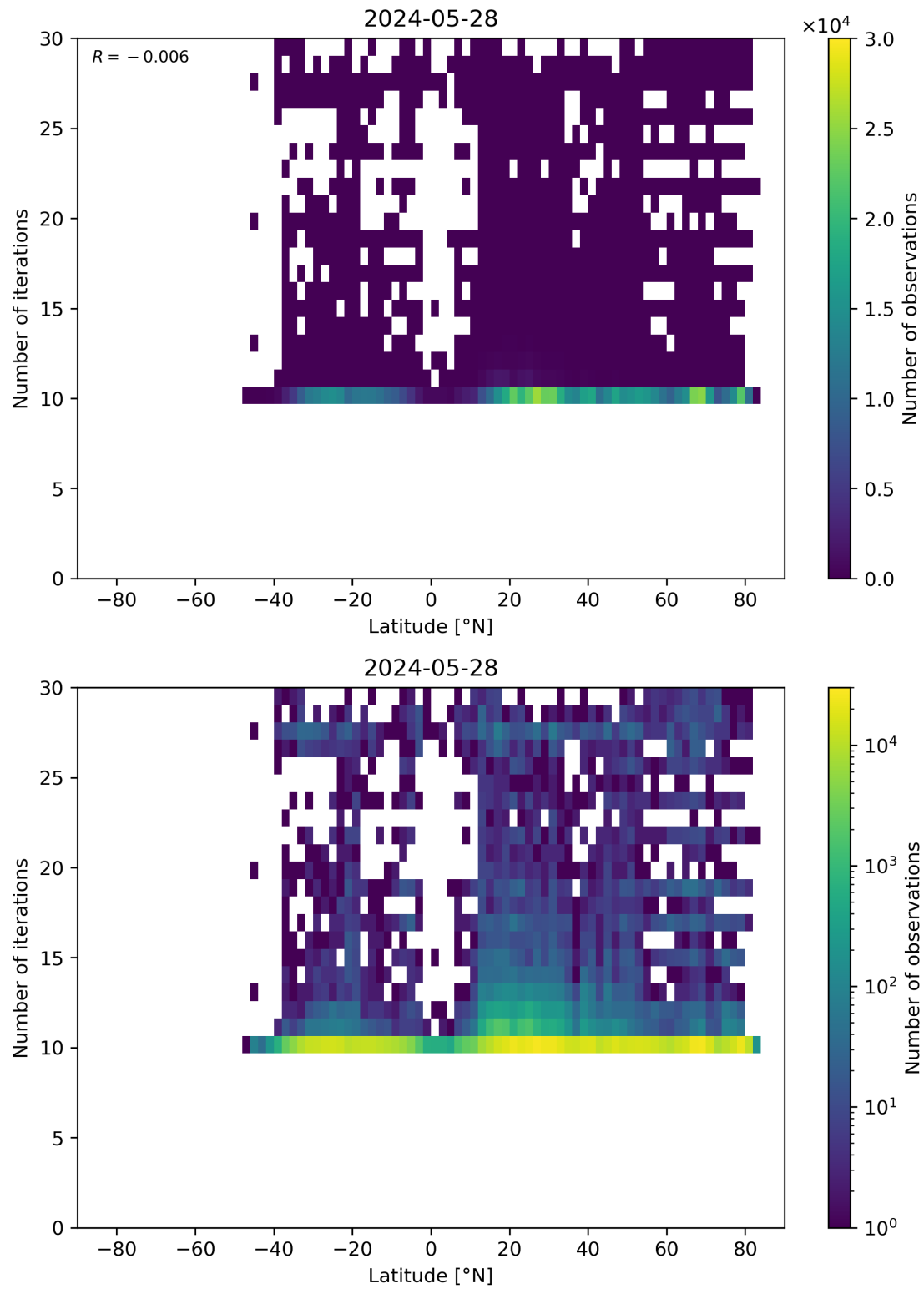
Figure 60: Scatter density plot of “Latitude” against “Number of iterations” for 2024-05-28 to 2024-05-29.
