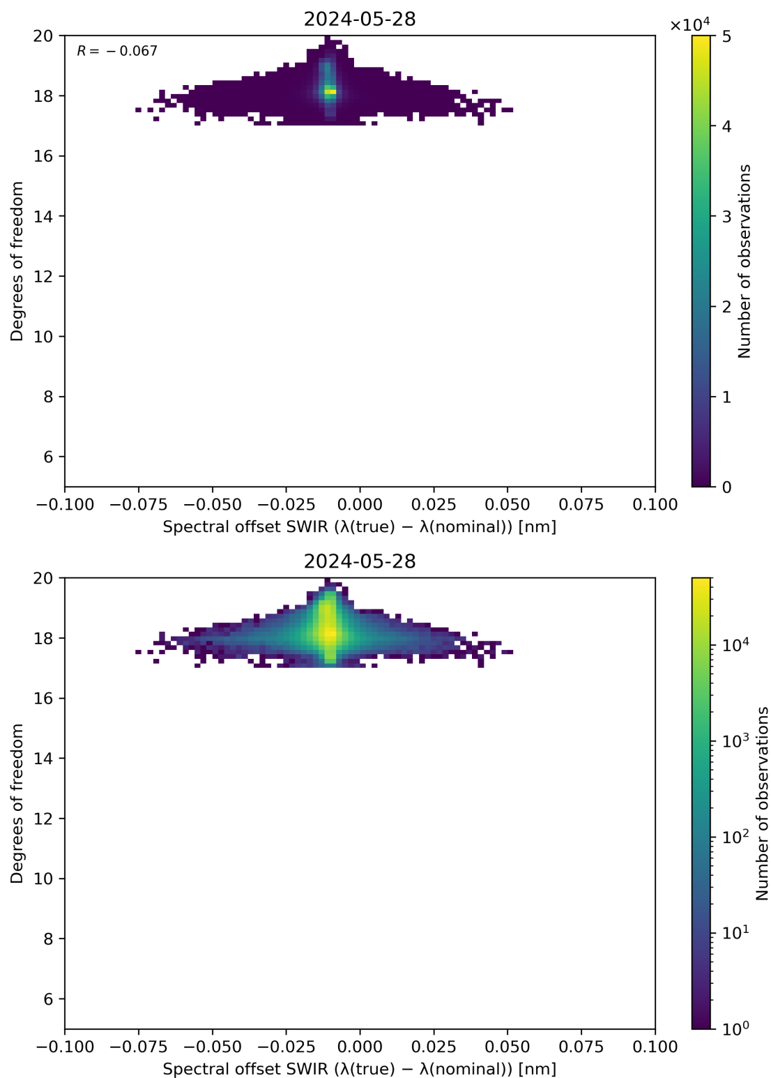
Figure 119: Scatter density plot of “Spectral offset SWIR ( \lambda(\text{true}) - \lambda(\text{nominal}) )” against “Degrees of freedom” for 2024-05-28 to 2024-05-29.
