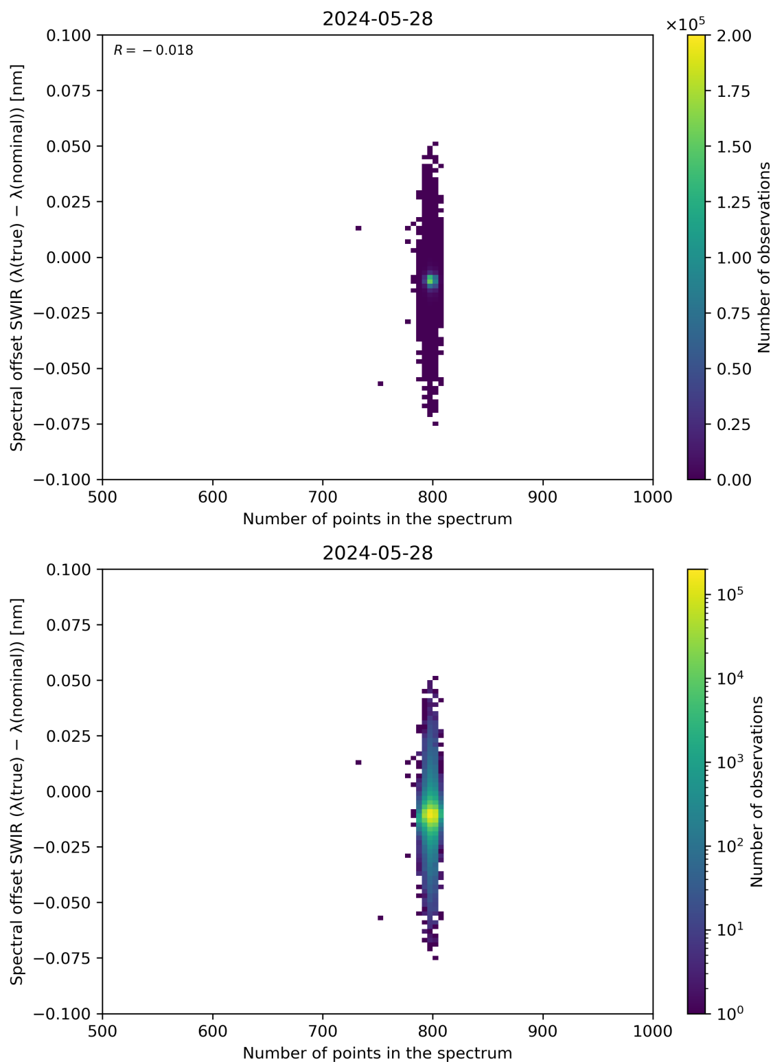
Figure 93: Scatter density plot of “Number of points in the spectrum” against “Spectral offset SWIR ( \lambda(\text{true}) - \lambda(\text{nominal}) )” for 2024-05-28 to 2024-05-29.
