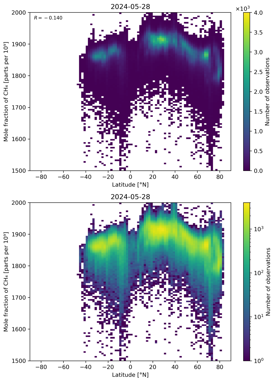
Figure 57: Scatter density plot of “Latitude” against “Mole fraction of \text{CH}_4 ” for 2024-05-28 to 2024-05-29.
