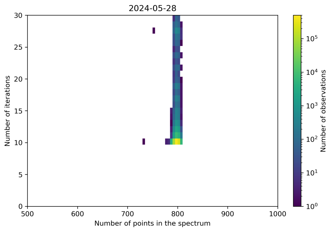
Figure 92: Scatter density plot of “Number of points in the spectrum” against “Number of iterations” for 2024-05-28 to 2024-05-29.
