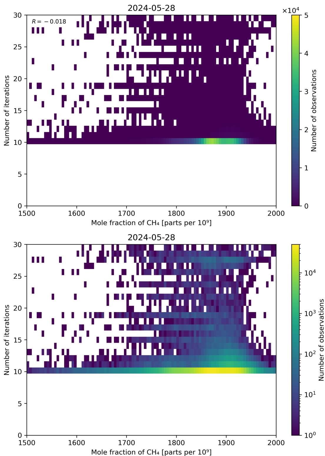
Figure 76: Scatter density plot of “Mole fraction of CH 4 ” against “Number of iterations” for 2024-05-28 to 2024-05-29.
