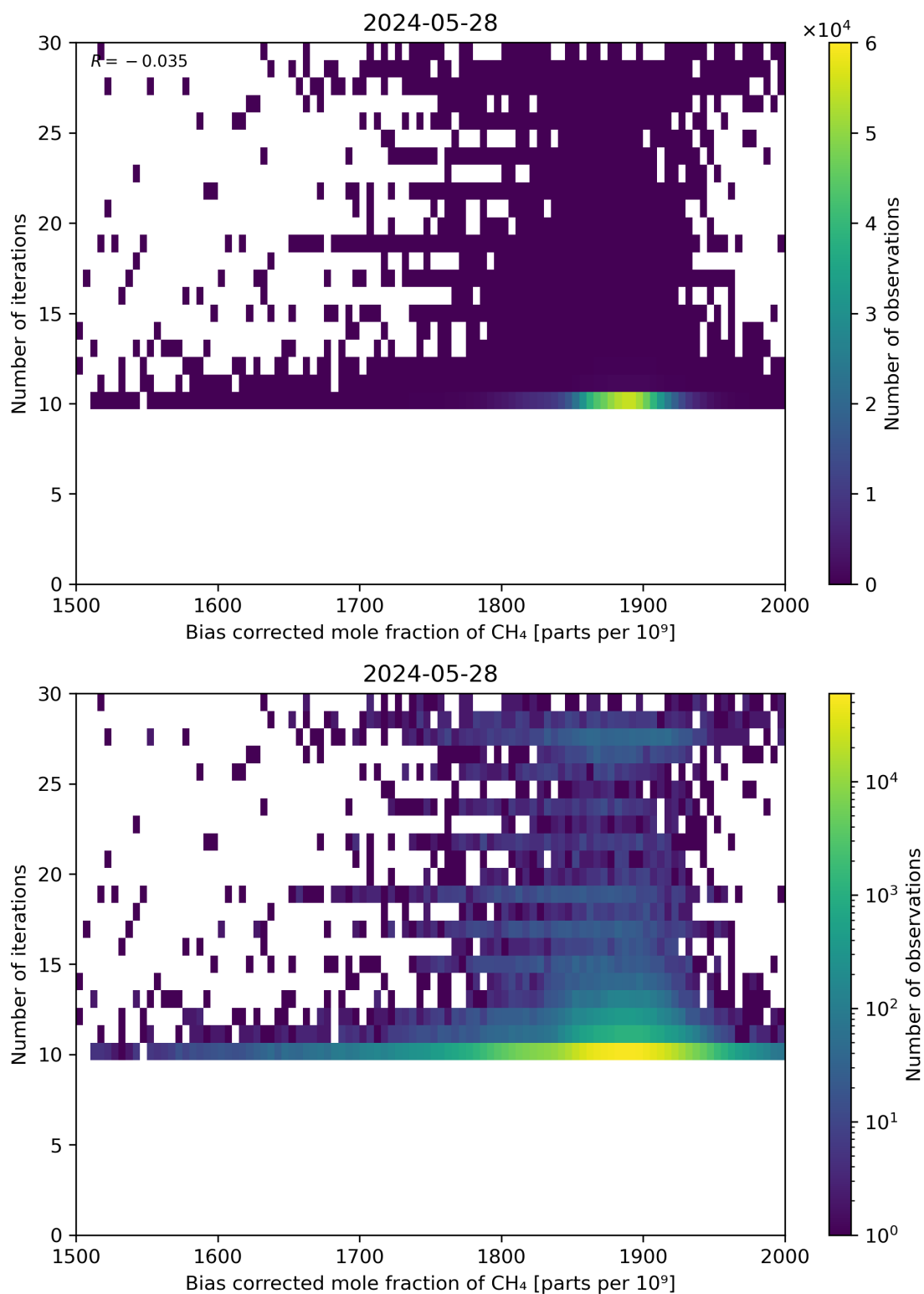
Figure 67: Scatter density plot of “Bias corrected mole fraction of CH 4 ” against “Number of iterations” for 2024-05-28 to 2024-05-29.
