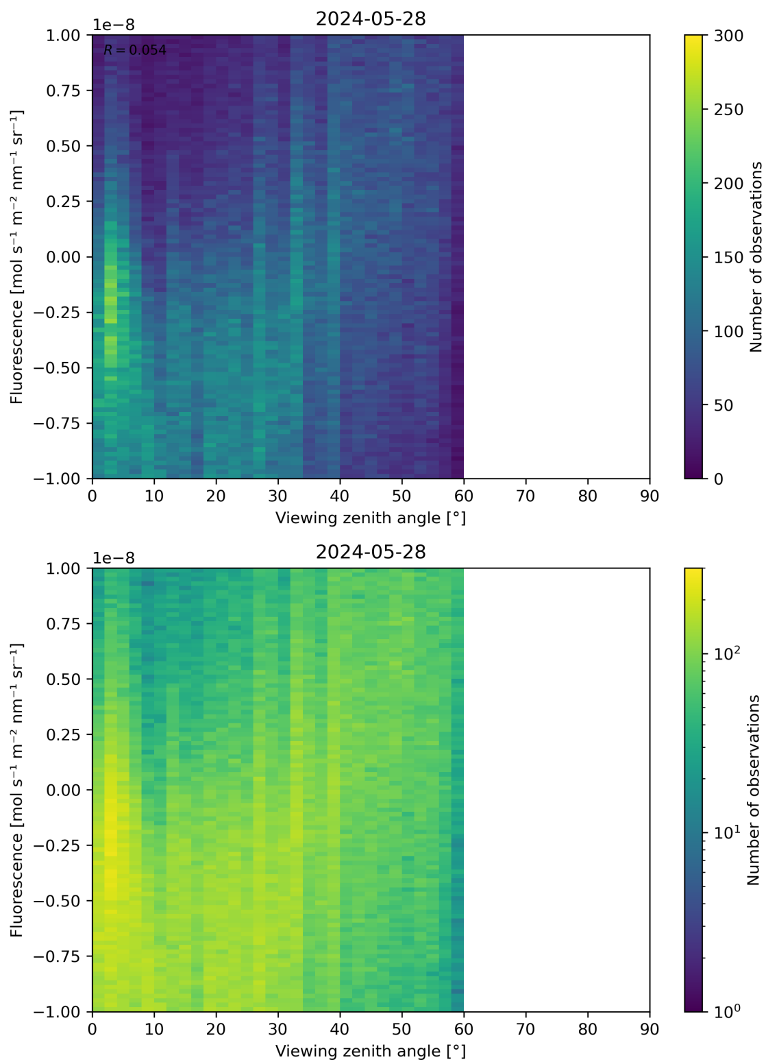
Figure 108: Scatter density plot of “Viewing zenith angle” against “Fluorescence” for 2024-05-28 to 2024-05-29.
