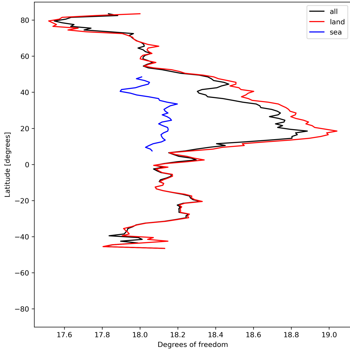
Figure 19: Zonal average of “Degrees of freedom” for 2024-05-28 to 2024-05-29.
