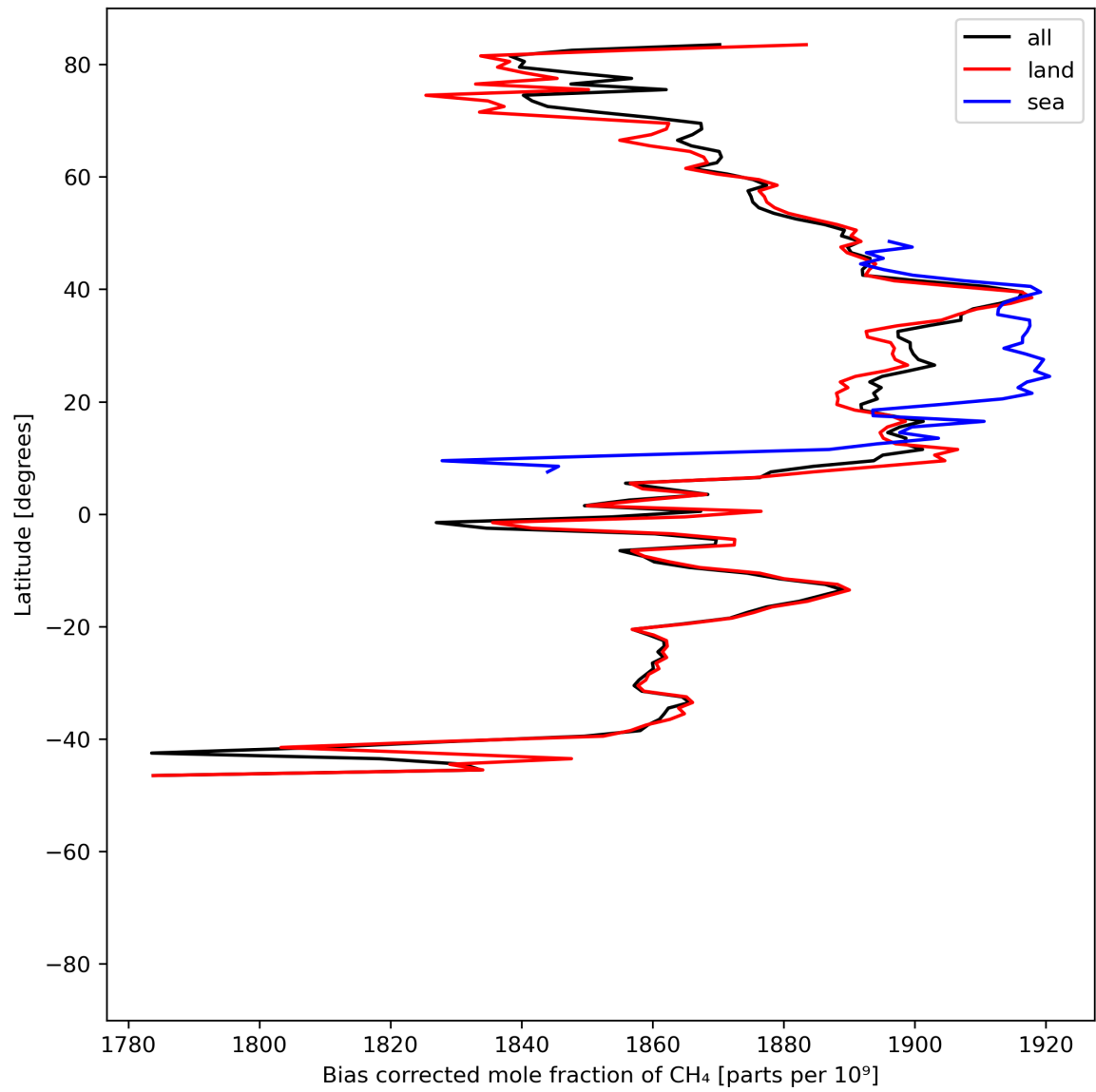
Figure 14: Zonal average of “Bias corrected mole fraction of \text{CH}_4 ” for 2024-05-28 to 2024-05-29.
