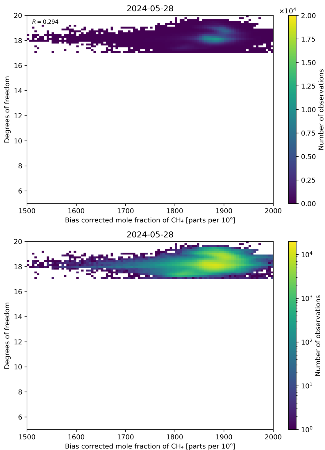
Figure 65: Scatter density plot of “Bias corrected mole fraction of CH 4 ” against “Degrees of freedom” for 2024-05-28 to 2024-05-29.
