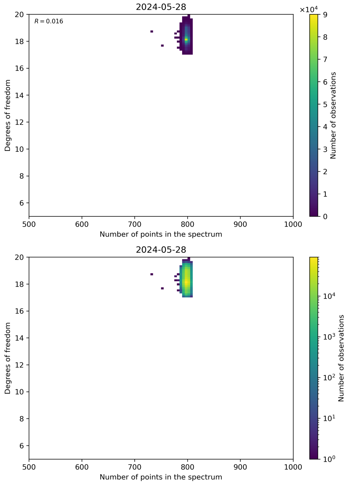
Figure 90: Scatter density plot of “Number of points in the spectrum” against “Degrees of freedom” for 2024-05-28 to 2024-05-29.
