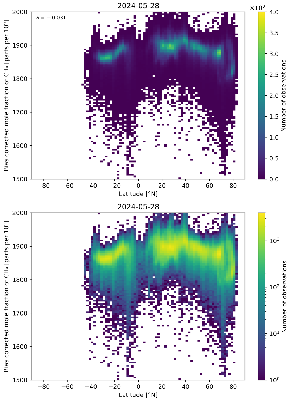
Figure 58: Scatter density plot of “Latitude” against “Bias corrected mole fraction of CH 4 ” for 2024-05-28 to 2024-05-29.
