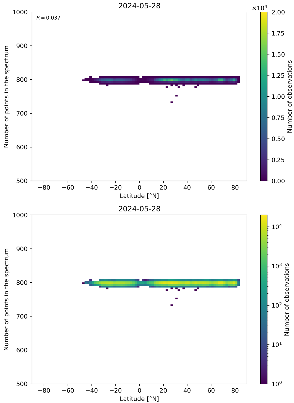
Figure 61: Scatter density plot of “Latitude” against “Number of points in the spectrum” for 2024-05-28 to 2024-05-29.
