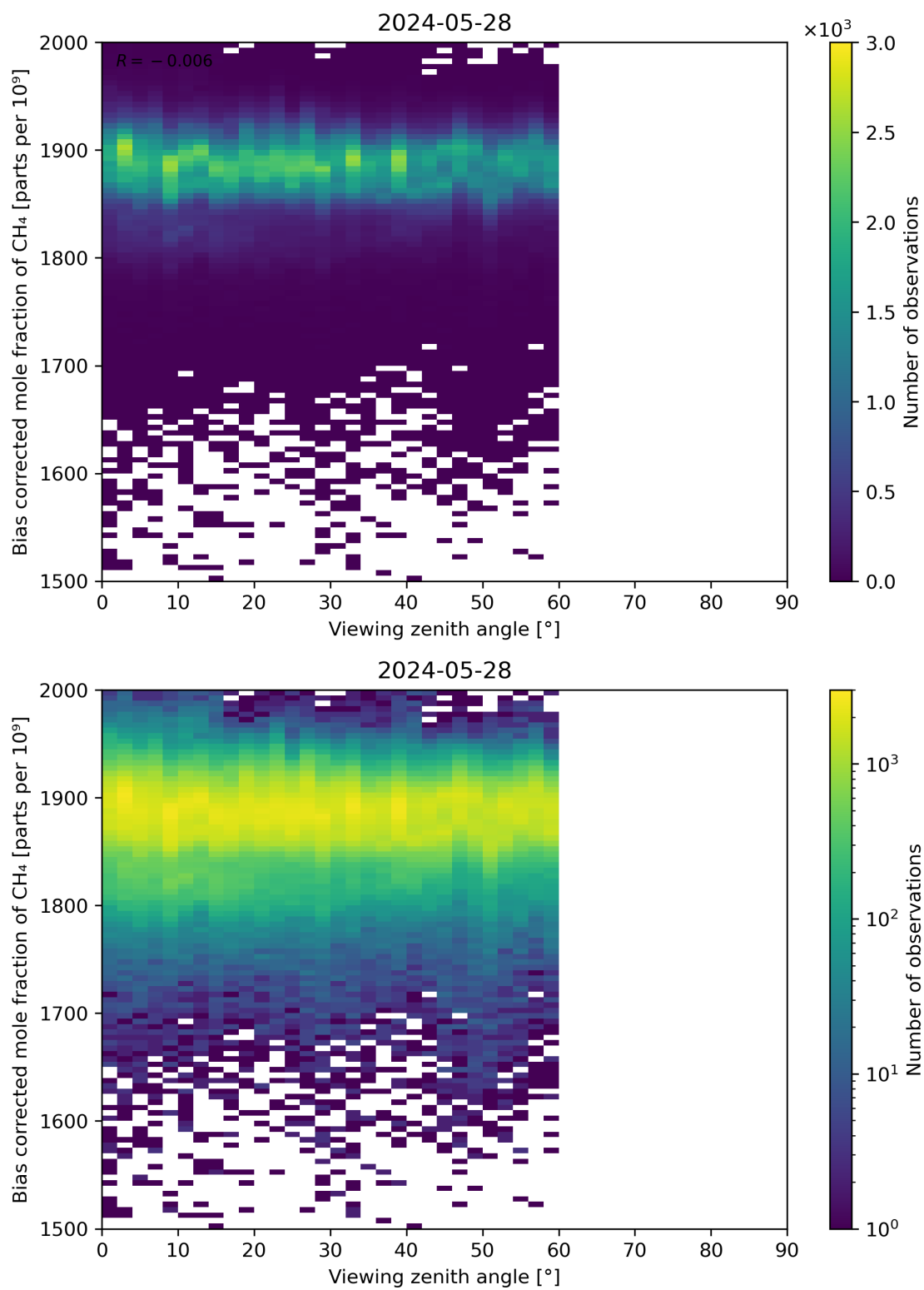
Figure 111: Scatter density plot of “Viewing zenith angle” against “Bias corrected mole fraction of CH 4 ” for 2024-05-28 to 2024-05-29.
