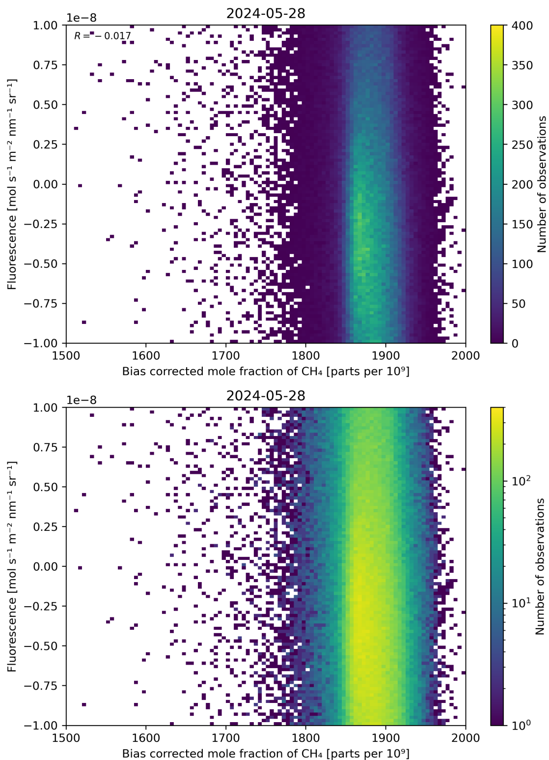
Figure 66: Scatter density plot of “Bias corrected mole fraction of \text{CH}_4 ” against “Fluorescence” for 2024-05-28 to 2024-05-29.
