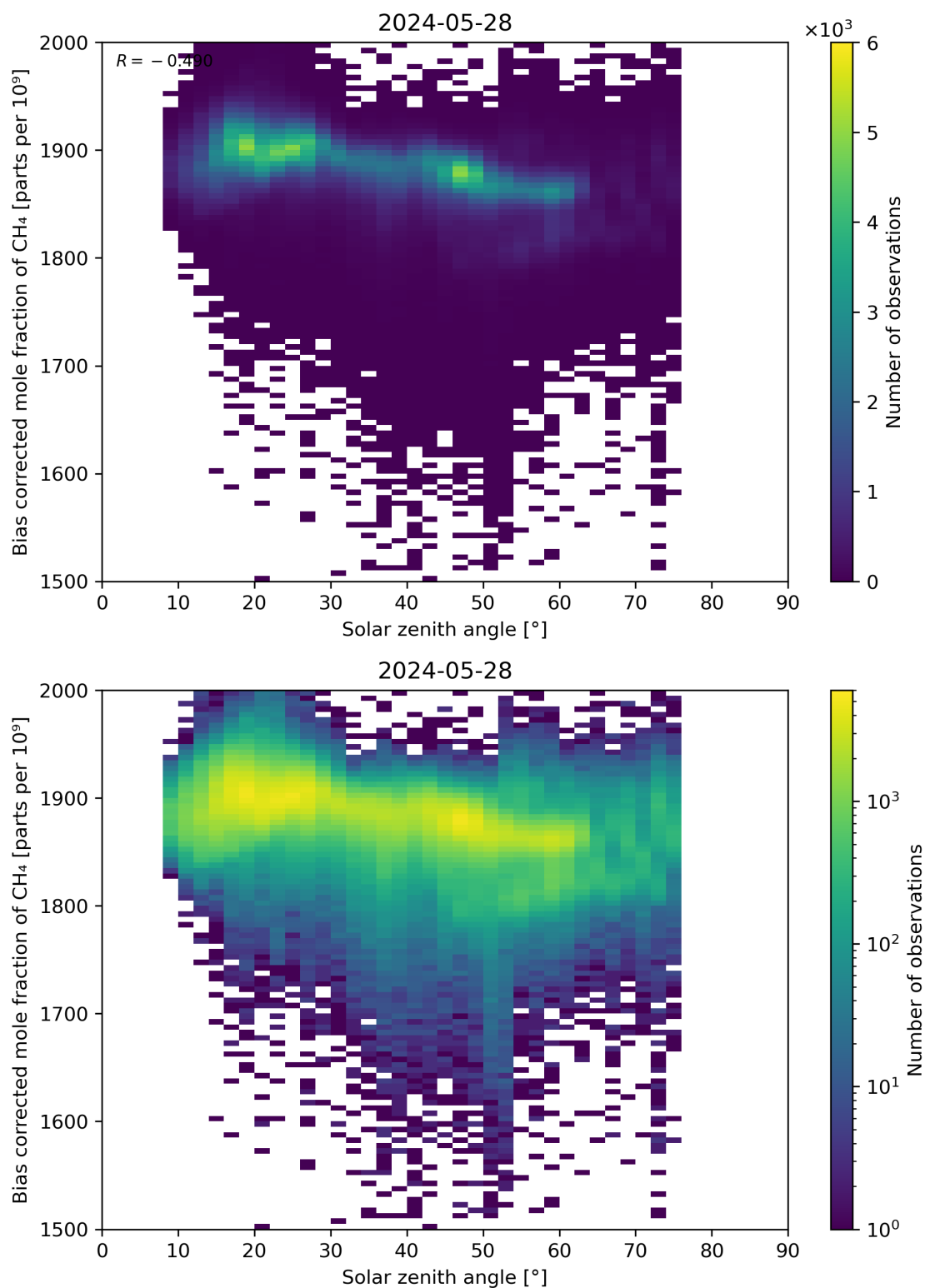
Figure 100: Scatter density plot of “Solar zenith angle” against “Bias corrected mole fraction of CH 4 ” for 2024-05-28 to 2024-05-29.
