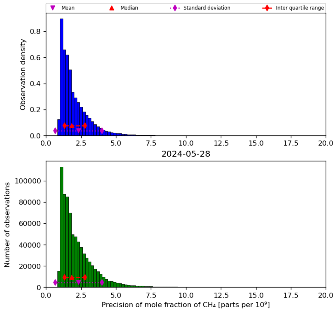
Figure 24: Histogram of “Precision of mole fraction of CH 4 ” for 2024-05-28 to 2024-05-29
