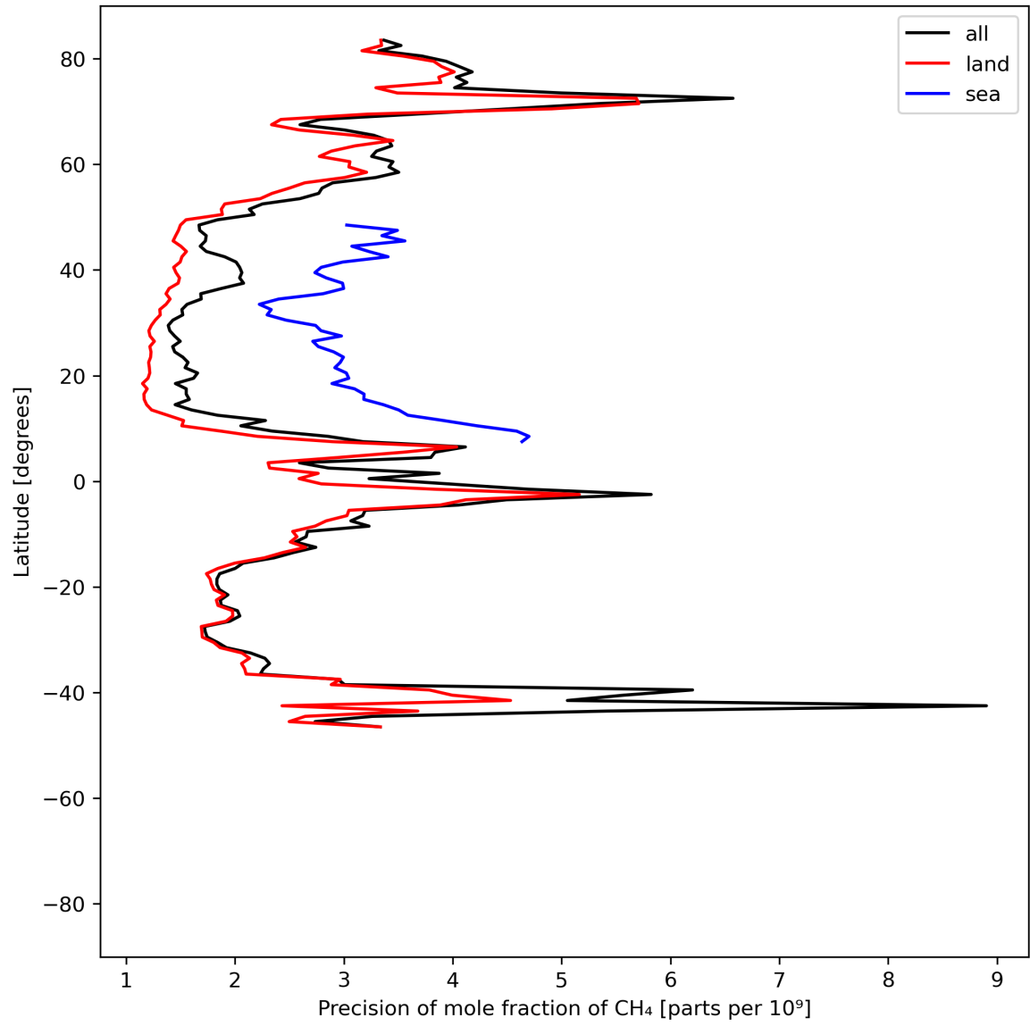
Figure 13: Zonal average of “Precision of mole fraction of CH 4 ” for 2024-05-28 to 2024-05-29.
