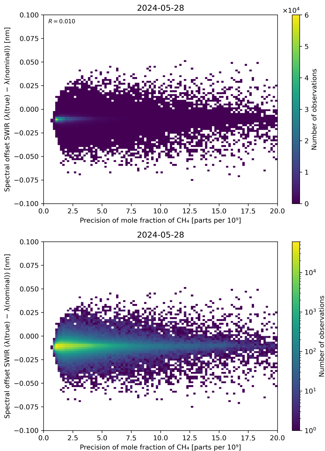
Figure 85: Scatter density plot of “Precision of mole fraction of CH 4 ” against “Spectral offset SWIR ( \lambda(\text{true}) - \lambda(\text{nominal}) )” for 2024-05-28 to 2024-05-29.
