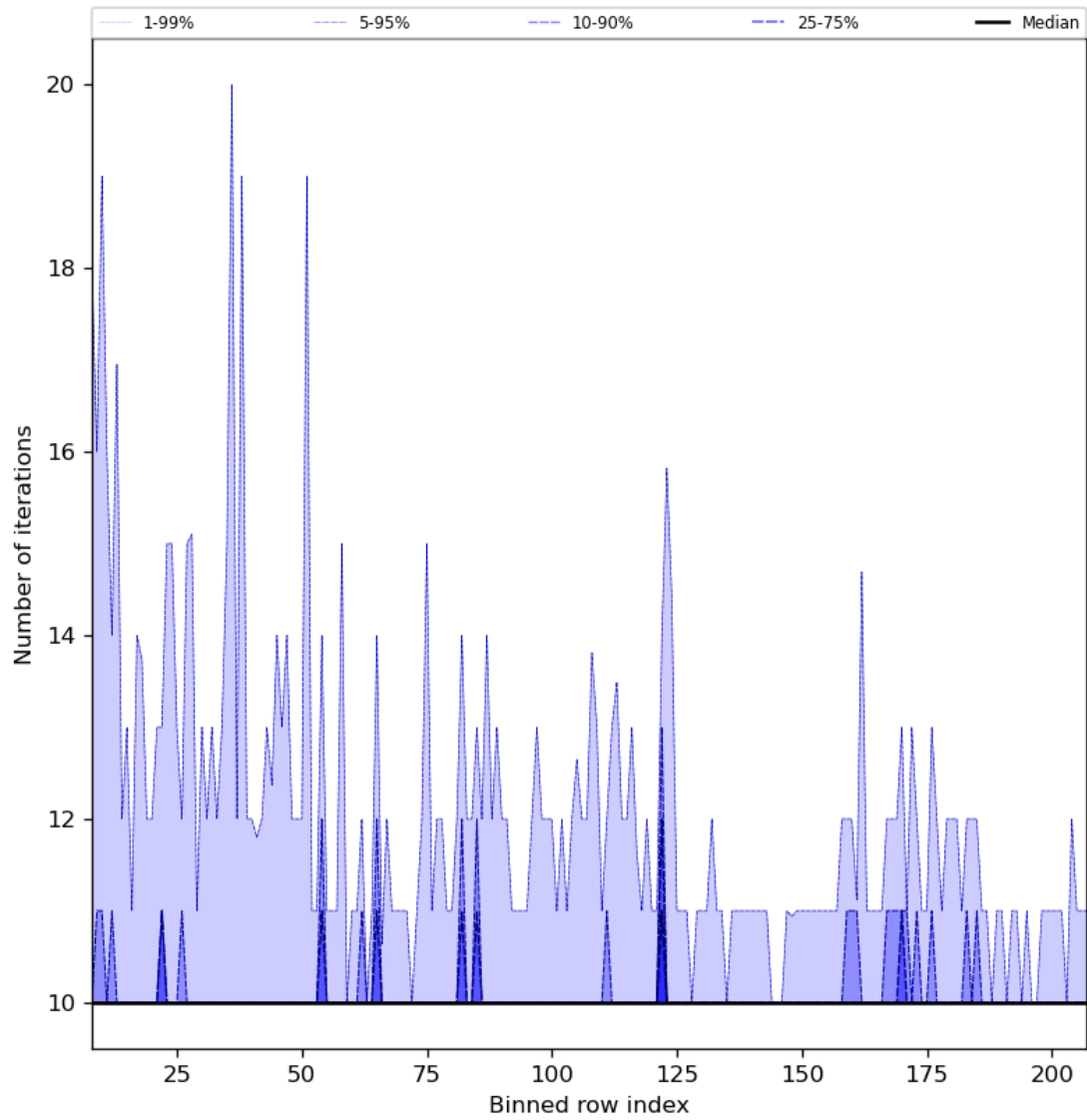
Figure 42: Along track statistics of “Number of iterations” for 2024-05-28 to 2024-05-29
