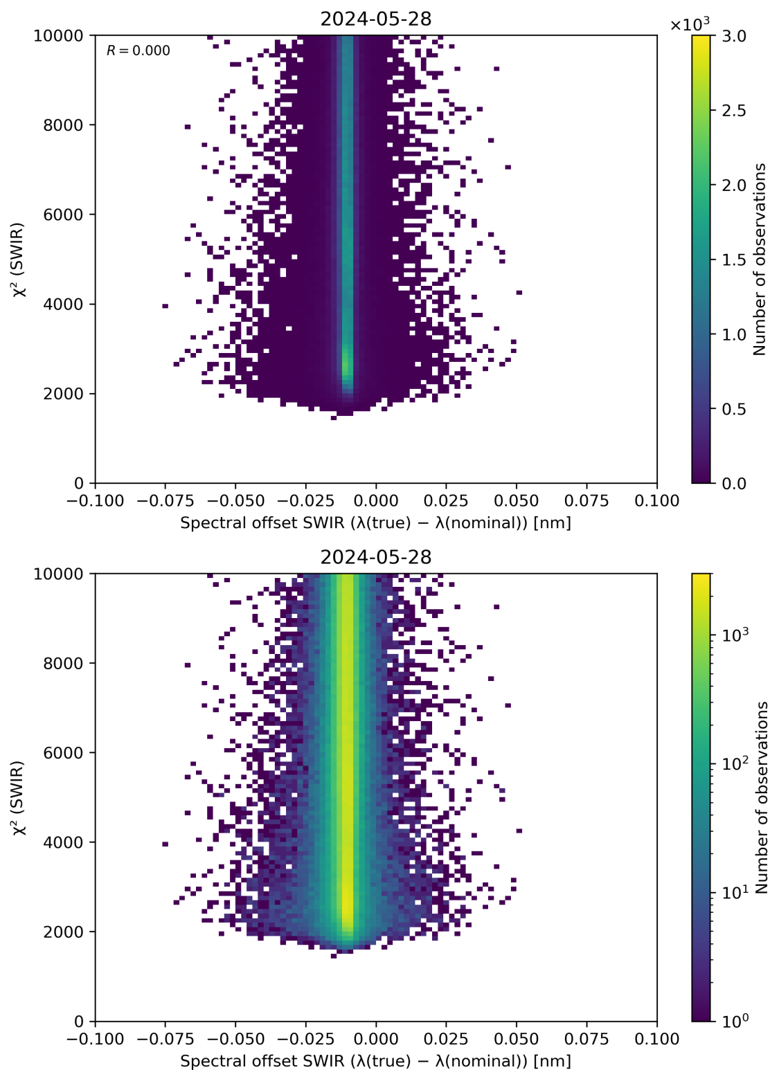
Figure 118: Scatter density plot of “Spectral offset SWIR ( \lambda(\text{true}) - \lambda(\text{nominal}) )” against “ \chi^2 (SWIR)” for 2024-05-28 to 2024-05-29.
