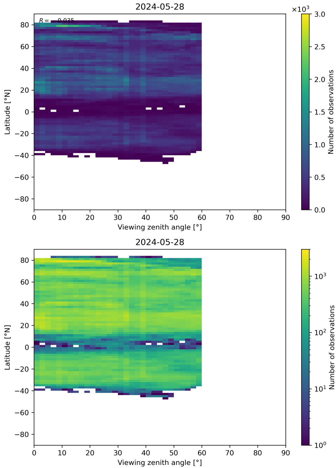
Figure 109: Scatter density plot of “Viewing zenith angle” against “Latitude” for 2024-05-28 to 2024-05-29.
