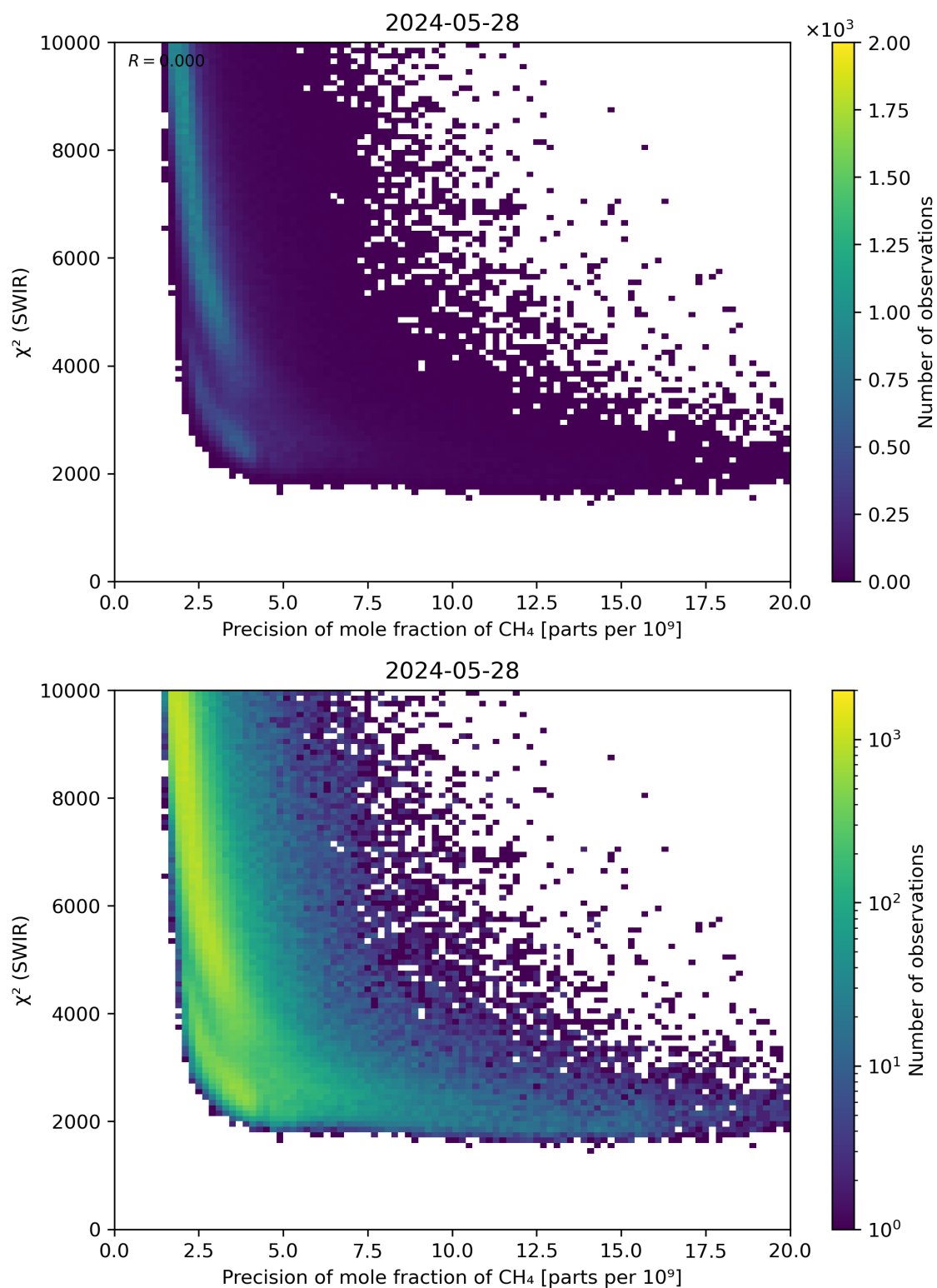
Figure 79: Scatter density plot of “Precision of mole fraction of \text{CH}_4 ” against “ \chi^2 (SWIR)” for 2024-05-28 to 2024-05-29.
