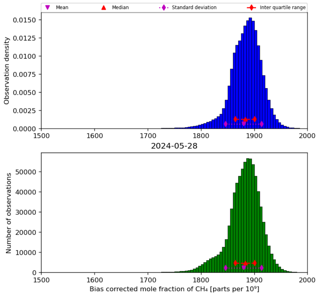
Figure 25: Histogram of “Bias corrected mole fraction of CH 4 ” for 2024-05-28 to 2024-05-29
