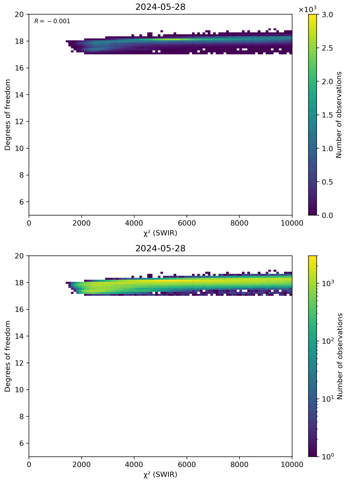
Figure 48: Scatter density plot of “ \chi^2 (SWIR)” against “Degrees of freedom” for 2024-05-28 to 2024-05-29.
