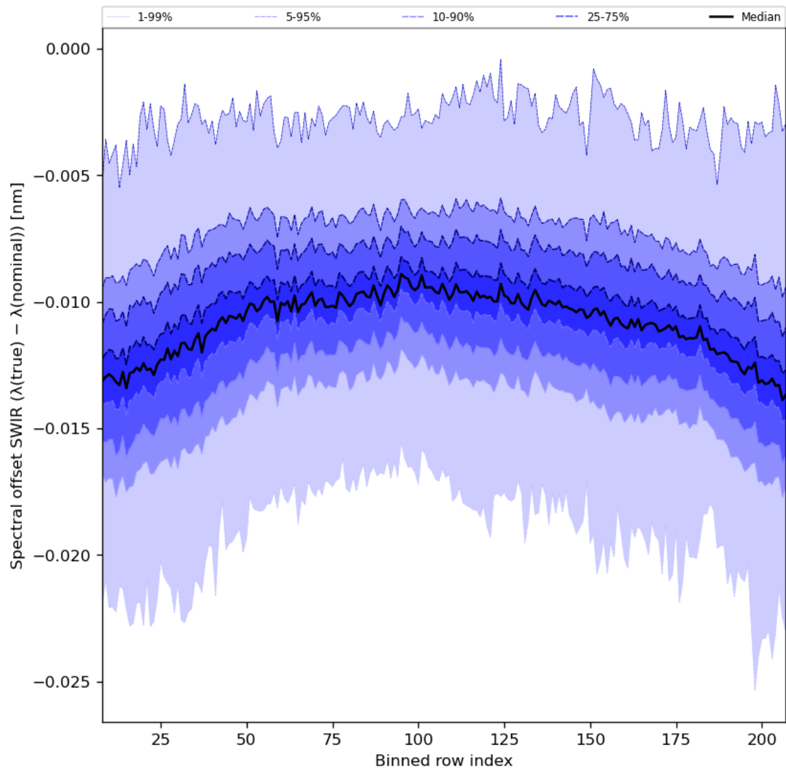
Figure 38: Along track statistics of “Spectral offset SWIR ( \lambda(\text{true}) - \lambda(\text{nominal}) )” for 2024-05-28 to 2024-05-29
