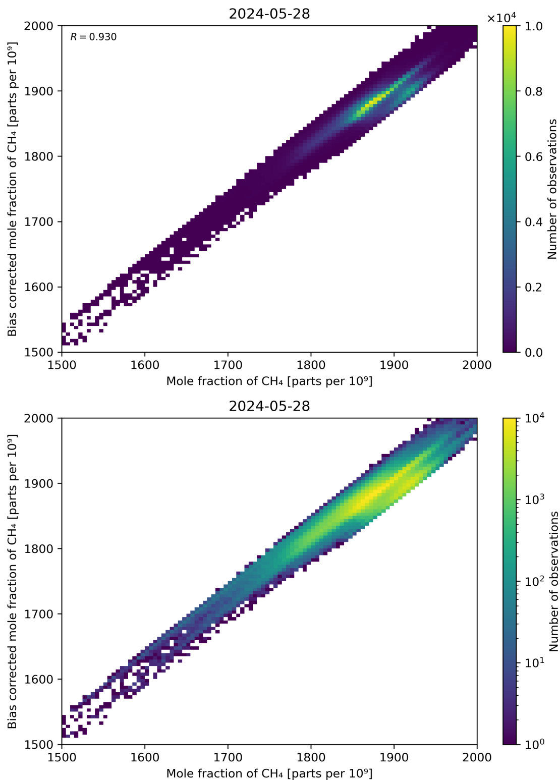
Figure 74: Scatter density plot of “Mole fraction of CH 4 ” against “Bias corrected mole fraction of CH 4 ” for 2024-05-28 to 2024-05-29.
