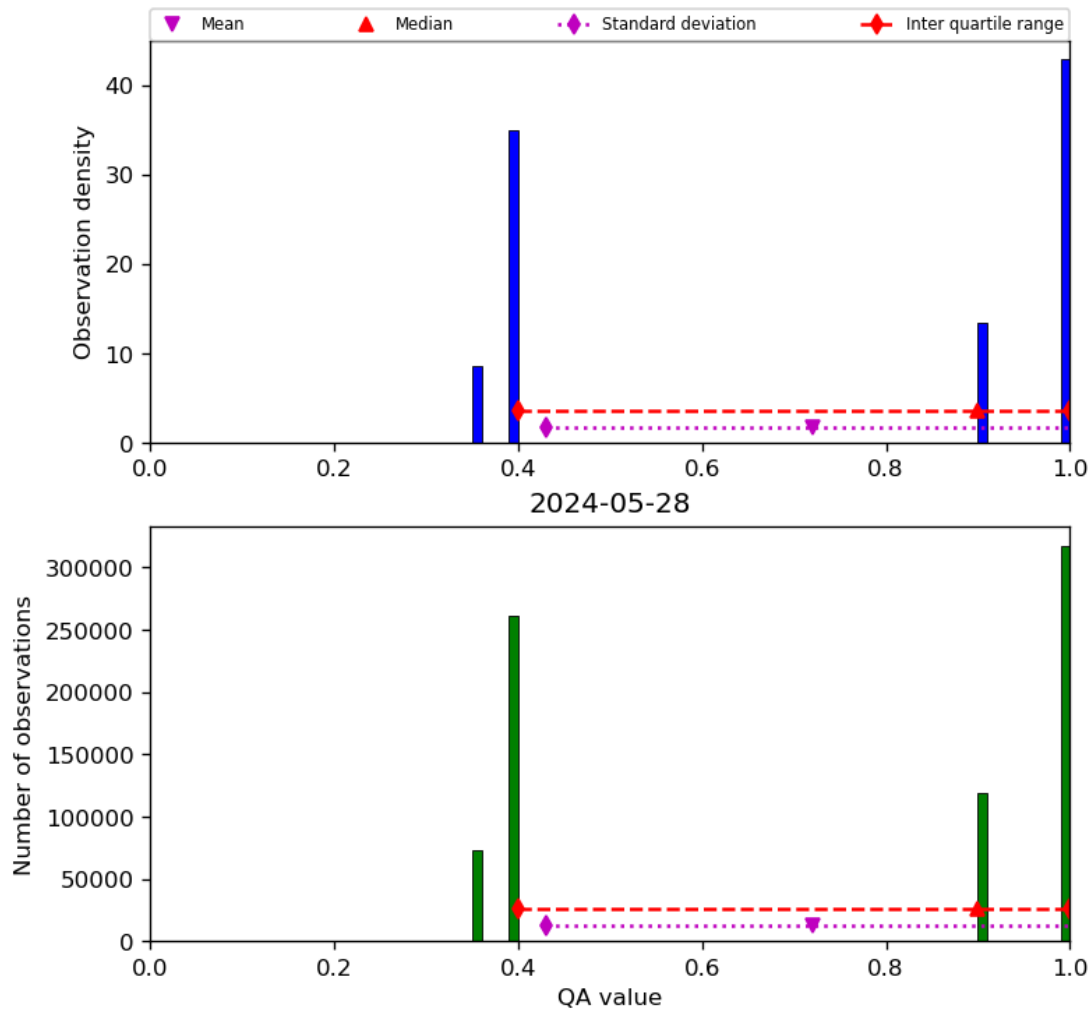
Figure 22: Histogram of “QA value” for 2024-05-28 to 2024-05-29
