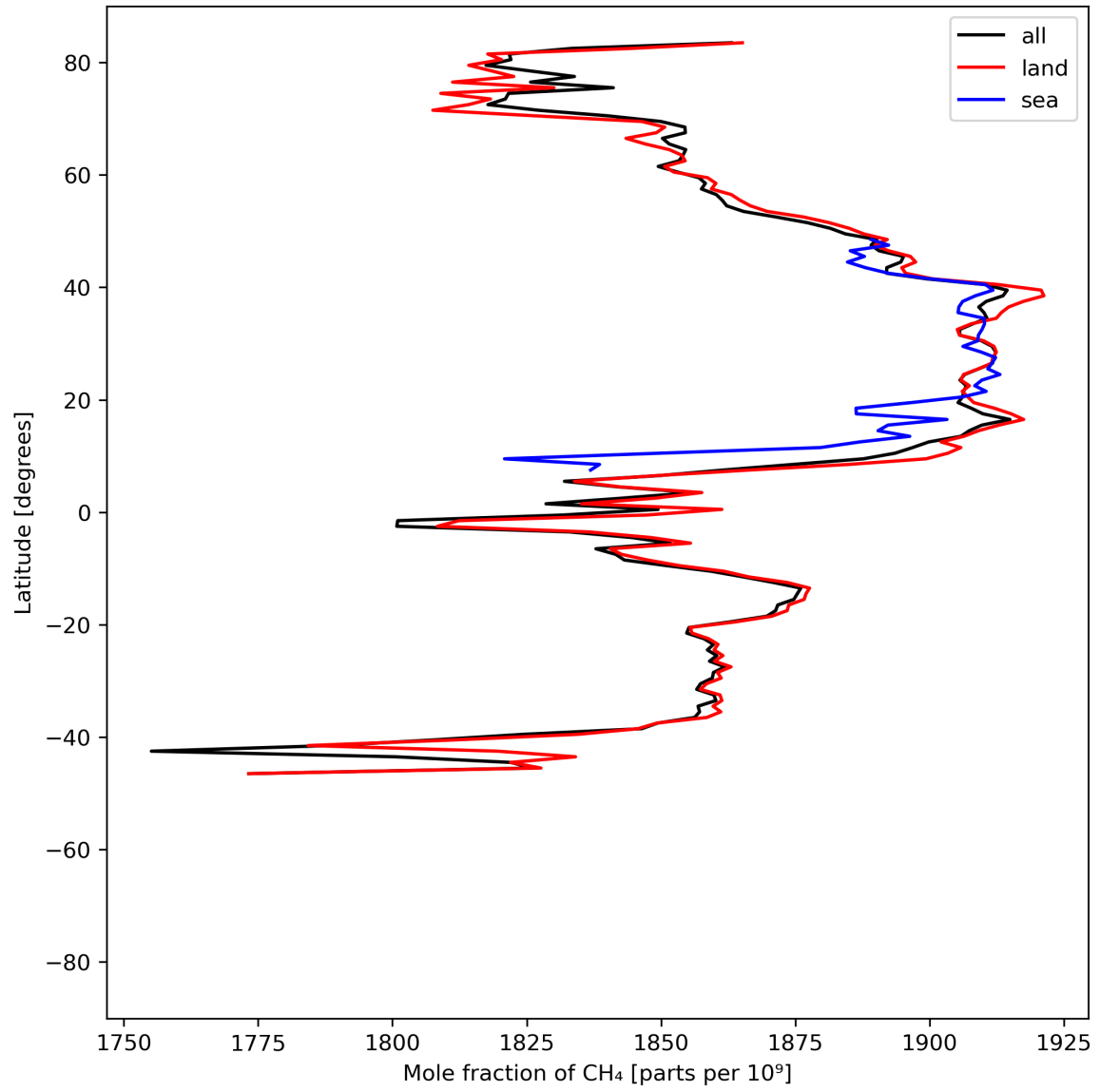
Figure 12: Zonal average of “Mole fraction of \text{CH}_4 ” for 2024-05-28 to 2024-05-29.
