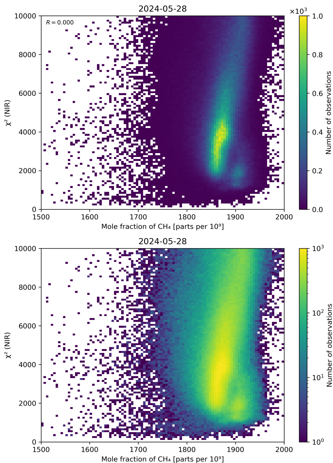
Figure 70: Scatter density plot of “Mole fraction of \text{CH}_4 ” against “ \chi^2 (NIR)” for 2024-05-28 to 2024-05-29.
