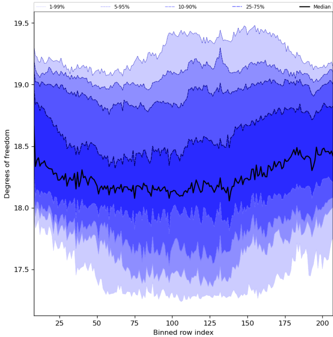
Figure 41: Along track statistics of “Degrees of freedom” for 2024-05-28 to 2024-05-29
