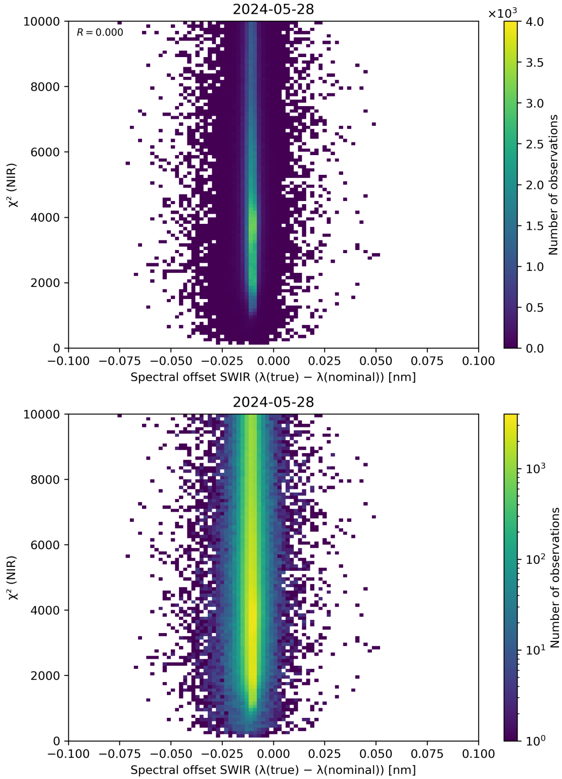
Figure 117: Scatter density plot of “Spectral offset SWIR ( \lambda(\text{true}) - \lambda(\text{nominal}) )” against “ \chi^2 (NIR)” for 2024-05-28 to 2024-05-29.
