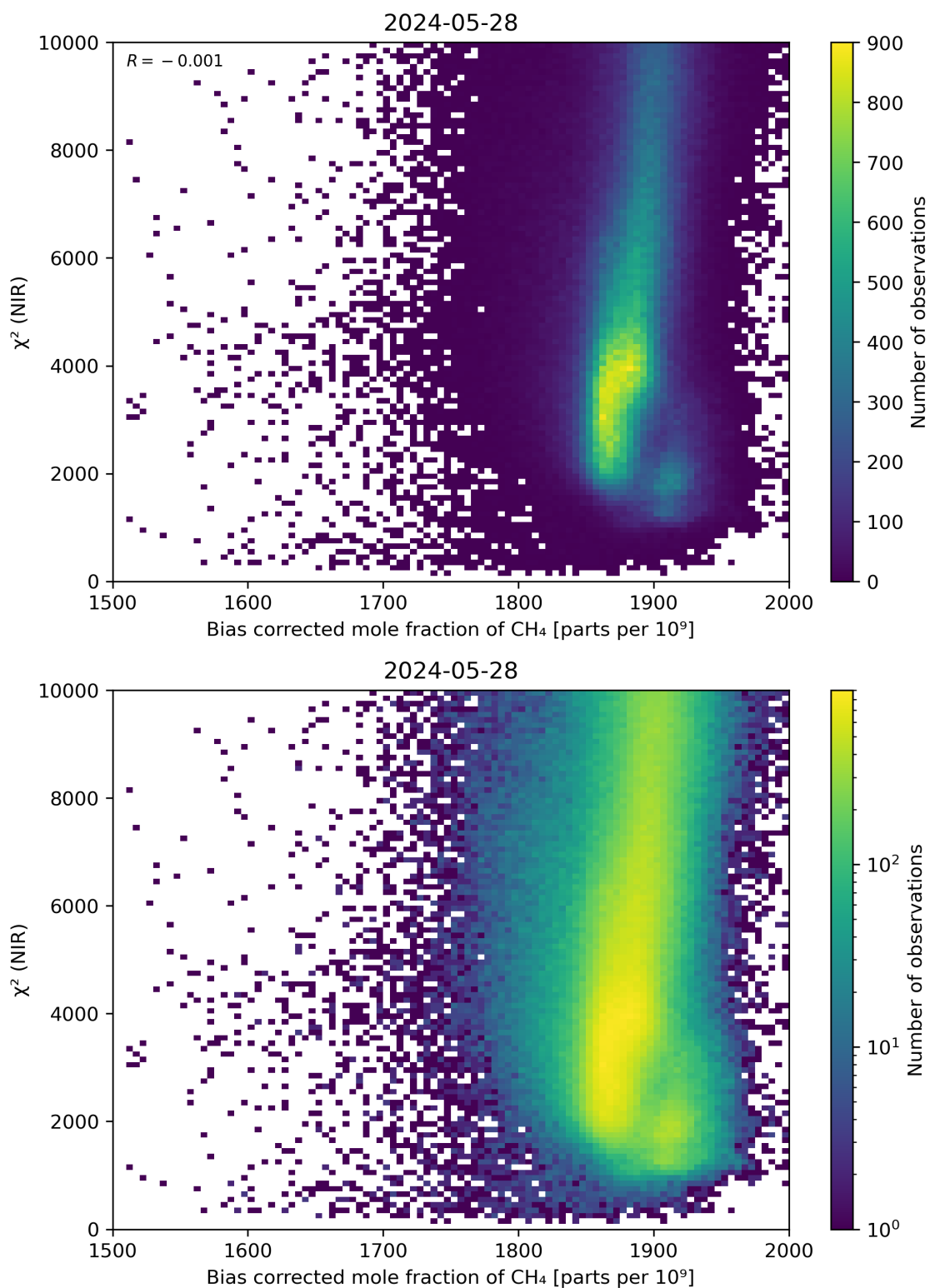
Figure 63: Scatter density plot of “Bias corrected mole fraction of CH 4 ” against “ \chi^2 (NIR)” for 2024-05-28 to 2024-05-29.
