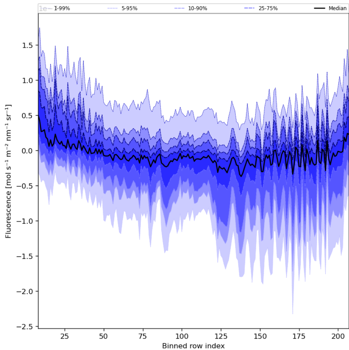
Figure 43: Along track statistics of “Fluorescence” for 2024-05-28 to 2024-05-29
