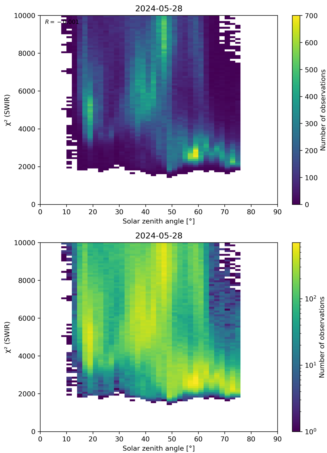
Figure 95: Scatter density plot of “Solar zenith angle” against “ \chi^2 (SWIR)” for 2024-05-28 to 2024-05-29.
