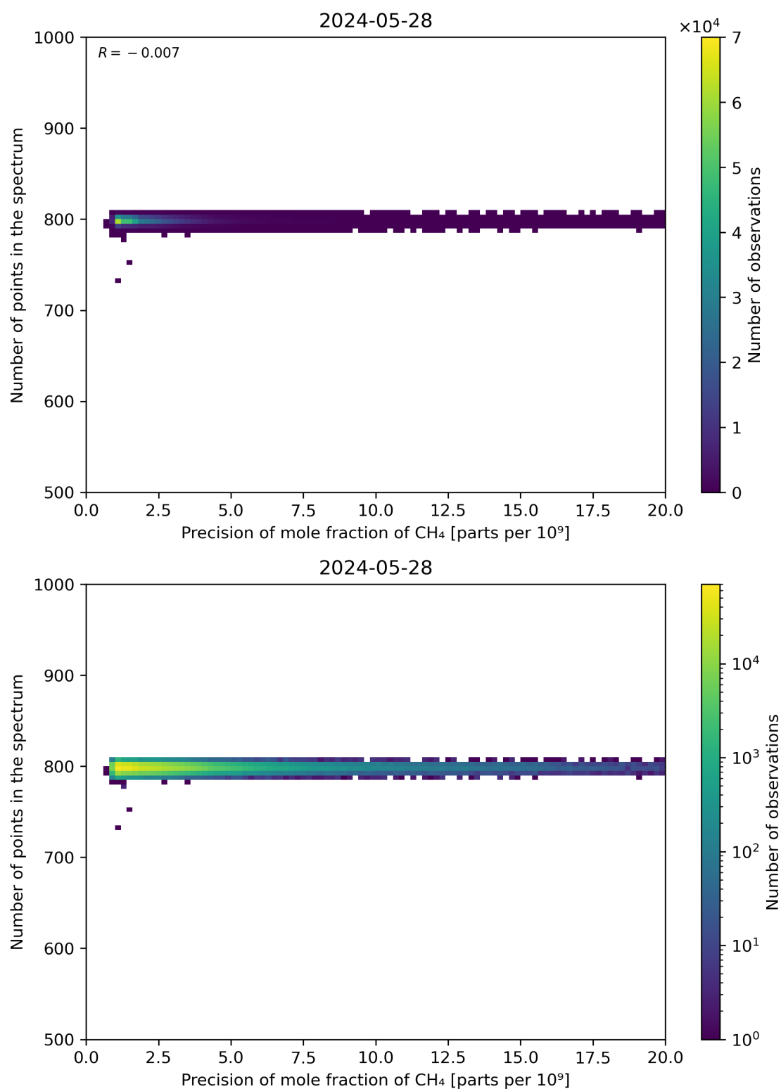
Figure 84: Scatter density plot of “Precision of mole fraction of CH 4 ” against “Number of points in the spectrum” for 2024-05-28 to 2024-05-29.
