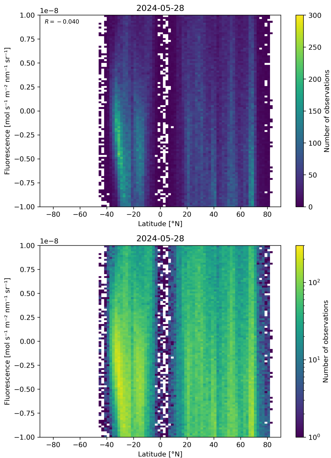
Figure 56: Scatter density plot of “Latitude” against “Fluorescence” for 2024-05-28 to 2024-05-29.
