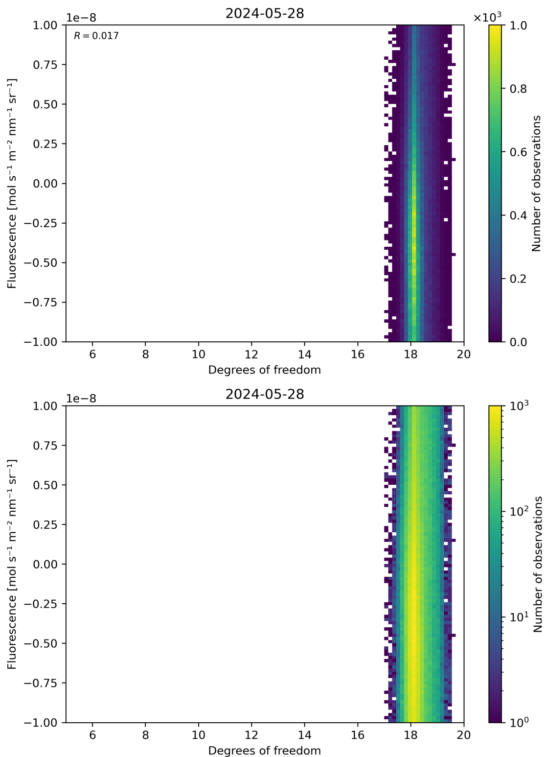
Figure 51: Scatter density plot of “Degrees of freedom” against “Fluorescence” for 2024-05-28 to 2024-05-29.
