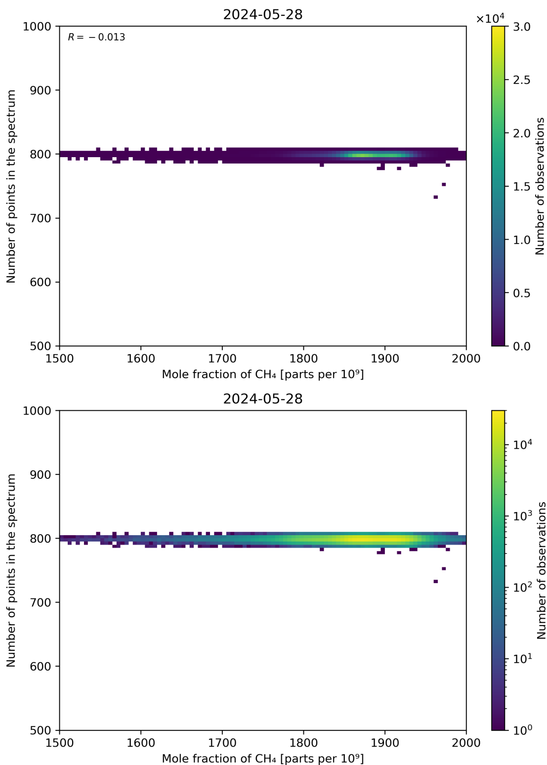
Figure 77: Scatter density plot of “Mole fraction of CH 4 ” against “Number of points in the spectrum” for 2024-05-28 to 2024-05-29.
