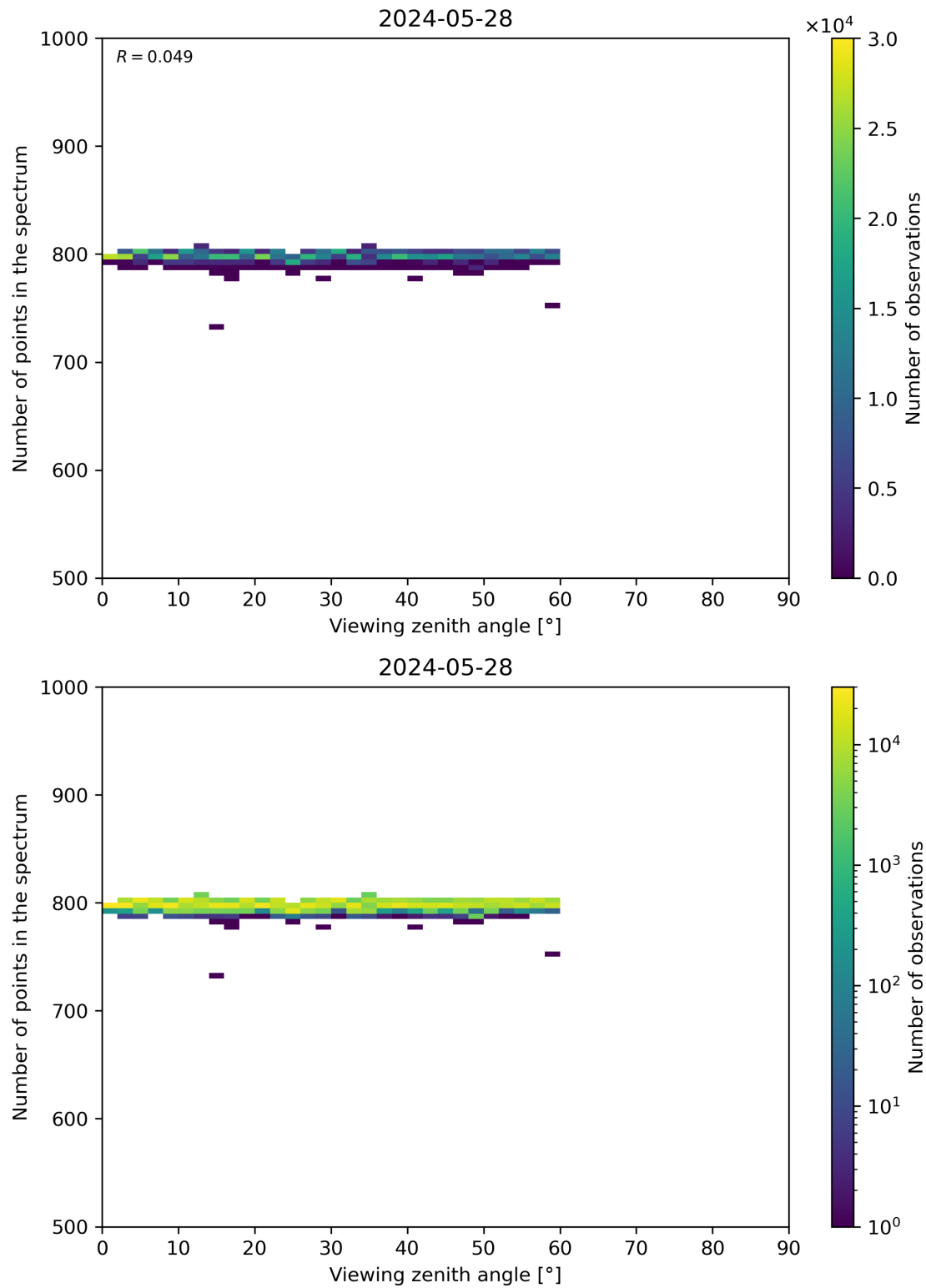
Figure 114: Scatter density plot of “Viewing zenith angle” against “Number of points in the spectrum” for 2024-05-28 to 2024-05-29.
