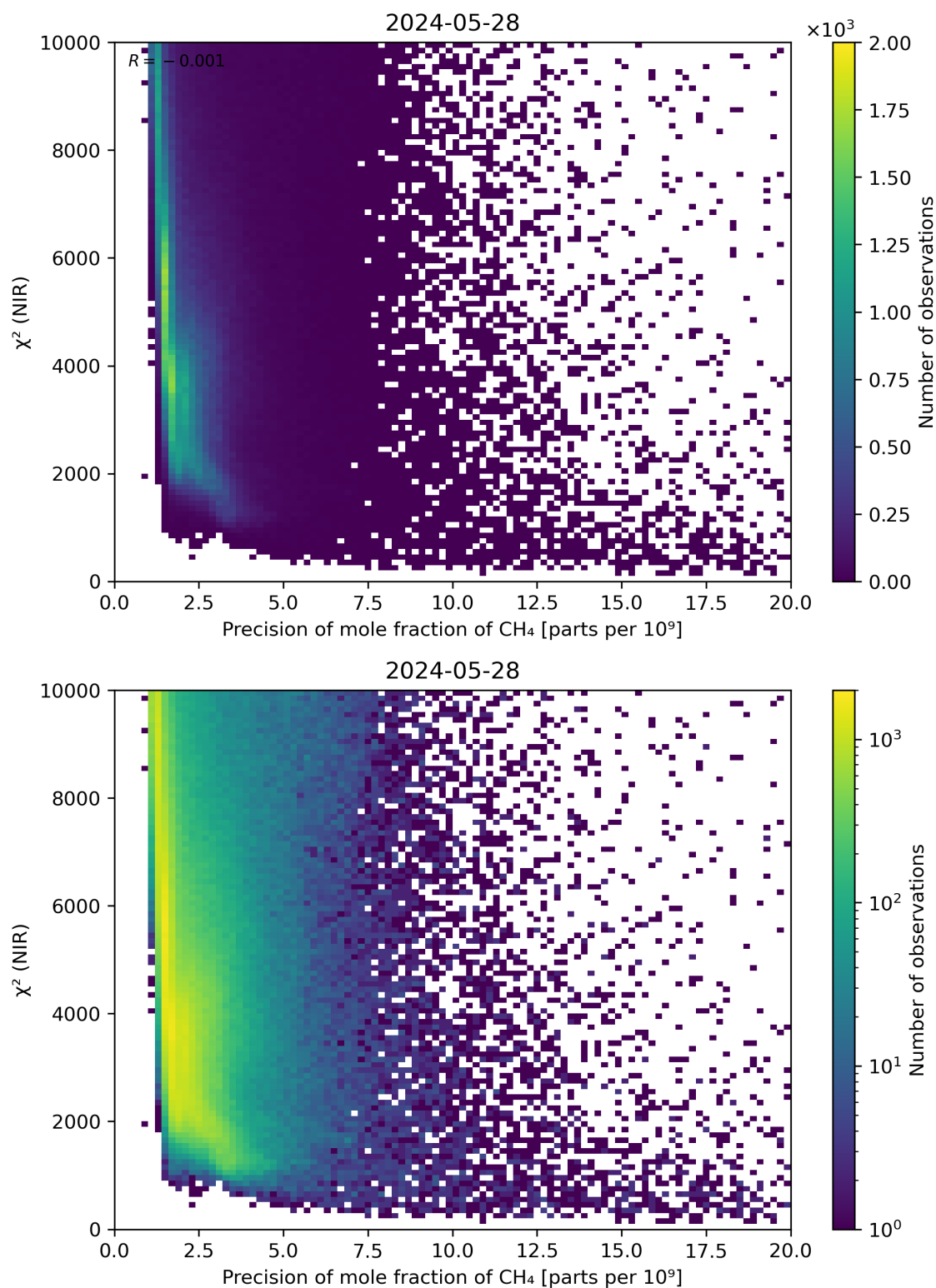
Figure 78: Scatter density plot of “Precision of mole fraction of \text{CH}_4 ” against “ \chi^2 (NIR)” for 2024-05-28 to 2024-05-29.
