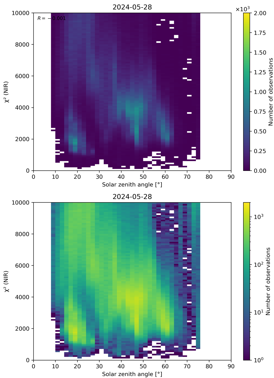
Figure 94: Scatter density plot of “Solar zenith angle” against “ \chi^2 (NIR)” for 2024-05-28 to 2024-05-29.
