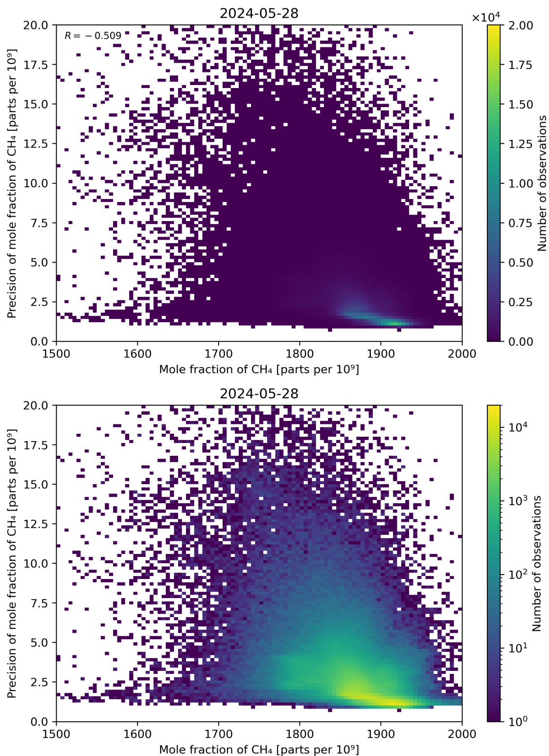
Figure 75: Scatter density plot of “Mole fraction of CH 4 ” against “Precision of mole fraction of CH 4 ” for 2024-05-28 to 2024-05-29.
