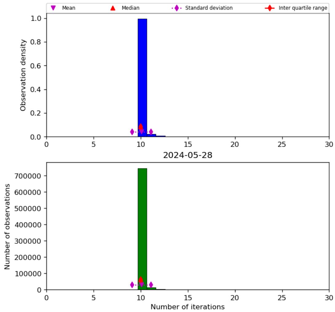
Figure 31: Histogram of “Number of iterations” for 2024-05-28 to 2024-05-29
