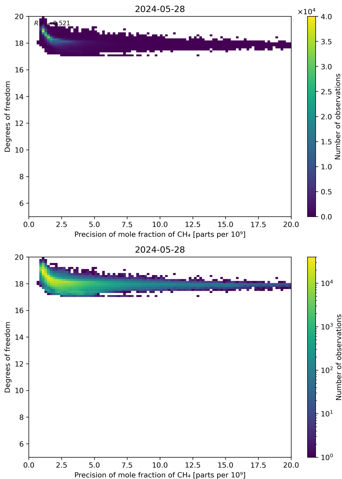
Figure 80: Scatter density plot of “Precision of mole fraction of CH 4 ” against “Degrees of freedom” for 2024-05-28 to 2024-05-29.
