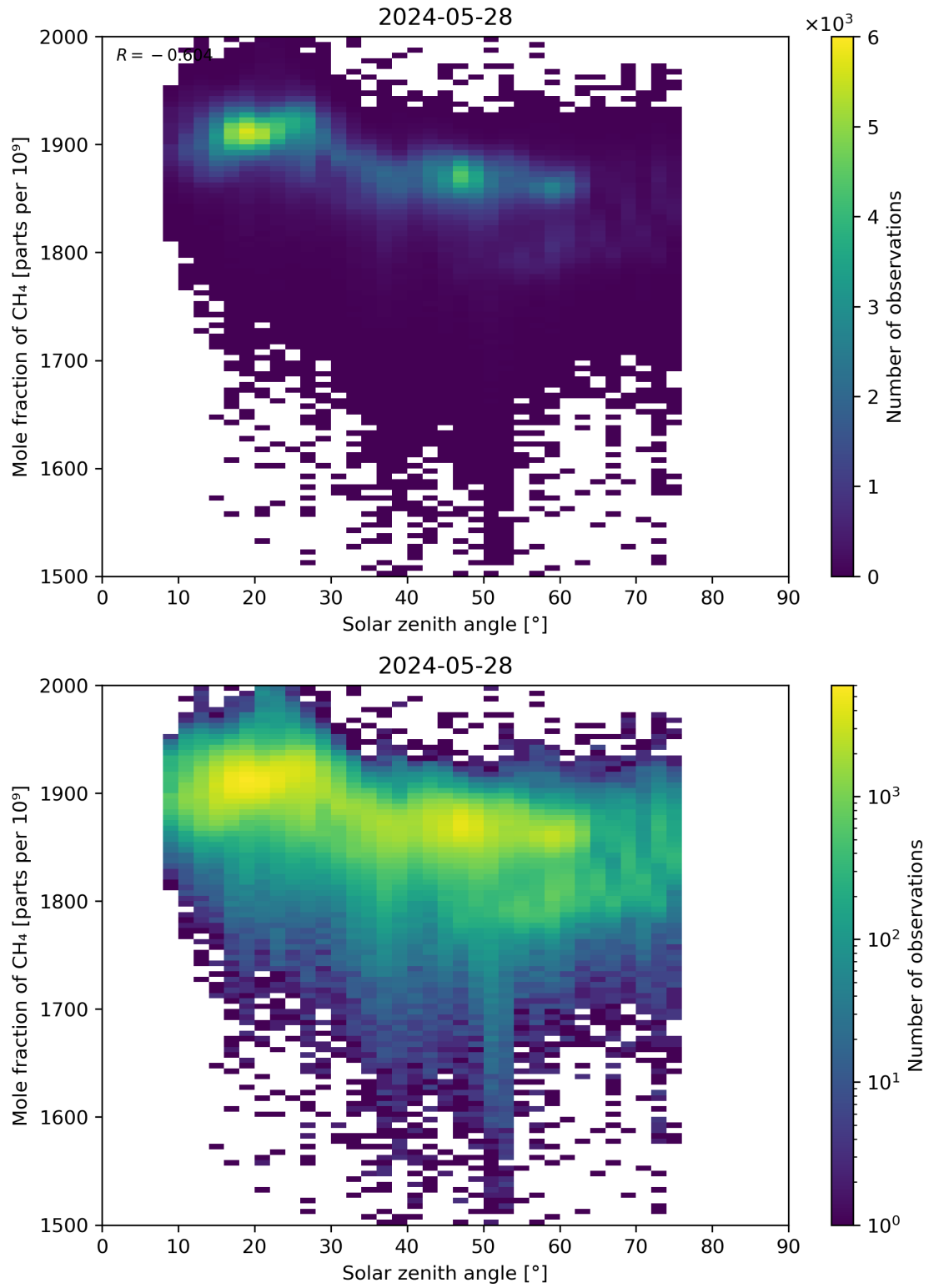
Figure 99: Scatter density plot of “Solar zenith angle” against “Mole fraction of \text{CH}_4 ” for 2024-05-28 to 2024-05-29.
