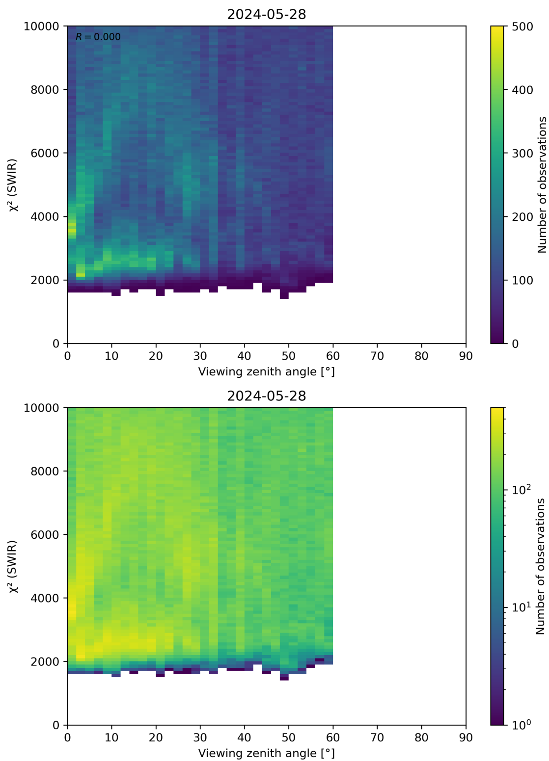
Figure 106: Scatter density plot of “Viewing zenith angle” against “ \chi^2 (SWIR)” for 2024-05-28 to 2024-05-29.
