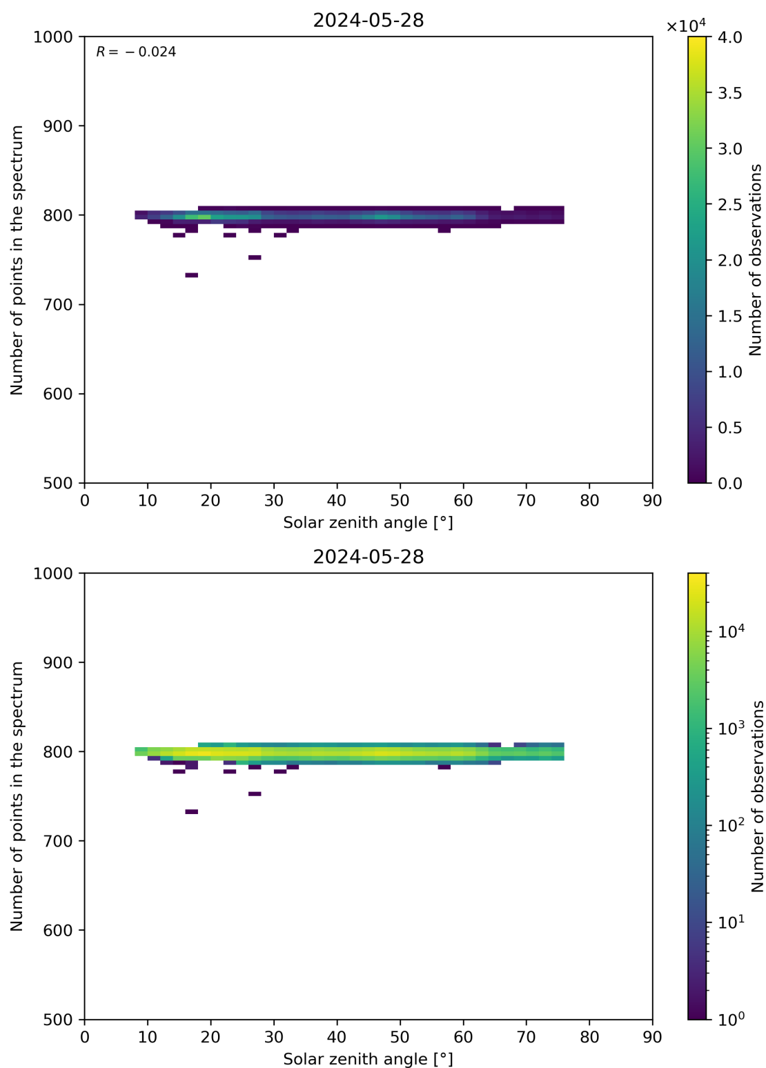
Figure 103: Scatter density plot of “Solar zenith angle” against “Number of points in the spectrum” for 2024-05-28 to 2024-05-29.
