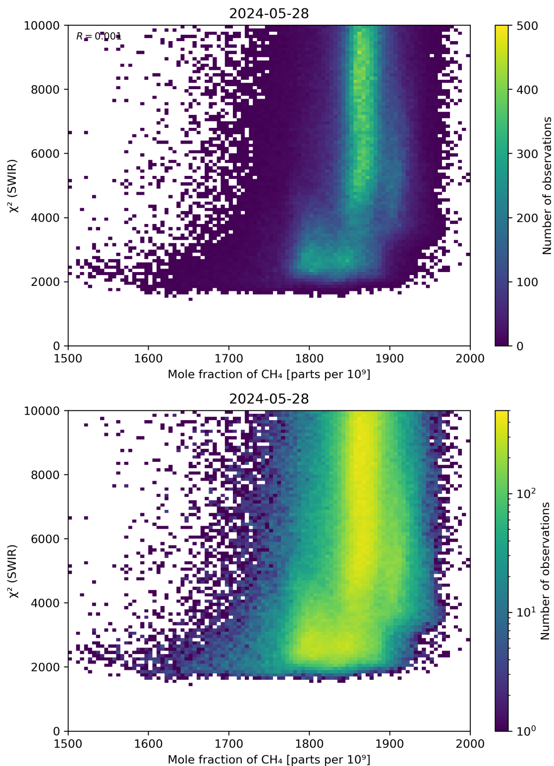
Figure 71: Scatter density plot of “Mole fraction of \text{CH}_4 ” against “ \chi^2 (SWIR)” for 2024-05-28 to 2024-05-29.
