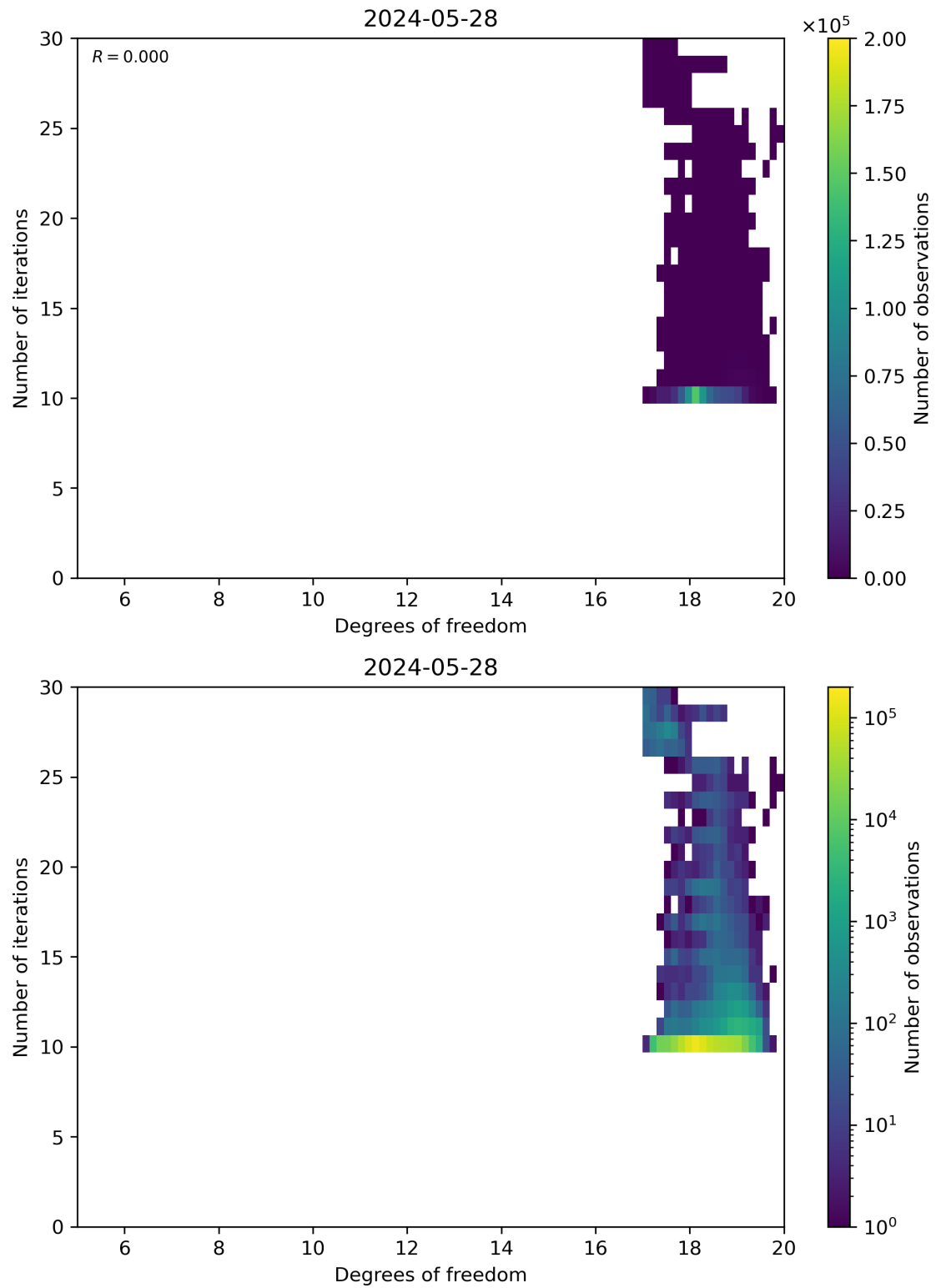
Figure 52: Scatter density plot of “Degrees of freedom” against “Number of iterations” for 2024-05-28 to 2024-05-29.
