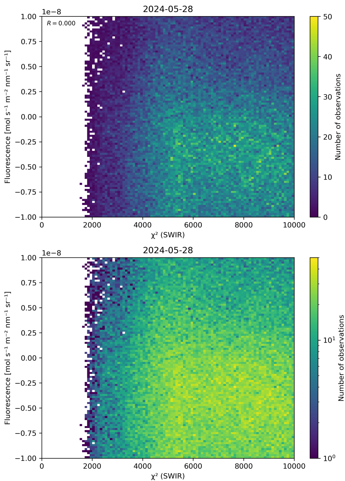
Figure 49: Scatter density plot of “ \chi^2 (SWIR)” against “Fluorescence” for 2024-05-28 to 2024-05-29.
