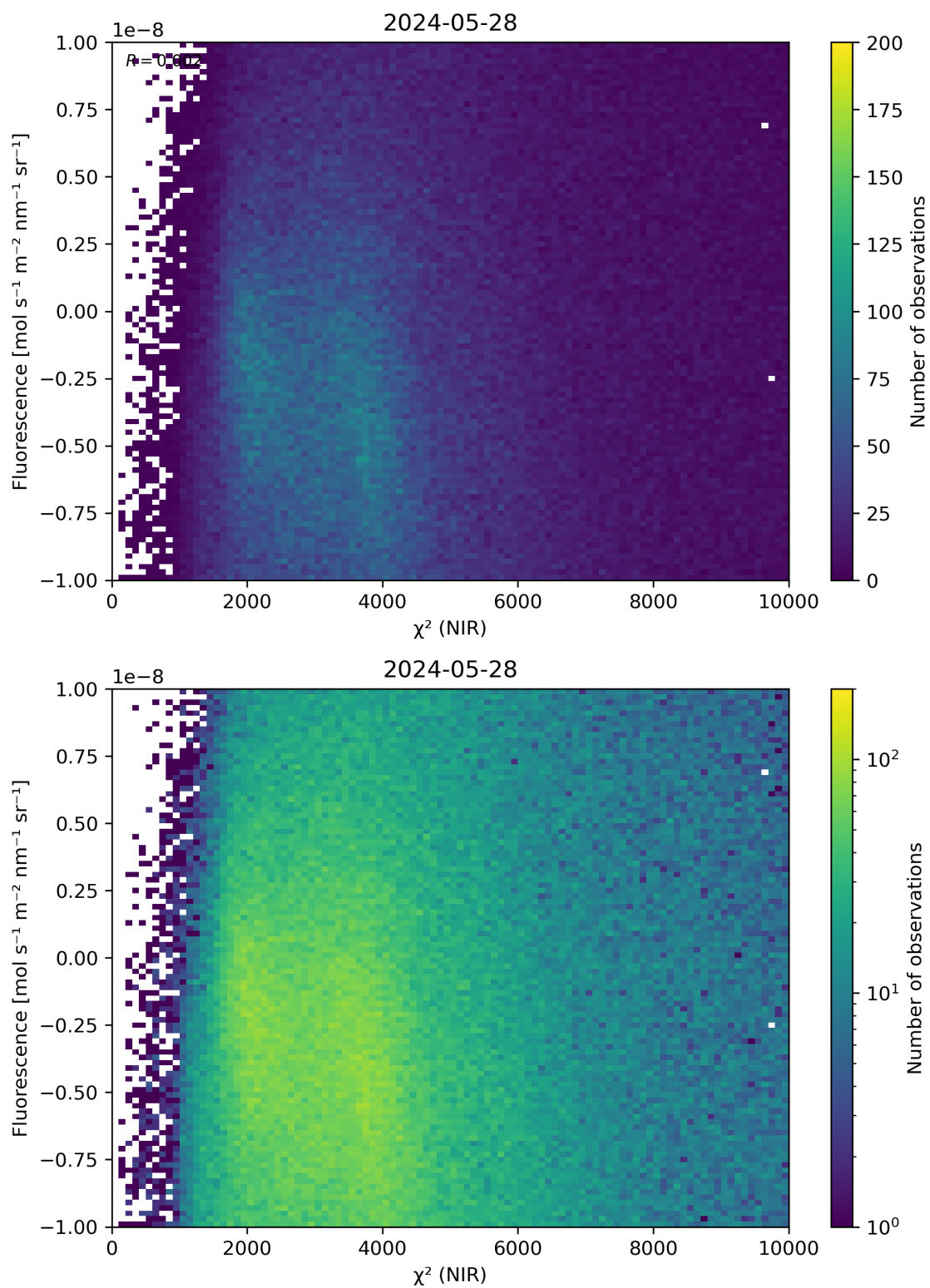
Figure 45: Scatter density plot of “ \chi^2 (NIR)” against “Fluorescence” for 2024-05-28 to 2024-05-29.
