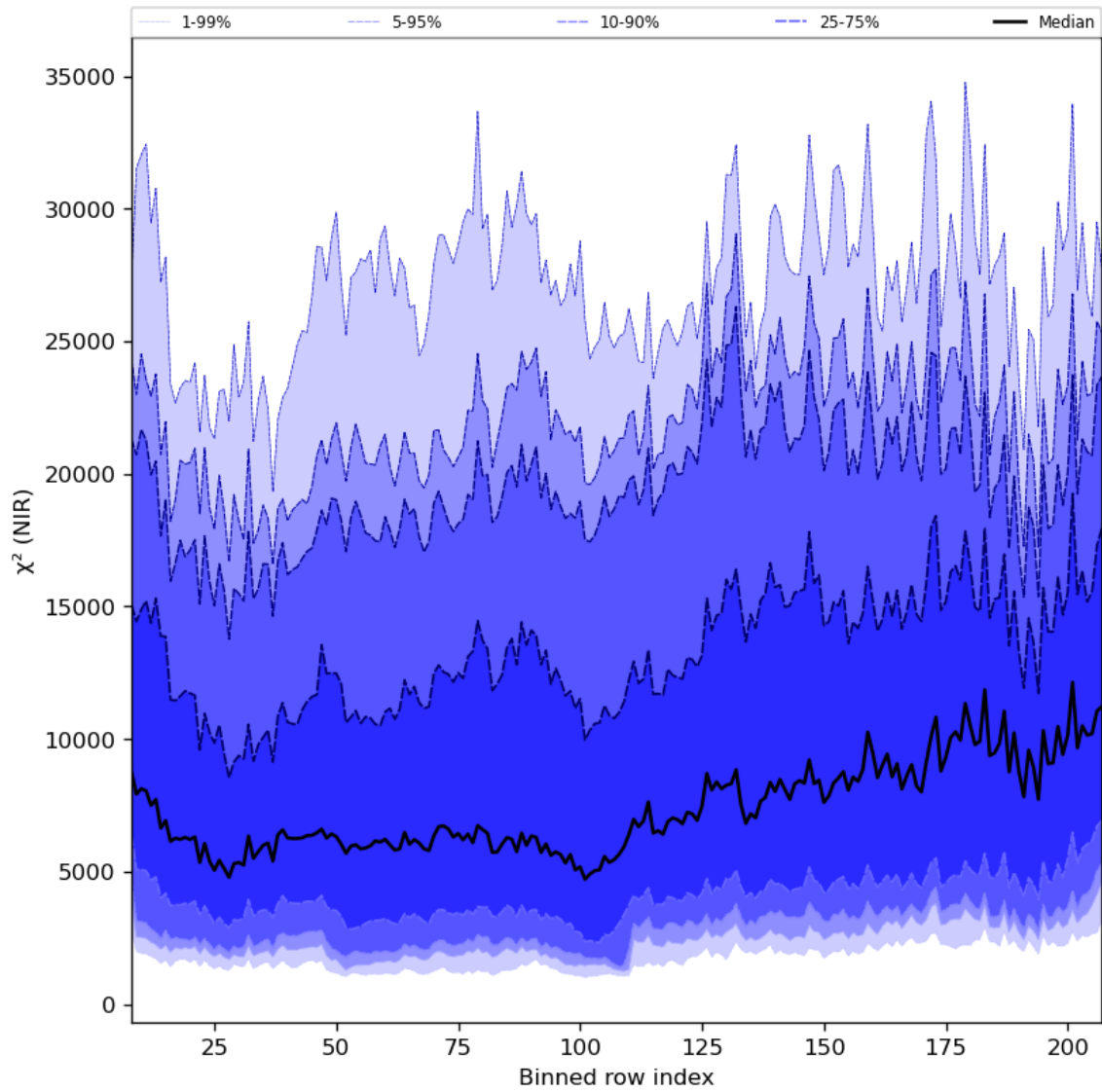
Figure 40: Along track statistics of “ \chi^2 (NIR)” for 2024-05-28 to 2024-05-29
