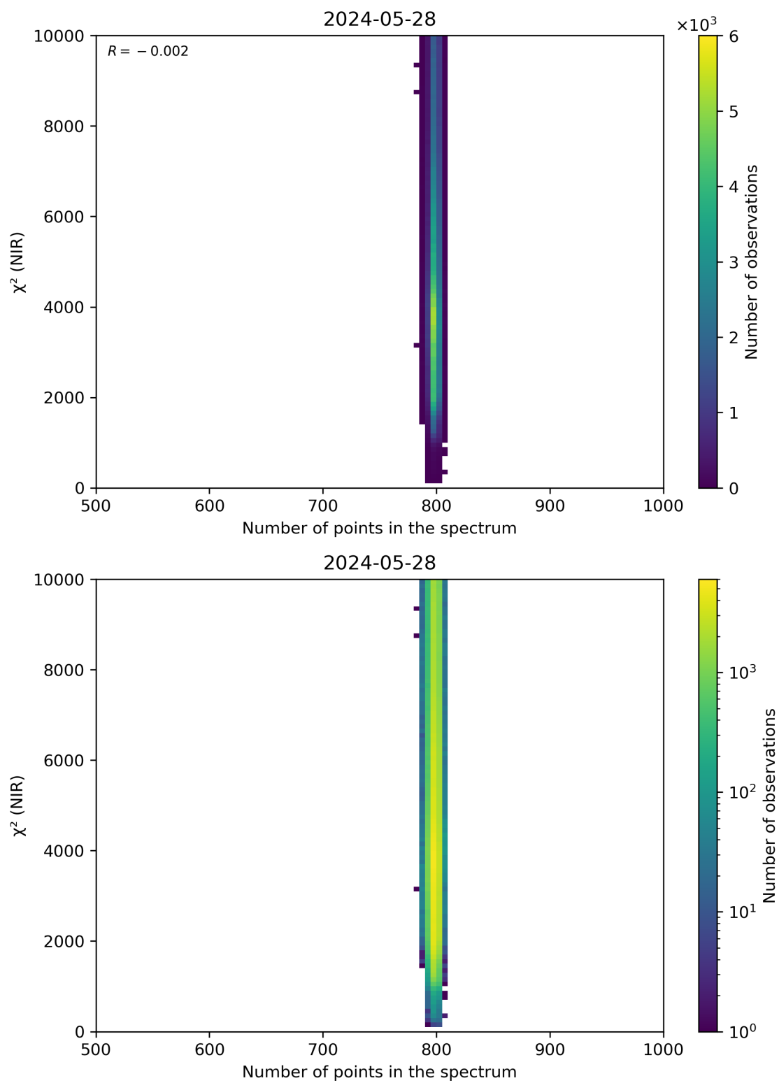
Figure 88: Scatter density plot of “Number of points in the spectrum” against “ \chi^2 (NIR)” for 2024-05-28 to 2024-05-29.
