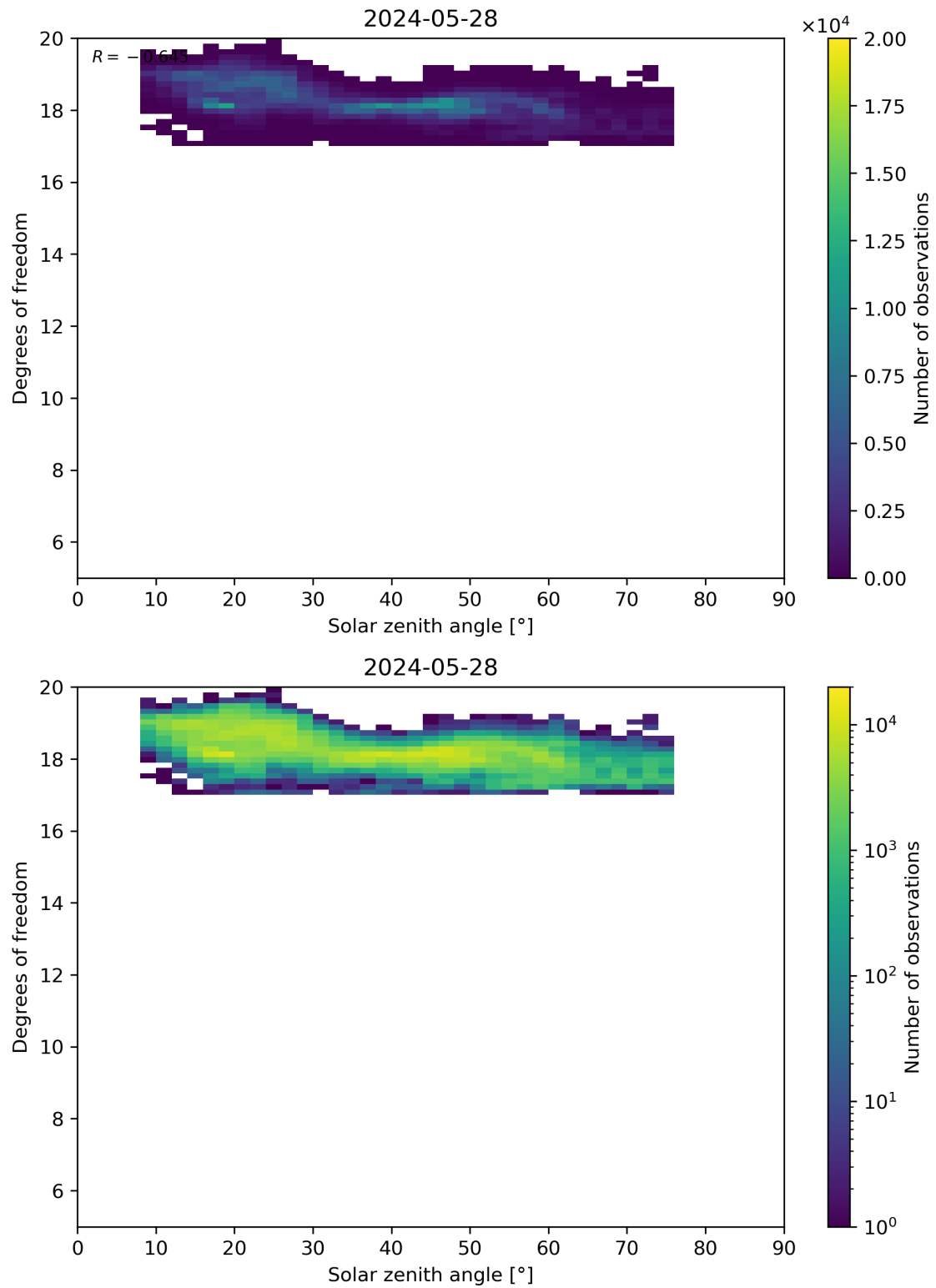
Figure 96: Scatter density plot of “Solar zenith angle” against “Degrees of freedom” for 2024-05-28 to 2024-05-29.
