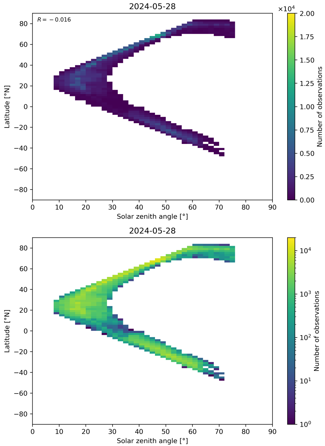
Figure 98: Scatter density plot of “Solar zenith angle” against “Latitude” for 2024-05-28 to 2024-05-29.
