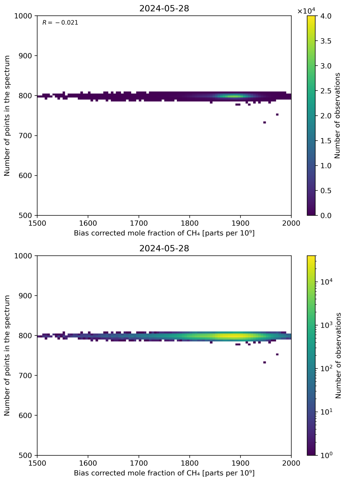
Figure 68: Scatter density plot of “Bias corrected mole fraction of CH 4 ” against “Number of points in the spectrum” for 2024-05-28 to 2024-05-29.
