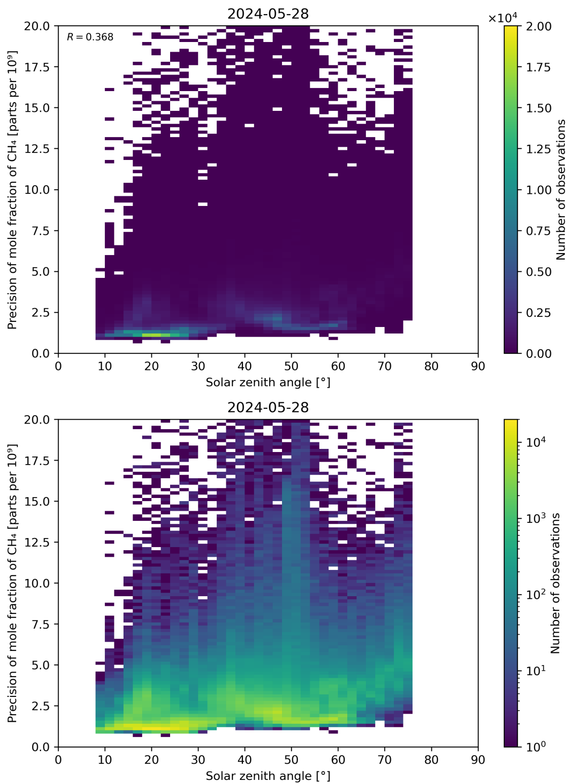
Figure 101: Scatter density plot of “Solar zenith angle” against “Precision of mole fraction of CH 4 ” for 2024-05-28 to 2024-05-29.
