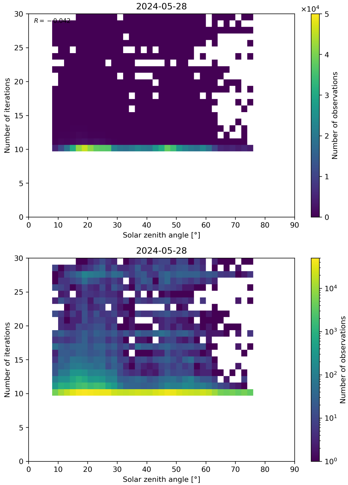
Figure 102: Scatter density plot of “Solar zenith angle” against “Number of iterations” for 2024-05-28 to 2024-05-29.
