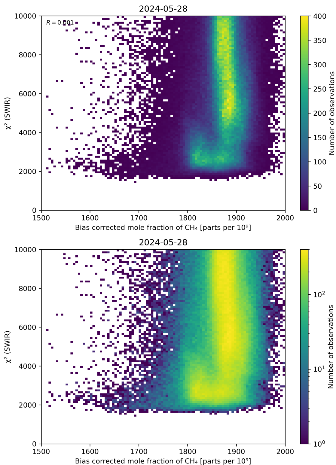
Figure 64: Scatter density plot of “Bias corrected mole fraction of CH 4 ” against “ \chi^2 (SWIR)” for 2024-05-28 to 2024-05-29.
