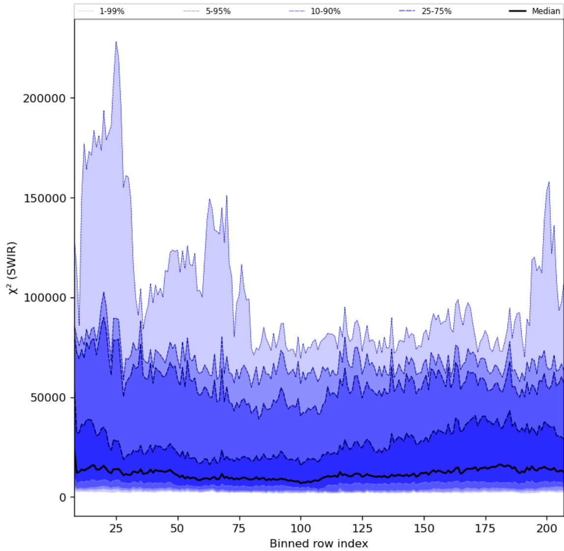
Figure 39: Along track statistics of " \chi^2 (SWIR)" for 2024-05-28 to 2024-05-29
