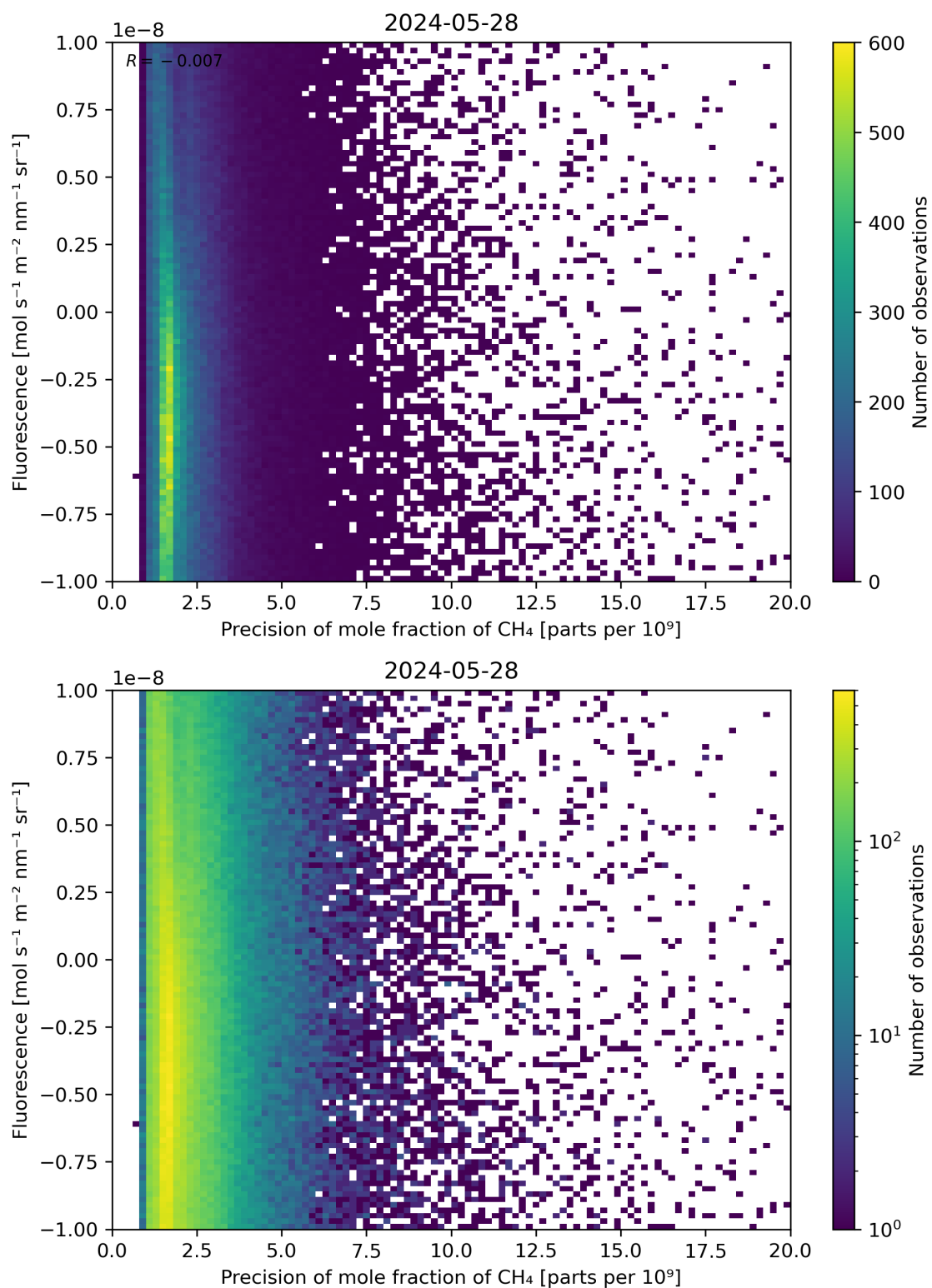
Figure 81: Scatter density plot of “Precision of mole fraction of CH 4 ” against “Fluorescence” for 2024-05-28 to 2024-05-29.
