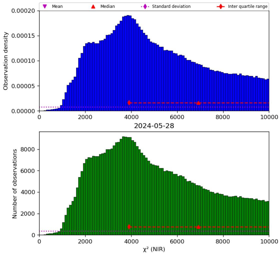
Figure 29: Histogram of “ \chi^2 (NIR)” for 2024-05-28 to 2024-05-29
