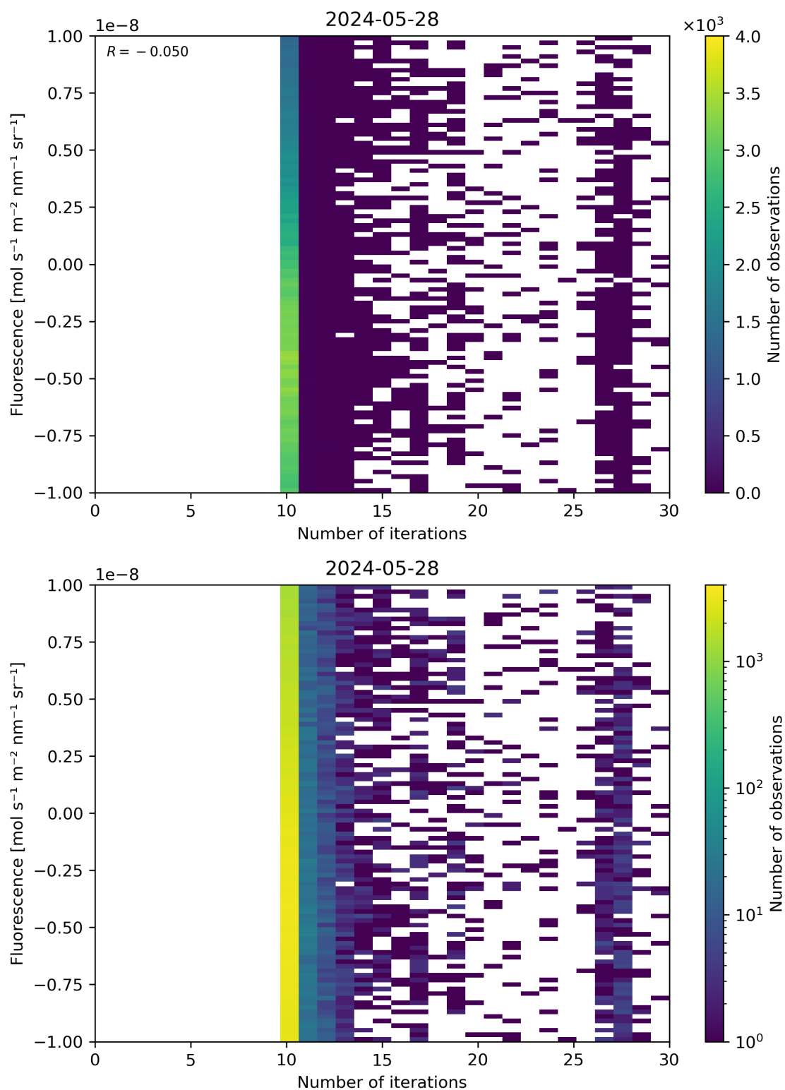
Figure 87: Scatter density plot of “Number of iterations” against “Fluorescence” for 2024-05-28 to 2024-05-29.
