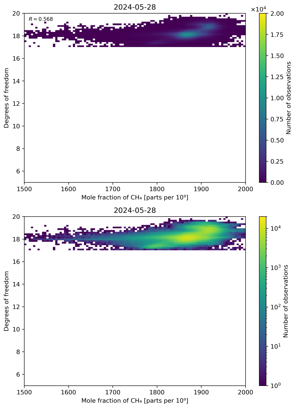
Figure 72: Scatter density plot of “Mole fraction of CH 4 ” against “Degrees of freedom” for 2024-05-28 to 2024-05-29.
