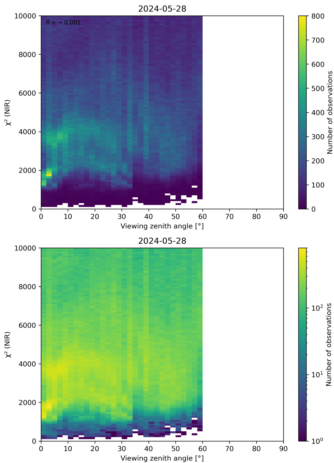
Figure 105: Scatter density plot of “Viewing zenith angle” against “ \chi^2 (NIR)” for 2024-05-28 to 2024-05-29.
