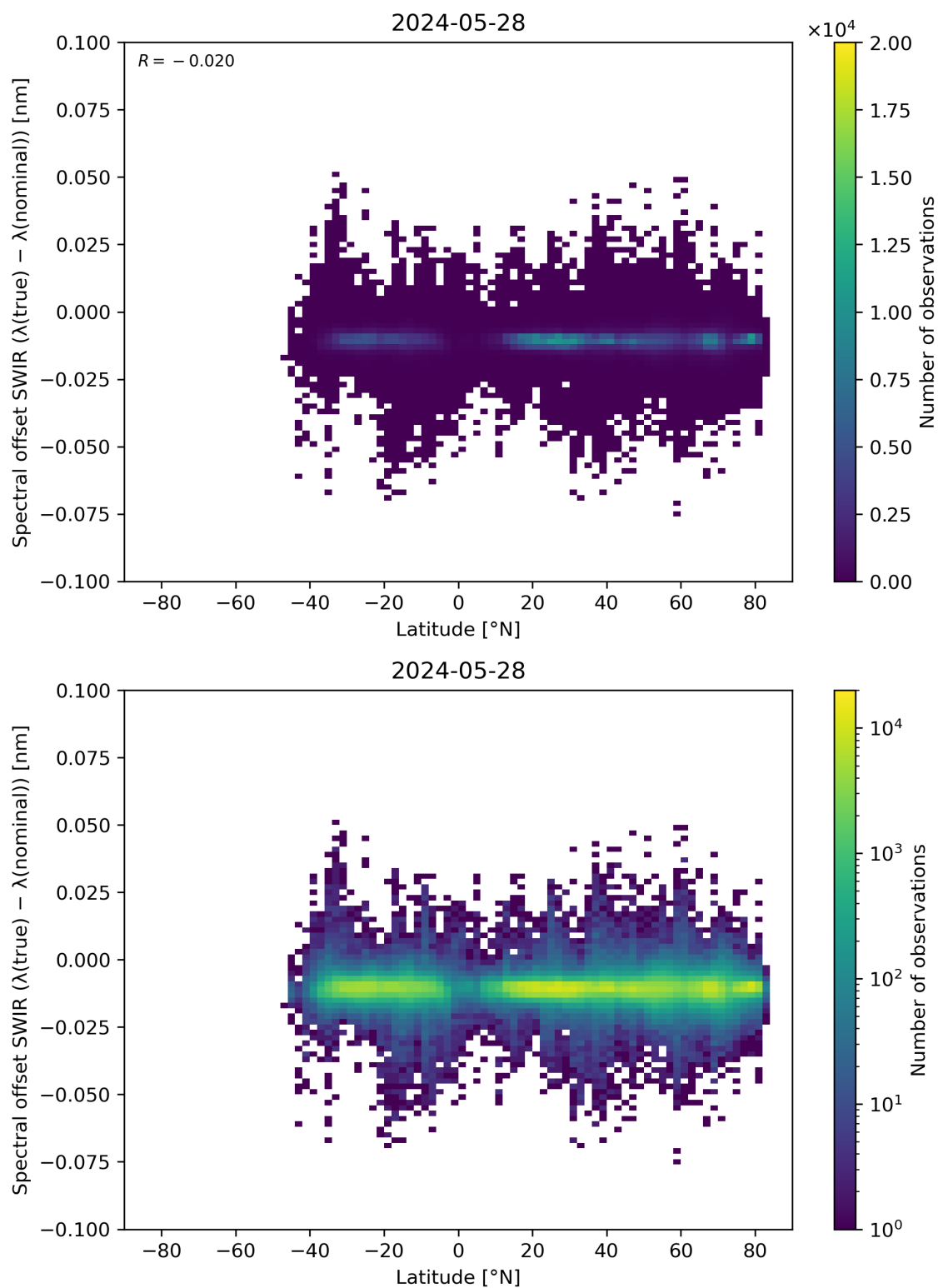
Figure 62: Scatter density plot of “Latitude” against “Spectral offset SWIR ( \lambda(\text{true}) - \lambda(\text{nominal}) )” for 2024-05-28 to 2024-05-29.
