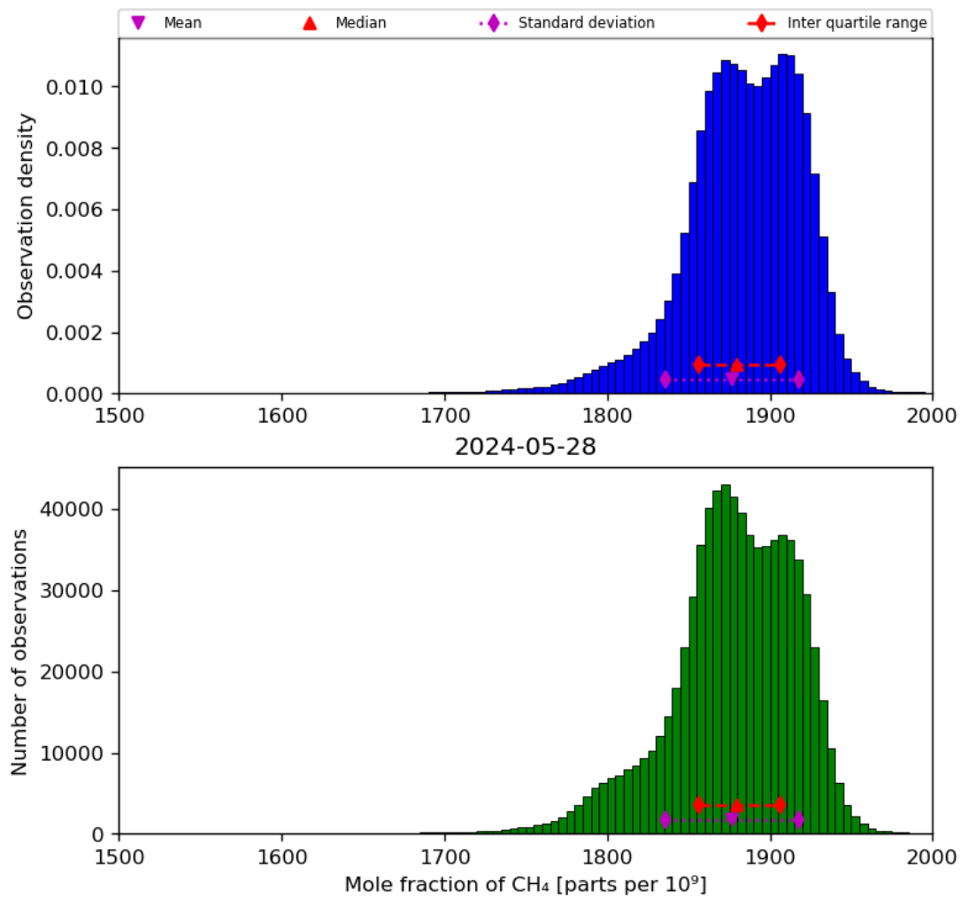
Figure 23: Histogram of “Mole fraction of CH 4 ” for 2024-05-28 to 2024-05-29
