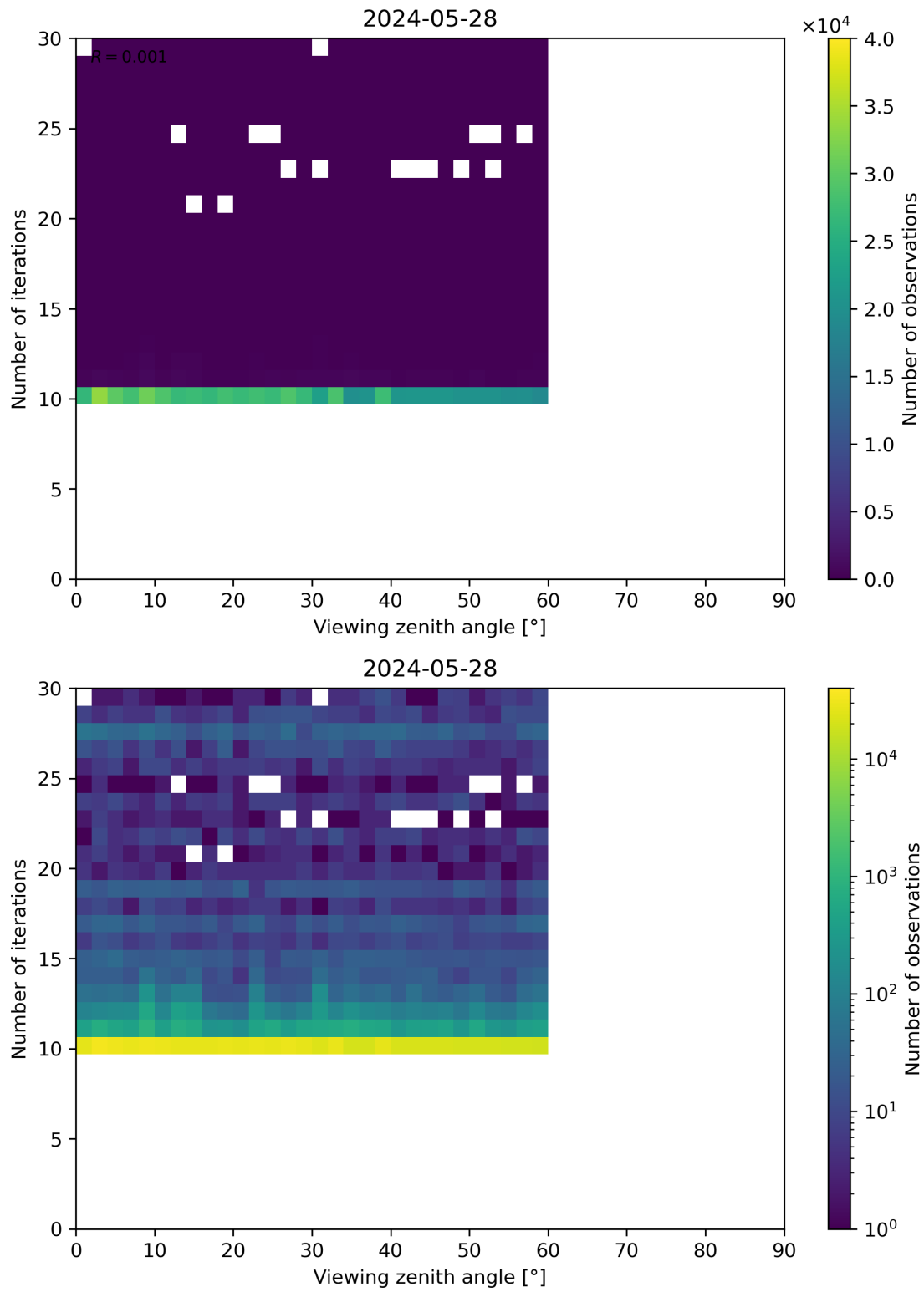
Figure 113: Scatter density plot of “Viewing zenith angle” against “Number of iterations” for 2024-05-28 to 2024-05-29.
