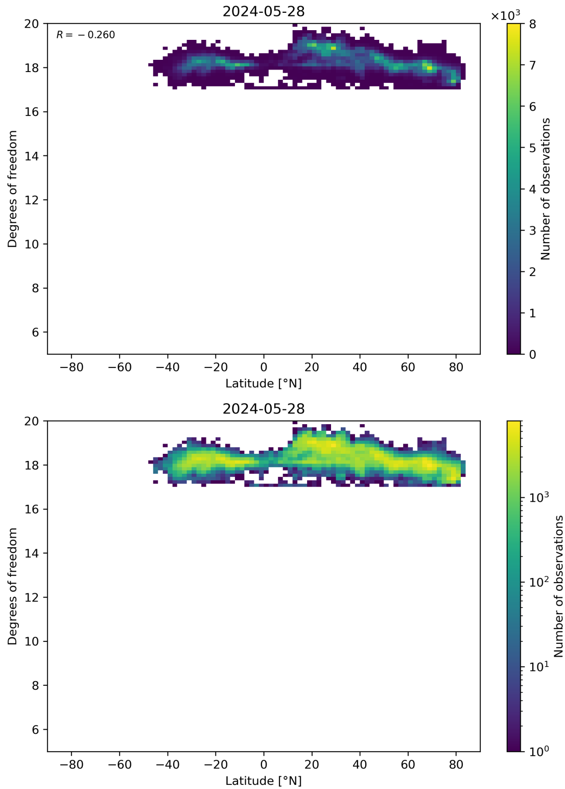
Figure 55: Scatter density plot of “Latitude” against “Degrees of freedom” for 2024-05-28 to 2024-05-29.
