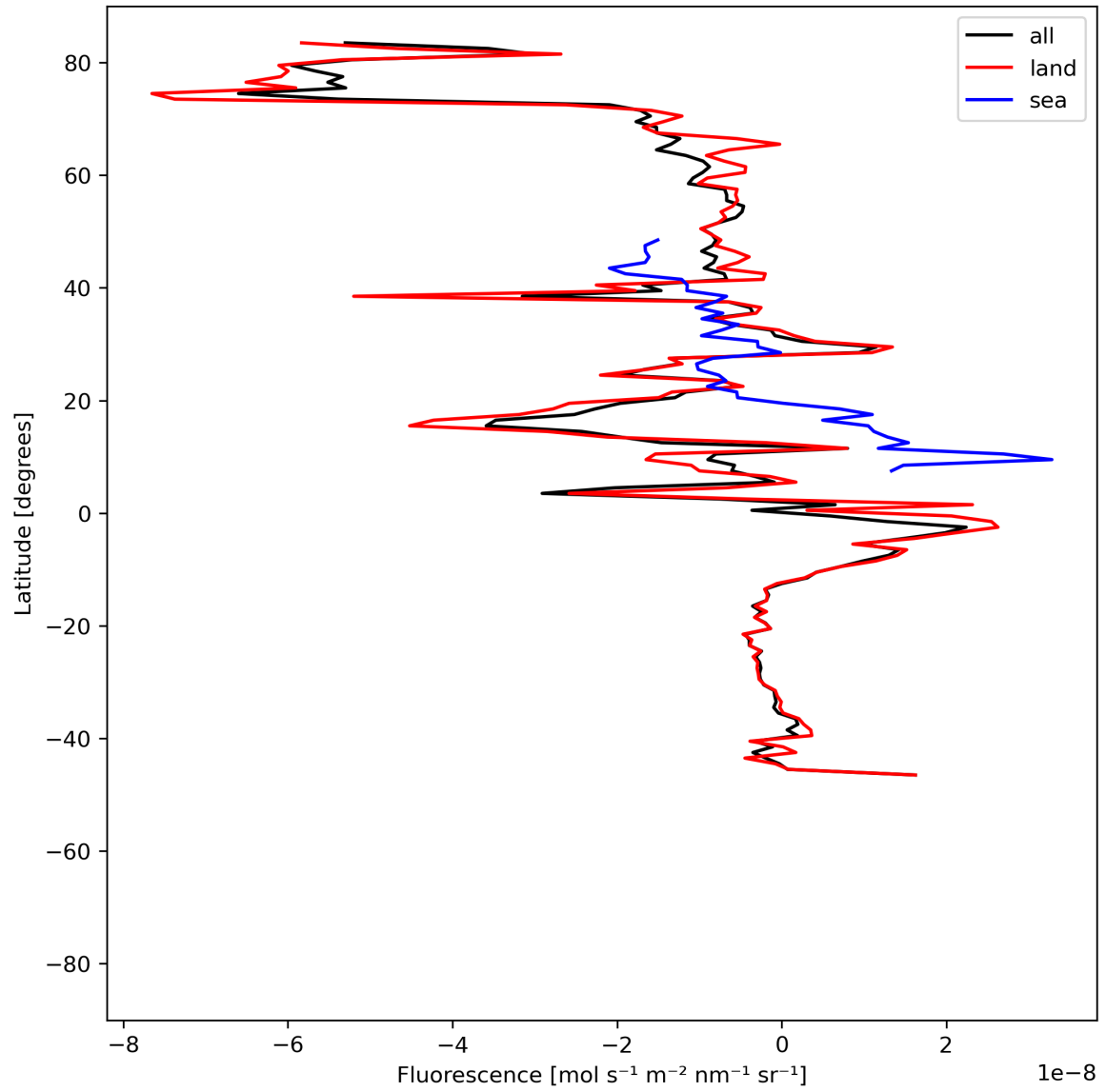
Figure 21: Zonal average of “Fluorescence” for 2024-05-28 to 2024-05-29.
