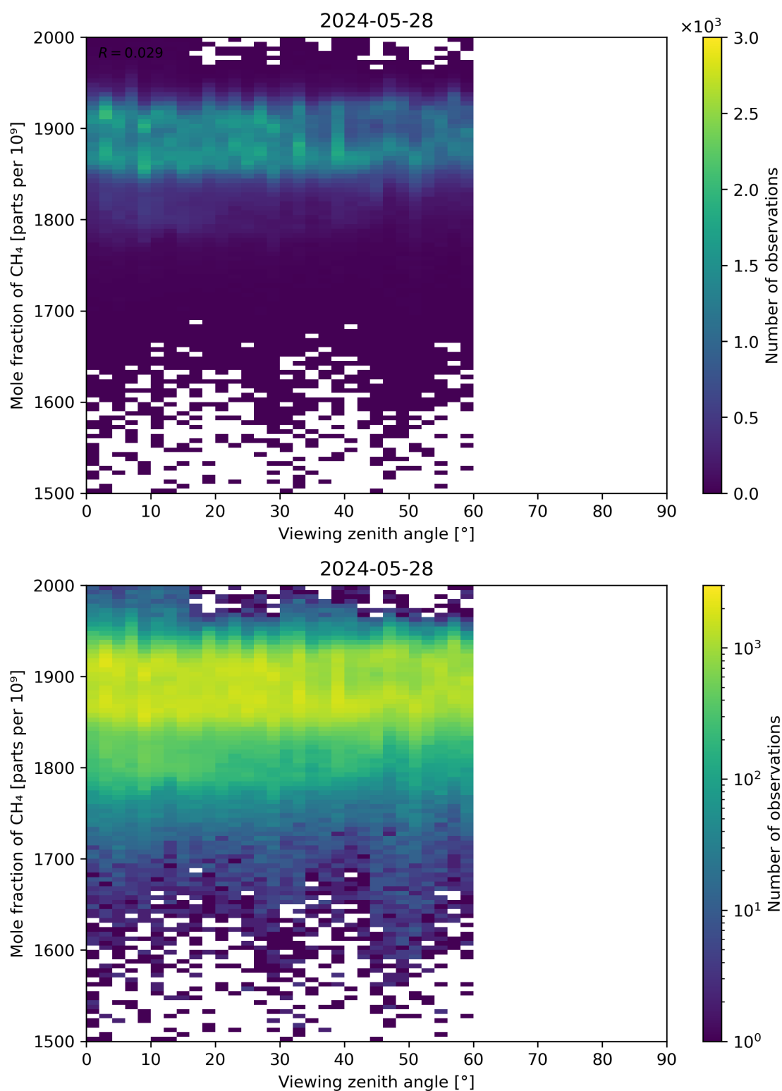
Figure 110: Scatter density plot of “Viewing zenith angle” against “Mole fraction of \text{CH}_4 ” for 2024-05-28 to 2024-05-29.
