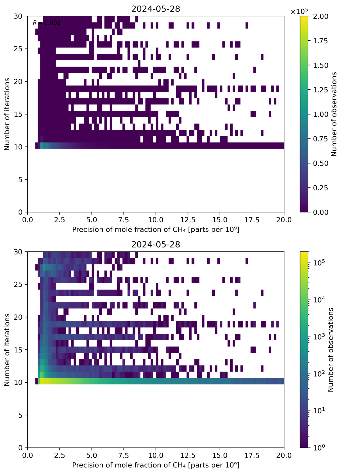
Figure 83: Scatter density plot of “Precision of mole fraction of CH 4 ” against “Number of iterations” for 2024-05-28 to 2024-05-29.
