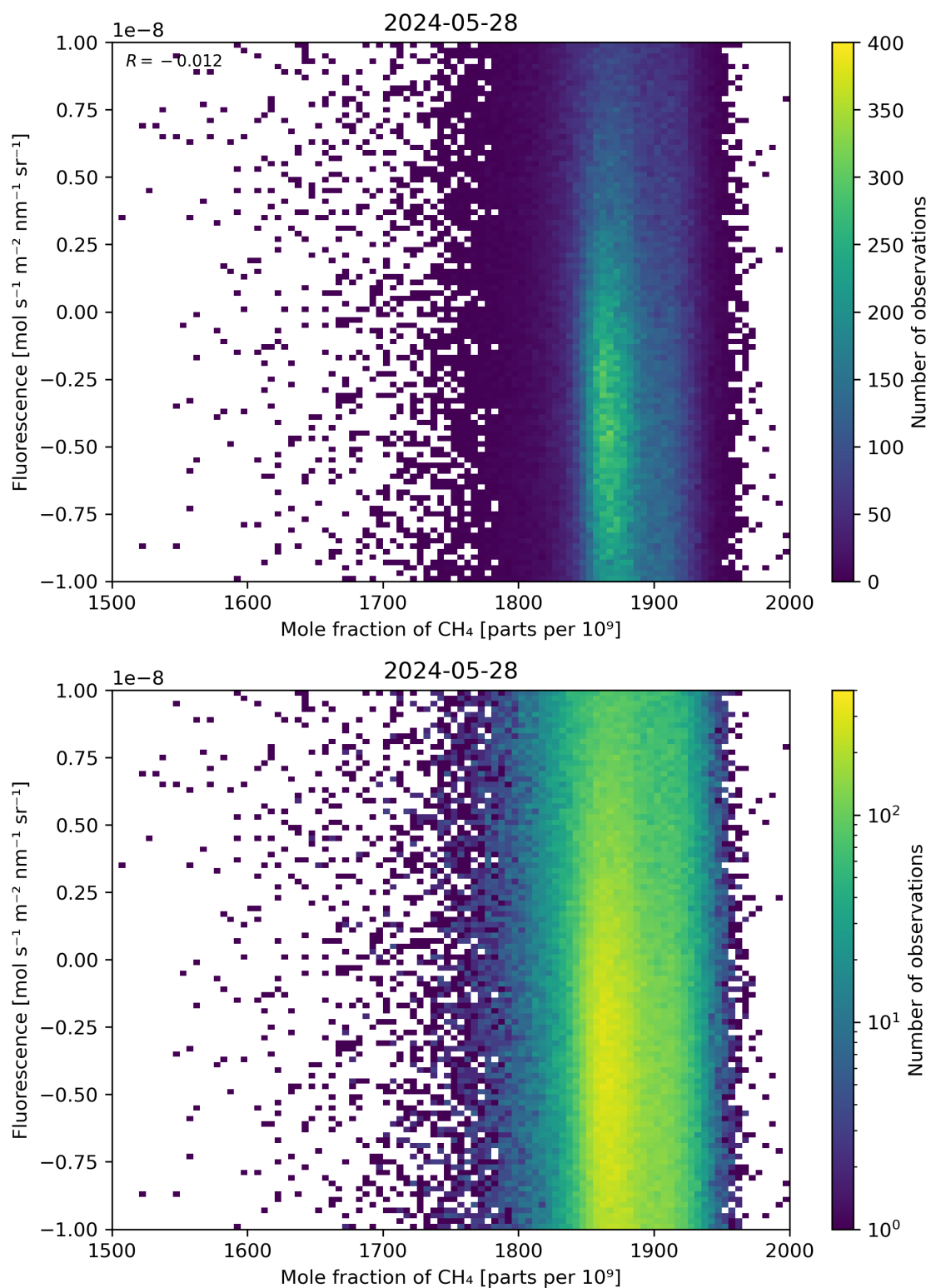
Figure 73: Scatter density plot of “Mole fraction of \text{CH}_4 ” against “Fluorescence” for 2024-05-28 to 2024-05-29.
