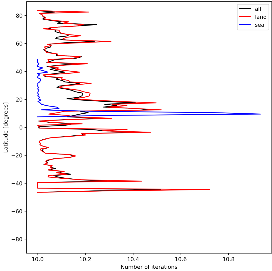
Figure 20: Zonal average of “Number of iterations” for 2024-05-28 to 2024-05-29.
