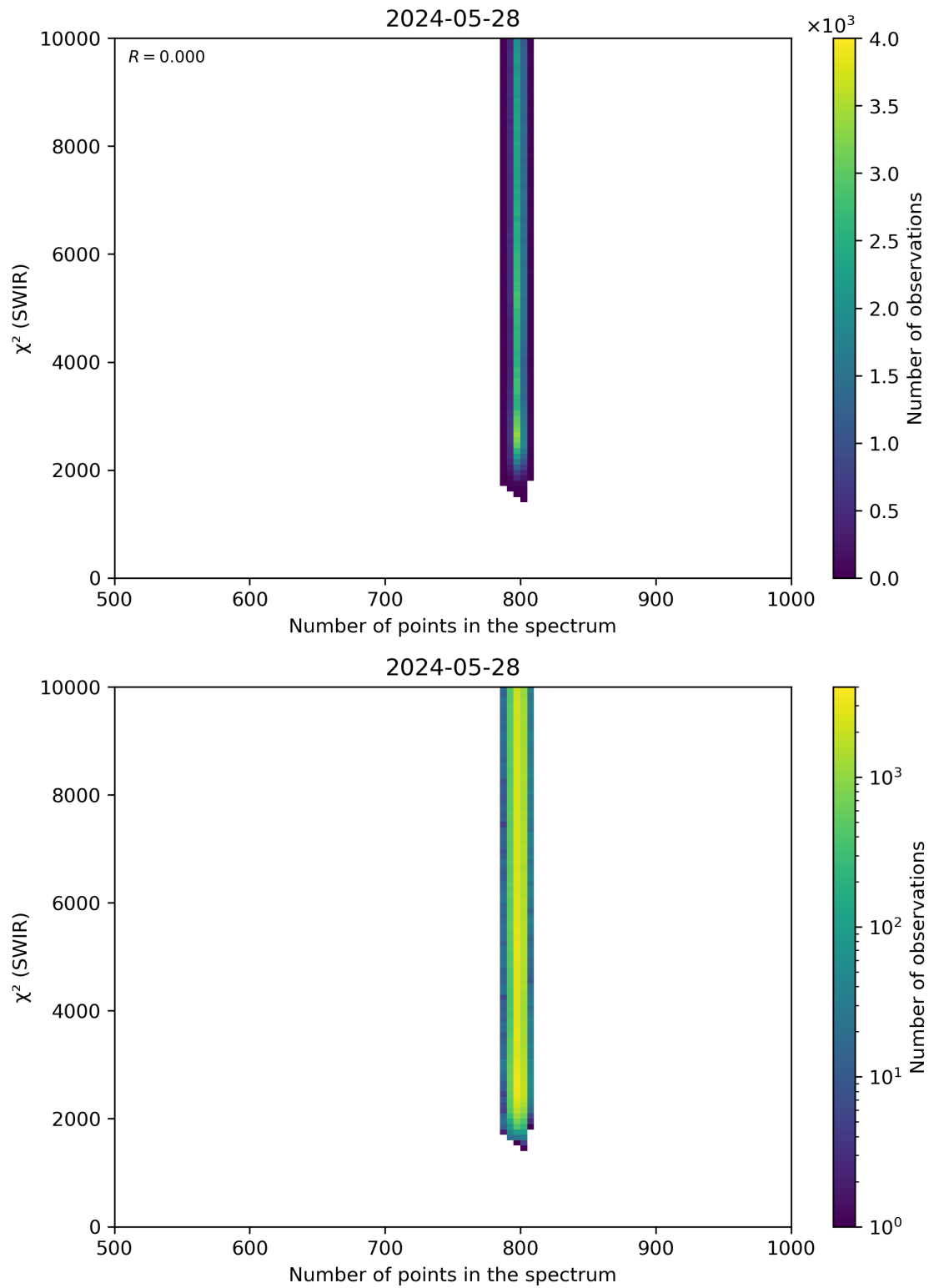
Figure 89: Scatter density plot of “Number of points in the spectrum” against “ \chi^2 (SWIR)” for 2024-05-28 to 2024-05-29.
