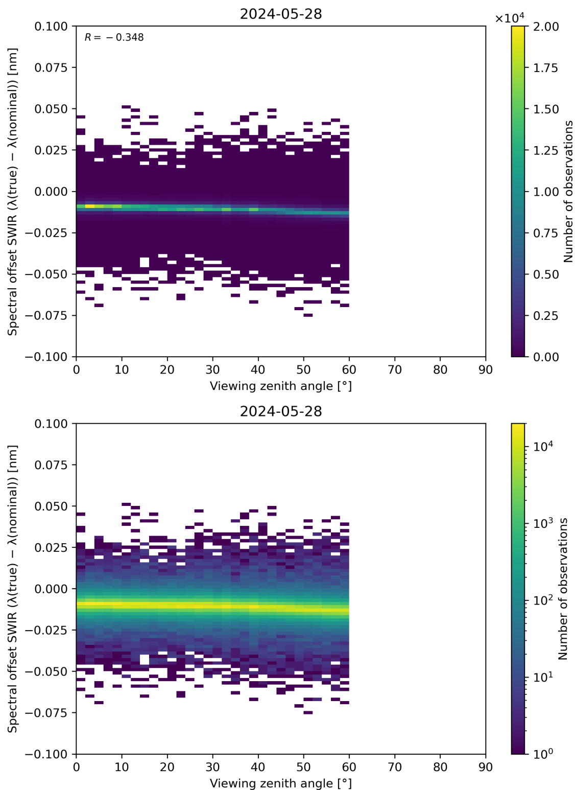
Figure 116: Scatter density plot of “Viewing zenith angle” against “Spectral offset SWIR ( \lambda(\text{true}) - \lambda(\text{nominal}) )” for 2024-05-28 to 2024-05-29.
