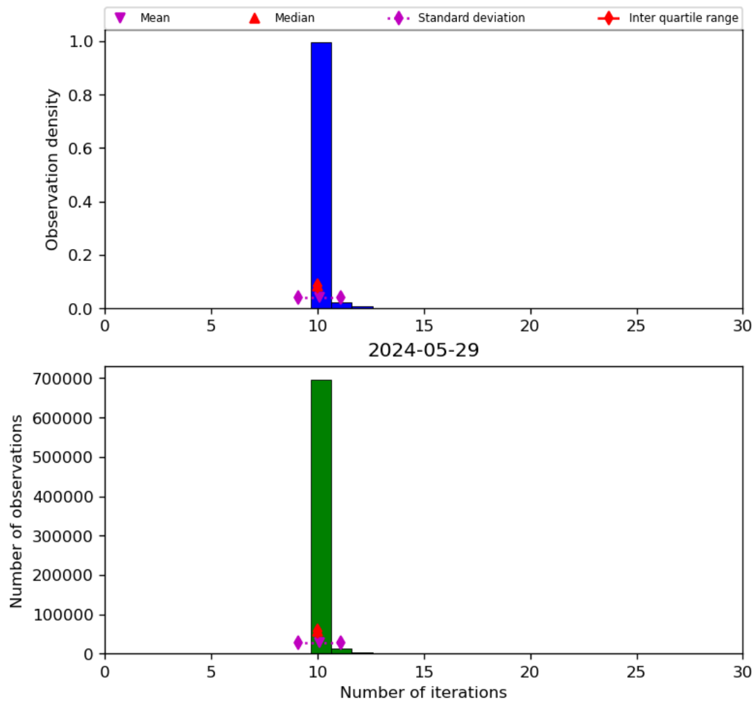
Figure 31: Histogram of “Number of iterations” for 2024-05-28 to 2024-05-30
