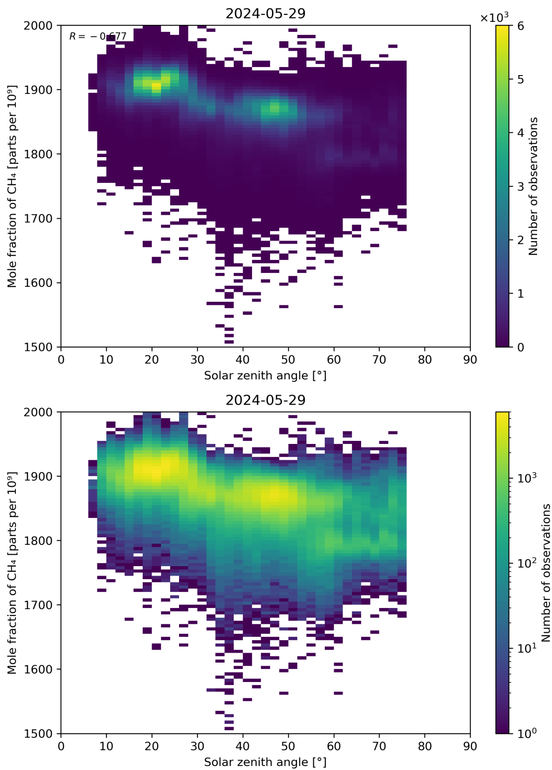
Figure 99: Scatter density plot of “Solar zenith angle” against “Mole fraction of CH 4 ” for 2024-05-28 to 2024-05-30.
