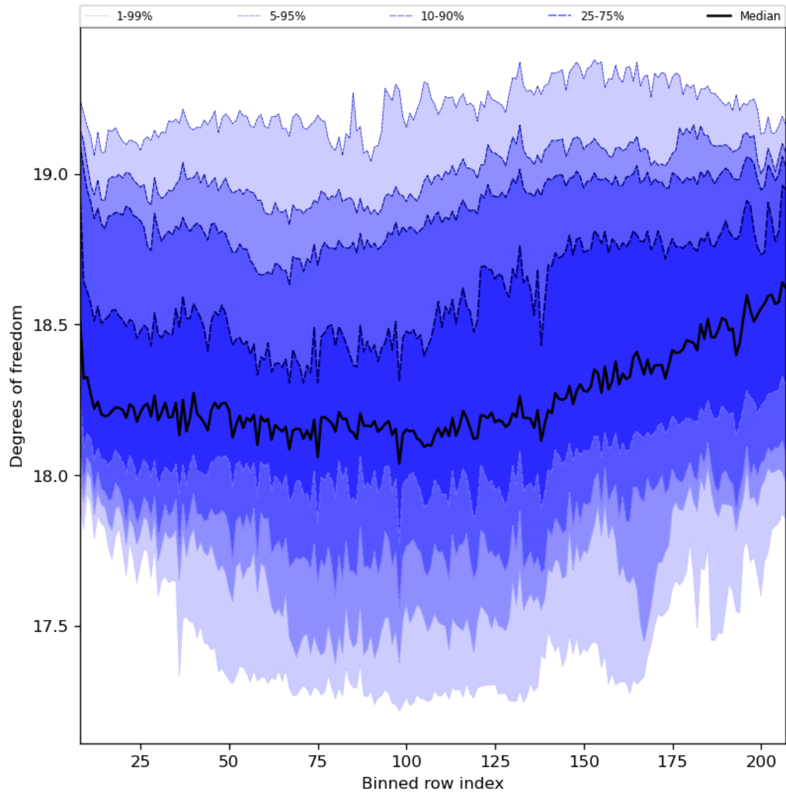
Figure 41: Along track statistics of “Degrees of freedom” for 2024-05-28 to 2024-05-30
