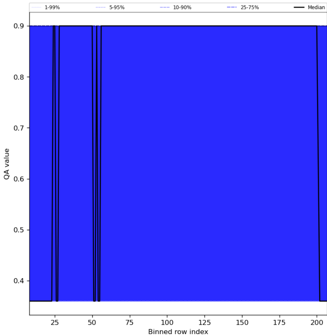
Figure 33: Along track statistics of “QA value” for 2024-05-28 to 2024-05-30
