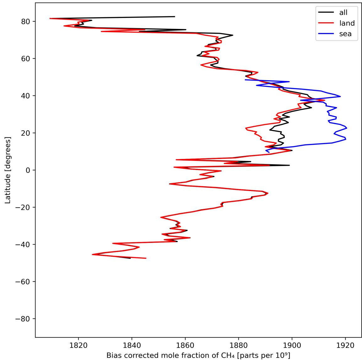
Figure 14: Zonal average of “Bias corrected mole fraction of CH 4 ” for 2024-05-28 to 2024-05-30.
