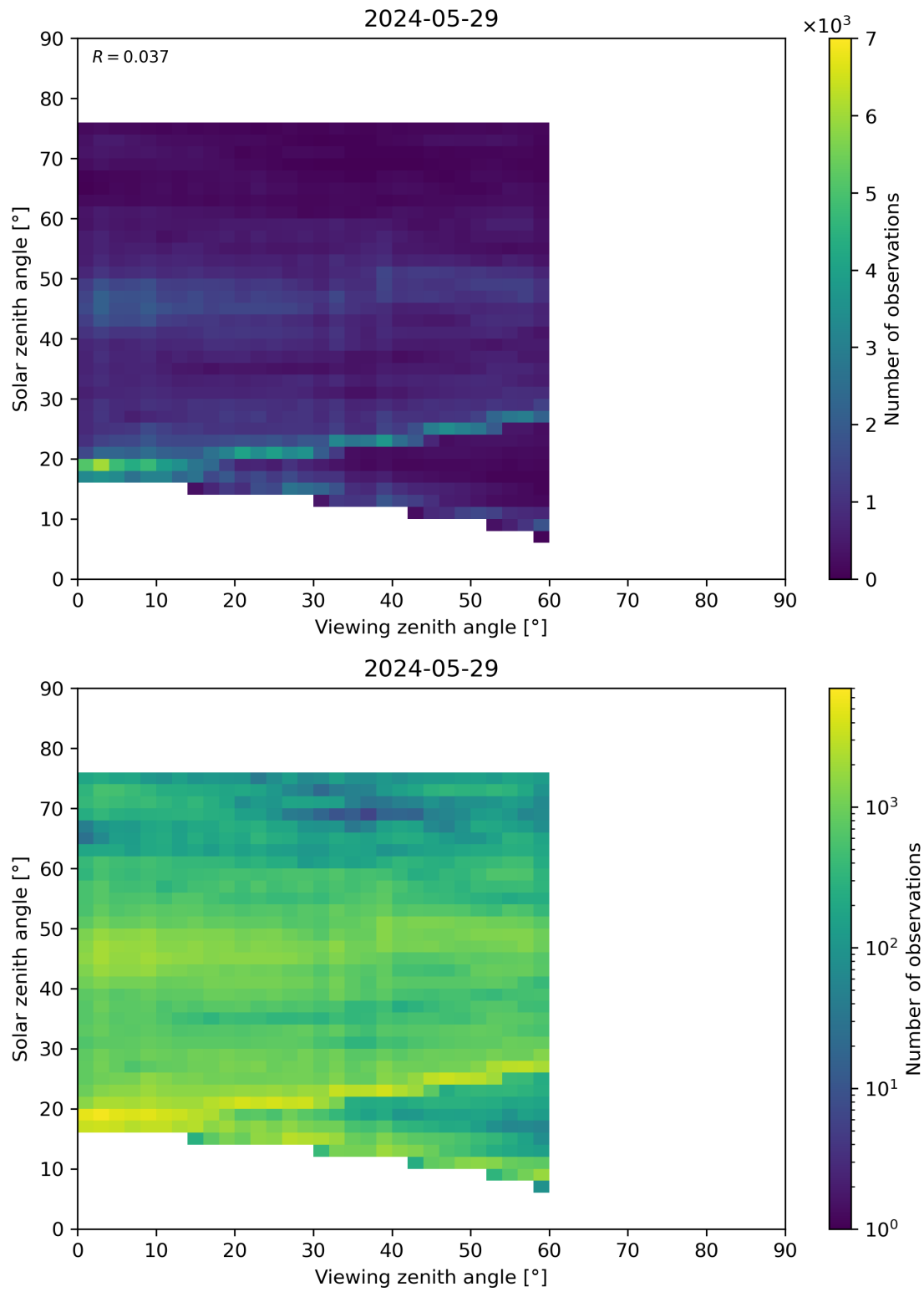
Figure 115: Scatter density plot of “Viewing zenith angle” against “Solar zenith angle” for 2024-05-28 to 2024-05-30.
