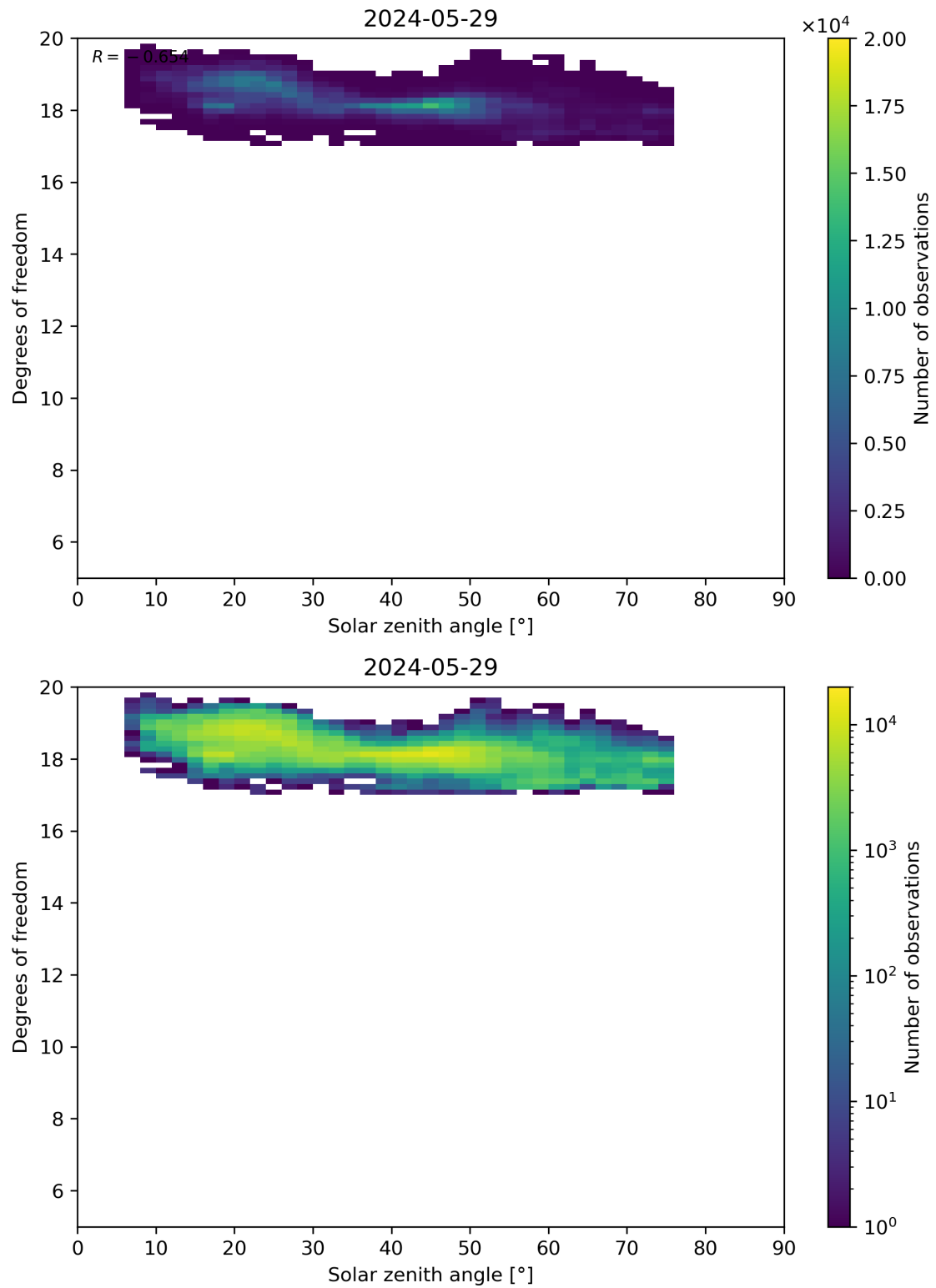
Figure 96: Scatter density plot of “Solar zenith angle” against “Degrees of freedom” for 2024-05-28 to 2024-05-30.
