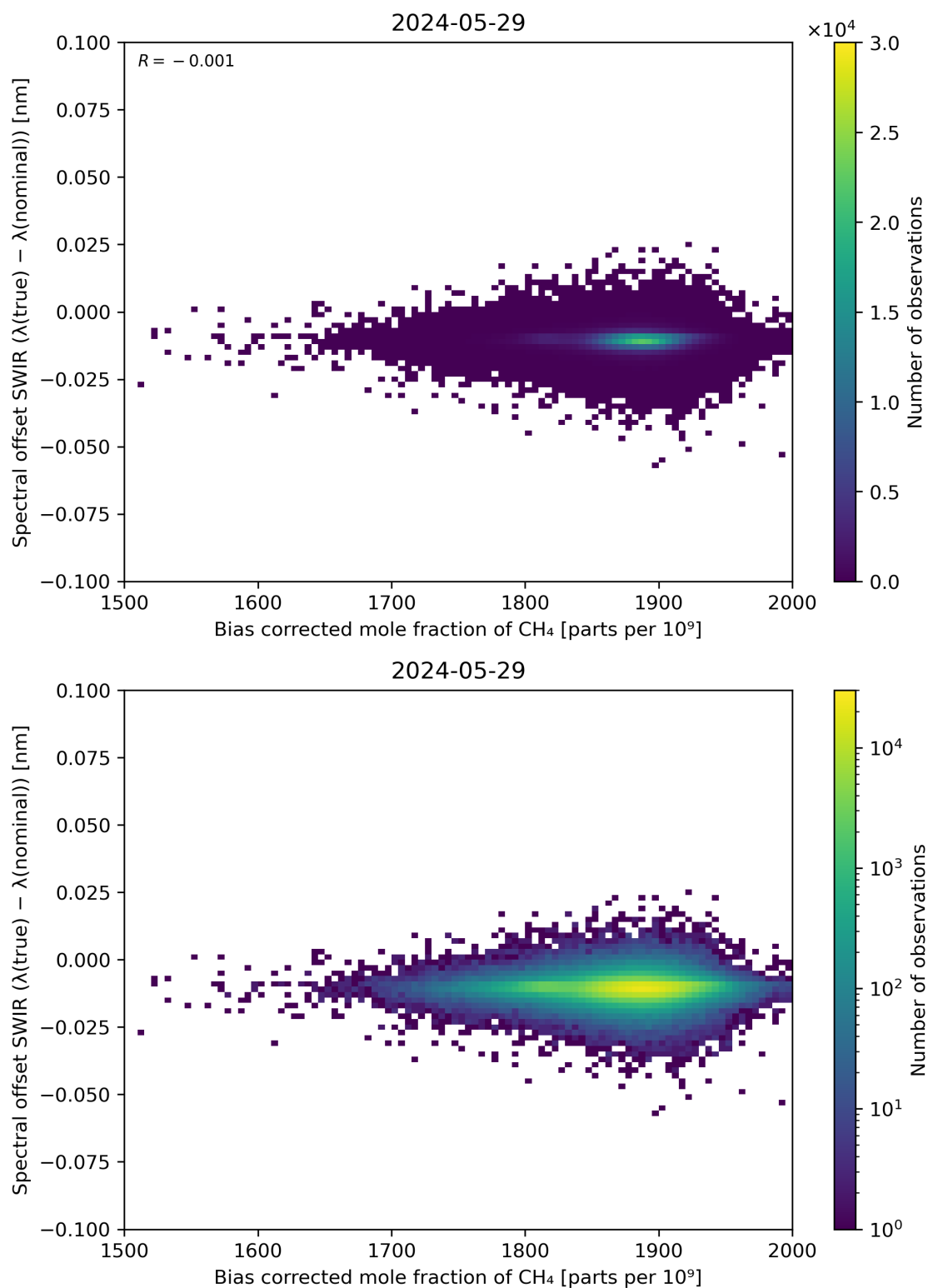
Figure 69: Scatter density plot of “Bias corrected mole fraction of \text{CH}_4 ” against “Spectral offset SWIR ( \lambda(\text{true}) - \lambda(\text{nominal}) )” for 2024-05-28 to 2024-05-30.
