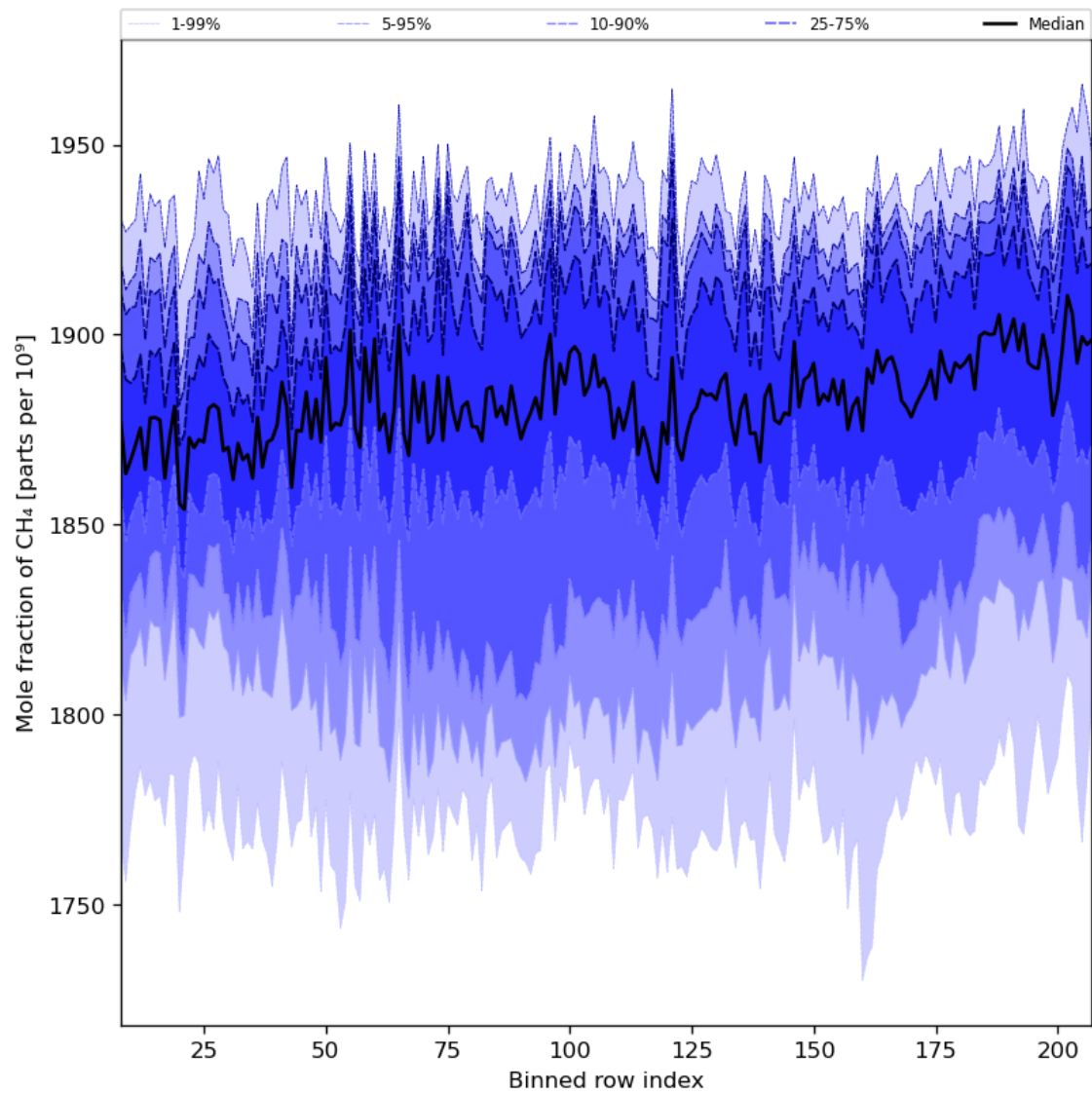
Figure 34: Along track statistics of “Mole fraction of CH 4 ” for 2024-05-28 to 2024-05-30
