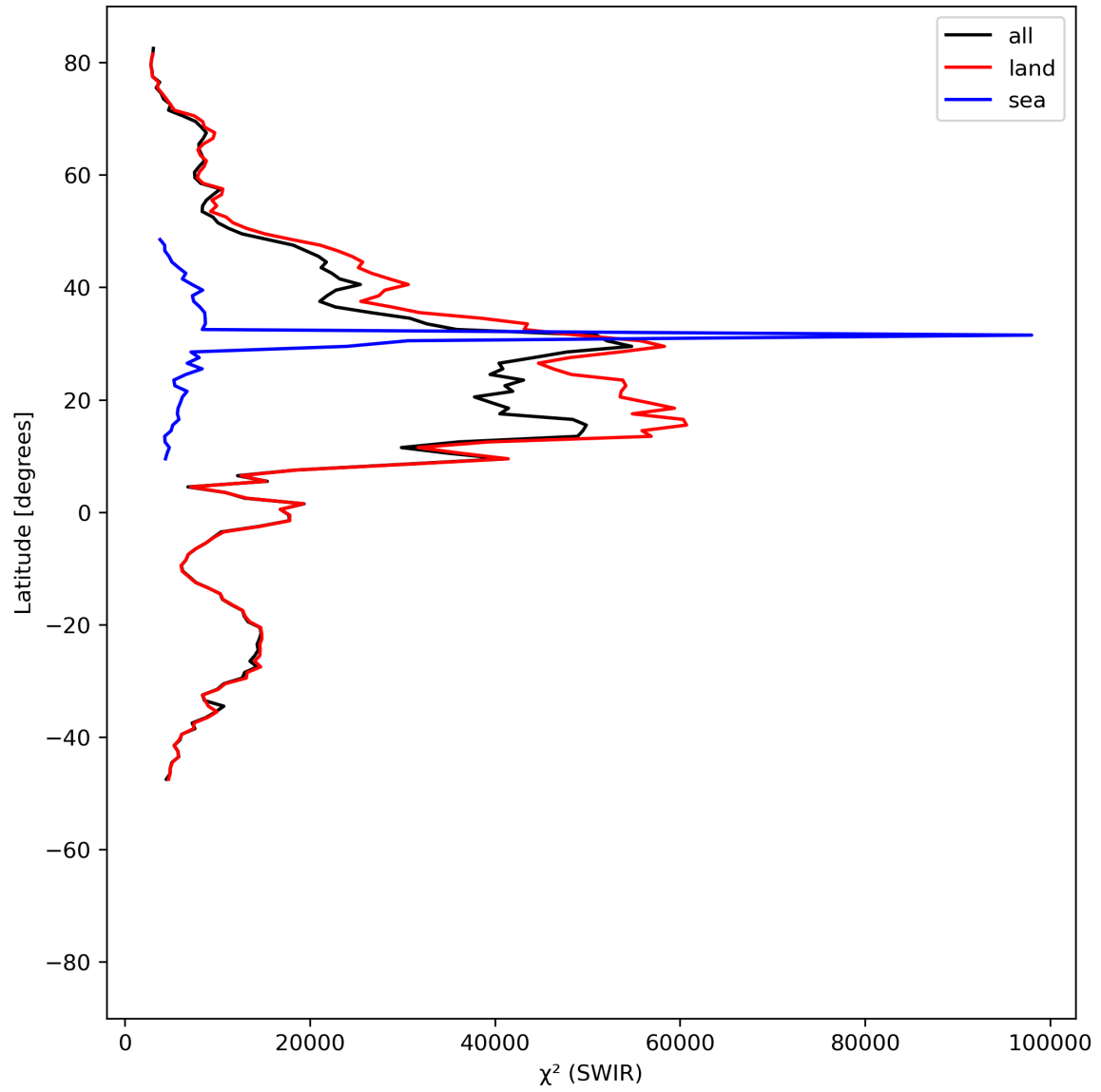
Figure 17: Zonal average of “ \chi^2 (SWIR)” for 2024-05-28 to 2024-05-30.
