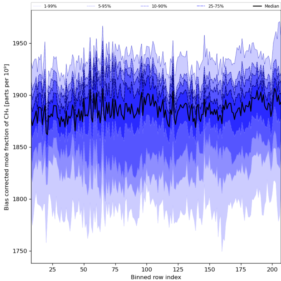
Figure 36: Along track statistics of “Bias corrected mole fraction of CH 4 ” for 2024-05-28 to 2024-05-30
