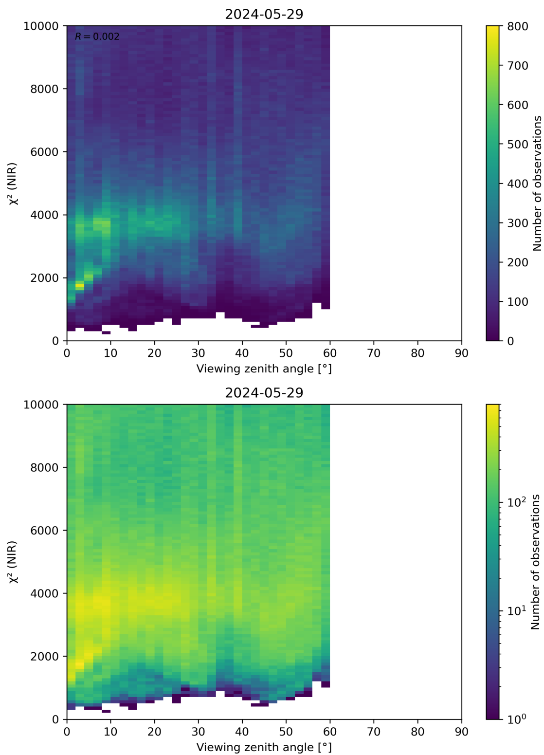
Figure 105: Scatter density plot of “Viewing zenith angle” against “ \chi^2 (NIR)” for 2024-05-28 to 2024-05-30.
