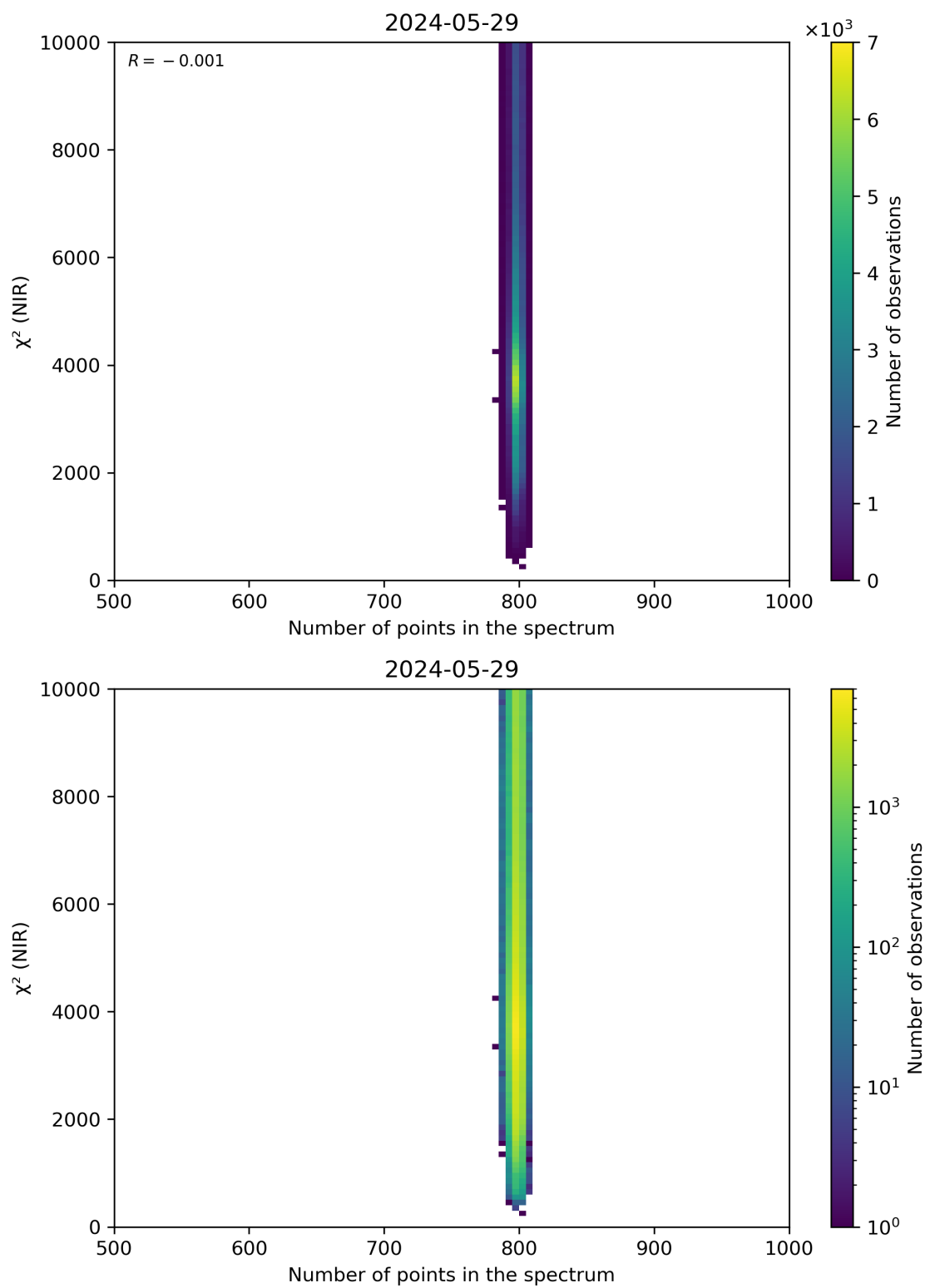
Figure 88: Scatter density plot of “Number of points in the spectrum” against “ \chi^2 (NIR)” for 2024-05-28 to 2024-05-30.
