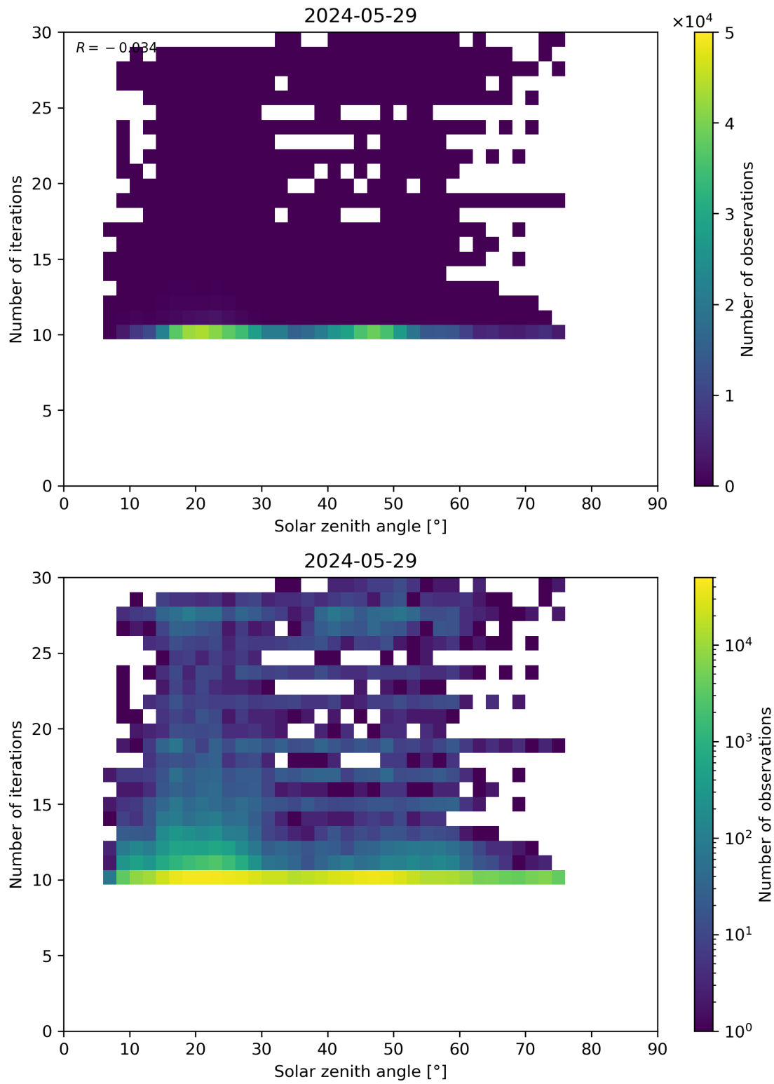
Figure 102: Scatter density plot of “Solar zenith angle” against “Number of iterations” for 2024-05-28 to 2024-05-30.
