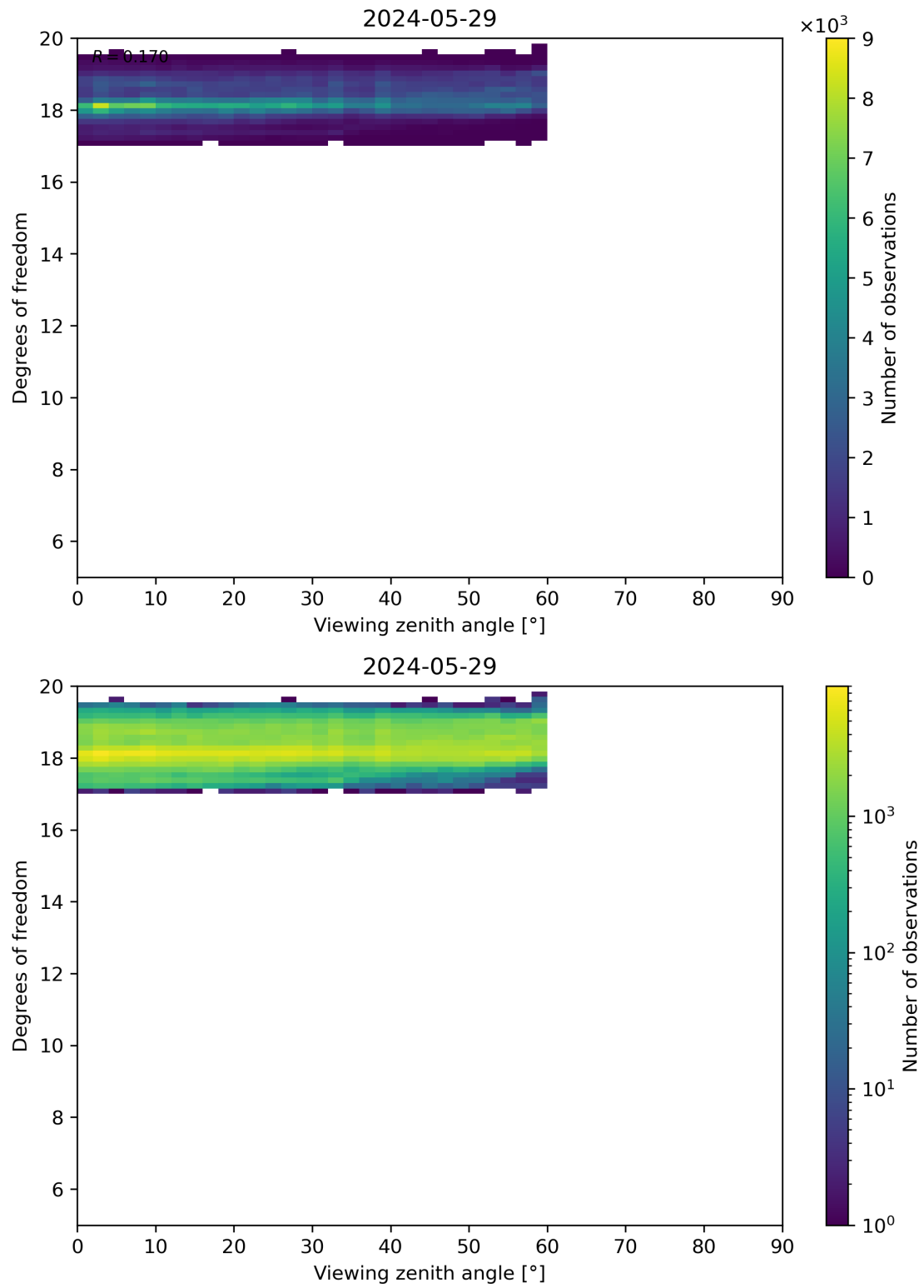
Figure 107: Scatter density plot of “Viewing zenith angle” against “Degrees of freedom” for 2024-05-28 to 2024-05-30.
