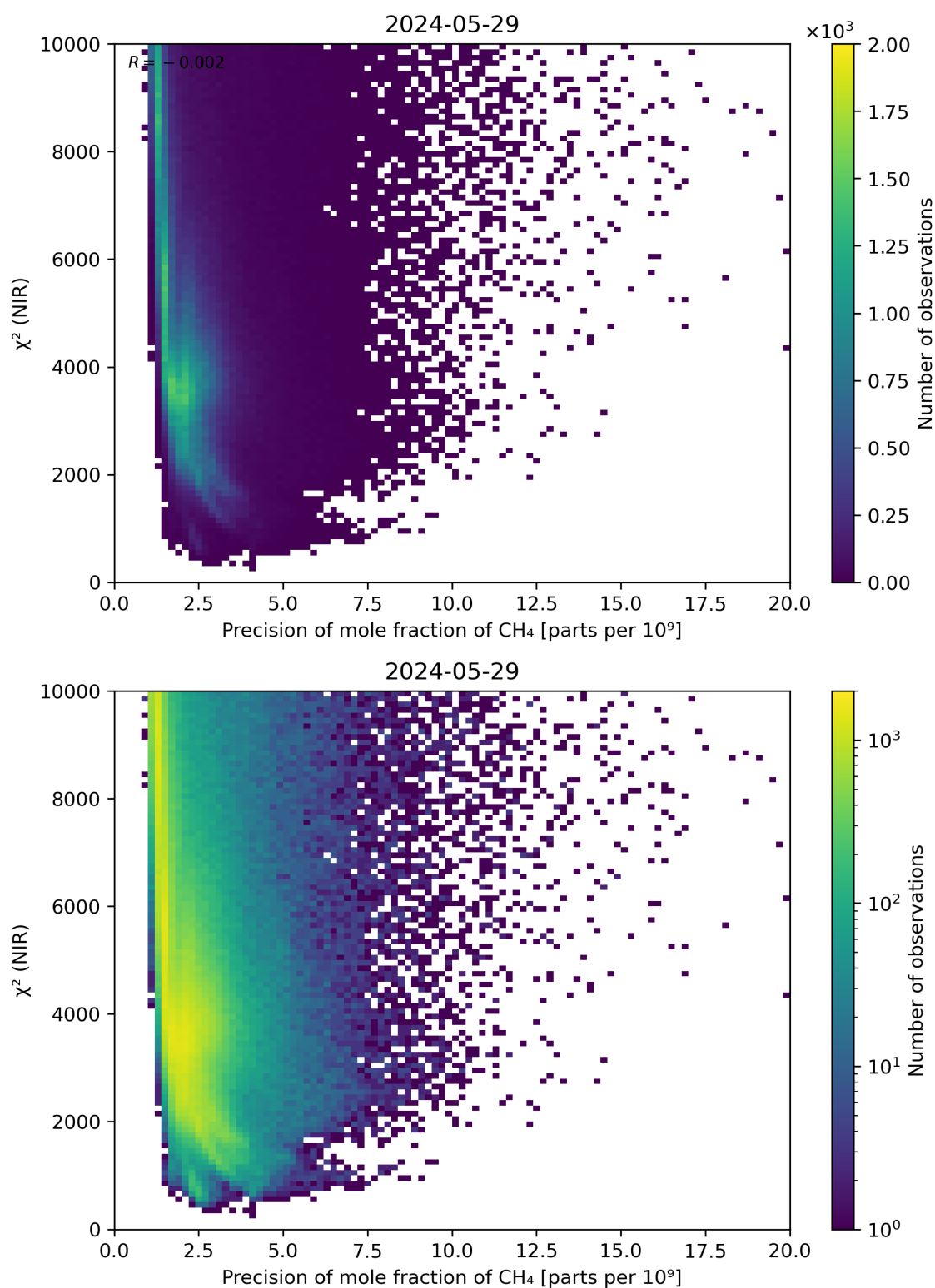
Figure 78: Scatter density plot of “Precision of mole fraction of \text{CH}_4 ” against “ \chi^2 (NIR)” for 2024-05-28 to 2024-05-30.
