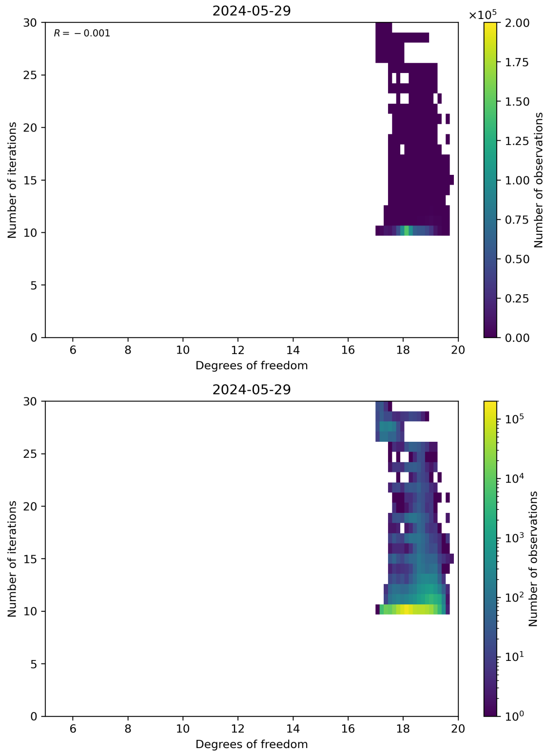
Figure 52: Scatter density plot of “Degrees of freedom” against “Number of iterations” for 2024-05-28 to 2024-05-30.
