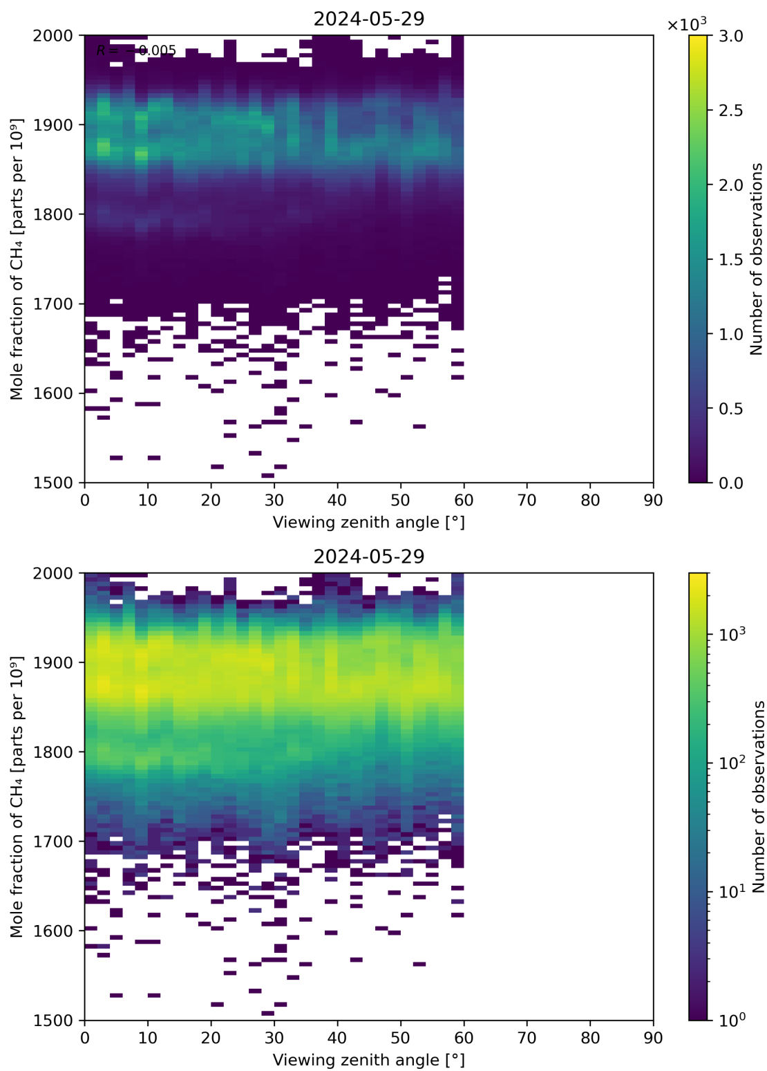
Figure 110: Scatter density plot of “Viewing zenith angle” against “Mole fraction of CH 4 ” for 2024-05-28 to 2024-05-30.
