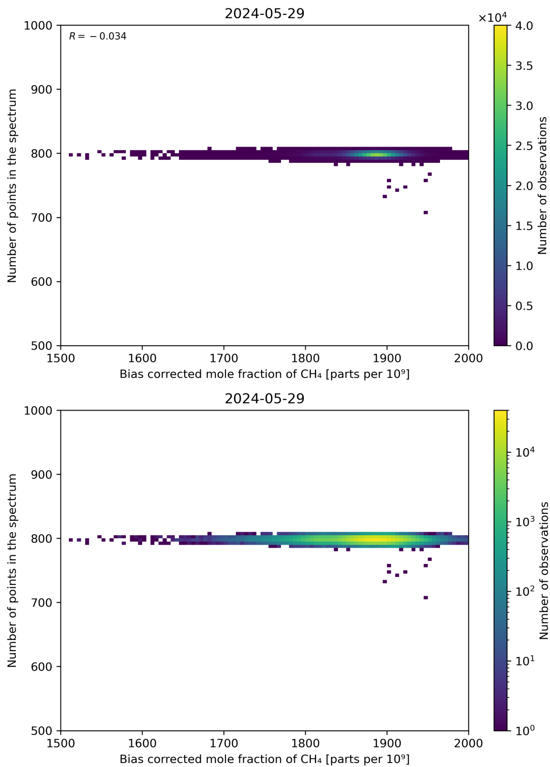
Figure 68: Scatter density plot of “Bias corrected mole fraction of CH 4 ” against “Number of points in the spectrum” for 2024-05-28 to 2024-05-30.
