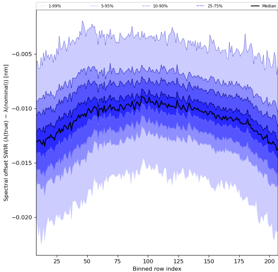
Figure 38: Along track statistics of “Spectral offset SWIR ( \lambda(\text{true}) - \lambda(\text{nominal}) )” for 2024-05-28 to 2024-05-30
