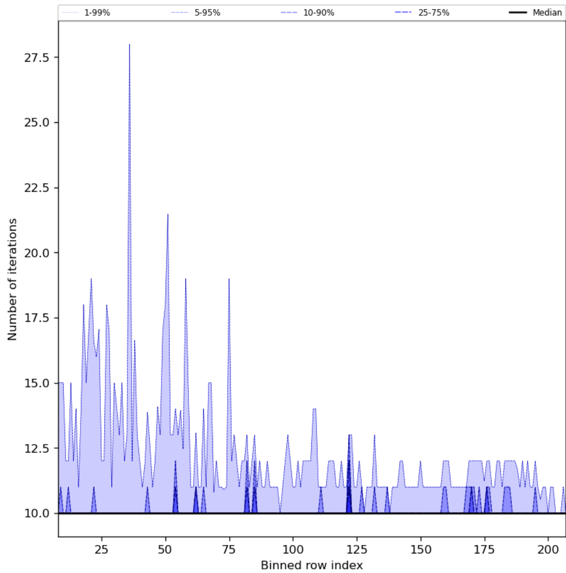
Figure 42: Along track statistics of “Number of iterations” for 2024-05-28 to 2024-05-30
