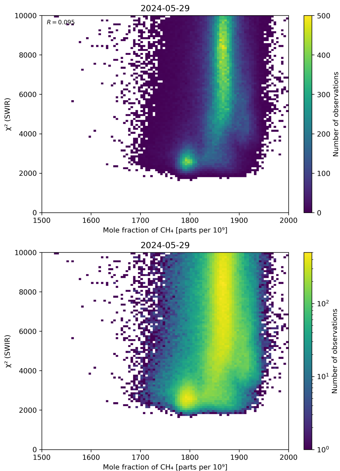
Figure 71: Scatter density plot of “Mole fraction of \text{CH}_4 ” against “ \chi^2 (SWIR)” for 2024-05-28 to 2024-05-30.
