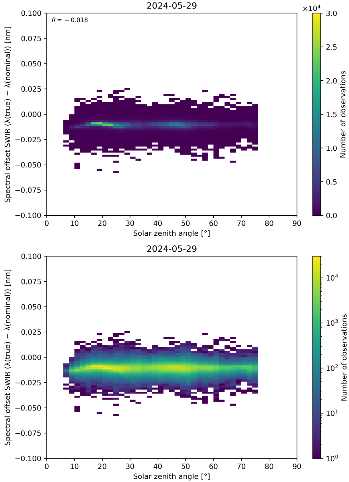
Figure 104: Scatter density plot of “Solar zenith angle” against “Spectral offset SWIR ( \lambda(\text{true}) - \lambda(\text{nominal}) )” for 2024-05-28 to 2024-05-30.
