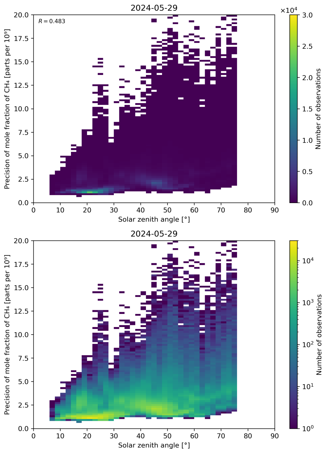
Figure 101: Scatter density plot of “Solar zenith angle” against “Precision of mole fraction of \text{CH}_4 ” for 2024-05-28 to 2024-05-30.
