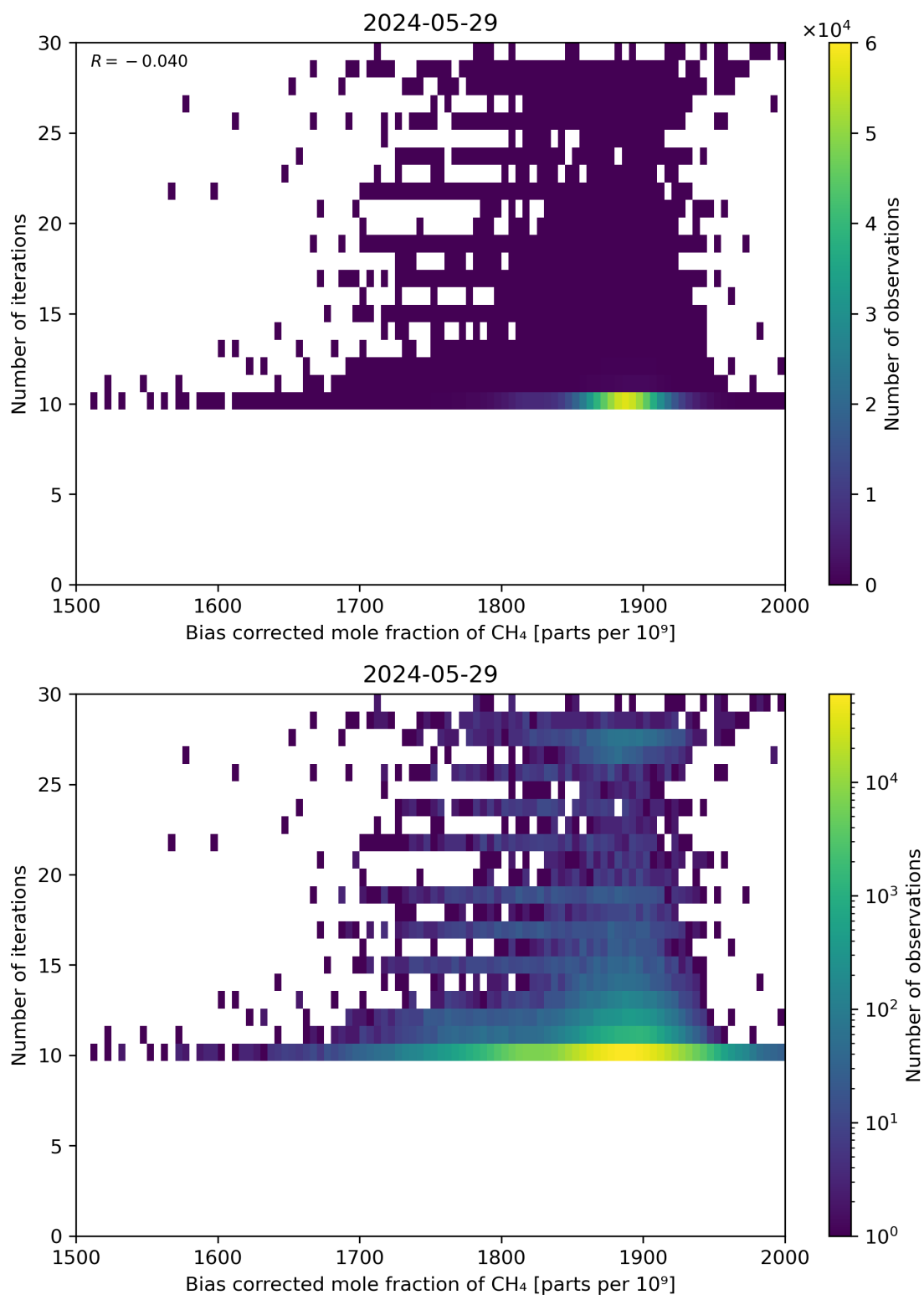
Figure 67: Scatter density plot of “Bias corrected mole fraction of \text{CH}_4 ” against “Number of iterations” for 2024-05-28 to 2024-05-30.
