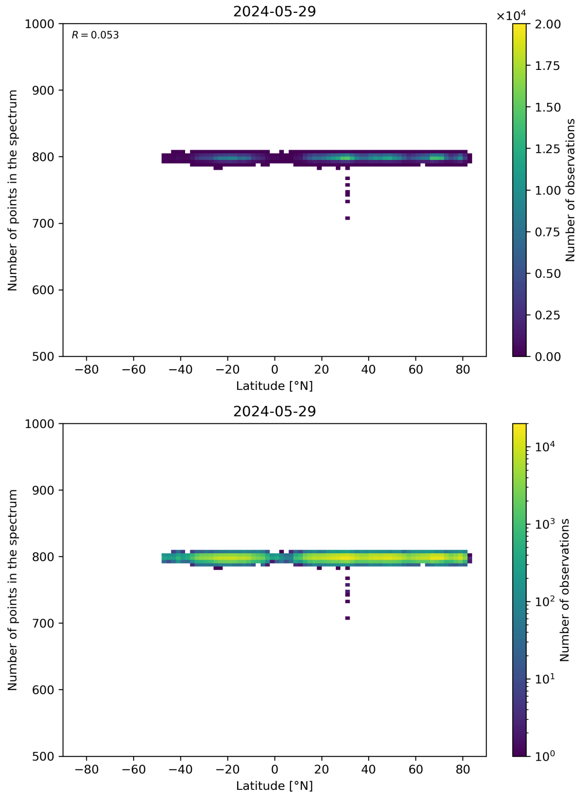
Figure 61: Scatter density plot of “Latitude” against “Number of points in the spectrum” for 2024-05-28 to 2024-05-30.
