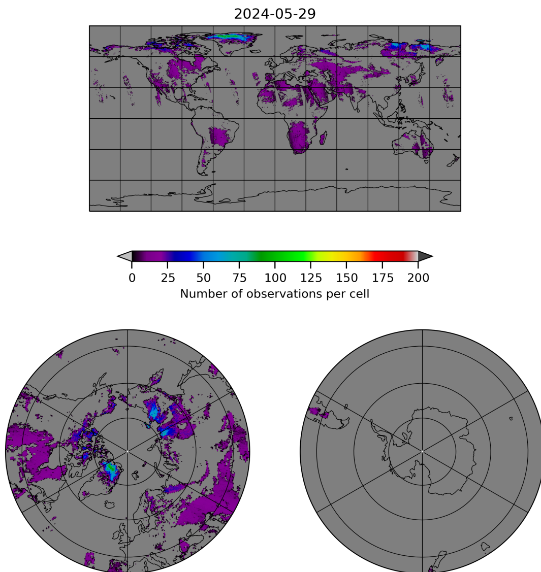
Figure 10: Map of the number of observations for 2024-05-28 to 2024-05-30
