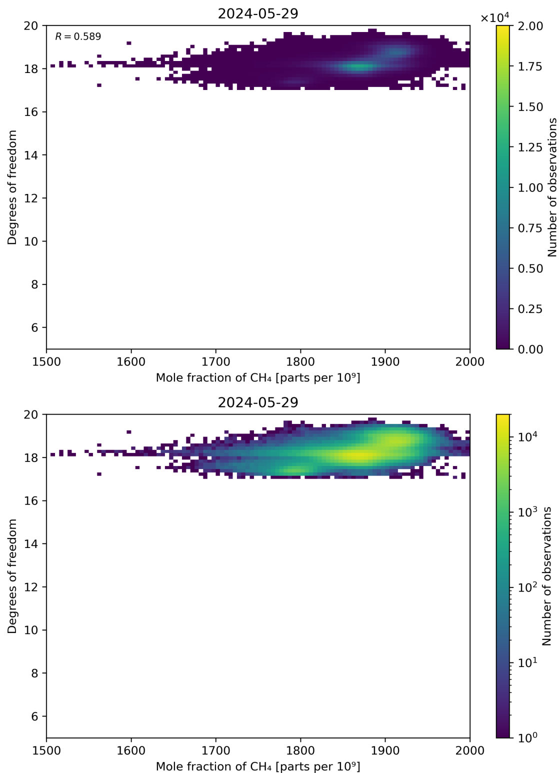
Figure 72: Scatter density plot of “Mole fraction of CH 4 ” against “Degrees of freedom” for 2024-05-28 to 2024-05-30.
