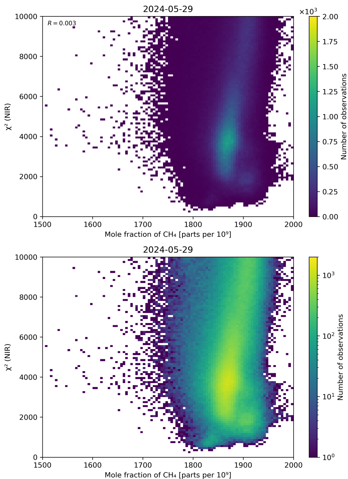
Figure 70: Scatter density plot of “Mole fraction of \text{CH}_4 ” against “ \chi^2 (NIR)” for 2024-05-28 to 2024-05-30.
