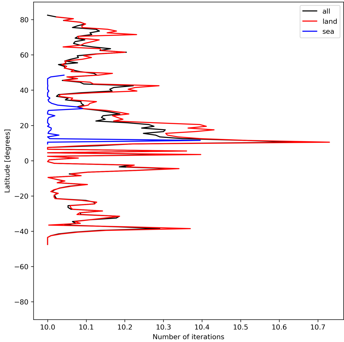
Figure 20: Zonal average of “Number of iterations” for 2024-05-28 to 2024-05-30.
