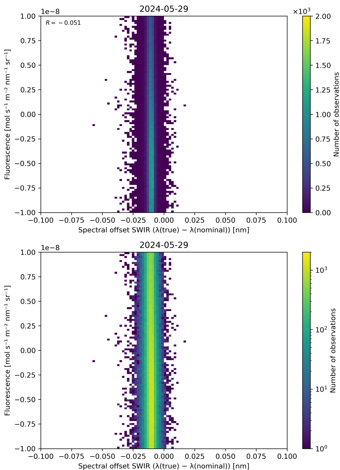
Figure 120: Scatter density plot of “Spectral offset SWIR ( \lambda(\text{true}) - \lambda(\text{nominal}) )” against “Fluorescence” for 2024-05-28 to 2024-05-30.
