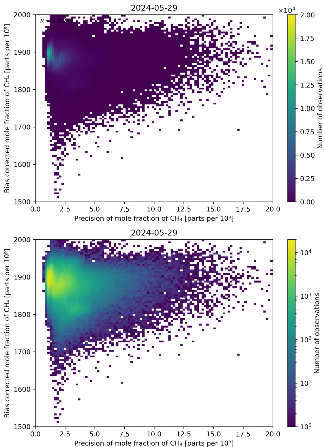
Figure 82: Scatter density plot of “Precision of mole fraction of CH 4 ” against “Bias corrected mole fraction of CH 4 ” for 2024-05-28 to 2024-05-30.
