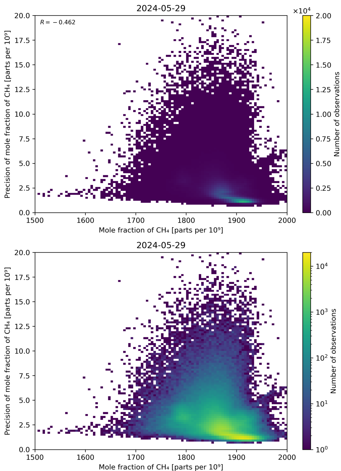
Figure 75: Scatter density plot of “Mole fraction of CH 4 ” against “Precision of mole fraction of CH 4 ” for 2024-05-28 to 2024-05-30.
