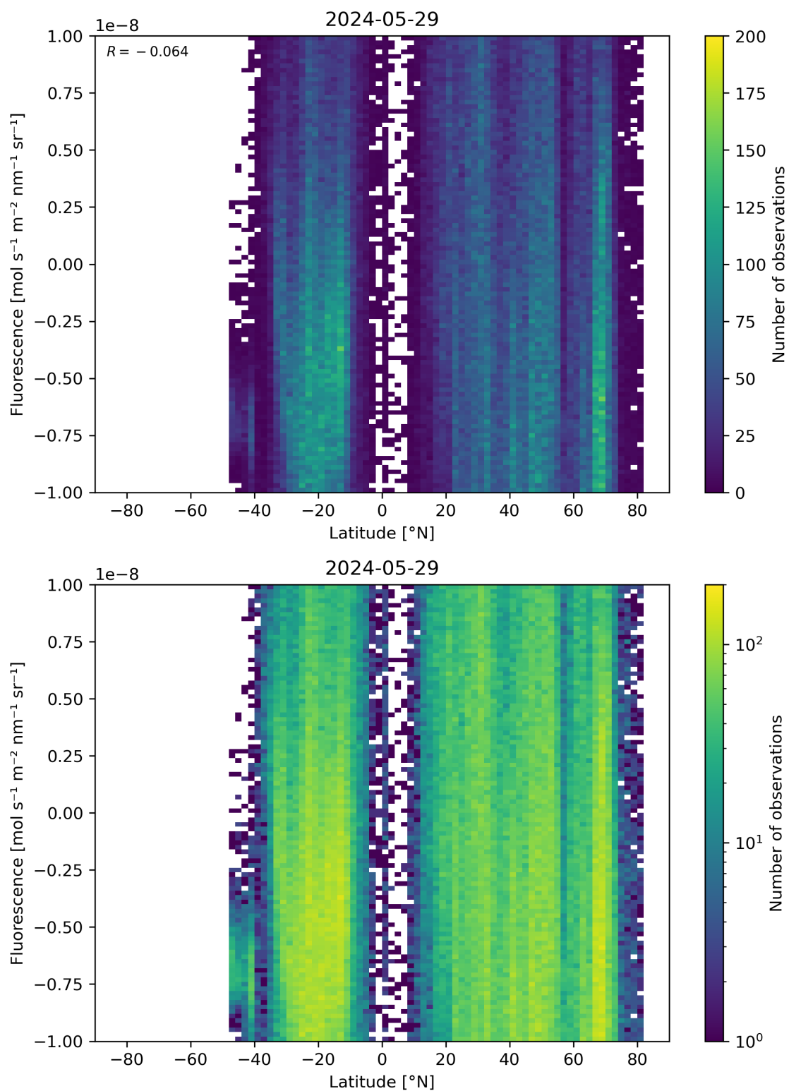
Figure 56: Scatter density plot of “Latitude” against “Fluorescence” for 2024-05-28 to 2024-05-30.
