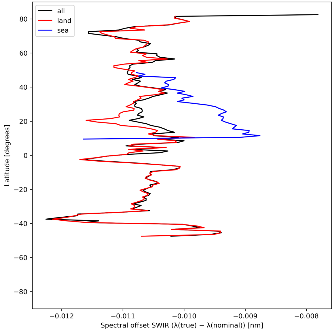
Figure 16: Zonal average of “Spectral offset SWIR ( \lambda(\text{true}) - \lambda(\text{nominal}) )” for 2024-05-28 to 2024-05-30.
