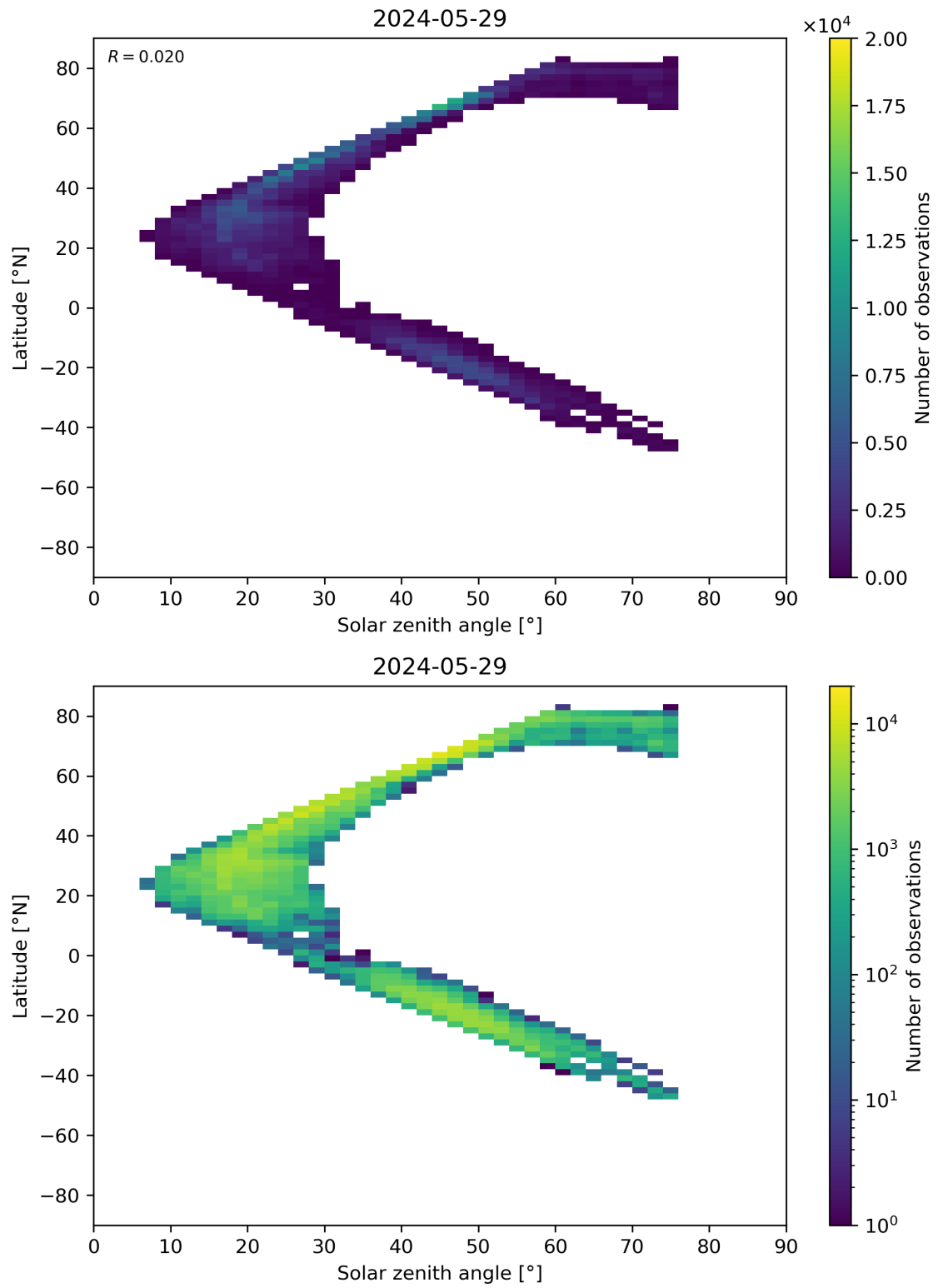
Figure 98: Scatter density plot of “Solar zenith angle” against “Latitude” for 2024-05-28 to 2024-05-30.
