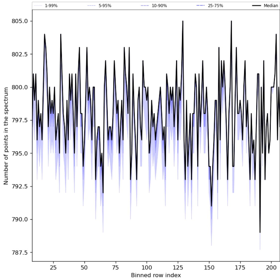
Figure 37: Along track statistics of “Number of points in the spectrum” for 2024-05-28 to 2024-05-30
