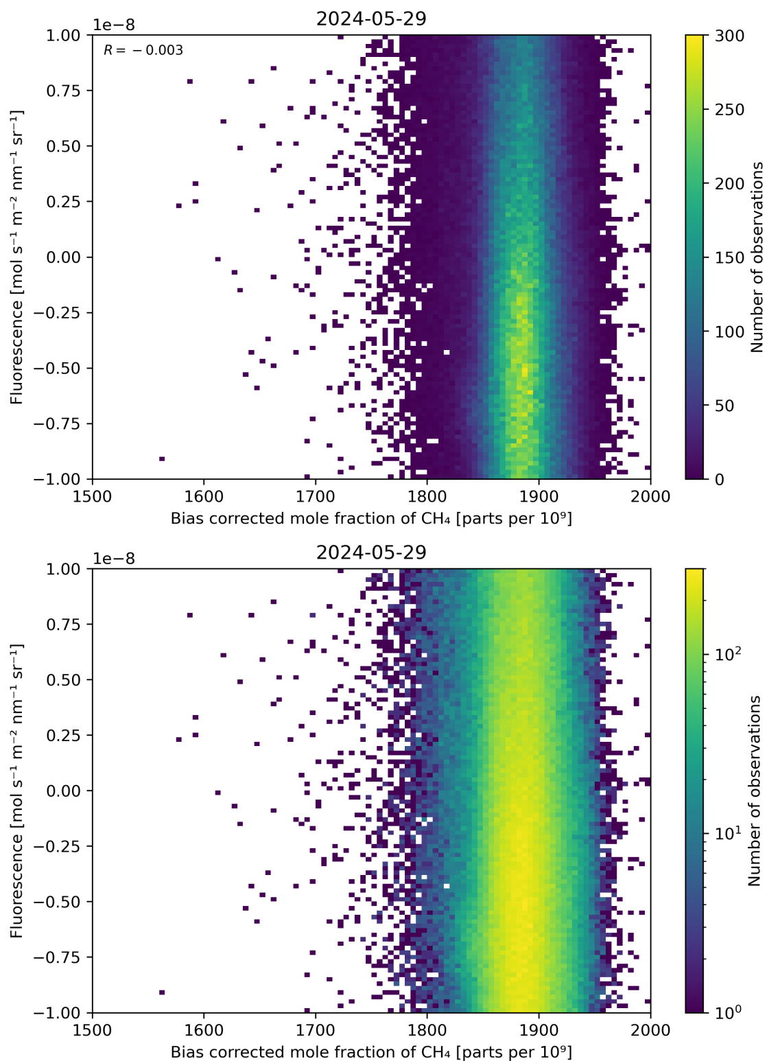
Figure 66: Scatter density plot of “Bias corrected mole fraction of \text{CH}_4 ” against “Fluorescence” for 2024-05-28 to 2024-05-30.
