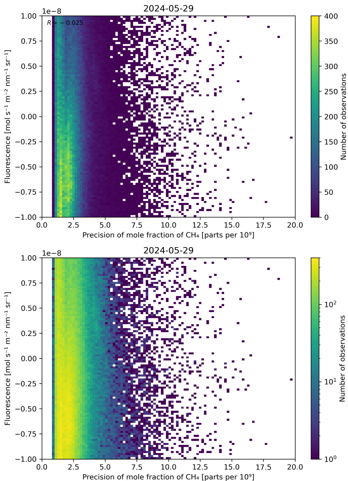
Figure 81: Scatter density plot of “Precision of mole fraction of CH 4 ” against “Fluorescence” for 2024-05-28 to 2024-05-30.
