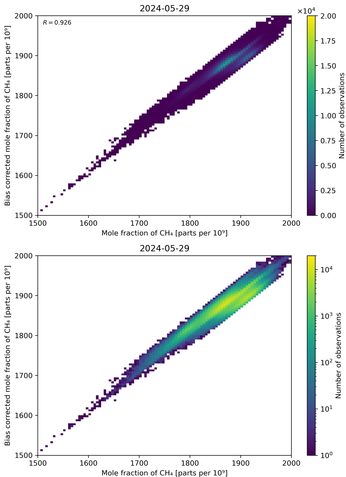
Figure 74: Scatter density plot of “Mole fraction of CH 4 ” against “Bias corrected mole fraction of CH 4 ” for 2024-05-28 to 2024-05-30.
