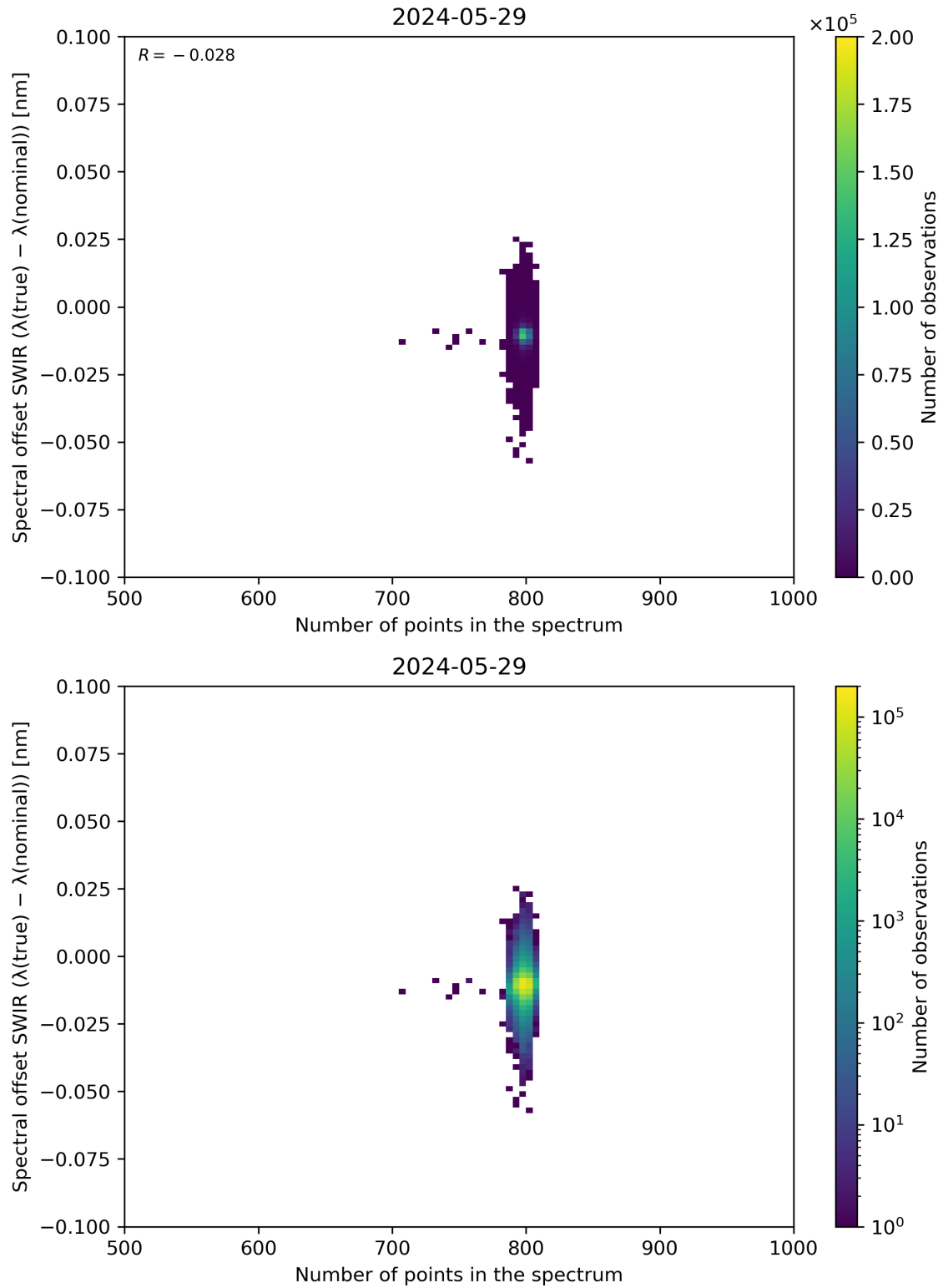
Figure 93: Scatter density plot of “Number of points in the spectrum” against “Spectral offset SWIR ( \lambda(\text{true}) - \lambda(\text{nominal}) )” for 2024-05-28 to 2024-05-30.
