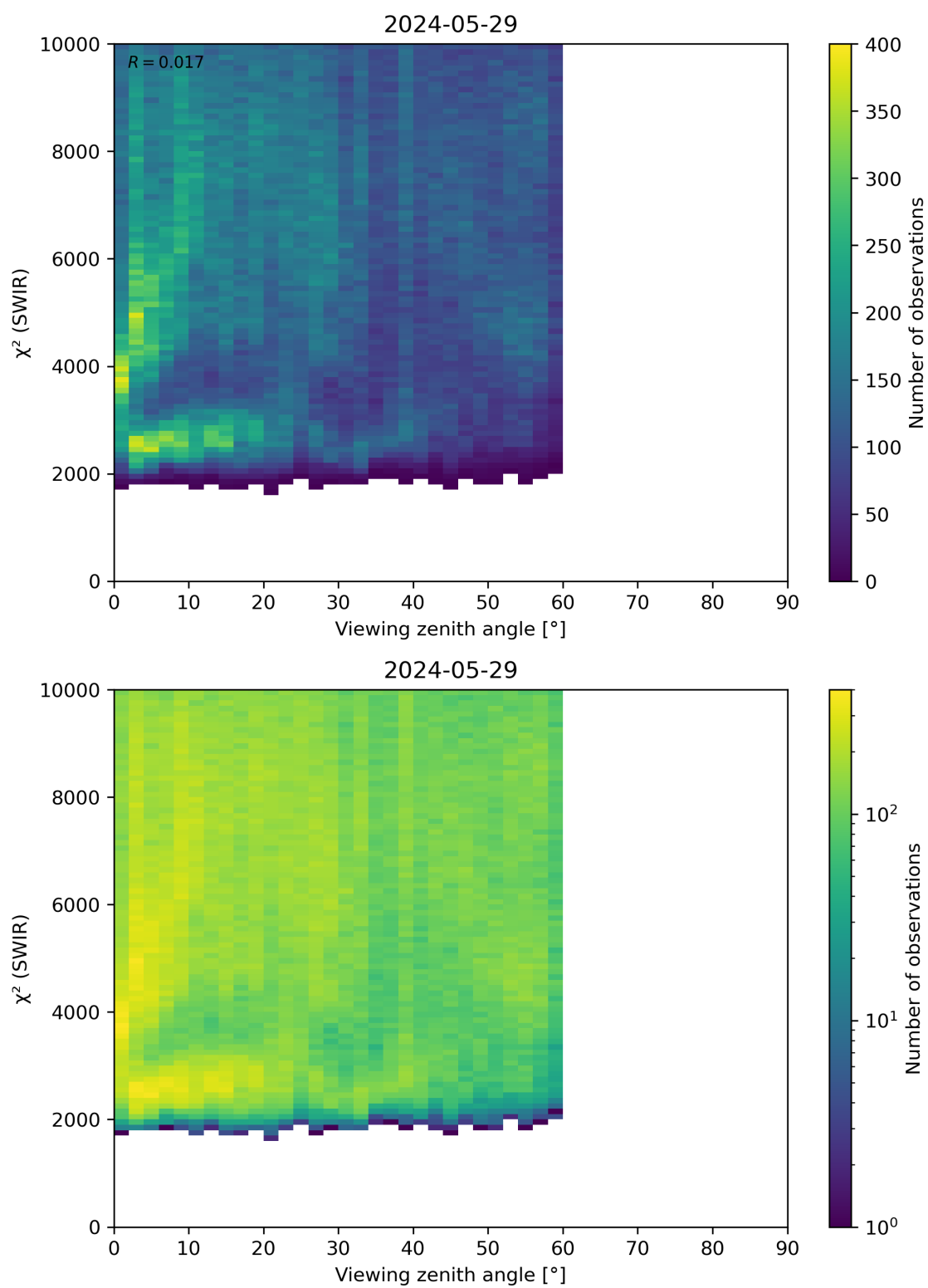
Figure 106: Scatter density plot of “Viewing zenith angle” against “ \chi^2 (SWIR)” for 2024-05-28 to 2024-05-30.
