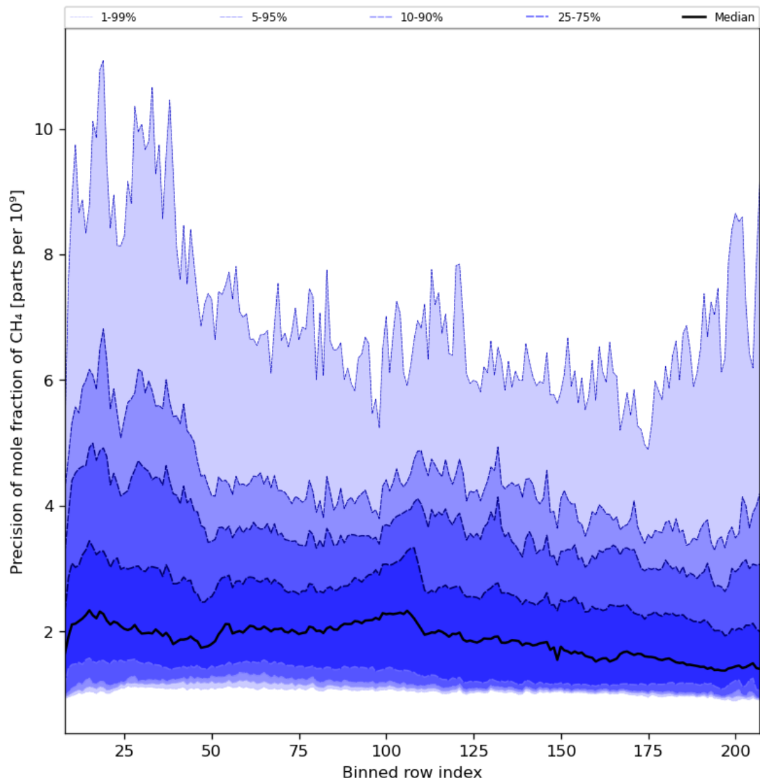
Figure 35: Along track statistics of “Precision of mole fraction of CH 4 ” for 2024-05-28 to 2024-05-30
