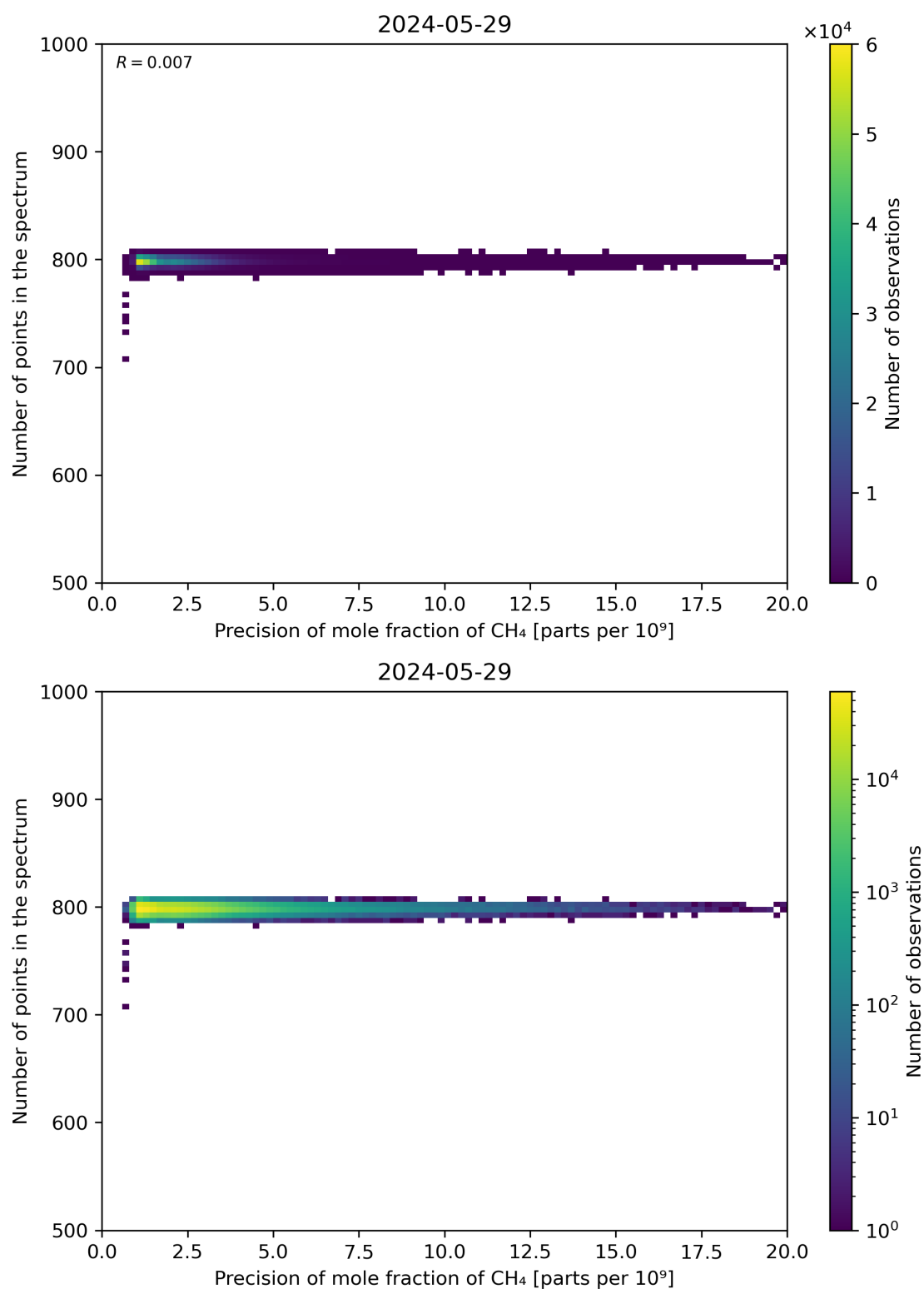
Figure 84: Scatter density plot of “Precision of mole fraction of CH 4 ” against “Number of points in the spectrum” for 2024-05-28 to 2024-05-30.
