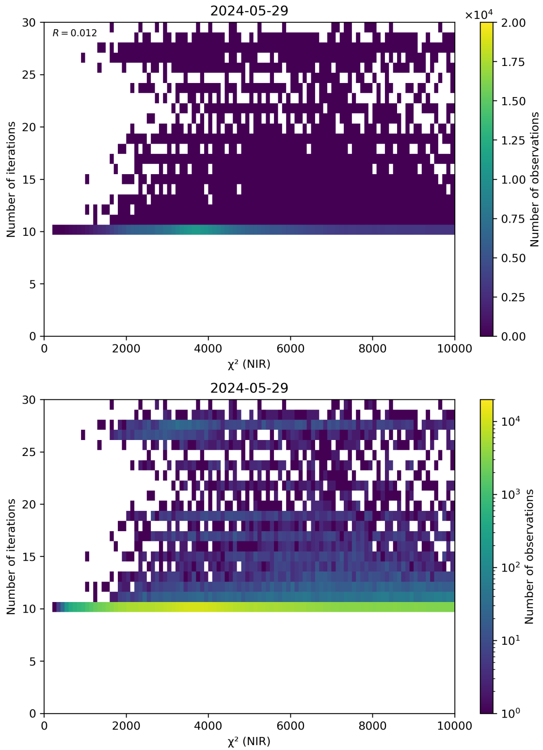
Figure 46: Scatter density plot of “ \chi^2 (NIR)” against “Number of iterations” for 2024-05-28 to 2024-05-30.
