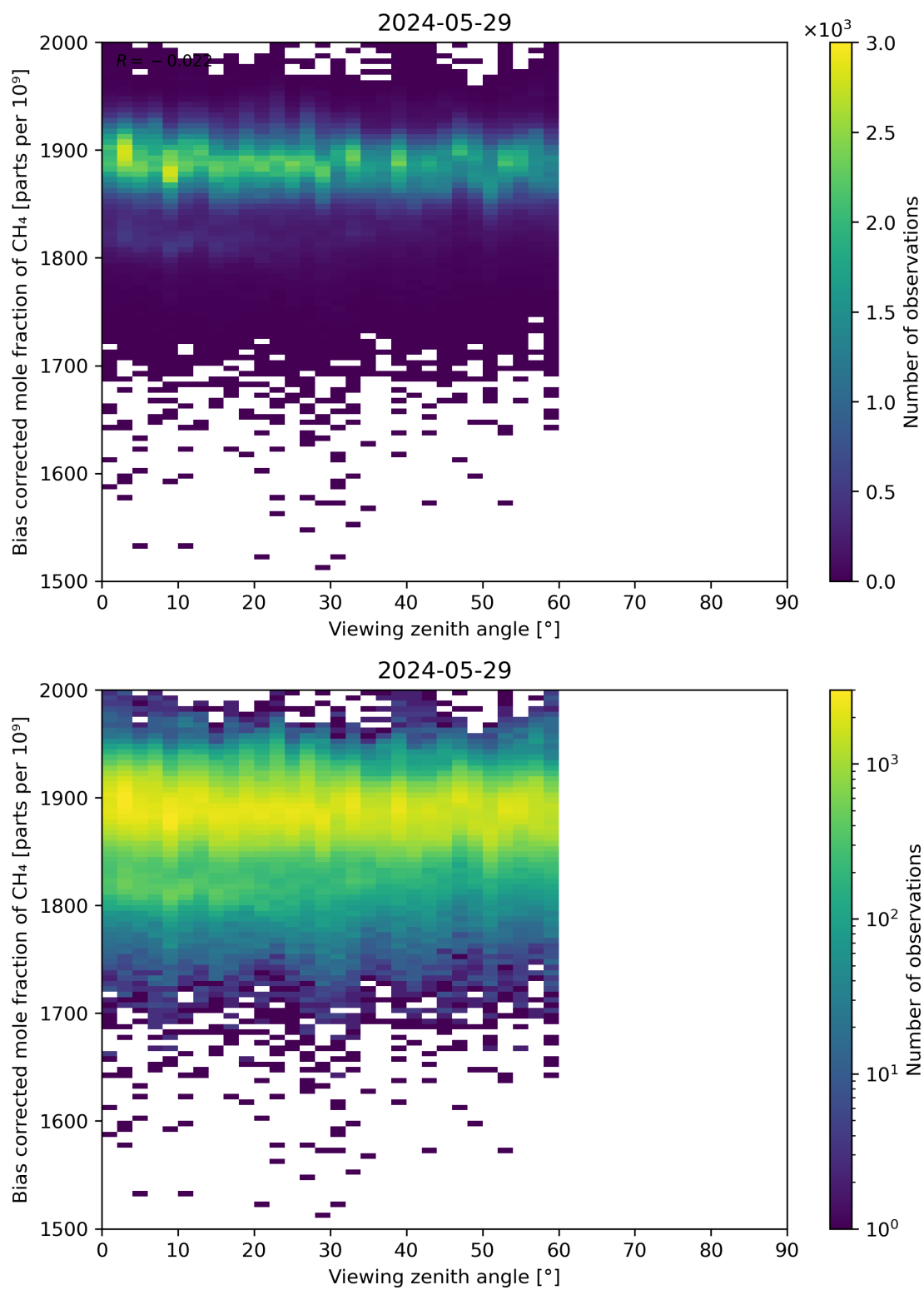
Figure 111: Scatter density plot of “Viewing zenith angle” against “Bias corrected mole fraction of CH 4 ” for 2024-05-28 to 2024-05-30.
