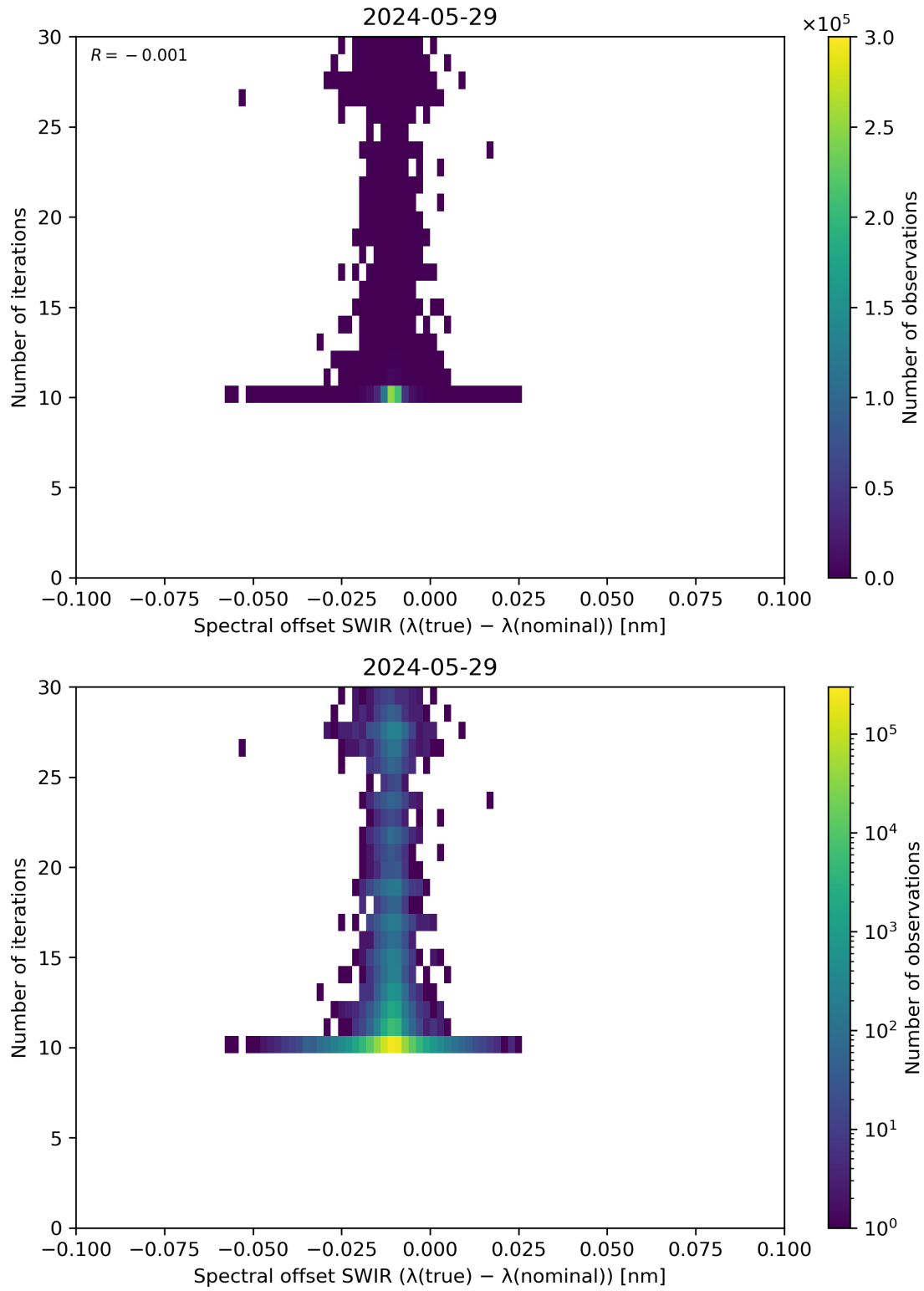
Figure 121: Scatter density plot of “Spectral offset SWIR ( \lambda(\text{true}) - \lambda(\text{nominal}) )” against “Number of iterations” for 2024-05-28 to 2024-05-30.
