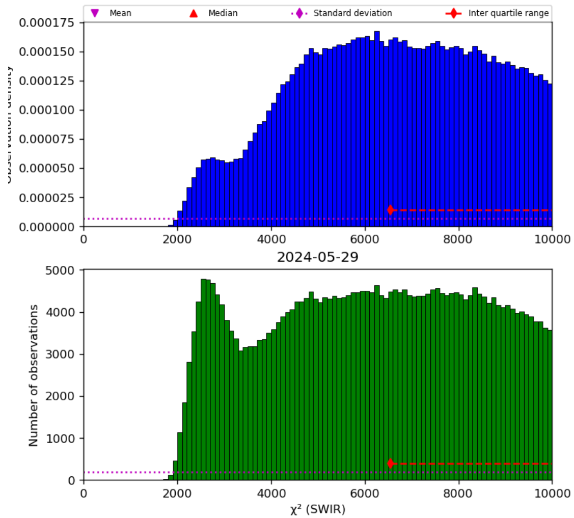
Figure 28: Histogram of “ \chi^2 (SWIR)” for 2024-05-28 to 2024-05-30
