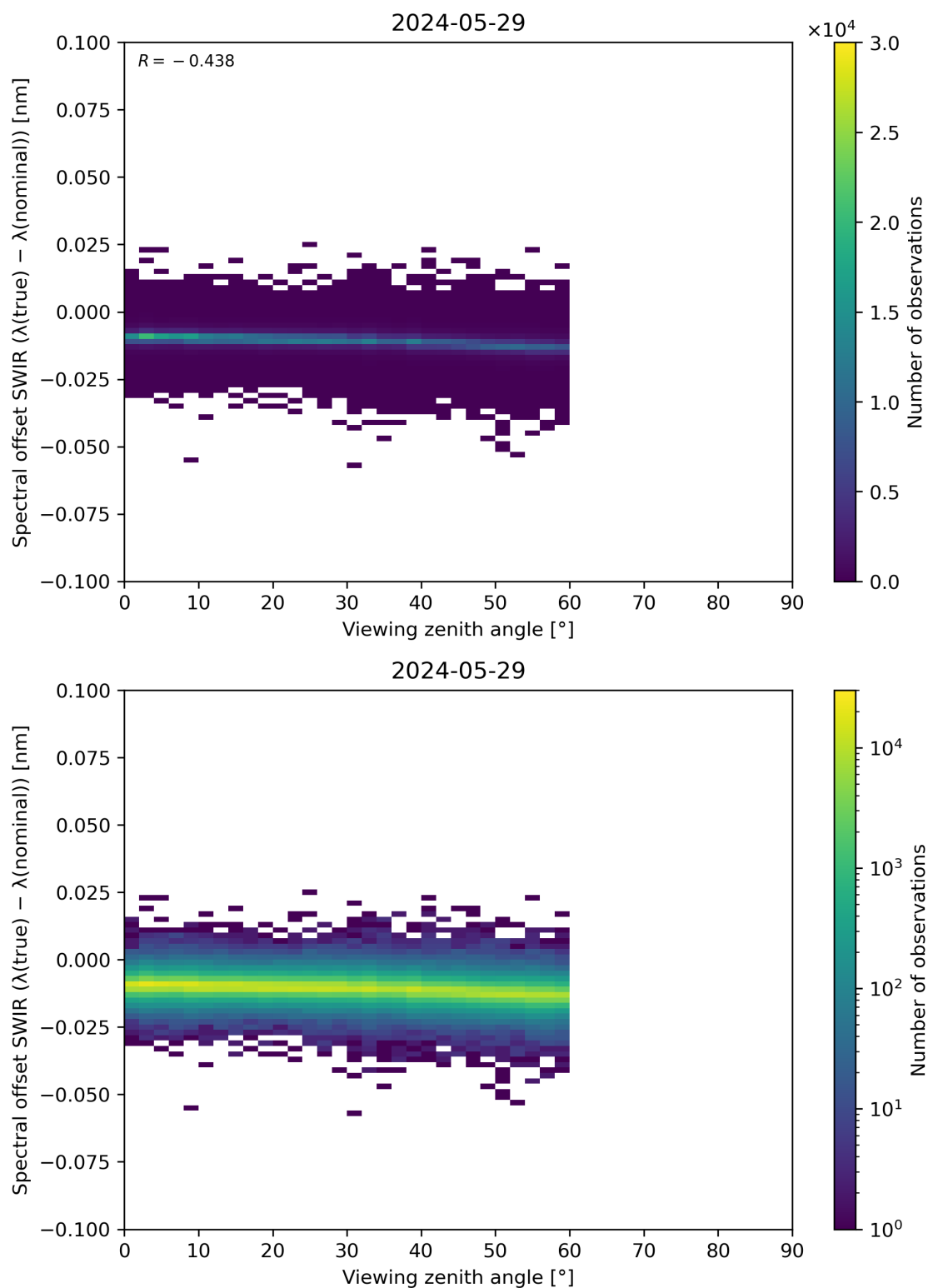
Figure 116: Scatter density plot of “Viewing zenith angle” against “Spectral offset SWIR ( \lambda(\text{true}) - \lambda(\text{nominal}) )” for 2024-05-28 to 2024-05-30.
