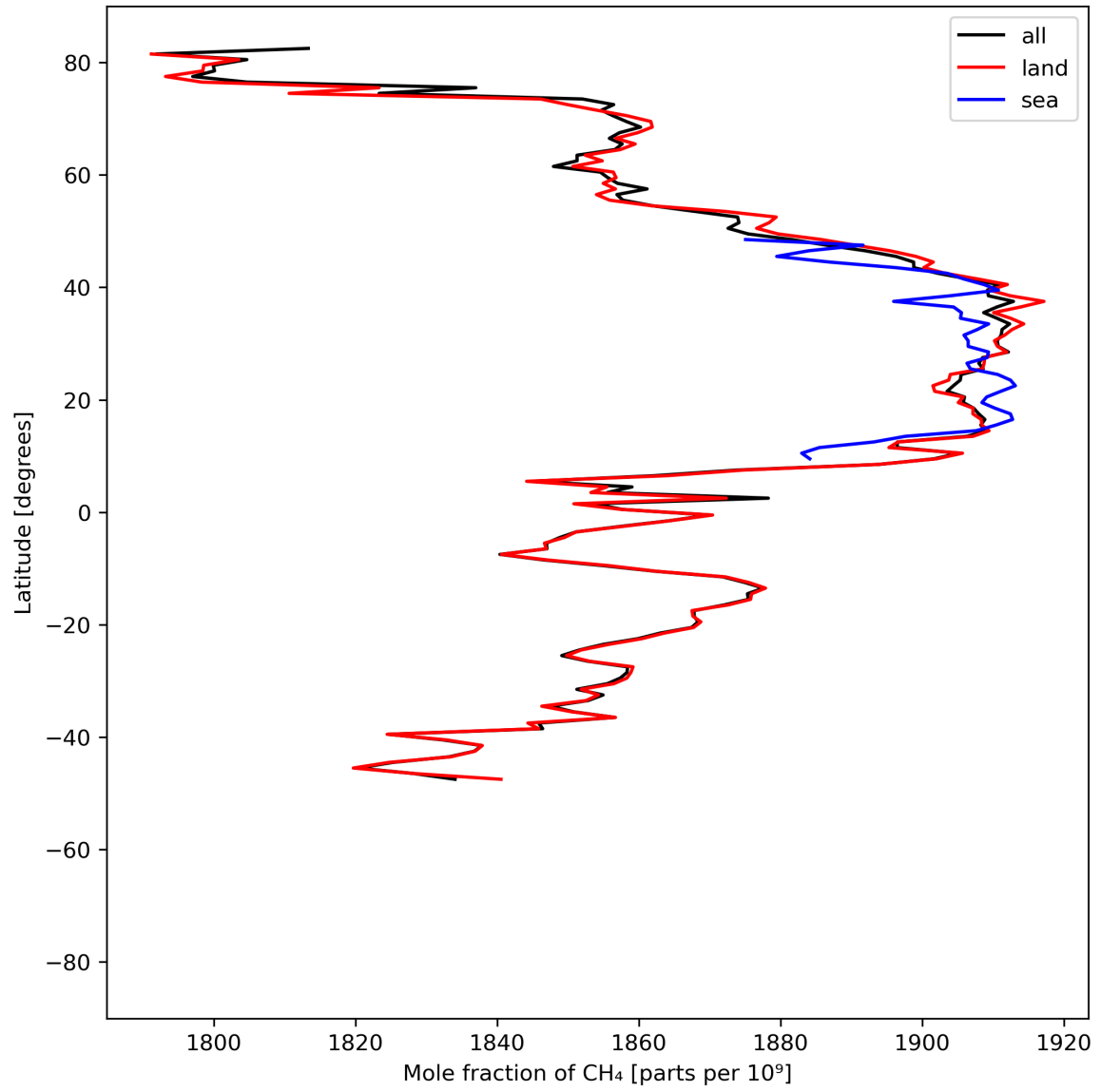
Figure 12: Zonal average of “Mole fraction of CH 4 ” for 2024-05-28 to 2024-05-30.
