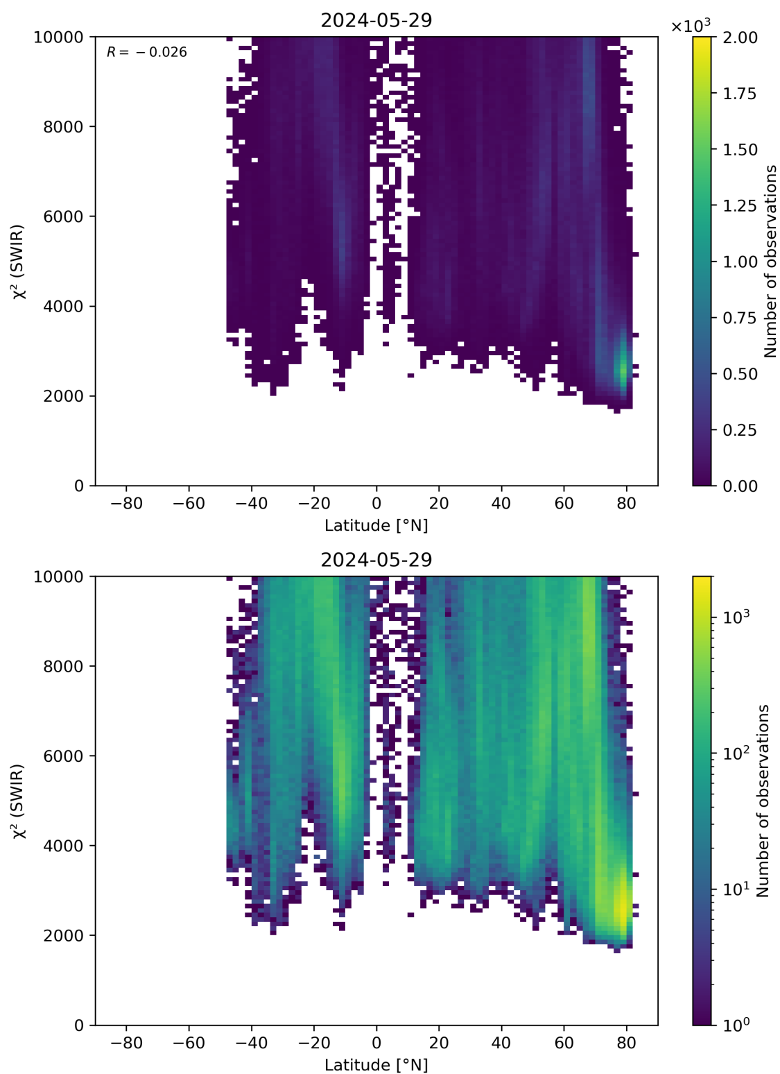
Figure 54: Scatter density plot of “Latitude” against “ \chi^2 (SWIR)” for 2024-05-28 to 2024-05-30.
