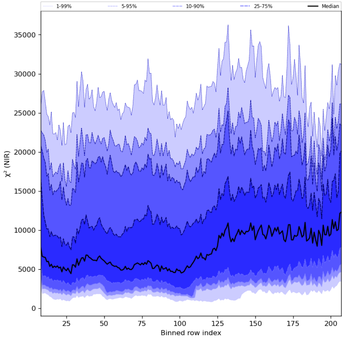
Figure 40: Along track statistics of “ \chi^2 (NIR)” for 2024-05-28 to 2024-05-30
