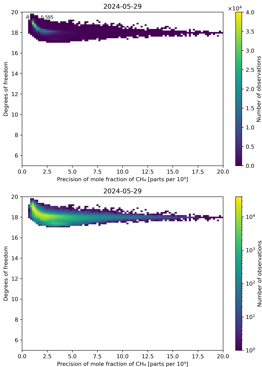
Figure 80: Scatter density plot of “Precision of mole fraction of CH 4 ” against “Degrees of freedom” for 2024-05-28 to 2024-05-30.
