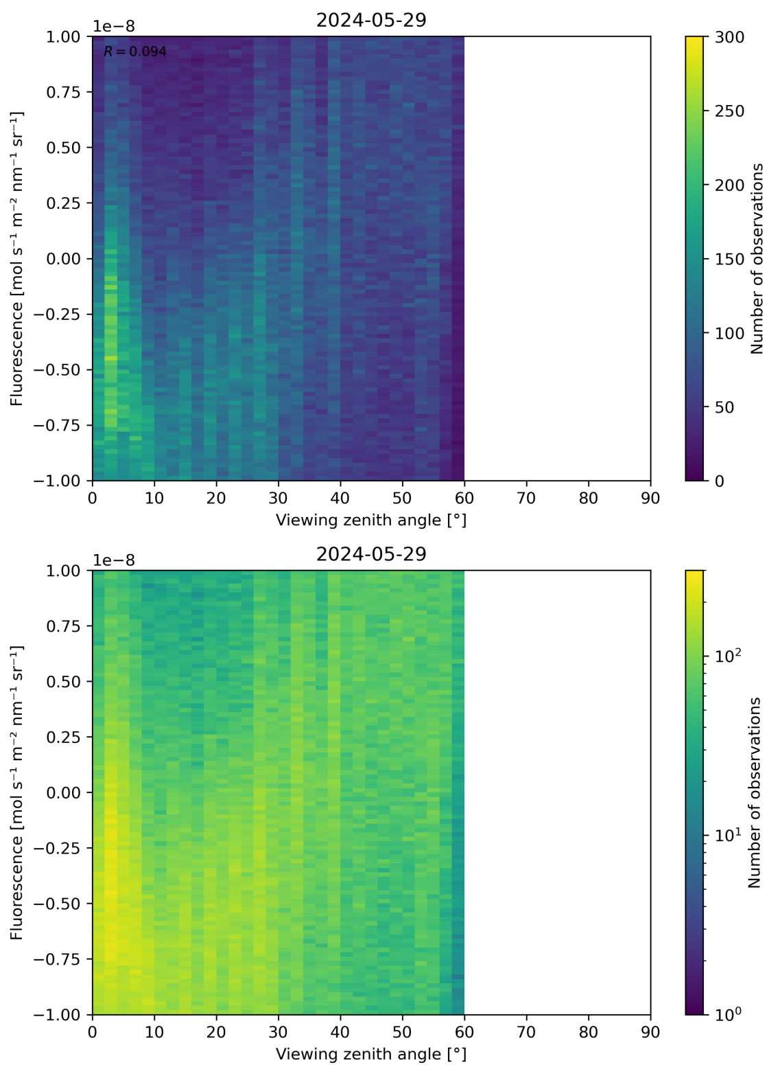
Figure 108: Scatter density plot of “Viewing zenith angle” against “Fluorescence” for 2024-05-28 to 2024-05-30.
