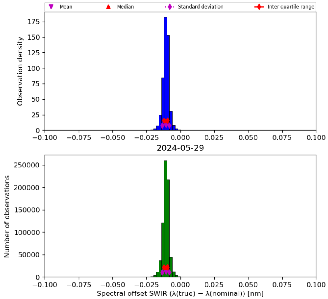
Figure 27: Histogram of “Spectral offset SWIR ( \lambda(\text{true}) - \lambda(\text{nominal}) )” for 2024-05-28 to 2024-05-30
