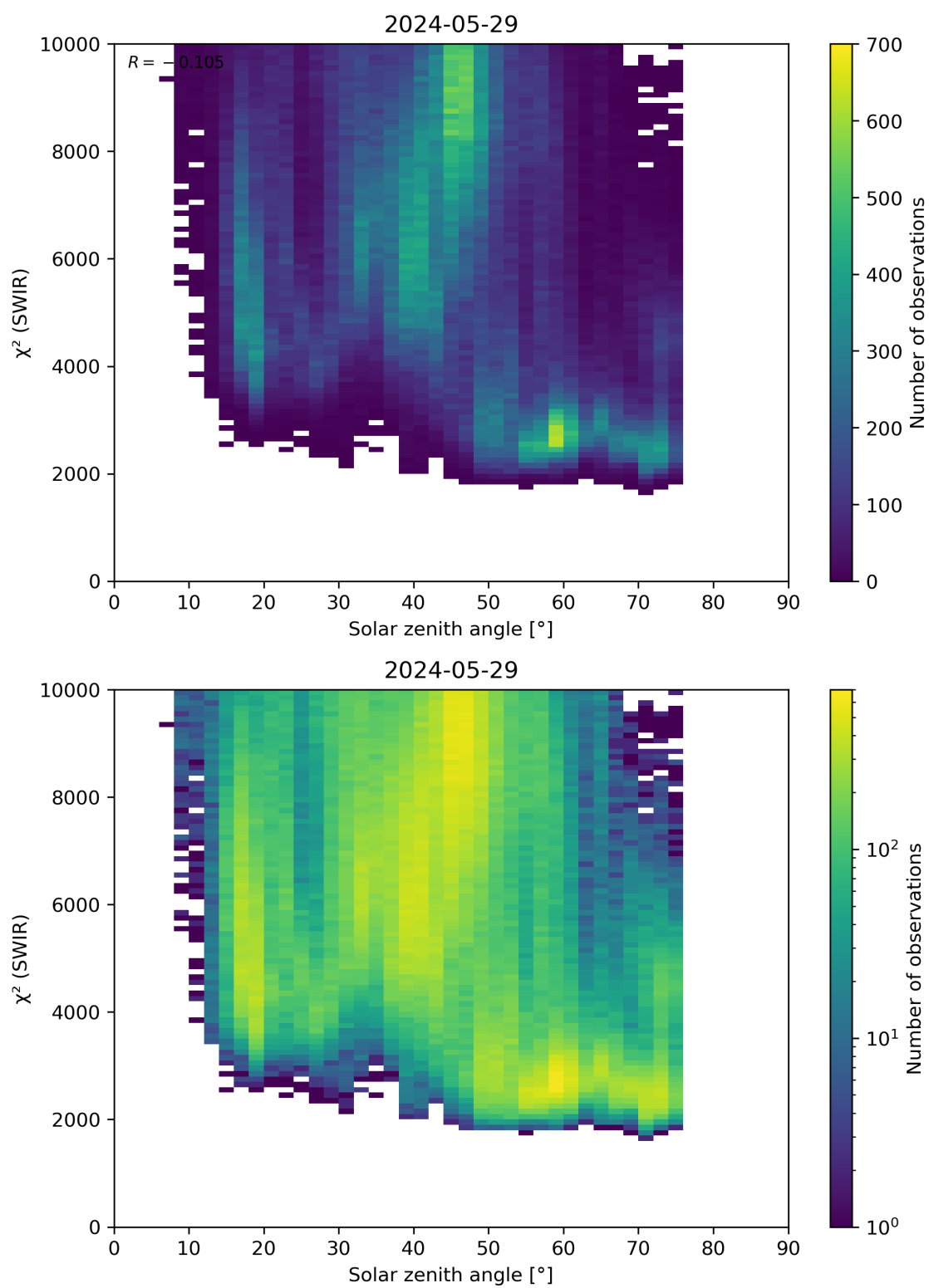
Figure 95: Scatter density plot of “Solar zenith angle” against “ \chi^2 (SWIR)” for 2024-05-28 to 2024-05-30.
