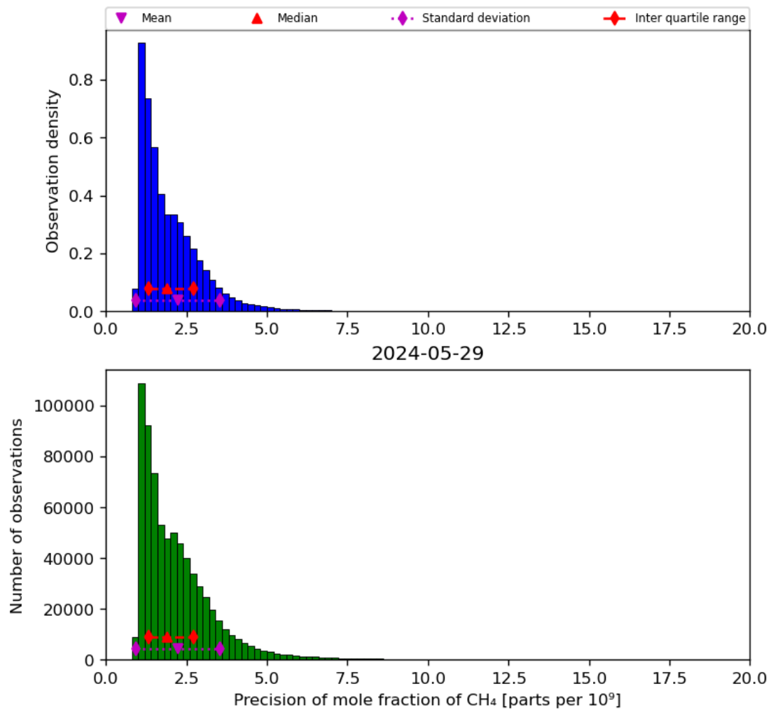
Figure 24: Histogram of “Precision of mole fraction of CH 4 ” for 2024-05-28 to 2024-05-30
