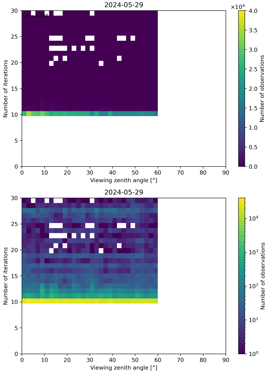
Figure 113: Scatter density plot of “Viewing zenith angle” against “Number of iterations” for 2024-05-28 to 2024-05-30.
