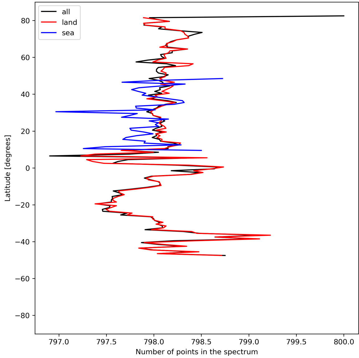
Figure 15: Zonal average of “Number of points in the spectrum” for 2024-05-28 to 2024-05-30.
