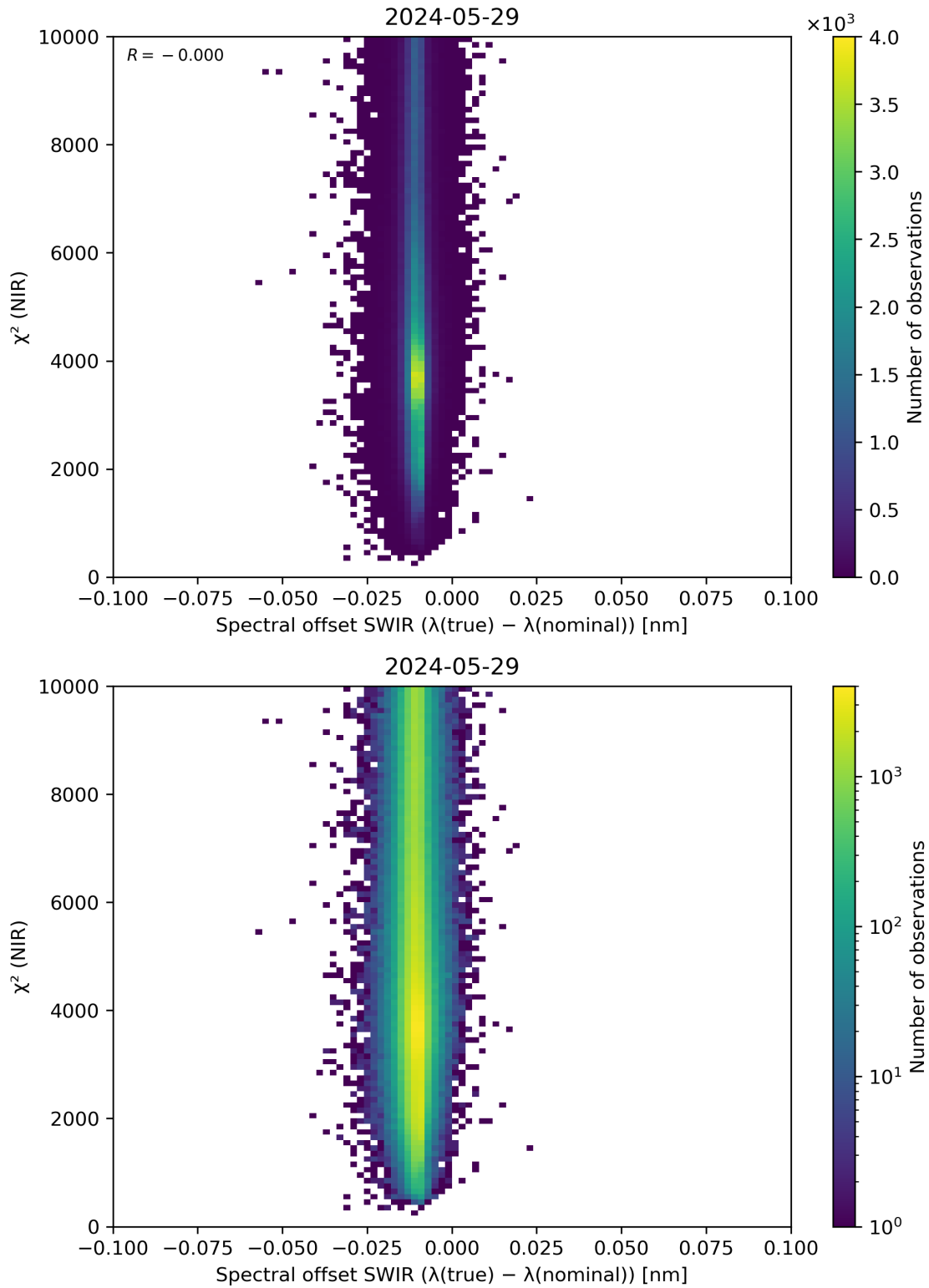
Figure 117: Scatter density plot of “Spectral offset SWIR ( \lambda(\text{true}) - \lambda(\text{nominal}) )” against “ \chi^2 (NIR)” for 2024-05-28 to 2024-05-30.
