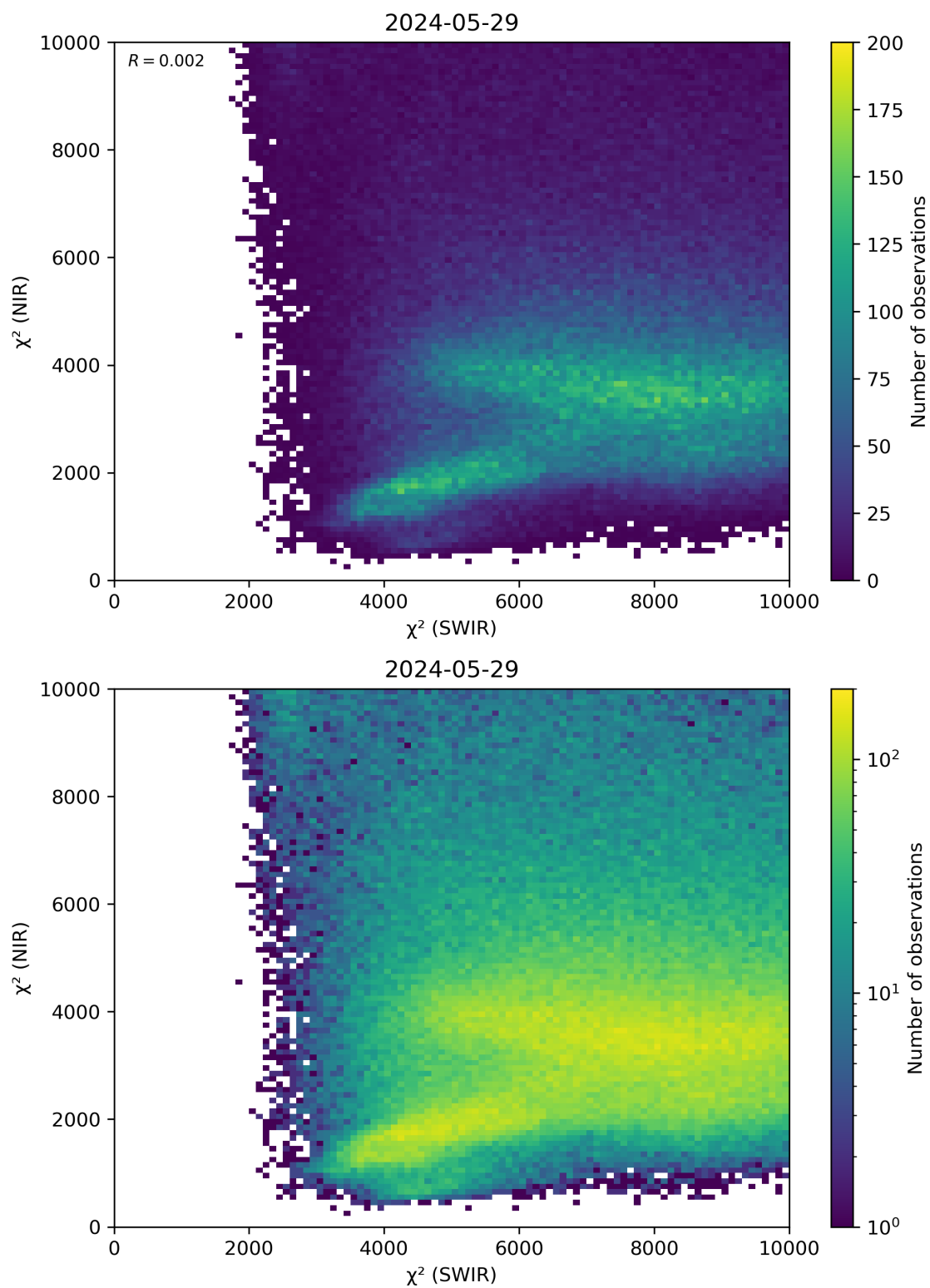
Figure 47: Scatter density plot of “ \chi^2 (SWIR)” against “ \chi^2 (NIR)” for 2024-05-28 to 2024-05-30.
