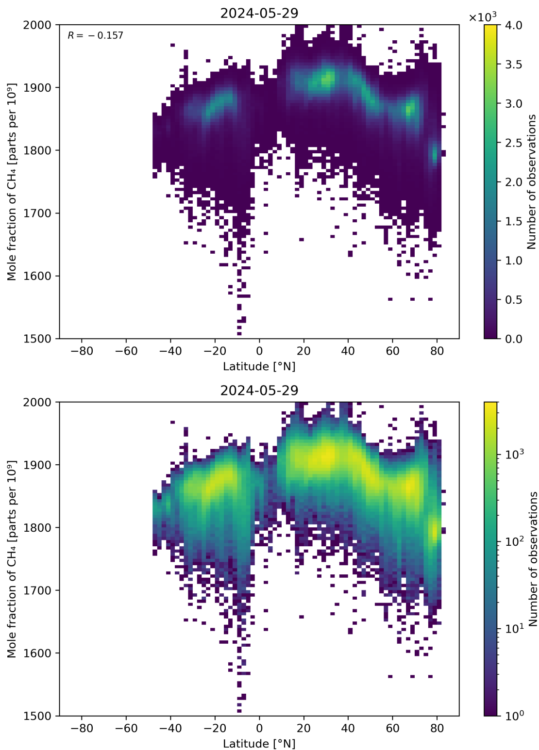
Figure 57: Scatter density plot of “Latitude” against “Mole fraction of CH 4 ” for 2024-05-28 to 2024-05-30.
