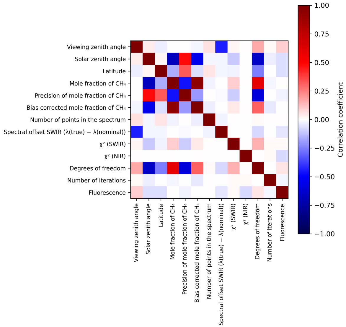
Figure 2: Map of correlation matrix for 2024-05-28 to 2024-05-30.
