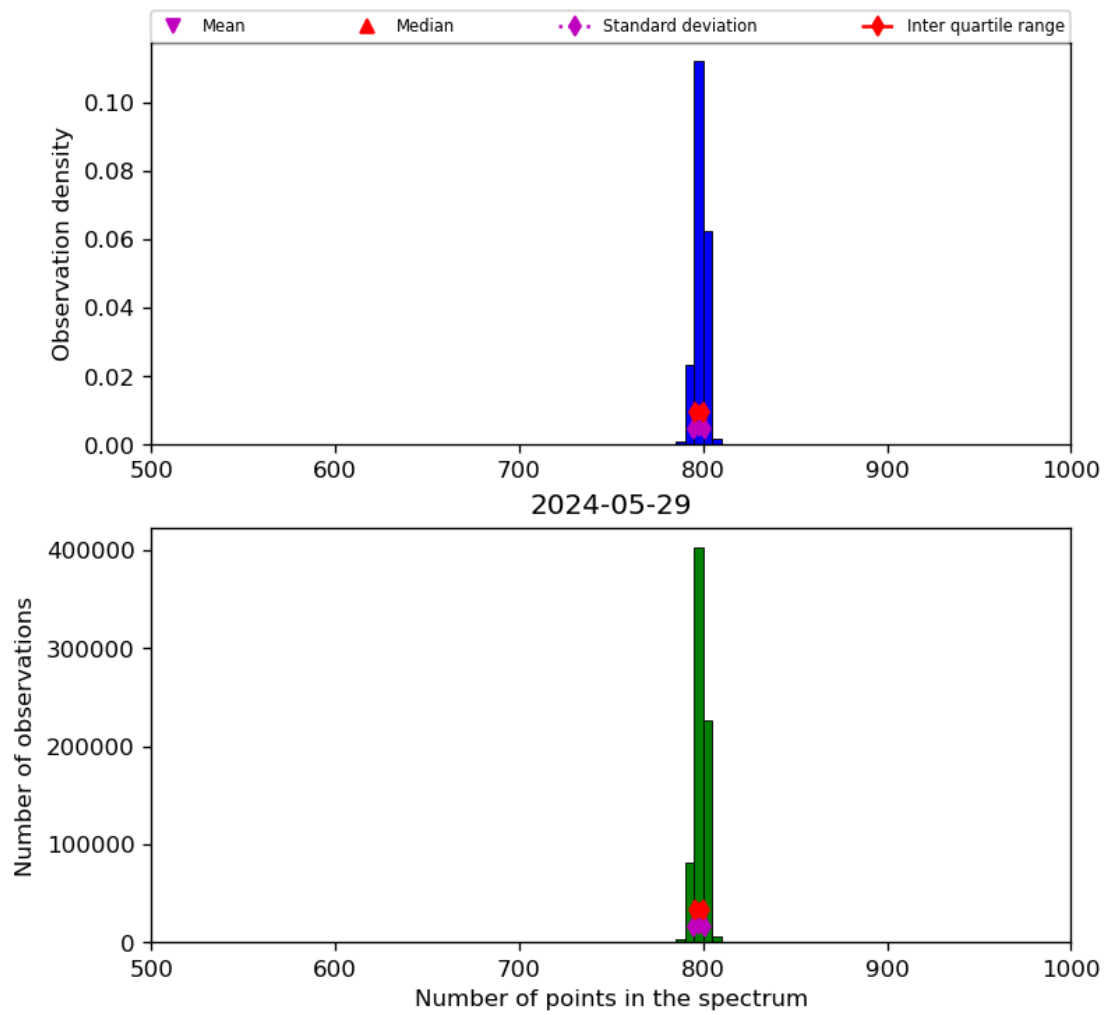
Figure 26: Histogram of “Number of points in the spectrum” for 2024-05-28 to 2024-05-30
