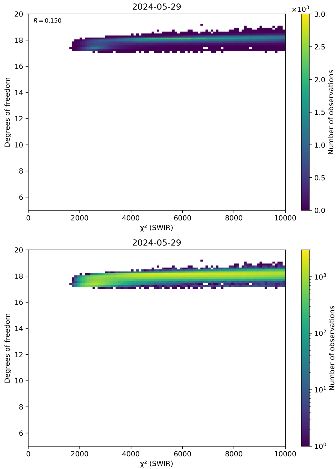
Figure 48: Scatter density plot of “ \chi^2 (SWIR)” against “Degrees of freedom” for 2024-05-28 to 2024-05-30.
