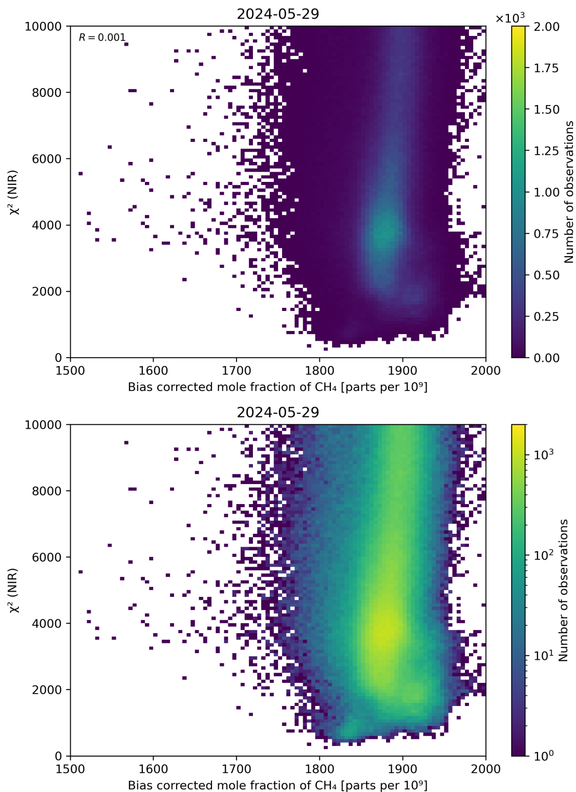
Figure 63: Scatter density plot of “Bias corrected mole fraction of CH 4 ” against “ \chi^2 (NIR)” for 2024-05-28 to 2024-05-30.
