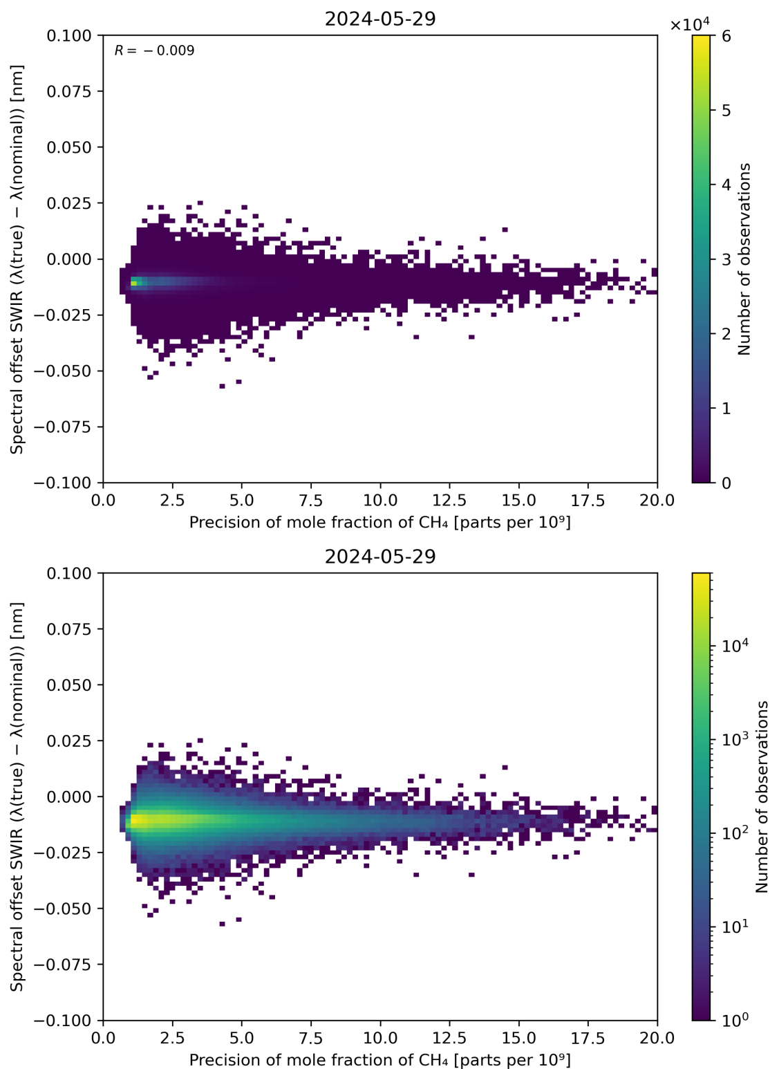
Figure 85: Scatter density plot of “Precision of mole fraction of CH 4 ” against “Spectral offset SWIR ( \lambda(\text{true}) - \lambda(\text{nominal}) )” for 2024-05-28 to 2024-05-30.
