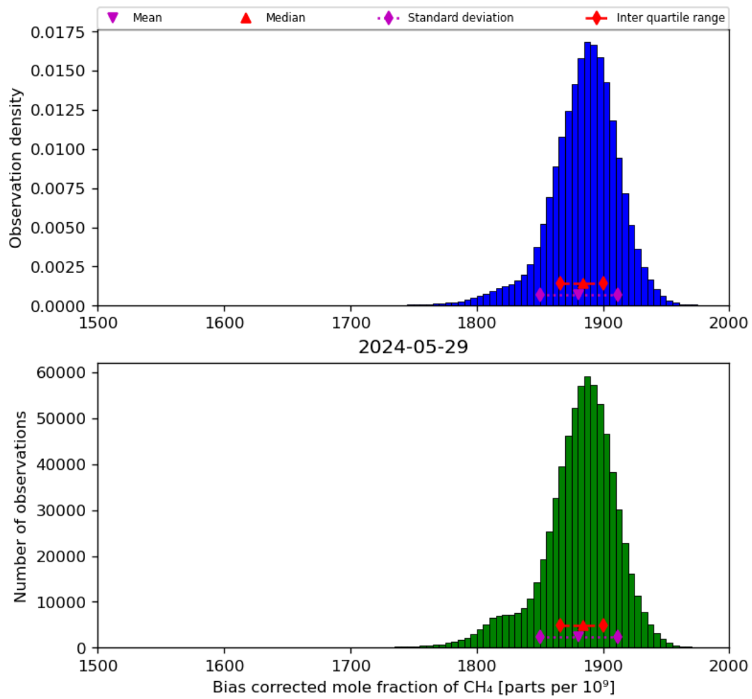
Figure 25: Histogram of “Bias corrected mole fraction of CH 4 ” for 2024-05-28 to 2024-05-30
