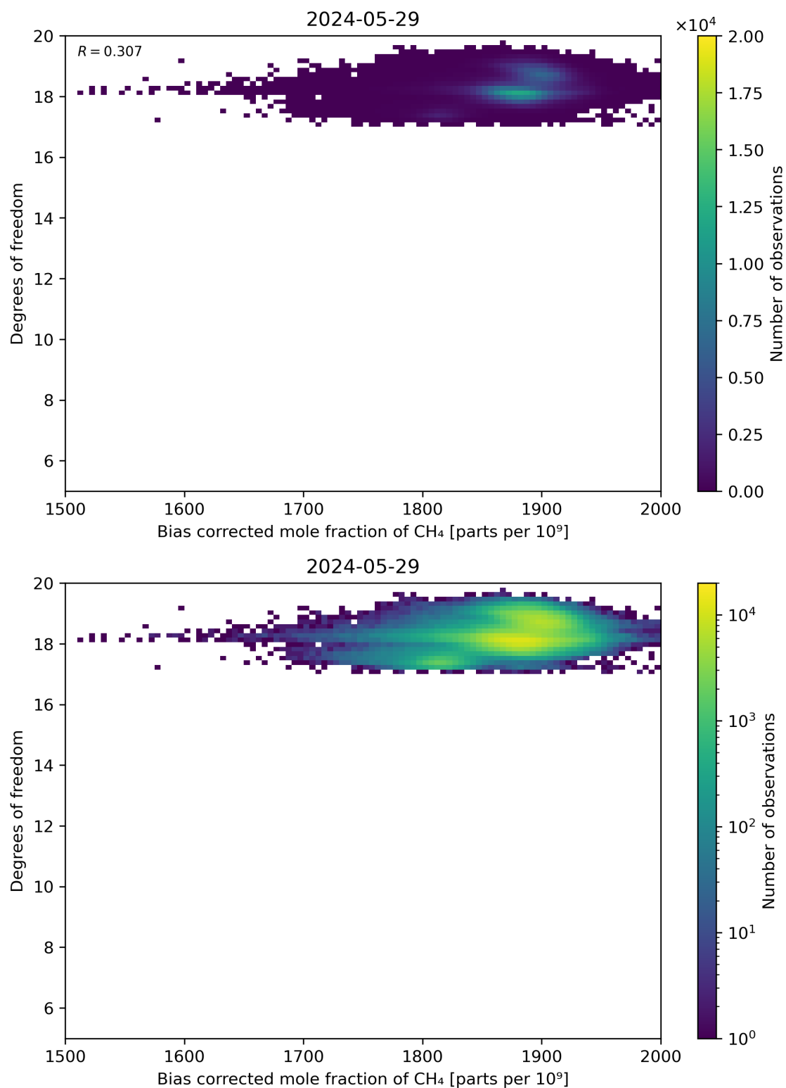
Figure 65: Scatter density plot of “Bias corrected mole fraction of CH 4 ” against “Degrees of freedom” for 2024-05-28 to 2024-05-30.
