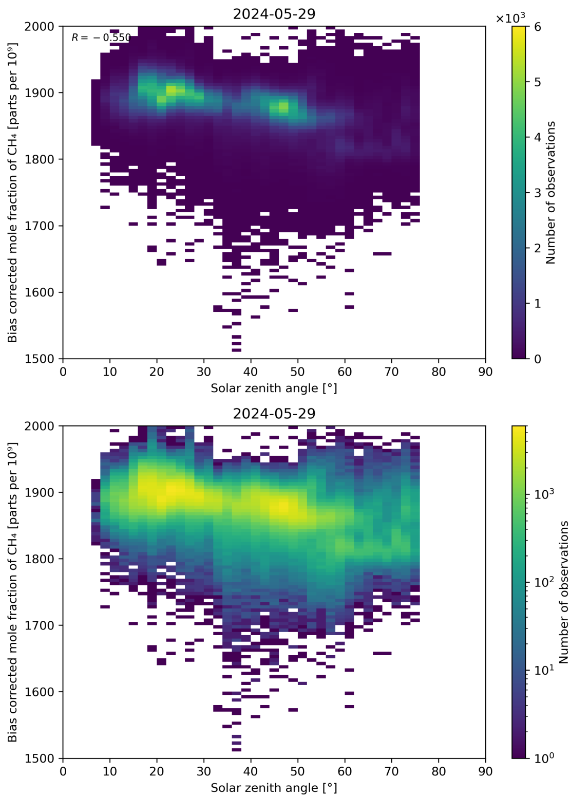
Figure 100: Scatter density plot of “Solar zenith angle” against “Bias corrected mole fraction of CH 4 ” for 2024-05-28 to 2024-05-30.
