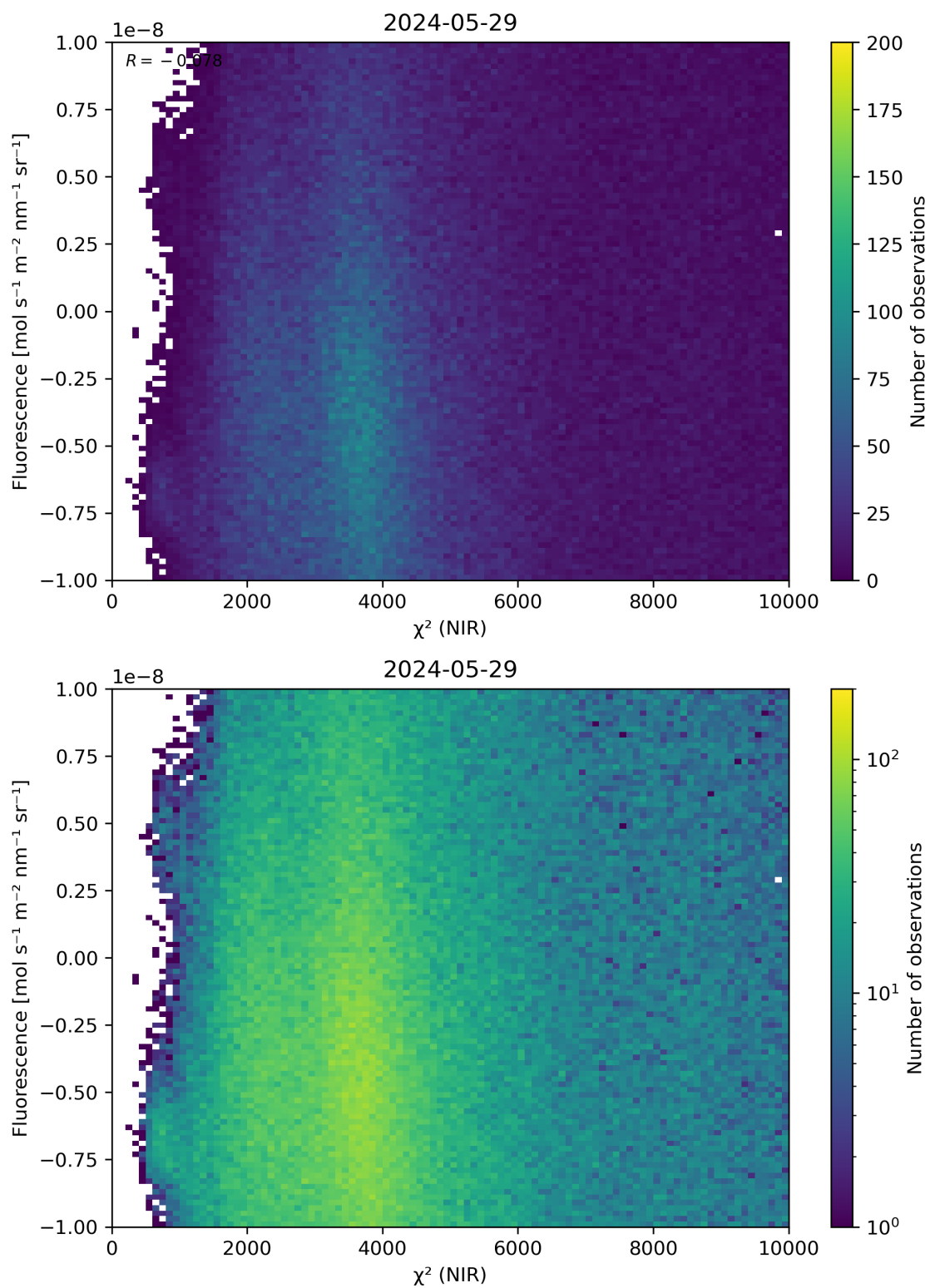
Figure 45: Scatter density plot of “ \chi^2 (NIR)” against “Fluorescence” for 2024-05-28 to 2024-05-30.
