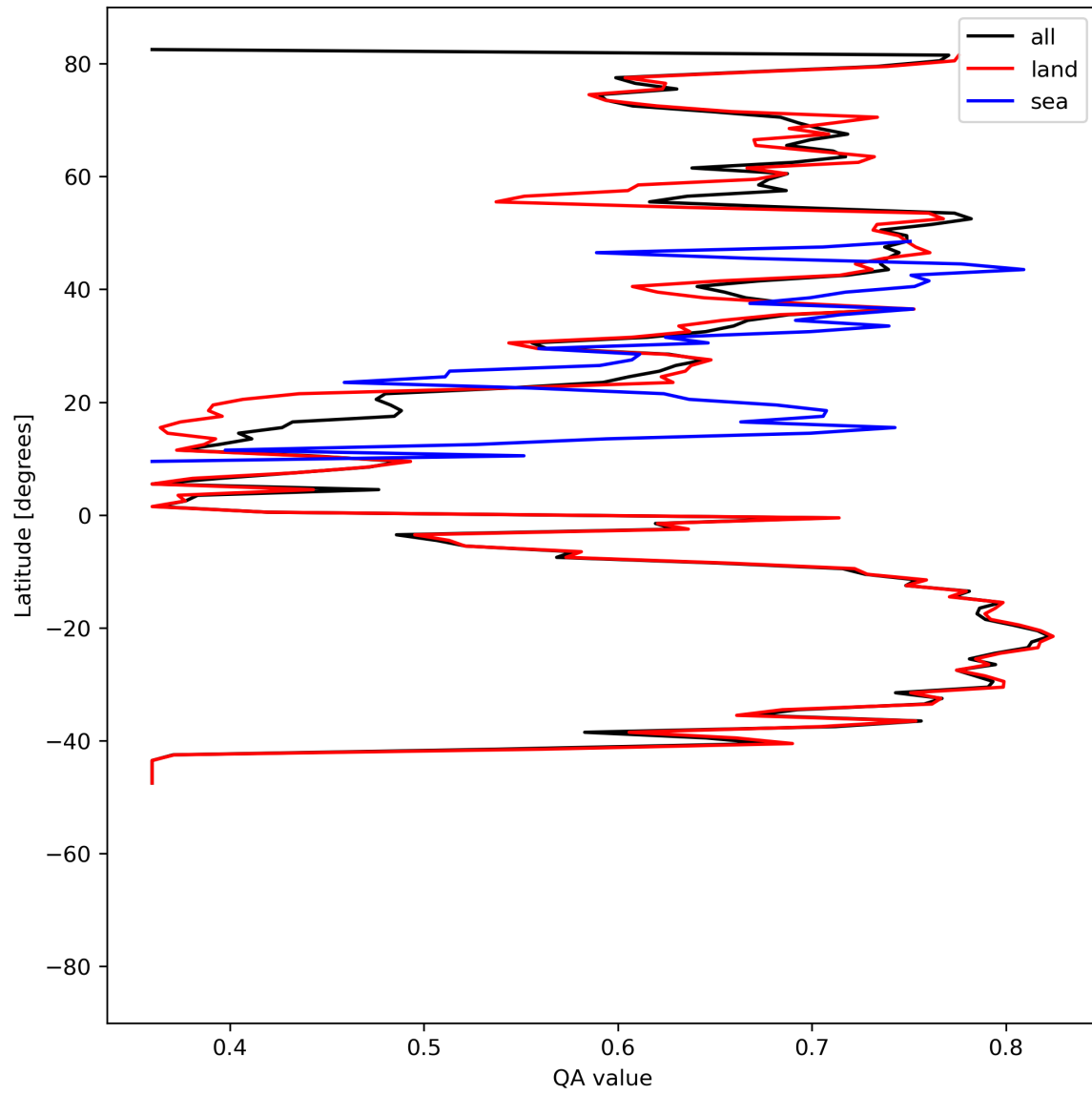
Figure 11: Zonal average of “QA value” for 2024-05-28 to 2024-05-30.
