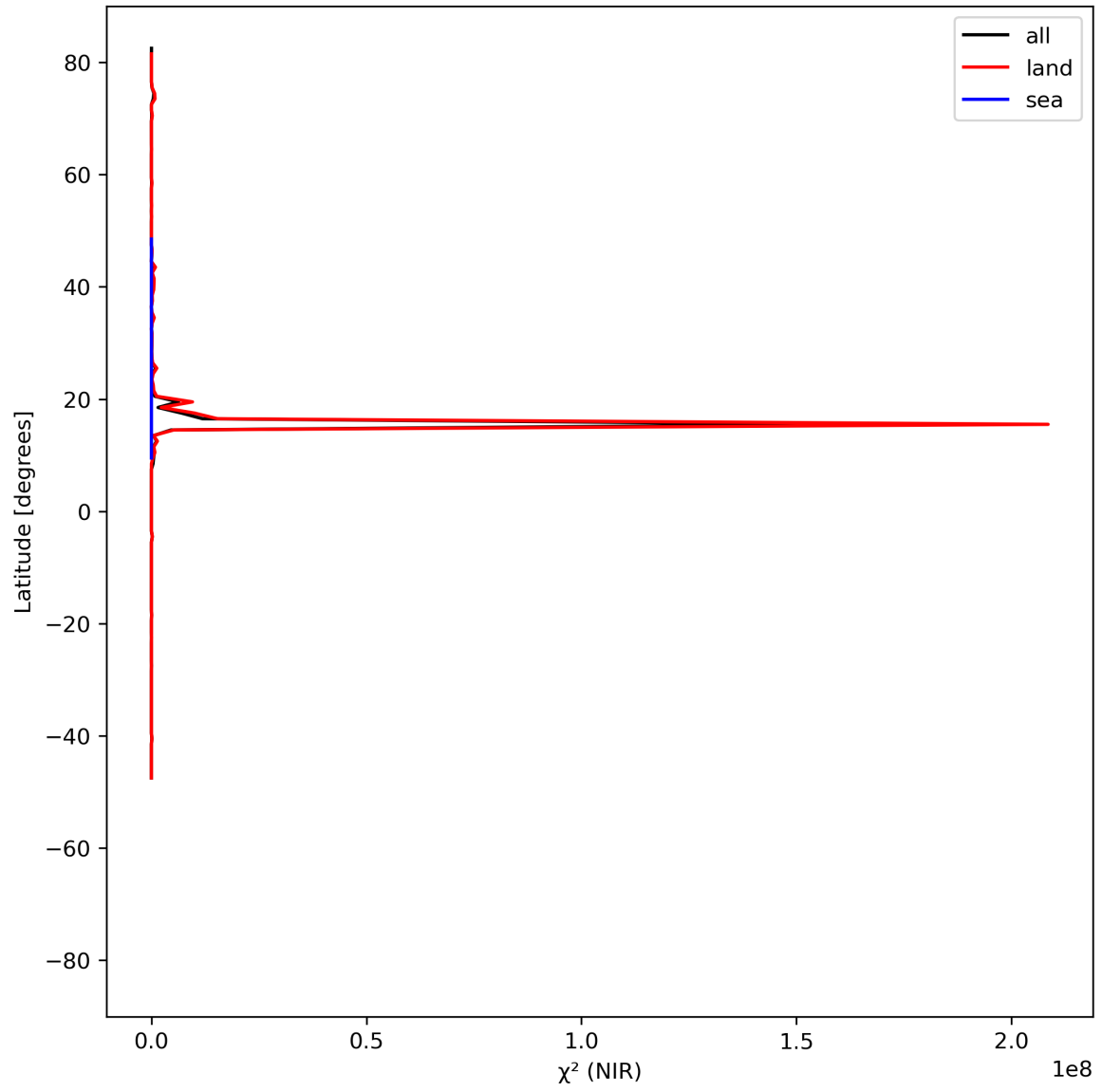
Figure 18: Zonal average of “ \chi^2 (NIR)” for 2024-05-28 to 2024-05-30.
