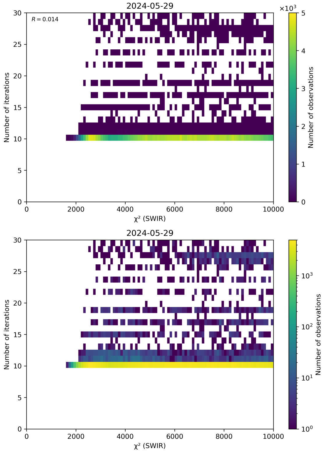
Figure 50: Scatter density plot of “ \chi^2 (SWIR)” against “Number of iterations” for 2024-05-28 to 2024-05-30.
