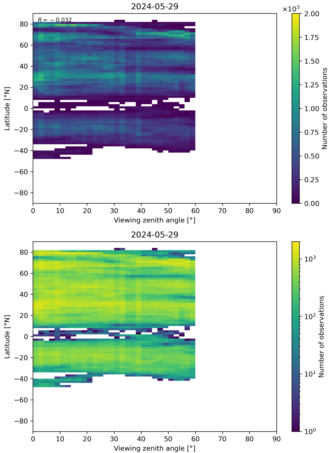
Figure 109: Scatter density plot of “Viewing zenith angle” against “Latitude” for 2024-05-28 to 2024-05-30.
