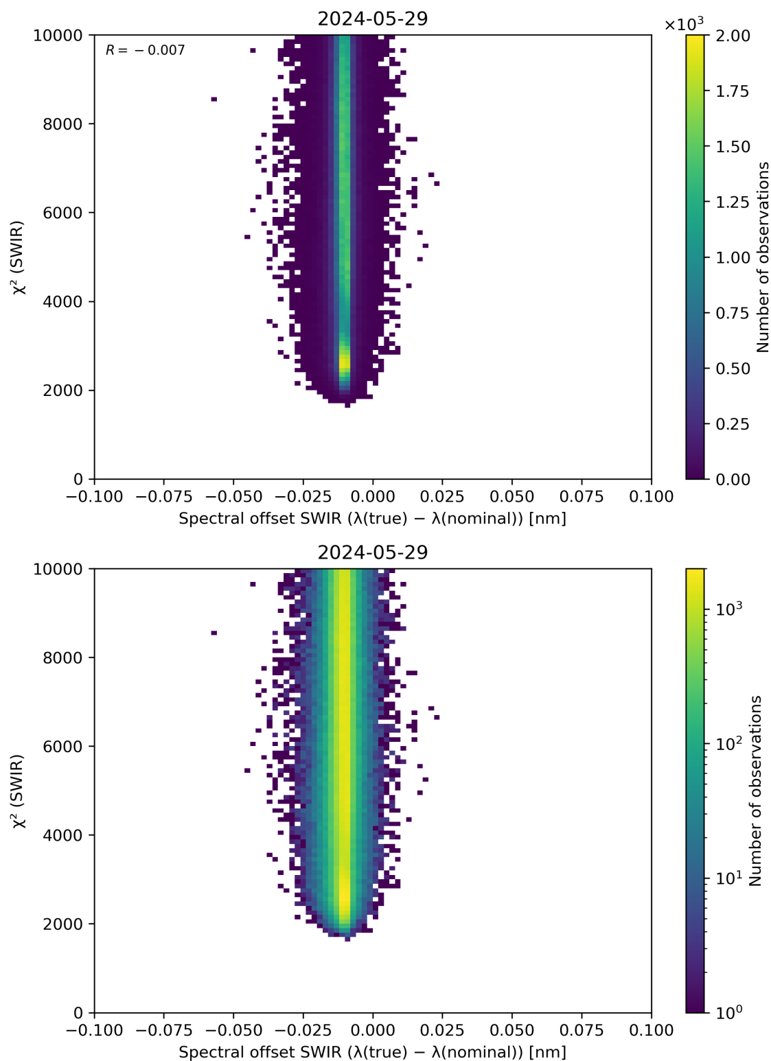
Figure 118: Scatter density plot of “Spectral offset SWIR ( \lambda(\text{true}) - \lambda(\text{nominal}) )” against “ \chi^2 (SWIR)” for 2024-05-28 to 2024-05-30.
