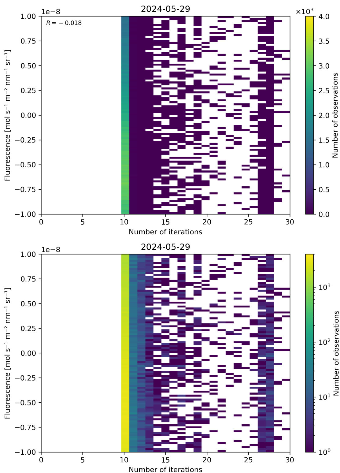
Figure 87: Scatter density plot of “Number of iterations” against “Fluorescence” for 2024-05-28 to 2024-05-30.
