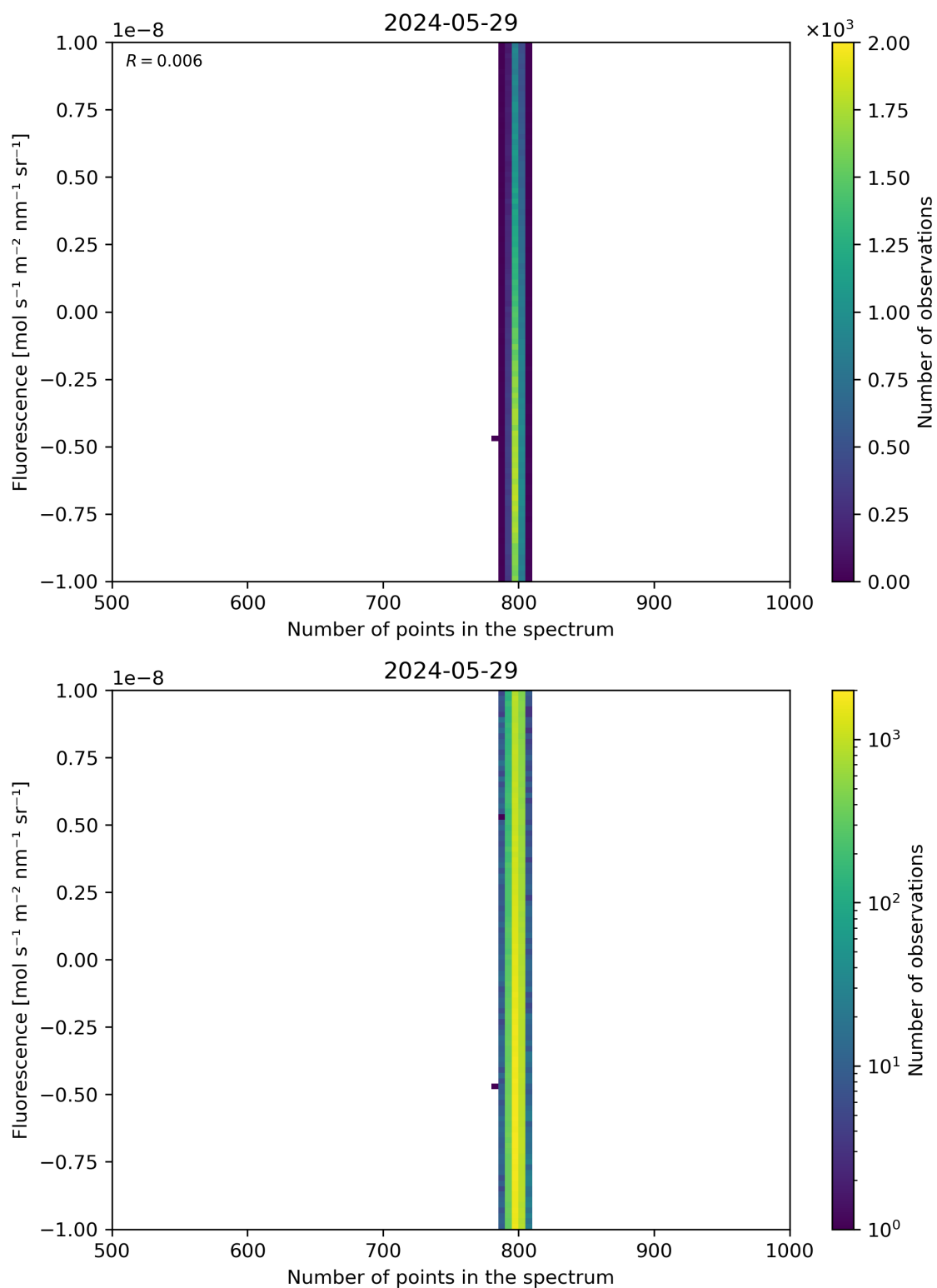
Figure 91: Scatter density plot of “Number of points in the spectrum” against “Fluorescence” for 2024-05-28 to 2024-05-30.
