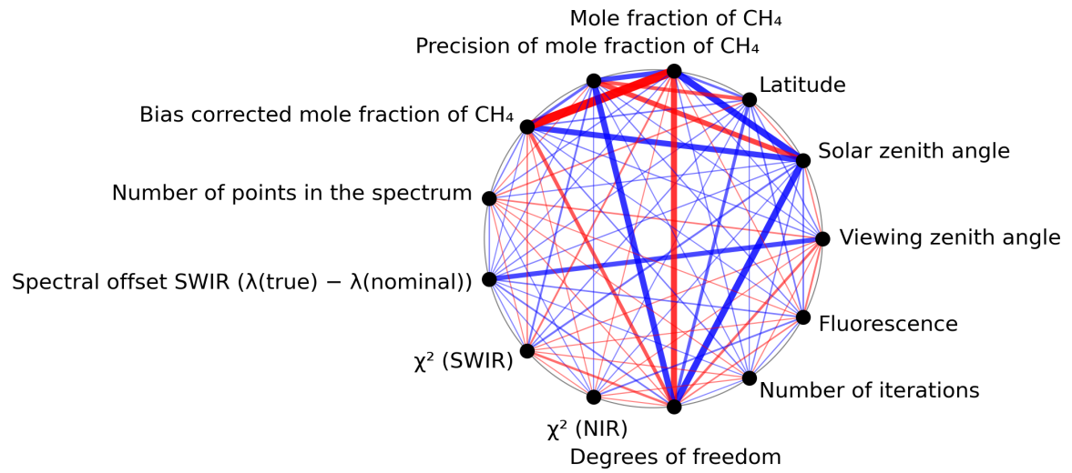
Figure 1: Map of correlation graph for 2024-05-28 to 2024-05-30.
