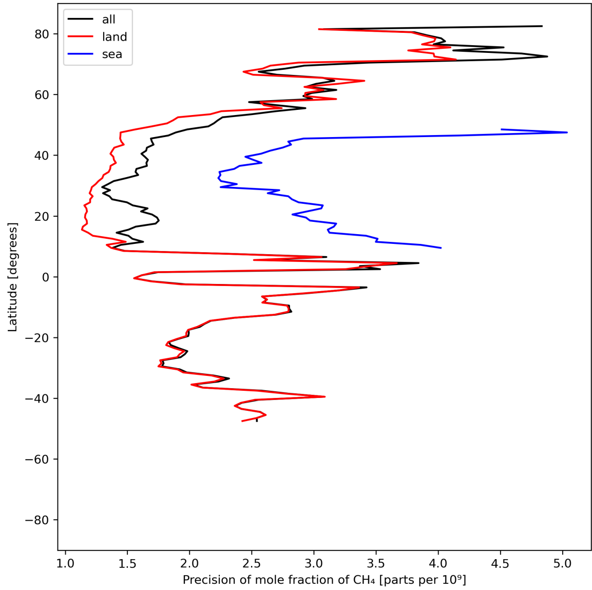
Figure 13: Zonal average of “Precision of mole fraction of CH 4 ” for 2024-05-28 to 2024-05-30.
