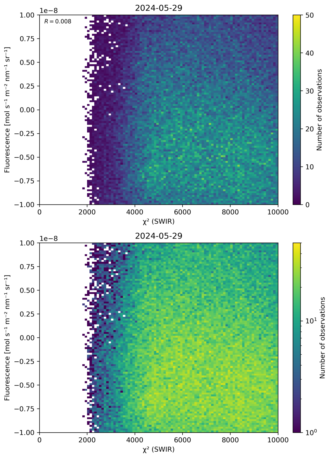
Figure 49: Scatter density plot of “ \chi^2 (SWIR)” against “Fluorescence” for 2024-05-28 to 2024-05-30.
