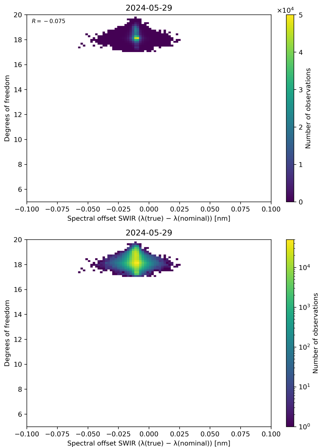
Figure 119: Scatter density plot of “Spectral offset SWIR ( \lambda(\text{true}) - \lambda(\text{nominal}) )” against “Degrees of freedom” for 2024-05-28 to 2024-05-30.
