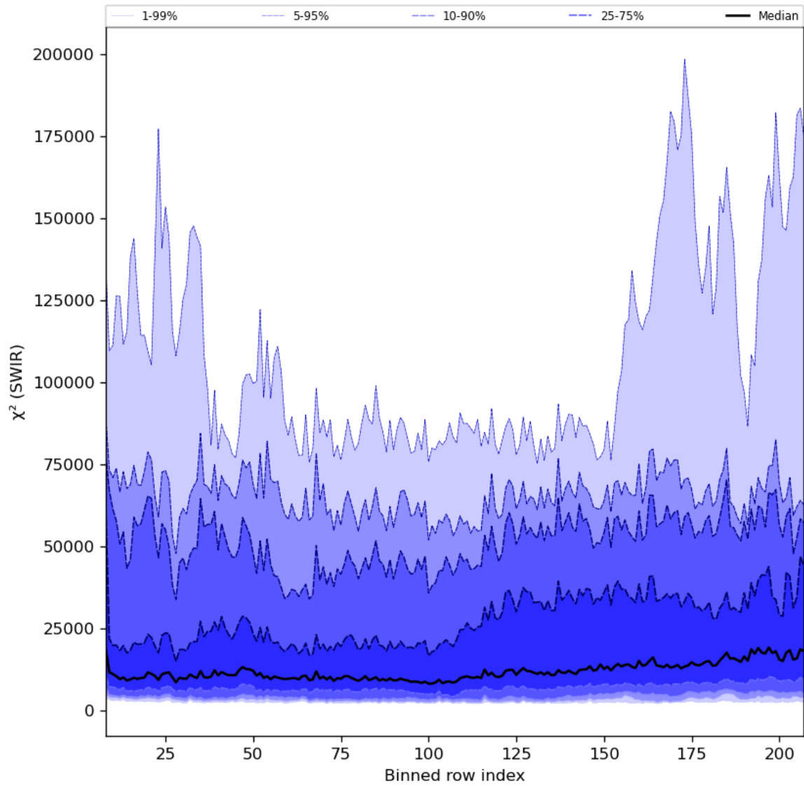
Figure 39: Along track statistics of " \chi^2 (SWIR)" for 2024-05-28 to 2024-05-30
