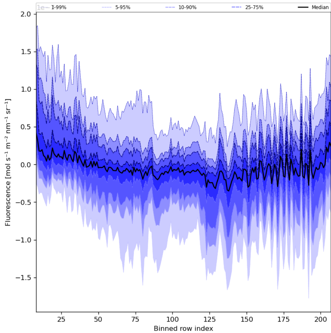
Figure 43: Along track statistics of “Fluorescence” for 2024-05-28 to 2024-05-30
