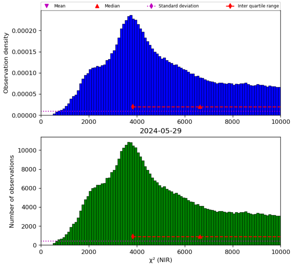
Figure 29: Histogram of “ \chi^2 (NIR)” for 2024-05-28 to 2024-05-30
