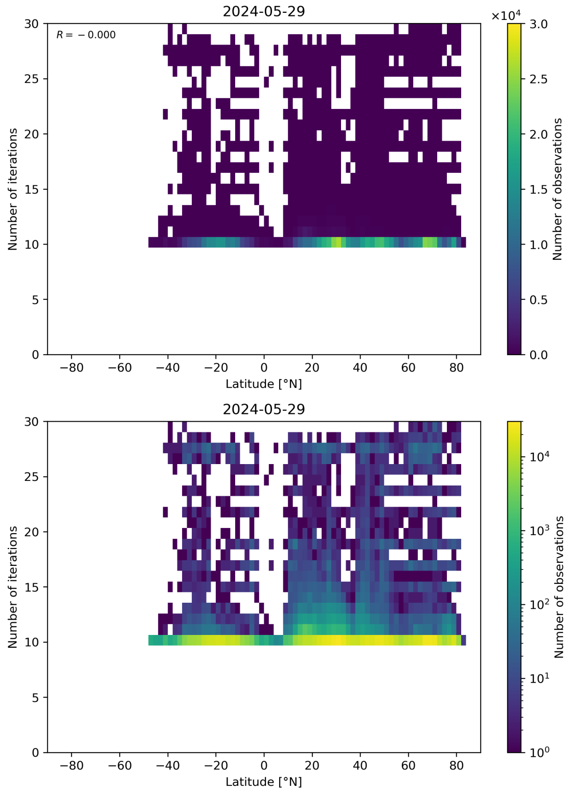
Figure 60: Scatter density plot of “Latitude” against “Number of iterations” for 2024-05-28 to 2024-05-30.
