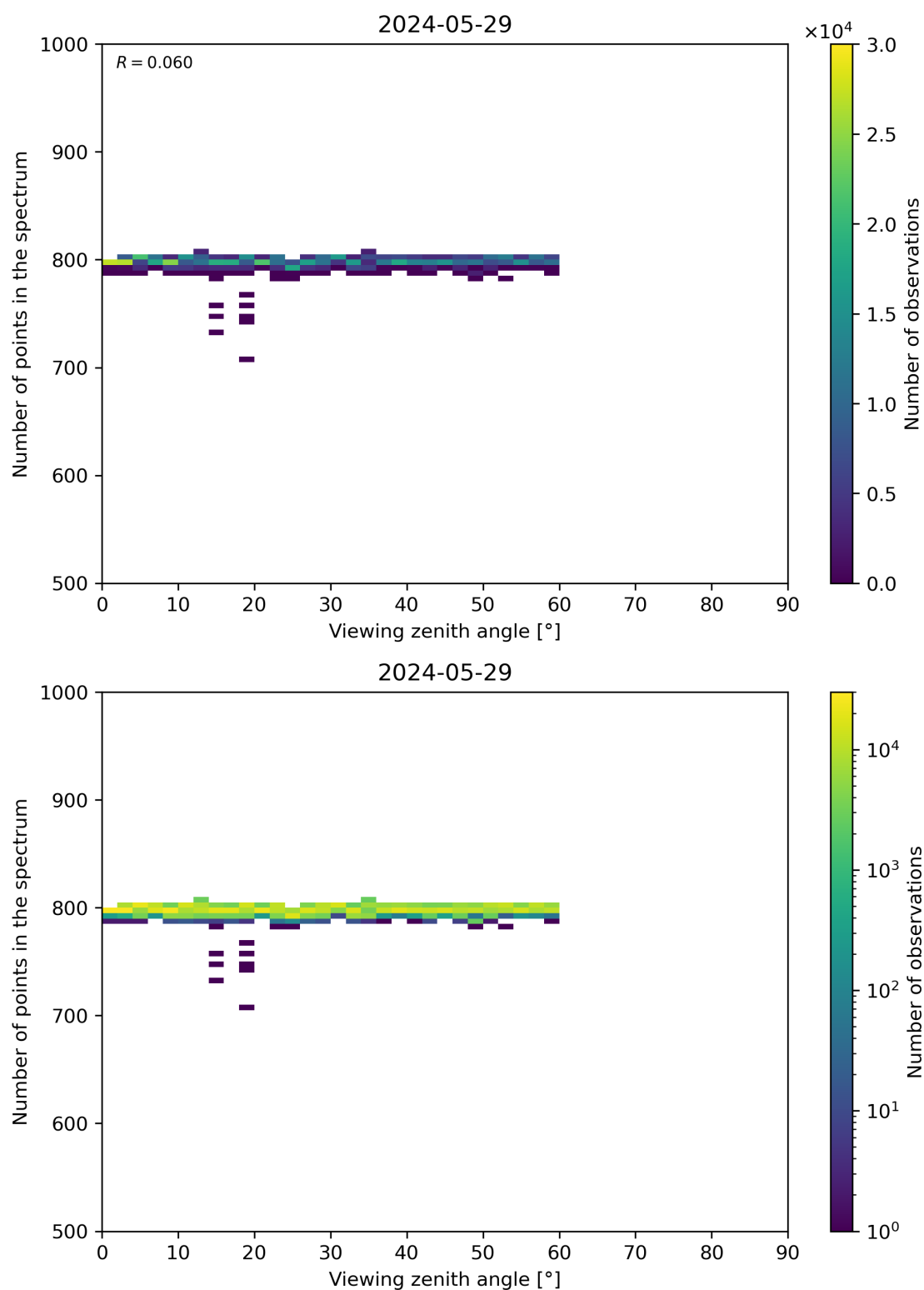
Figure 114: Scatter density plot of “Viewing zenith angle” against “Number of points in the spectrum” for 2024-05-28 to 2024-05-30.
