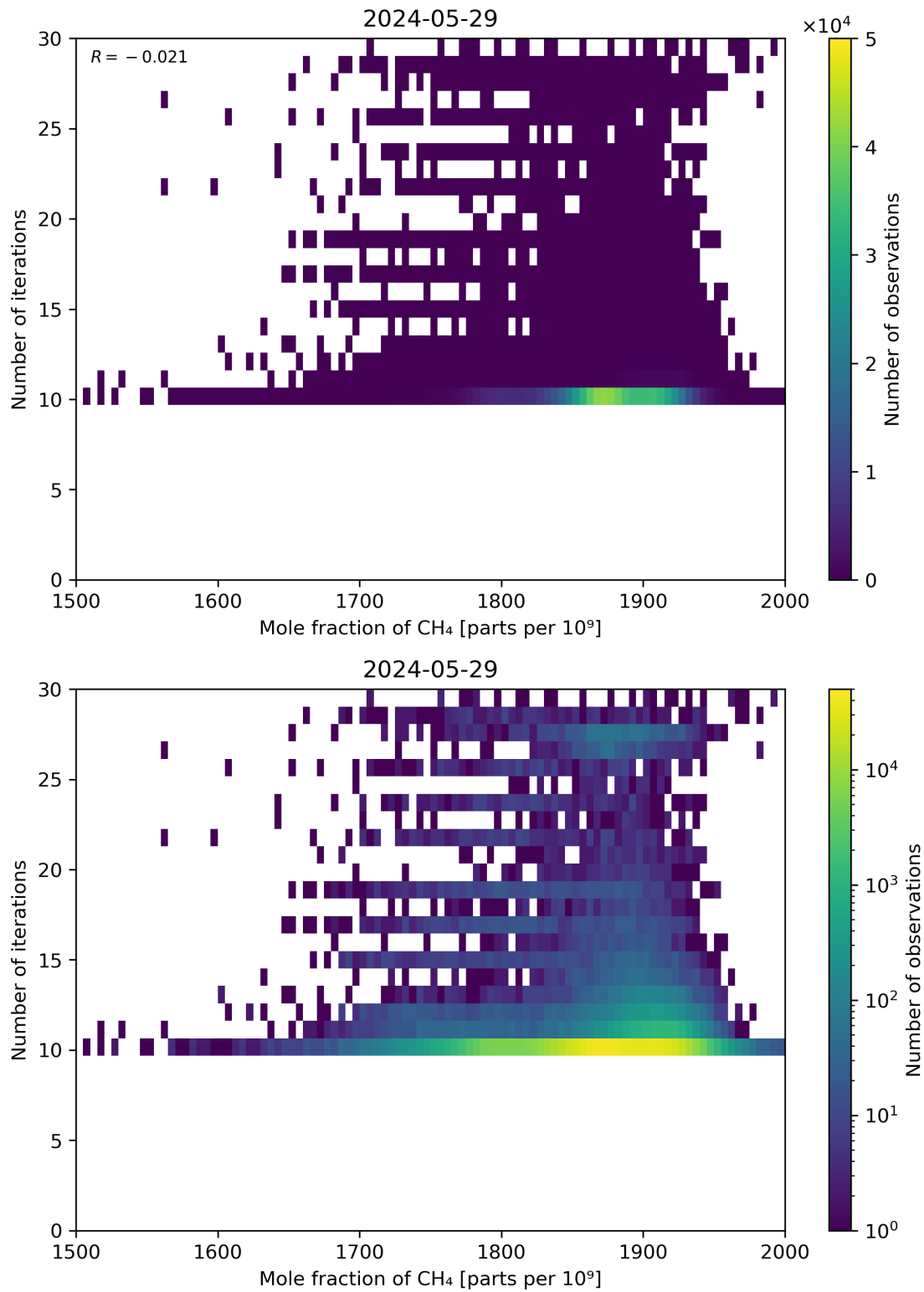
Figure 76: Scatter density plot of “Mole fraction of CH 4 ” against “Number of iterations” for 2024-05-28 to 2024-05-30.
