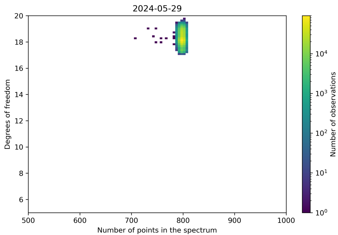
Figure 90: Scatter density plot of “Number of points in the spectrum” against “Degrees of freedom” for 2024-05-28 to 2024-05-30.
