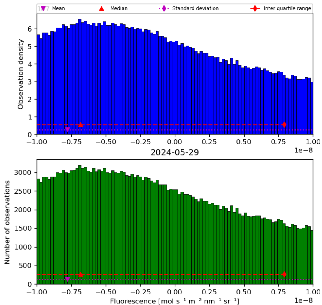
Figure 32: Histogram of “Fluorescence” for 2024-05-28 to 2024-05-30
