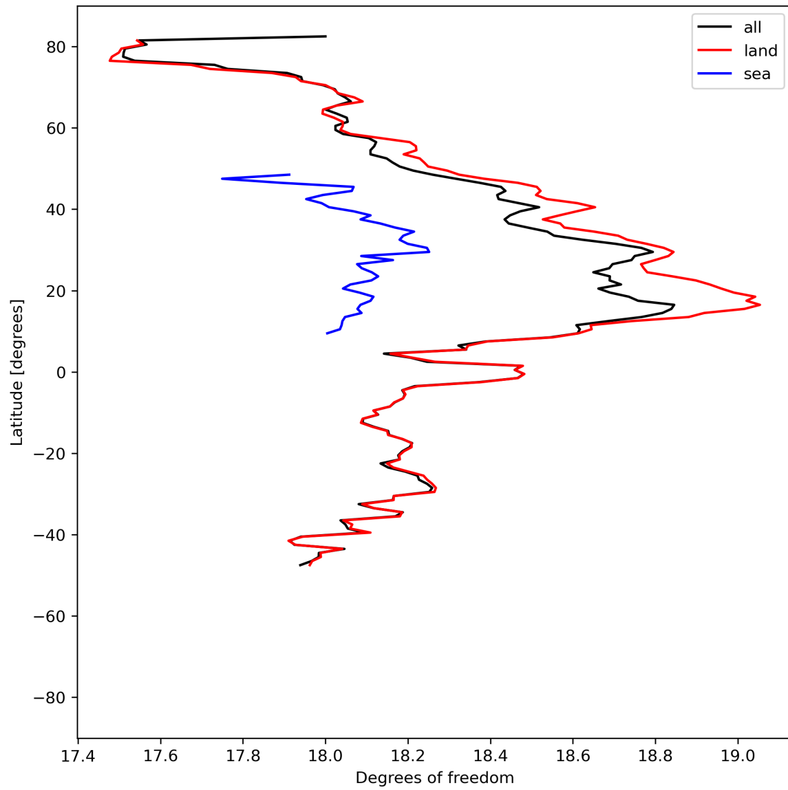
Figure 19: Zonal average of “Degrees of freedom” for 2024-05-28 to 2024-05-30.
