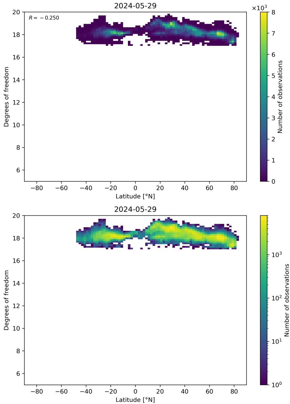
Figure 55: Scatter density plot of “Latitude” against “Degrees of freedom” for 2024-05-28 to 2024-05-30.
