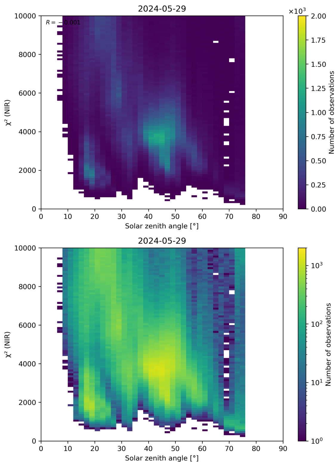
Figure 94: Scatter density plot of “Solar zenith angle” against “ \chi^2 (NIR)” for 2024-05-28 to 2024-05-30.
