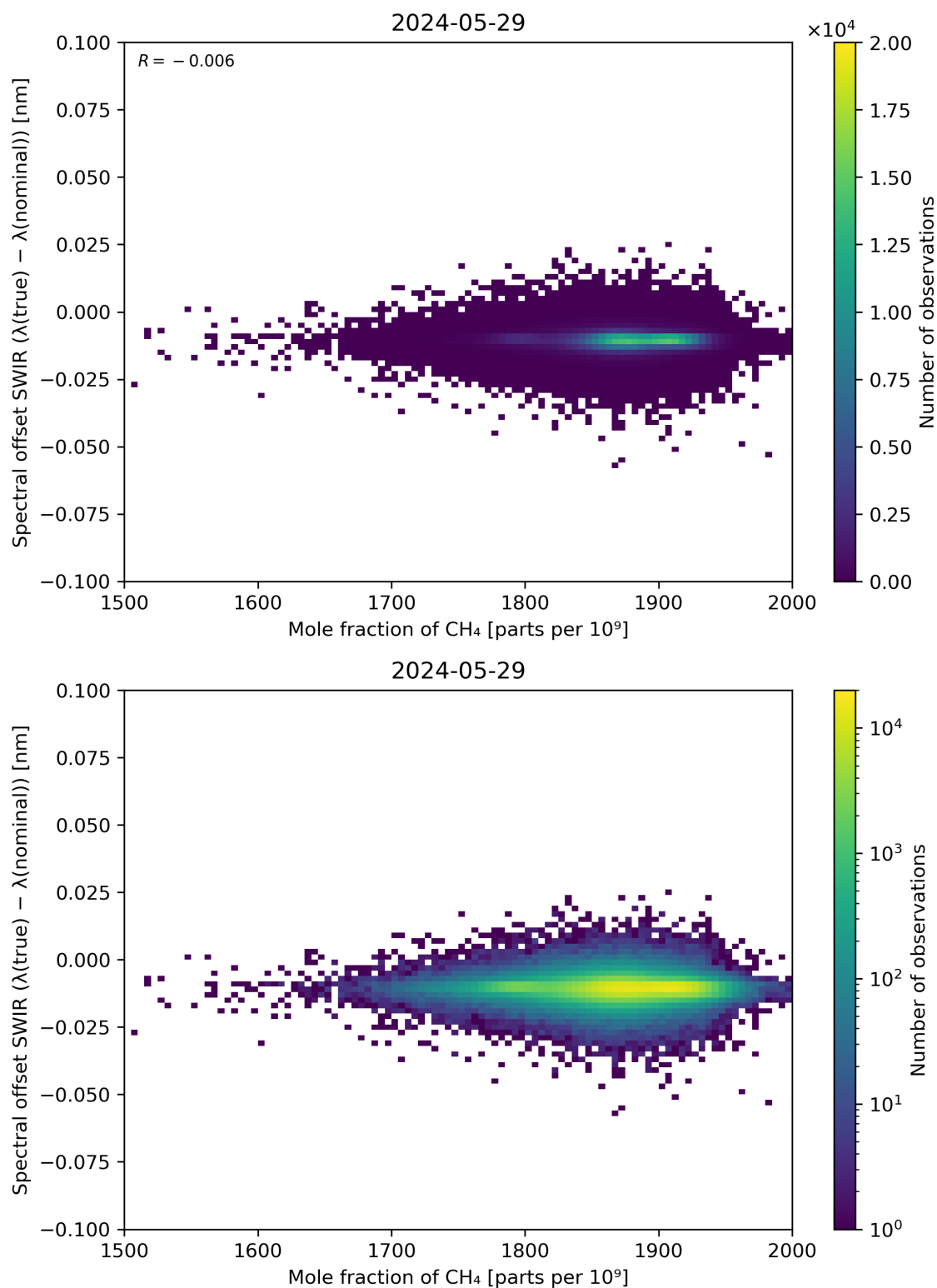
Figure 86: Scatter density plot of “Mole fraction of CH 4 ” against “Spectral offset SWIR ( \lambda(\text{true}) - \lambda(\text{nominal}) )” for 2024-05-28 to 2024-05-30.
