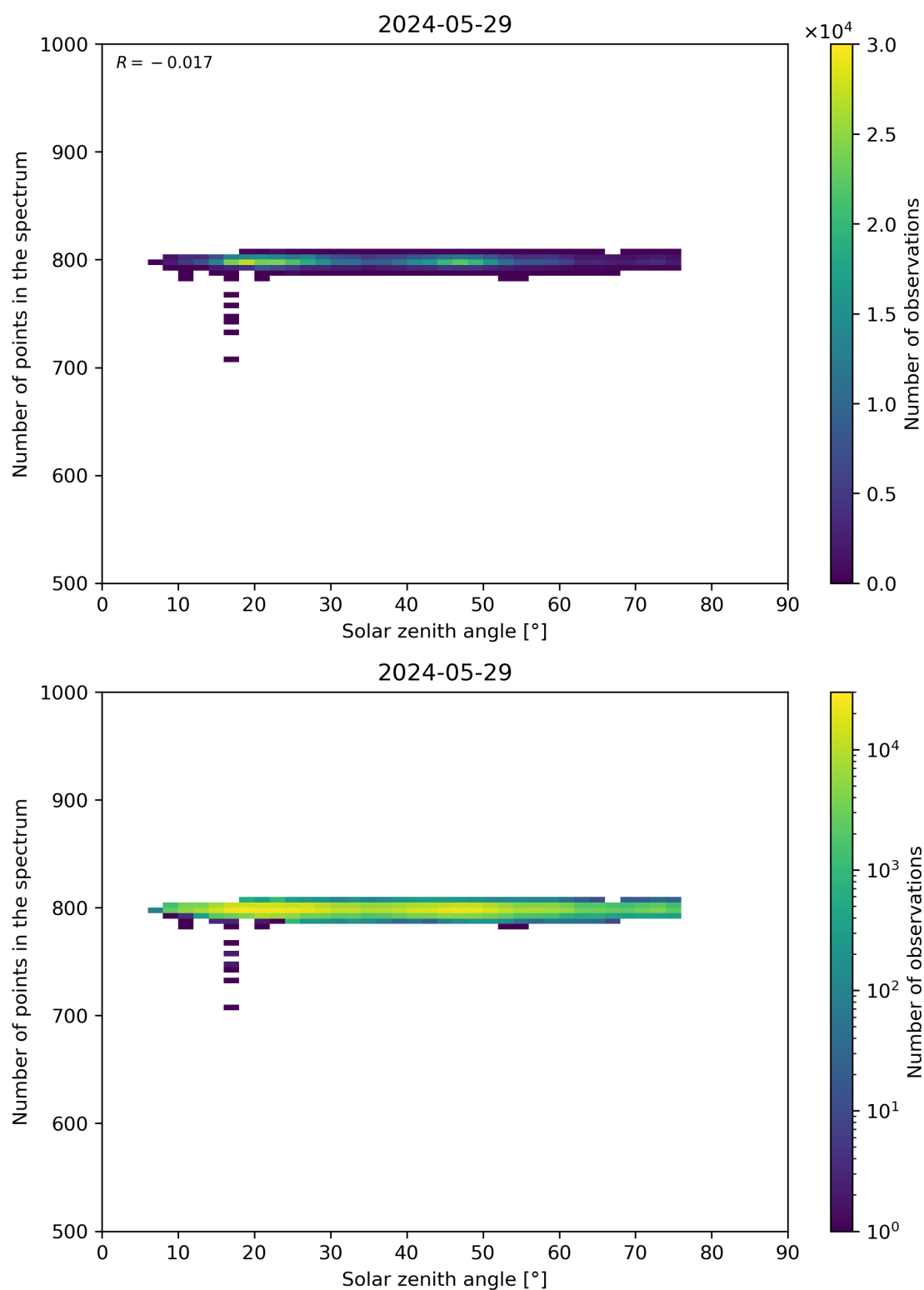
Figure 103: Scatter density plot of “Solar zenith angle” against “Number of points in the spectrum” for 2024-05-28 to 2024-05-30.
