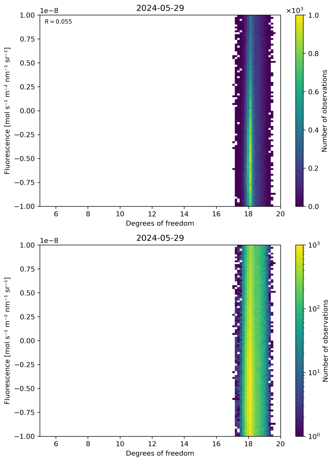
Figure 51: Scatter density plot of “Degrees of freedom” against “Fluorescence” for 2024-05-28 to 2024-05-30.
