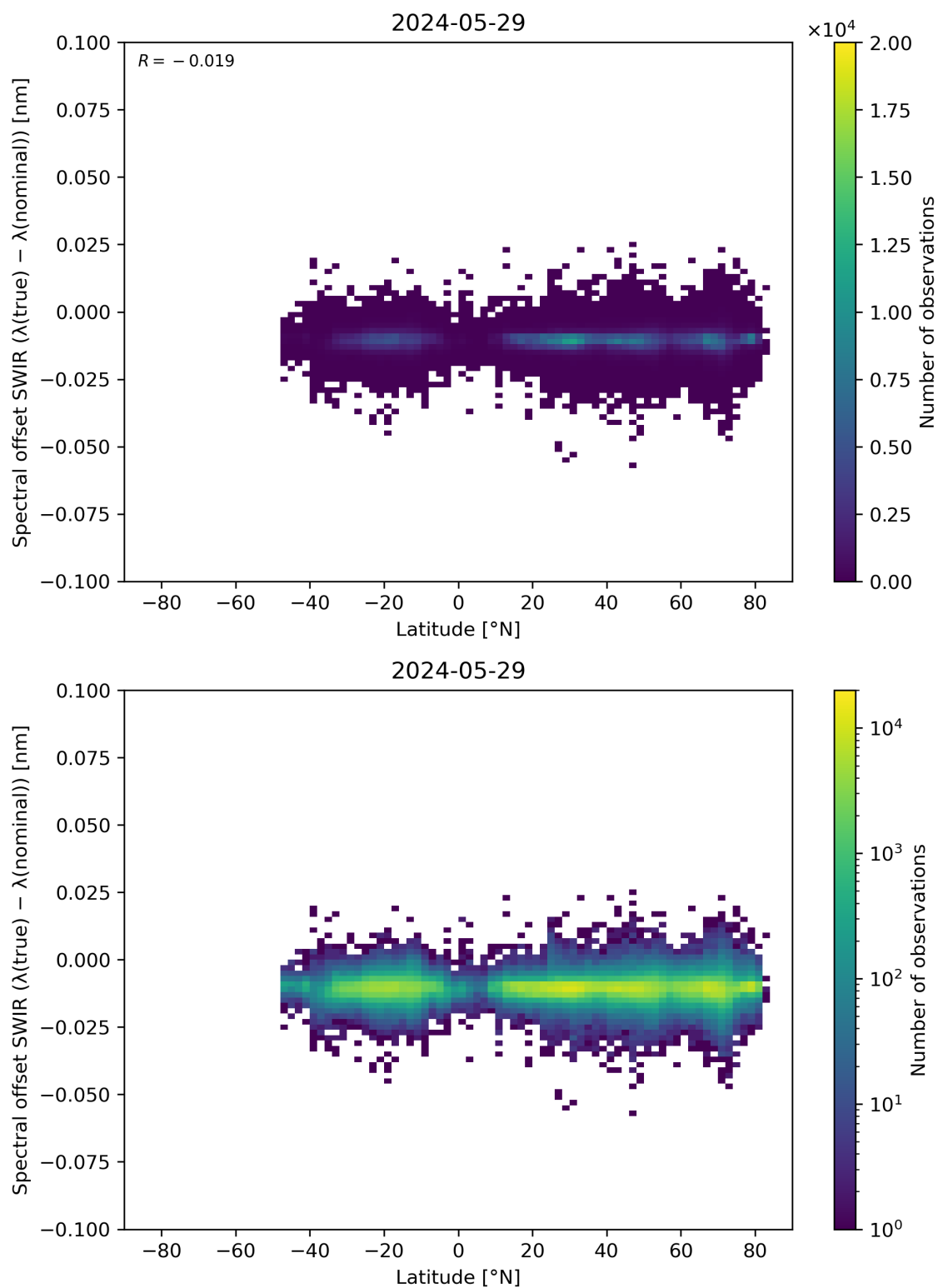
Figure 62: Scatter density plot of “Latitude” against “Spectral offset SWIR ( \lambda(\text{true}) - \lambda(\text{nominal}) )” for 2024-05-28 to 2024-05-30.
