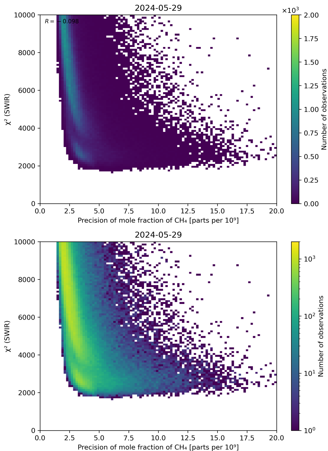
Figure 79: Scatter density plot of “Precision of mole fraction of \text{CH}_4 ” against “ \chi^2 (SWIR)” for 2024-05-28 to 2024-05-30.
