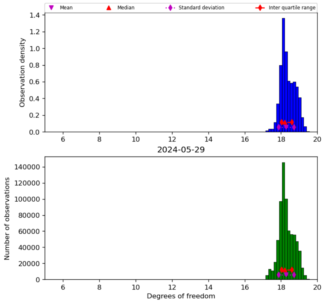
Figure 30: Histogram of “Degrees of freedom” for 2024-05-28 to 2024-05-30
