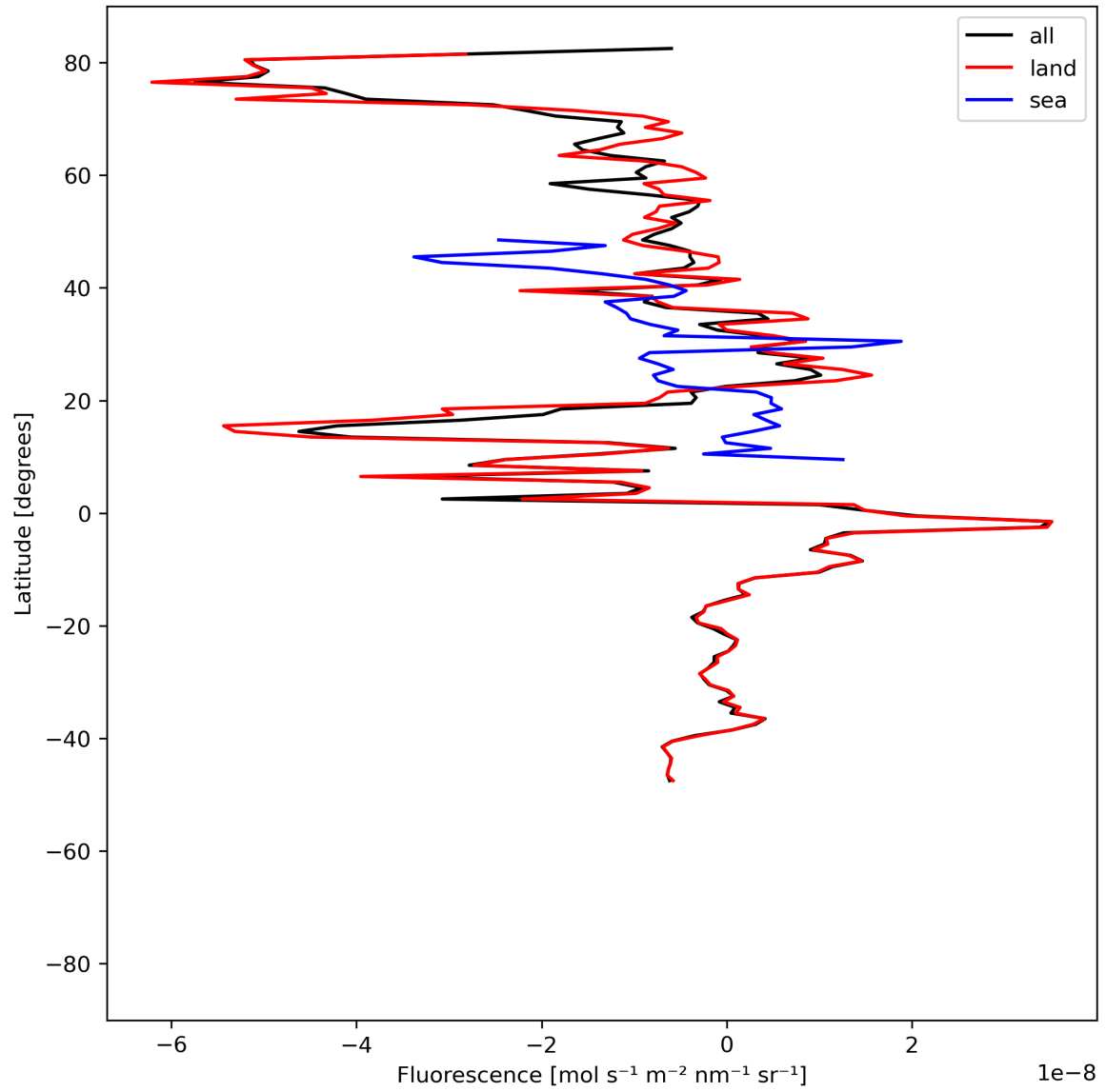
Figure 21: Zonal average of “Fluorescence” for 2024-05-28 to 2024-05-30.
