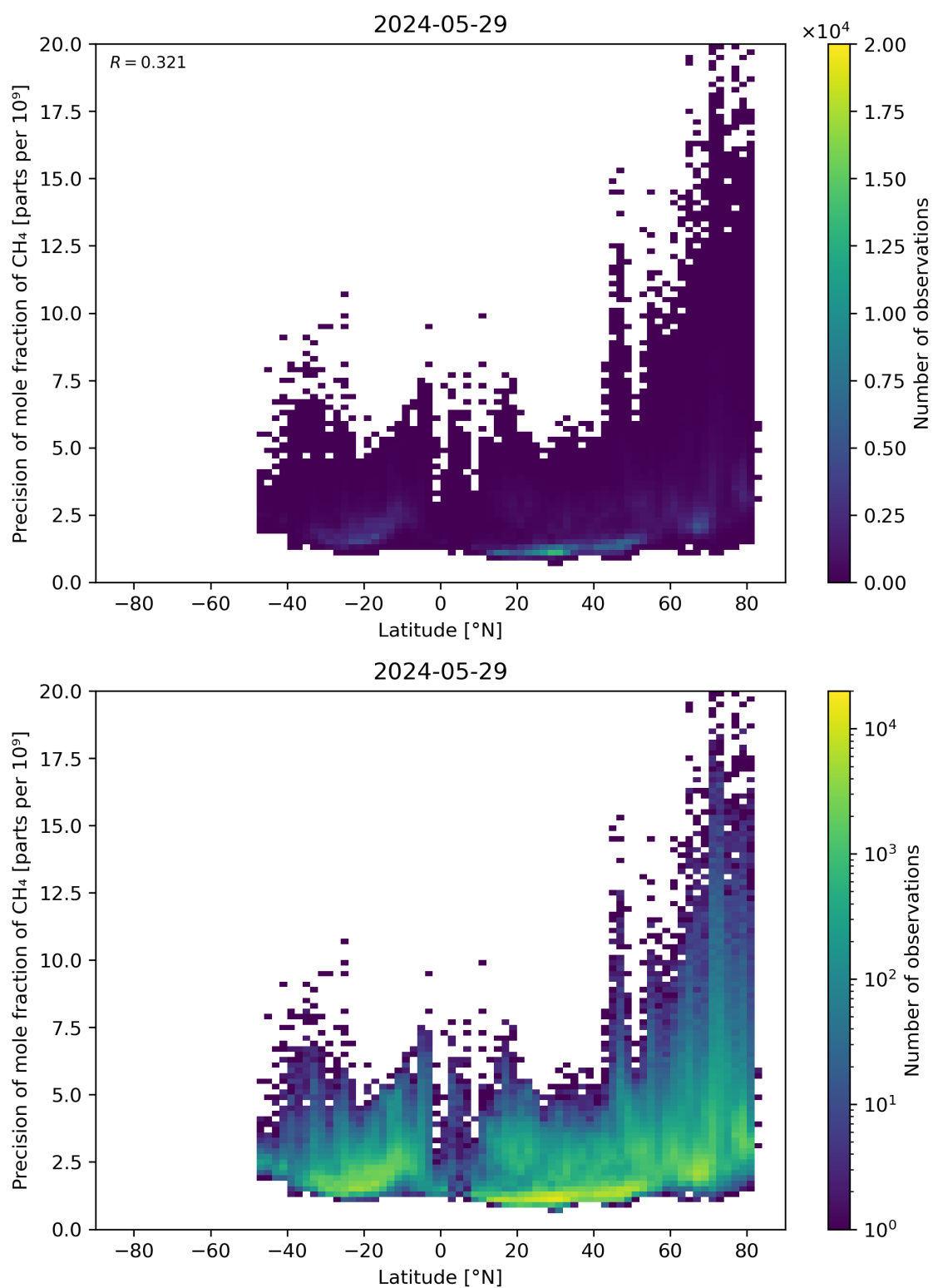
Figure 59: Scatter density plot of “Latitude” against “Precision of mole fraction of \text{CH}_4 ” for 2024-05-28 to 2024-05-30.
