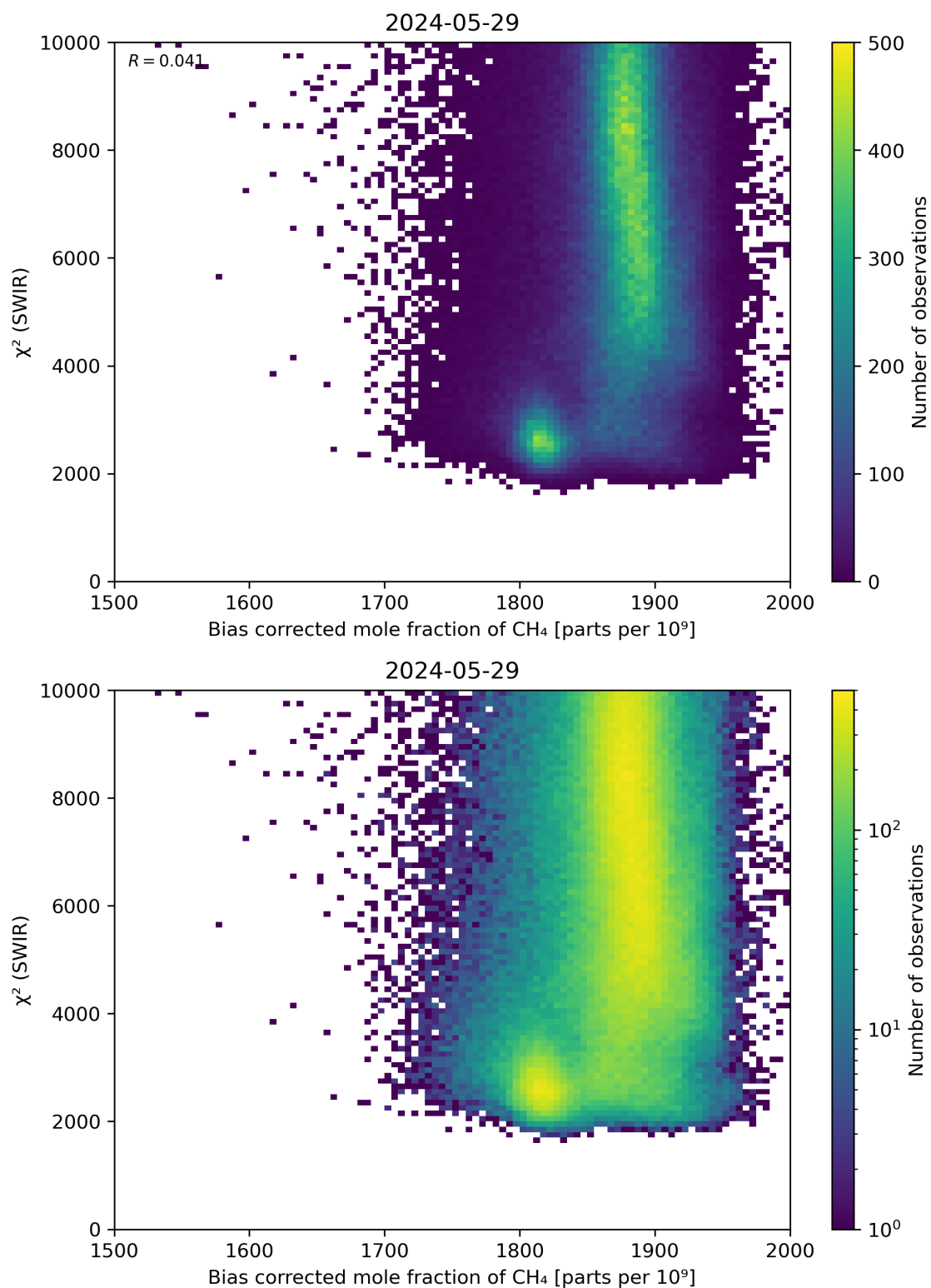
Figure 64: Scatter density plot of “Bias corrected mole fraction of \text{CH}_4 ” against “ \chi^2 (SWIR)” for 2024-05-28 to 2024-05-30.
