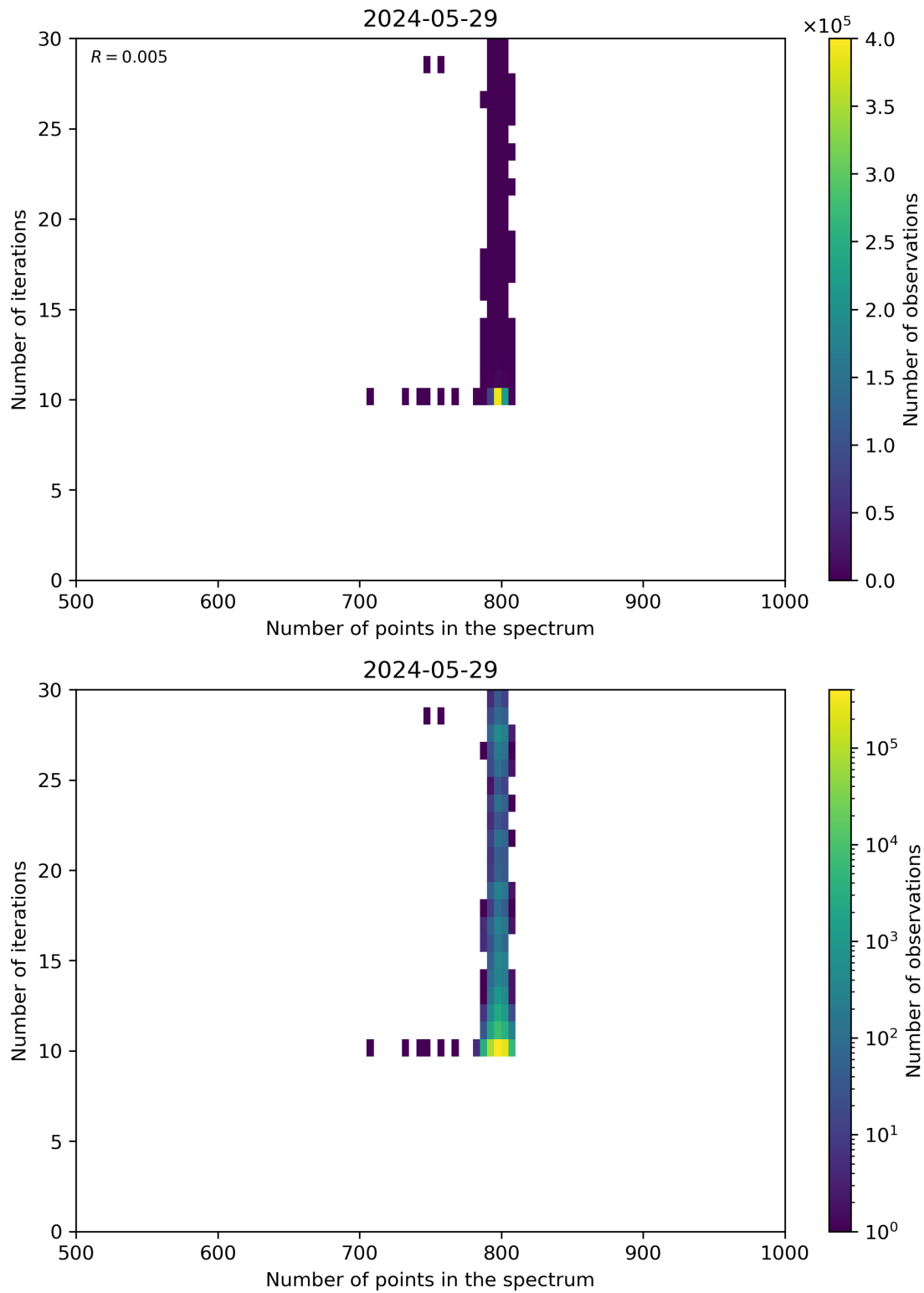
Figure 92: Scatter density plot of “Number of points in the spectrum” against “Number of iterations” for 2024-05-28 to 2024-05-30.
