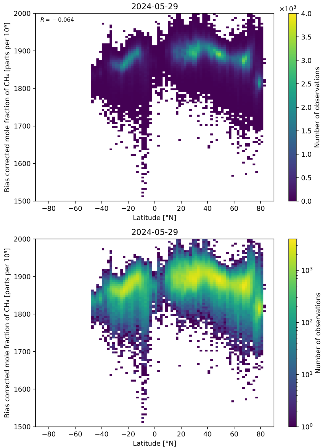
Figure 58: Scatter density plot of “Latitude” against “Bias corrected mole fraction of \text{CH}_4 ” for 2024-05-28 to 2024-05-30.
