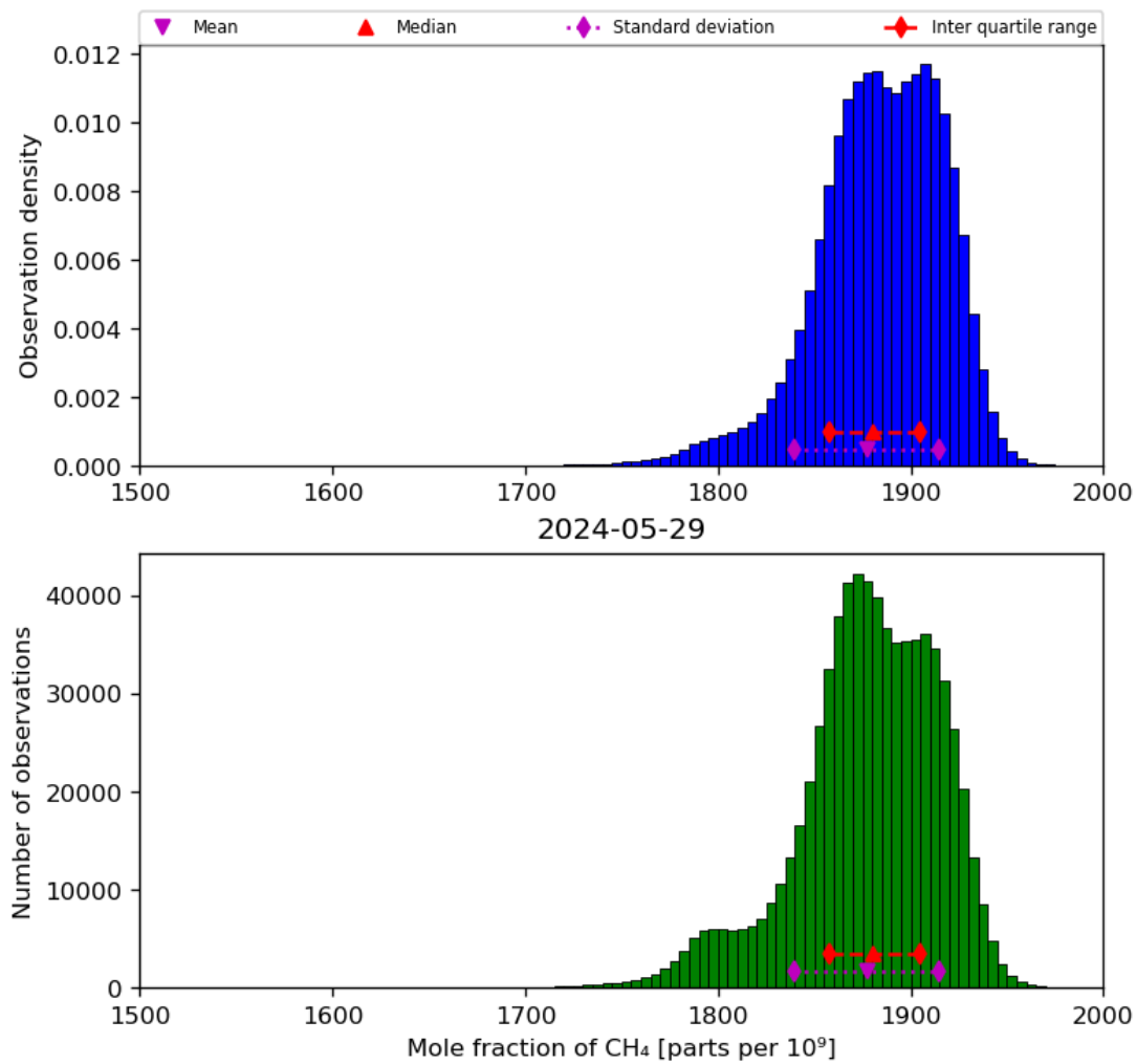
Figure 23: Histogram of “Mole fraction of CH 4 ” for 2024-05-28 to 2024-05-30
