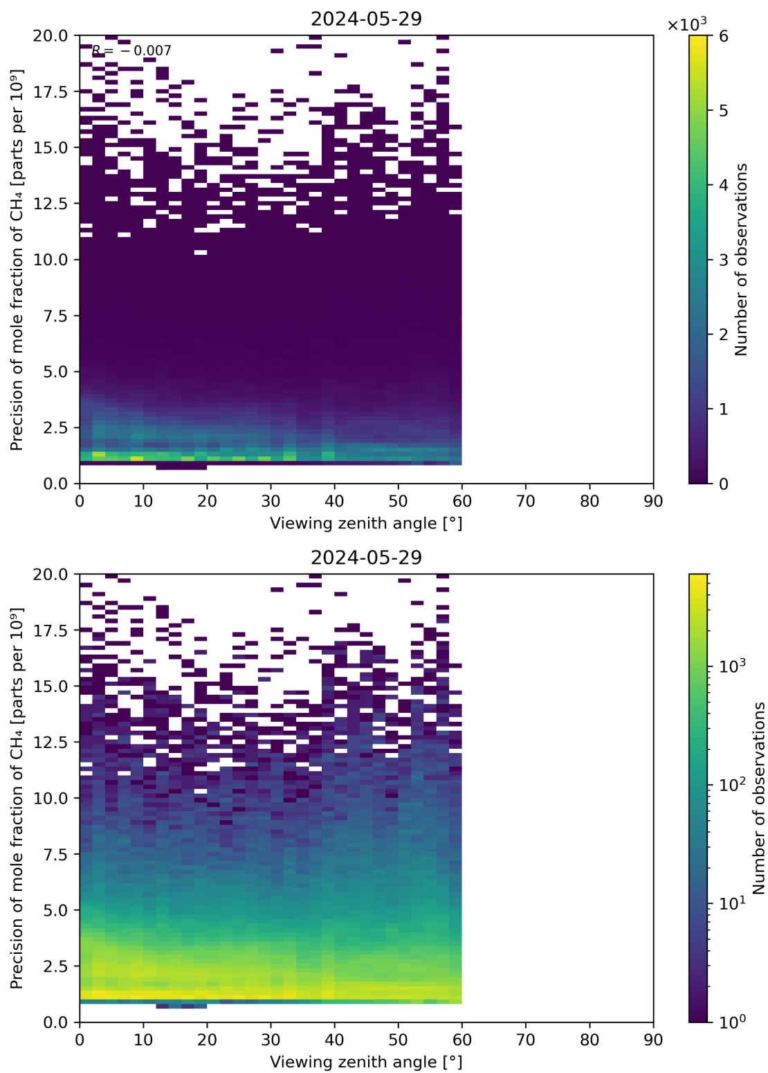
Figure 112: Scatter density plot of “Viewing zenith angle” against “Precision of mole fraction of CH 4 ” for 2024-05-28 to 2024-05-30.
