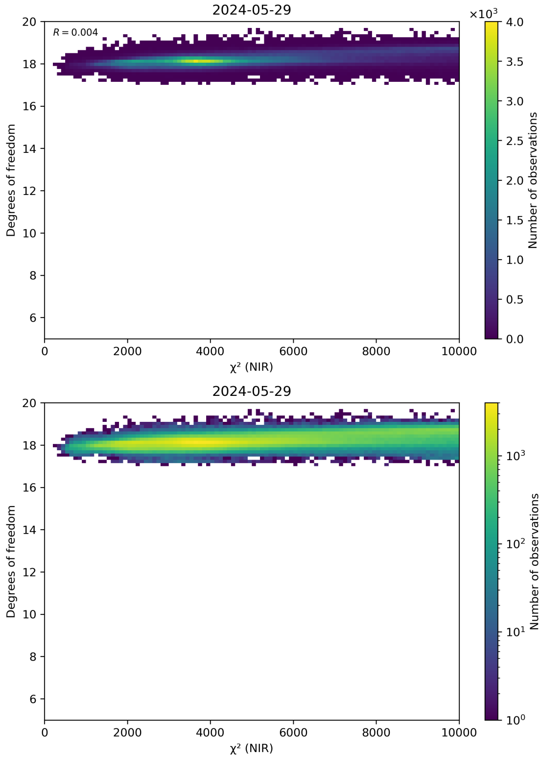
Figure 44: Scatter density plot of “ \chi^2 (NIR)” against “Degrees of freedom” for 2024-05-28 to 2024-05-30.
