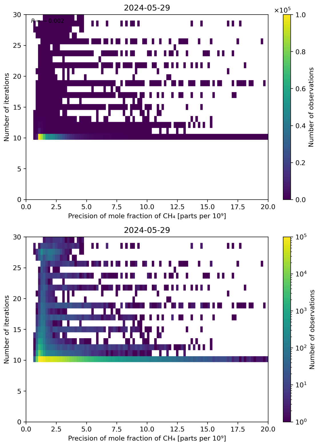
Figure 83: Scatter density plot of “Precision of mole fraction of CH 4 ” against “Number of iterations” for 2024-05-28 to 2024-05-30.
