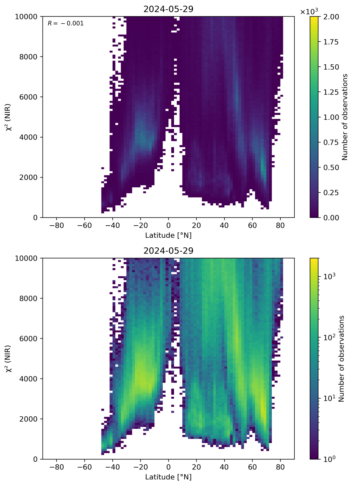
Figure 53: Scatter density plot of “Latitude” against “ \chi^2 (NIR)” for 2024-05-28 to 2024-05-30.
