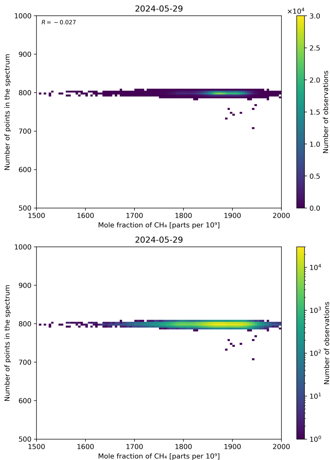
Figure 77: Scatter density plot of “Mole fraction of CH 4 ” against “Number of points in the spectrum” for 2024-05-28 to 2024-05-30.
