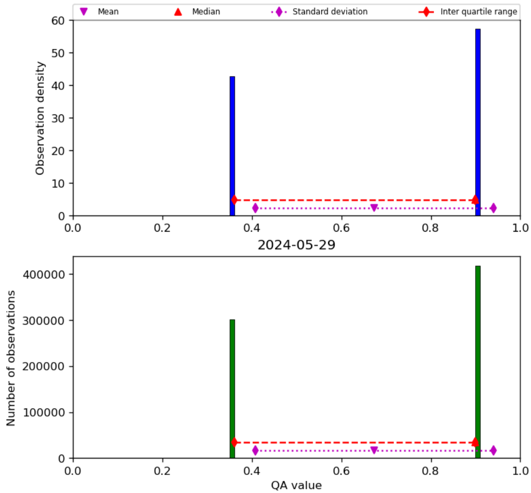
Figure 22: Histogram of “QA value” for 2024-05-28 to 2024-05-30
