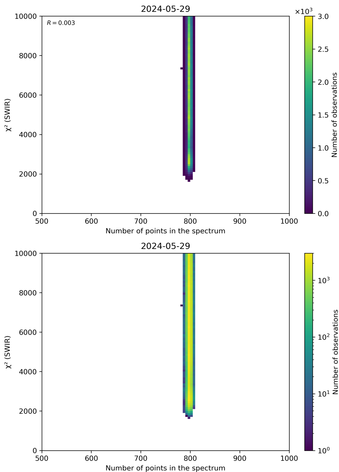
Figure 89: Scatter density plot of “Number of points in the spectrum” against “ \chi^2 (SWIR)” for 2024-05-28 to 2024-05-30.
