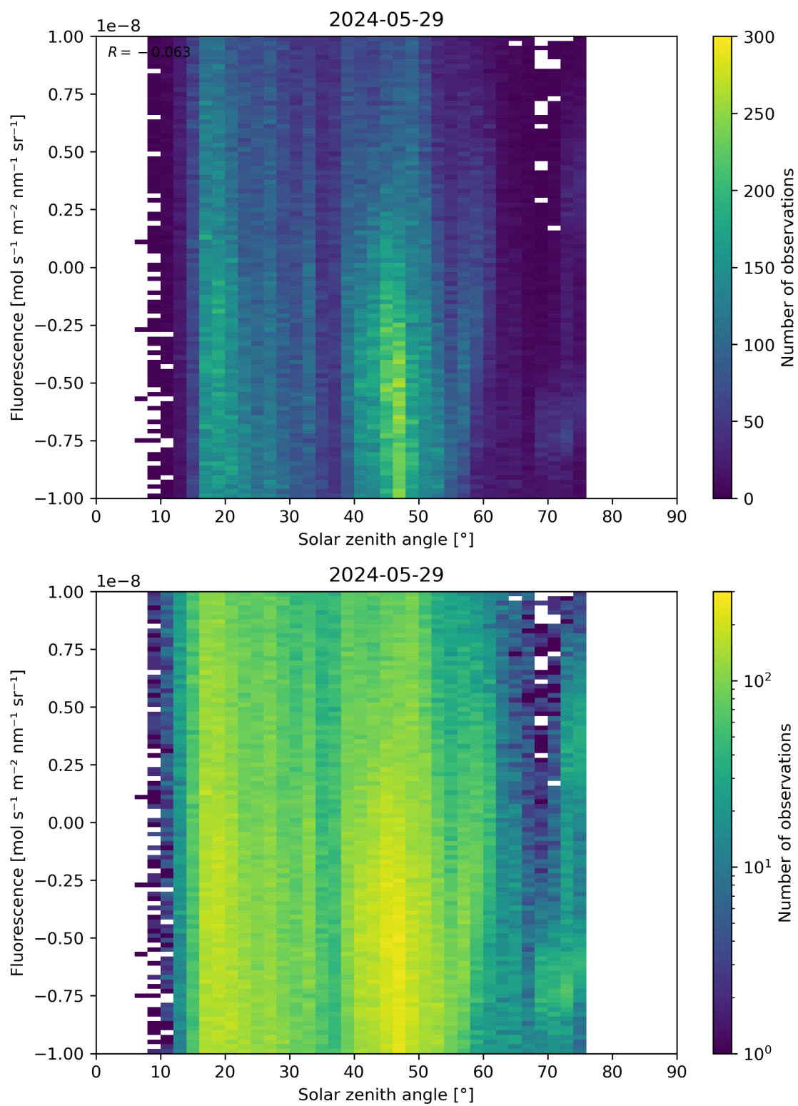
Figure 97: Scatter density plot of “Solar zenith angle” against “Fluorescence” for 2024-05-28 to 2024-05-30.
