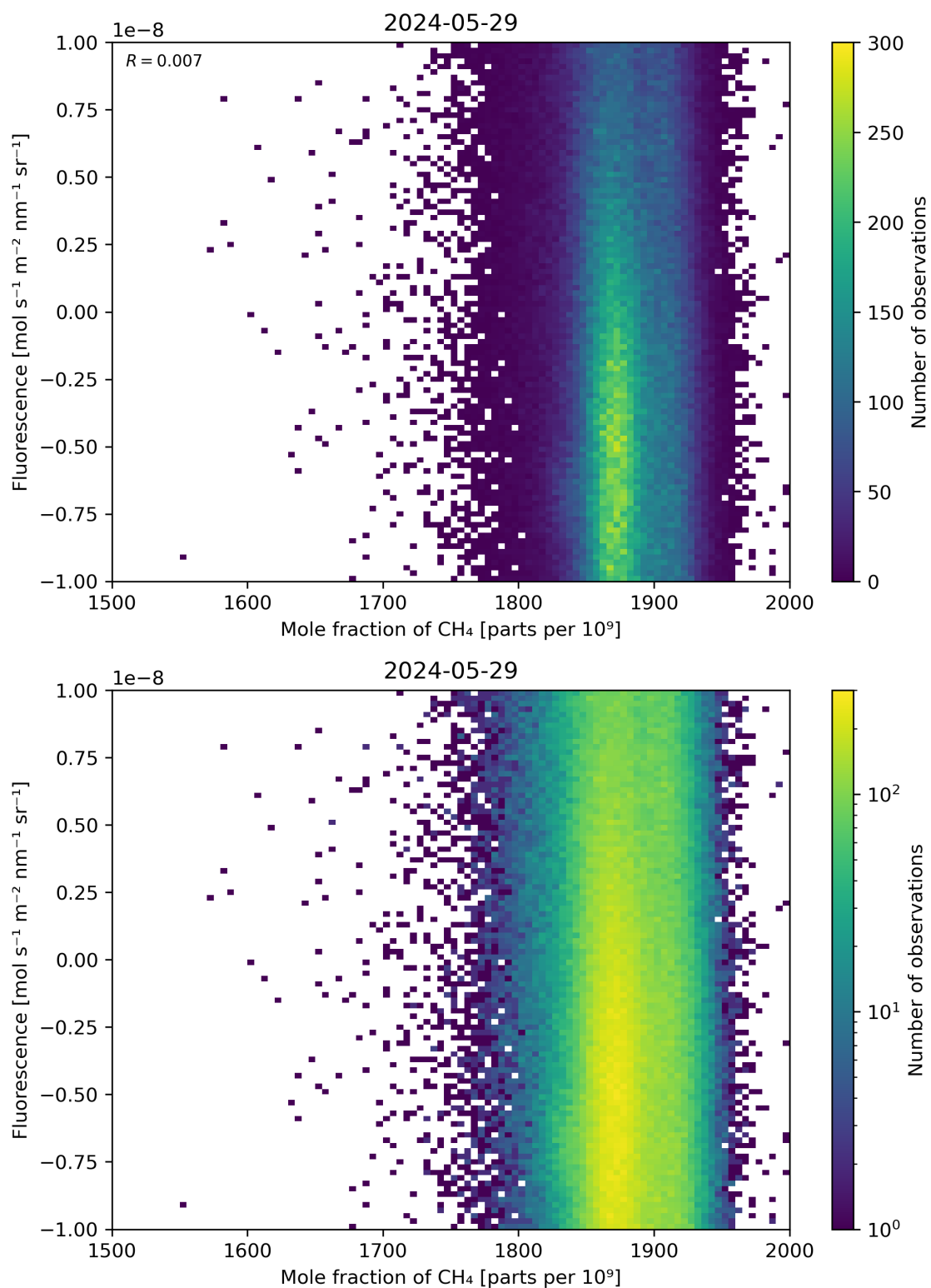
Figure 73: Scatter density plot of “Mole fraction of \text{CH}_4 ” against “Fluorescence” for 2024-05-28 to 2024-05-30.
