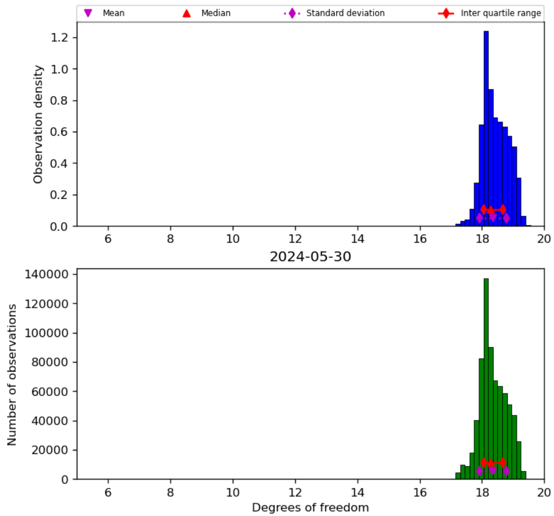
Figure 30: Histogram of “Degrees of freedom” for 2024-05-29 to 2024-05-31
