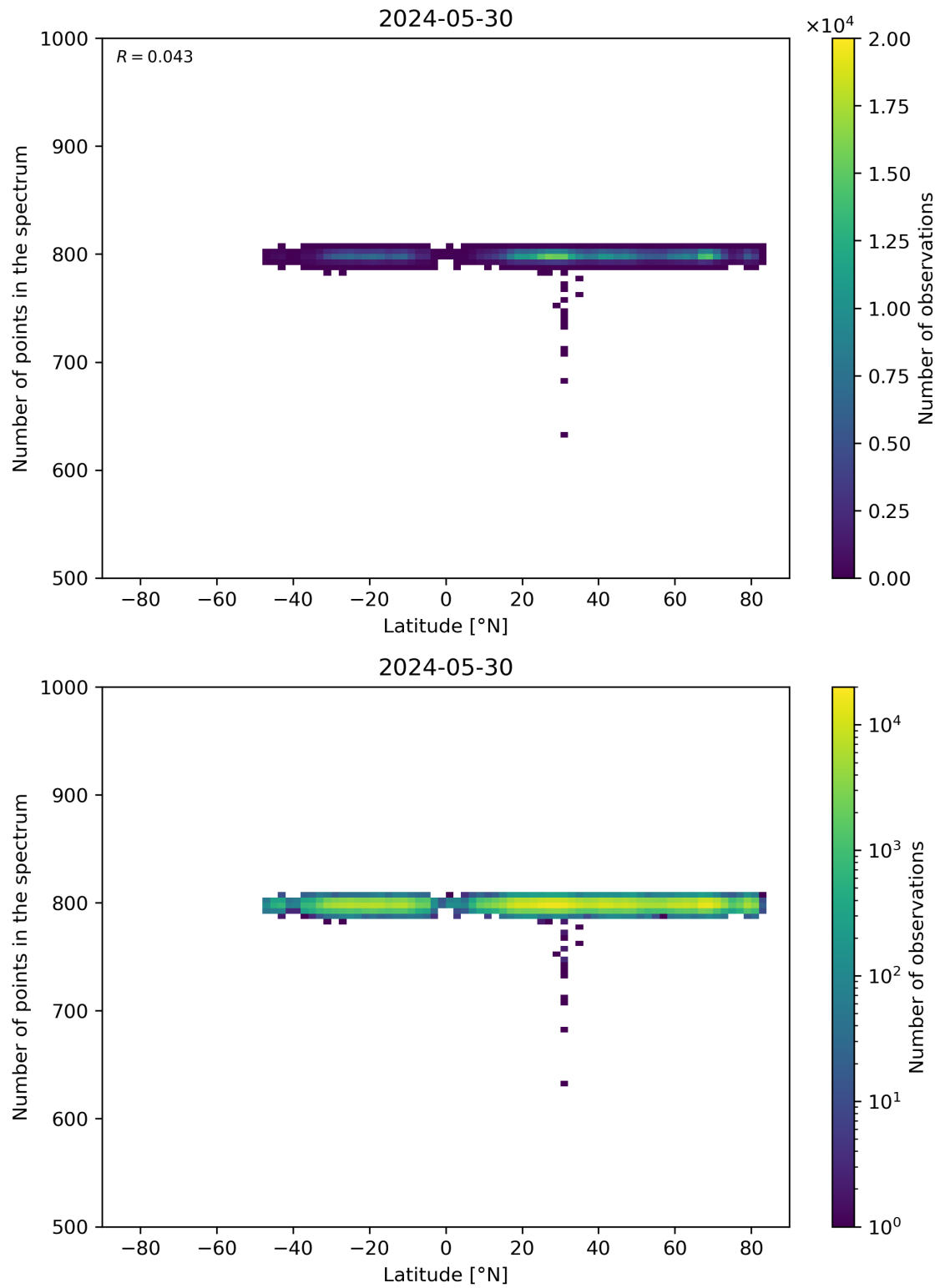
Figure 61: Scatter density plot of “Latitude” against “Number of points in the spectrum” for 2024-05-29 to 2024-05-31.
