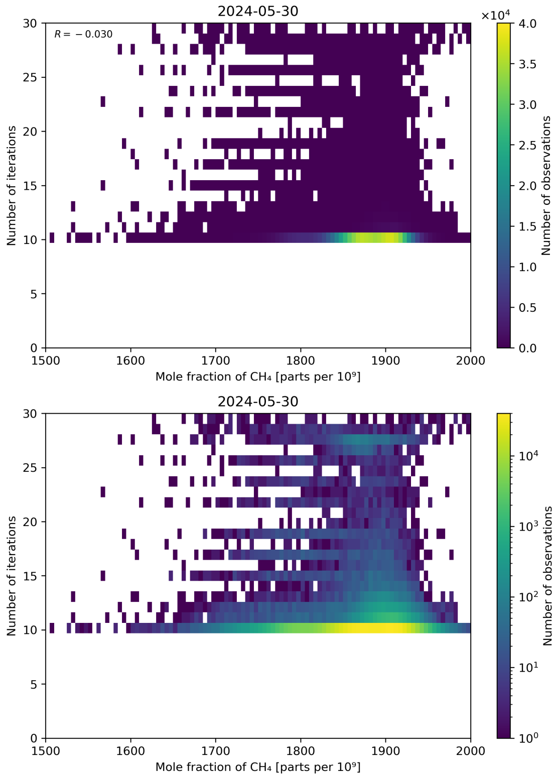
Figure 76: Scatter density plot of “Mole fraction of CH 4 ” against “Number of iterations” for 2024-05-29 to 2024-05-31.
