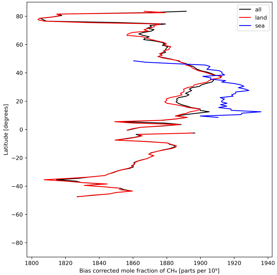
Figure 14: Zonal average of “Bias corrected mole fraction of \text{CH}_4 ” for 2024-05-29 to 2024-05-31.
