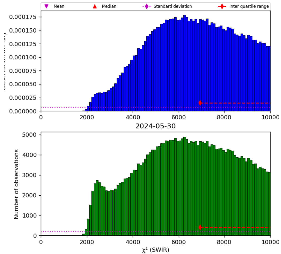
Figure 28: Histogram of “ \chi^2 (SWIR)” for 2024-05-29 to 2024-05-31
