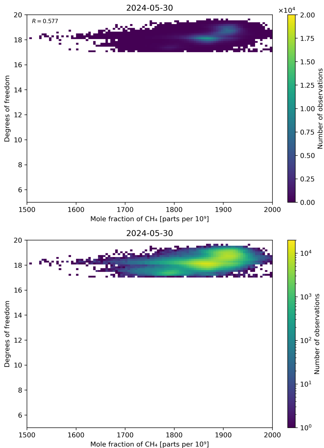
Figure 72: Scatter density plot of “Mole fraction of CH 4 ” against “Degrees of freedom” for 2024-05-29 to 2024-05-31.
