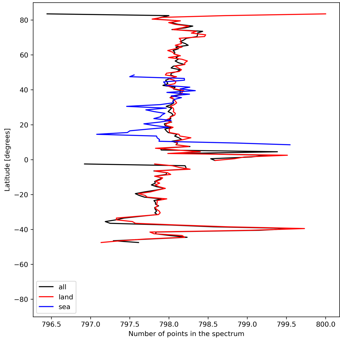
Figure 15: Zonal average of “Number of points in the spectrum” for 2024-05-29 to 2024-05-31.
