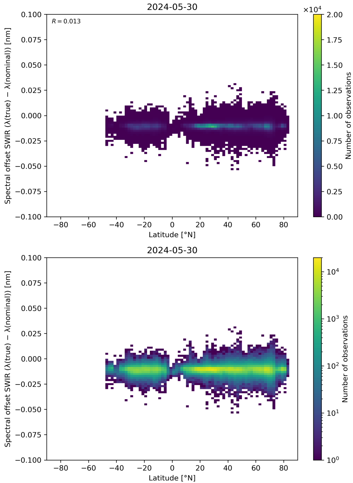
Figure 62: Scatter density plot of “Latitude” against “Spectral offset SWIR ( \lambda(\text{true}) - \lambda(\text{nominal}) )” for 2024-05-29 to 2024-05-31.
