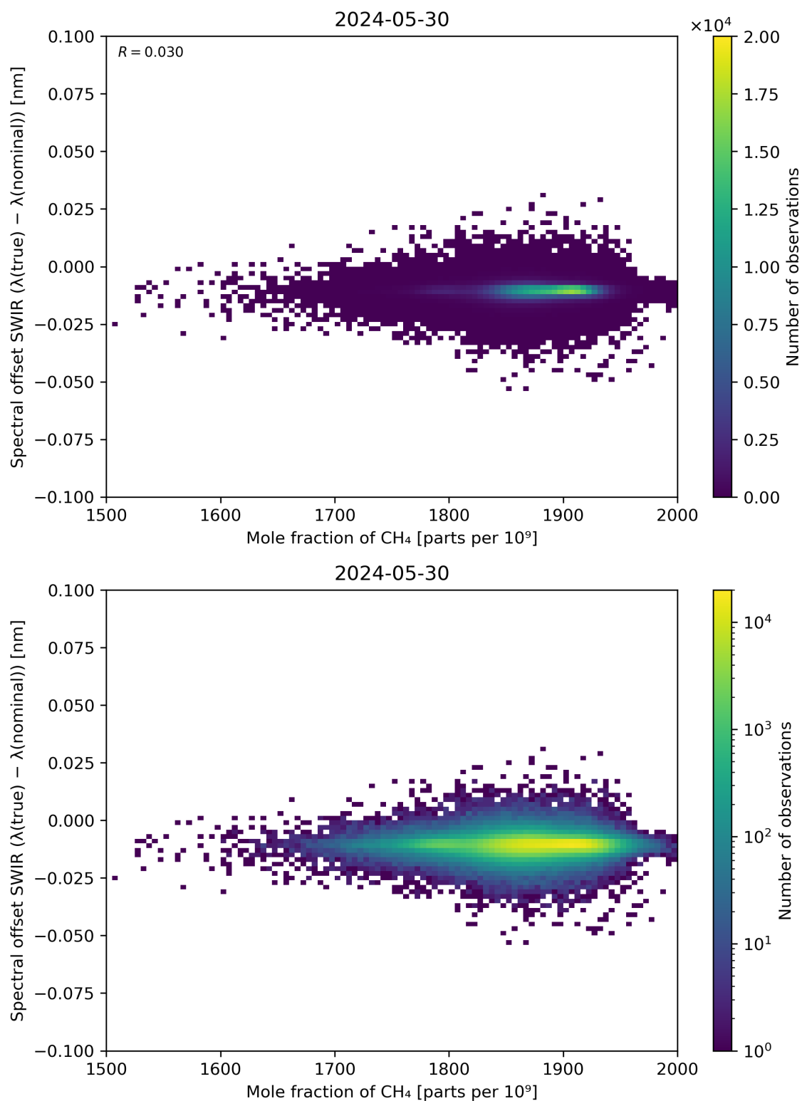
Figure 86: Scatter density plot of “Mole fraction of CH 4 ” against “Spectral offset SWIR ( \lambda(\text{true}) - \lambda(\text{nominal}) )” for 2024-05-29 to 2024-05-31.
