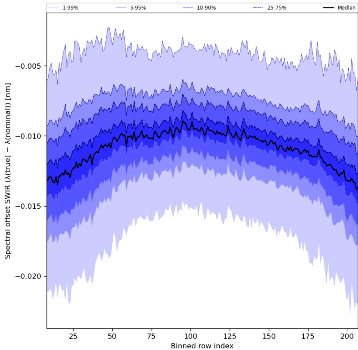
Figure 38: Along track statistics of “Spectral offset SWIR ( \lambda(\text{true}) - \lambda(\text{nominal}) )” for 2024-05-29 to 2024-05-31
