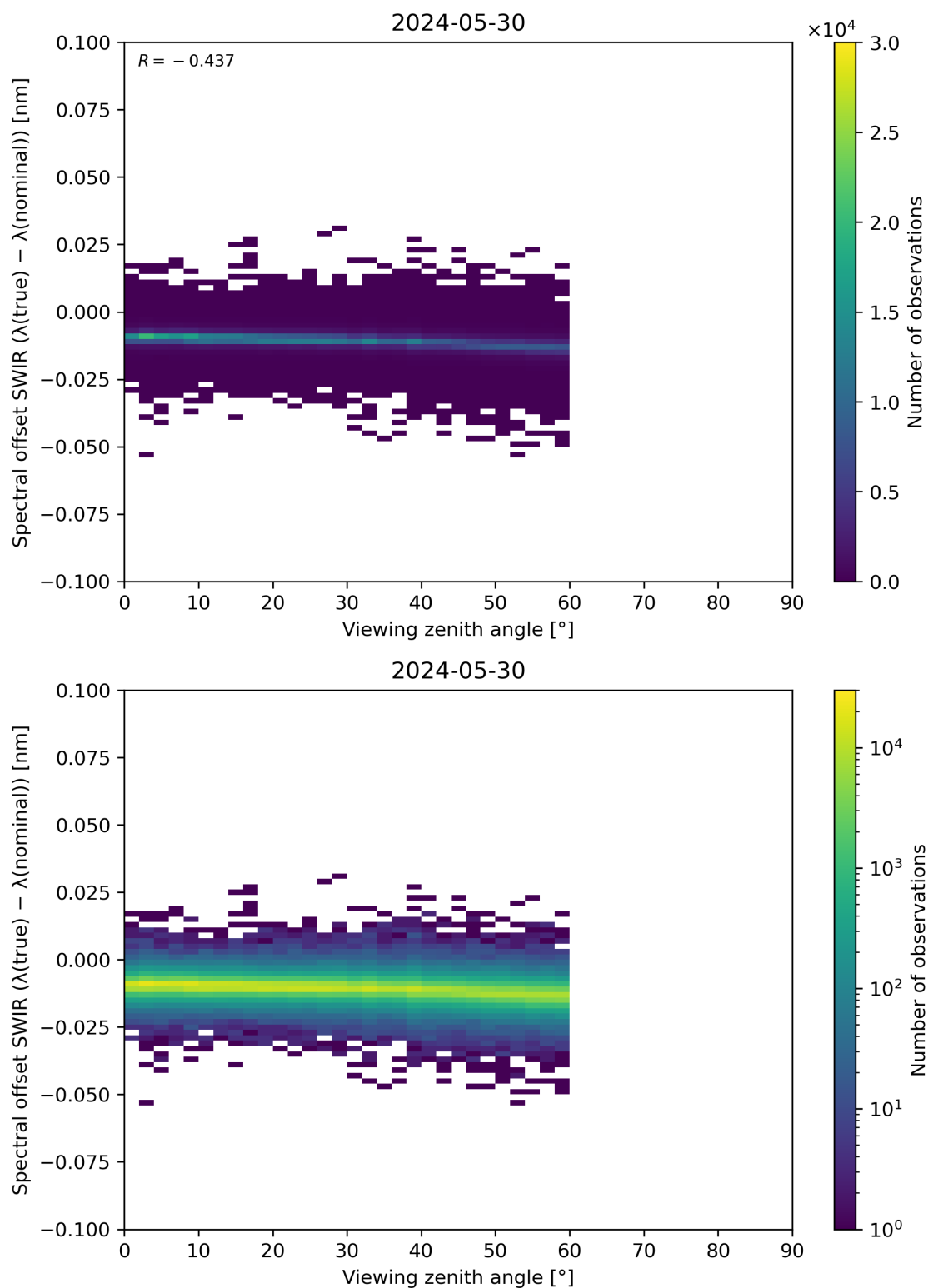
Figure 116: Scatter density plot of “Viewing zenith angle” against “Spectral offset SWIR ( \lambda(\text{true}) - \lambda(\text{nominal}) )” for 2024-05-29 to 2024-05-31.
