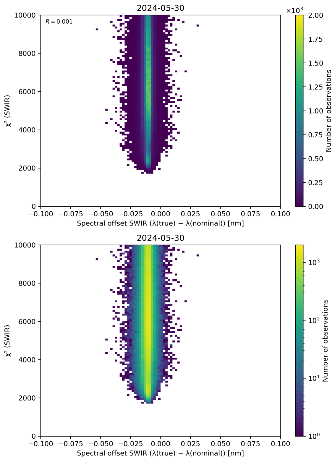
Figure 118: Scatter density plot of “Spectral offset SWIR ( \lambda(\text{true}) - \lambda(\text{nominal}) )” against “ \chi^2 (SWIR)” for 2024-05-29 to 2024-05-31.
