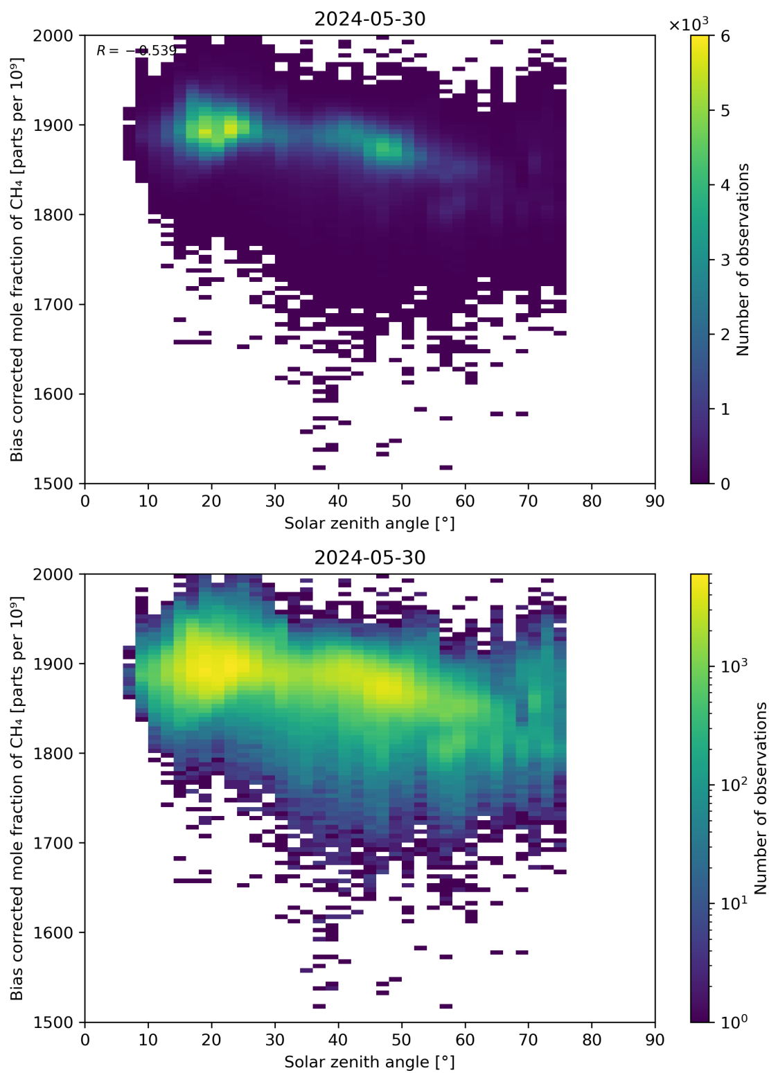
Figure 100: Scatter density plot of “Solar zenith angle” against “Bias corrected mole fraction of CH 4 ” for 2024-05-29 to 2024-05-31.
