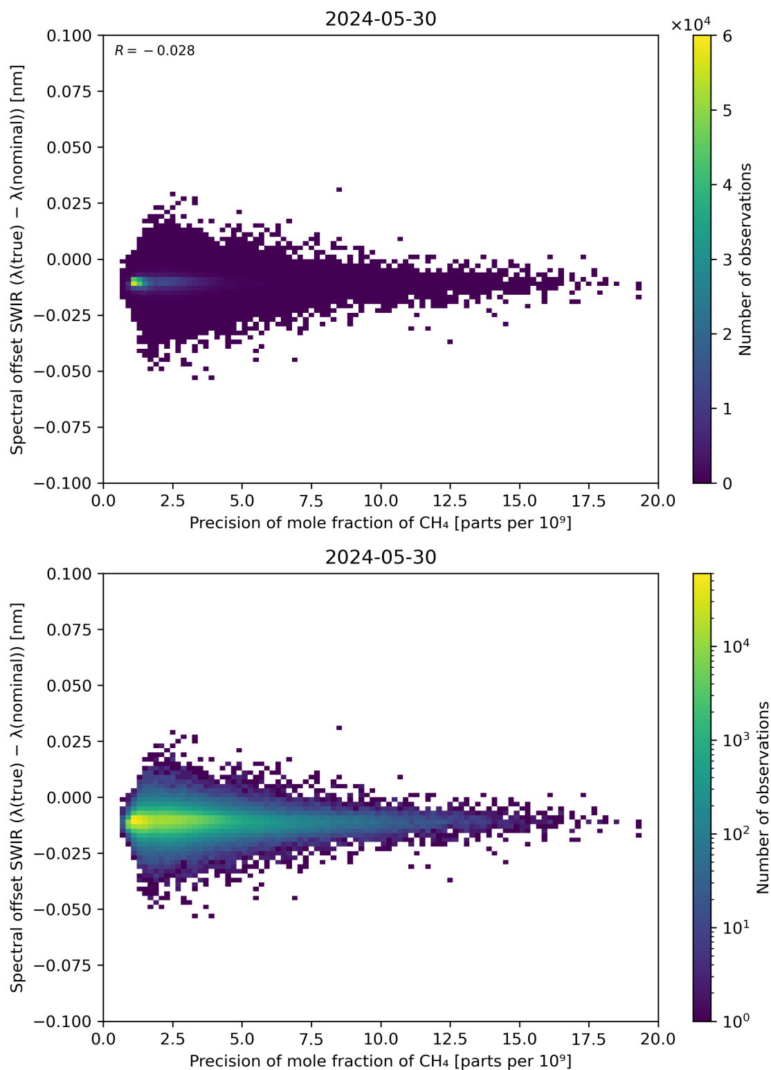
Figure 85: Scatter density plot of “Precision of mole fraction of CH 4 ” against “Spectral offset SWIR ( \lambda(\text{true}) - \lambda(\text{nominal}) )” for 2024-05-29 to 2024-05-31.
