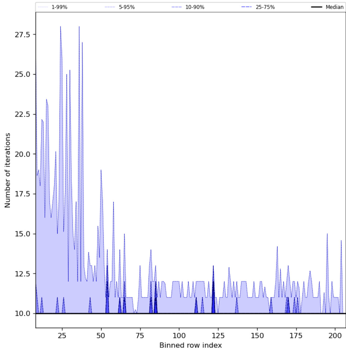
Figure 42: Along track statistics of “Number of iterations” for 2024-05-29 to 2024-05-31
