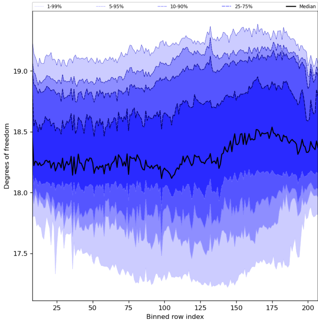
Figure 41: Along track statistics of “Degrees of freedom” for 2024-05-29 to 2024-05-31
