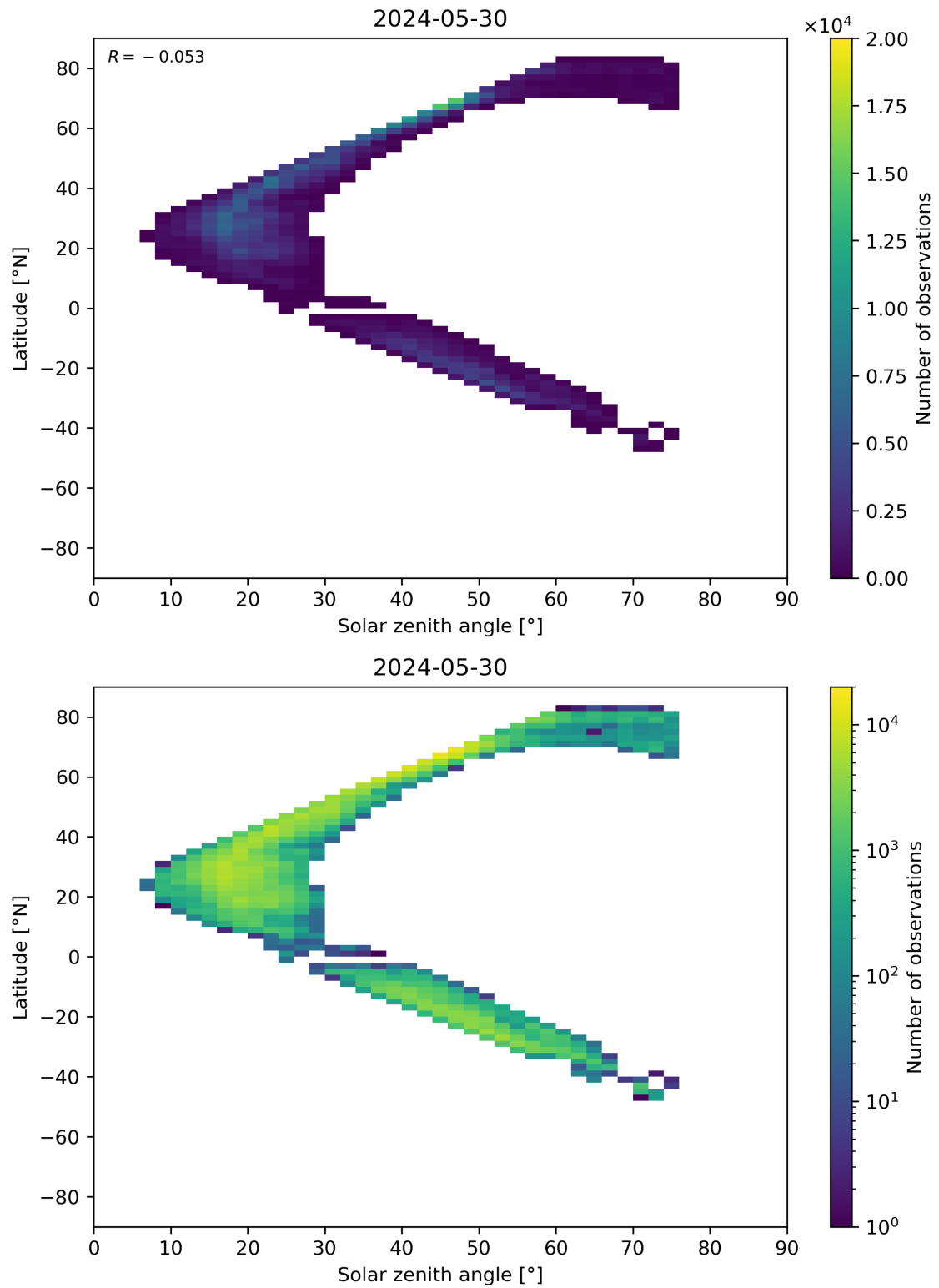
Figure 98: Scatter density plot of “Solar zenith angle” against “Latitude” for 2024-05-29 to 2024-05-31.
