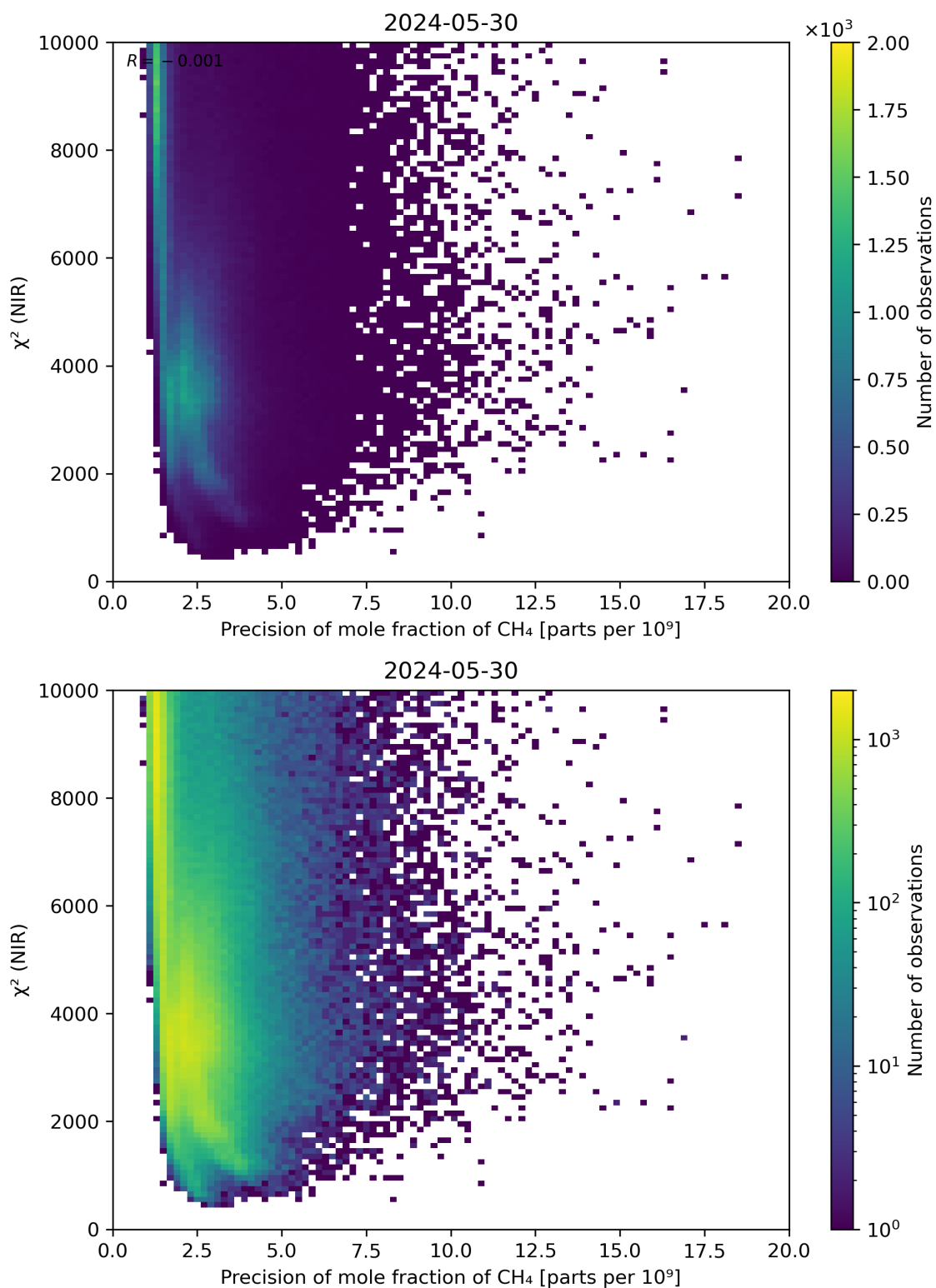
Figure 78: Scatter density plot of “Precision of mole fraction of CH 4 ” against “ \chi^2 (NIR)” for 2024-05-29 to 2024-05-31.
