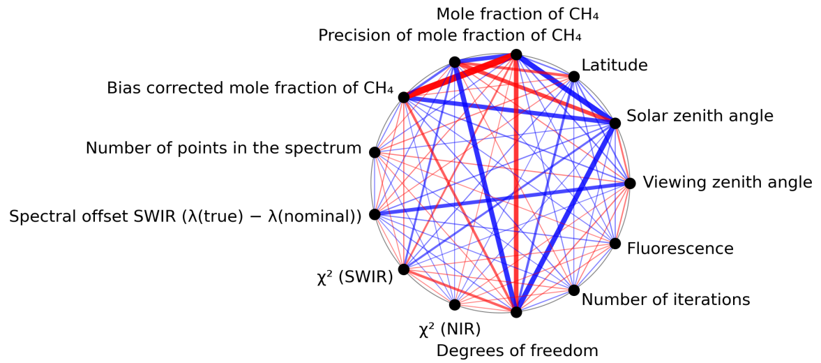
Figure 1: Map of correlation graph for 2024-05-29 to 2024-05-31.
