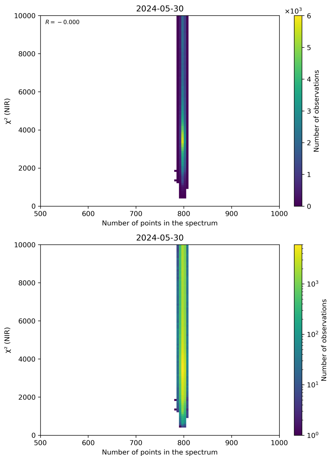
Figure 88: Scatter density plot of “Number of points in the spectrum” against “ \chi^2 (NIR)” for 2024-05-29 to 2024-05-31.
