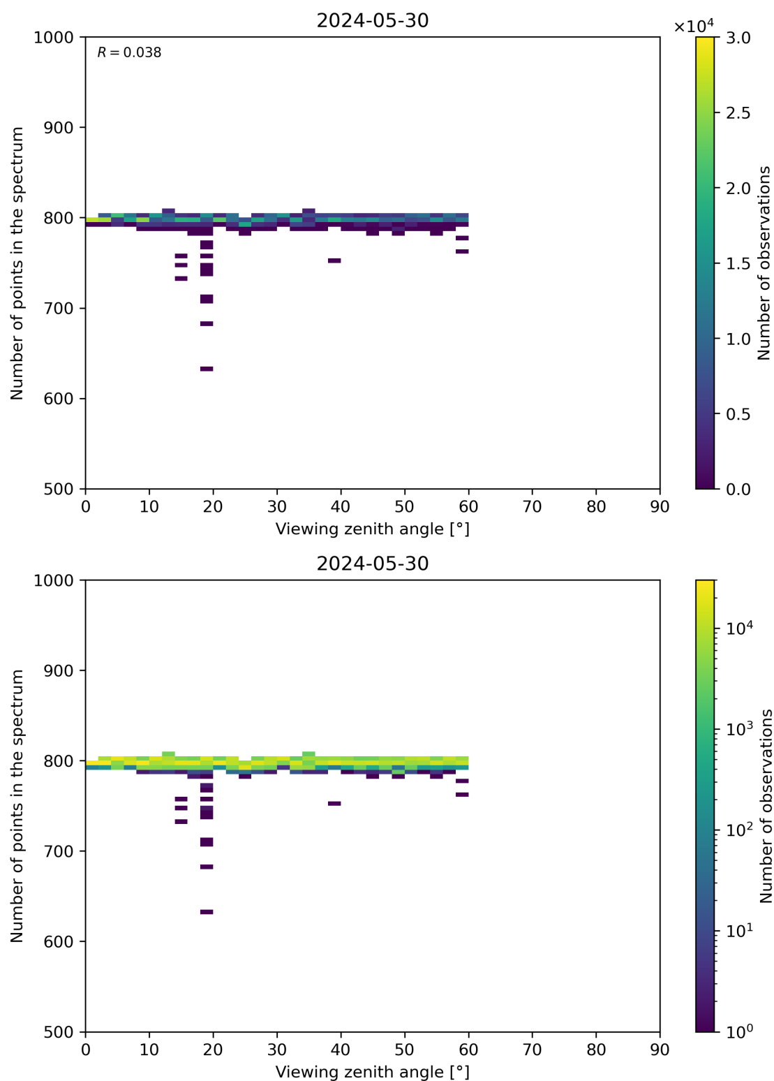
Figure 114: Scatter density plot of “Viewing zenith angle” against “Number of points in the spectrum” for 2024-05-29 to 2024-05-31.
