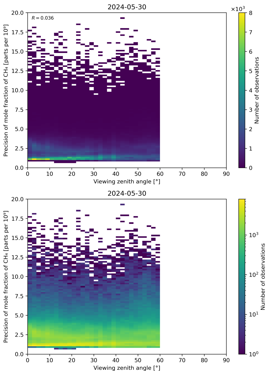
Figure 112: Scatter density plot of “Viewing zenith angle” against “Precision of mole fraction of CH 4 ” for 2024-05-29 to 2024-05-31.
