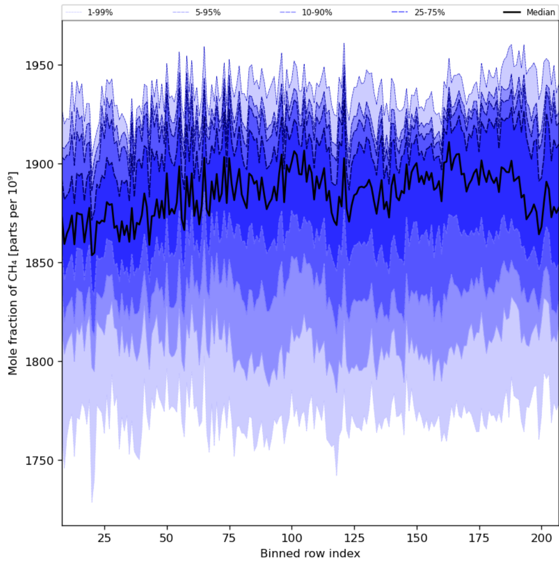
Figure 34: Along track statistics of “Mole fraction of CH 4 ” for 2024-05-29 to 2024-05-31
