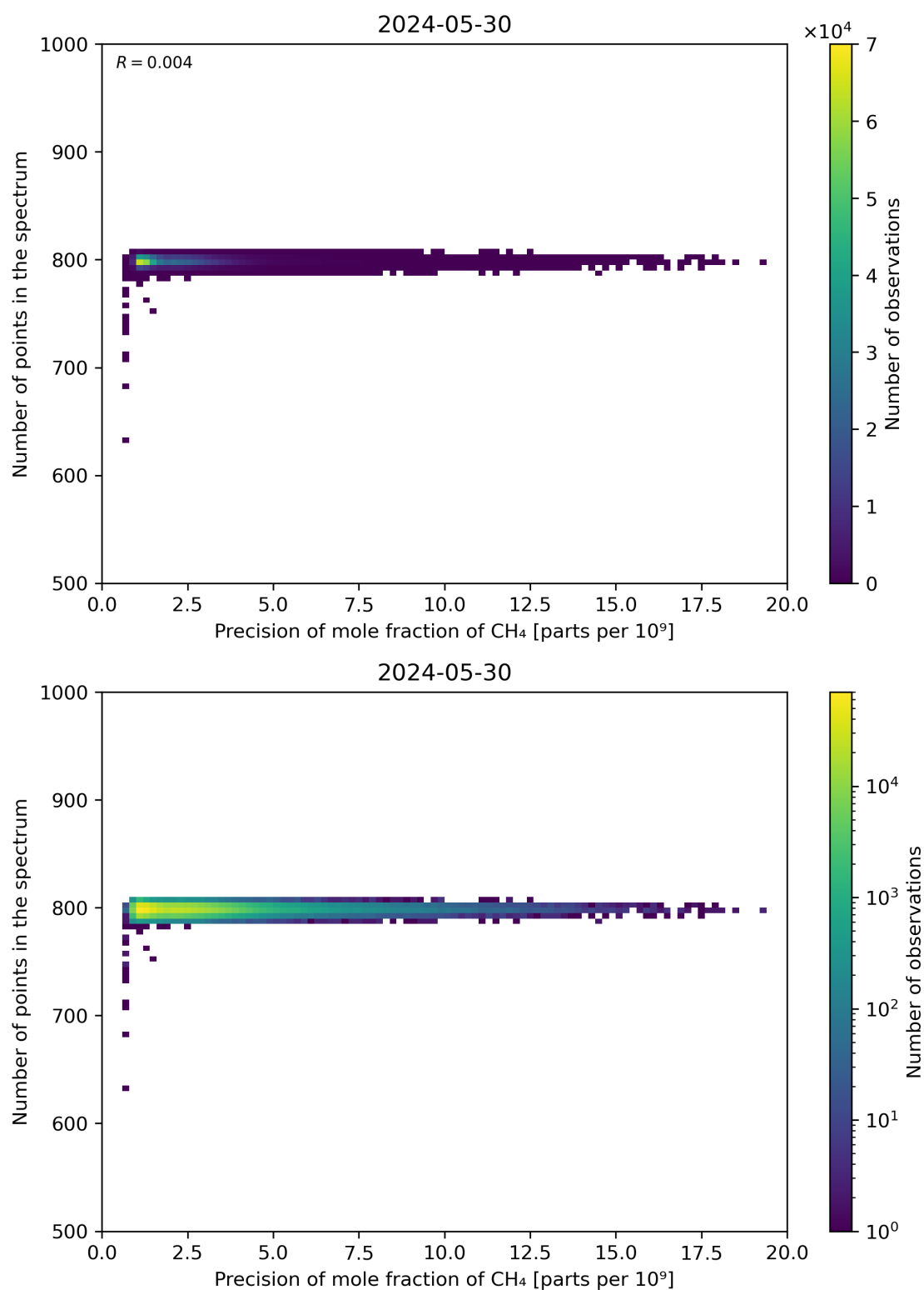
Figure 84: Scatter density plot of “Precision of mole fraction of CH 4 ” against “Number of points in the spectrum” for 2024-05-29 to 2024-05-31.
