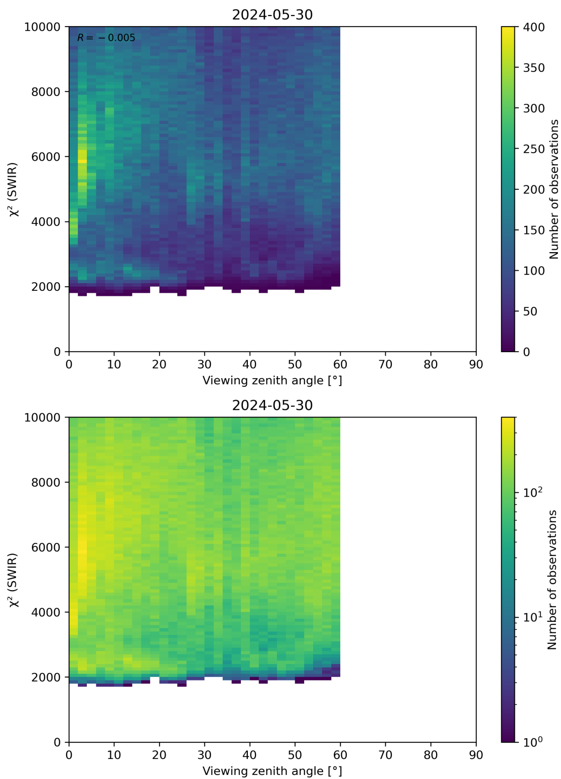
Figure 106: Scatter density plot of “Viewing zenith angle” against “ \chi^2 (SWIR)” for 2024-05-29 to 2024-05-31.
