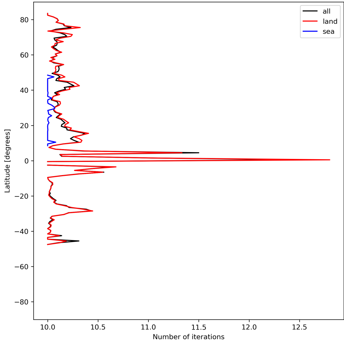
Figure 20: Zonal average of “Number of iterations” for 2024-05-29 to 2024-05-31.
