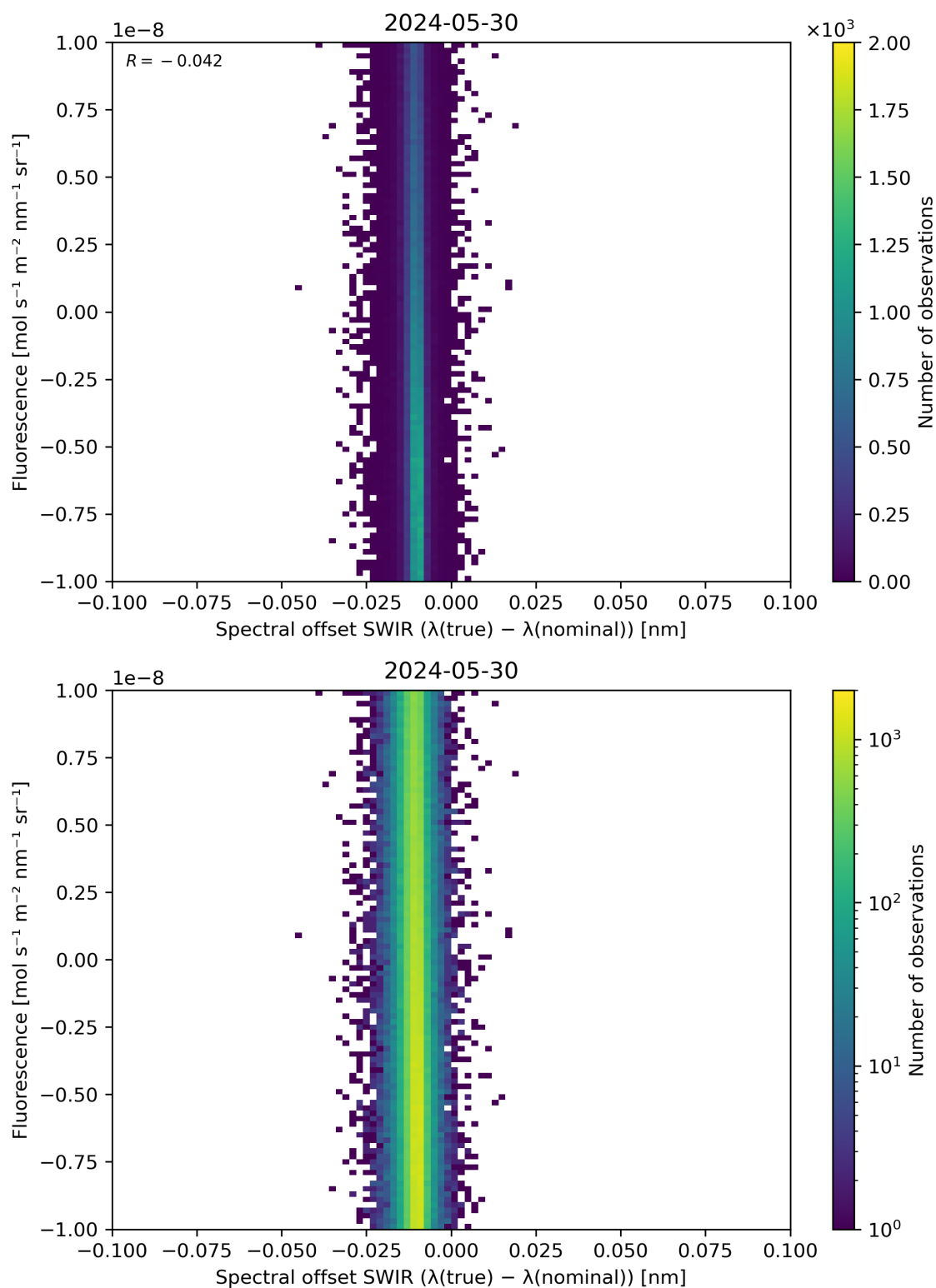
Figure 120: Scatter density plot of “Spectral offset SWIR ( \lambda(\text{true}) - \lambda(\text{nominal}) )” against “Fluorescence” for 2024-05-29 to 2024-05-31.
