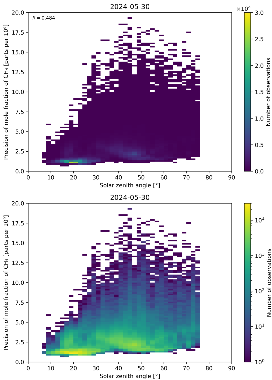
Figure 101: Scatter density plot of “Solar zenith angle” against “Precision of mole fraction of CH 4 ” for 2024-05-29 to 2024-05-31.
