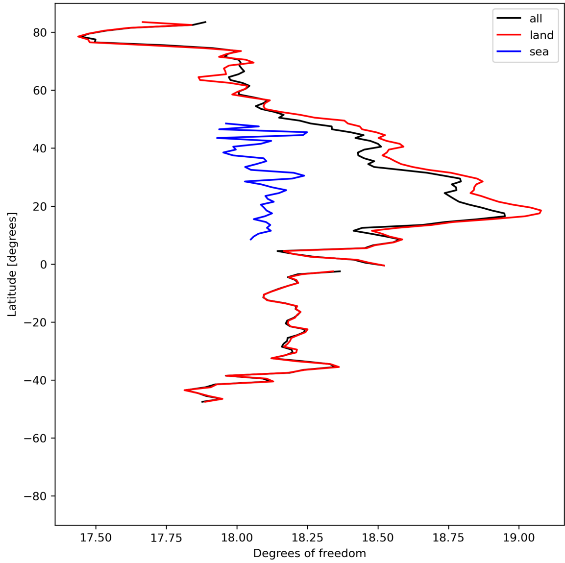
Figure 19: Zonal average of “Degrees of freedom” for 2024-05-29 to 2024-05-31.
