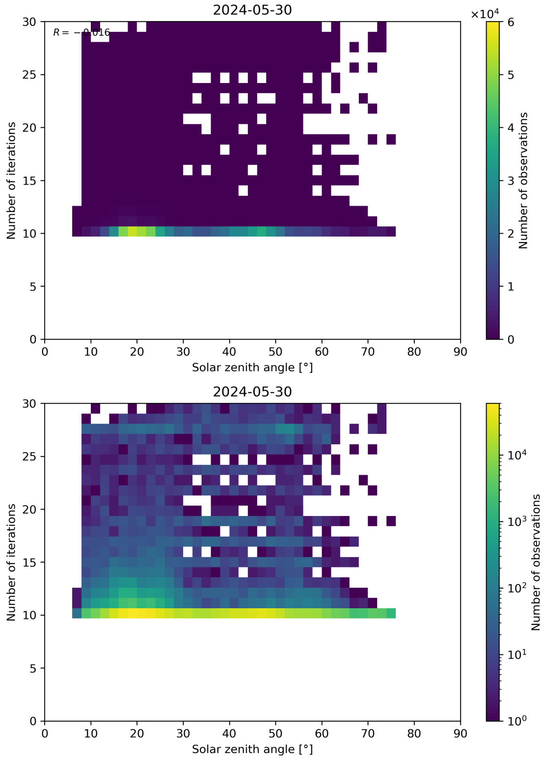
Figure 102: Scatter density plot of “Solar zenith angle” against “Number of iterations” for 2024-05-29 to 2024-05-31.
