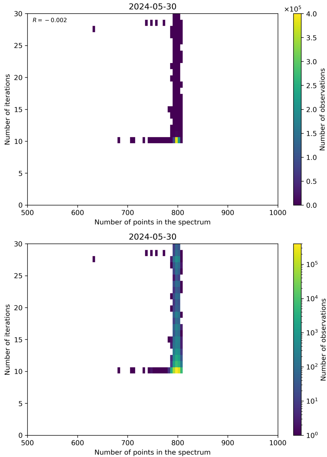
Figure 92: Scatter density plot of “Number of points in the spectrum” against “Number of iterations” for 2024-05-29 to 2024-05-31.
