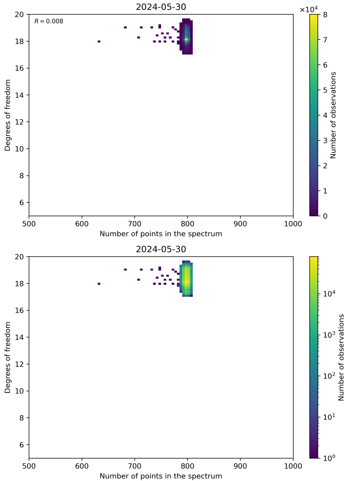
Figure 90: Scatter density plot of “Number of points in the spectrum” against “Degrees of freedom” for 2024-05-29 to 2024-05-31.
