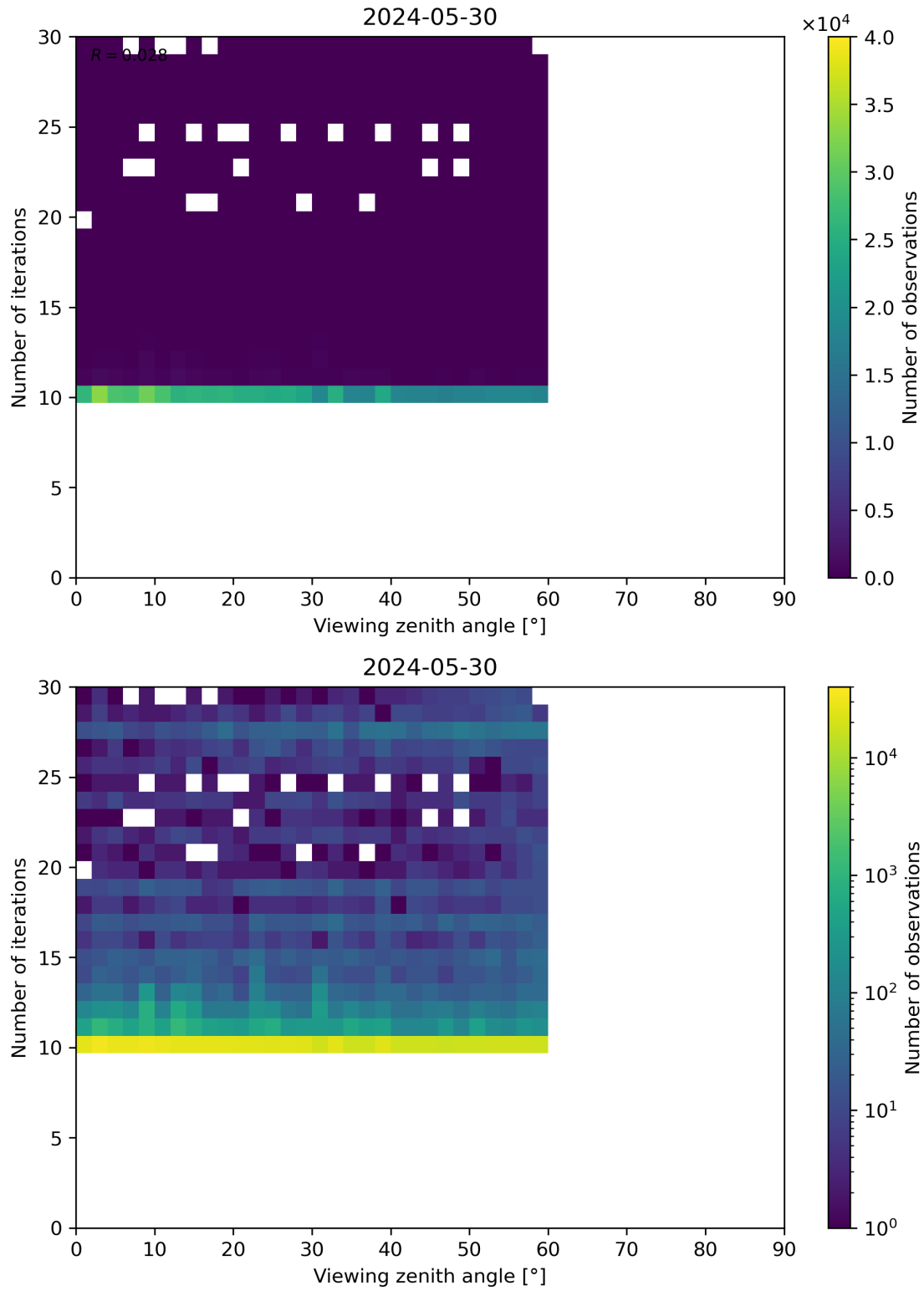
Figure 113: Scatter density plot of “Viewing zenith angle” against “Number of iterations” for 2024-05-29 to 2024-05-31.
