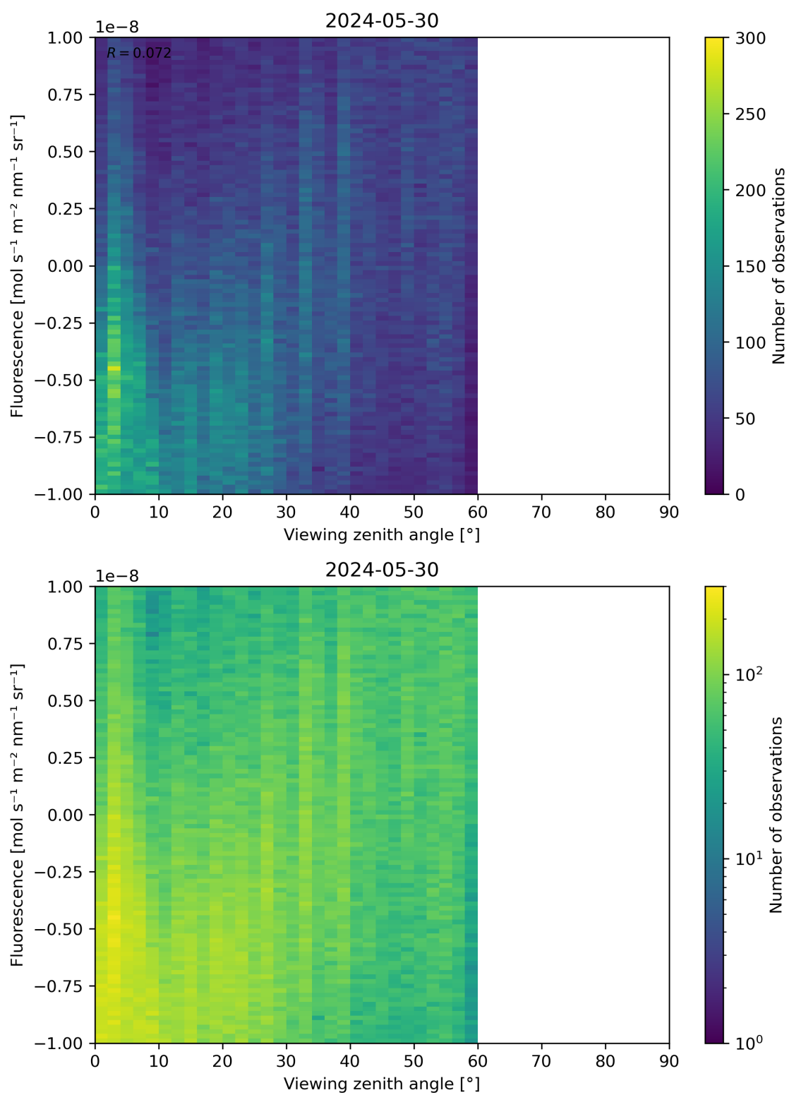
Figure 108: Scatter density plot of “Viewing zenith angle” against “Fluorescence” for 2024-05-29 to 2024-05-31.
