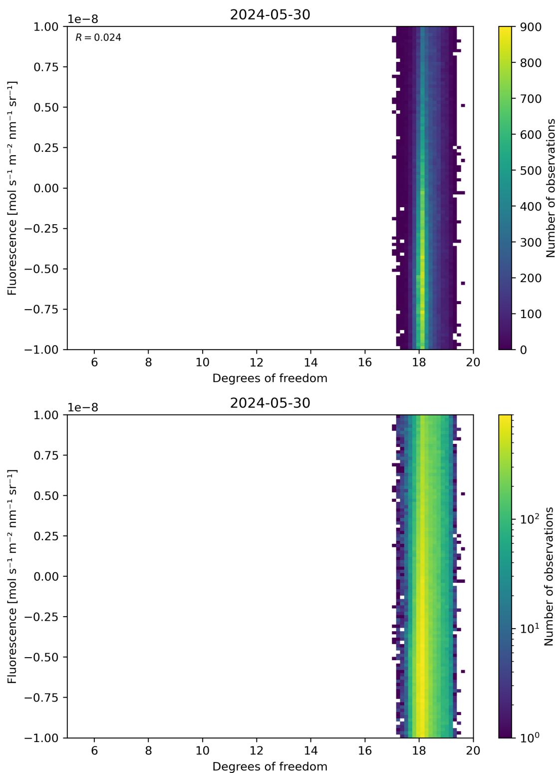
Figure 51: Scatter density plot of “Degrees of freedom” against “Fluorescence” for 2024-05-29 to 2024-05-31.
