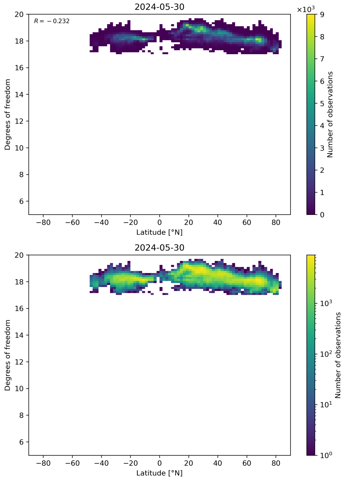
Figure 55: Scatter density plot of “Latitude” against “Degrees of freedom” for 2024-05-29 to 2024-05-31.
