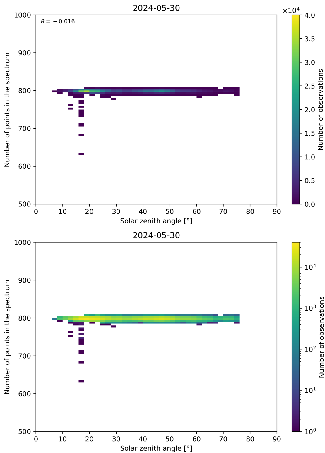
Figure 103: Scatter density plot of “Solar zenith angle” against “Number of points in the spectrum” for 2024-05-29 to 2024-05-31.
