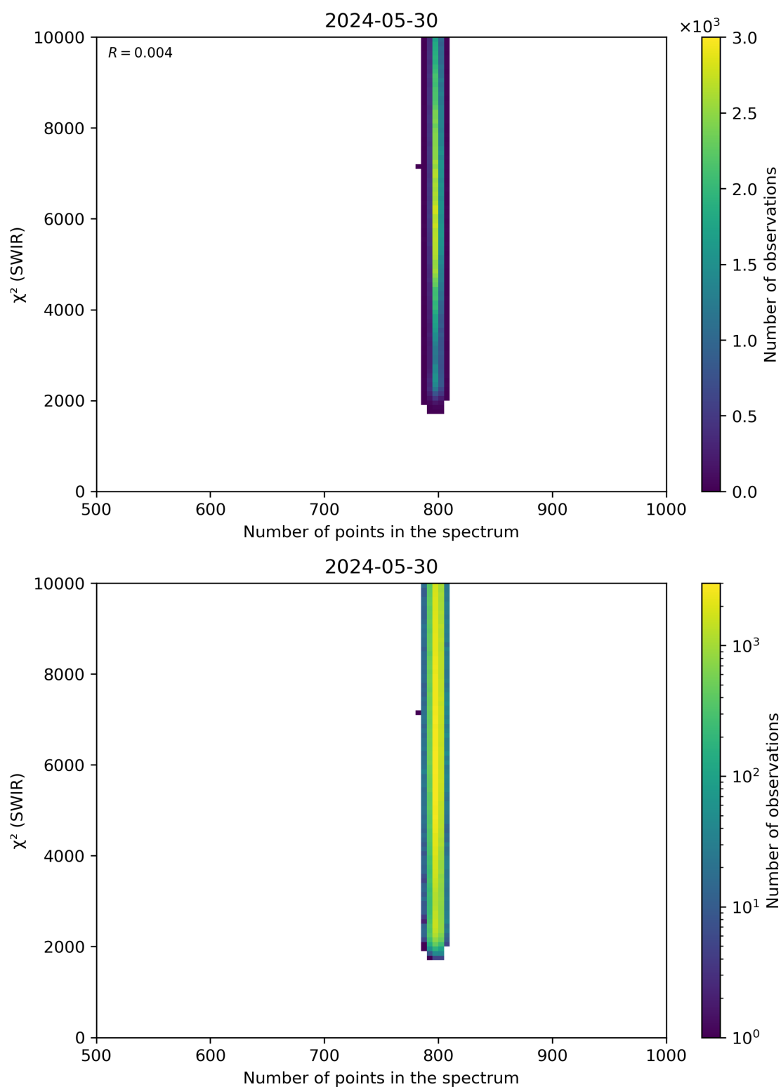
Figure 89: Scatter density plot of “Number of points in the spectrum” against “ \chi^2 (SWIR)” for 2024-05-29 to 2024-05-31.
