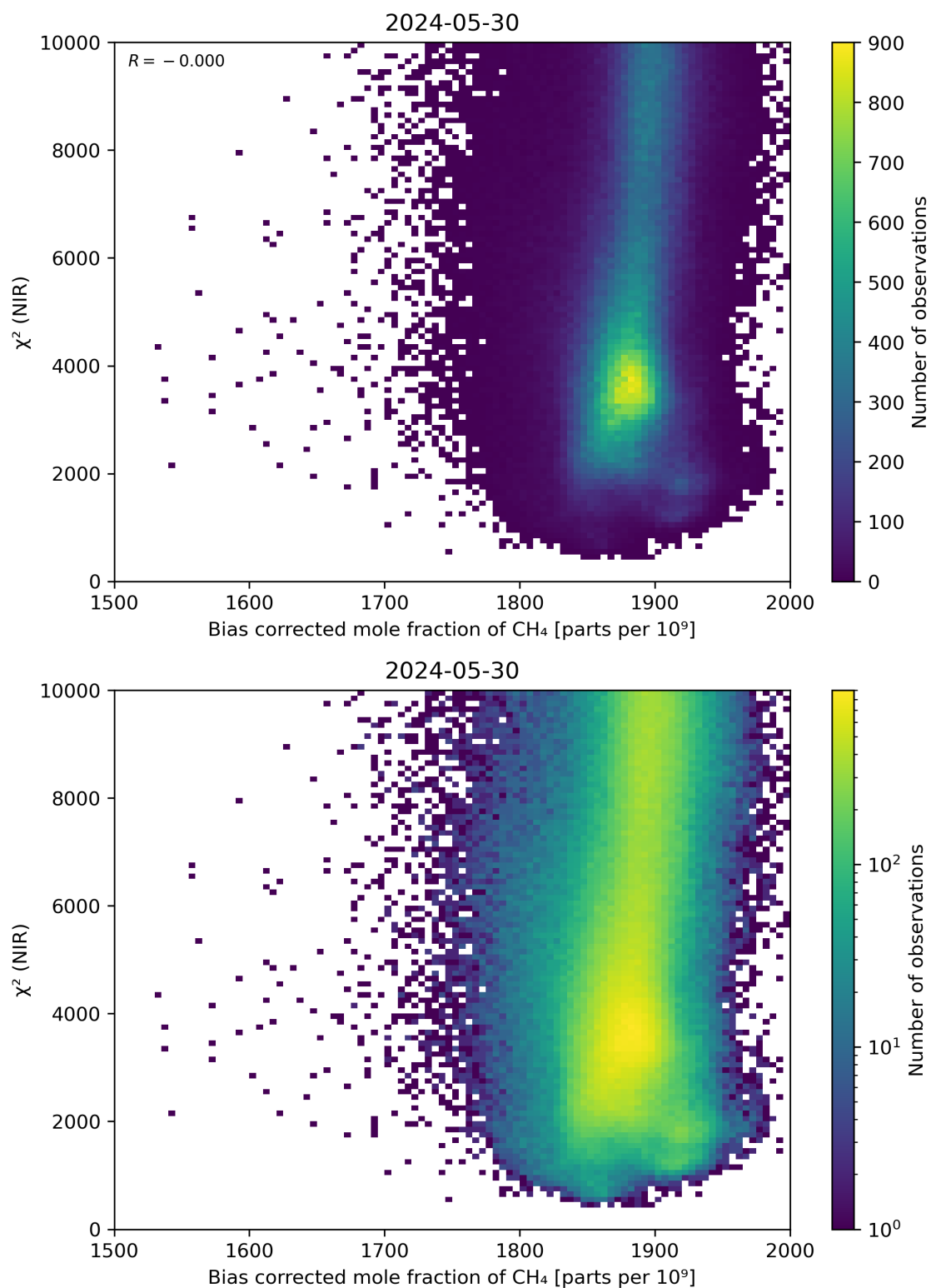
Figure 63: Scatter density plot of “Bias corrected mole fraction of CH 4 ” against “ \chi^2 (NIR)” for 2024-05-29 to 2024-05-31.
