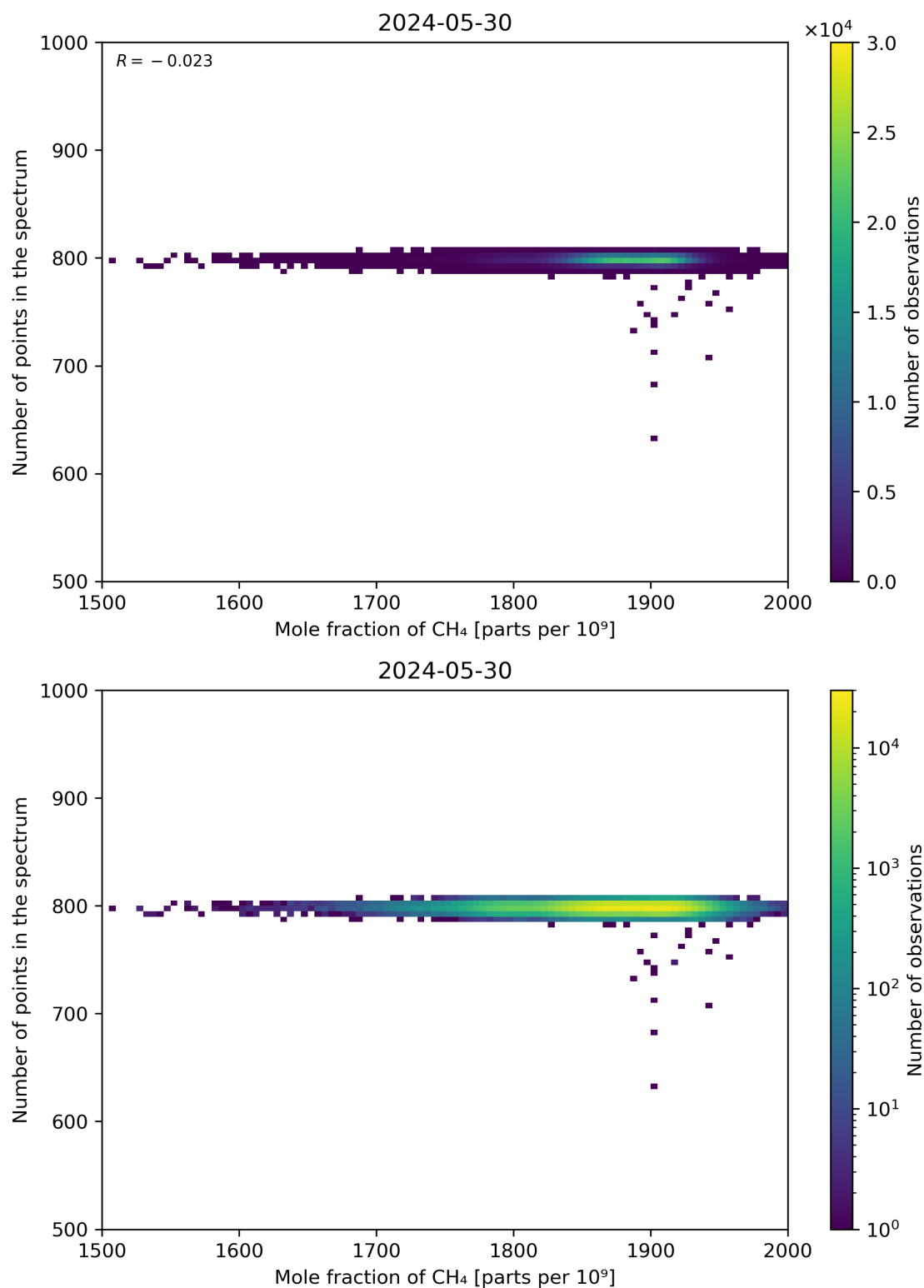
Figure 77: Scatter density plot of “Mole fraction of CH 4 ” against “Number of points in the spectrum” for 2024-05-29 to 2024-05-31.
