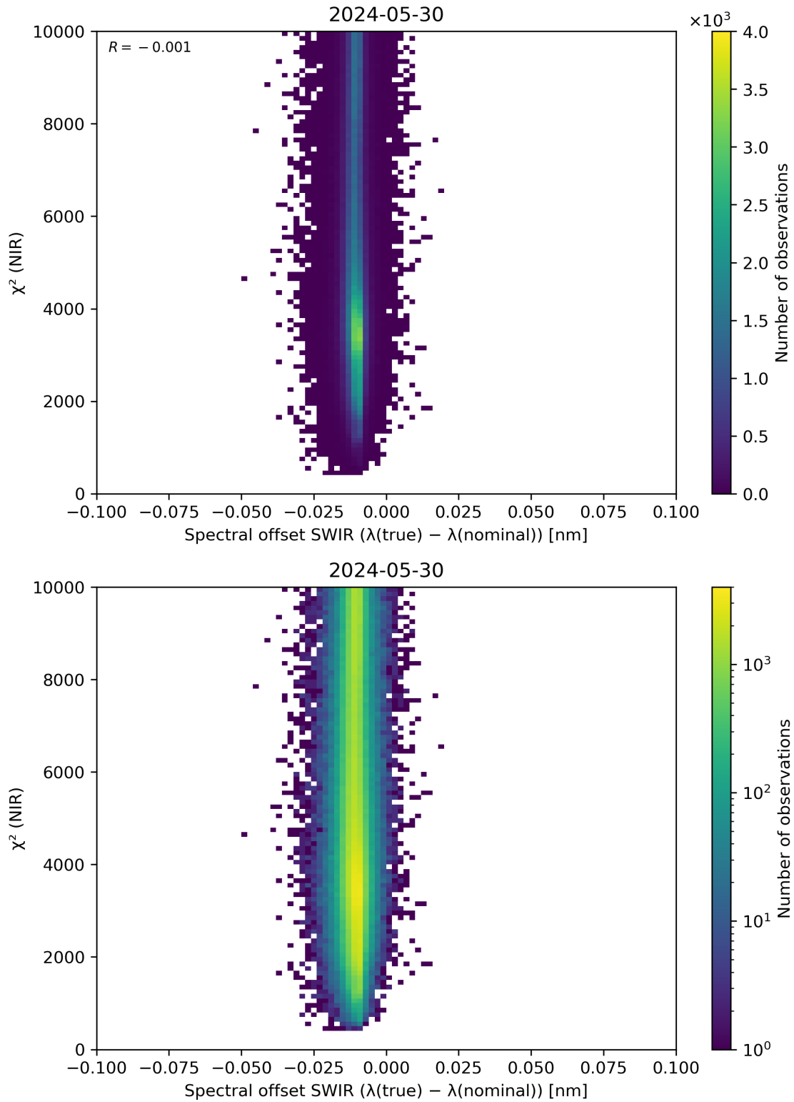
Figure 117: Scatter density plot of “Spectral offset SWIR ( \lambda(\text{true}) - \lambda(\text{nominal}) )” against “ \chi^2 (NIR)” for 2024-05-29 to 2024-05-31.
