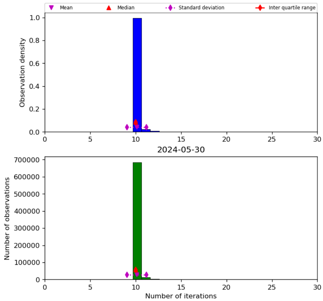
Figure 31: Histogram of “Number of iterations” for 2024-05-29 to 2024-05-31
