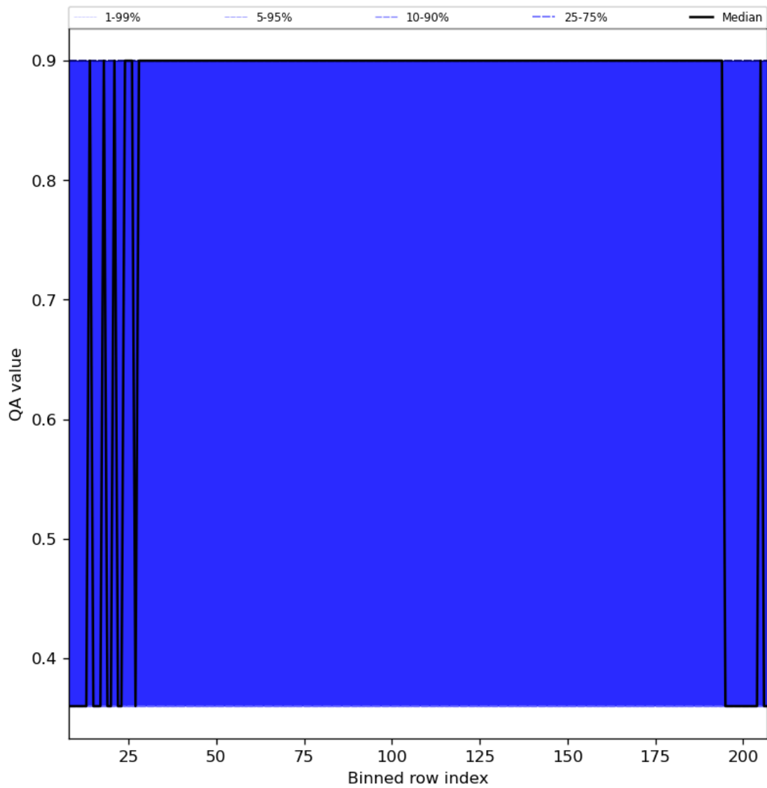
Figure 33: Along track statistics of “QA value” for 2024-05-29 to 2024-05-31
