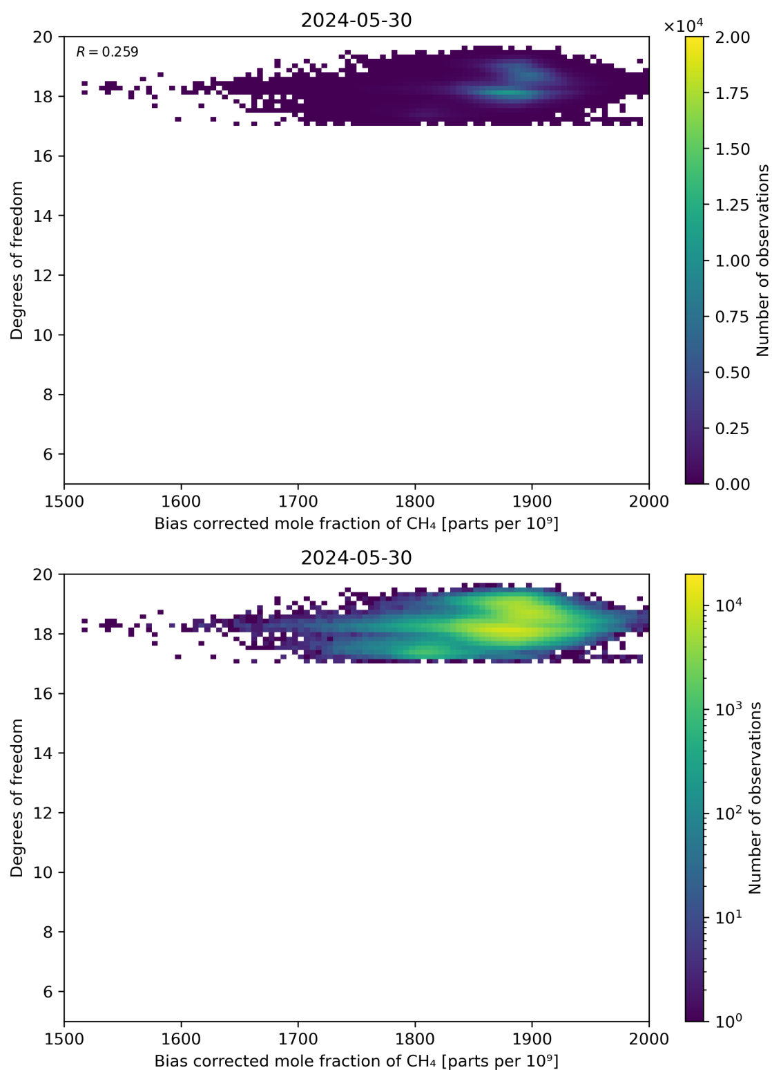
Figure 65: Scatter density plot of “Bias corrected mole fraction of CH 4 ” against “Degrees of freedom” for 2024-05-29 to 2024-05-31.
