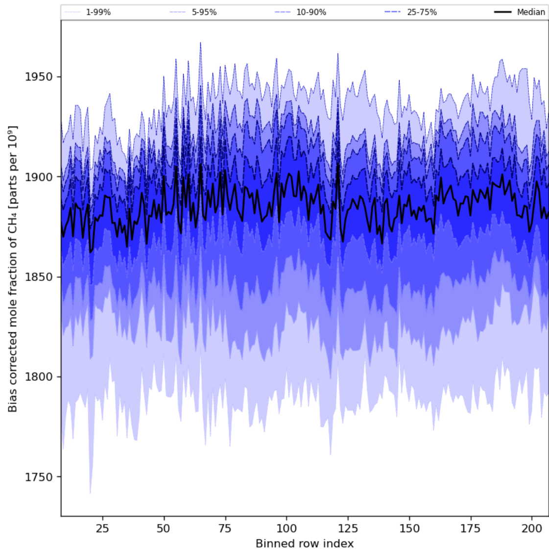
Figure 36: Along track statistics of “Bias corrected mole fraction of CH 4 ” for 2024-05-29 to 2024-05-31
