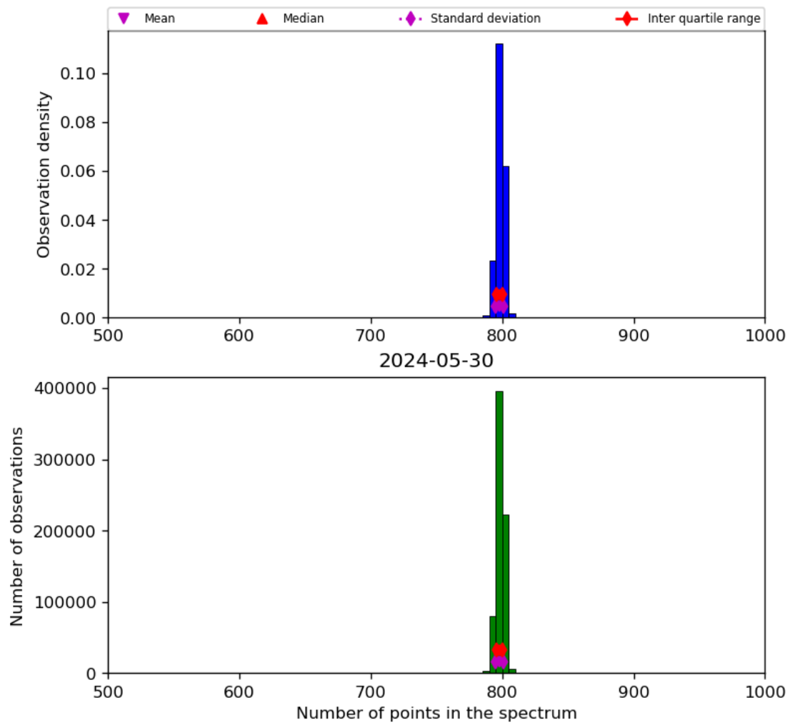
Figure 26: Histogram of “Number of points in the spectrum” for 2024-05-29 to 2024-05-31
