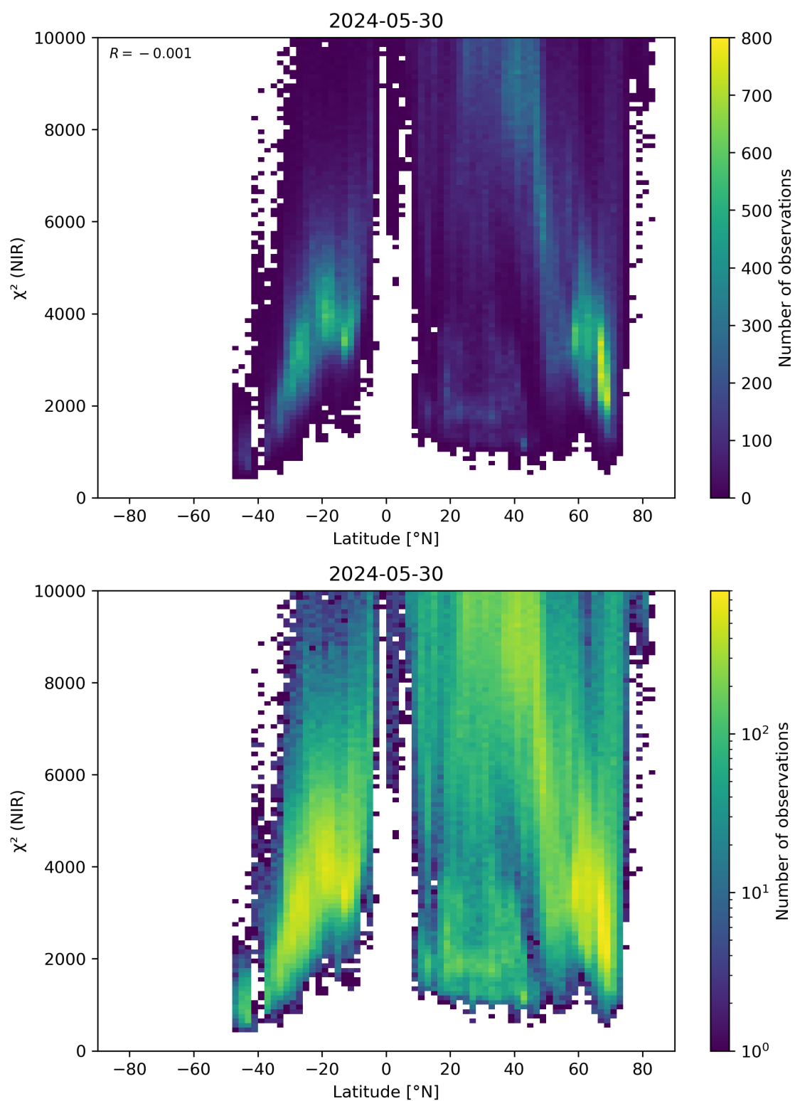
Figure 53: Scatter density plot of “Latitude” against “ \chi^2 (NIR)” for 2024-05-29 to 2024-05-31.
