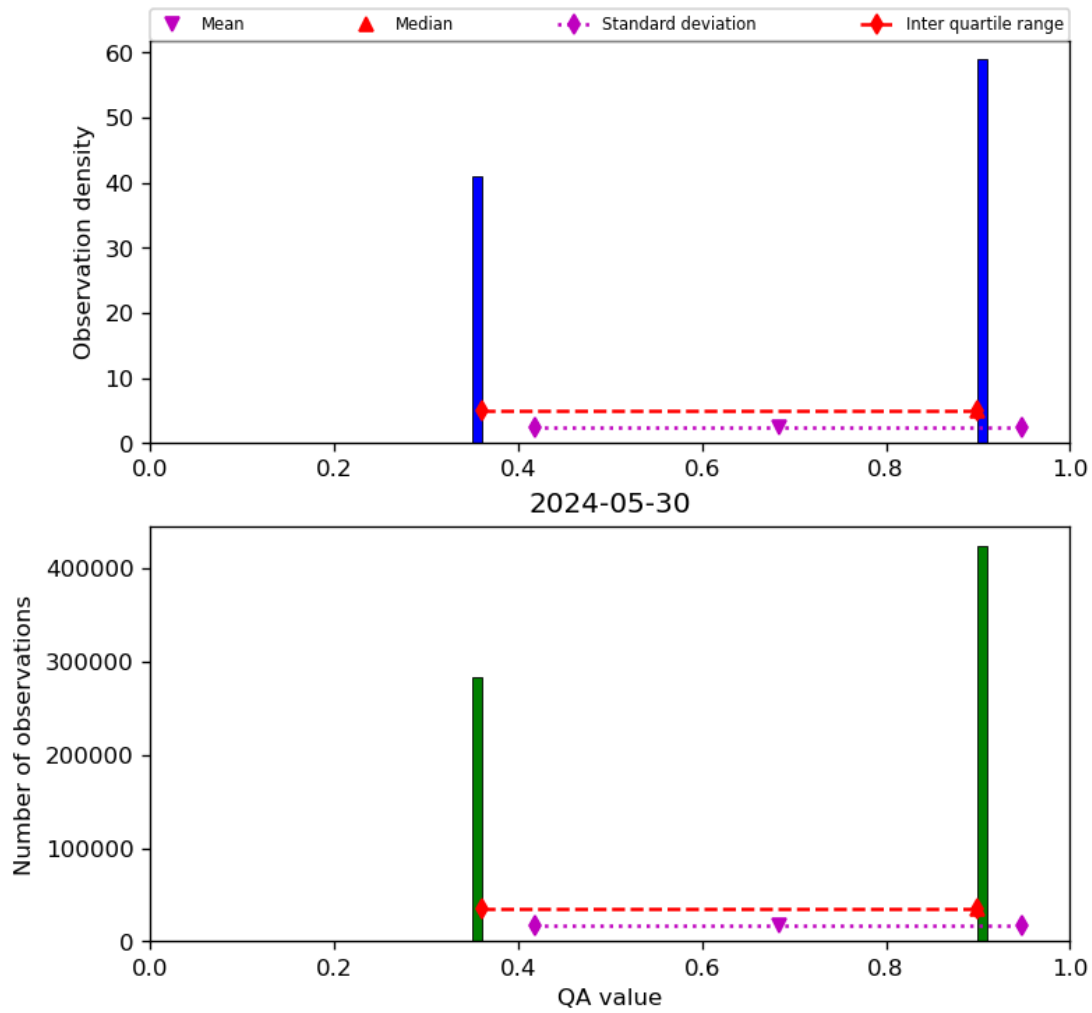
Figure 22: Histogram of “QA value” for 2024-05-29 to 2024-05-31
