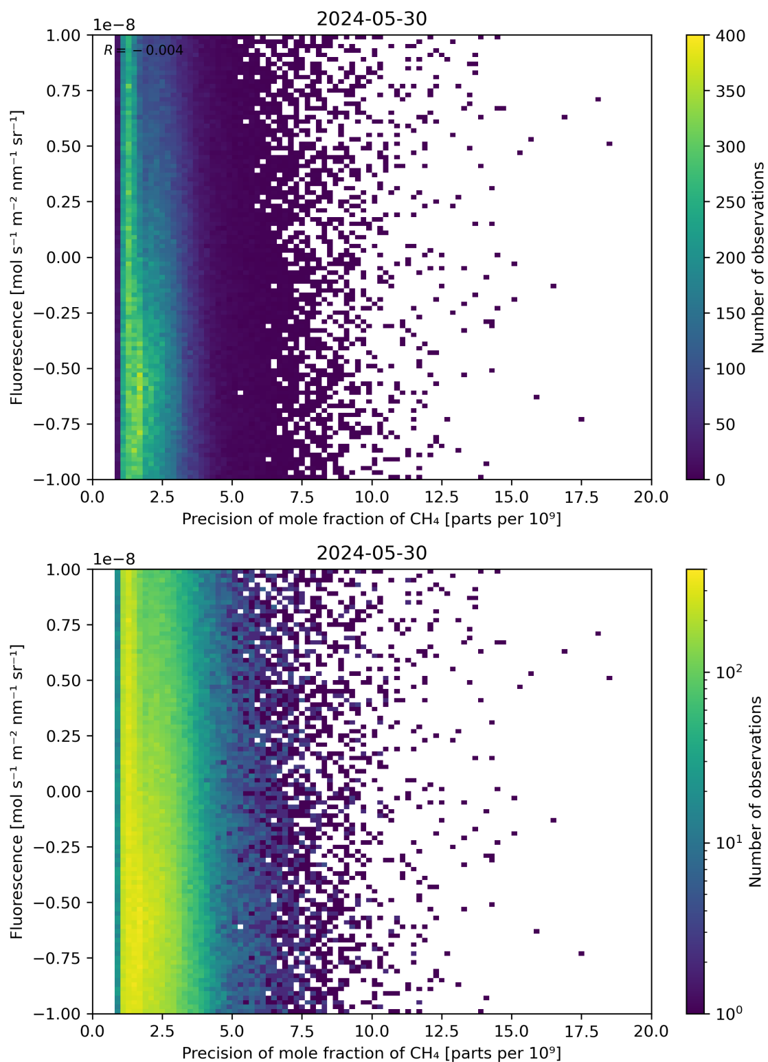
Figure 81: Scatter density plot of “Precision of mole fraction of \text{CH}_4 ” against “Fluorescence” for 2024-05-29 to 2024-05-31.
