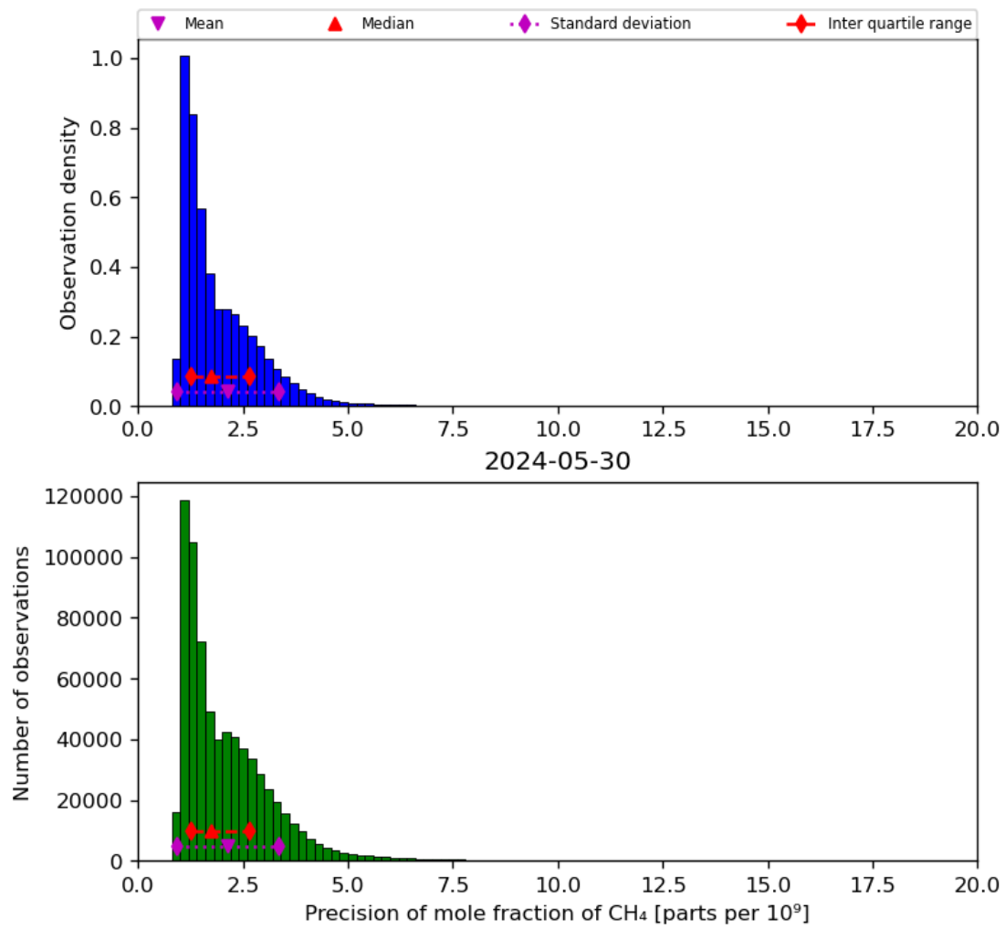
Figure 24: Histogram of “Precision of mole fraction of CH 4 ” for 2024-05-29 to 2024-05-31
