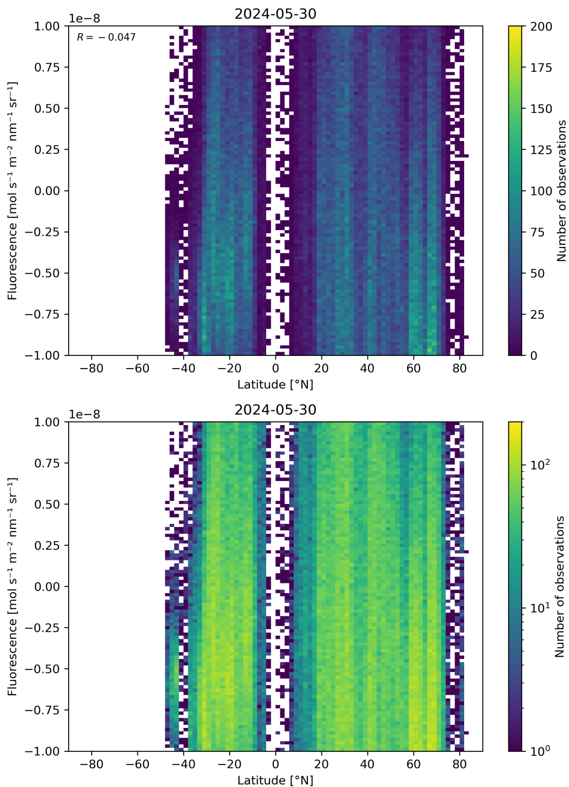
Figure 56: Scatter density plot of “Latitude” against “Fluorescence” for 2024-05-29 to 2024-05-31.
