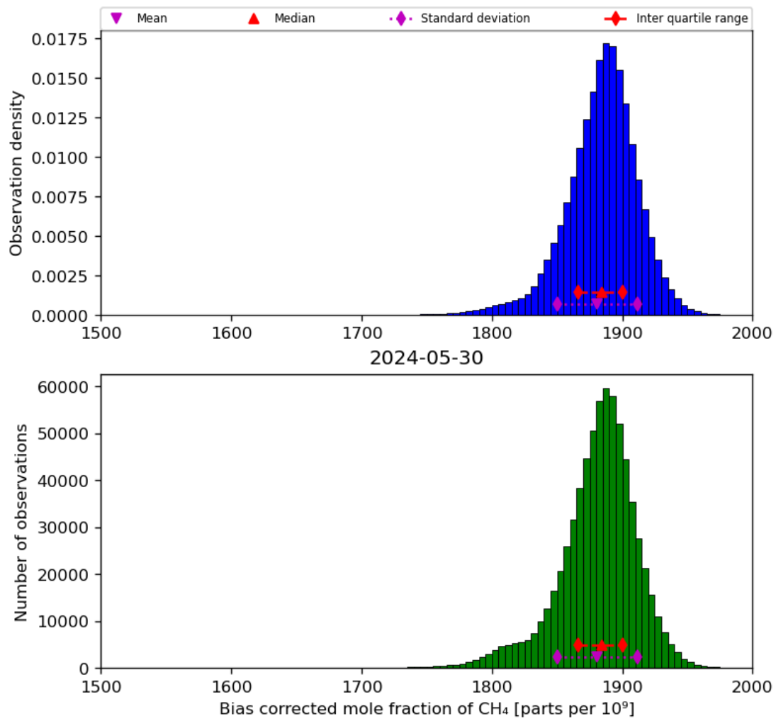
Figure 25: Histogram of “Bias corrected mole fraction of CH 4 ” for 2024-05-29 to 2024-05-31
