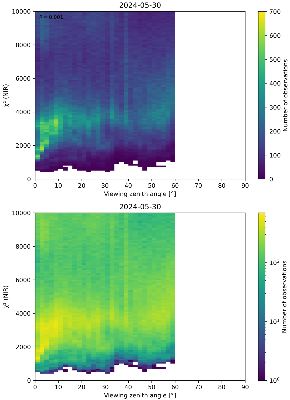
Figure 105: Scatter density plot of “Viewing zenith angle” against “ \chi^2 (NIR)” for 2024-05-29 to 2024-05-31.
