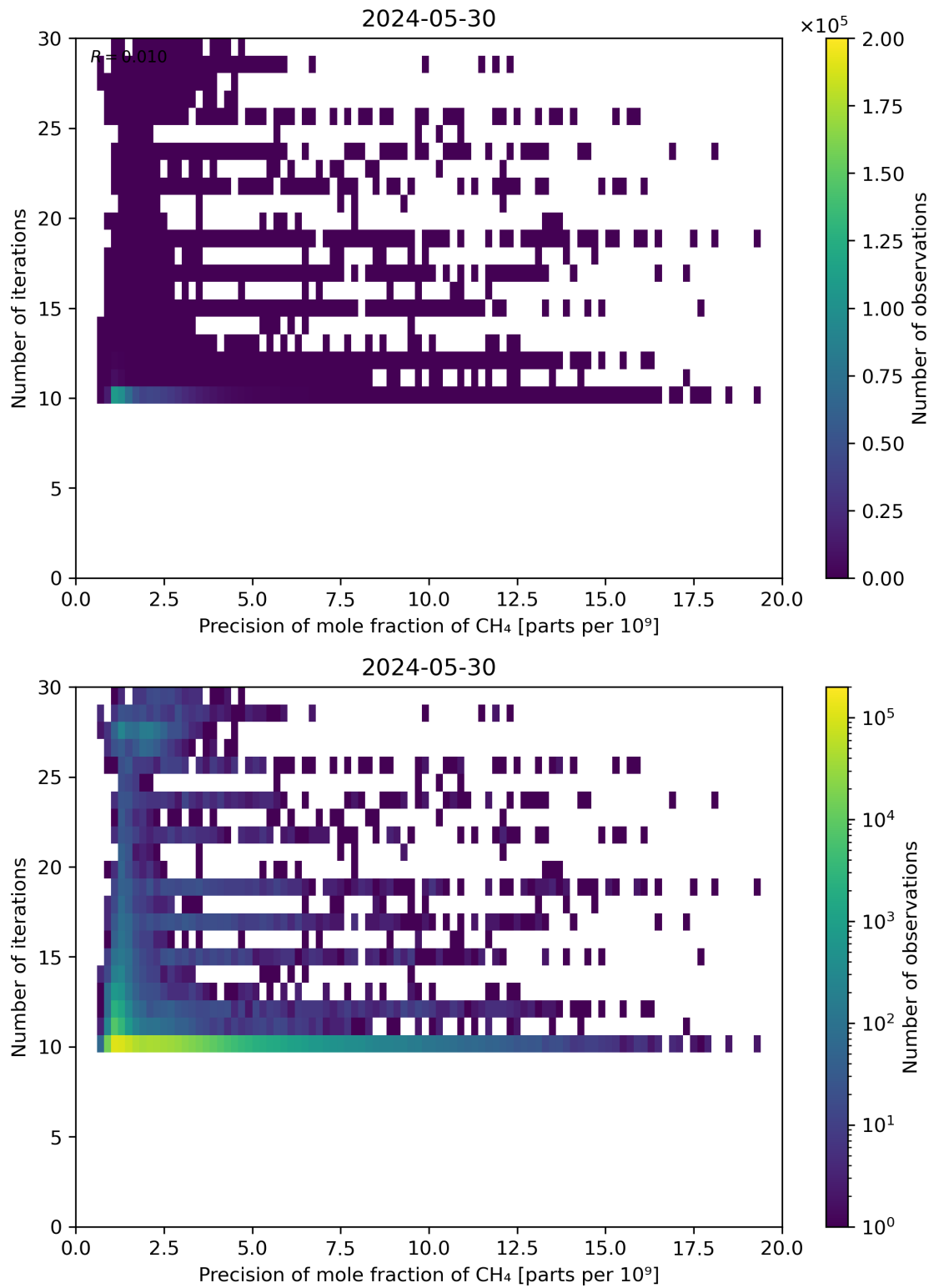
Figure 83: Scatter density plot of “Precision of mole fraction of CH 4 ” against “Number of iterations” for 2024-05-29 to 2024-05-31.
