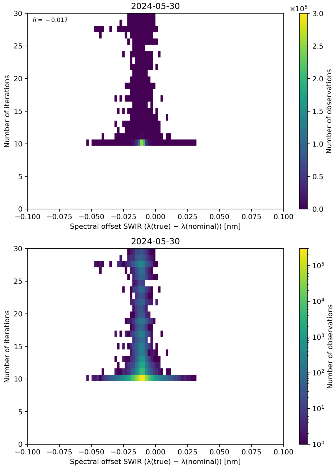
Figure 121: Scatter density plot of “Spectral offset SWIR ( \lambda(\text{true}) - \lambda(\text{nominal}) )” against “Number of iterations” for 2024-05-29 to 2024-05-31.
