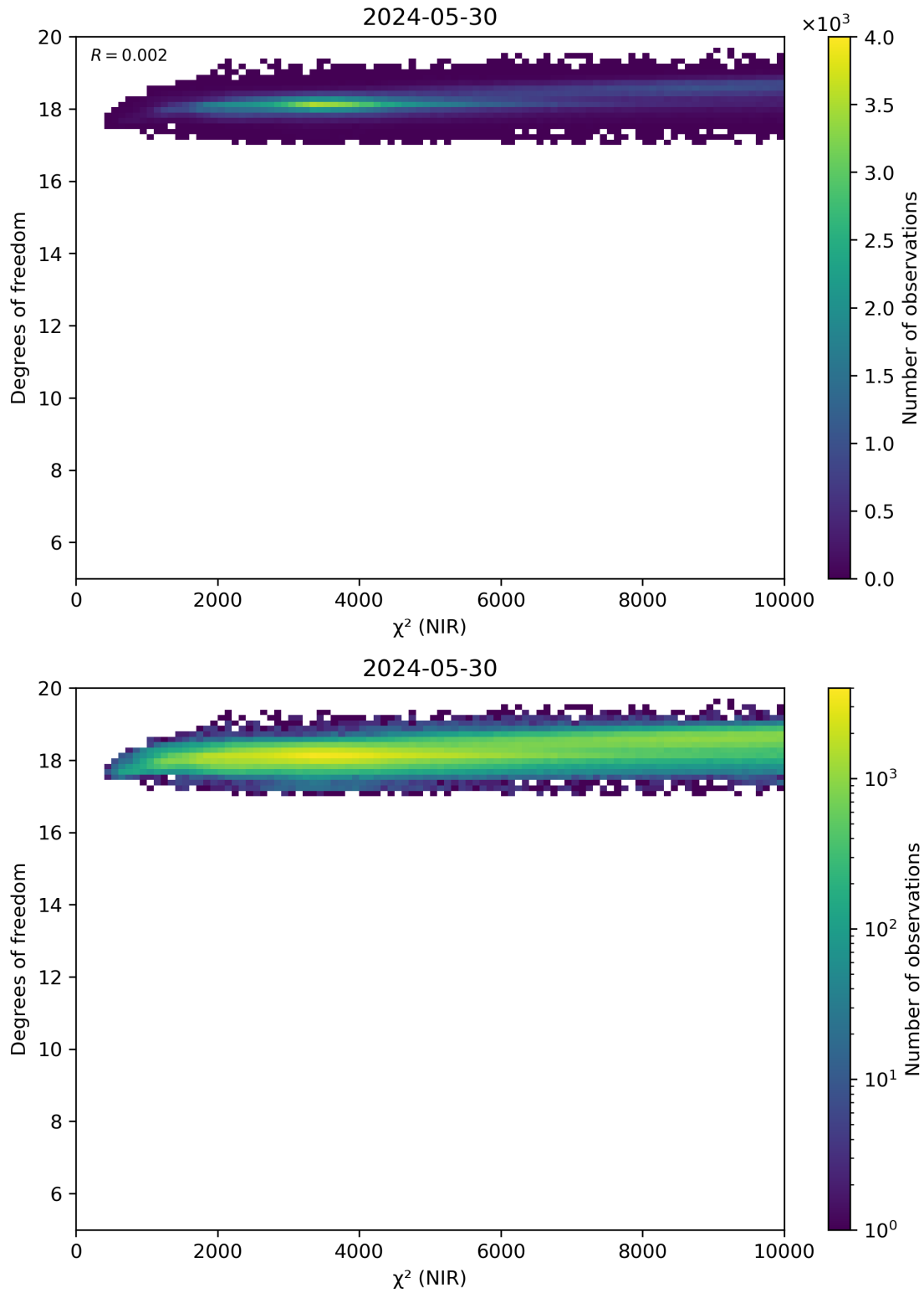
Figure 44: Scatter density plot of “ \chi^2 (NIR)” against “Degrees of freedom” for 2024-05-29 to 2024-05-31.
