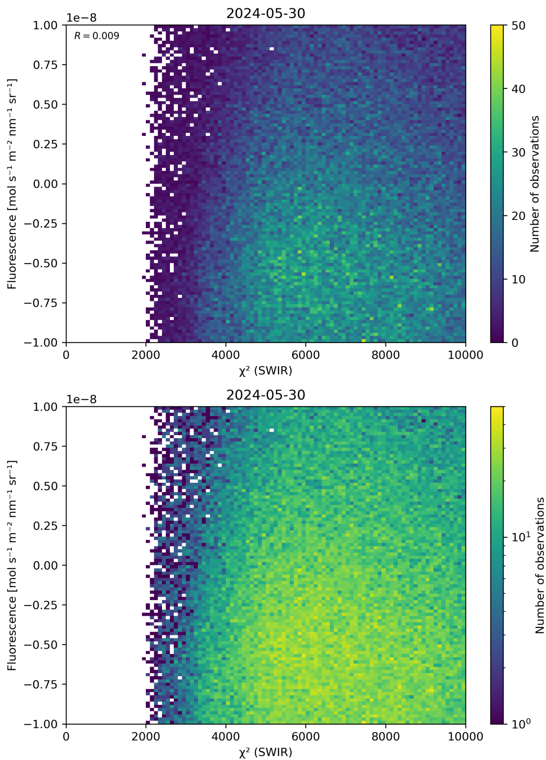
Figure 49: Scatter density plot of “ \chi^2 (SWIR)” against “Fluorescence” for 2024-05-29 to 2024-05-31.
