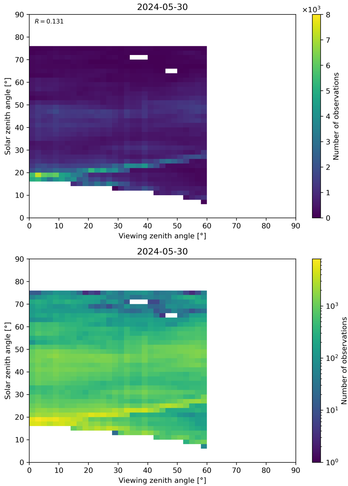
Figure 115: Scatter density plot of “Viewing zenith angle” against “Solar zenith angle” for 2024-05-29 to 2024-05-31.
