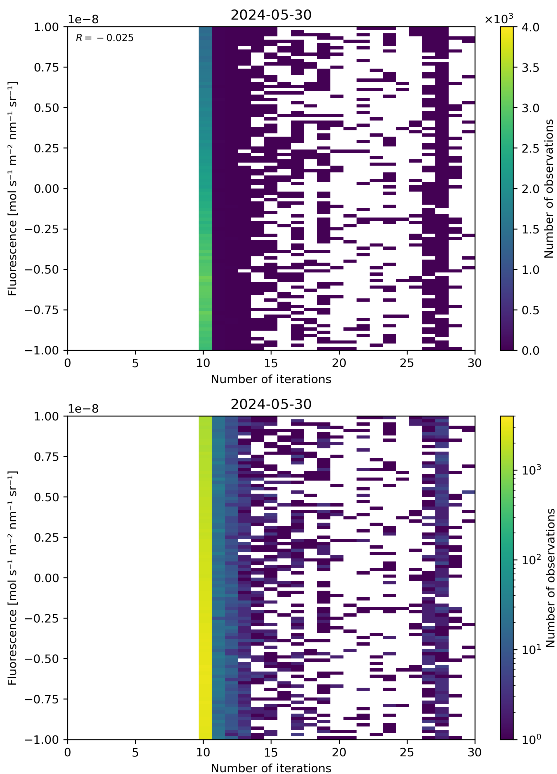
Figure 87: Scatter density plot of “Number of iterations” against “Fluorescence” for 2024-05-29 to 2024-05-31.
