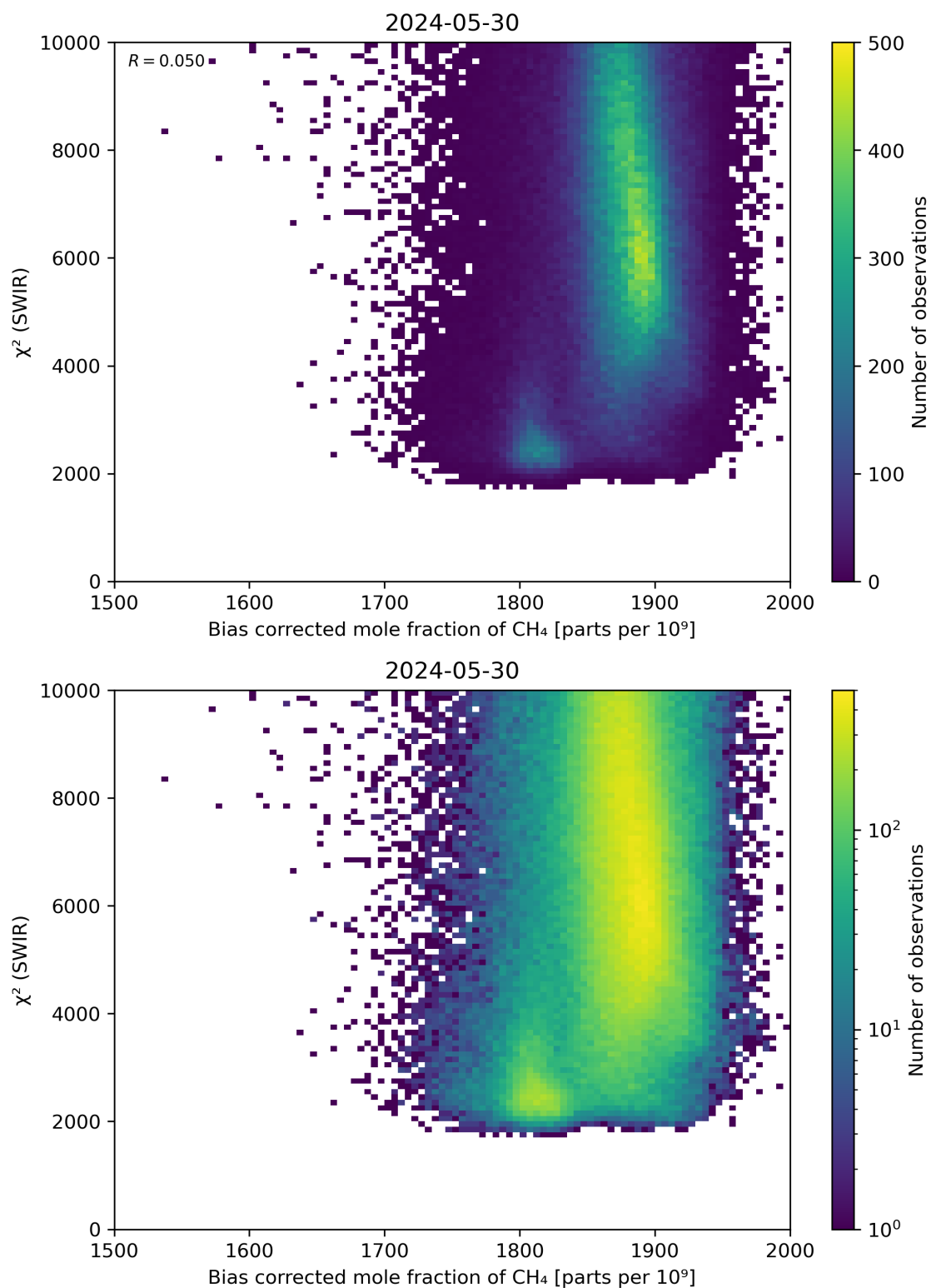
Figure 64: Scatter density plot of “Bias corrected mole fraction of \text{CH}_4 ” against “ \chi^2 (SWIR)” for 2024-05-29 to 2024-05-31.
