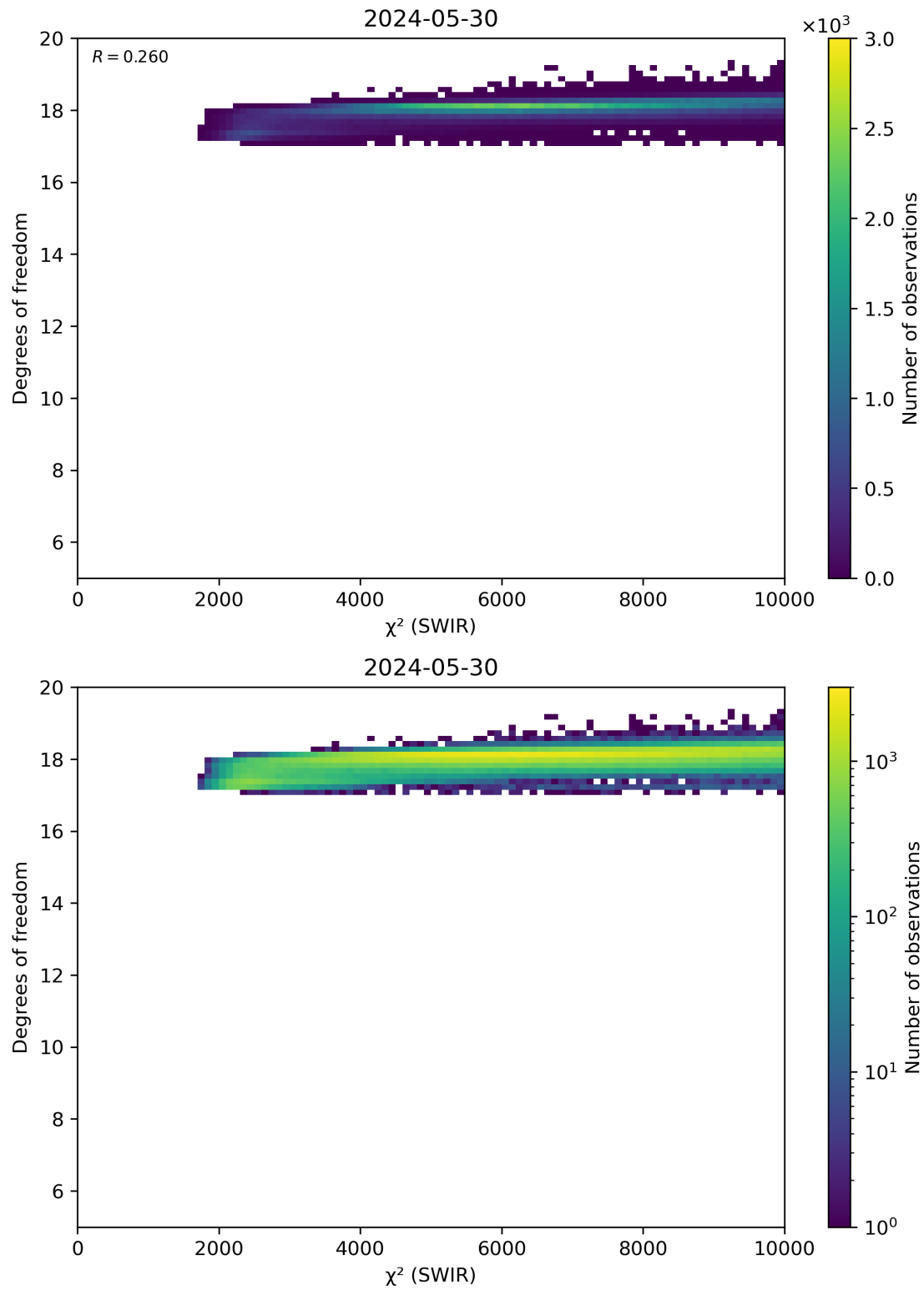
Figure 48: Scatter density plot of “ \chi^2 (SWIR)” against “Degrees of freedom” for 2024-05-29 to 2024-05-31.
