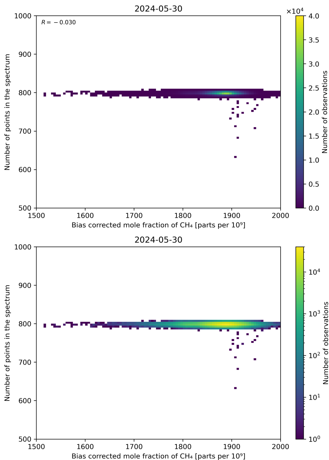
Figure 68: Scatter density plot of “Bias corrected mole fraction of CH 4 ” against “Number of points in the spectrum” for 2024-05-29 to 2024-05-31.
