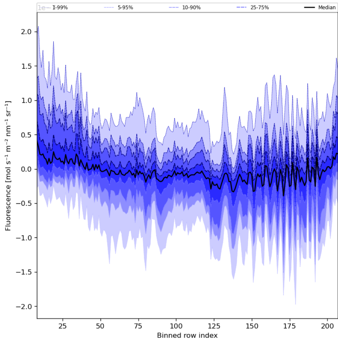
Figure 43: Along track statistics of “Fluorescence” for 2024-05-29 to 2024-05-31
