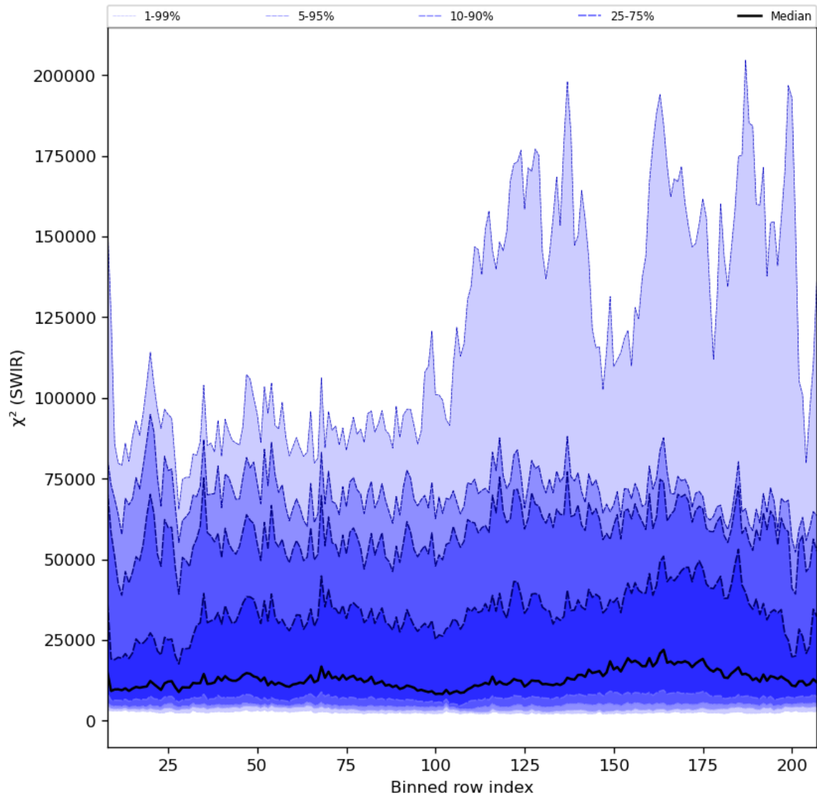
Figure 39: Along track statistics of “ \chi^2 (SWIR)” for 2024-05-29 to 2024-05-31
