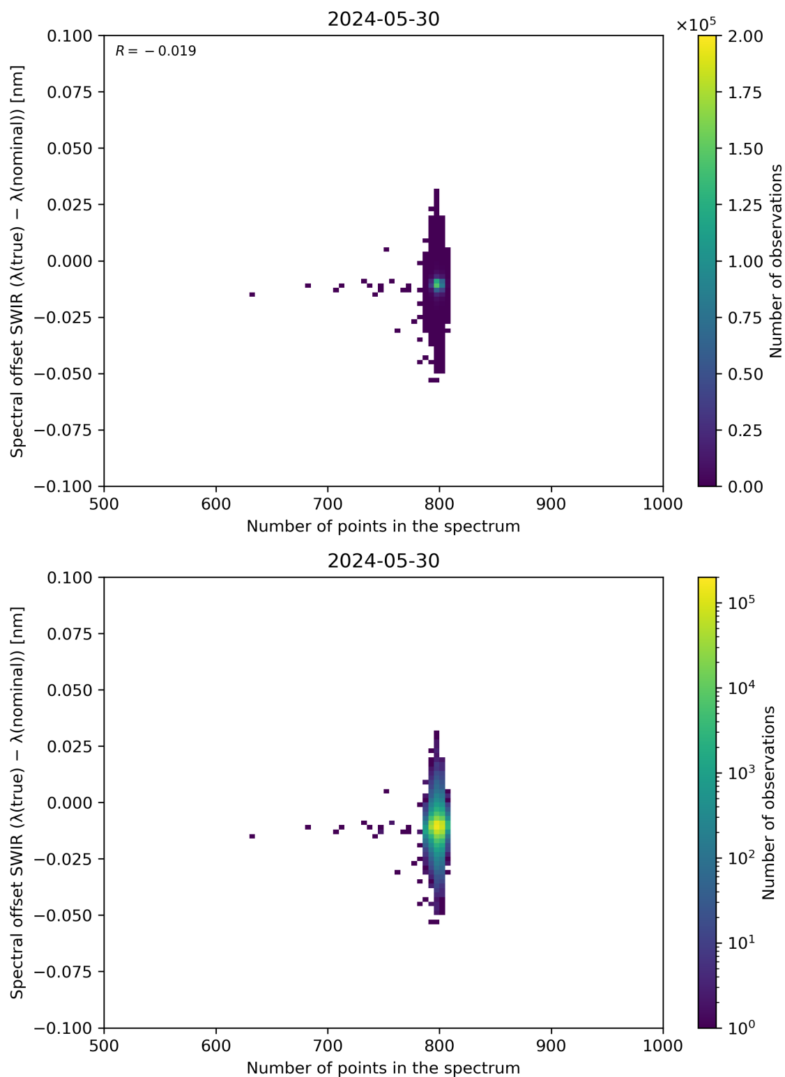
Figure 93: Scatter density plot of “Number of points in the spectrum” against “Spectral offset SWIR ( \lambda(\text{true}) - \lambda(\text{nominal}) )” for 2024-05-29 to 2024-05-31.
