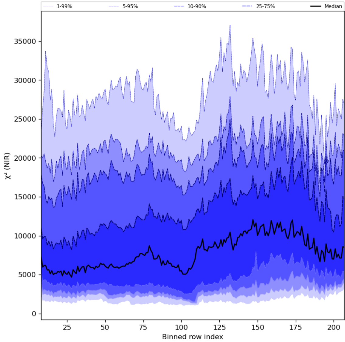
Figure 40: Along track statistics of “ \chi^2 (NIR)” for 2024-05-29 to 2024-05-31
