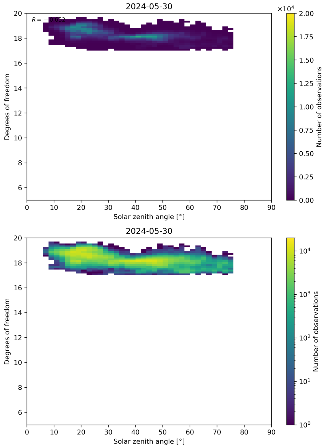
Figure 96: Scatter density plot of “Solar zenith angle” against “Degrees of freedom” for 2024-05-29 to 2024-05-31.
