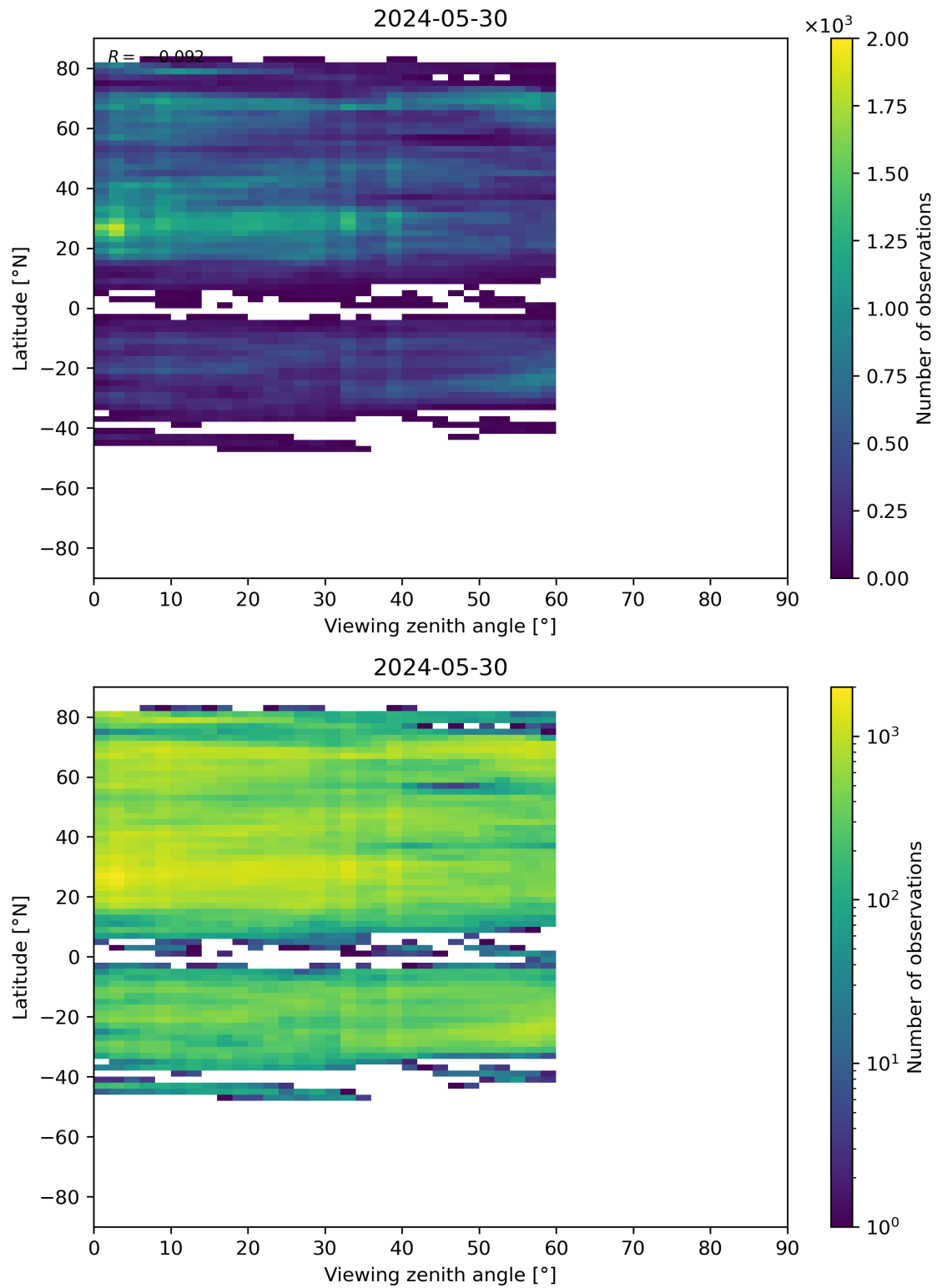
Figure 109: Scatter density plot of “Viewing zenith angle” against “Latitude” for 2024-05-29 to 2024-05-31.
