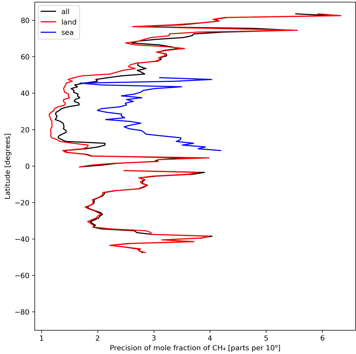
Figure 13: Zonal average of “Precision of mole fraction of CH 4 ” for 2024-05-29 to 2024-05-31.
