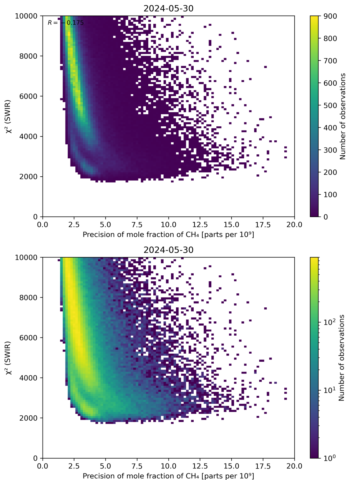
Figure 79: Scatter density plot of “Precision of mole fraction of \text{CH}_4 ” against “ \chi^2 (SWIR)” for 2024-05-29 to 2024-05-31.
