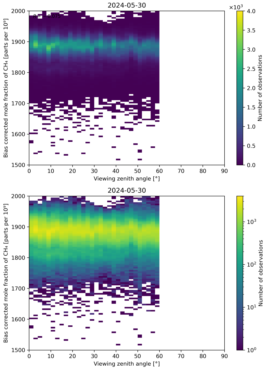
Figure 111: Scatter density plot of “Viewing zenith angle” against “Bias corrected mole fraction of CH 4 ” for 2024-05-29 to 2024-05-31.
