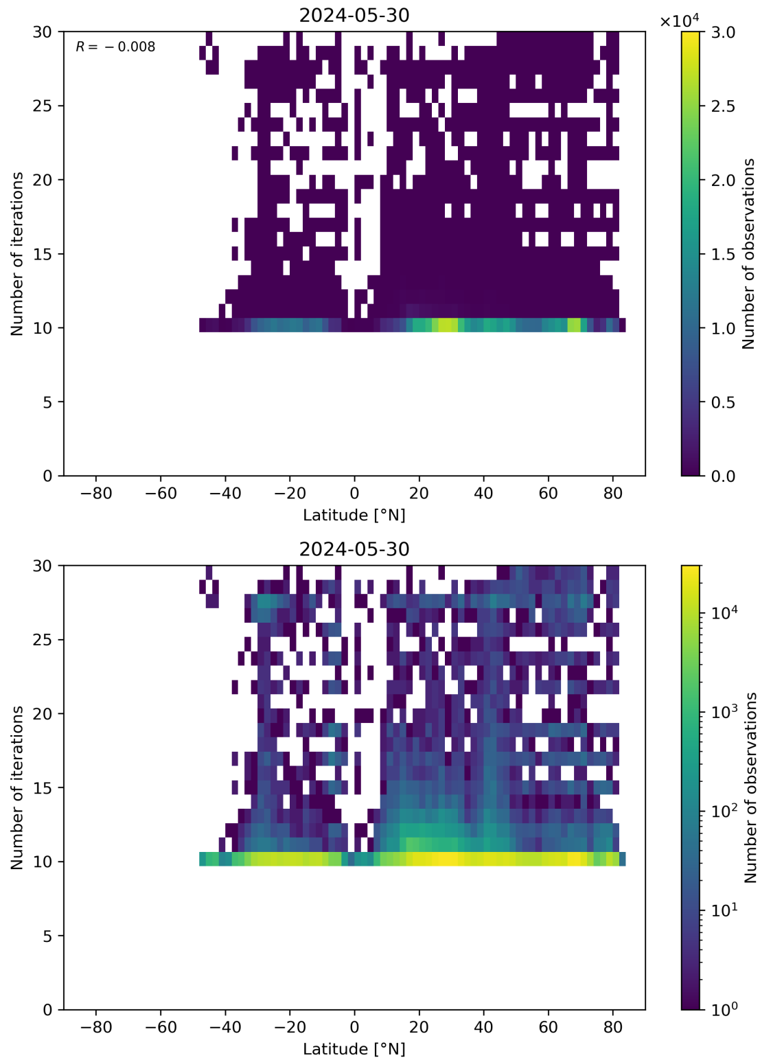
Figure 60: Scatter density plot of “Latitude” against “Number of iterations” for 2024-05-29 to 2024-05-31.
