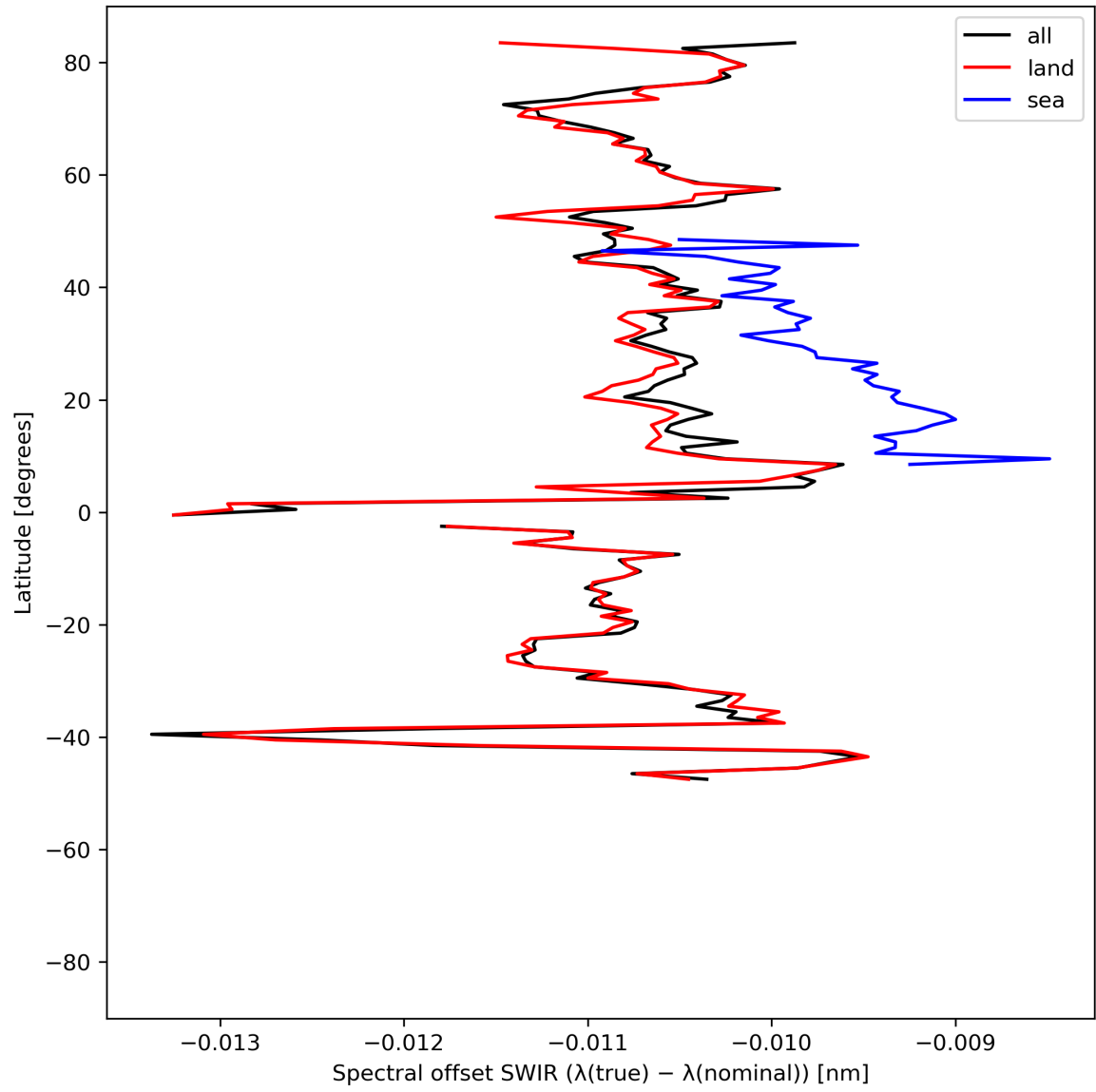
Figure 16: Zonal average of “Spectral offset SWIR ( \lambda(\text{true}) - \lambda(\text{nominal}) )” for 2024-05-29 to 2024-05-31.
