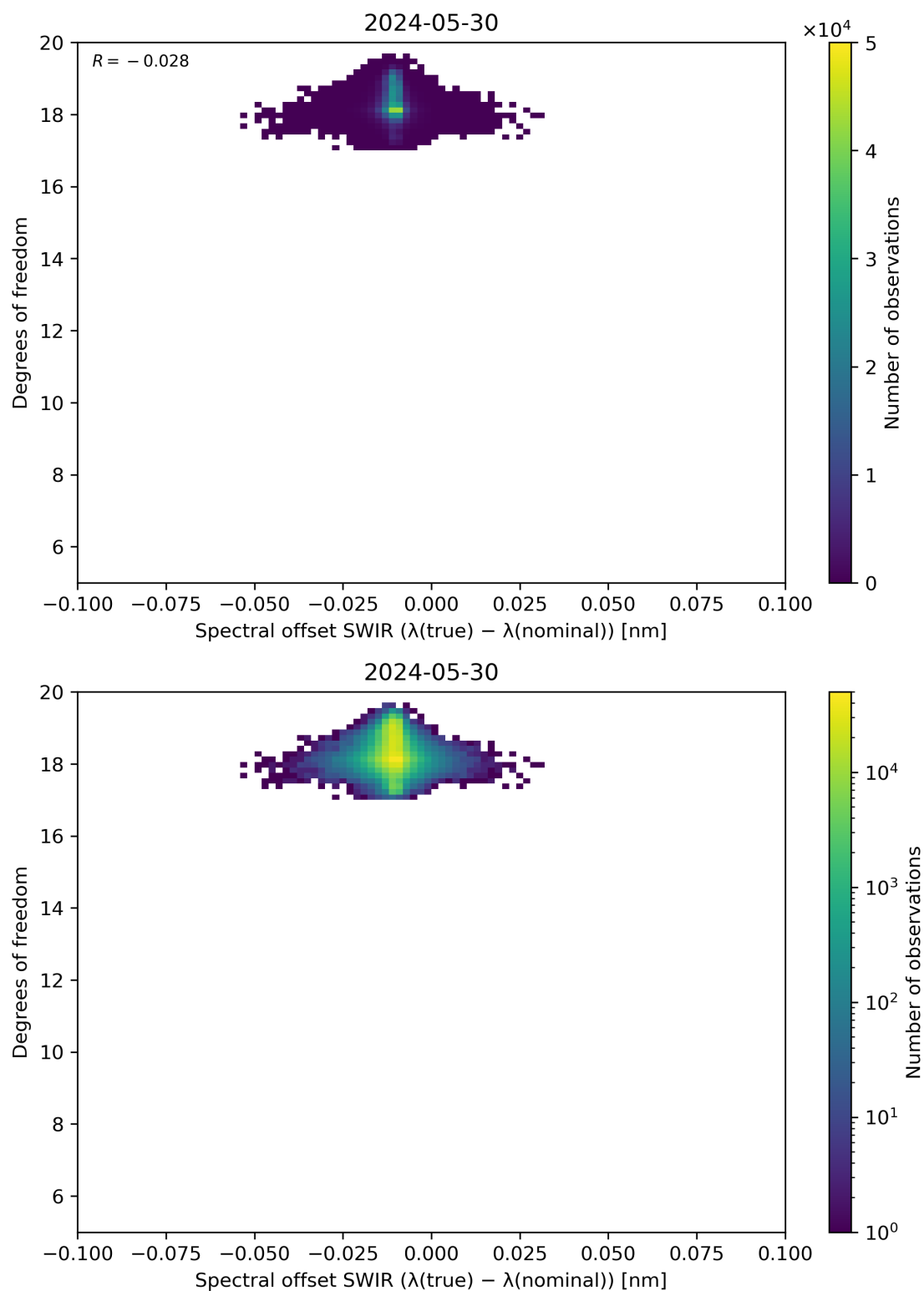
Figure 119: Scatter density plot of “Spectral offset SWIR ( \lambda(\text{true}) - \lambda(\text{nominal}) )” against “Degrees of freedom” for 2024-05-29 to 2024-05-31.
