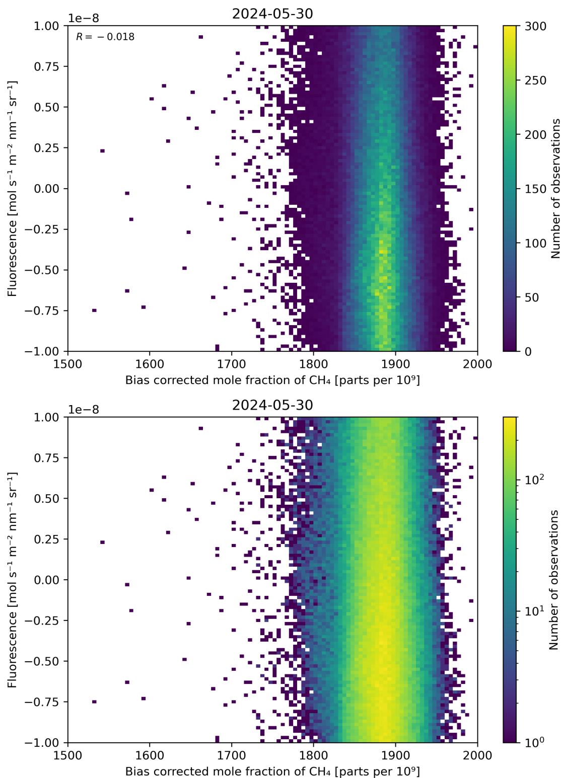
Figure 66: Scatter density plot of “Bias corrected mole fraction of \text{CH}_4 ” against “Fluorescence” for 2024-05-29 to 2024-05-31.
