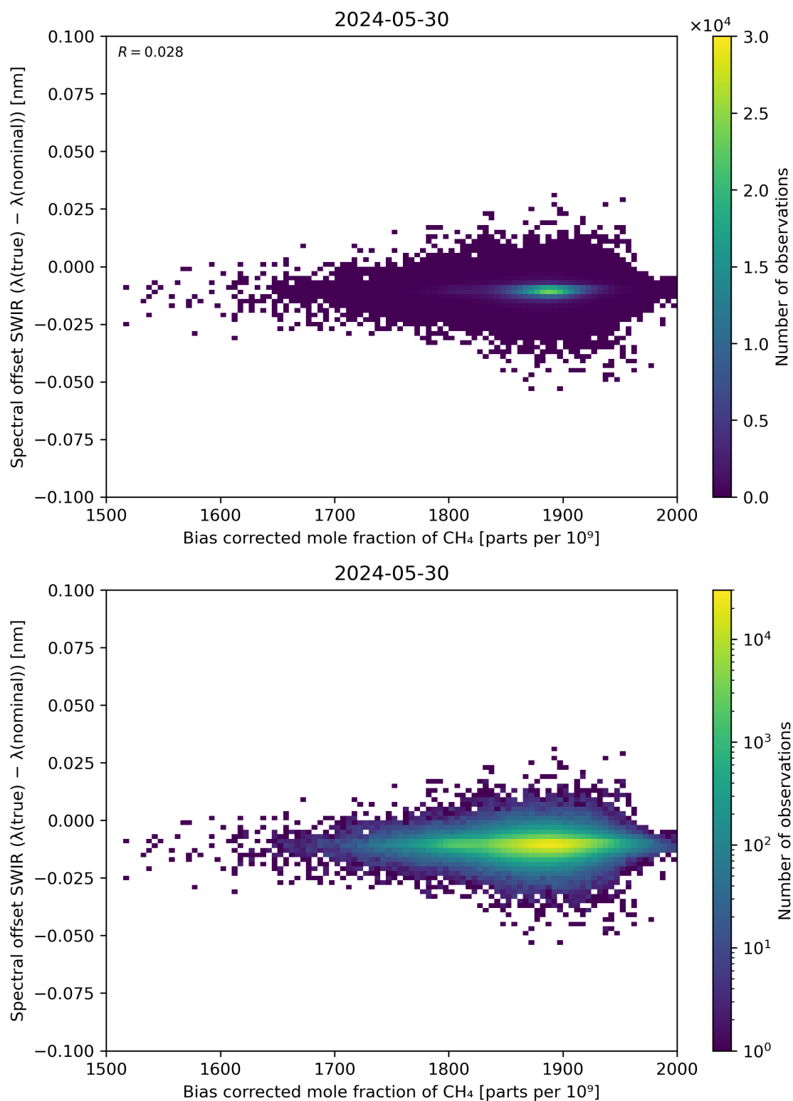
Figure 69: Scatter density plot of “Bias corrected mole fraction of \text{CH}_4 ” against “Spectral offset SWIR ( \lambda(\text{true}) - \lambda(\text{nominal}) )” for 2024-05-29 to 2024-05-31.
