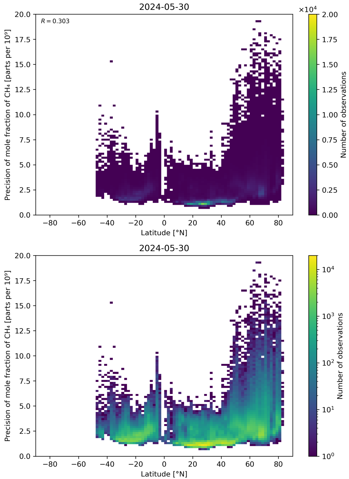
Figure 59: Scatter density plot of “Latitude” against “Precision of mole fraction of \text{CH}_4 ” for 2024-05-29 to 2024-05-31.
