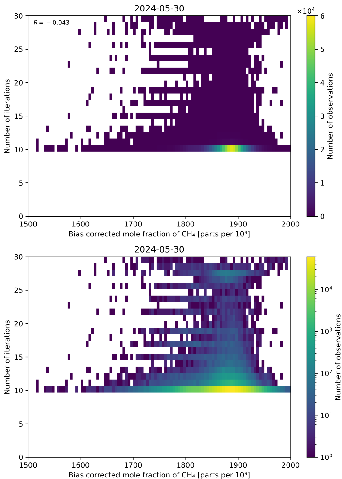
Figure 67: Scatter density plot of “Bias corrected mole fraction of CH 4 ” against “Number of iterations” for 2024-05-29 to 2024-05-31.
