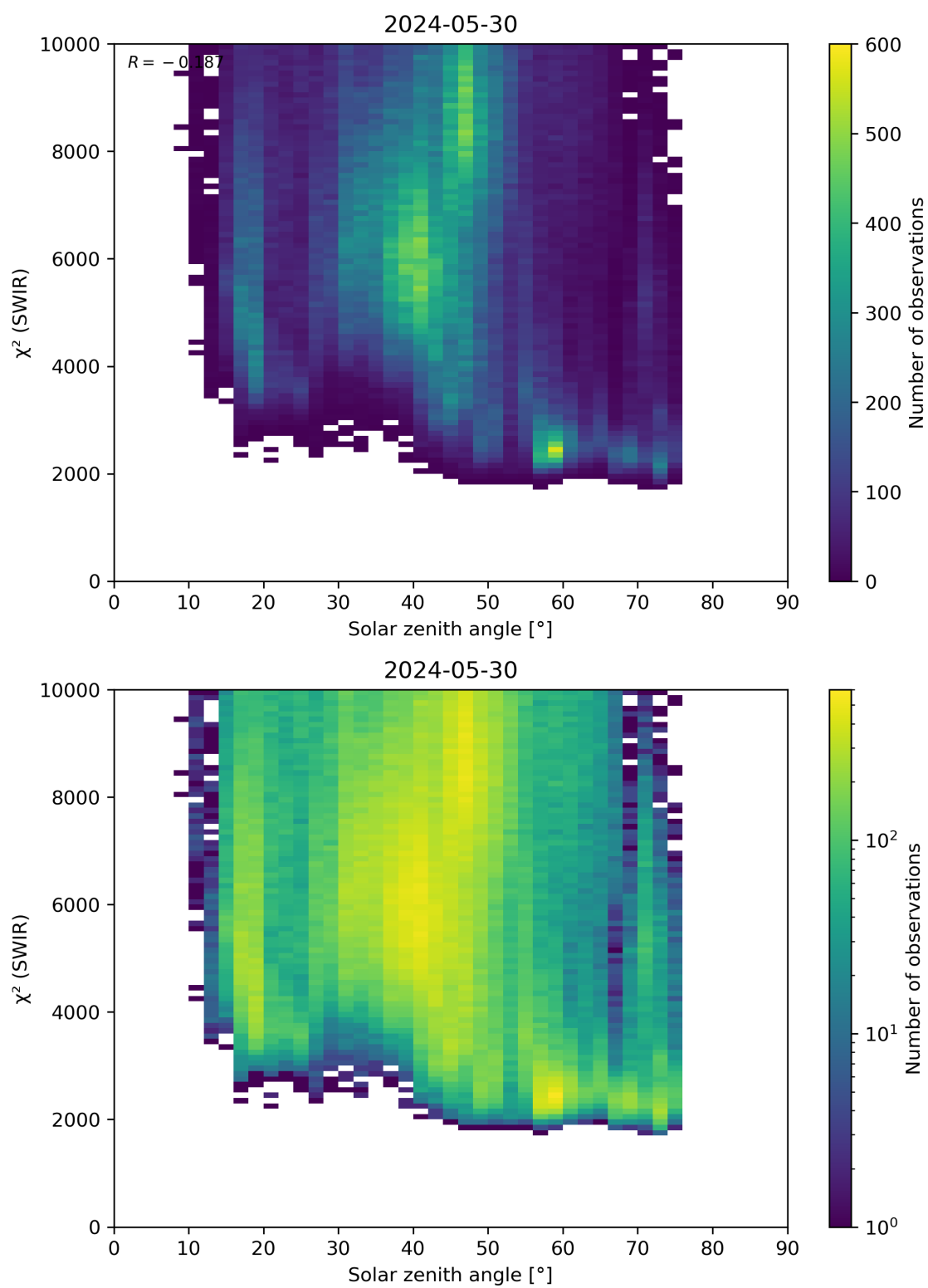
Figure 95: Scatter density plot of “Solar zenith angle” against “ \chi^2 (SWIR)” for 2024-05-29 to 2024-05-31.
