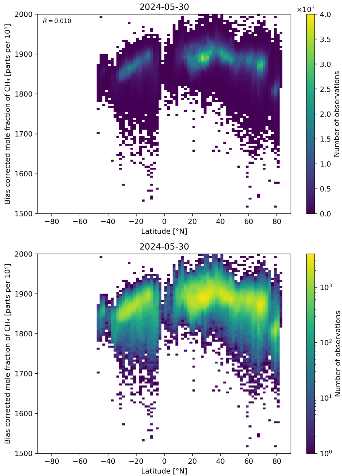
Figure 58: Scatter density plot of “Latitude” against “Bias corrected mole fraction of CH 4 ” for 2024-05-29 to 2024-05-31.
