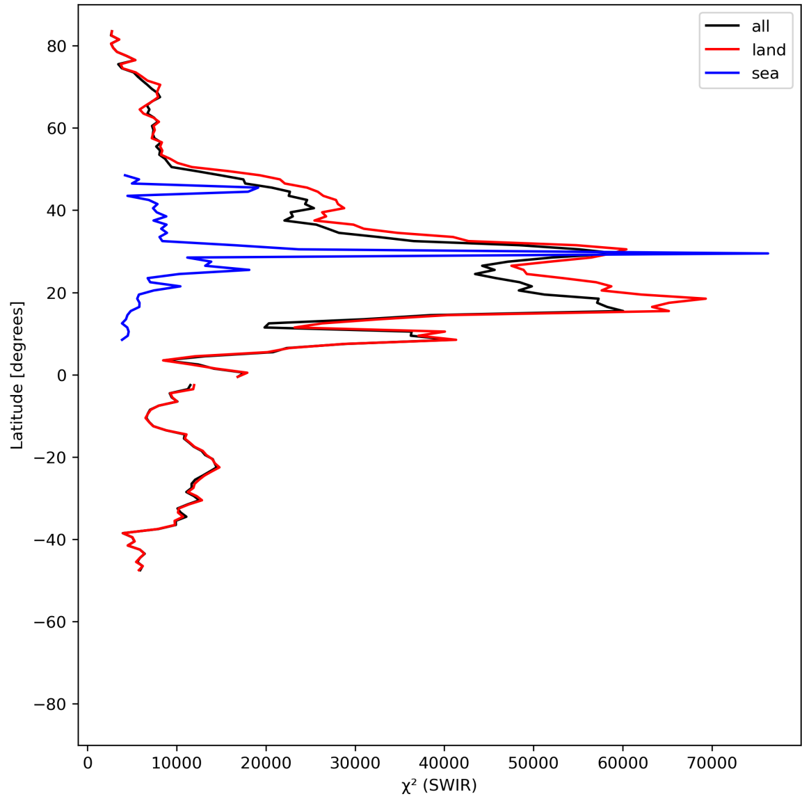
Figure 17: Zonal average of “ \chi^2 (SWIR)” for 2024-05-29 to 2024-05-31.
