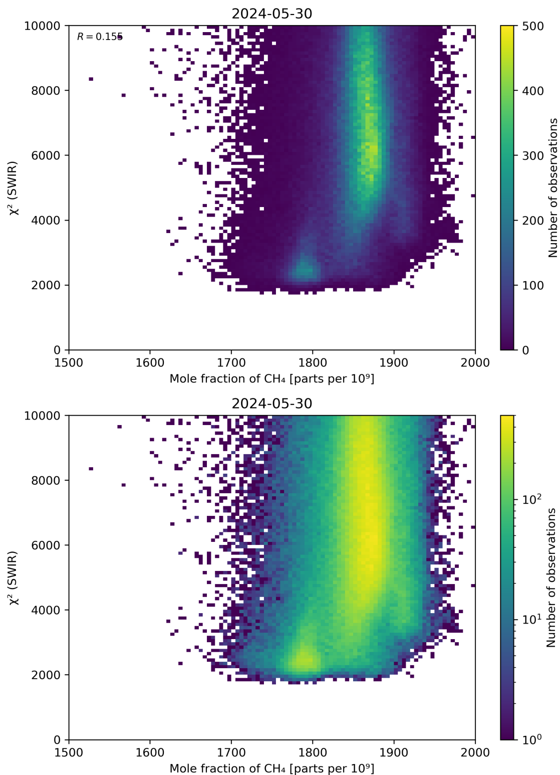
Figure 71: Scatter density plot of “Mole fraction of \text{CH}_4 ” against “ \chi^2 (SWIR)” for 2024-05-29 to 2024-05-31.
