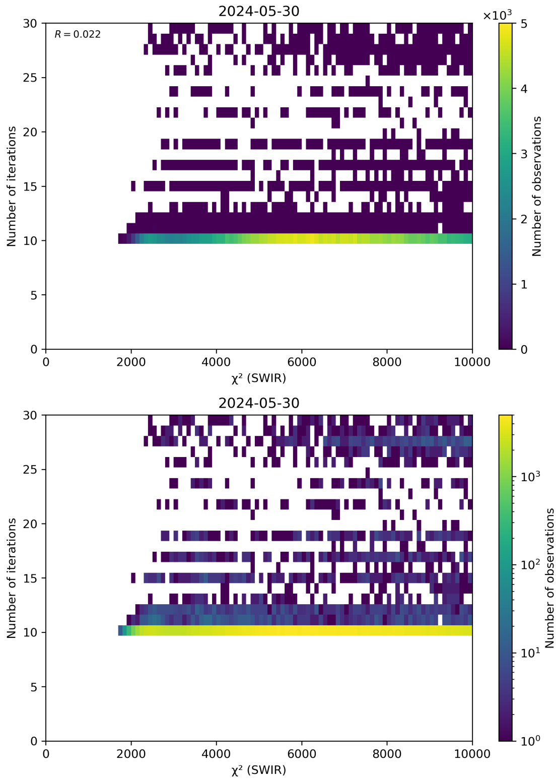
Figure 50: Scatter density plot of " \chi^2 (SWIR)" against "Number of iterations" for 2024-05-29 to 2024-05-31.
