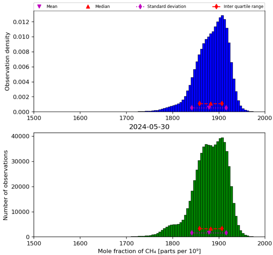
Figure 23: Histogram of “Mole fraction of CH 4 ” for 2024-05-29 to 2024-05-31
