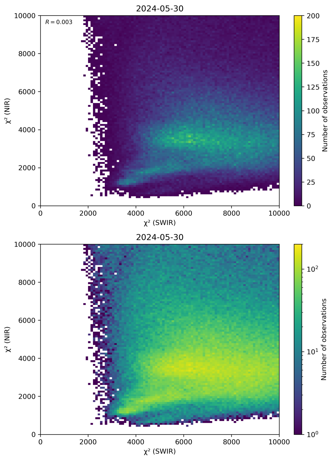
Figure 47: Scatter density plot of “ \chi^2 (SWIR)” against “ \chi^2 (NIR)” for 2024-05-29 to 2024-05-31.
