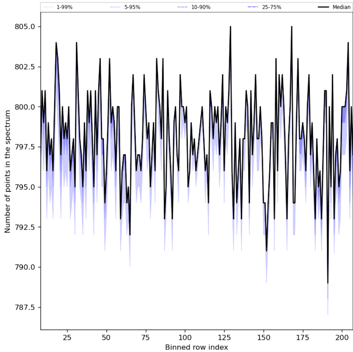
Figure 37: Along track statistics of “Number of points in the spectrum” for 2024-05-29 to 2024-05-31
