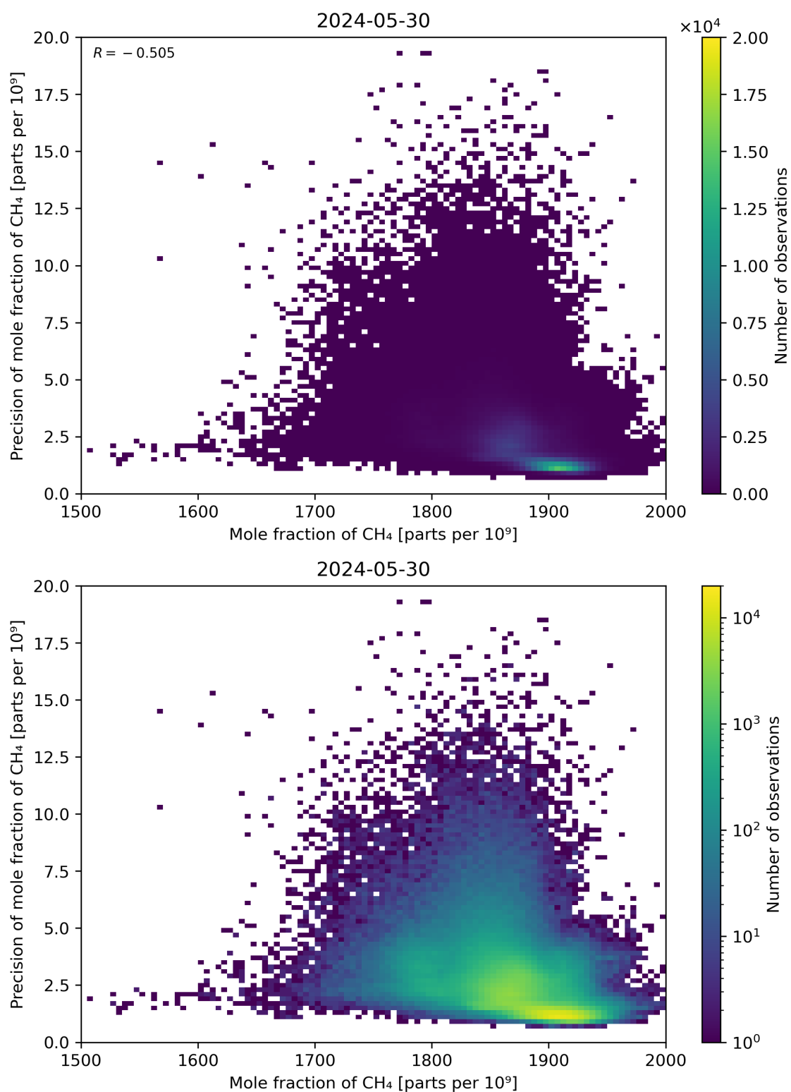
Figure 75: Scatter density plot of “Mole fraction of CH 4 ” against “Precision of mole fraction of CH 4 ” for 2024-05-29 to 2024-05-31.
