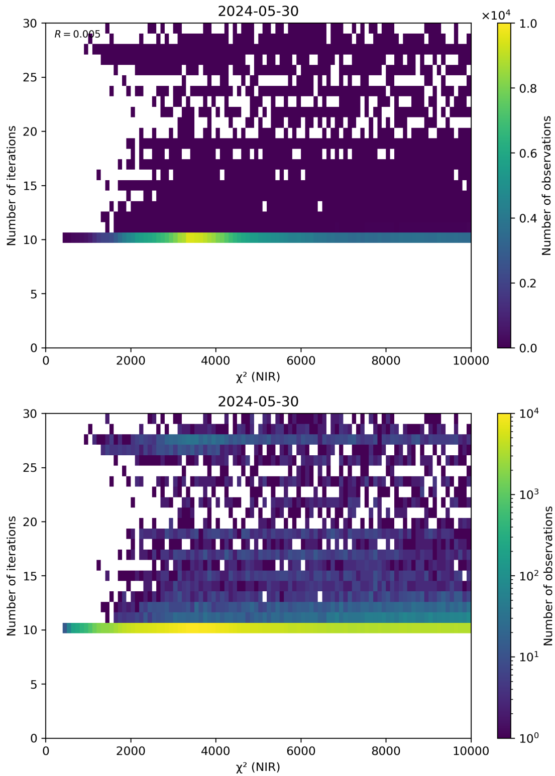
Figure 46: Scatter density plot of “ \chi^2 (NIR)” against “Number of iterations” for 2024-05-29 to 2024-05-31.
