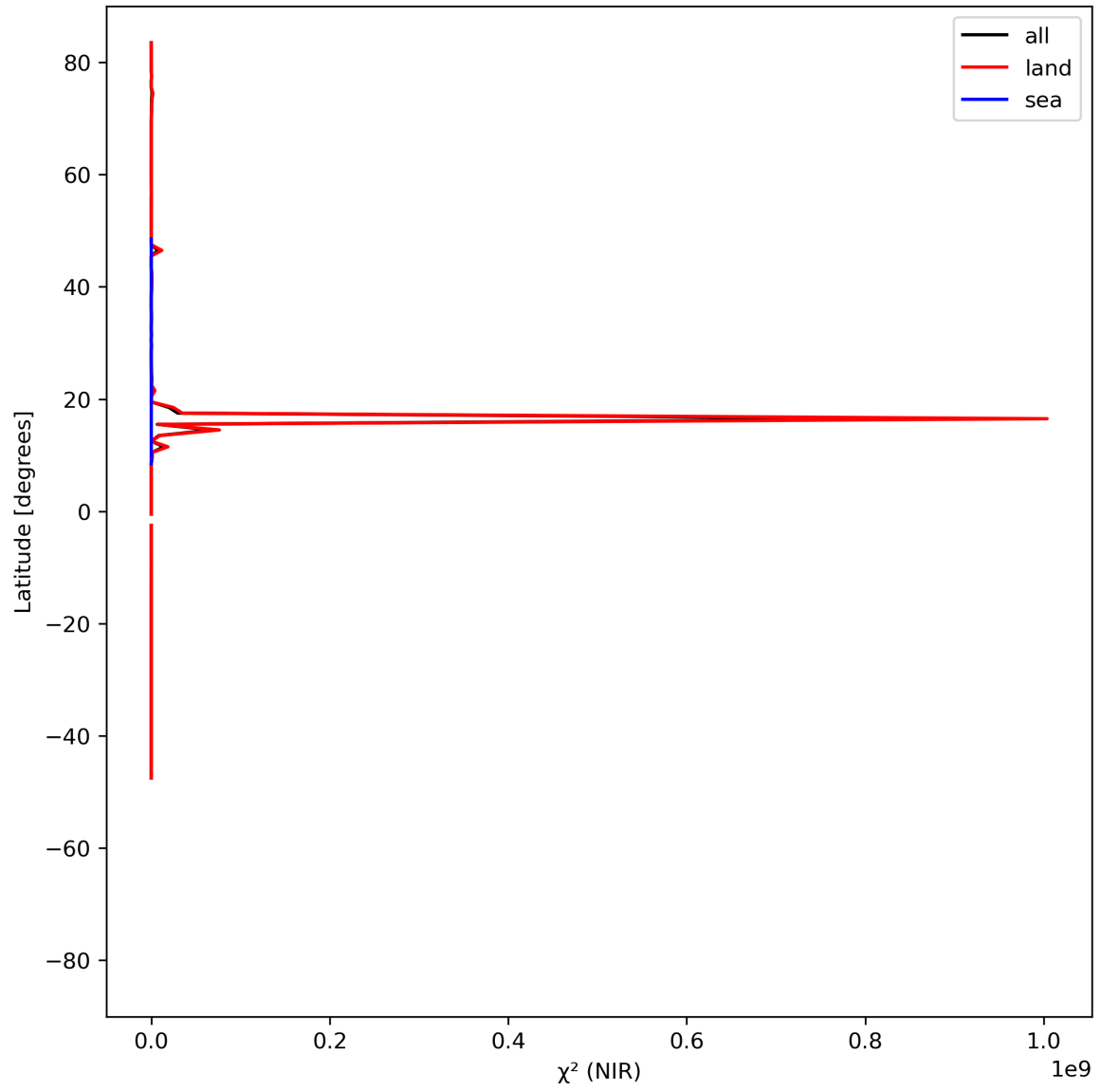
Figure 18: Zonal average of “ \chi^2 (NIR)” for 2024-05-29 to 2024-05-31.
