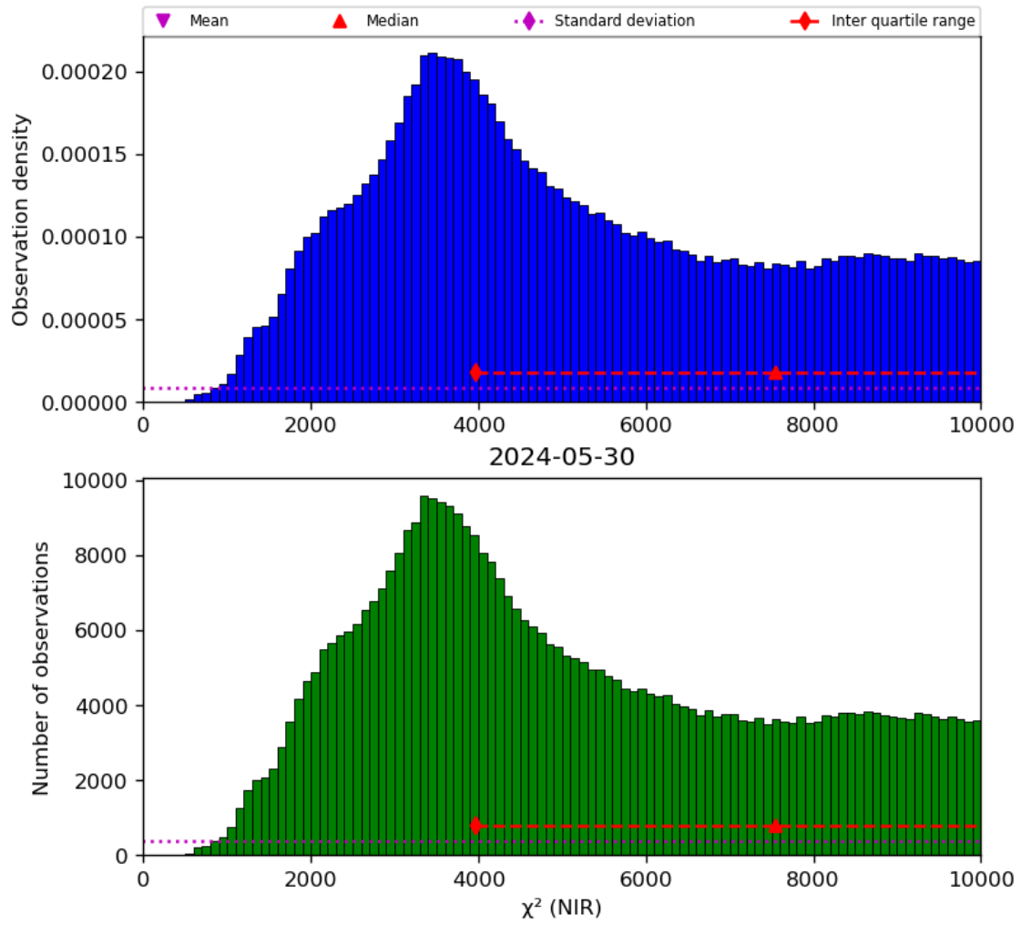
Figure 29: Histogram of " \chi^2 (NIR)" for 2024-05-29 to 2024-05-31
