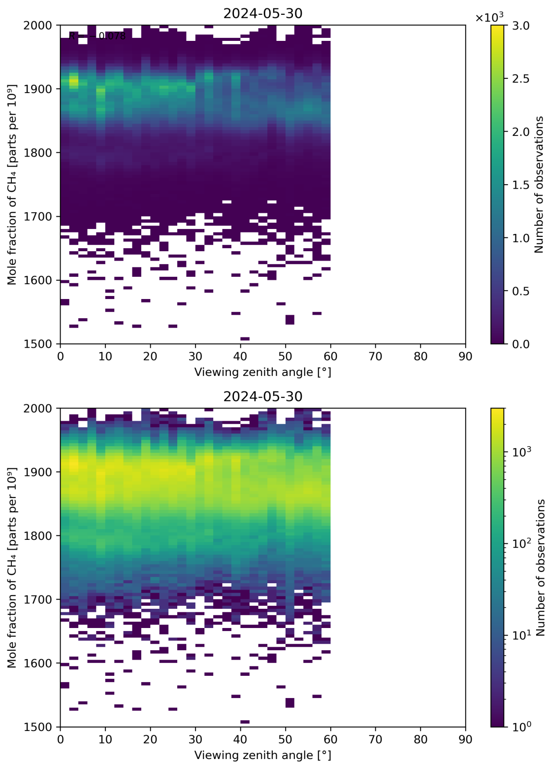
Figure 110: Scatter density plot of “Viewing zenith angle” against “Mole fraction of CH 4 ” for 2024-05-29 to 2024-05-31.
