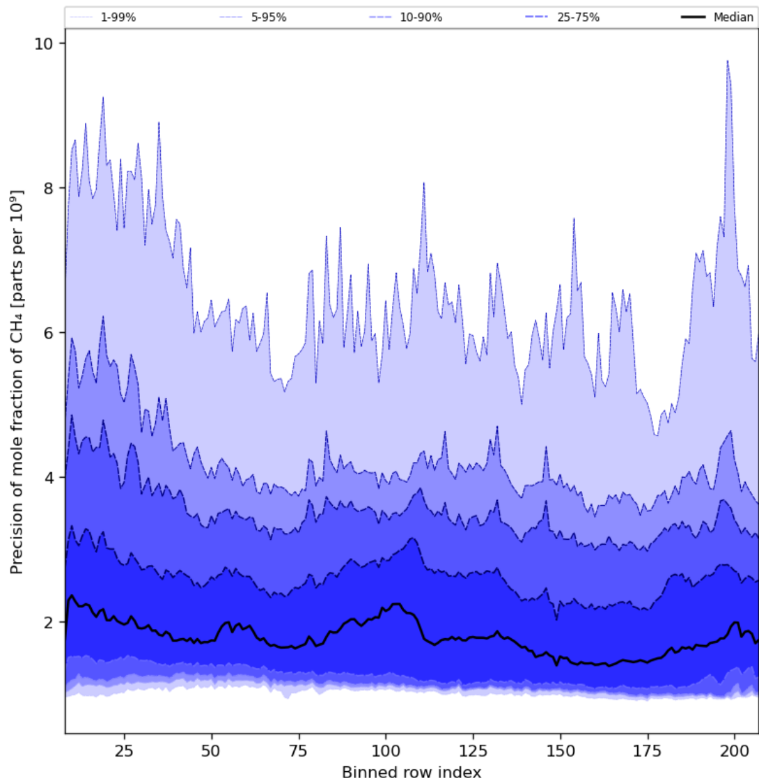
Figure 35: Along track statistics of “Precision of mole fraction of CH 4 ” for 2024-05-29 to 2024-05-31
