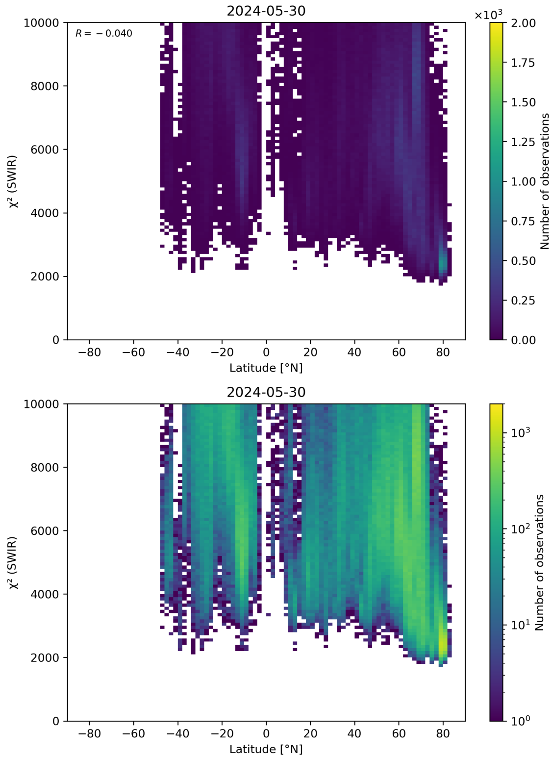
Figure 54: Scatter density plot of “Latitude” against “ \chi^2 (SWIR)” for 2024-05-29 to 2024-05-31.
