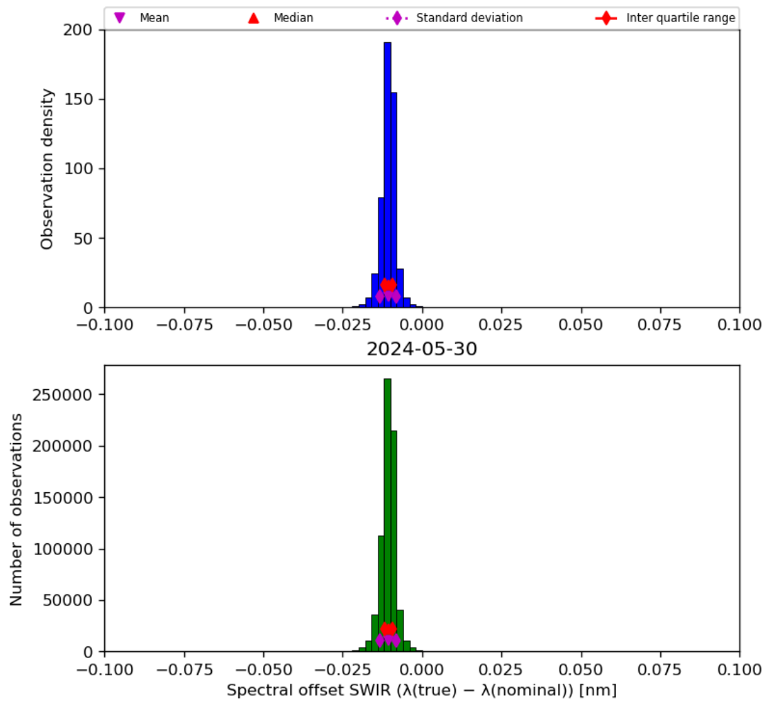
Figure 27: Histogram of “Spectral offset SWIR ( \lambda(\text{true}) - \lambda(\text{nominal}) )” for 2024-05-29 to 2024-05-31
