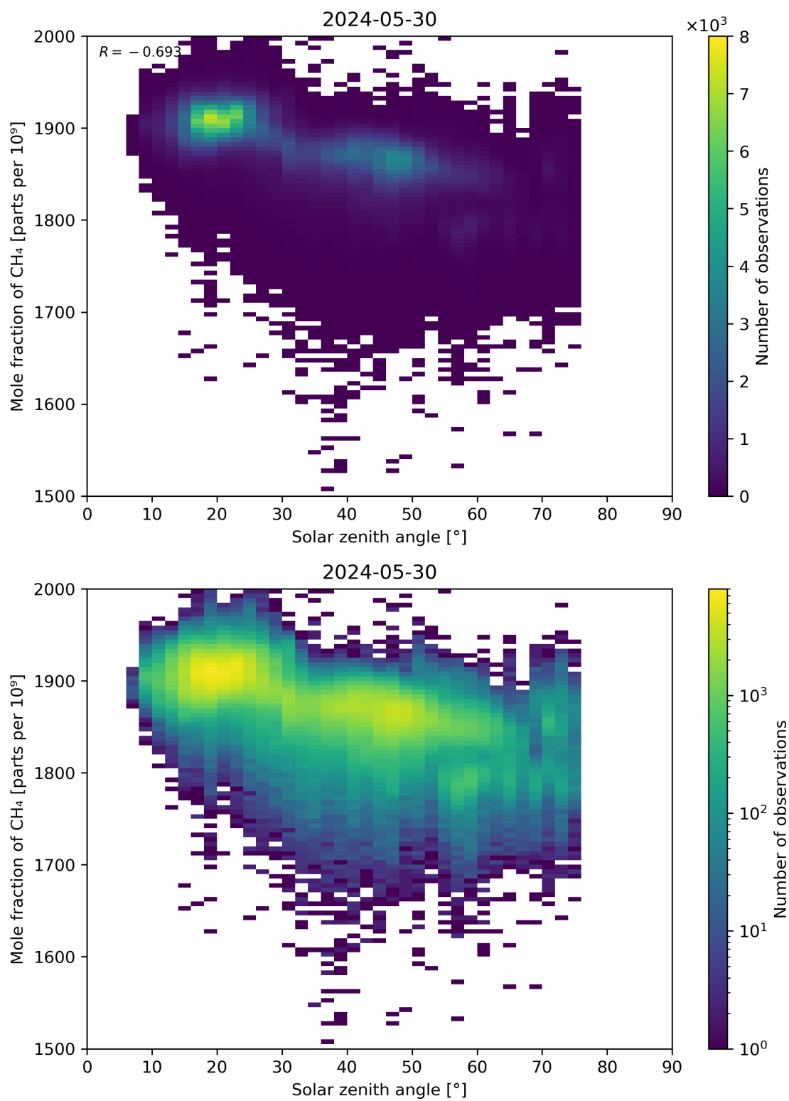
Figure 99: Scatter density plot of “Solar zenith angle” against “Mole fraction of CH 4 ” for 2024-05-29 to 2024-05-31.
