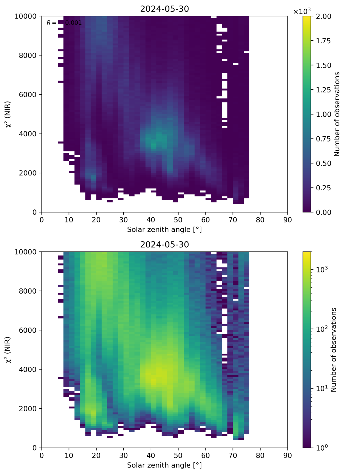
Figure 94: Scatter density plot of “Solar zenith angle” against “ \chi^2 (NIR)” for 2024-05-29 to 2024-05-31.
