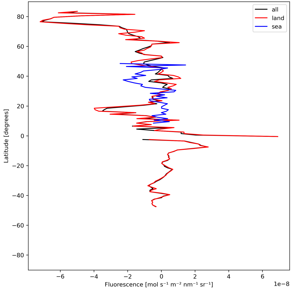
Figure 21: Zonal average of “Fluorescence” for 2024-05-29 to 2024-05-31.
