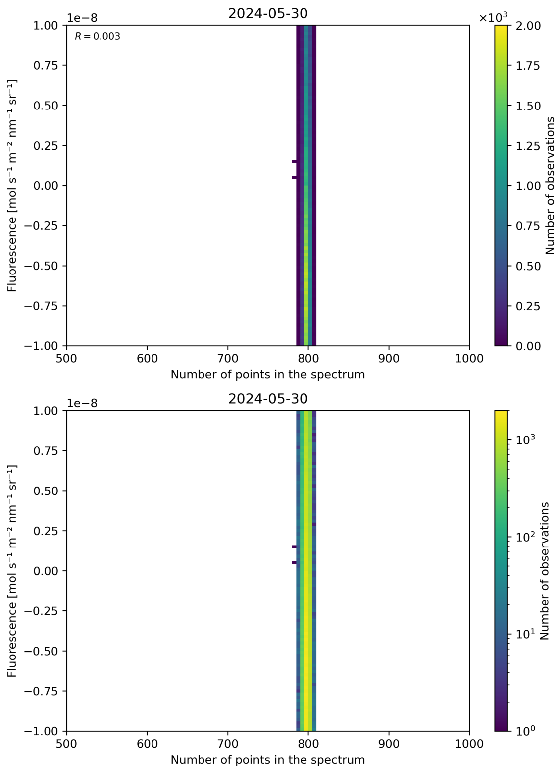
Figure 91: Scatter density plot of “Number of points in the spectrum” against “Fluorescence” for 2024-05-29 to 2024-05-31.
