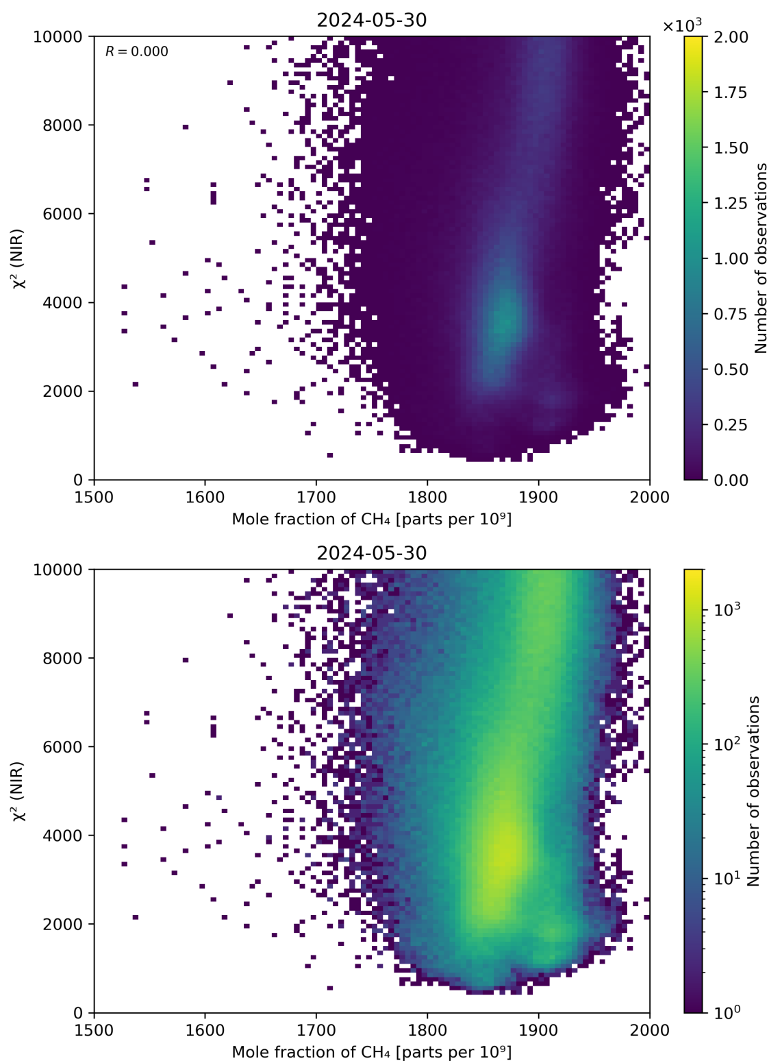
Figure 70: Scatter density plot of “Mole fraction of \text{CH}_4 ” against “ \chi^2 (NIR)” for 2024-05-29 to 2024-05-31.
