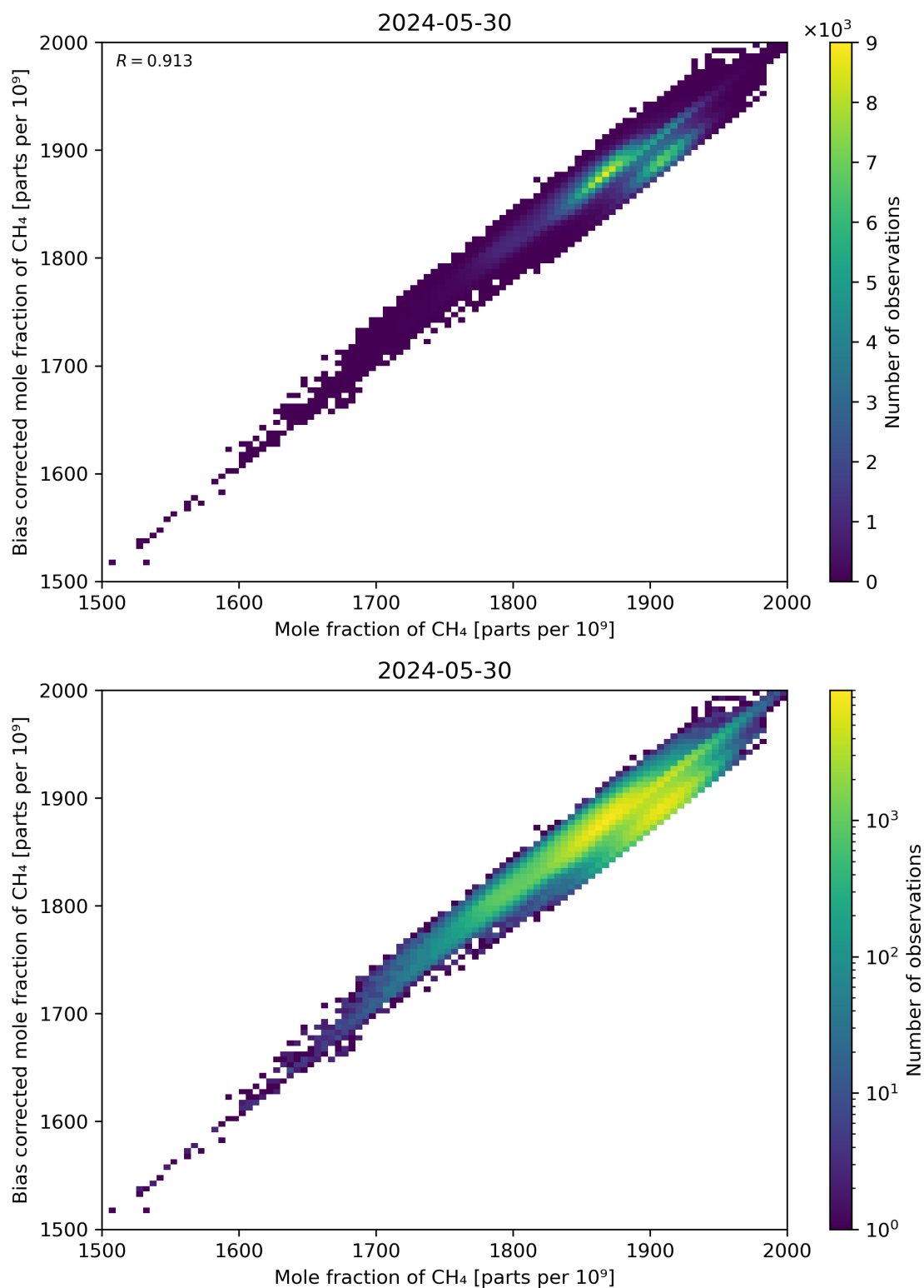
Figure 74: Scatter density plot of “Mole fraction of CH 4 ” against “Bias corrected mole fraction of CH 4 ” for 2024-05-29 to 2024-05-31.
