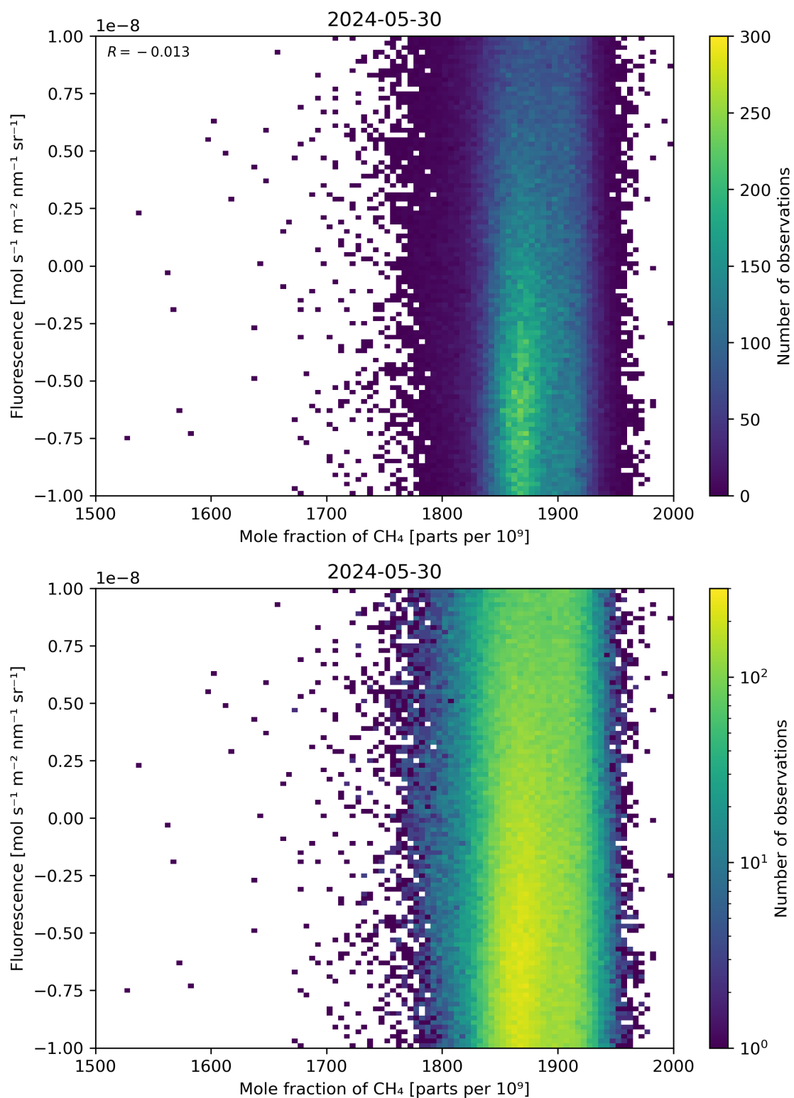
Figure 73: Scatter density plot of “Mole fraction of \text{CH}_4 ” against “Fluorescence” for 2024-05-29 to 2024-05-31.
