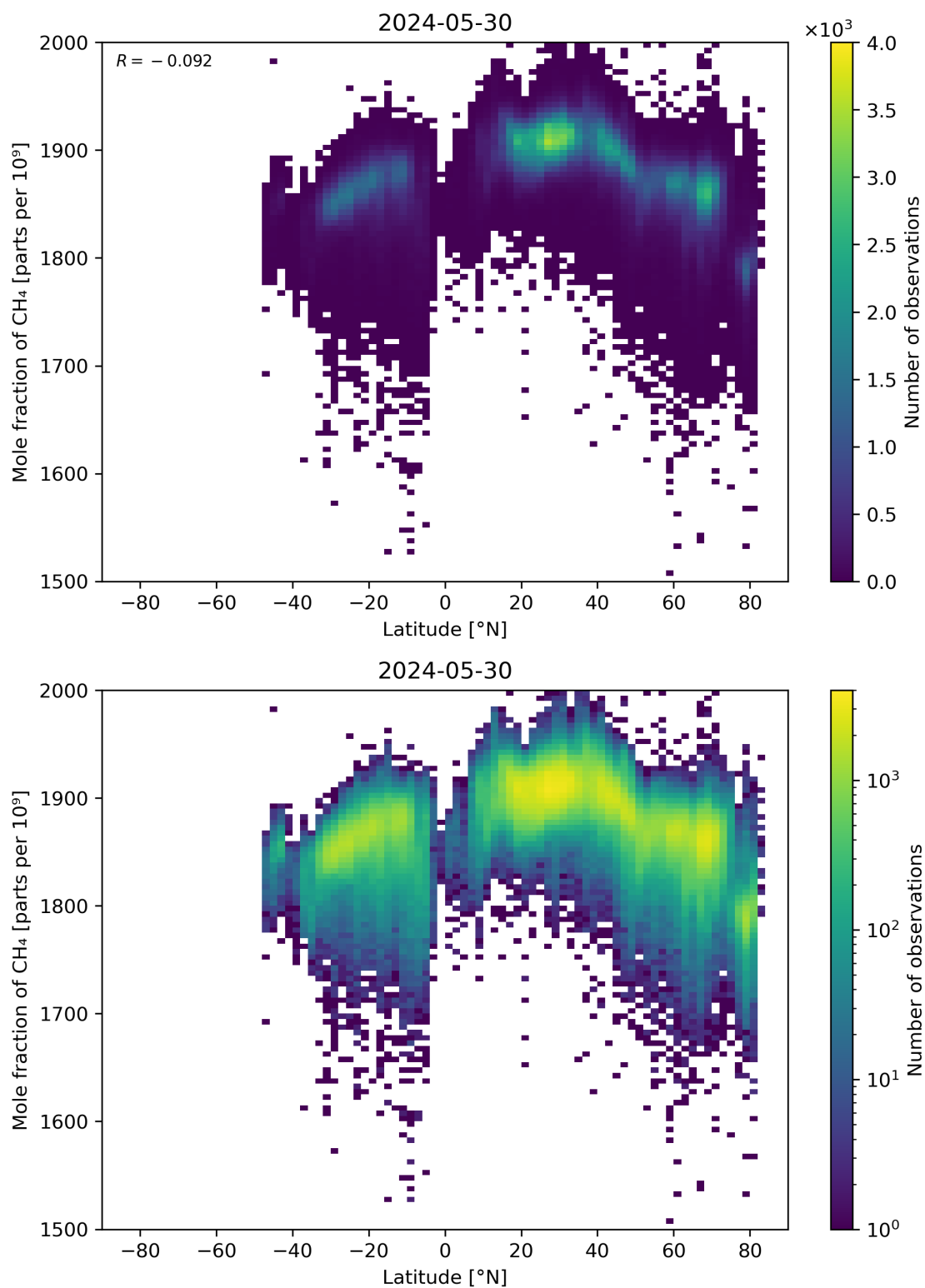
Figure 57: Scatter density plot of “Latitude” against “Mole fraction of \text{CH}_4 ” for 2024-05-29 to 2024-05-31.
