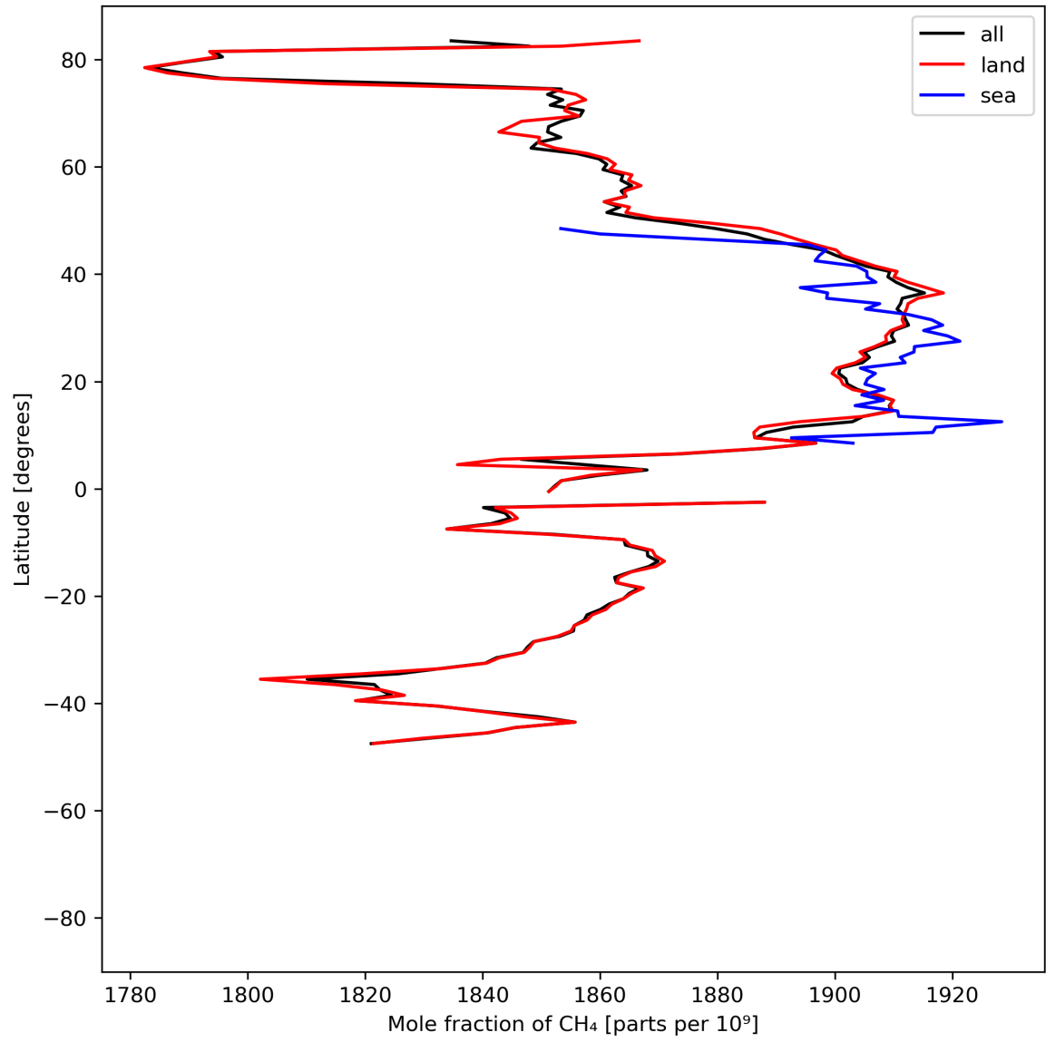
Figure 12: Zonal average of “Mole fraction of \text{CH}_4 ” for 2024-05-29 to 2024-05-31.
