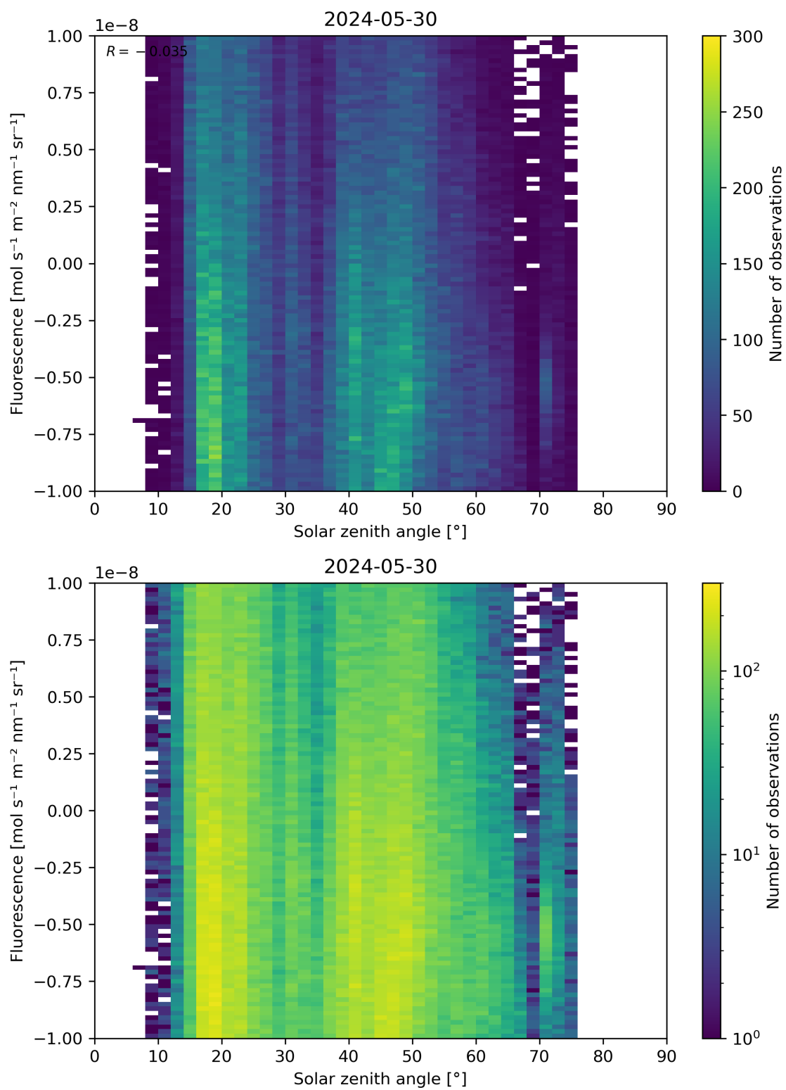
Figure 97: Scatter density plot of “Solar zenith angle” against “Fluorescence” for 2024-05-29 to 2024-05-31.
