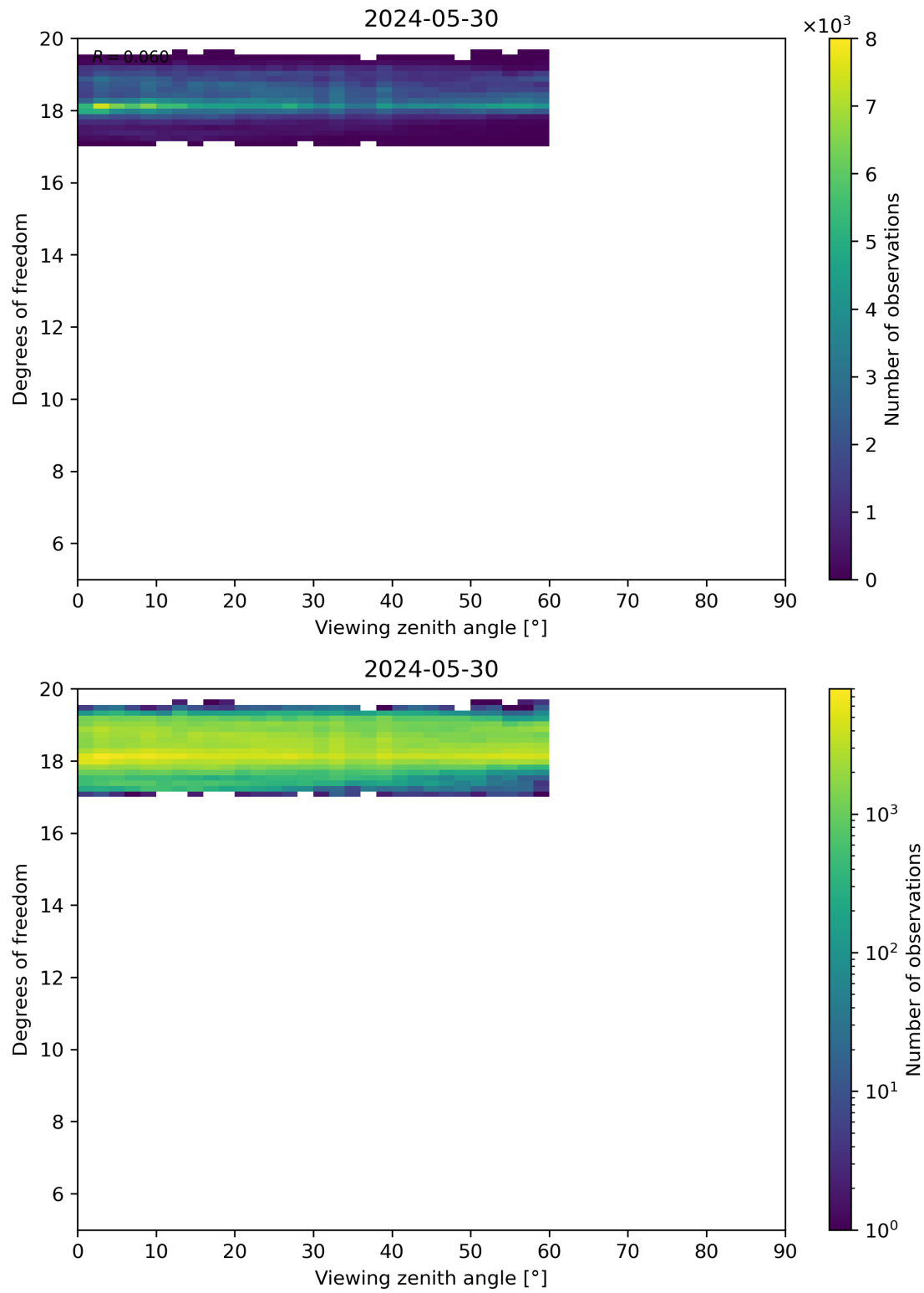
Figure 107: Scatter density plot of “Viewing zenith angle” against “Degrees of freedom” for 2024-05-29 to 2024-05-31.
