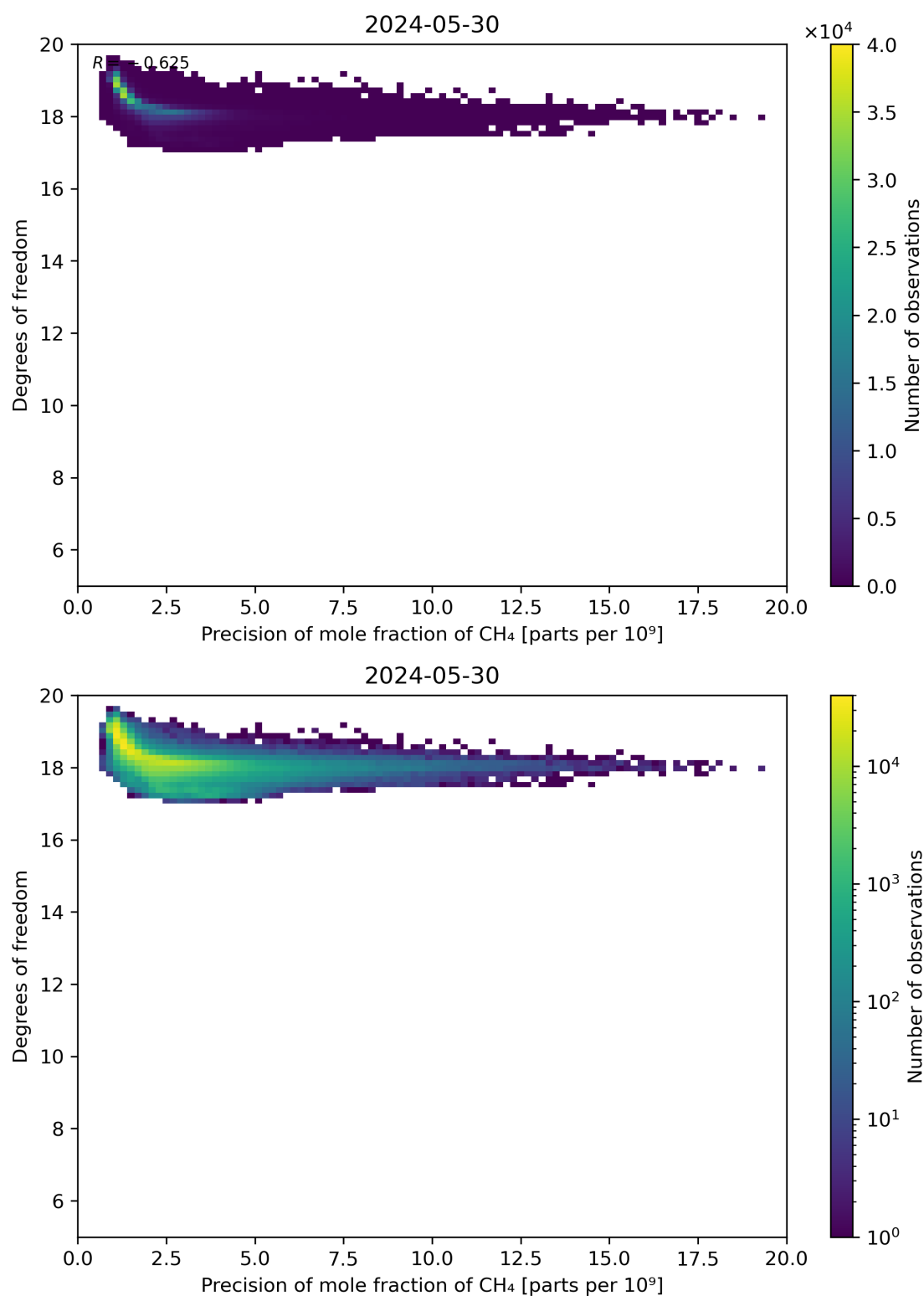
Figure 80: Scatter density plot of “Precision of mole fraction of CH 4 ” against “Degrees of freedom” for 2024-05-29 to 2024-05-31.
