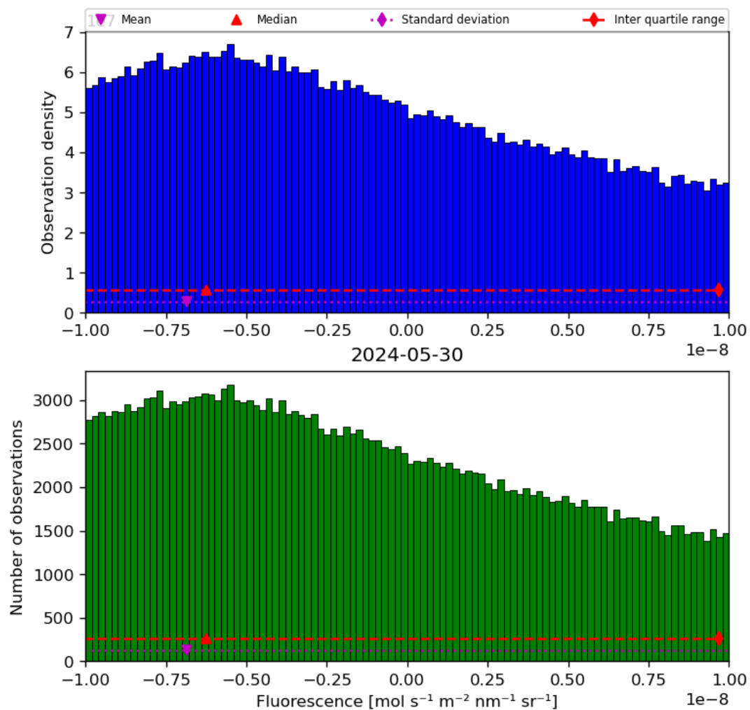
Figure 32: Histogram of “Fluorescence” for 2024-05-29 to 2024-05-31
