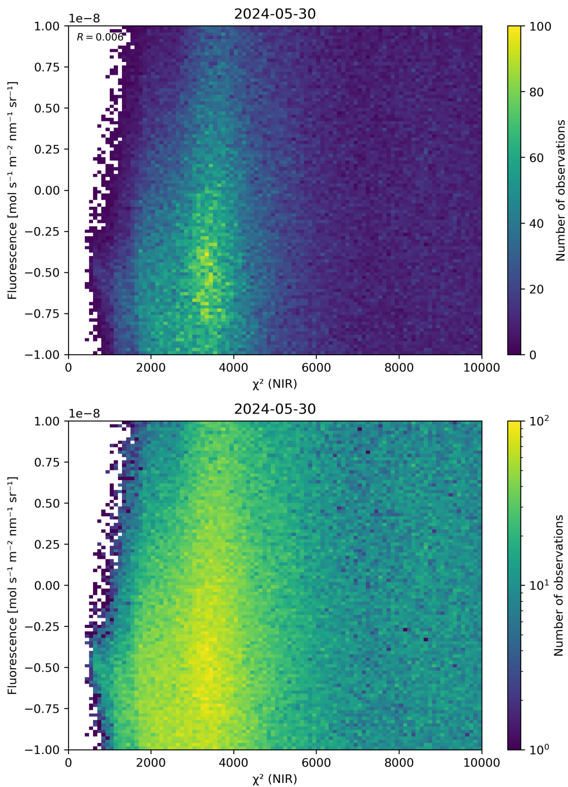
Figure 45: Scatter density plot of “ \chi^2 (NIR)” against “Fluorescence” for 2024-05-29 to 2024-05-31.
