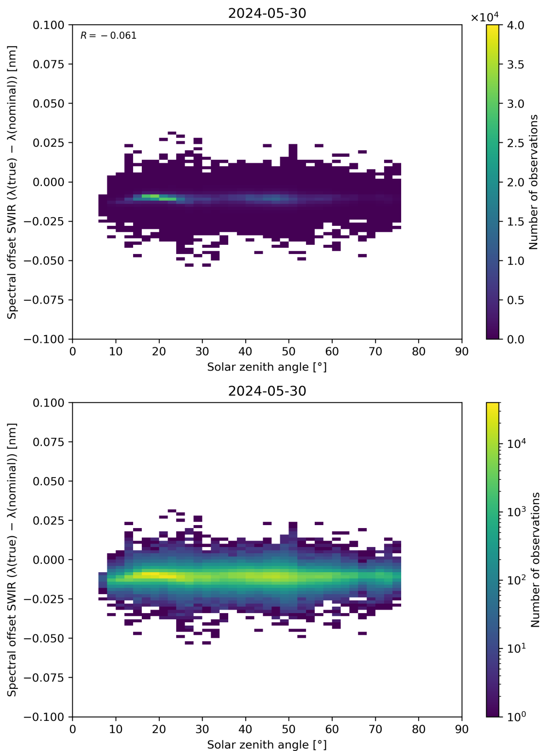
Figure 104: Scatter density plot of “Solar zenith angle” against “Spectral offset SWIR ( \lambda(\text{true}) - \lambda(\text{nominal}) )” for 2024-05-29 to 2024-05-31.
