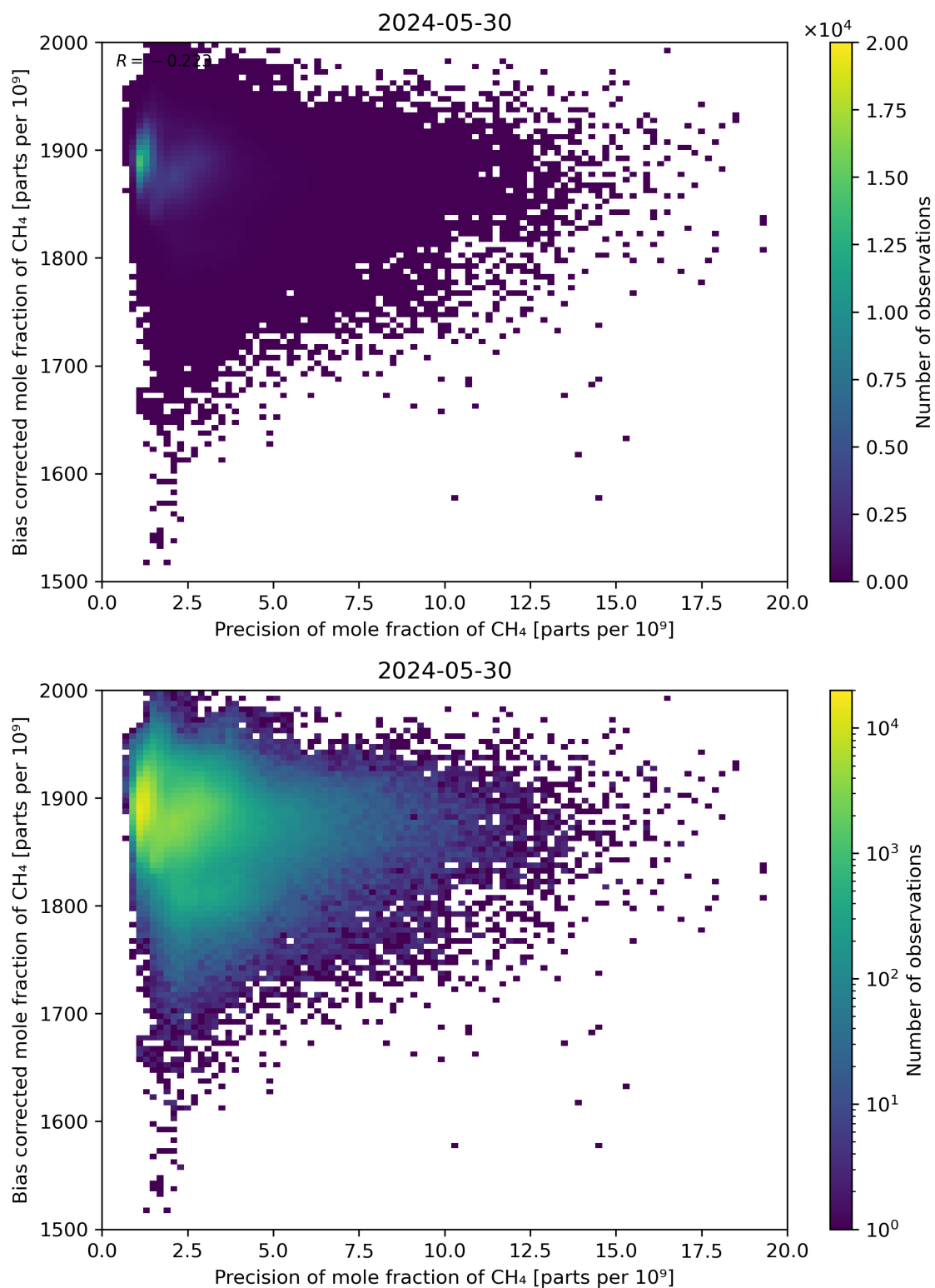
Figure 82: Scatter density plot of “Precision of mole fraction of CH 4 ” against “Bias corrected mole fraction of CH 4 ” for 2024-05-29 to 2024-05-31.
