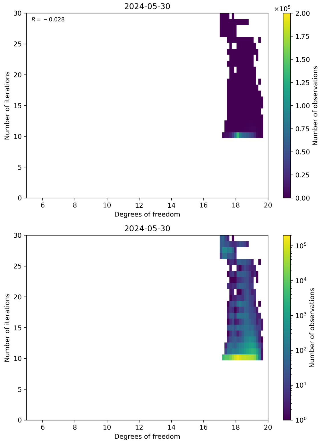
Figure 52: Scatter density plot of “Degrees of freedom” against “Number of iterations” for 2024-05-29 to 2024-05-31.
