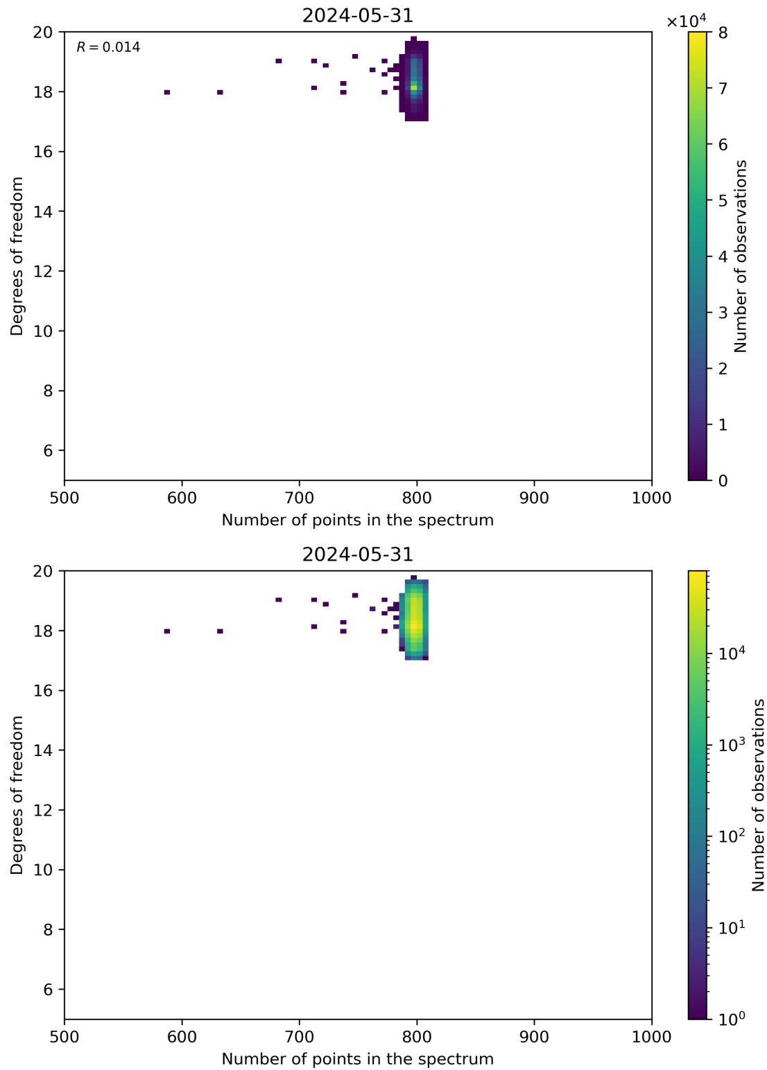
Figure 90: Scatter density plot of “Number of points in the spectrum” against “Degrees of freedom” for 2024-05-30 to 2024-06-01.
