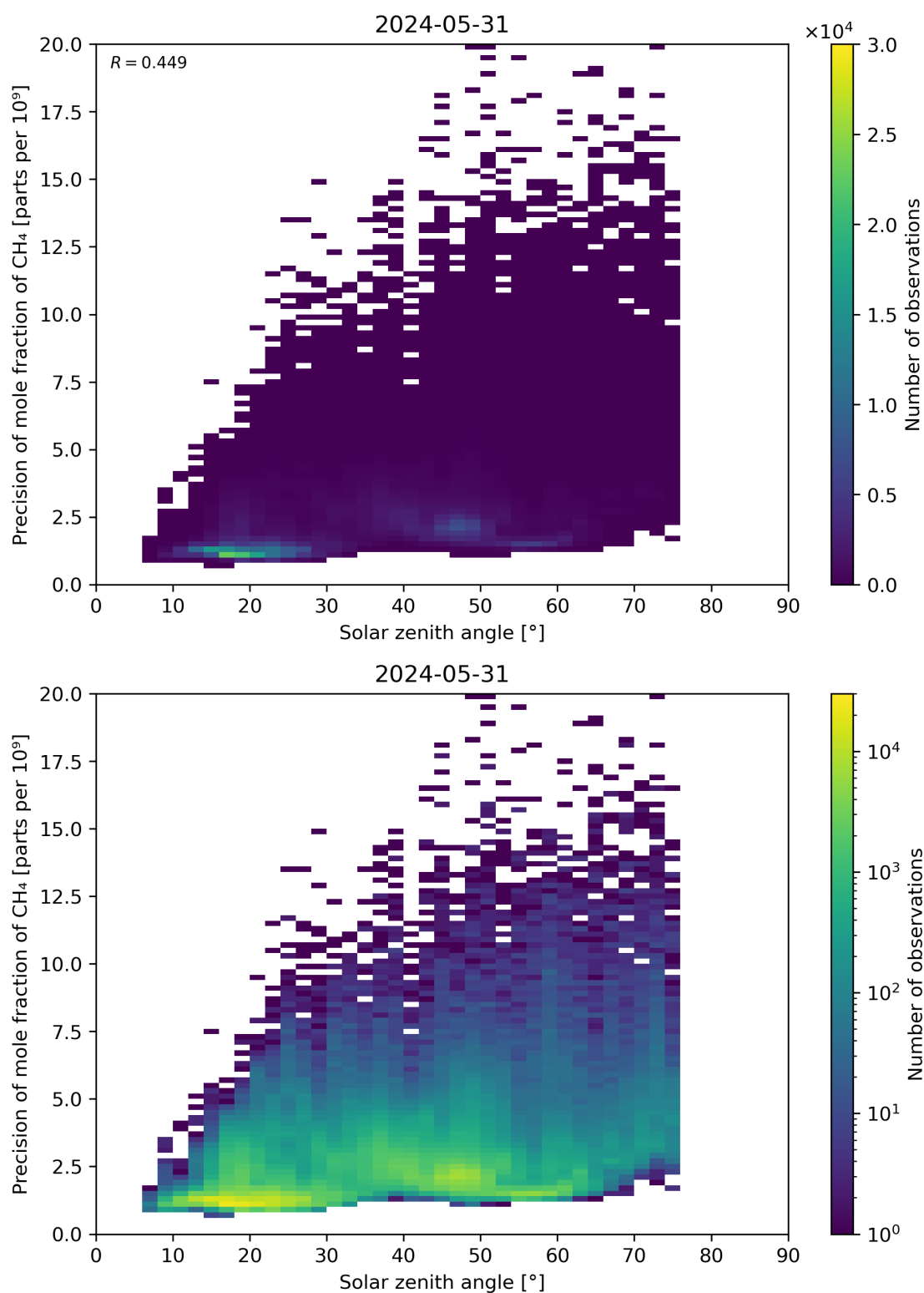
Figure 101: Scatter density plot of “Solar zenith angle” against “Precision of mole fraction of CH 4 ” for 2024-05-30 to 2024-06-01.
