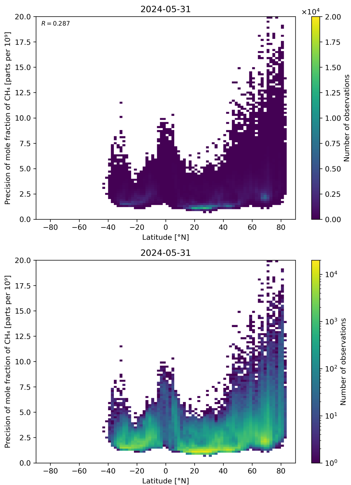
Figure 59: Scatter density plot of “Latitude” against “Precision of mole fraction of \text{CH}_4 ” for 2024-05-30 to 2024-06-01.
