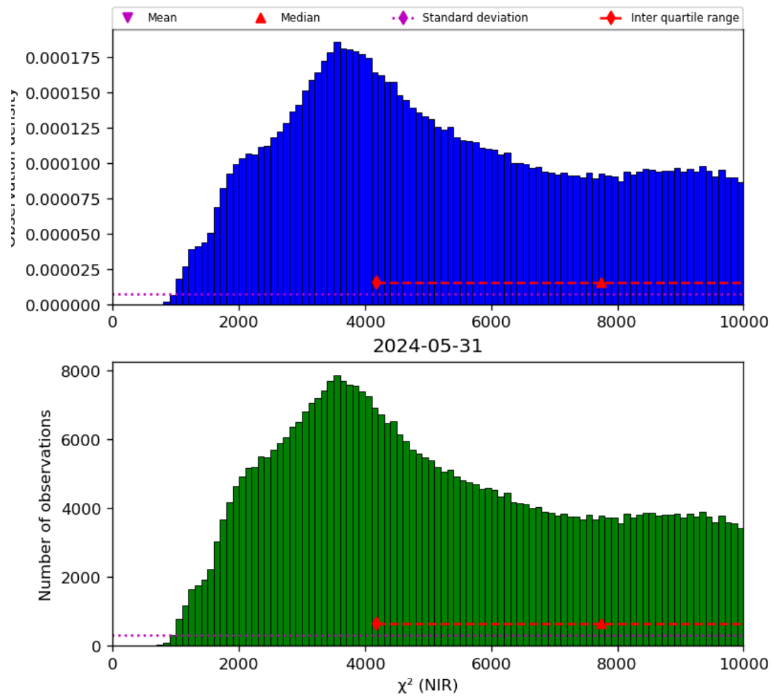
Figure 29: Histogram of “ \chi^2 (NIR)” for 2024-05-30 to 2024-06-01
