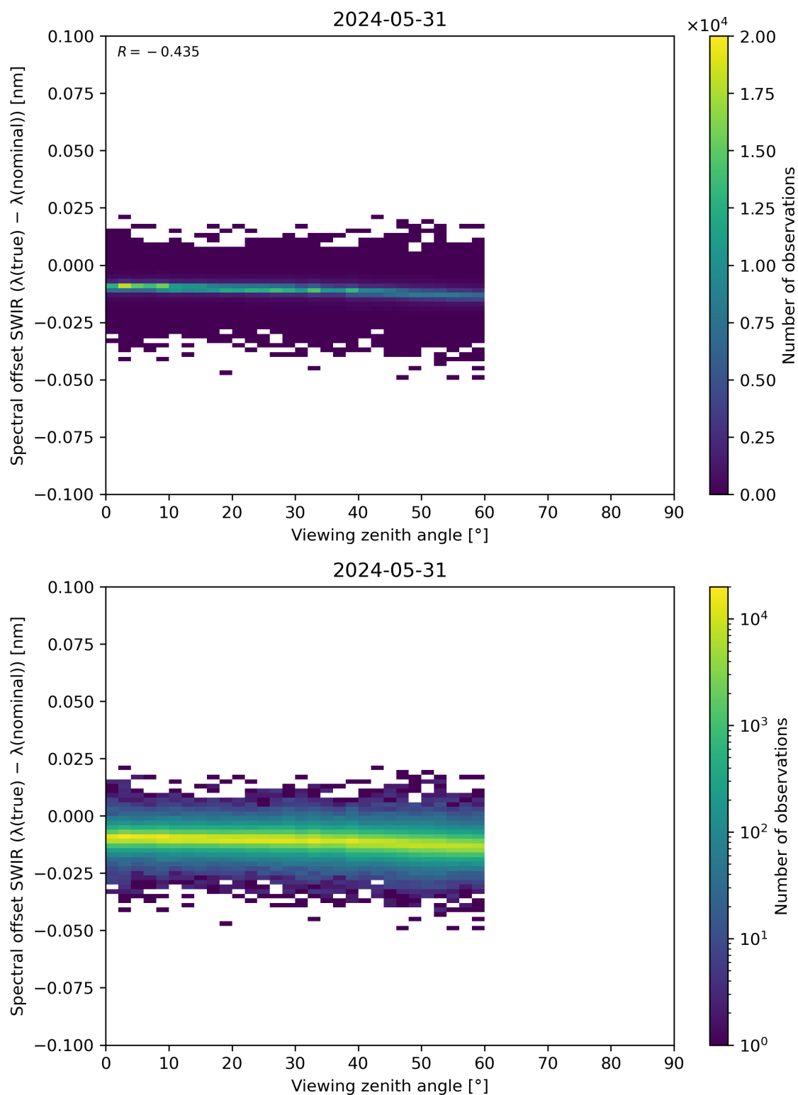
Figure 116: Scatter density plot of “Viewing zenith angle” against “Spectral offset SWIR ( \lambda(\text{true}) - \lambda(\text{nominal}) )” for 2024-05-30 to 2024-06-01.
