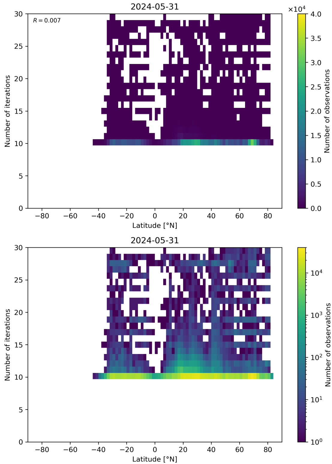
Figure 60: Scatter density plot of “Latitude” against “Number of iterations” for 2024-05-30 to 2024-06-01.
