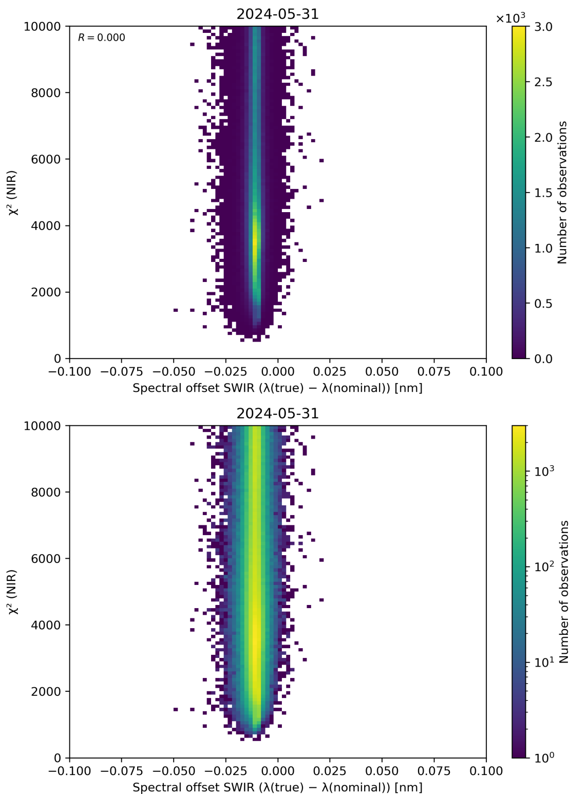
Figure 117: Scatter density plot of “Spectral offset SWIR ( \lambda(\text{true}) - \lambda(\text{nominal}) )” against “ \chi^2 (NIR)” for 2024-05-30 to 2024-06-01.
