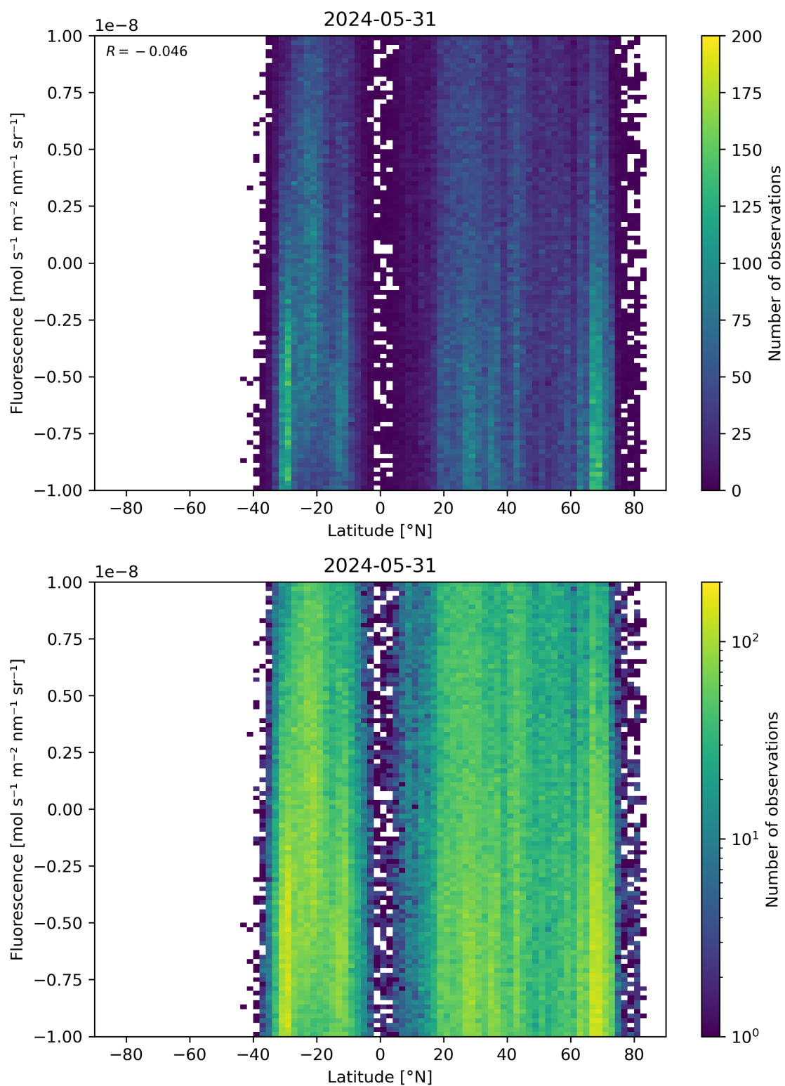
Figure 56: Scatter density plot of “Latitude” against “Fluorescence” for 2024-05-30 to 2024-06-01.
