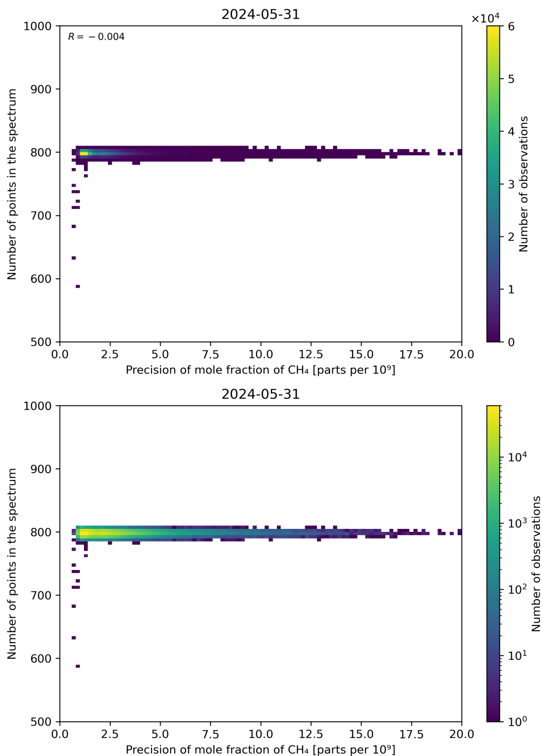
Figure 84: Scatter density plot of “Precision of mole fraction of CH 4 ” against “Number of points in the spectrum” for 2024-05-30 to 2024-06-01.
