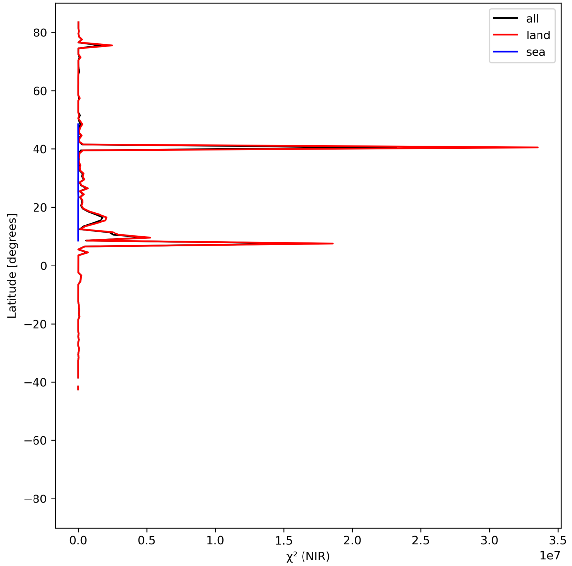
Figure 18: Zonal average of “ \chi^2 (NIR)” for 2024-05-30 to 2024-06-01.
