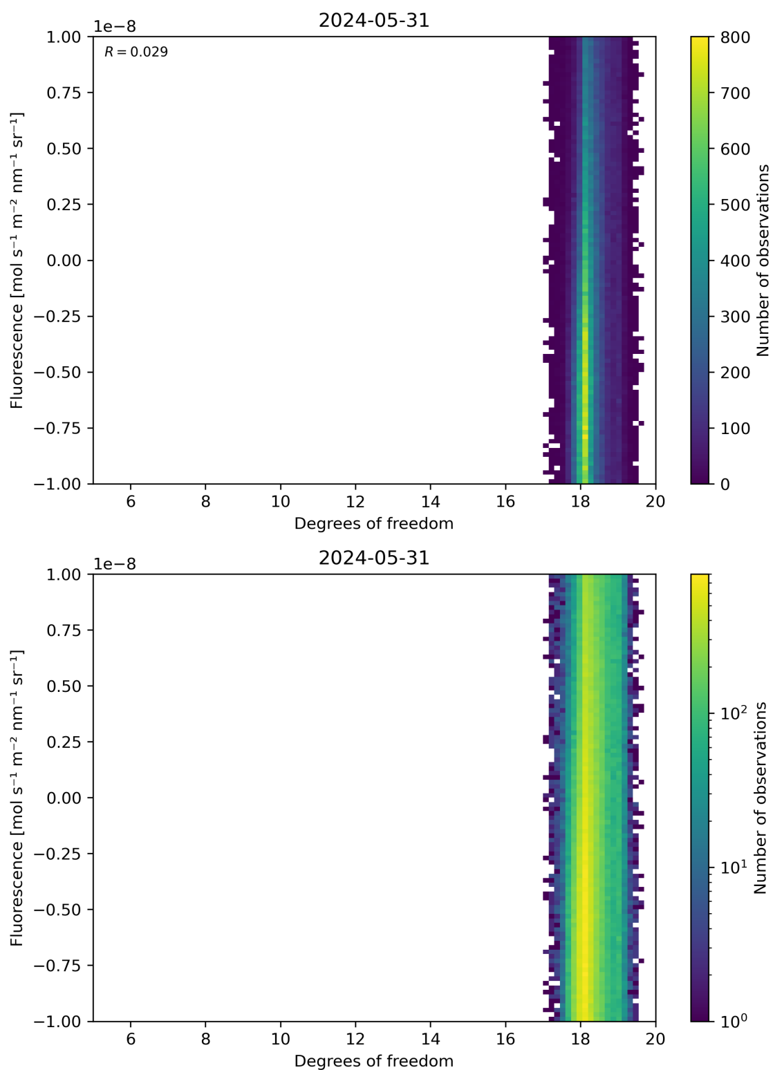
Figure 51: Scatter density plot of “Degrees of freedom” against “Fluorescence” for 2024-05-30 to 2024-06-01.
