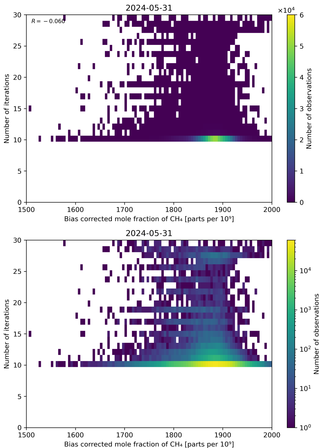
Figure 67: Scatter density plot of “Bias corrected mole fraction of CH 4 ” against “Number of iterations” for 2024-05-30 to 2024-06-01.
