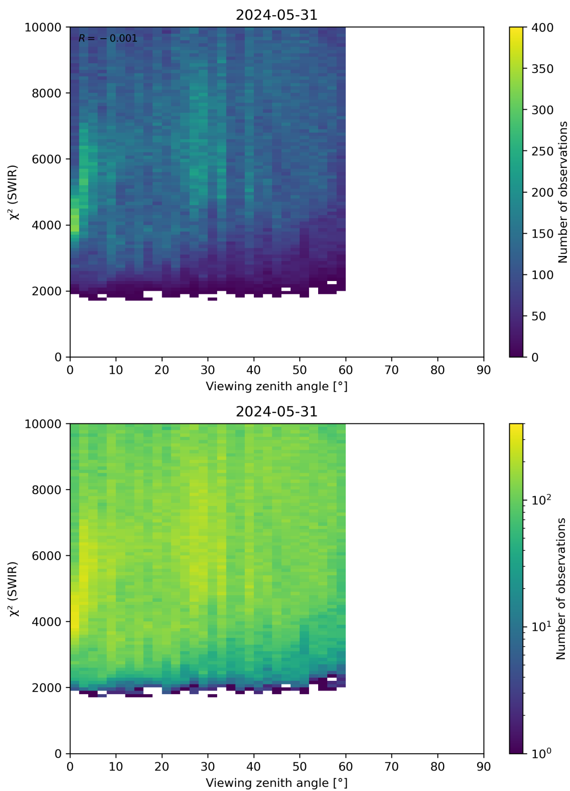
Figure 106: Scatter density plot of “Viewing zenith angle” against “ \chi^2 (SWIR)” for 2024-05-30 to 2024-06-01.
