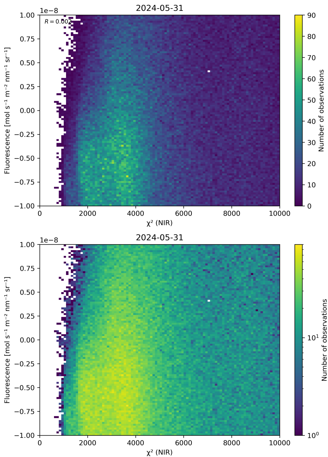
Figure 45: Scatter density plot of “ \chi^2 (NIR)” against “Fluorescence” for 2024-05-30 to 2024-06-01.
