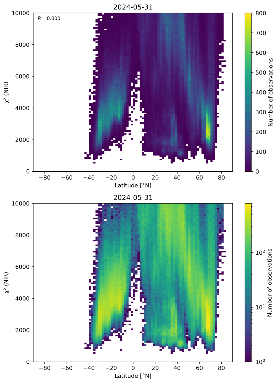
Figure 53: Scatter density plot of “Latitude” against “ \chi^2 (NIR)” for 2024-05-30 to 2024-06-01.
