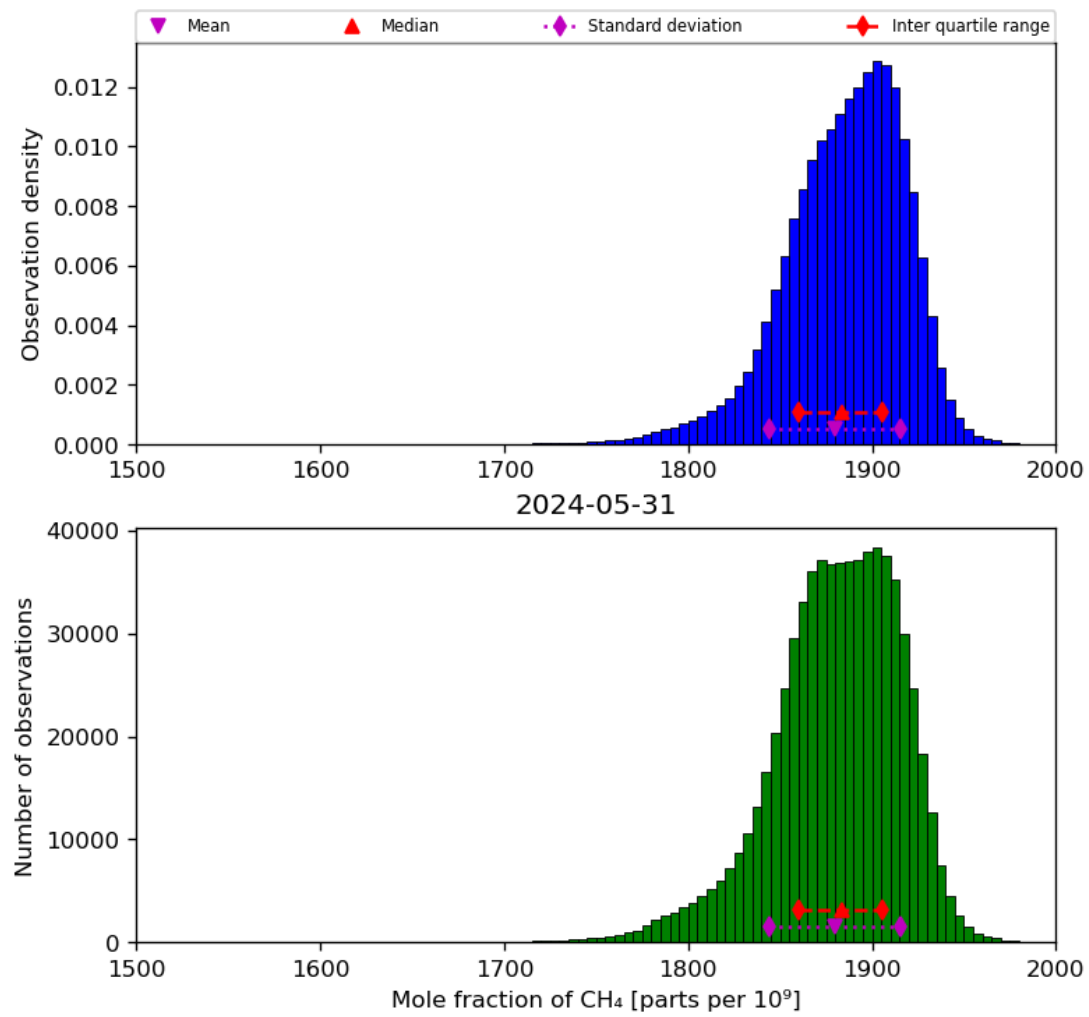
Figure 23: Histogram of “Mole fraction of CH 4 ” for 2024-05-30 to 2024-06-01
