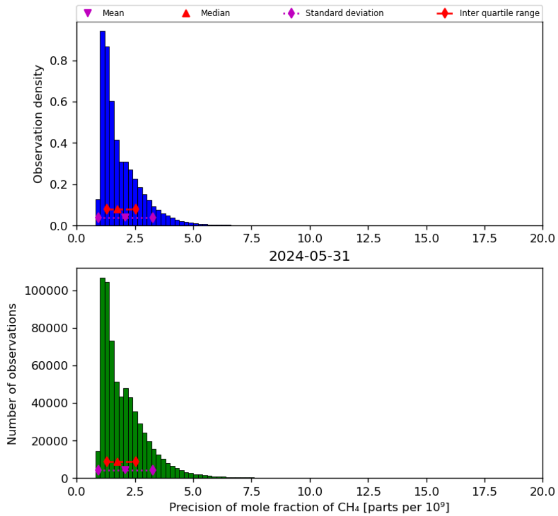
Figure 24: Histogram of “Precision of mole fraction of CH 4 ” for 2024-05-30 to 2024-06-01
