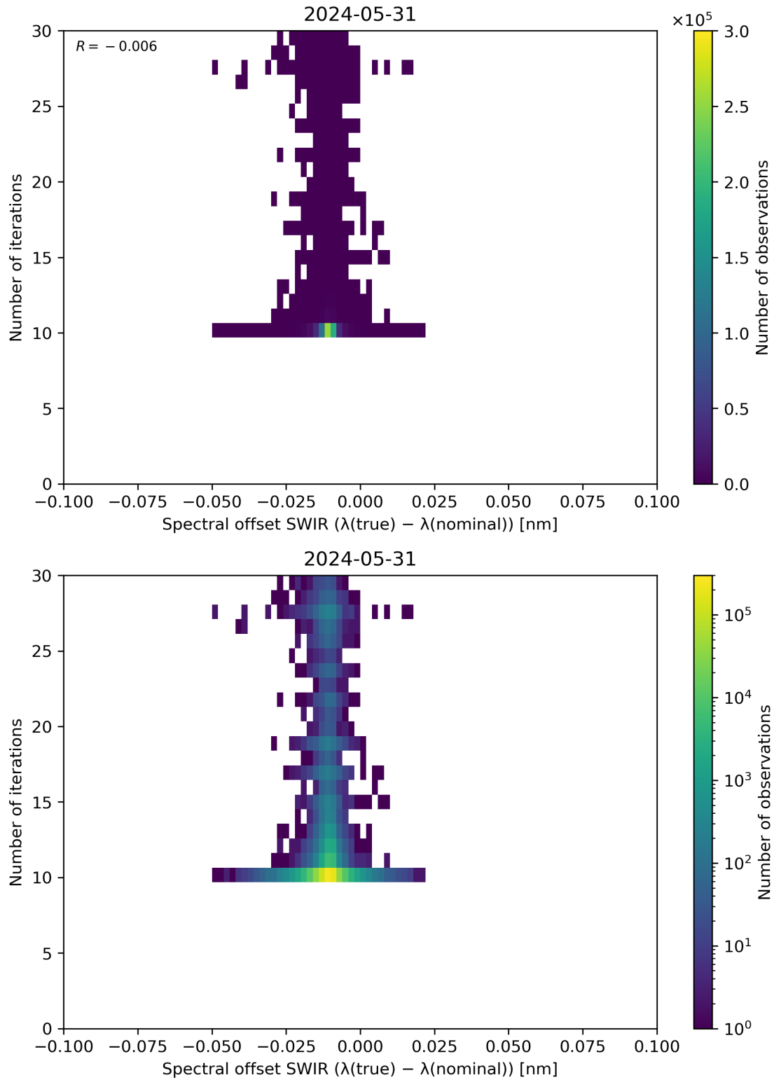
Figure 121: Scatter density plot of “Spectral offset SWIR ( \lambda(\text{true}) - \lambda(\text{nominal}) )” against “Number of iterations” for 2024-05-30 to 2024-06-01.
