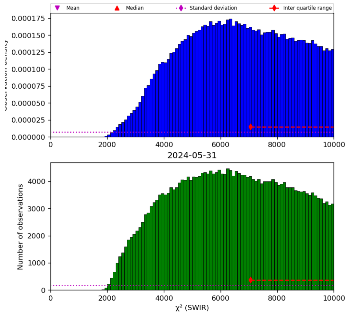
Figure 28: Histogram of “ \chi^2 (SWIR)” for 2024-05-30 to 2024-06-01
