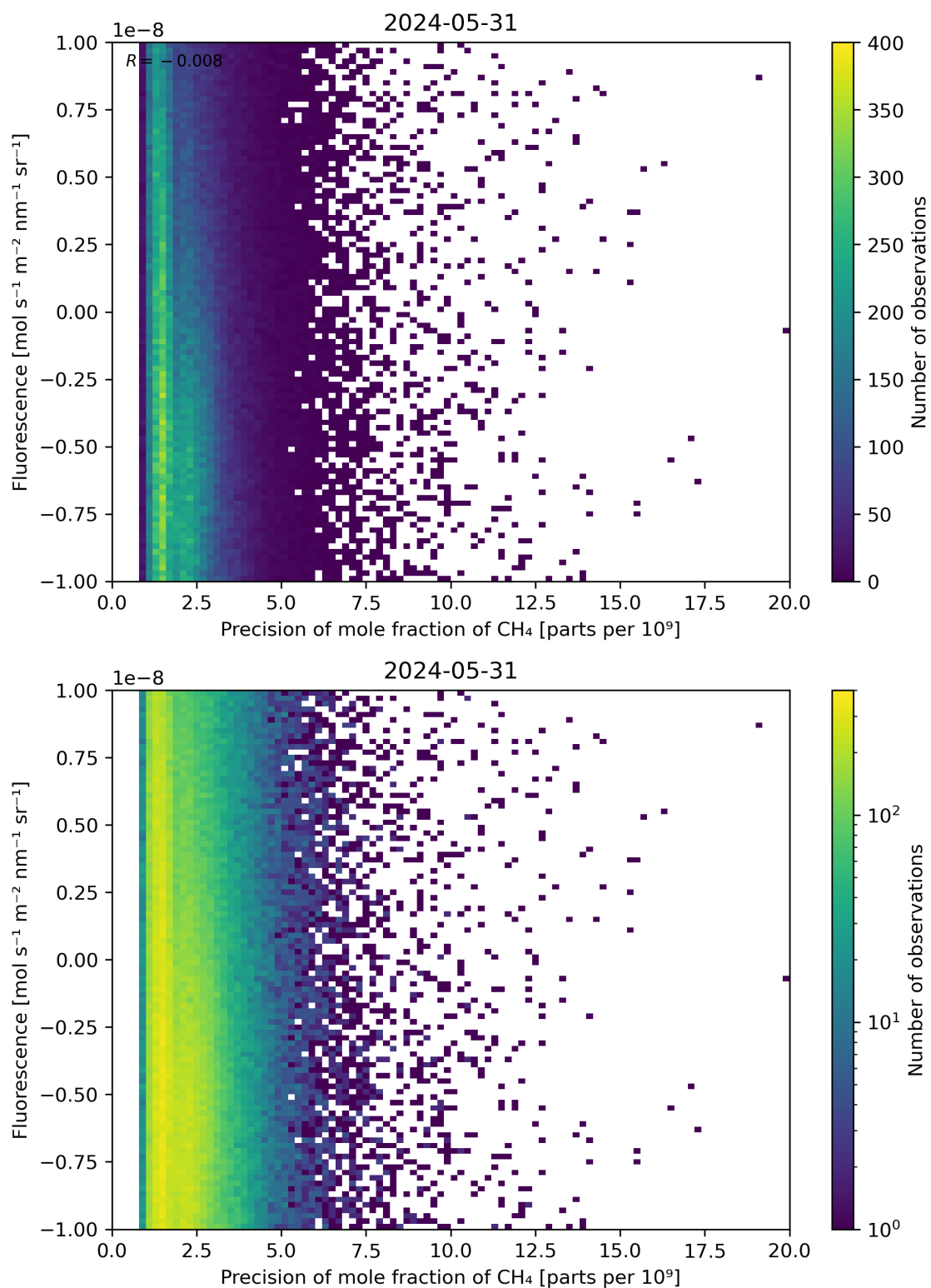
Figure 81: Scatter density plot of “Precision of mole fraction of CH 4 ” against “Fluorescence” for 2024-05-30 to 2024-06-01.
