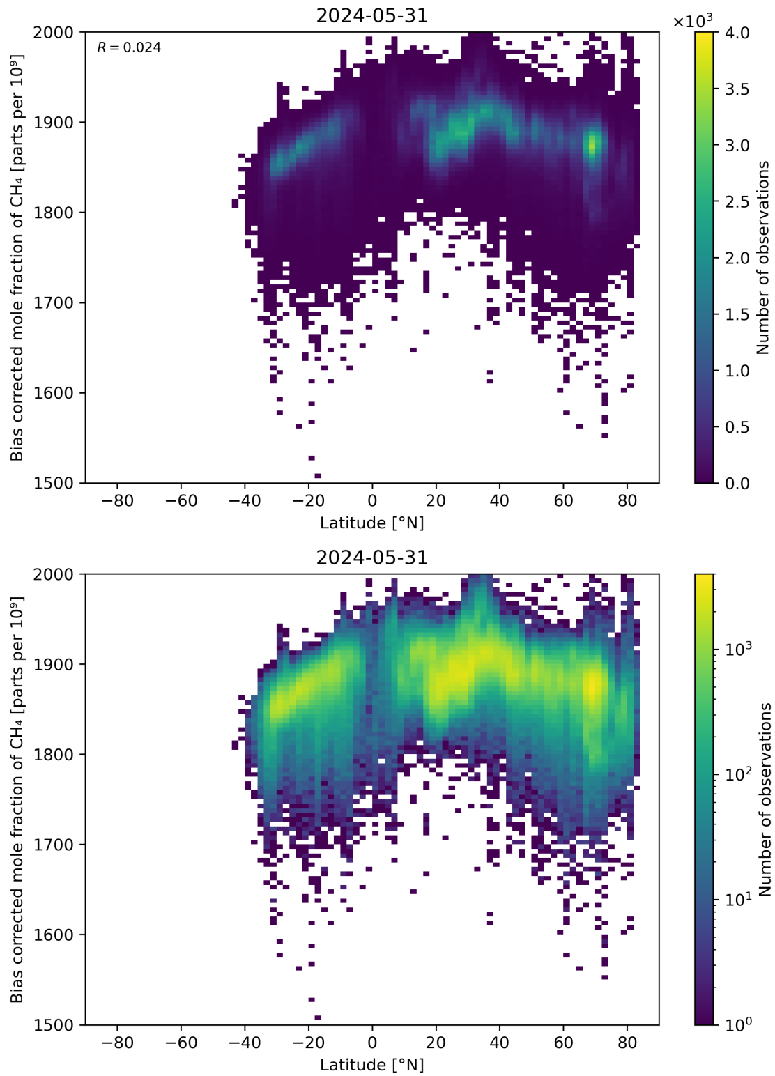
Figure 58: Scatter density plot of “Latitude” against “Bias corrected mole fraction of CH 4 ” for 2024-05-30 to 2024-06-01.
