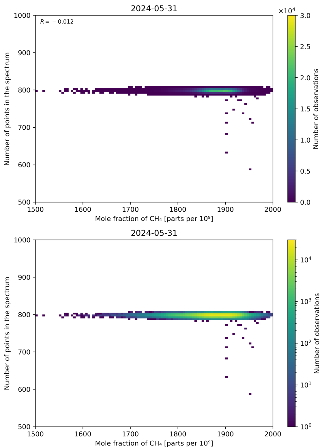
Figure 77: Scatter density plot of “Mole fraction of CH 4 ” against “Number of points in the spectrum” for 2024-05-30 to 2024-06-01.
