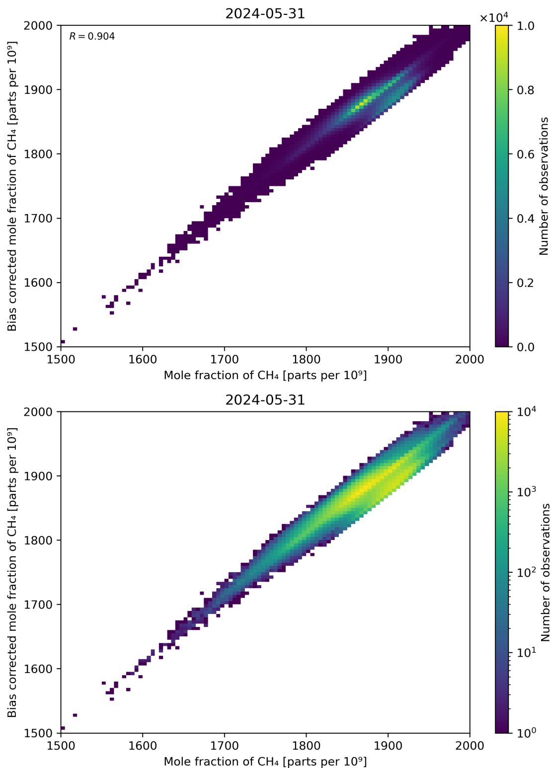
Figure 74: Scatter density plot of “Mole fraction of CH 4 ” against “Bias corrected mole fraction of CH 4 ” for 2024-05-30 to 2024-06-01.
