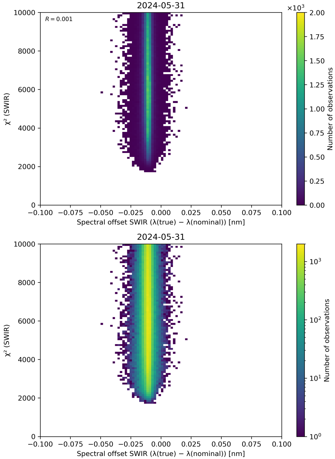
Figure 118: Scatter density plot of “Spectral offset SWIR ( \lambda(\text{true}) - \lambda(\text{nominal}) )” against “ \chi^2 (SWIR)” for 2024-05-30 to 2024-06-01.
