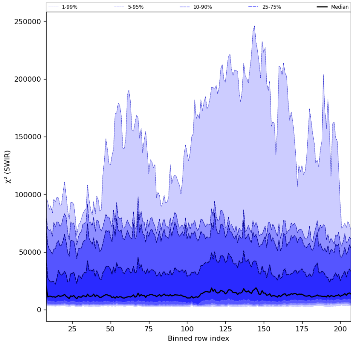
Figure 39: Along track statistics of “ \chi^2 (SWIR)” for 2024-05-30 to 2024-06-01
