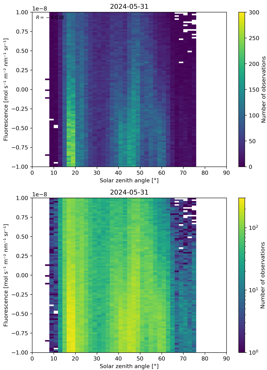
Figure 97: Scatter density plot of “Solar zenith angle” against “Fluorescence” for 2024-05-30 to 2024-06-01.
