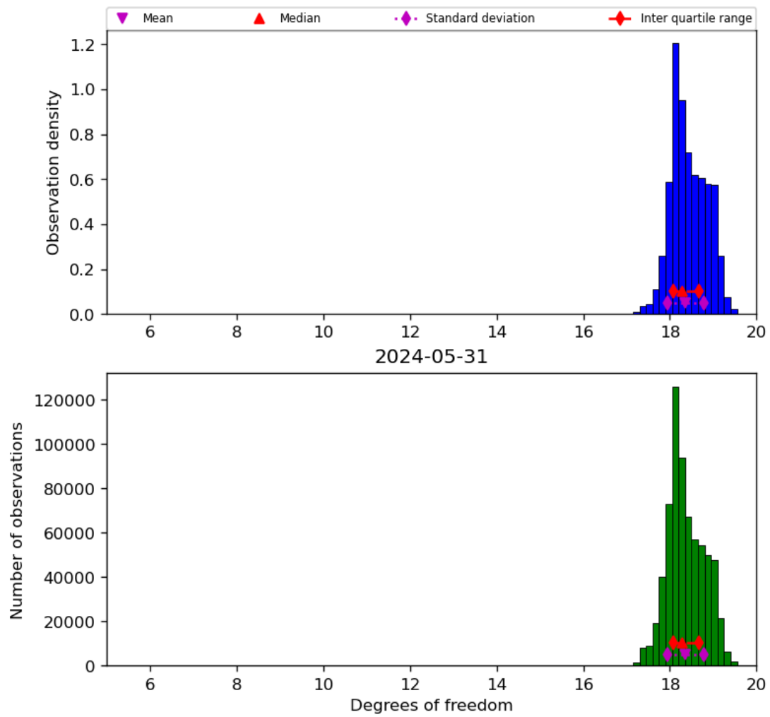
Figure 30: Histogram of “Degrees of freedom” for 2024-05-30 to 2024-06-01
