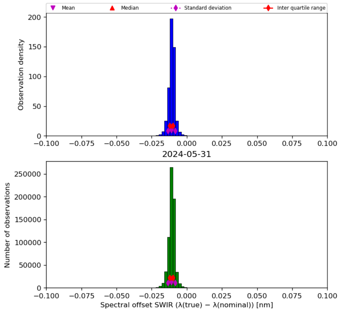
Figure 27: Histogram of “Spectral offset SWIR ( \lambda(\text{true}) - \lambda(\text{nominal}) )” for 2024-05-30 to 2024-06-01
