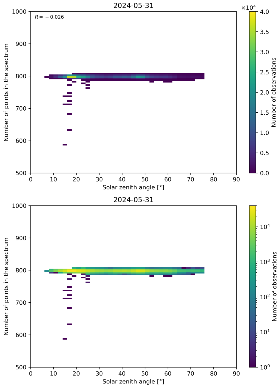
Figure 103: Scatter density plot of “Solar zenith angle” against “Number of points in the spectrum” for 2024-05-30 to 2024-06-01.
