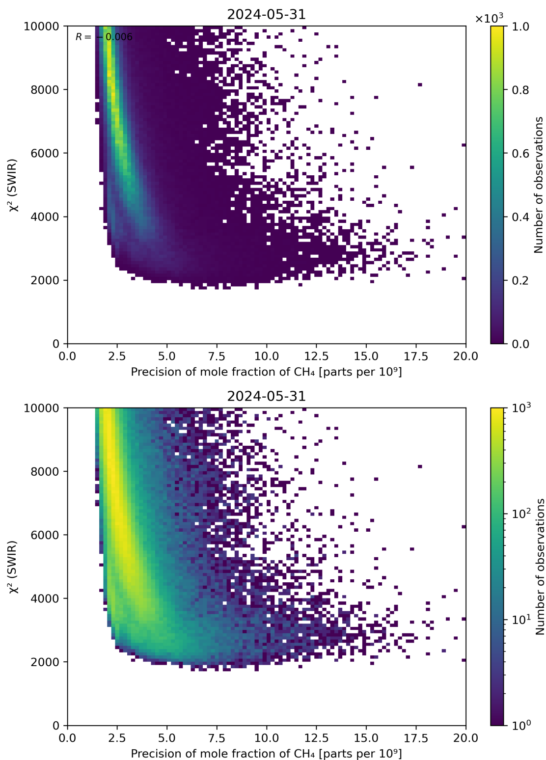
Figure 79: Scatter density plot of “Precision of mole fraction of \text{CH}_4 ” against “ \chi^2 (SWIR)” for 2024-05-30 to 2024-06-01.
