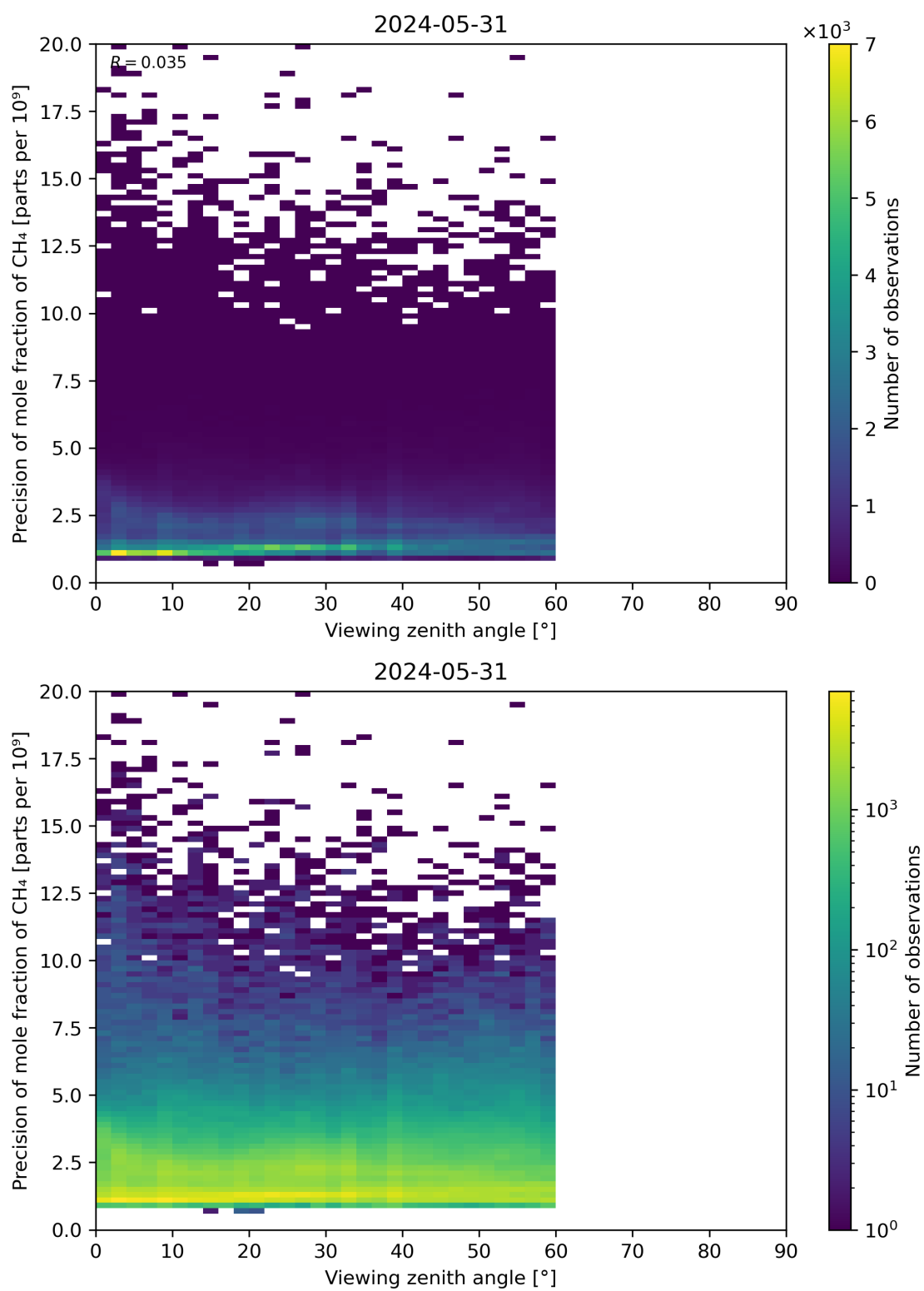
Figure 112: Scatter density plot of “Viewing zenith angle” against “Precision of mole fraction of CH 4 ” for 2024-05-30 to 2024-06-01.
