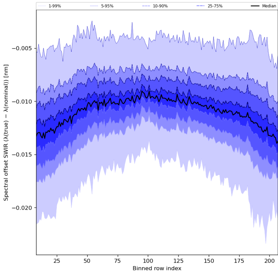
Figure 38: Along track statistics of “Spectral offset SWIR ( \lambda(\text{true}) - \lambda(\text{nominal}) )” for 2024-05-30 to 2024-06-01
