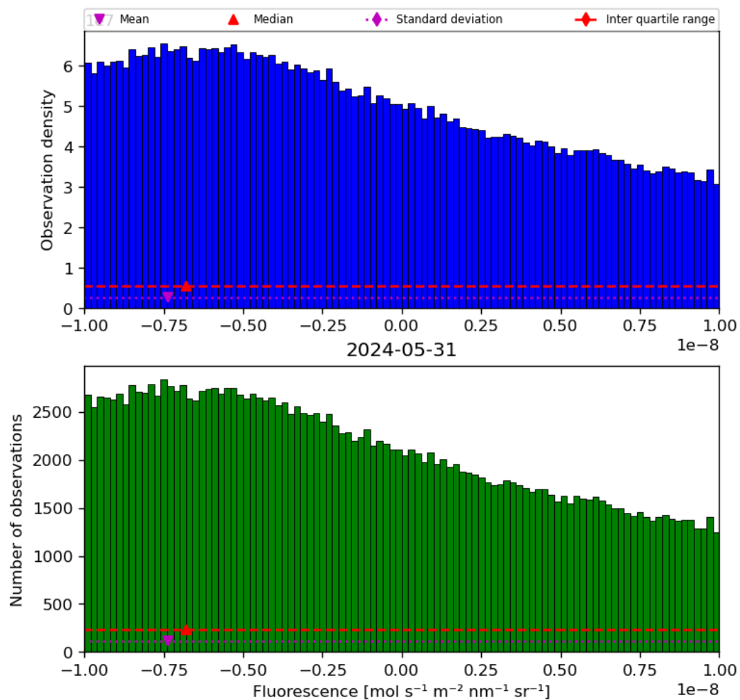
Figure 32: Histogram of “Fluorescence” for 2024-05-30 to 2024-06-01
