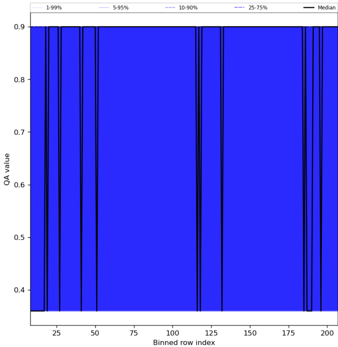
Figure 33: Along track statistics of “QA value” for 2024-05-30 to 2024-06-01
