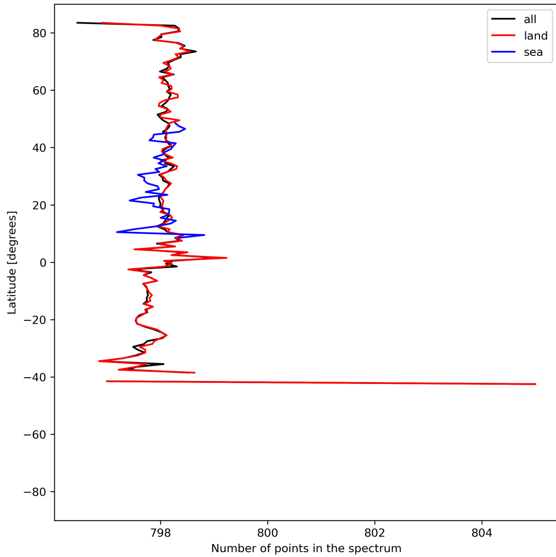
Figure 15: Zonal average of “Number of points in the spectrum” for 2024-05-30 to 2024-06-01.
