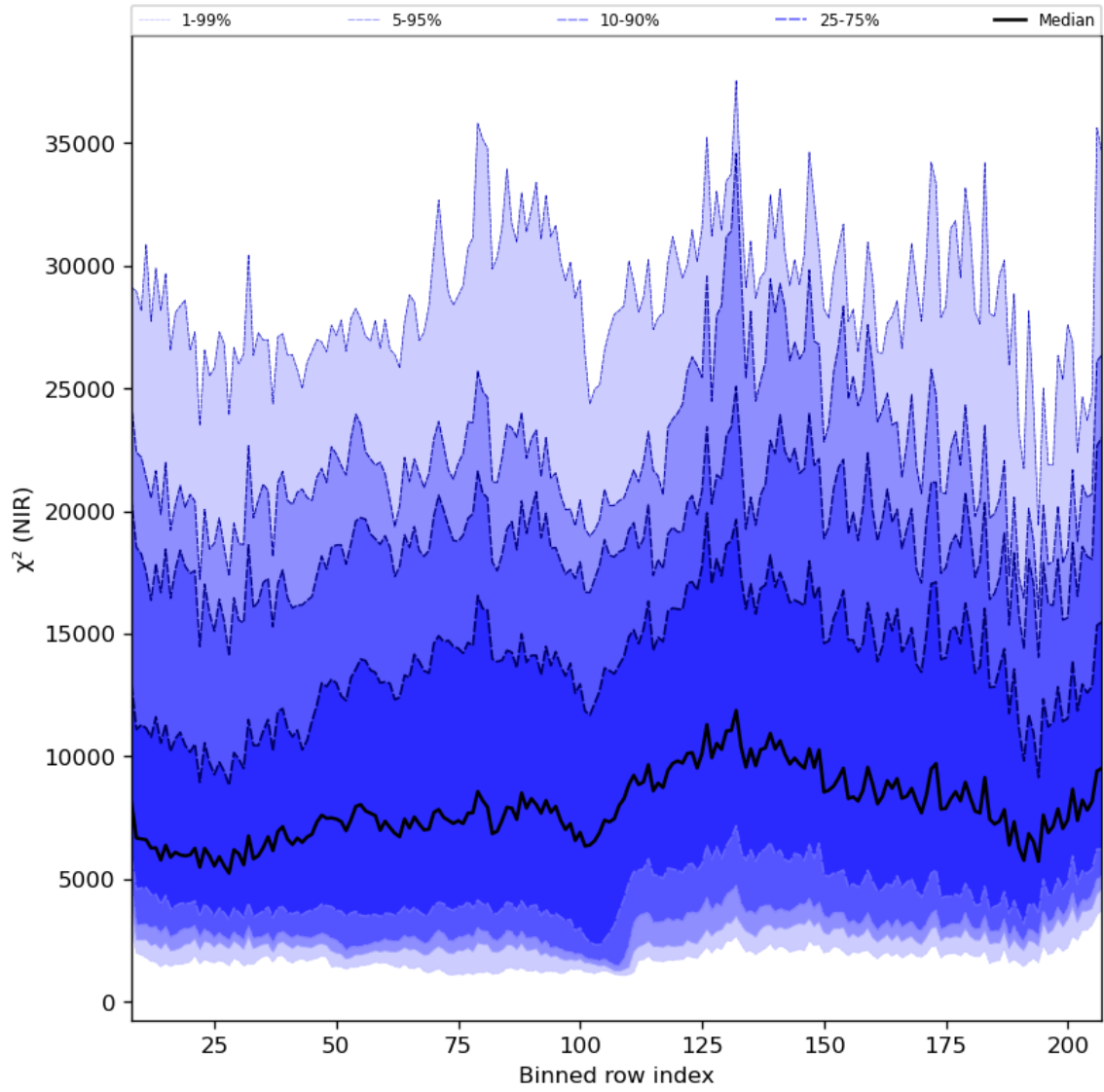
Figure 40: Along track statistics of “ \chi^2 (NIR)” for 2024-05-30 to 2024-06-01
