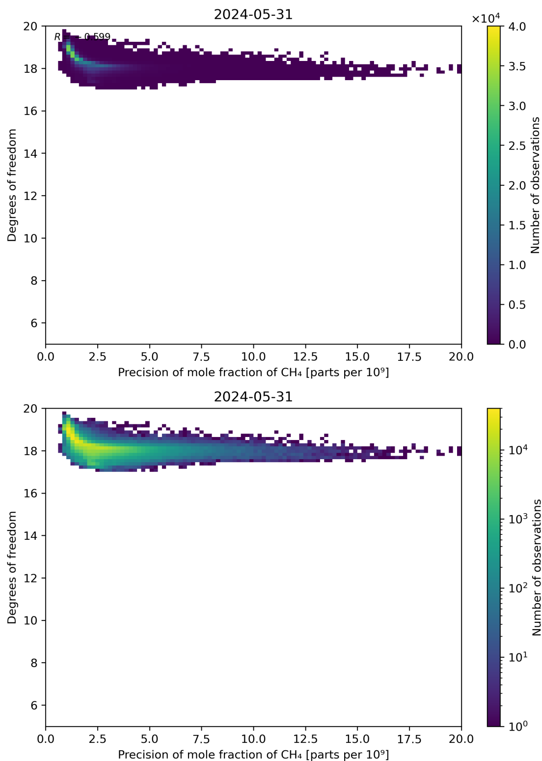
Figure 80: Scatter density plot of “Precision of mole fraction of CH 4 ” against “Degrees of freedom” for 2024-05-30 to 2024-06-01.
