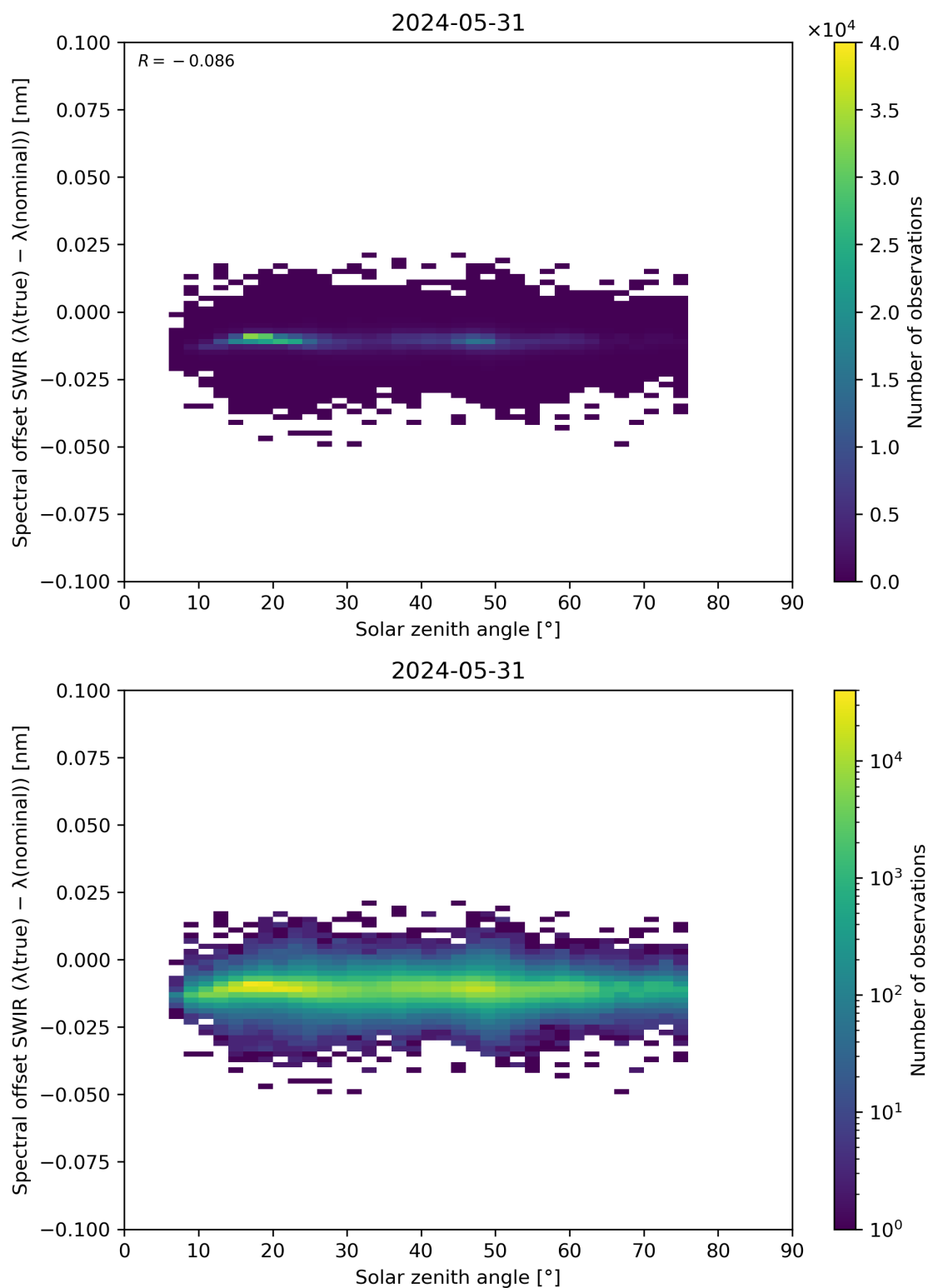
Figure 104: Scatter density plot of “Solar zenith angle” against “Spectral offset SWIR ( \lambda(\text{true}) - \lambda(\text{nominal}) )” for 2024-05-30 to 2024-06-01.
