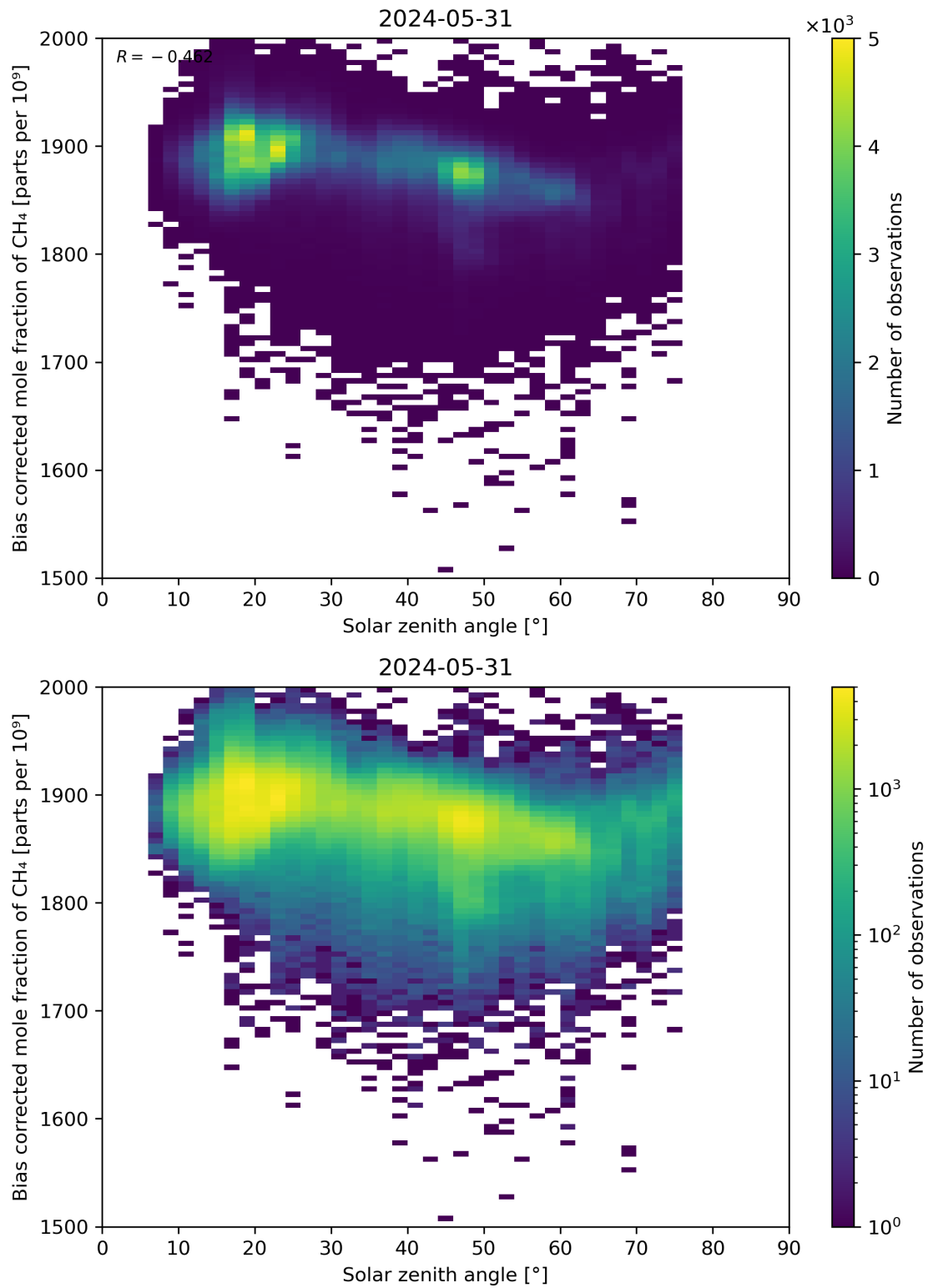
Figure 100: Scatter density plot of “Solar zenith angle” against “Bias corrected mole fraction of CH 4 ” for 2024-05-30 to 2024-06-01.
