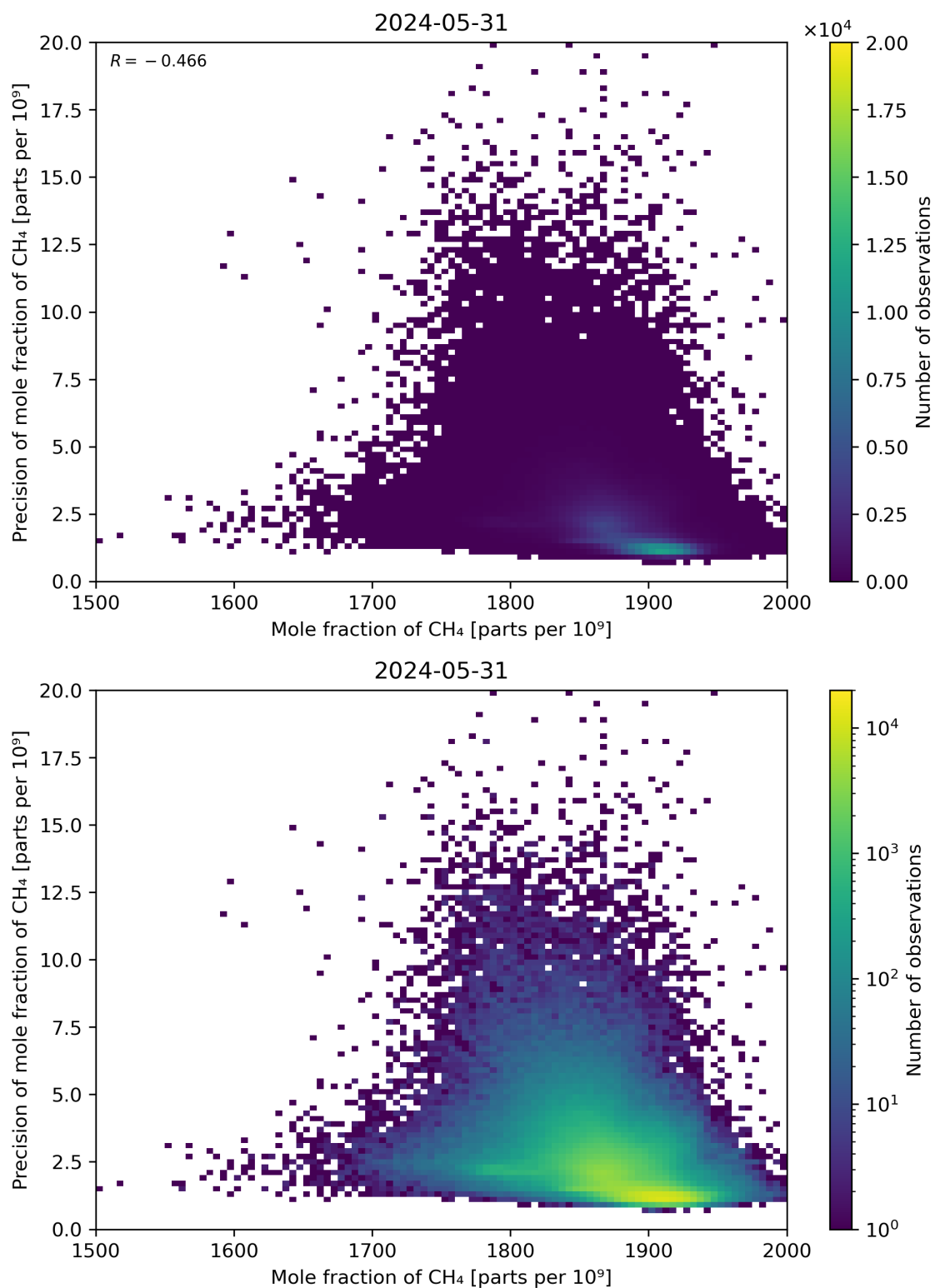
Figure 75: Scatter density plot of “Mole fraction of CH 4 ” against “Precision of mole fraction of CH 4 ” for 2024-05-30 to 2024-06-01.
