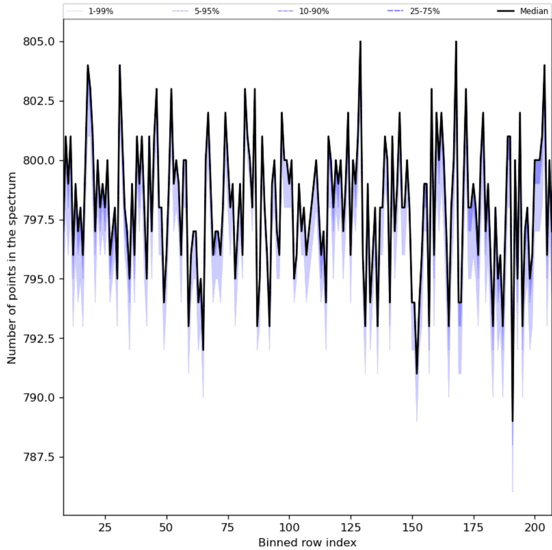
Figure 37: Along track statistics of “Number of points in the spectrum” for 2024-05-30 to 2024-06-01
