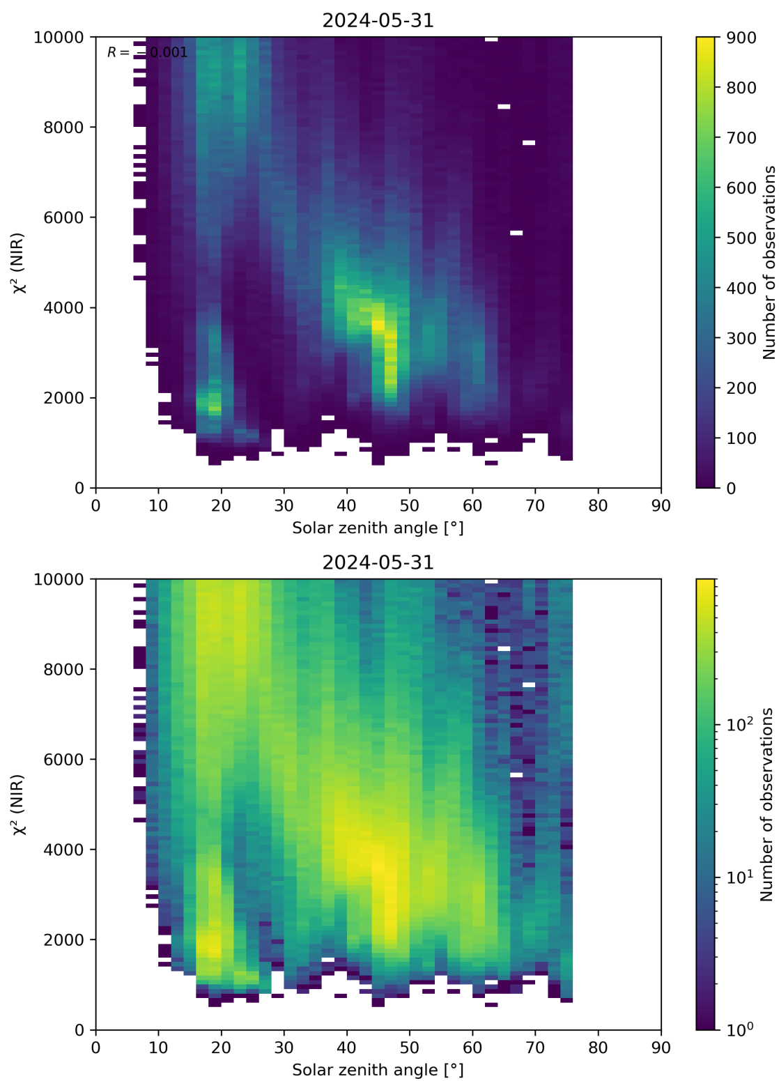
Figure 94: Scatter density plot of “Solar zenith angle” against “ \chi^2 (NIR)” for 2024-05-30 to 2024-06-01.
