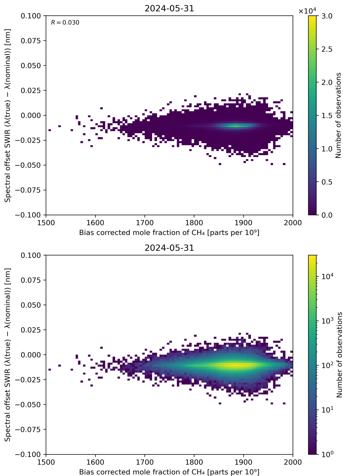
Figure 69: Scatter density plot of “Bias corrected mole fraction of \text{CH}_4 ” against “Spectral offset SWIR ( \lambda(\text{true}) - \lambda(\text{nominal}) )” for 2024-05-30 to 2024-06-01.
