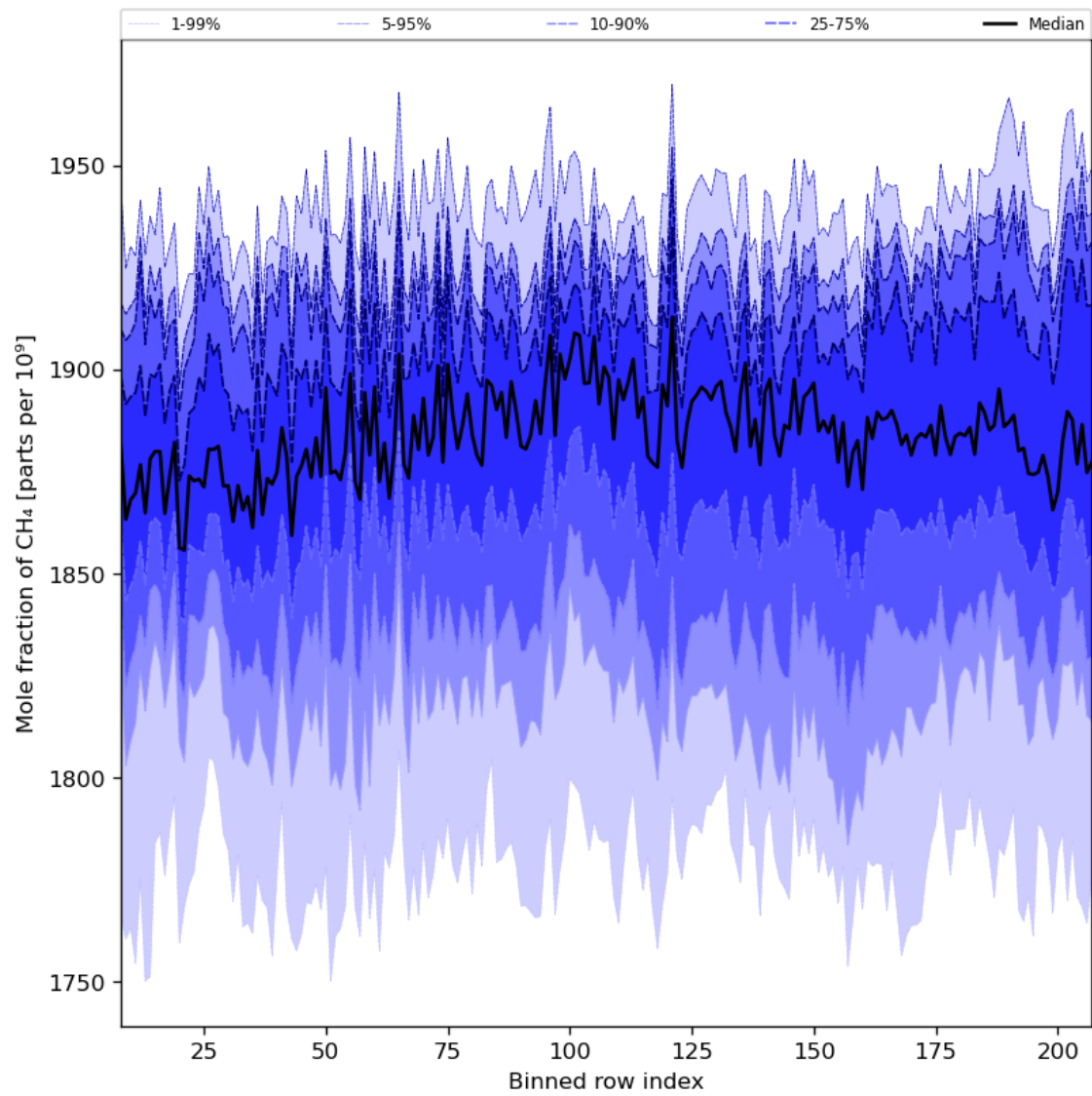
Figure 34: Along track statistics of “Mole fraction of CH 4 ” for 2024-05-30 to 2024-06-01
