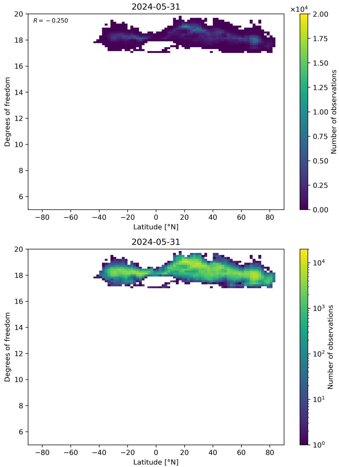
Figure 55: Scatter density plot of “Latitude” against “Degrees of freedom” for 2024-05-30 to 2024-06-01.
