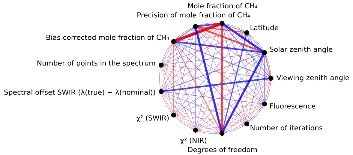
Figure 1: Map of correlation graph for 2024-05-30 to 2024-06-01.
