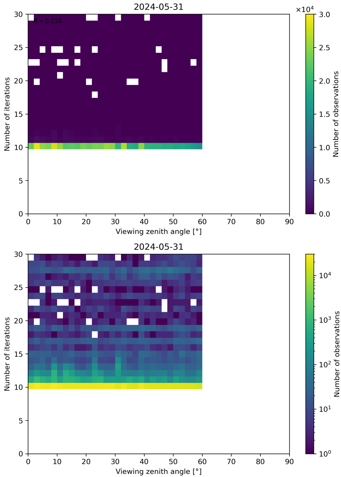
Figure 113: Scatter density plot of “Viewing zenith angle” against “Number of iterations” for 2024-05-30 to 2024-06-01.
