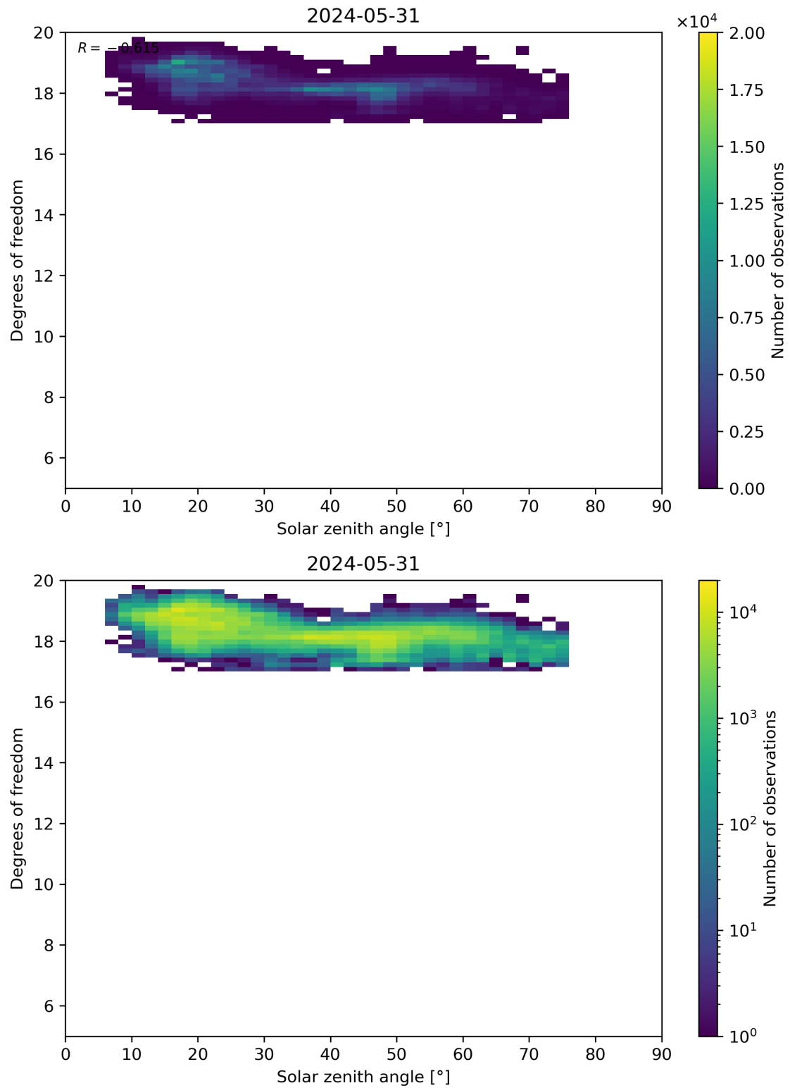
Figure 96: Scatter density plot of “Solar zenith angle” against “Degrees of freedom” for 2024-05-30 to 2024-06-01.
