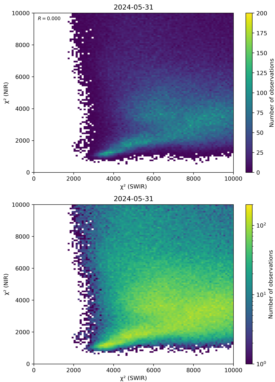
Figure 47: Scatter density plot of “ \chi^2 (SWIR)” against “ \chi^2 (NIR)” for 2024-05-30 to 2024-06-01.
