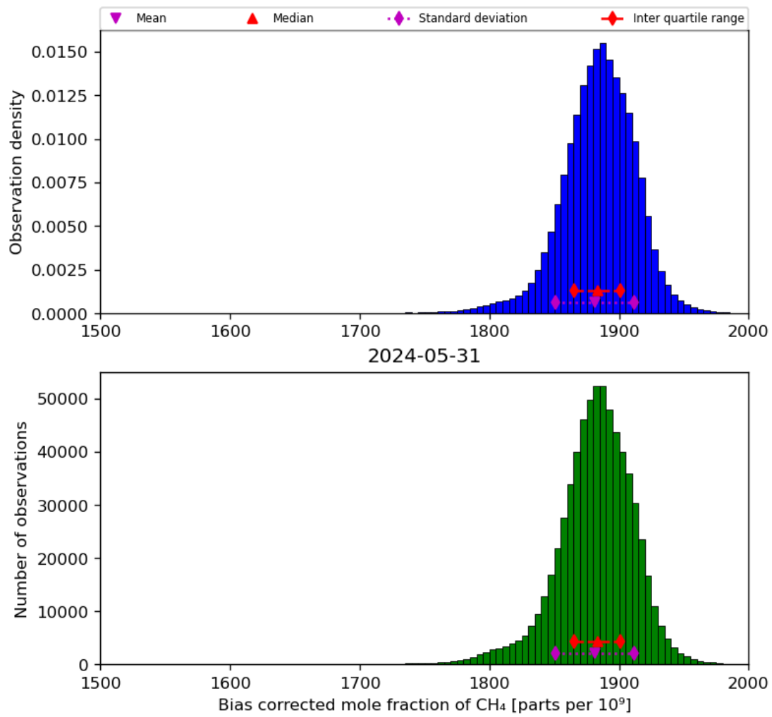
Figure 25: Histogram of “Bias corrected mole fraction of CH 4 ” for 2024-05-30 to 2024-06-01
