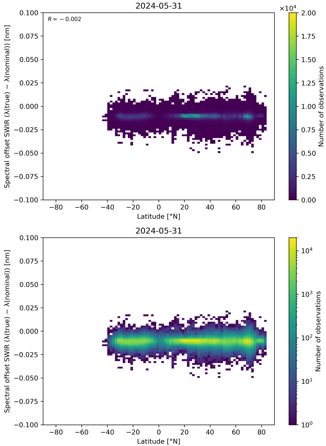
Figure 62: Scatter density plot of “Latitude” against “Spectral offset SWIR ( \lambda(\text{true}) - \lambda(\text{nominal}) )” for 2024-05-30 to 2024-06-01.
