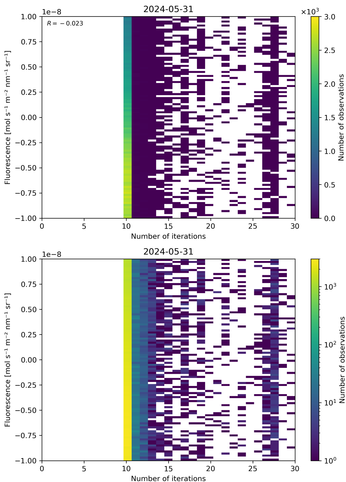
Figure 87: Scatter density plot of “Number of iterations” against “Fluorescence” for 2024-05-30 to 2024-06-01.
