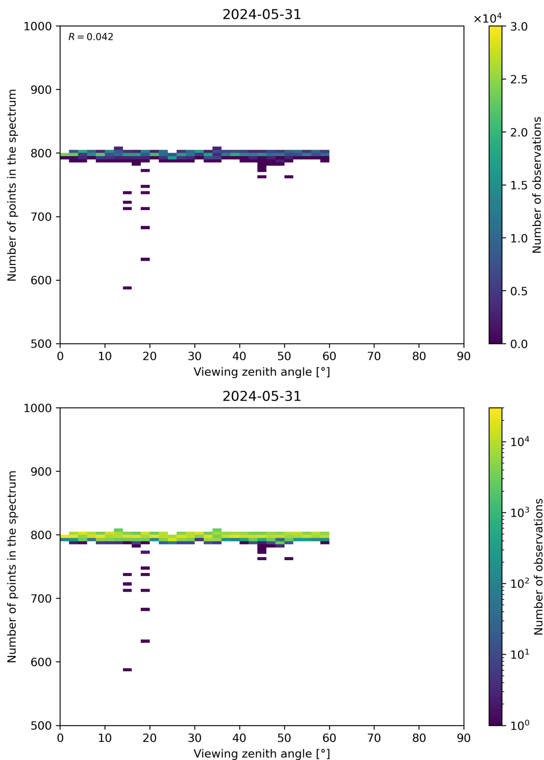
Figure 114: Scatter density plot of “Viewing zenith angle” against “Number of points in the spectrum” for 2024-05-30 to 2024-06-01.
