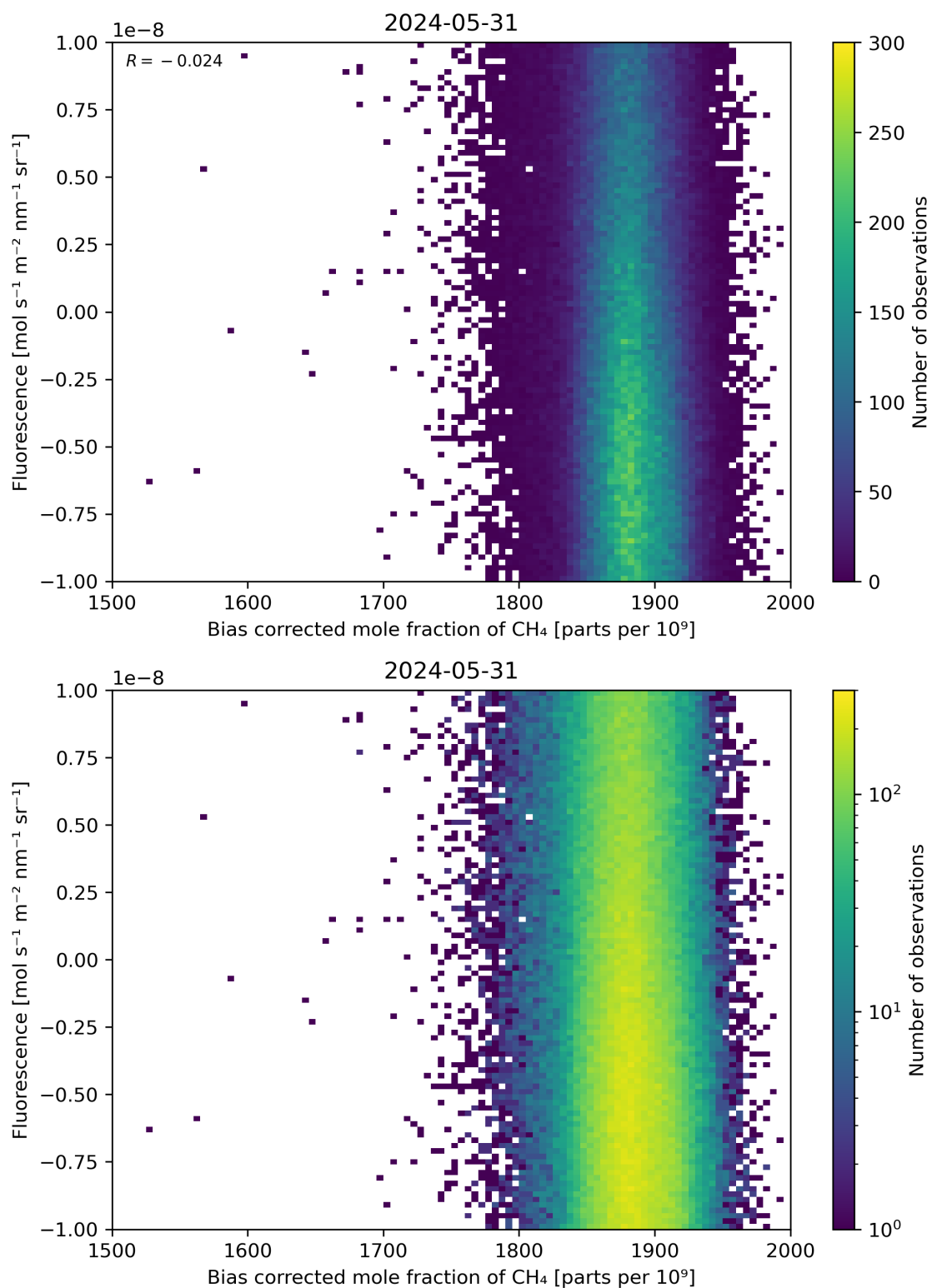
Figure 66: Scatter density plot of “Bias corrected mole fraction of \text{CH}_4 ” against “Fluorescence” for 2024-05-30 to 2024-06-01.
