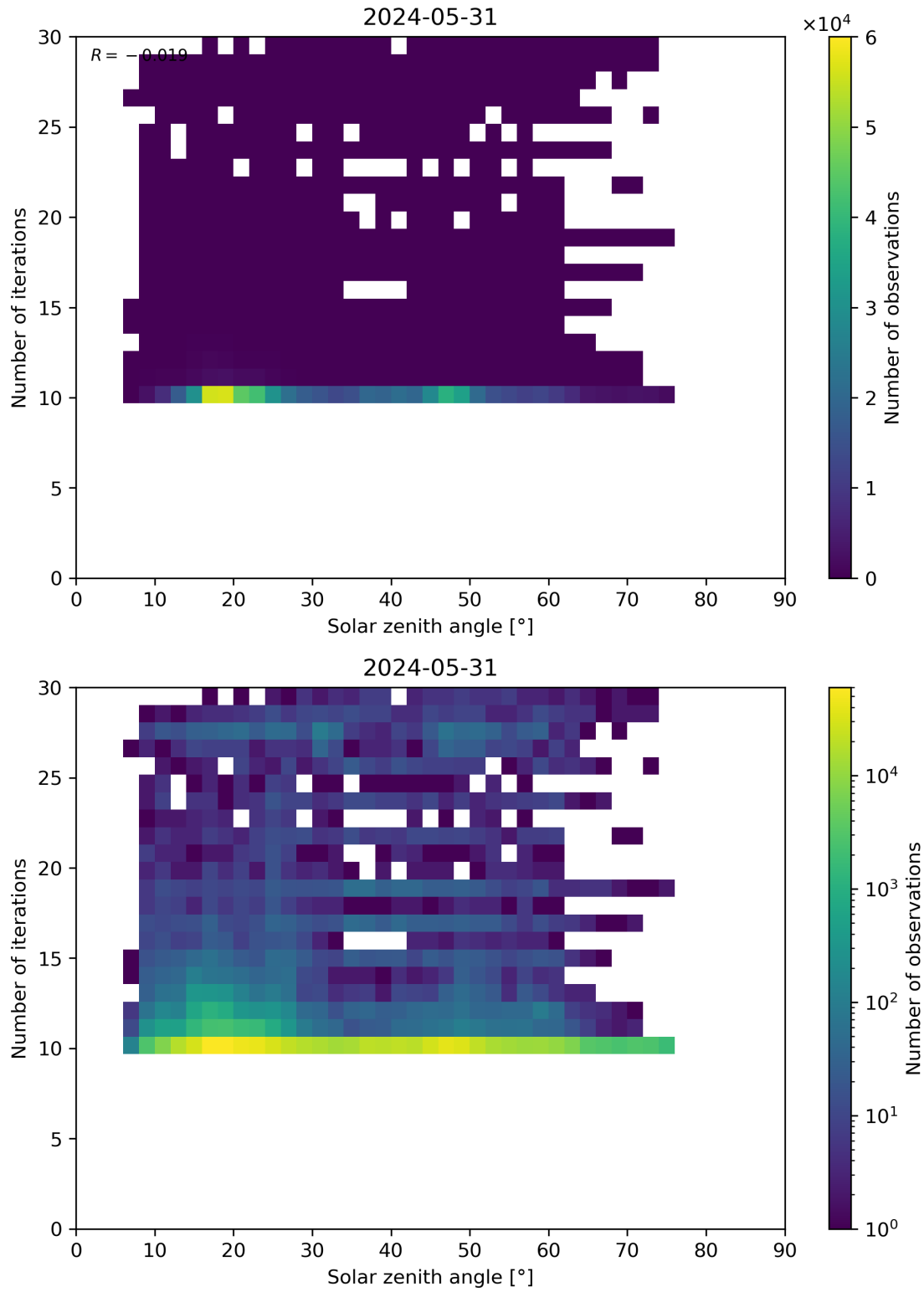
Figure 102: Scatter density plot of “Solar zenith angle” against “Number of iterations” for 2024-05-30 to 2024-06-01.
