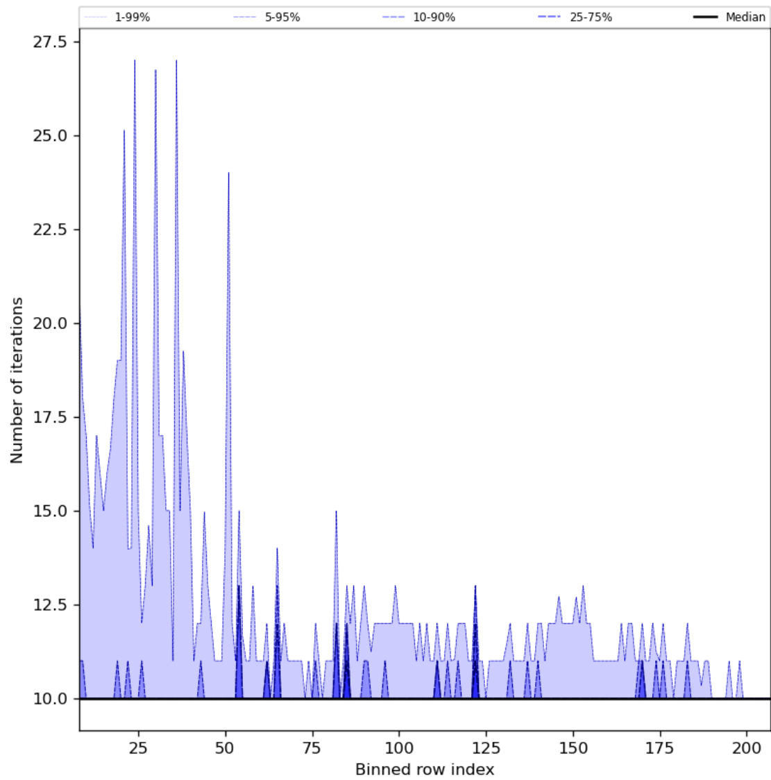
Figure 42: Along track statistics of “Number of iterations” for 2024-05-30 to 2024-06-01
