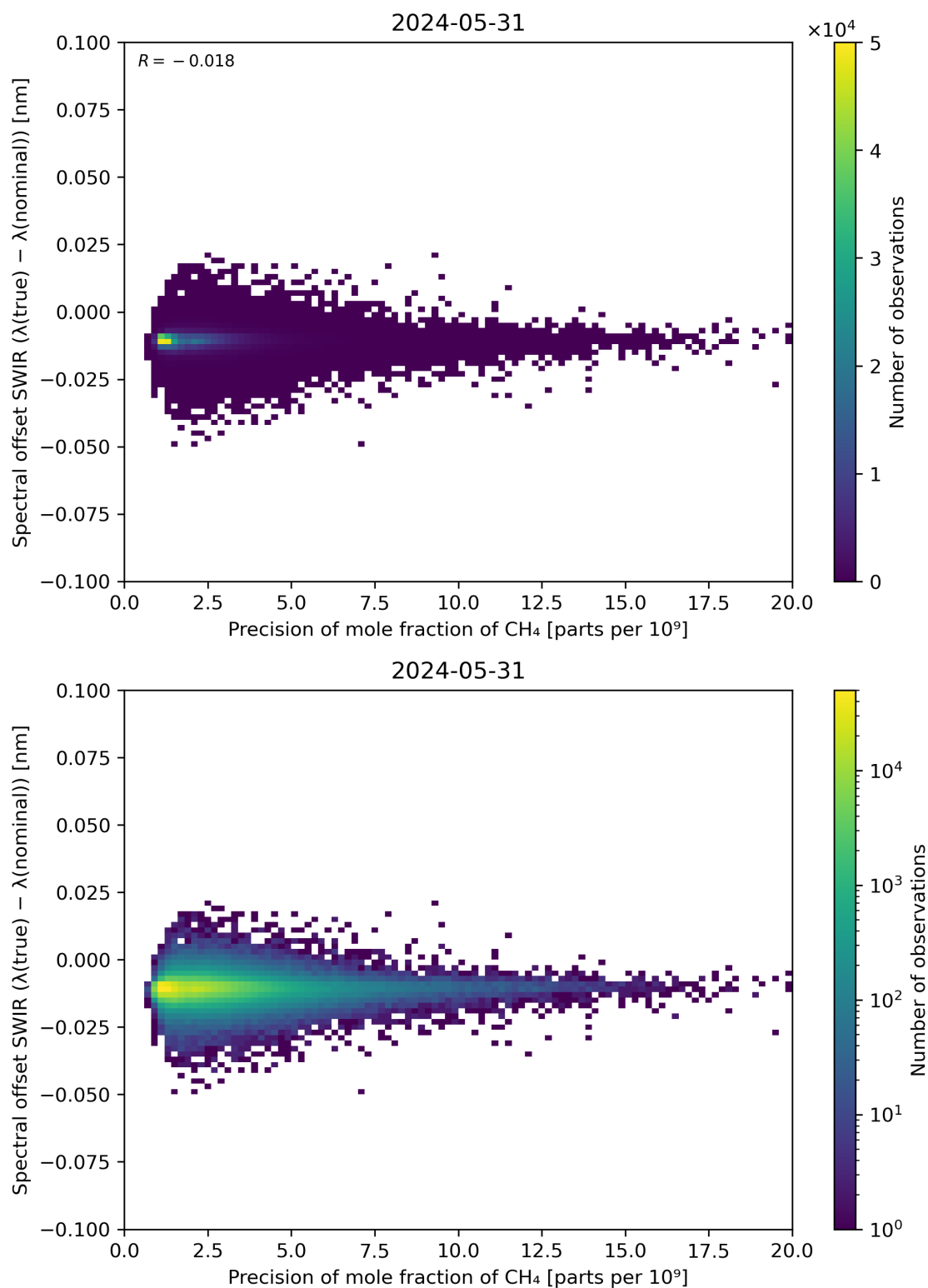
Figure 85: Scatter density plot of “Precision of mole fraction of CH 4 ” against “Spectral offset SWIR ( \lambda(\text{true}) - \lambda(\text{nominal}) )” for 2024-05-30 to 2024-06-01.
