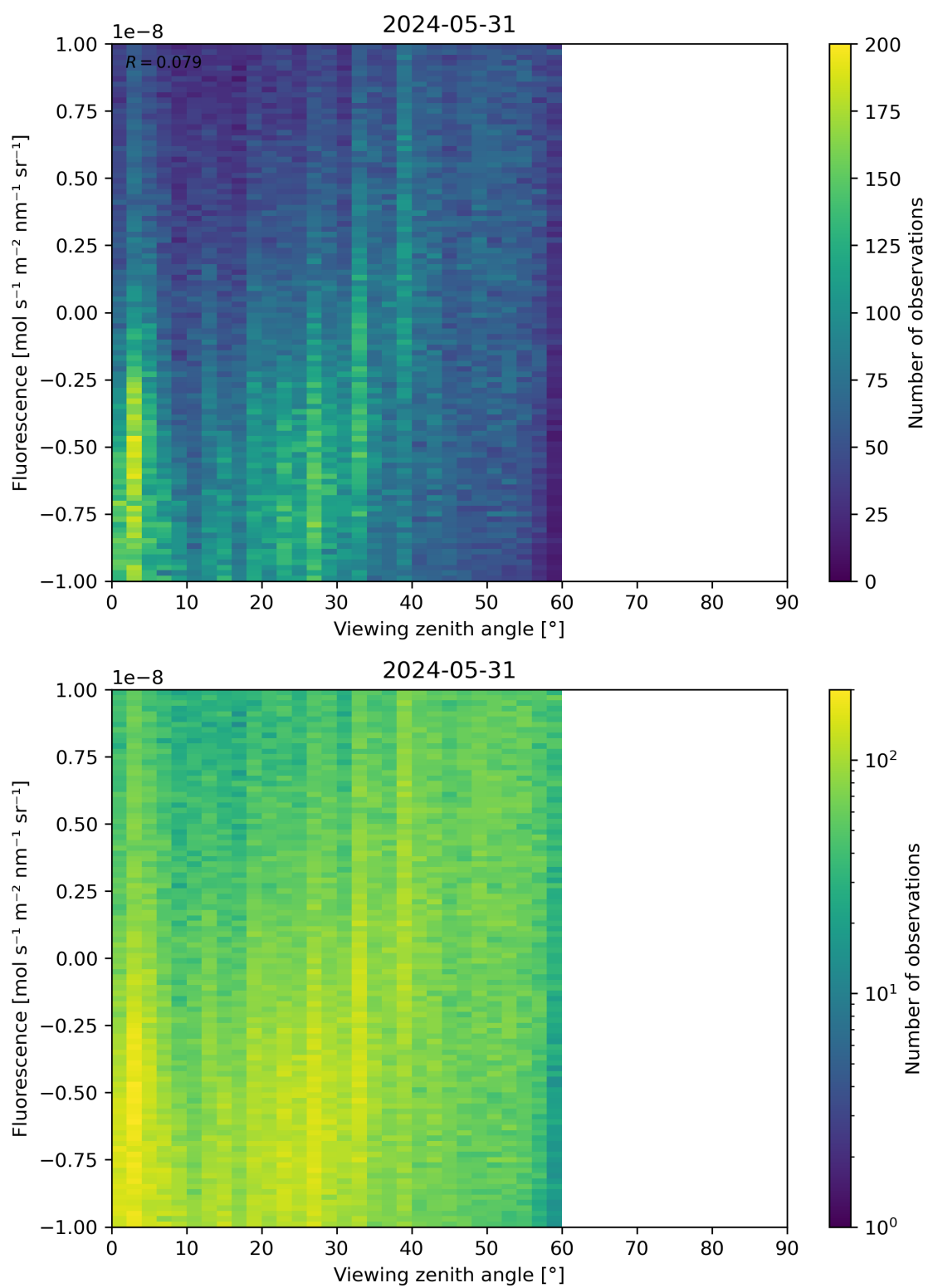
Figure 108: Scatter density plot of “Viewing zenith angle” against “Fluorescence” for 2024-05-30 to 2024-06-01.
