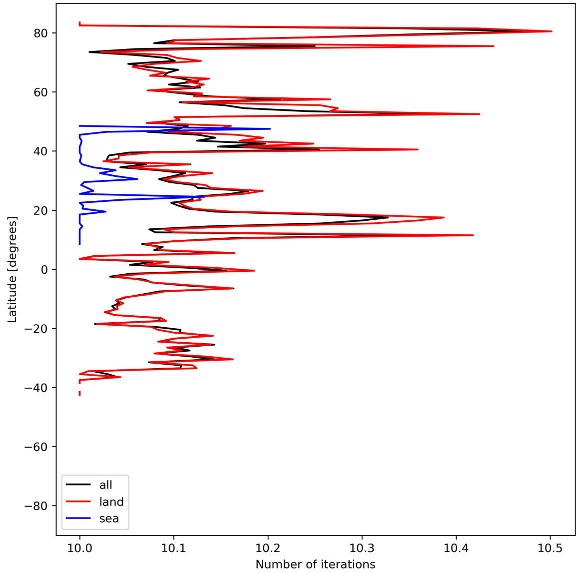
Figure 20: Zonal average of “Number of iterations” for 2024-05-30 to 2024-06-01.
