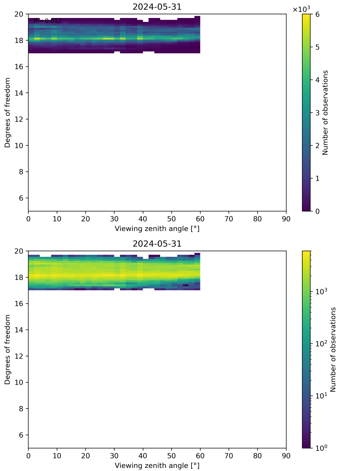
Figure 107: Scatter density plot of “Viewing zenith angle” against “Degrees of freedom” for 2024-05-30 to 2024-06-01.
