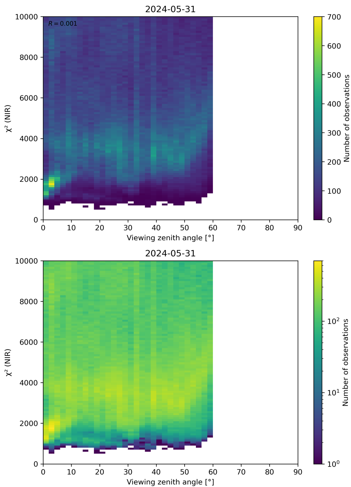
Figure 105: Scatter density plot of “Viewing zenith angle” against “ \chi^2 (NIR)” for 2024-05-30 to 2024-06-01.
