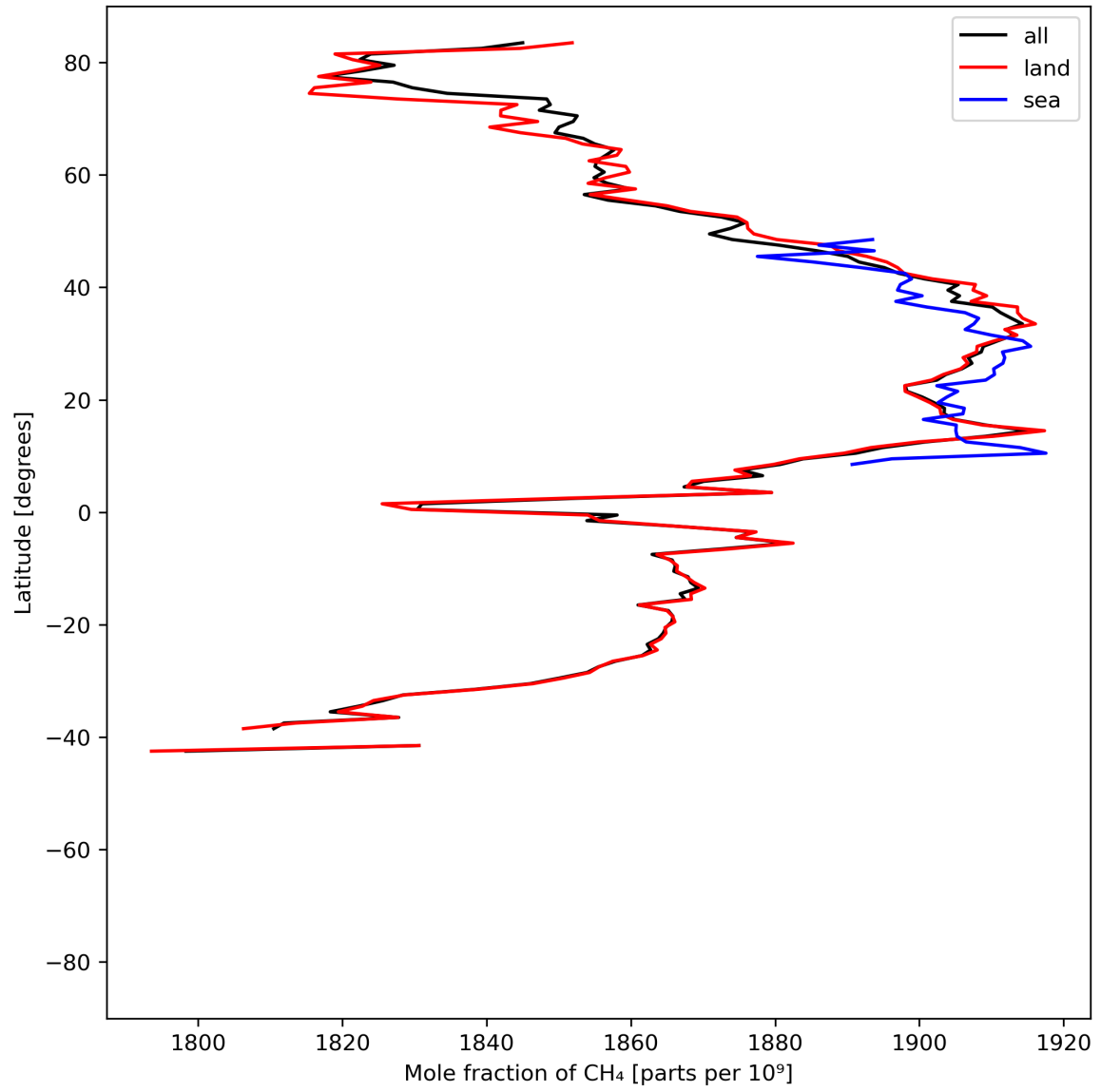
Figure 12: Zonal average of “Mole fraction of \text{CH}_4 ” for 2024-05-30 to 2024-06-01.
