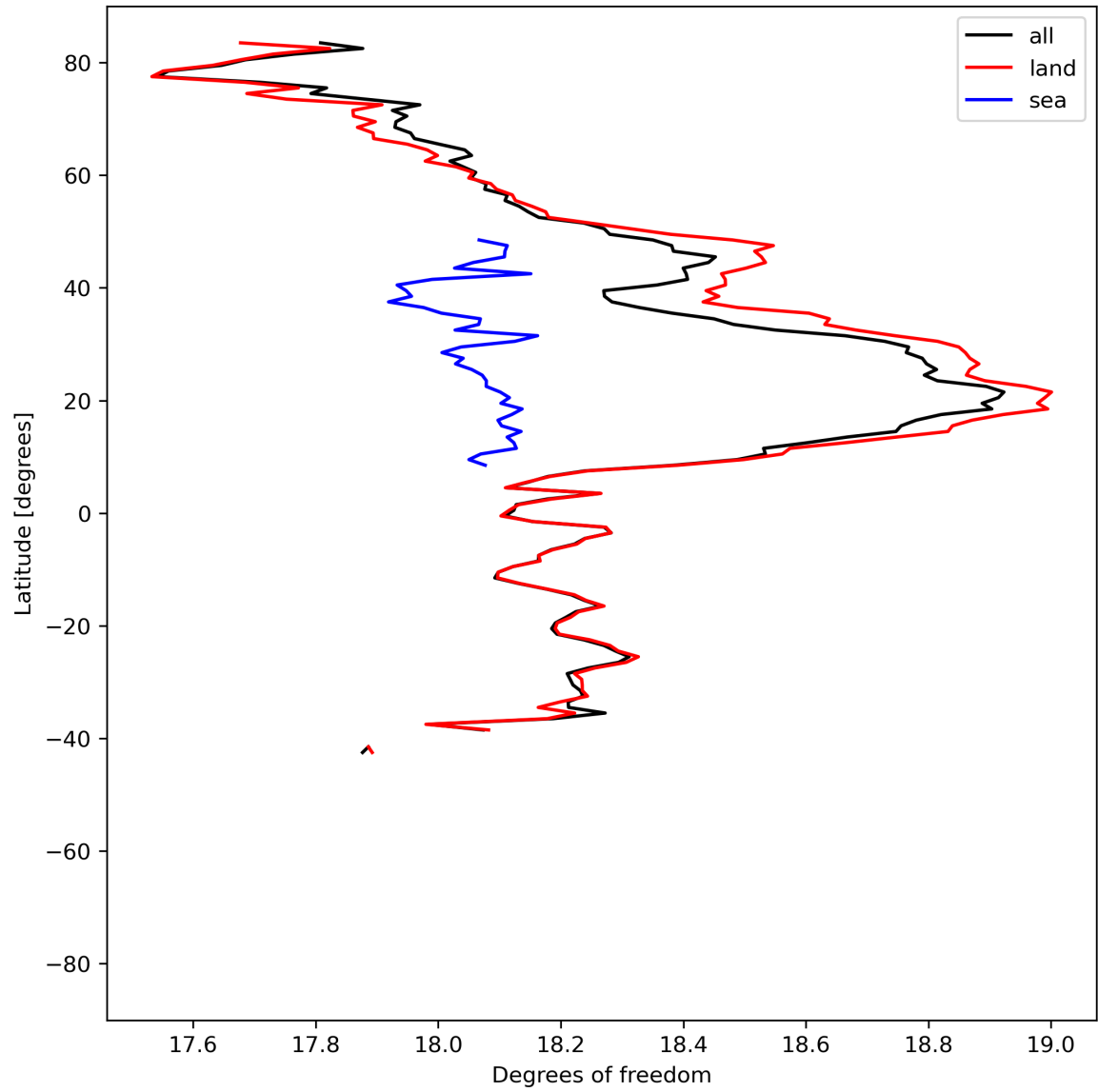
Figure 19: Zonal average of “Degrees of freedom” for 2024-05-30 to 2024-06-01.
