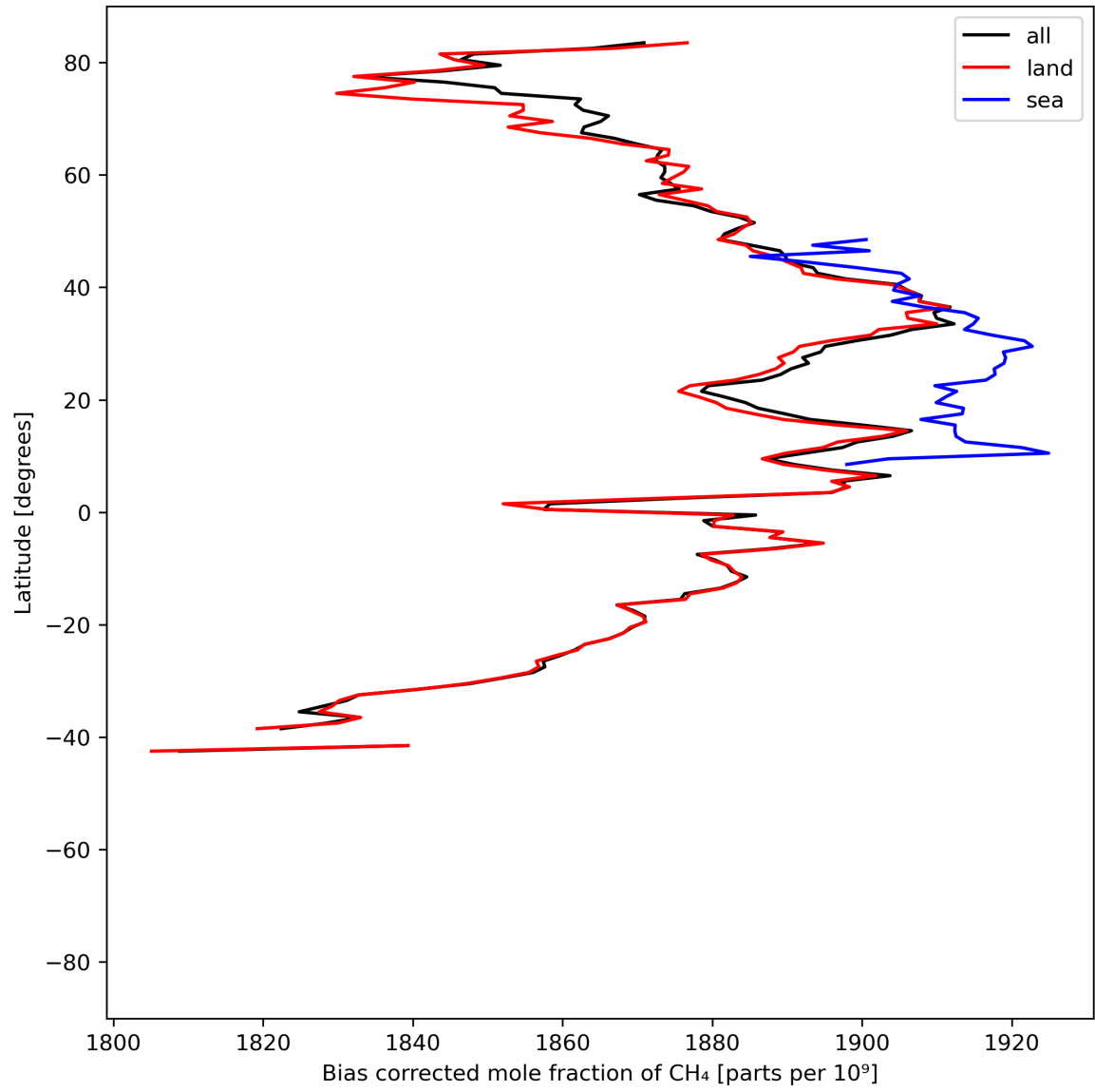
Figure 14: Zonal average of “Bias corrected mole fraction of \text{CH}_4 ” for 2024-05-30 to 2024-06-01.
