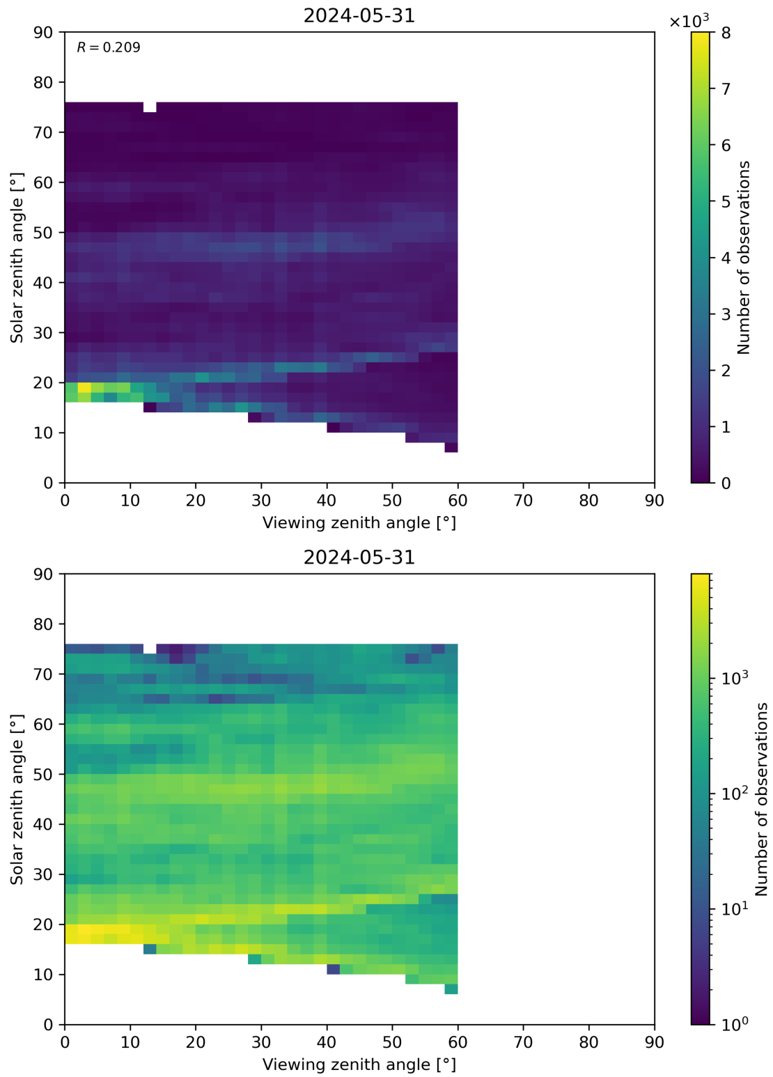
Figure 115: Scatter density plot of “Viewing zenith angle” against “Solar zenith angle” for 2024-05-30 to 2024-06-01.
