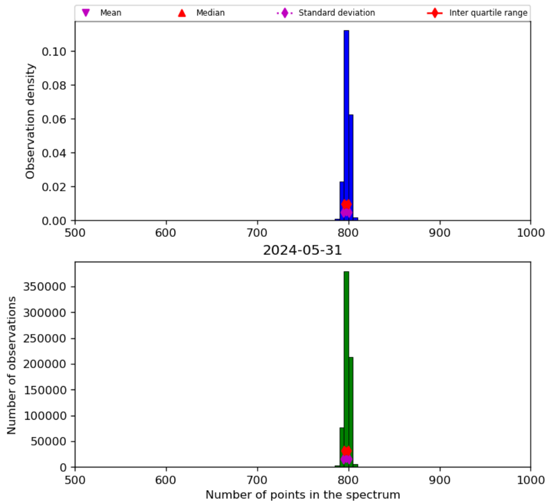
Figure 26: Histogram of “Number of points in the spectrum” for 2024-05-30 to 2024-06-01
