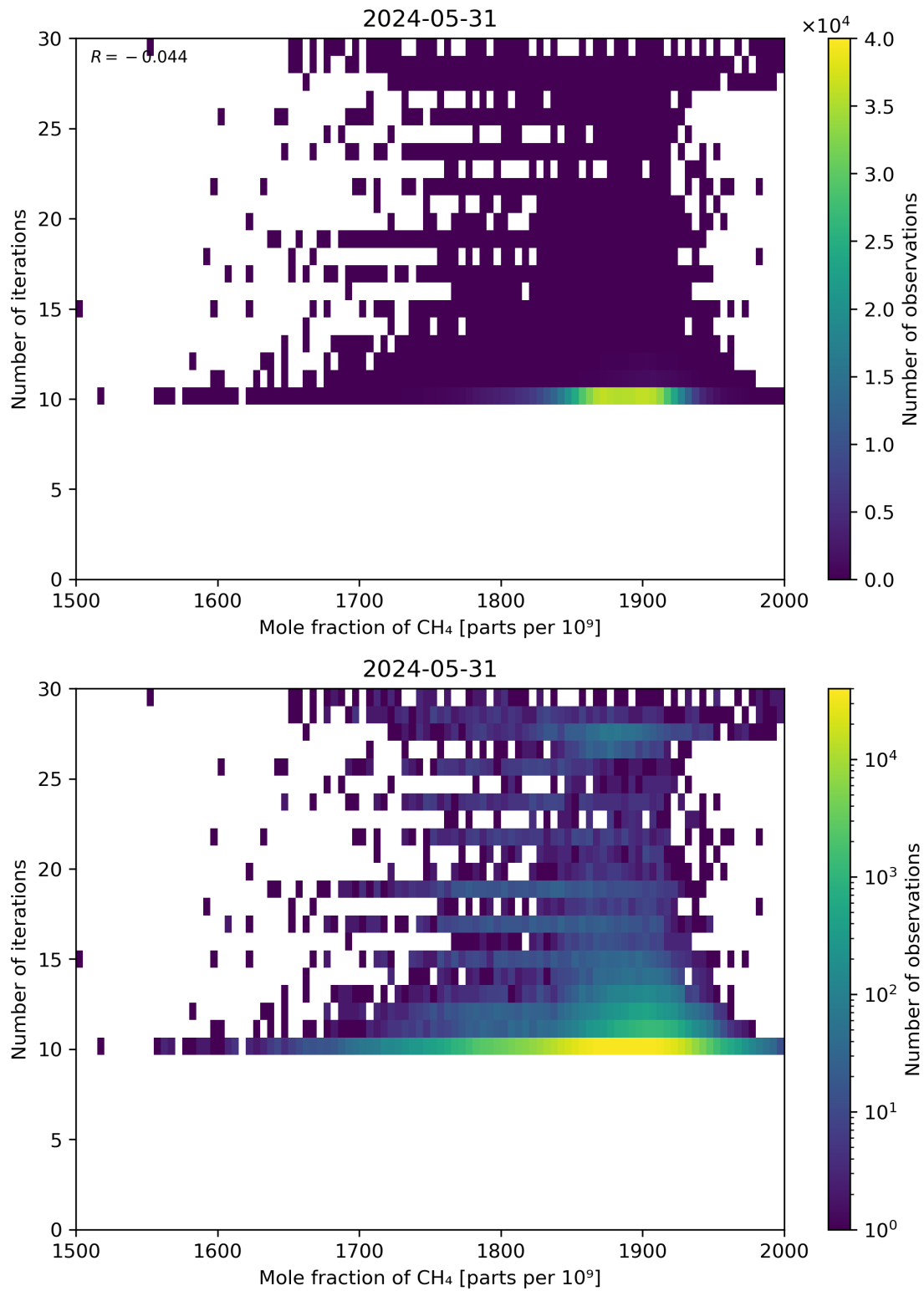
Figure 76: Scatter density plot of “Mole fraction of CH 4 ” against “Number of iterations” for 2024-05-30 to 2024-06-01.
