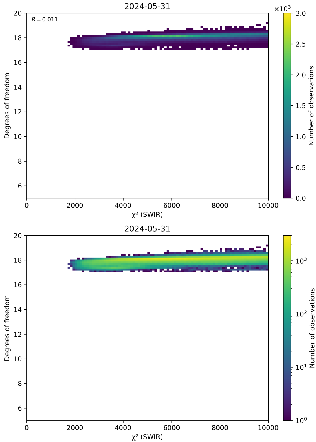
Figure 48: Scatter density plot of " \chi^2 (SWIR)" against "Degrees of freedom" for 2024-05-30 to 2024-06-01.
