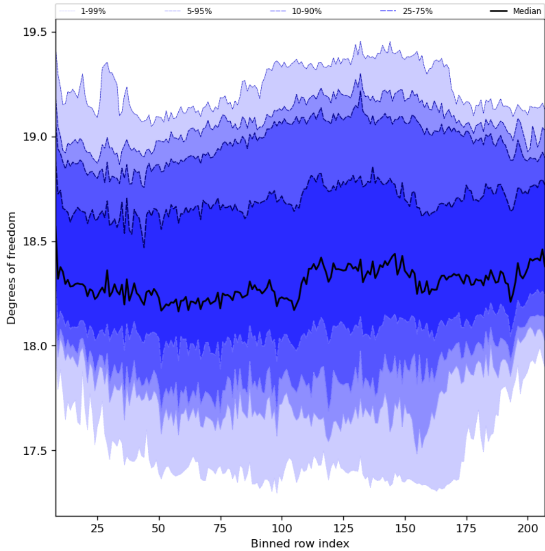
Figure 41: Along track statistics of “Degrees of freedom” for 2024-05-30 to 2024-06-01
