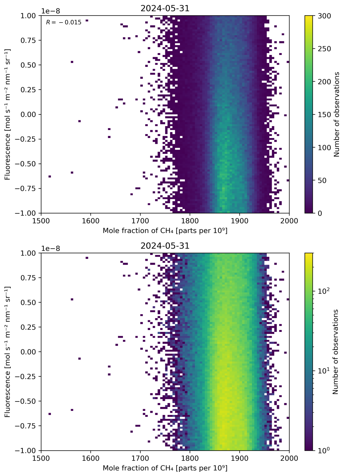
Figure 73: Scatter density plot of “Mole fraction of CH 4 ” against “Fluorescence” for 2024-05-30 to 2024-06-01.
