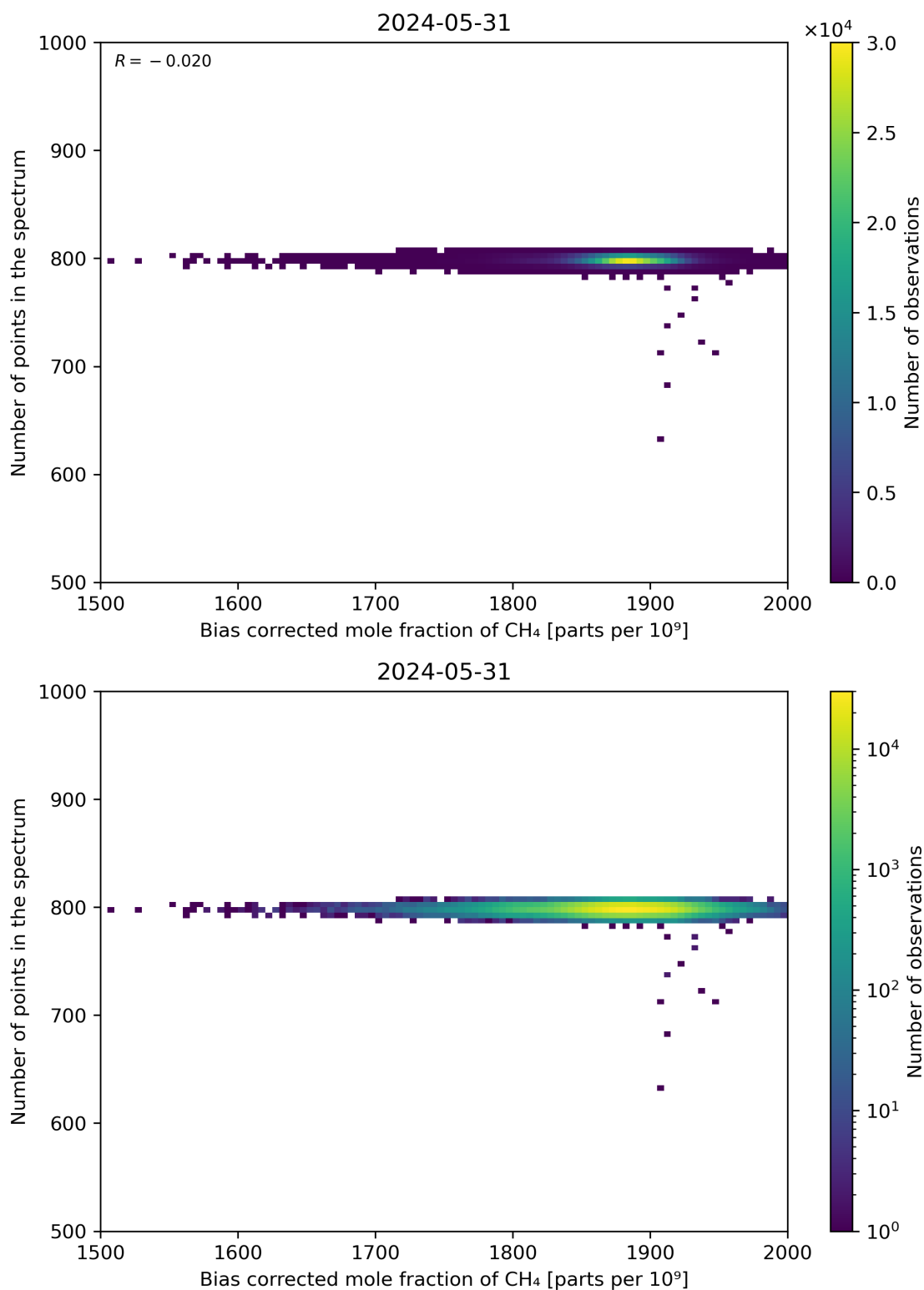
Figure 68: Scatter density plot of “Bias corrected mole fraction of CH 4 ” against “Number of points in the spectrum” for 2024-05-30 to 2024-06-01.
