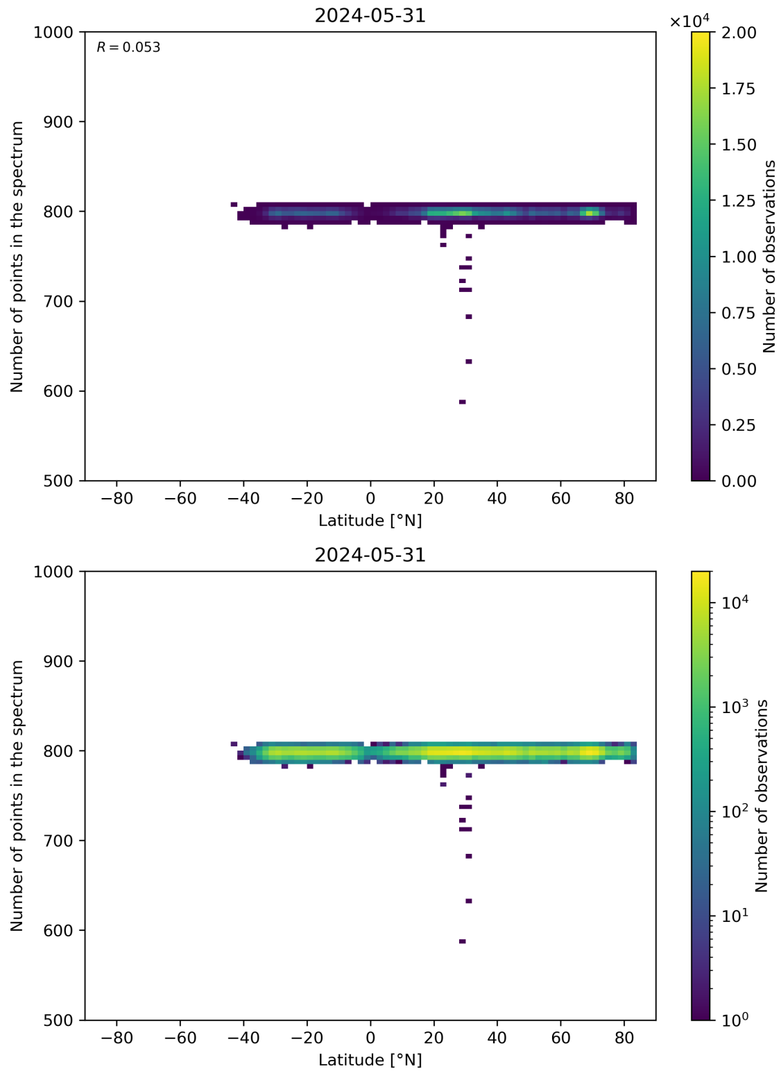
Figure 61: Scatter density plot of “Latitude” against “Number of points in the spectrum” for 2024-05-30 to 2024-06-01.
