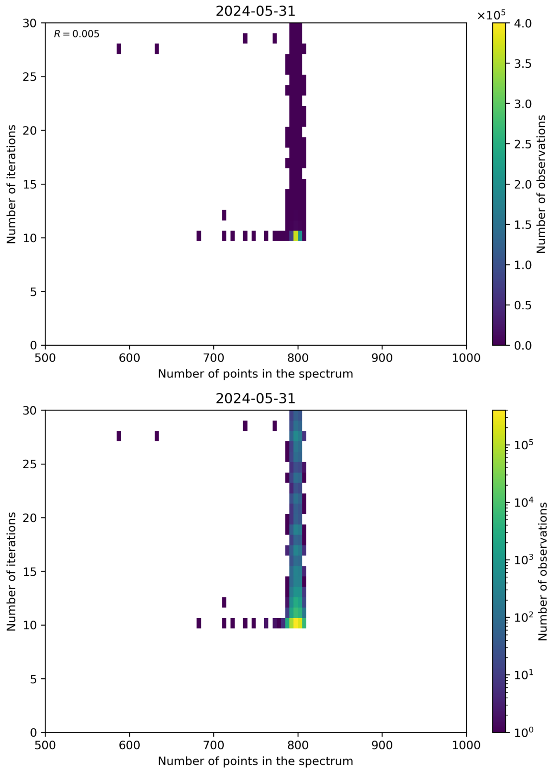
Figure 92: Scatter density plot of “Number of points in the spectrum” against “Number of iterations” for 2024-05-30 to 2024-06-01.
