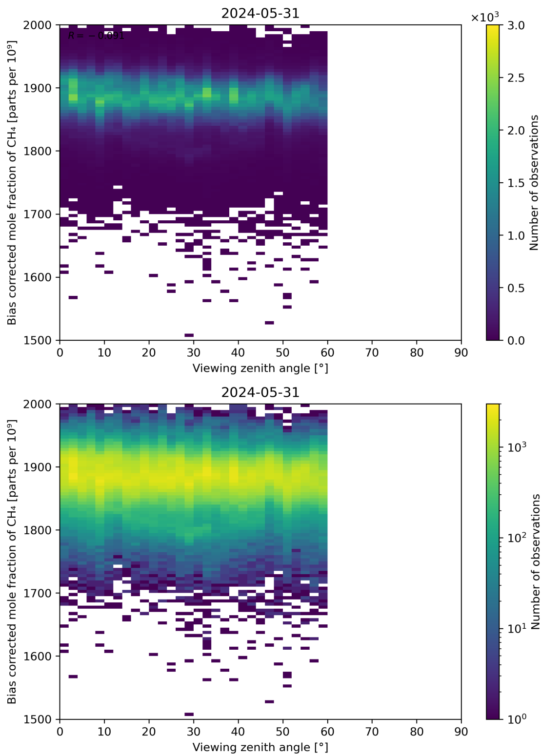
Figure 111: Scatter density plot of “Viewing zenith angle” against “Bias corrected mole fraction of CH 4 ” for 2024-05-30 to 2024-06-01.
