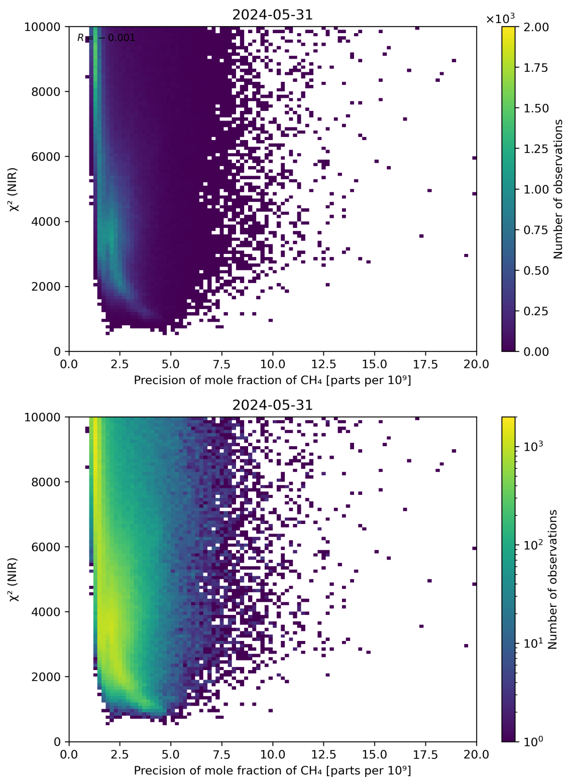
Figure 78: Scatter density plot of “Precision of mole fraction of \text{CH}_4 ” against “ \chi^2 (NIR)” for 2024-05-30 to 2024-06-01.
