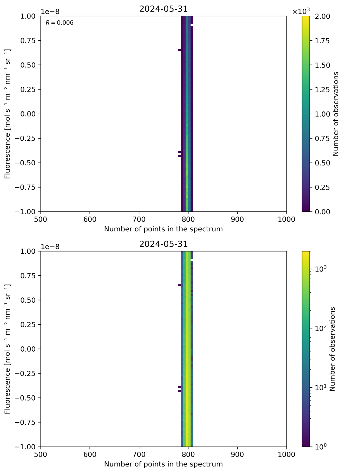
Figure 91: Scatter density plot of “Number of points in the spectrum” against “Fluorescence” for 2024-05-30 to 2024-06-01.
