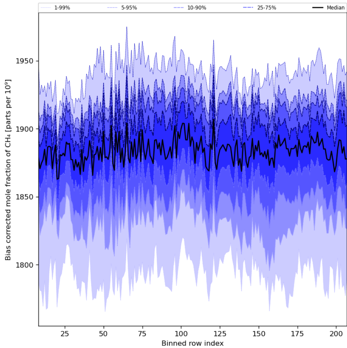
Figure 36: Along track statistics of “Bias corrected mole fraction of CH 4 ” for 2024-05-30 to 2024-06-01
