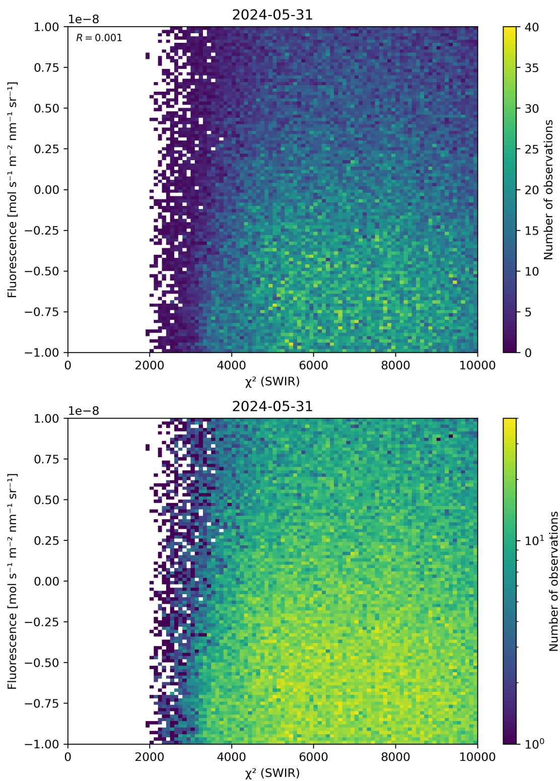
Figure 49: Scatter density plot of “ \chi^2 (SWIR)” against “Fluorescence” for 2024-05-30 to 2024-06-01.
