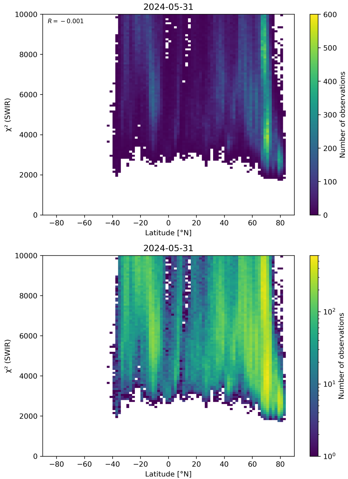
Figure 54: Scatter density plot of “Latitude” against “ \chi^2 (SWIR)” for 2024-05-30 to 2024-06-01.
