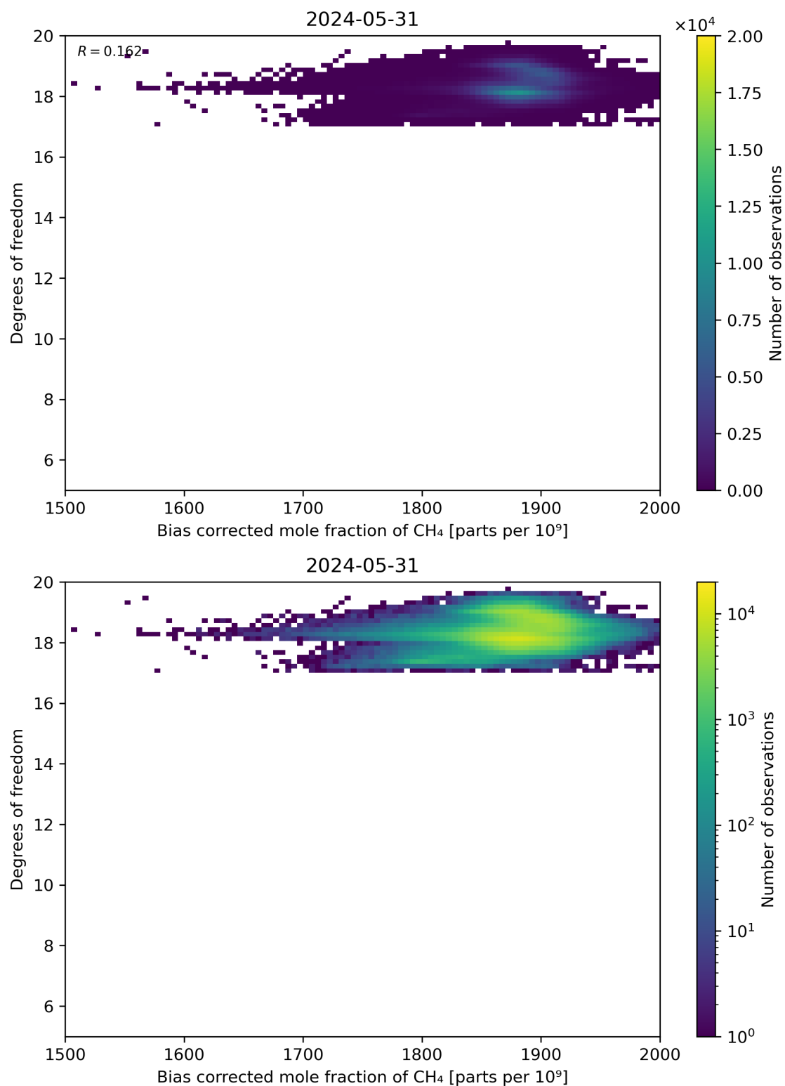
Figure 65: Scatter density plot of “Bias corrected mole fraction of CH 4 ” against “Degrees of freedom” for 2024-05-30 to 2024-06-01.
