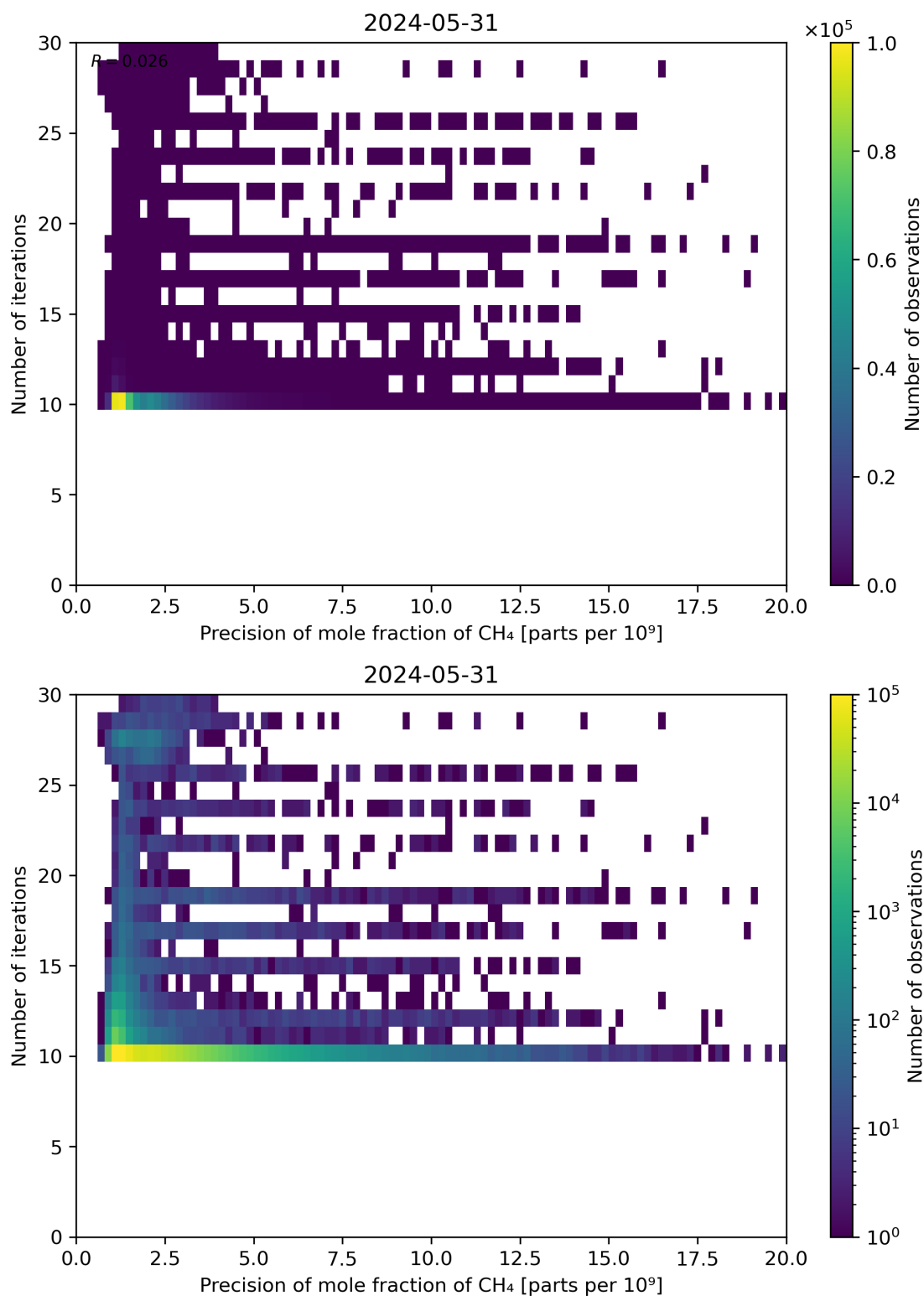
Figure 83: Scatter density plot of “Precision of mole fraction of CH 4 ” against “Number of iterations” for 2024-05-30 to 2024-06-01.
