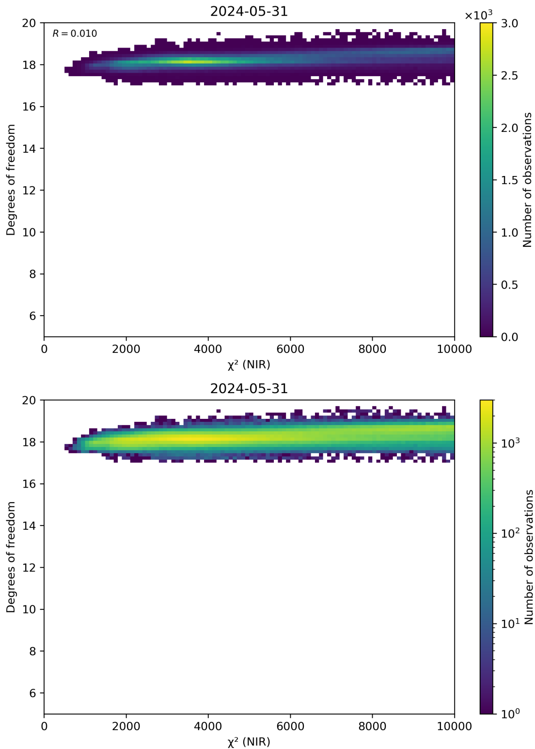
Figure 44: Scatter density plot of “ \chi^2 (NIR)” against “Degrees of freedom” for 2024-05-30 to 2024-06-01.
