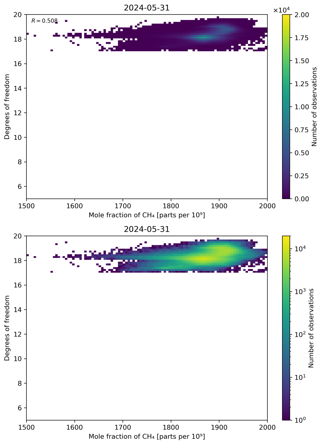
Figure 72: Scatter density plot of “Mole fraction of CH 4 ” against “Degrees of freedom” for 2024-05-30 to 2024-06-01.
