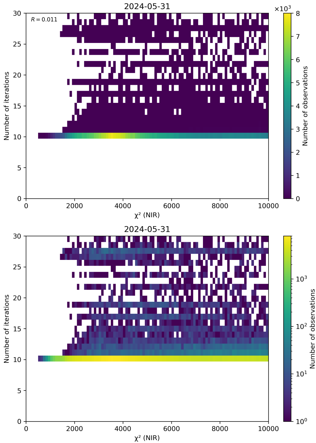
Figure 46: Scatter density plot of “ \chi^2 (NIR)” against “Number of iterations” for 2024-05-30 to 2024-06-01.
