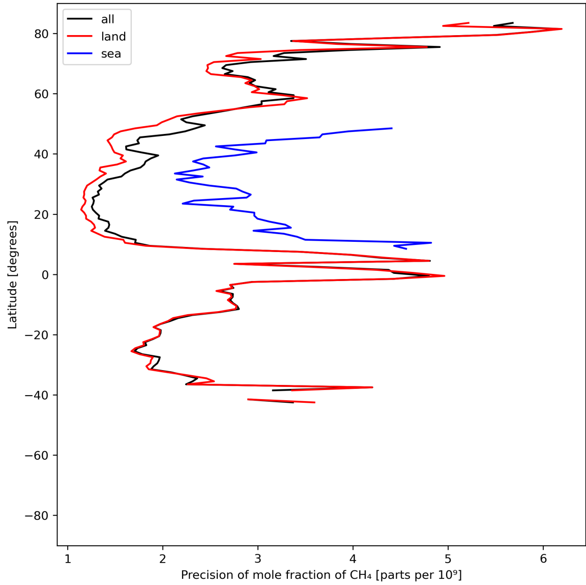
Figure 13: Zonal average of “Precision of mole fraction of CH 4 ” for 2024-05-30 to 2024-06-01.
