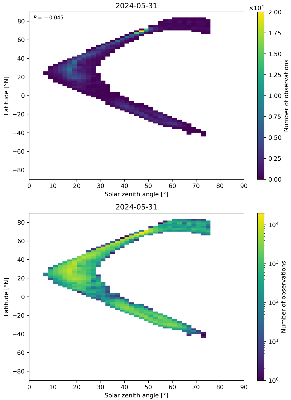
Figure 98: Scatter density plot of “Solar zenith angle” against “Latitude” for 2024-05-30 to 2024-06-01.
