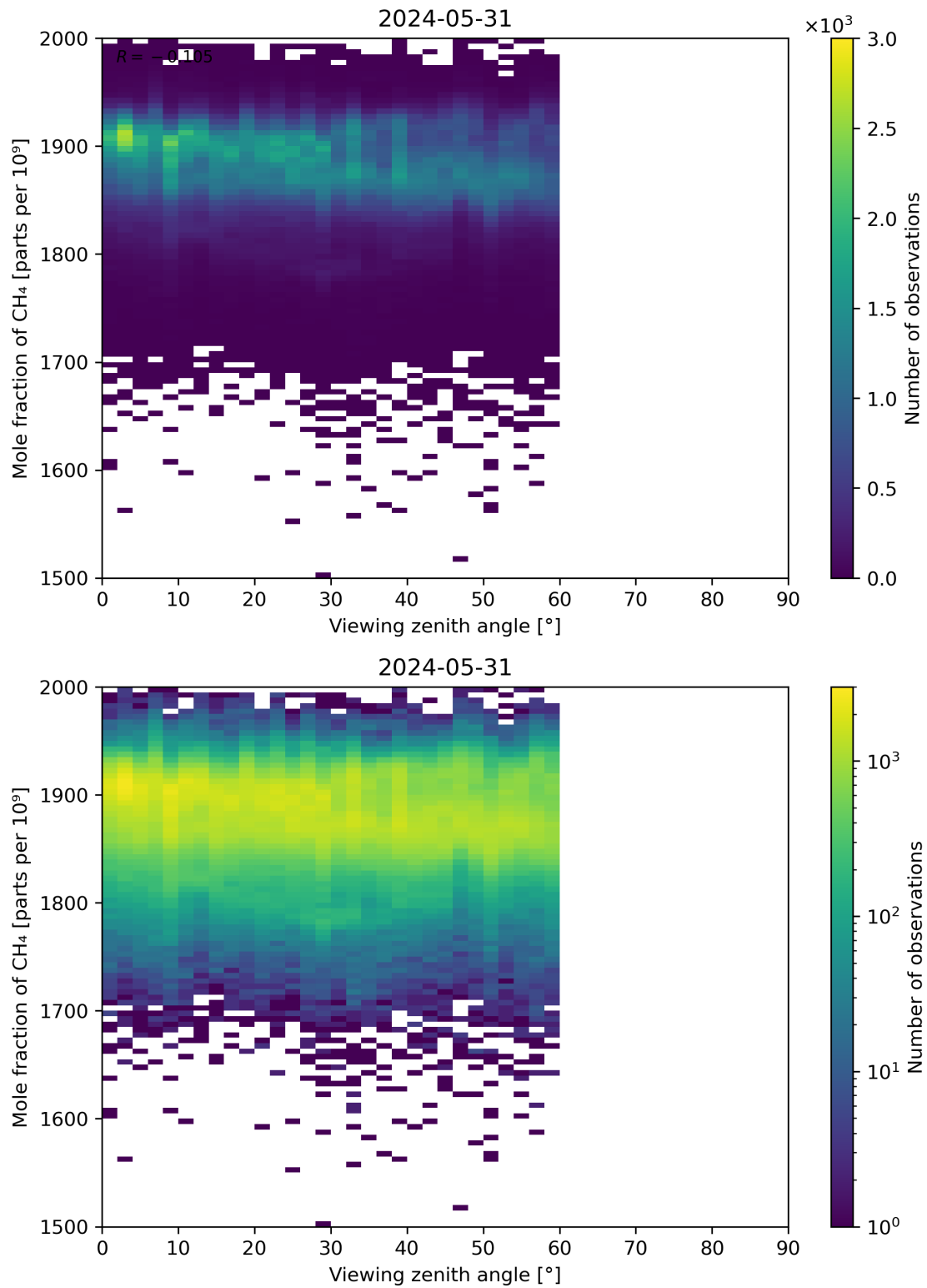
Figure 110: Scatter density plot of “Viewing zenith angle” against “Mole fraction of CH 4 ” for 2024-05-30 to 2024-06-01.
