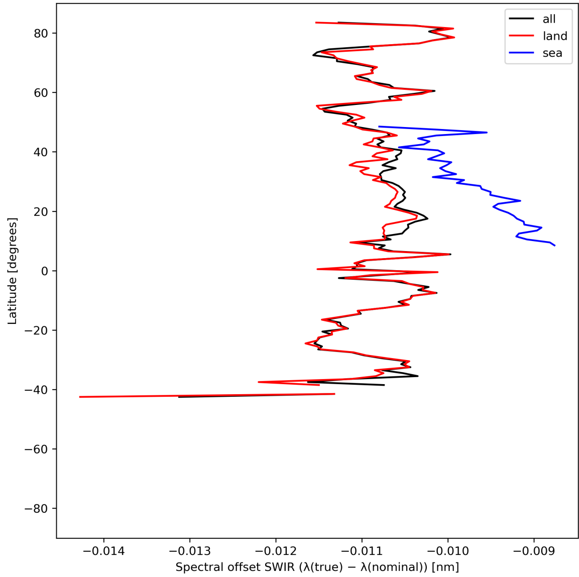
Figure 16: Zonal average of “Spectral offset SWIR ( \lambda(\text{true}) - \lambda(\text{nominal}) )” for 2024-05-30 to 2024-06-01.
