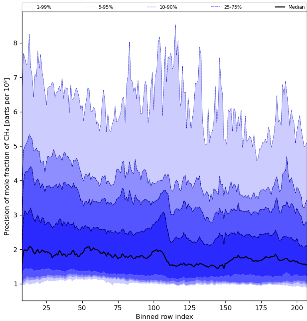
Figure 35: Along track statistics of “Precision of mole fraction of CH 4 ” for 2024-05-30 to 2024-06-01
