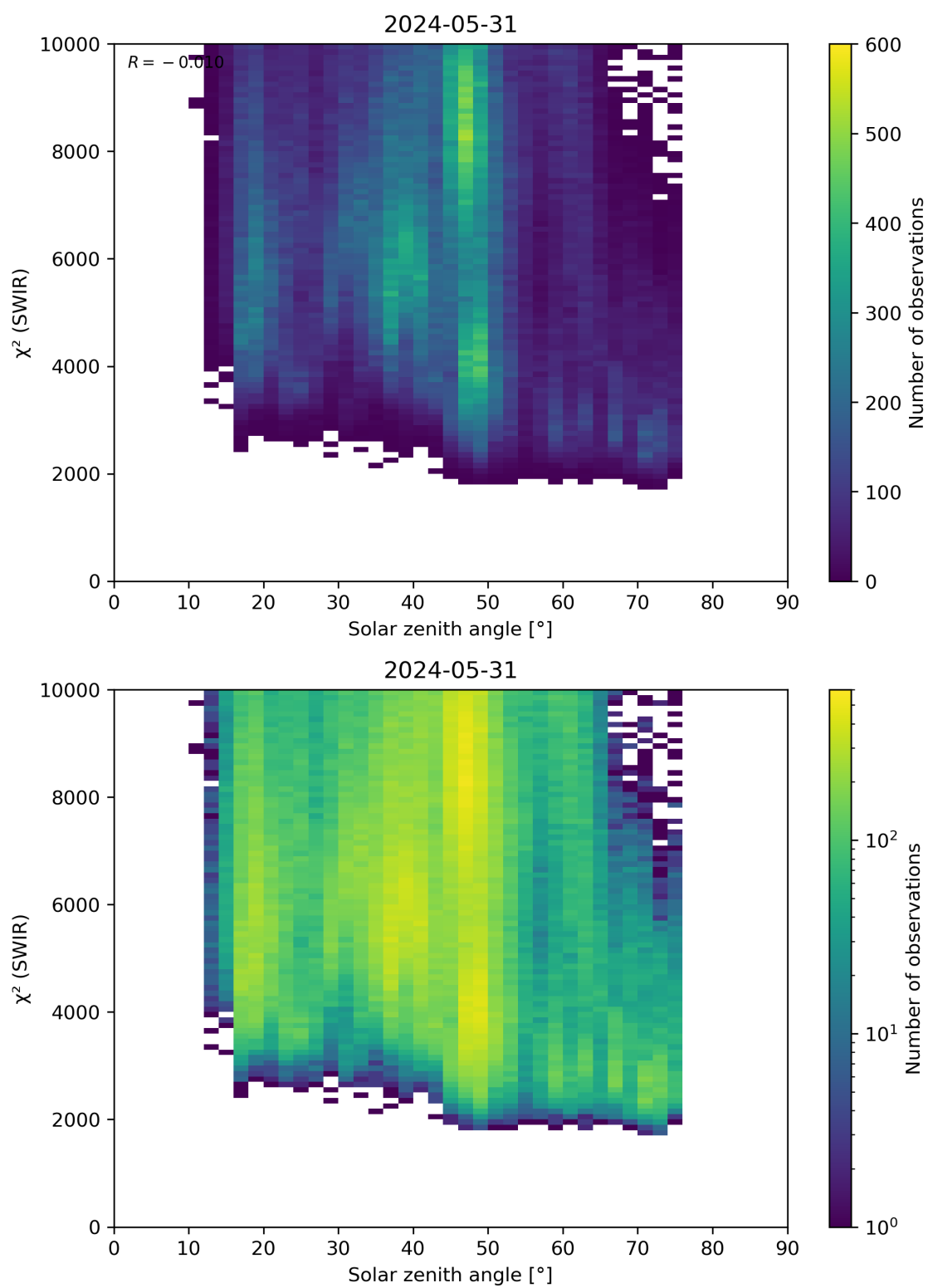
Figure 95: Scatter density plot of “Solar zenith angle” against “ \chi^2 (SWIR)” for 2024-05-30 to 2024-06-01.
