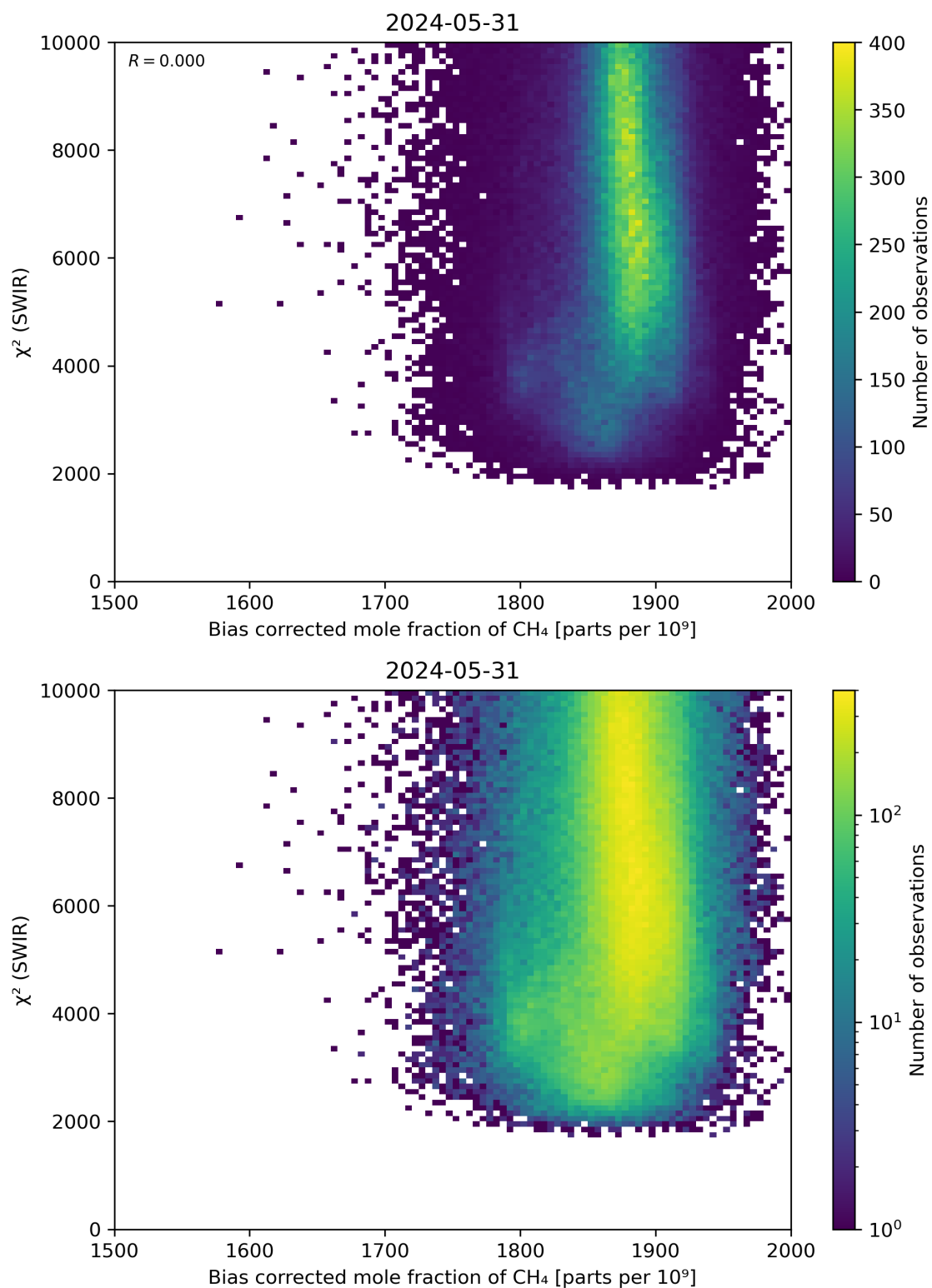
Figure 64: Scatter density plot of “Bias corrected mole fraction of \text{CH}_4 ” against “ \chi^2 (SWIR)” for 2024-05-30 to 2024-06-01.
