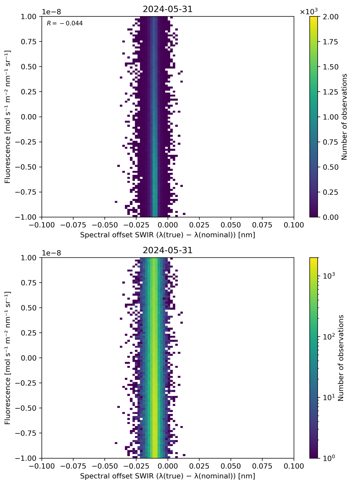
Figure 120: Scatter density plot of “Spectral offset SWIR ( \lambda(\text{true}) - \lambda(\text{nominal}) )” against “Fluorescence” for 2024-05-30 to 2024-06-01.
