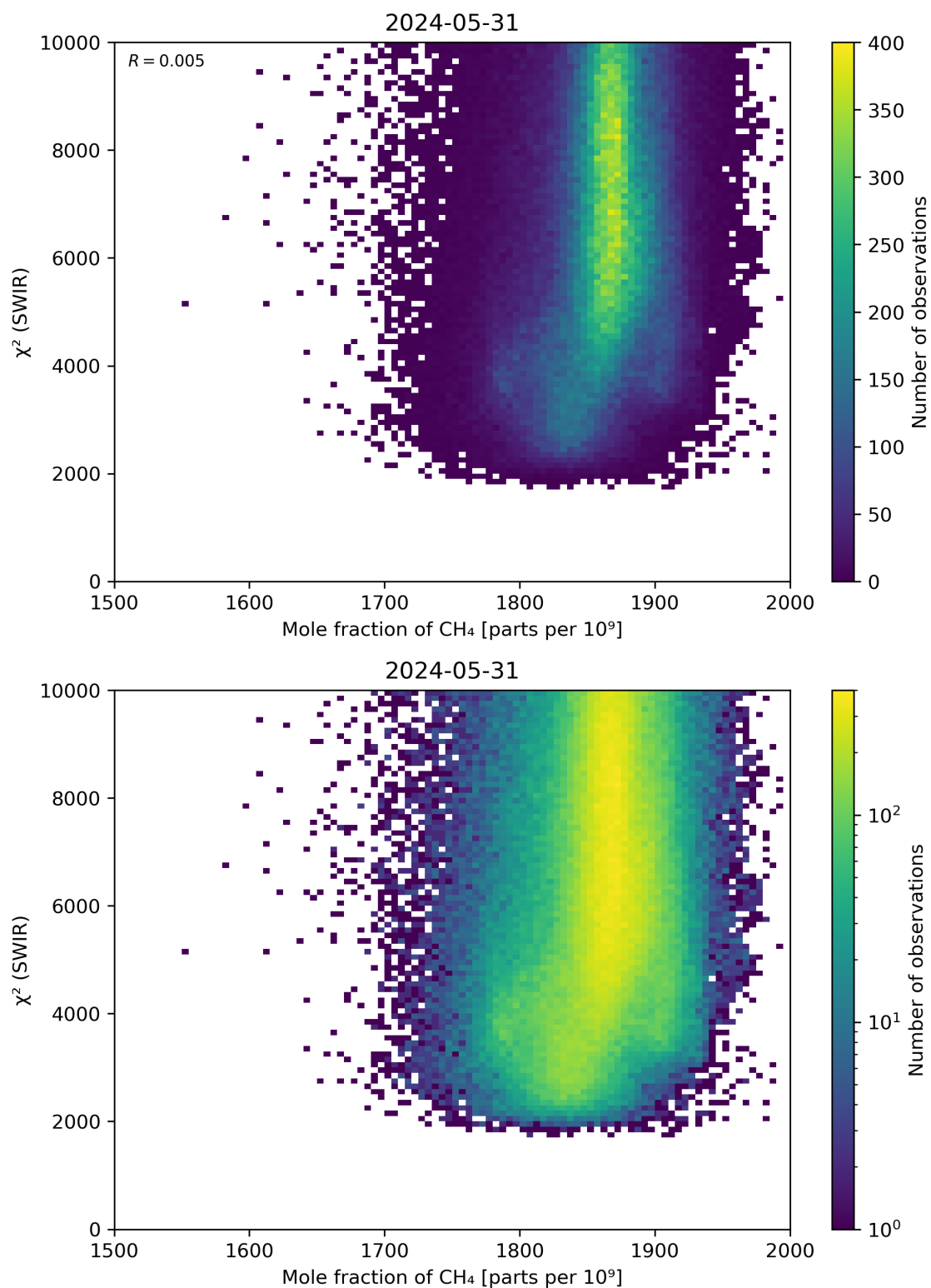
Figure 71: Scatter density plot of “Mole fraction of \text{CH}_4 ” against “ \chi^2 (SWIR)” for 2024-05-30 to 2024-06-01.
