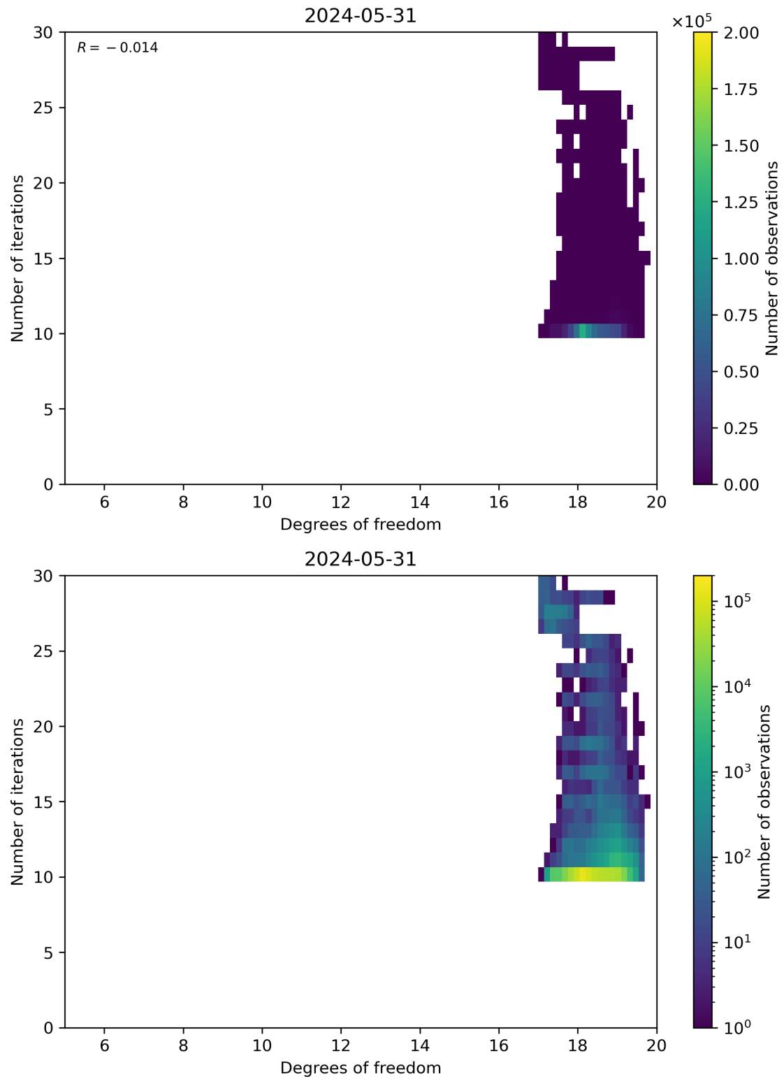
Figure 52: Scatter density plot of “Degrees of freedom” against “Number of iterations” for 2024-05-30 to 2024-06-01.
