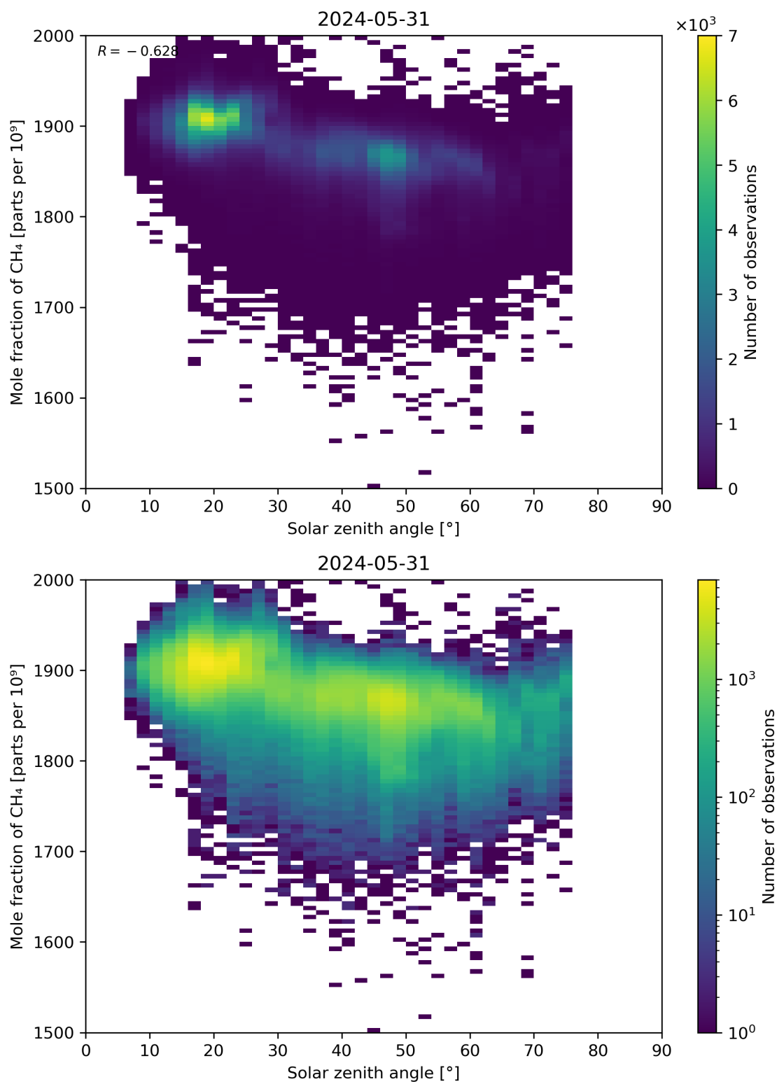
Figure 99: Scatter density plot of “Solar zenith angle” against “Mole fraction of CH 4 ” for 2024-05-30 to 2024-06-01.
