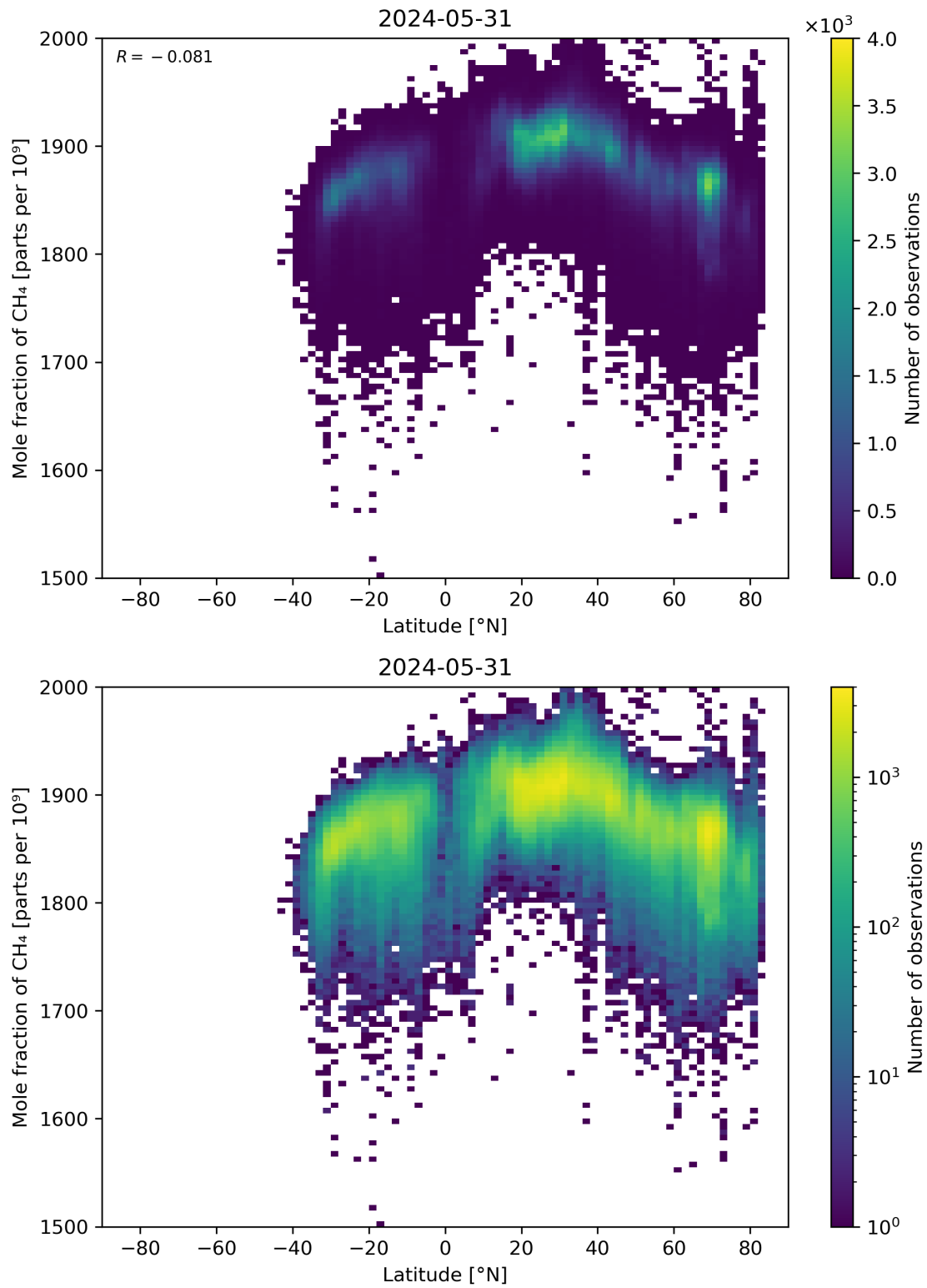
Figure 57: Scatter density plot of “Latitude” against “Mole fraction of \text{CH}_4 ” for 2024-05-30 to 2024-06-01.
