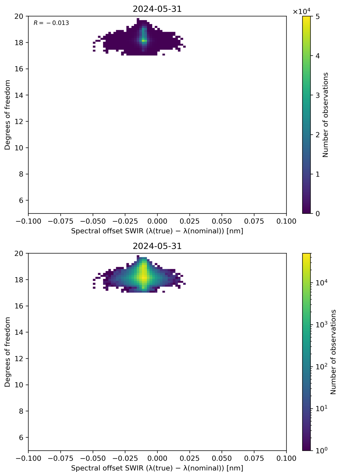
Figure 119: Scatter density plot of “Spectral offset SWIR ( \lambda(\text{true}) - \lambda(\text{nominal}) )” against “Degrees of freedom” for 2024-05-30 to 2024-06-01.
