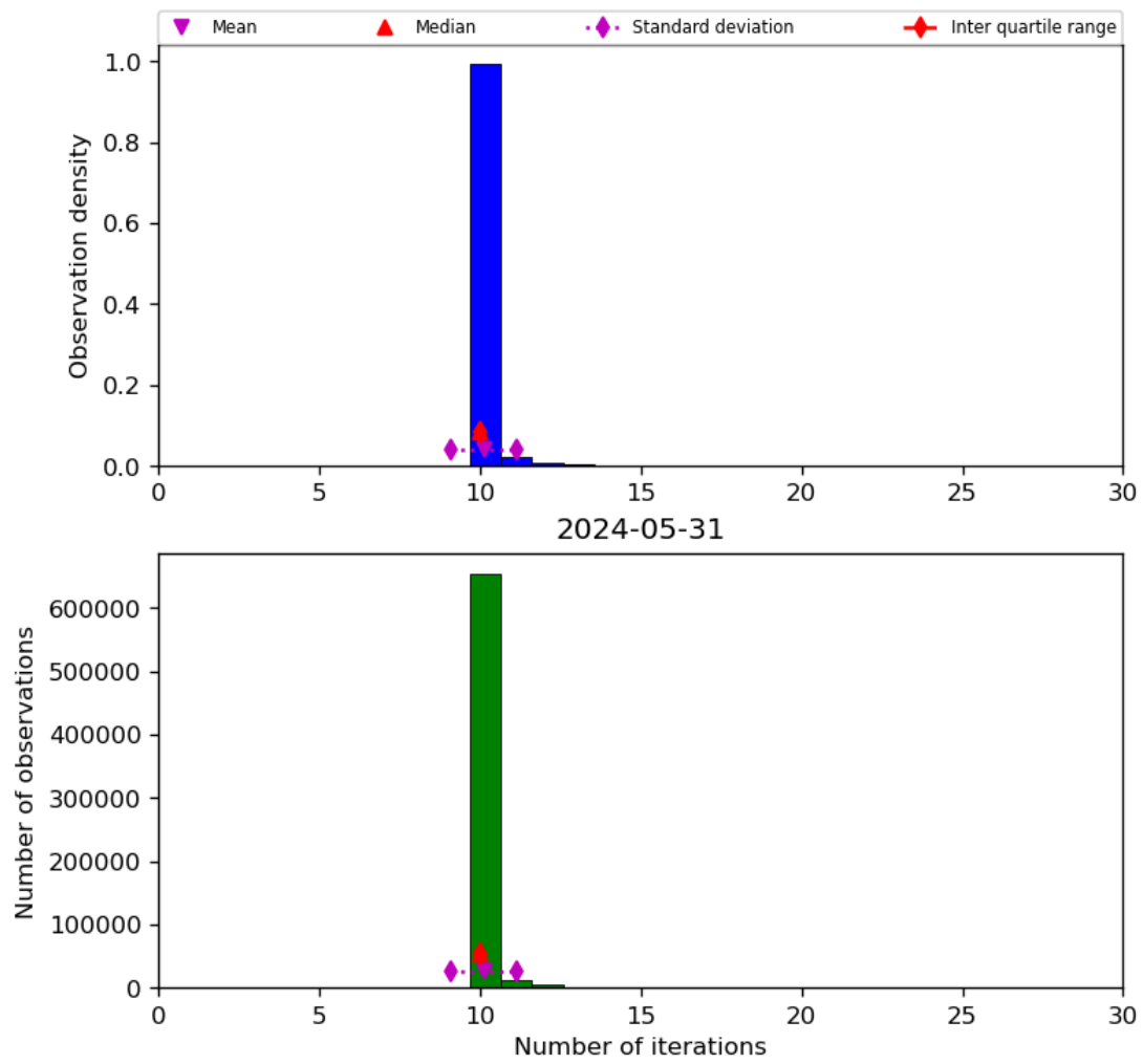
Figure 31: Histogram of "Number of iterations" for 2024-05-30 to 2024-06-01
