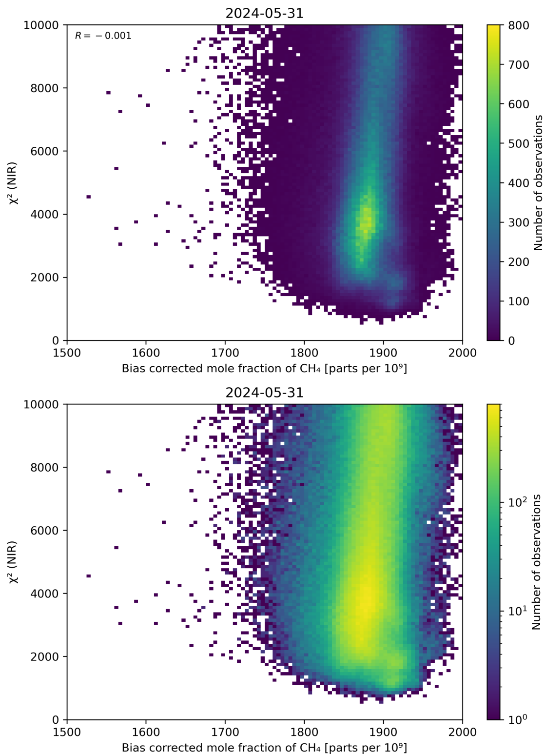
Figure 63: Scatter density plot of “Bias corrected mole fraction of CH 4 ” against “ \chi^2 (NIR)” for 2024-05-30 to 2024-06-01.
