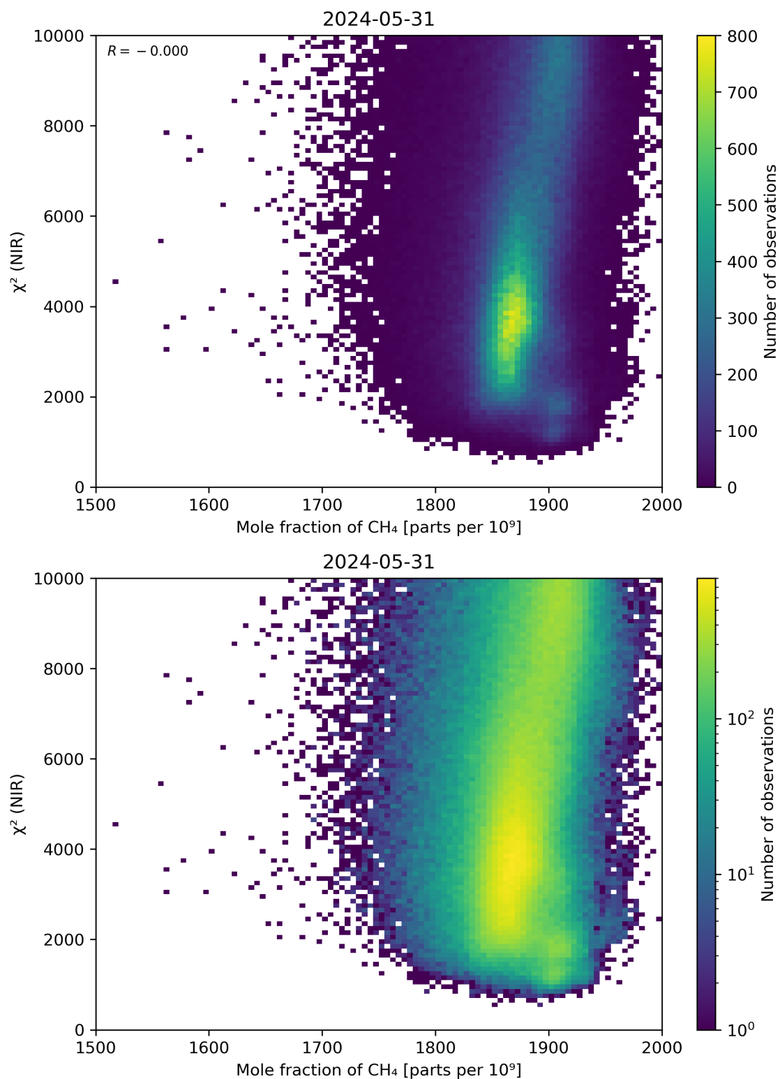
Figure 70: Scatter density plot of “Mole fraction of \text{CH}_4 ” against “ \chi^2 (NIR)” for 2024-05-30 to 2024-06-01.
