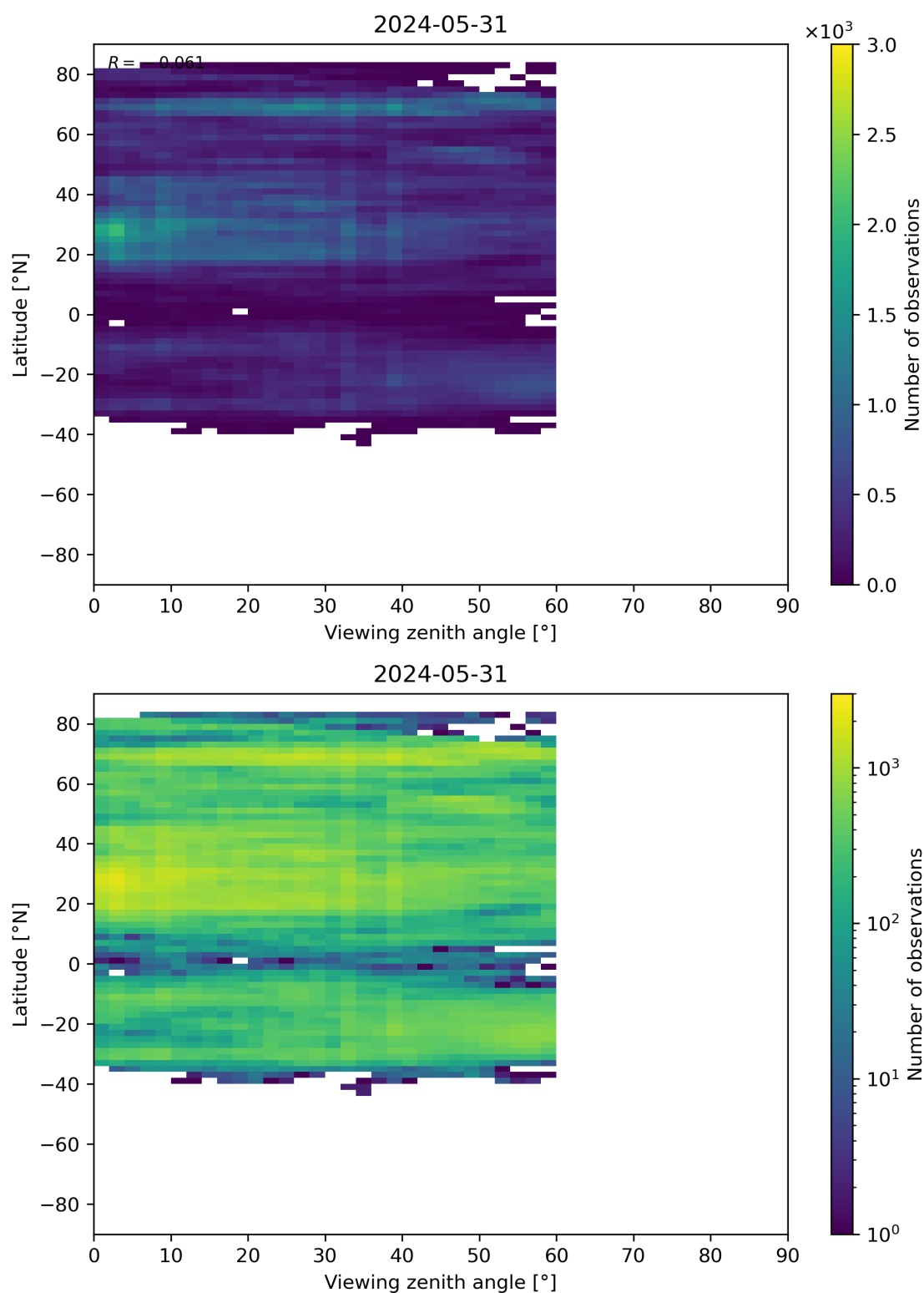
Figure 109: Scatter density plot of “Viewing zenith angle” against “Latitude” for 2024-05-30 to 2024-06-01.
