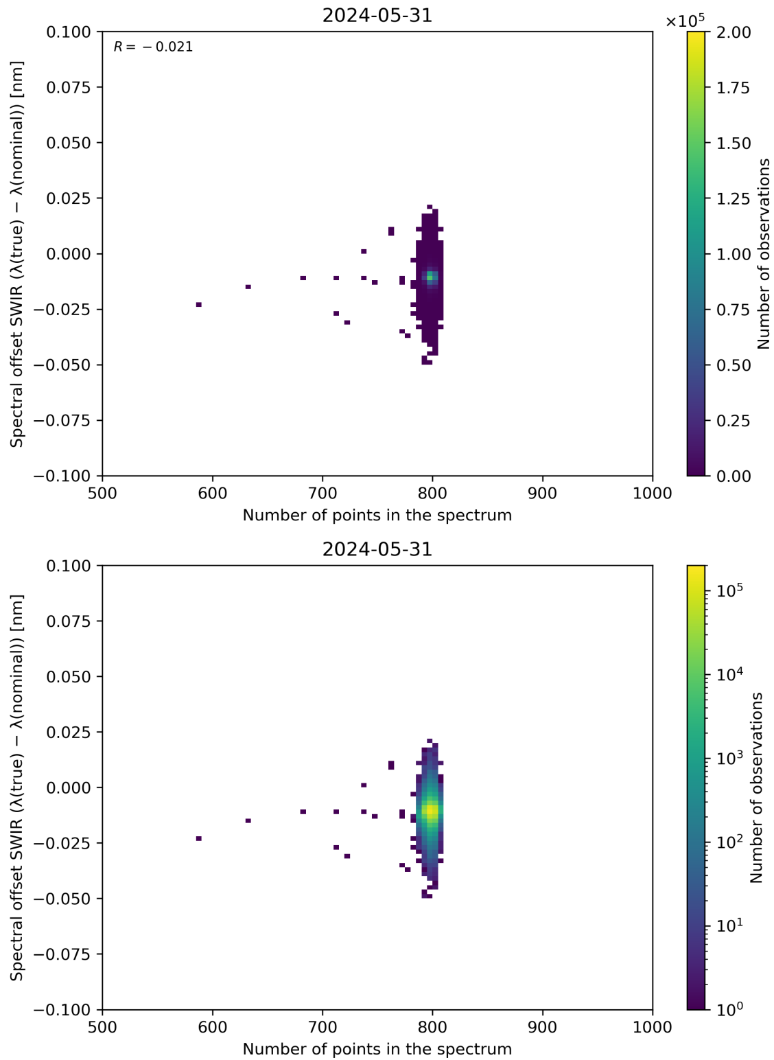
Figure 93: Scatter density plot of “Number of points in the spectrum” against “Spectral offset SWIR ( \lambda(\text{true}) - \lambda(\text{nominal}) )” for 2024-05-30 to 2024-06-01.
