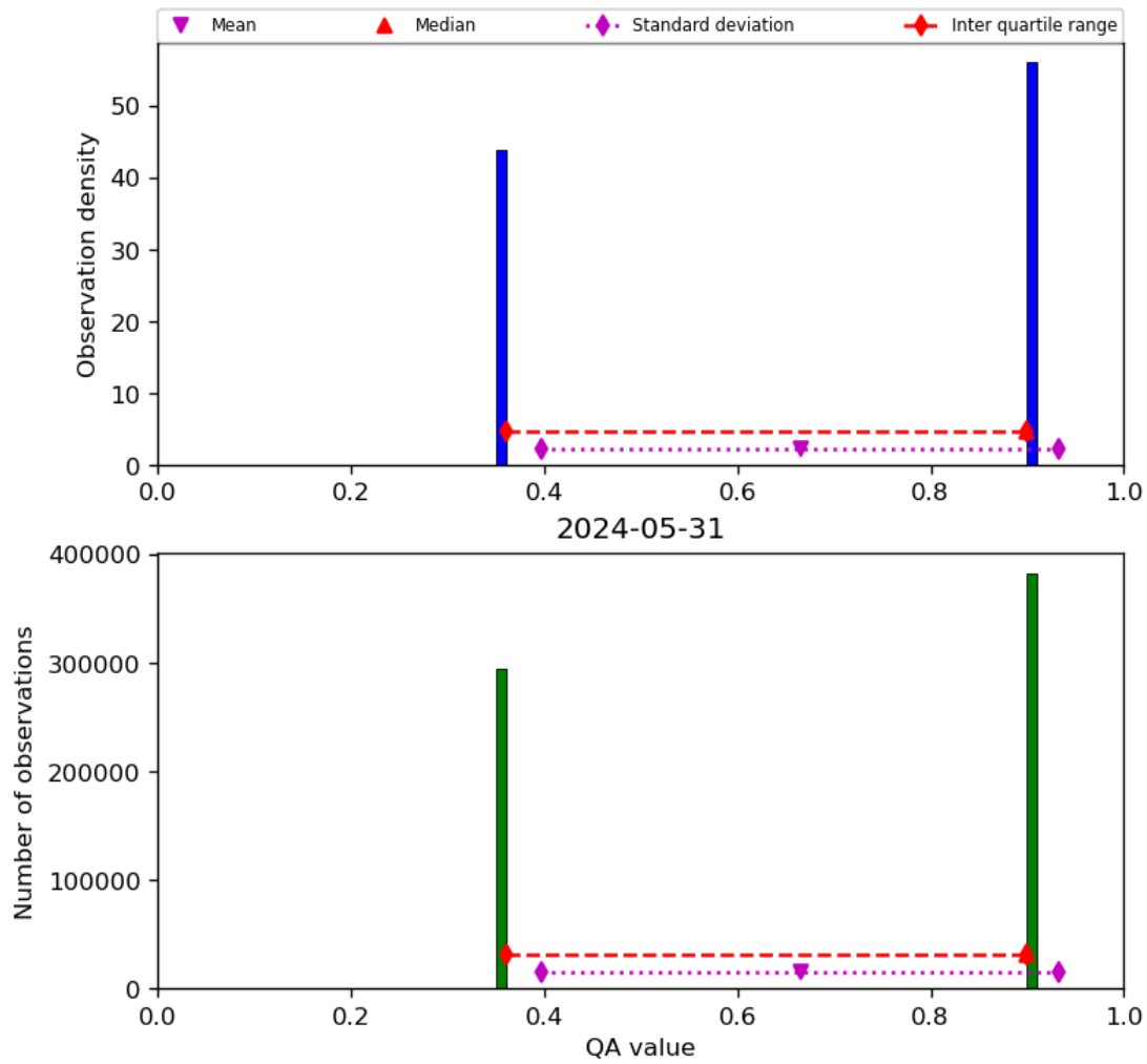
Figure 22: Histogram of "QA value" for 2024-05-30 to 2024-06-01
