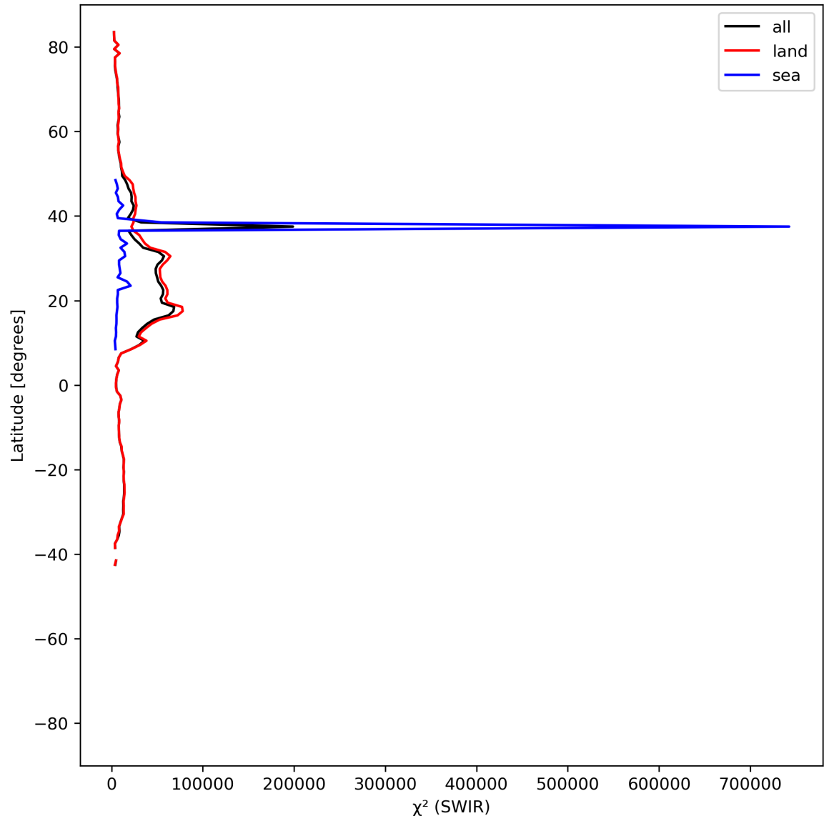
Figure 17: Zonal average of “ \chi^2 (SWIR)” for 2024-05-30 to 2024-06-01.
