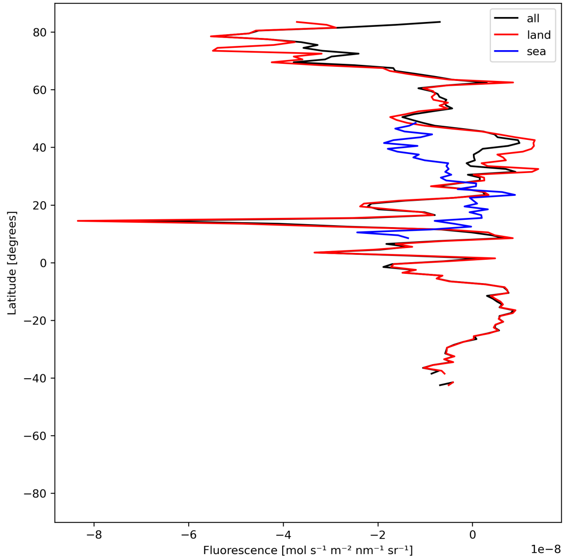
Figure 21: Zonal average of “Fluorescence” for 2024-05-30 to 2024-06-01.
