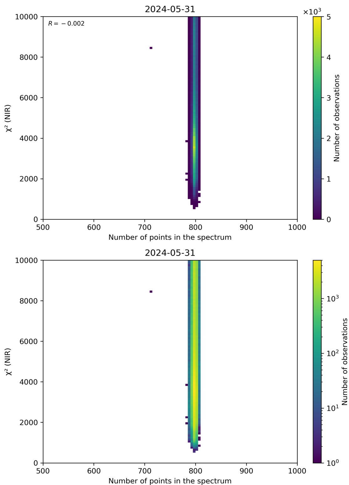
Figure 88: Scatter density plot of “Number of points in the spectrum” against “ \chi^2 (NIR)” for 2024-05-30 to 2024-06-01.
