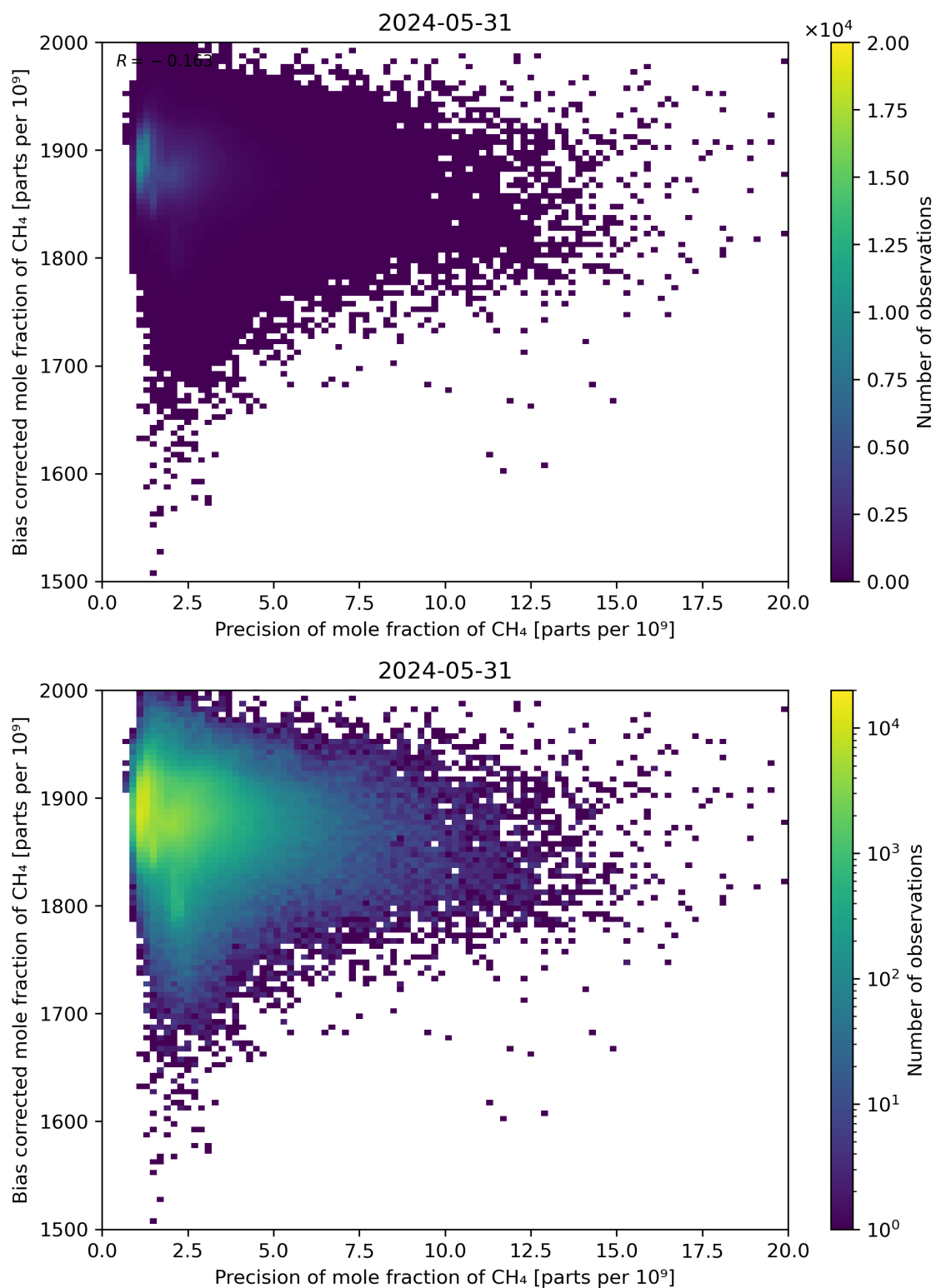
Figure 82: Scatter density plot of “Precision of mole fraction of \text{CH}_4 ” against “Bias corrected mole fraction of \text{CH}_4 ” for 2024-05-30 to 2024-06-01.
