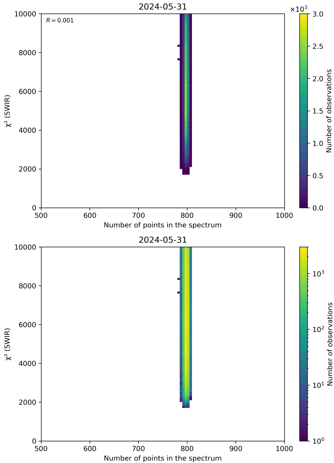
Figure 89: Scatter density plot of “Number of points in the spectrum” against “ \chi^2 (SWIR)” for 2024-05-30 to 2024-06-01.
