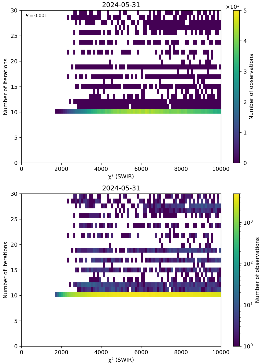
Figure 50: Scatter density plot of “ \chi^2 (SWIR)” against “Number of iterations” for 2024-05-30 to 2024-06-01.
