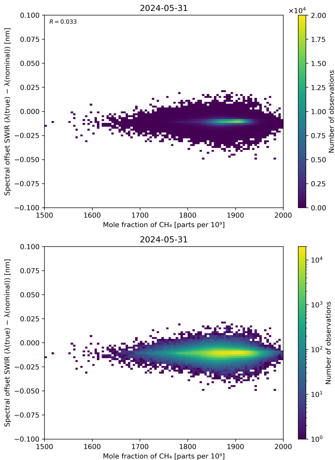
Figure 86: Scatter density plot of “Mole fraction of CH 4 ” against “Spectral offset SWIR ( \lambda(\text{true}) - \lambda(\text{nominal}) )” for 2024-05-30 to 2024-06-01.
