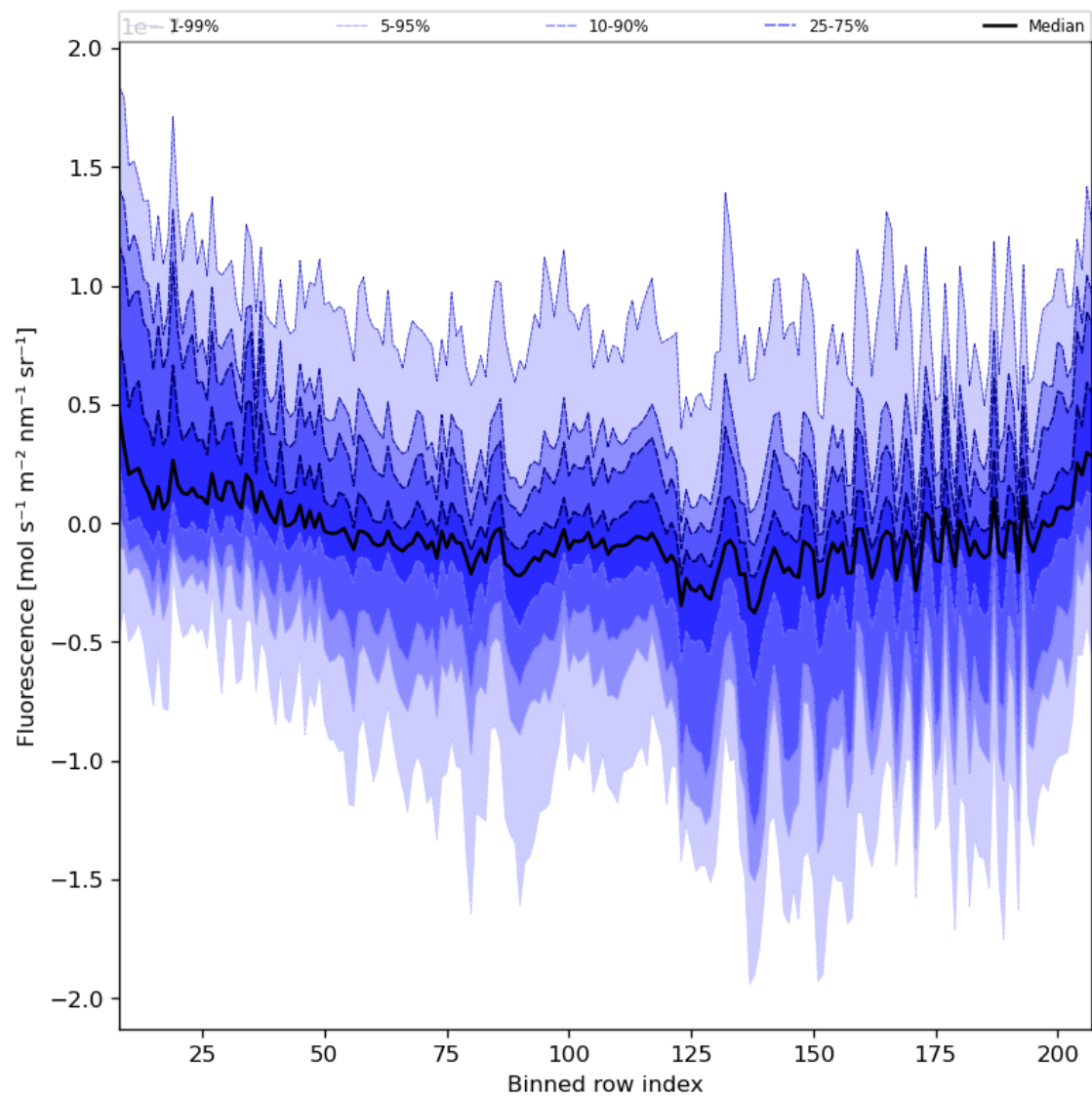
Figure 43: Along track statistics of “Fluorescence” for 2024-05-30 to 2024-06-01
