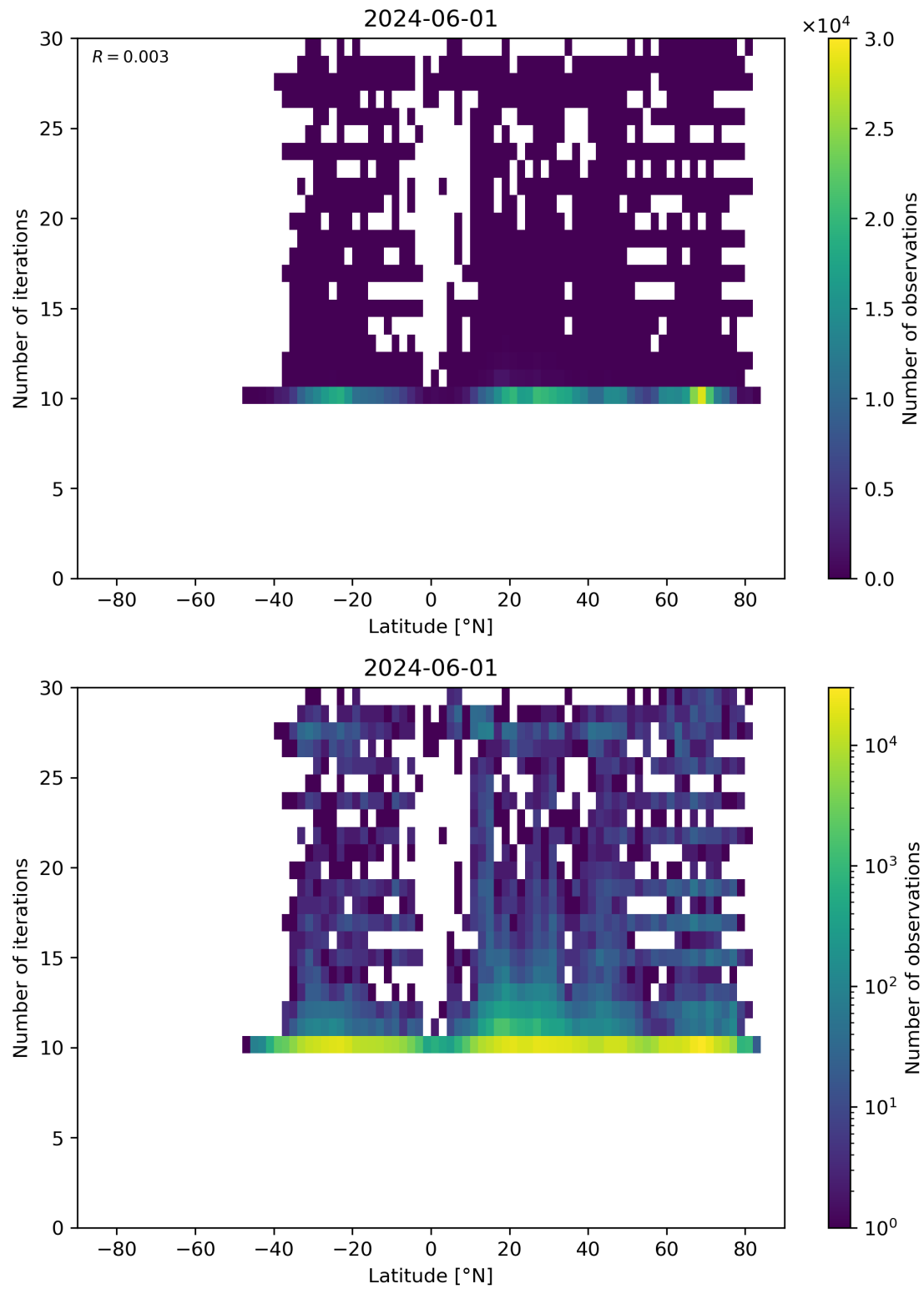
Figure 60: Scatter density plot of “Latitude” against “Number of iterations” for 2024-05-31 to 2024-06-02.
