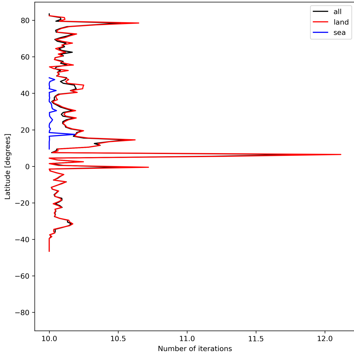
Figure 20: Zonal average of “Number of iterations” for 2024-05-31 to 2024-06-02.
