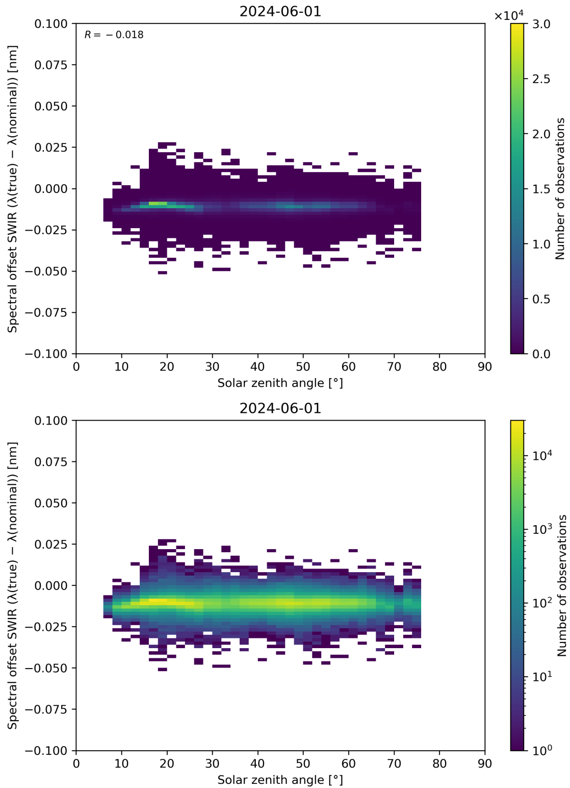
Figure 104: Scatter density plot of “Solar zenith angle” against “Spectral offset SWIR ( \lambda(\text{true}) - \lambda(\text{nominal}) )” for 2024-05-31 to 2024-06-02.
