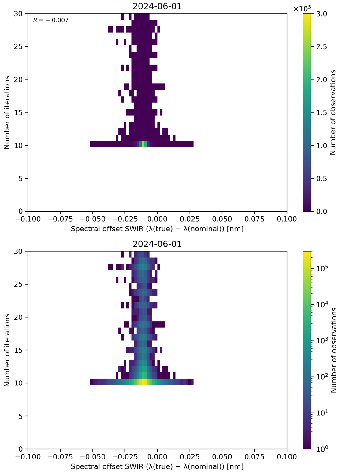
Figure 121: Scatter density plot of “Spectral offset SWIR ( \lambda(\text{true}) - \lambda(\text{nominal}) )” against “Number of iterations” for 2024-05-31 to 2024-06-02.
