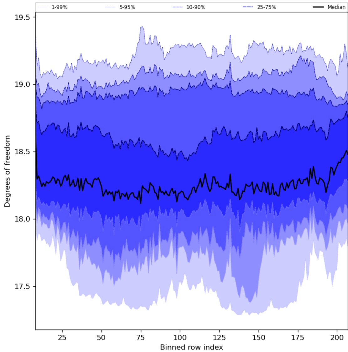
Figure 41: Along track statistics of “Degrees of freedom” for 2024-05-31 to 2024-06-02
