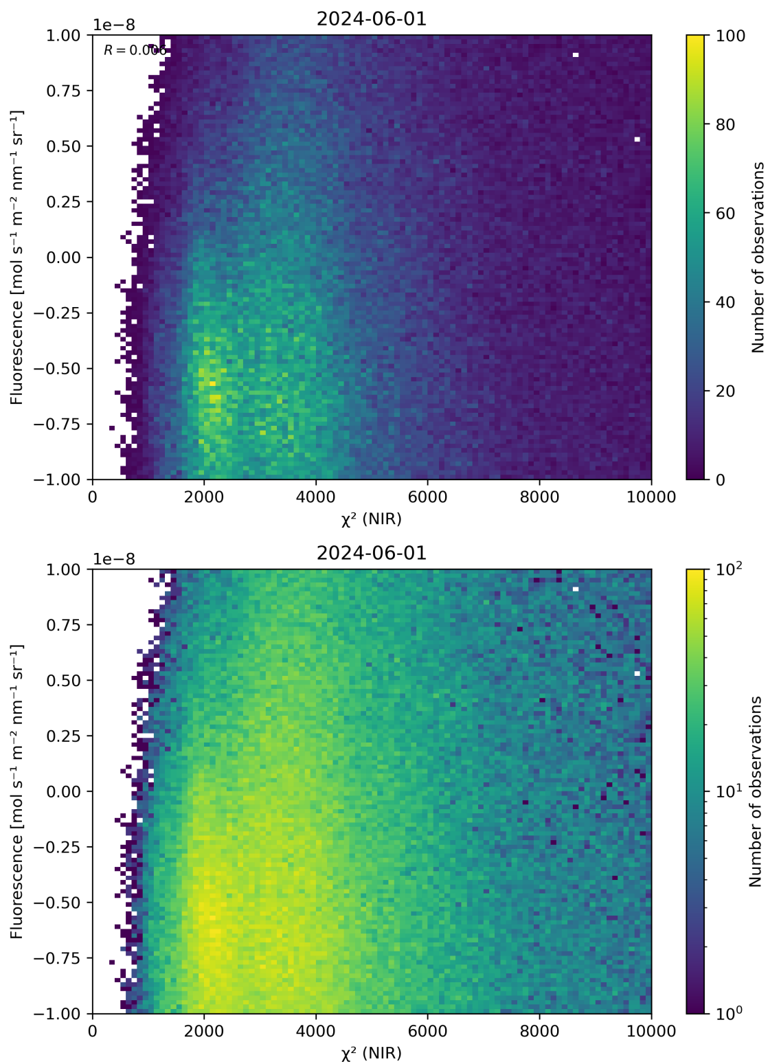
Figure 45: Scatter density plot of “ \chi^2 (NIR)” against “Fluorescence” for 2024-05-31 to 2024-06-02.
