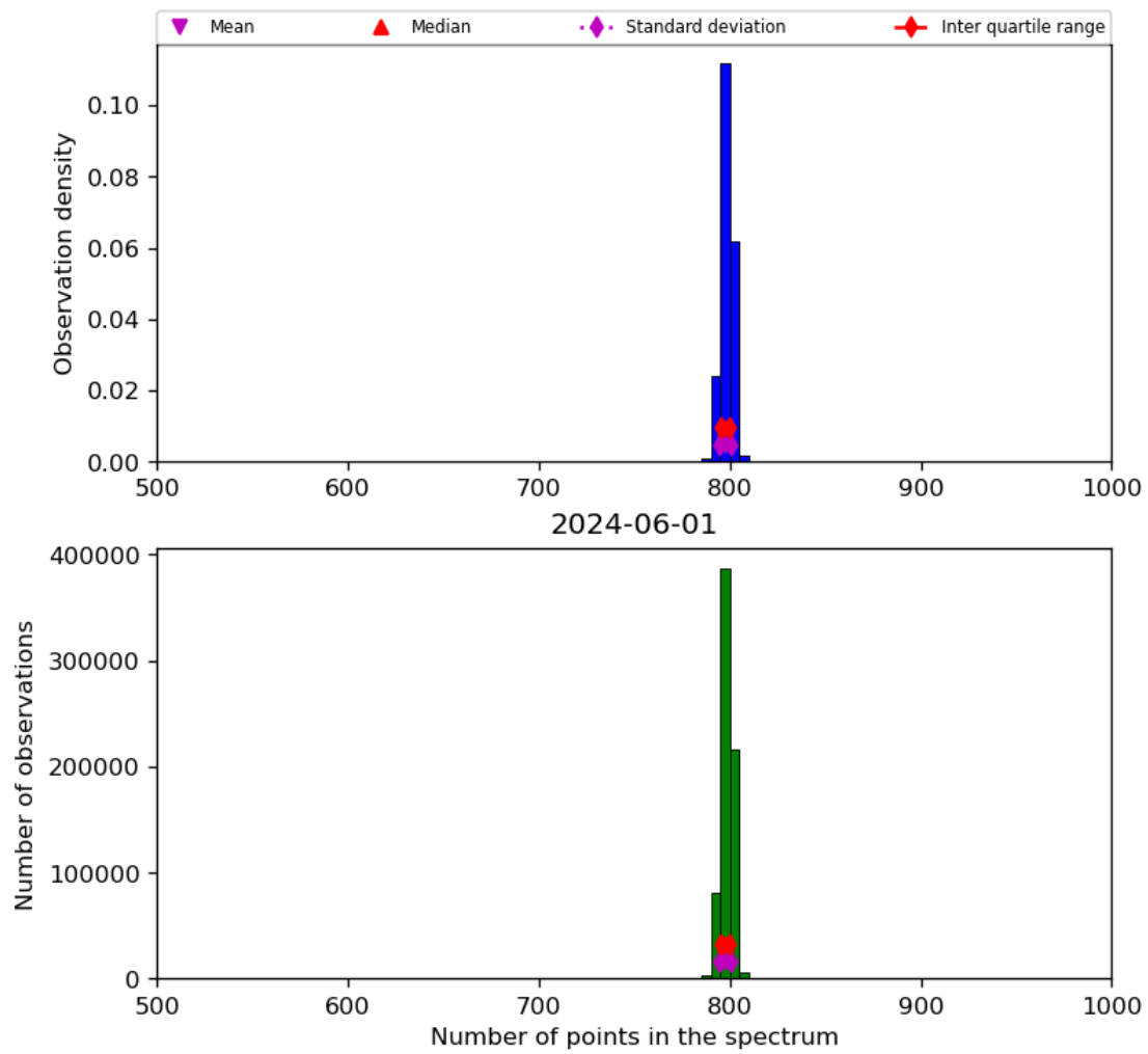
Figure 26: Histogram of “Number of points in the spectrum” for 2024-05-31 to 2024-06-02
