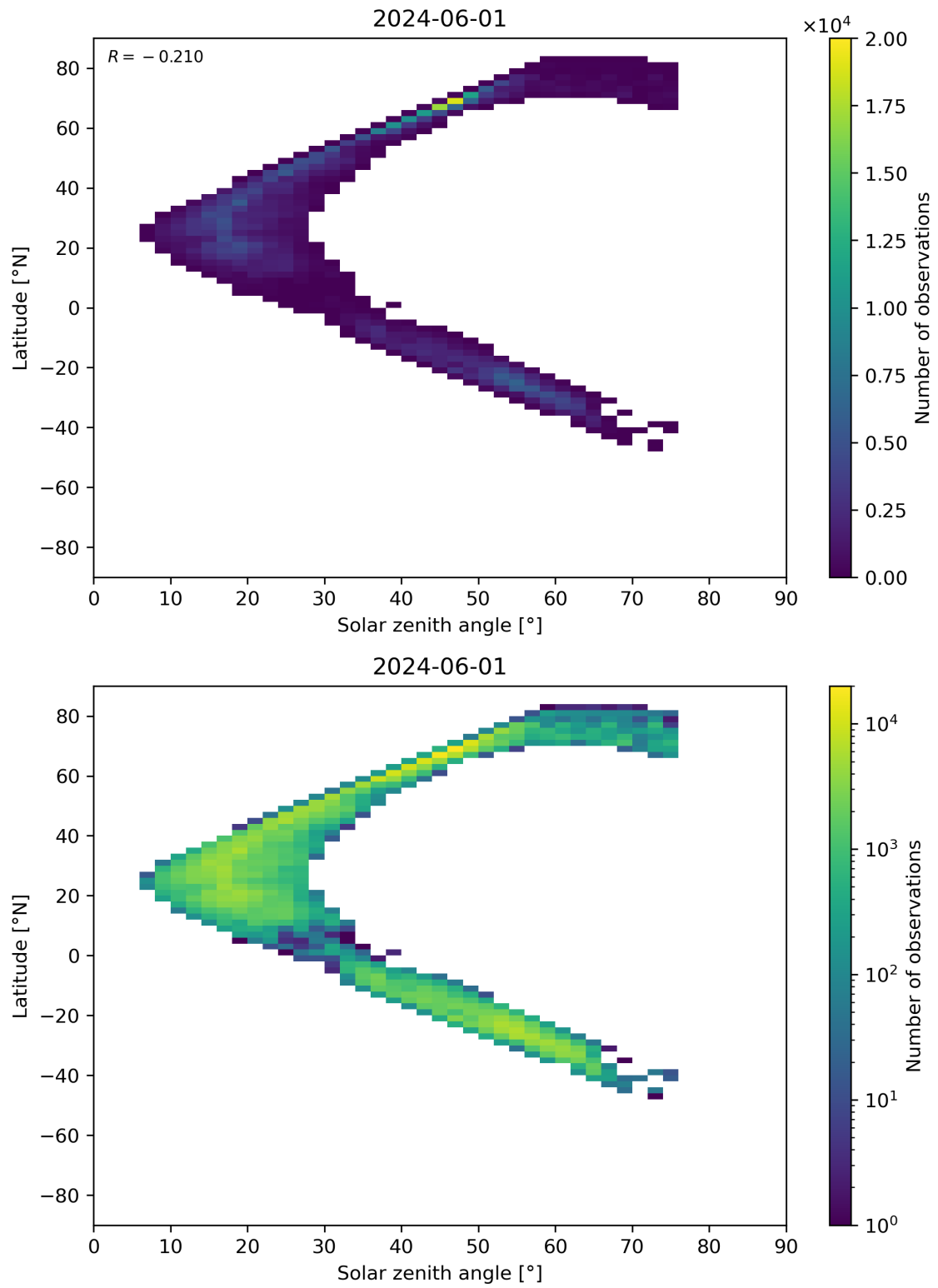
Figure 98: Scatter density plot of “Solar zenith angle” against “Latitude” for 2024-05-31 to 2024-06-02.
