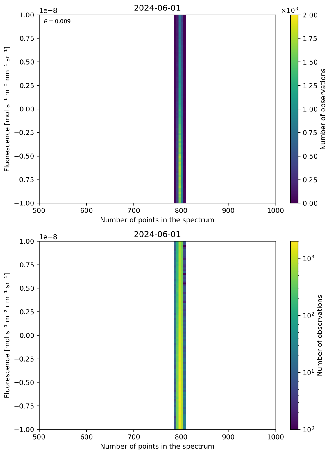
Figure 91: Scatter density plot of “Number of points in the spectrum” against “Fluorescence” for 2024-05-31 to 2024-06-02.
