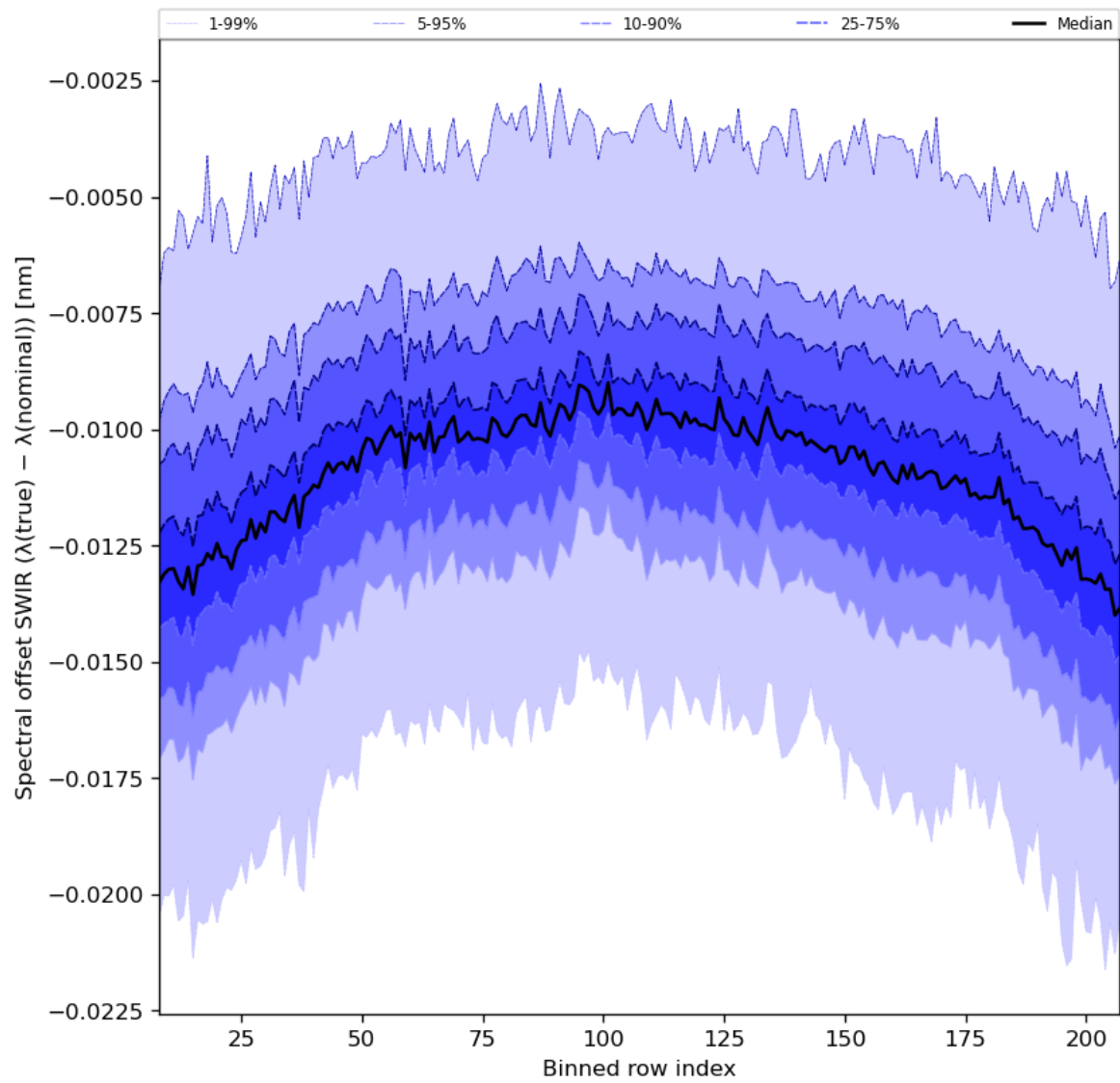
Figure 38: Along track statistics of “Spectral offset SWIR ( \lambda(\text{true}) - \lambda(\text{nominal}) )” for 2024-05-31 to 2024-06-02
