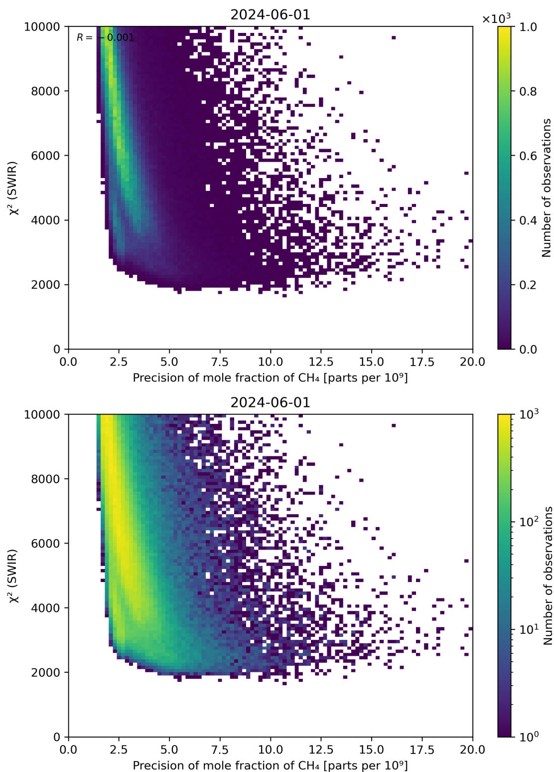
Figure 79: Scatter density plot of “Precision of mole fraction of \text{CH}_4 ” against “ \chi^2 (SWIR)” for 2024-05-31 to 2024-06-02.
