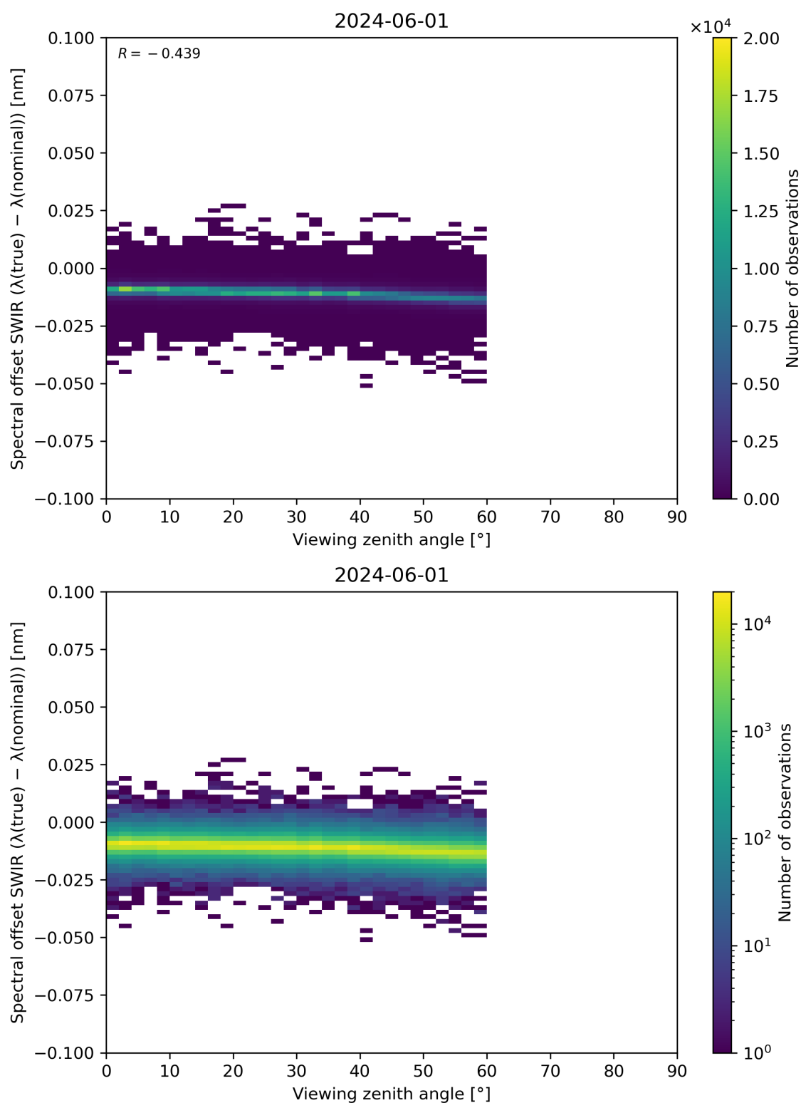
Figure 116: Scatter density plot of “Viewing zenith angle” against “Spectral offset SWIR ( \lambda(\text{true}) - \lambda(\text{nominal}) )” for 2024-05-31 to 2024-06-02.
