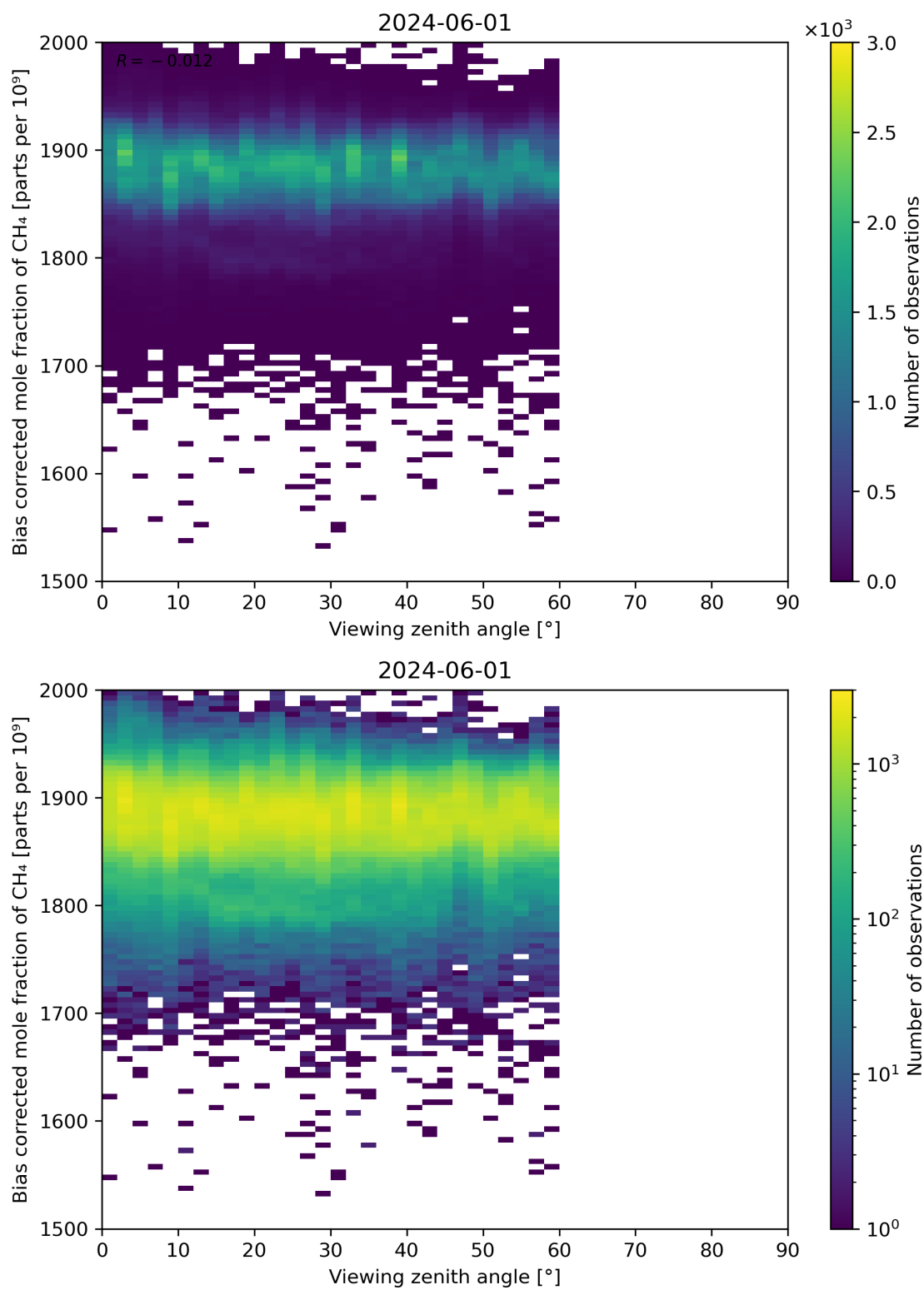
Figure 111: Scatter density plot of “Viewing zenith angle” against “Bias corrected mole fraction of CH 4 ” for 2024-05-31 to 2024-06-02.
