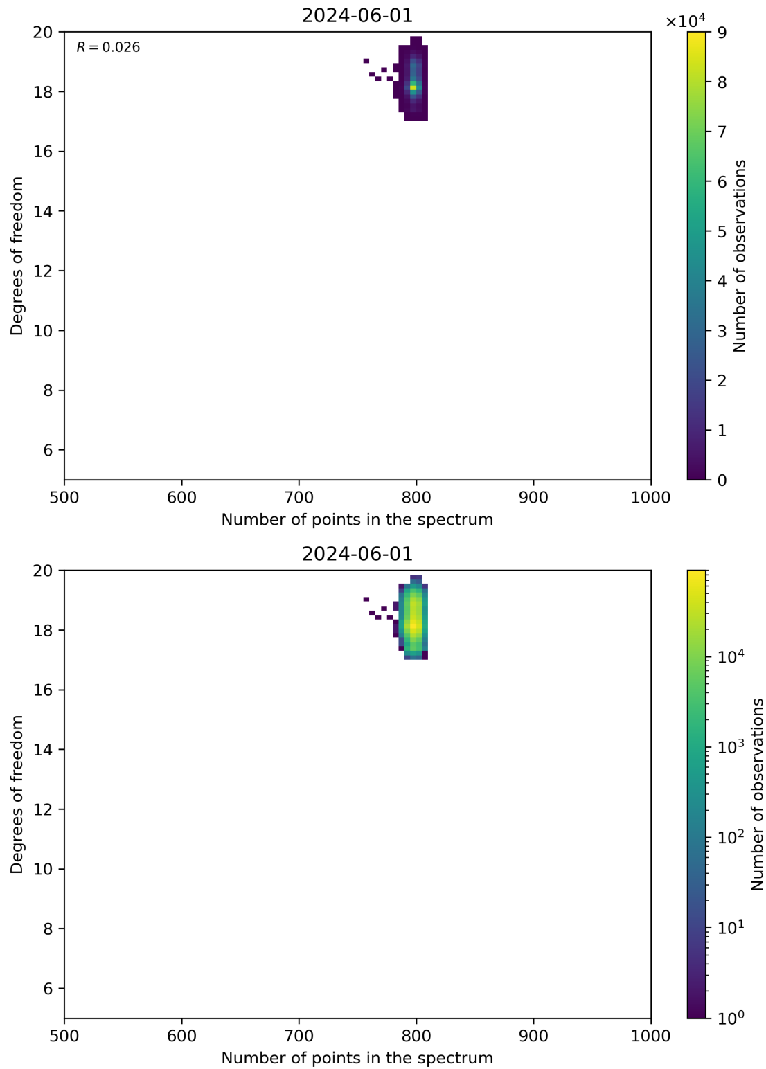
Figure 90: Scatter density plot of “Number of points in the spectrum” against “Degrees of freedom” for 2024-05-31 to 2024-06-02.
