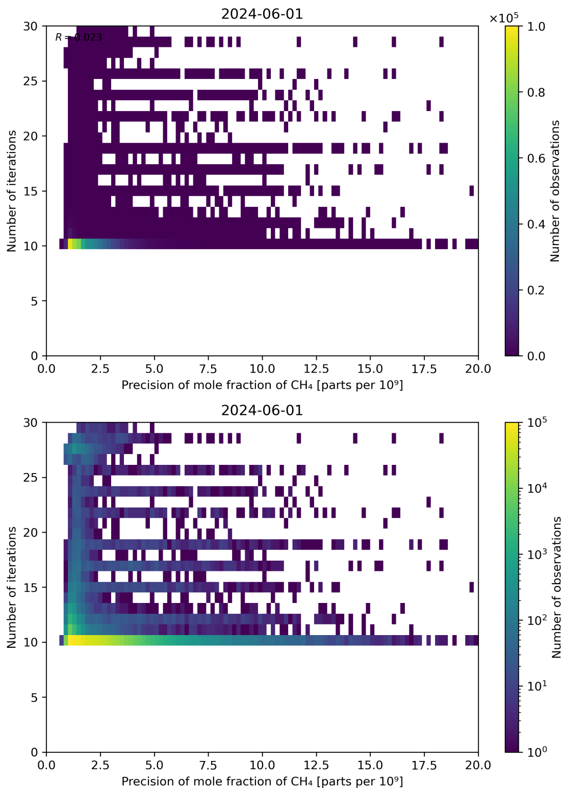
Figure 83: Scatter density plot of “Precision of mole fraction of CH 4 ” against “Number of iterations” for 2024-05-31 to 2024-06-02.
