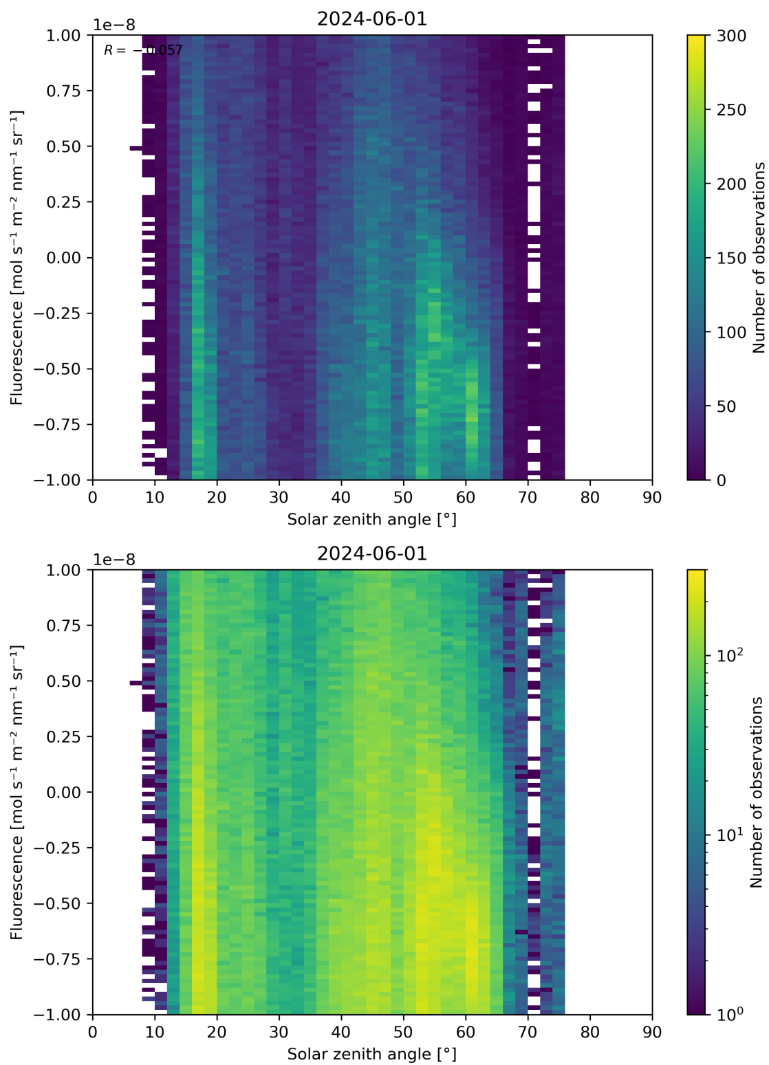
Figure 97: Scatter density plot of “Solar zenith angle” against “Fluorescence” for 2024-05-31 to 2024-06-02.
