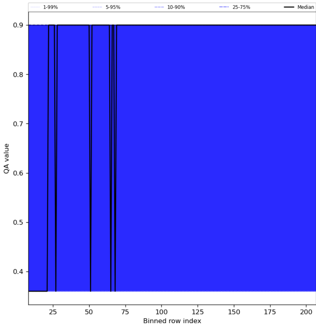
Figure 33: Along track statistics of "QA value" for 2024-05-31 to 2024-06-02
