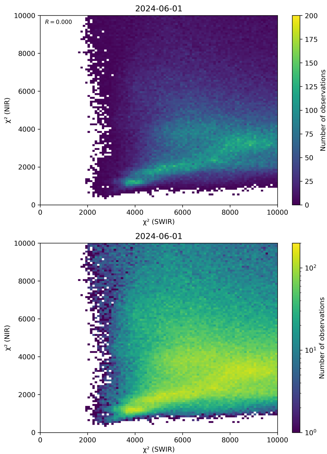
Figure 47: Scatter density plot of “ \chi^2 (SWIR)” against “ \chi^2 (NIR)” for 2024-05-31 to 2024-06-02.
