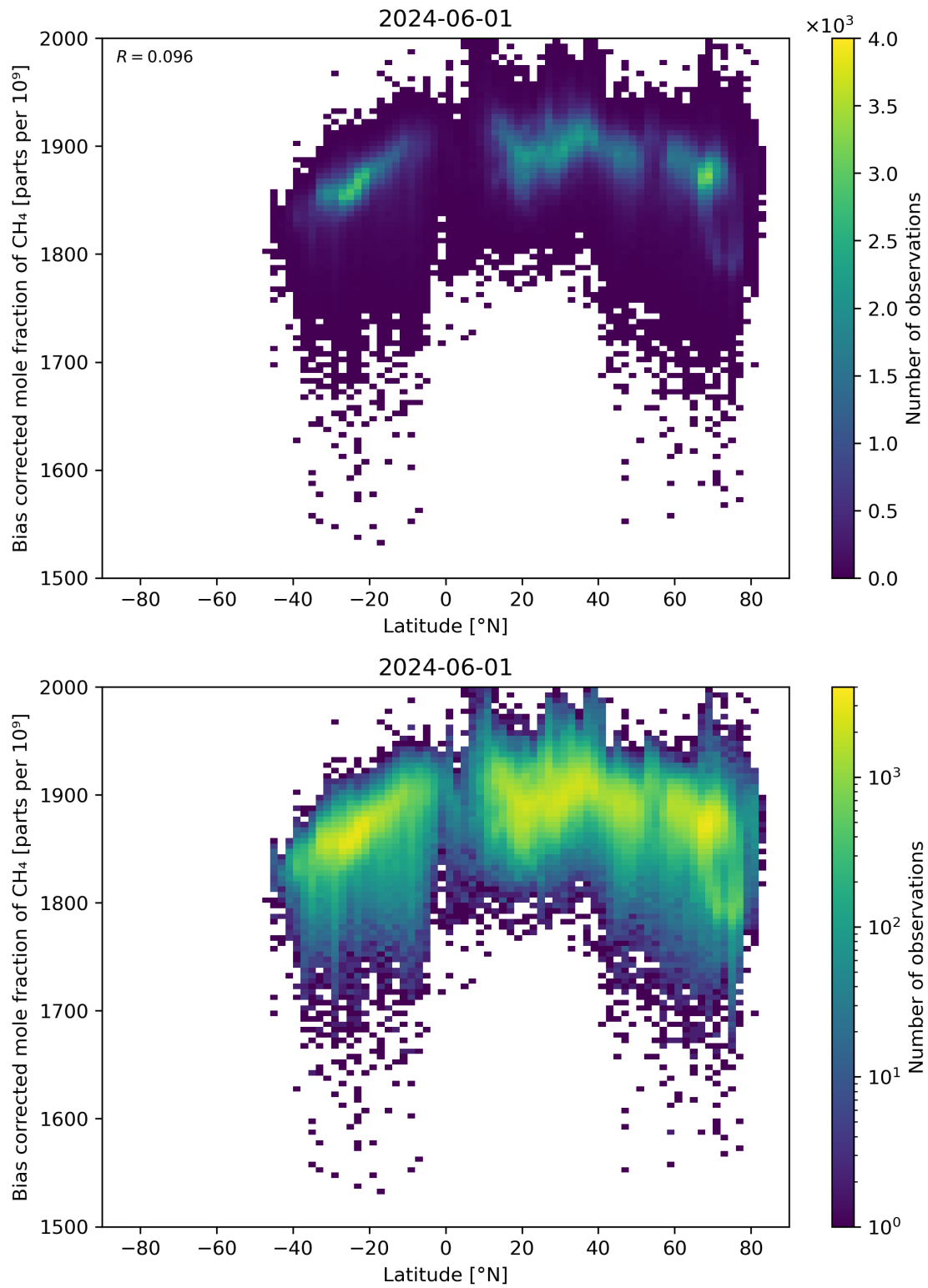
Figure 58: Scatter density plot of “Latitude” against “Bias corrected mole fraction of CH 4 ” for 2024-05-31 to 2024-06-02.
