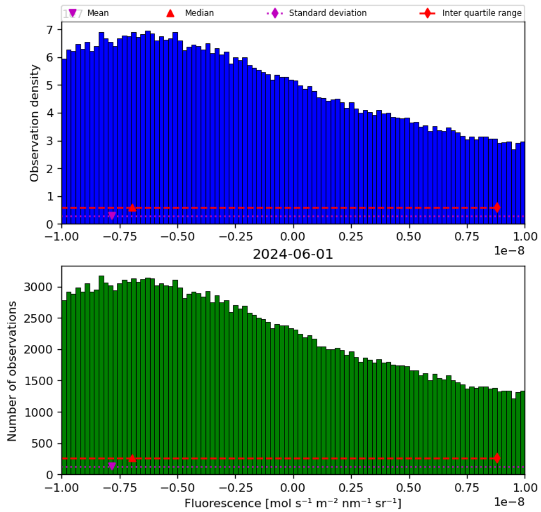
Figure 32: Histogram of “Fluorescence” for 2024-05-31 to 2024-06-02
