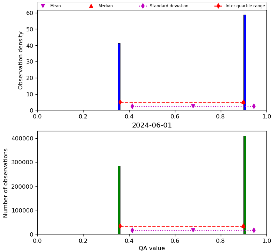
Figure 22: Histogram of “QA value” for 2024-05-31 to 2024-06-02
