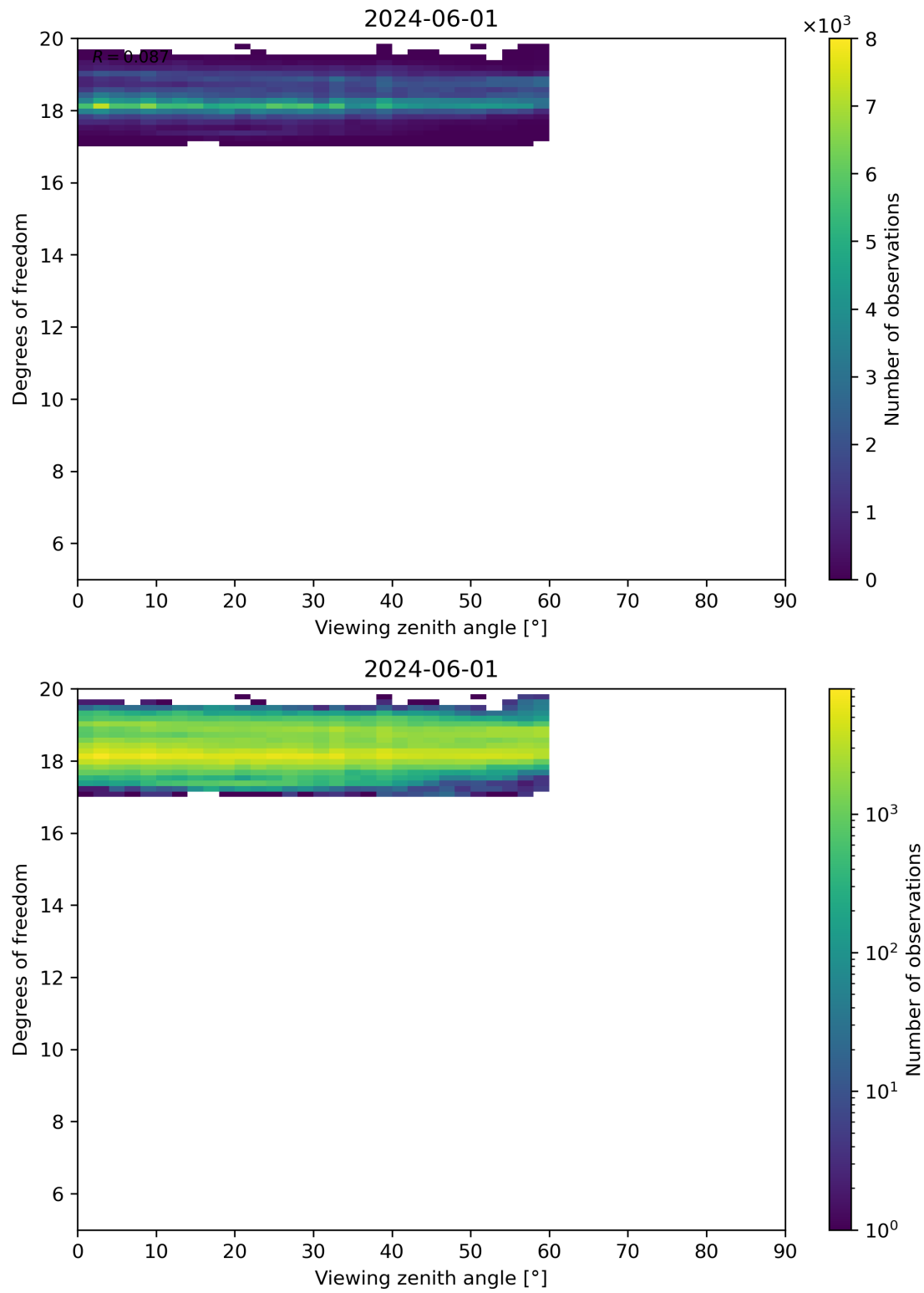
Figure 107: Scatter density plot of “Viewing zenith angle” against “Degrees of freedom” for 2024-05-31 to 2024-06-02.
