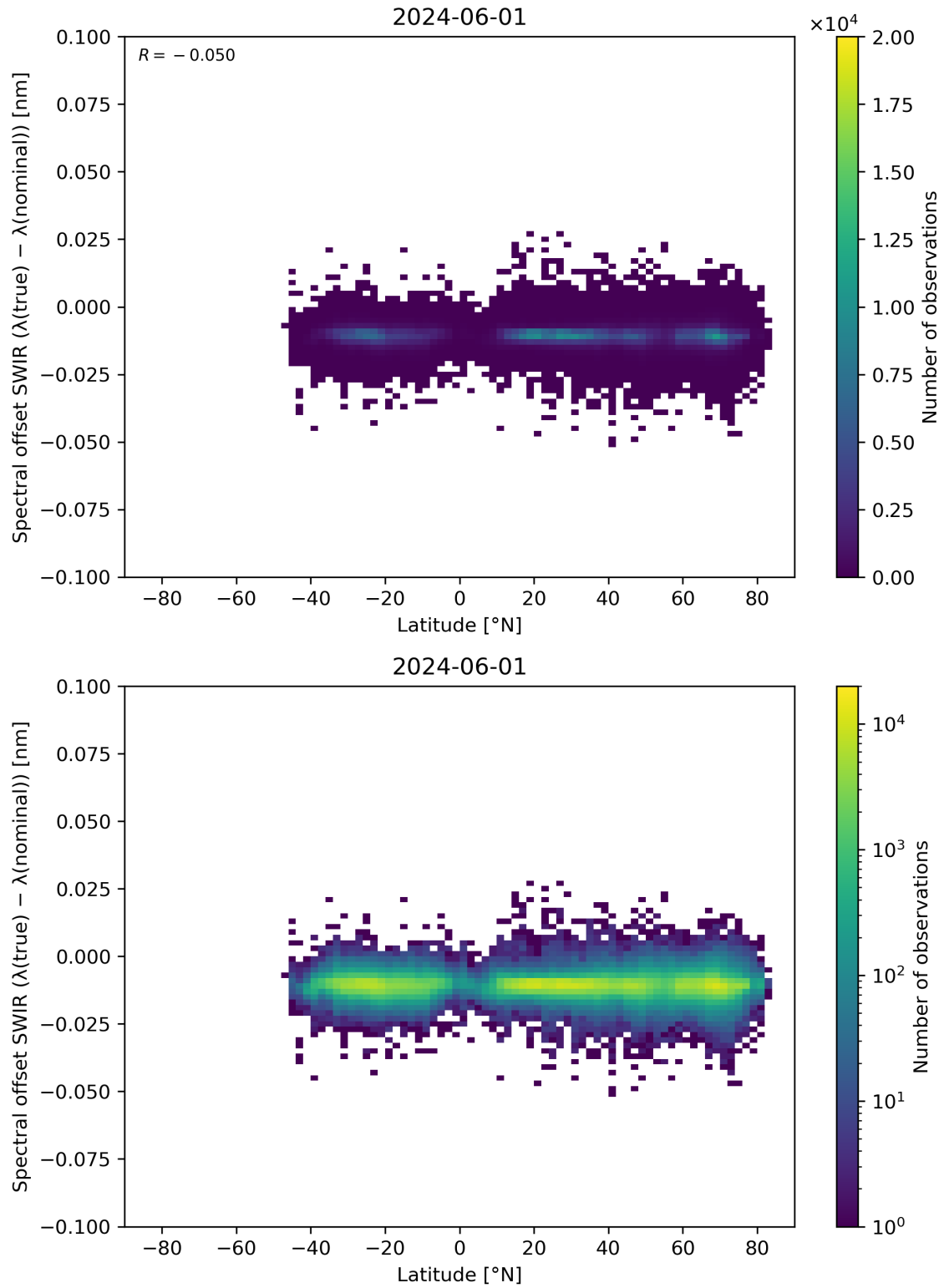
Figure 62: Scatter density plot of “Latitude” against “Spectral offset SWIR ( \lambda(\text{true}) - \lambda(\text{nominal}) )” for 2024-05-31 to 2024-06-02.
