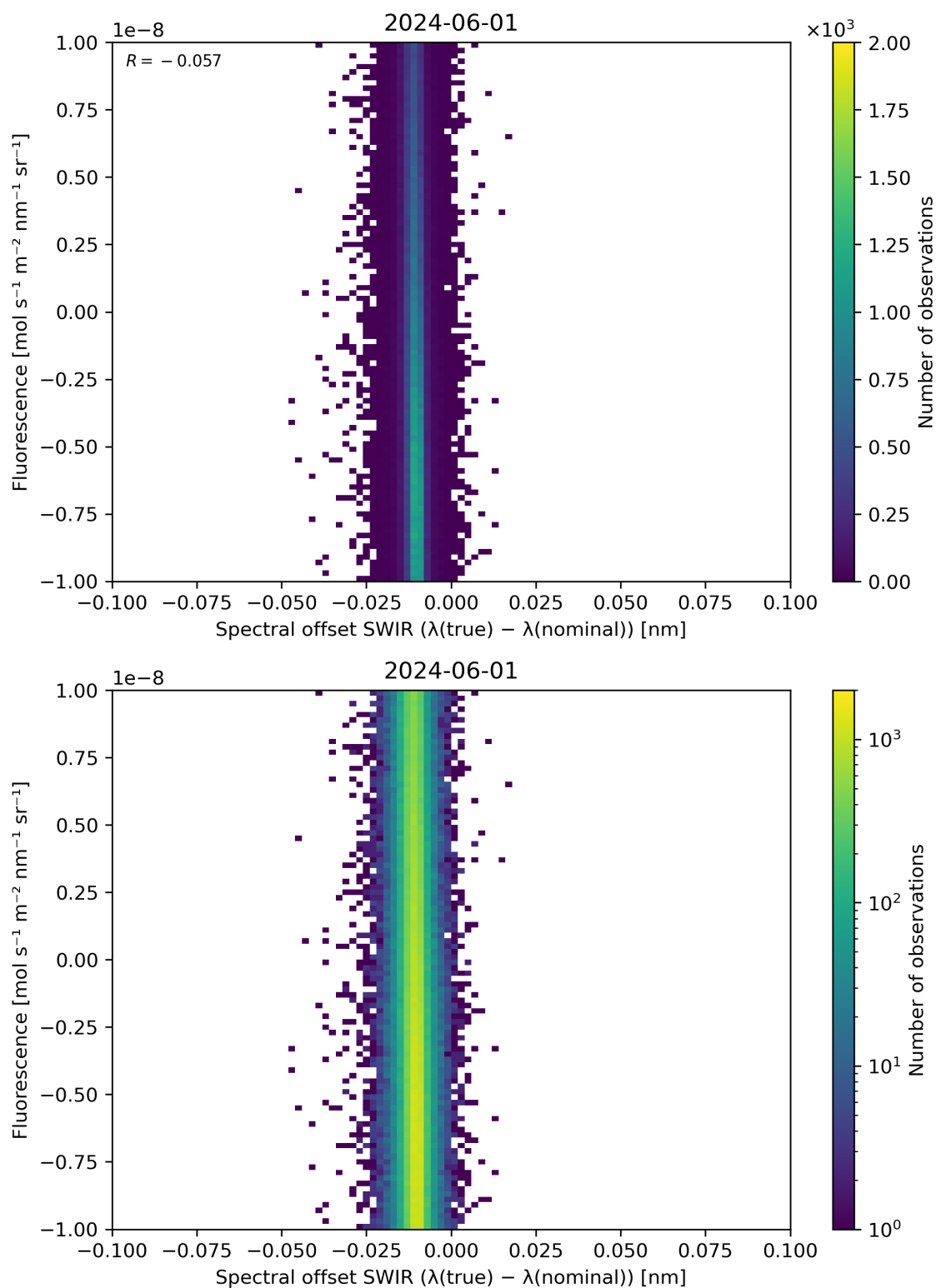
Figure 120: Scatter density plot of “Spectral offset SWIR ( \lambda(\text{true}) - \lambda(\text{nominal}) )” against “Fluorescence” for 2024-05-31 to 2024-06-02.
