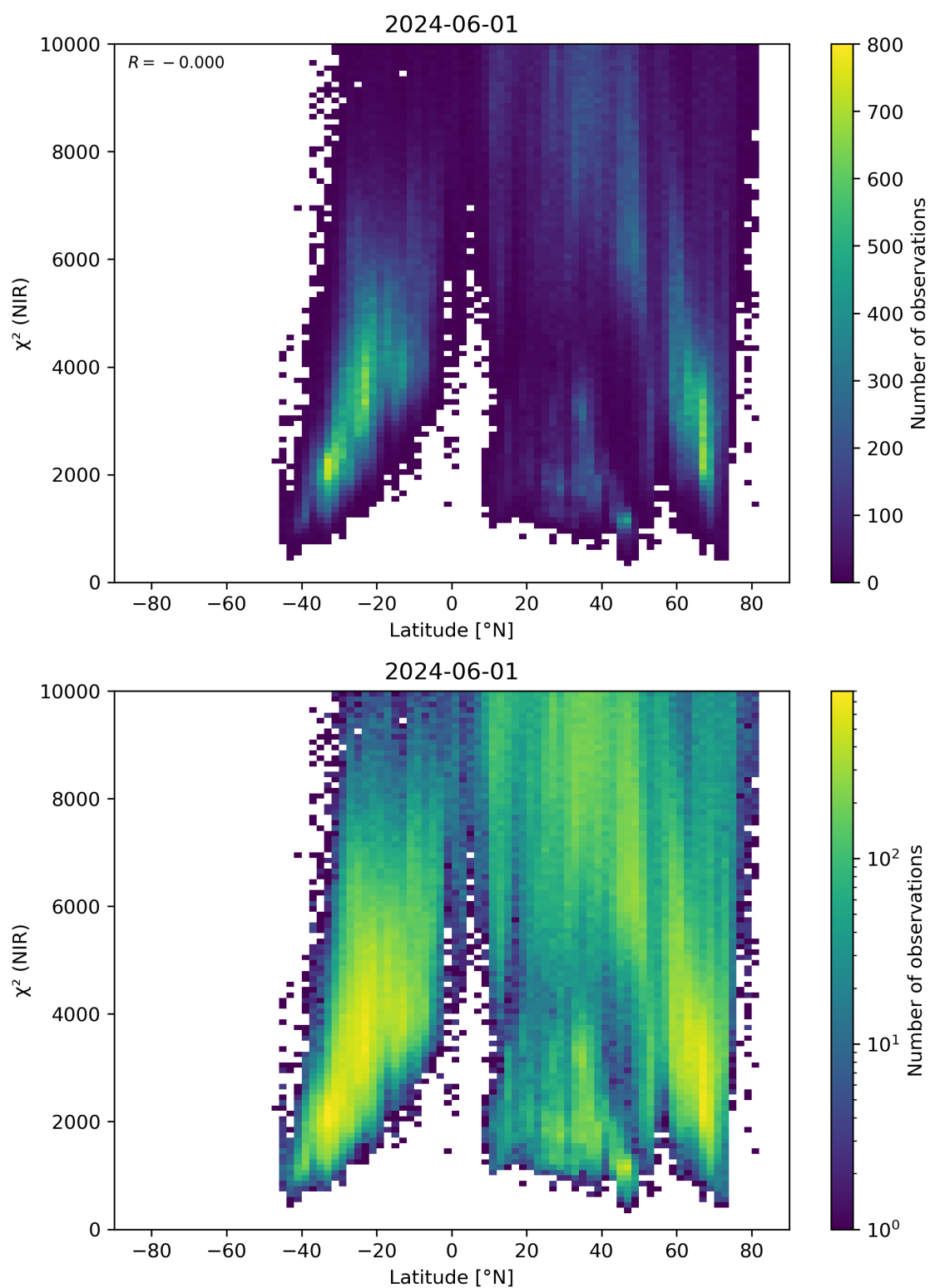
Figure 53: Scatter density plot of “Latitude” against “ \chi^2 (NIR)” for 2024-05-31 to 2024-06-02.
