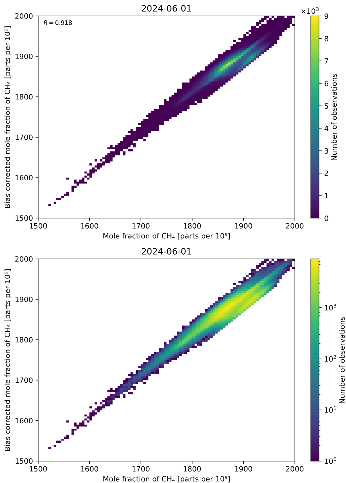
Figure 74: Scatter density plot of “Mole fraction of CH 4 ” against “Bias corrected mole fraction of CH 4 ” for 2024-05-31 to 2024-06-02.
