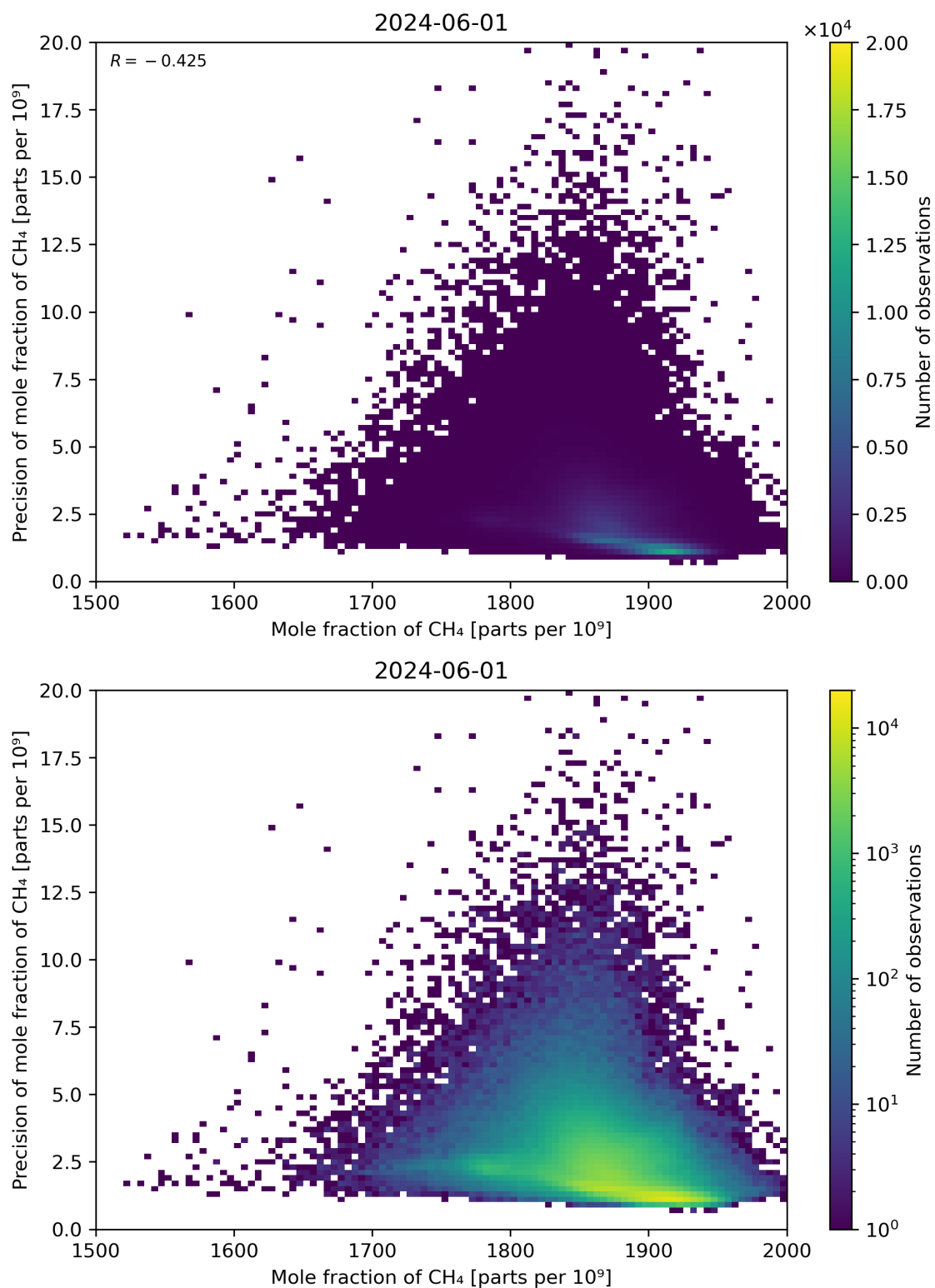
Figure 75: Scatter density plot of “Mole fraction of CH 4 ” against “Precision of mole fraction of CH 4 ” for 2024-05-31 to 2024-06-02.
