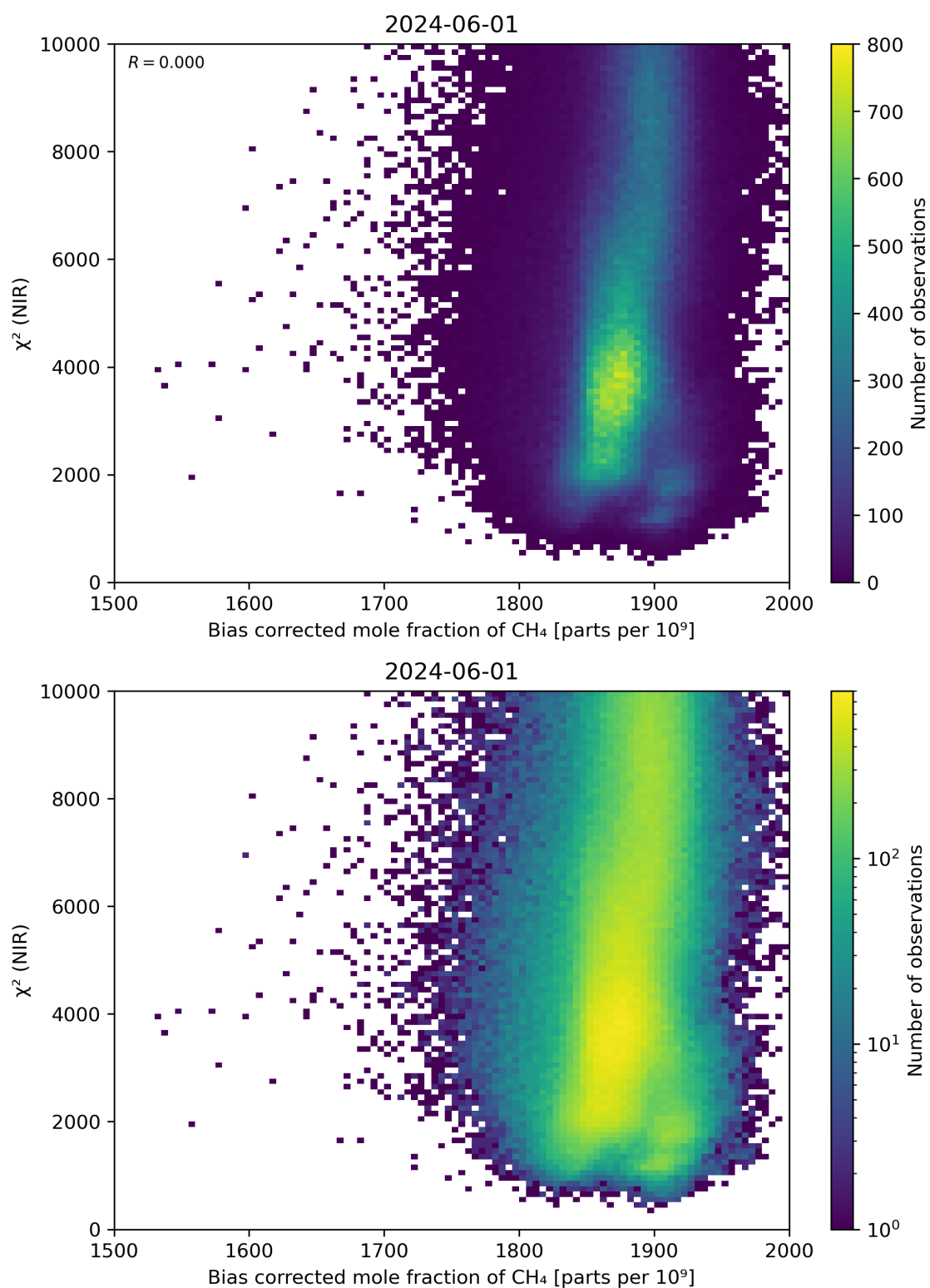
Figure 63: Scatter density plot of “Bias corrected mole fraction of \text{CH}_4 ” against “ \chi^2 (NIR)” for 2024-05-31 to 2024-06-02.
