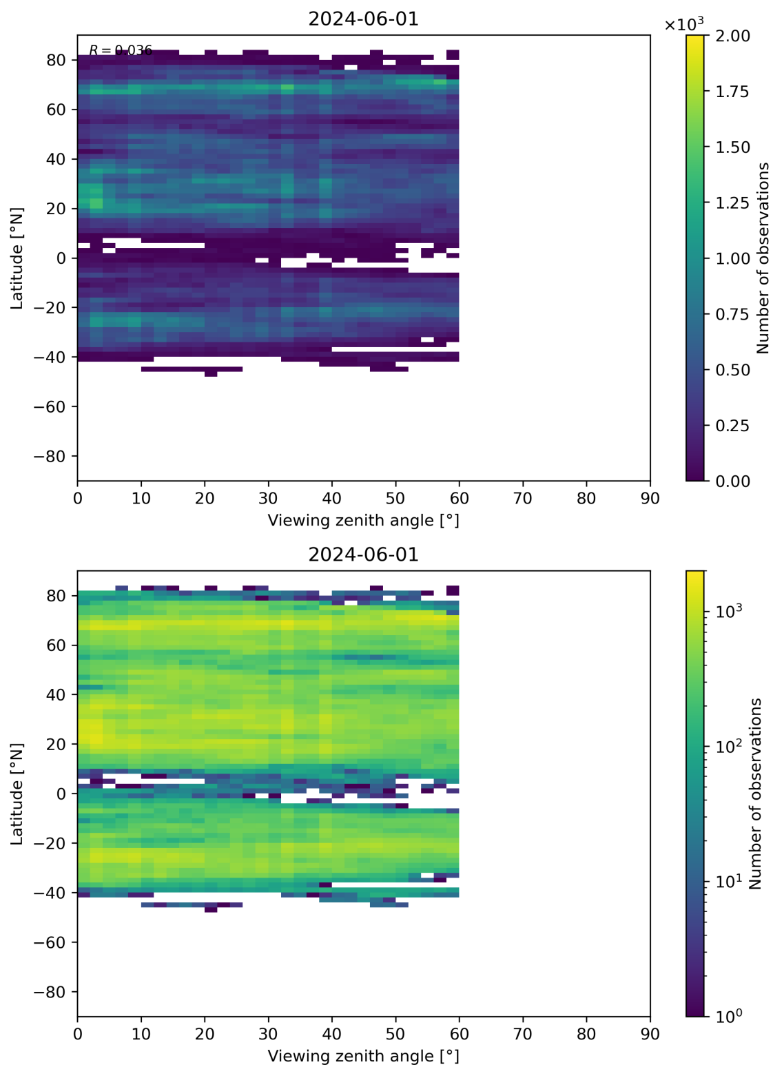
Figure 109: Scatter density plot of “Viewing zenith angle” against “Latitude” for 2024-05-31 to 2024-06-02.
