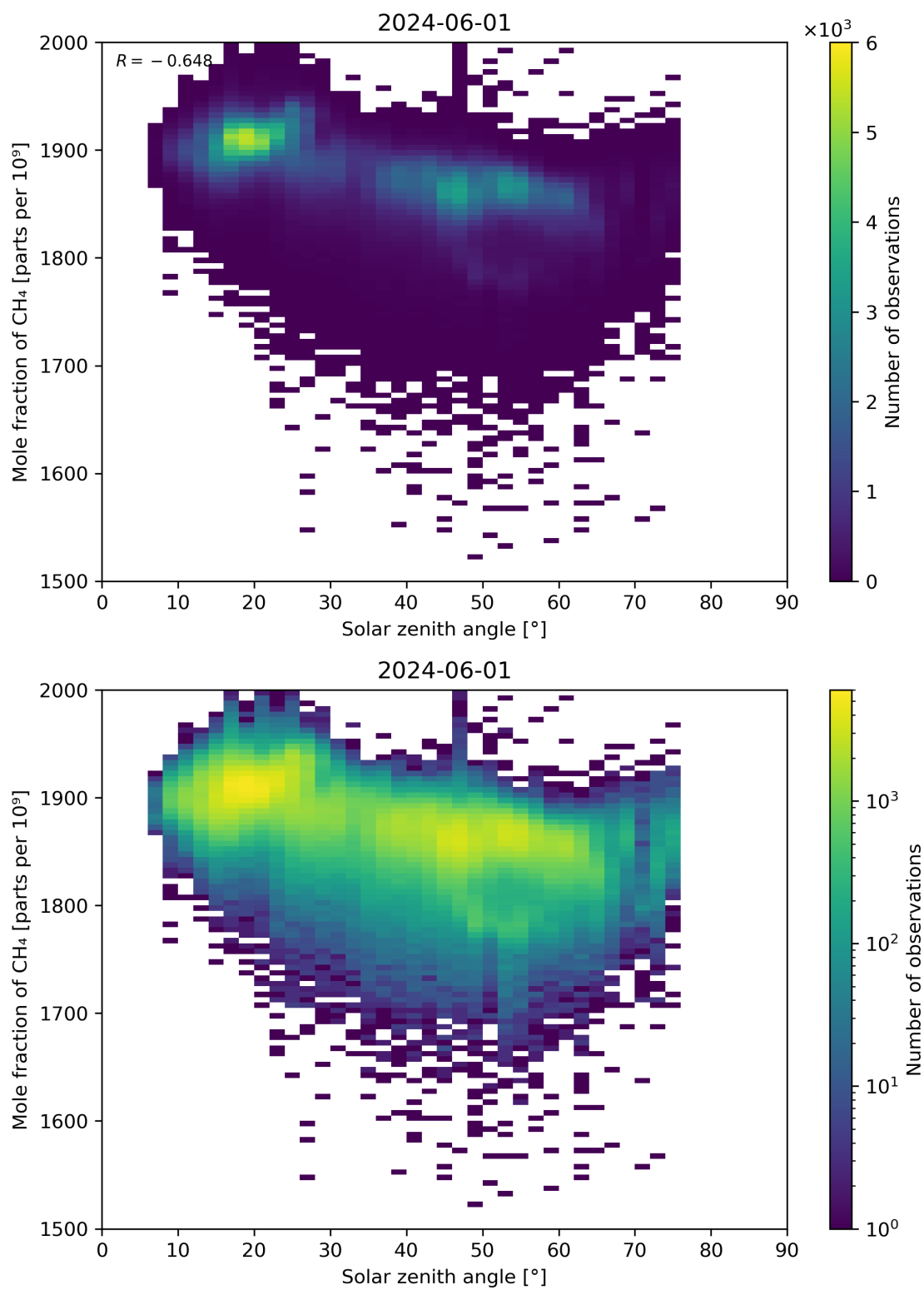
Figure 99: Scatter density plot of “Solar zenith angle” against “Mole fraction of CH 4 ” for 2024-05-31 to 2024-06-02.
