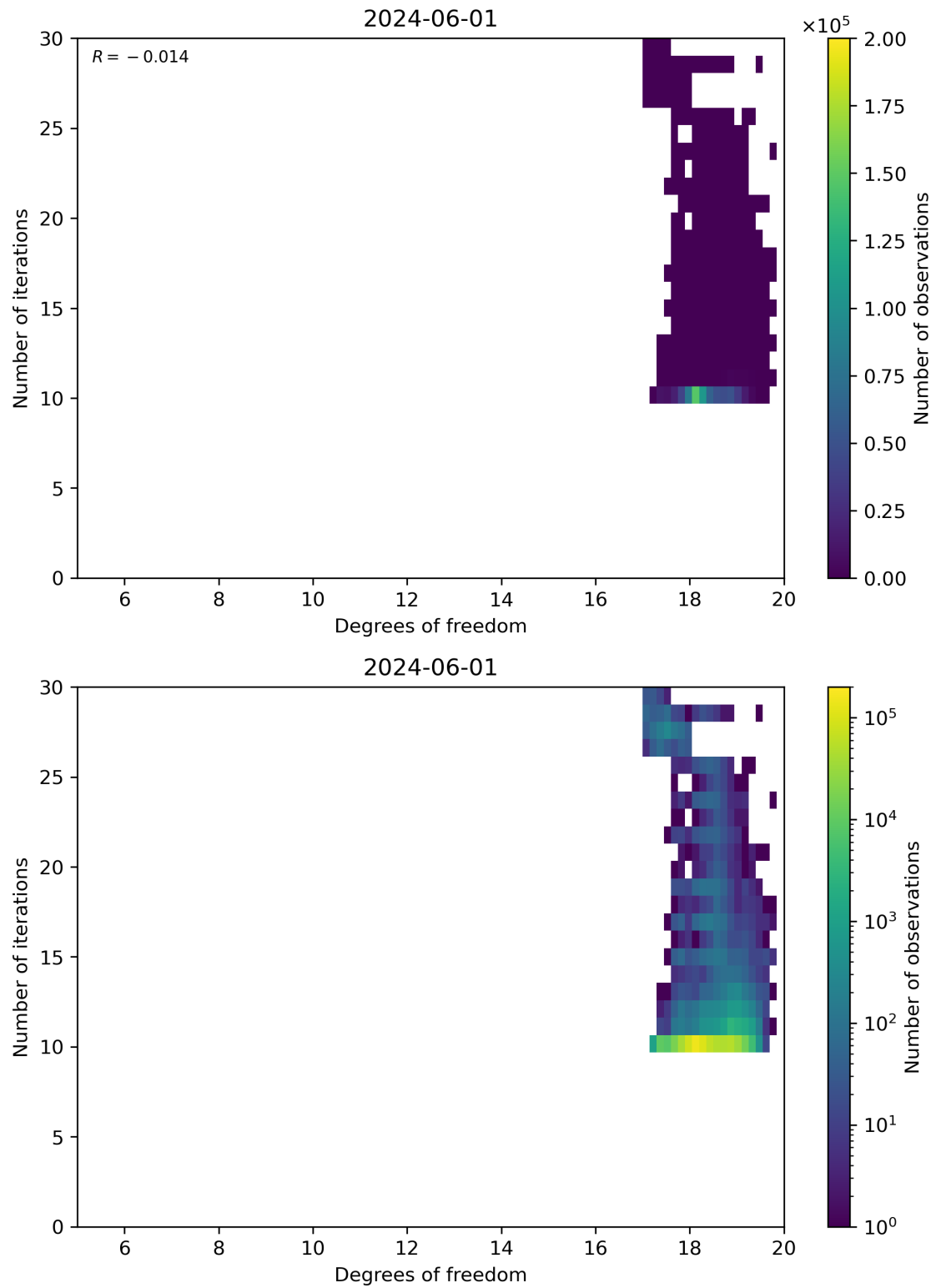
Figure 52: Scatter density plot of “Degrees of freedom” against “Number of iterations” for 2024-05-31 to 2024-06-02.
