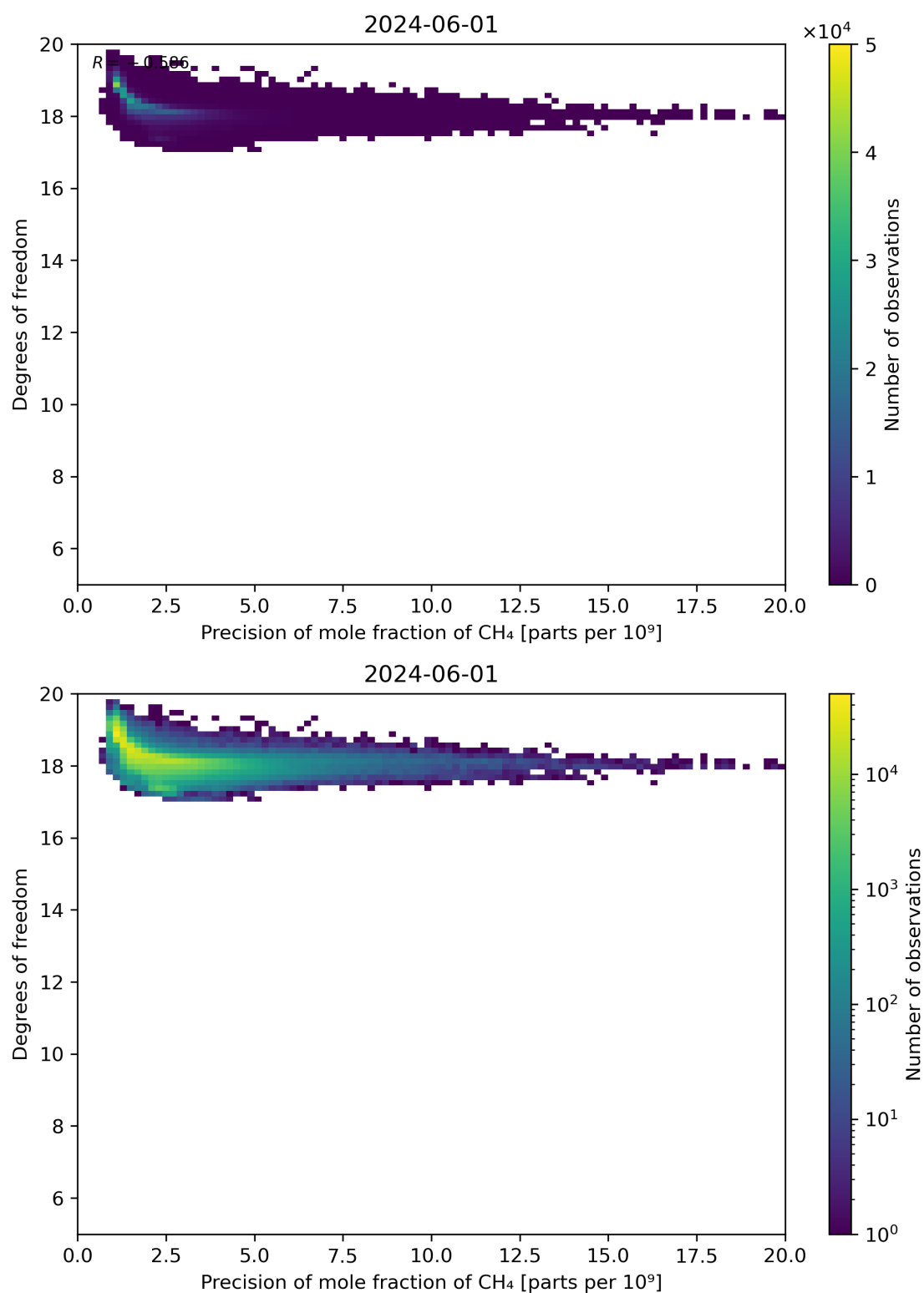
Figure 80: Scatter density plot of “Precision of mole fraction of CH 4 ” against “Degrees of freedom” for 2024-05-31 to 2024-06-02.
