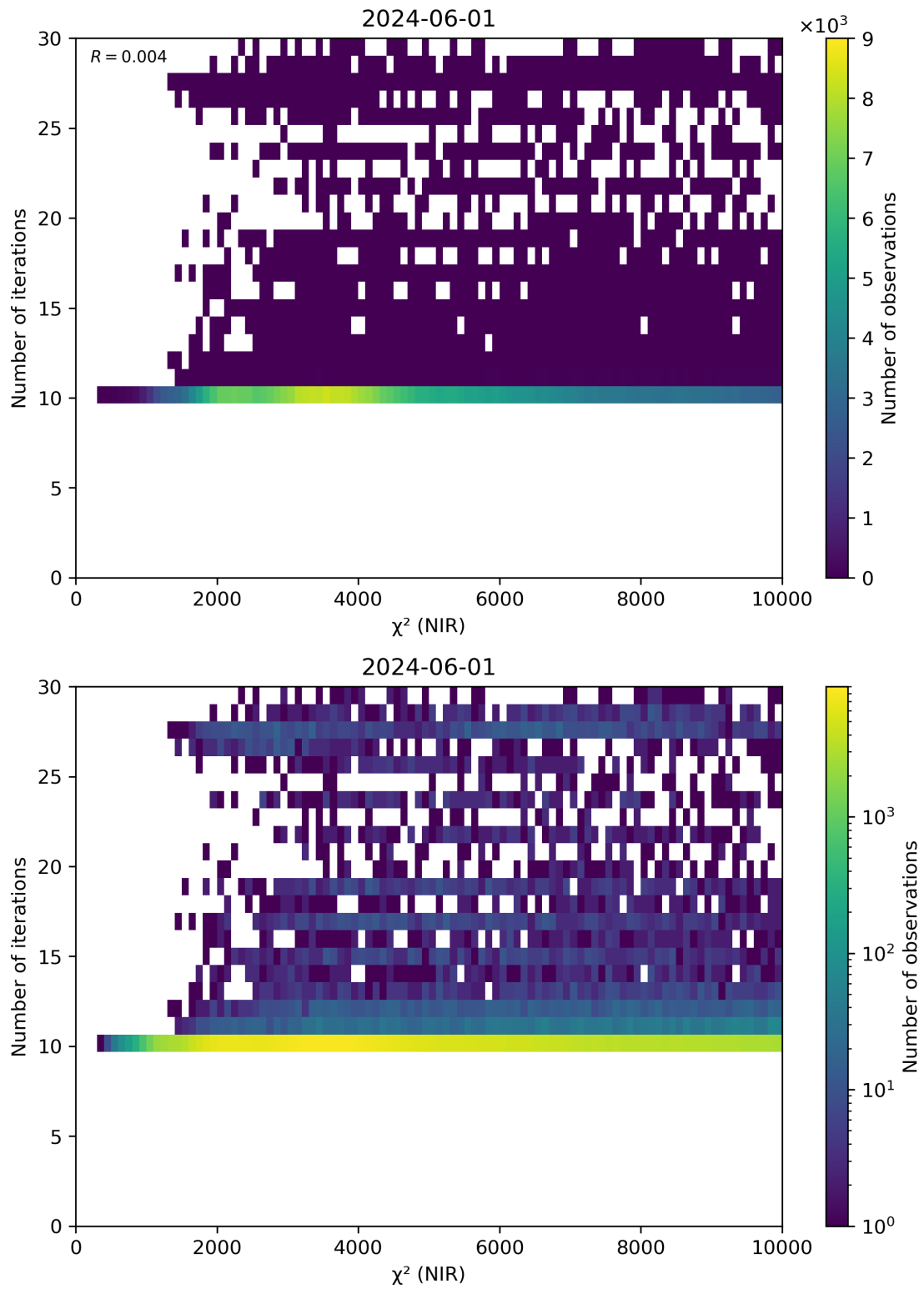
Figure 46: Scatter density plot of “ \chi^2 (NIR)” against “Number of iterations” for 2024-05-31 to 2024-06-02.
