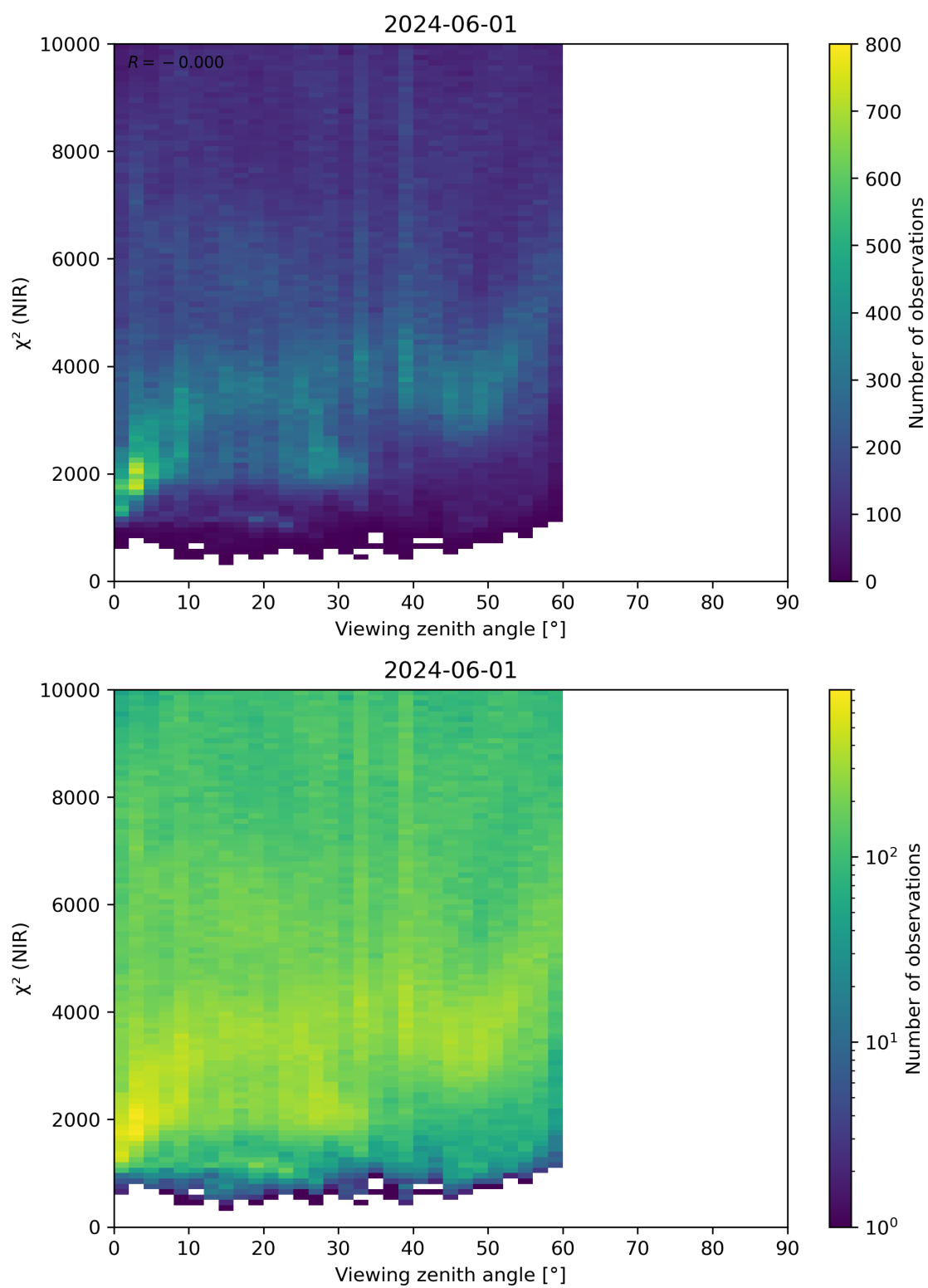
Figure 105: Scatter density plot of “Viewing zenith angle” against “ \chi^2 (NIR)” for 2024-05-31 to 2024-06-02.
