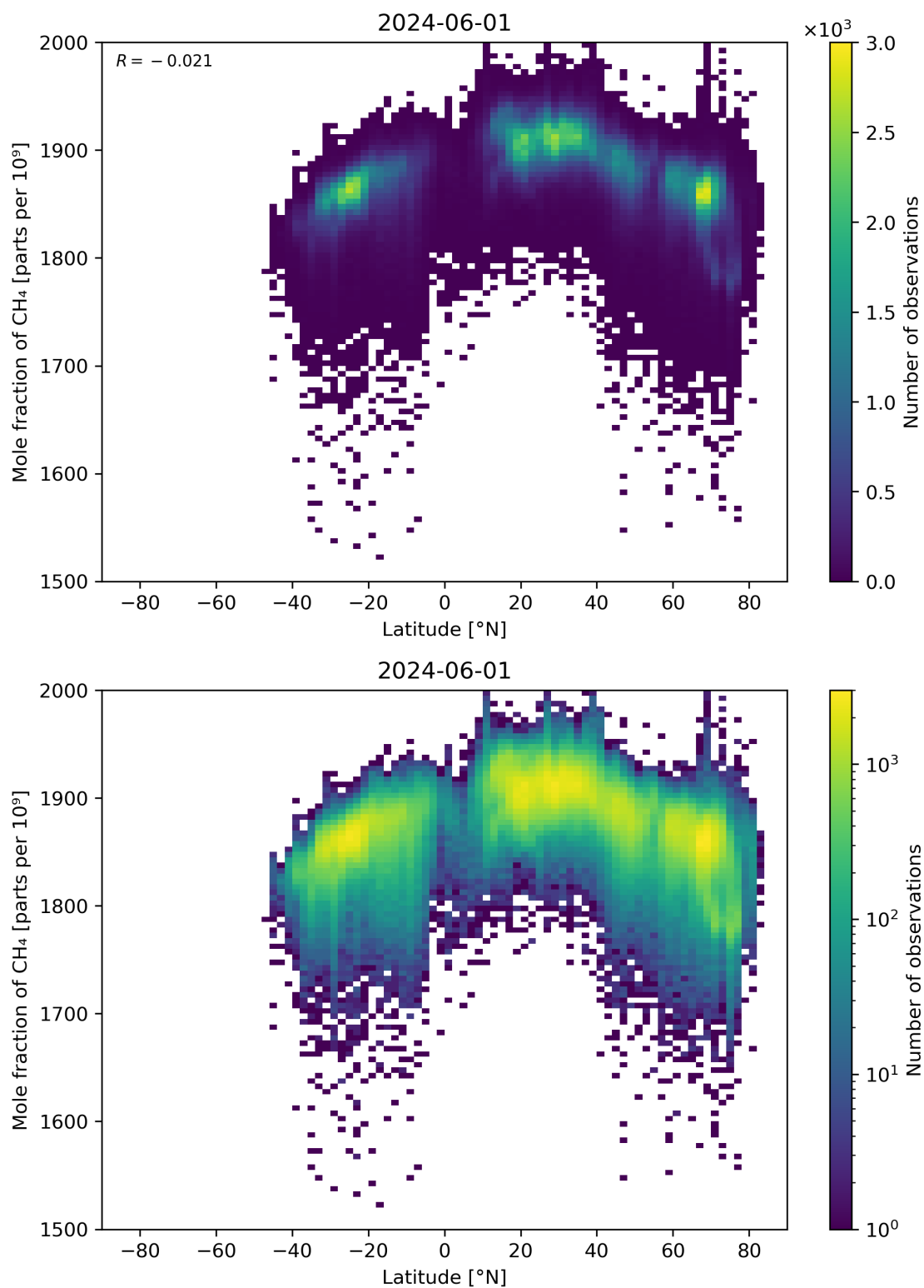
Figure 57: Scatter density plot of “Latitude” against “Mole fraction of \text{CH}_4 ” for 2024-05-31 to 2024-06-02.
