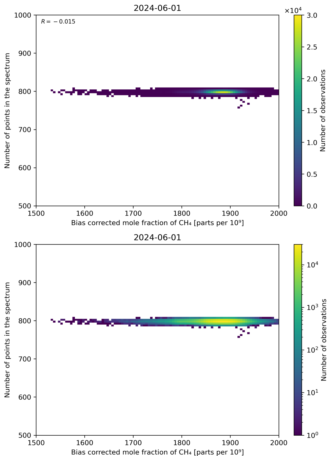
Figure 68: Scatter density plot of “Bias corrected mole fraction of CH 4 ” against “Number of points in the spectrum” for 2024-05-31 to 2024-06-02.
