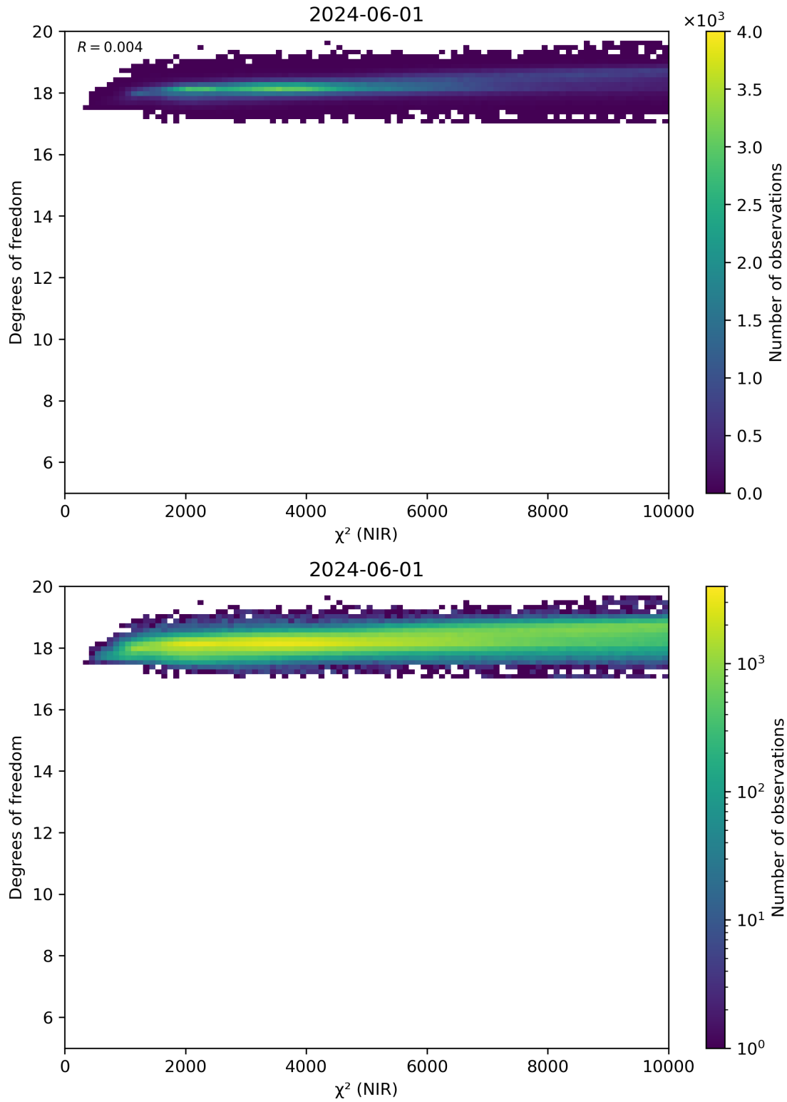
Figure 44: Scatter density plot of “ \chi^2 (NIR)” against “Degrees of freedom” for 2024-05-31 to 2024-06-02.
