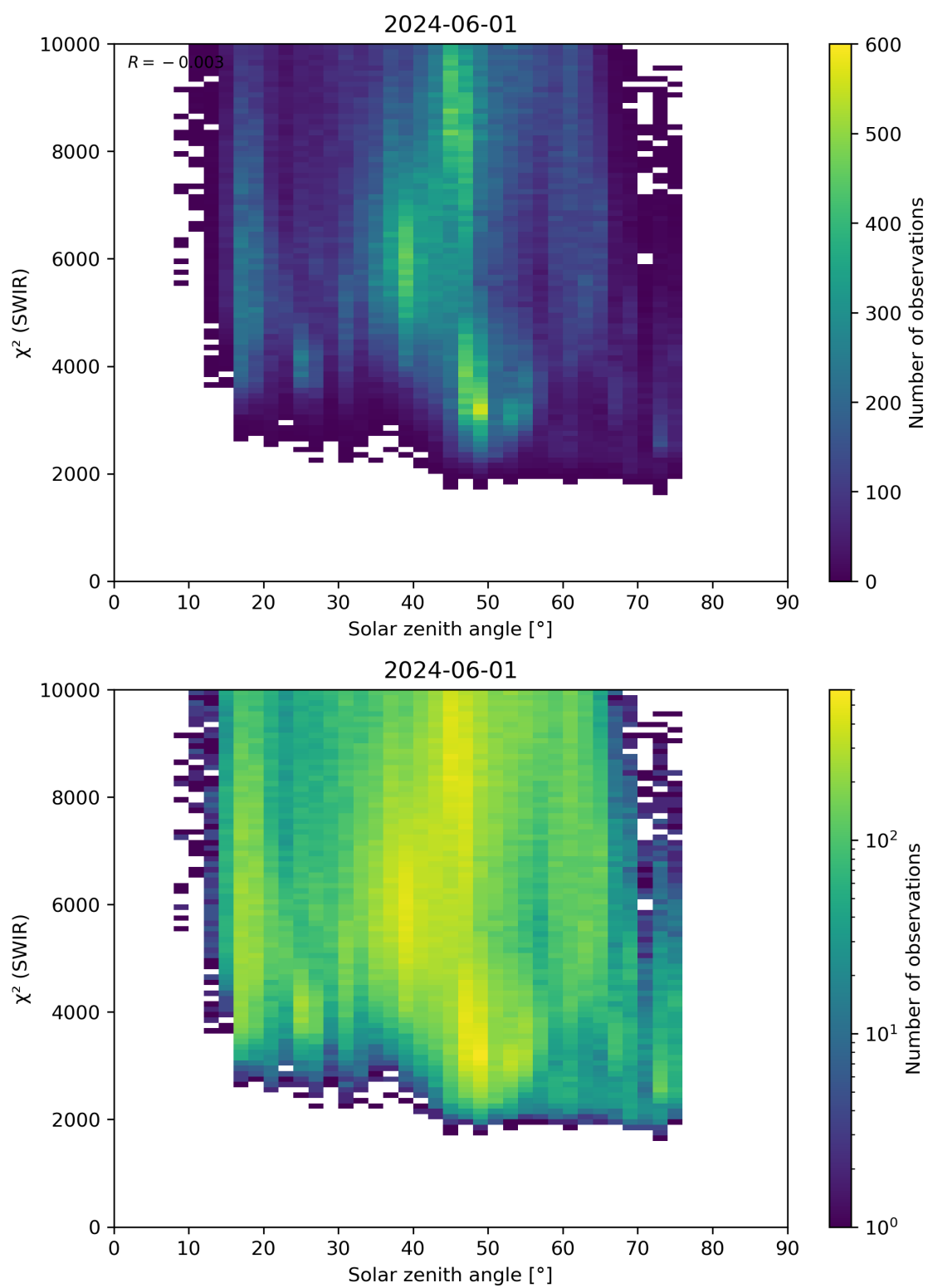
Figure 95: Scatter density plot of “Solar zenith angle” against “ \chi^2 (SWIR)” for 2024-05-31 to 2024-06-02.
