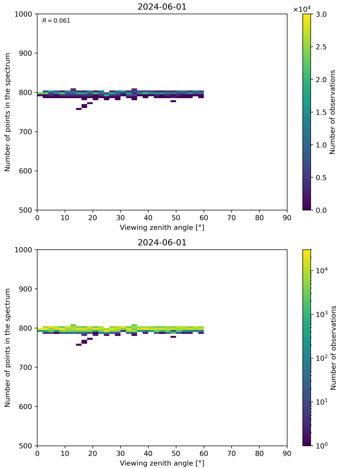
Figure 114: Scatter density plot of “Viewing zenith angle” against “Number of points in the spectrum” for 2024-05-31 to 2024-06-02.
