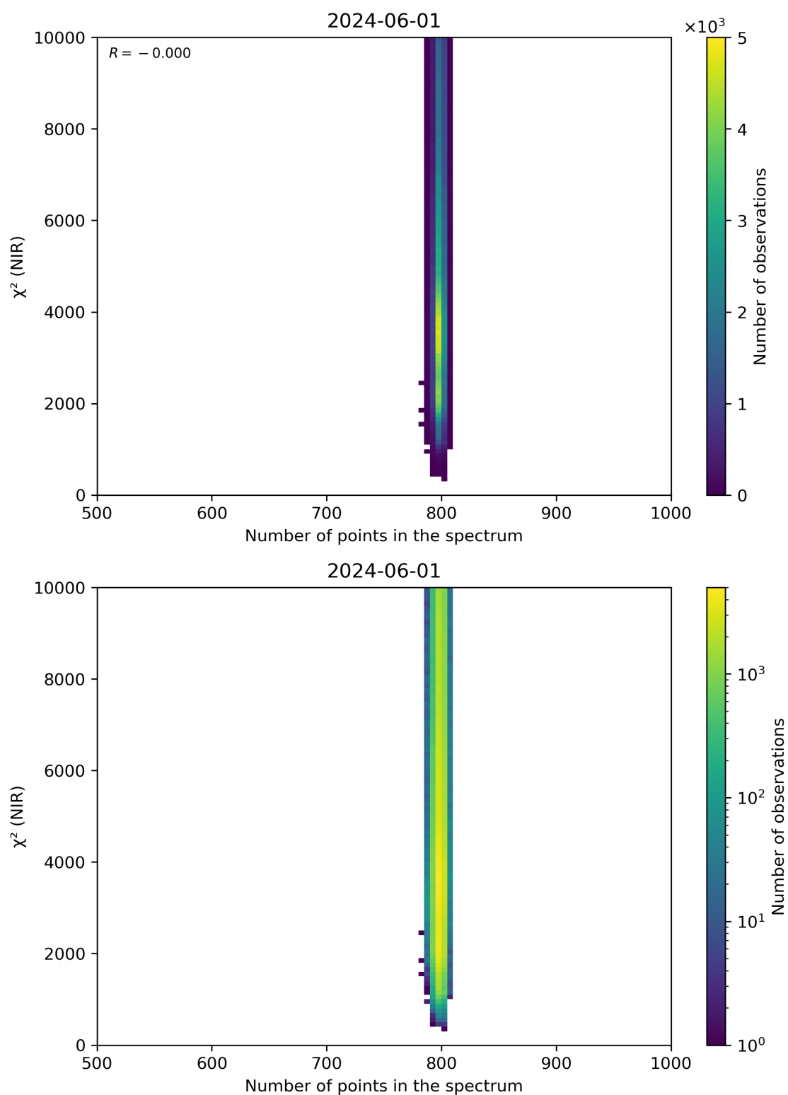
Figure 88: Scatter density plot of “Number of points in the spectrum” against “ \chi^2 (NIR)” for 2024-05-31 to 2024-06-02.
