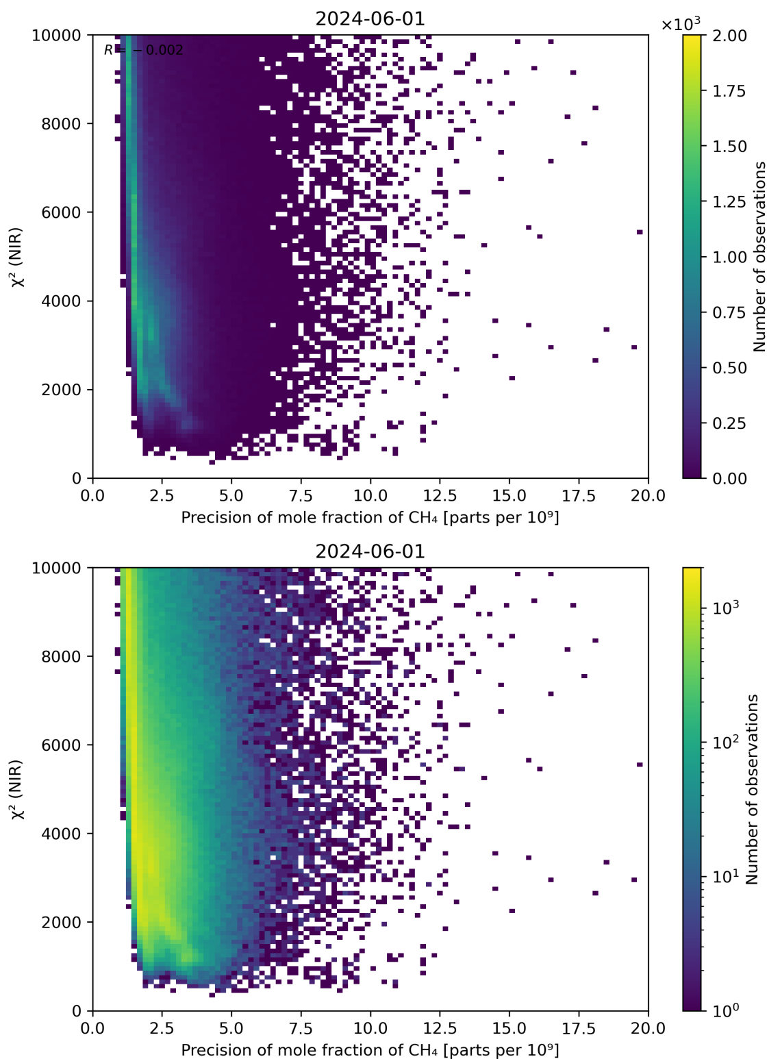
Figure 78: Scatter density plot of “Precision of mole fraction of \text{CH}_4 ” against “ \chi^2 (NIR)” for 2024-05-31 to 2024-06-02.
