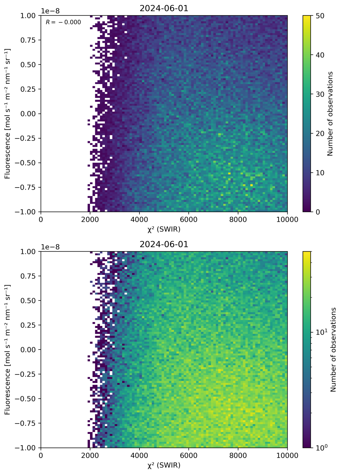
Figure 49: Scatter density plot of “ \chi^2 (SWIR)” against “Fluorescence” for 2024-05-31 to 2024-06-02.
