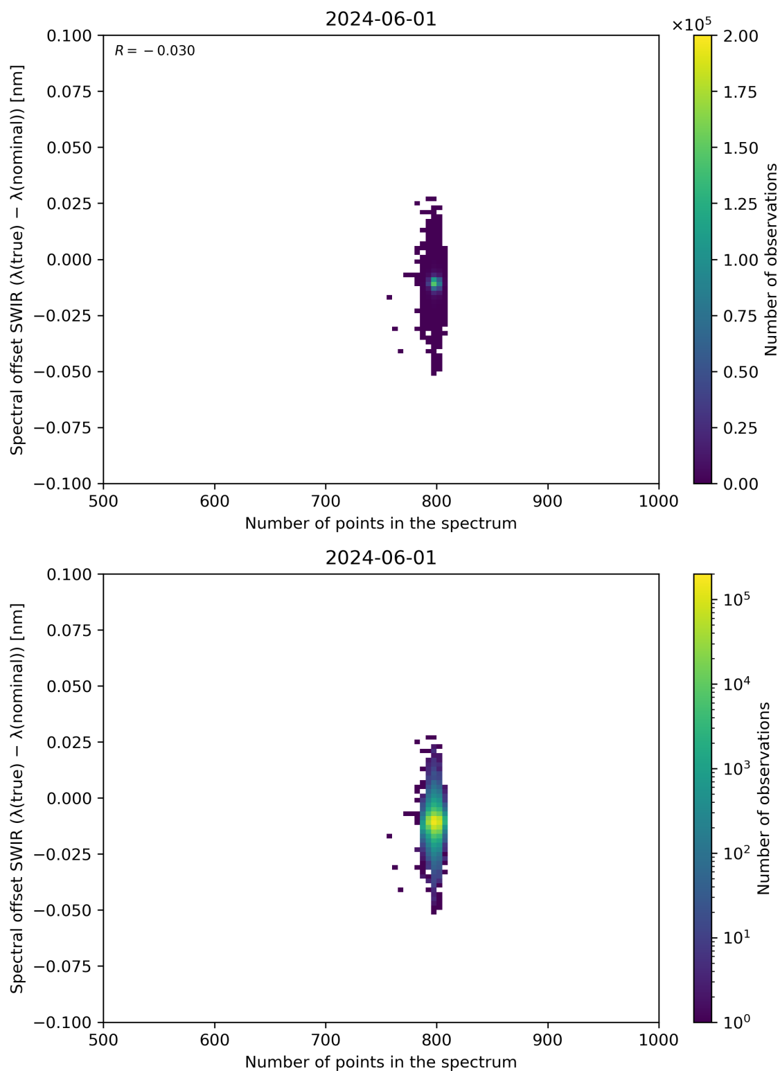
Figure 93: Scatter density plot of “Number of points in the spectrum” against “Spectral offset SWIR ( \lambda(\text{true}) - \lambda(\text{nominal}) )” for 2024-05-31 to 2024-06-02.
