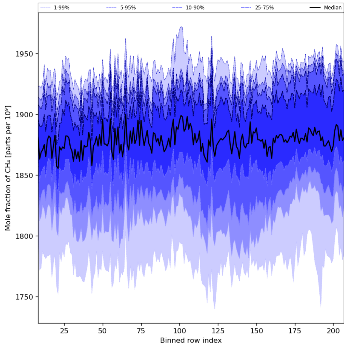
Figure 34: Along track statistics of “Mole fraction of CH 4 ” for 2024-05-31 to 2024-06-02
