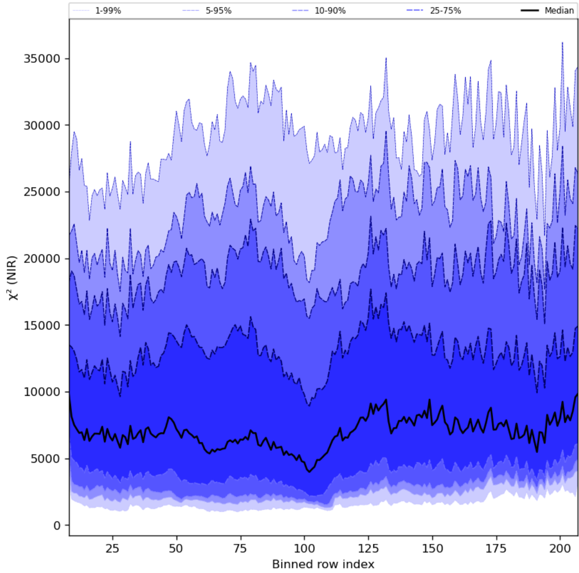
Figure 40: Along track statistics of “ \chi^2 (NIR)” for 2024-05-31 to 2024-06-02
