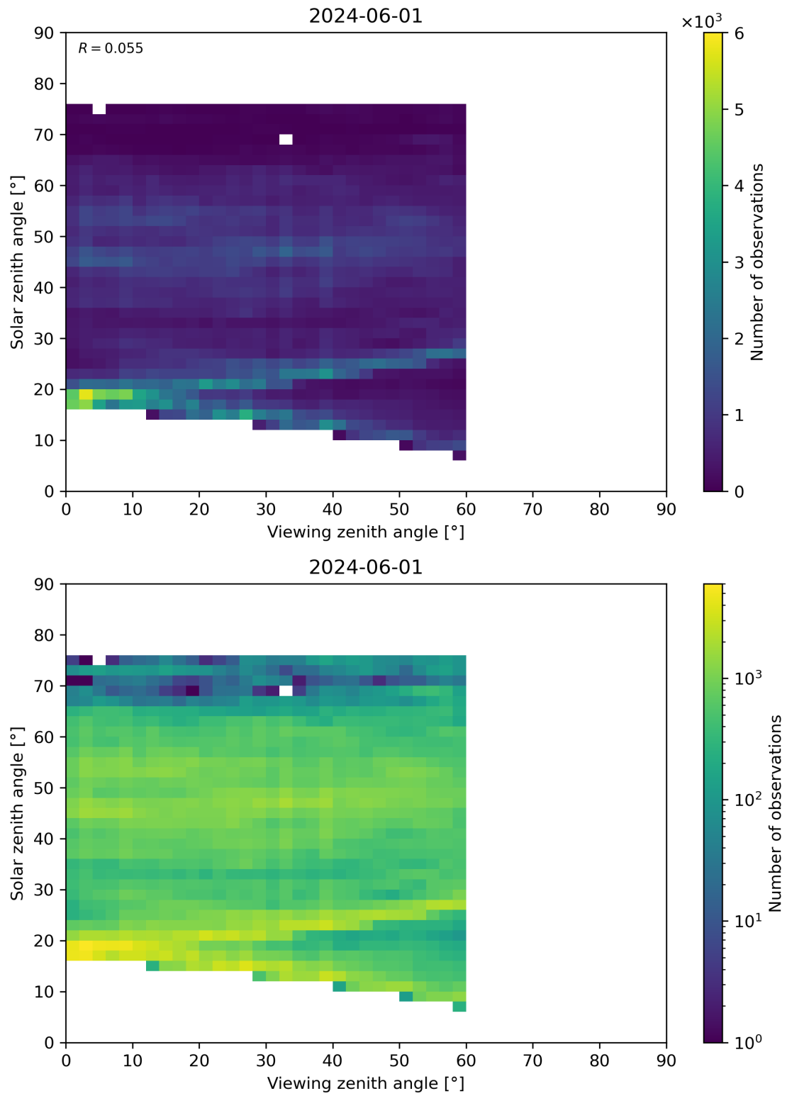
Figure 115: Scatter density plot of “Viewing zenith angle” against “Solar zenith angle” for 2024-05-31 to 2024-06-02.
