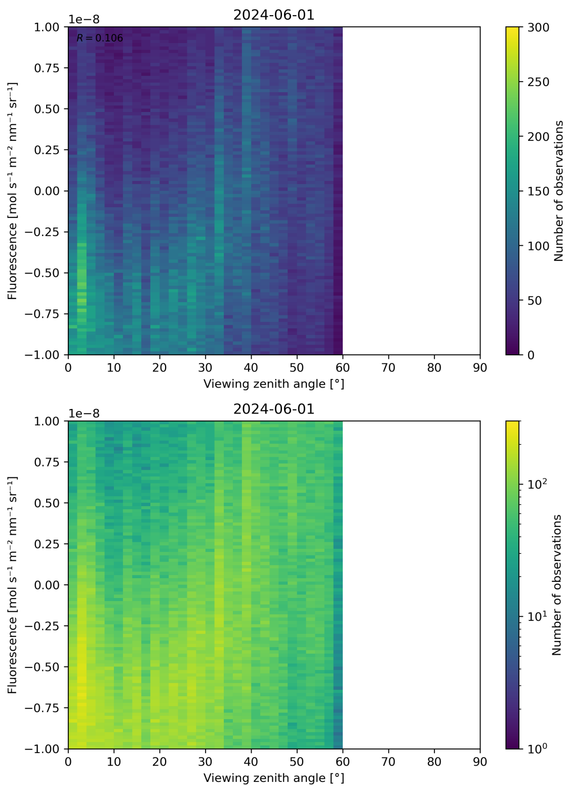
Figure 108: Scatter density plot of “Viewing zenith angle” against “Fluorescence” for 2024-05-31 to 2024-06-02.
