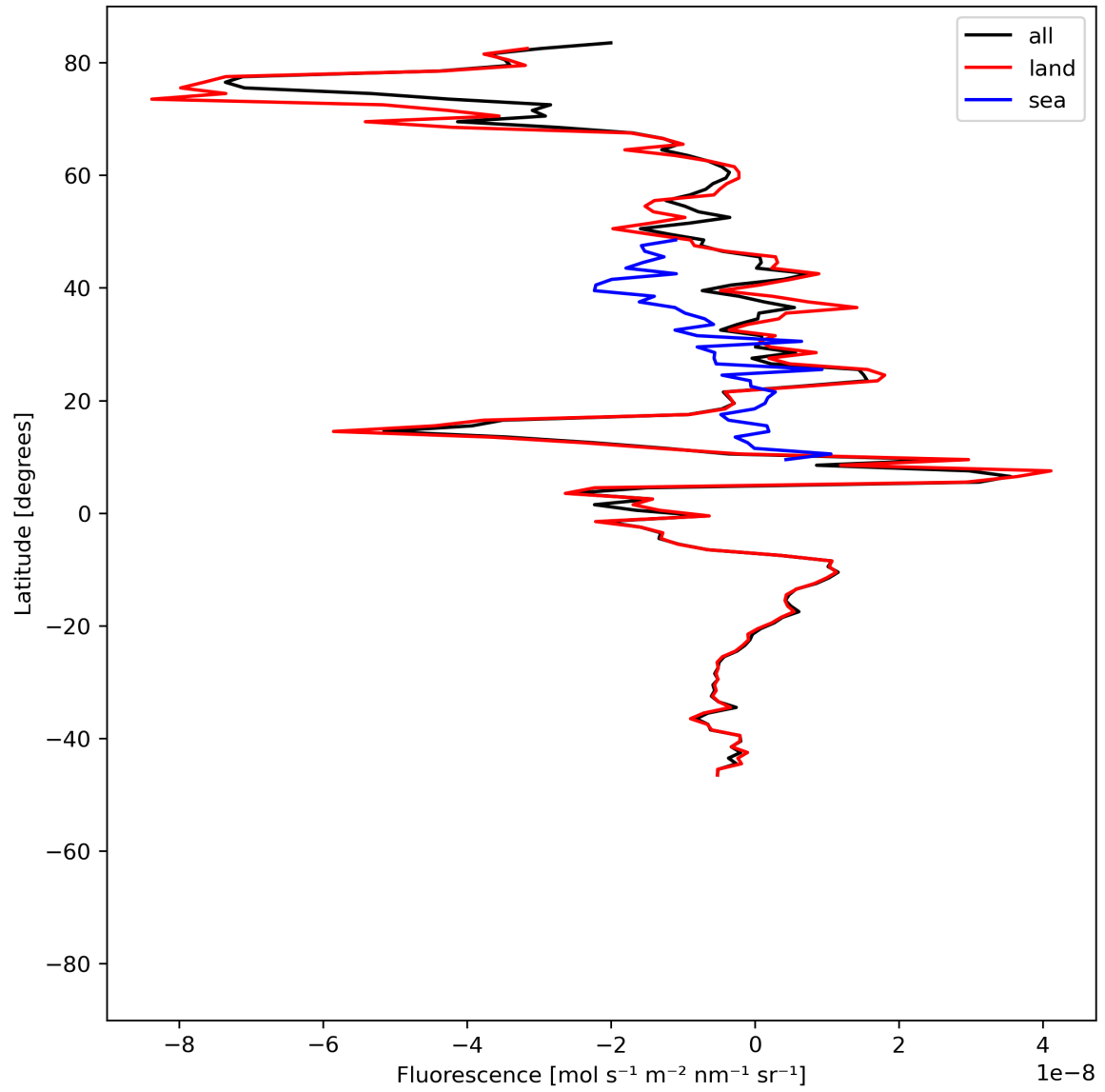
Figure 21: Zonal average of “Fluorescence” for 2024-05-31 to 2024-06-02.
