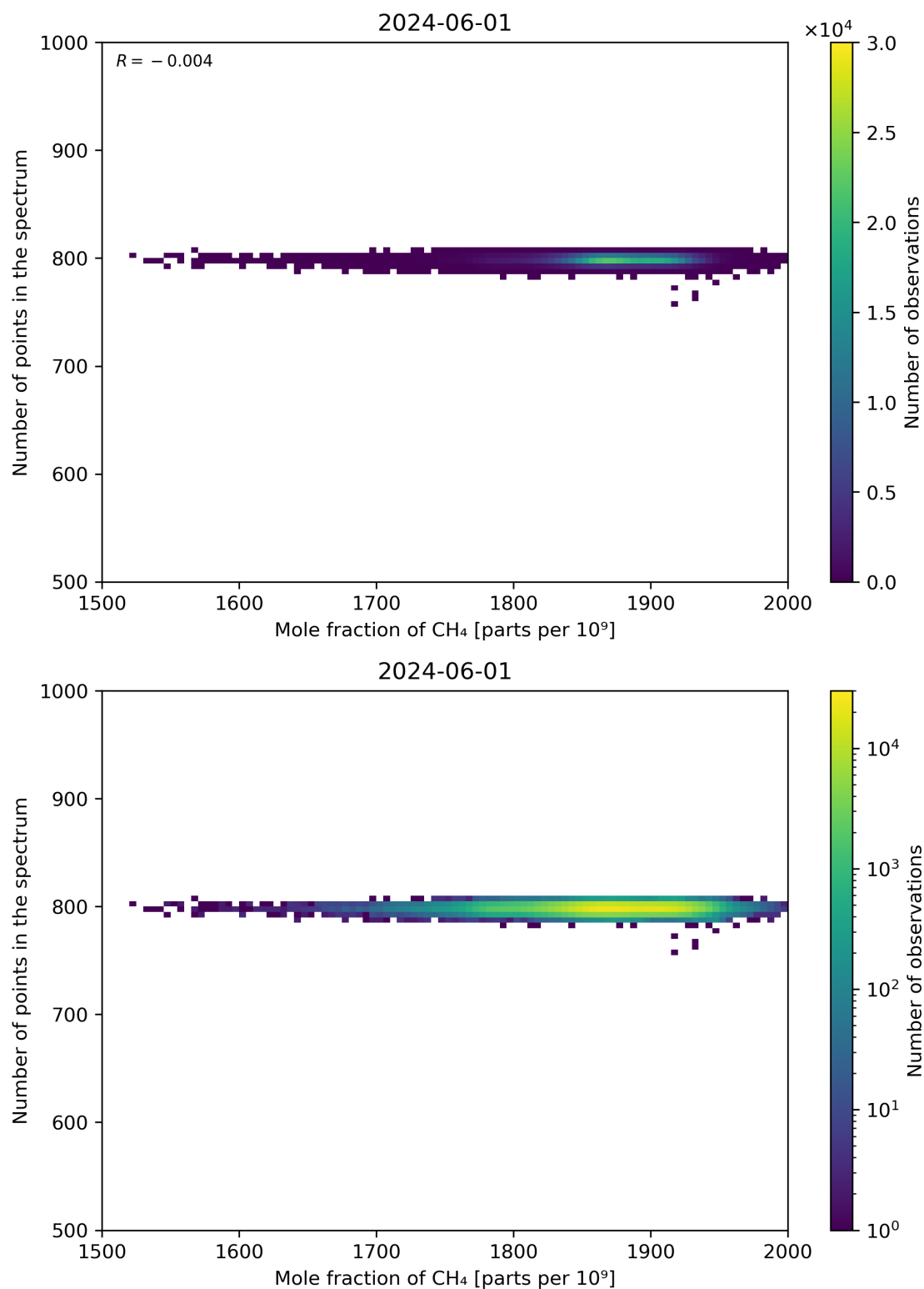
Figure 77: Scatter density plot of “Mole fraction of CH 4 ” against “Number of points in the spectrum” for 2024-05-31 to 2024-06-02.
