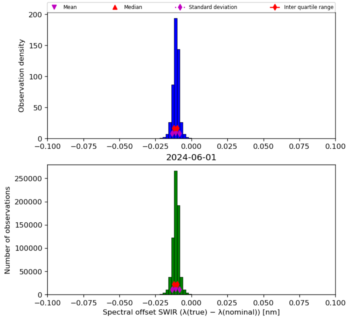
Figure 27: Histogram of “Spectral offset SWIR ( \lambda(\text{true}) - \lambda(\text{nominal}) )” for 2024-05-31 to 2024-06-02
