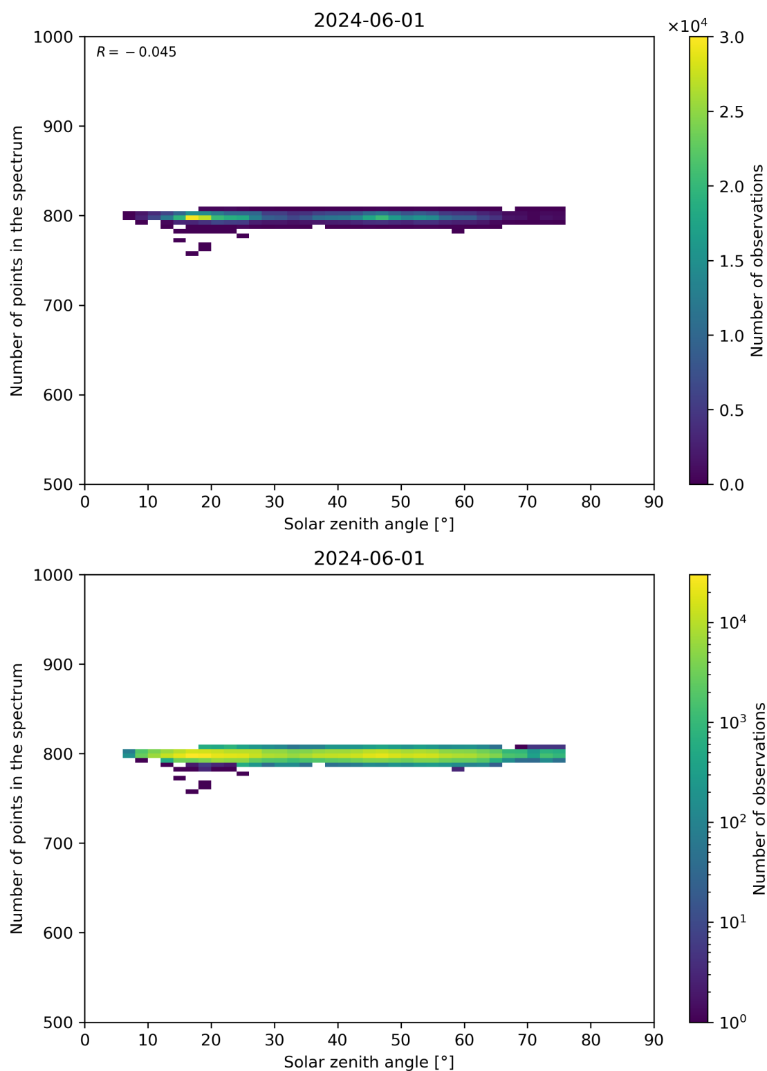
Figure 103: Scatter density plot of “Solar zenith angle” against “Number of points in the spectrum” for 2024-05-31 to 2024-06-02.
