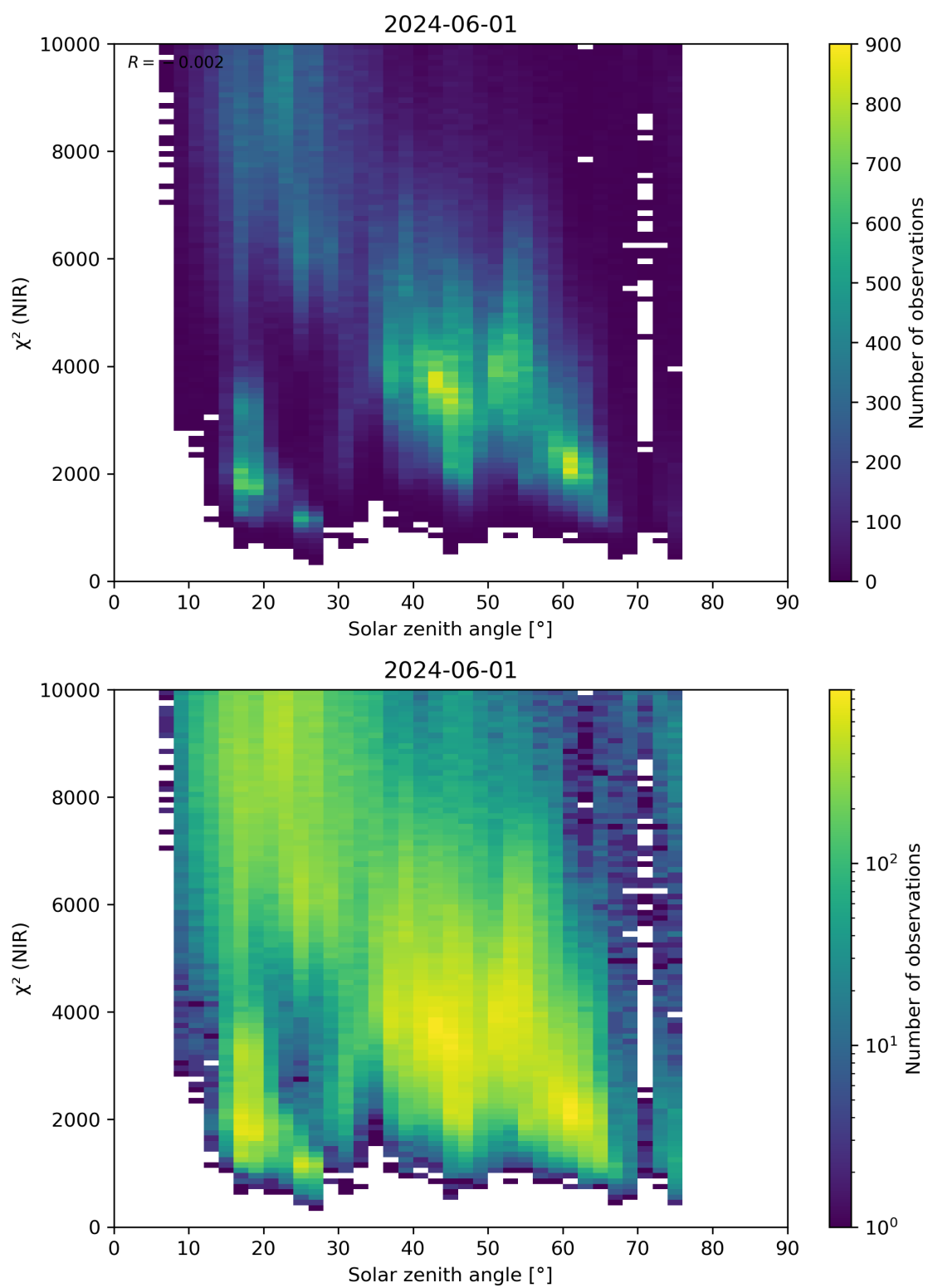
Figure 94: Scatter density plot of “Solar zenith angle” against “ \chi^2 (NIR)” for 2024-05-31 to 2024-06-02.
