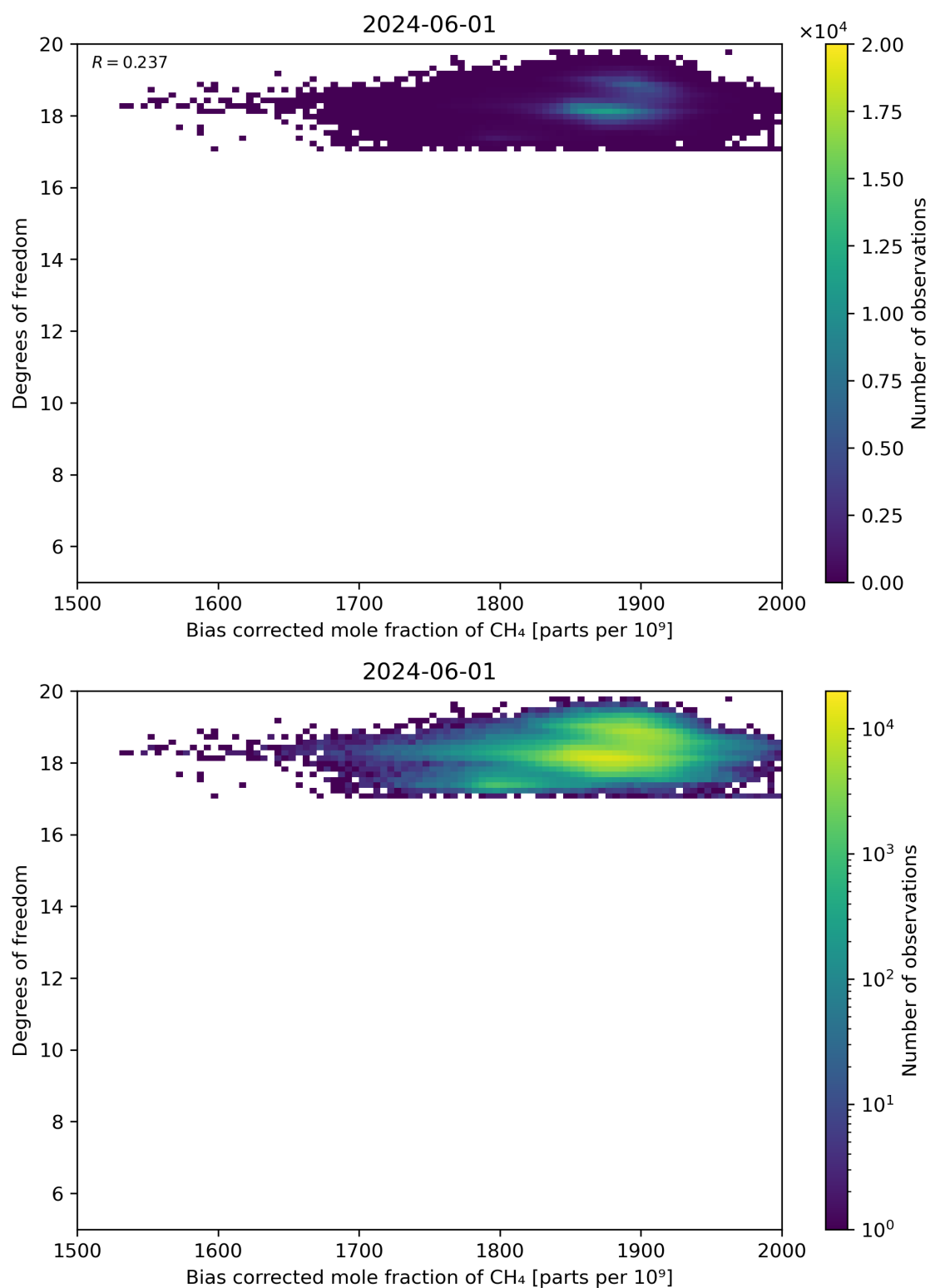
Figure 65: Scatter density plot of “Bias corrected mole fraction of CH 4 ” against “Degrees of freedom” for 2024-05-31 to 2024-06-02.
