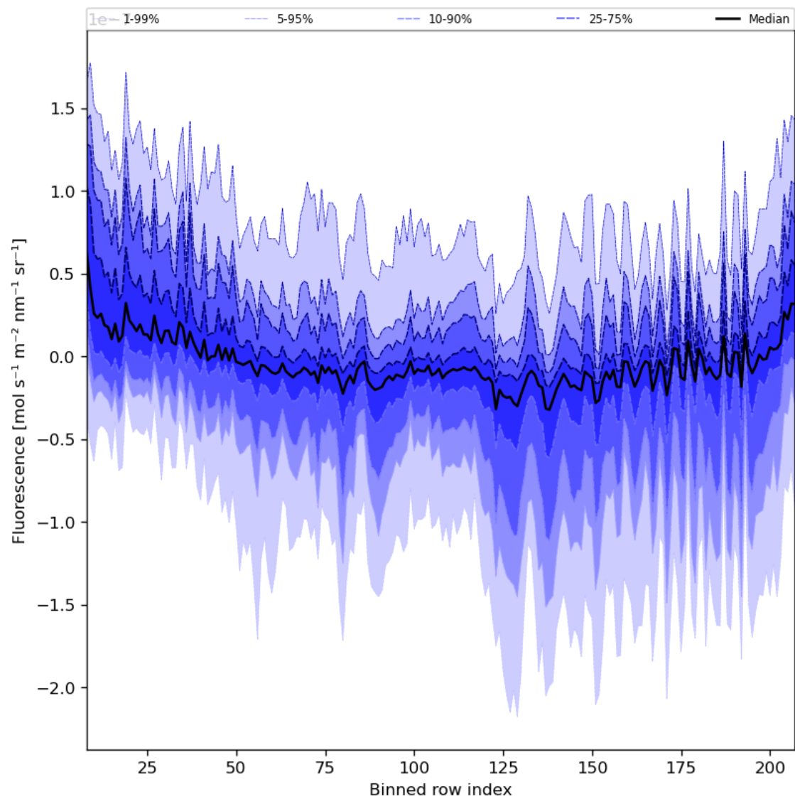
Figure 43: Along track statistics of “Fluorescence” for 2024-05-31 to 2024-06-02
