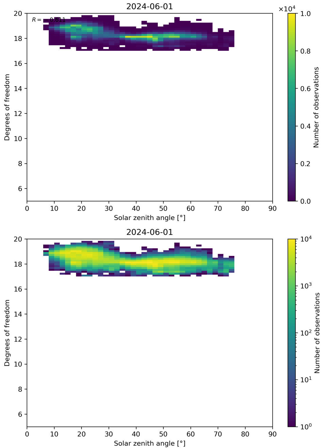
Figure 96: Scatter density plot of “Solar zenith angle” against “Degrees of freedom” for 2024-05-31 to 2024-06-02.
