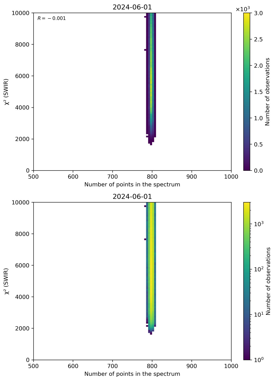
Figure 89: Scatter density plot of “Number of points in the spectrum” against “ \chi^2 (SWIR)” for 2024-05-31 to 2024-06-02.
