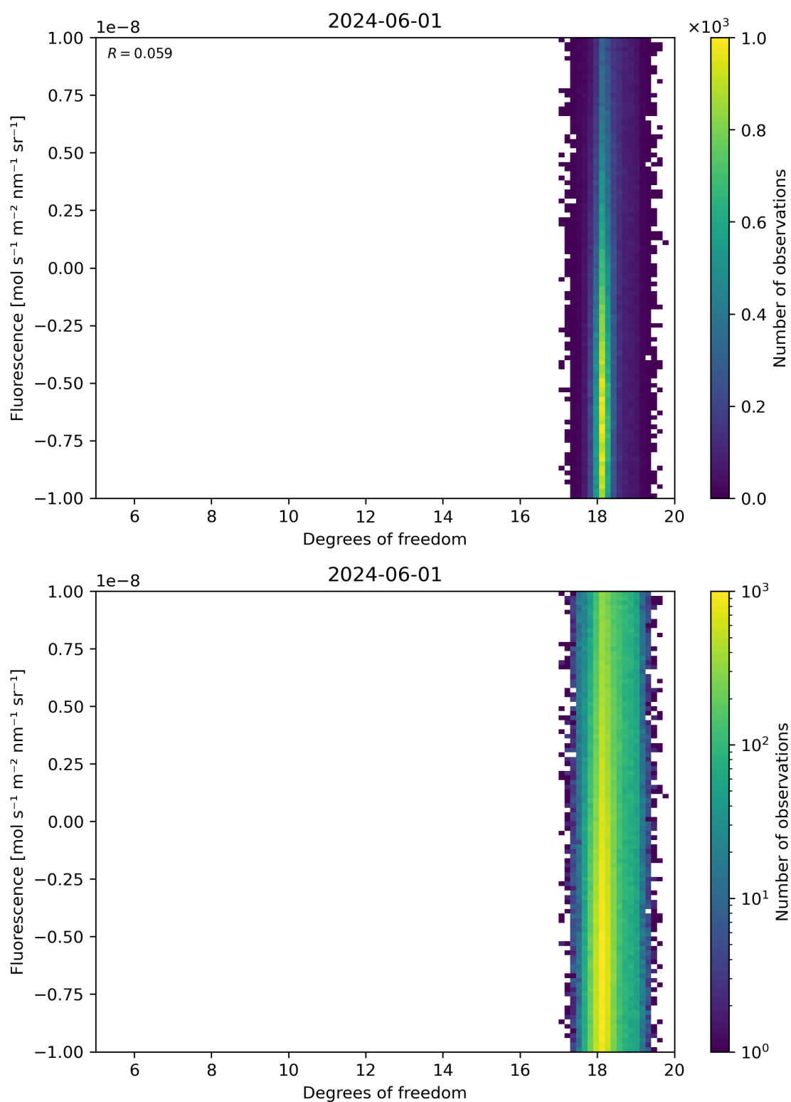
Figure 51: Scatter density plot of “Degrees of freedom” against “Fluorescence” for 2024-05-31 to 2024-06-02.
