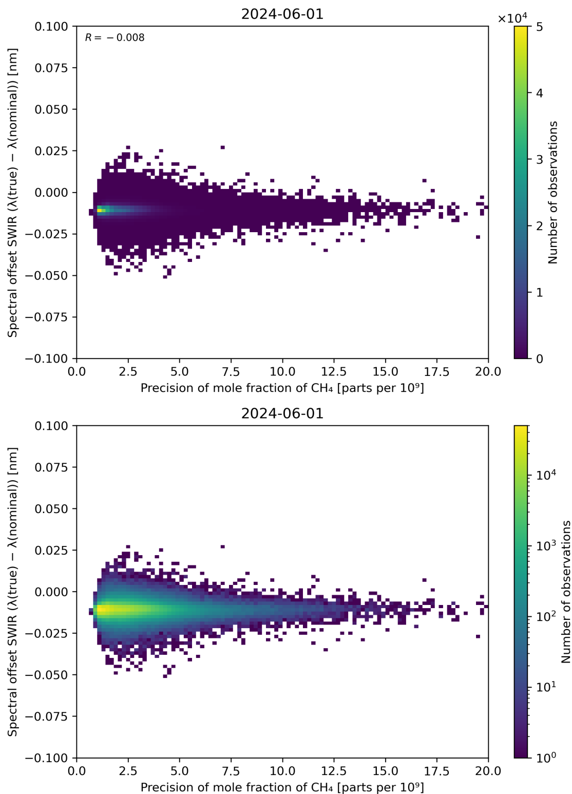
Figure 85: Scatter density plot of “Precision of mole fraction of CH 4 ” against “Spectral offset SWIR ( \lambda(\text{true}) - \lambda(\text{nominal}) )” for 2024-05-31 to 2024-06-02.
