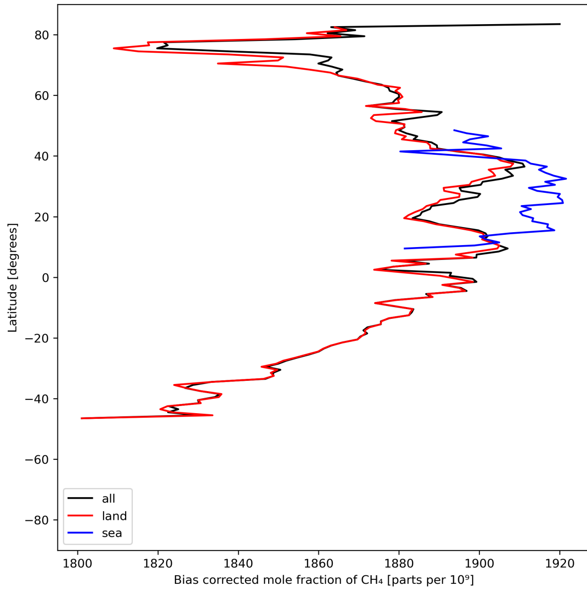
Figure 14: Zonal average of “Bias corrected mole fraction of \text{CH}_4 ” for 2024-05-31 to 2024-06-02.
