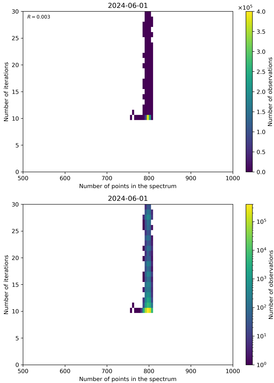
Figure 92: Scatter density plot of “Number of points in the spectrum” against “Number of iterations” for 2024-05-31 to 2024-06-02.
