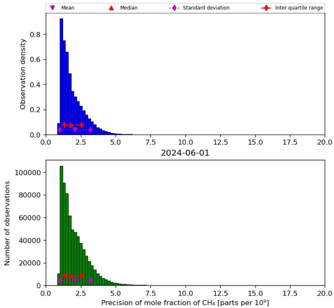
Figure 24: Histogram of “Precision of mole fraction of CH 4 ” for 2024-05-31 to 2024-06-02
