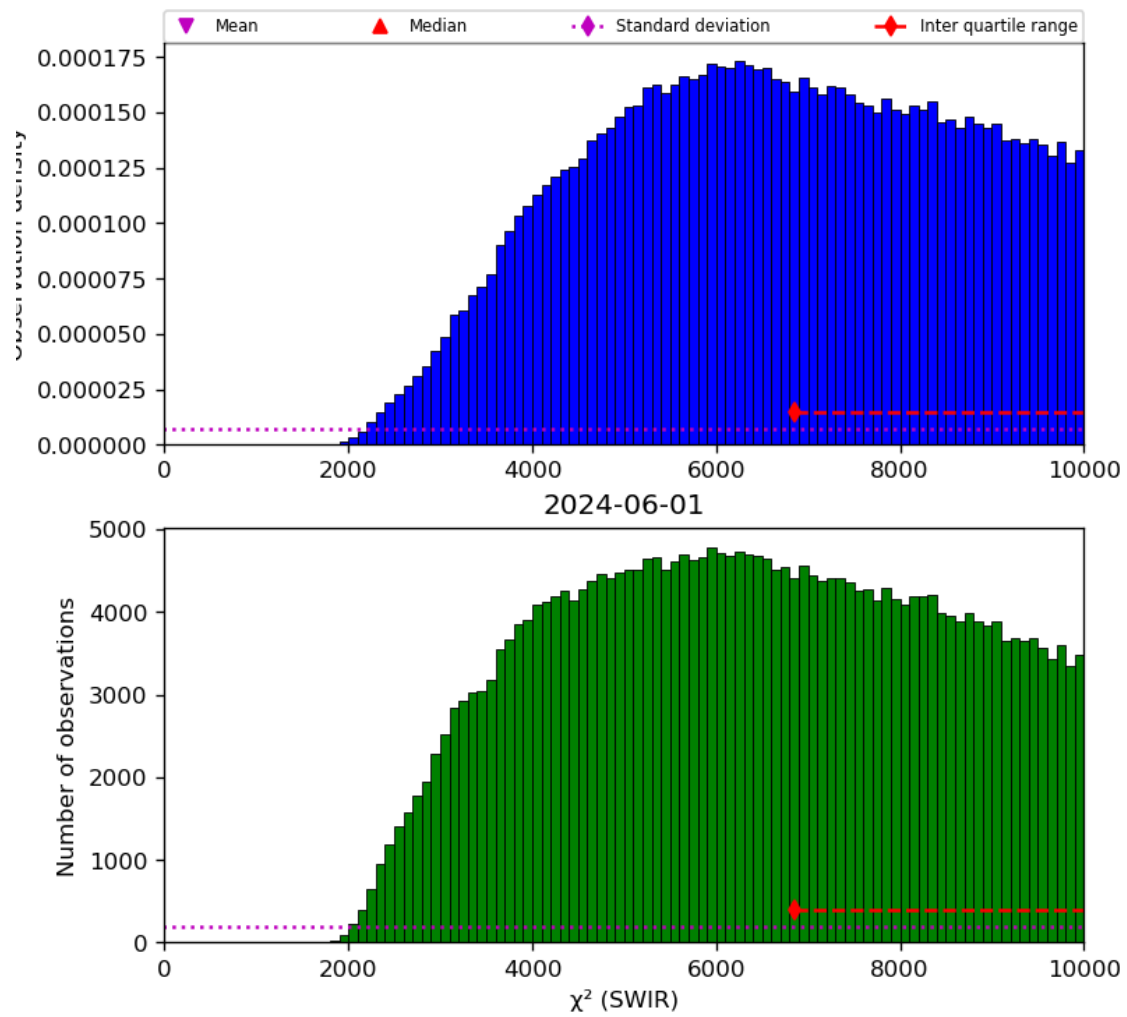
Figure 28: Histogram of “ \chi^2 (SWIR)” for 2024-05-31 to 2024-06-02
