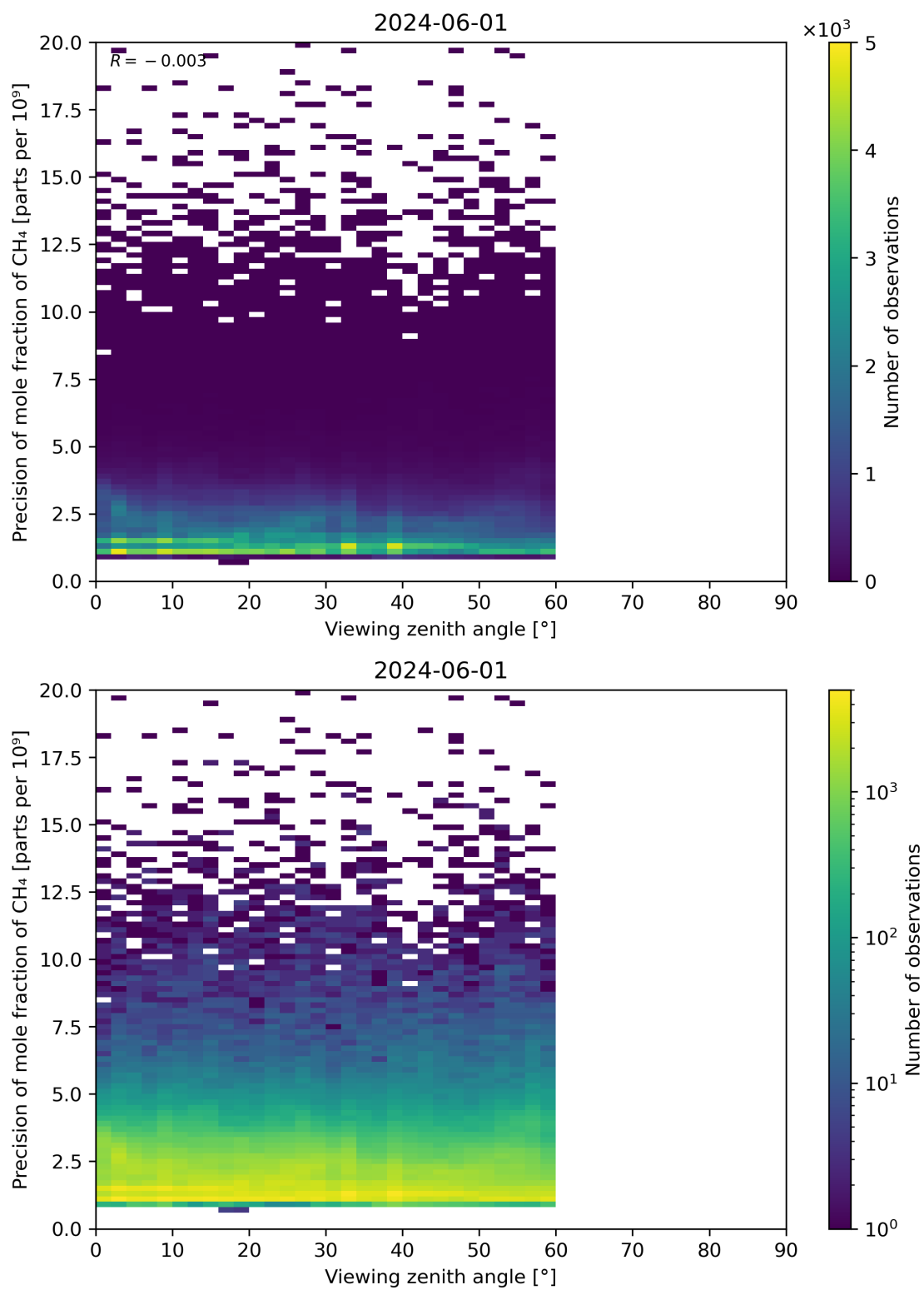
Figure 112: Scatter density plot of “Viewing zenith angle” against “Precision of mole fraction of CH 4 ” for 2024-05-31 to 2024-06-02.
