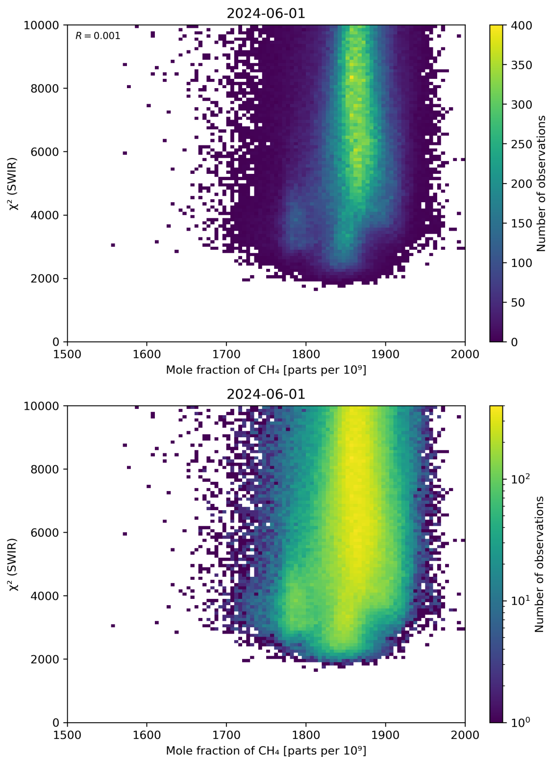
Figure 71: Scatter density plot of “Mole fraction of \text{CH}_4 ” against “ \chi^2 (SWIR)” for 2024-05-31 to 2024-06-02.
