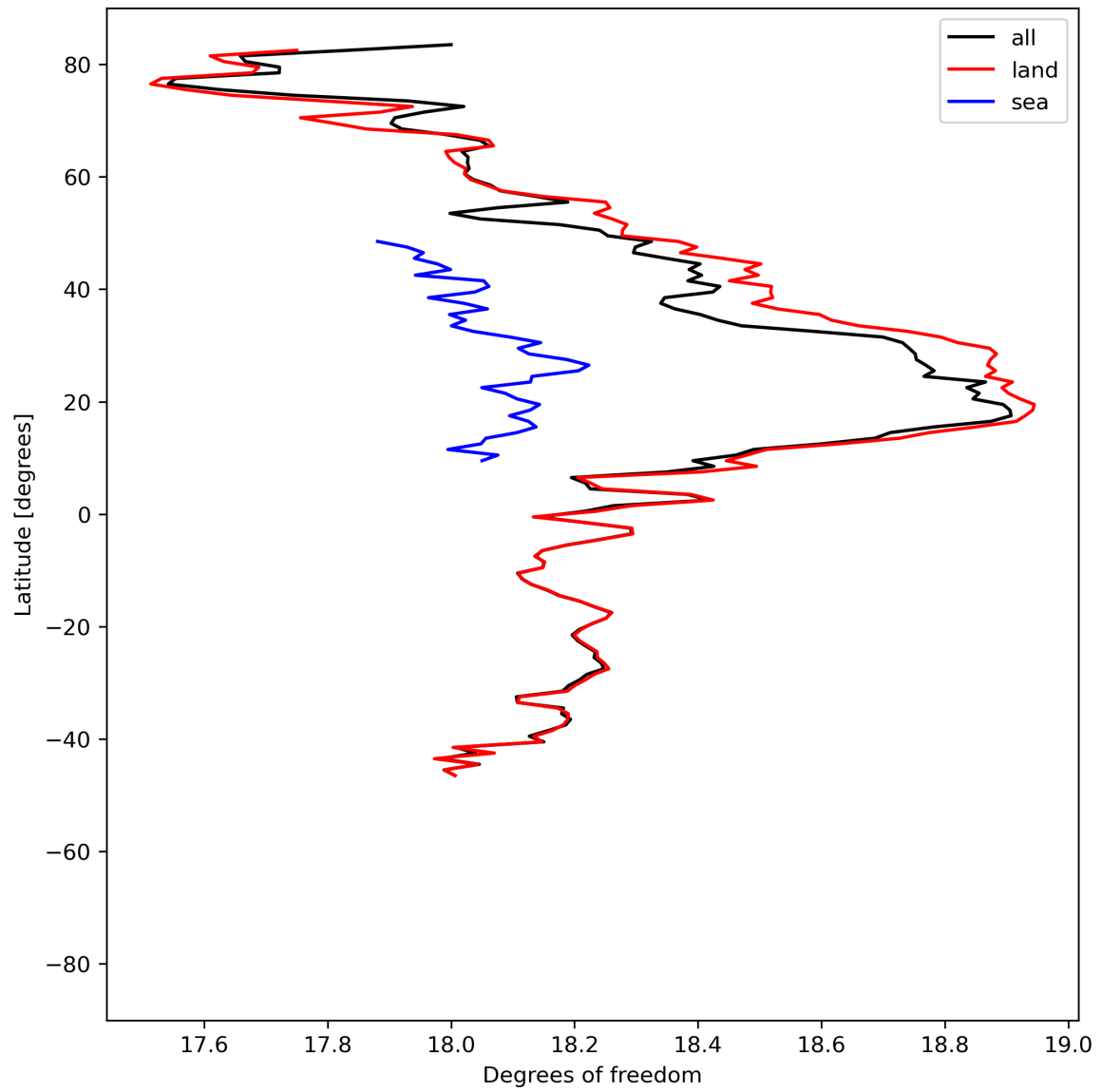
Figure 19: Zonal average of “Degrees of freedom” for 2024-05-31 to 2024-06-02.
