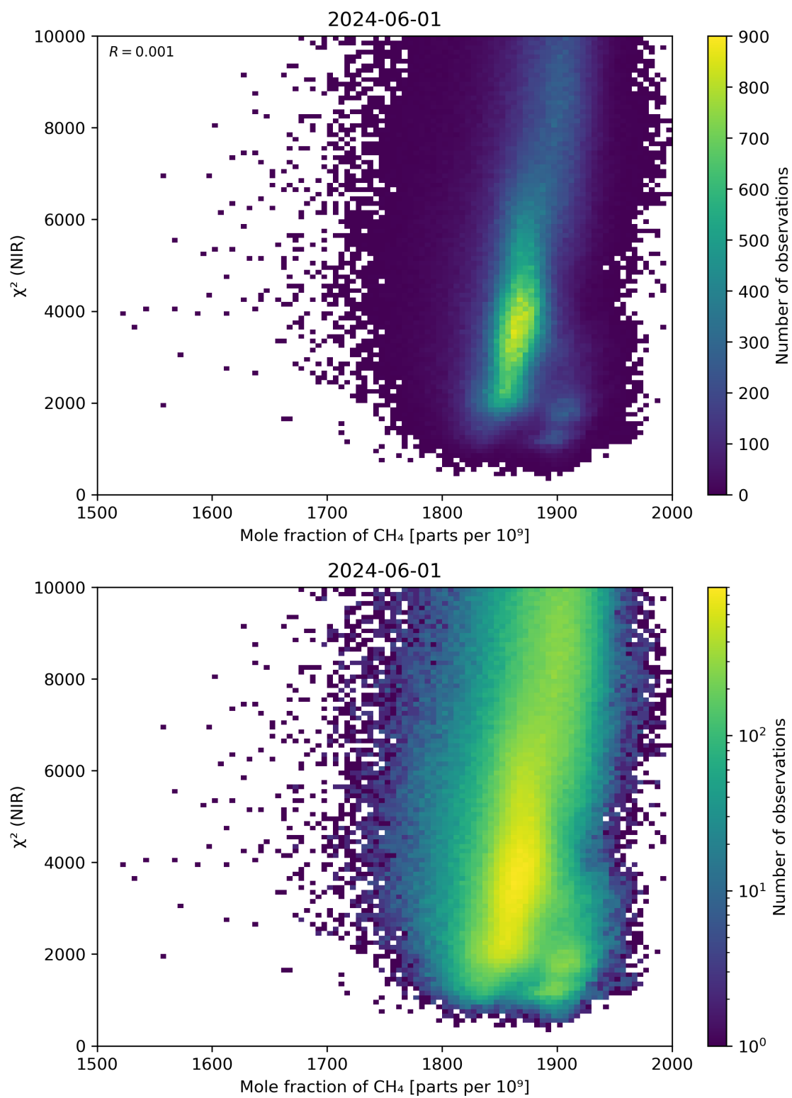
Figure 70: Scatter density plot of “Mole fraction of \text{CH}_4 ” against “ \chi^2 (NIR)” for 2024-05-31 to 2024-06-02.
