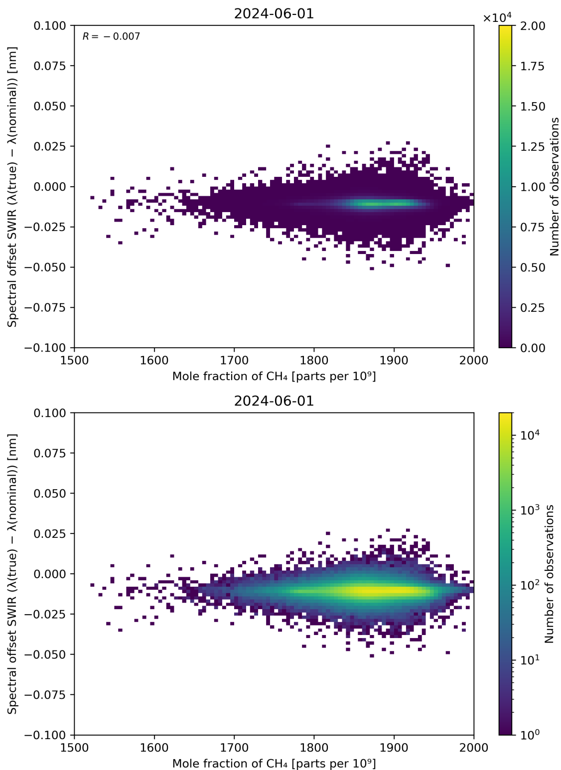
Figure 86: Scatter density plot of “Mole fraction of CH 4 ” against “Spectral offset SWIR ( \lambda(\text{true}) - \lambda(\text{nominal}) )” for 2024-05-31 to 2024-06-02.
