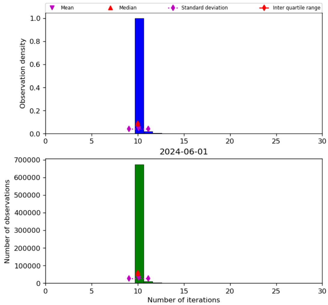
Figure 31: Histogram of “Number of iterations” for 2024-05-31 to 2024-06-02
