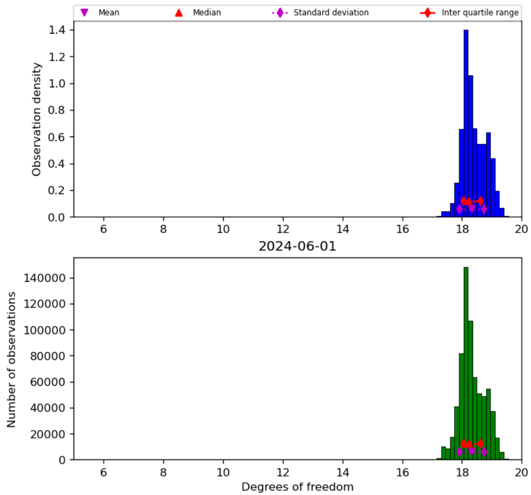
Figure 30: Histogram of “Degrees of freedom” for 2024-05-31 to 2024-06-02
