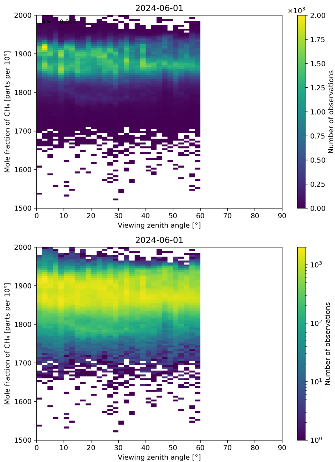
Figure 110: Scatter density plot of “Viewing zenith angle” against “Mole fraction of CH 4 ” for 2024-05-31 to 2024-06-02.
