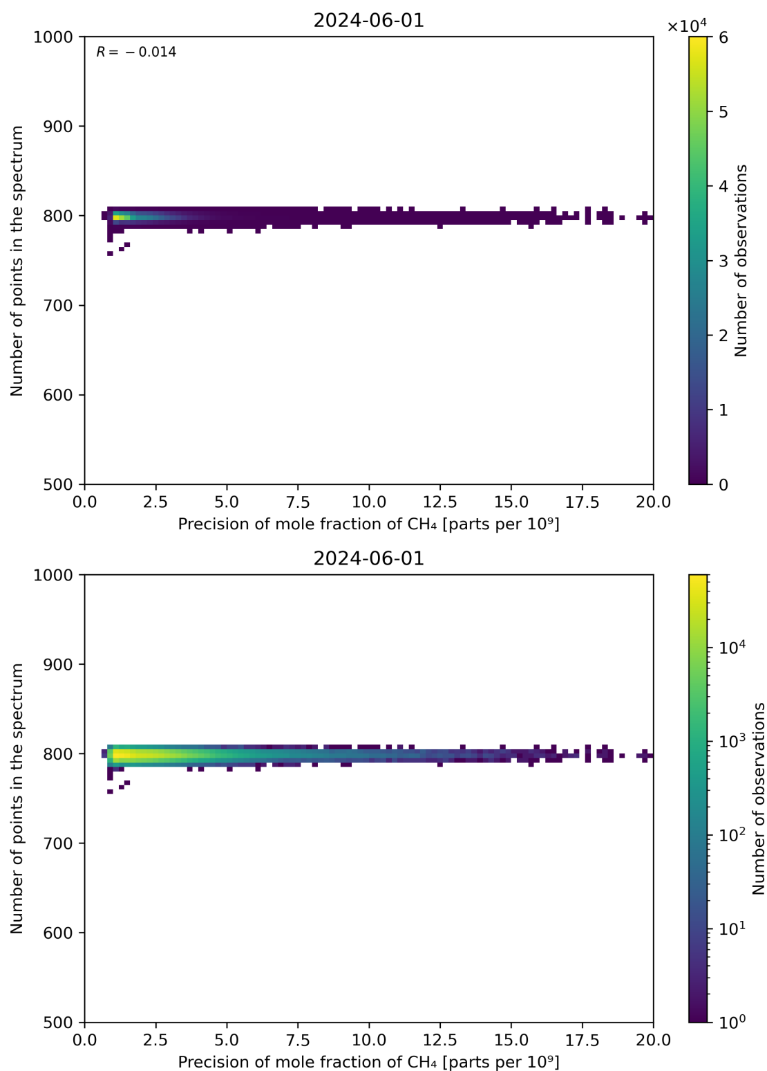
Figure 84: Scatter density plot of “Precision of mole fraction of CH 4 ” against “Number of points in the spectrum” for 2024-05-31 to 2024-06-02.
