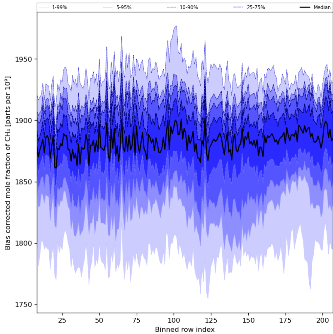
Figure 36: Along track statistics of “Bias corrected mole fraction of CH 4 ” for 2024-05-31 to 2024-06-02
