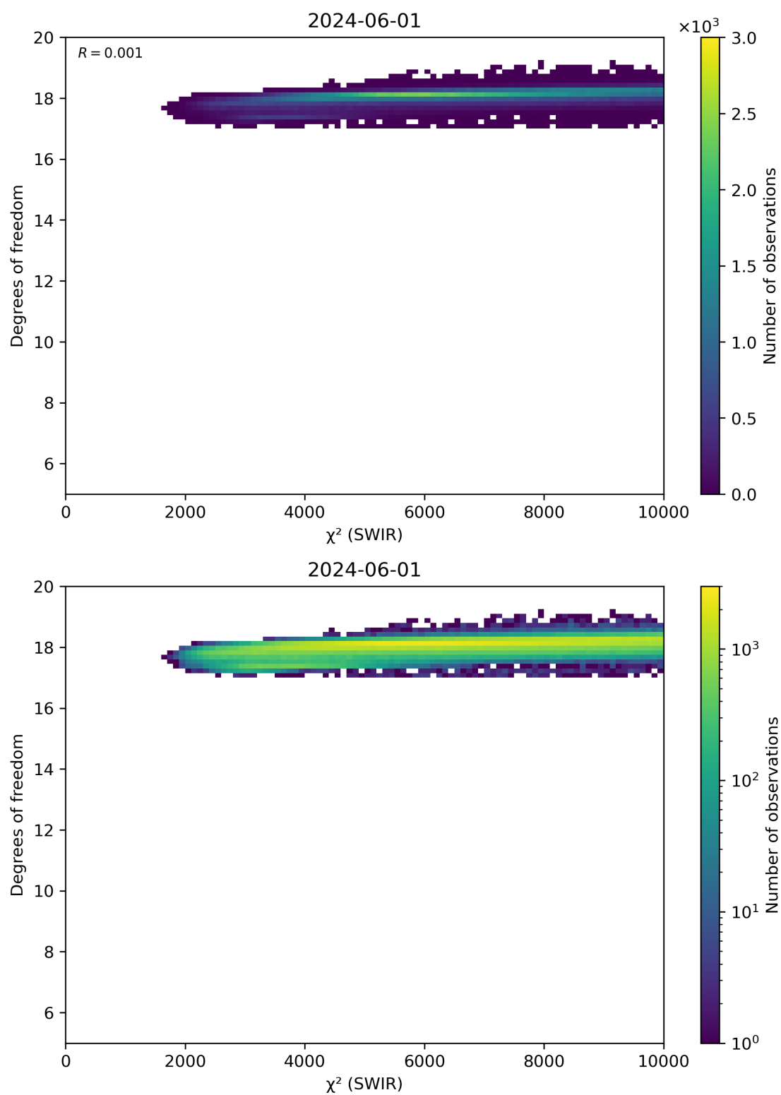
Figure 48: Scatter density plot of “ \chi^2 (SWIR)” against “Degrees of freedom” for 2024-05-31 to 2024-06-02.
