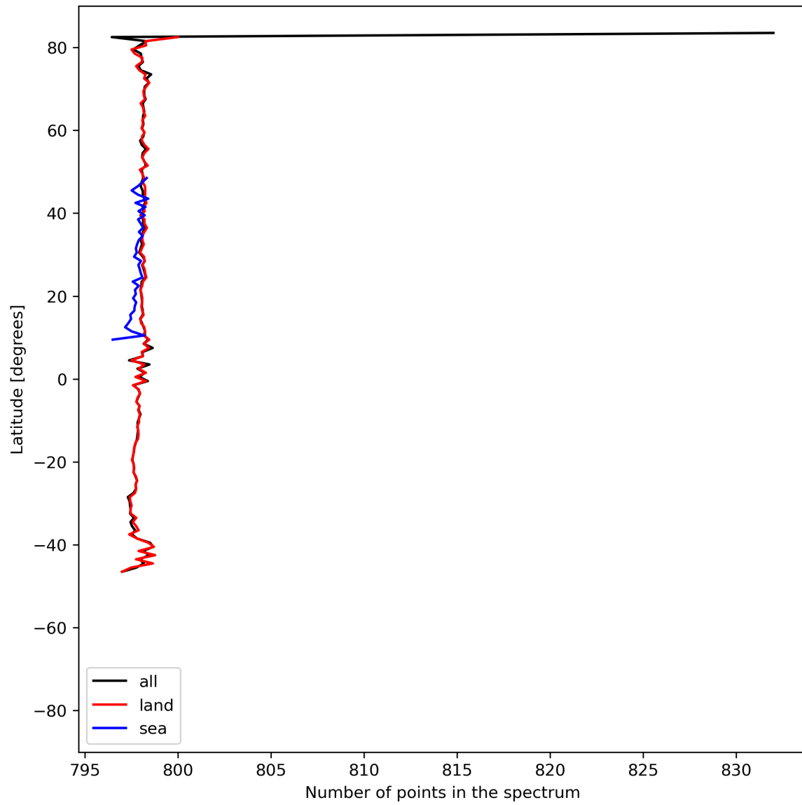
Figure 15: Zonal average of “Number of points in the spectrum” for 2024-05-31 to 2024-06-02.
