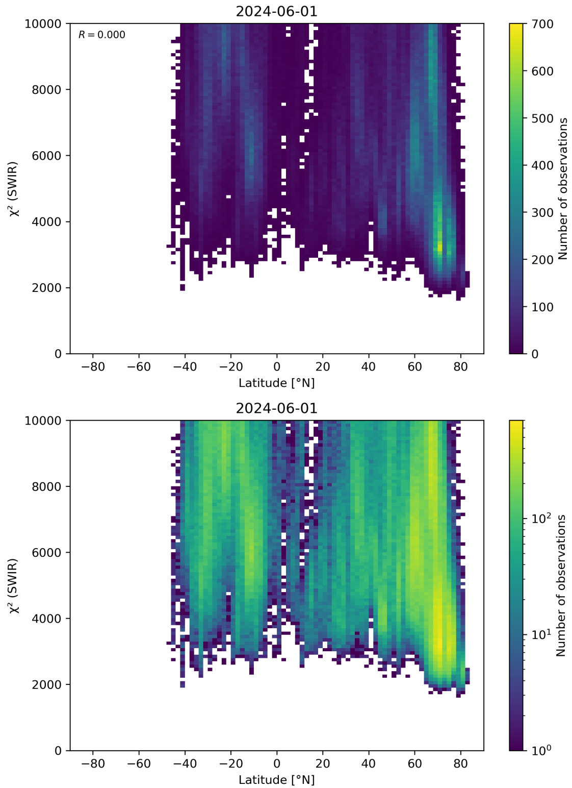
Figure 54: Scatter density plot of “Latitude” against “ \chi^2 (SWIR)” for 2024-05-31 to 2024-06-02.
