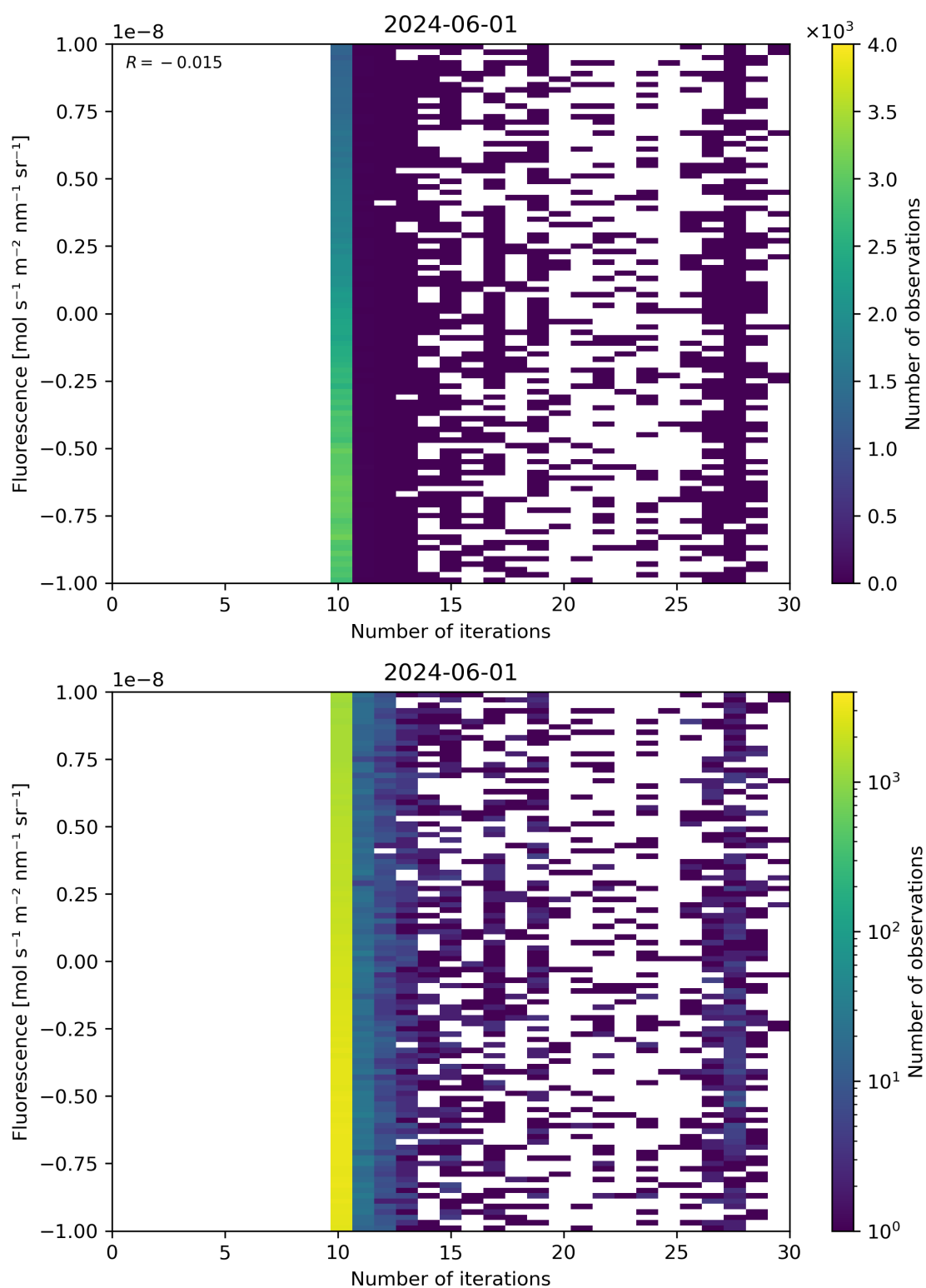
Figure 87: Scatter density plot of “Number of iterations” against “Fluorescence” for 2024-05-31 to 2024-06-02.
