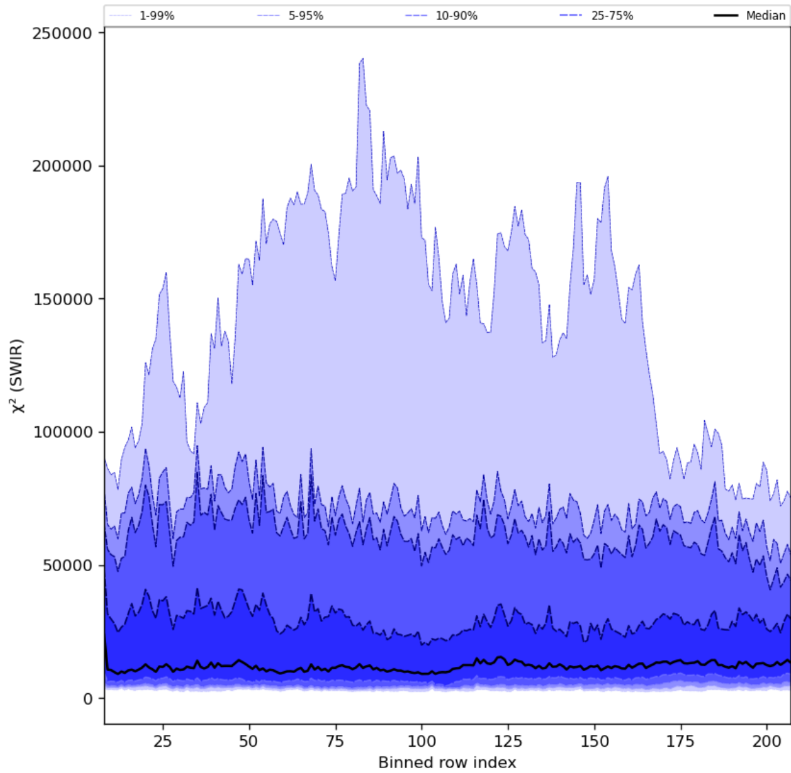
Figure 39: Along track statistics of " \chi^2 (SWIR)" for 2024-05-31 to 2024-06-02
