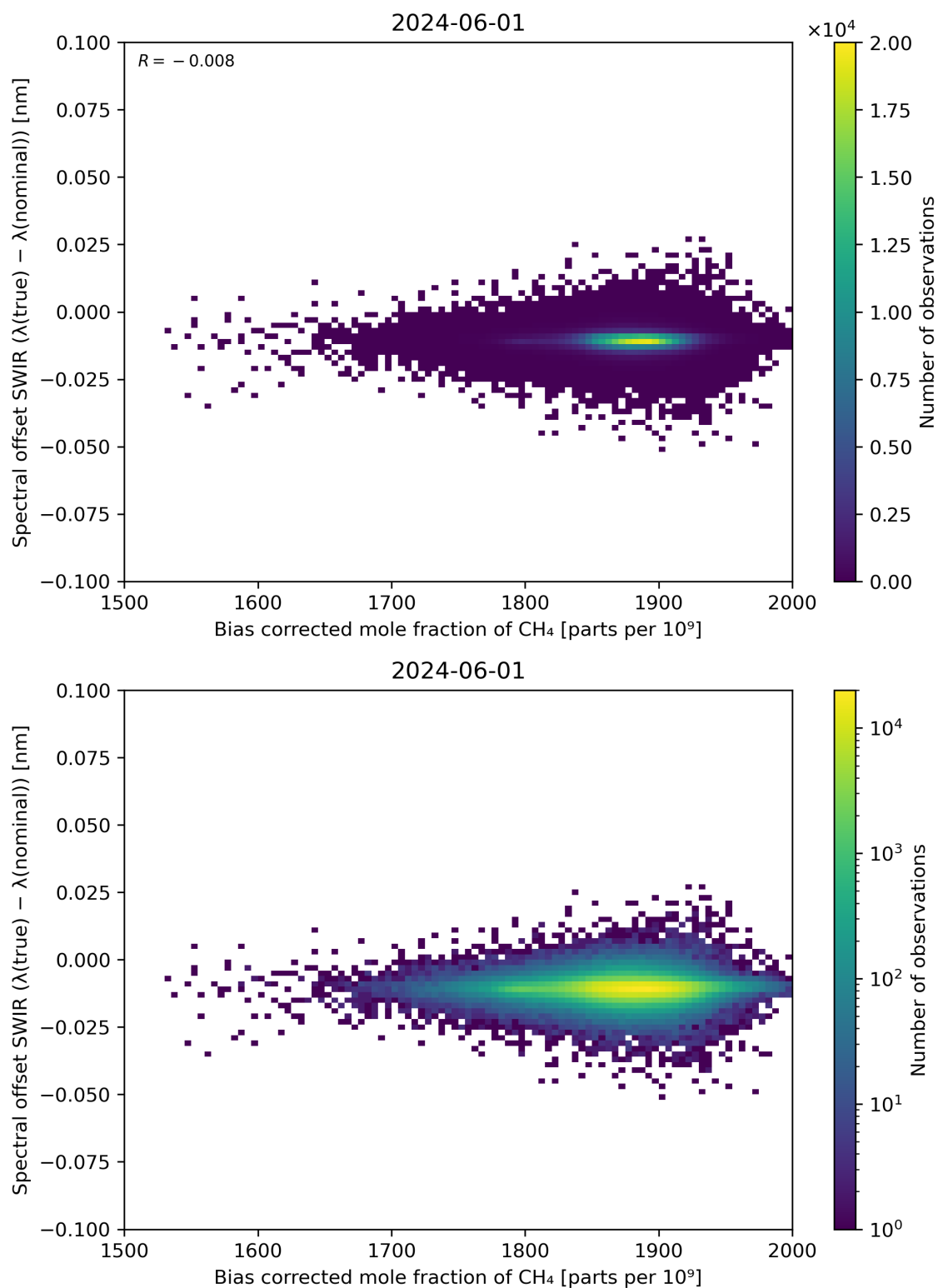
Figure 69: Scatter density plot of “Bias corrected mole fraction of CH 4 ” against “Spectral offset SWIR ( \lambda(\text{true}) - \lambda(\text{nominal}) )” for 2024-05-31 to 2024-06-02.
