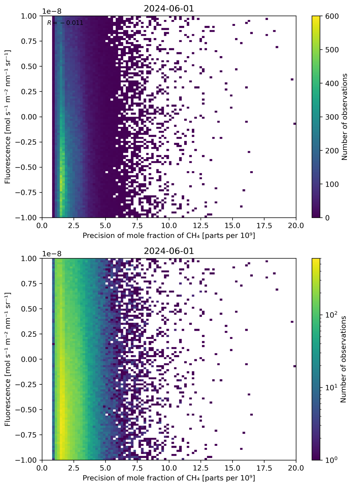
Figure 81: Scatter density plot of “Precision of mole fraction of \text{CH}_4 ” against “Fluorescence” for 2024-05-31 to 2024-06-02.
