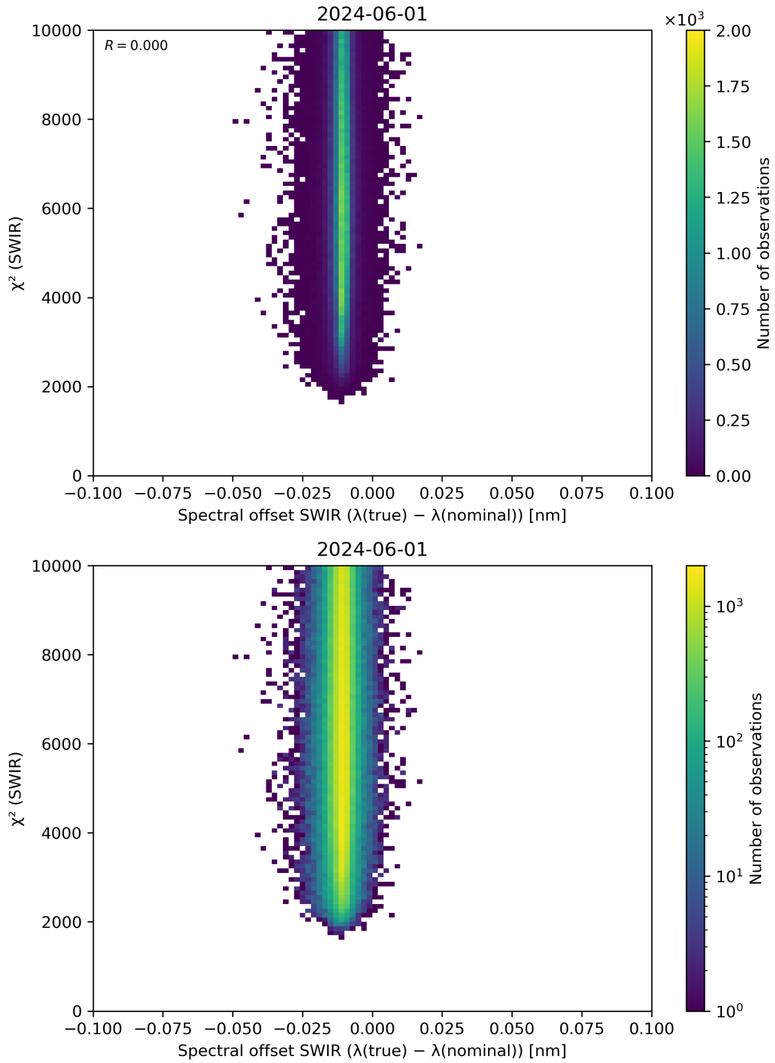
Figure 118: Scatter density plot of “Spectral offset SWIR ( \lambda(\text{true}) - \lambda(\text{nominal}) )” against “ \chi^2 (SWIR)” for 2024-05-31 to 2024-06-02.
