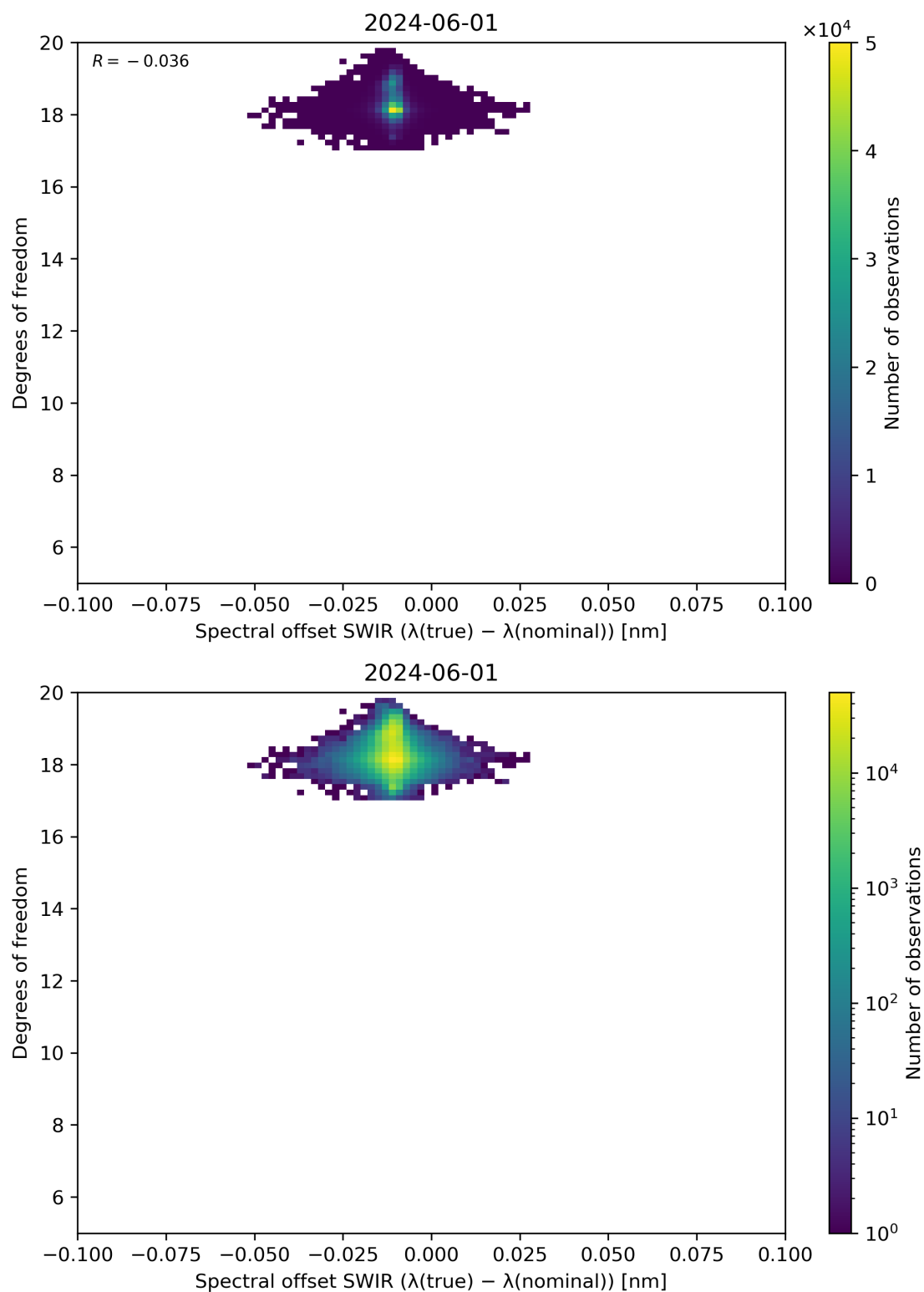
Figure 119: Scatter density plot of “Spectral offset SWIR ( \lambda(\text{true}) - \lambda(\text{nominal}) )” against “Degrees of freedom” for 2024-05-31 to 2024-06-02.
