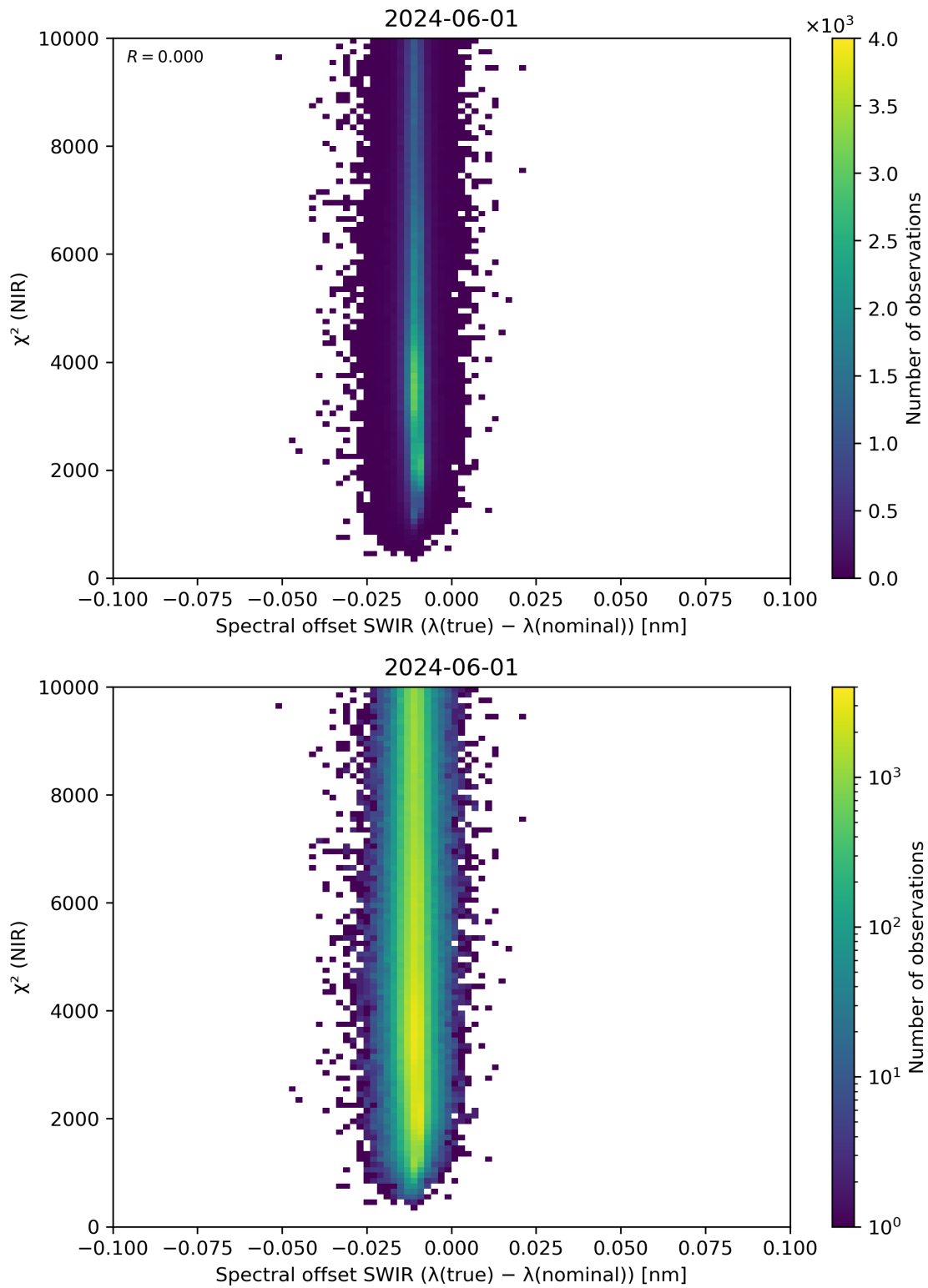
Figure 117: Scatter density plot of “Spectral offset SWIR ( \lambda(\text{true}) - \lambda(\text{nominal}) )” against “ \chi^2 (NIR)” for 2024-05-31 to 2024-06-02.
