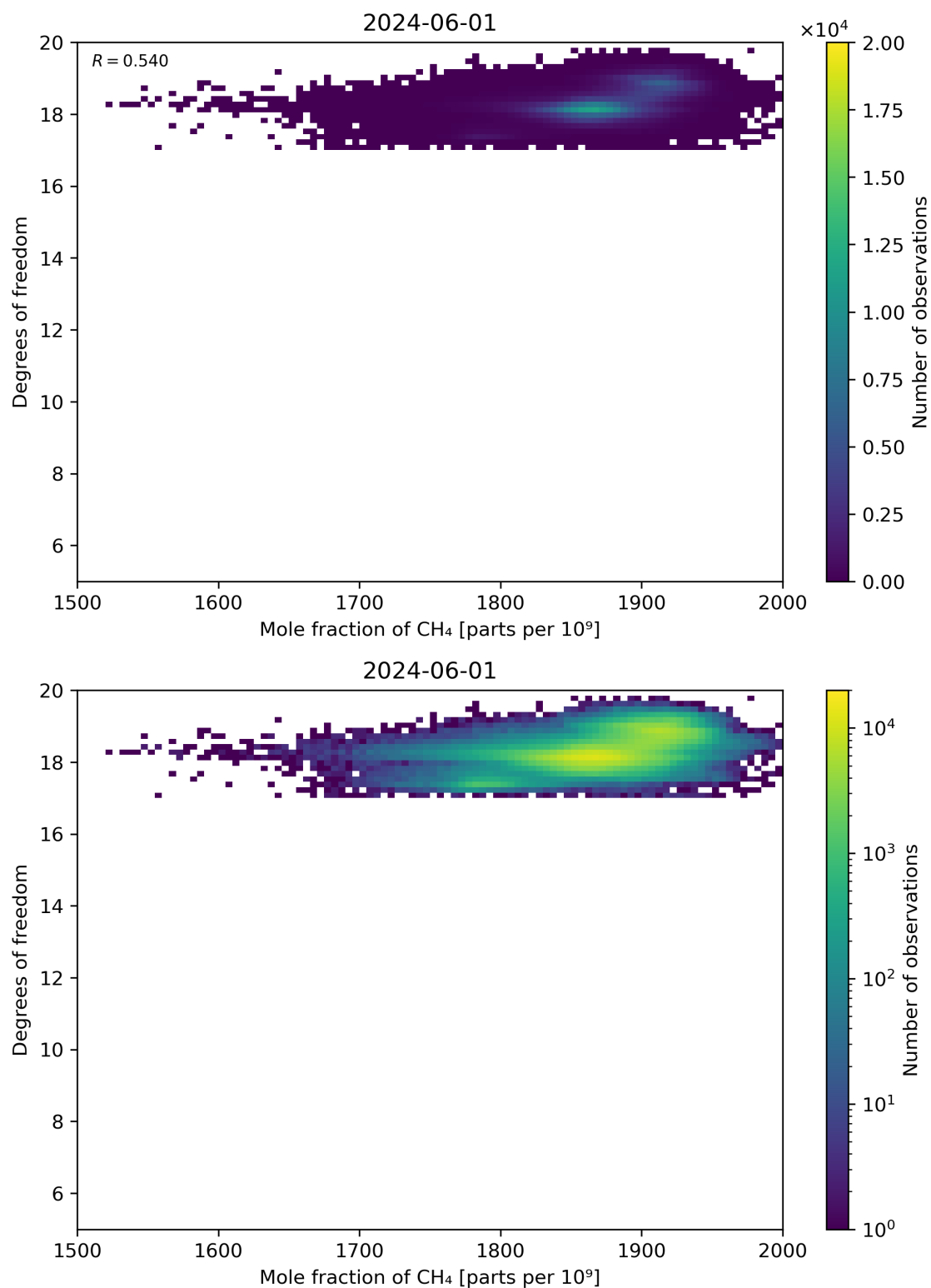
Figure 72: Scatter density plot of “Mole fraction of CH 4 ” against “Degrees of freedom” for 2024-05-31 to 2024-06-02.
