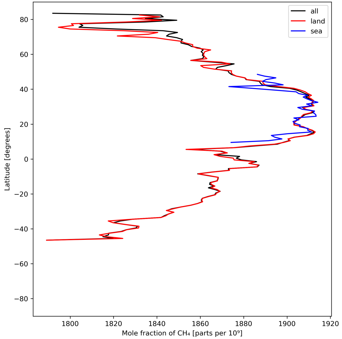
Figure 12: Zonal average of “Mole fraction of \text{CH}_4 ” for 2024-05-31 to 2024-06-02.
