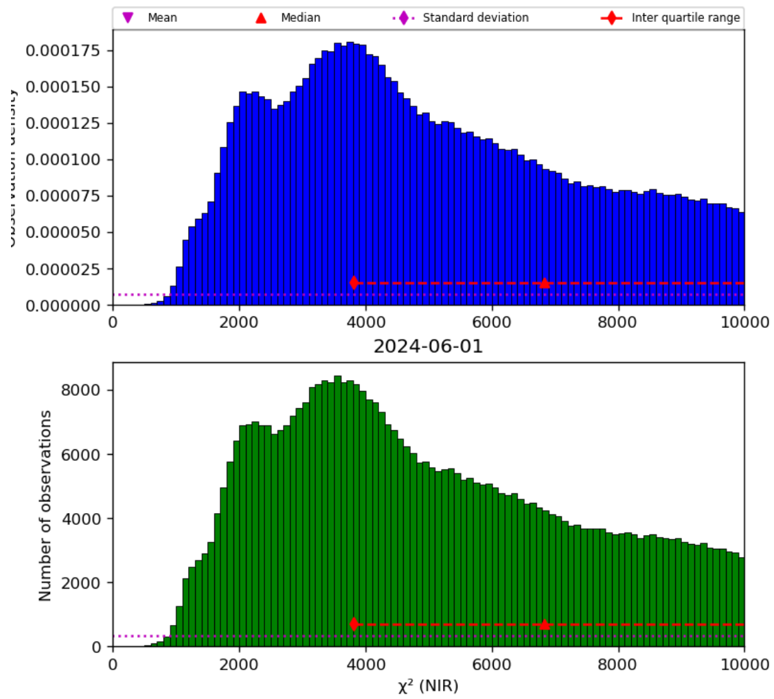
Figure 29: Histogram of “ \chi^2 (NIR)” for 2024-05-31 to 2024-06-02
