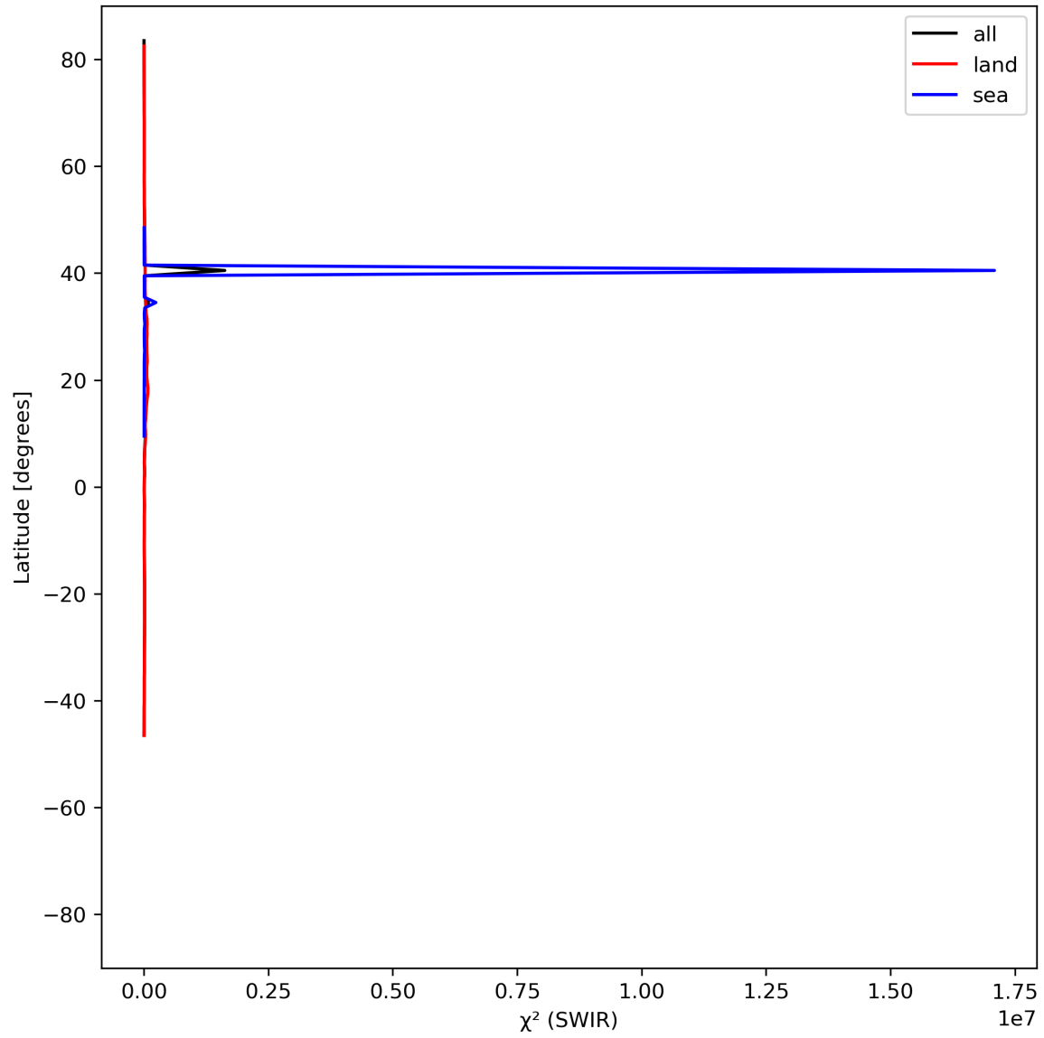
Figure 17: Zonal average of “ \chi^2 (SWIR)” for 2024-05-31 to 2024-06-02.
