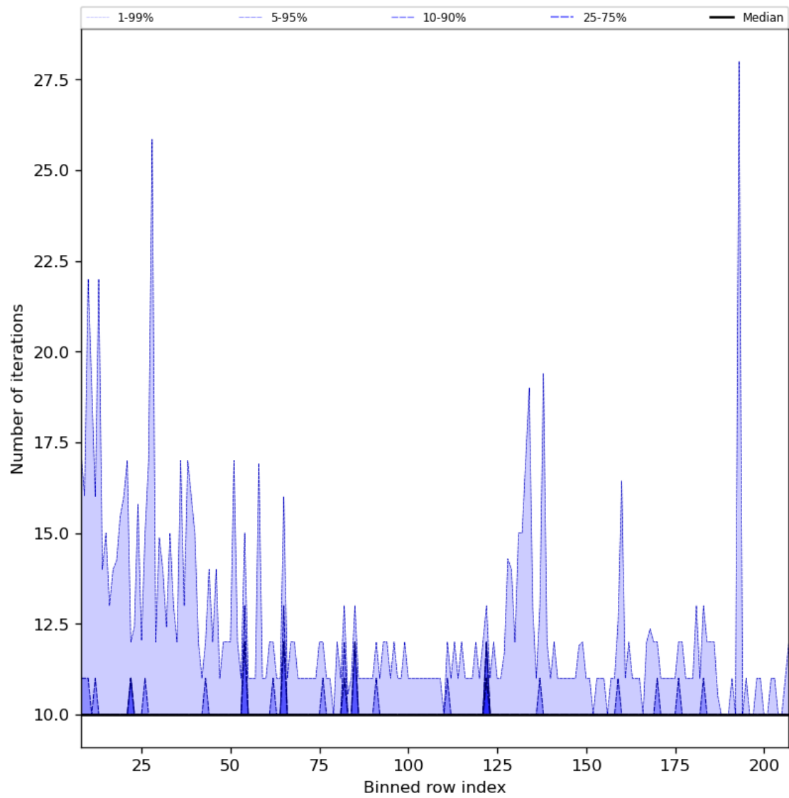
Figure 42: Along track statistics of “Number of iterations” for 2024-05-31 to 2024-06-02
