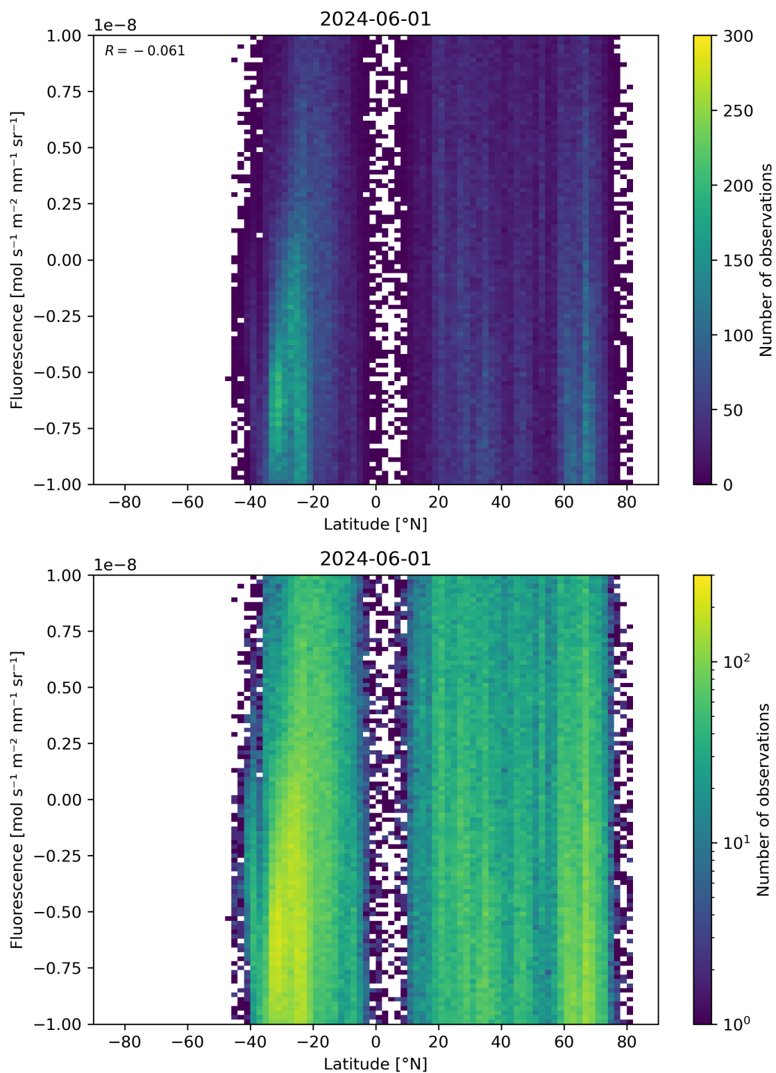
Figure 56: Scatter density plot of “Latitude” against “Fluorescence” for 2024-05-31 to 2024-06-02.
