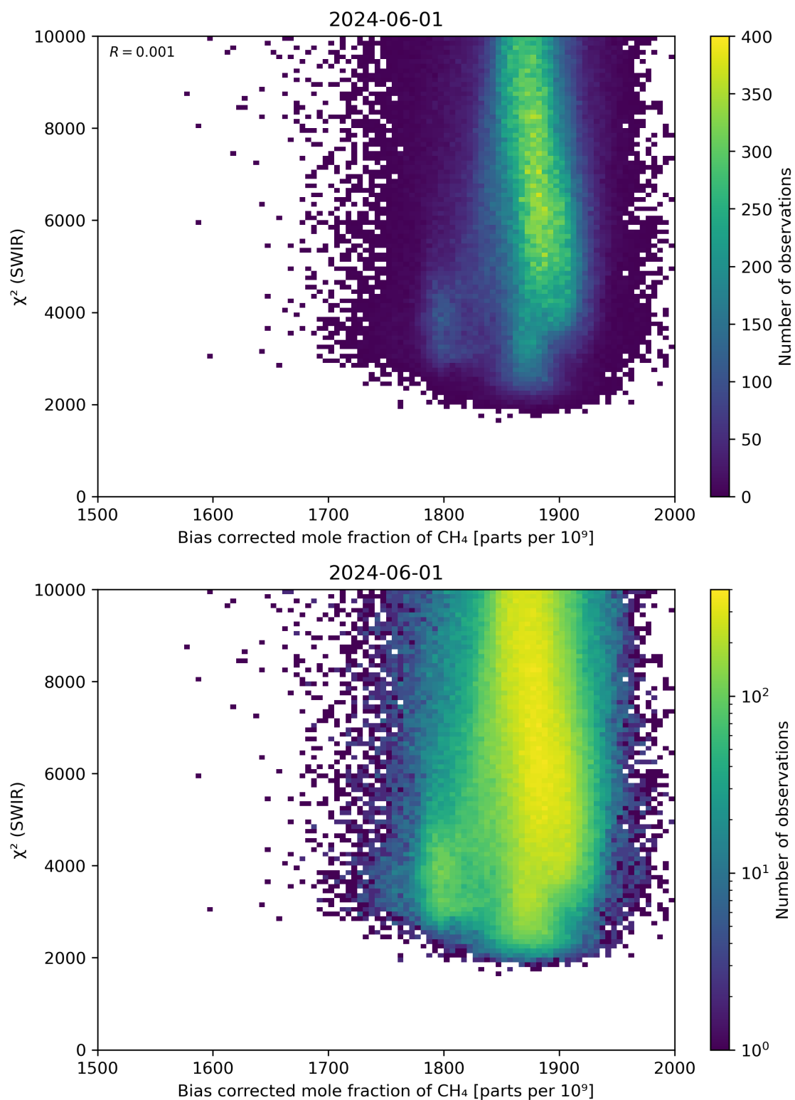
Figure 64: Scatter density plot of “Bias corrected mole fraction of CH 4 ” against “ \chi^2 (SWIR)” for 2024-05-31 to 2024-06-02.
