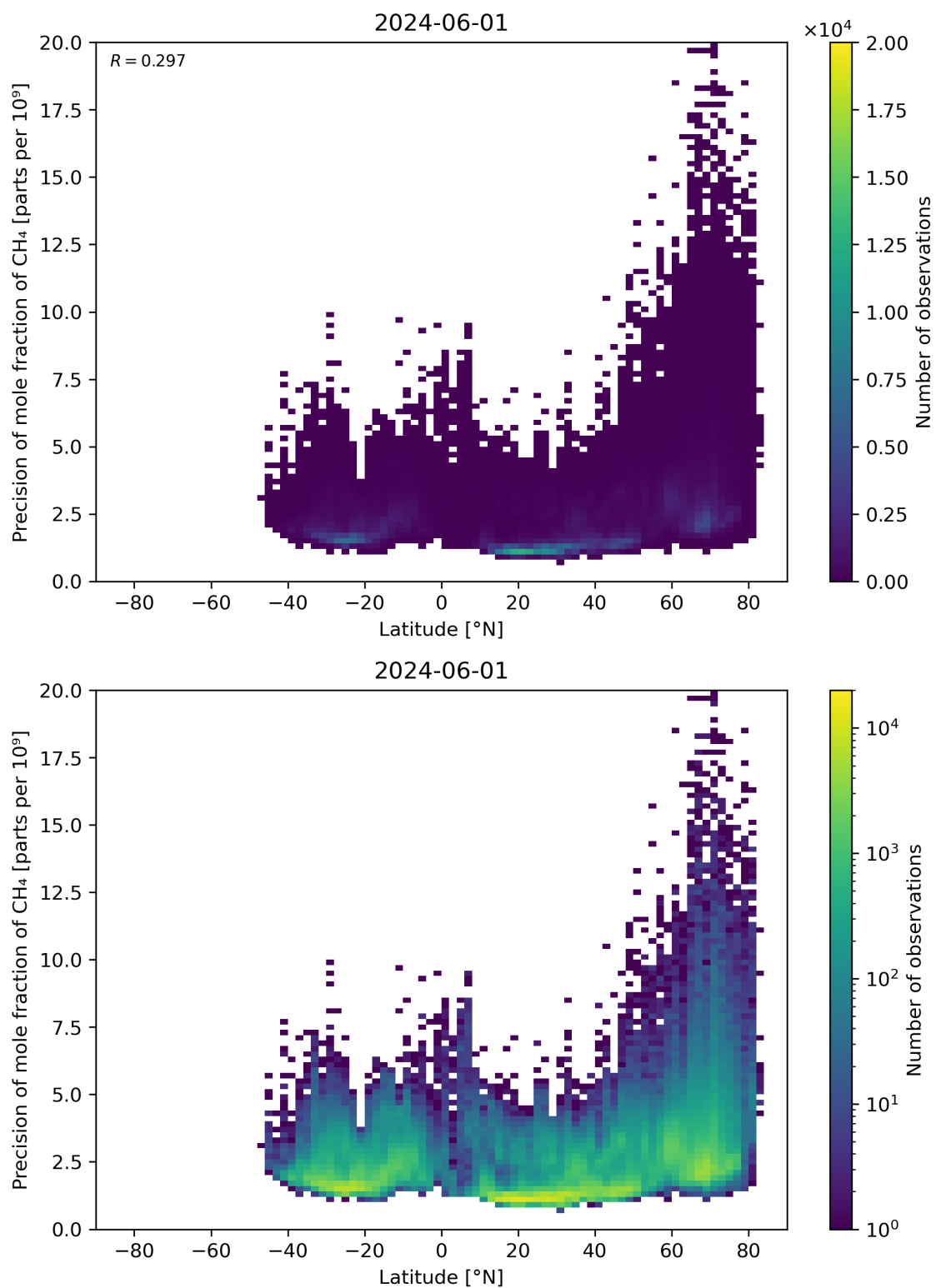
Figure 59: Scatter density plot of “Latitude” against “Precision of mole fraction of \text{CH}_4 ” for 2024-05-31 to 2024-06-02.
