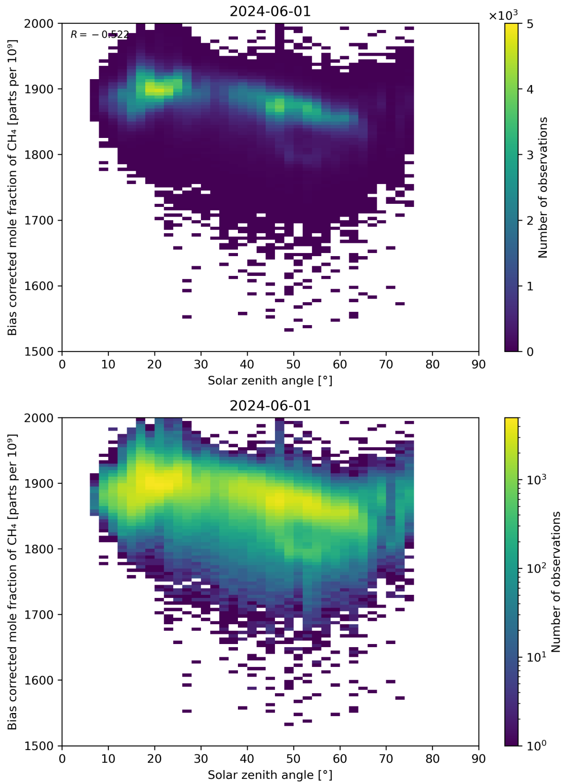
Figure 100: Scatter density plot of “Solar zenith angle” against “Bias corrected mole fraction of \text{CH}_4 ” for 2024-05-31 to 2024-06-02.
