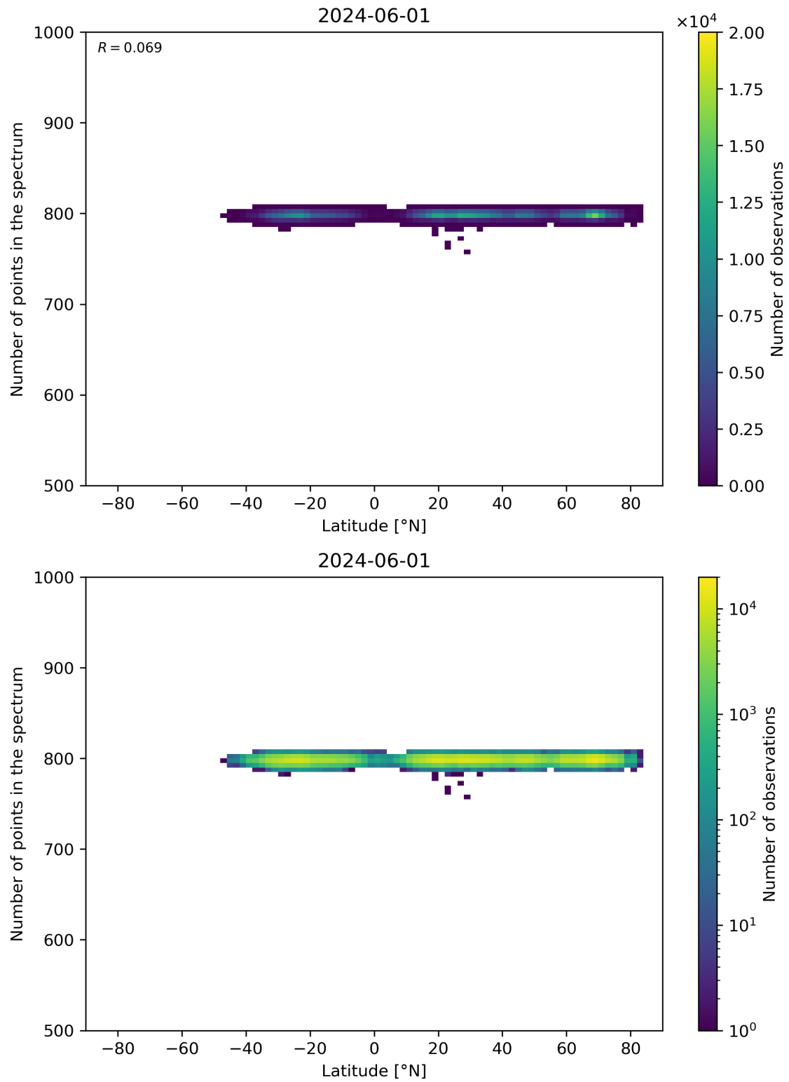
Figure 61: Scatter density plot of “Latitude” against “Number of points in the spectrum” for 2024-05-31 to 2024-06-02.
