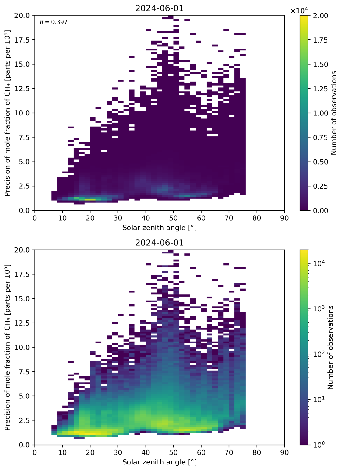
Figure 101: Scatter density plot of “Solar zenith angle” against “Precision of mole fraction of CH 4 ” for 2024-05-31 to 2024-06-02.
