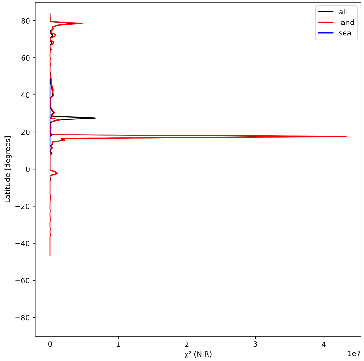
Figure 18: Zonal average of “ \chi^2 (NIR)” for 2024-05-31 to 2024-06-02.
