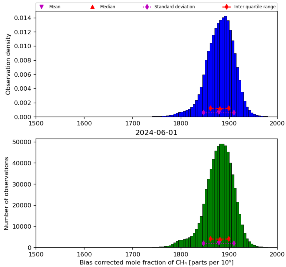
Figure 25: Histogram of “Bias corrected mole fraction of CH 4 ” for 2024-05-31 to 2024-06-02
