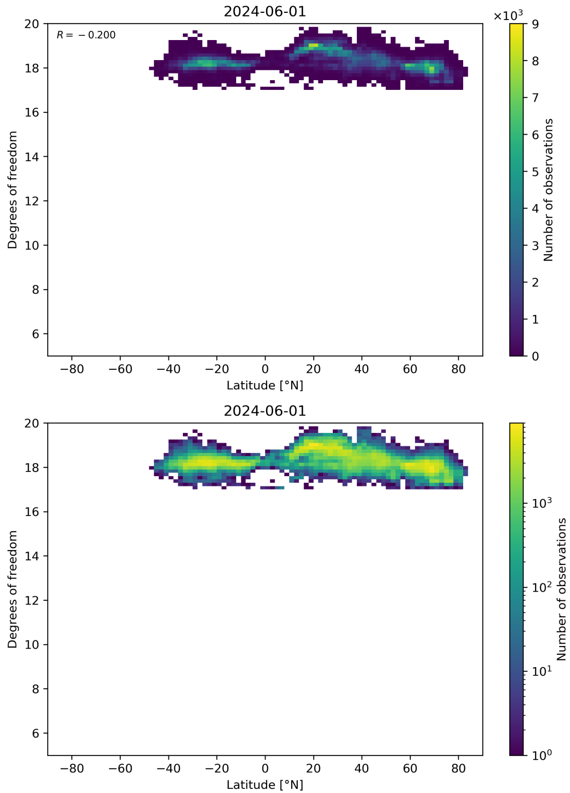
Figure 55: Scatter density plot of “Latitude” against “Degrees of freedom” for 2024-05-31 to 2024-06-02.
