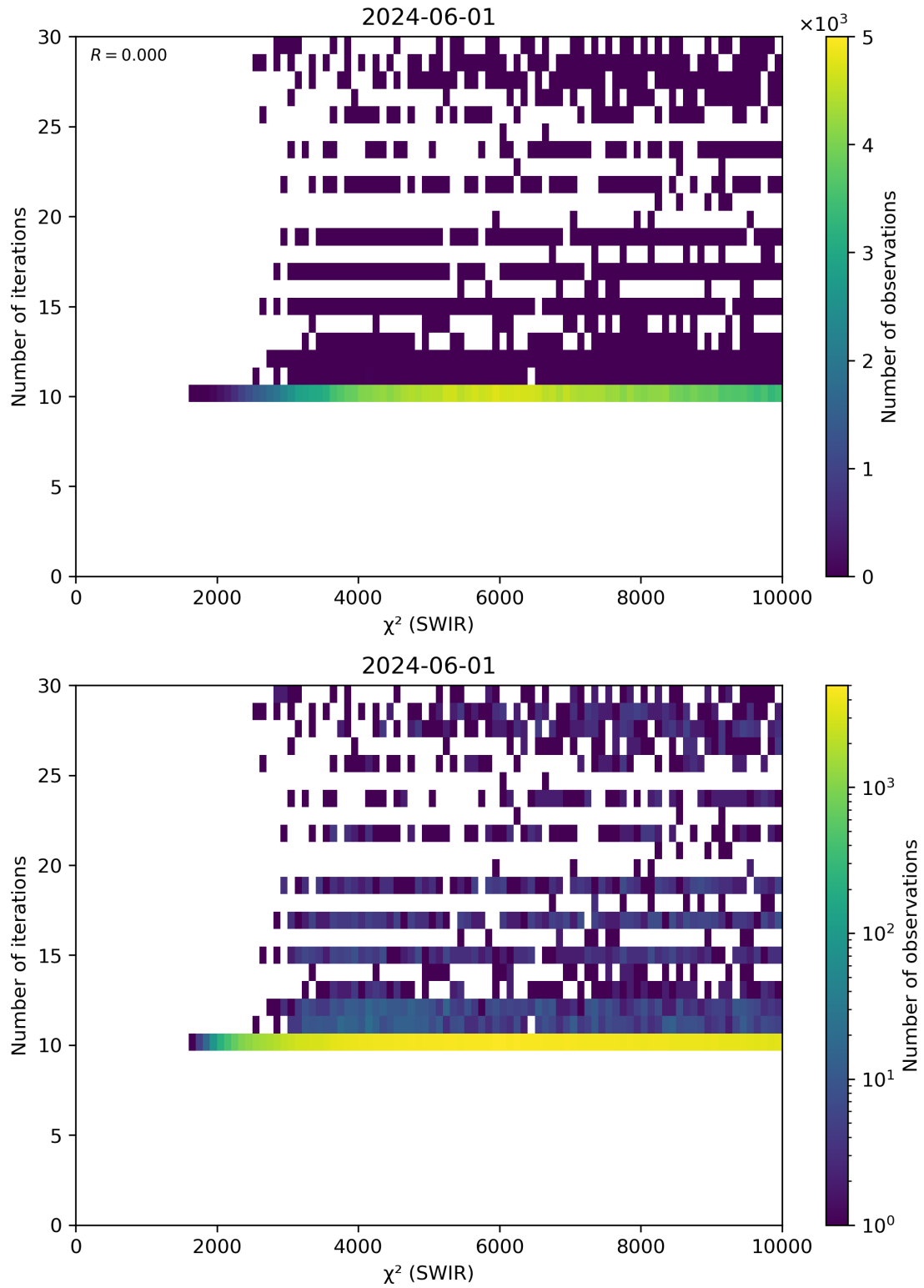
Figure 50: Scatter density plot of “ \chi^2 (SWIR)” against “Number of iterations” for 2024-05-31 to 2024-06-02.
