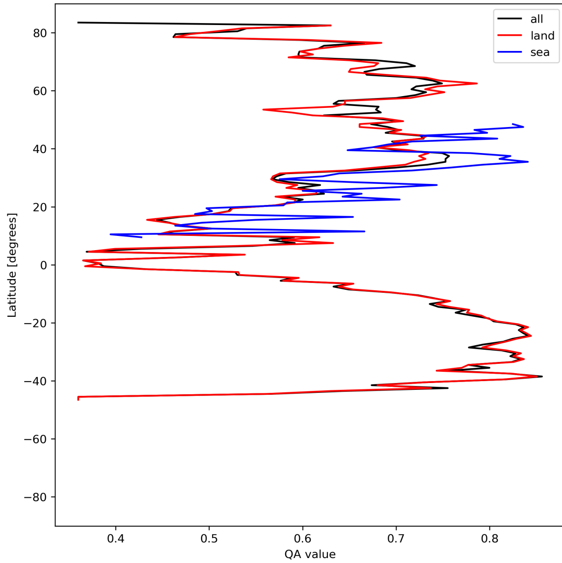
Figure 11: Zonal average of “QA value” for 2024-05-31 to 2024-06-02.
