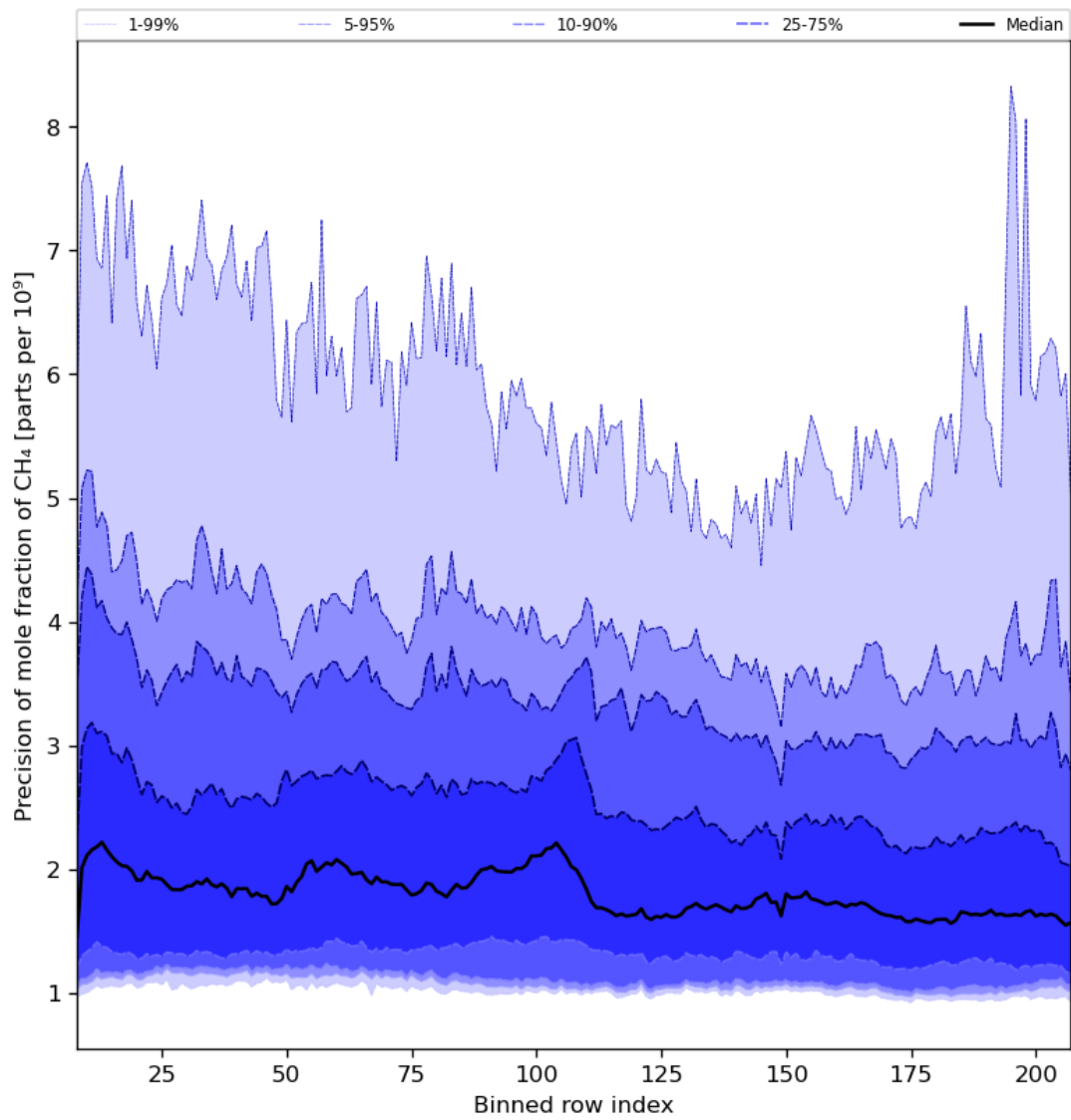
Figure 35: Along track statistics of “Precision of mole fraction of CH 4 ” for 2024-05-31 to 2024-06-02
