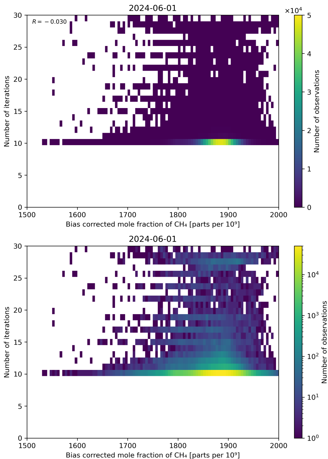
Figure 67: Scatter density plot of “Bias corrected mole fraction of CH 4 ” against “Number of iterations” for 2024-05-31 to 2024-06-02.
