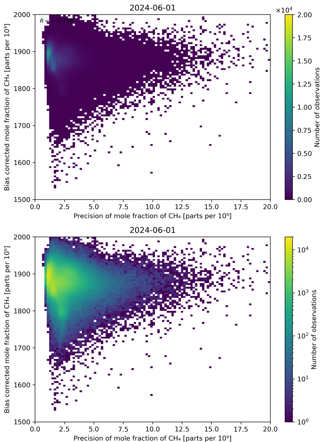
Figure 82: Scatter density plot of “Precision of mole fraction of CH 4 ” against “Bias corrected mole fraction of CH 4 ” for 2024-05-31 to 2024-06-02.
