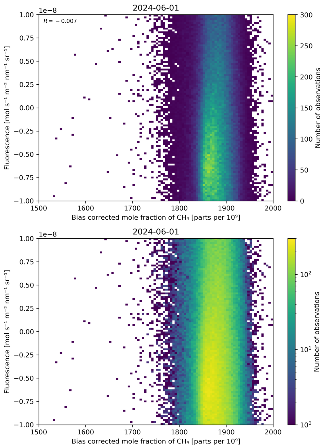
Figure 66: Scatter density plot of “Bias corrected mole fraction of \text{CH}_4 ” against “Fluorescence” for 2024-05-31 to 2024-06-02.
