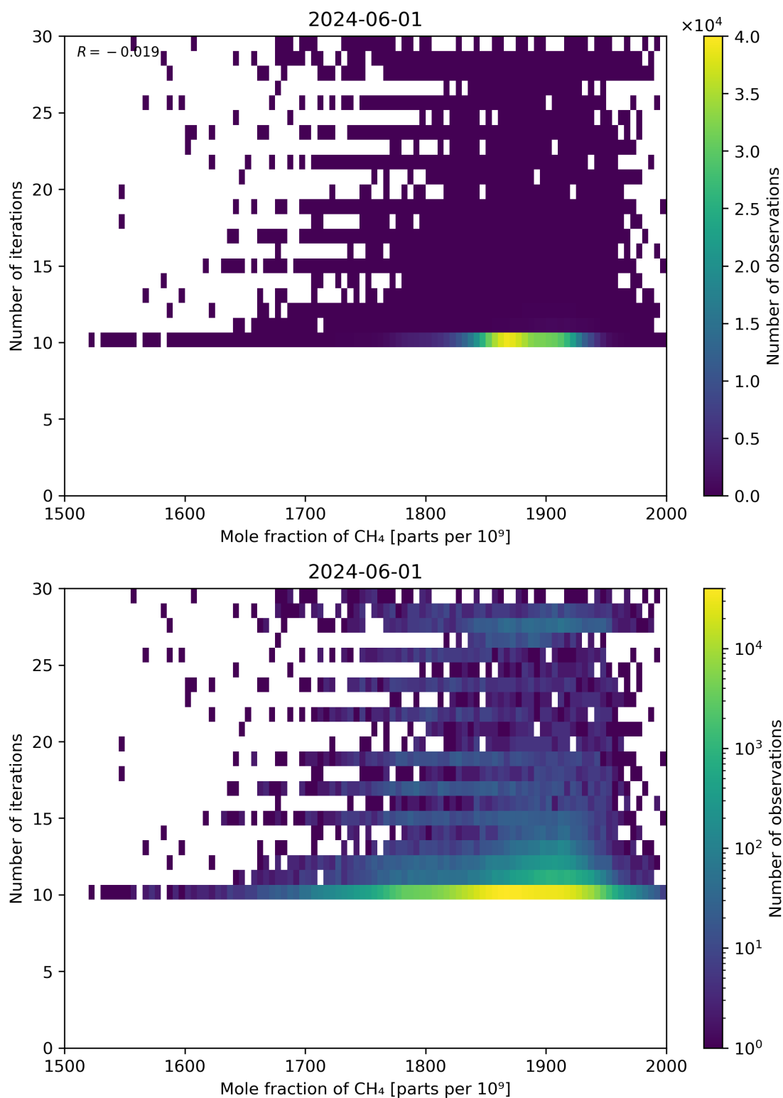
Figure 76: Scatter density plot of “Mole fraction of CH 4 ” against “Number of iterations” for 2024-05-31 to 2024-06-02.
