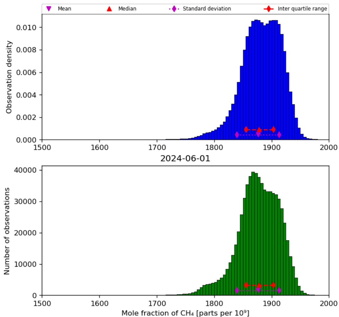
Figure 23: Histogram of “Mole fraction of CH 4 ” for 2024-05-31 to 2024-06-02
