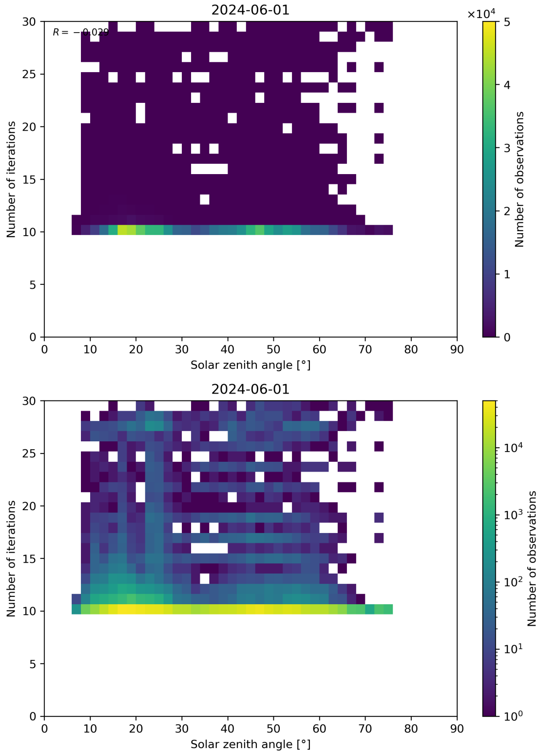
Figure 102: Scatter density plot of “Solar zenith angle” against “Number of iterations” for 2024-05-31 to 2024-06-02.
