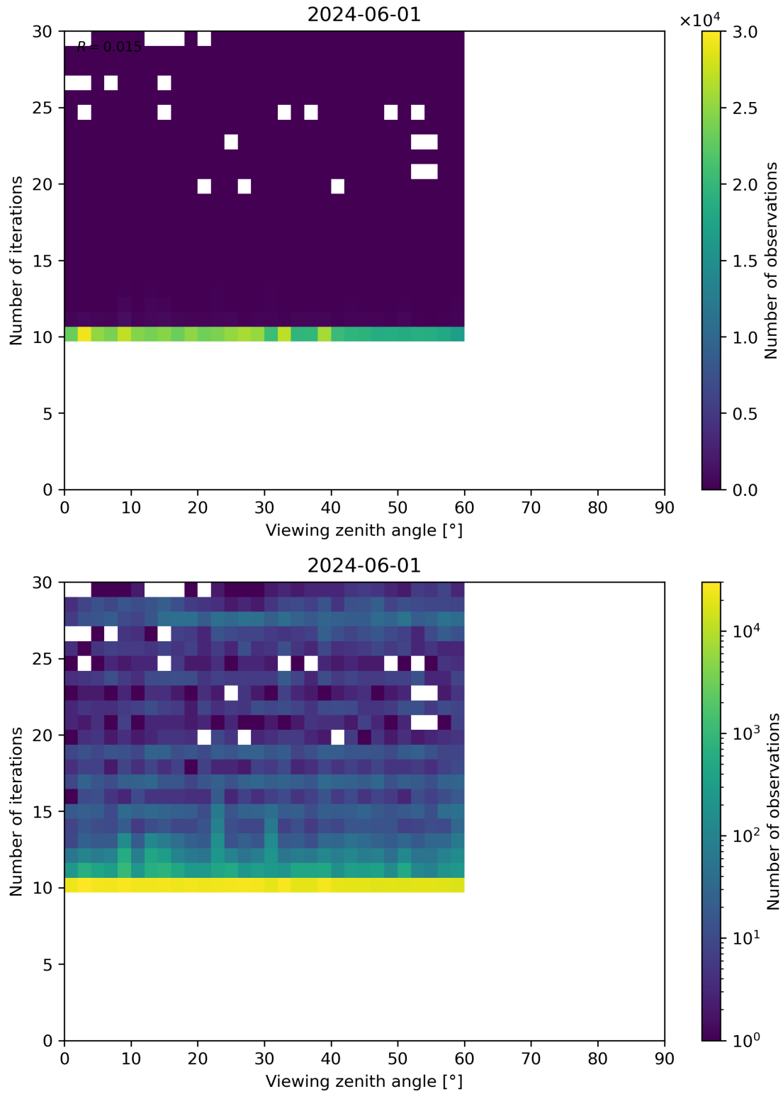
Figure 113: Scatter density plot of “Viewing zenith angle” against “Number of iterations” for 2024-05-31 to 2024-06-02.
