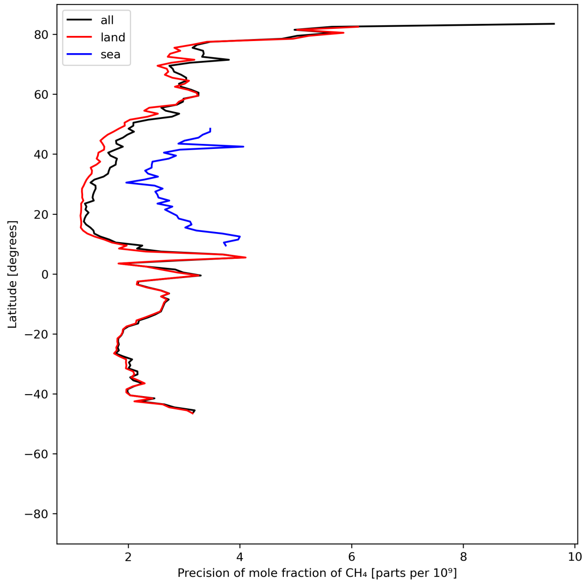
Figure 13: Zonal average of “Precision of mole fraction of CH 4 ” for 2024-05-31 to 2024-06-02.
