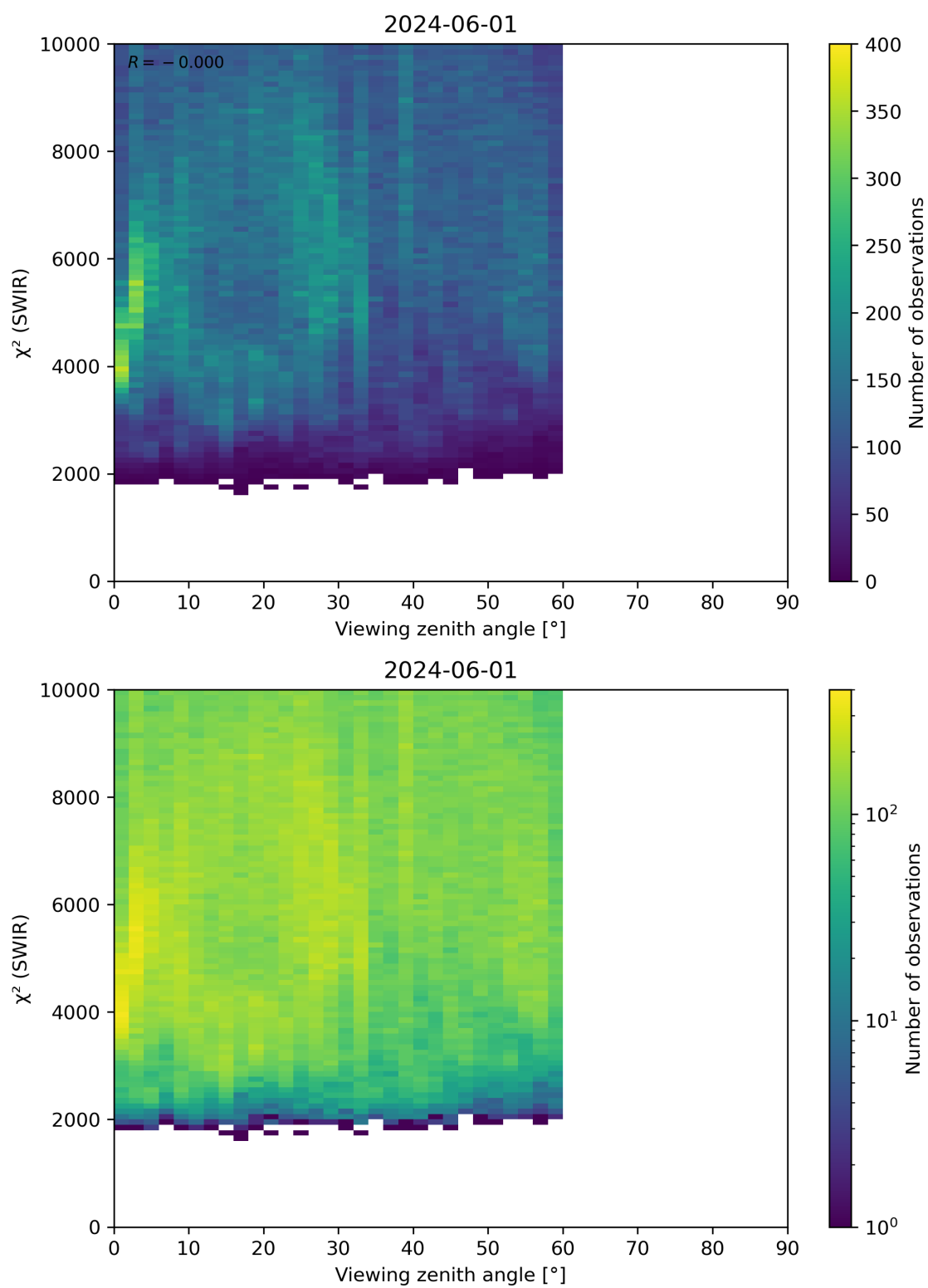
Figure 106: Scatter density plot of “Viewing zenith angle” against “ \chi^2 (SWIR)” for 2024-05-31 to 2024-06-02.
