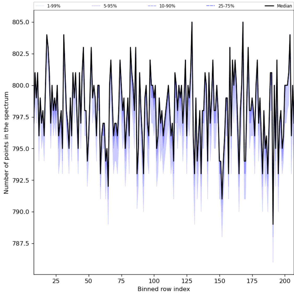
Figure 37: Along track statistics of “Number of points in the spectrum” for 2024-05-31 to 2024-06-02
