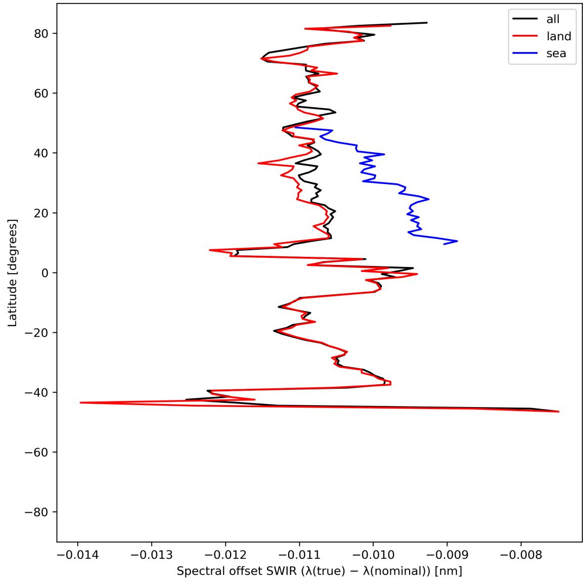
Figure 16: Zonal average of “Spectral offset SWIR ( \lambda(\text{true}) - \lambda(\text{nominal}) )” for 2024-05-31 to 2024-06-02.
