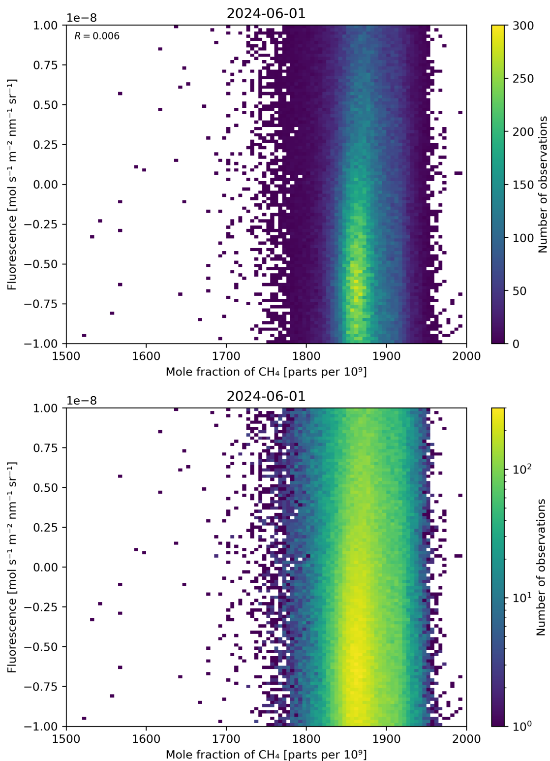
Figure 73: Scatter density plot of “Mole fraction of \text{CH}_4 ” against “Fluorescence” for 2024-05-31 to 2024-06-02.
