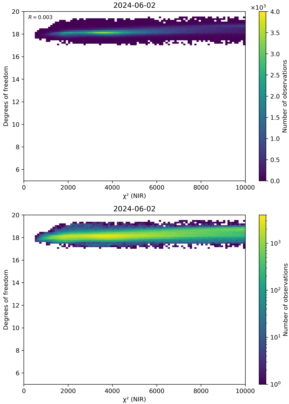
Figure 44: Scatter density plot of “ \chi^2 (NIR)” against “Degrees of freedom” for 2024-06-01 to 2024-06-03.
