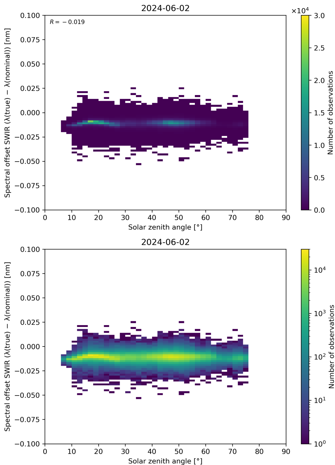
Figure 104: Scatter density plot of “Solar zenith angle” against “Spectral offset SWIR ( \lambda(\text{true}) - \lambda(\text{nominal}) )” for 2024-06-01 to 2024-06-03.
