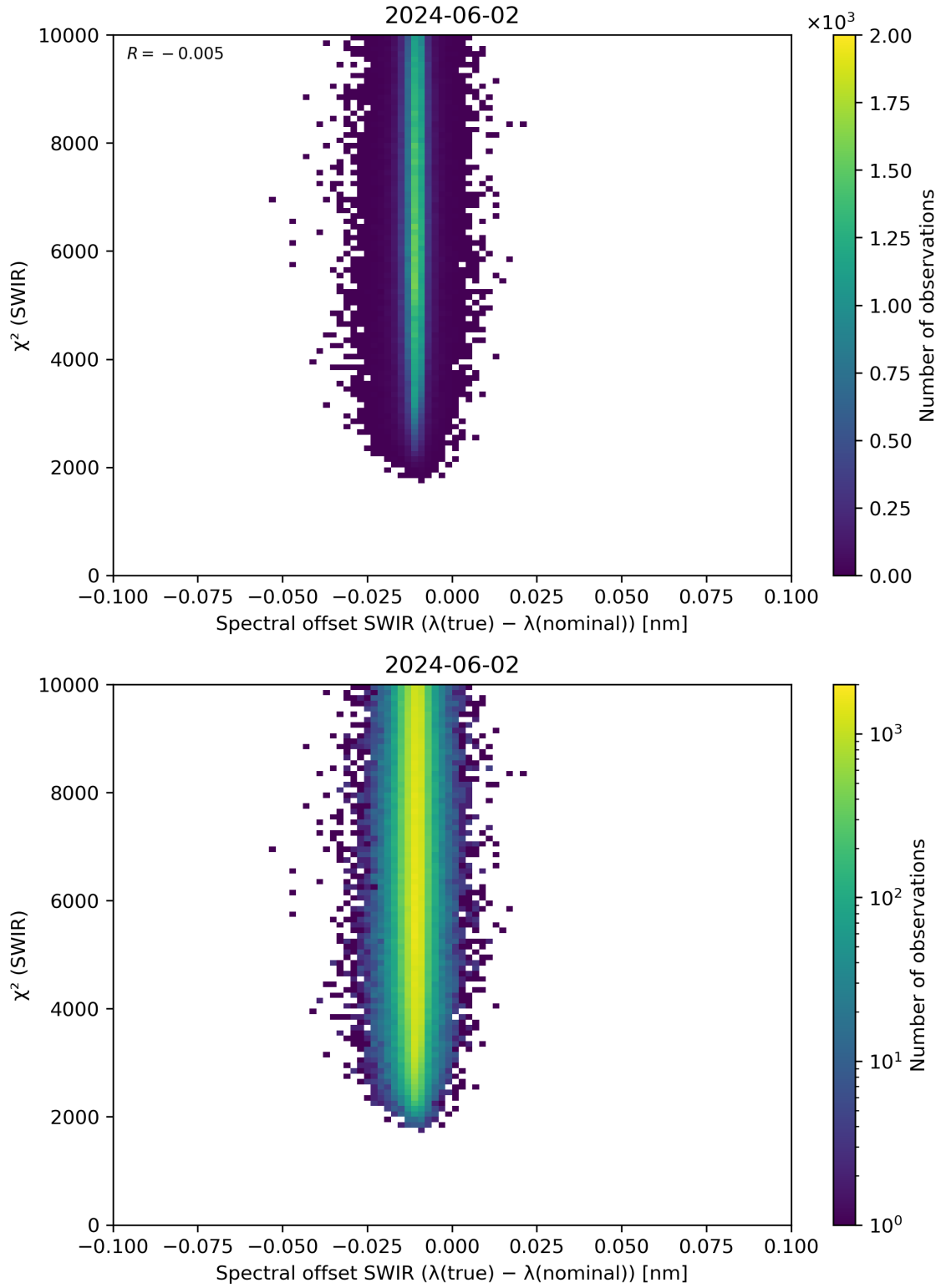
Figure 118: Scatter density plot of “Spectral offset SWIR ( \lambda(\text{true}) - \lambda(\text{nominal}) )” against “ \chi^2 (SWIR)” for 2024-06-01 to 2024-06-03.
