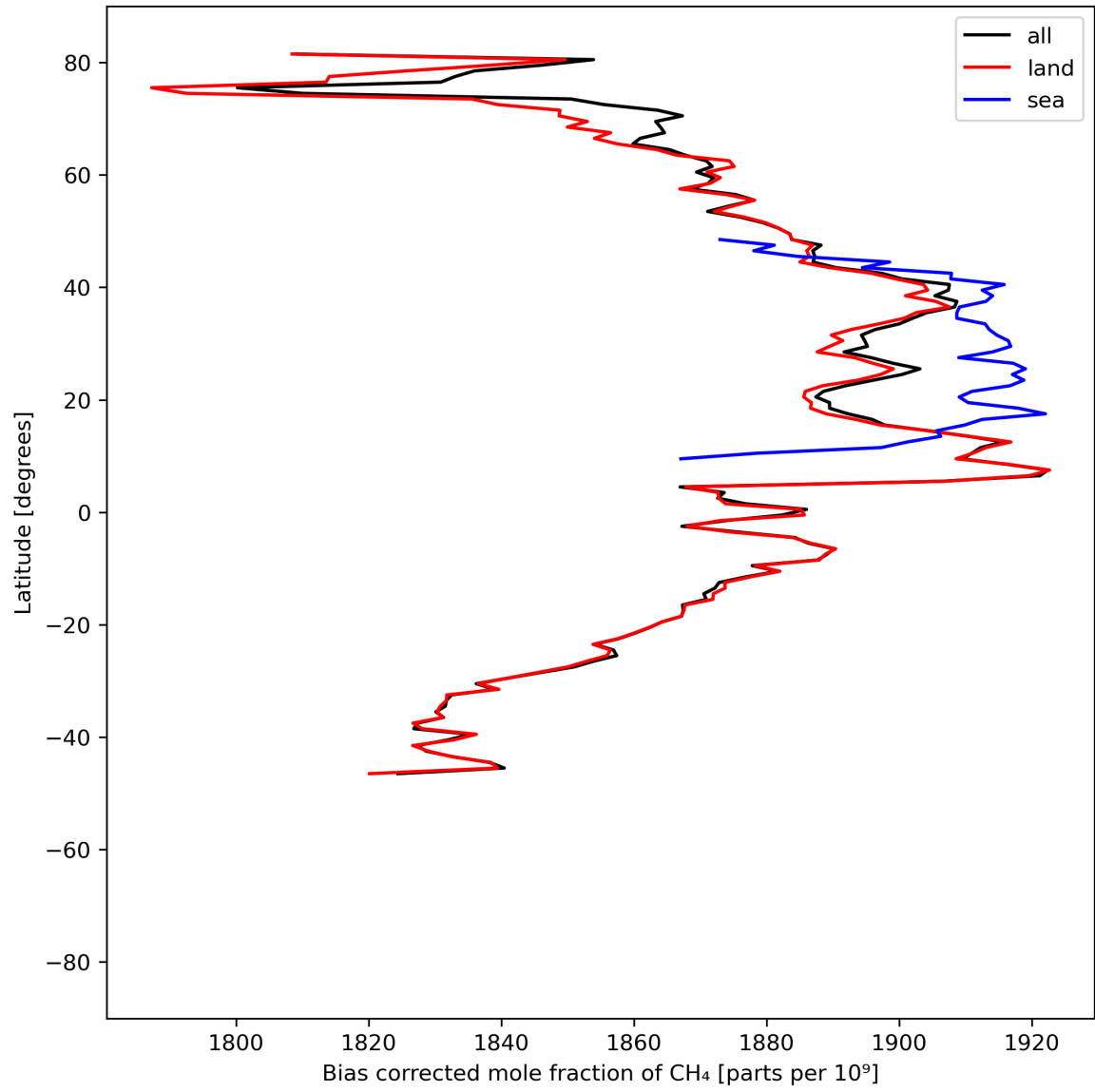
Figure 14: Zonal average of “Bias corrected mole fraction of \text{CH}_4 ” for 2024-06-01 to 2024-06-03.
