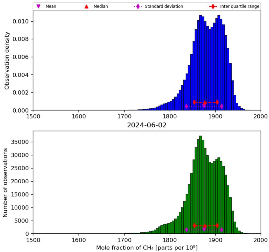
Figure 23: Histogram of “Mole fraction of CH 4 ” for 2024-06-01 to 2024-06-03
