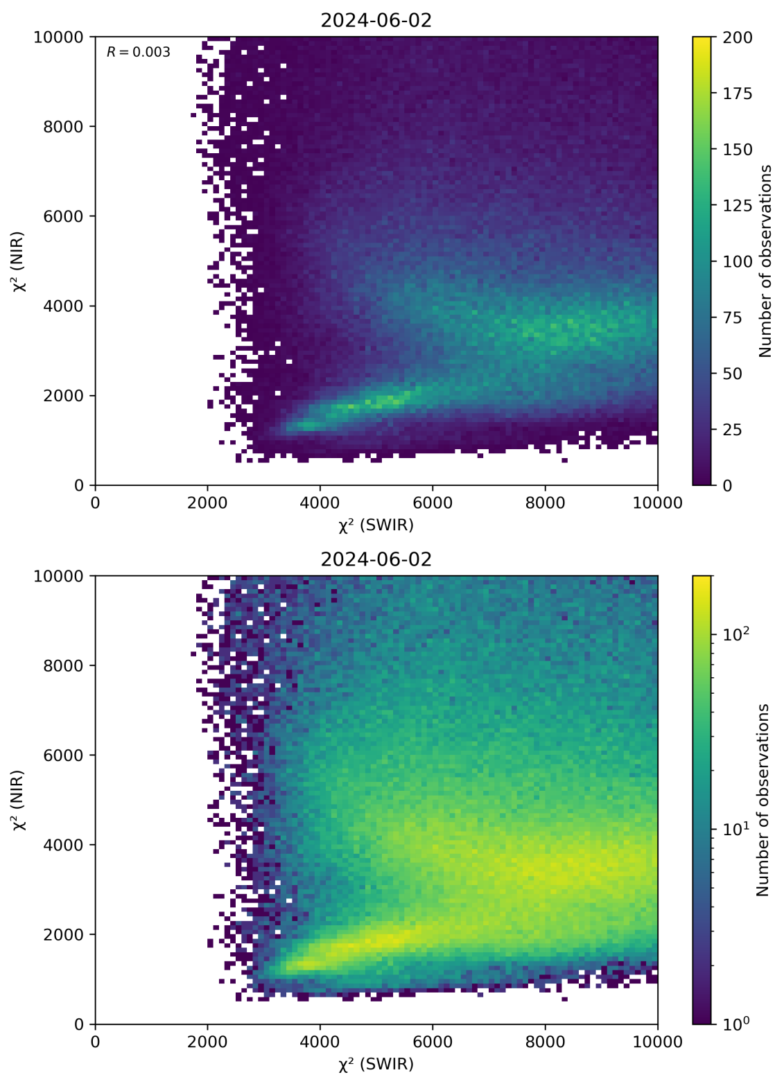
Figure 47: Scatter density plot of “ \chi^2 (SWIR)” against “ \chi^2 (NIR)” for 2024-06-01 to 2024-06-03.
