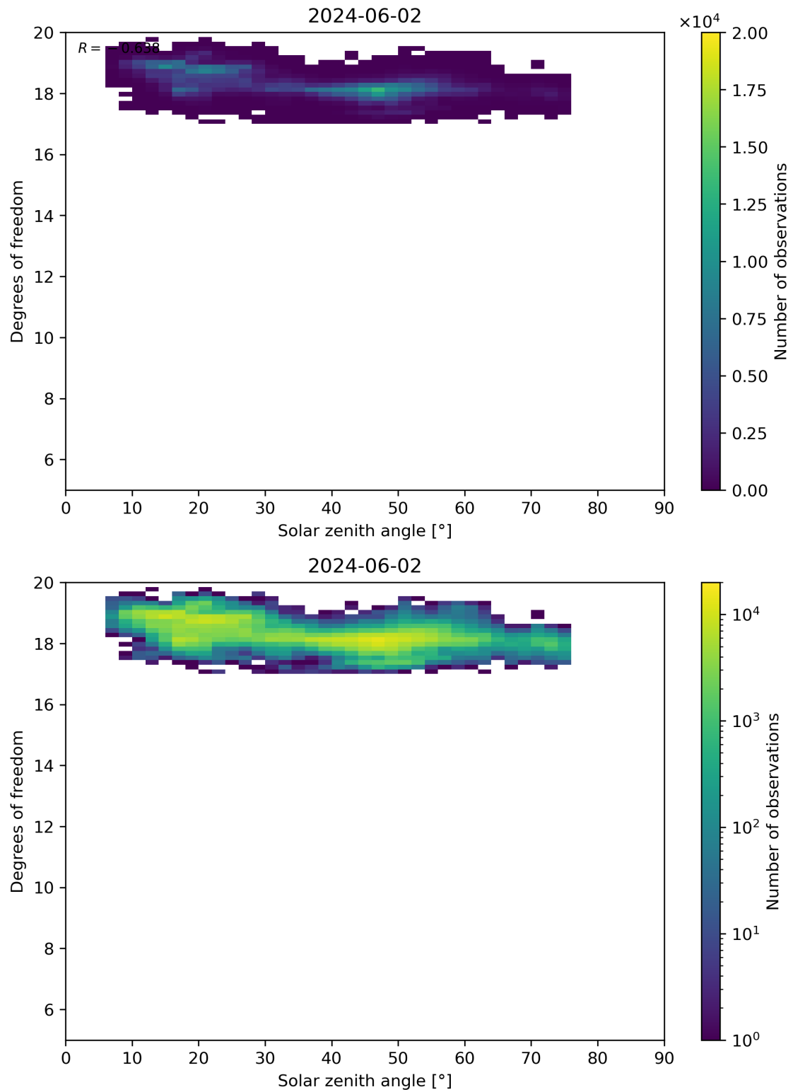
Figure 96: Scatter density plot of “Solar zenith angle” against “Degrees of freedom” for 2024-06-01 to 2024-06-03.
