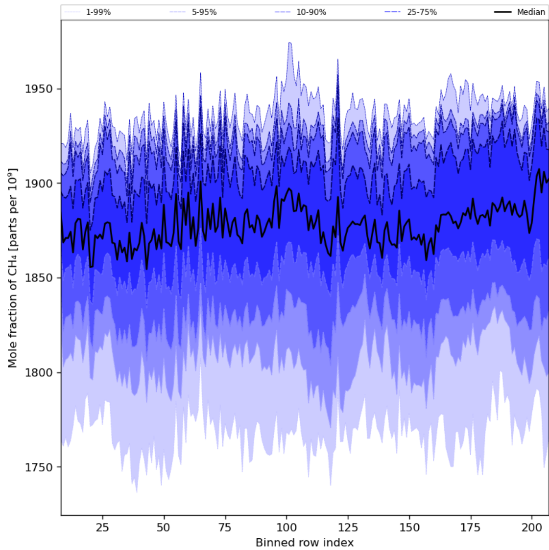
Figure 34: Along track statistics of “Mole fraction of CH 4 ” for 2024-06-01 to 2024-06-03
