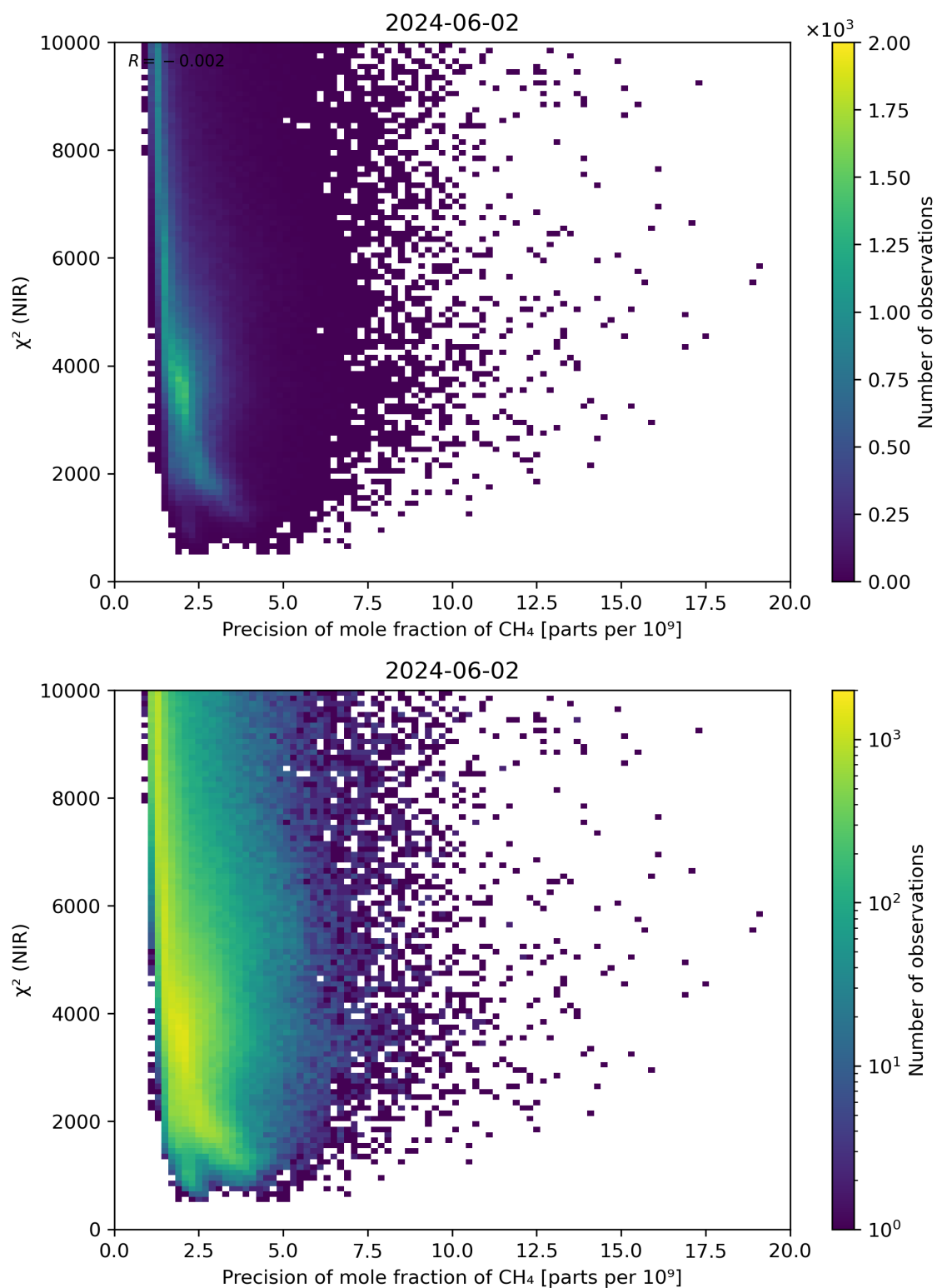
Figure 78: Scatter density plot of “Precision of mole fraction of CH 4 ” against “ \chi^2 (NIR)” for 2024-06-01 to 2024-06-03.
