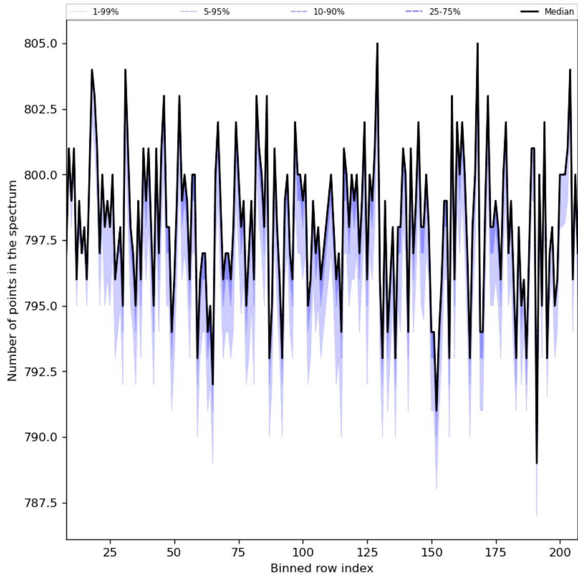
Figure 37: Along track statistics of “Number of points in the spectrum” for 2024-06-01 to 2024-06-03
