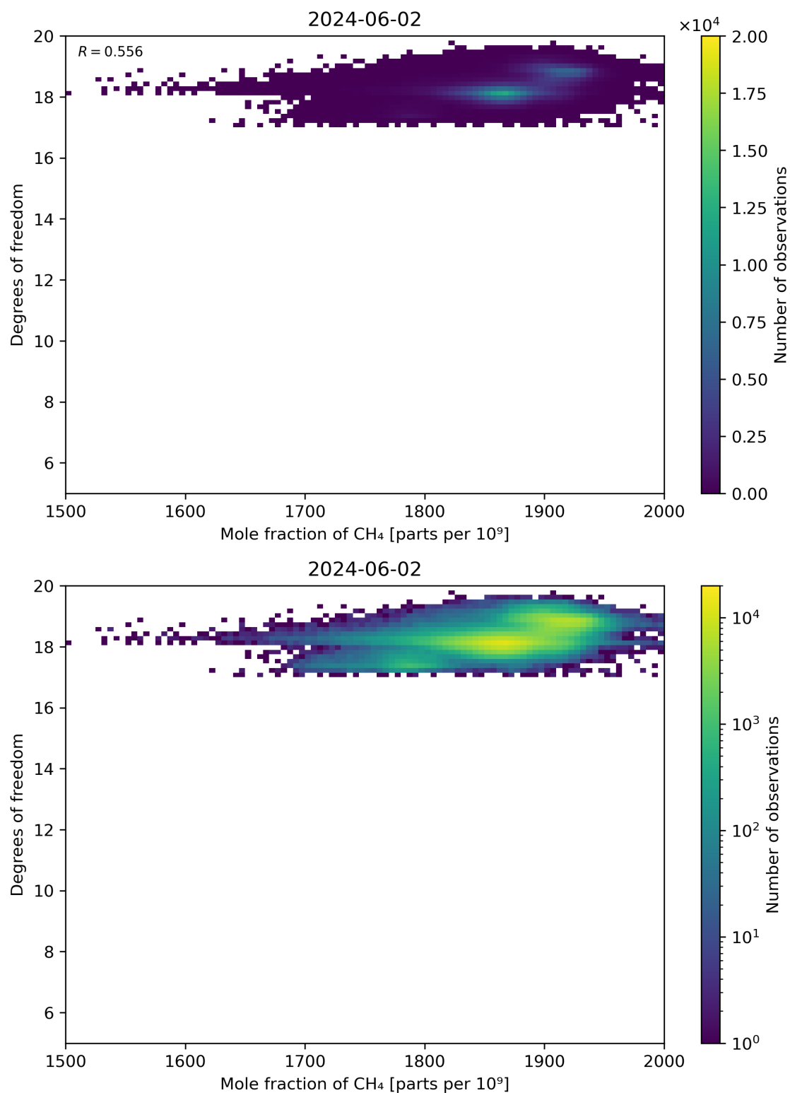
Figure 72: Scatter density plot of “Mole fraction of CH 4 ” against “Degrees of freedom” for 2024-06-01 to 2024-06-03.
