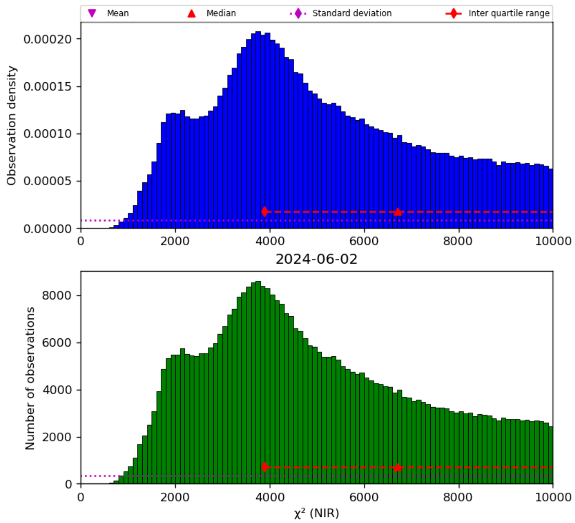
Figure 29: Histogram of “ \chi^2 (NIR)” for 2024-06-01 to 2024-06-03
