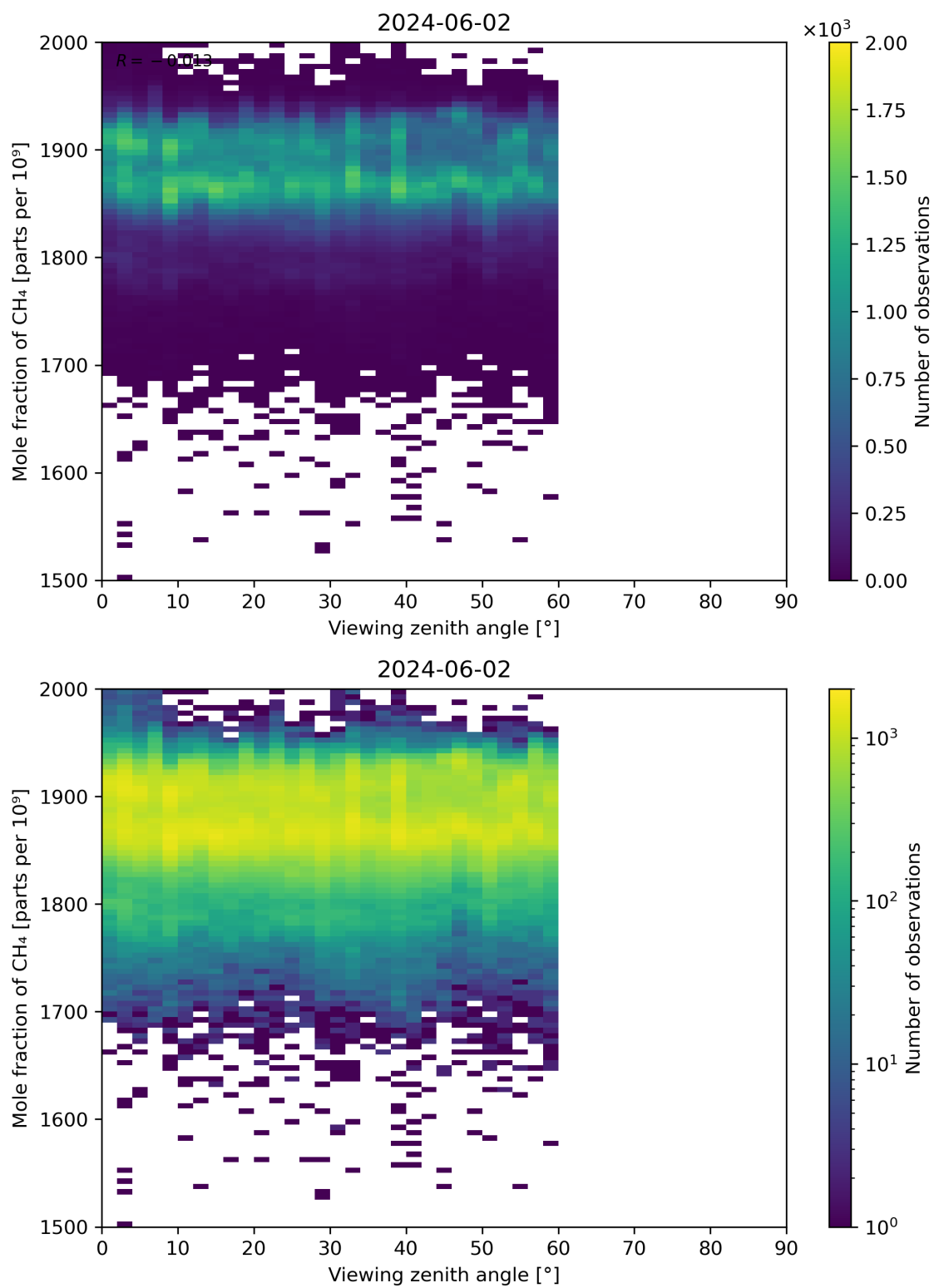
Figure 110: Scatter density plot of “Viewing zenith angle” against “Mole fraction of CH 4 ” for 2024-06-01 to 2024-06-03.
