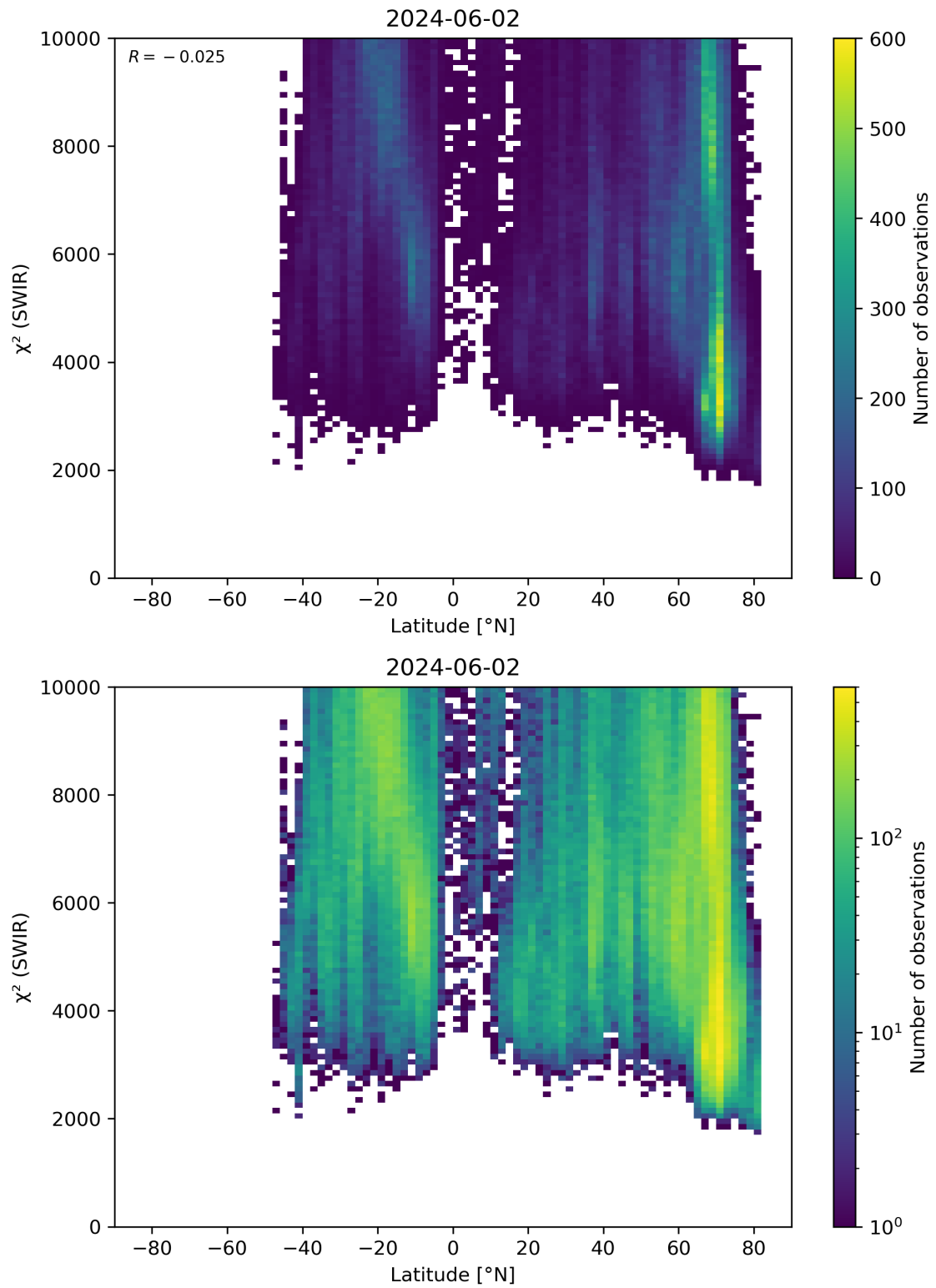
Figure 54: Scatter density plot of “Latitude” against “ \chi^2 (SWIR)” for 2024-06-01 to 2024-06-03.
