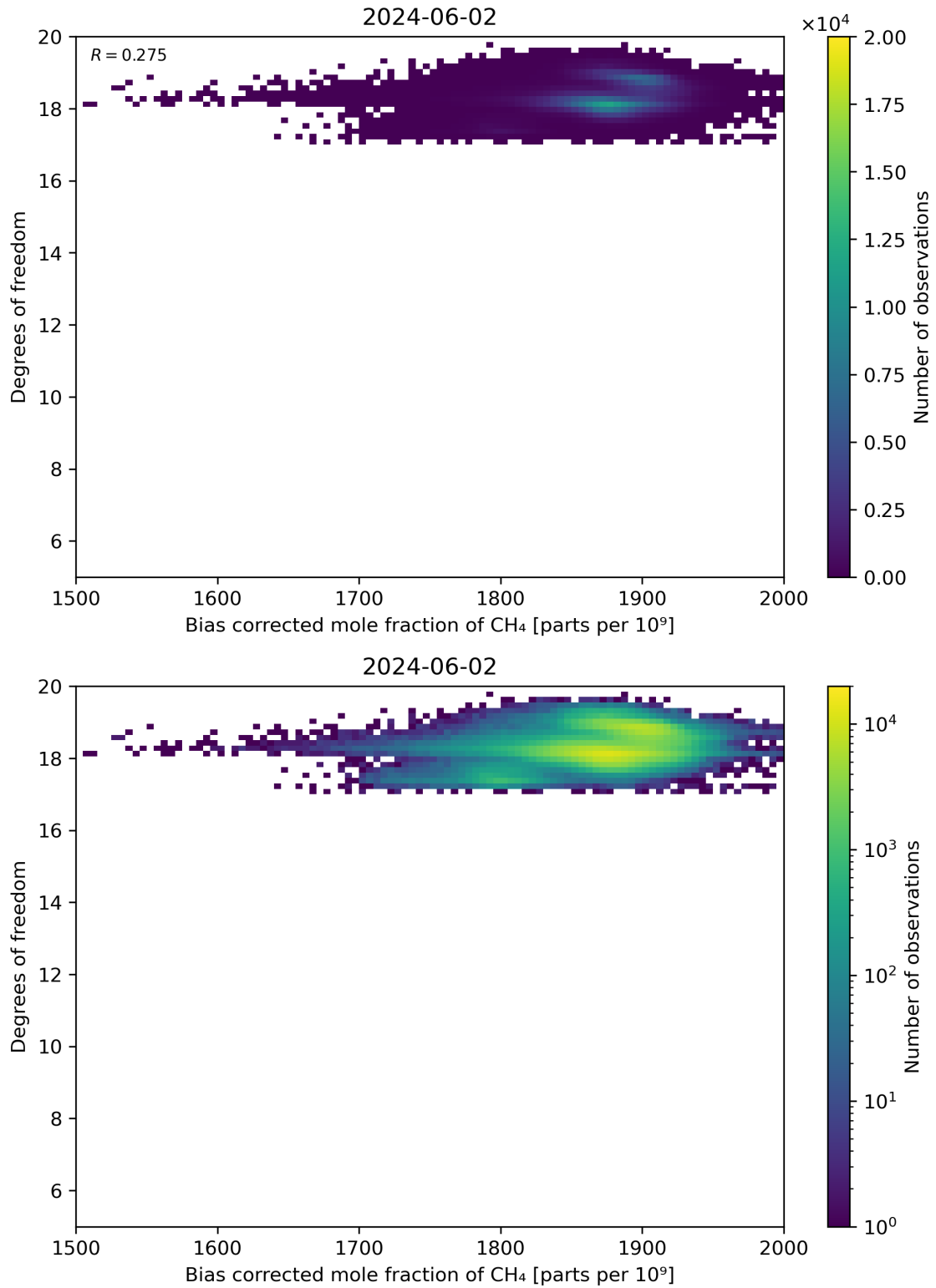
Figure 65: Scatter density plot of “Bias corrected mole fraction of CH 4 ” against “Degrees of freedom” for 2024-06-01 to 2024-06-03.
