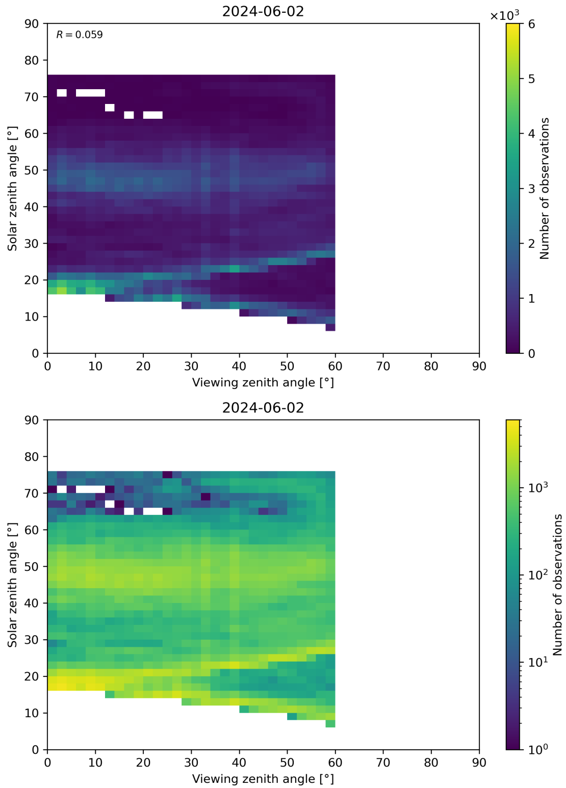
Figure 115: Scatter density plot of “Viewing zenith angle” against “Solar zenith angle” for 2024-06-01 to 2024-06-03.
