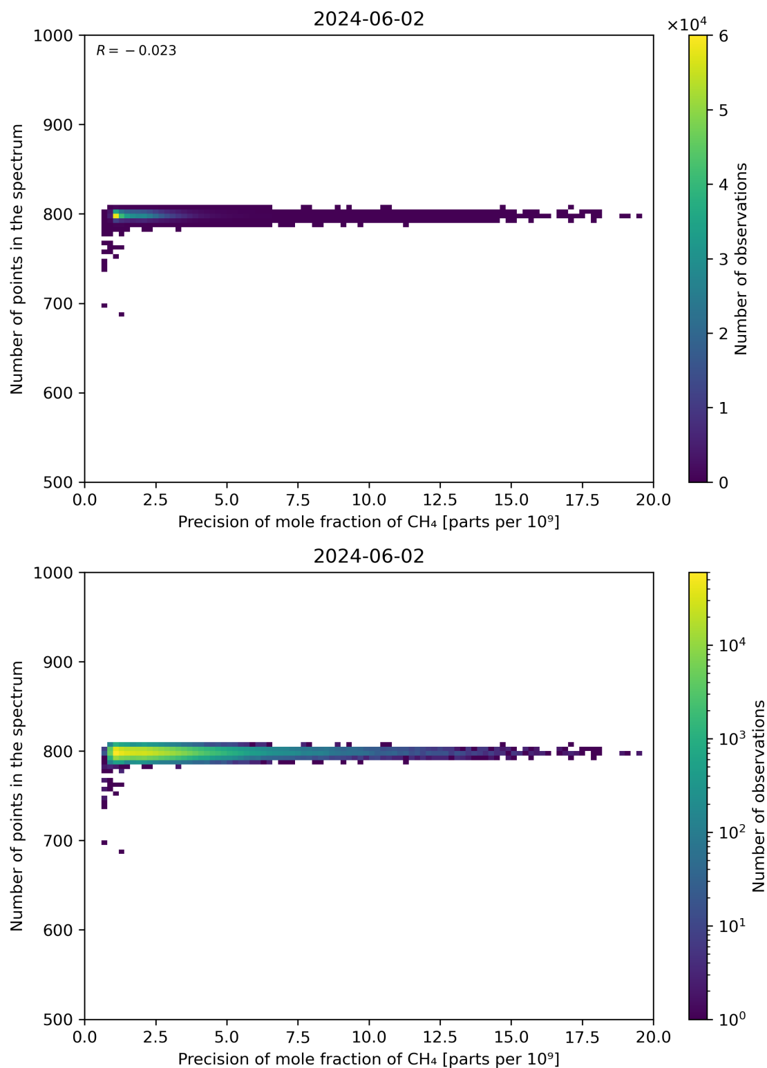
Figure 84: Scatter density plot of “Precision of mole fraction of CH 4 ” against “Number of points in the spectrum” for 2024-06-01 to 2024-06-03.
