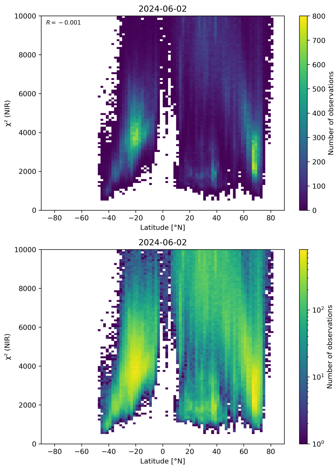
Figure 53: Scatter density plot of “Latitude” against “ \chi^2 (NIR)” for 2024-06-01 to 2024-06-03.
