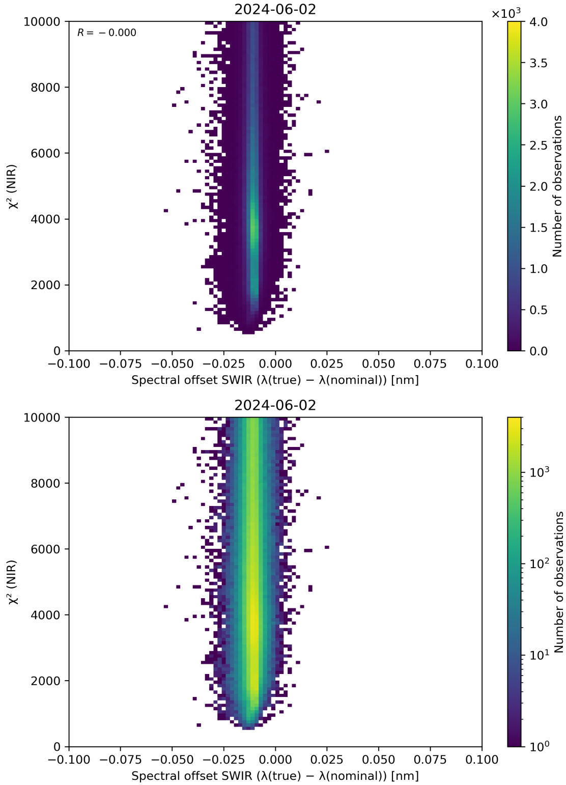
Figure 117: Scatter density plot of “Spectral offset SWIR ( \lambda(\text{true}) - \lambda(\text{nominal}) )” against “ \chi^2 (NIR)” for 2024-06-01 to 2024-06-03.
