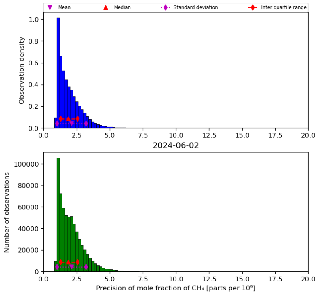
Figure 24: Histogram of “Precision of mole fraction of CH 4 ” for 2024-06-01 to 2024-06-03
