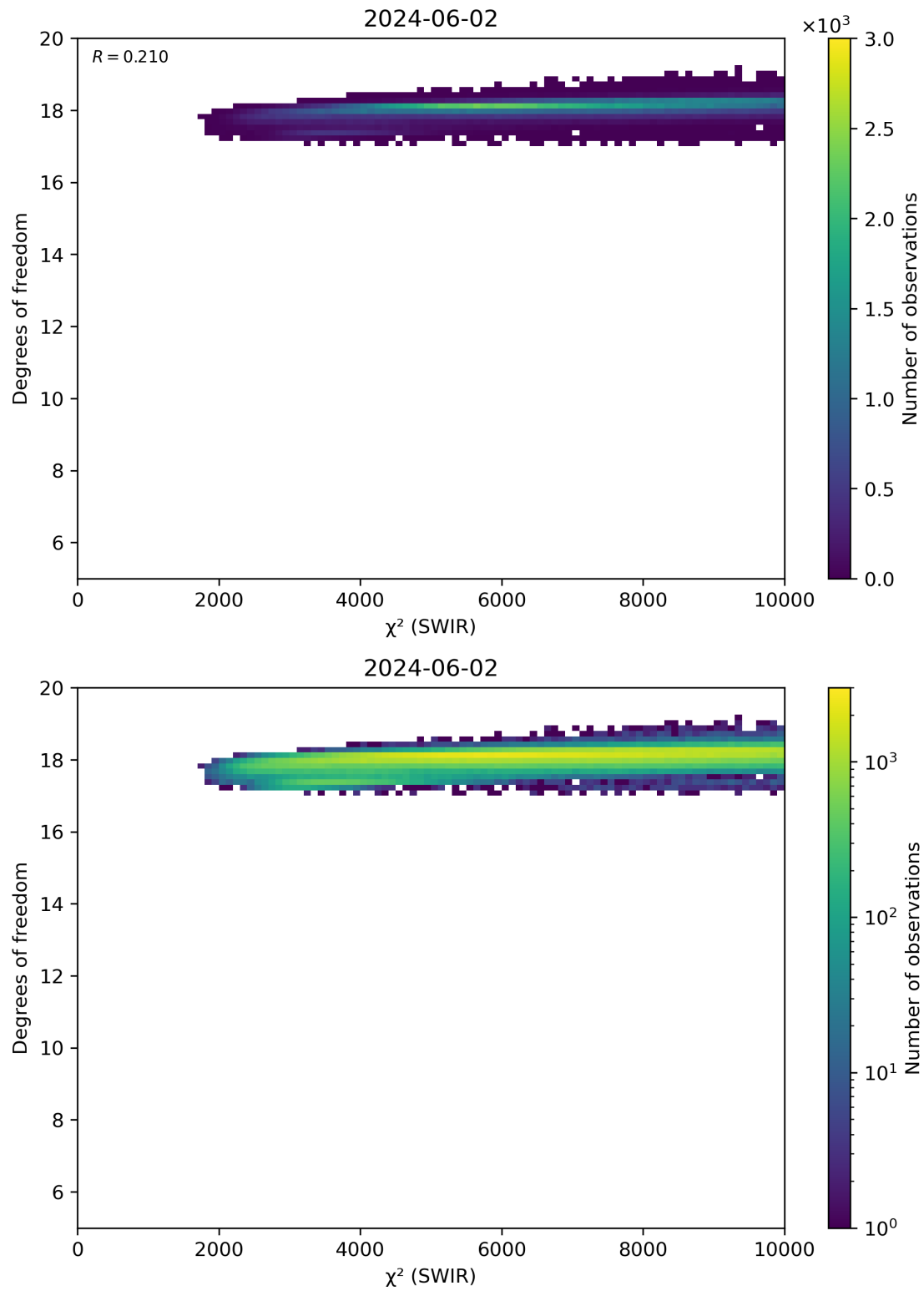
Figure 48: Scatter density plot of “ \chi^2 (SWIR)” against “Degrees of freedom” for 2024-06-01 to 2024-06-03.
