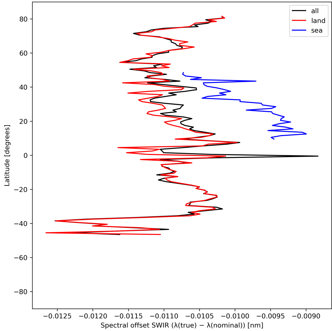
Figure 16: Zonal average of “Spectral offset SWIR ( \lambda(\text{true}) - \lambda(\text{nominal}) )” for 2024-06-01 to 2024-06-03.
