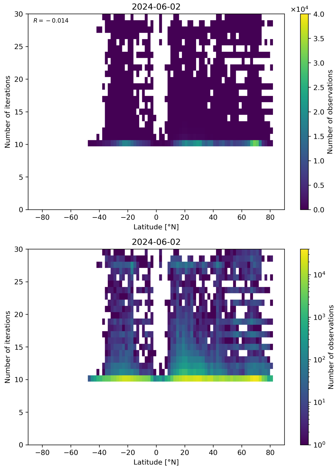
Figure 60: Scatter density plot of “Latitude” against “Number of iterations” for 2024-06-01 to 2024-06-03.
