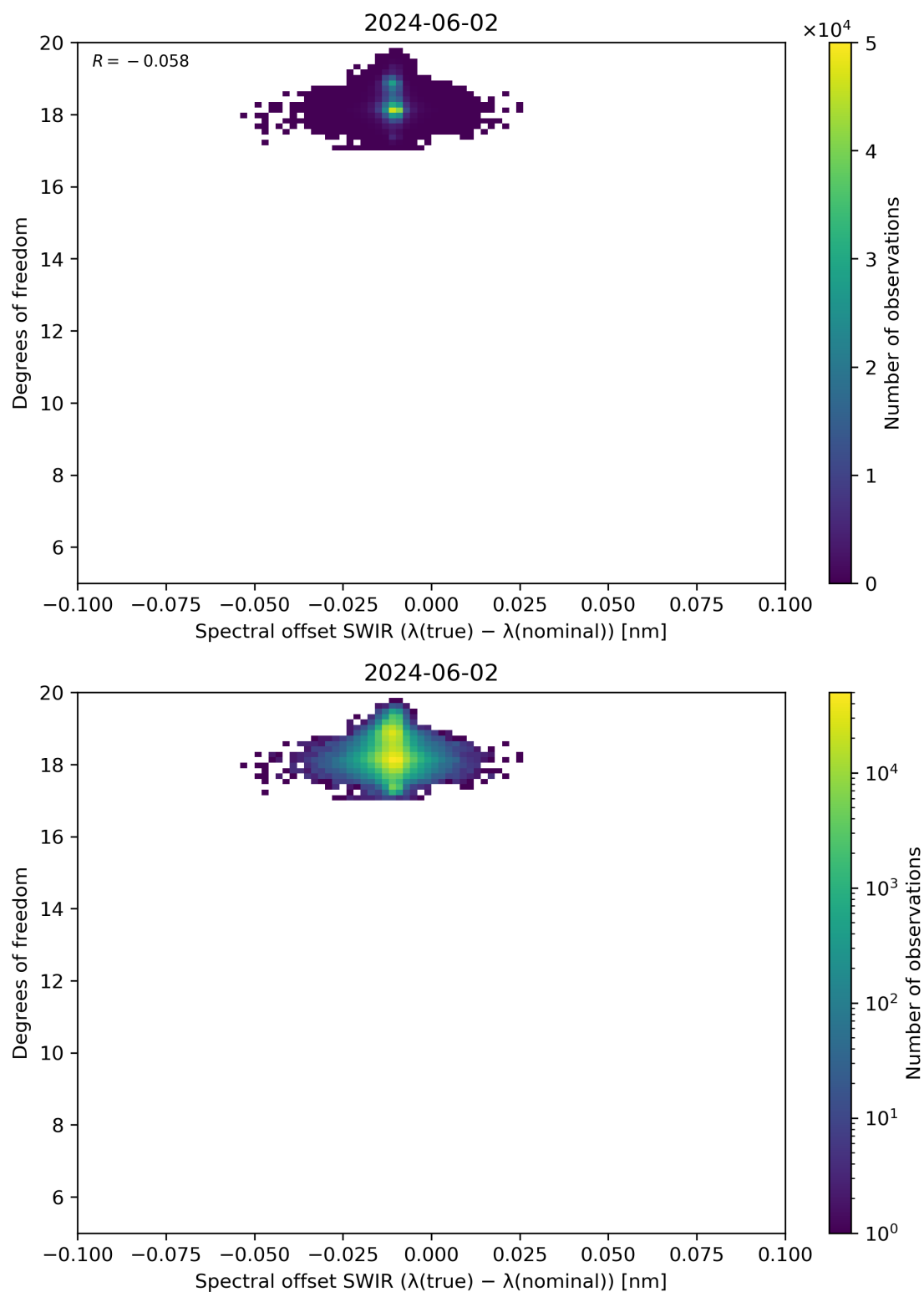
Figure 119: Scatter density plot of “Spectral offset SWIR ( \lambda(\text{true}) - \lambda(\text{nominal}) )” against “Degrees of freedom” for 2024-06-01 to 2024-06-03.
