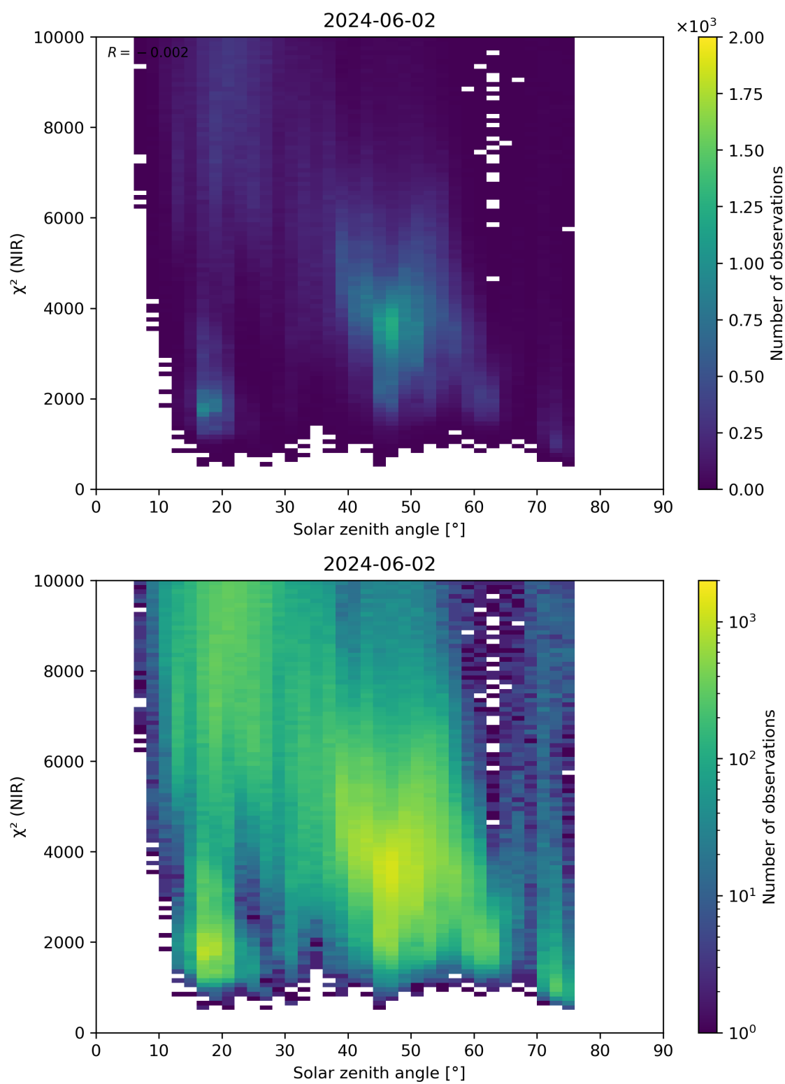
Figure 94: Scatter density plot of “Solar zenith angle” against “ \chi^2 (NIR)” for 2024-06-01 to 2024-06-03.
