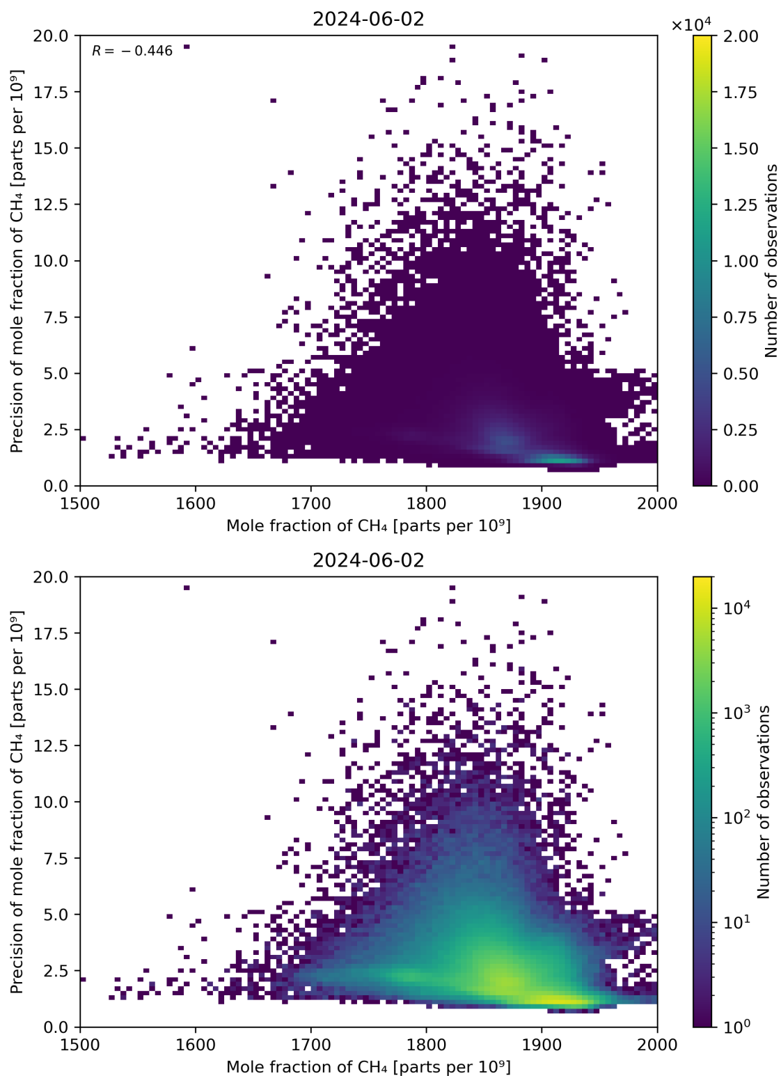
Figure 75: Scatter density plot of “Mole fraction of CH 4 ” against “Precision of mole fraction of CH 4 ” for 2024-06-01 to 2024-06-03.
