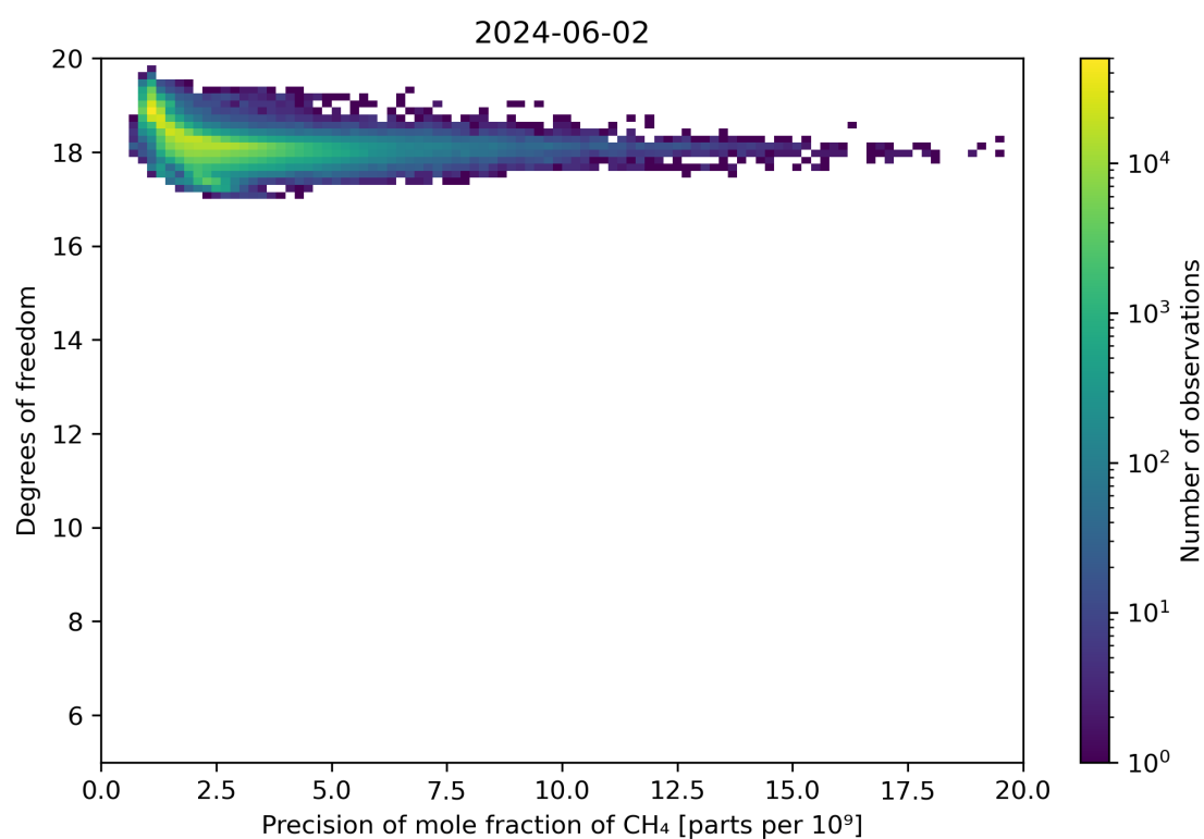
Figure 80: Scatter density plot of “Precision of mole fraction of CH 4 ” against “Degrees of freedom” for 2024-06-01 to 2024-06-03.
