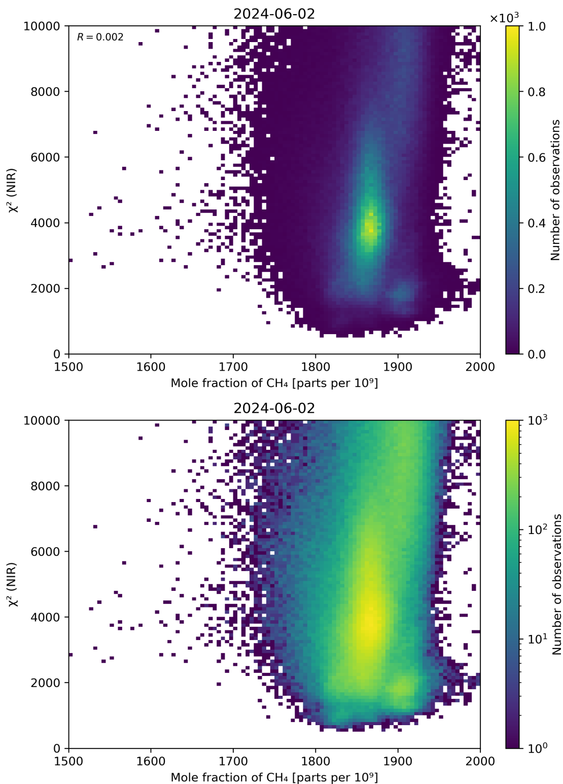
Figure 70: Scatter density plot of “Mole fraction of \text{CH}_4 ” against “ \chi^2 (NIR)” for 2024-06-01 to 2024-06-03.
