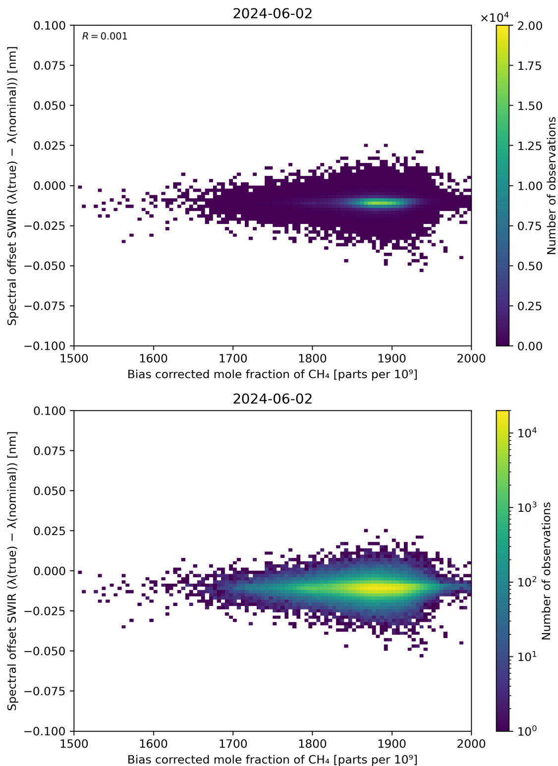
Figure 69: Scatter density plot of “Bias corrected mole fraction of \text{CH}_4 ” against “Spectral offset SWIR ( \lambda(\text{true}) - \lambda(\text{nominal}) )” for 2024-06-01 to 2024-06-03.
