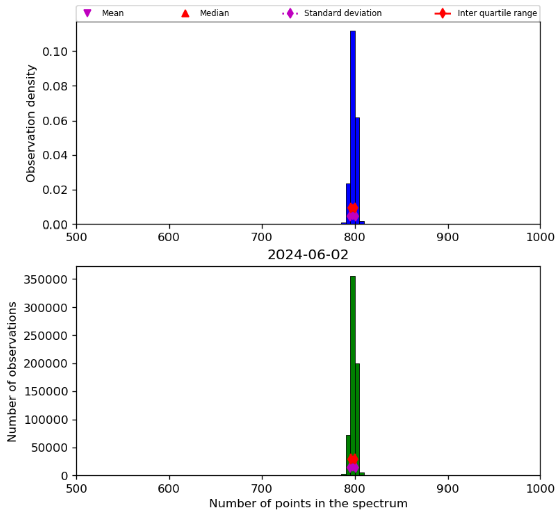
Figure 26: Histogram of “Number of points in the spectrum” for 2024-06-01 to 2024-06-03
