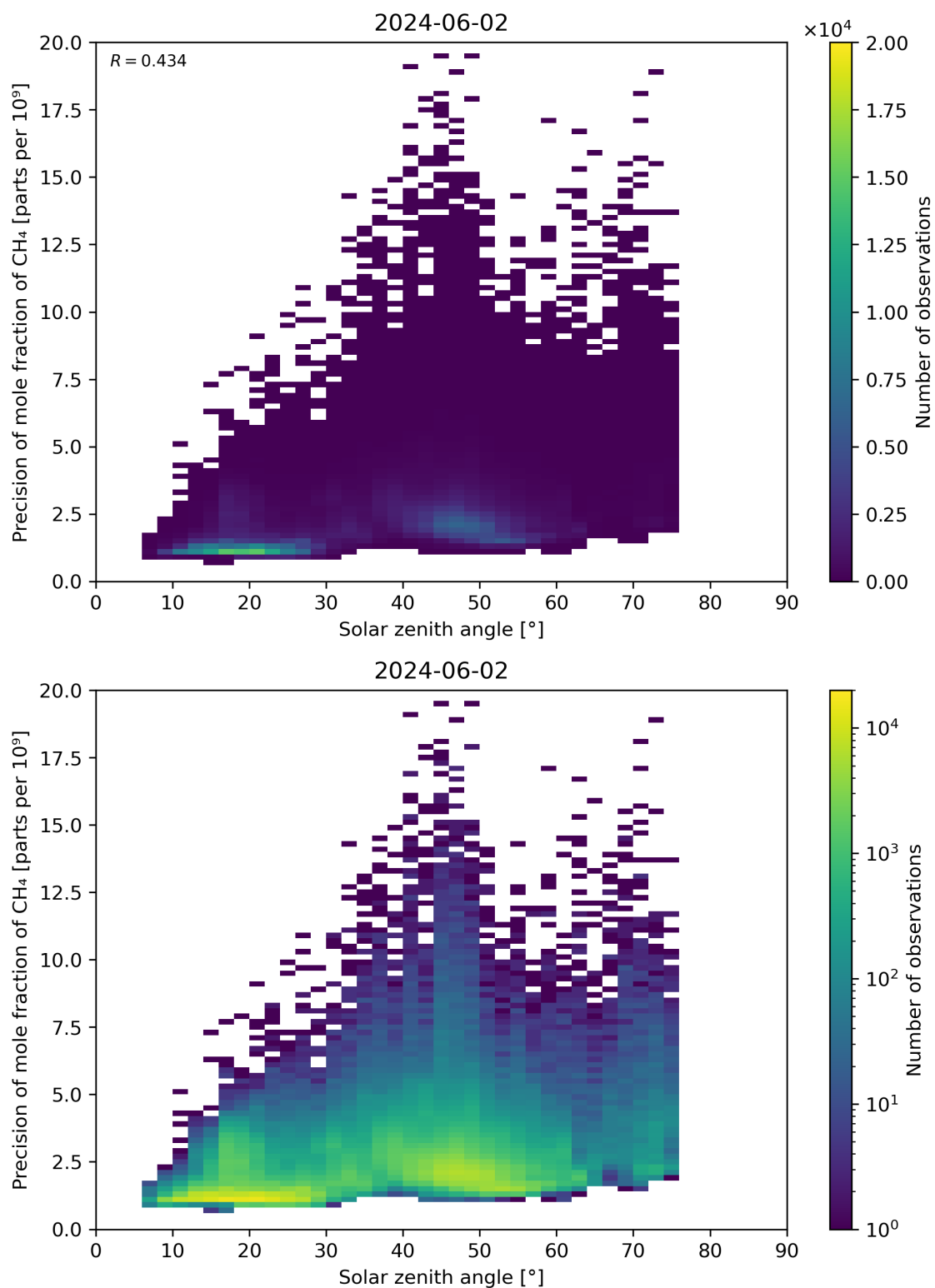
Figure 101: Scatter density plot of “Solar zenith angle” against “Precision of mole fraction of \text{CH}_4 ” for 2024-06-01 to 2024-06-03.
