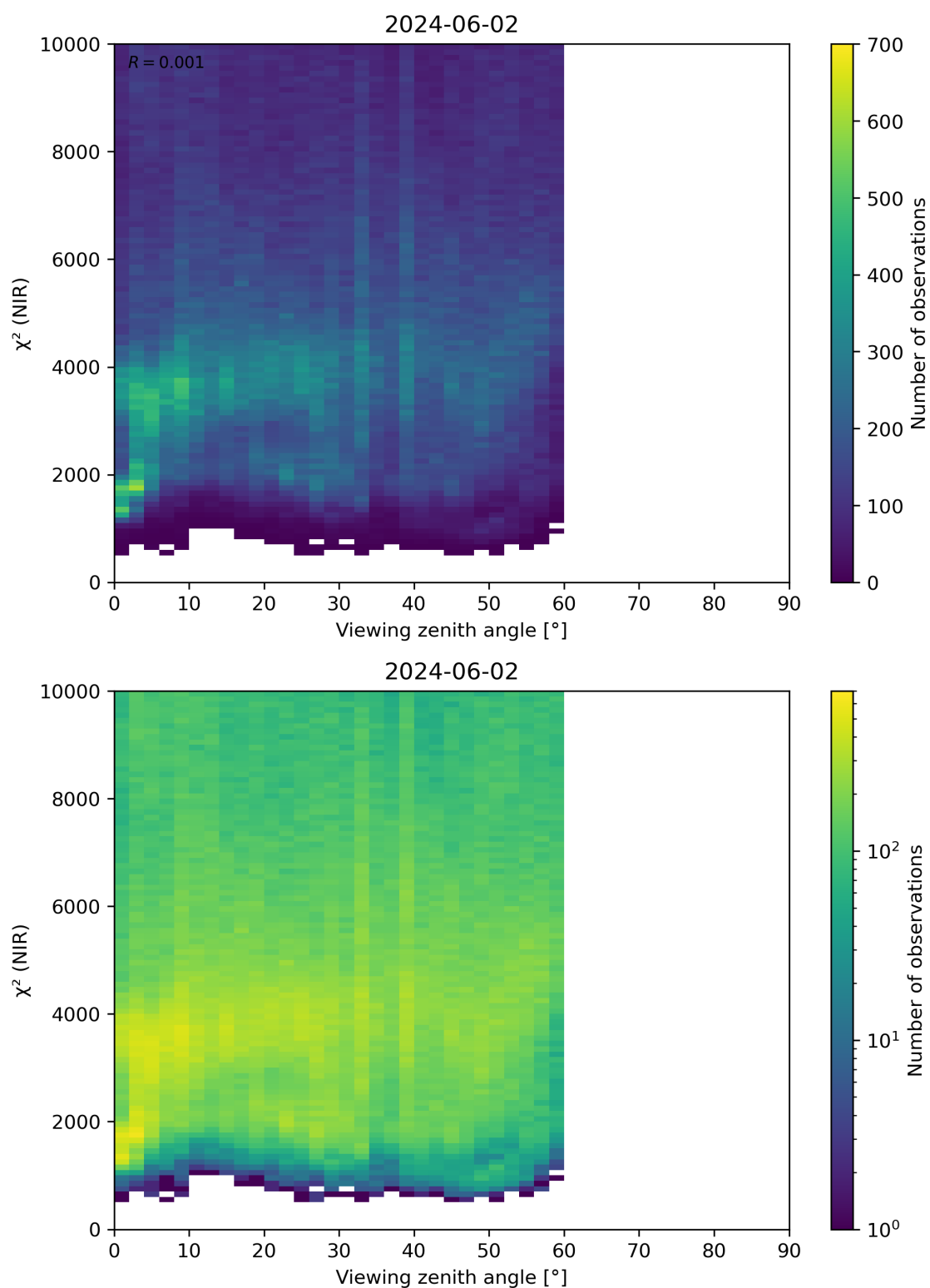
Figure 105: Scatter density plot of “Viewing zenith angle” against “ \chi^2 (NIR)” for 2024-06-01 to 2024-06-03.
