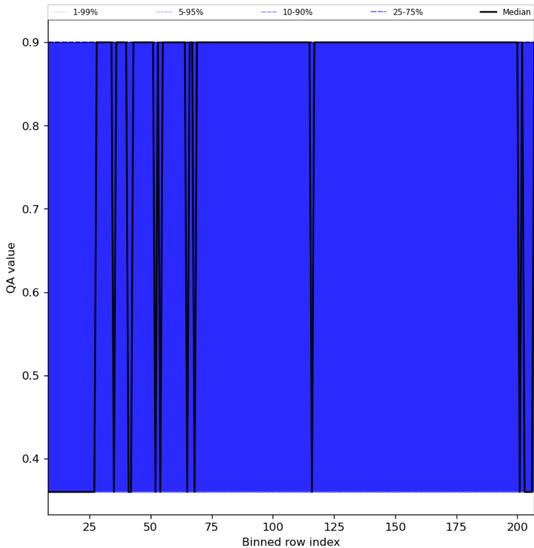
Figure 33: Along track statistics of “QA value” for 2024-06-01 to 2024-06-03
