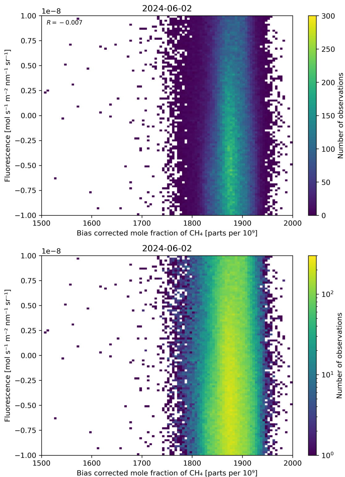
Figure 66: Scatter density plot of “Bias corrected mole fraction of \text{CH}_4 ” against “Fluorescence” for 2024-06-01 to 2024-06-03.
