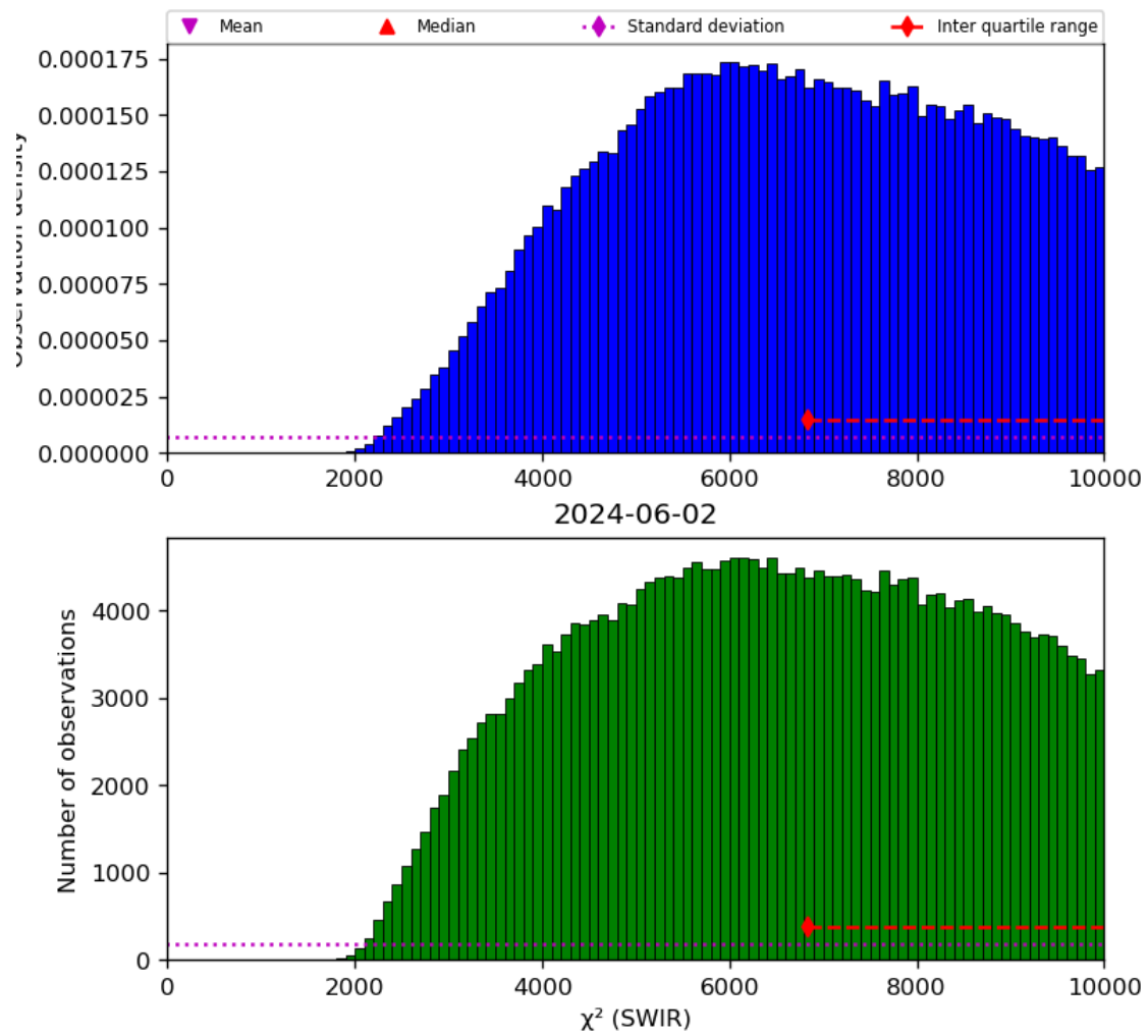
Figure 28: Histogram of “ \chi^2 (SWIR)” for 2024-06-01 to 2024-06-03
