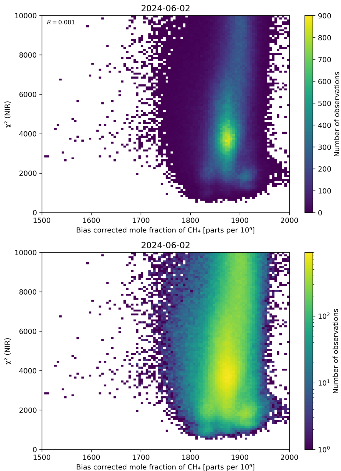
Figure 63: Scatter density plot of “Bias corrected mole fraction of CH 4 ” against “ \chi^2 (NIR)” for 2024-06-01 to 2024-06-03.
