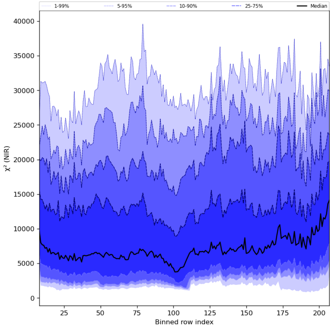
Figure 40: Along track statistics of " \chi^2 (NIR)" for 2024-06-01 to 2024-06-03
