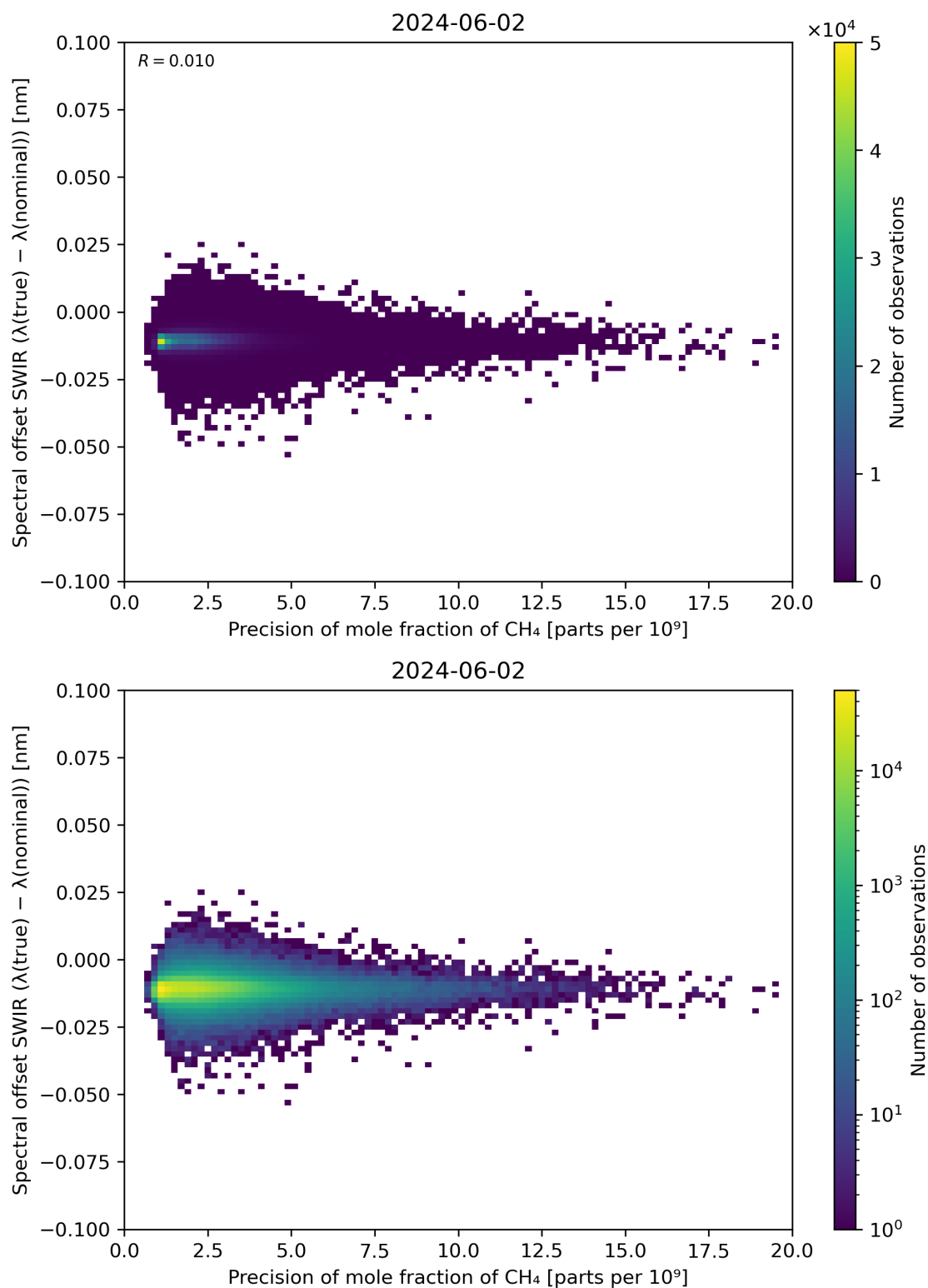
Figure 85: Scatter density plot of “Precision of mole fraction of CH 4 ” against “Spectral offset SWIR ( \lambda(\text{true}) - \lambda(\text{nominal}) )” for 2024-06-01 to 2024-06-03.
