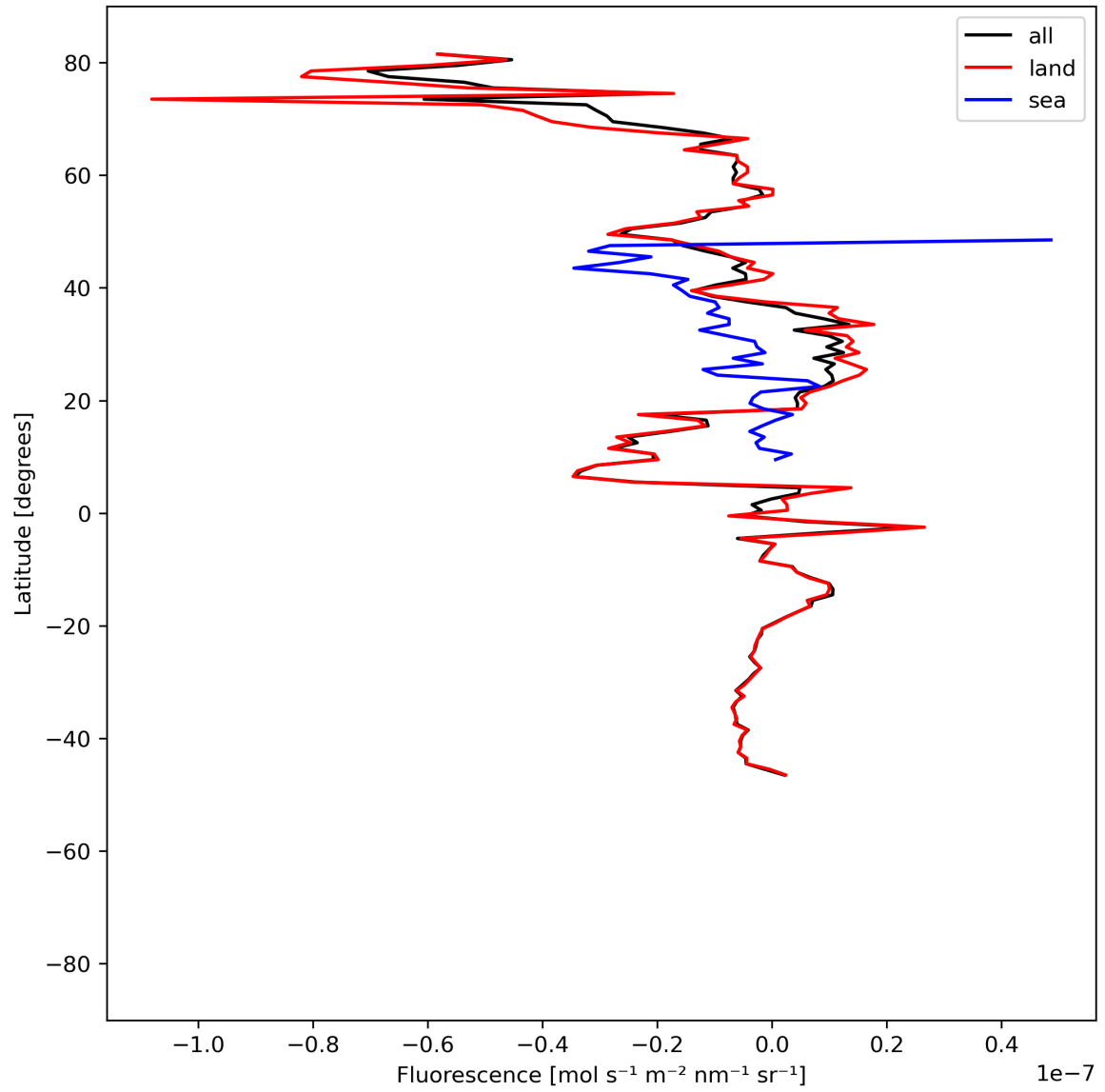
Figure 21: Zonal average of “Fluorescence” for 2024-06-01 to 2024-06-03.
