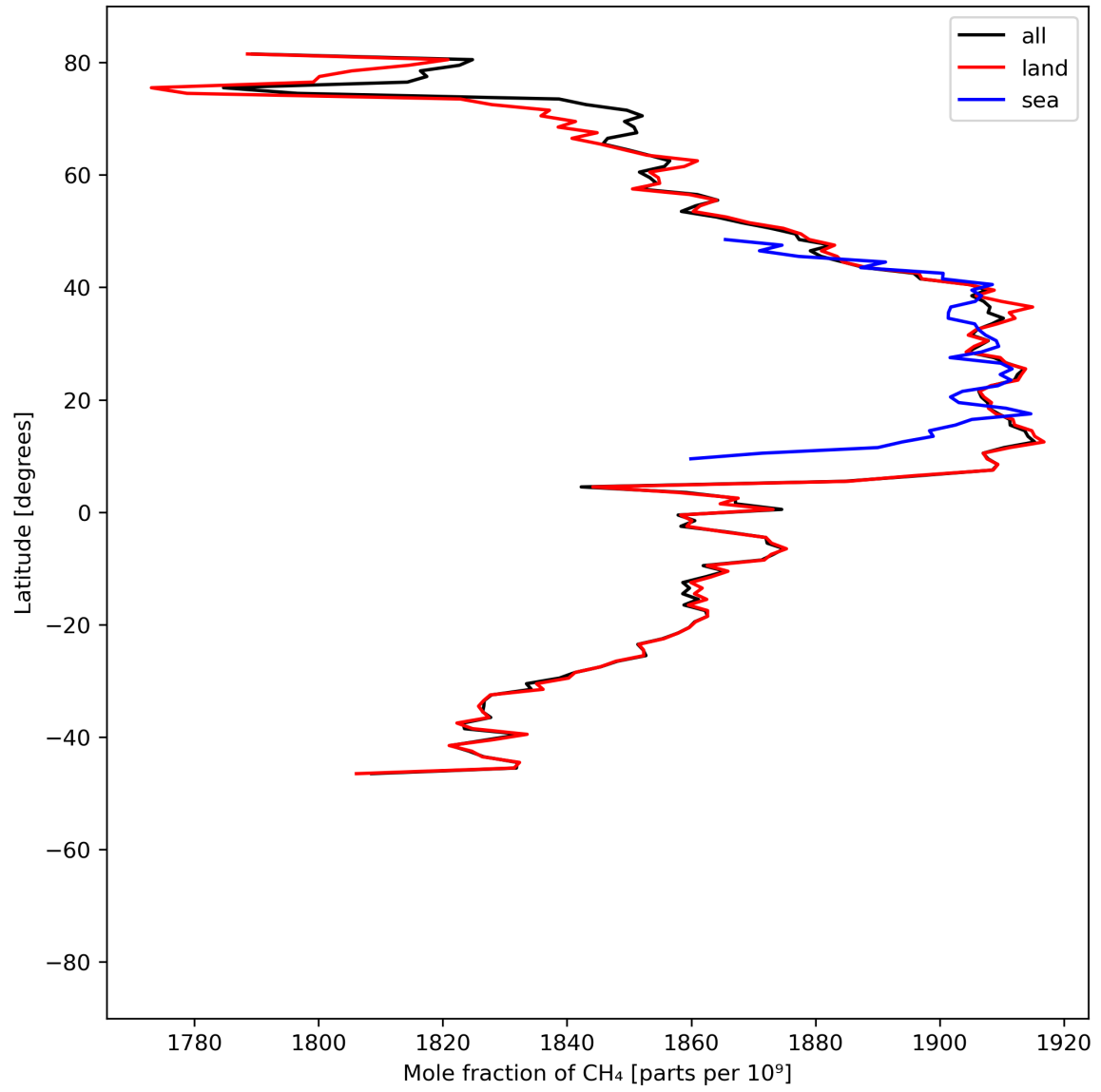
Figure 12: Zonal average of “Mole fraction of \text{CH}_4 ” for 2024-06-01 to 2024-06-03.
