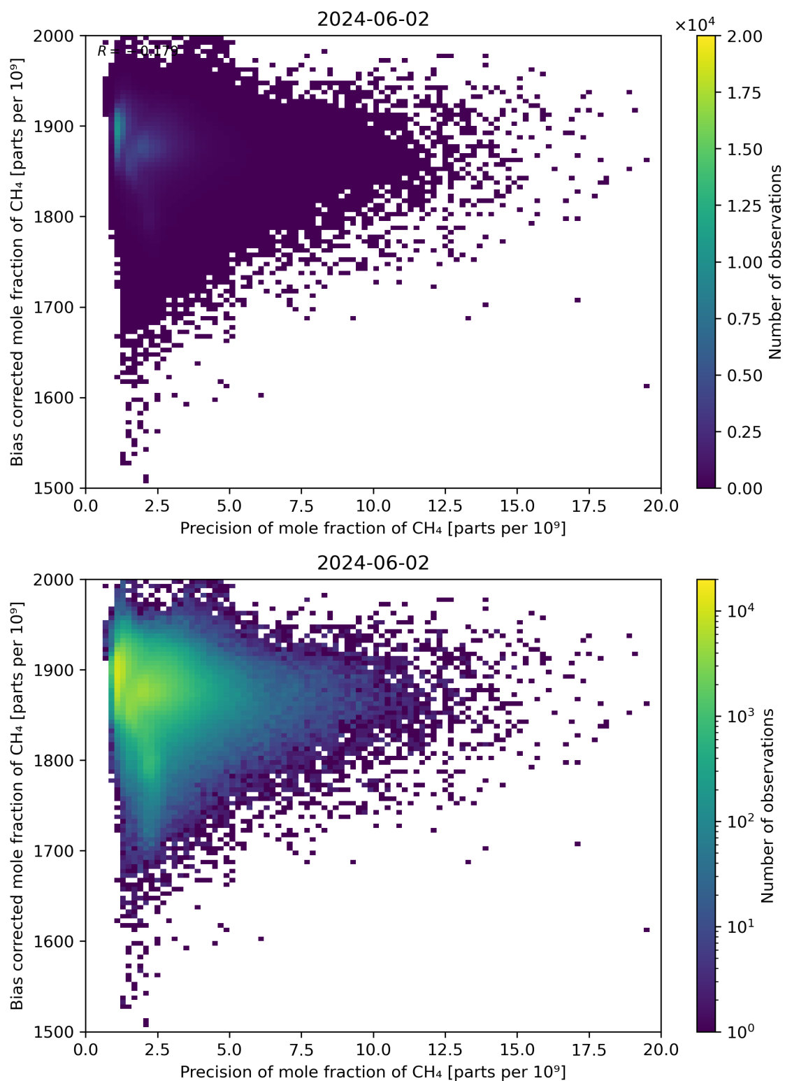
Figure 82: Scatter density plot of “Precision of mole fraction of CH 4 ” against “Bias corrected mole fraction of CH 4 ” for 2024-06-01 to 2024-06-03.
