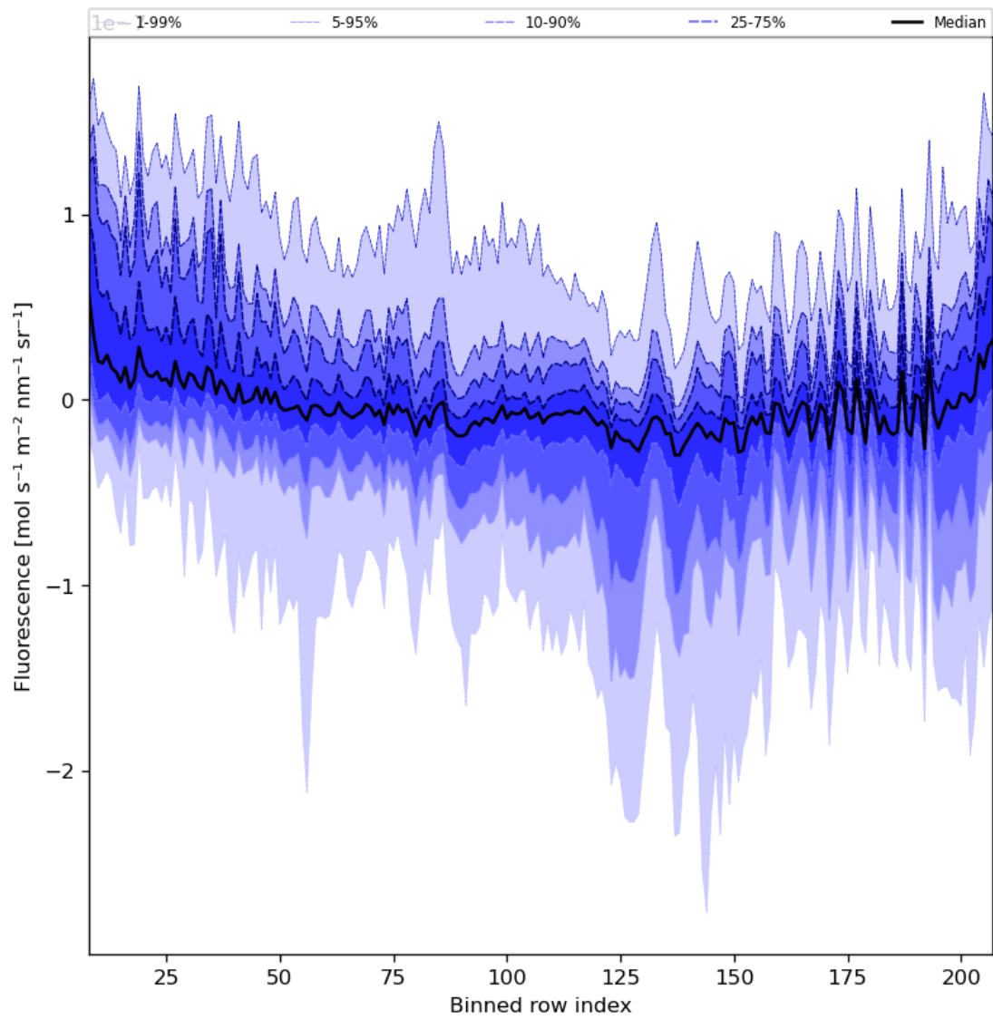
Figure 43: Along track statistics of “Fluorescence” for 2024-06-01 to 2024-06-03
