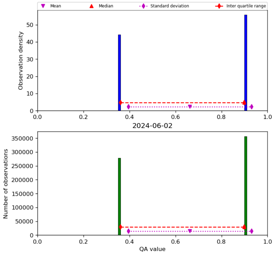
Figure 22: Histogram of “QA value” for 2024-06-01 to 2024-06-03
