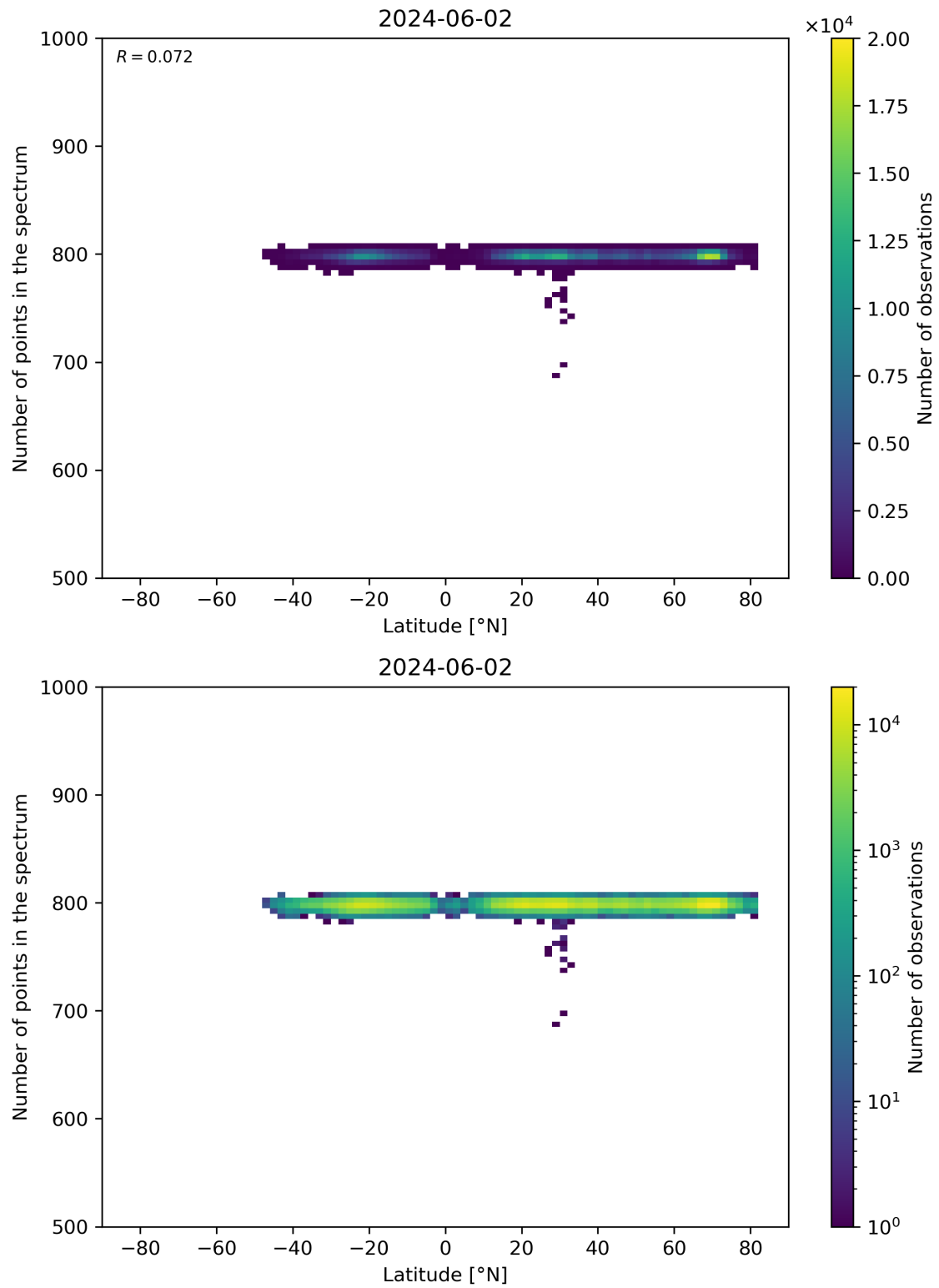
Figure 61: Scatter density plot of “Latitude” against “Number of points in the spectrum” for 2024-06-01 to 2024-06-03.
