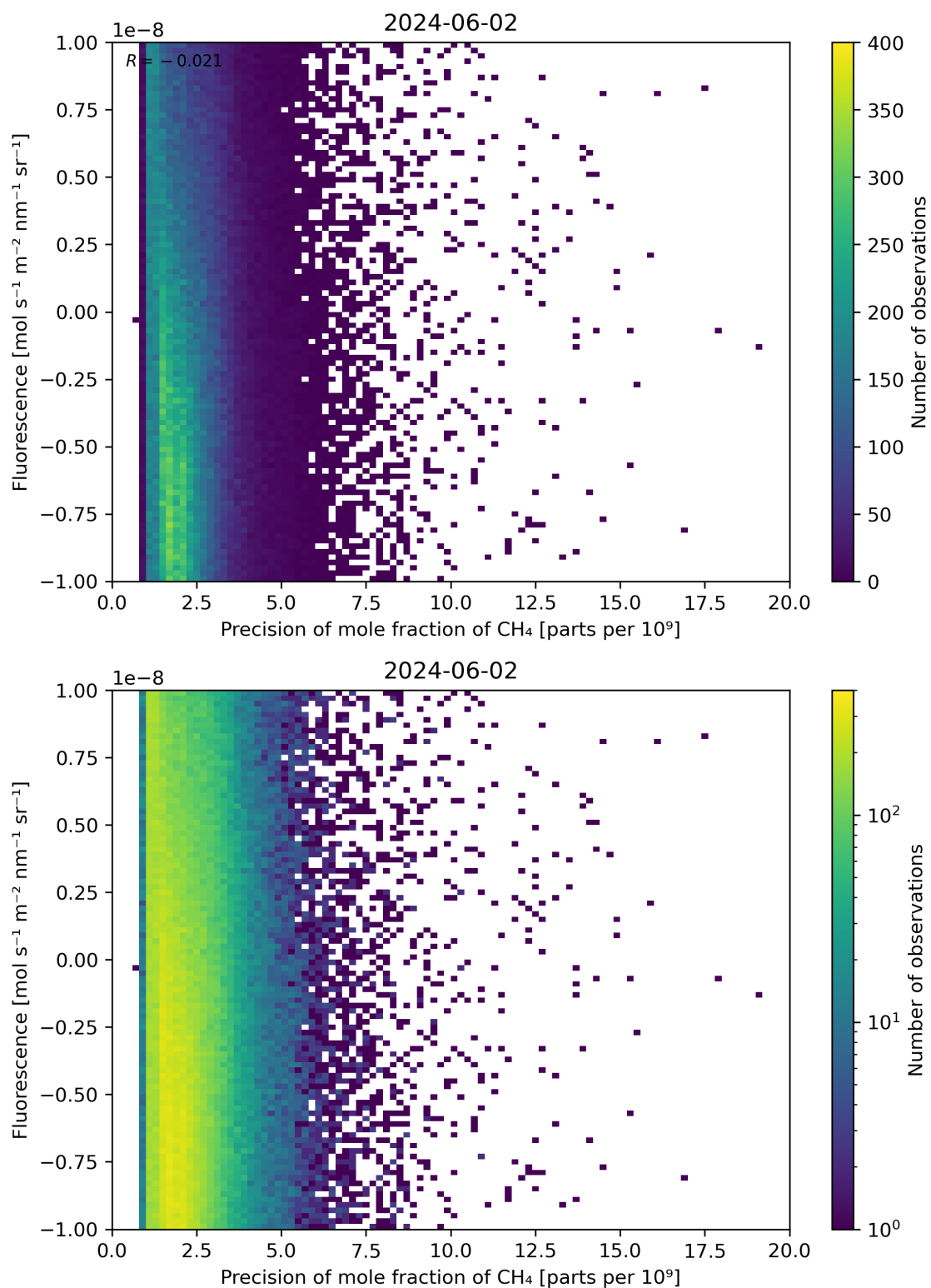
Figure 81: Scatter density plot of “Precision of mole fraction of \text{CH}_4 ” against “Fluorescence” for 2024-06-01 to 2024-06-03.
