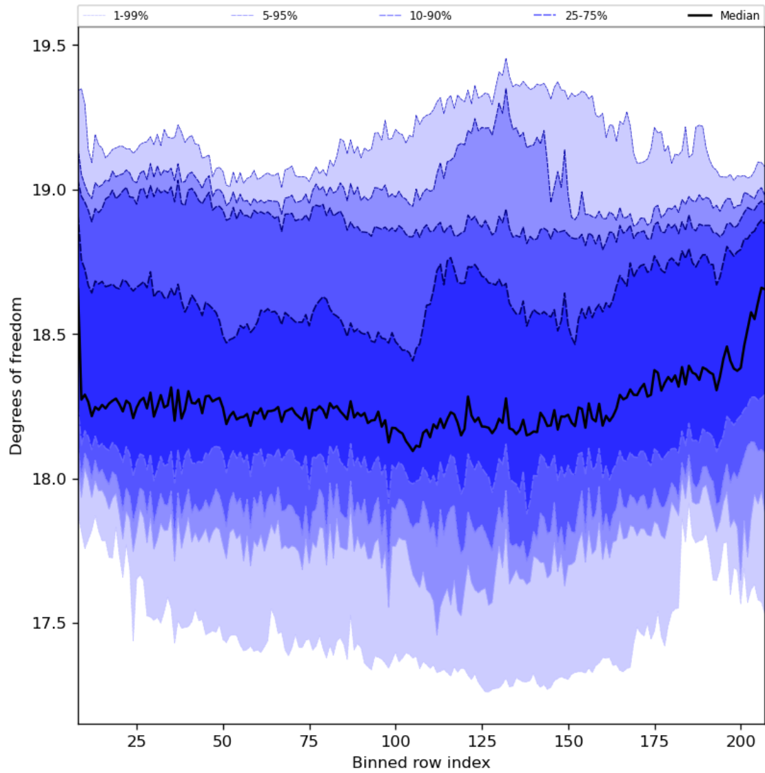
Figure 41: Along track statistics of “Degrees of freedom” for 2024-06-01 to 2024-06-03
