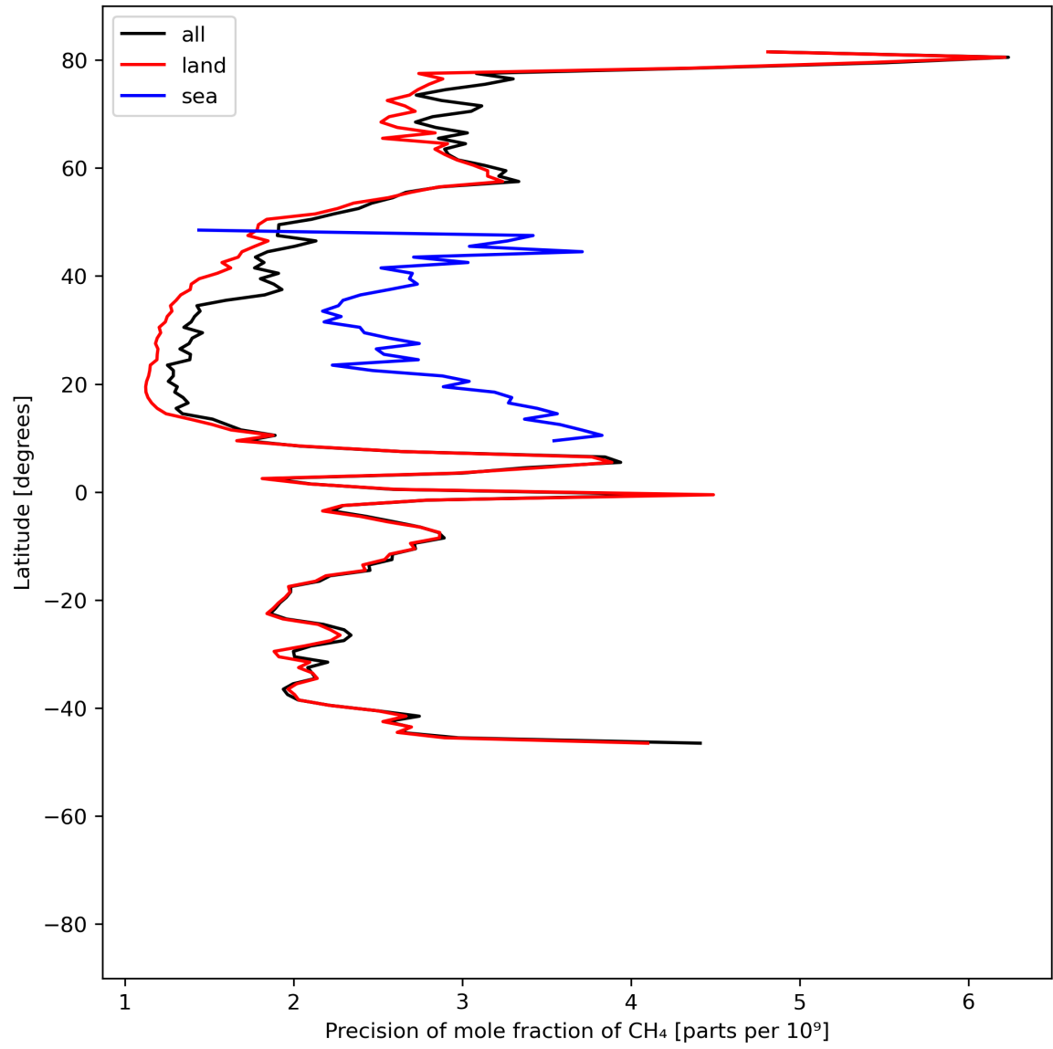
Figure 13: Zonal average of “Precision of mole fraction of CH 4 ” for 2024-06-01 to 2024-06-03.
