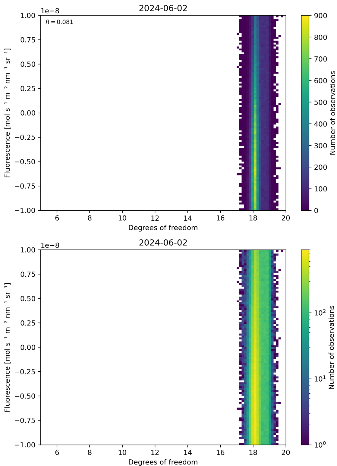
Figure 51: Scatter density plot of “Degrees of freedom” against “Fluorescence” for 2024-06-01 to 2024-06-03.
