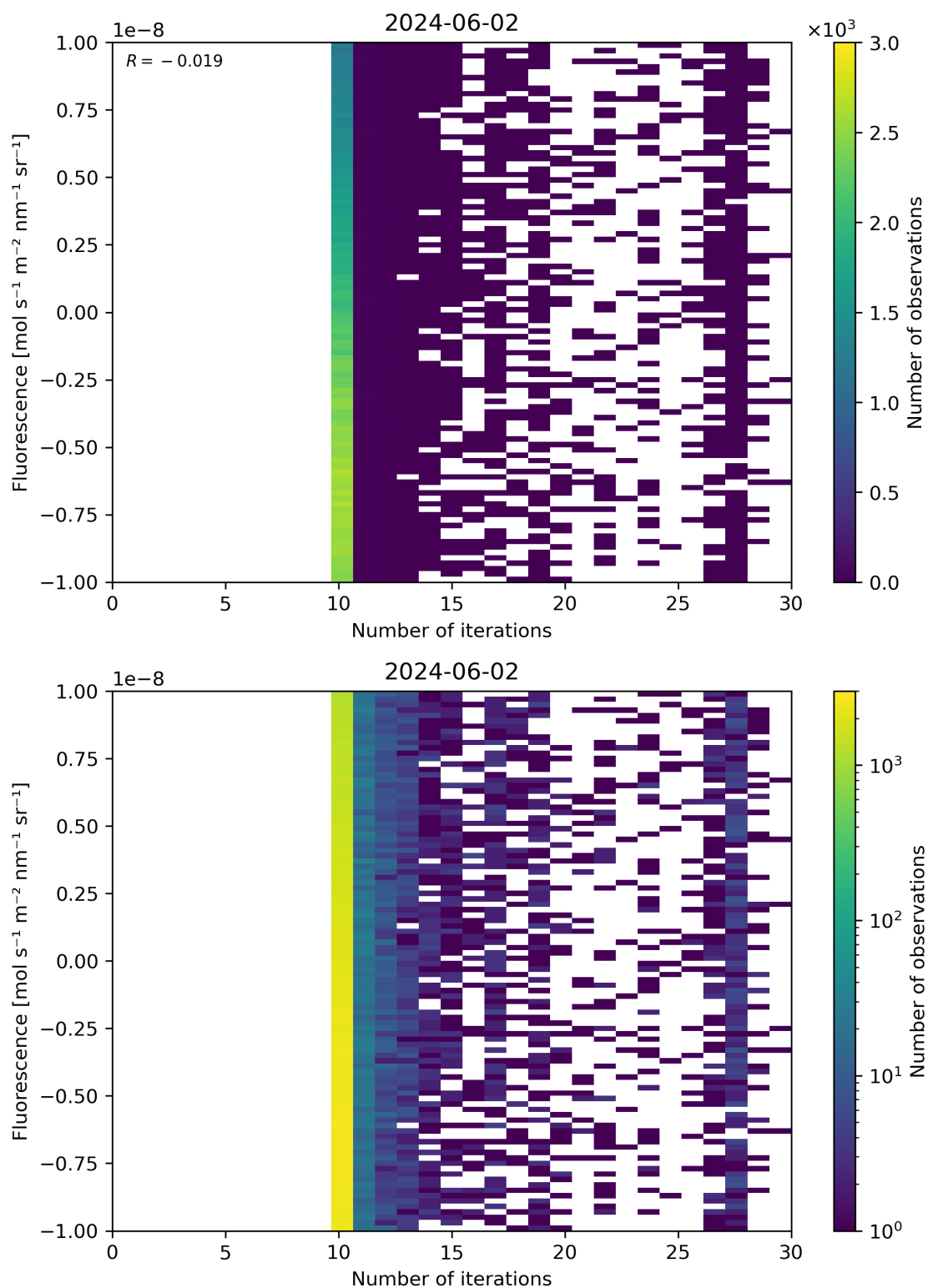
Figure 87: Scatter density plot of “Number of iterations” against “Fluorescence” for 2024-06-01 to 2024-06-03.
