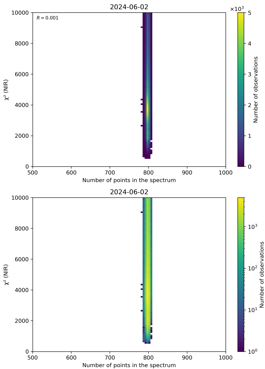
Figure 88: Scatter density plot of “Number of points in the spectrum” against “ \chi^2 (NIR)” for 2024-06-01 to 2024-06-03.
