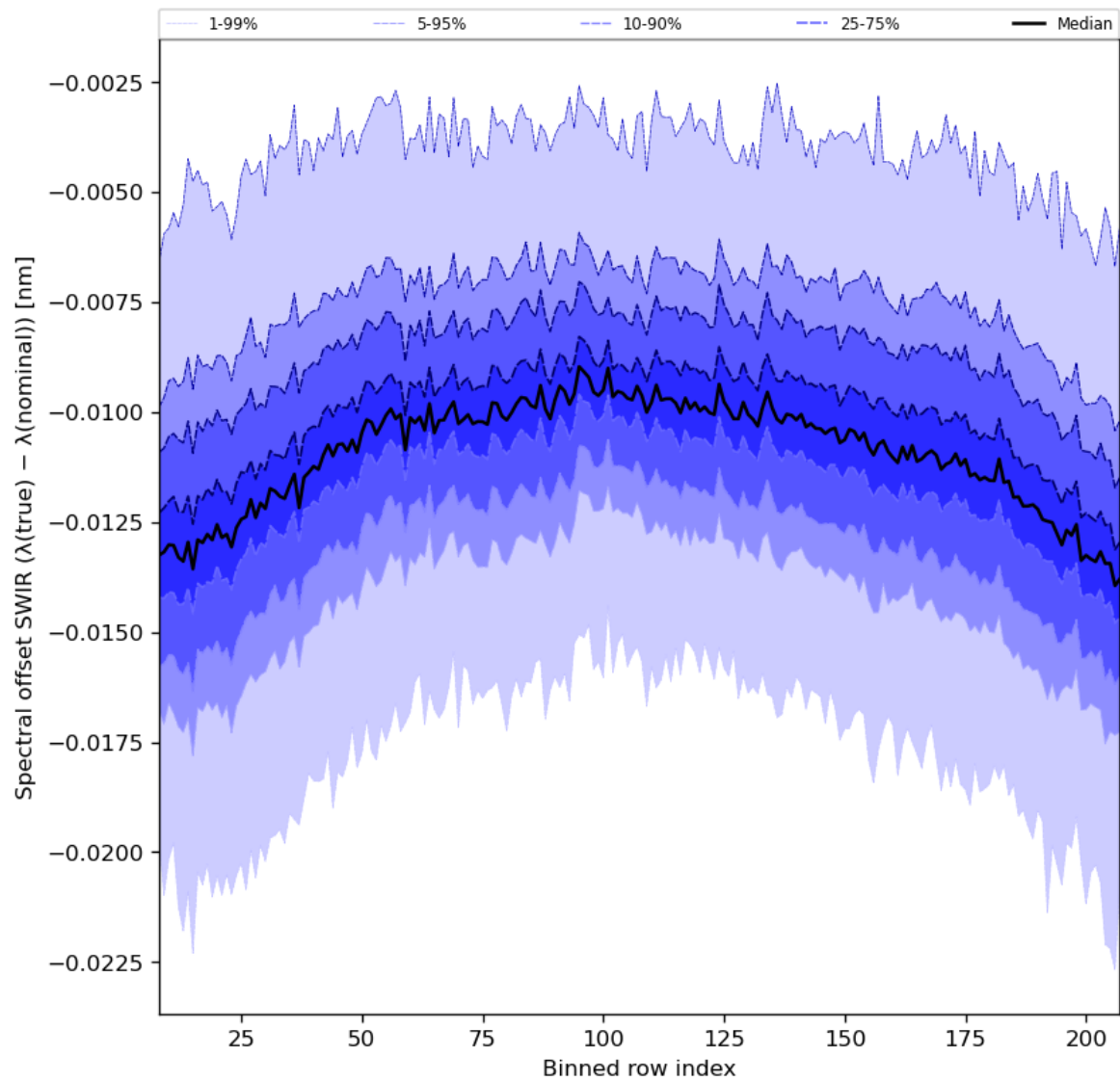
Figure 38: Along track statistics of “Spectral offset SWIR ( \lambda(\text{true}) - \lambda(\text{nominal}) )” for 2024-06-01 to 2024-06-03
