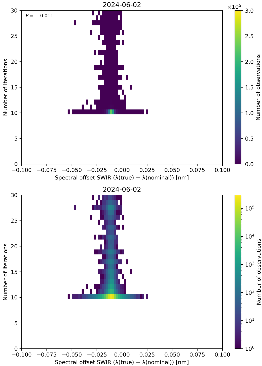
Figure 121: Scatter density plot of “Spectral offset SWIR ( \lambda(\text{true}) - \lambda(\text{nominal}) )” against “Number of iterations” for 2024-06-01 to 2024-06-03.
