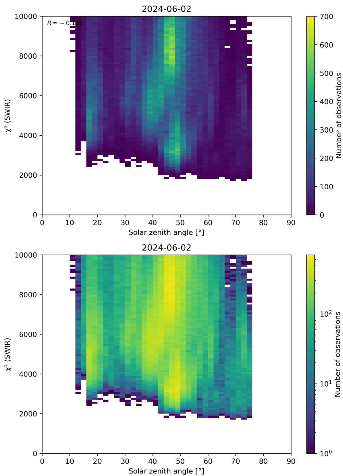
Figure 95: Scatter density plot of “Solar zenith angle” against “ \chi^2 (SWIR)” for 2024-06-01 to 2024-06-03.
