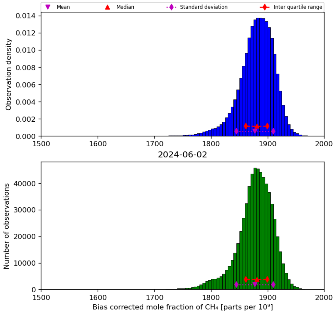
Figure 25: Histogram of “Bias corrected mole fraction of CH 4 ” for 2024-06-01 to 2024-06-03
