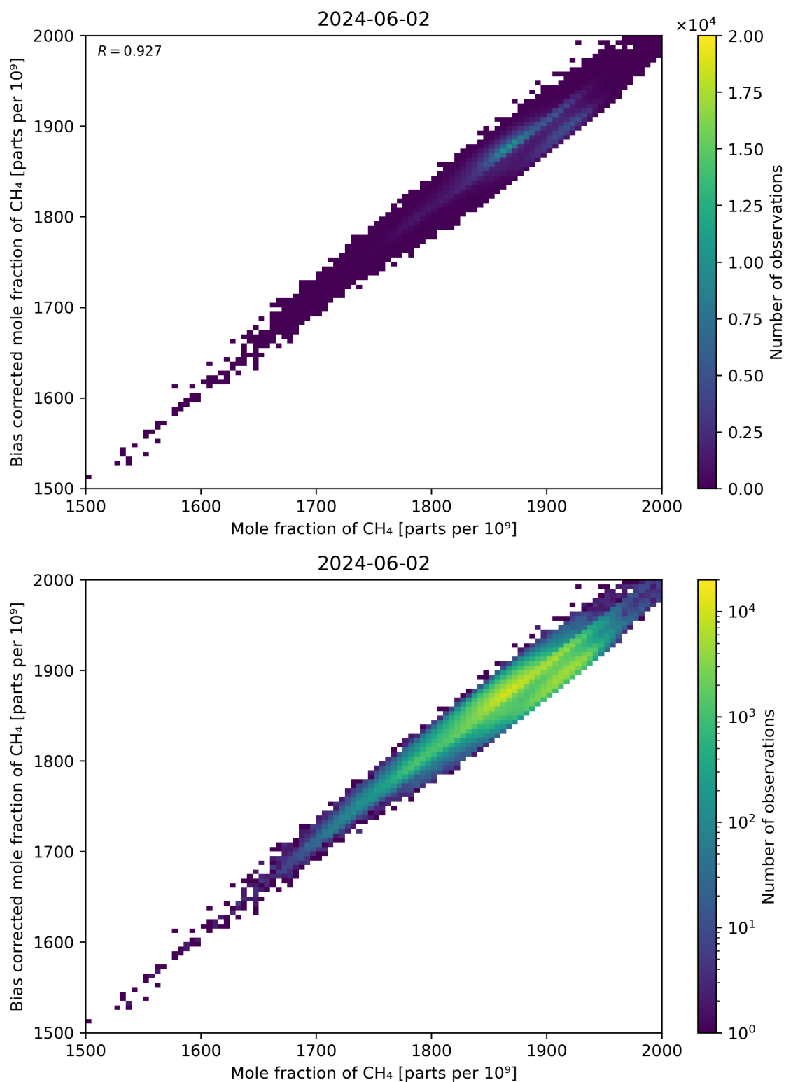
Figure 74: Scatter density plot of “Mole fraction of CH 4 ” against “Bias corrected mole fraction of CH 4 ” for 2024-06-01 to 2024-06-03.
