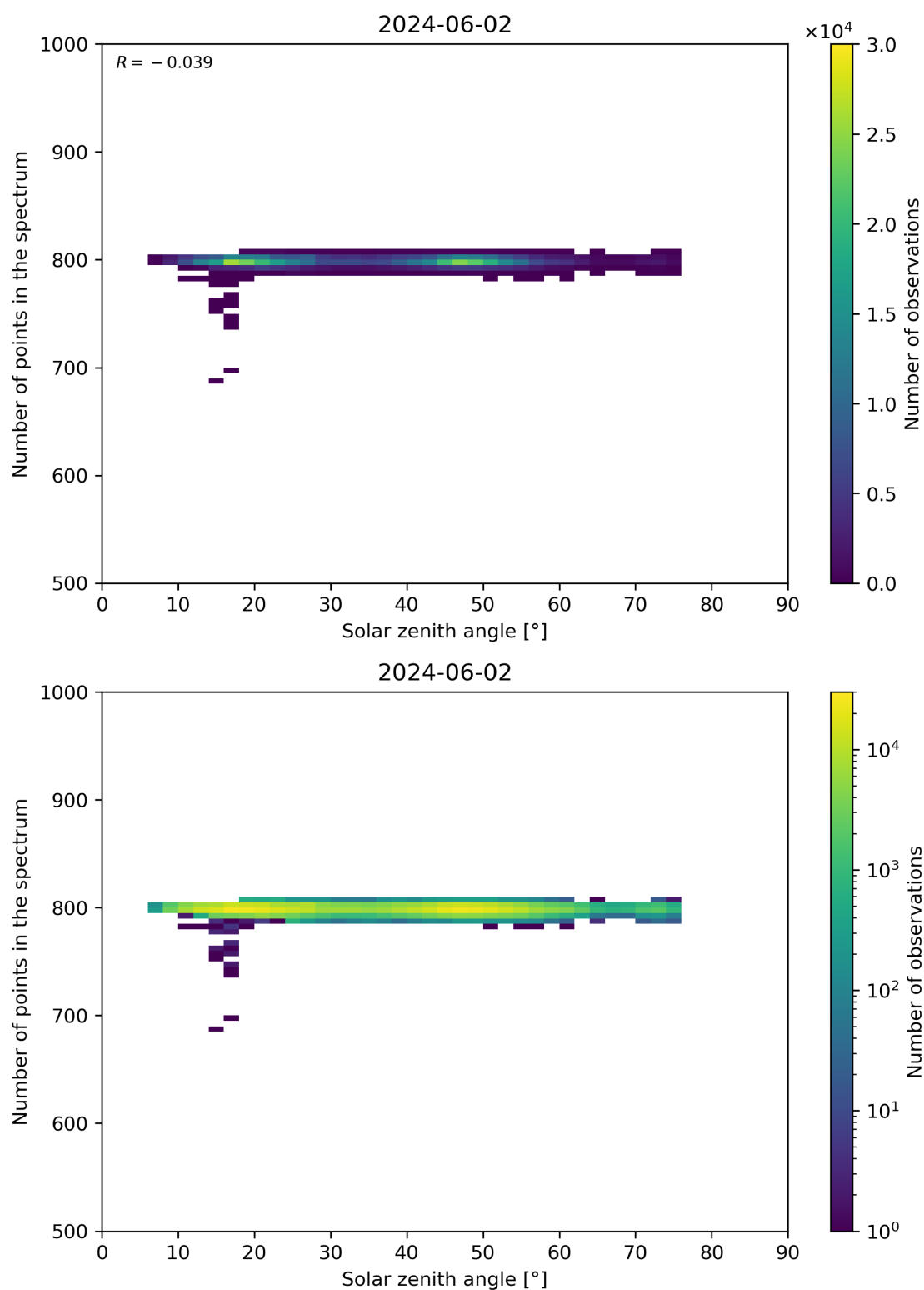
Figure 103: Scatter density plot of “Solar zenith angle” against “Number of points in the spectrum” for 2024-06-01 to 2024-06-03.
