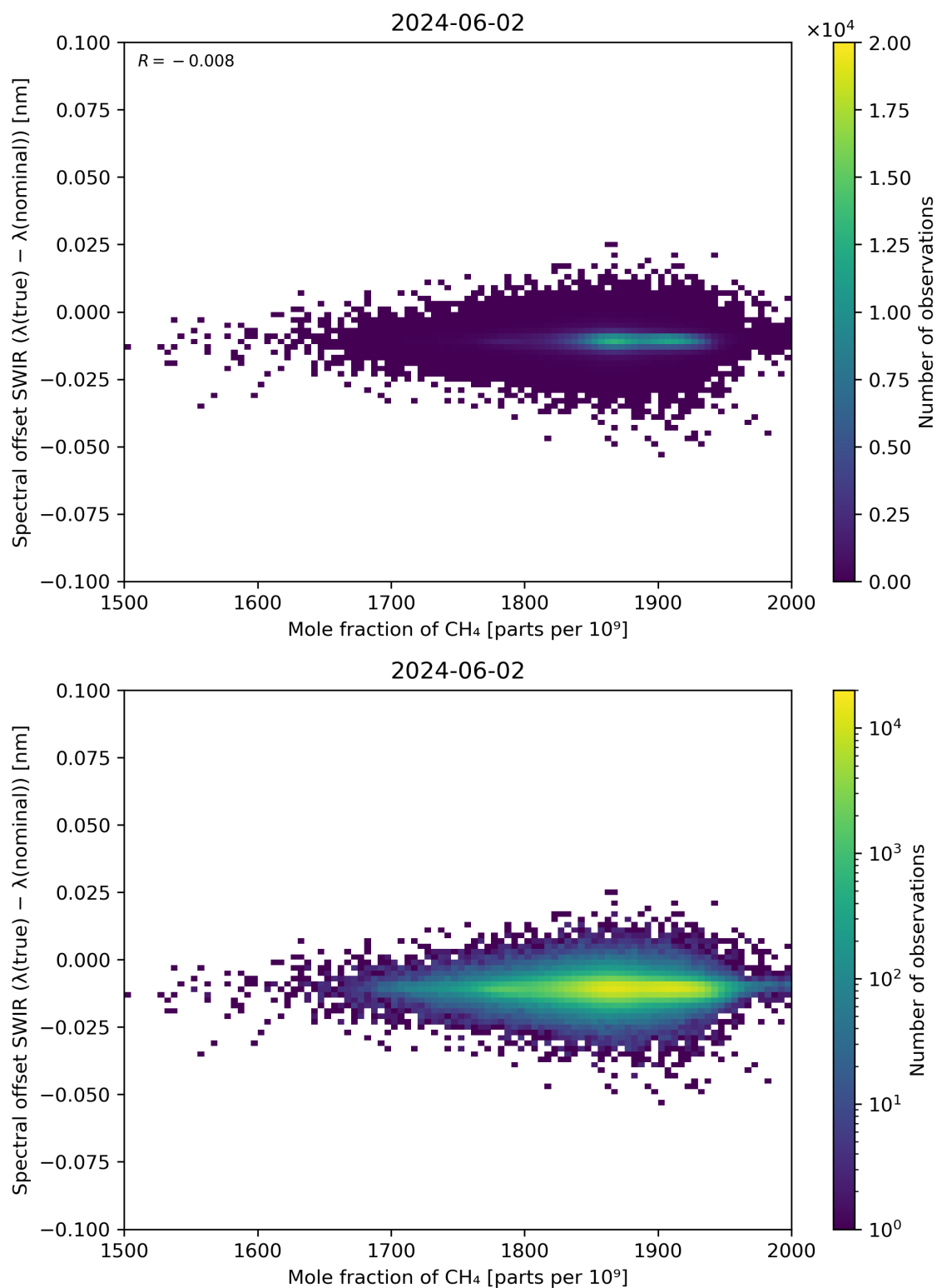
Figure 86: Scatter density plot of “Mole fraction of CH 4 ” against “Spectral offset SWIR ( \lambda(\text{true}) - \lambda(\text{nominal}) )” for 2024-06-01 to 2024-06-03.
