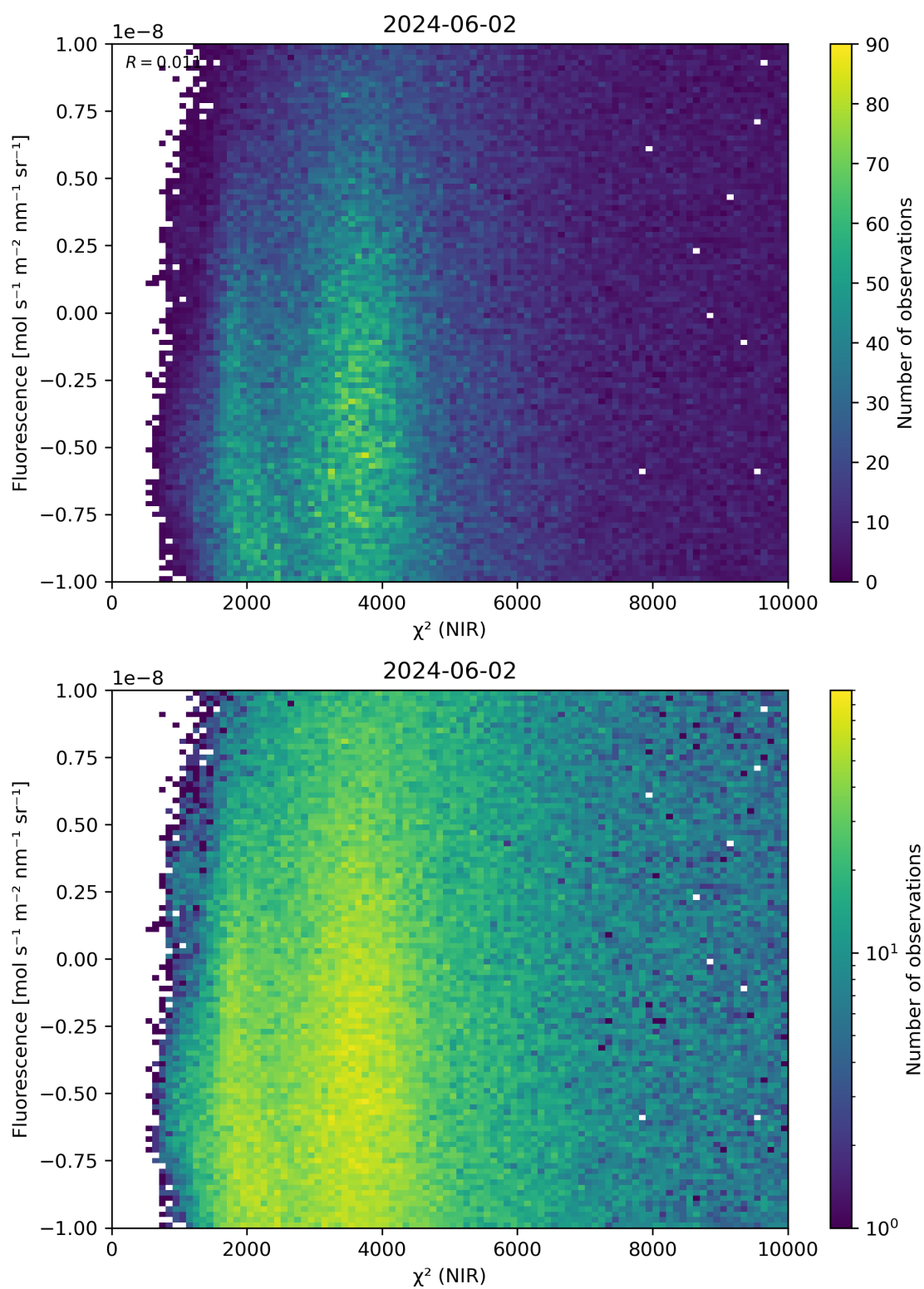
Figure 45: Scatter density plot of “ \chi^2 (NIR)” against “Fluorescence” for 2024-06-01 to 2024-06-03.
