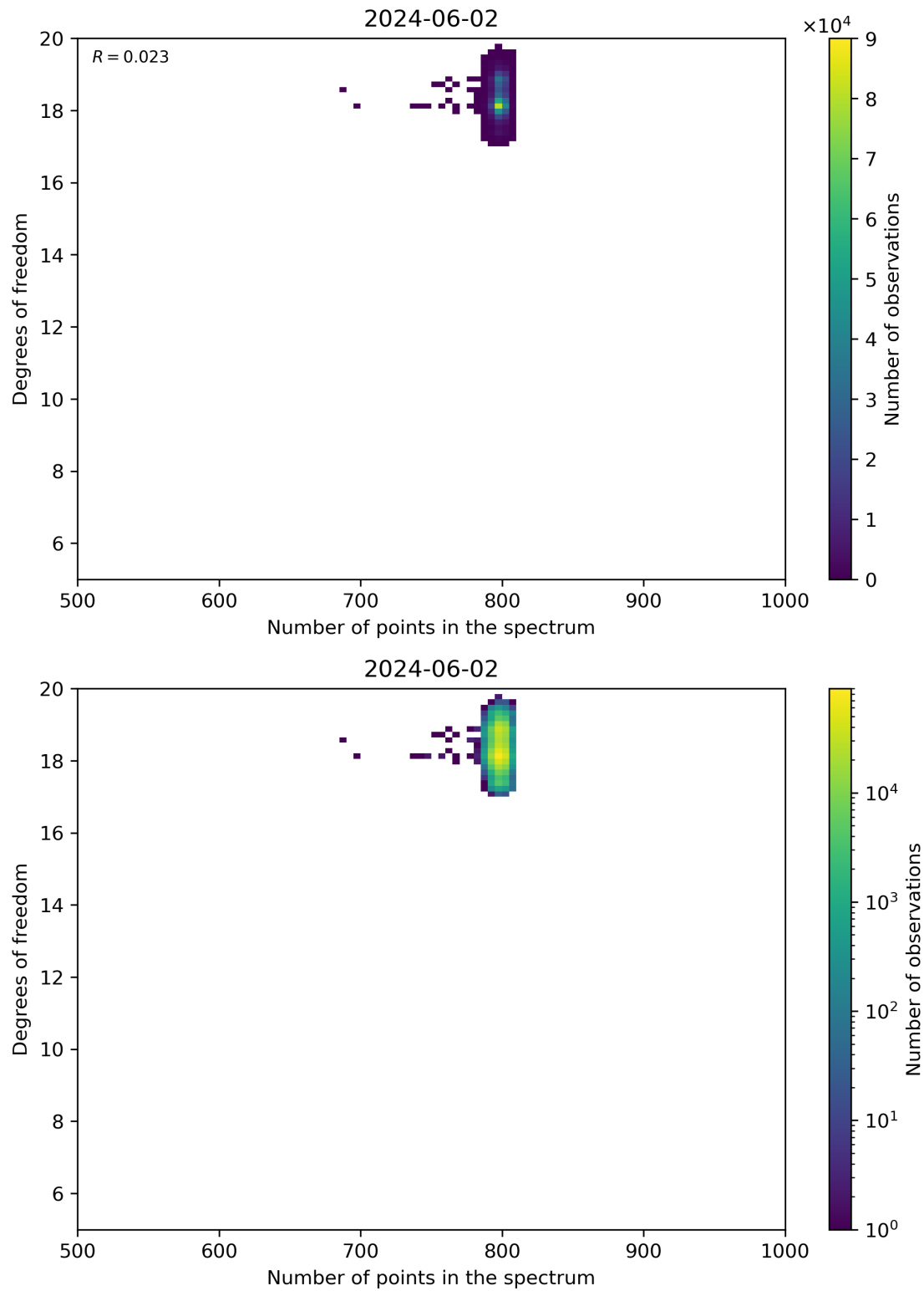
Figure 90: Scatter density plot of “Number of points in the spectrum” against “Degrees of freedom” for 2024-06-01 to 2024-06-03.
