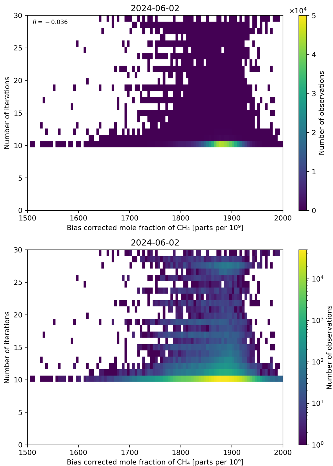
Figure 67: Scatter density plot of “Bias corrected mole fraction of \text{CH}_4 ” against “Number of iterations” for 2024-06-01 to 2024-06-03.
