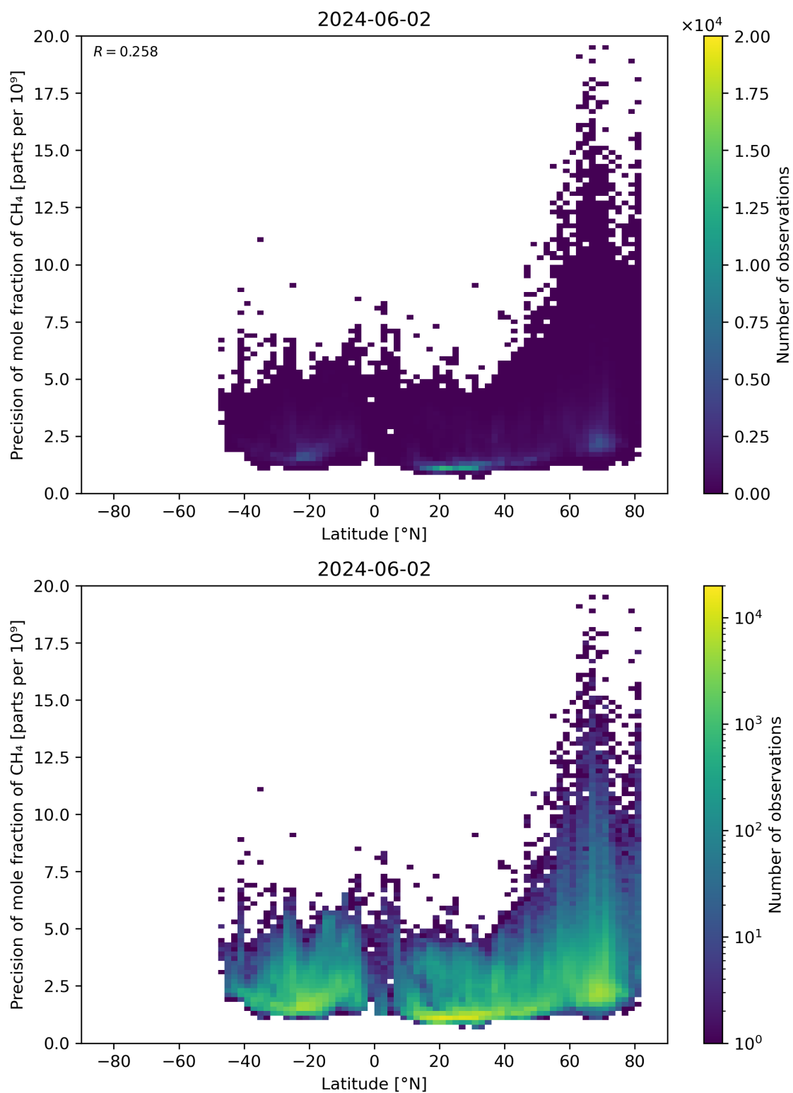
Figure 59: Scatter density plot of “Latitude” against “Precision of mole fraction of CH 4 ” for 2024-06-01 to 2024-06-03.
