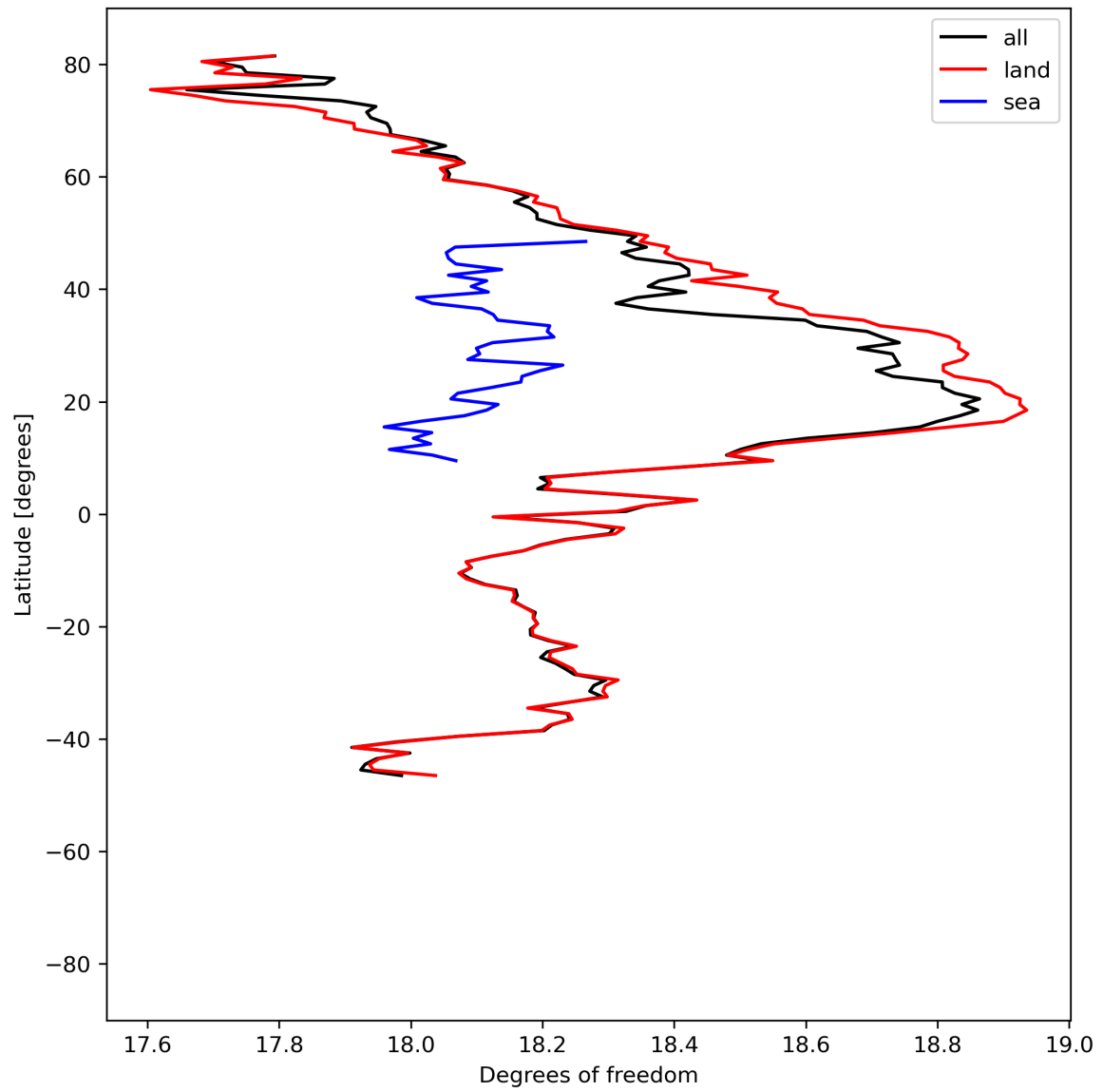
Figure 19: Zonal average of “Degrees of freedom” for 2024-06-01 to 2024-06-03.
