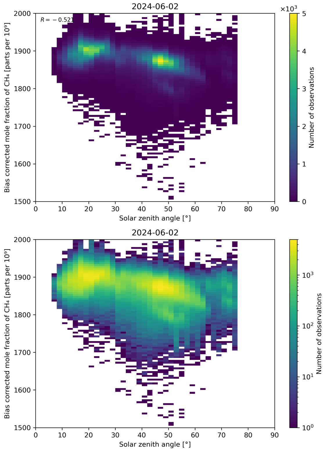
Figure 100: Scatter density plot of “Solar zenith angle” against “Bias corrected mole fraction of CH 4 ” for 2024-06-01 to 2024-06-03.
