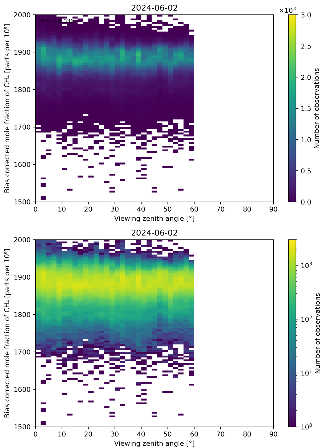
Figure 111: Scatter density plot of “Viewing zenith angle” against “Bias corrected mole fraction of CH 4 ” for 2024-06-01 to 2024-06-03.
