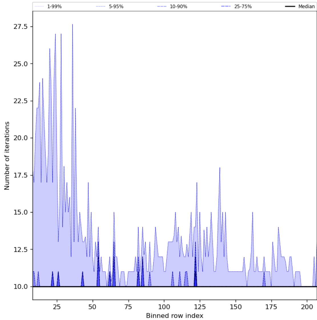
Figure 42: Along track statistics of “Number of iterations” for 2024-06-01 to 2024-06-03
