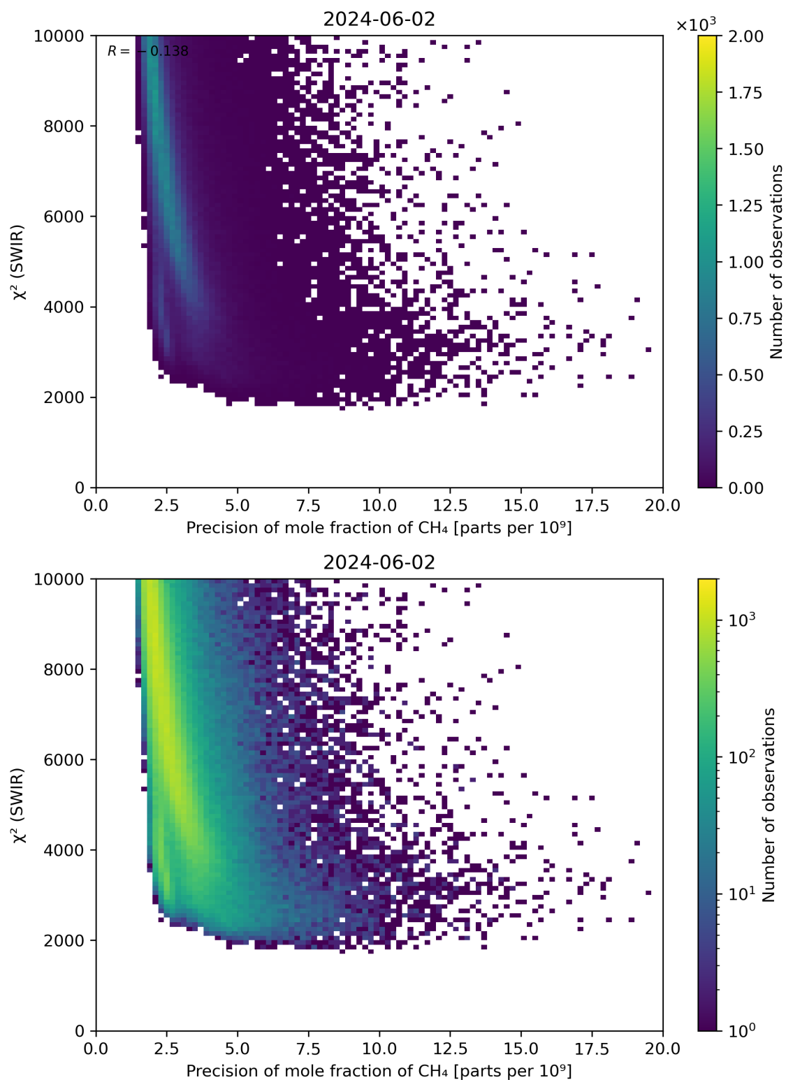
Figure 79: Scatter density plot of “Precision of mole fraction of \text{CH}_4 ” against “ \chi^2 (SWIR)” for 2024-06-01 to 2024-06-03.
