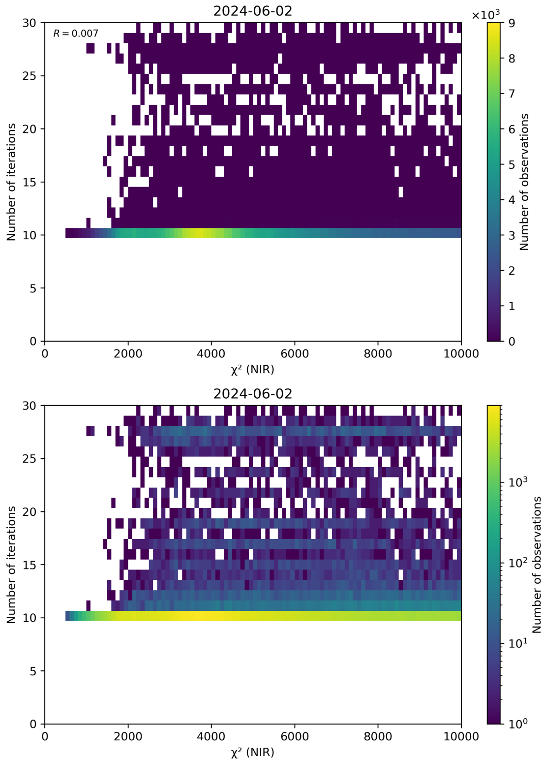
Figure 46: Scatter density plot of “ \chi^2 (NIR)” against “Number of iterations” for 2024-06-01 to 2024-06-03.
