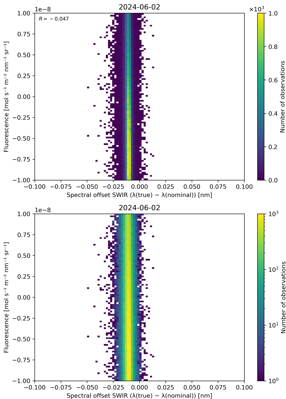
Figure 120: Scatter density plot of “Spectral offset SWIR ( \lambda(\text{true}) - \lambda(\text{nominal}) )” against “Fluorescence” for 2024-06-01 to 2024-06-03.
