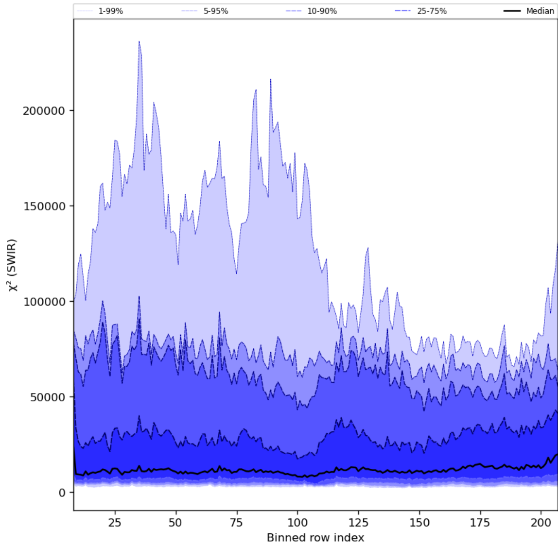
Figure 39: Along track statistics of “ \chi^2 (SWIR)” for 2024-06-01 to 2024-06-03
