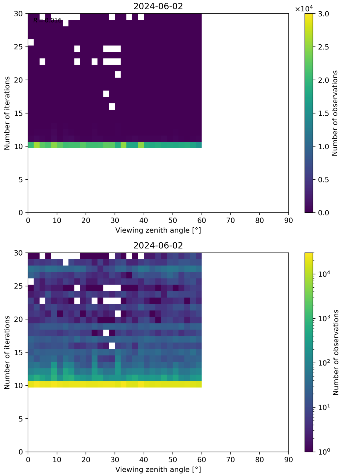
Figure 113: Scatter density plot of “Viewing zenith angle” against “Number of iterations” for 2024-06-01 to 2024-06-03.
