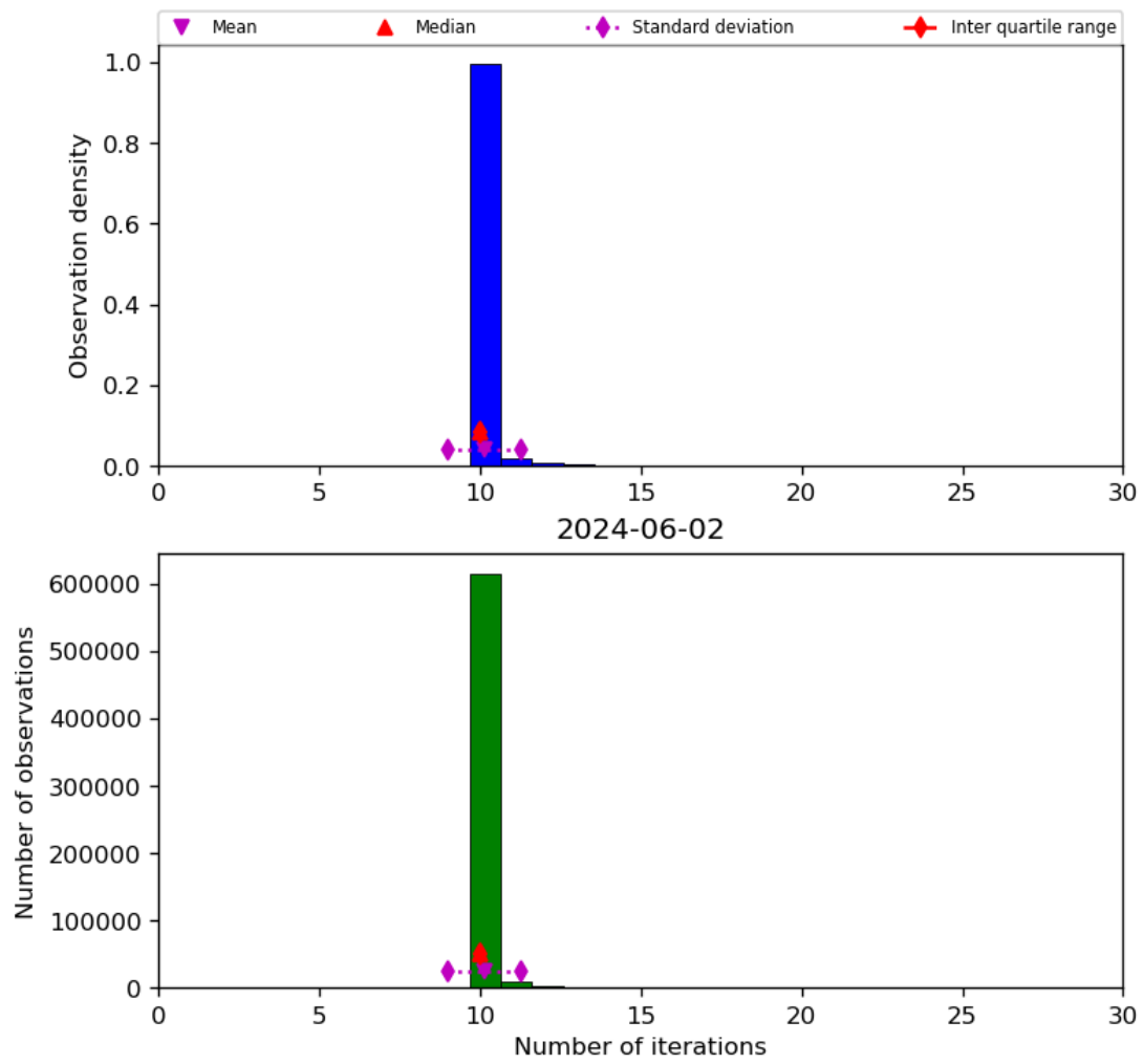
Figure 31: Histogram of “Number of iterations” for 2024-06-01 to 2024-06-03
