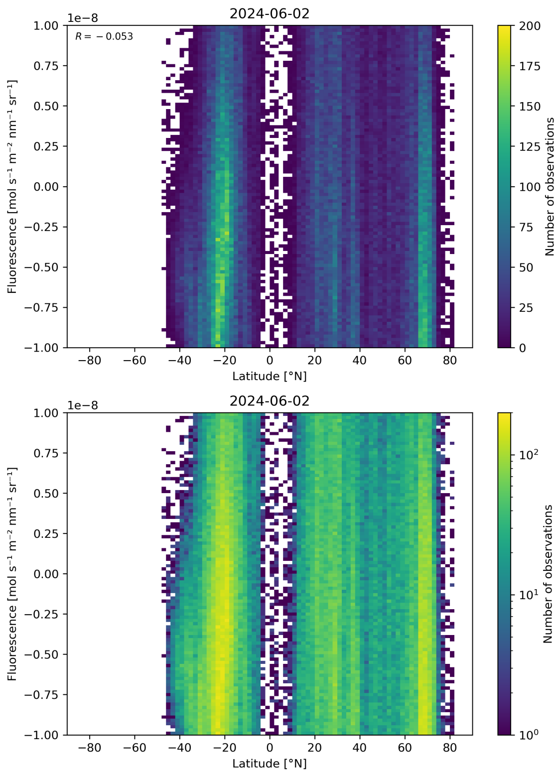
Figure 56: Scatter density plot of “Latitude” against “Fluorescence” for 2024-06-01 to 2024-06-03.
