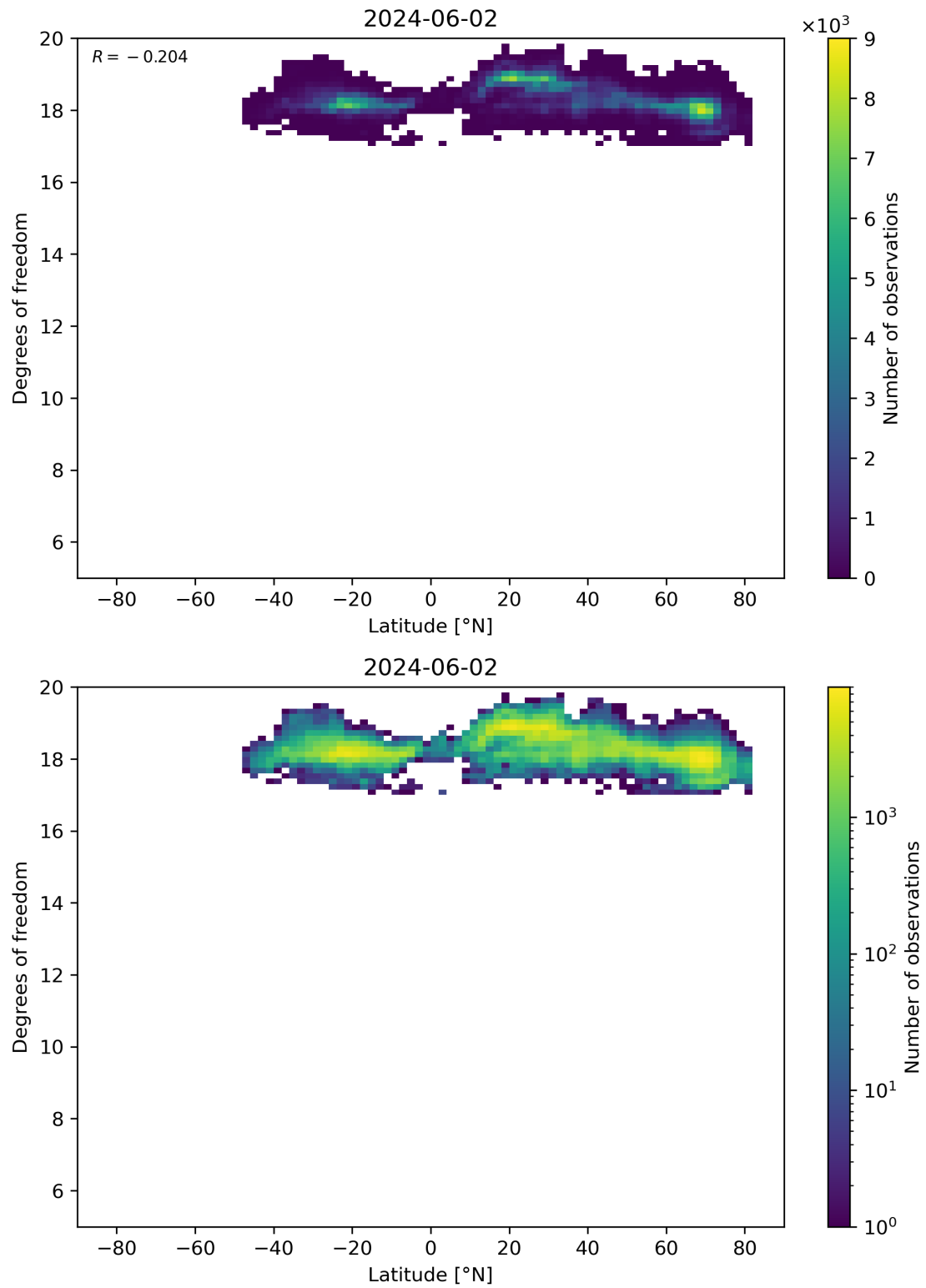
Figure 55: Scatter density plot of “Latitude” against “Degrees of freedom” for 2024-06-01 to 2024-06-03.
