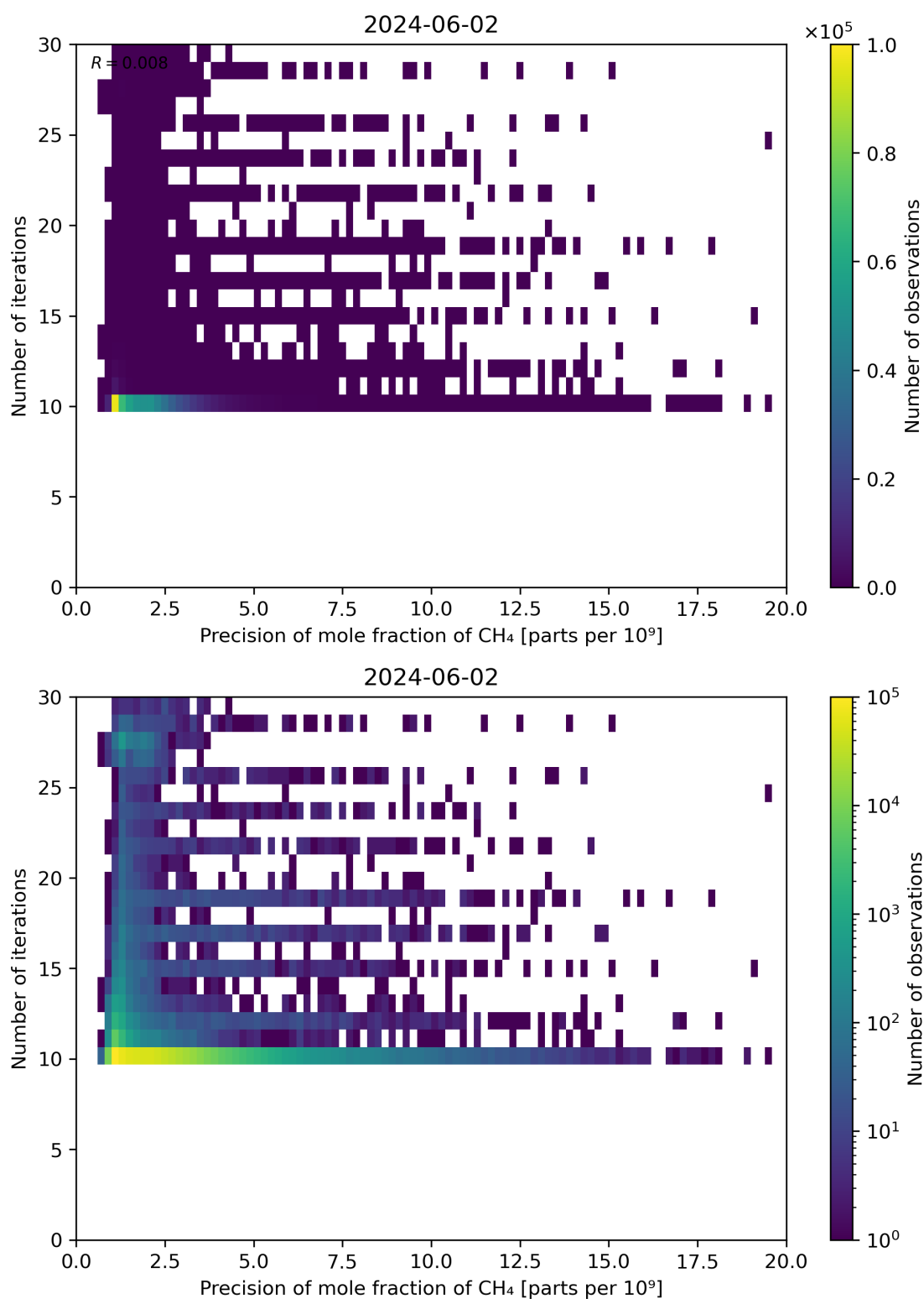
Figure 83: Scatter density plot of “Precision of mole fraction of CH 4 ” against “Number of iterations” for 2024-06-01 to 2024-06-03.
