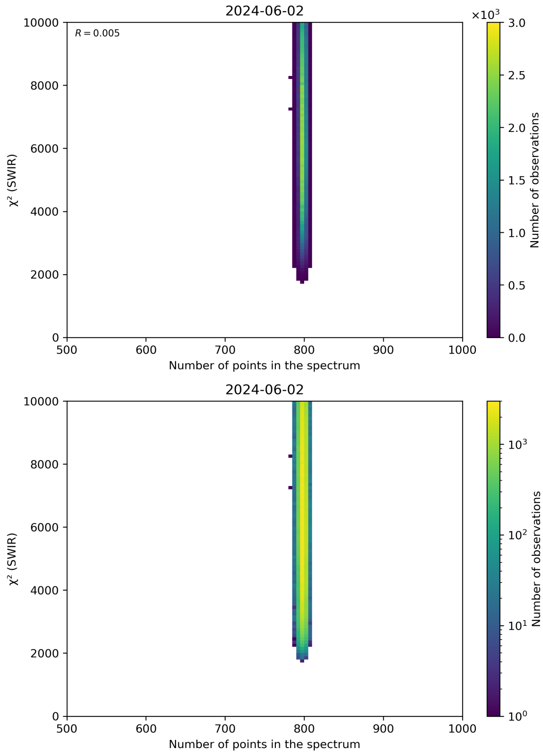
Figure 89: Scatter density plot of “Number of points in the spectrum” against “ \chi^2 (SWIR)” for 2024-06-01 to 2024-06-03.
