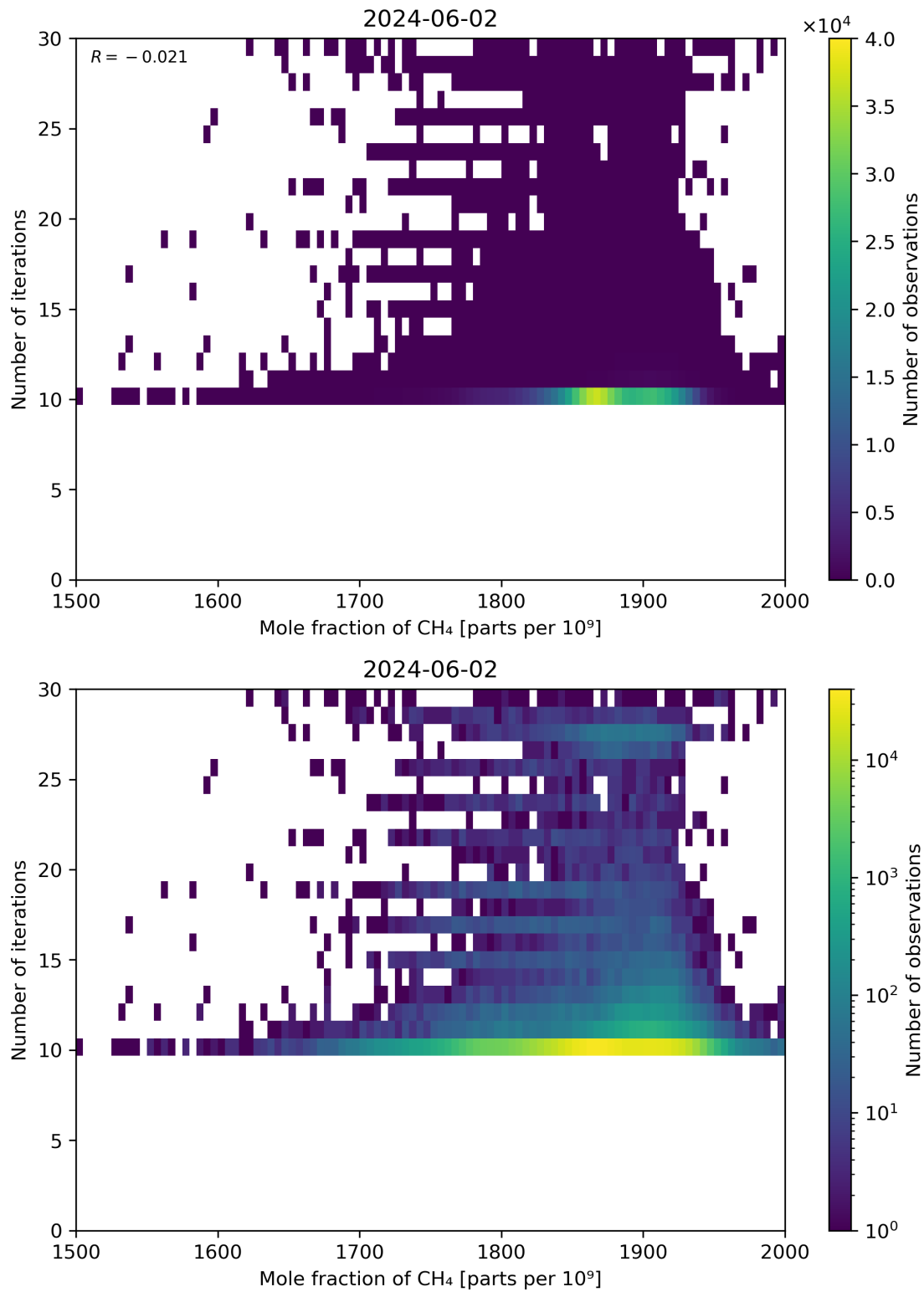
Figure 76: Scatter density plot of “Mole fraction of CH 4 ” against “Number of iterations” for 2024-06-01 to 2024-06-03.
