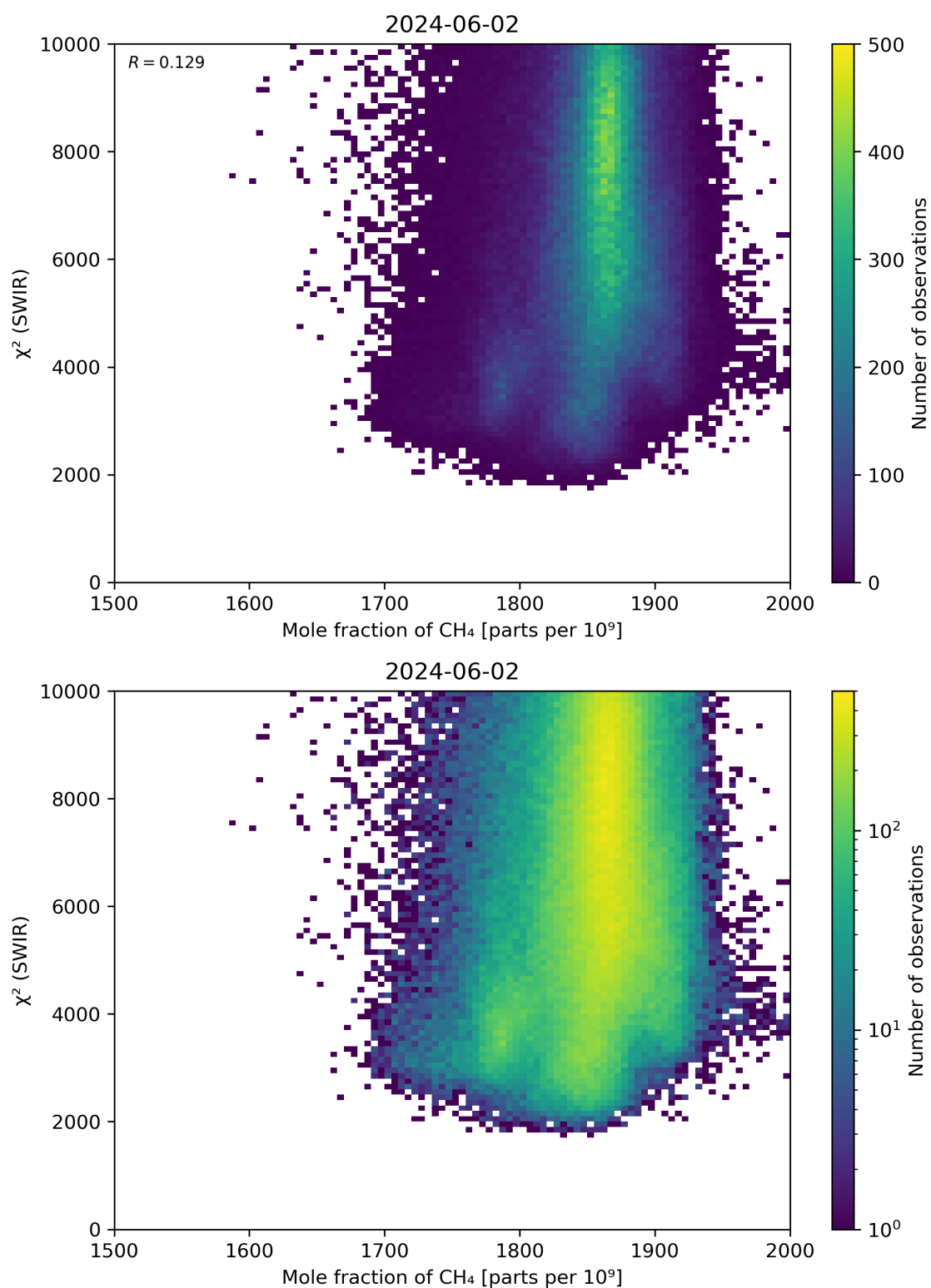
Figure 71: Scatter density plot of “Mole fraction of \text{CH}_4 ” against “ \chi^2 (SWIR)” for 2024-06-01 to 2024-06-03.
