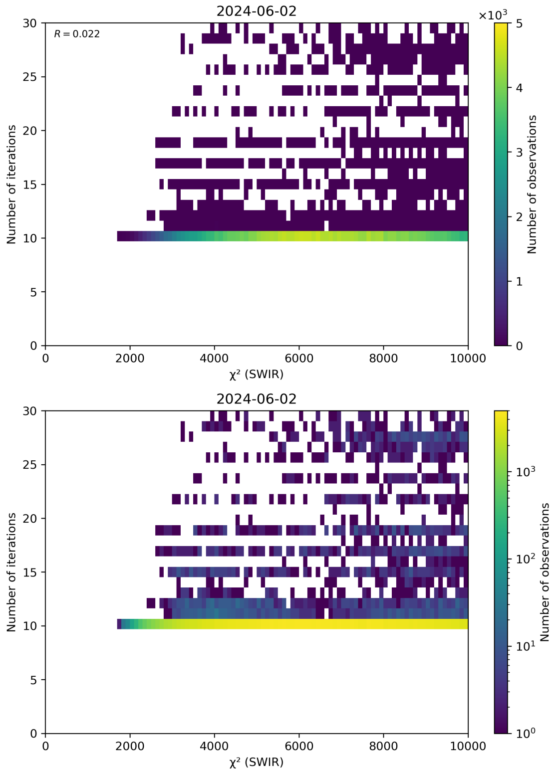
Figure 50: Scatter density plot of “ \chi^2 (SWIR)” against “Number of iterations” for 2024-06-01 to 2024-06-03.
