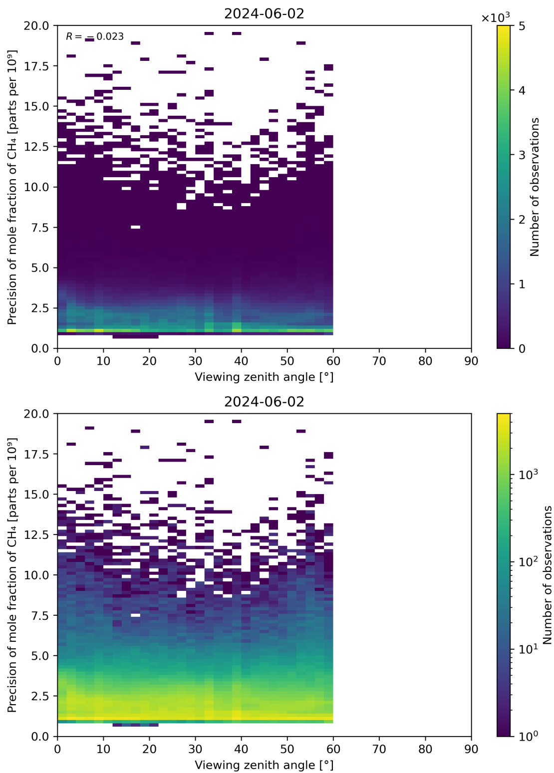
Figure 112: Scatter density plot of “Viewing zenith angle” against “Precision of mole fraction of \text{CH}_4 ” for 2024-06-01 to 2024-06-03.
