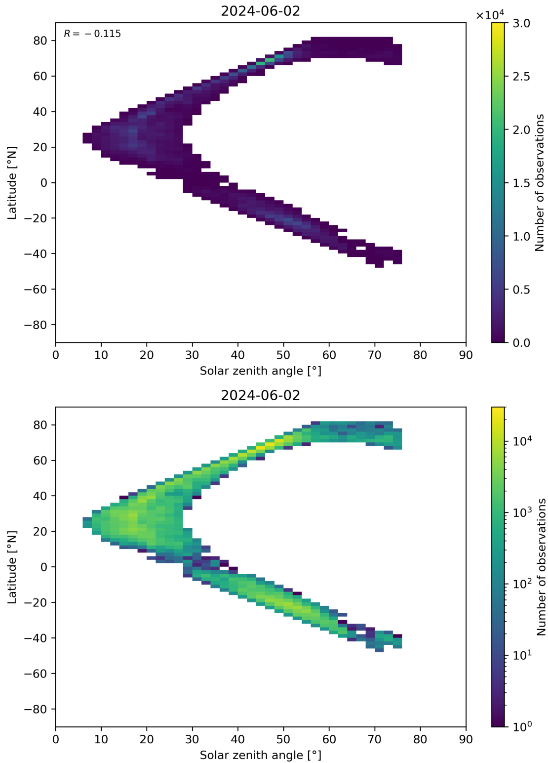
Figure 98: Scatter density plot of “Solar zenith angle” against “Latitude” for 2024-06-01 to 2024-06-03.
