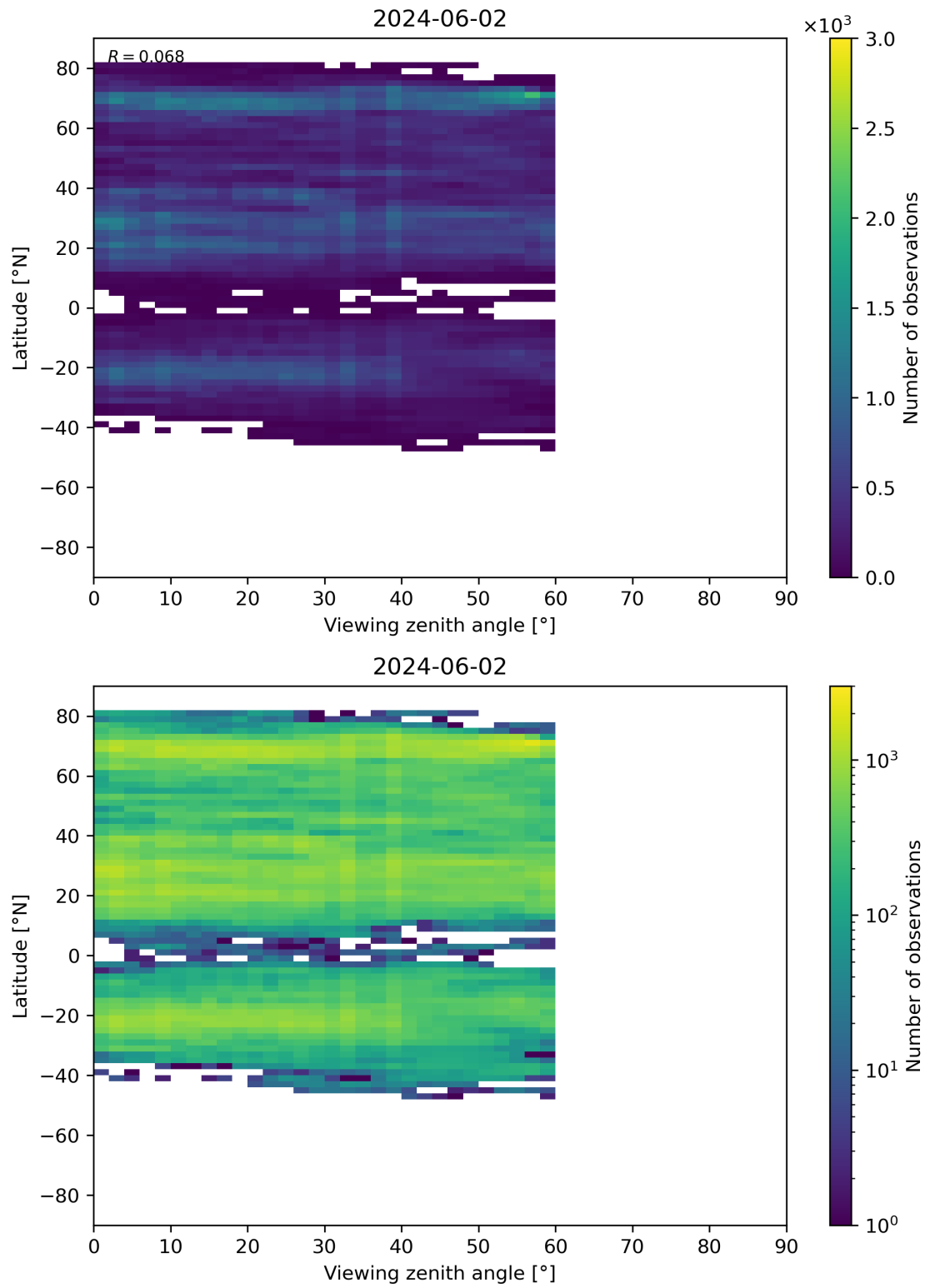
Figure 109: Scatter density plot of “Viewing zenith angle” against “Latitude” for 2024-06-01 to 2024-06-03.
