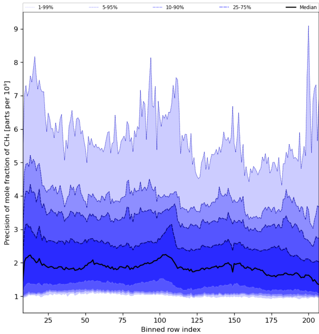
Figure 35: Along track statistics of “Precision of mole fraction of CH 4 ” for 2024-06-01 to 2024-06-03
