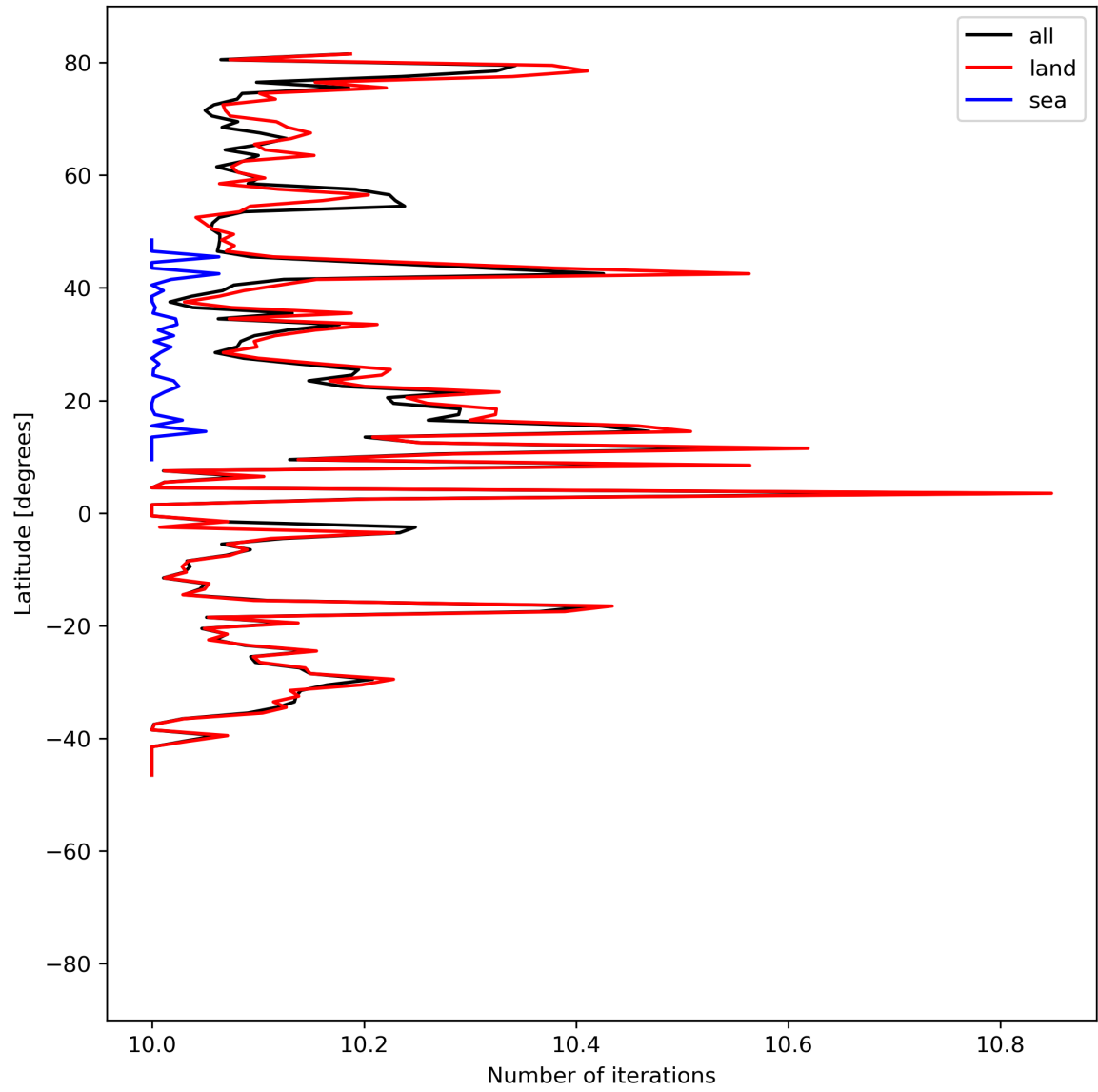
Figure 20: Zonal average of “Number of iterations” for 2024-06-01 to 2024-06-03.
