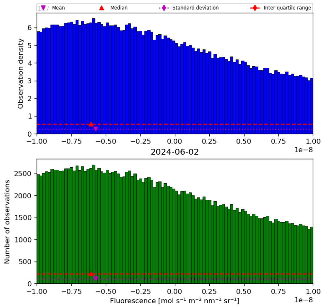
Figure 32: Histogram of “Fluorescence” for 2024-06-01 to 2024-06-03
