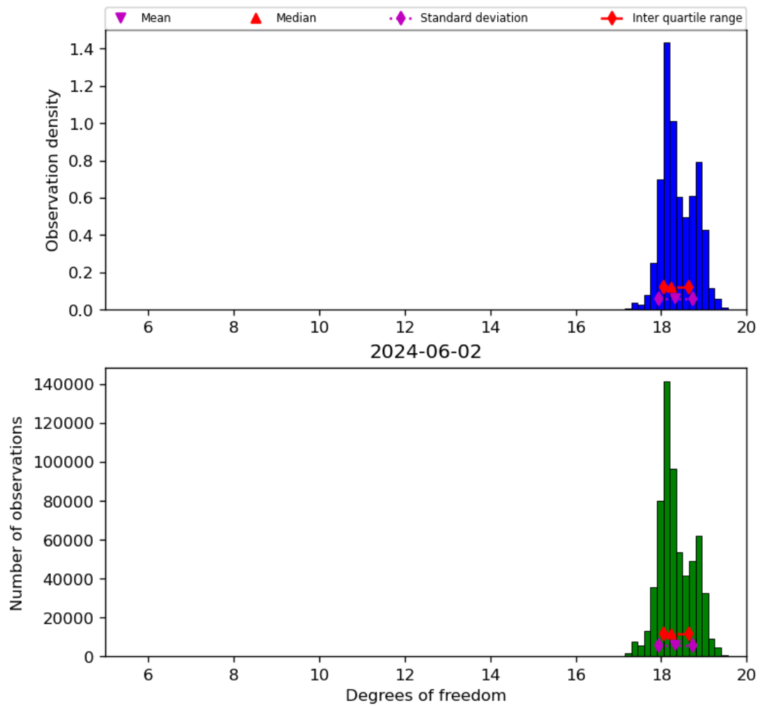
Figure 30: Histogram of “Degrees of freedom” for 2024-06-01 to 2024-06-03
