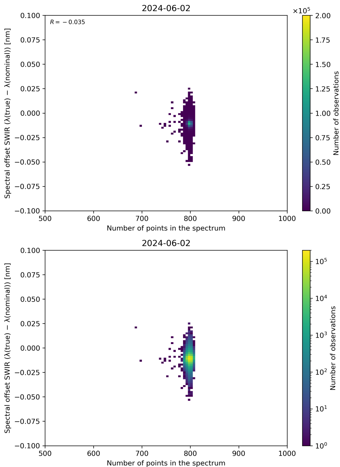
Figure 93: Scatter density plot of “Number of points in the spectrum” against “Spectral offset SWIR ( \lambda(\text{true}) - \lambda(\text{nominal}) )” for 2024-06-01 to 2024-06-03.
