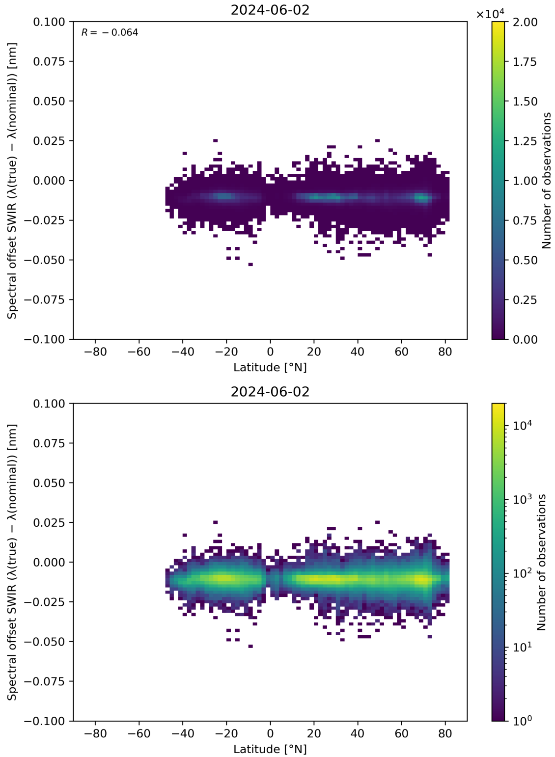
Figure 62: Scatter density plot of “Latitude” against “Spectral offset SWIR ( \lambda(\text{true}) - \lambda(\text{nominal}) )” for 2024-06-01 to 2024-06-03.
