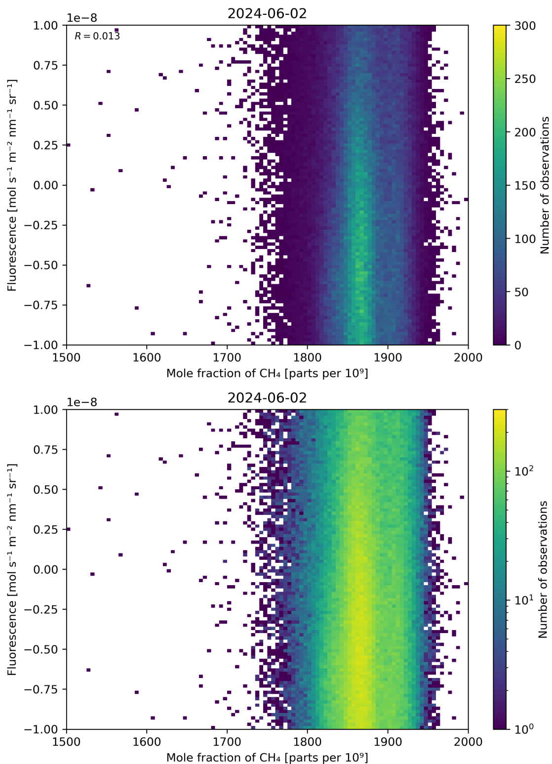
Figure 73: Scatter density plot of “Mole fraction of \text{CH}_4 ” against “Fluorescence” for 2024-06-01 to 2024-06-03.
