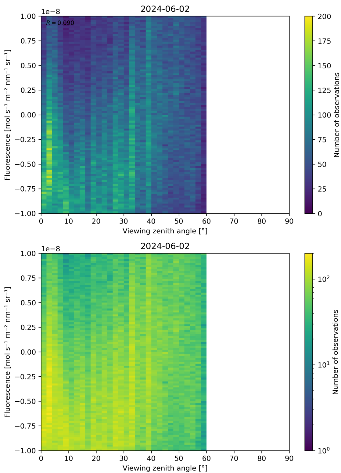
Figure 108: Scatter density plot of “Viewing zenith angle” against “Fluorescence” for 2024-06-01 to 2024-06-03.
