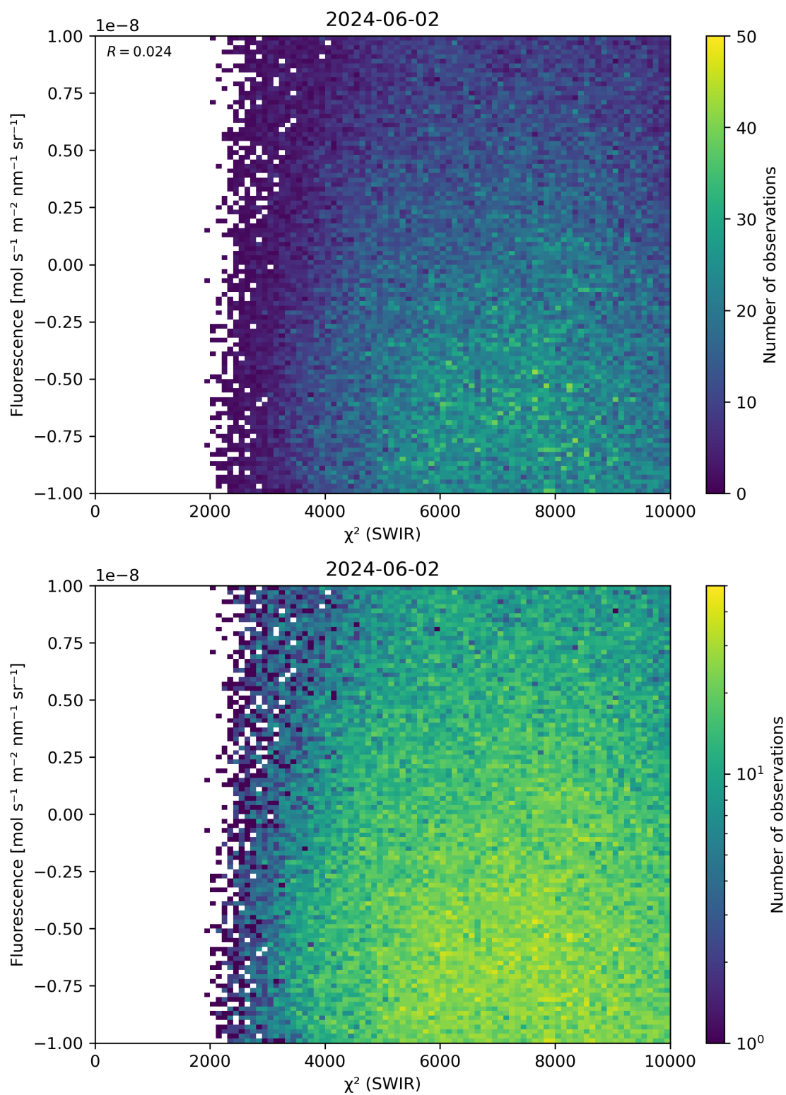
Figure 49: Scatter density plot of “ \chi^2 (SWIR)” against “Fluorescence” for 2024-06-01 to 2024-06-03.
