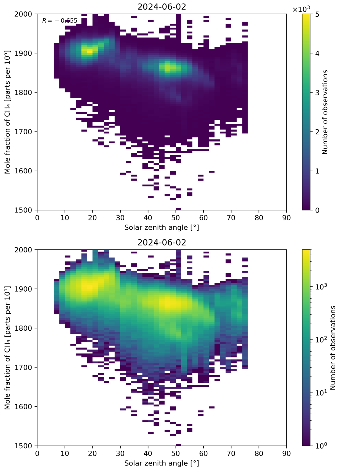
Figure 99: Scatter density plot of “Solar zenith angle” against “Mole fraction of CH 4 ” for 2024-06-01 to 2024-06-03.
