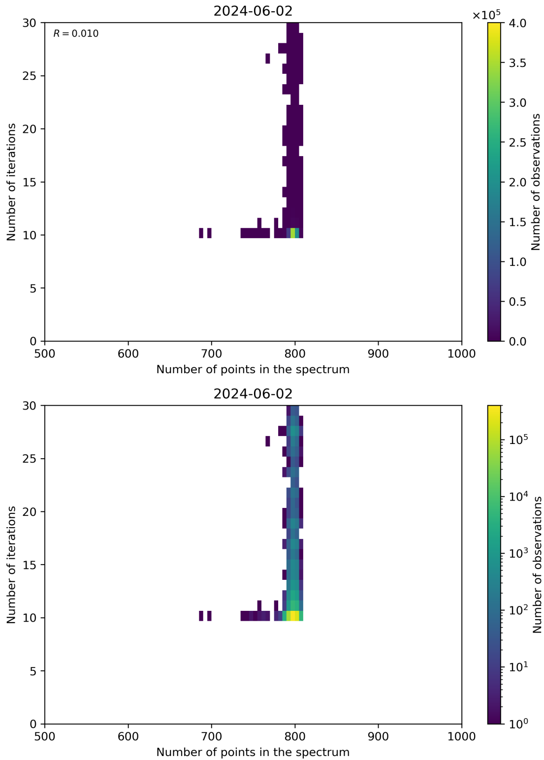
Figure 92: Scatter density plot of “Number of points in the spectrum” against “Number of iterations” for 2024-06-01 to 2024-06-03.
