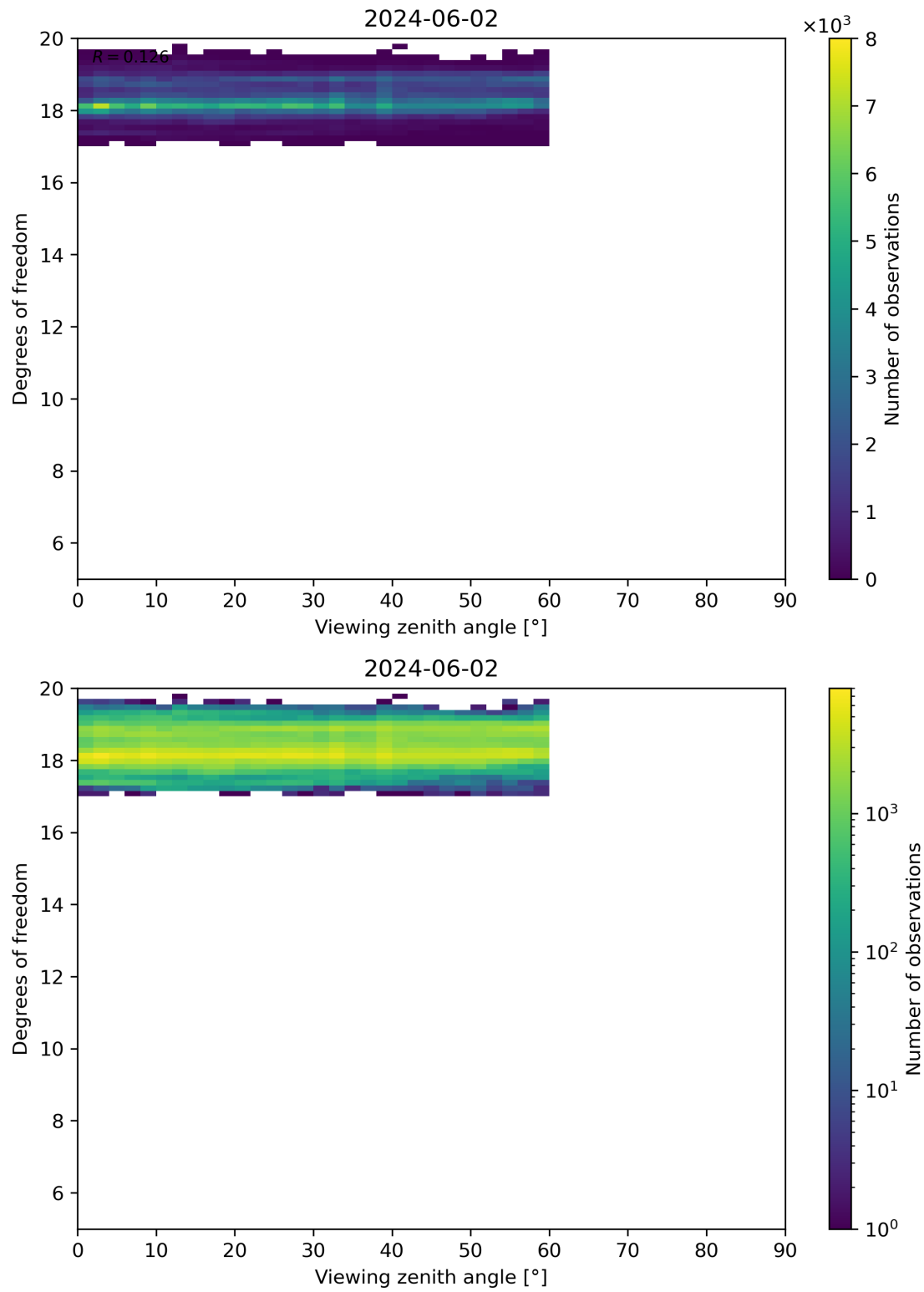
Figure 107: Scatter density plot of “Viewing zenith angle” against “Degrees of freedom” for 2024-06-01 to 2024-06-03.
