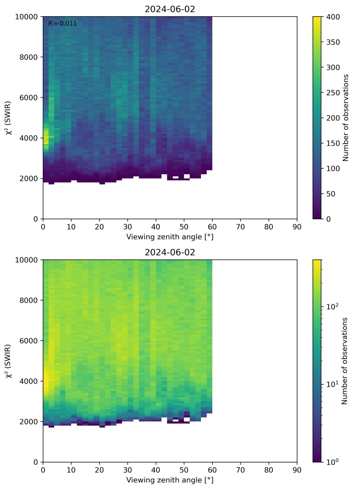
Figure 106: Scatter density plot of “Viewing zenith angle” against “ \chi^2 (SWIR)” for 2024-06-01 to 2024-06-03.
