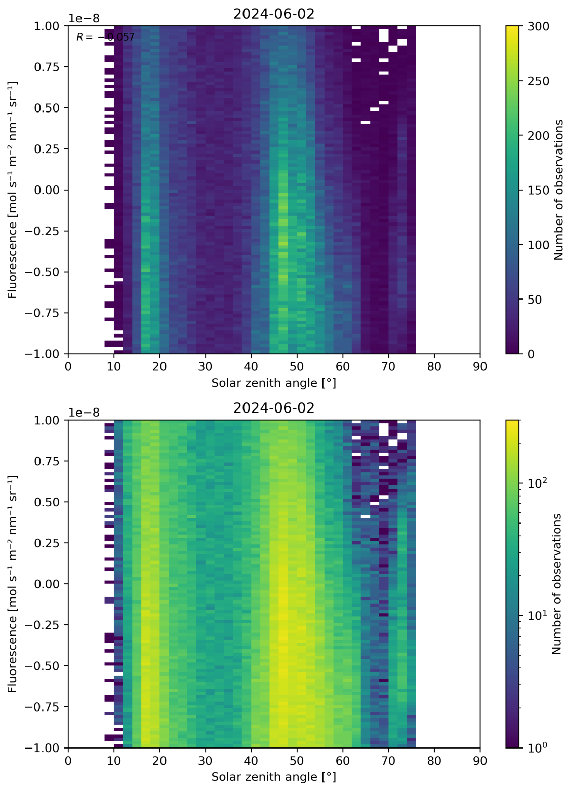
Figure 97: Scatter density plot of “Solar zenith angle” against “Fluorescence” for 2024-06-01 to 2024-06-03.
