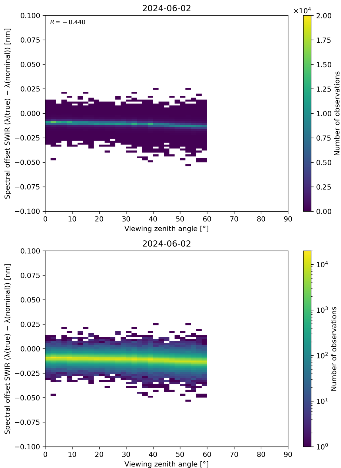
Figure 116: Scatter density plot of “Viewing zenith angle” against “Spectral offset SWIR ( \lambda(\text{true}) - \lambda(\text{nominal}) )” for 2024-06-01 to 2024-06-03.
