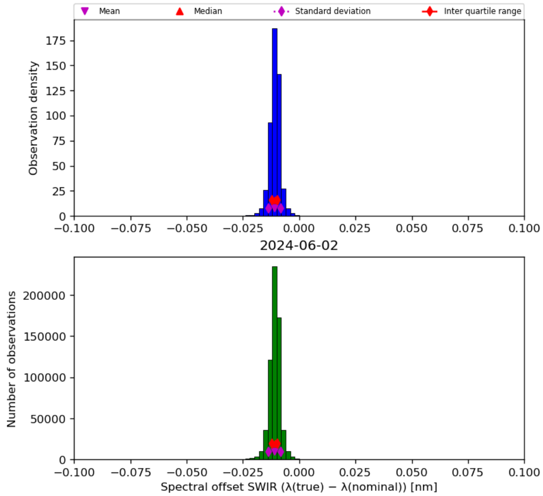
Figure 27: Histogram of “Spectral offset SWIR ( \lambda(\text{true}) - \lambda(\text{nominal}) )” for 2024-06-01 to 2024-06-03
