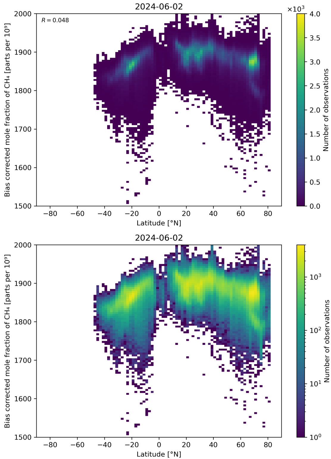
Figure 58: Scatter density plot of “Latitude” against “Bias corrected mole fraction of CH 4 ” for 2024-06-01 to 2024-06-03.
