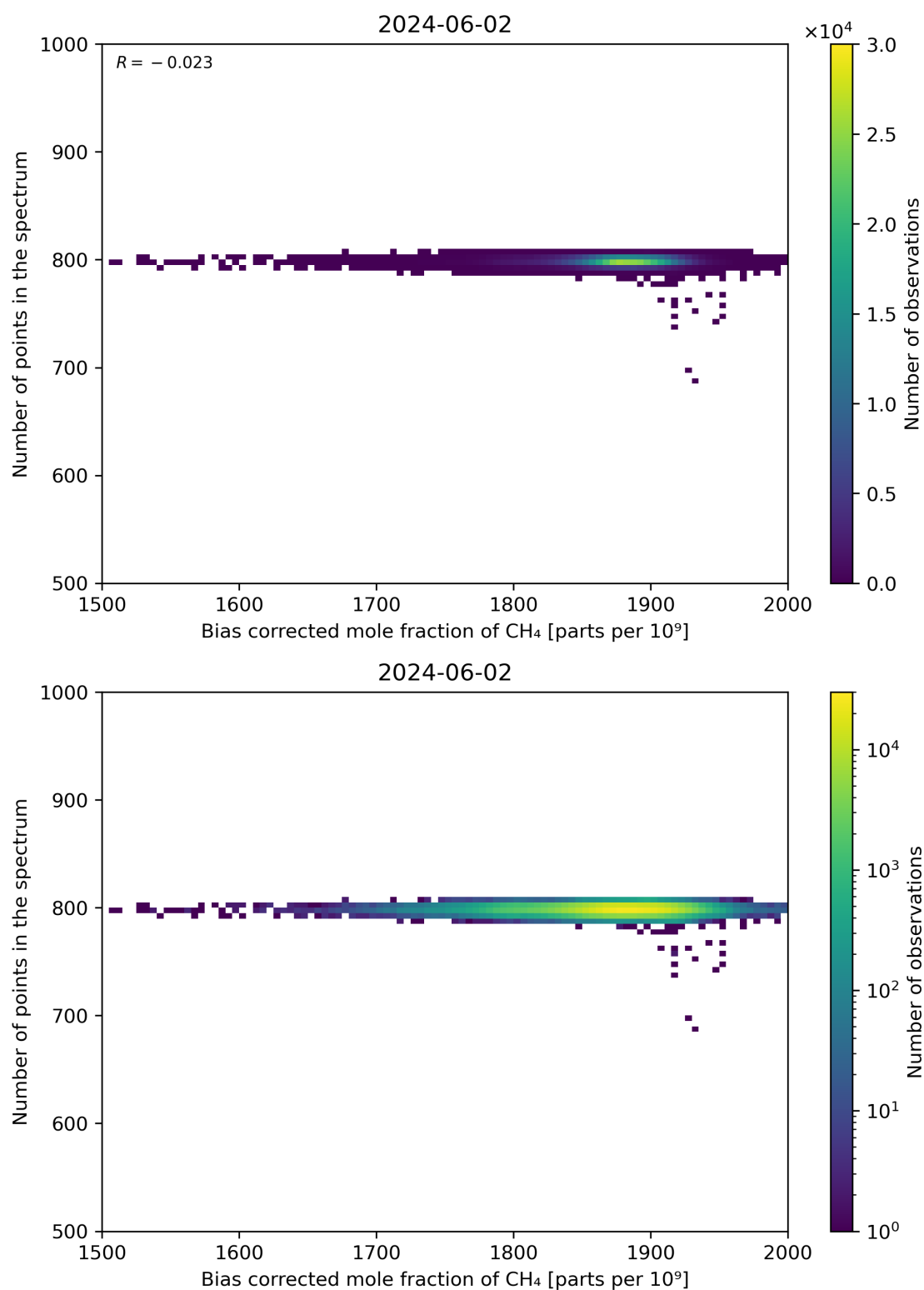
Figure 68: Scatter density plot of “Bias corrected mole fraction of CH 4 ” against “Number of points in the spectrum” for 2024-06-01 to 2024-06-03.
