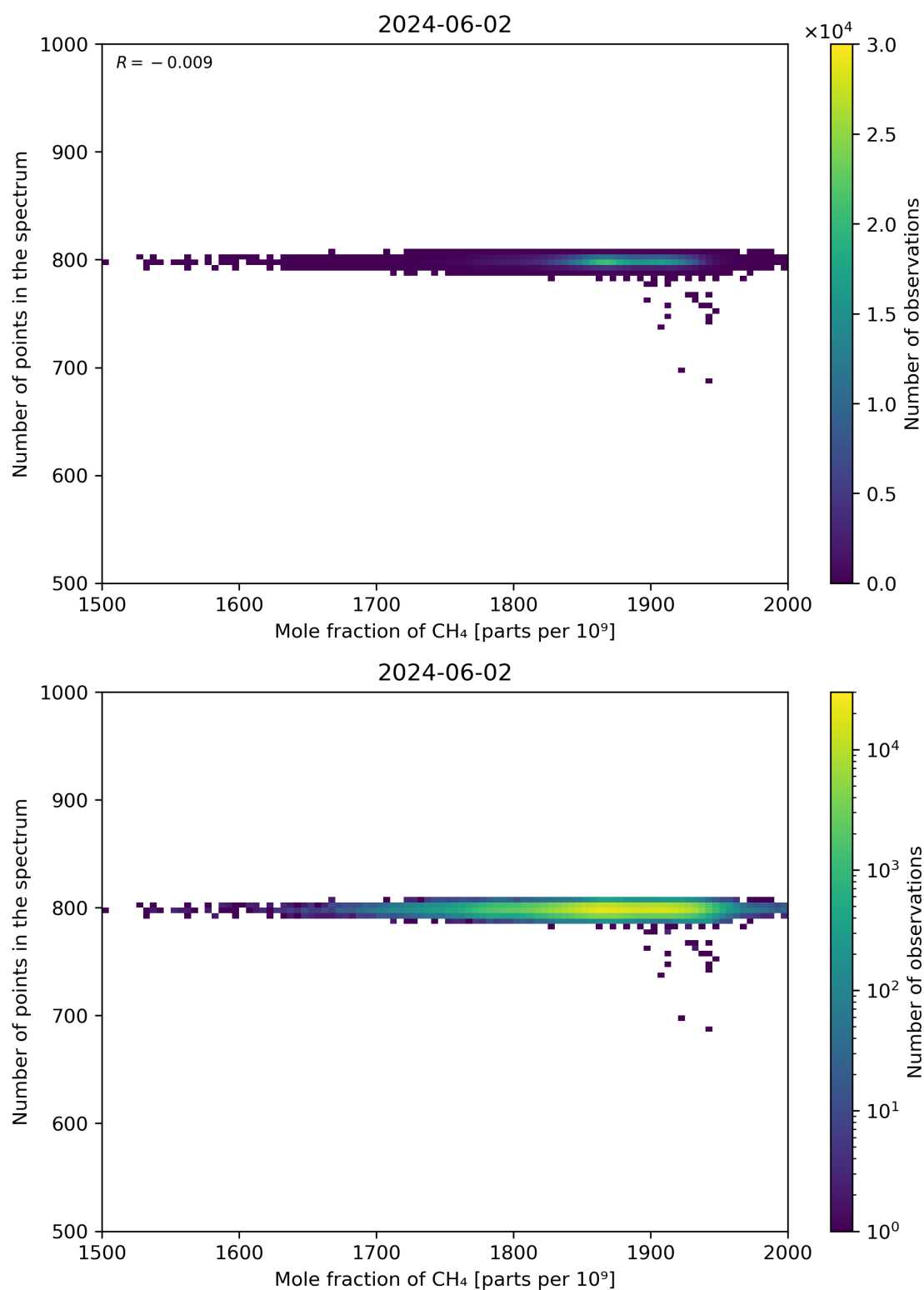
Figure 77: Scatter density plot of “Mole fraction of CH 4 ” against “Number of points in the spectrum” for 2024-06-01 to 2024-06-03.
