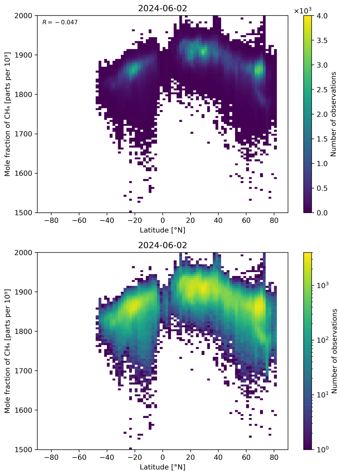
Figure 57: Scatter density plot of “Latitude” against “Mole fraction of CH 4 ” for 2024-06-01 to 2024-06-03.
