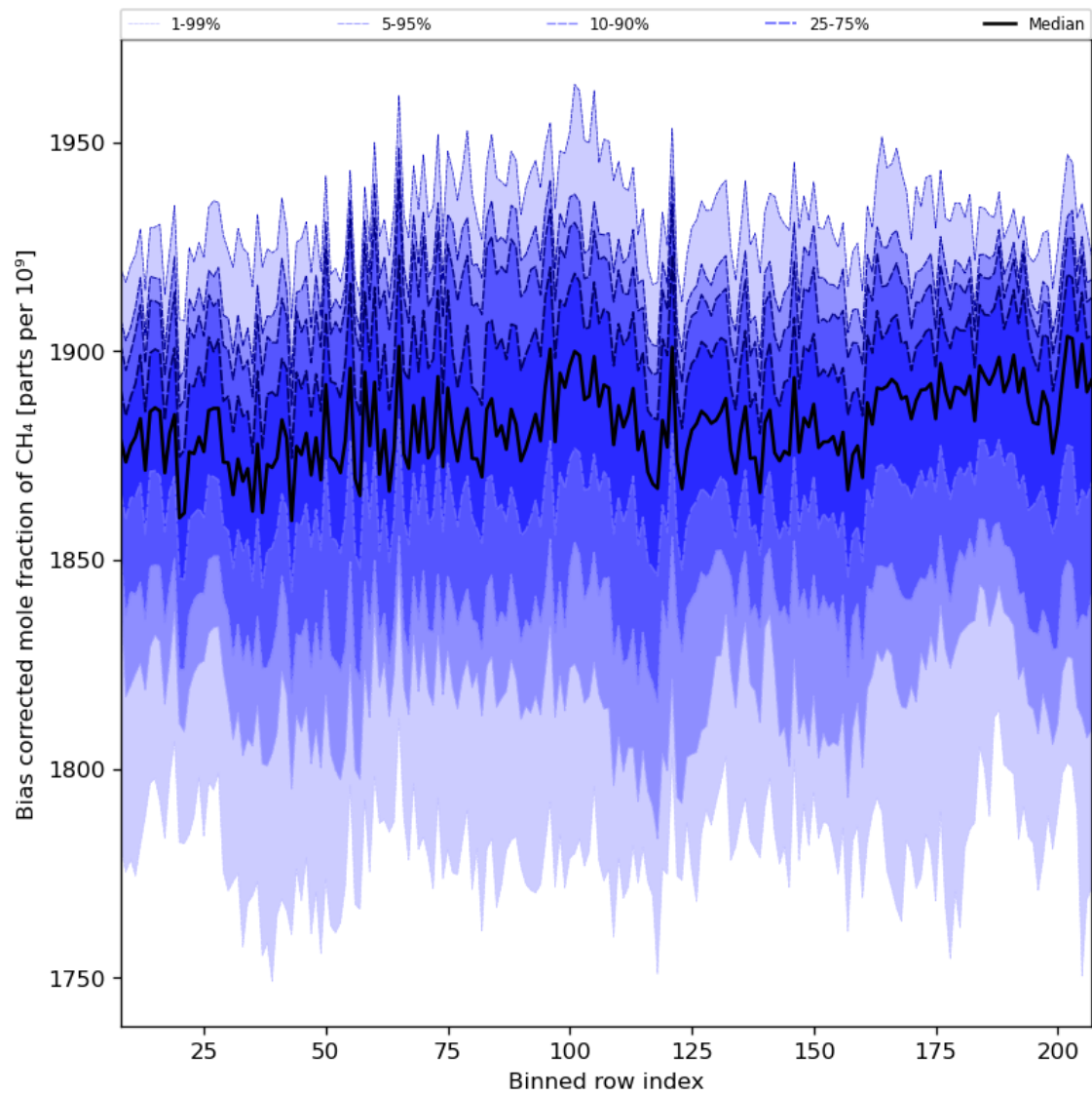
Figure 36: Along track statistics of “Bias corrected mole fraction of CH 4 ” for 2024-06-01 to 2024-06-03
