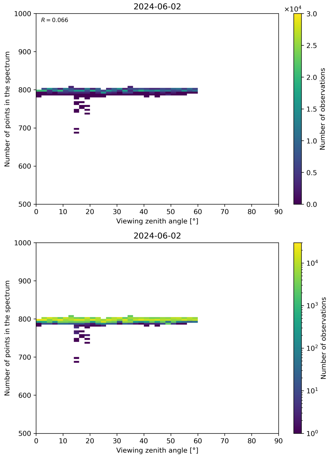
Figure 114: Scatter density plot of “Viewing zenith angle” against “Number of points in the spectrum” for 2024-06-01 to 2024-06-03.
