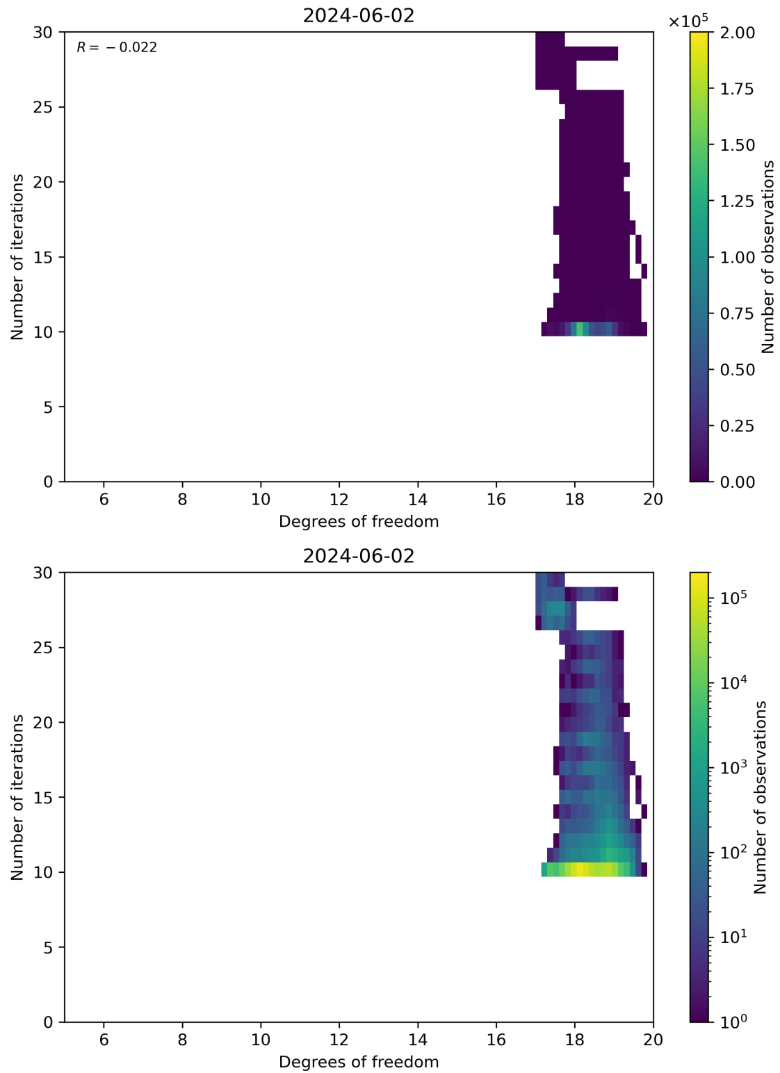
Figure 52: Scatter density plot of “Degrees of freedom” against “Number of iterations” for 2024-06-01 to 2024-06-03.
