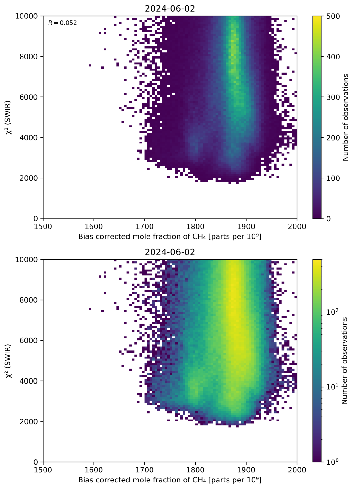
Figure 64: Scatter density plot of “Bias corrected mole fraction of \text{CH}_4 ” against “ \chi^2 (SWIR)” for 2024-06-01 to 2024-06-03.
