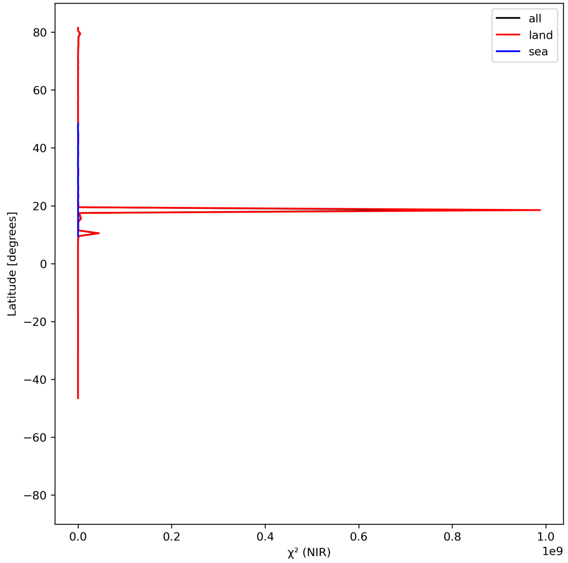
Figure 18: Zonal average of “ \chi^2 (NIR)” for 2024-06-01 to 2024-06-03.
