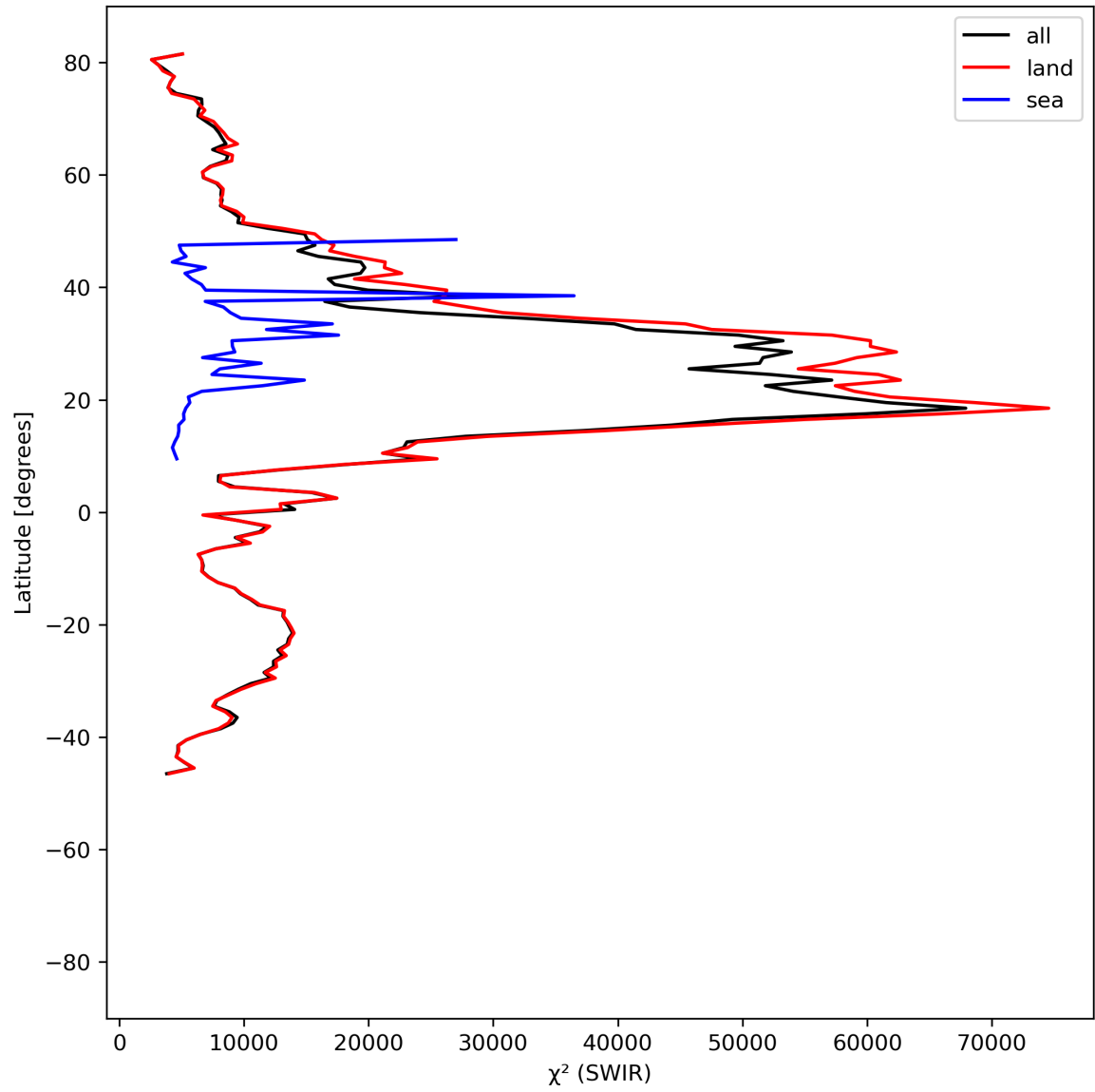
Figure 17: Zonal average of “ \chi^2 (SWIR)” for 2024-06-01 to 2024-06-03.
