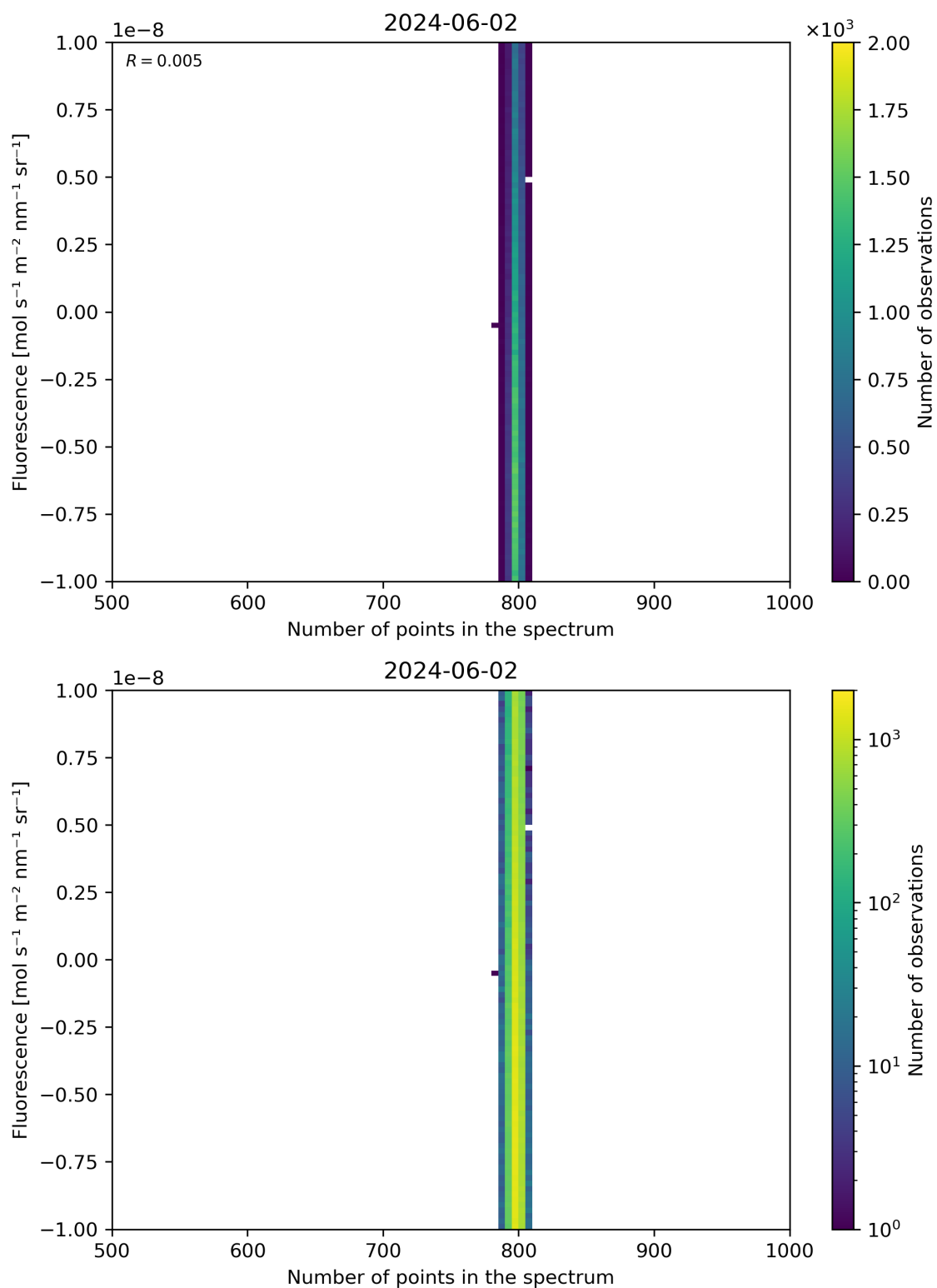
Figure 91: Scatter density plot of “Number of points in the spectrum” against “Fluorescence” for 2024-06-01 to 2024-06-03.
