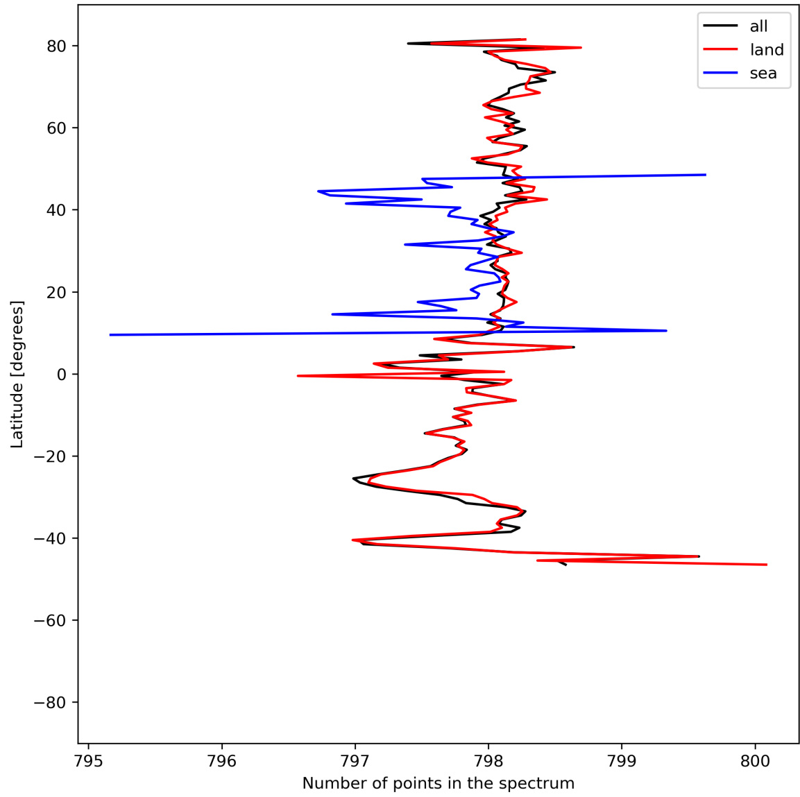
Figure 15: Zonal average of “Number of points in the spectrum” for 2024-06-01 to 2024-06-03.
