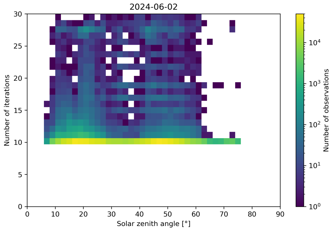
Figure 102: Scatter density plot of “Solar zenith angle” against “Number of iterations” for 2024-06-01 to 2024-06-03.
