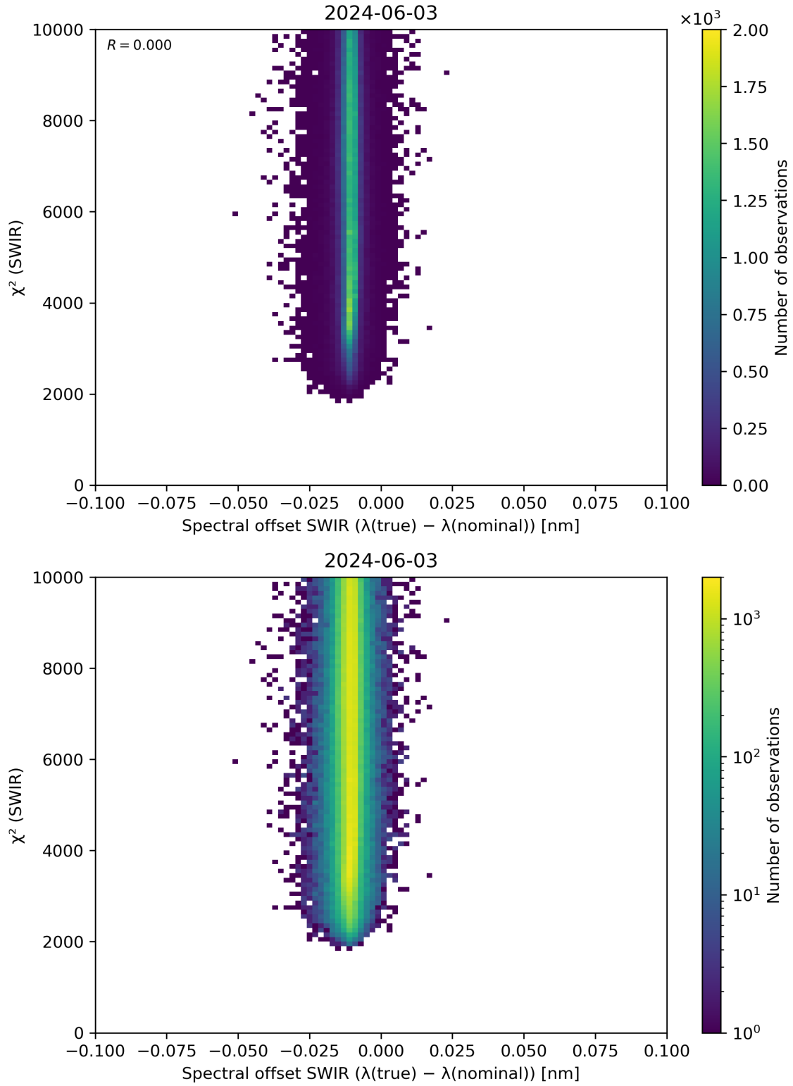
Figure 118: Scatter density plot of “Spectral offset SWIR ( \lambda(\text{true}) - \lambda(\text{nominal}) )” against “ \chi^2 (SWIR)” for 2024-06-03 to 2024-06-04.
