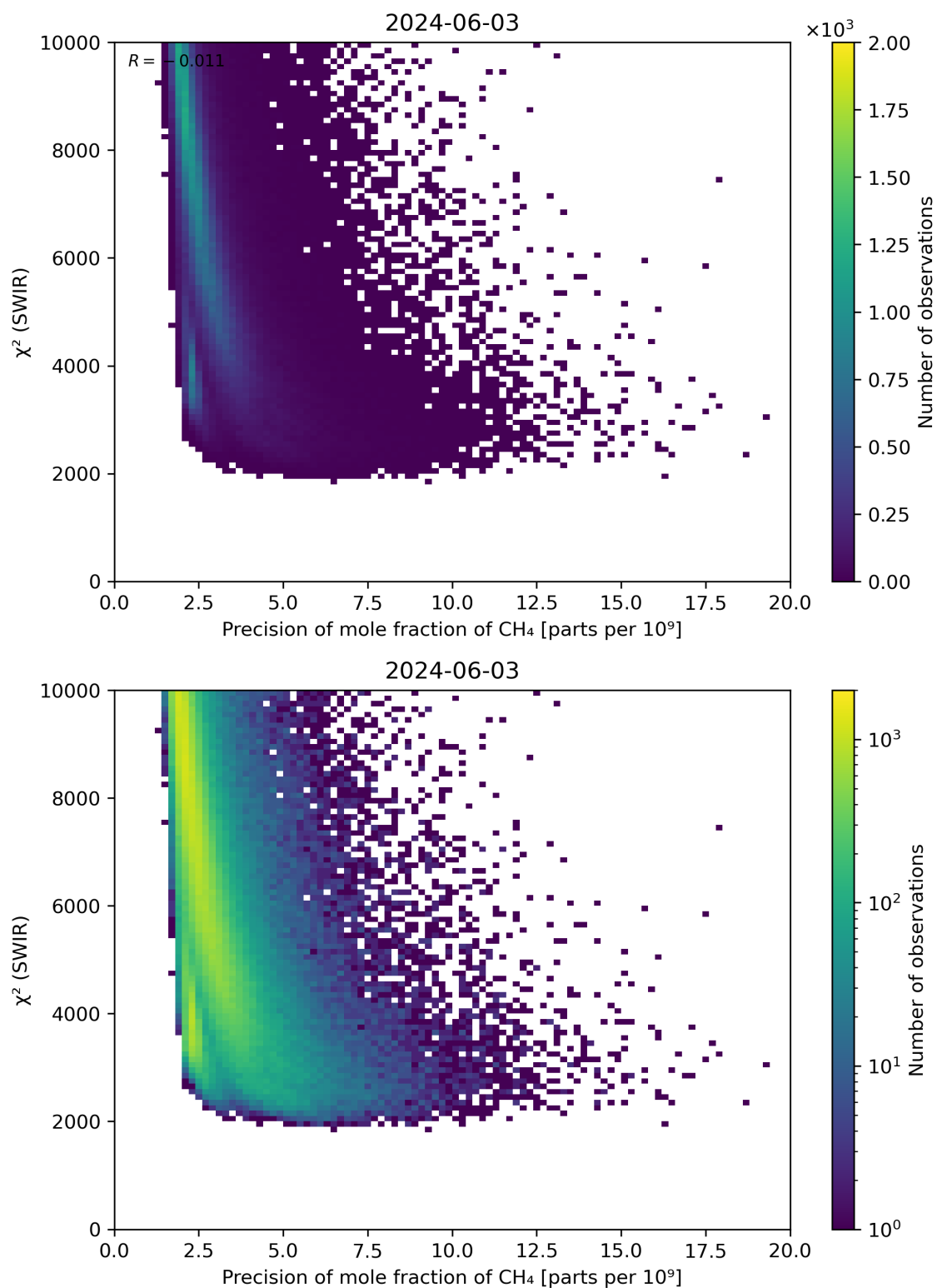
Figure 79: Scatter density plot of “Precision of mole fraction of \text{CH}_4 ” against “ \chi^2 (SWIR)” for 2024-06-03 to 2024-06-04.
