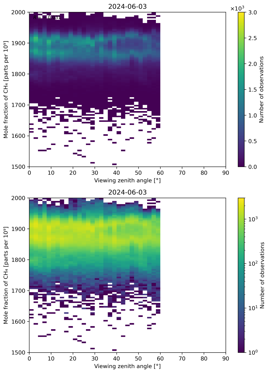
Figure 110: Scatter density plot of “Viewing zenith angle” against “Mole fraction of CH 4 ” for 2024-06-03 to 2024-06-04.
