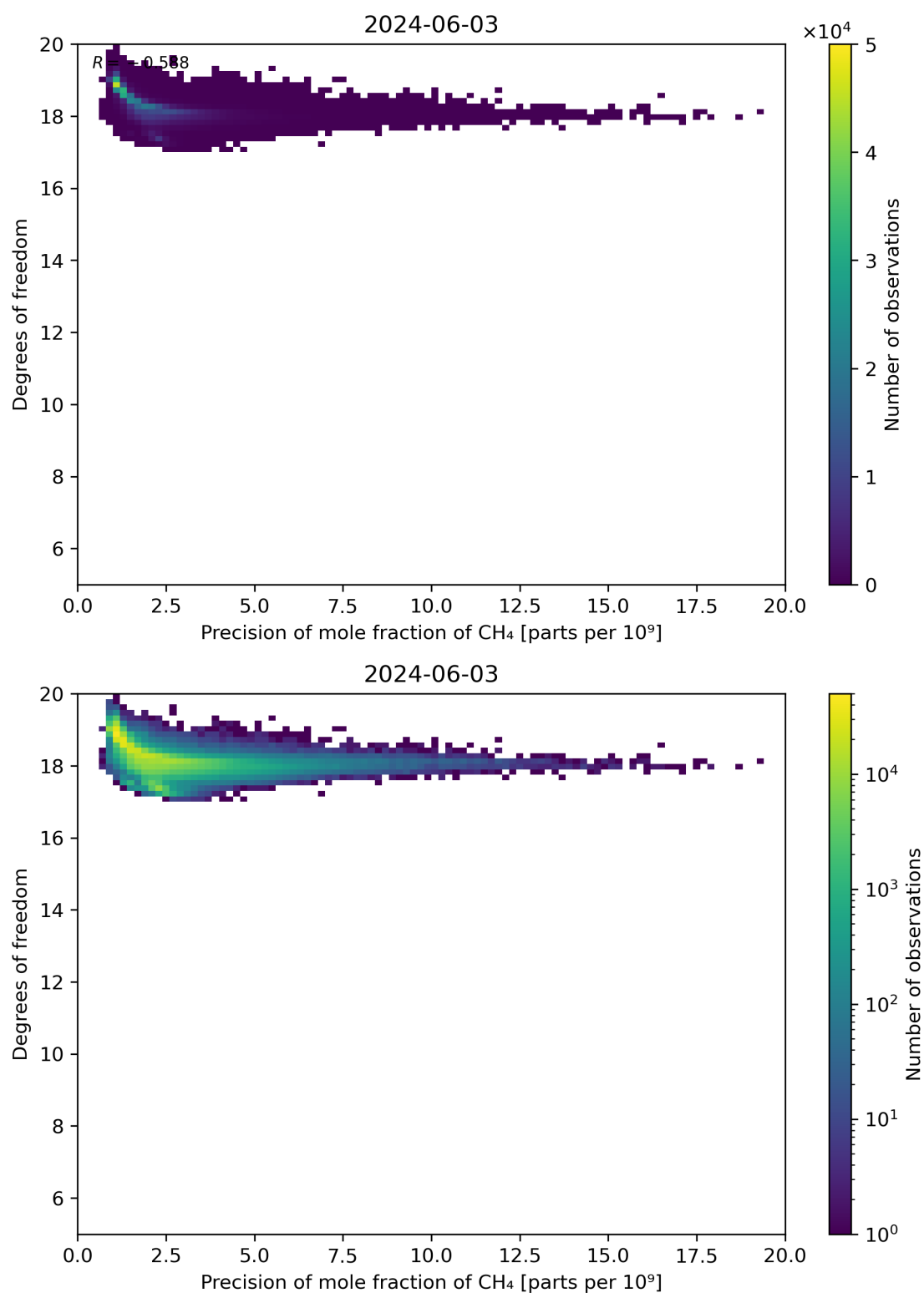
Figure 80: Scatter density plot of “Precision of mole fraction of CH 4 ” against “Degrees of freedom” for 2024-06-03 to 2024-06-04.
