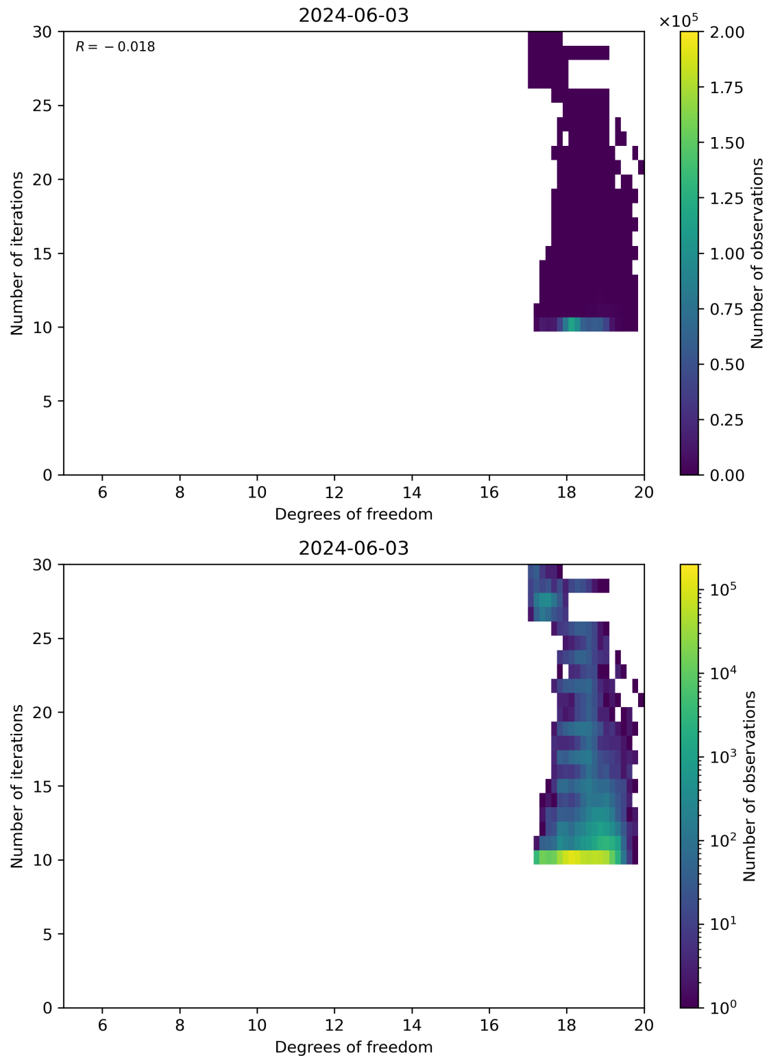
Figure 52: Scatter density plot of “Degrees of freedom” against “Number of iterations” for 2024-06-03 to 2024-06-04.
