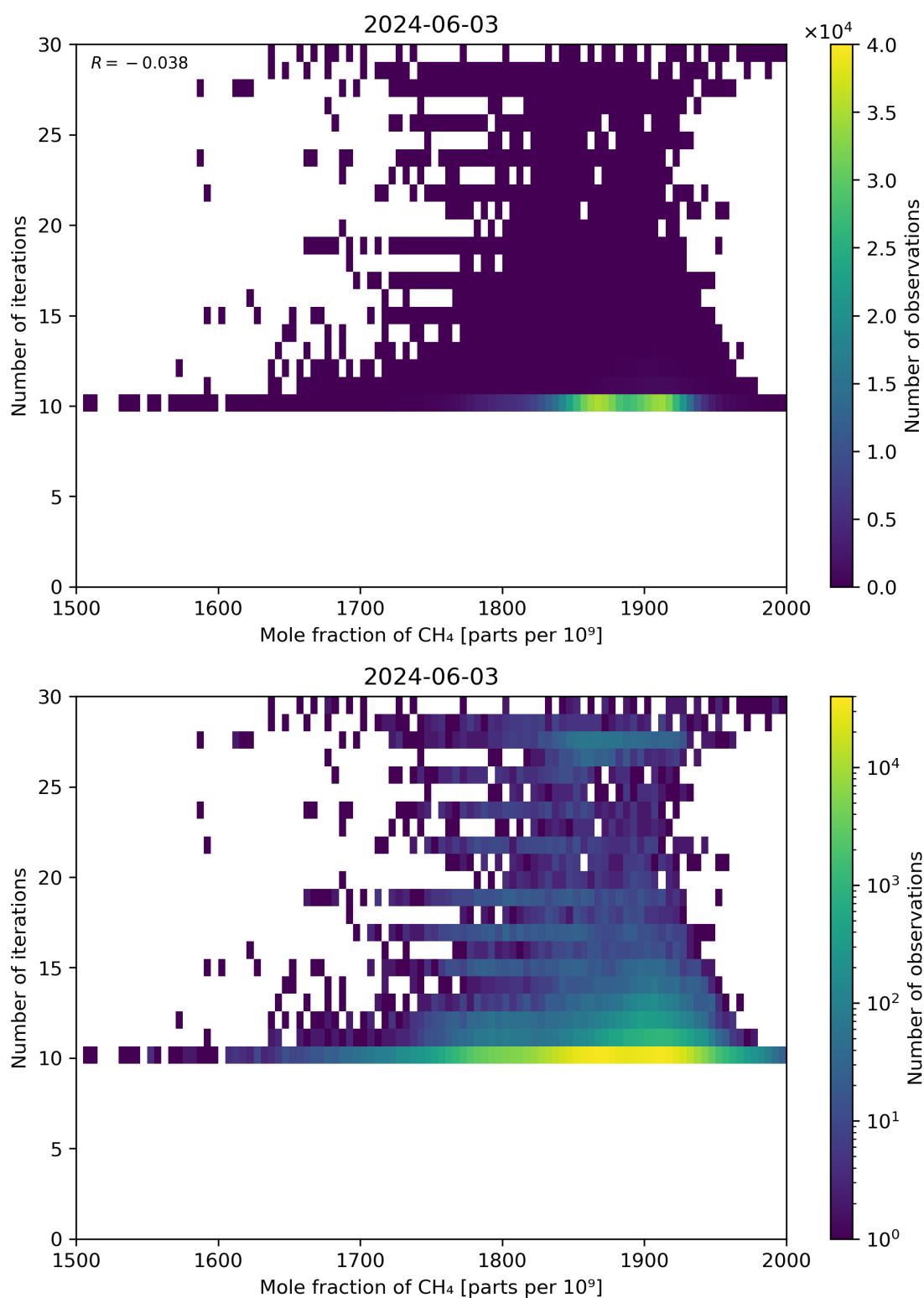
Figure 76: Scatter density plot of “Mole fraction of CH 4 ” against “Number of iterations” for 2024-06-03 to 2024-06-04.
