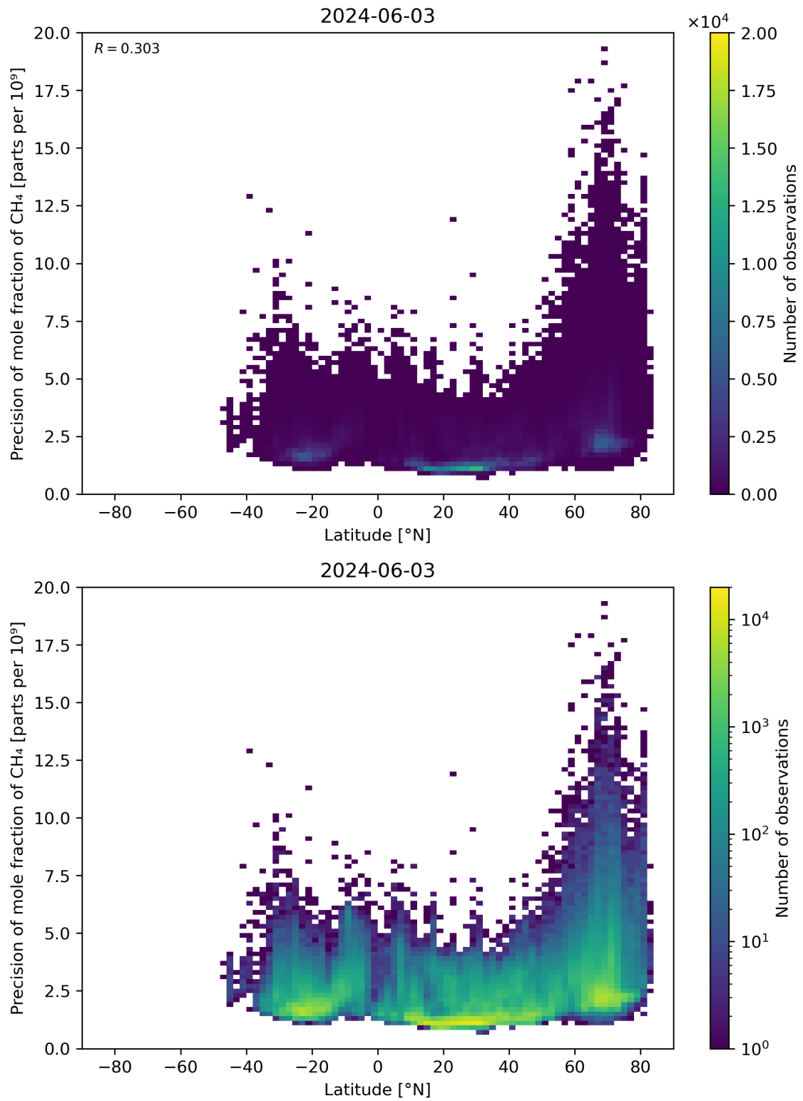
Figure 59: Scatter density plot of “Latitude” against “Precision of mole fraction of \text{CH}_4 ” for 2024-06-03 to 2024-06-04.
