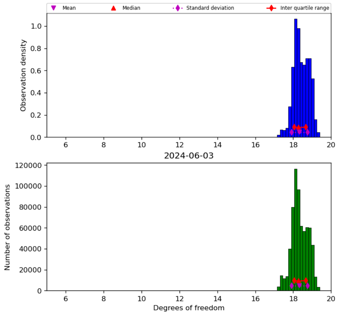
Figure 30: Histogram of “Degrees of freedom” for 2024-06-03 to 2024-06-04
