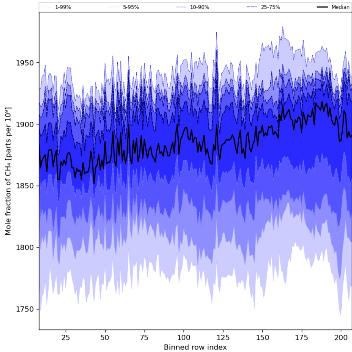
Figure 34: Along track statistics of “Mole fraction of CH 4 ” for 2024-06-03 to 2024-06-04
