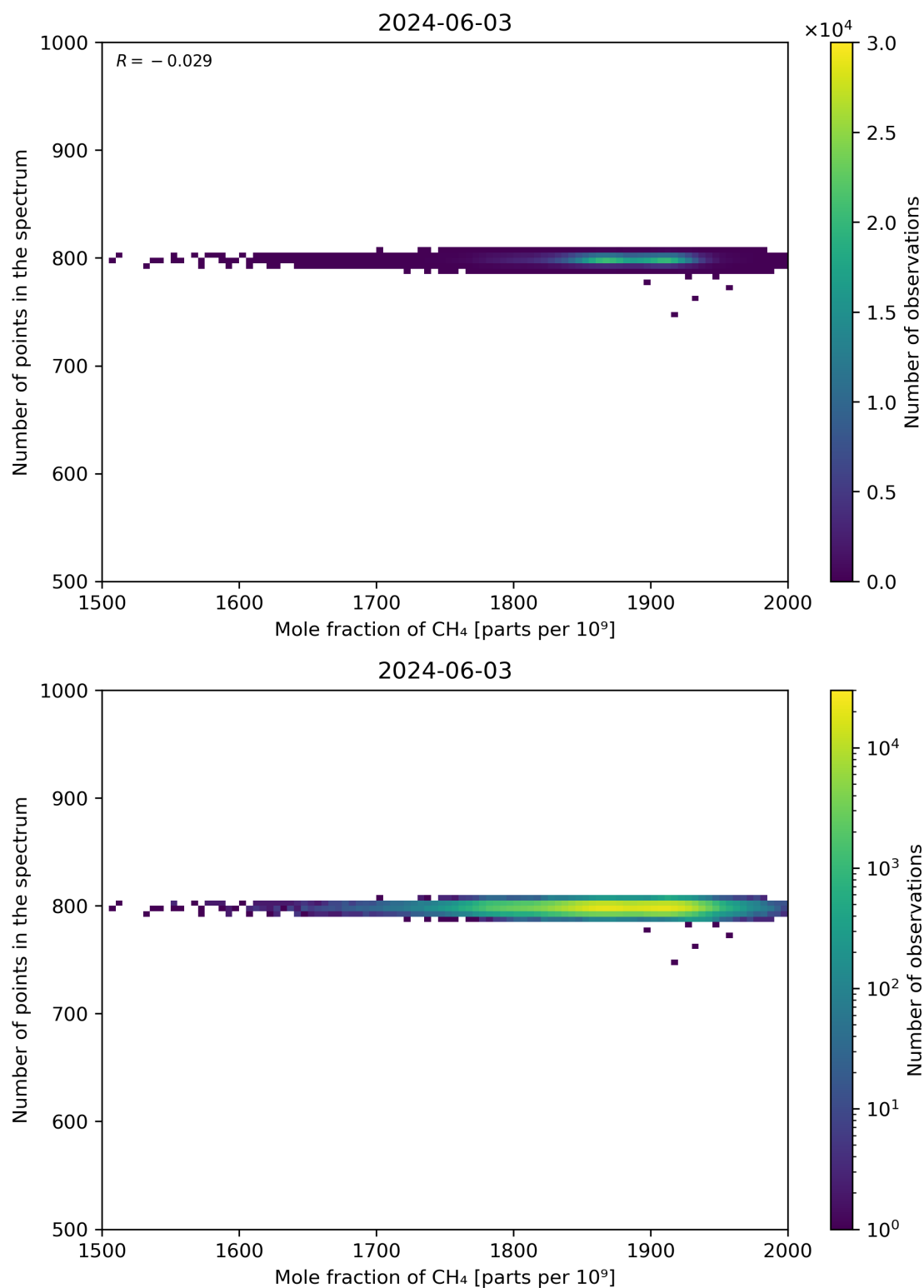
Figure 77: Scatter density plot of “Mole fraction of CH 4 ” against “Number of points in the spectrum” for 2024-06-03 to 2024-06-04.
