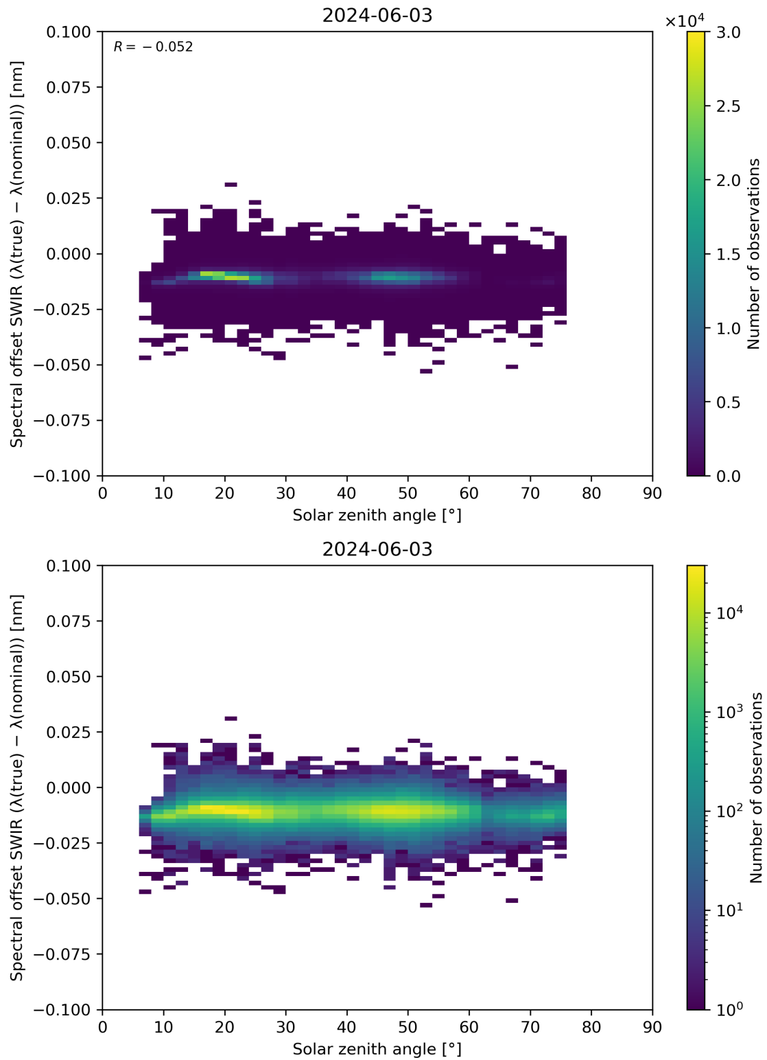
Figure 104: Scatter density plot of “Solar zenith angle” against “Spectral offset SWIR ( \lambda(\text{true}) - \lambda(\text{nominal}) )” for 2024-06-03 to 2024-06-04.
