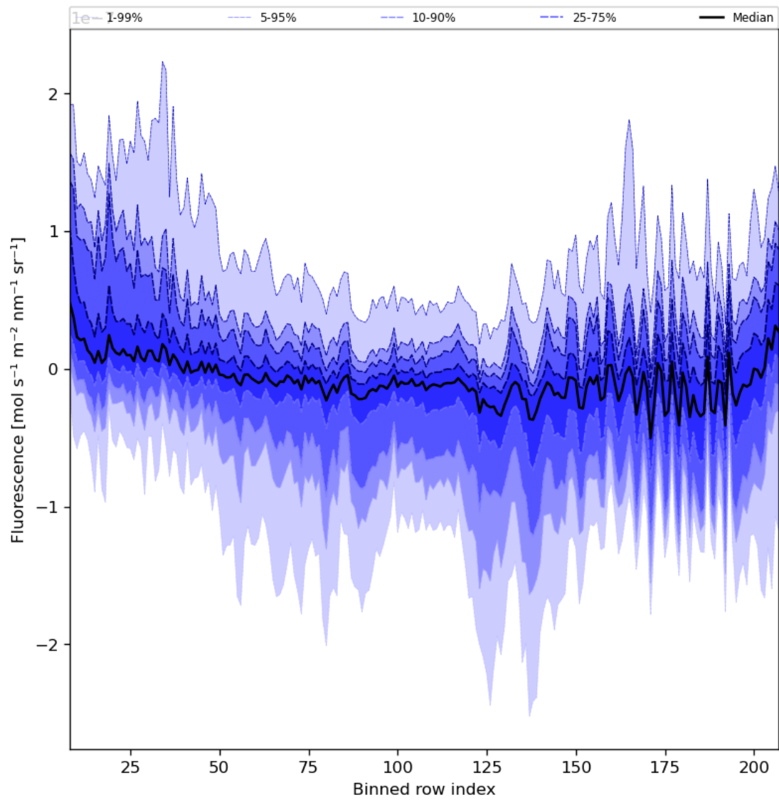
Figure 43: Along track statistics of “Fluorescence” for 2024-06-03 to 2024-06-04
