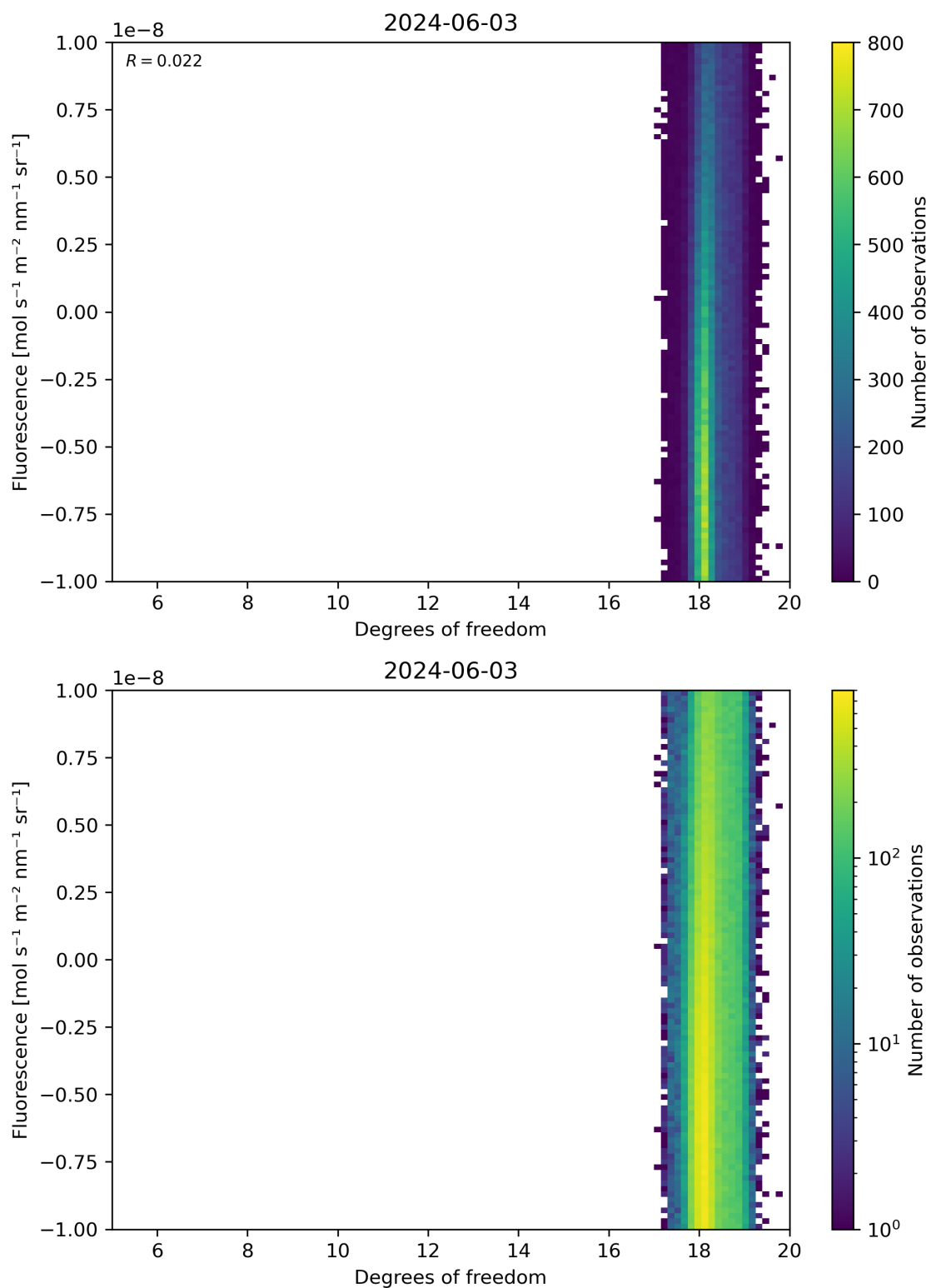
Figure 51: Scatter density plot of “Degrees of freedom” against “Fluorescence” for 2024-06-03 to 2024-06-04.
