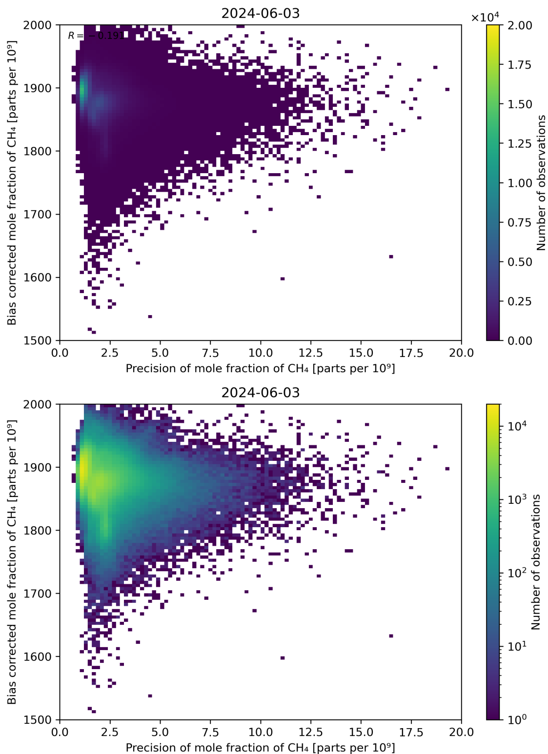
Figure 82: Scatter density plot of “Precision of mole fraction of CH 4 ” against “Bias corrected mole fraction of CH 4 ” for 2024-06-03 to 2024-06-04.
