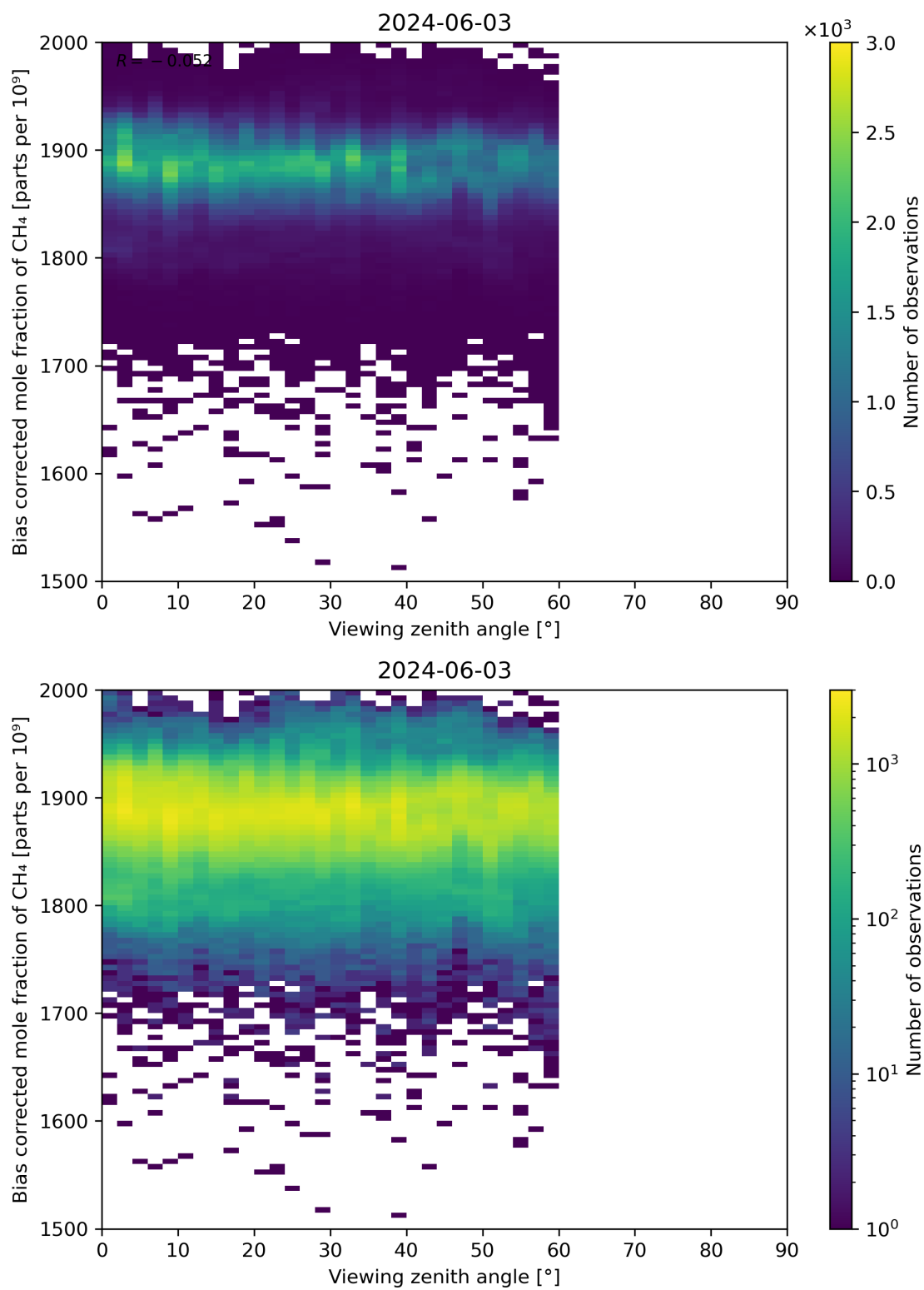
Figure 111: Scatter density plot of “Viewing zenith angle” against “Bias corrected mole fraction of CH 4 ” for 2024-06-03 to 2024-06-04.
