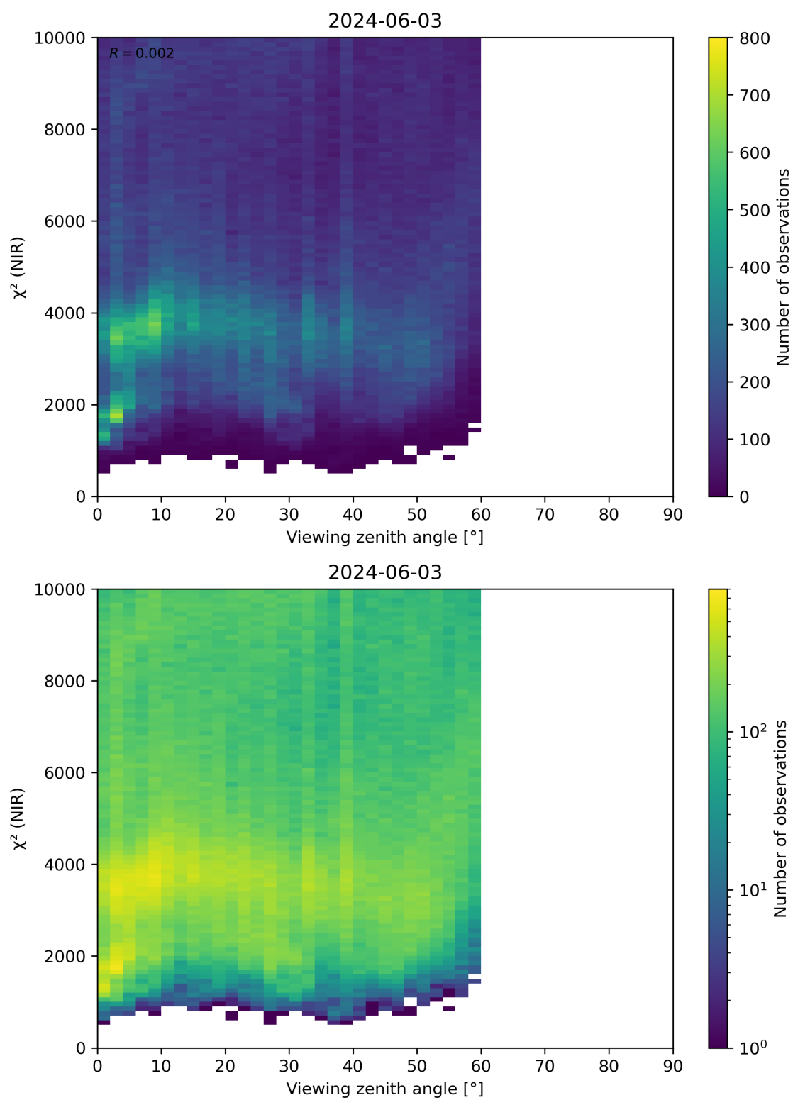
Figure 105: Scatter density plot of “Viewing zenith angle” against “ \chi^2 (NIR)” for 2024-06-03 to 2024-06-04.
