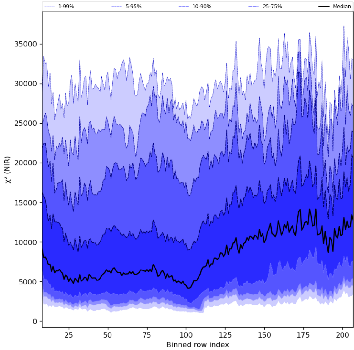
Figure 40: Along track statistics of “ \chi^2 (NIR)” for 2024-06-03 to 2024-06-04
