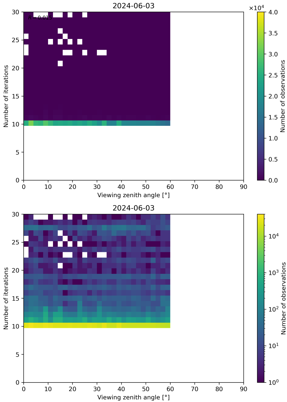
Figure 113: Scatter density plot of “Viewing zenith angle” against “Number of iterations” for 2024-06-03 to 2024-06-04.
