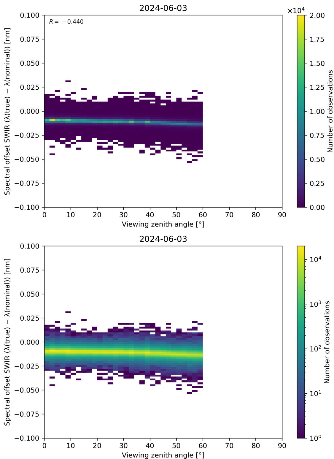
Figure 116: Scatter density plot of “Viewing zenith angle” against “Spectral offset SWIR ( \lambda(\text{true}) - \lambda(\text{nominal}) )” for 2024-06-03 to 2024-06-04.
