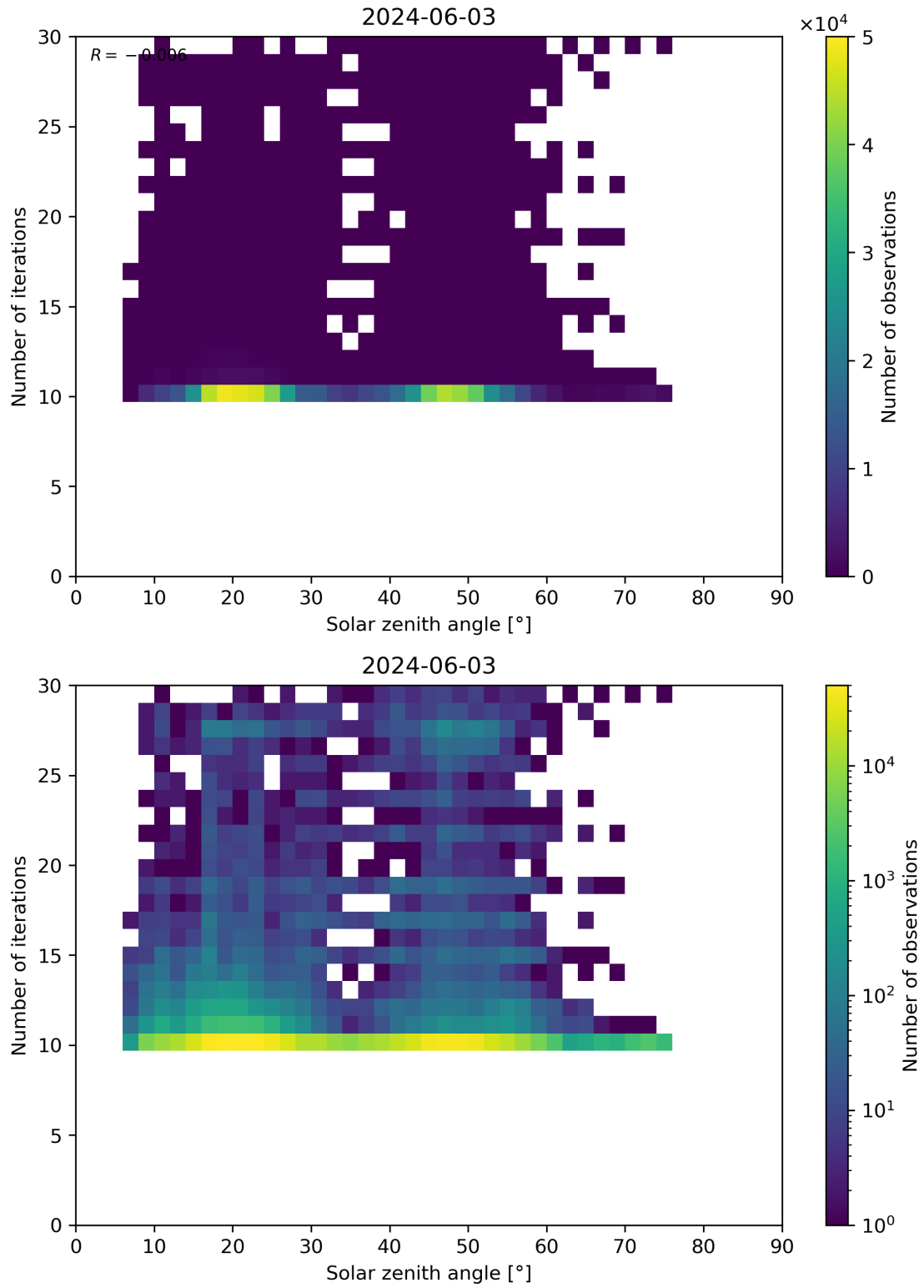
Figure 102: Scatter density plot of “Solar zenith angle” against “Number of iterations” for 2024-06-03 to 2024-06-04.
