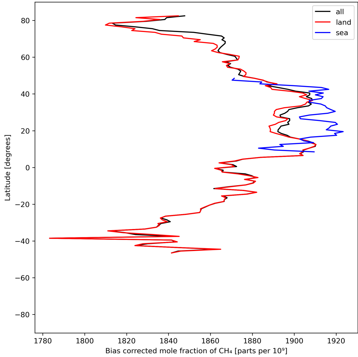
Figure 14: Zonal average of “Bias corrected mole fraction of CH 4 ” for 2024-06-03 to 2024-06-04.
