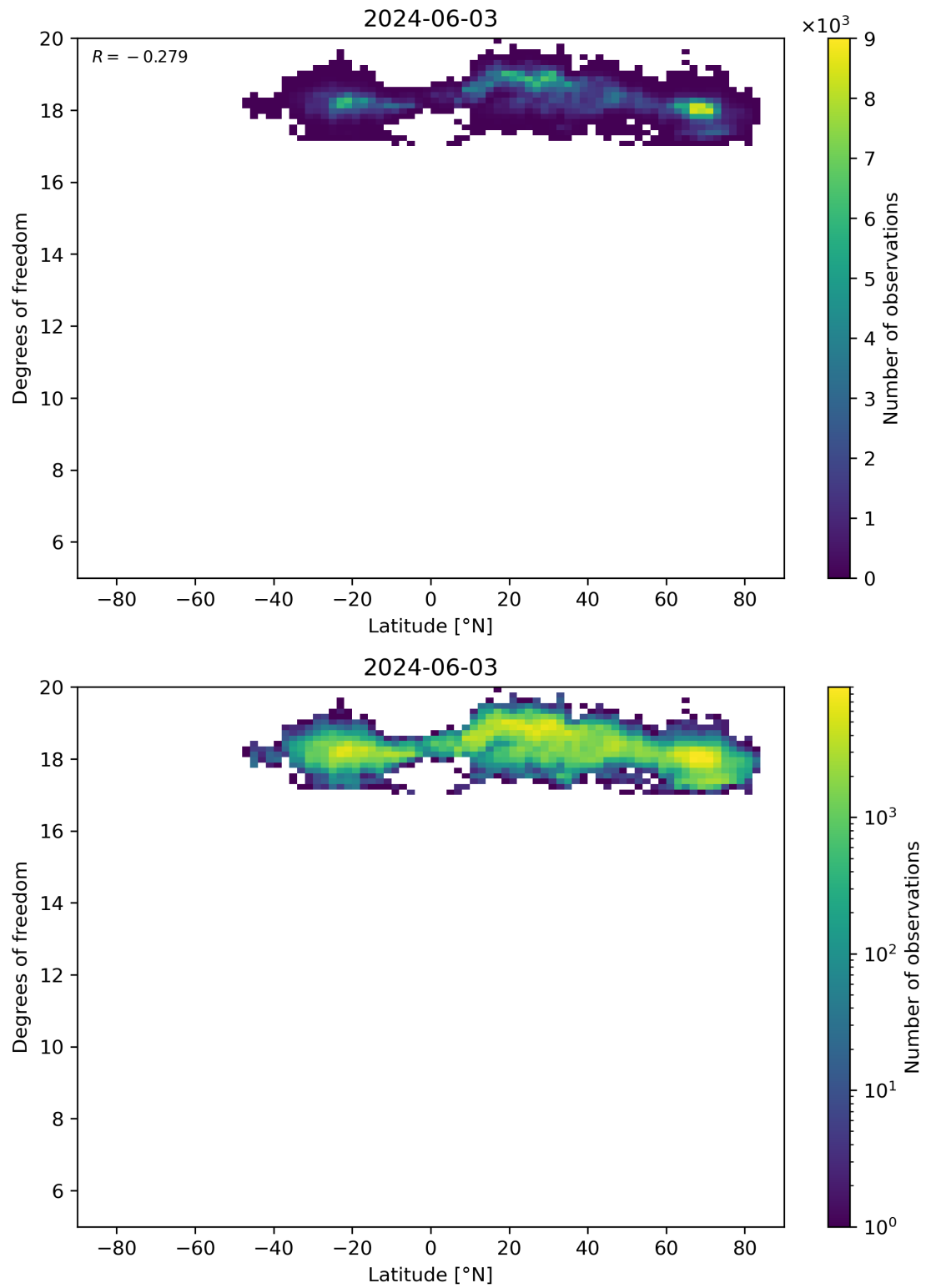
Figure 55: Scatter density plot of “Latitude” against “Degrees of freedom” for 2024-06-03 to 2024-06-04.
