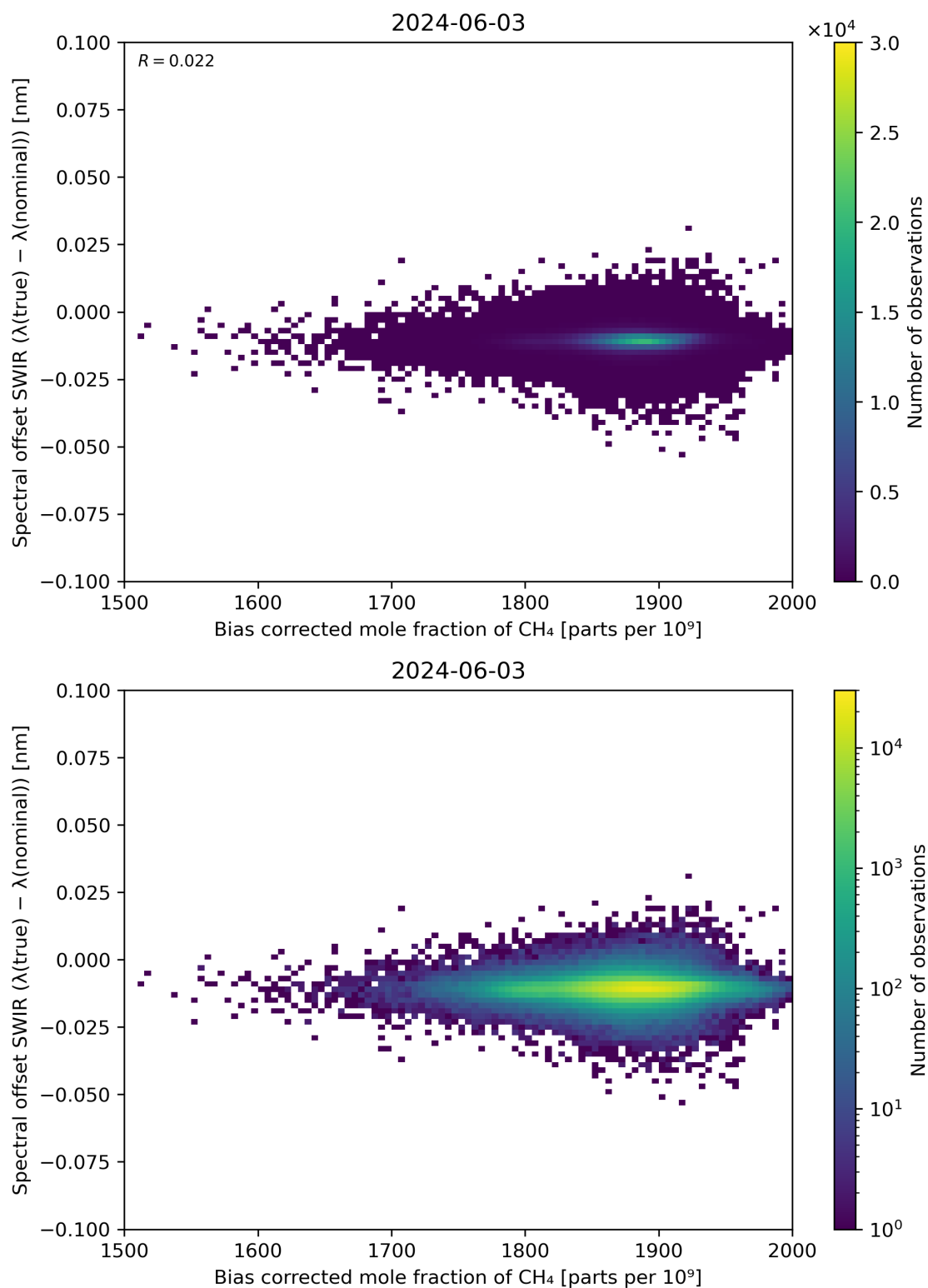
Figure 69: Scatter density plot of “Bias corrected mole fraction of \text{CH}_4 ” against “Spectral offset SWIR ( \lambda(\text{true}) - \lambda(\text{nominal}) )” for 2024-06-03 to 2024-06-04.
