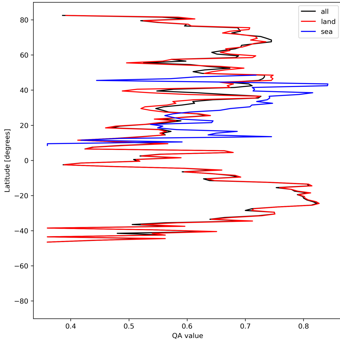
Figure 11: Zonal average of “QA value” for 2024-06-03 to 2024-06-04.
