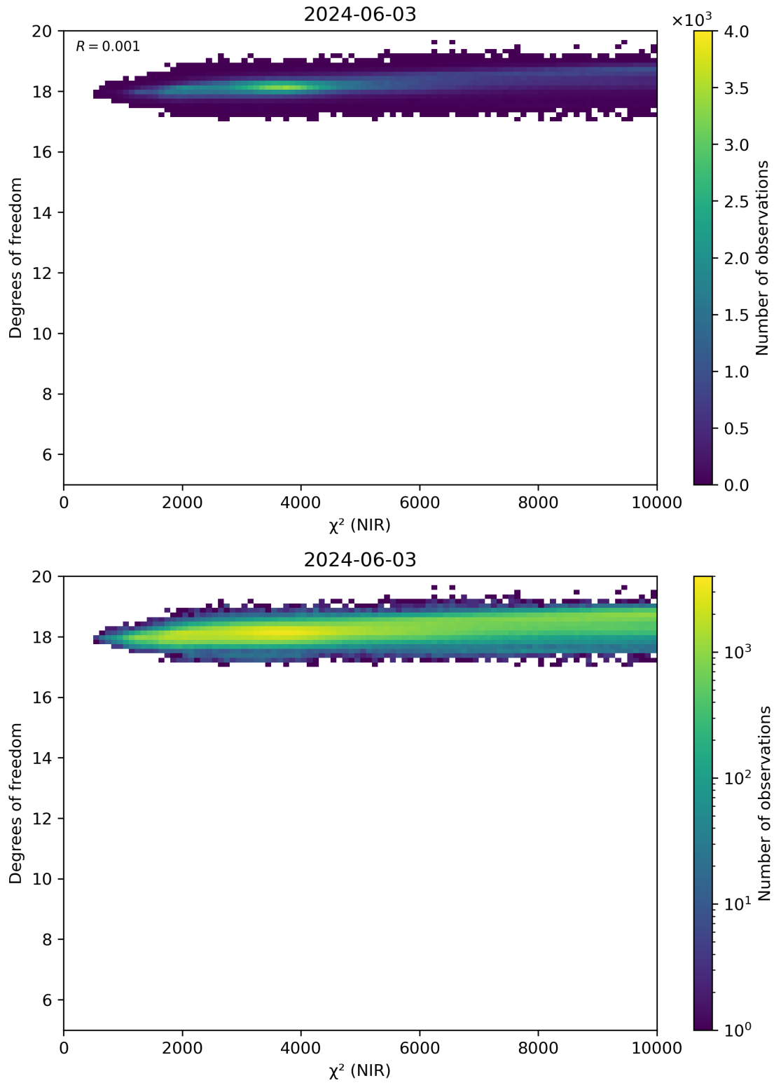
Figure 44: Scatter density plot of “ \chi^2 (NIR)” against “Degrees of freedom” for 2024-06-03 to 2024-06-04.
