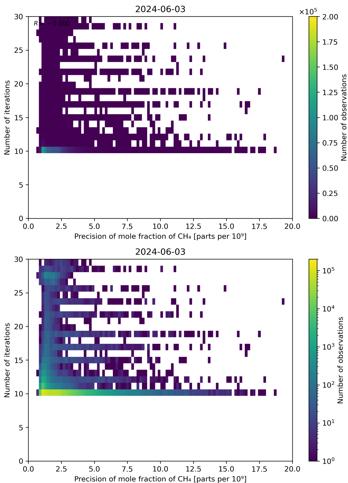
Figure 83: Scatter density plot of “Precision of mole fraction of CH 4 ” against “Number of iterations” for 2024-06-03 to 2024-06-04.
