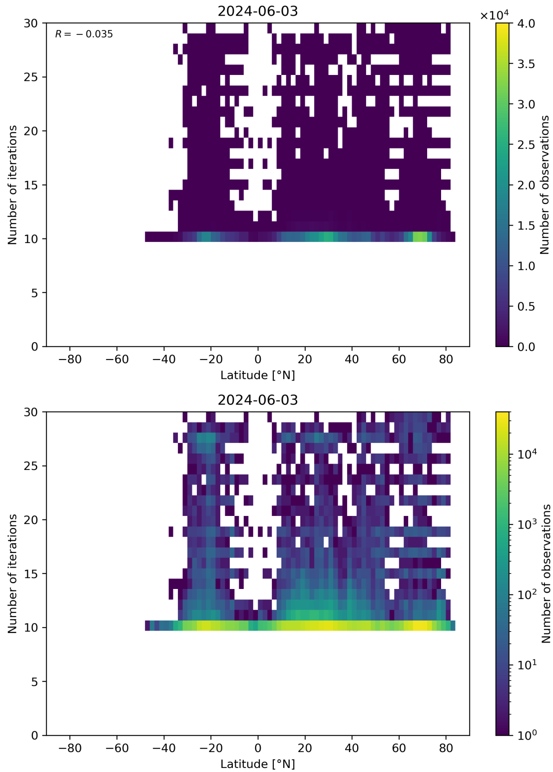
Figure 60: Scatter density plot of “Latitude” against “Number of iterations” for 2024-06-03 to 2024-06-04.
