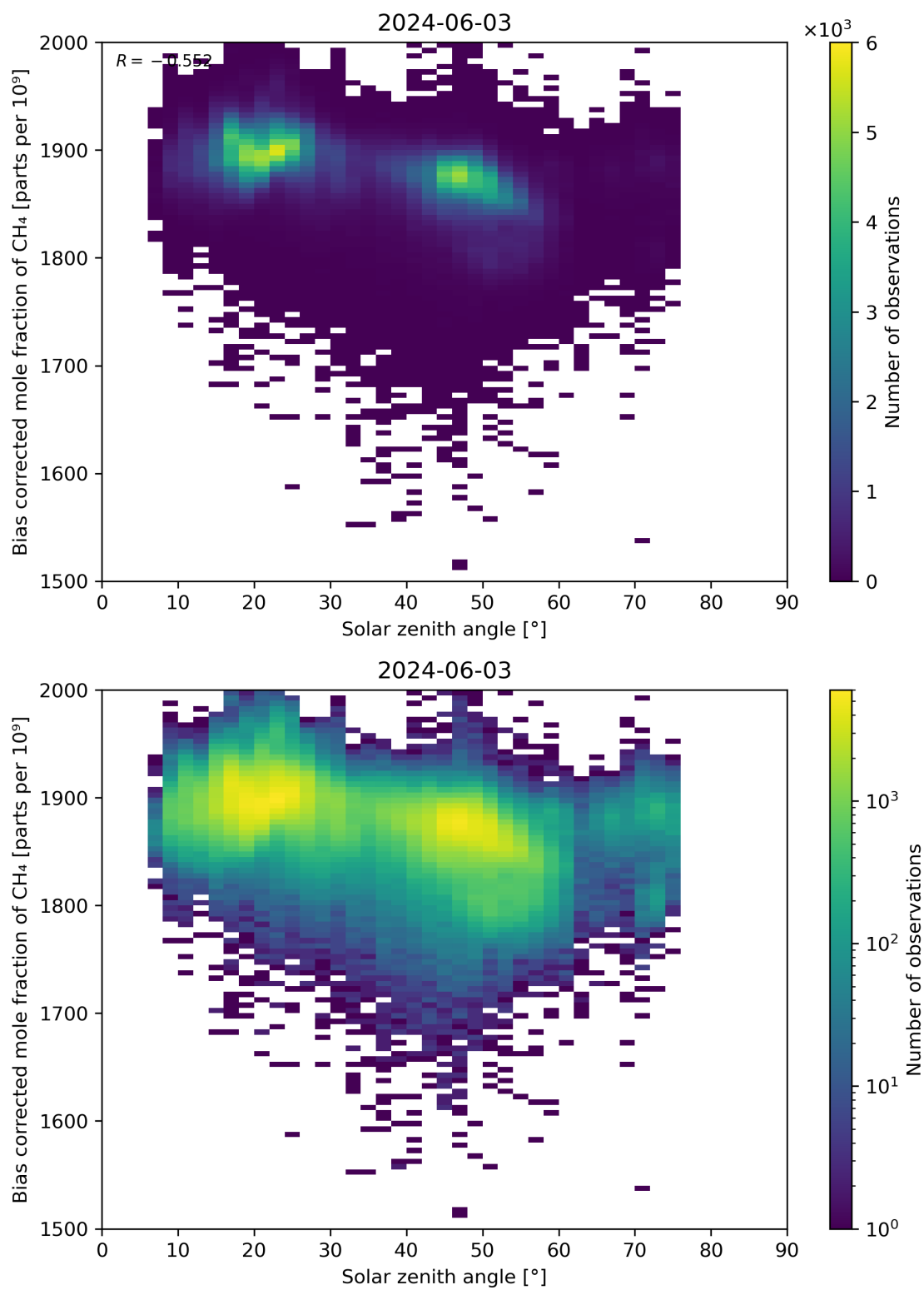
Figure 100: Scatter density plot of “Solar zenith angle” against “Bias corrected mole fraction of CH 4 ” for 2024-06-03 to 2024-06-04.
