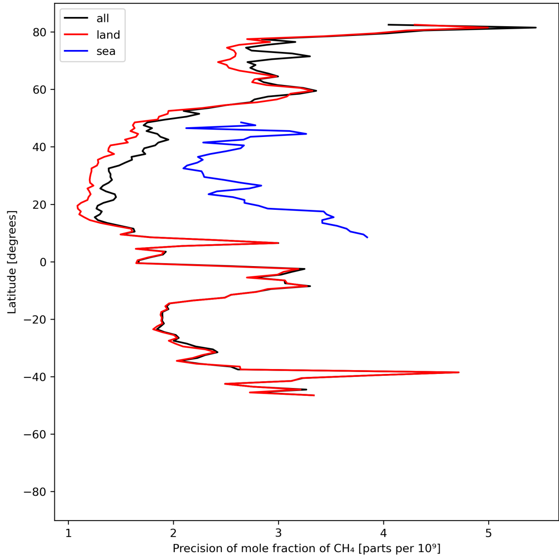
Figure 13: Zonal average of “Precision of mole fraction of CH 4 ” for 2024-06-03 to 2024-06-04.
