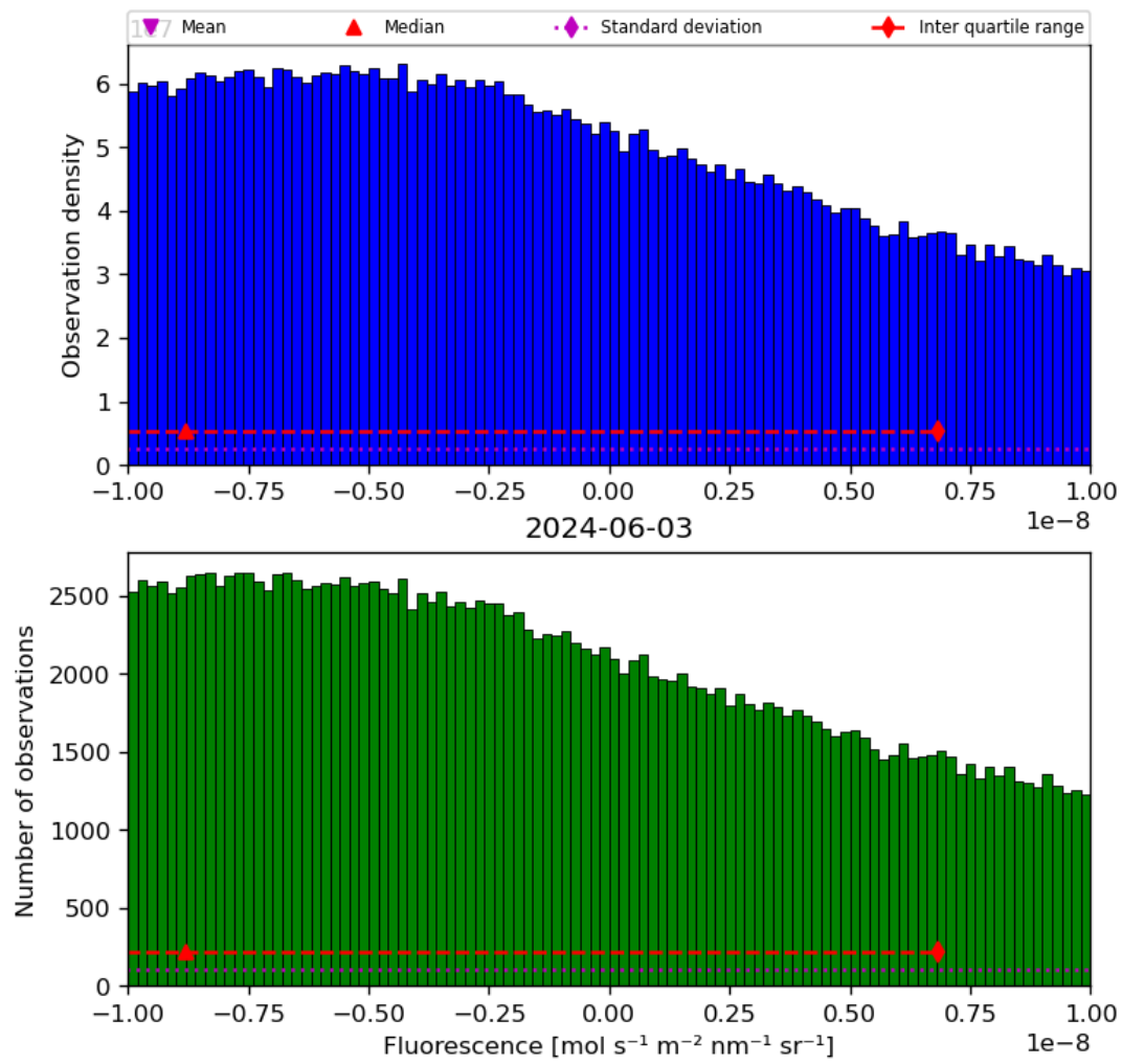
Figure 32: Histogram of “Fluorescence” for 2024-06-03 to 2024-06-04
