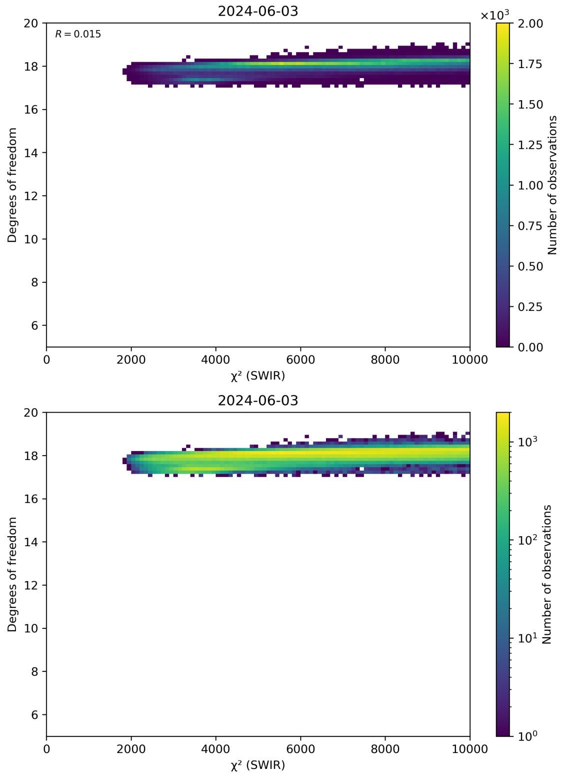
Figure 48: Scatter density plot of “ \chi^2 (SWIR)” against “Degrees of freedom” for 2024-06-03 to 2024-06-04.
