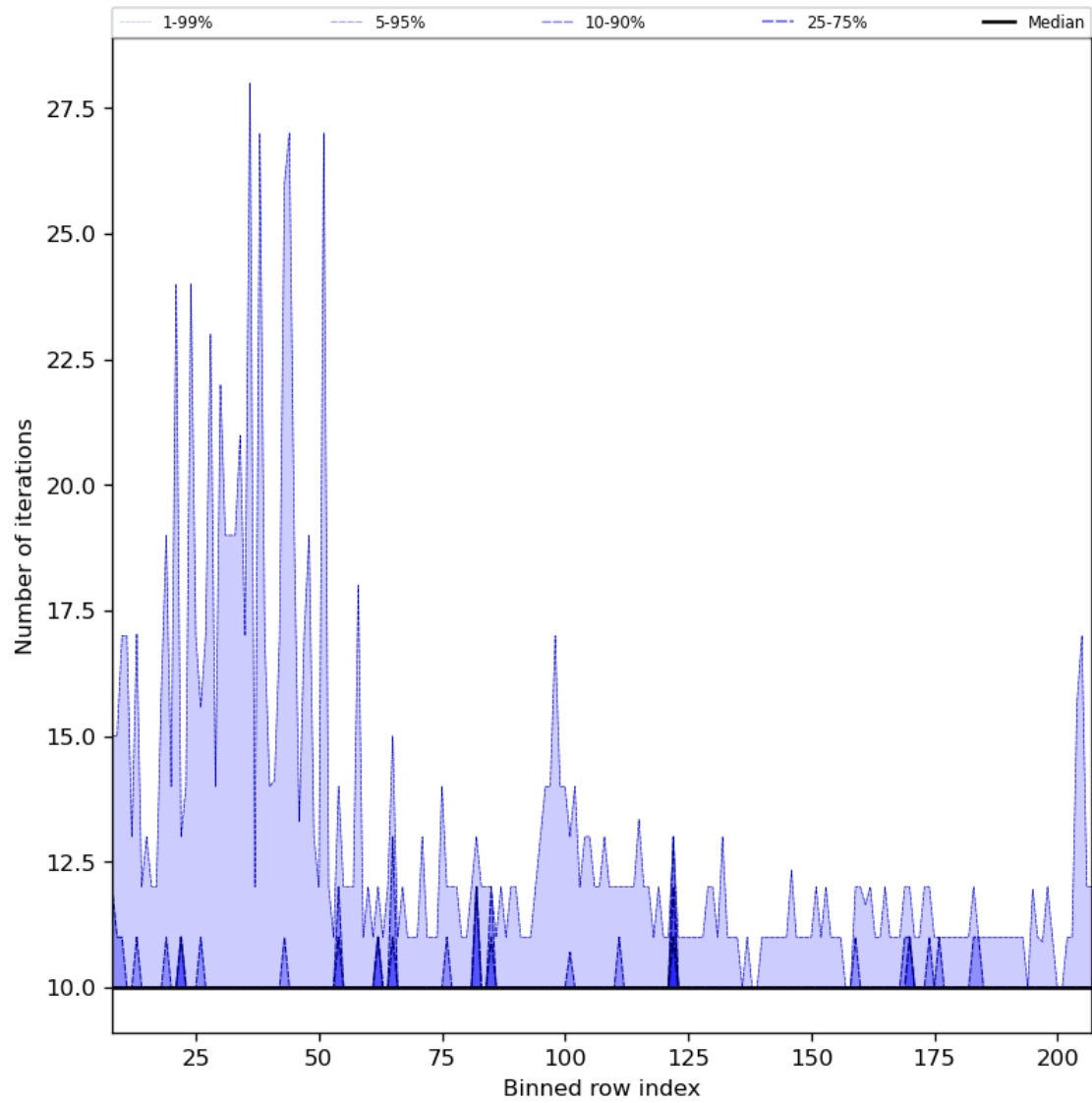
Figure 42: Along track statistics of “Number of iterations” for 2024-06-03 to 2024-06-04
