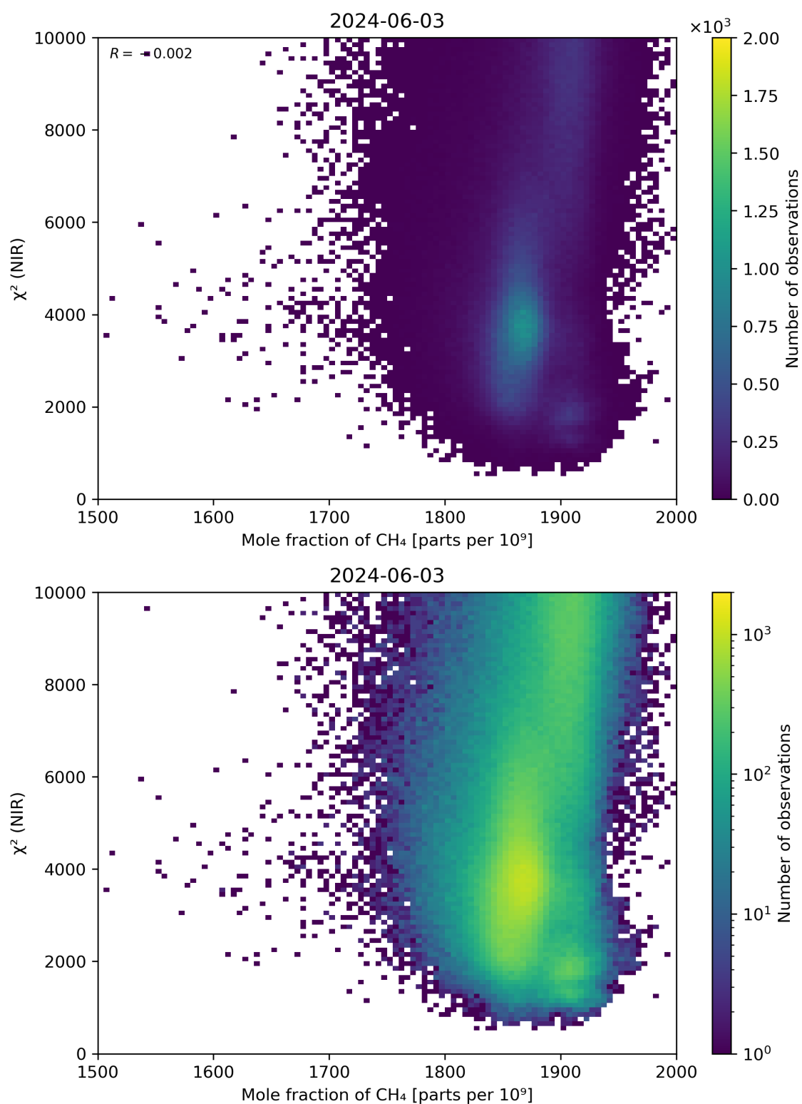
Figure 70: Scatter density plot of “Mole fraction of \text{CH}_4 ” against “ \chi^2 (NIR)” for 2024-06-03 to 2024-06-04.
