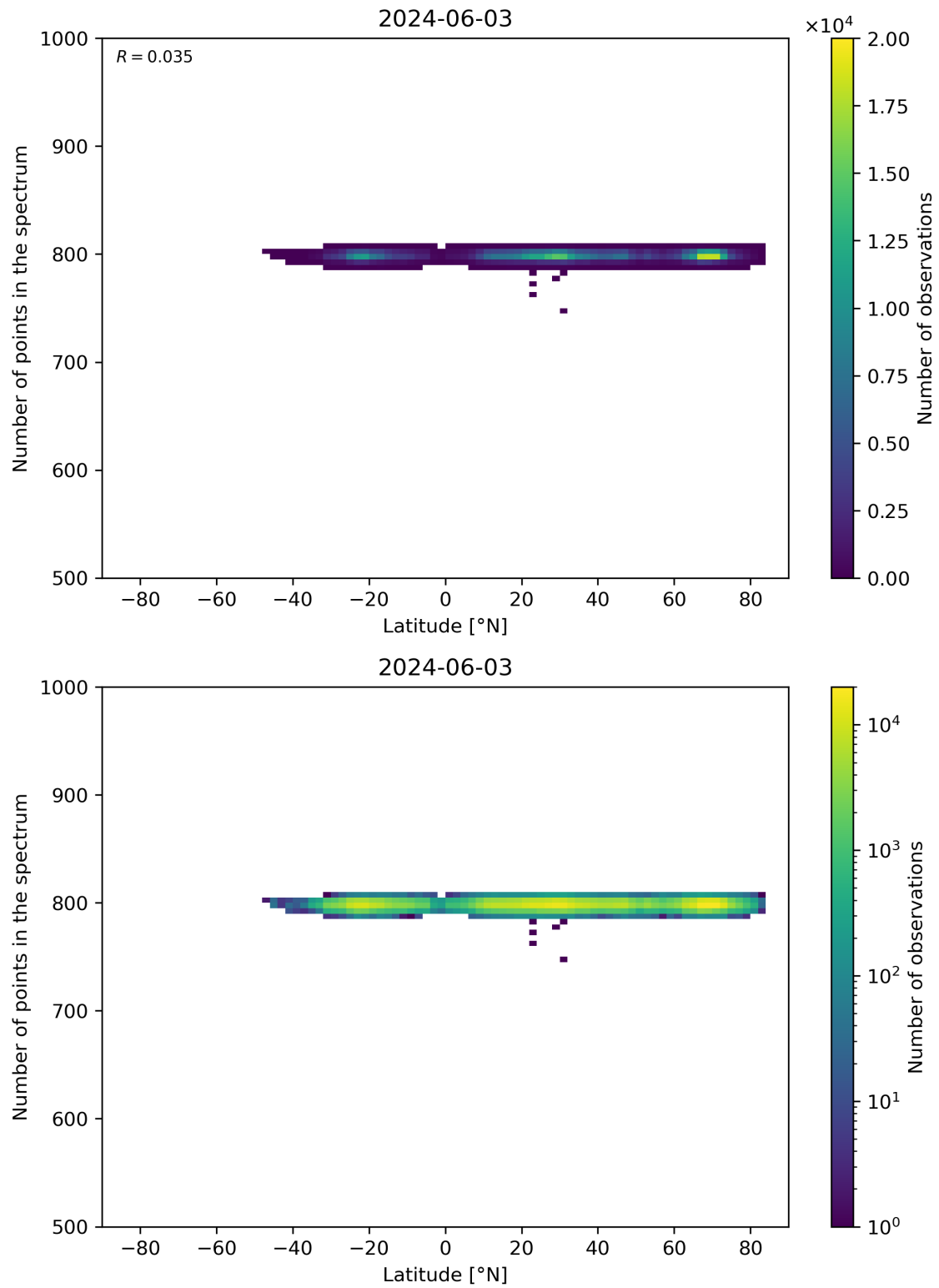
Figure 61: Scatter density plot of “Latitude” against “Number of points in the spectrum” for 2024-06-03 to 2024-06-04.
