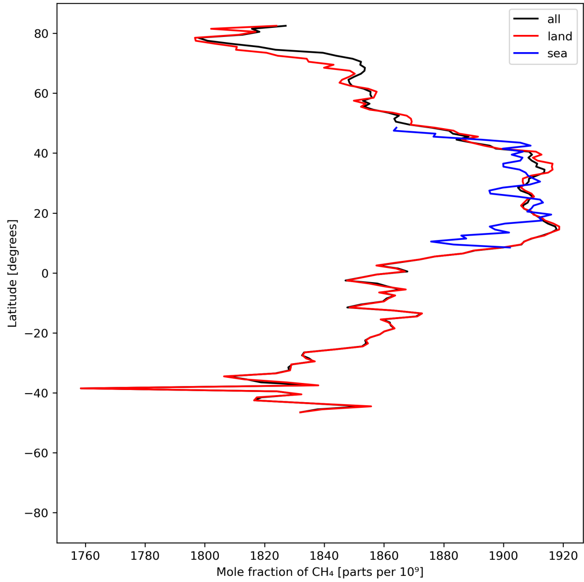
Figure 12: Zonal average of “Mole fraction of \text{CH}_4 ” for 2024-06-03 to 2024-06-04.
