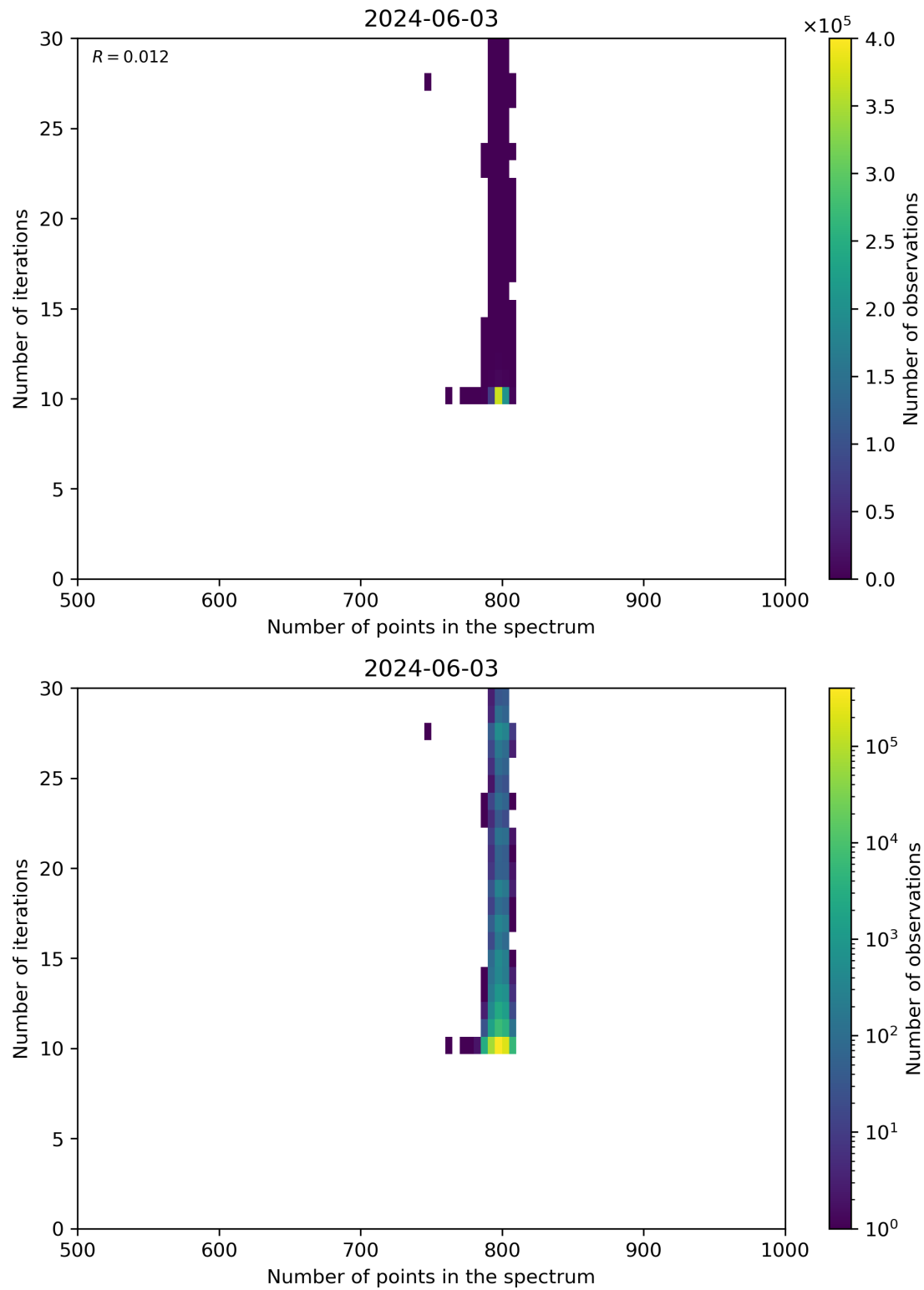
Figure 92: Scatter density plot of “Number of points in the spectrum” against “Number of iterations” for 2024-06-03 to 2024-06-04.
