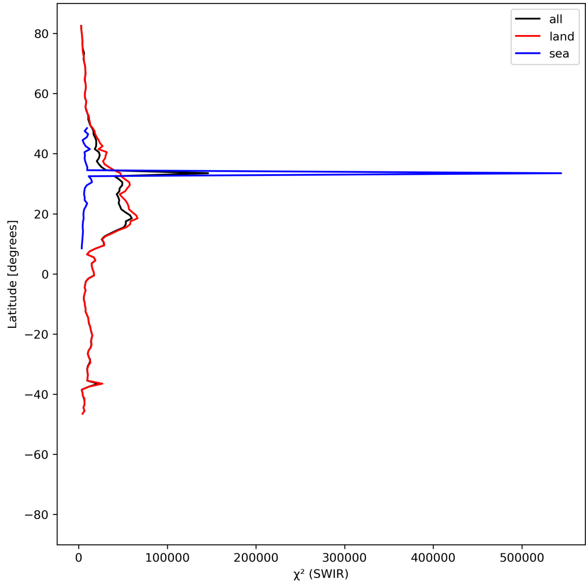
Figure 17: Zonal average of “ \chi^2 (SWIR)” for 2024-06-03 to 2024-06-04.
