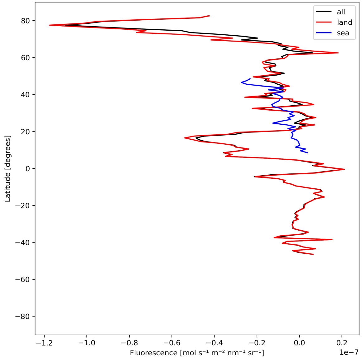
Figure 21: Zonal average of “Fluorescence” for 2024-06-03 to 2024-06-04.
