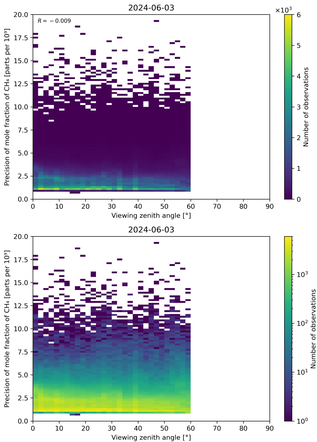
Figure 112: Scatter density plot of “Viewing zenith angle” against “Precision of mole fraction of CH 4 ” for 2024-06-03 to 2024-06-04.
