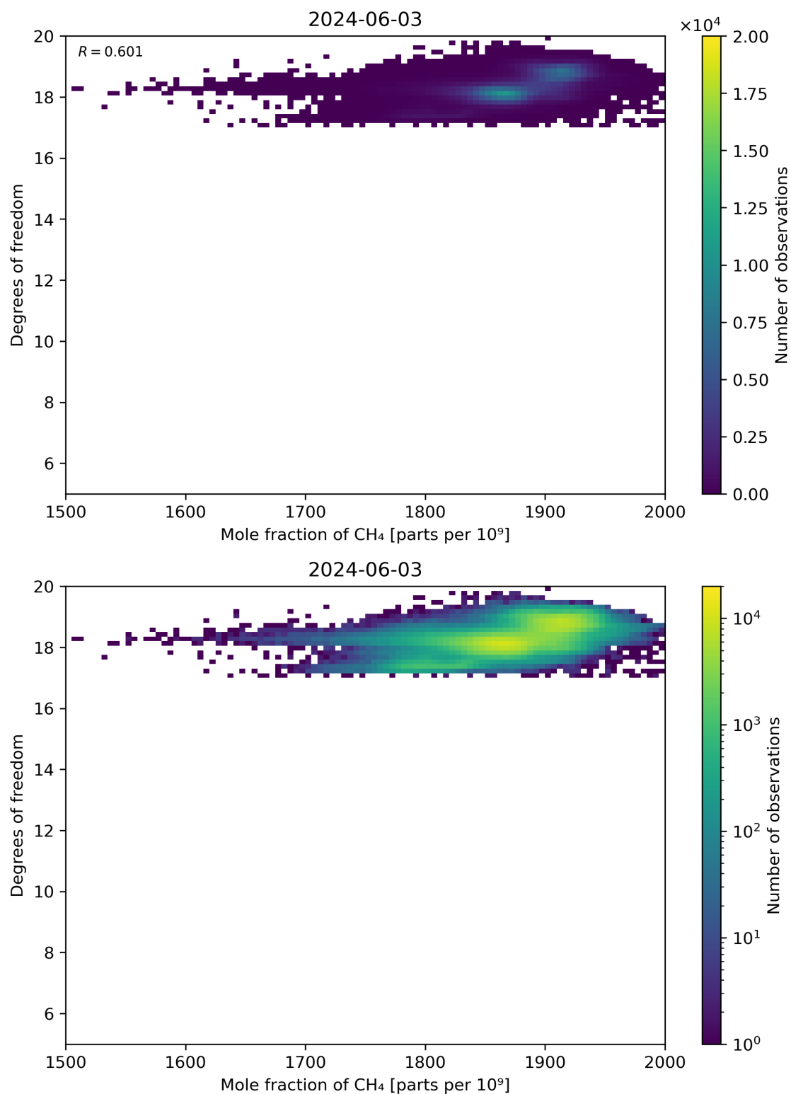
Figure 72: Scatter density plot of “Mole fraction of CH 4 ” against “Degrees of freedom” for 2024-06-03 to 2024-06-04.
