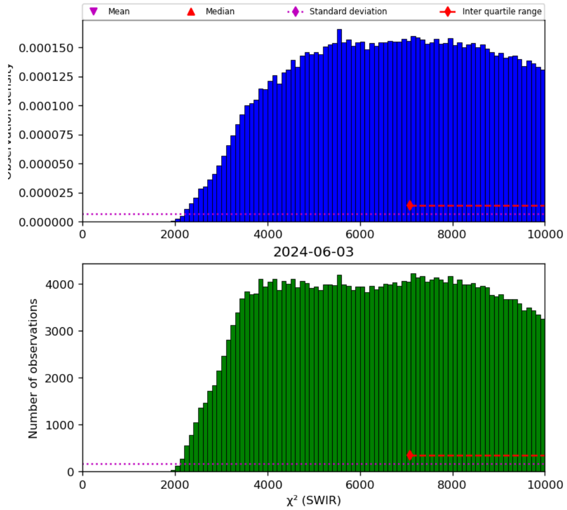
Figure 28: Histogram of “ \chi^2 (SWIR)” for 2024-06-03 to 2024-06-04
