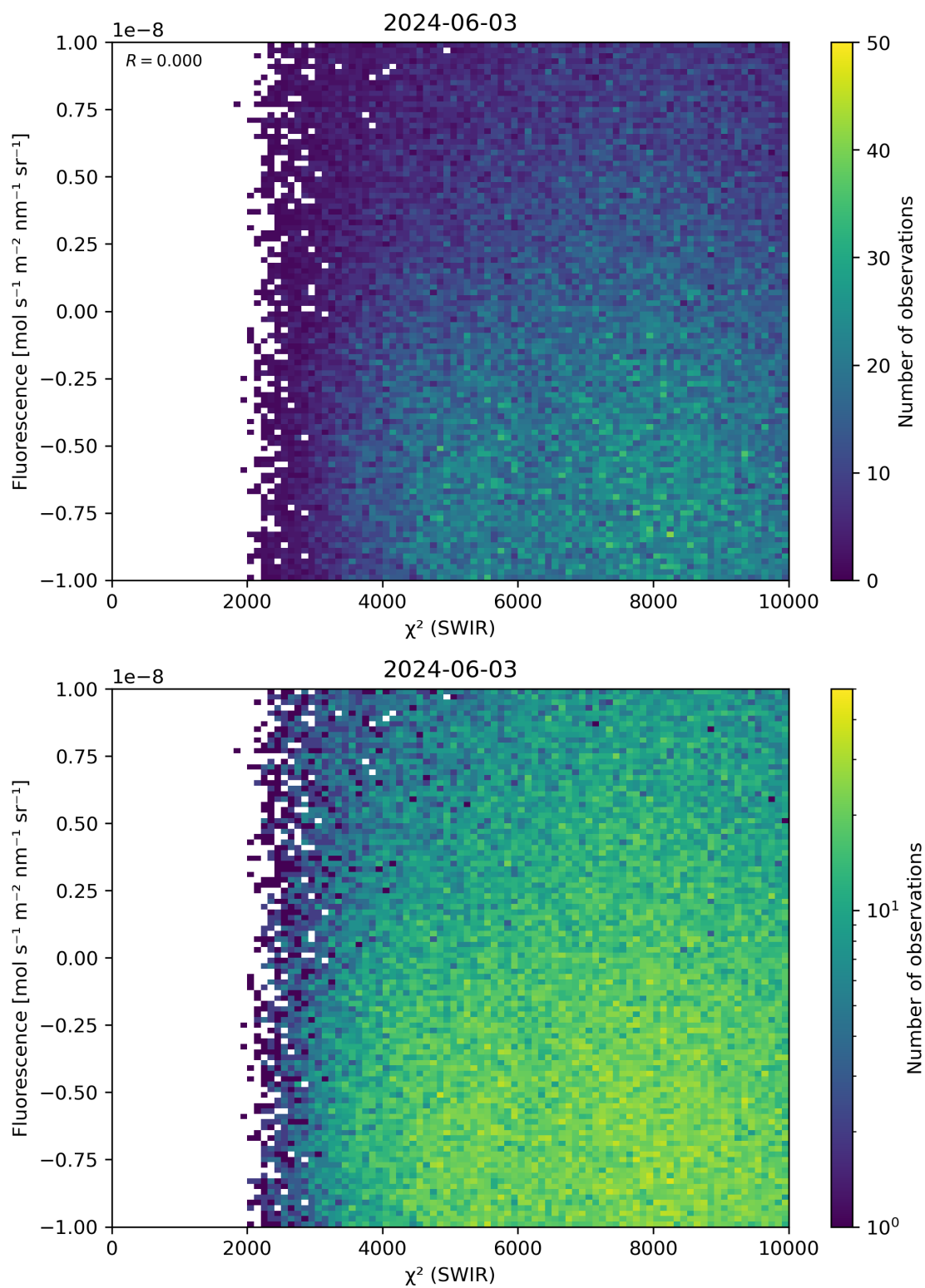
Figure 49: Scatter density plot of “ \chi^2 (SWIR)” against “Fluorescence” for 2024-06-03 to 2024-06-04.
