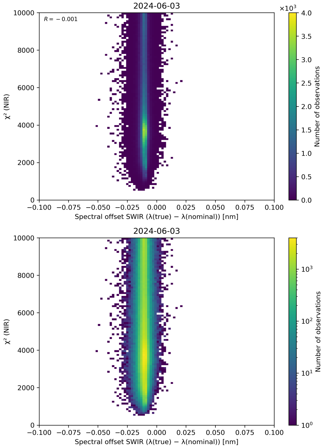
Figure 117: Scatter density plot of “Spectral offset SWIR ( \lambda(\text{true}) - \lambda(\text{nominal}) )” against “ \chi^2 (NIR)” for 2024-06-03 to 2024-06-04.
