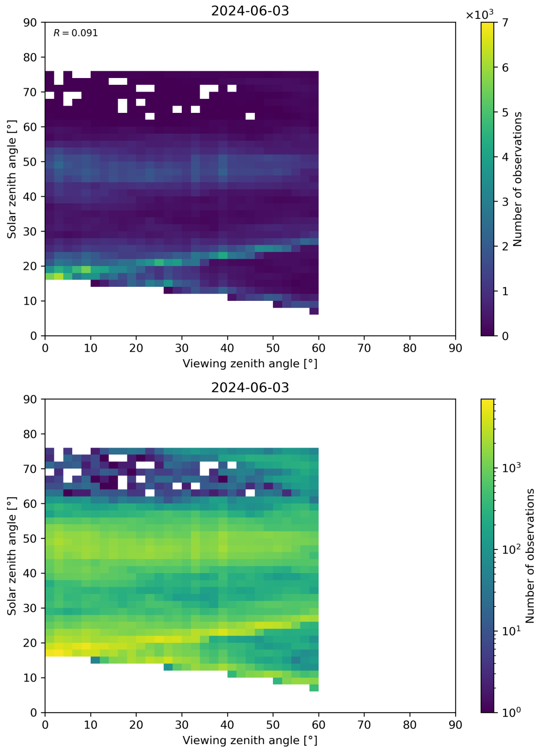
Figure 115: Scatter density plot of “Viewing zenith angle” against “Solar zenith angle” for 2024-06-03 to 2024-06-04.
