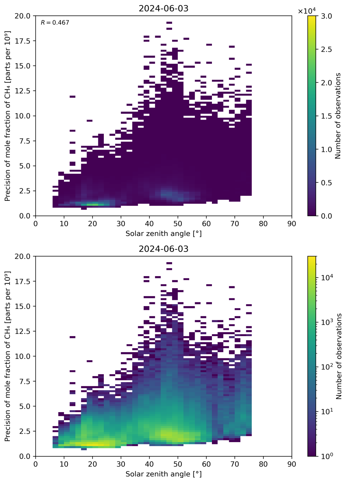
Figure 101: Scatter density plot of “Solar zenith angle” against “Precision of mole fraction of CH 4 ” for 2024-06-03 to 2024-06-04.
