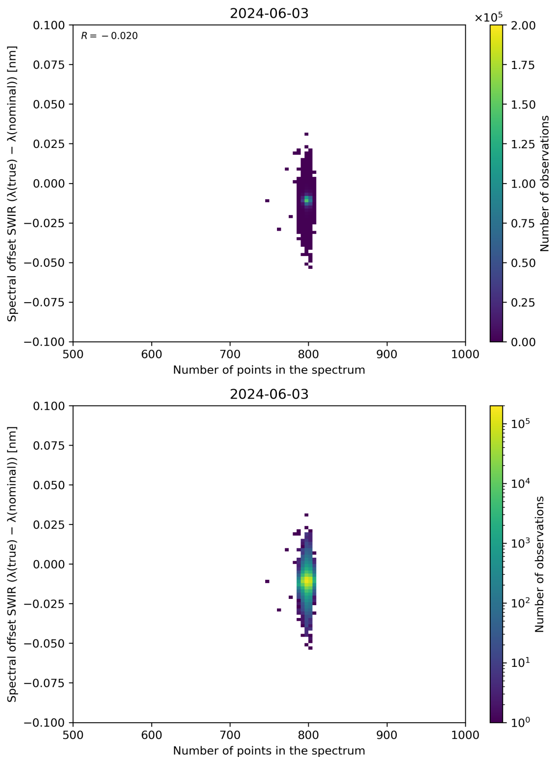
Figure 93: Scatter density plot of “Number of points in the spectrum” against “Spectral offset SWIR ( \lambda(\text{true}) - \lambda(\text{nominal}) )” for 2024-06-03 to 2024-06-04.
