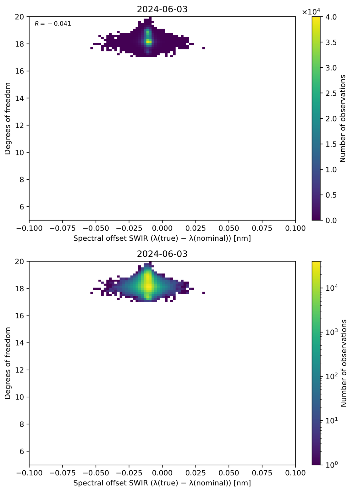
Figure 119: Scatter density plot of “Spectral offset SWIR ( \lambda(\text{true}) - \lambda(\text{nominal}) )” against “Degrees of freedom” for 2024-06-03 to 2024-06-04.
