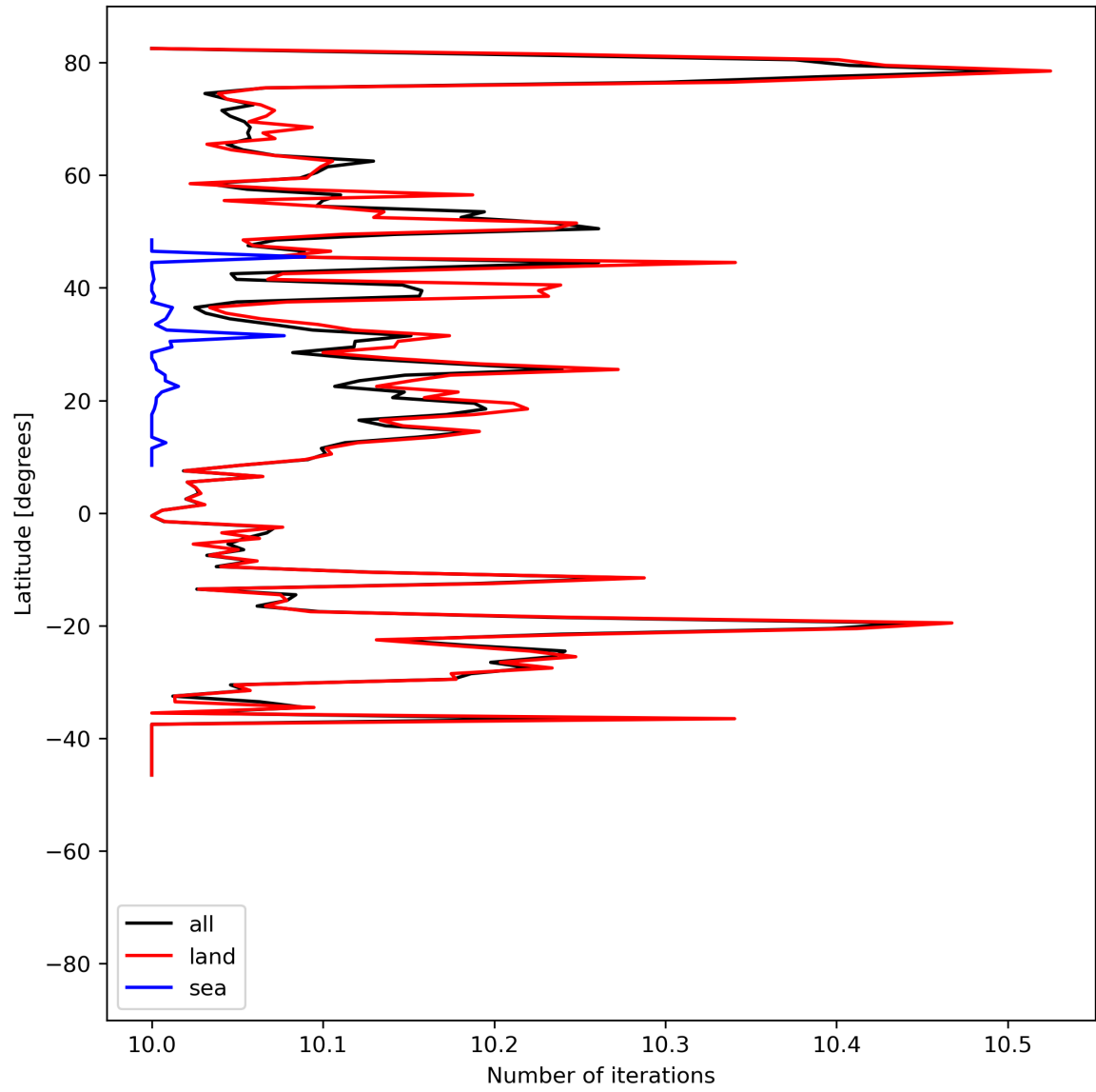
Figure 20: Zonal average of “Number of iterations” for 2024-06-03 to 2024-06-04.
