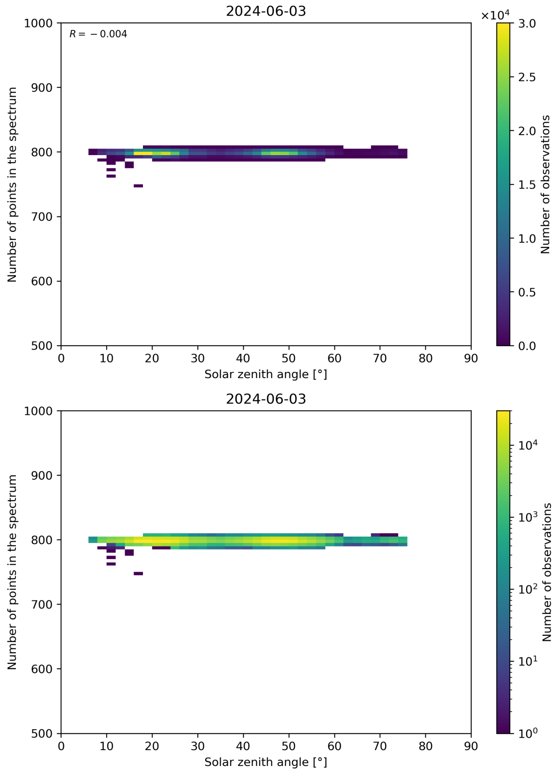
Figure 103: Scatter density plot of “Solar zenith angle” against “Number of points in the spectrum” for 2024-06-03 to 2024-06-04.
