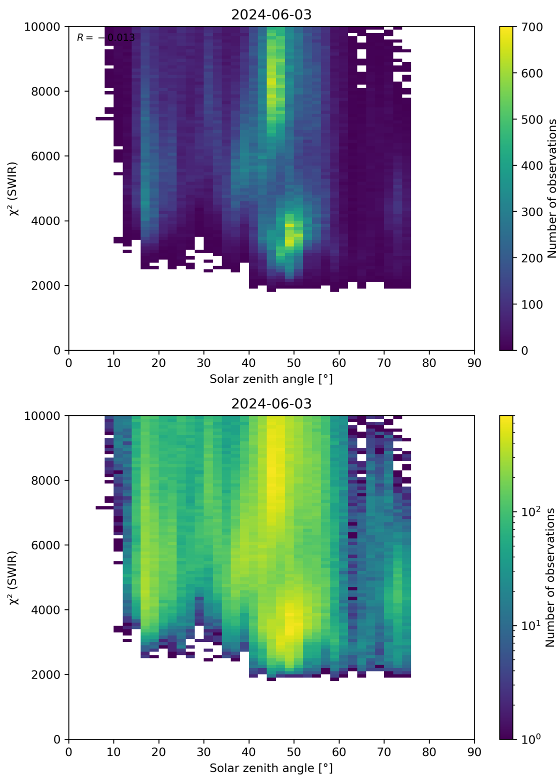
Figure 95: Scatter density plot of “Solar zenith angle” against “ \chi^2 (SWIR)” for 2024-06-03 to 2024-06-04.
