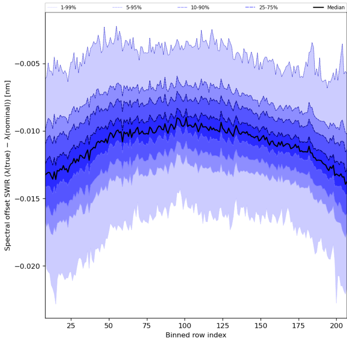
Figure 38: Along track statistics of “Spectral offset SWIR ( \lambda(\text{true}) - \lambda(\text{nominal}) )” for 2024-06-03 to 2024-06-04
