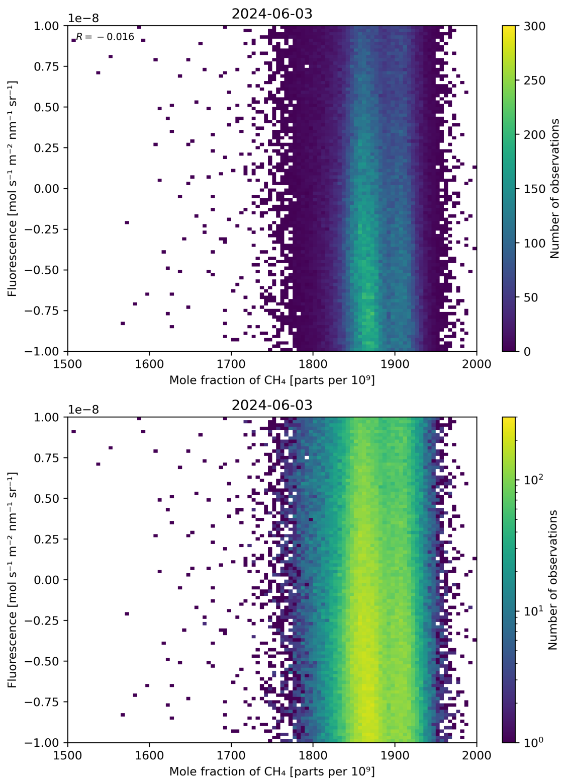
Figure 73: Scatter density plot of “Mole fraction of \text{CH}_4 ” against “Fluorescence” for 2024-06-03 to 2024-06-04.
