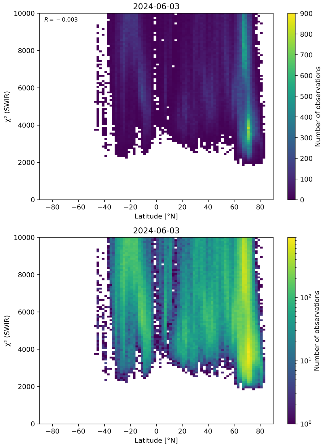
Figure 54: Scatter density plot of “Latitude” against “ \chi^2 (SWIR)” for 2024-06-03 to 2024-06-04.
