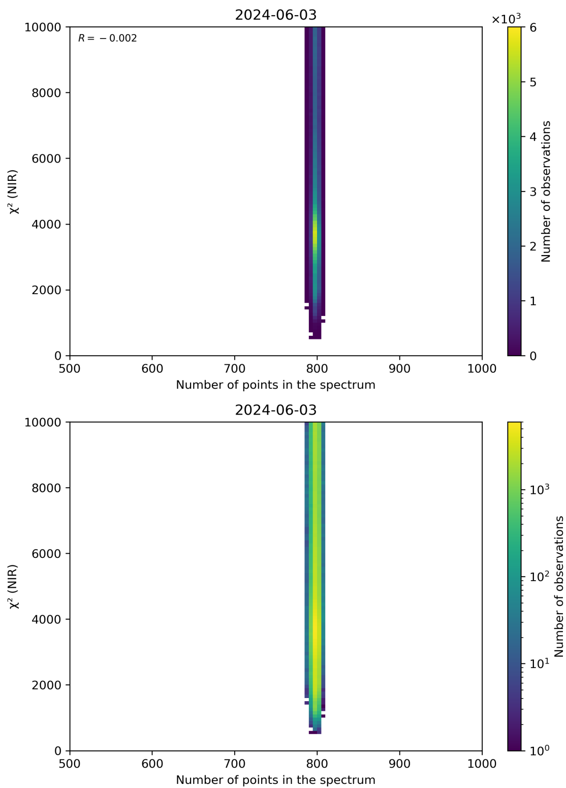
Figure 88: Scatter density plot of “Number of points in the spectrum” against “ \chi^2 (NIR)” for 2024-06-03 to 2024-06-04.
