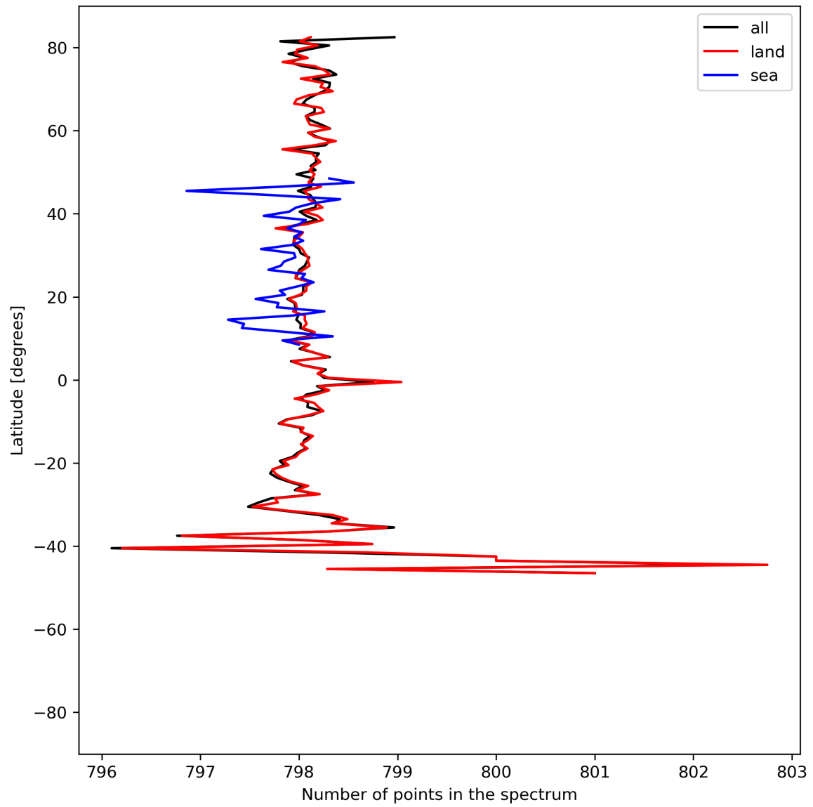
Figure 15: Zonal average of “Number of points in the spectrum” for 2024-06-03 to 2024-06-04.
