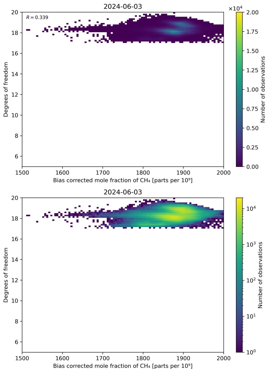
Figure 65: Scatter density plot of “Bias corrected mole fraction of CH 4 ” against “Degrees of freedom” for 2024-06-03 to 2024-06-04.
