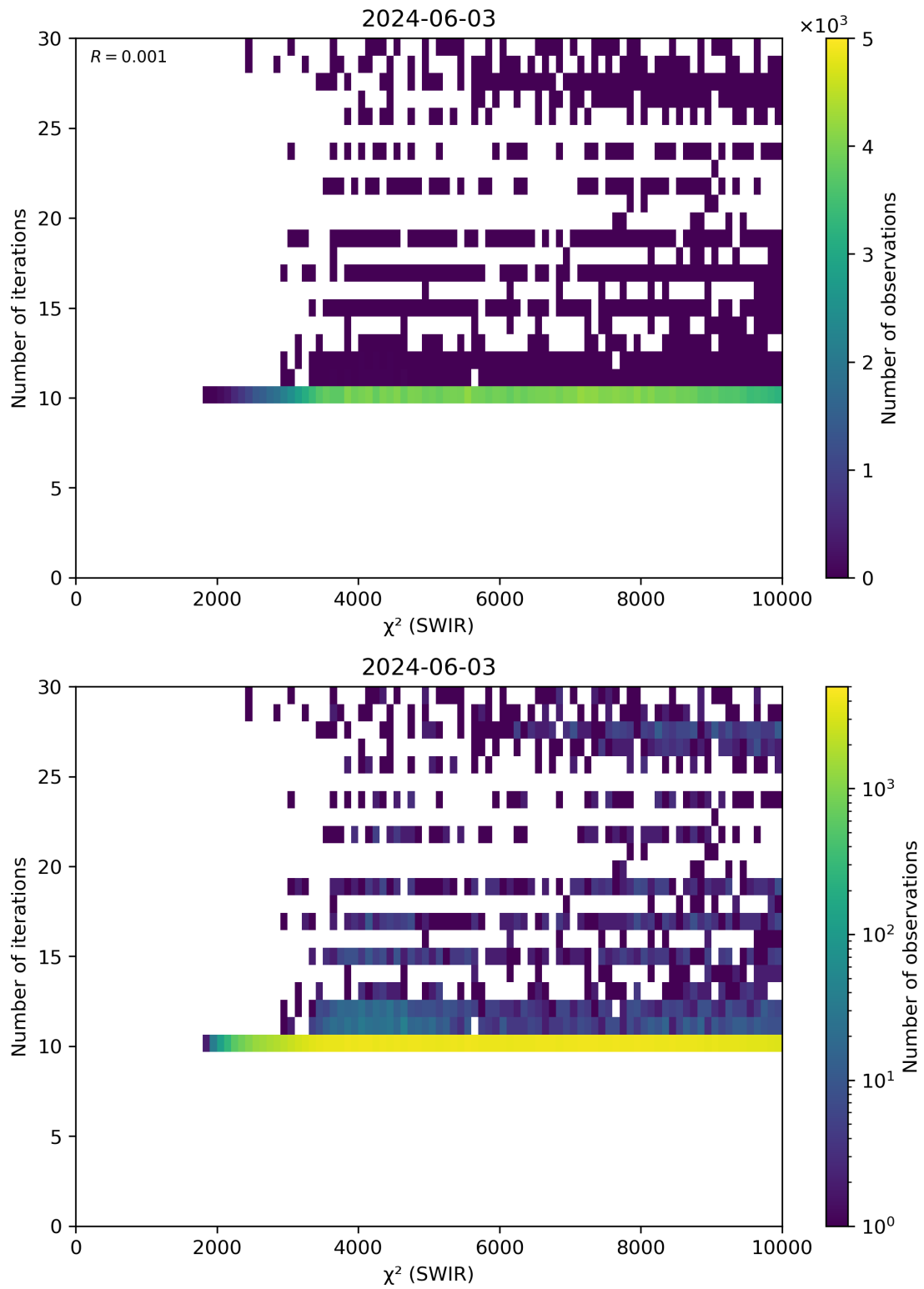
Figure 50: Scatter density plot of “ \chi^2 (SWIR)” against “Number of iterations” for 2024-06-03 to 2024-06-04.
