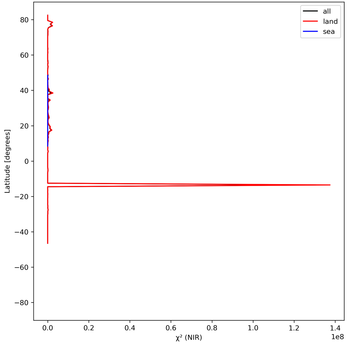
Figure 18: Zonal average of “ \chi^2 (NIR)” for 2024-06-03 to 2024-06-04.
