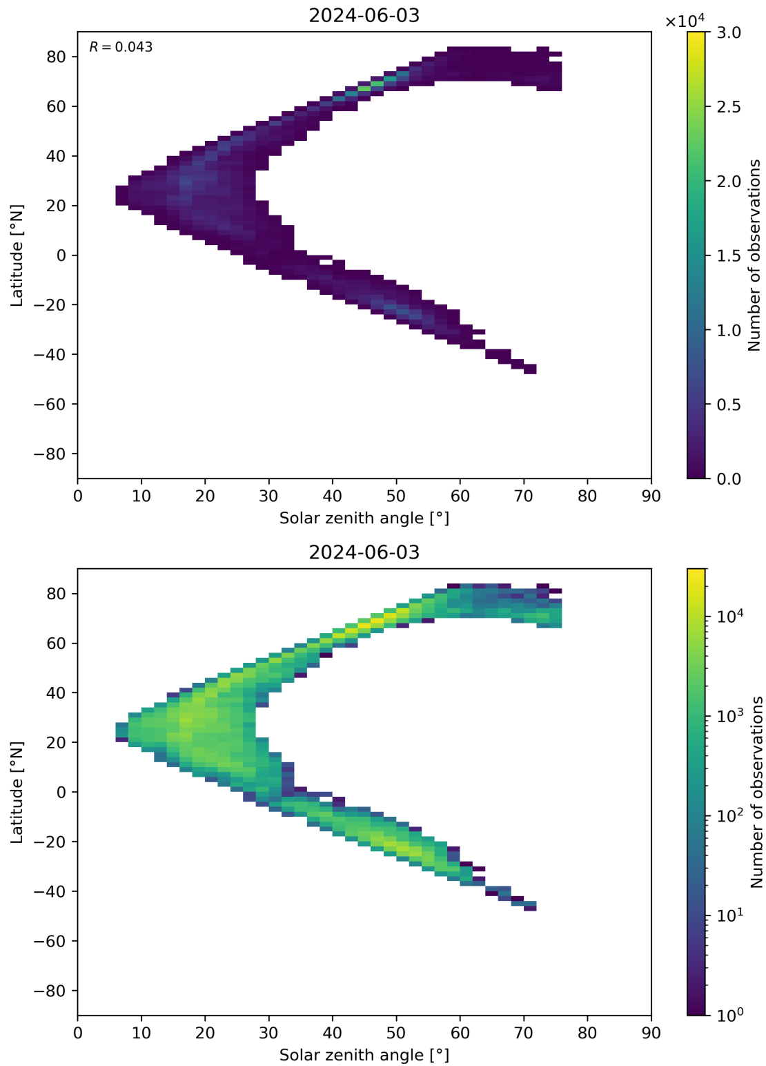
Figure 98: Scatter density plot of “Solar zenith angle” against “Latitude” for 2024-06-03 to 2024-06-04.
