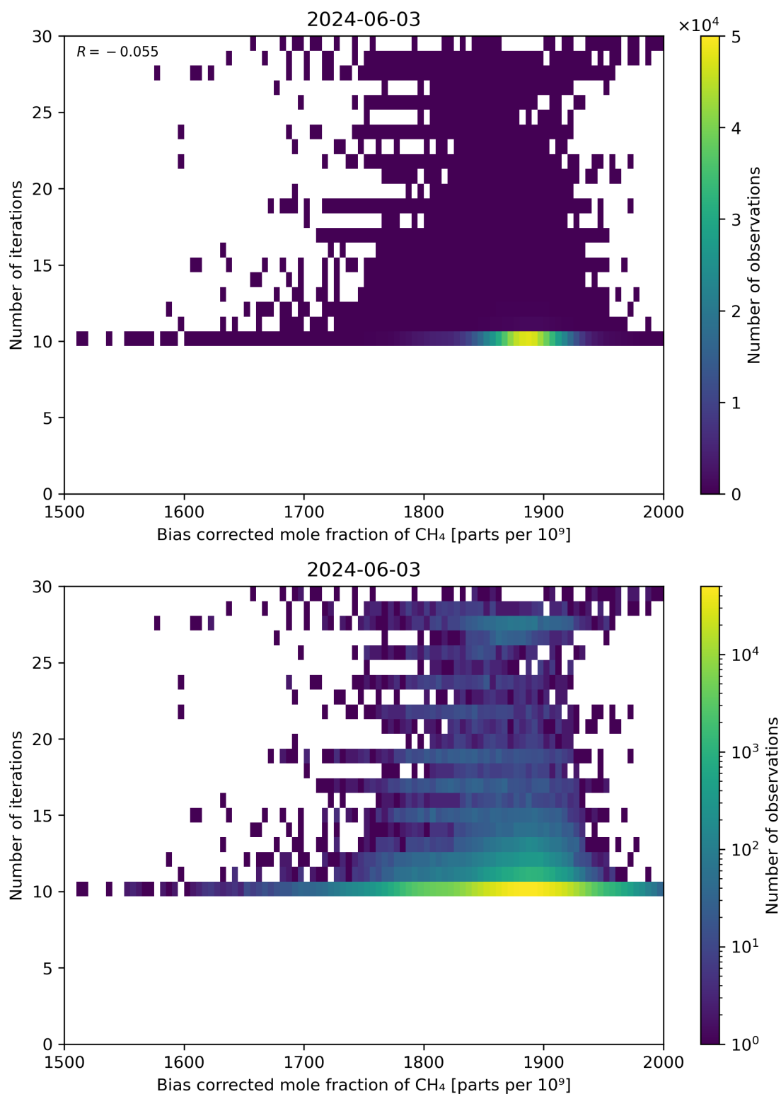
Figure 67: Scatter density plot of “Bias corrected mole fraction of CH 4 ” against “Number of iterations” for 2024-06-03 to 2024-06-04.
