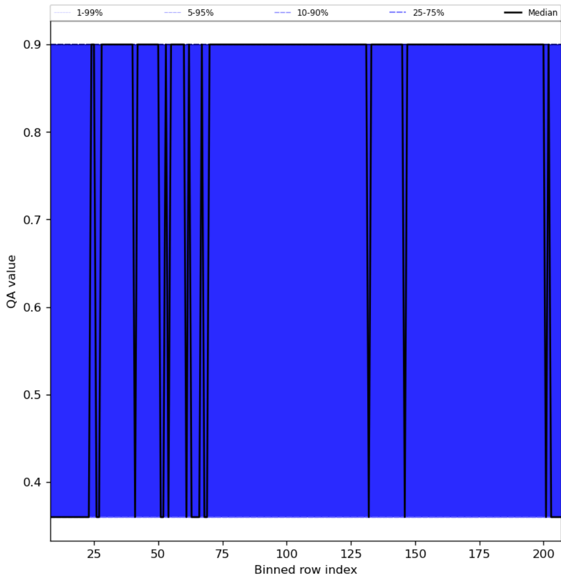
Figure 33: Along track statistics of “QA value” for 2024-06-03 to 2024-06-04
