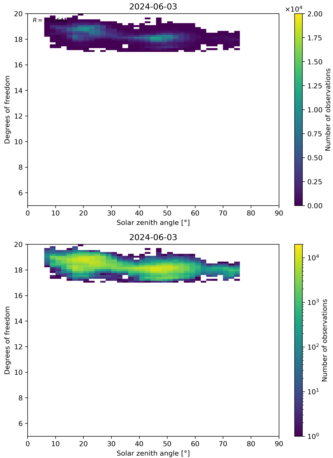
Figure 96: Scatter density plot of “Solar zenith angle” against “Degrees of freedom” for 2024-06-03 to 2024-06-04.
