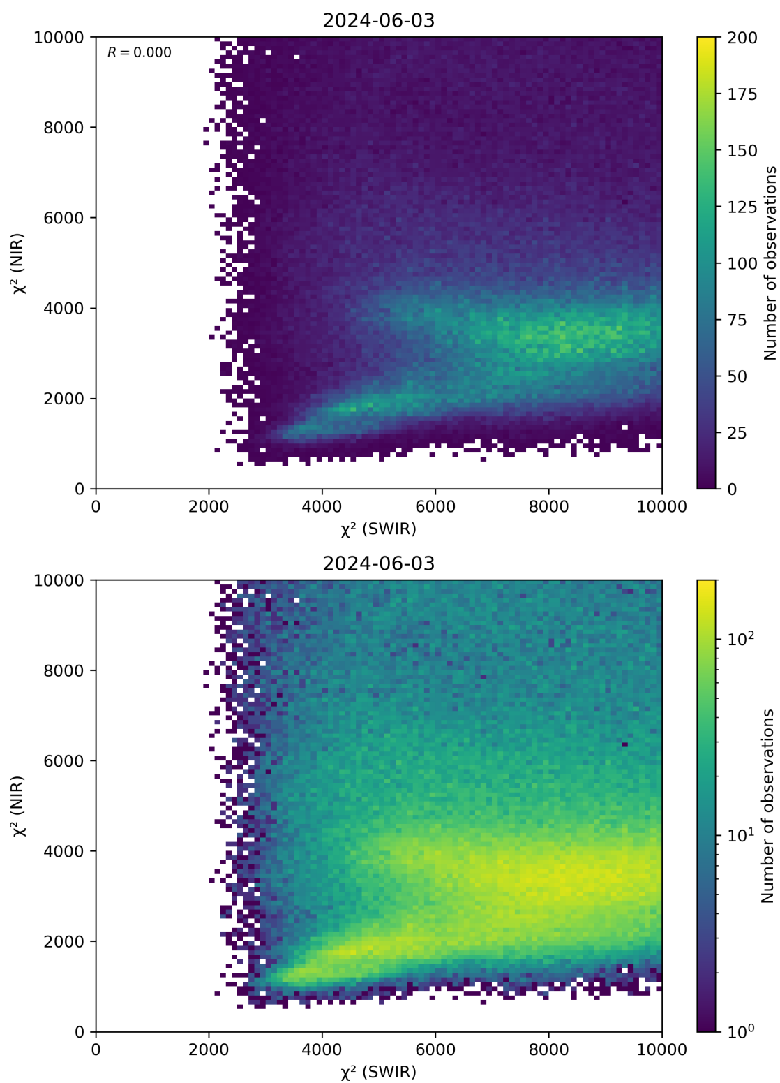
Figure 47: Scatter density plot of “ \chi^2 (SWIR)” against “ \chi^2 (NIR)” for 2024-06-03 to 2024-06-04.
