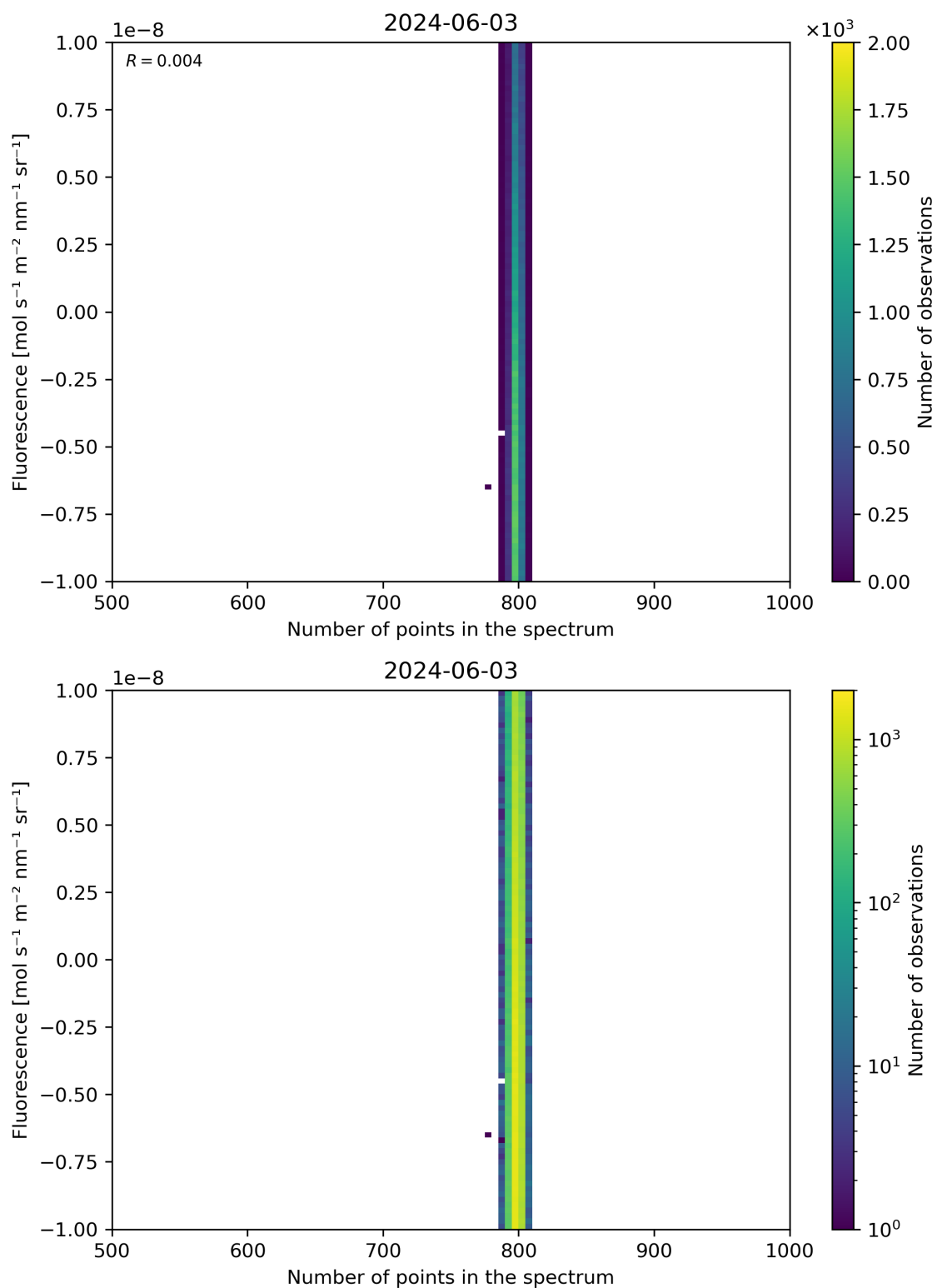
Figure 91: Scatter density plot of “Number of points in the spectrum” against “Fluorescence” for 2024-06-03 to 2024-06-04.
