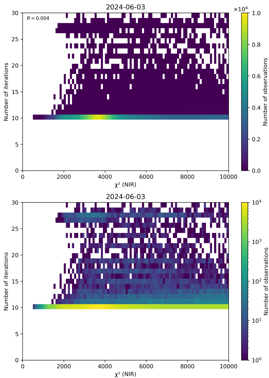
Figure 46: Scatter density plot of “ \chi^2 (NIR)” against “Number of iterations” for 2024-06-03 to 2024-06-04.
