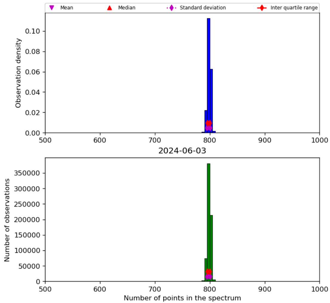
Figure 26: Histogram of “Number of points in the spectrum” for 2024-06-03 to 2024-06-04
