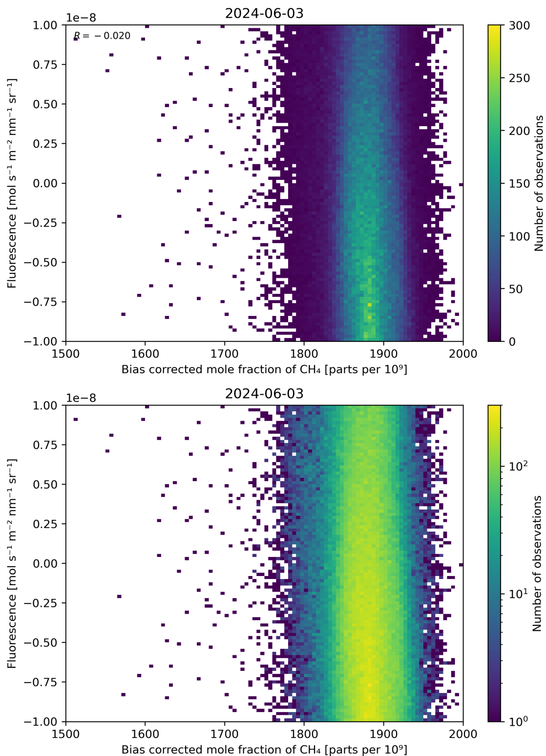
Figure 66: Scatter density plot of “Bias corrected mole fraction of \text{CH}_4 ” against “Fluorescence” for 2024-06-03 to 2024-06-04.
