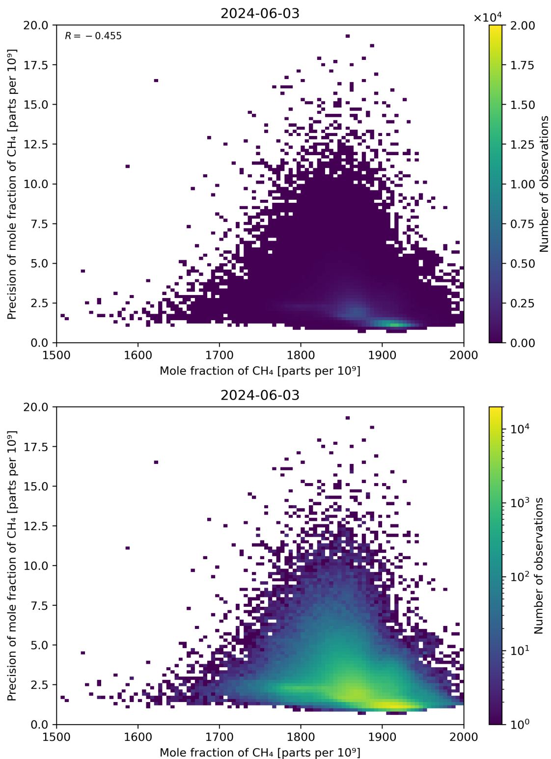
Figure 75: Scatter density plot of “Mole fraction of CH 4 ” against “Precision of mole fraction of CH 4 ” for 2024-06-03 to 2024-06-04.
