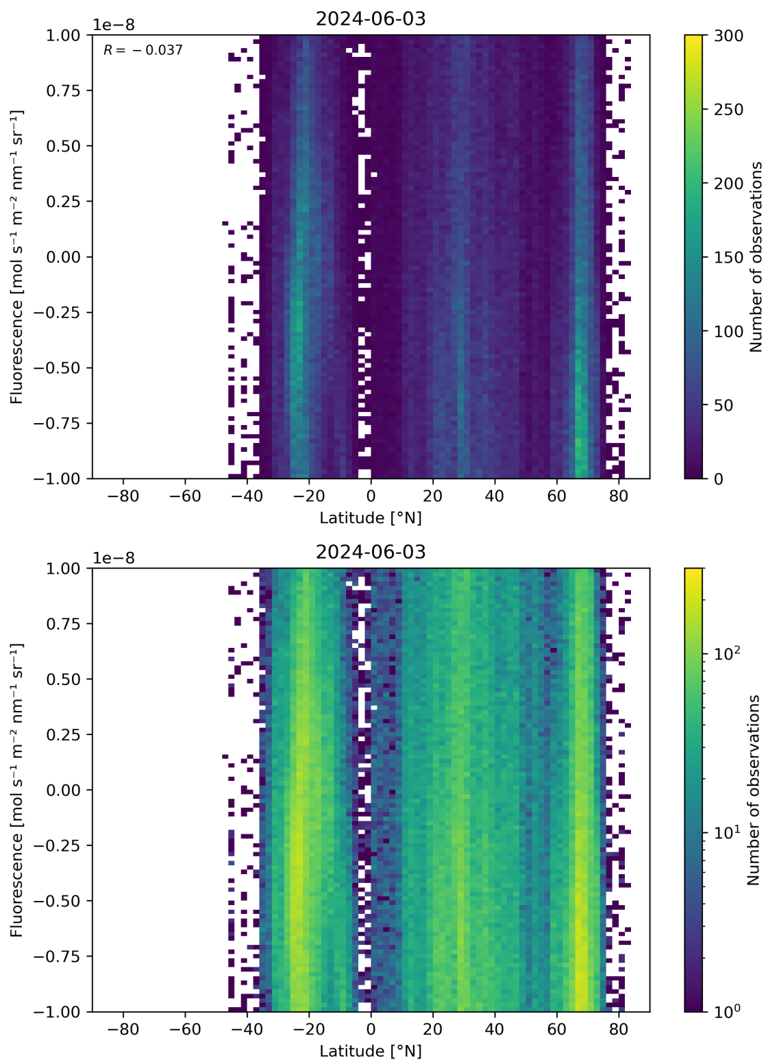
Figure 56: Scatter density plot of “Latitude” against “Fluorescence” for 2024-06-03 to 2024-06-04.
