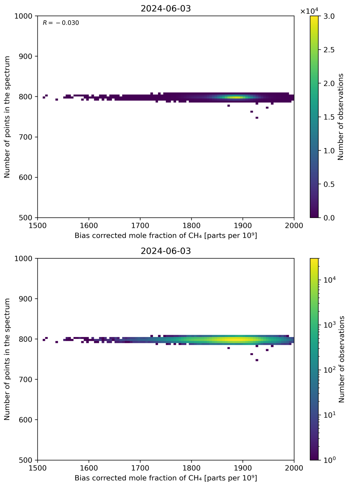
Figure 68: Scatter density plot of “Bias corrected mole fraction of CH 4 ” against “Number of points in the spectrum” for 2024-06-03 to 2024-06-04.
