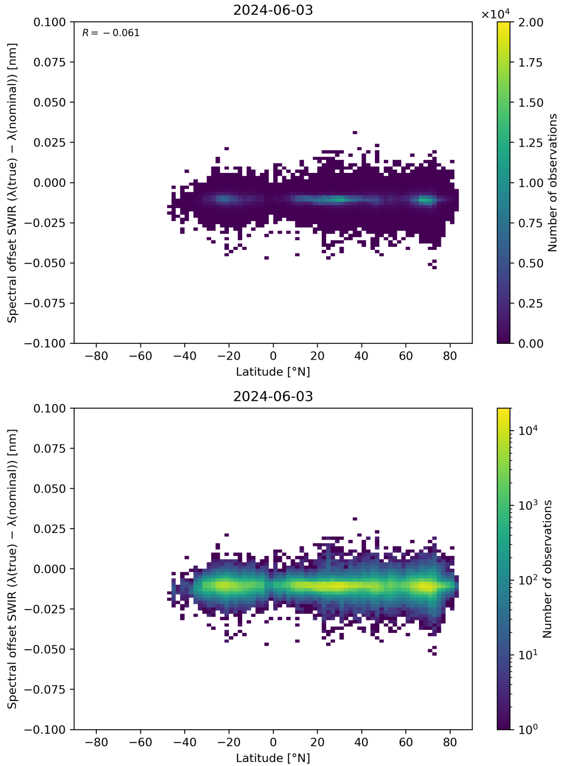
Figure 62: Scatter density plot of “Latitude” against “Spectral offset SWIR ( \lambda(\text{true}) - \lambda(\text{nominal}) )” for 2024-06-03 to 2024-06-04.
