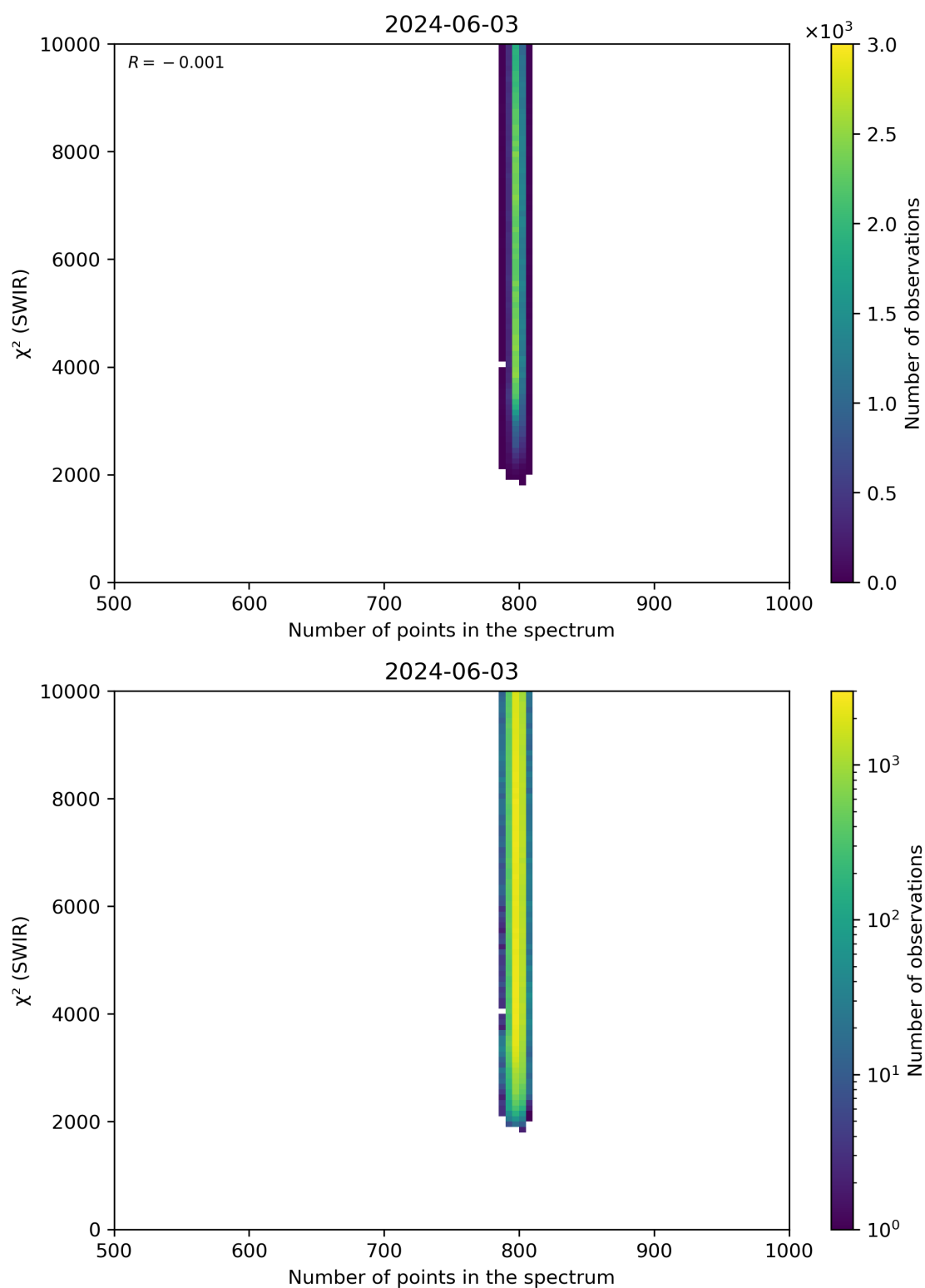
Figure 89: Scatter density plot of “Number of points in the spectrum” against “ \chi^2 (SWIR)” for 2024-06-03 to 2024-06-04.
