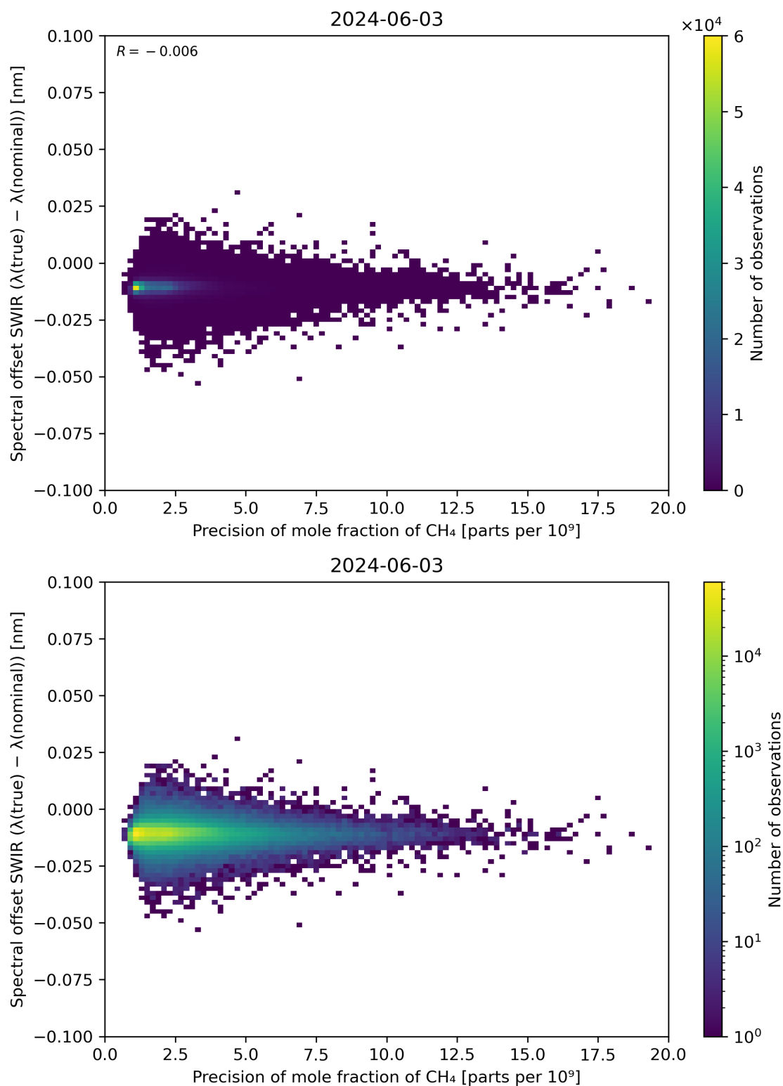
Figure 85: Scatter density plot of “Precision of mole fraction of CH 4 ” against “Spectral offset SWIR ( \lambda(\text{true}) - \lambda(\text{nominal}) )” for 2024-06-03 to 2024-06-04.
