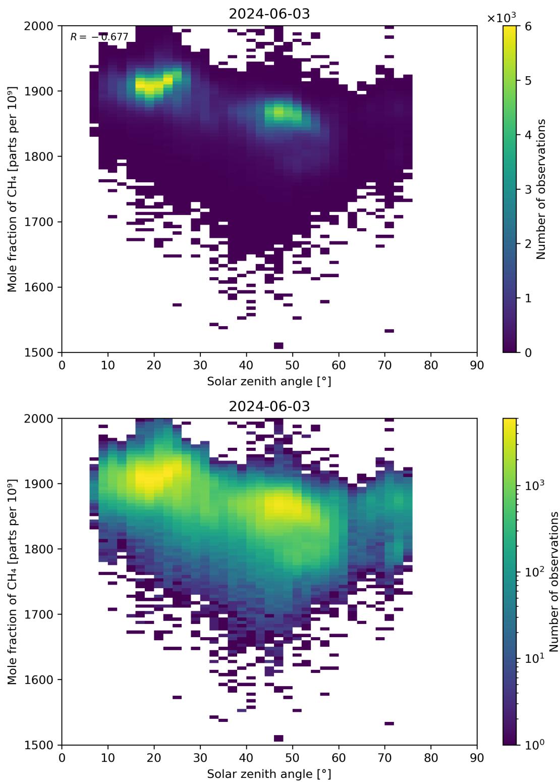
Figure 99: Scatter density plot of “Solar zenith angle” against “Mole fraction of \text{CH}_4 ” for 2024-06-03 to 2024-06-04.
