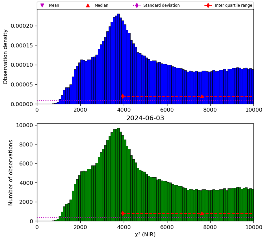
Figure 29: Histogram of " \chi^2 (NIR)" for 2024-06-03 to 2024-06-04
