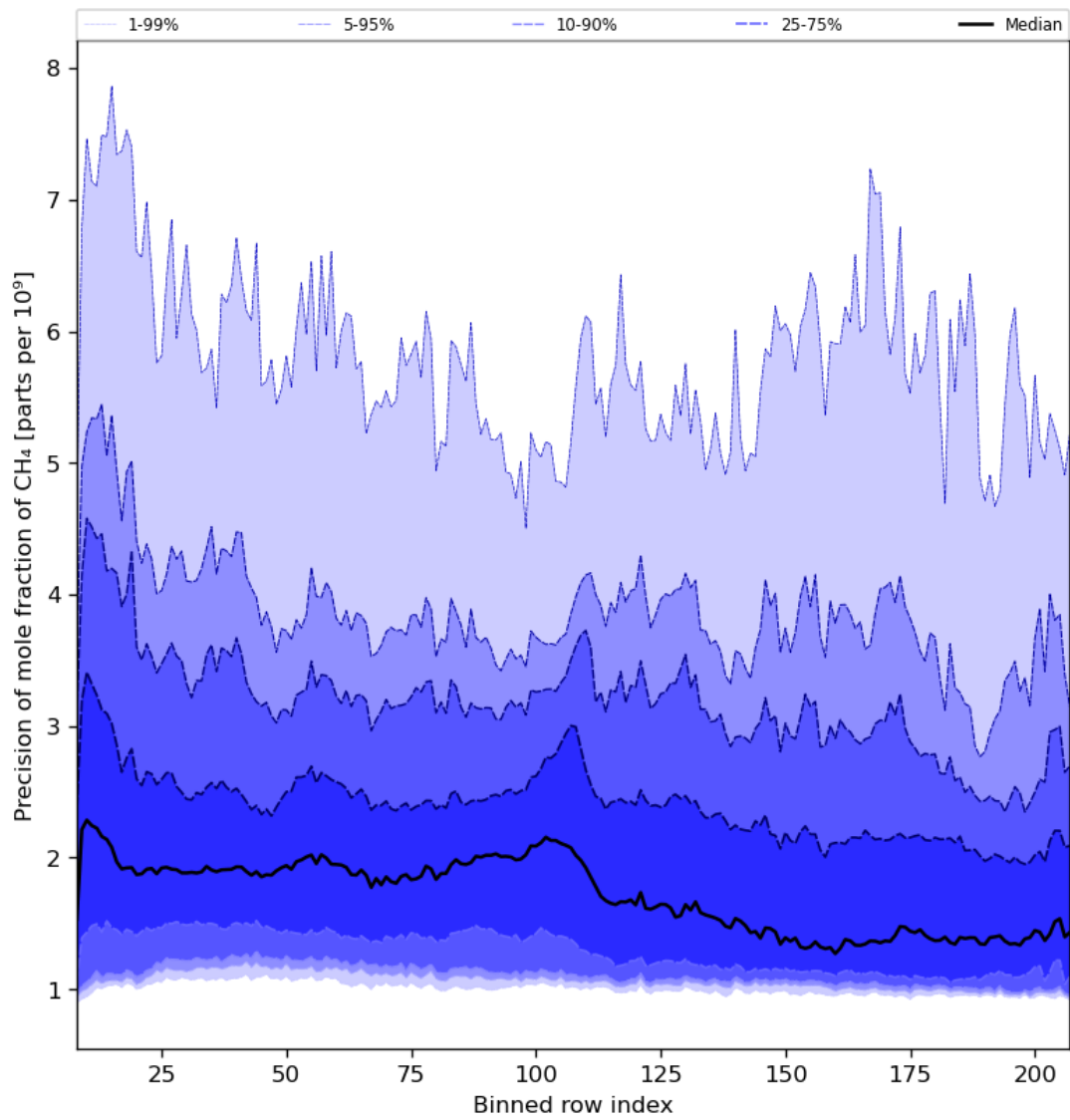
Figure 35: Along track statistics of “Precision of mole fraction of CH 4 ” for 2024-06-03 to 2024-06-04
