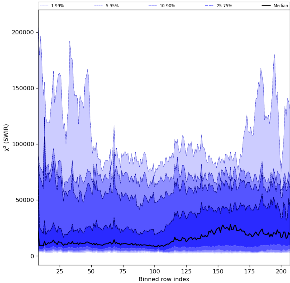
Figure 39: Along track statistics of “ \chi^2 (SWIR)” for 2024-06-03 to 2024-06-04
