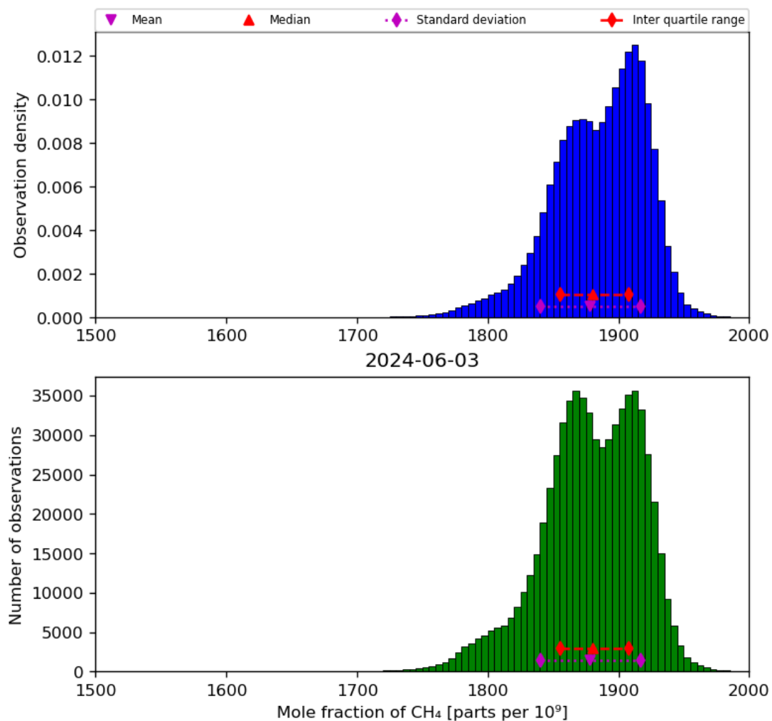
Figure 23: Histogram of “Mole fraction of CH 4 ” for 2024-06-03 to 2024-06-04
