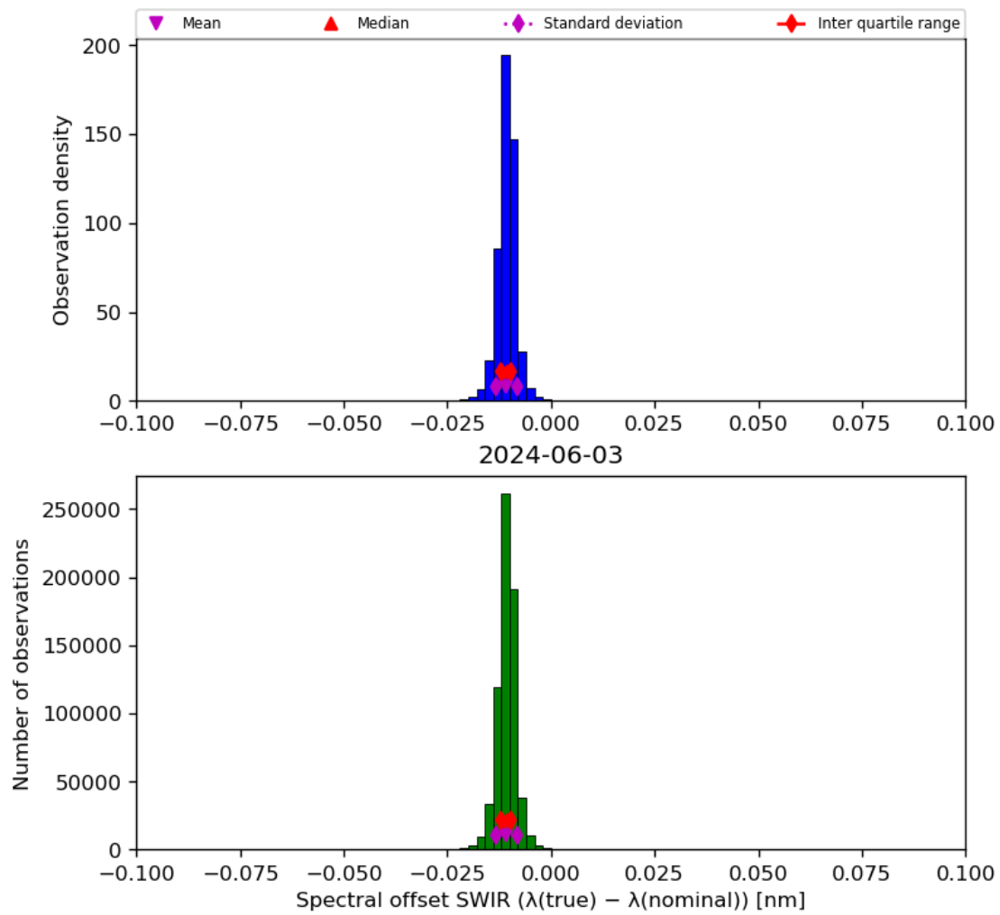
Figure 27: Histogram of “Spectral offset SWIR ( \lambda(\text{true}) - \lambda(\text{nominal}) )” for 2024-06-03 to 2024-06-04
