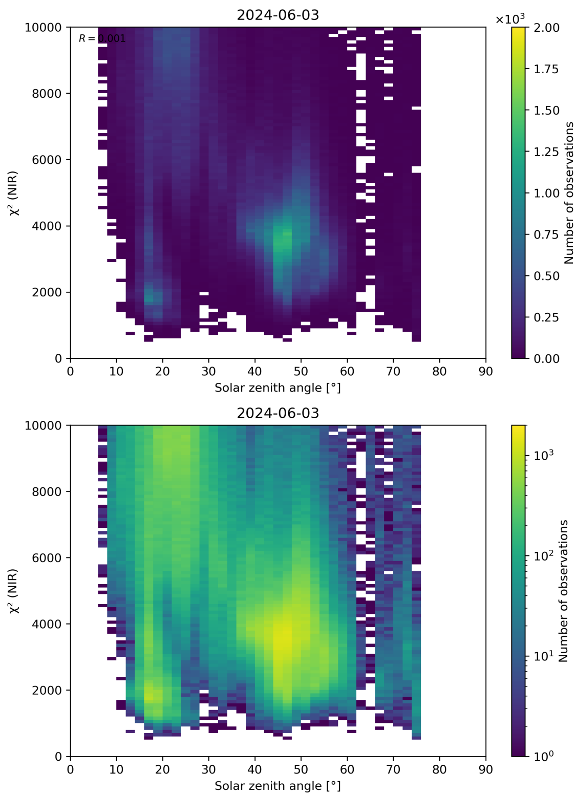
Figure 94: Scatter density plot of “Solar zenith angle” against “ \chi^2 (NIR)” for 2024-06-03 to 2024-06-04.
