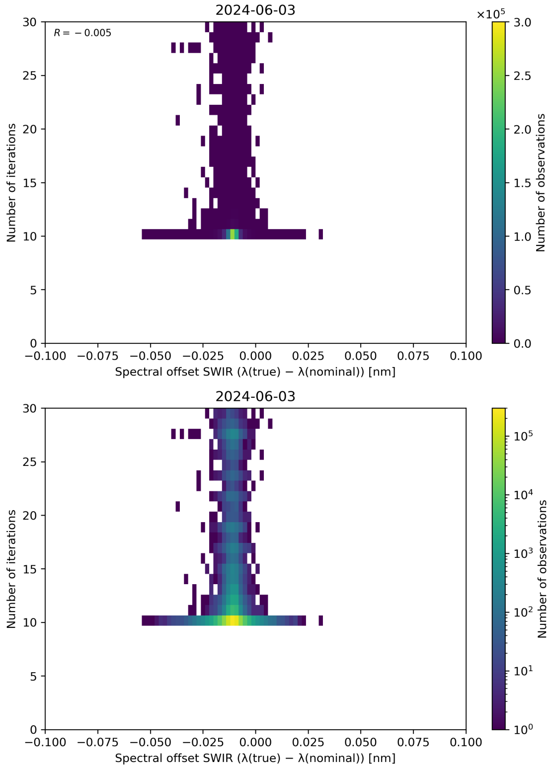
Figure 121: Scatter density plot of “Spectral offset SWIR ( \lambda(\text{true}) - \lambda(\text{nominal}) )” against “Number of iterations” for 2024-06-03 to 2024-06-04.
