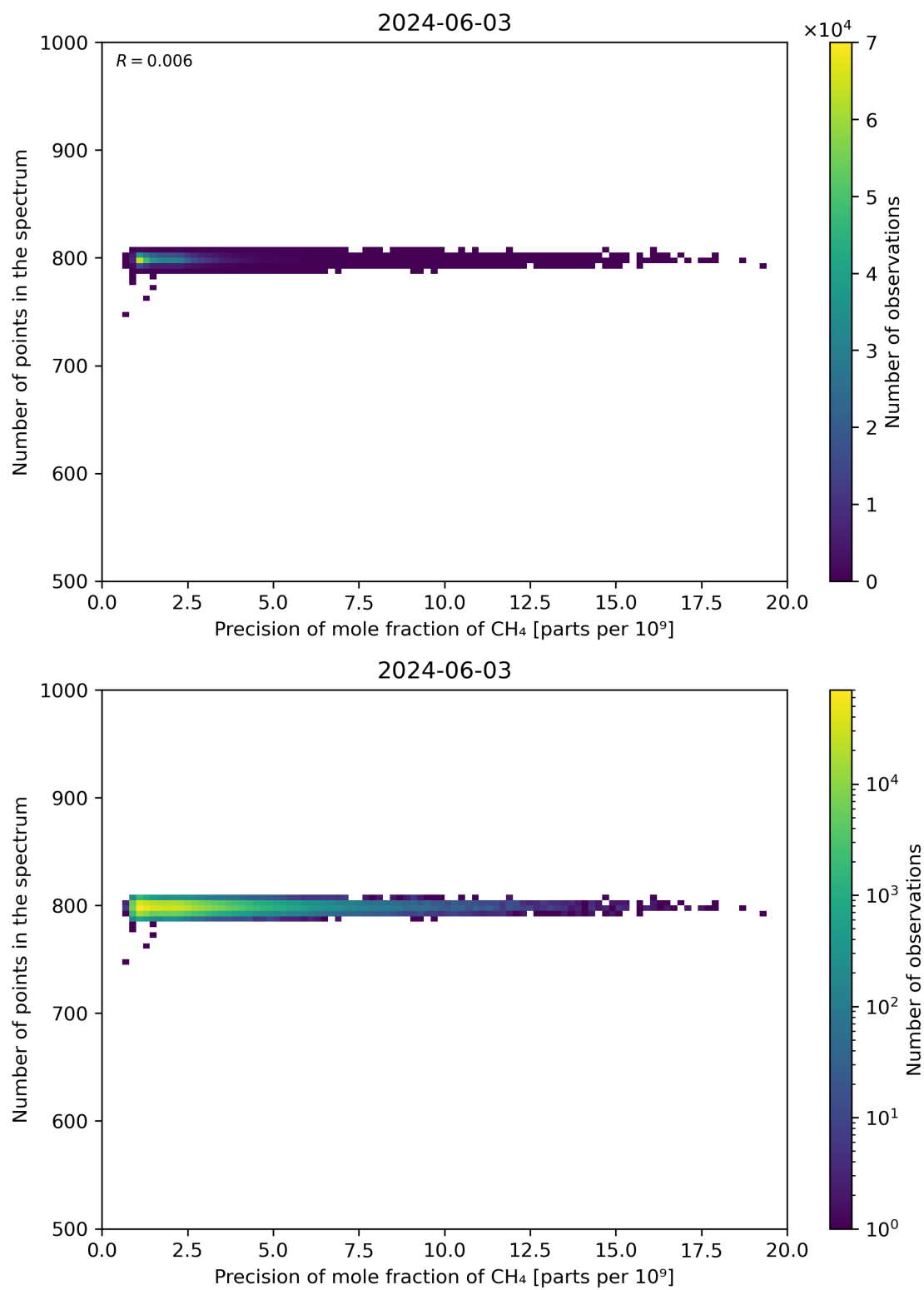
Figure 84: Scatter density plot of “Precision of mole fraction of CH 4 ” against “Number of points in the spectrum” for 2024-06-03 to 2024-06-04.
