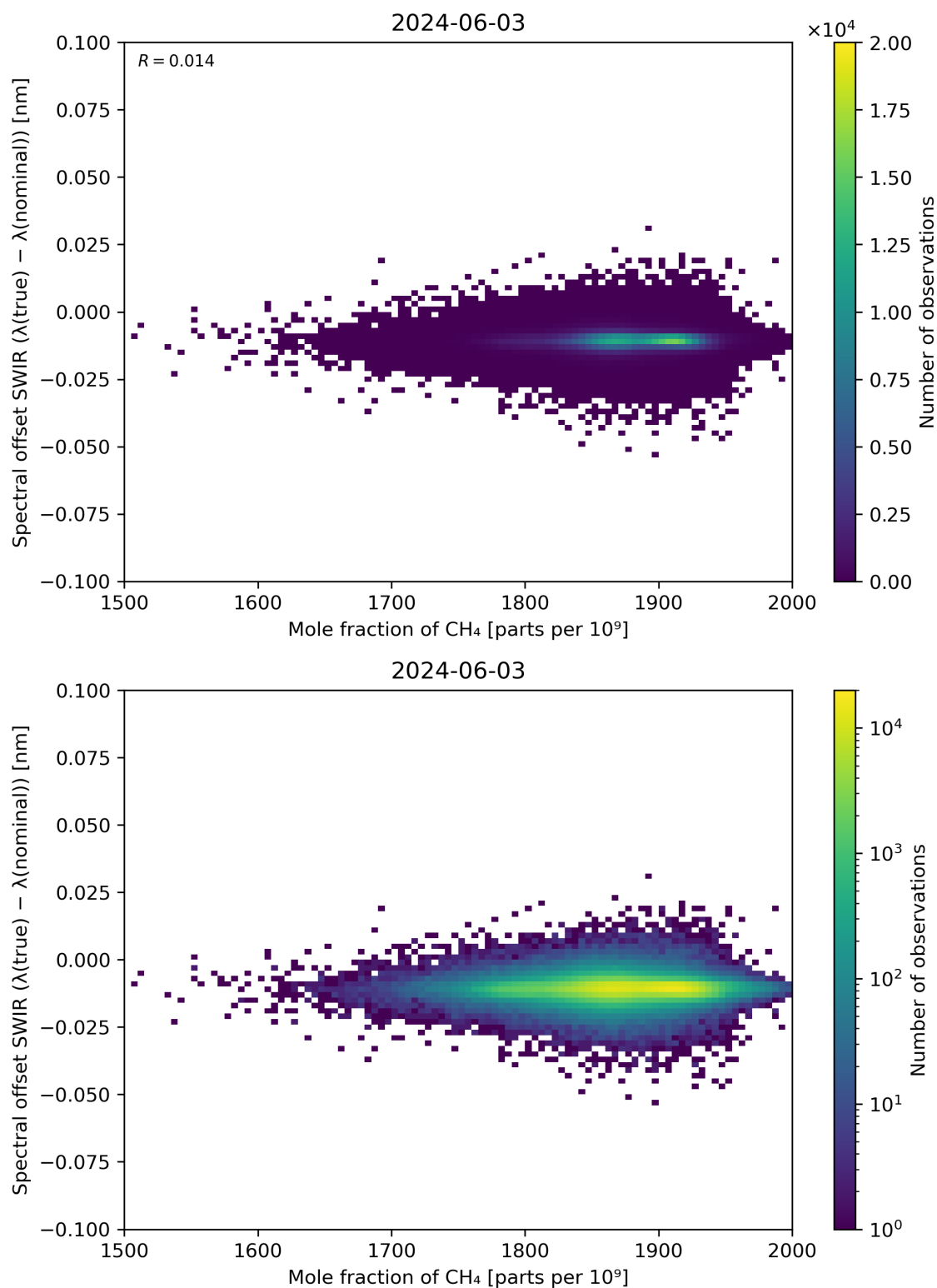
Figure 86: Scatter density plot of “Mole fraction of CH 4 ” against “Spectral offset SWIR ( \lambda(\text{true}) - \lambda(\text{nominal}) )” for 2024-06-03 to 2024-06-04.
