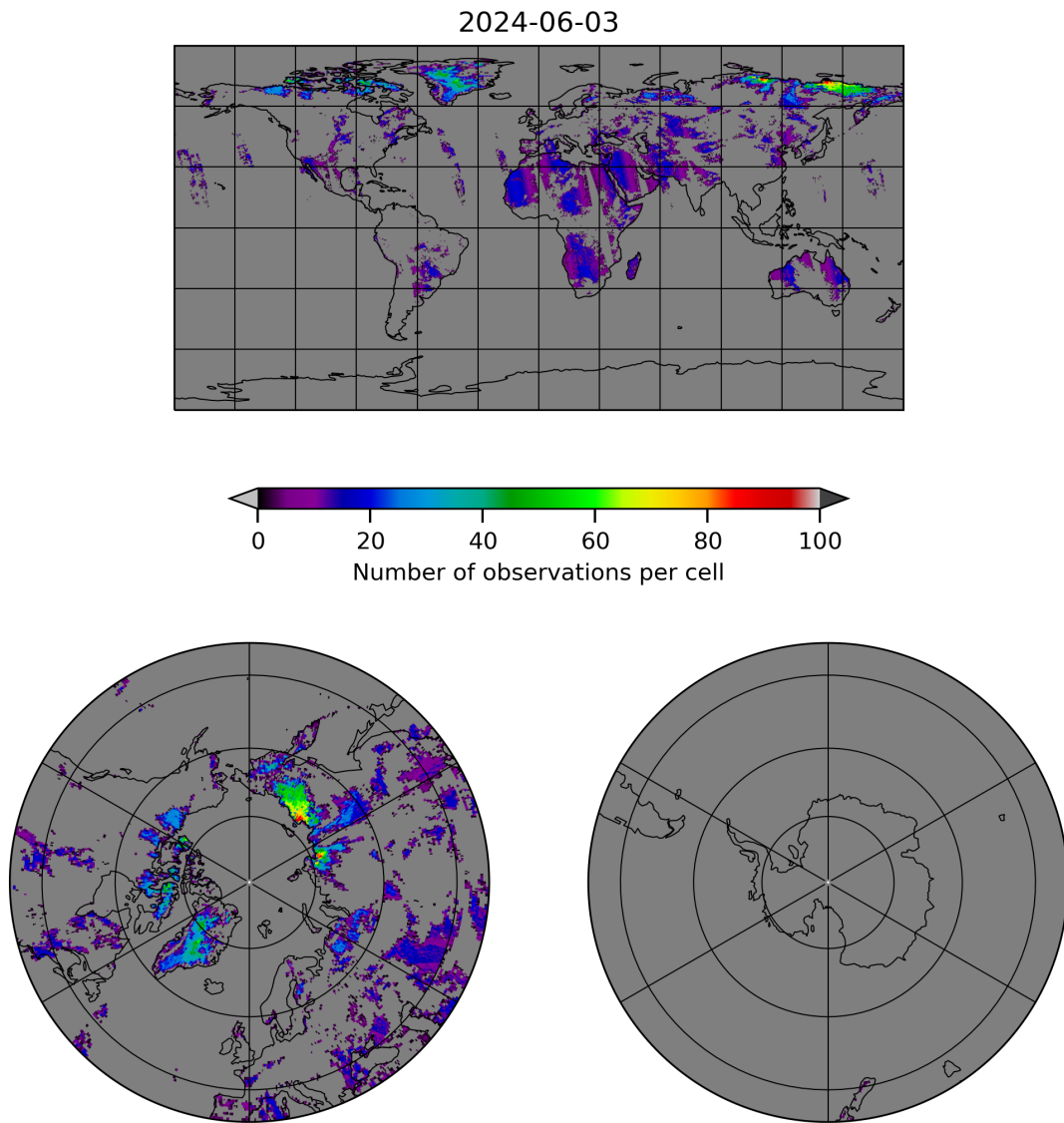
Figure 10: Map of the number of observations for 2024-06-03 to 2024-06-04
