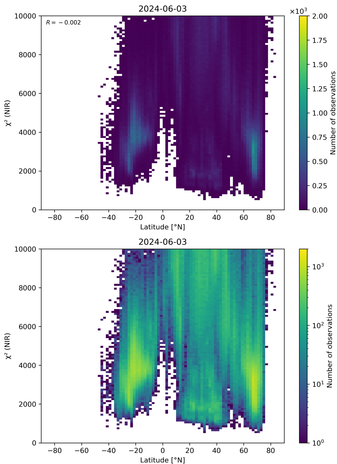
Figure 53: Scatter density plot of “Latitude” against “ \chi^2 (NIR)” for 2024-06-03 to 2024-06-04.
