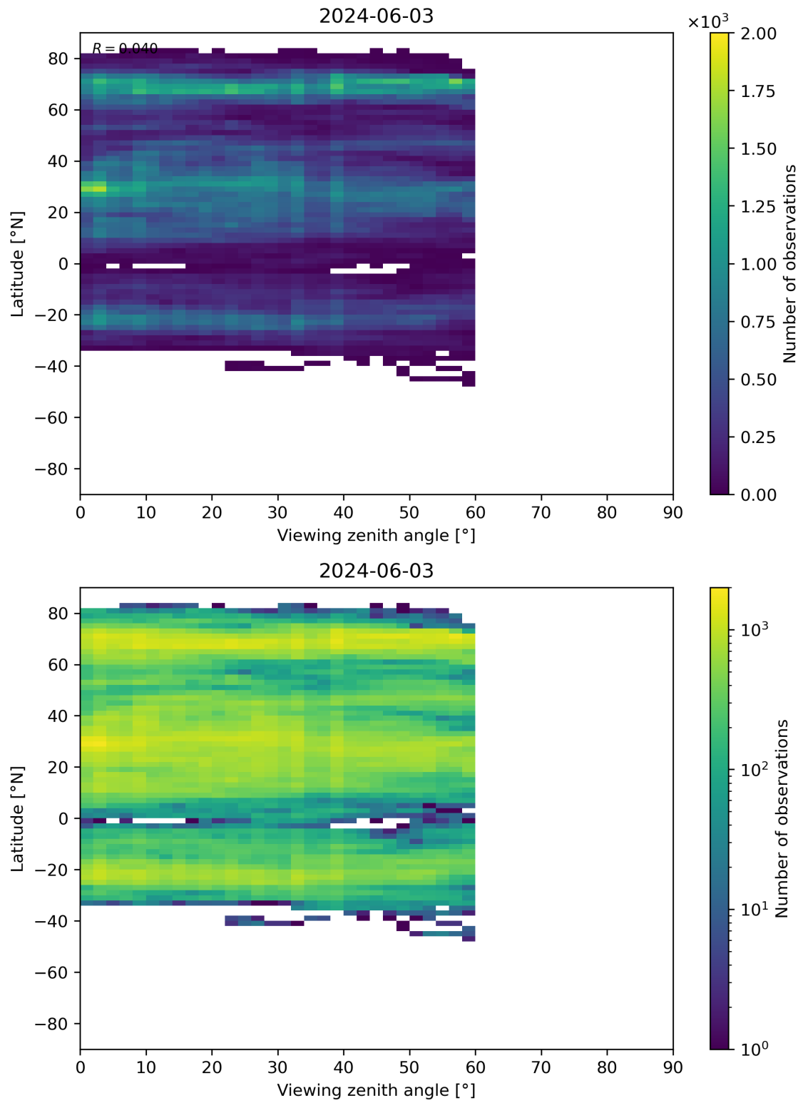
Figure 109: Scatter density plot of “Viewing zenith angle” against “Latitude” for 2024-06-03 to 2024-06-04.
