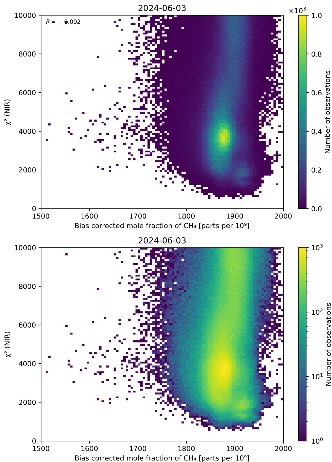
Figure 63: Scatter density plot of “Bias corrected mole fraction of CH 4 ” against “ \chi^2 (NIR)” for 2024-06-03 to 2024-06-04.
