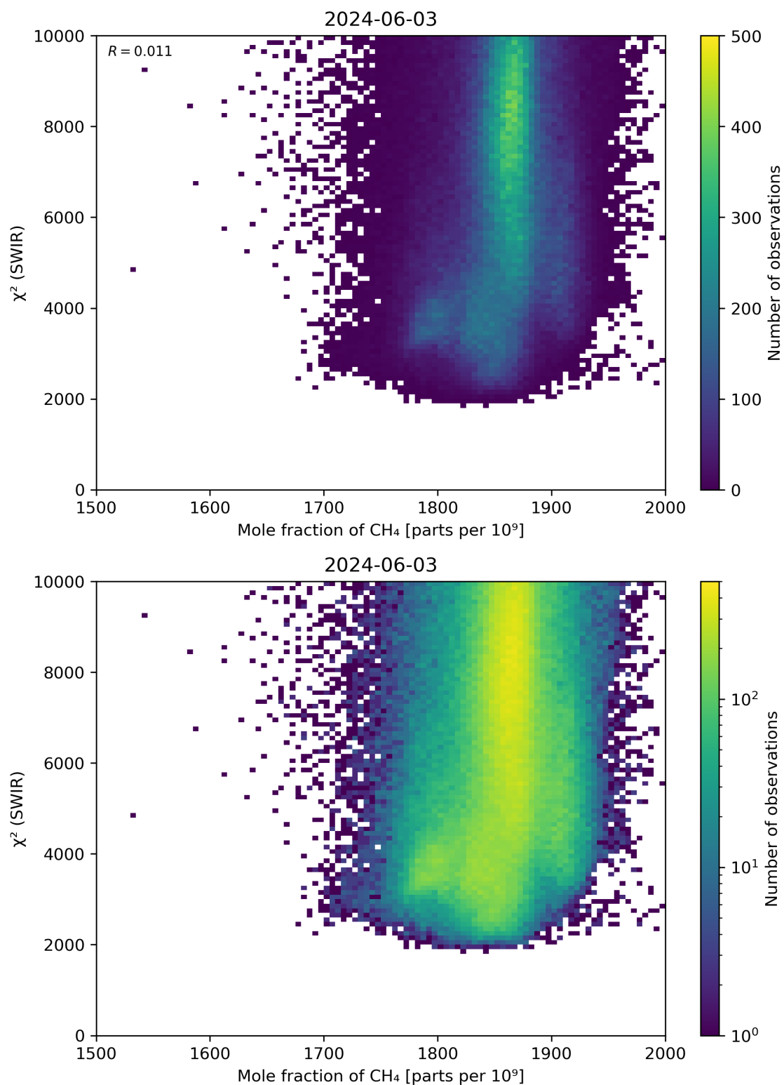
Figure 71: Scatter density plot of “Mole fraction of \text{CH}_4 ” against “ \chi^2 (SWIR)” for 2024-06-03 to 2024-06-04.
