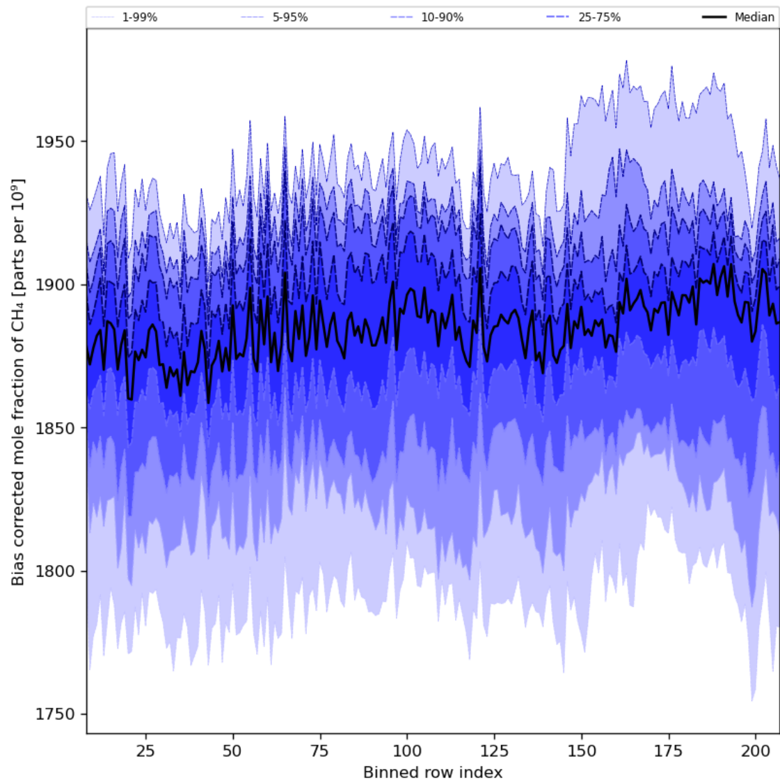
Figure 36: Along track statistics of “Bias corrected mole fraction of CH 4 ” for 2024-06-03 to 2024-06-04
