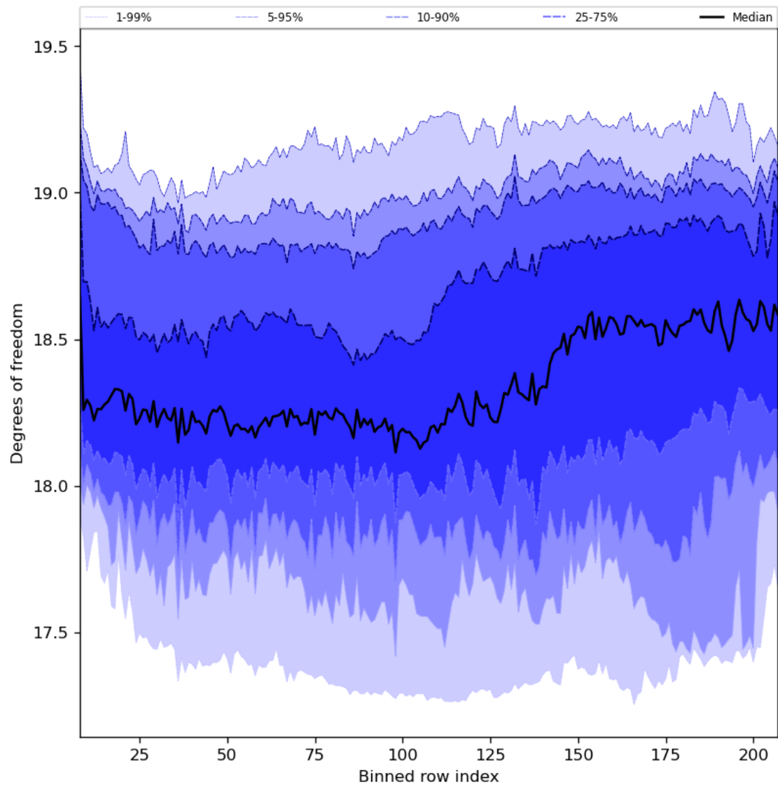
Figure 41: Along track statistics of “Degrees of freedom” for 2024-06-03 to 2024-06-04
