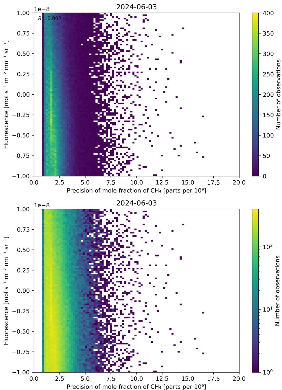
Figure 81: Scatter density plot of “Precision of mole fraction of \text{CH}_4 ” against “Fluorescence” for 2024-06-03 to 2024-06-04.
