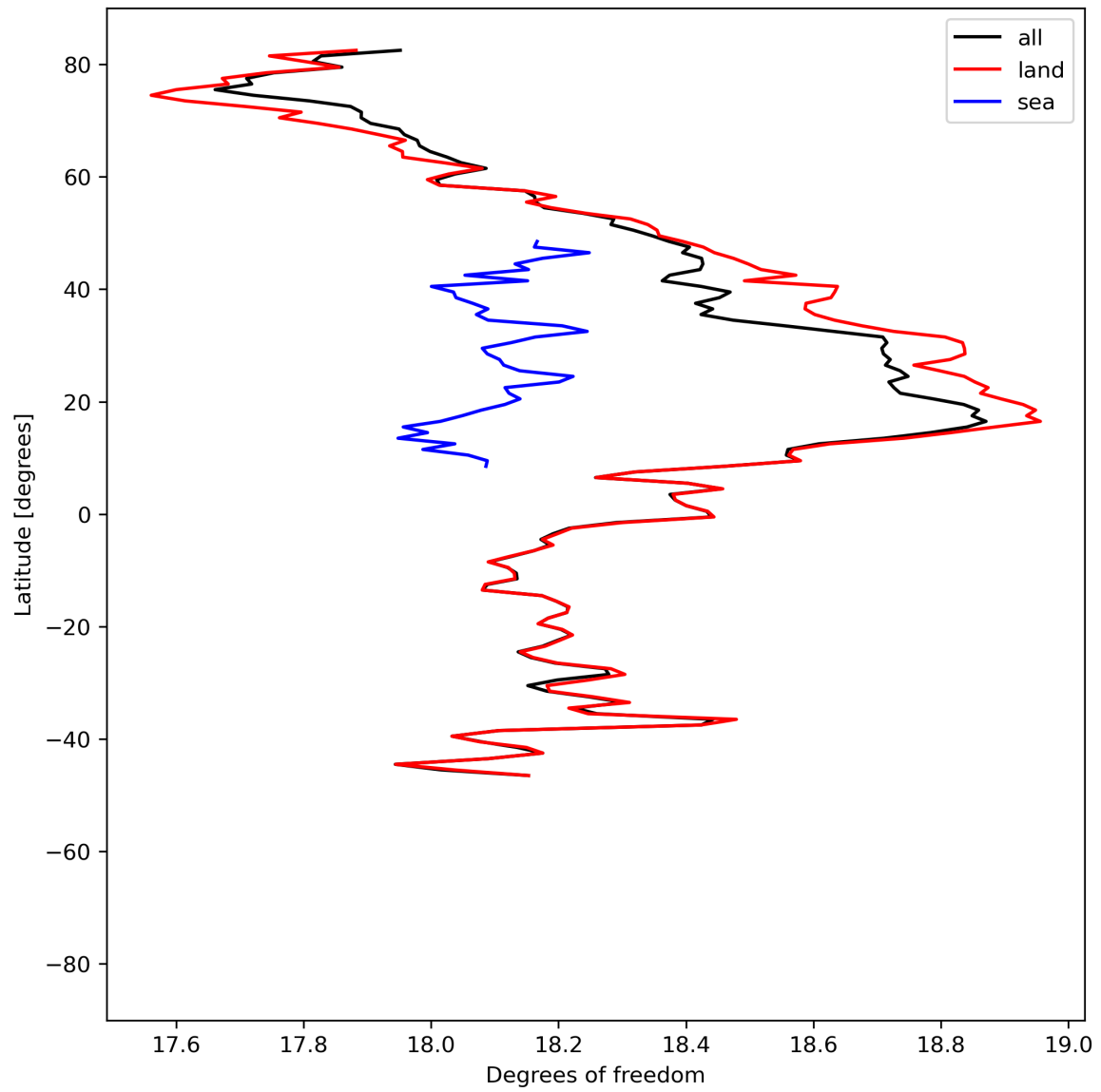
Figure 19: Zonal average of “Degrees of freedom” for 2024-06-03 to 2024-06-04.
