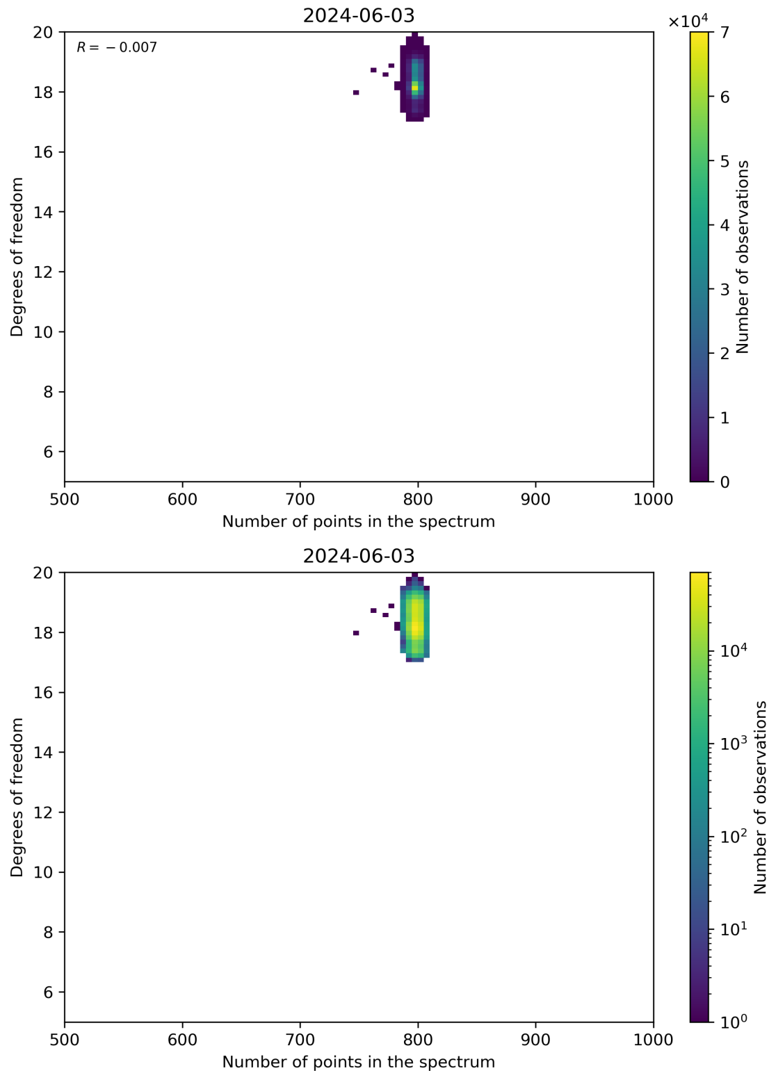
Figure 90: Scatter density plot of “Number of points in the spectrum” against “Degrees of freedom” for 2024-06-03 to 2024-06-04.
