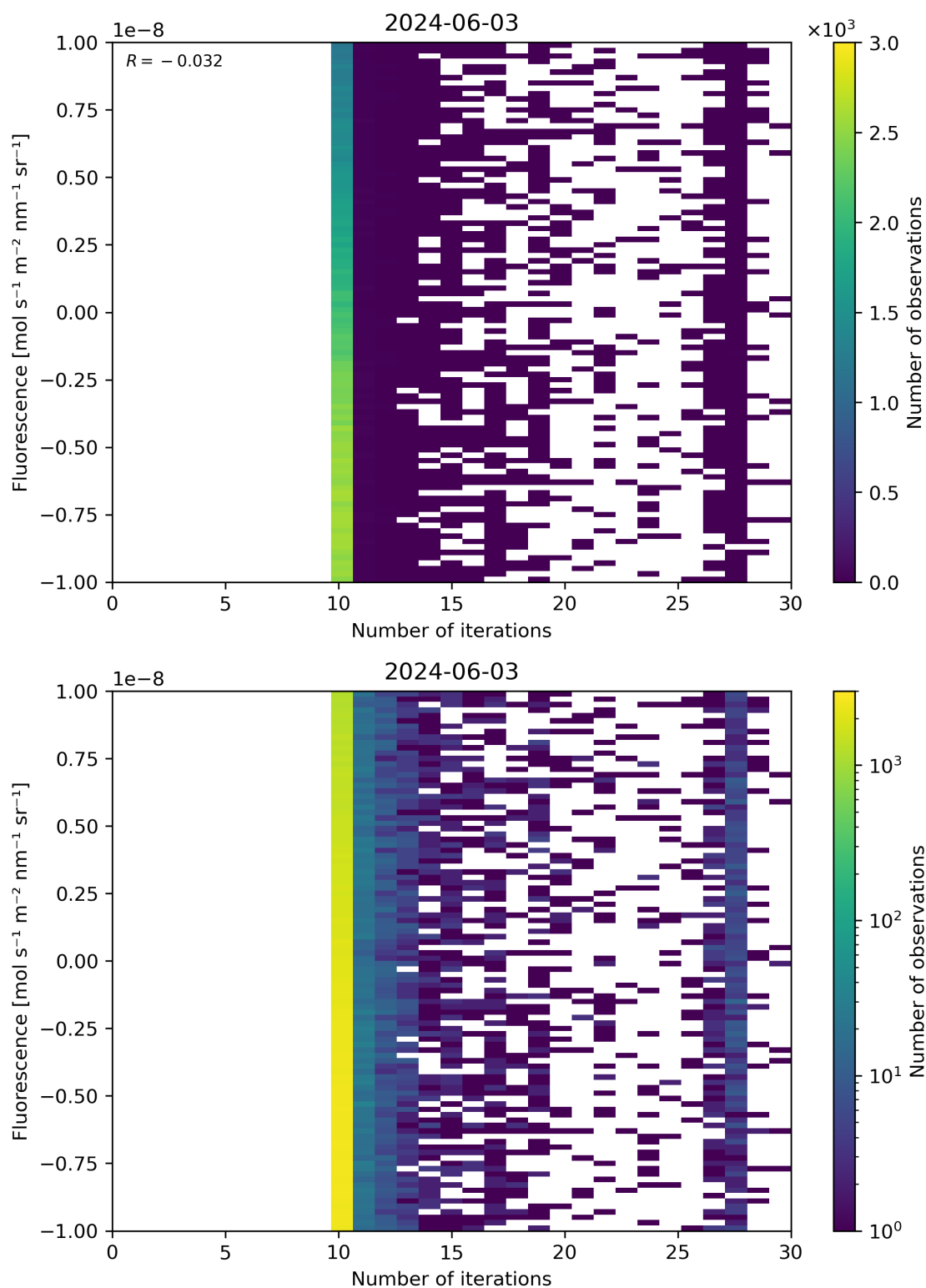
Figure 87: Scatter density plot of “Number of iterations” against “Fluorescence” for 2024-06-03 to 2024-06-04.
