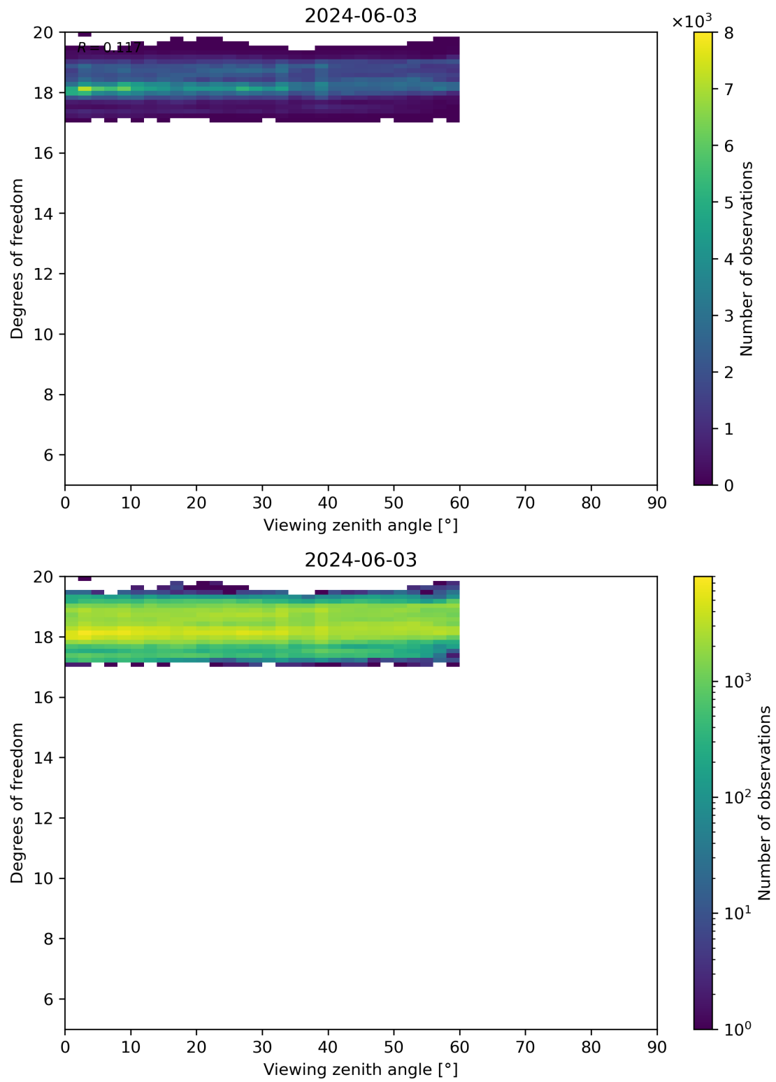
Figure 107: Scatter density plot of “Viewing zenith angle” against “Degrees of freedom” for 2024-06-03 to 2024-06-04.
