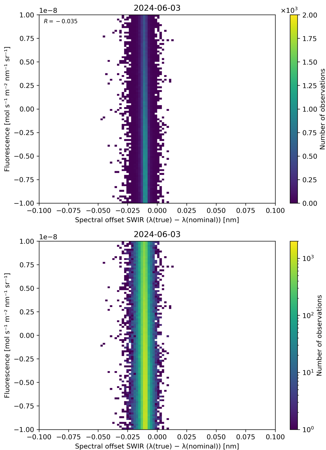
Figure 120: Scatter density plot of “Spectral offset SWIR ( \lambda(\text{true}) - \lambda(\text{nominal}) )” against “Fluorescence” for 2024-06-03 to 2024-06-04.
