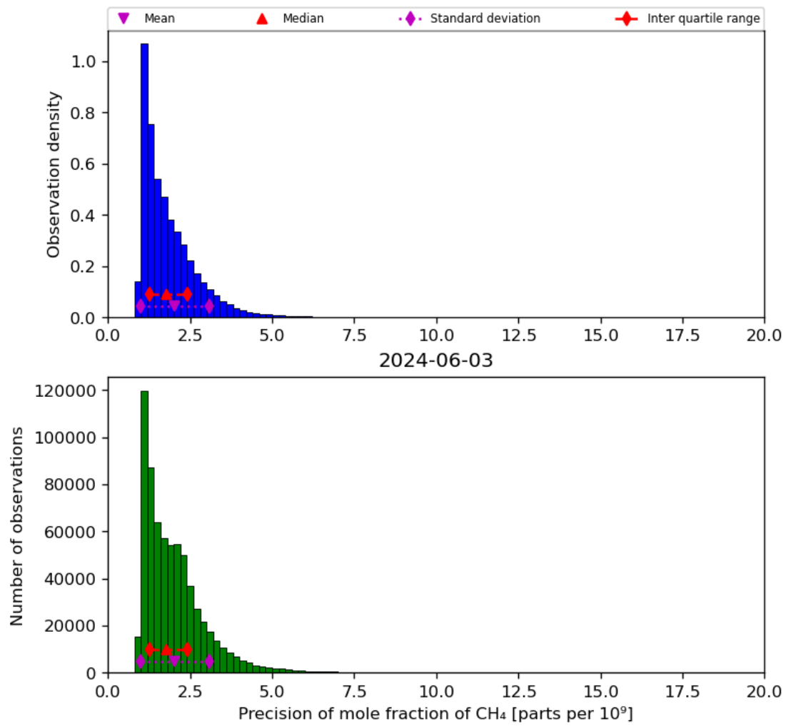
Figure 24: Histogram of “Precision of mole fraction of CH 4 ” for 2024-06-03 to 2024-06-04
