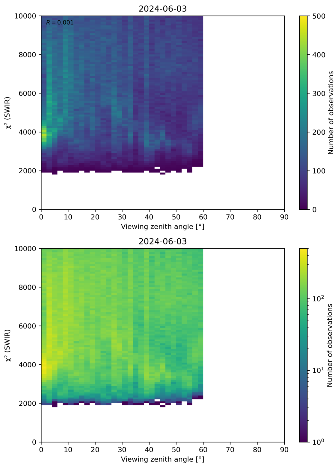
Figure 106: Scatter density plot of “Viewing zenith angle” against “ \chi^2 (SWIR)” for 2024-06-03 to 2024-06-04.
