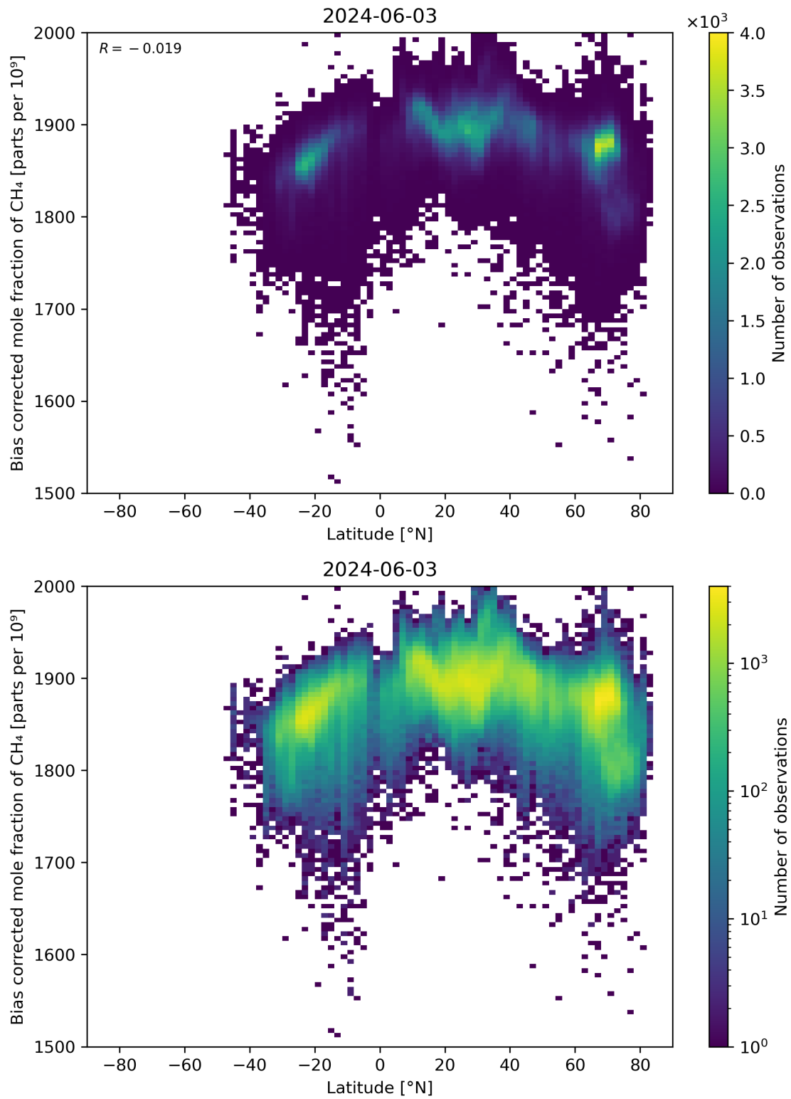
Figure 58: Scatter density plot of “Latitude” against “Bias corrected mole fraction of \text{CH}_4 ” for 2024-06-03 to 2024-06-04.
