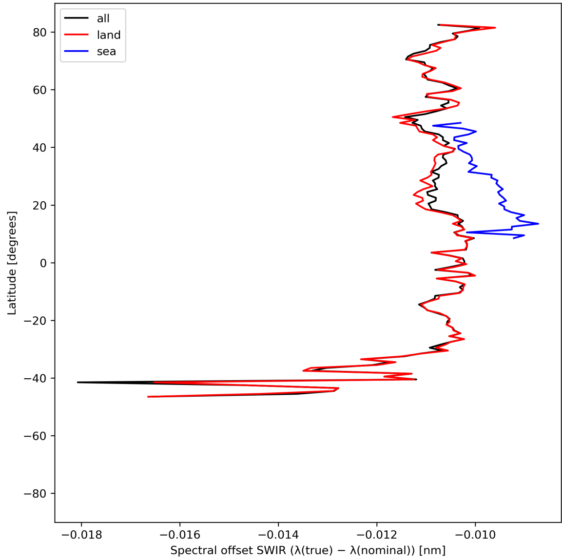
Figure 16: Zonal average of “Spectral offset SWIR ( \lambda(\text{true}) - \lambda(\text{nominal}) )” for 2024-06-03 to 2024-06-04.
