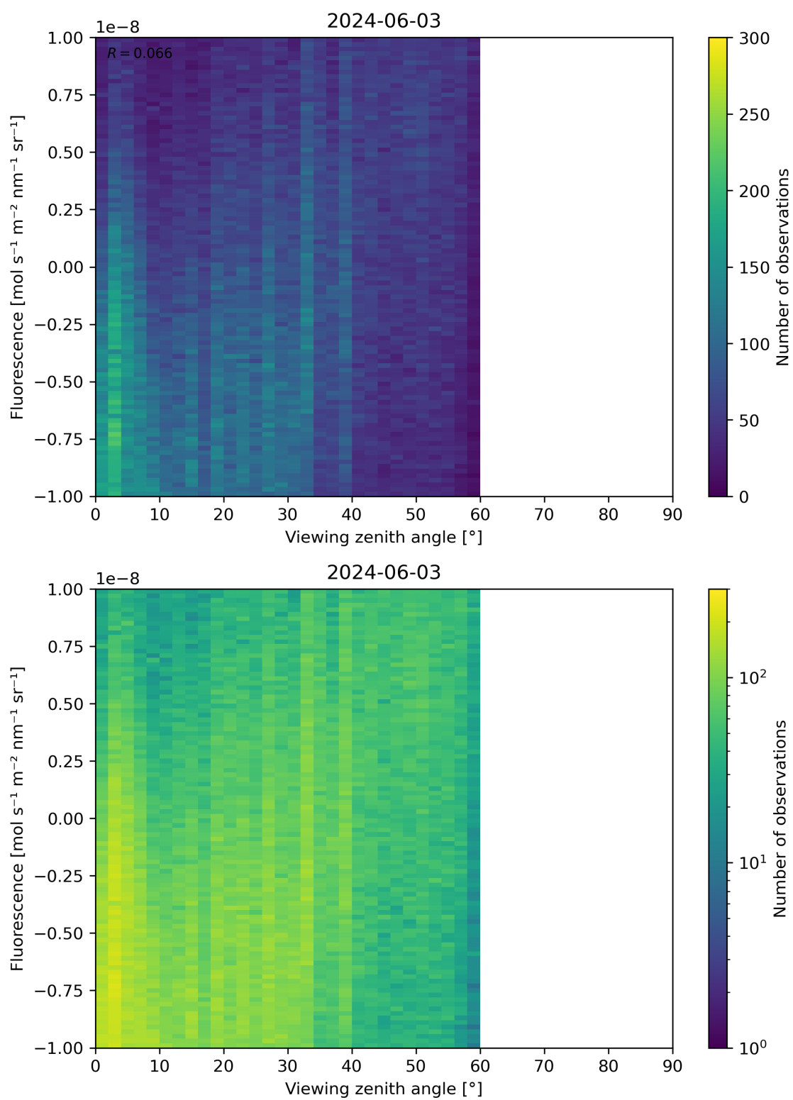
Figure 108: Scatter density plot of “Viewing zenith angle” against “Fluorescence” for 2024-06-03 to 2024-06-04.
