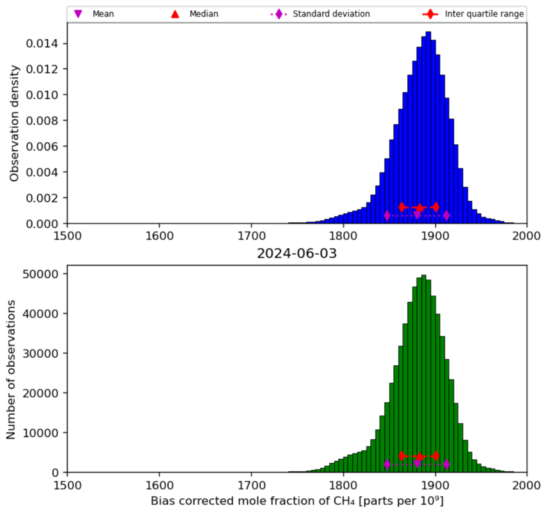
Figure 25: Histogram of “Bias corrected mole fraction of CH 4 ” for 2024-06-03 to 2024-06-04
