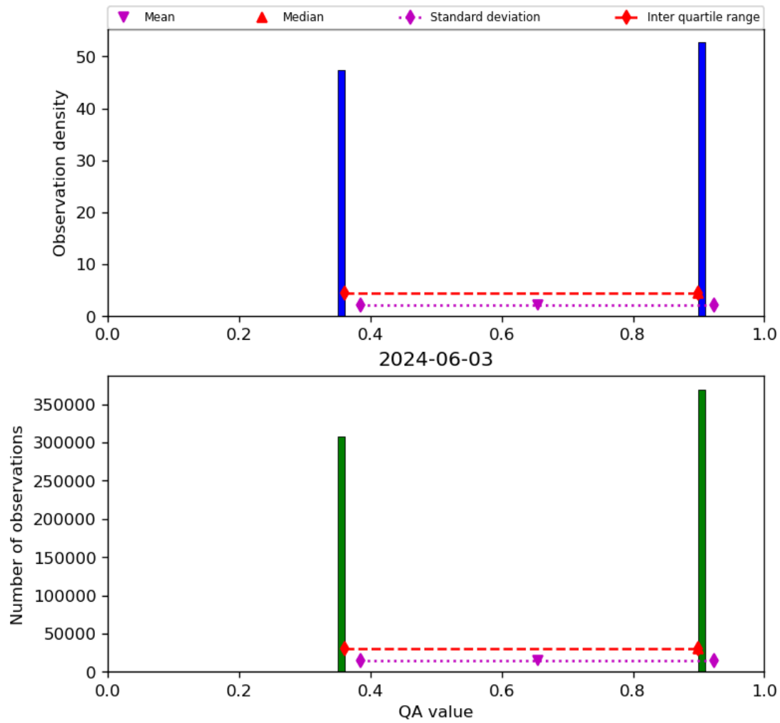
Figure 22: Histogram of “QA value” for 2024-06-03 to 2024-06-04
