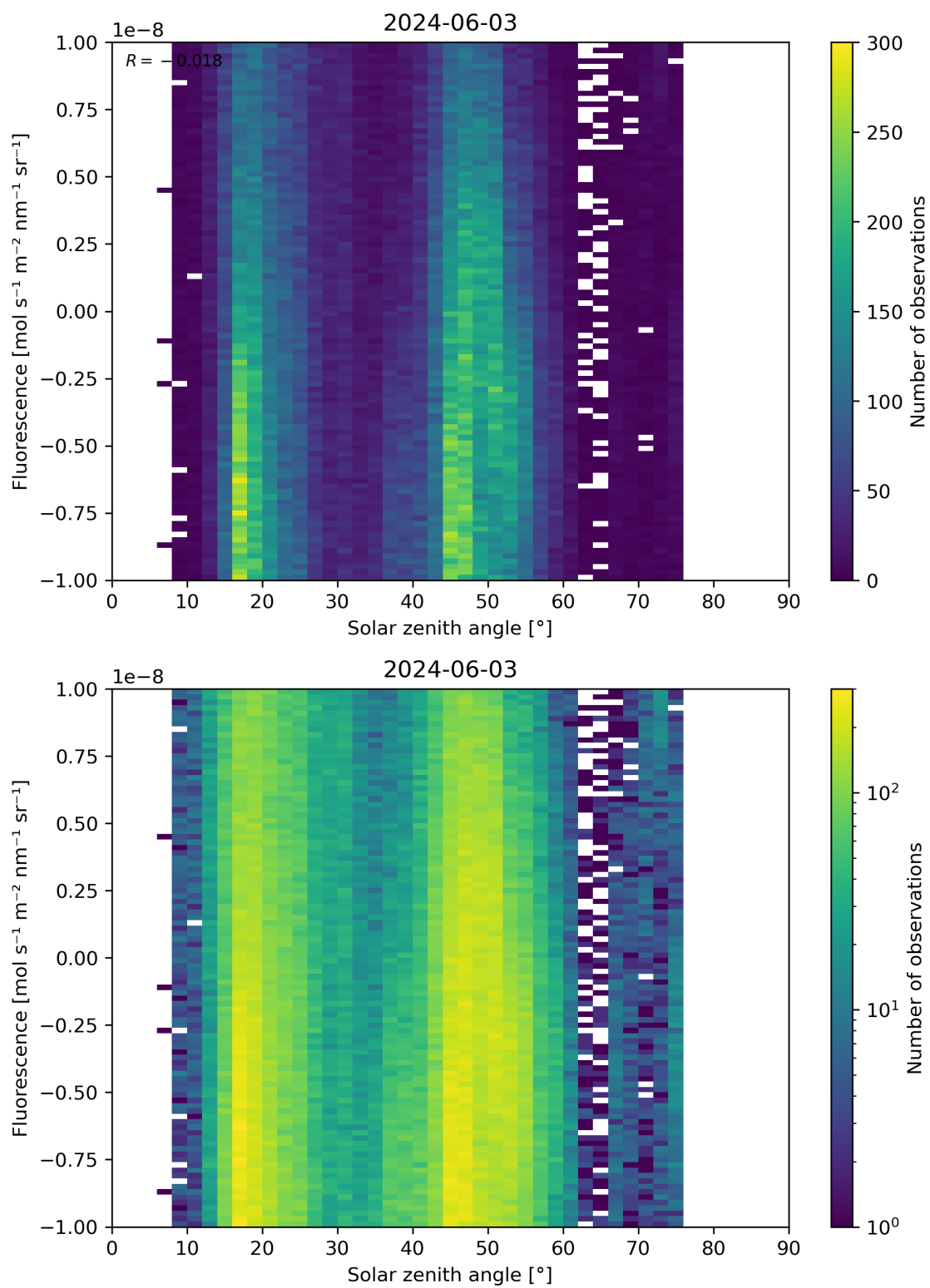
Figure 97: Scatter density plot of “Solar zenith angle” against “Fluorescence” for 2024-06-03 to 2024-06-04.
