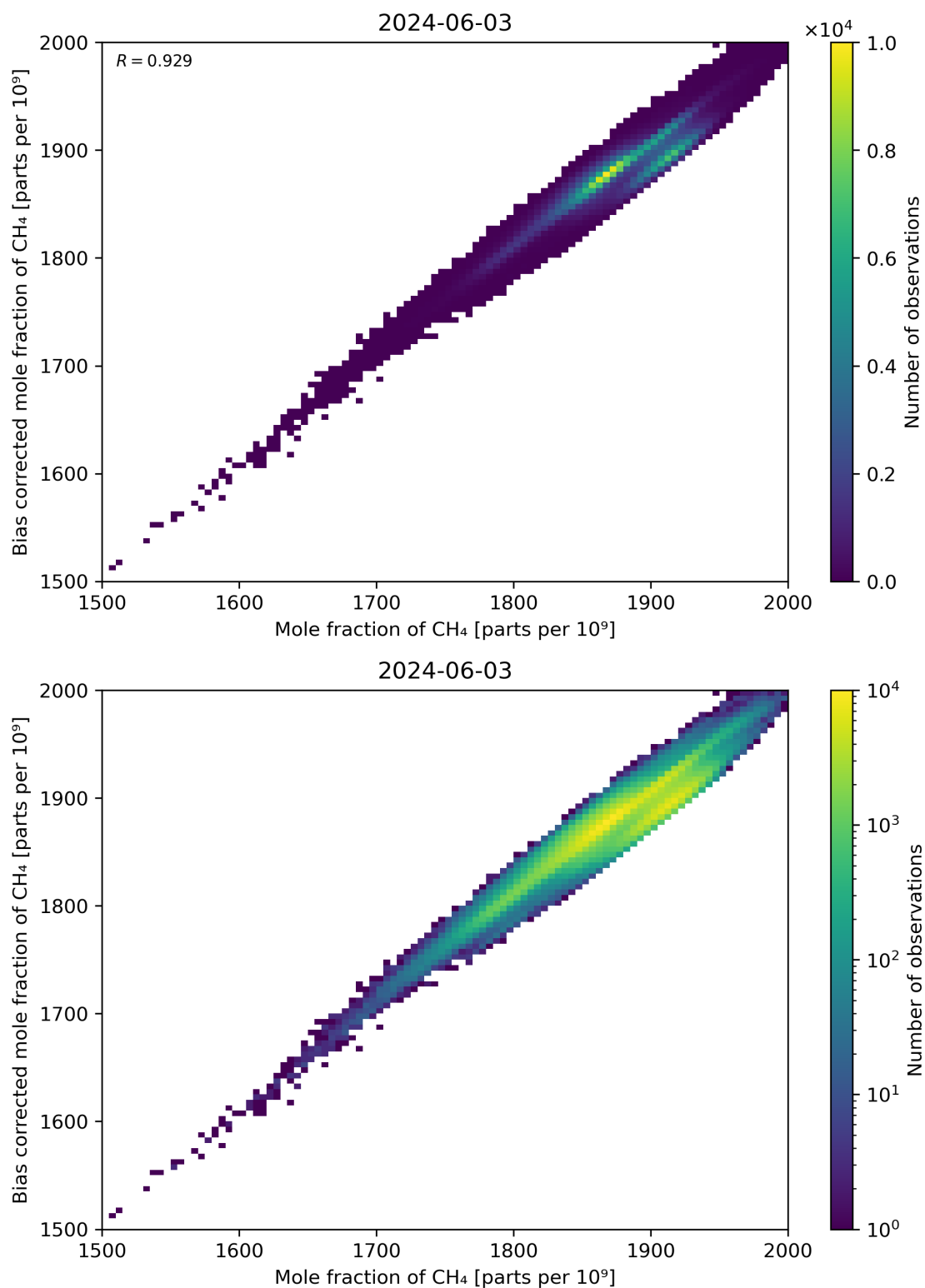
Figure 74: Scatter density plot of “Mole fraction of CH 4 ” against “Bias corrected mole fraction of CH 4 ” for 2024-06-03 to 2024-06-04.
