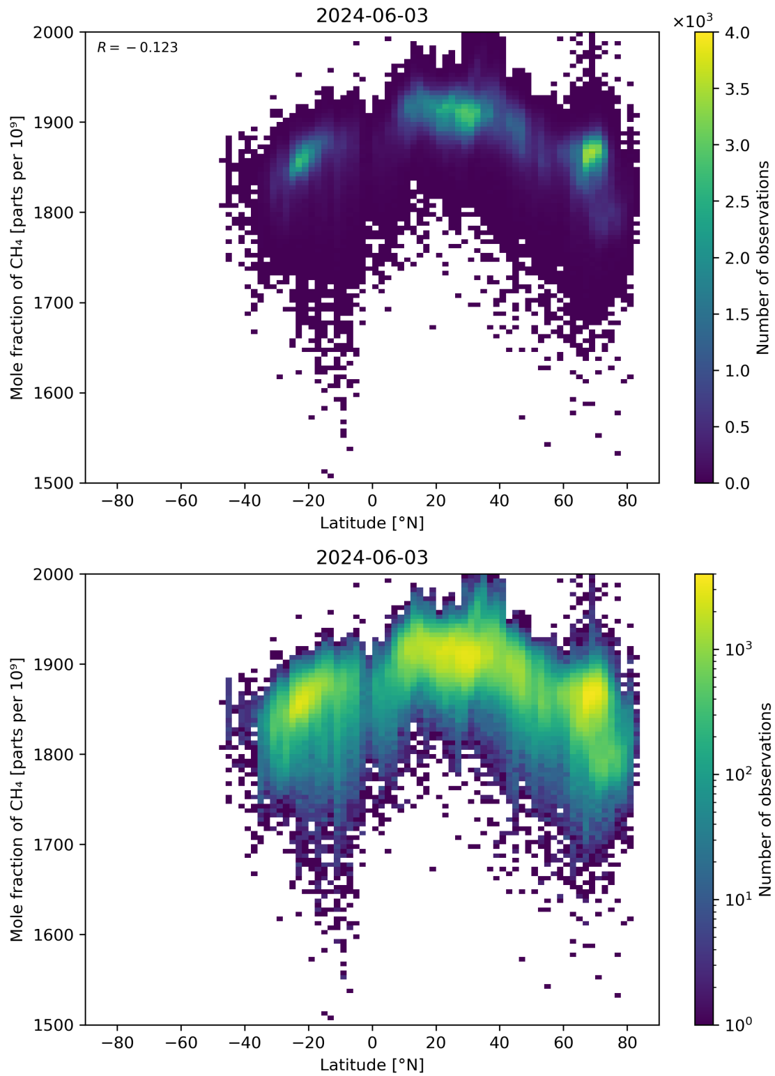
Figure 57: Scatter density plot of “Latitude” against “Mole fraction of \text{CH}_4 ” for 2024-06-03 to 2024-06-04.
