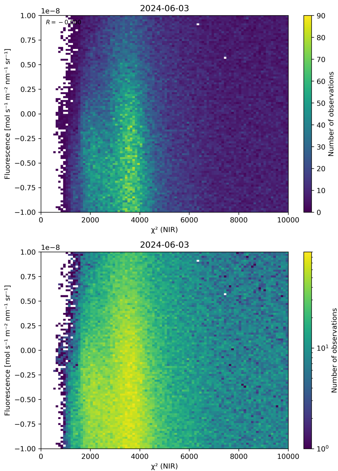
Figure 45: Scatter density plot of “ \chi^2 (NIR)” against “Fluorescence” for 2024-06-03 to 2024-06-04.
