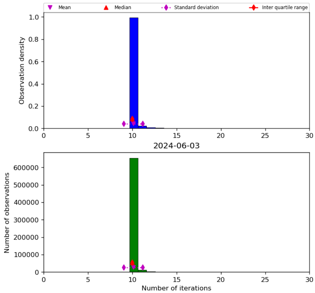
Figure 31: Histogram of “Number of iterations” for 2024-06-03 to 2024-06-04
