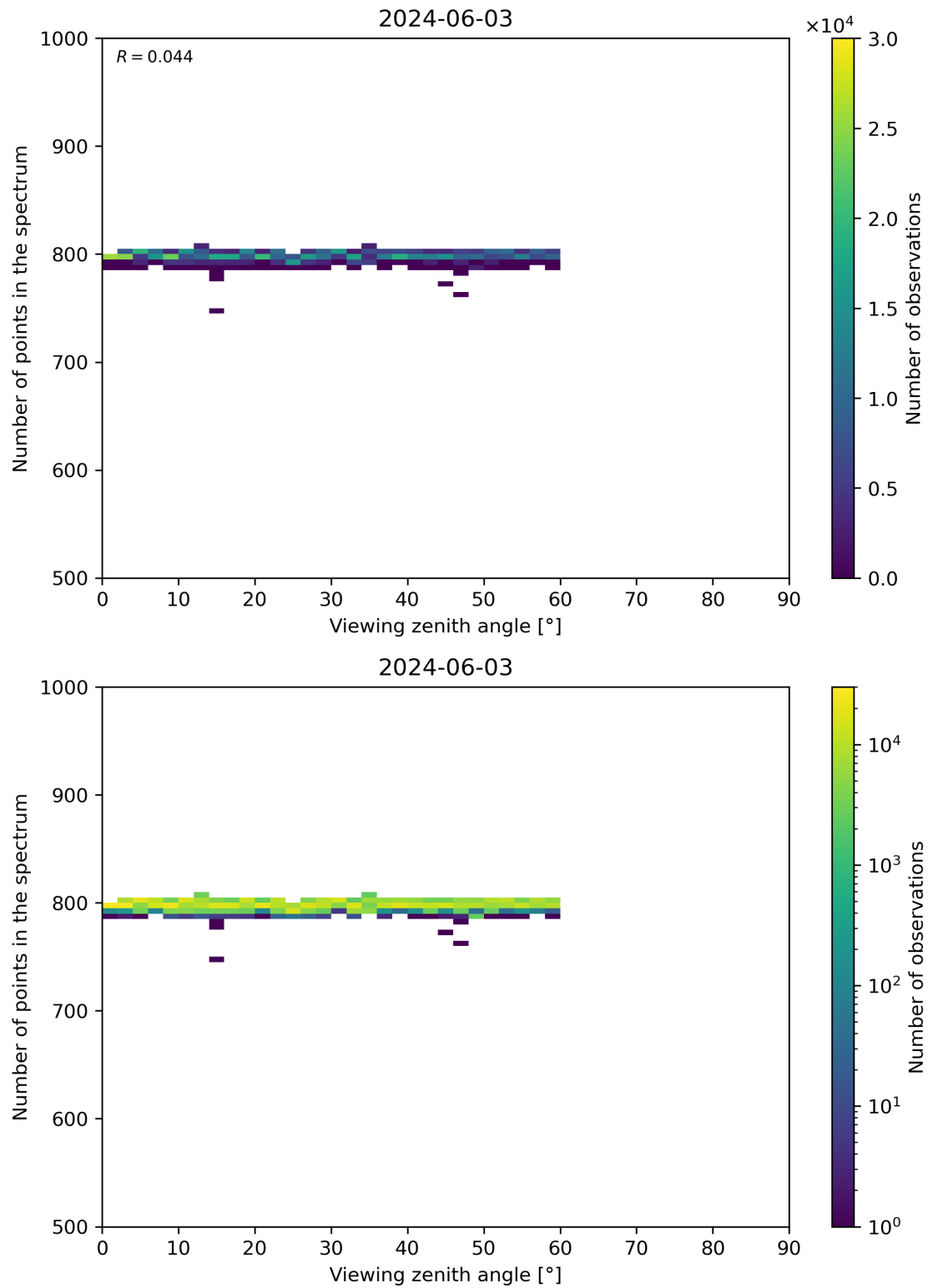
Figure 114: Scatter density plot of “Viewing zenith angle” against “Number of points in the spectrum” for 2024-06-03 to 2024-06-04.
