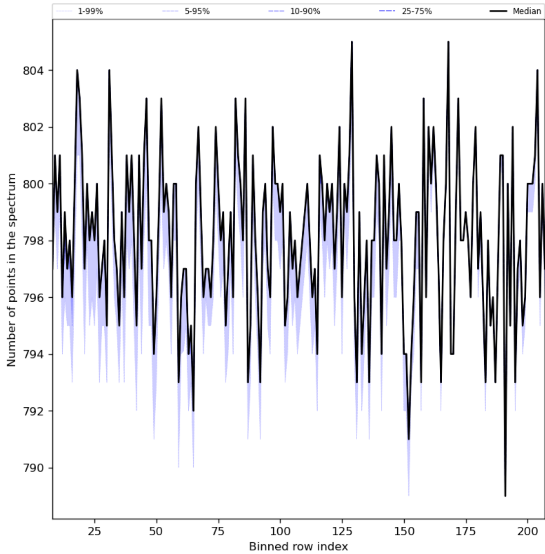
Figure 37: Along track statistics of “Number of points in the spectrum” for 2024-06-03 to 2024-06-04
