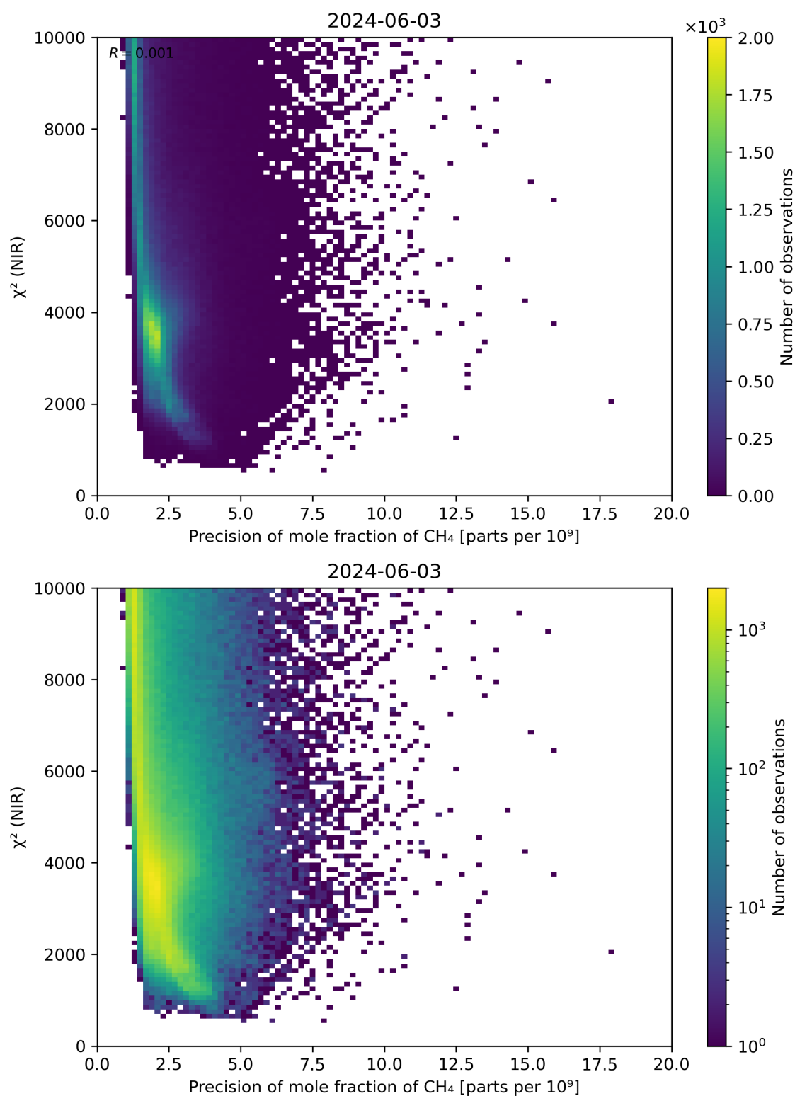
Figure 78: Scatter density plot of “Precision of mole fraction of \text{CH}_4 ” against “ \chi^2 (NIR)” for 2024-06-03 to 2024-06-04.
