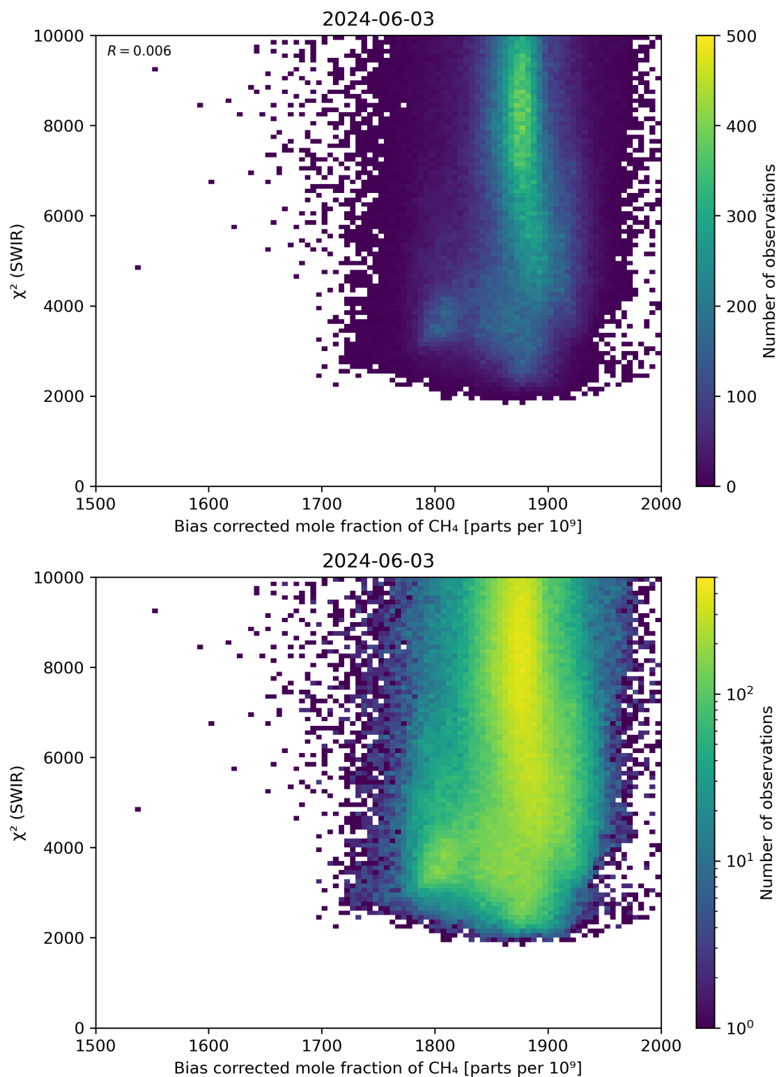
Figure 64: Scatter density plot of “Bias corrected mole fraction of CH 4 ” against “ \chi^2 (SWIR)” for 2024-06-03 to 2024-06-04.
