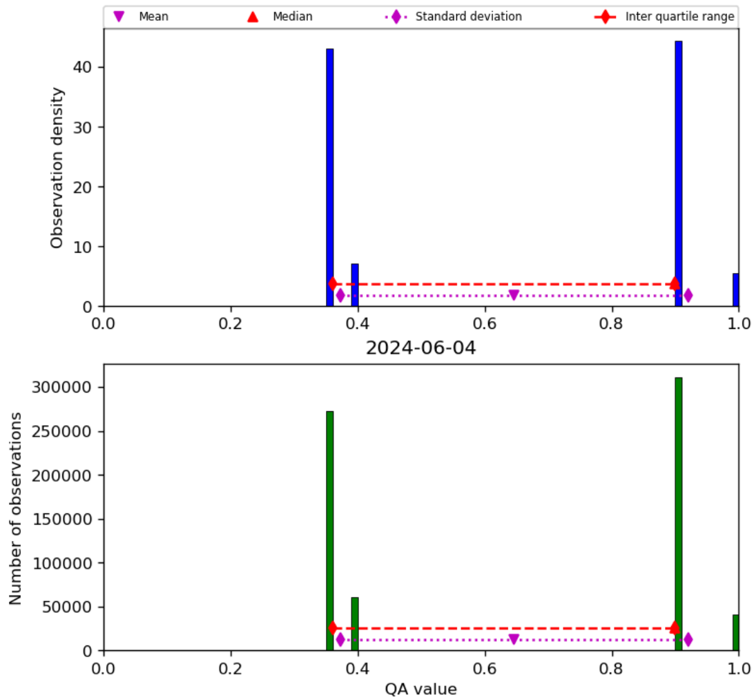
Figure 22: Histogram of “QA value” for 2024-06-03 to 2024-06-05
