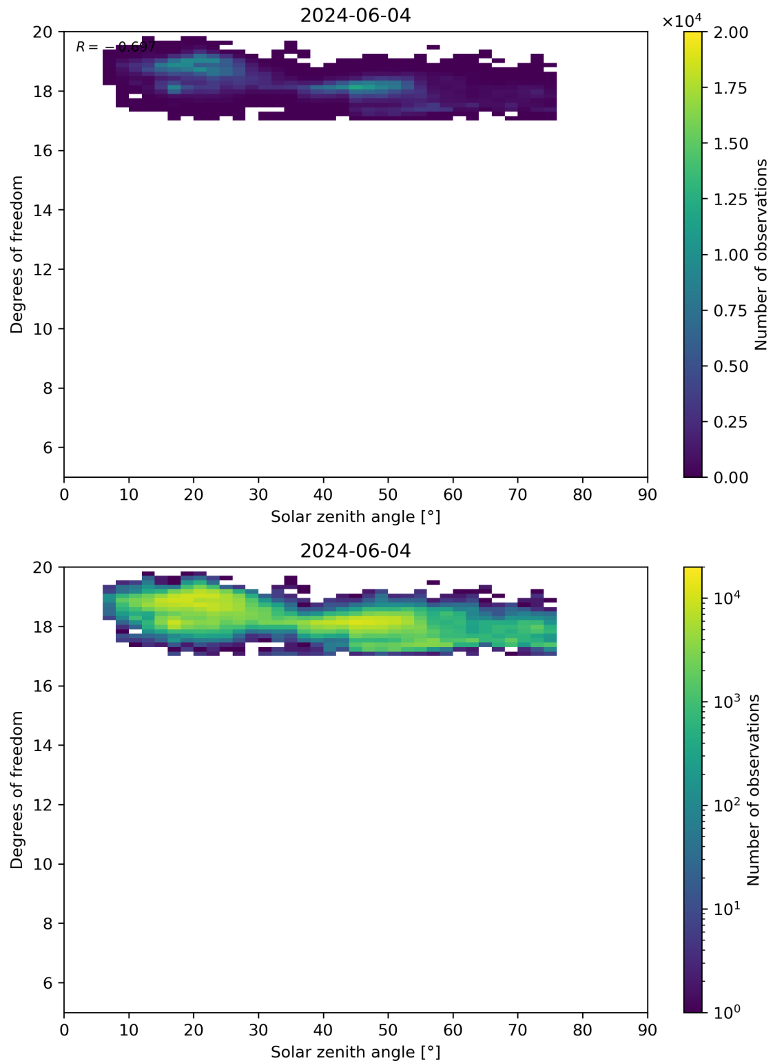
Figure 96: Scatter density plot of “Solar zenith angle” against “Degrees of freedom” for 2024-06-03 to 2024-06-05.
