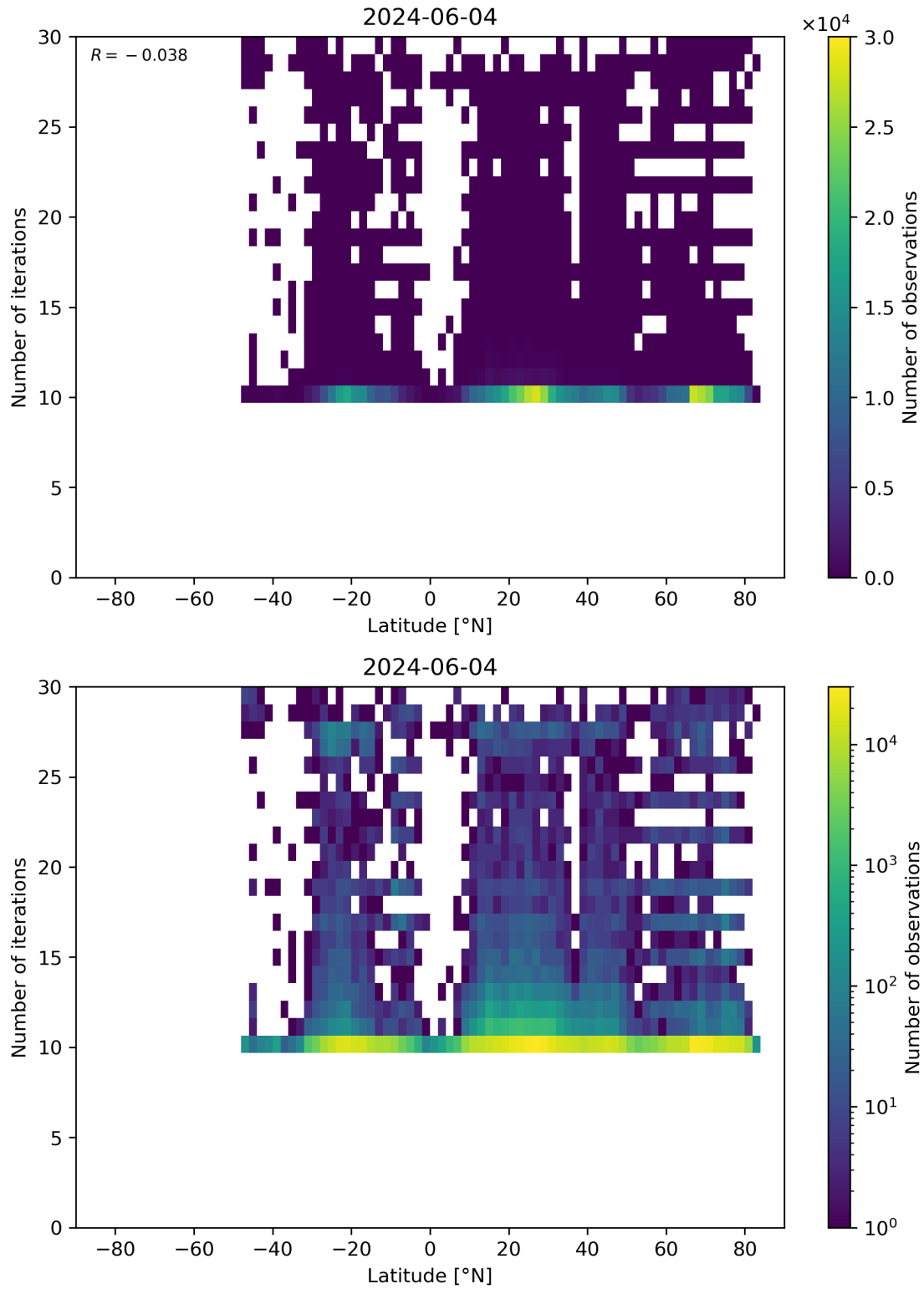
Figure 60: Scatter density plot of “Latitude” against “Number of iterations” for 2024-06-03 to 2024-06-05.
