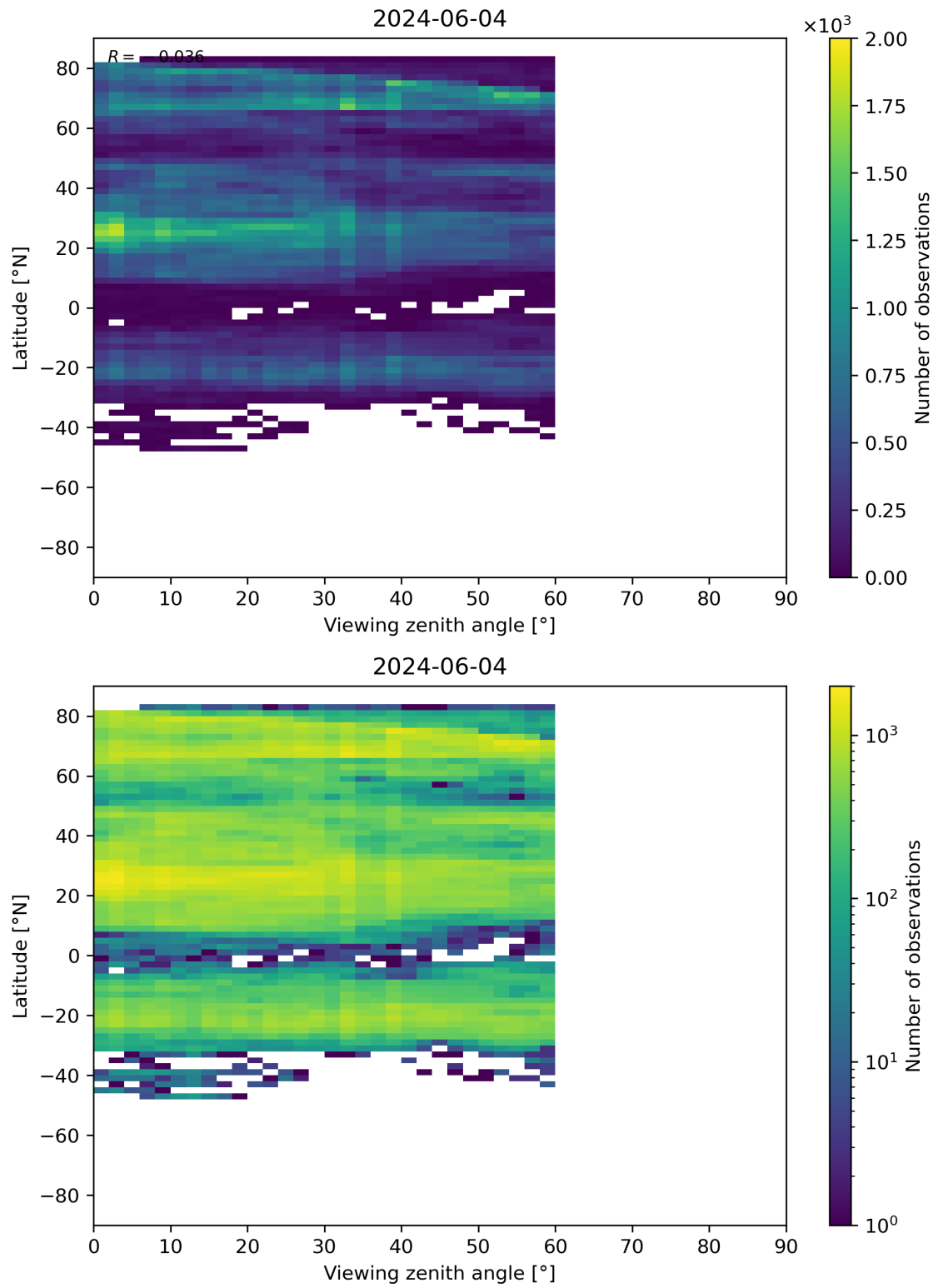
Figure 109: Scatter density plot of “Viewing zenith angle” against “Latitude” for 2024-06-03 to 2024-06-05.
