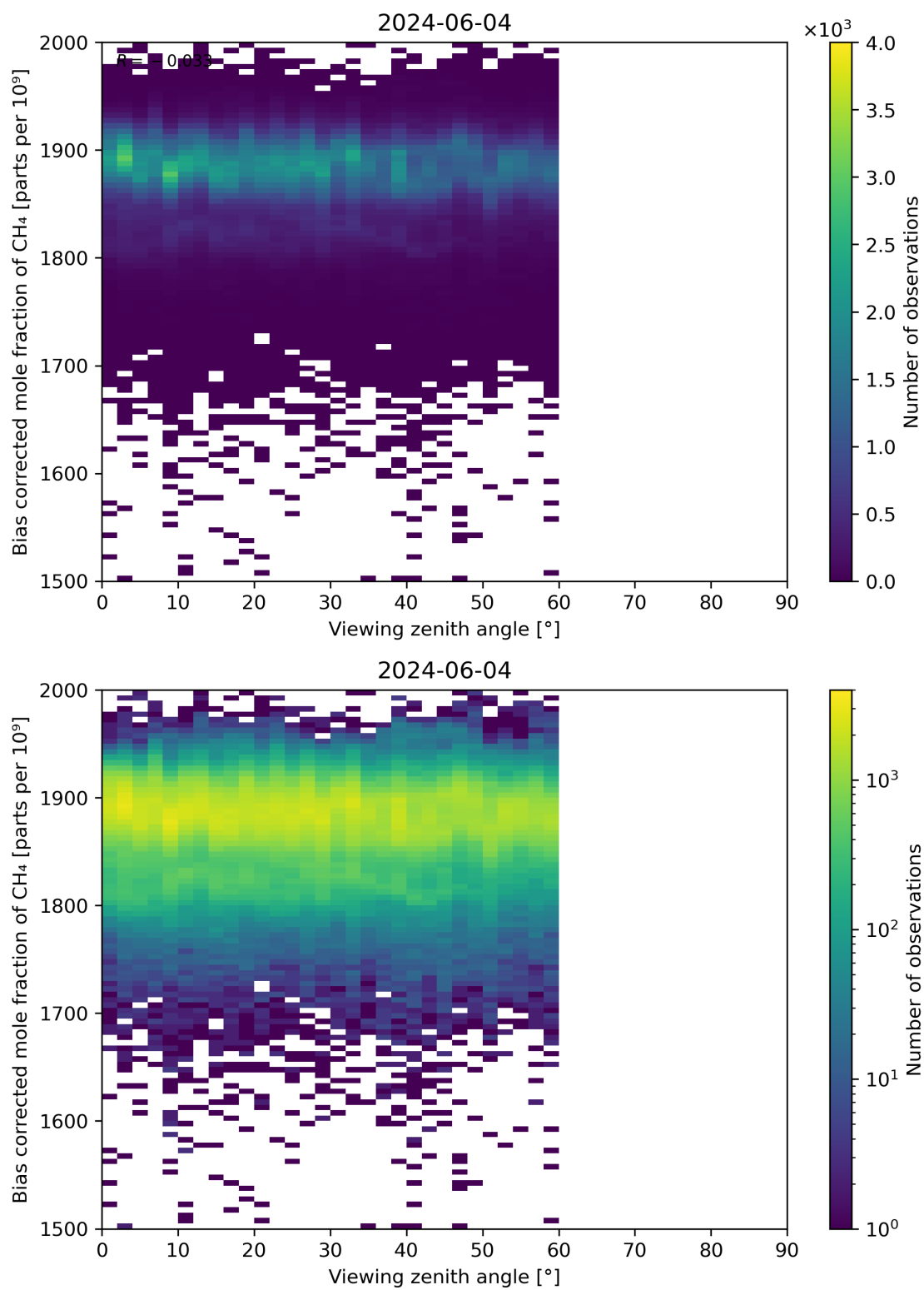
Figure 111: Scatter density plot of “Viewing zenith angle” against “Bias corrected mole fraction of CH 4 ” for 2024-06-03 to 2024-06-05.
