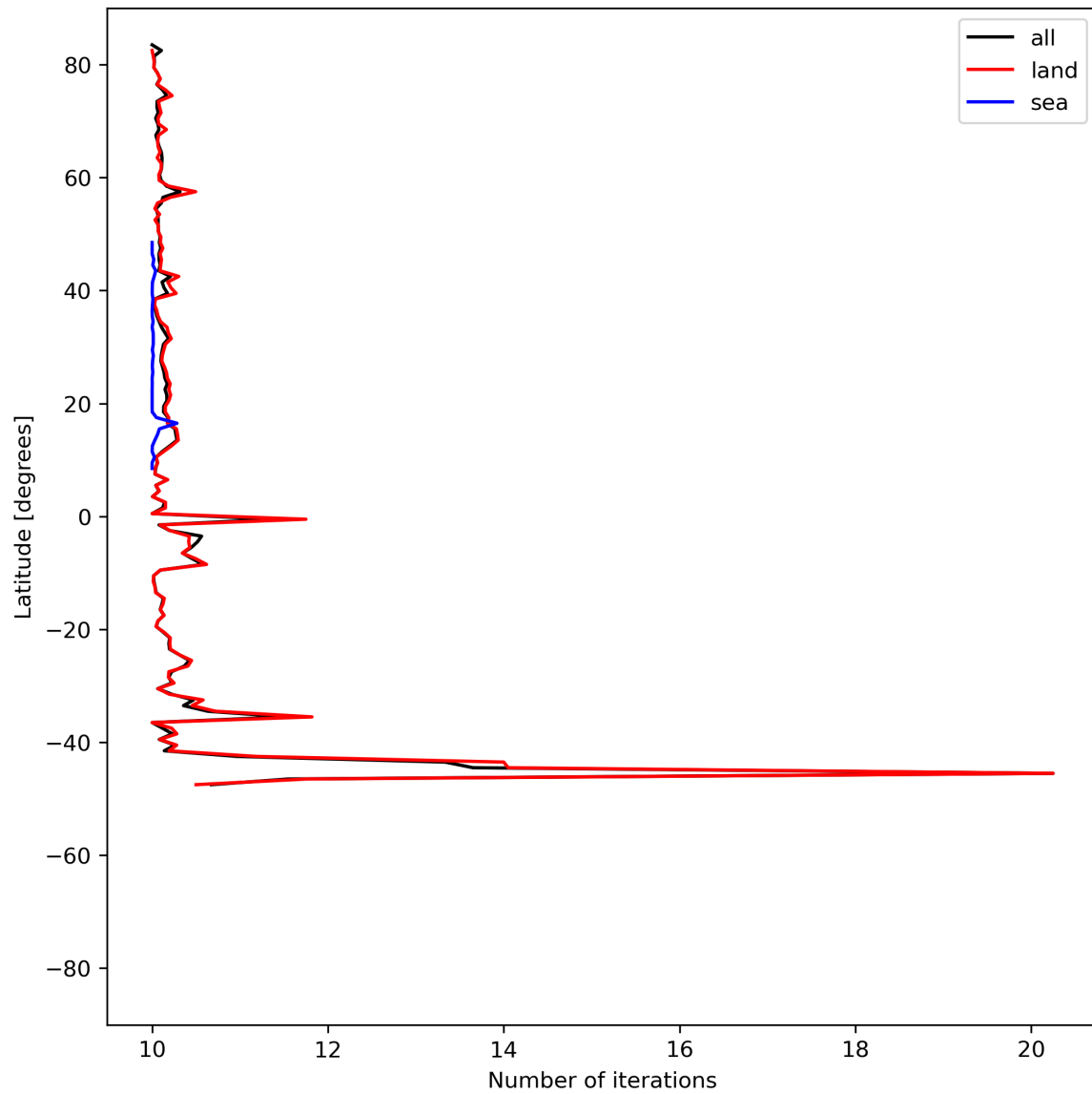
Figure 20: Zonal average of “Number of iterations” for 2024-06-03 to 2024-06-05.
