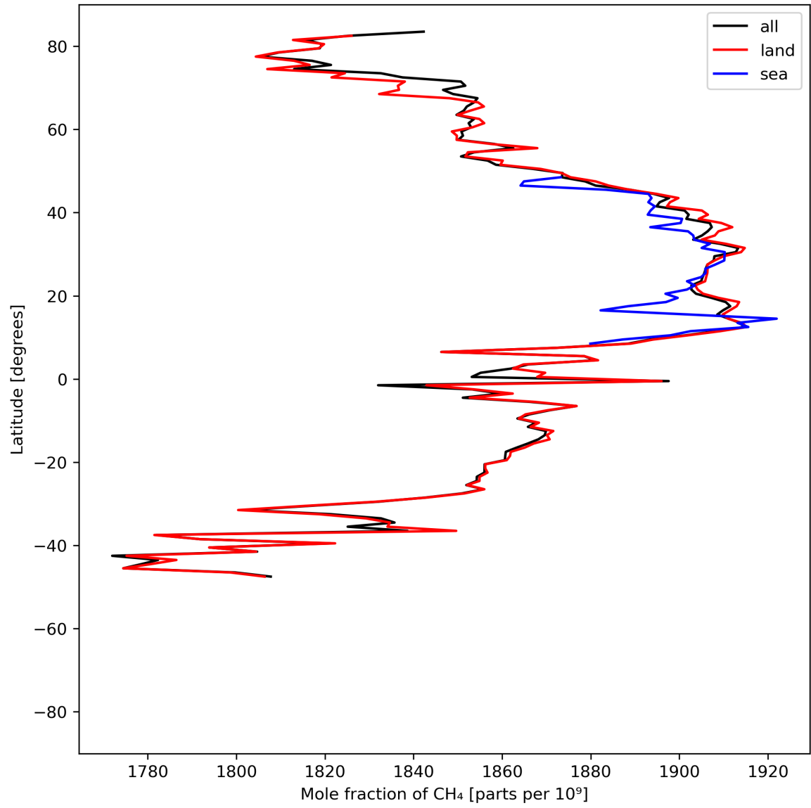
Figure 12: Zonal average of “Mole fraction of \text{CH}_4 ” for 2024-06-03 to 2024-06-05.
