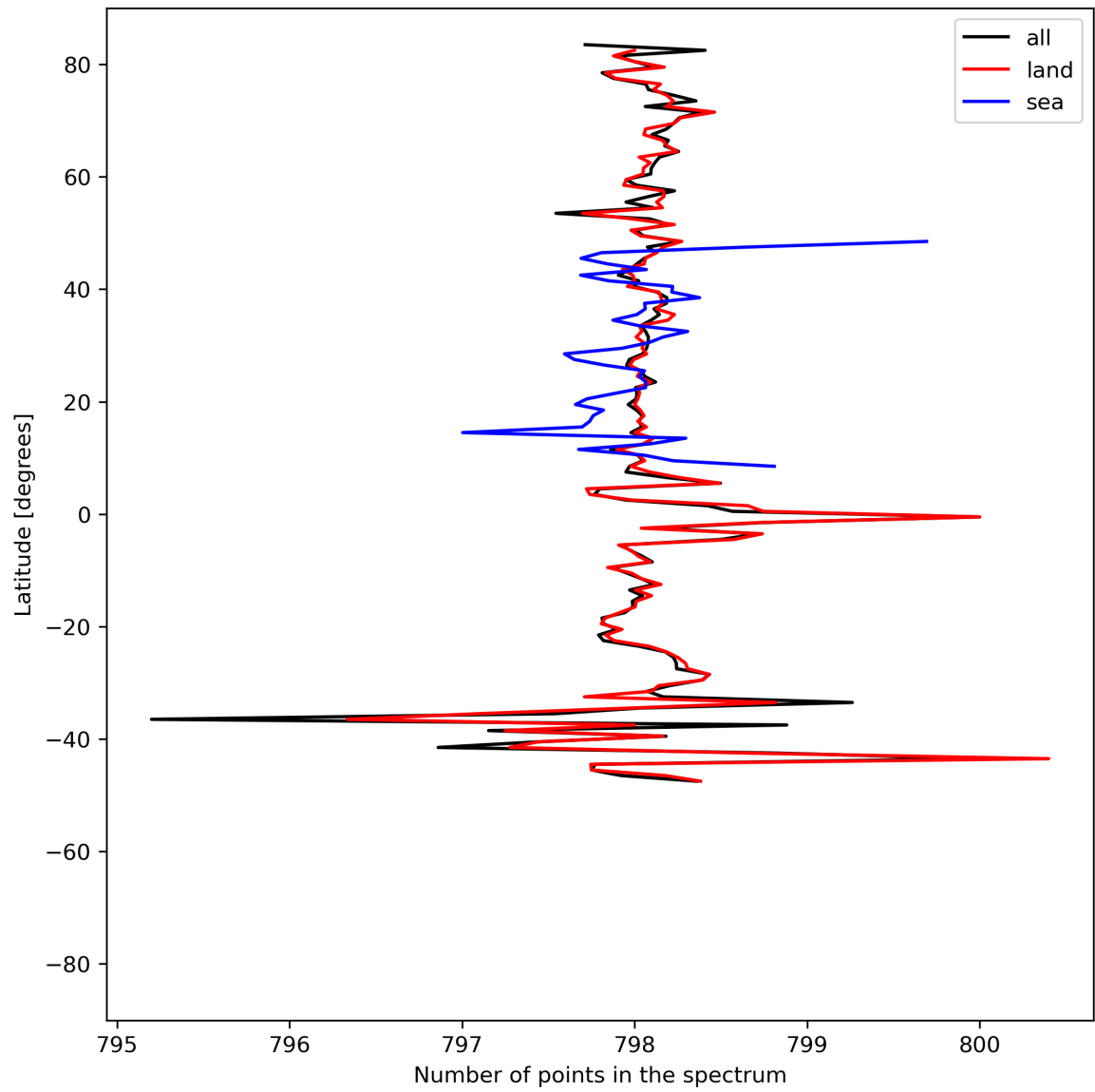
Figure 15: Zonal average of “Number of points in the spectrum” for 2024-06-03 to 2024-06-05.
