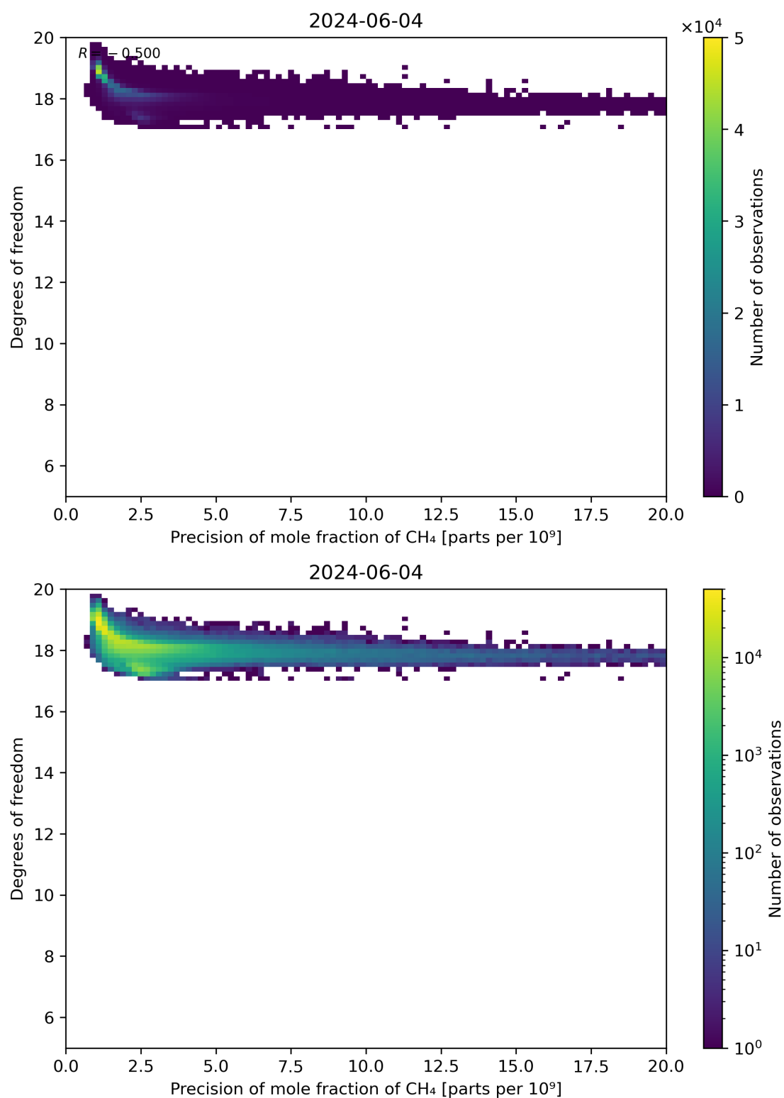
Figure 80: Scatter density plot of “Precision of mole fraction of CH 4 ” against “Degrees of freedom” for 2024-06-03 to 2024-06-05.
