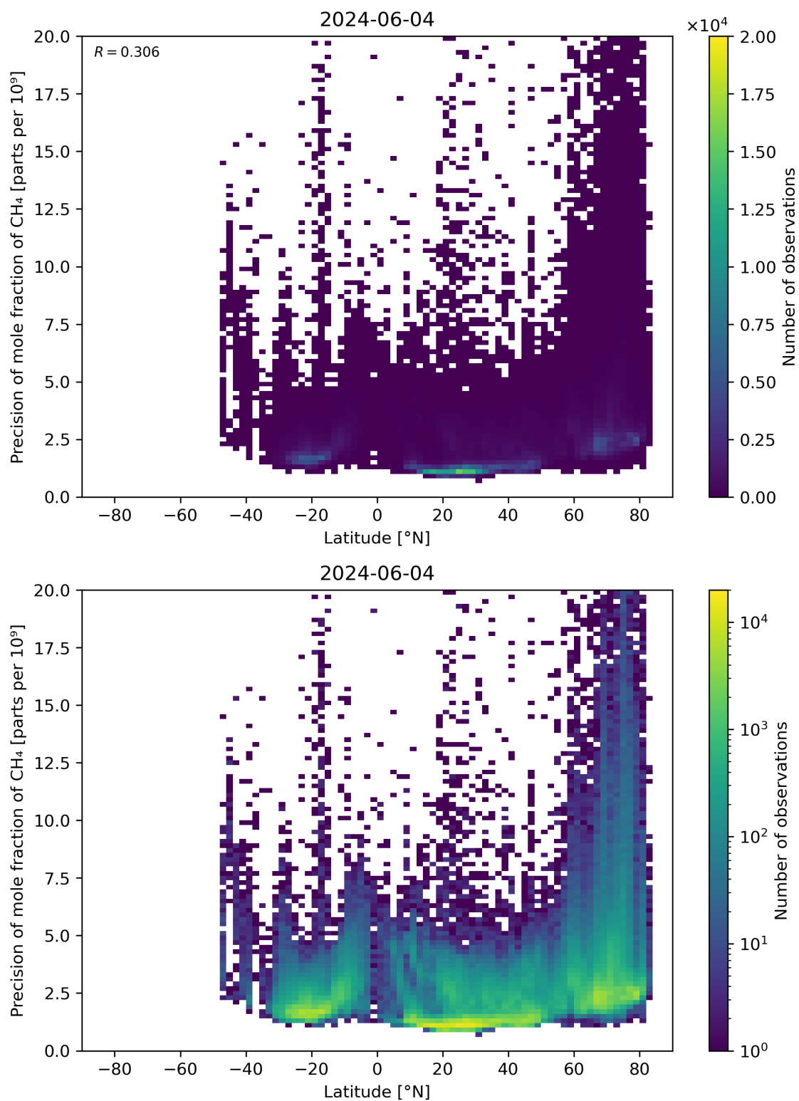
Figure 59: Scatter density plot of “Latitude” against “Precision of mole fraction of \text{CH}_4 ” for 2024-06-03 to 2024-06-05.
