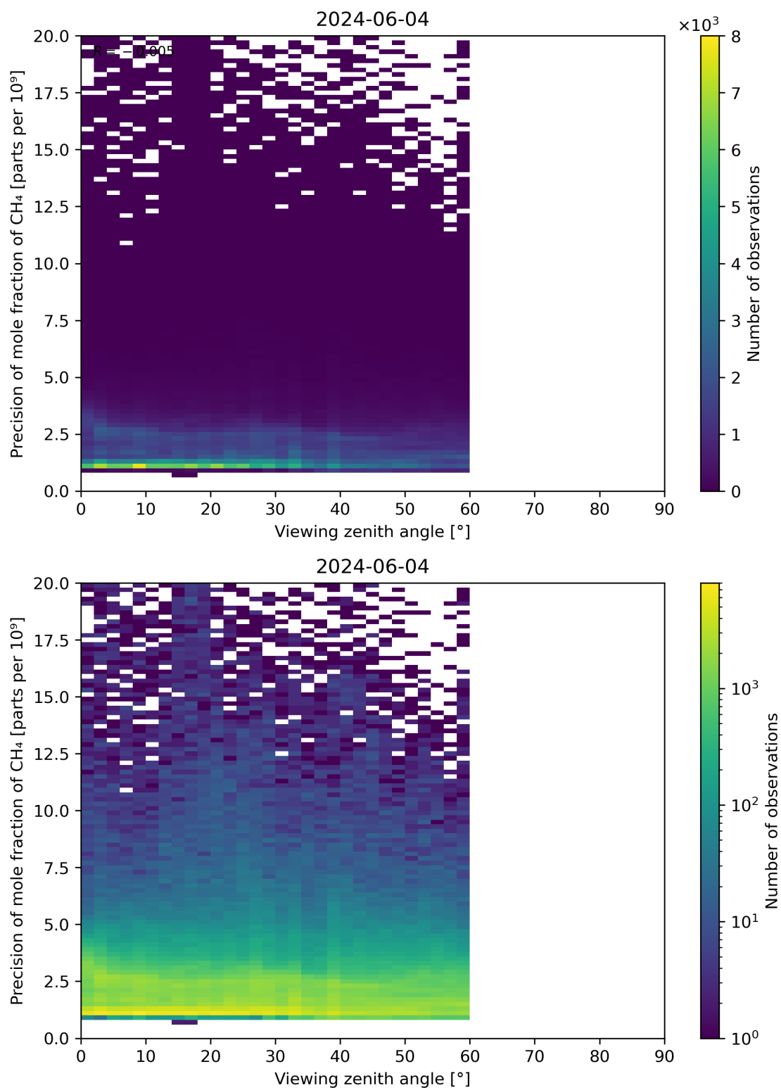
Figure 112: Scatter density plot of “Viewing zenith angle” against “Precision of mole fraction of \text{CH}_4 ” for 2024-06-03 to 2024-06-05.
