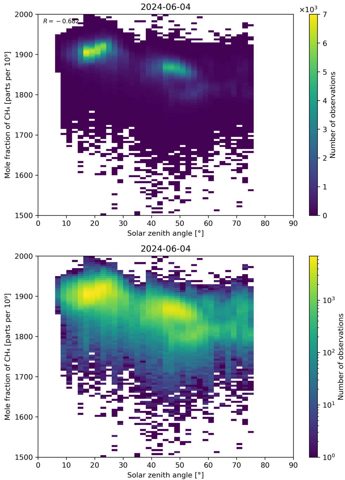
Figure 99: Scatter density plot of “Solar zenith angle” against “Mole fraction of CH 4 ” for 2024-06-03 to 2024-06-05.
