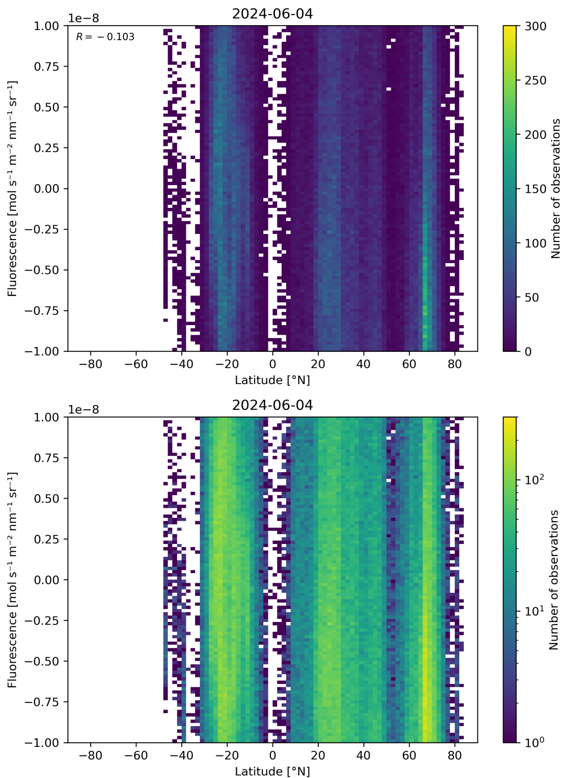
Figure 56: Scatter density plot of “Latitude” against “Fluorescence” for 2024-06-03 to 2024-06-05.
