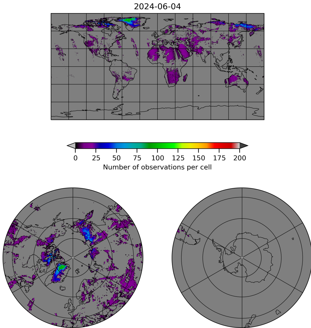
Figure 10: Map of the number of observations for 2024-06-03 to 2024-06-05
