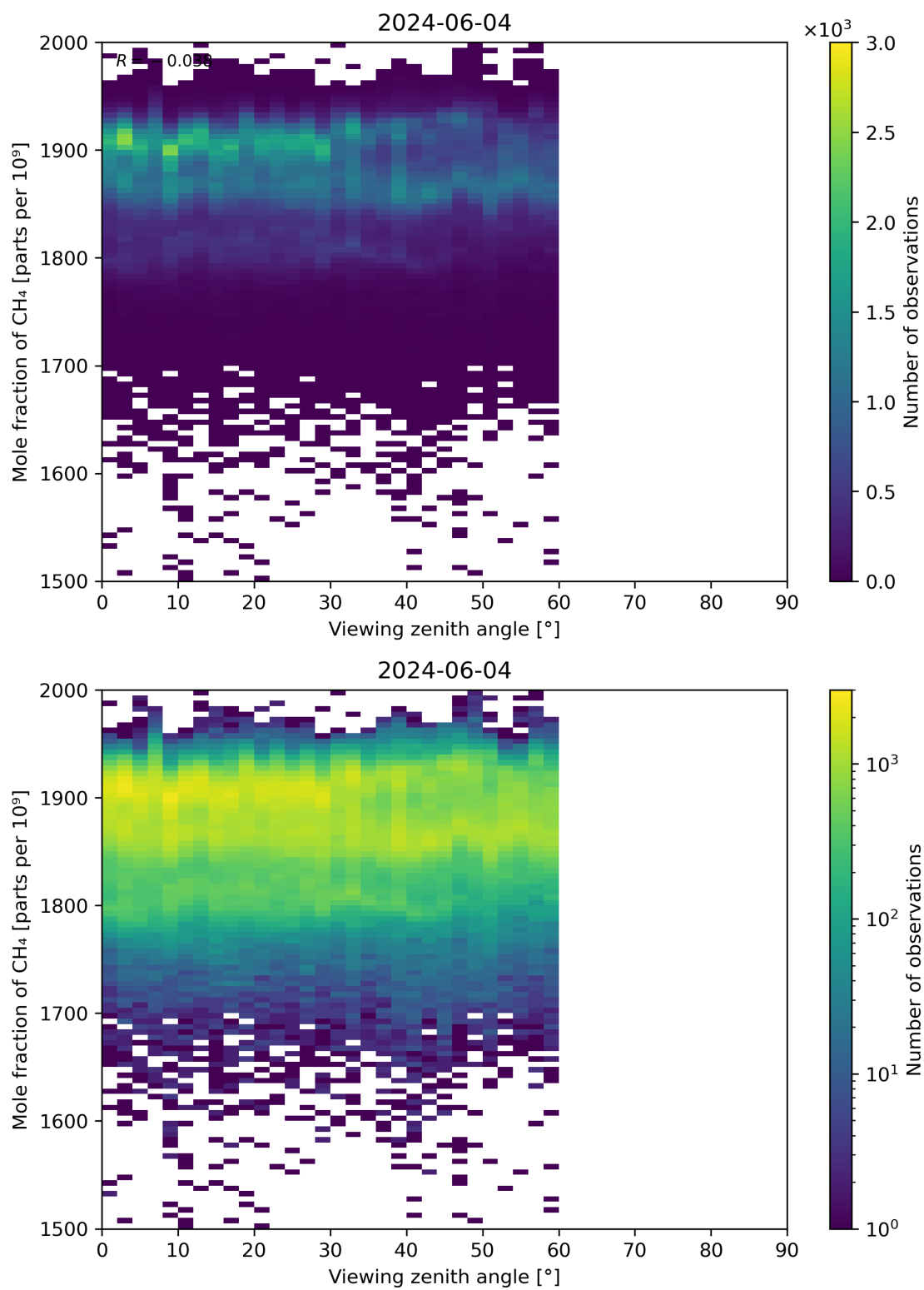
Figure 110: Scatter density plot of “Viewing zenith angle” against “Mole fraction of CH 4 ” for 2024-06-03 to 2024-06-05.
