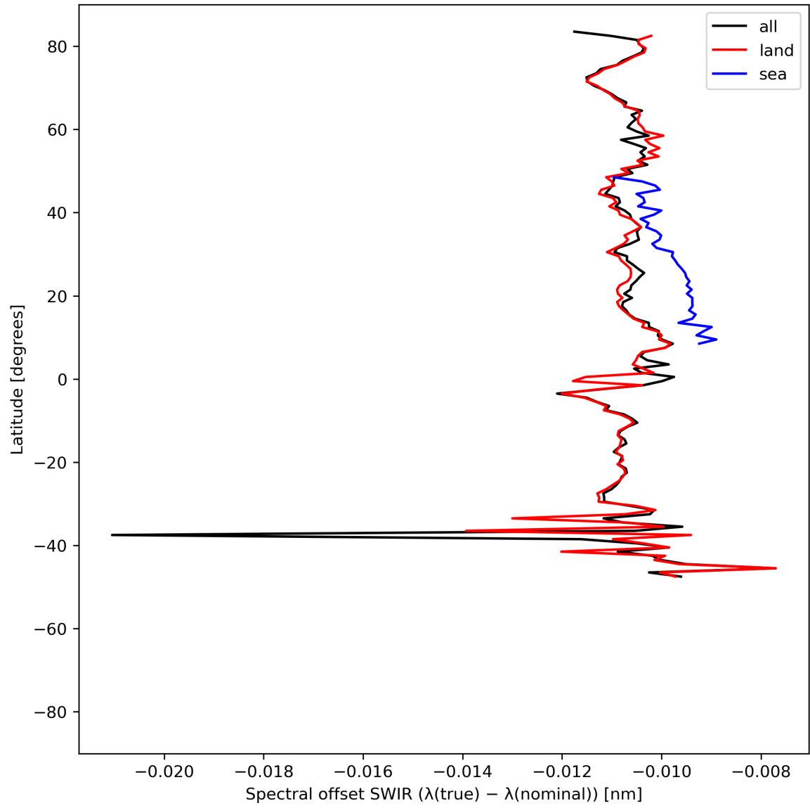
Figure 16: Zonal average of “Spectral offset SWIR ( \lambda(\text{true}) - \lambda(\text{nominal}) )” for 2024-06-03 to 2024-06-05.
