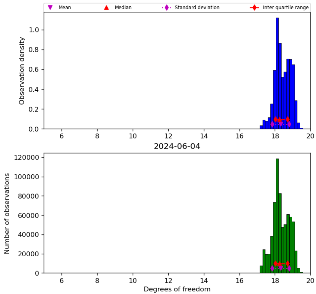
Figure 30: Histogram of “Degrees of freedom” for 2024-06-03 to 2024-06-05
