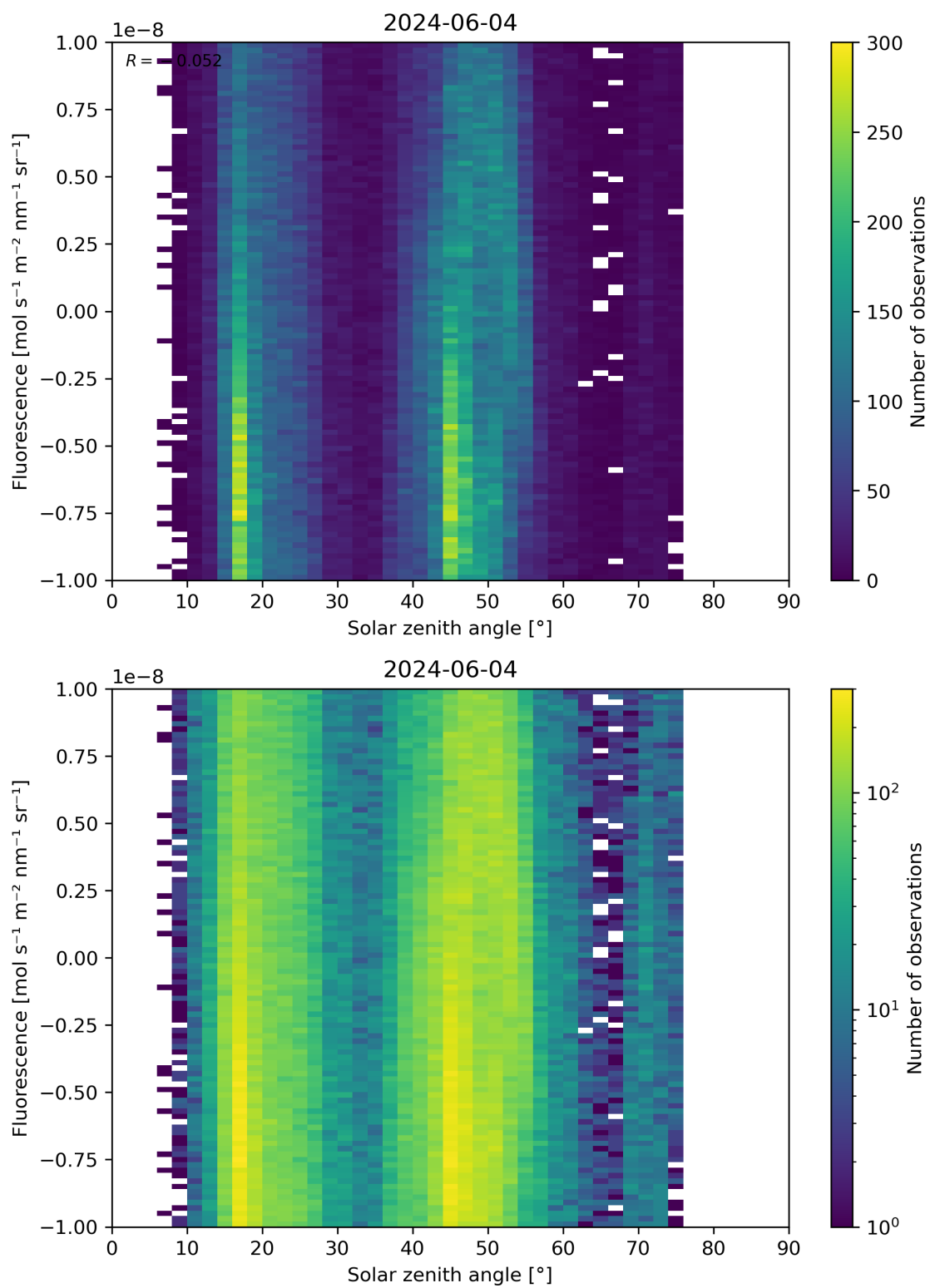
Figure 97: Scatter density plot of “Solar zenith angle” against “Fluorescence” for 2024-06-03 to 2024-06-05.
