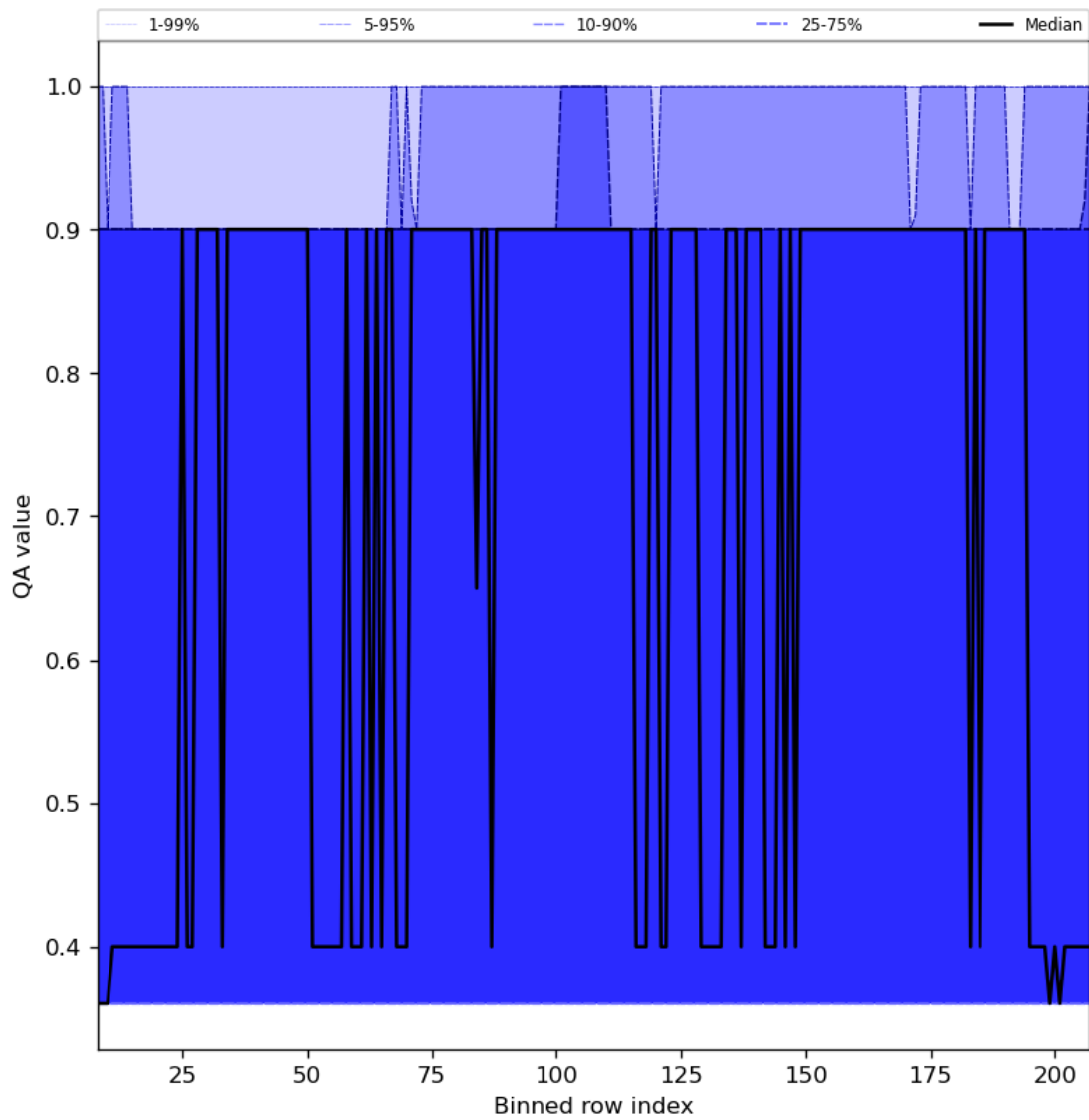
Figure 33: Along track statistics of “QA value” for 2024-06-03 to 2024-06-05
