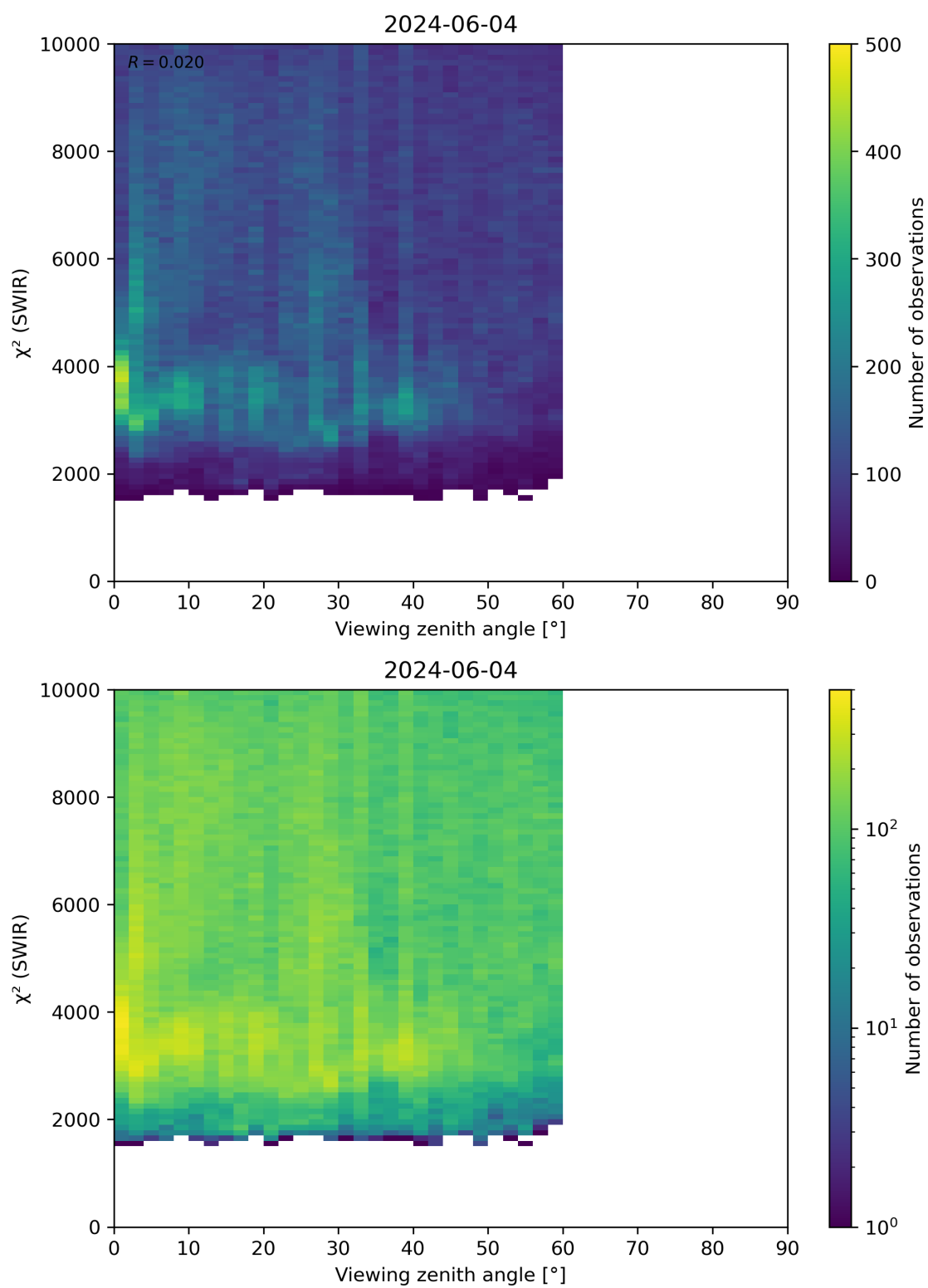
Figure 106: Scatter density plot of “Viewing zenith angle” against “ \chi^2 (SWIR)” for 2024-06-03 to 2024-06-05.
