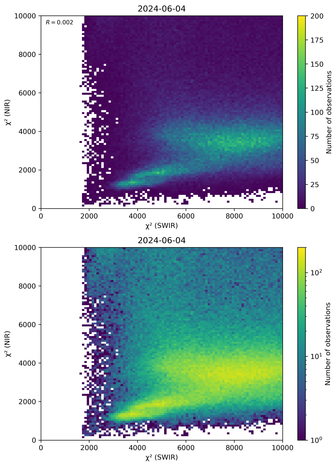
Figure 47: Scatter density plot of “ \chi^2 (SWIR)” against “ \chi^2 (NIR)” for 2024-06-03 to 2024-06-05.
