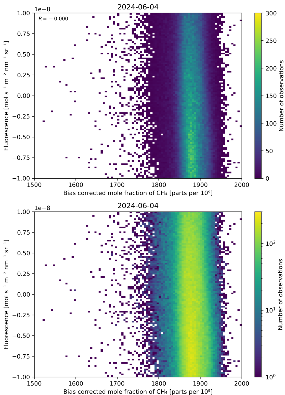
Figure 66: Scatter density plot of “Bias corrected mole fraction of \text{CH}_4 ” against “Fluorescence” for 2024-06-03 to 2024-06-05.
