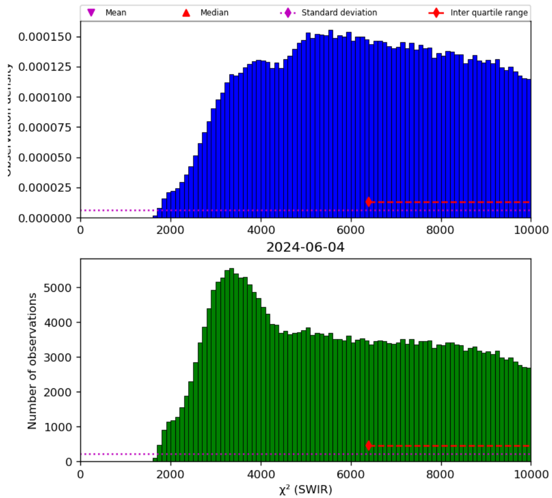
Figure 28: Histogram of “ \chi^2 (SWIR)” for 2024-06-03 to 2024-06-05
