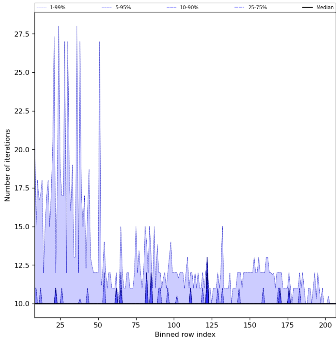
Figure 42: Along track statistics of “Number of iterations” for 2024-06-03 to 2024-06-05
