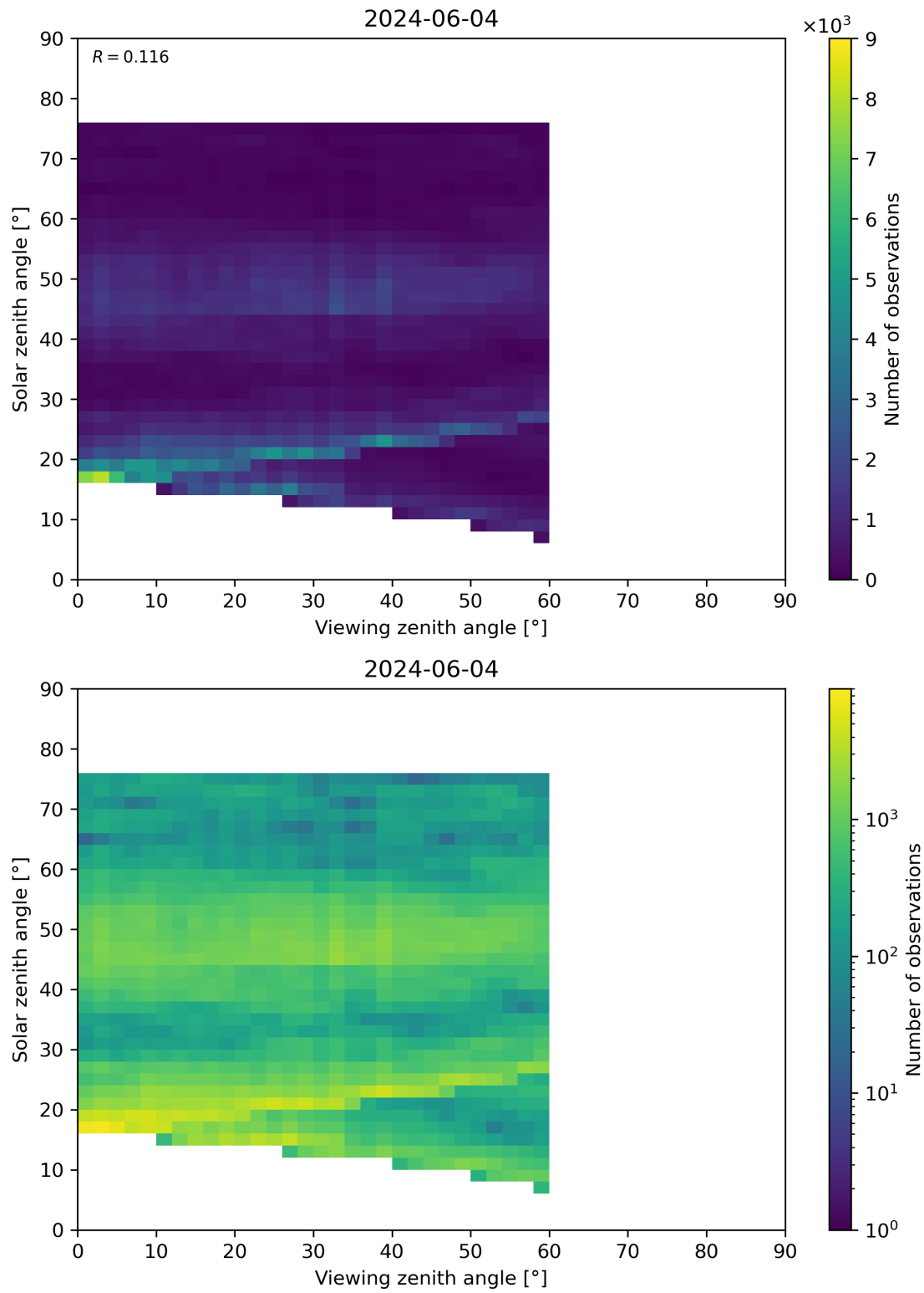
Figure 115: Scatter density plot of “Viewing zenith angle” against “Solar zenith angle” for 2024-06-03 to 2024-06-05.
