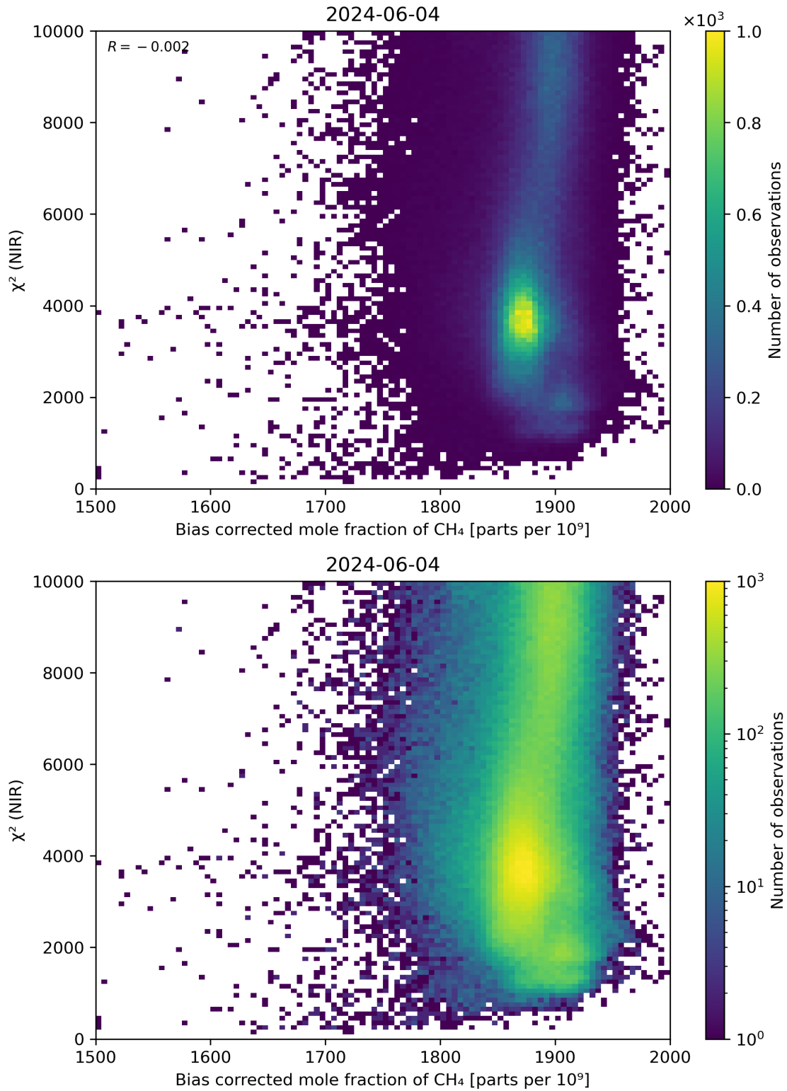
Figure 63: Scatter density plot of “Bias corrected mole fraction of CH 4 ” against “ \chi^2 (NIR)” for 2024-06-03 to 2024-06-05.
