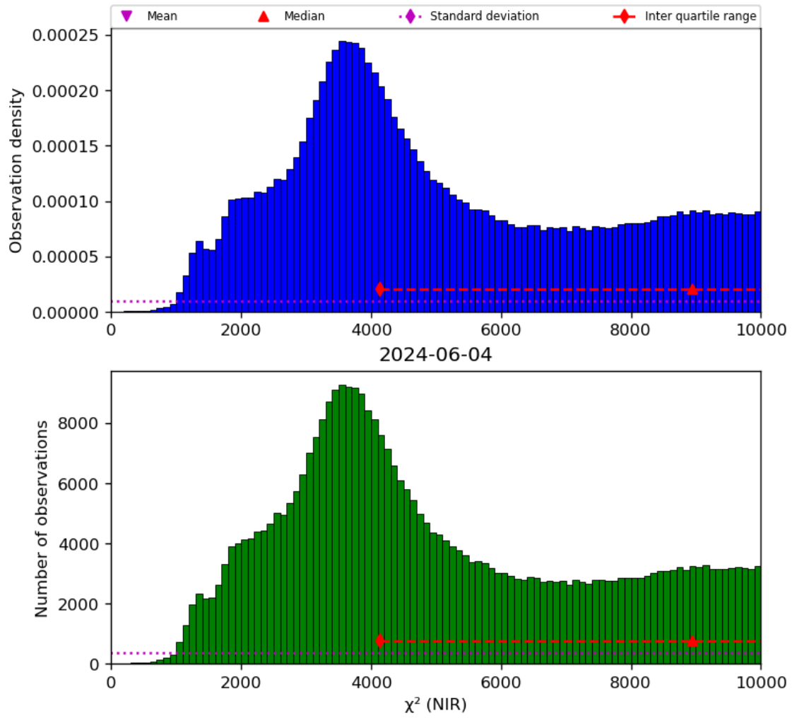
Figure 29: Histogram of “ \chi^2 (NIR)” for 2024-06-03 to 2024-06-05
