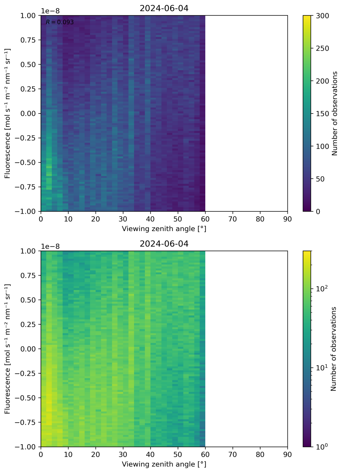
Figure 108: Scatter density plot of “Viewing zenith angle” against “Fluorescence” for 2024-06-03 to 2024-06-05.
