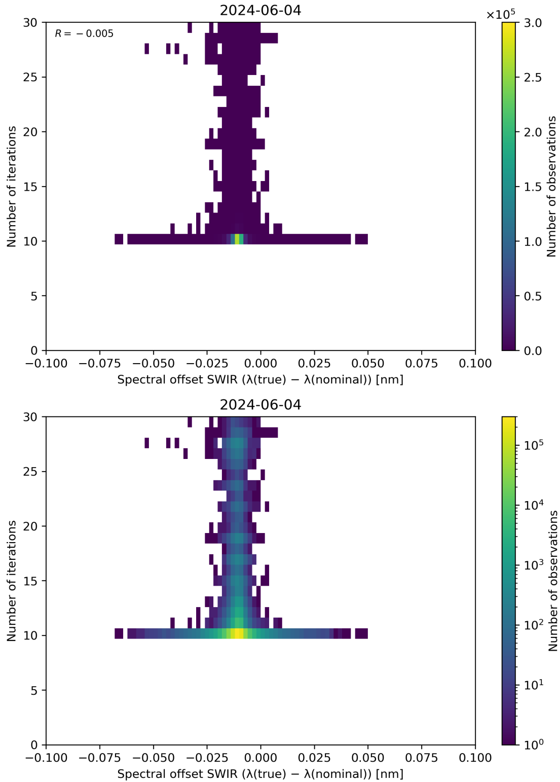
Figure 121: Scatter density plot of “Spectral offset SWIR ( \lambda(\text{true}) - \lambda(\text{nominal}) )” against “Number of iterations” for 2024-06-03 to 2024-06-05.
