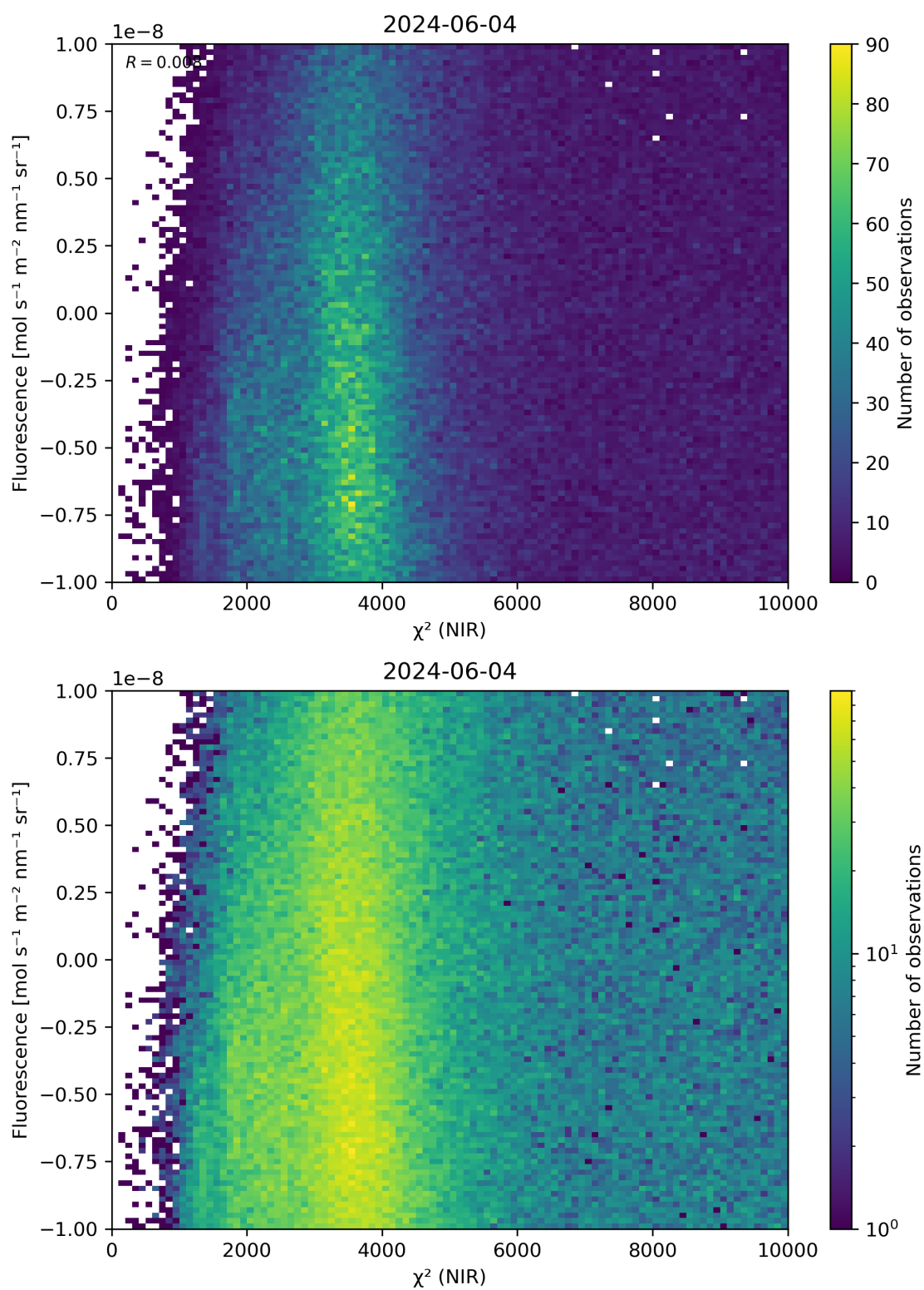
Figure 45: Scatter density plot of “ \chi^2 (NIR)” against “Fluorescence” for 2024-06-03 to 2024-06-05.
