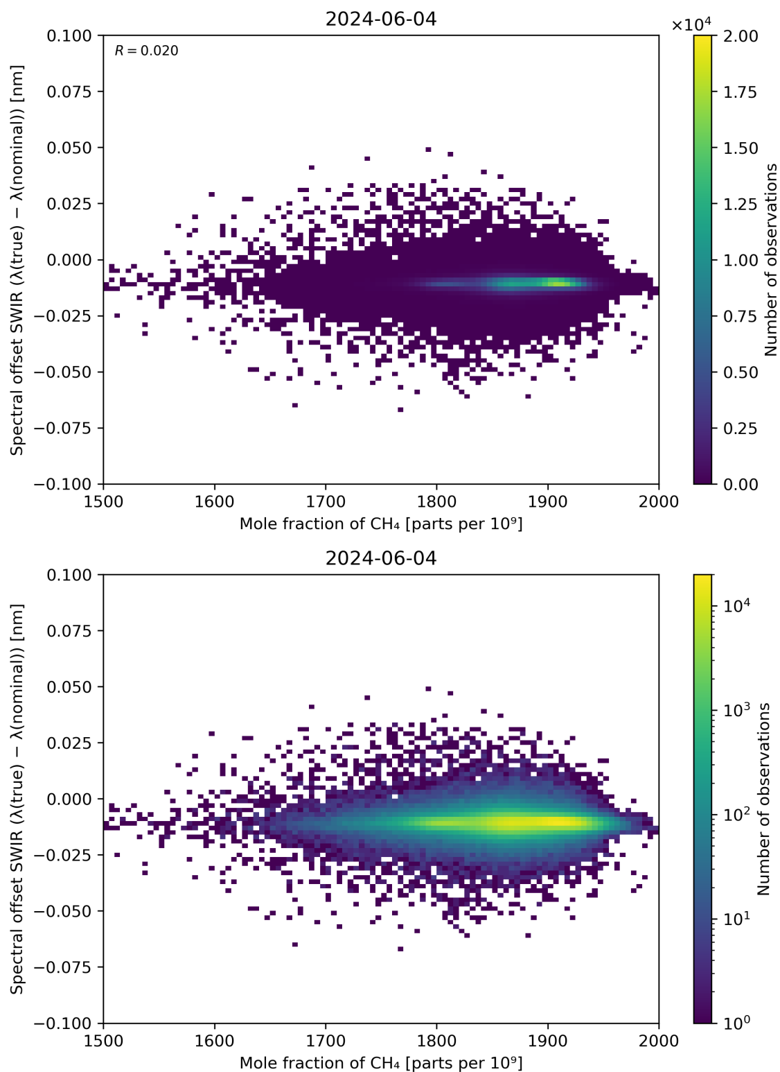
Figure 86: Scatter density plot of “Mole fraction of CH 4 ” against “Spectral offset SWIR ( \lambda(\text{true}) - \lambda(\text{nominal}) )” for 2024-06-03 to 2024-06-05.
