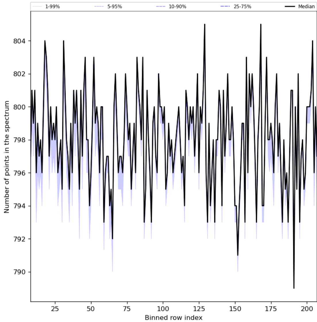
Figure 37: Along track statistics of “Number of points in the spectrum” for 2024-06-03 to 2024-06-05
