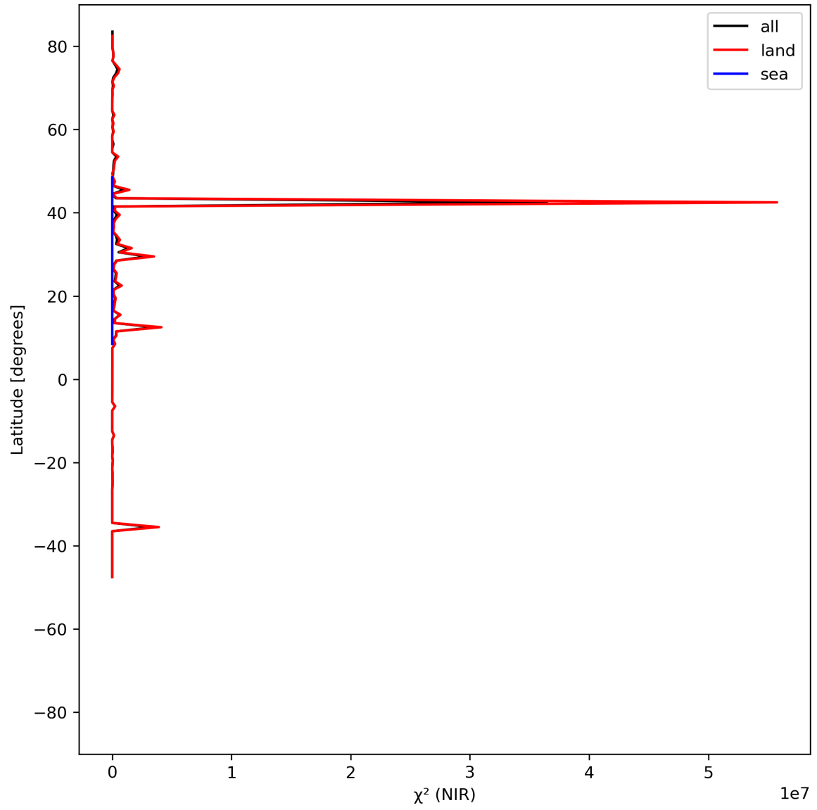
Figure 18: Zonal average of “ \chi^2 (NIR)” for 2024-06-03 to 2024-06-05.
