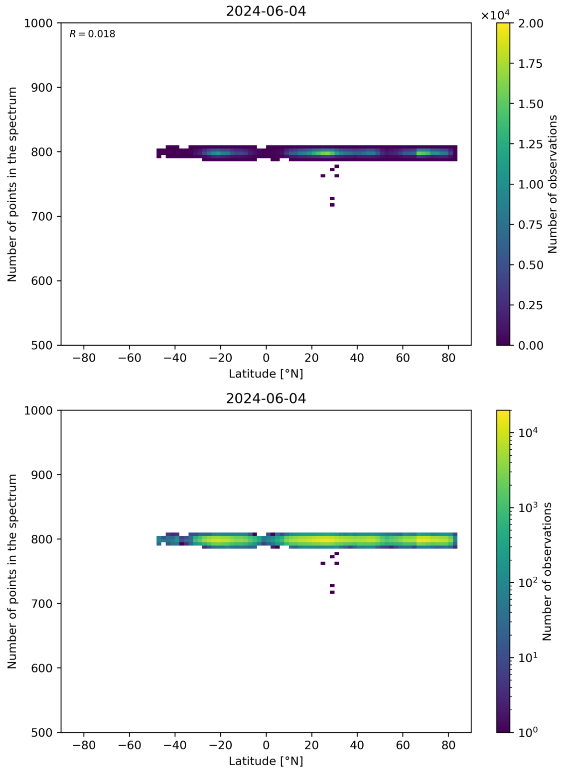
Figure 61: Scatter density plot of “Latitude” against “Number of points in the spectrum” for 2024-06-03 to 2024-06-05.
