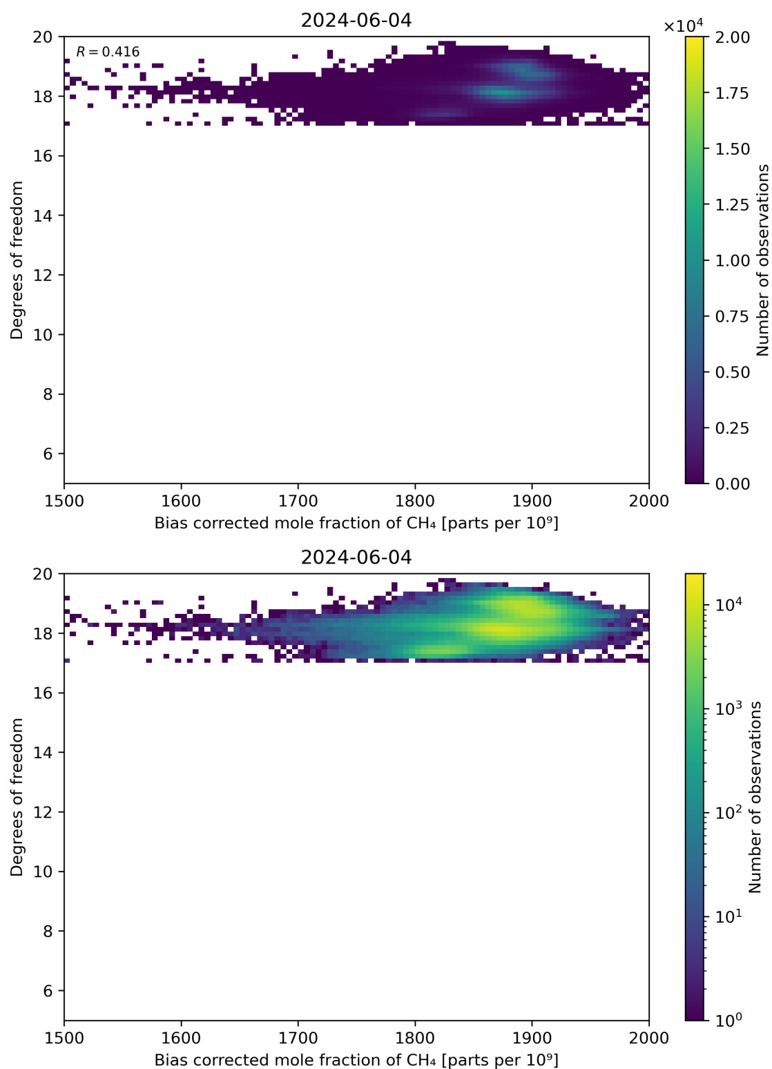
Figure 65: Scatter density plot of “Bias corrected mole fraction of CH 4 ” against “Degrees of freedom” for 2024-06-03 to 2024-06-05.
