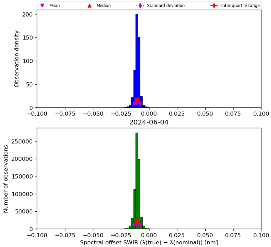
Figure 27: Histogram of “Spectral offset SWIR ( \lambda(\text{true}) - \lambda(\text{nominal}) )” for 2024-06-03 to 2024-06-05
