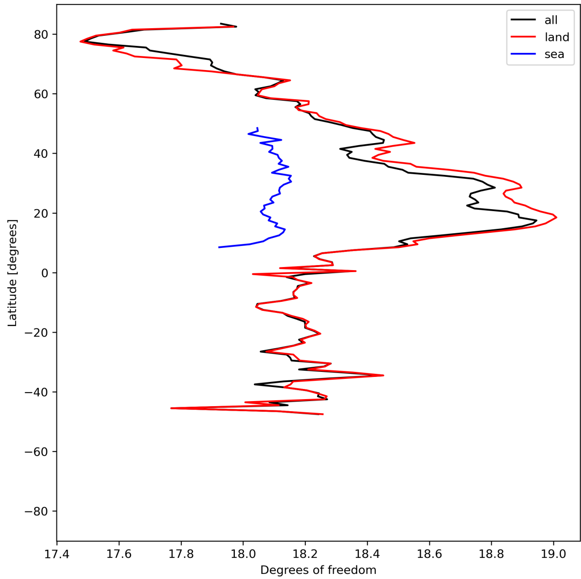
Figure 19: Zonal average of “Degrees of freedom” for 2024-06-03 to 2024-06-05.
