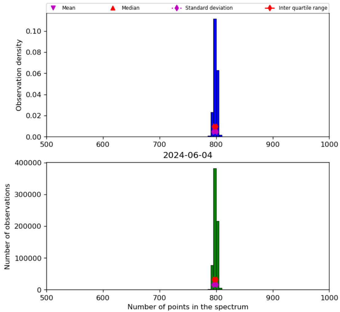
Figure 26: Histogram of “Number of points in the spectrum” for 2024-06-03 to 2024-06-05
