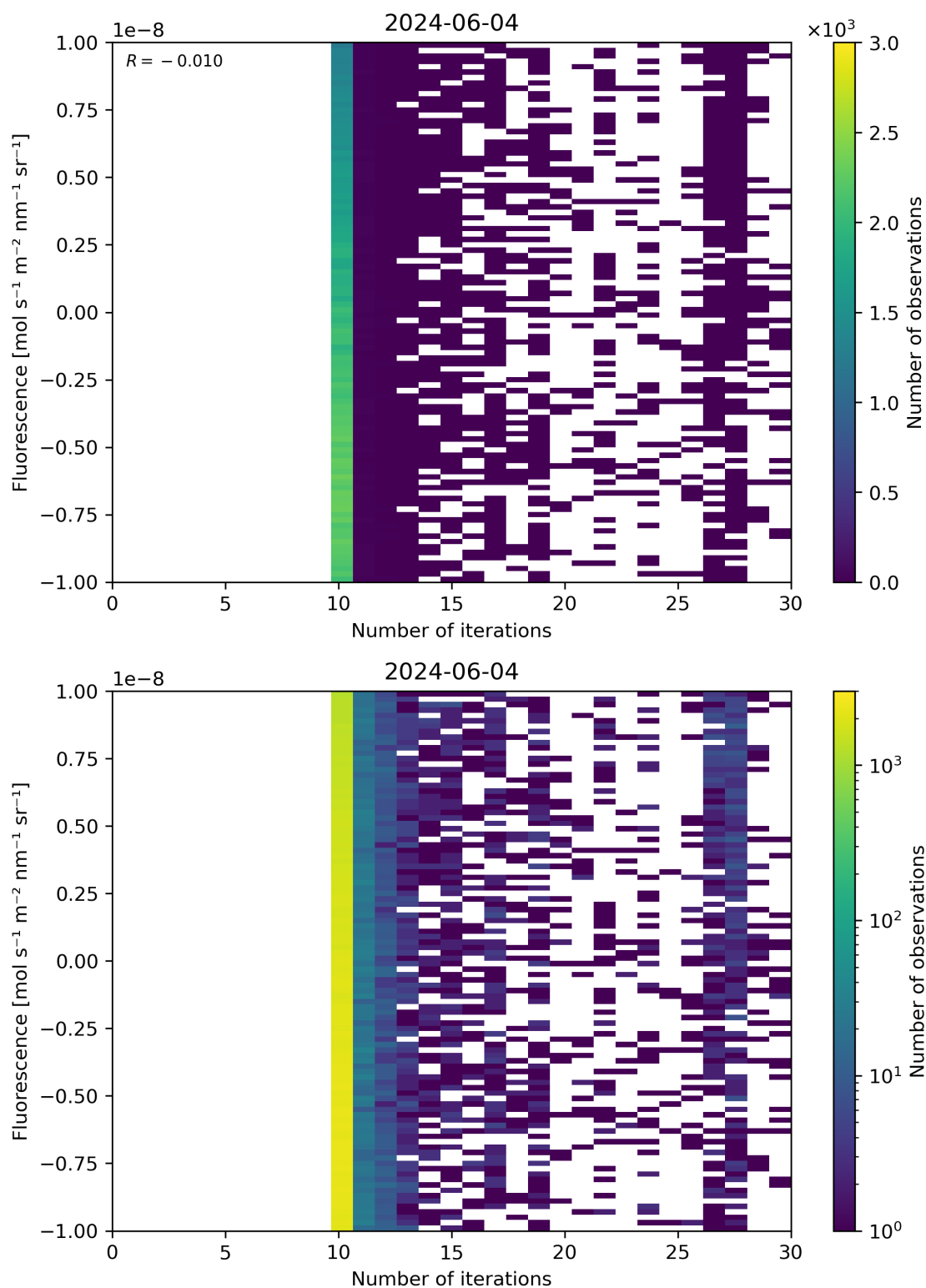
Figure 87: Scatter density plot of “Number of iterations” against “Fluorescence” for 2024-06-03 to 2024-06-05.
