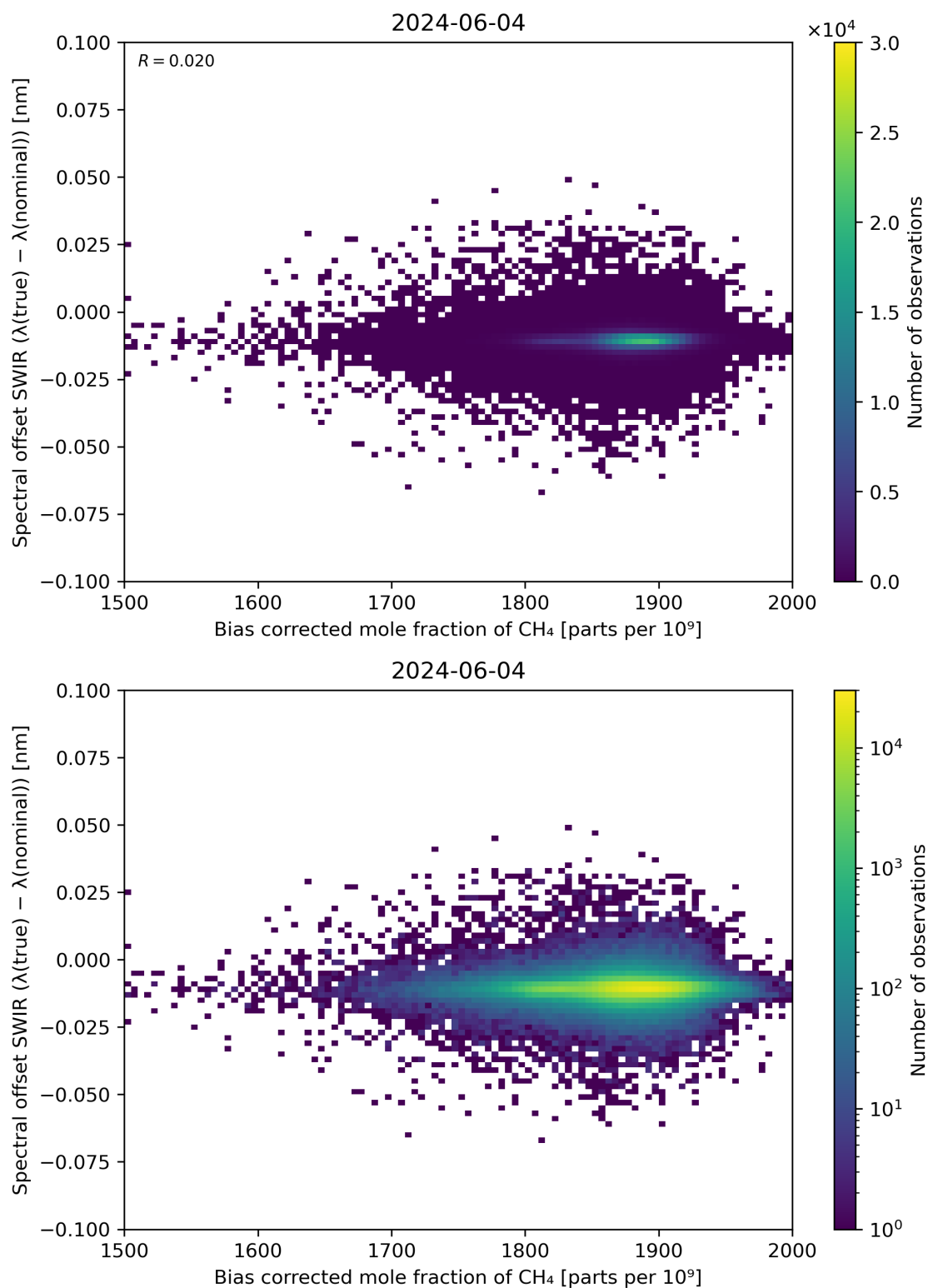
Figure 69: Scatter density plot of “Bias corrected mole fraction of \text{CH}_4 ” against “Spectral offset SWIR ( \lambda(\text{true}) - \lambda(\text{nominal}) )” for 2024-06-03 to 2024-06-05.
