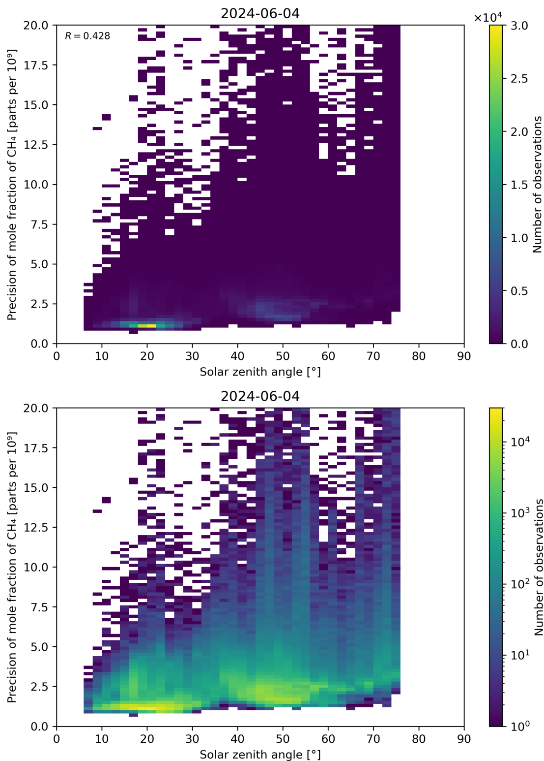
Figure 101: Scatter density plot of “Solar zenith angle” against “Precision of mole fraction of CH 4 ” for 2024-06-03 to 2024-06-05.
