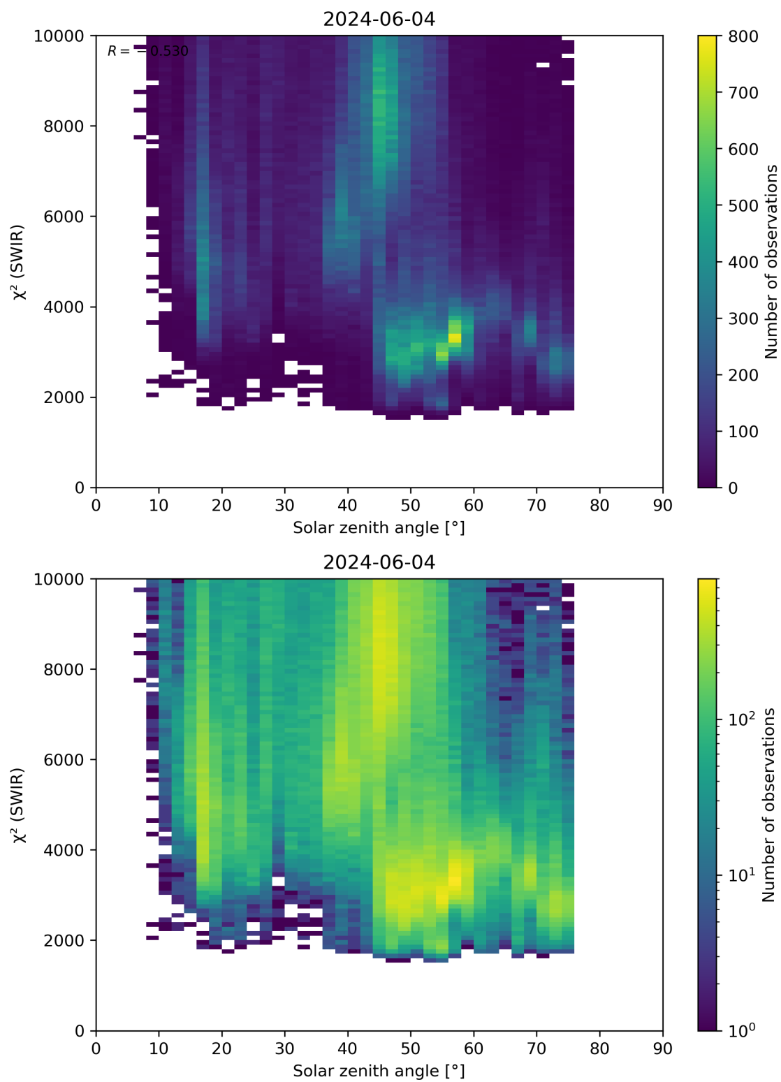
Figure 95: Scatter density plot of “Solar zenith angle” against “ \chi^2 (SWIR)” for 2024-06-03 to 2024-06-05.
