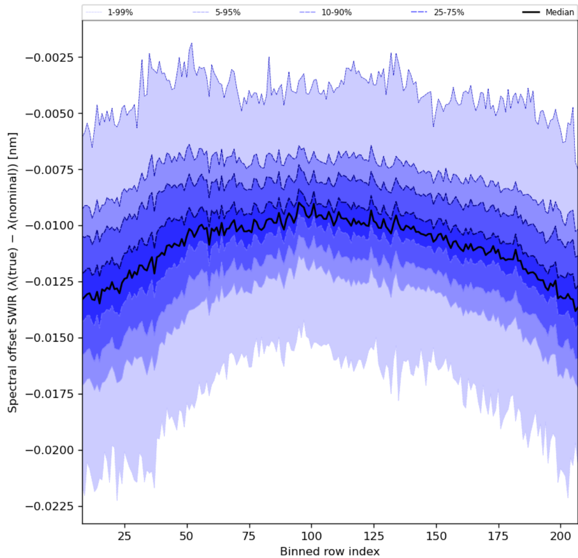
Figure 38: Along track statistics of "Spectral offset SWIR ( \lambda(\text{true}) - \lambda(\text{nominal}) )" for 2024-06-03 to 2024-06-05
