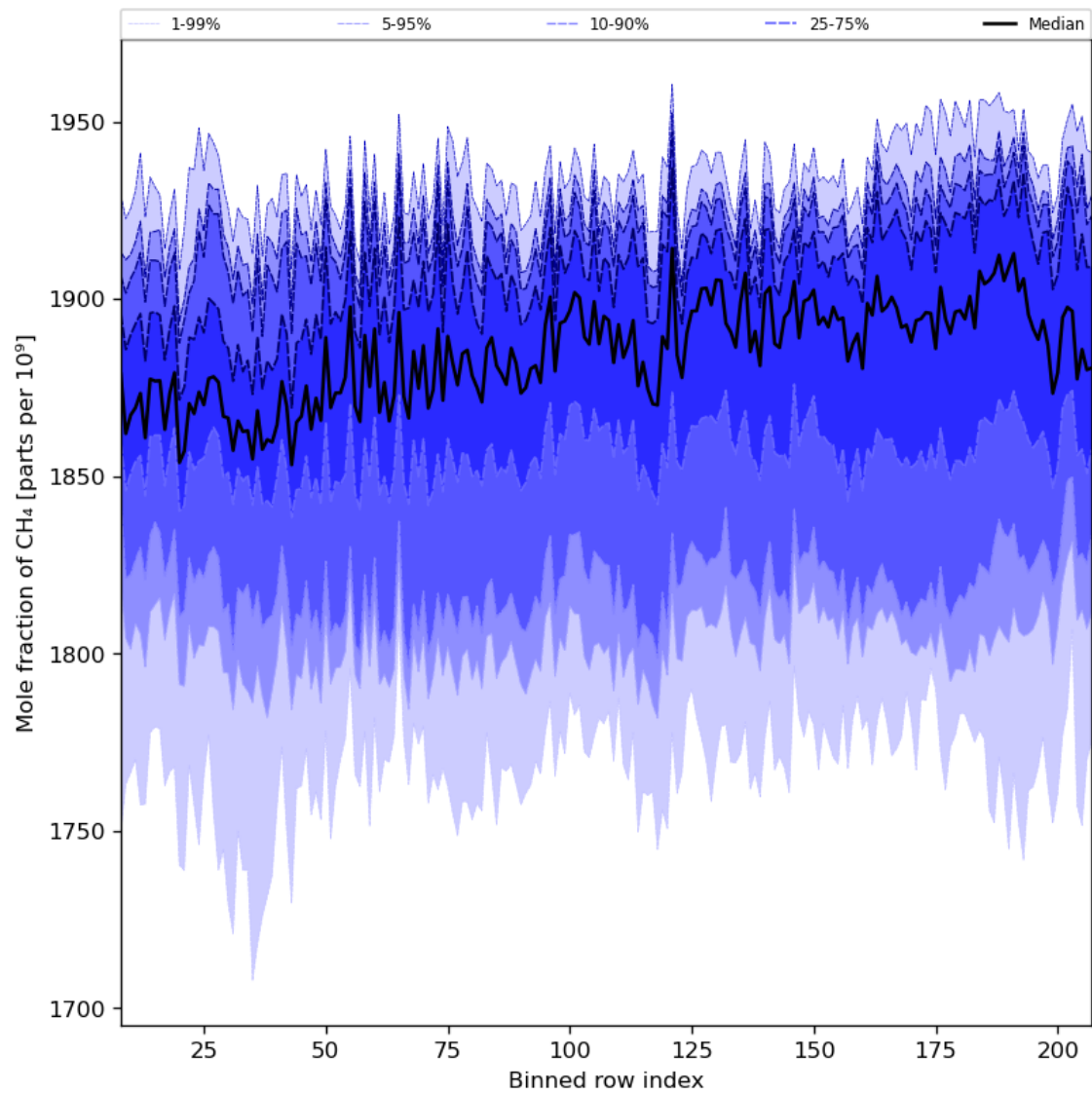
Figure 34: Along track statistics of “Mole fraction of CH 4 ” for 2024-06-03 to 2024-06-05
