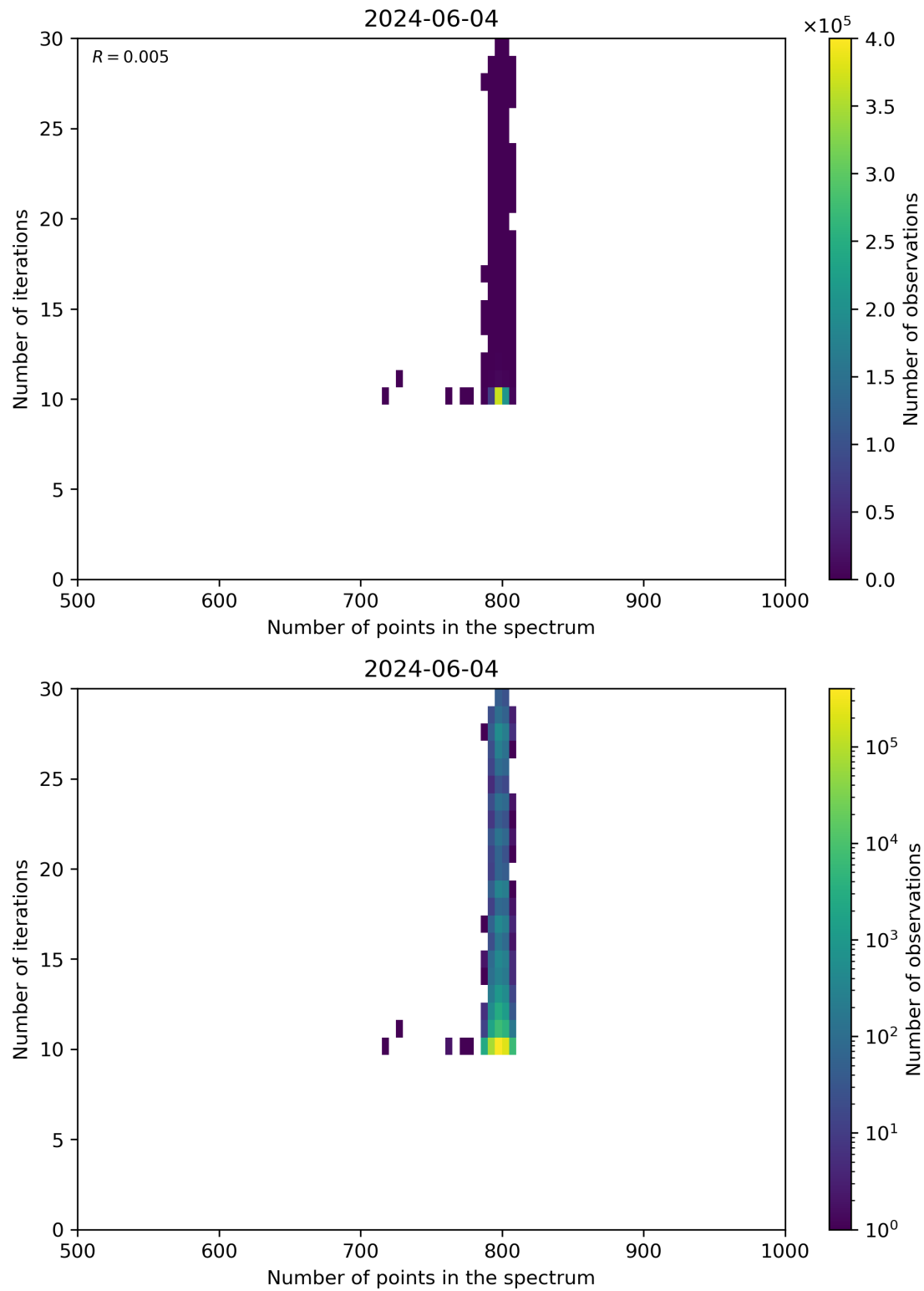
Figure 92: Scatter density plot of “Number of points in the spectrum” against “Number of iterations” for 2024-06-03 to 2024-06-05.
