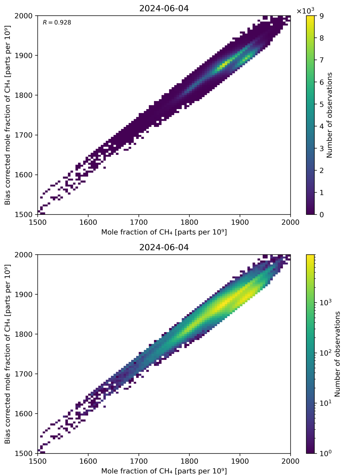
Figure 74: Scatter density plot of “Mole fraction of CH 4 ” against “Bias corrected mole fraction of CH 4 ” for 2024-06-03 to 2024-06-05.
