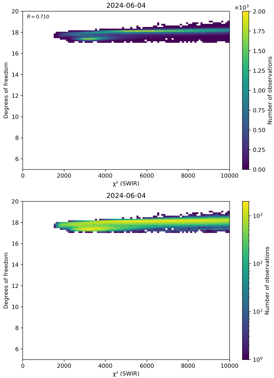
Figure 48: Scatter density plot of “ \chi^2 (SWIR)” against “Degrees of freedom” for 2024-06-03 to 2024-06-05.
