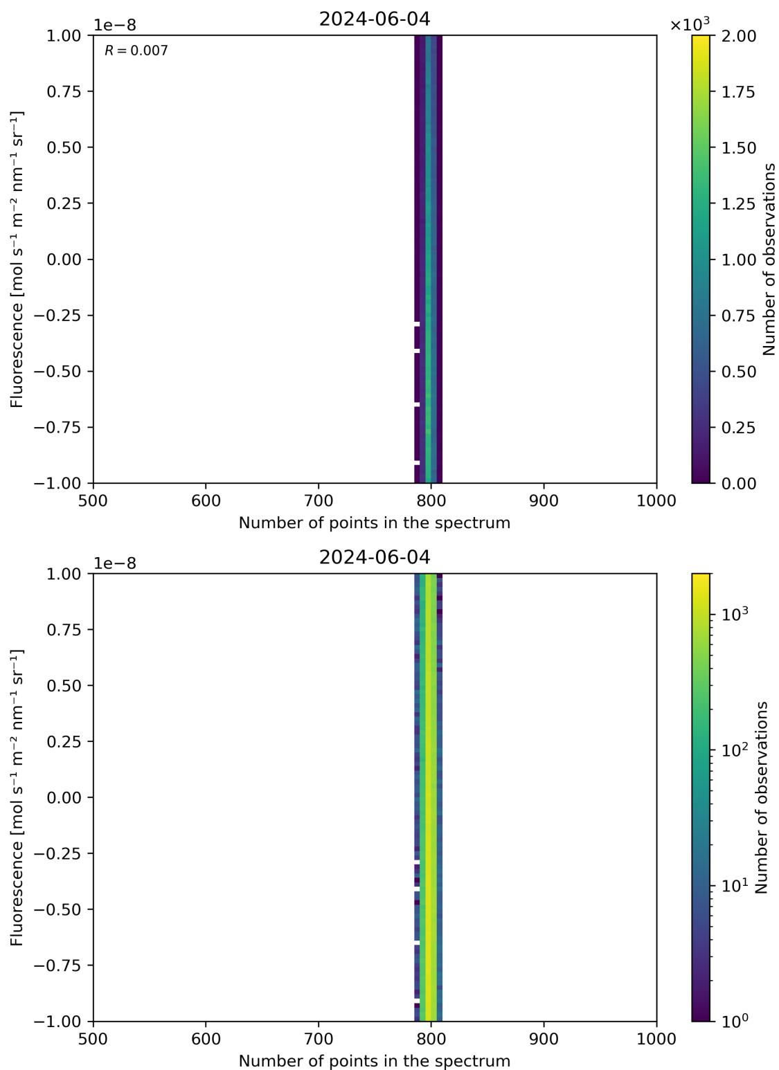
Figure 91: Scatter density plot of “Number of points in the spectrum” against “Fluorescence” for 2024-06-03 to 2024-06-05.
