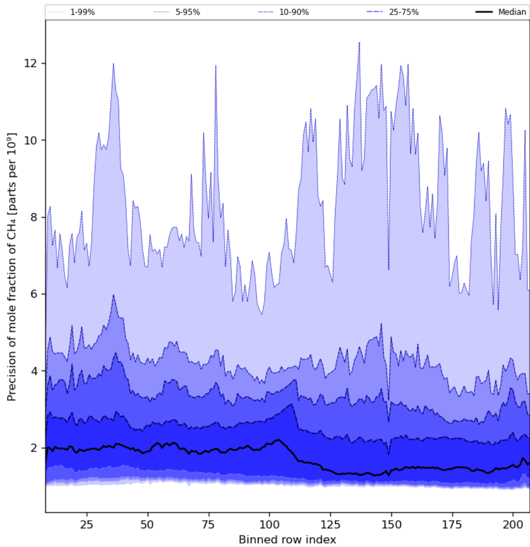
Figure 35: Along track statistics of “Precision of mole fraction of CH 4 ” for 2024-06-03 to 2024-06-05
