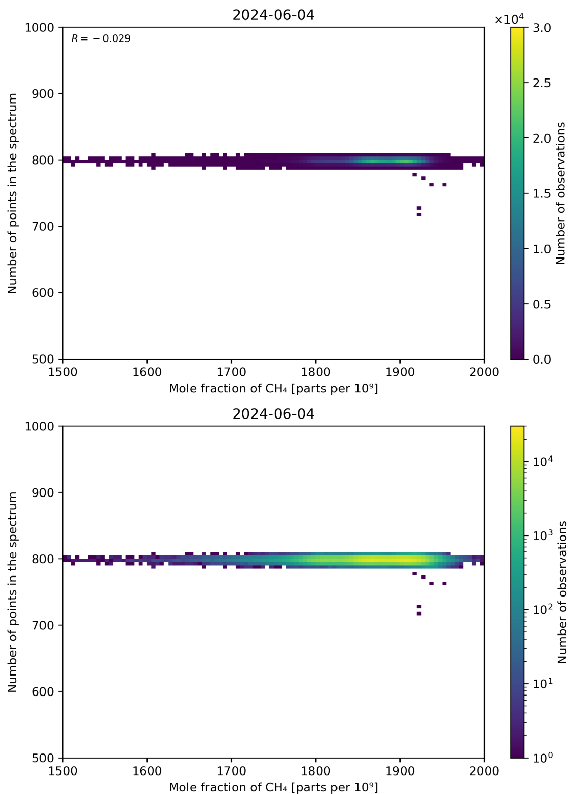
Figure 77: Scatter density plot of “Mole fraction of CH 4 ” against “Number of points in the spectrum” for 2024-06-03 to 2024-06-05.
