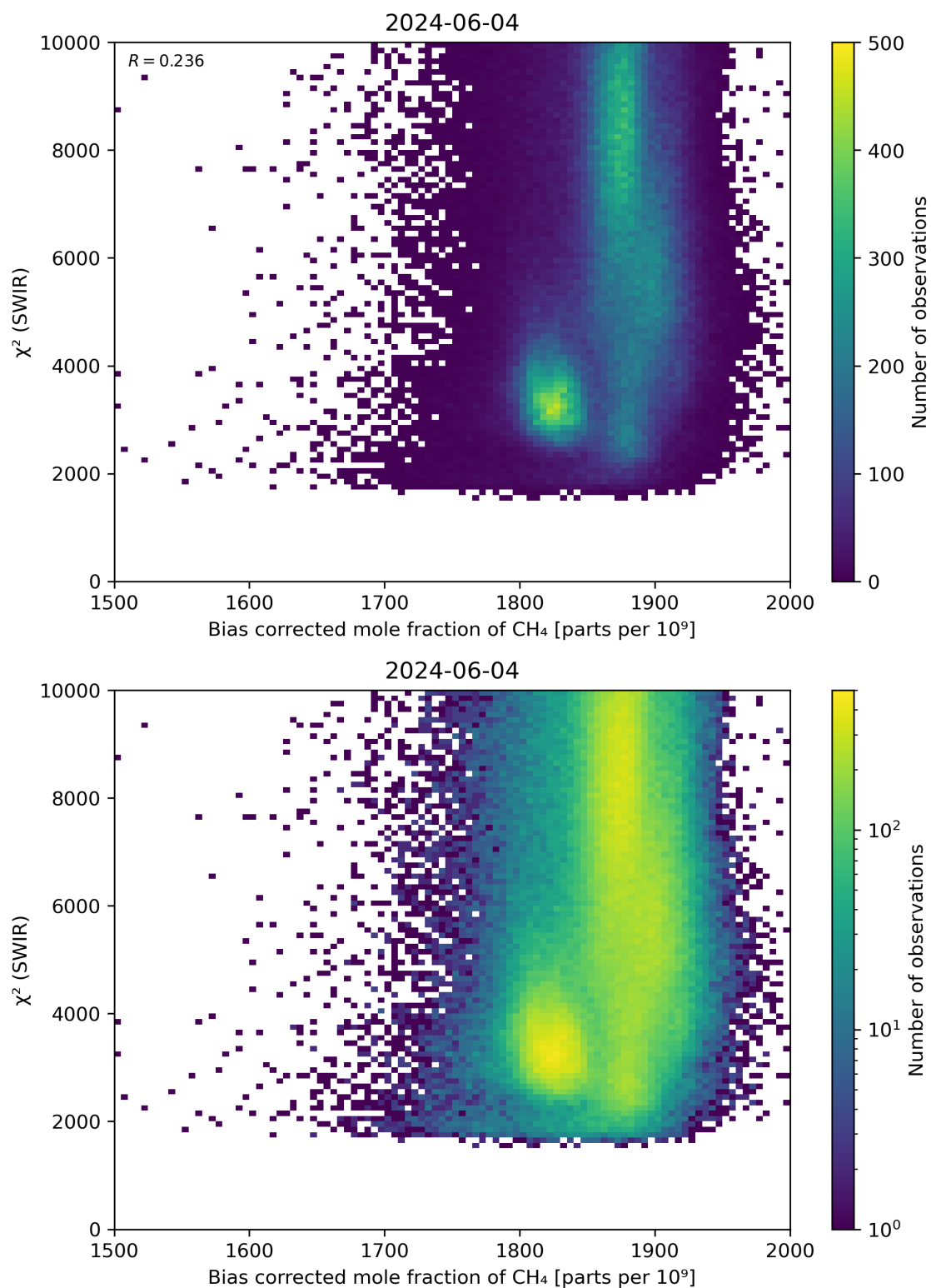
Figure 64: Scatter density plot of “Bias corrected mole fraction of \text{CH}_4 ” against “ \chi^2 (SWIR)” for 2024-06-03 to 2024-06-05.
