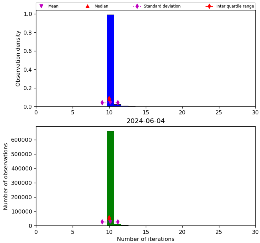
Figure 31: Histogram of “Number of iterations” for 2024-06-03 to 2024-06-05
