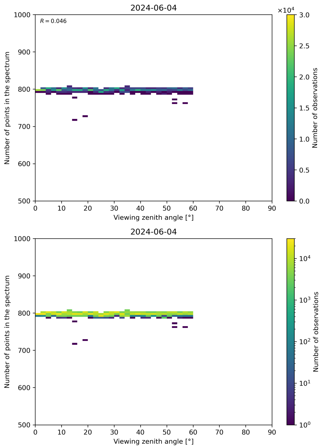
Figure 114: Scatter density plot of “Viewing zenith angle” against “Number of points in the spectrum” for 2024-06-03 to 2024-06-05.
