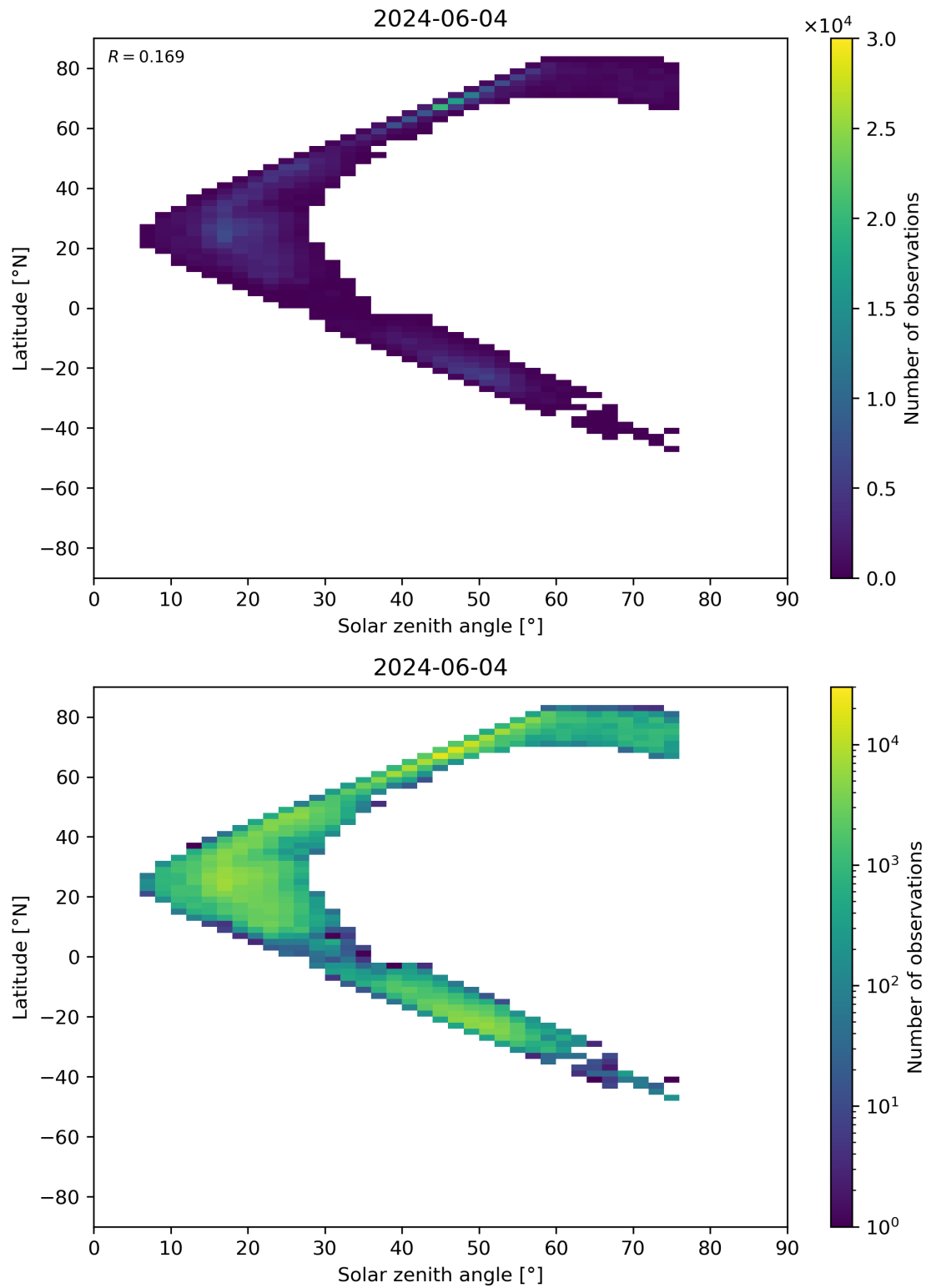
Figure 98: Scatter density plot of “Solar zenith angle” against “Latitude” for 2024-06-03 to 2024-06-05.
