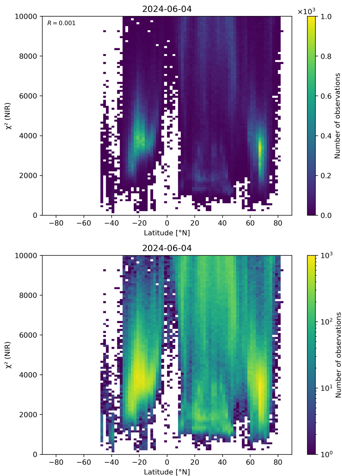
Figure 53: Scatter density plot of “Latitude” against “ \chi^2 (NIR)” for 2024-06-03 to 2024-06-05.
