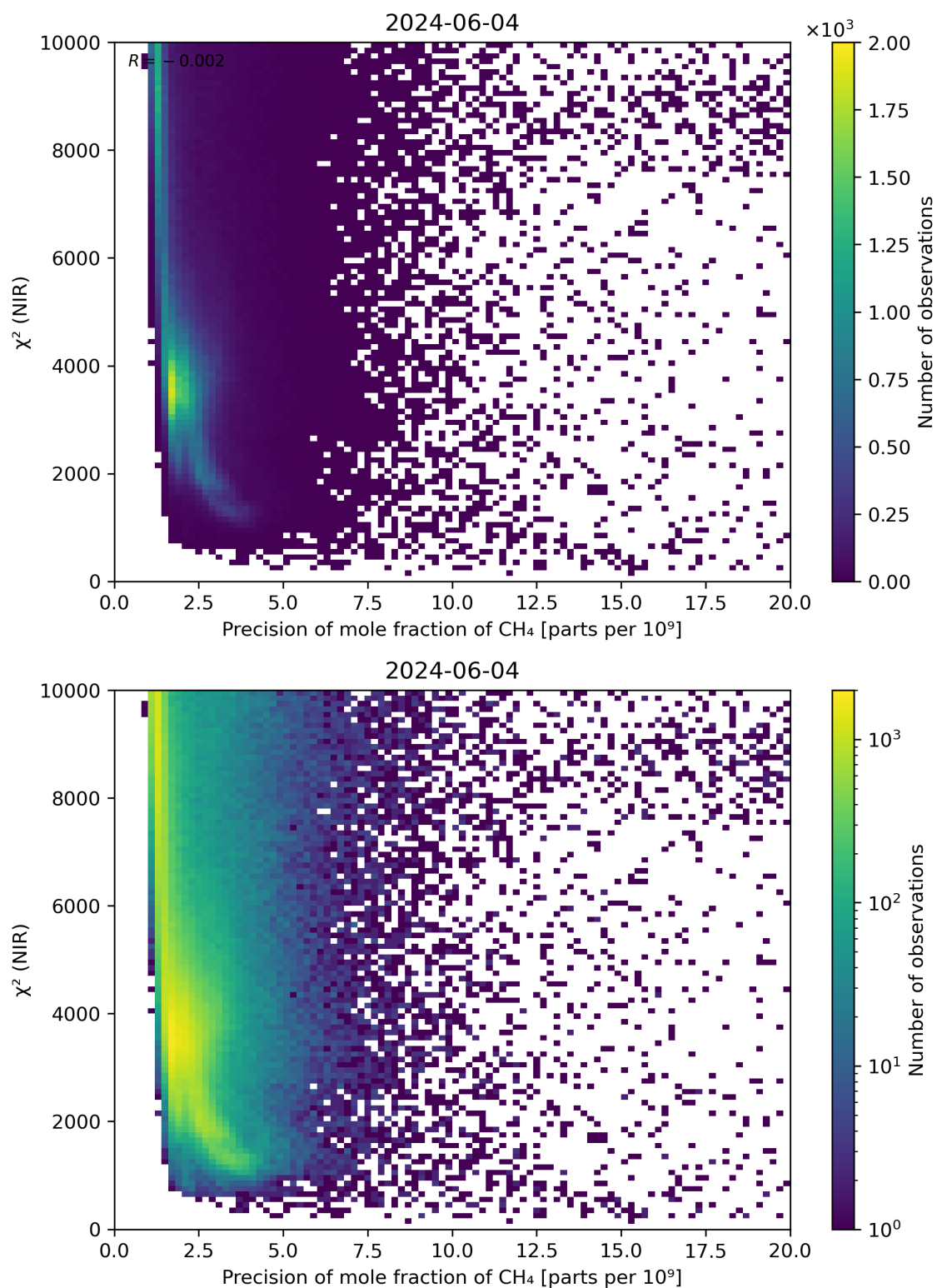
Figure 78: Scatter density plot of “Precision of mole fraction of \text{CH}_4 ” against “ \chi^2 (NIR)” for 2024-06-03 to 2024-06-05.
