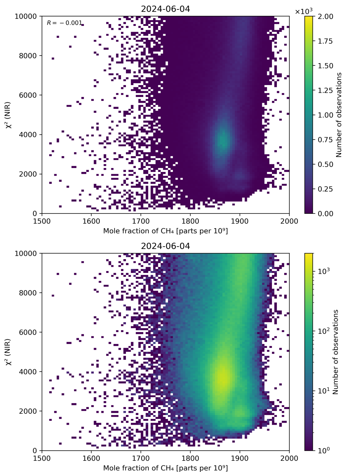
Figure 70: Scatter density plot of “Mole fraction of \text{CH}_4 ” against “ \chi^2 (NIR)” for 2024-06-03 to 2024-06-05.
