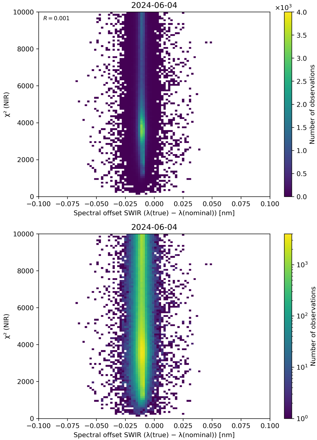
Figure 117: Scatter density plot of “Spectral offset SWIR ( \lambda(\text{true}) - \lambda(\text{nominal}) )” against “ \chi^2 (NIR)” for 2024-06-03 to 2024-06-05.
