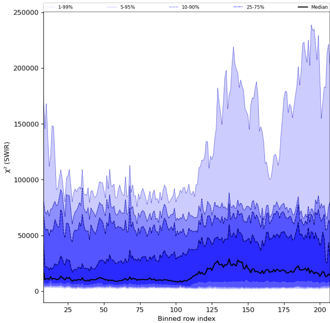
Figure 39: Along track statistics of " \chi^2 (SWIR)" for 2024-06-03 to 2024-06-05
