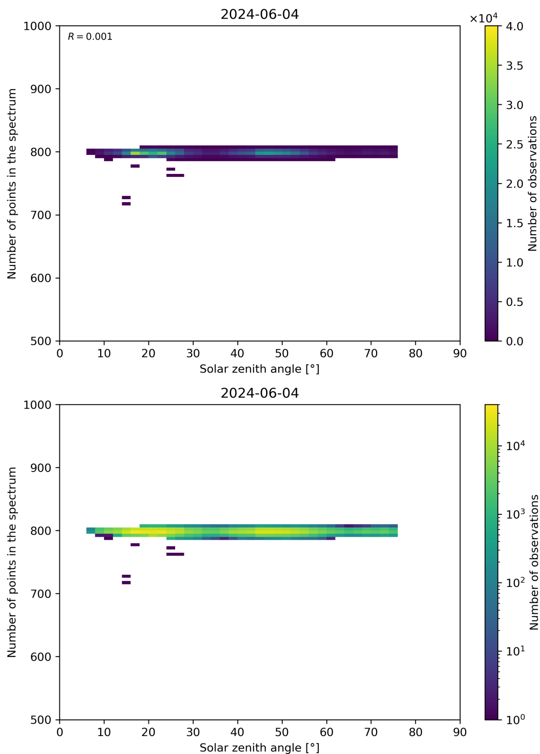
Figure 103: Scatter density plot of “Solar zenith angle” against “Number of points in the spectrum” for 2024-06-03 to 2024-06-05.
