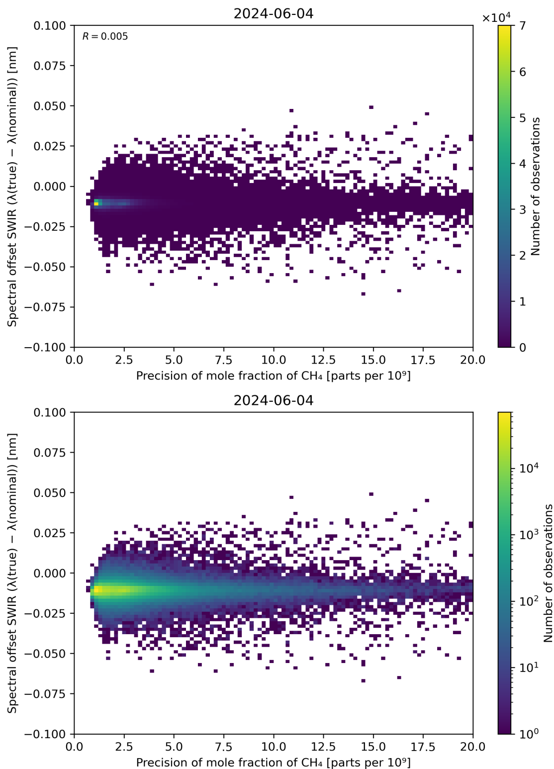
Figure 85: Scatter density plot of “Precision of mole fraction of CH 4 ” against “Spectral offset SWIR ( \lambda(\text{true}) - \lambda(\text{nominal}) )” for 2024-06-03 to 2024-06-05.
