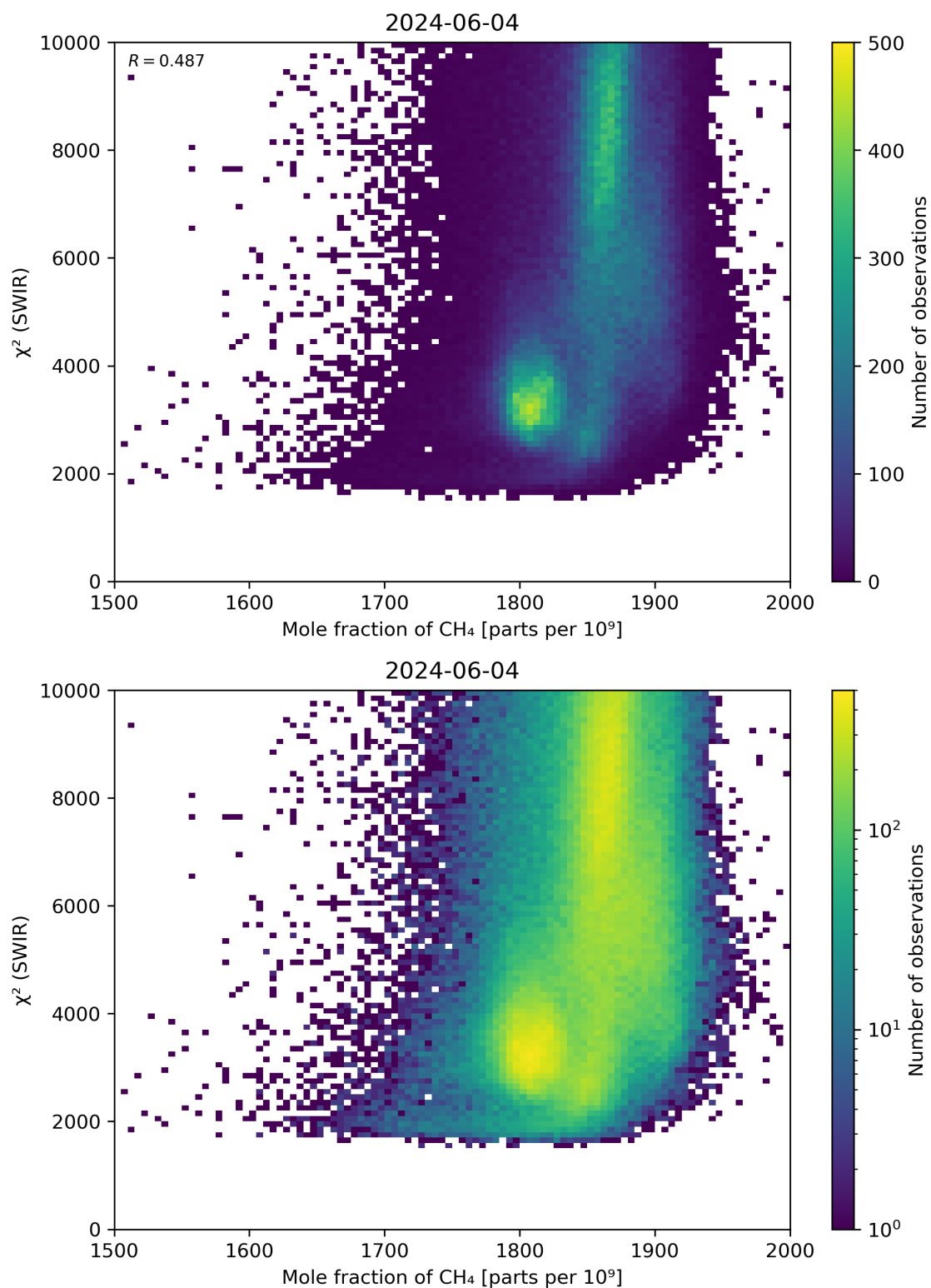
Figure 71: Scatter density plot of “Mole fraction of \text{CH}_4 ” against “ \chi^2 (SWIR)” for 2024-06-03 to 2024-06-05.
