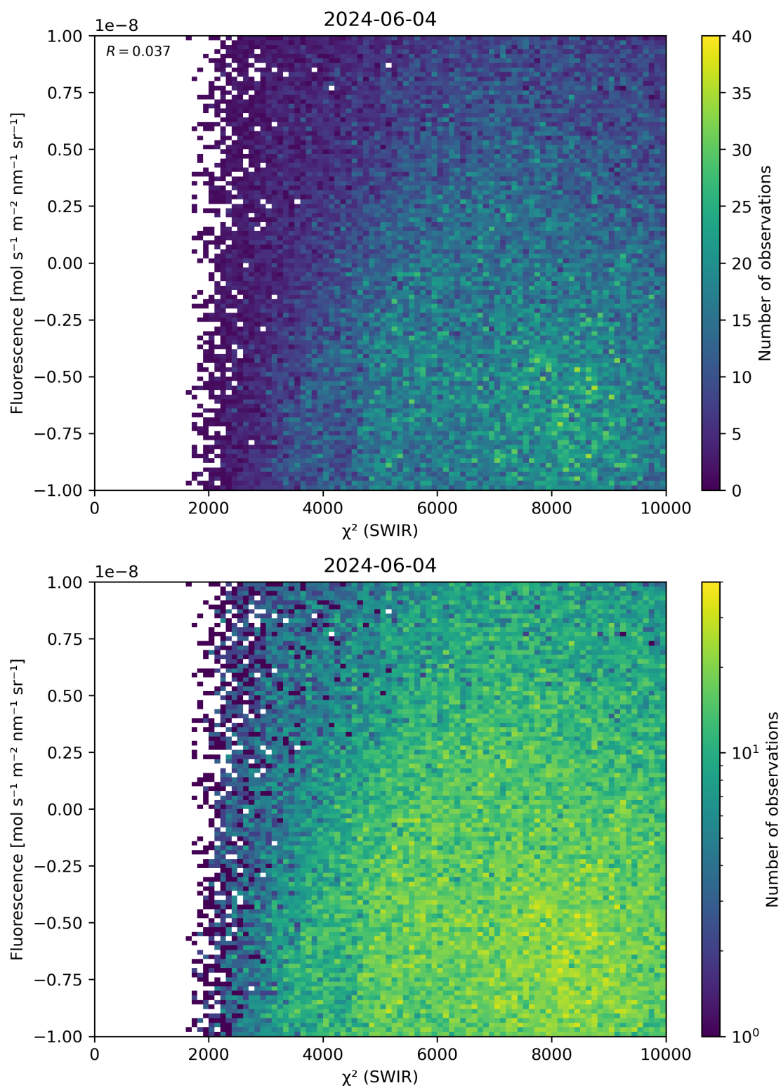
Figure 49: Scatter density plot of “ \chi^2 (SWIR)” against “Fluorescence” for 2024-06-03 to 2024-06-05.
