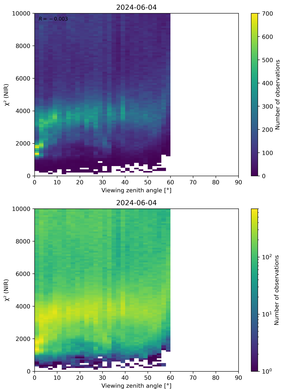
Figure 105: Scatter density plot of “Viewing zenith angle” against “ \chi^2 (NIR)” for 2024-06-03 to 2024-06-05.
