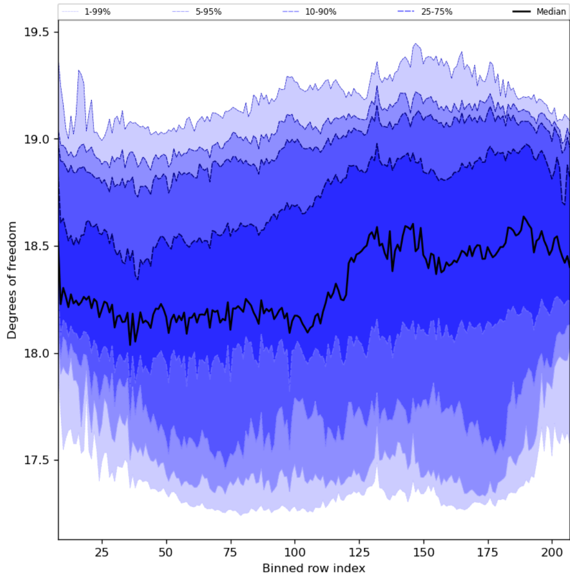
Figure 41: Along track statistics of “Degrees of freedom” for 2024-06-03 to 2024-06-05
