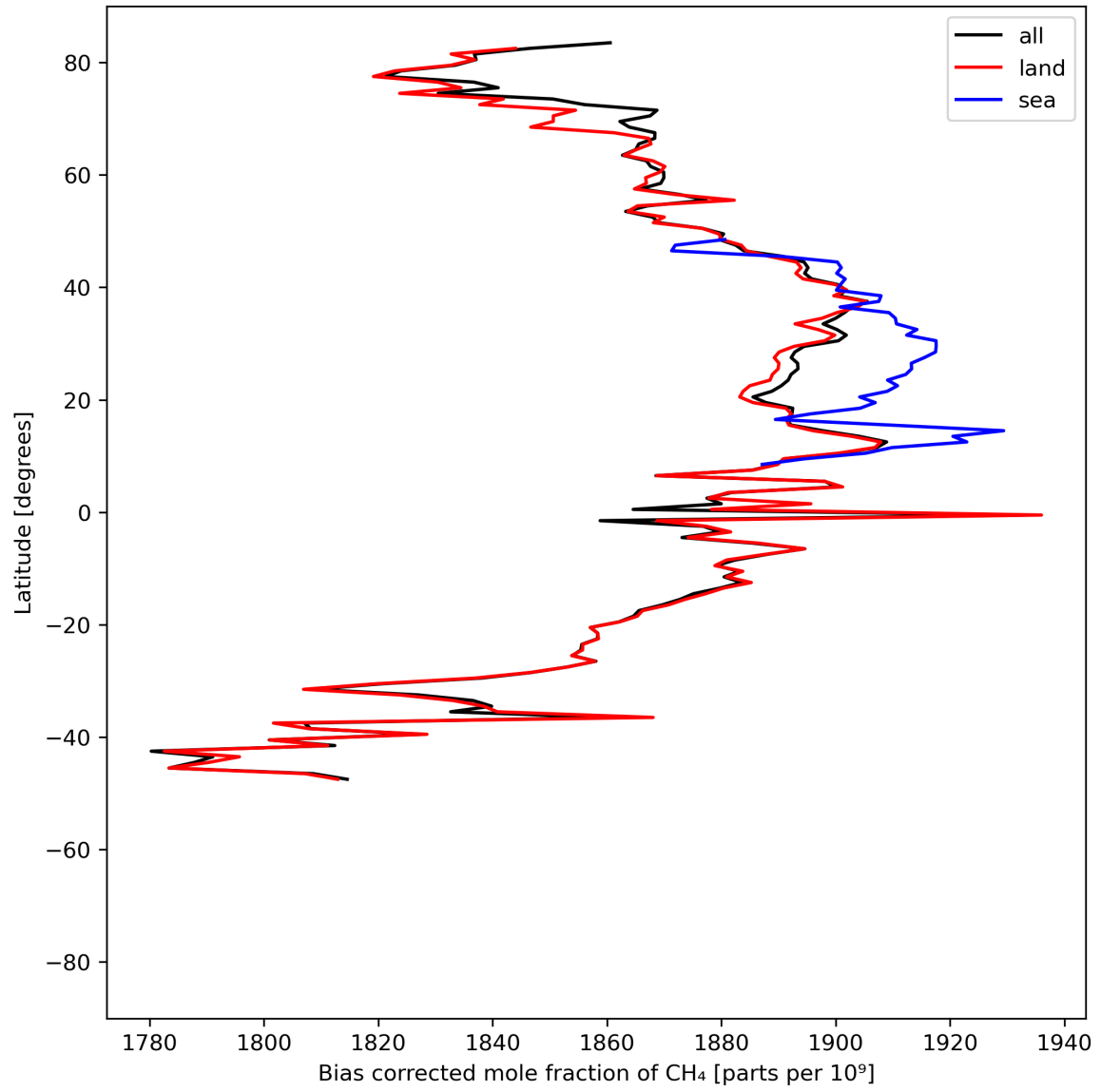
Figure 14: Zonal average of “Bias corrected mole fraction of CH 4 ” for 2024-06-03 to 2024-06-05.
