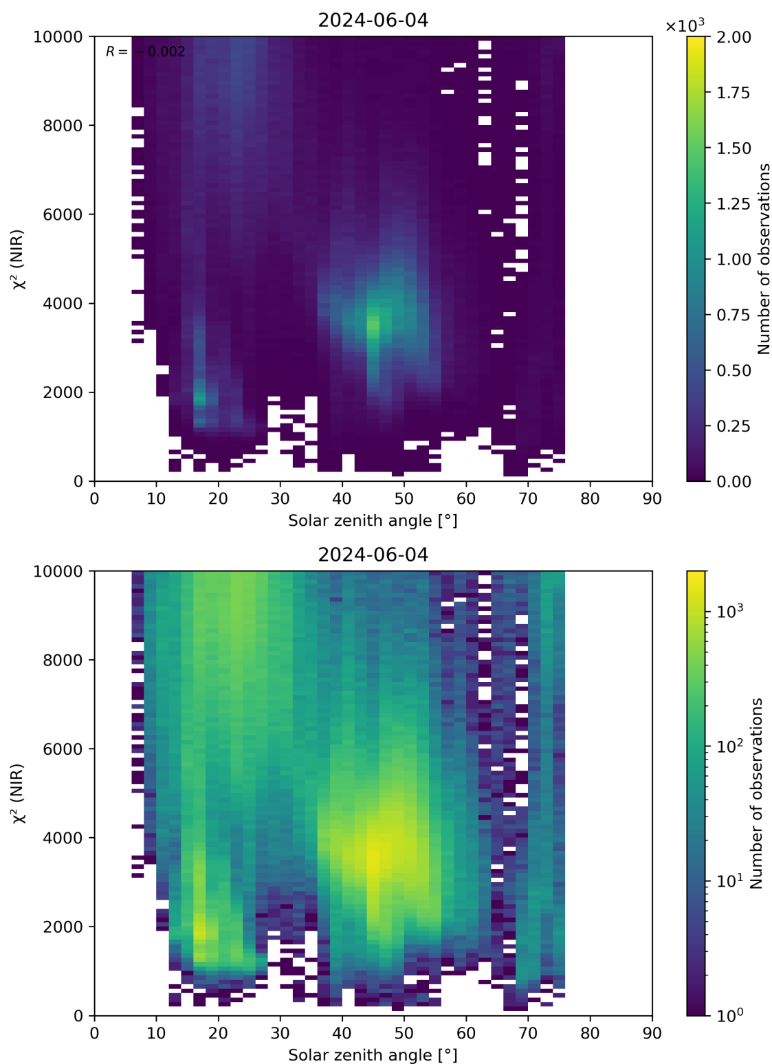
Figure 94: Scatter density plot of “Solar zenith angle” against “ \chi^2 (NIR)” for 2024-06-03 to 2024-06-05.
