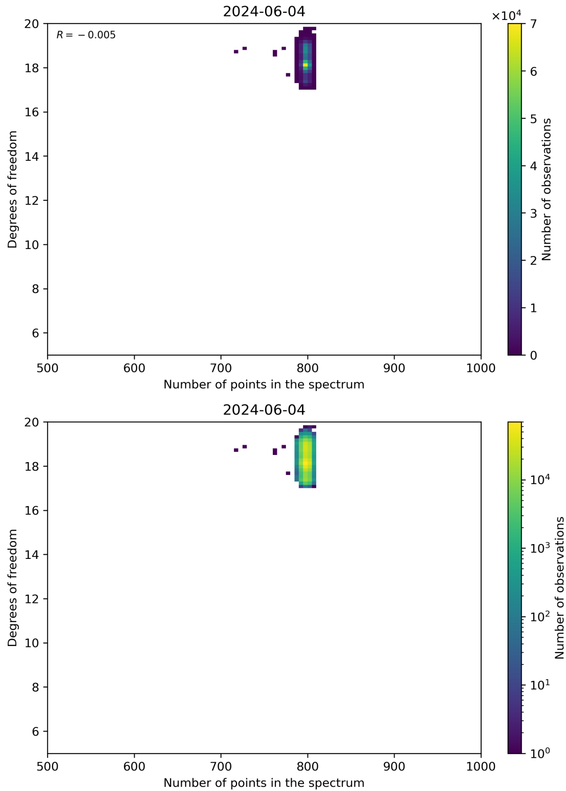
Figure 90: Scatter density plot of “Number of points in the spectrum” against “Degrees of freedom” for 2024-06-03 to 2024-06-05.
