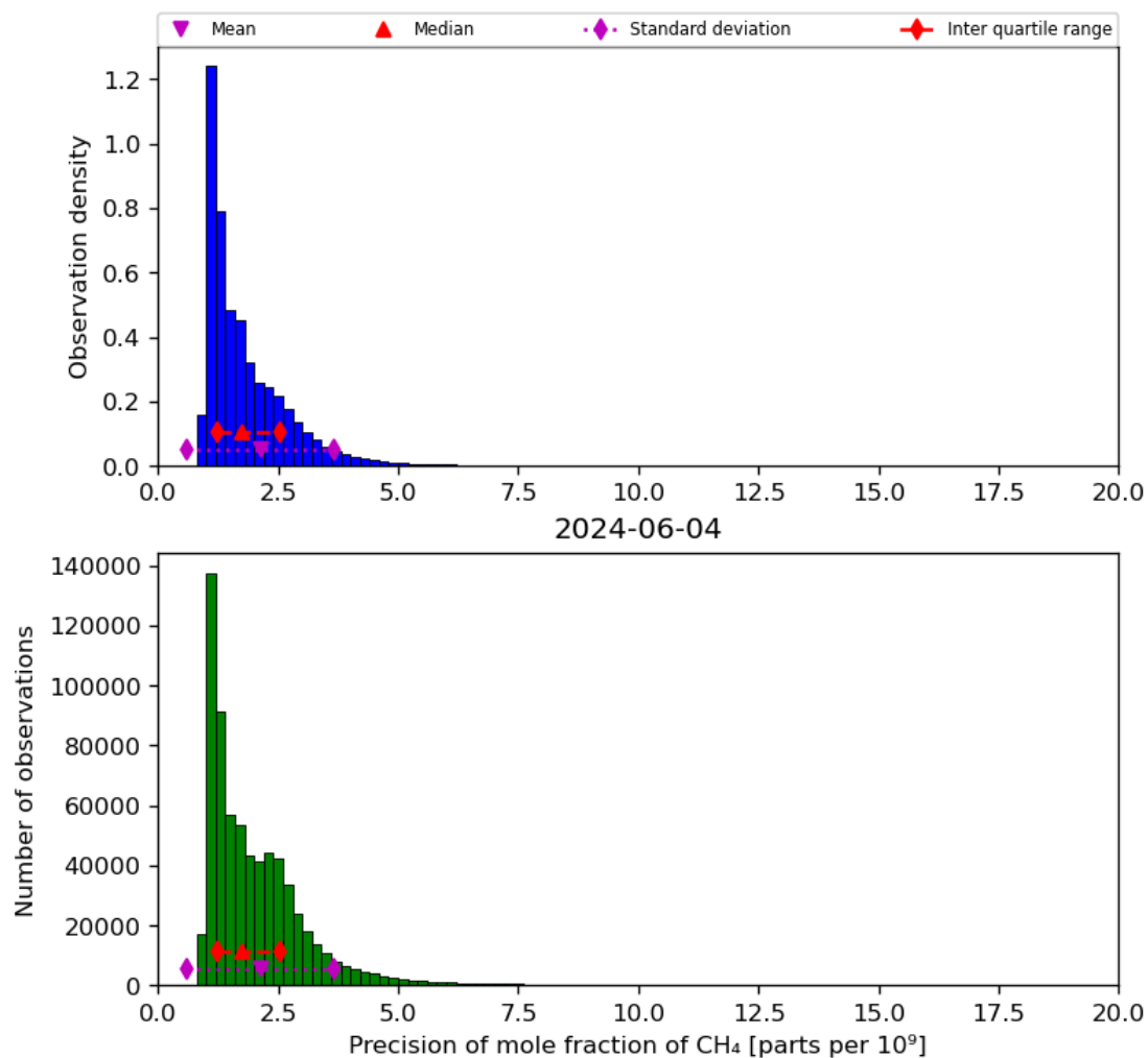
Figure 24: Histogram of “Precision of mole fraction of CH 4 ” for 2024-06-03 to 2024-06-05
