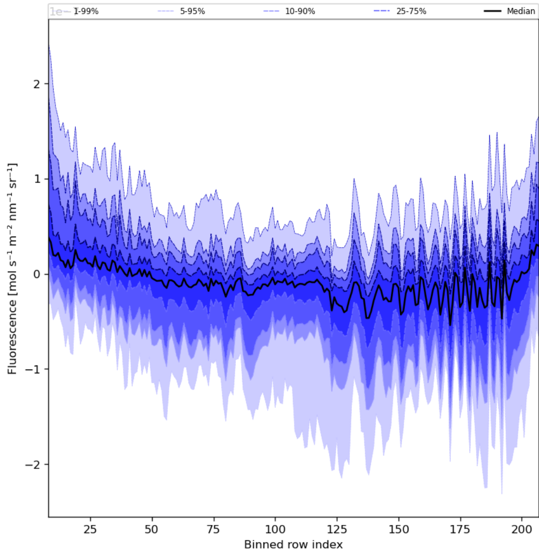
Figure 43: Along track statistics of “Fluorescence” for 2024-06-03 to 2024-06-05
