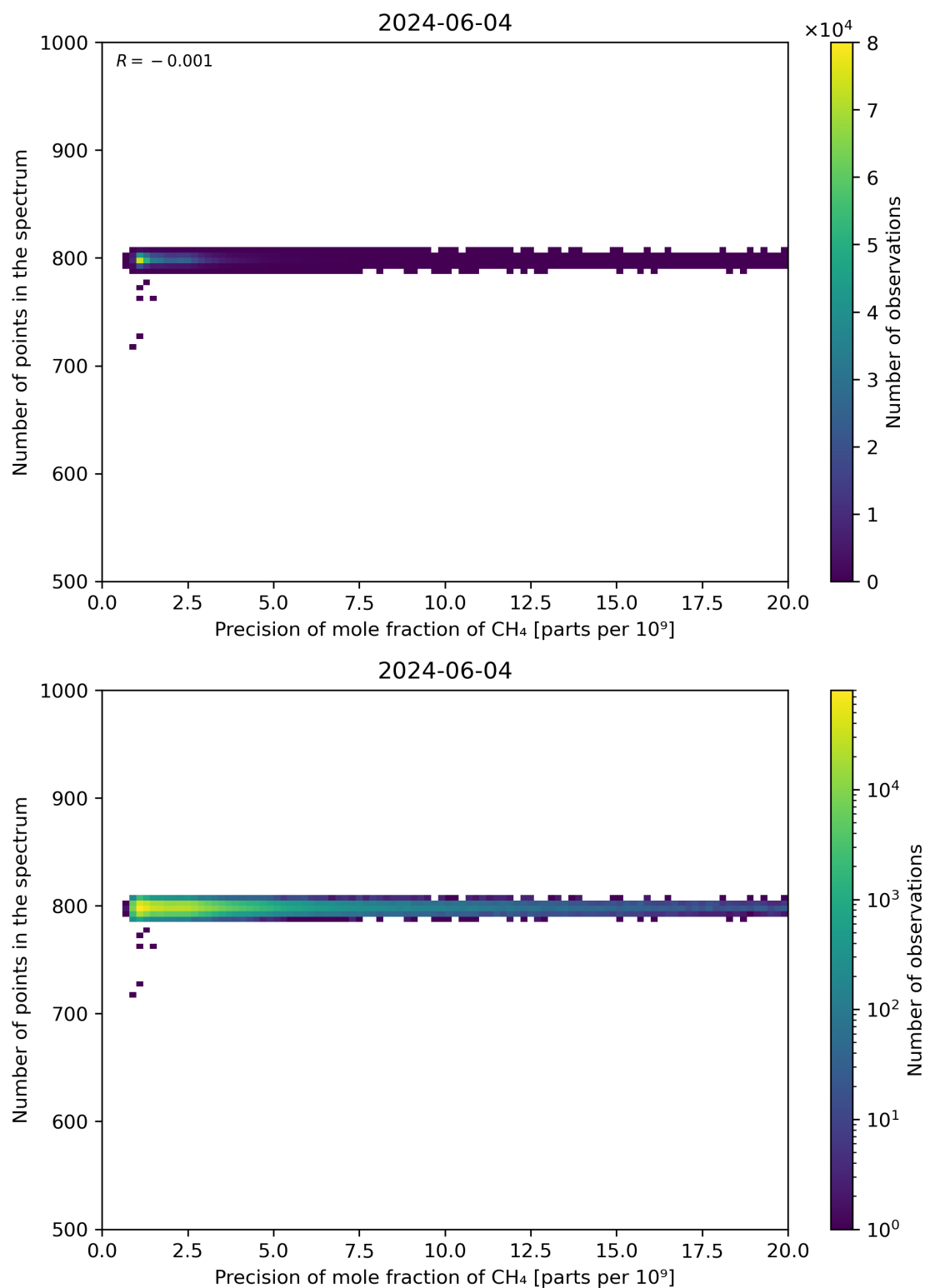
Figure 84: Scatter density plot of “Precision of mole fraction of CH 4 ” against “Number of points in the spectrum” for 2024-06-03 to 2024-06-05.
