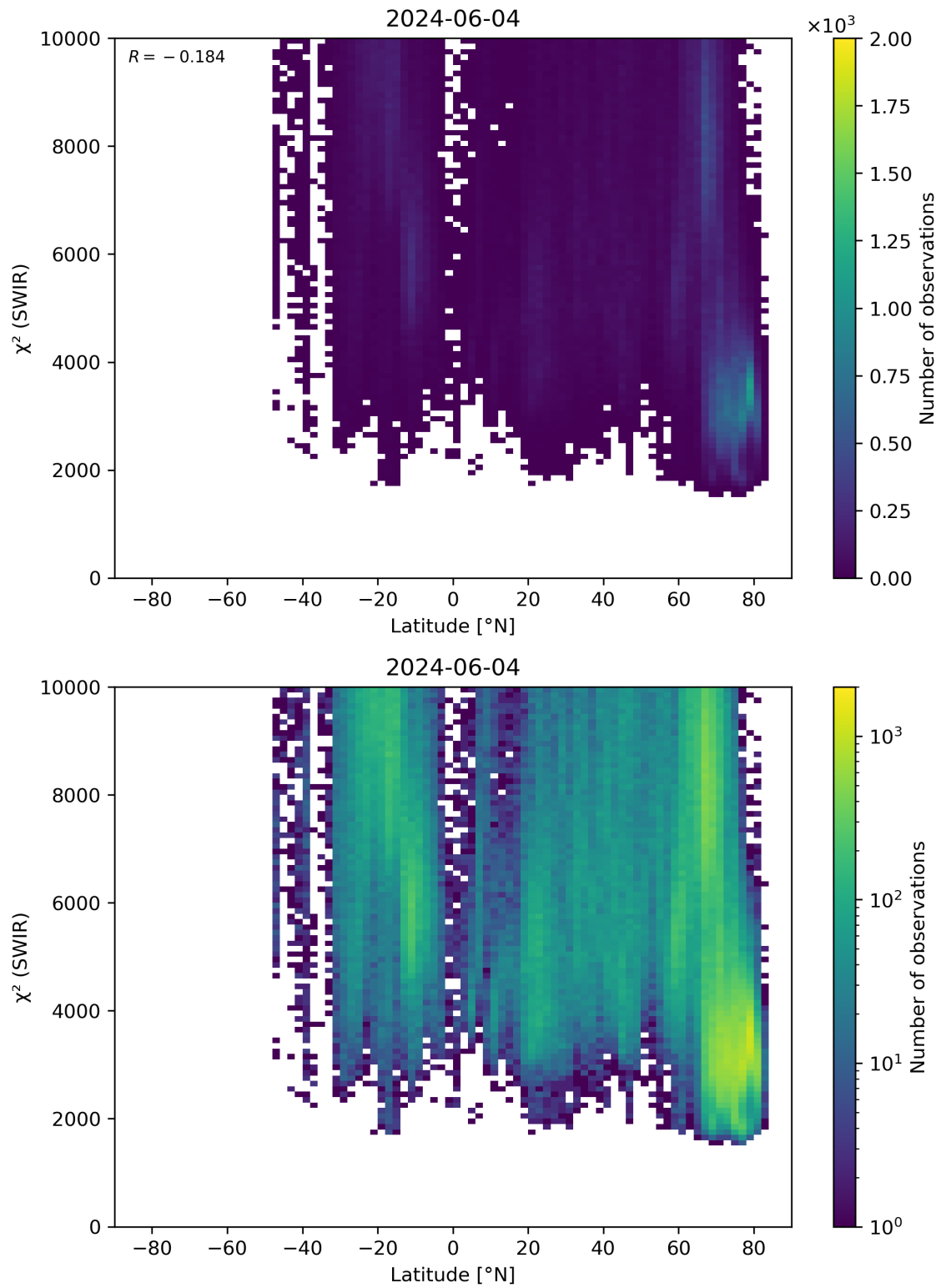
Figure 54: Scatter density plot of “Latitude” against “ \chi^2 (SWIR)” for 2024-06-03 to 2024-06-05.
