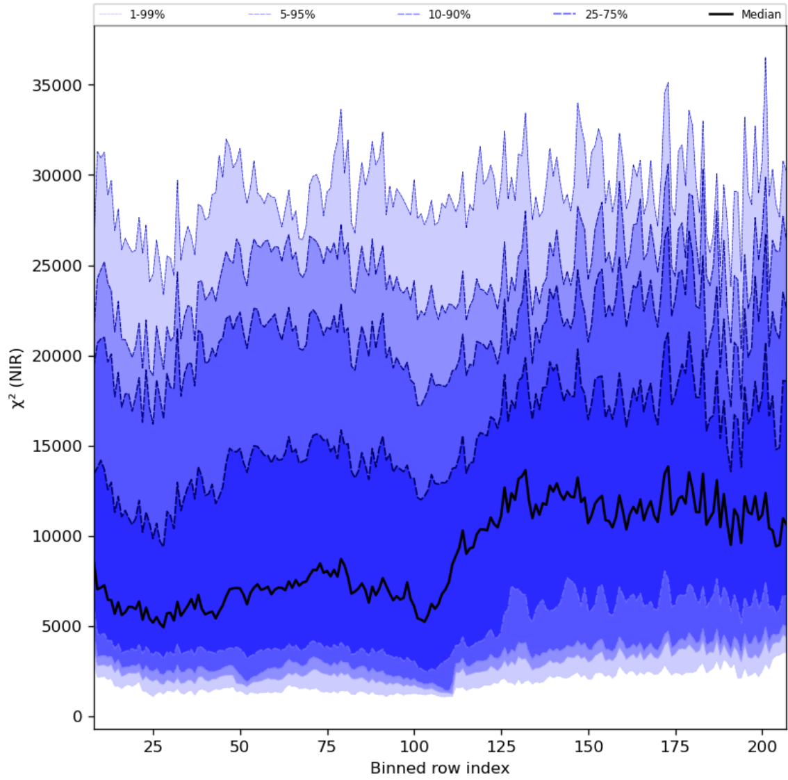
Figure 40: Along track statistics of " \chi^2 (NIR)" for 2024-06-03 to 2024-06-05
