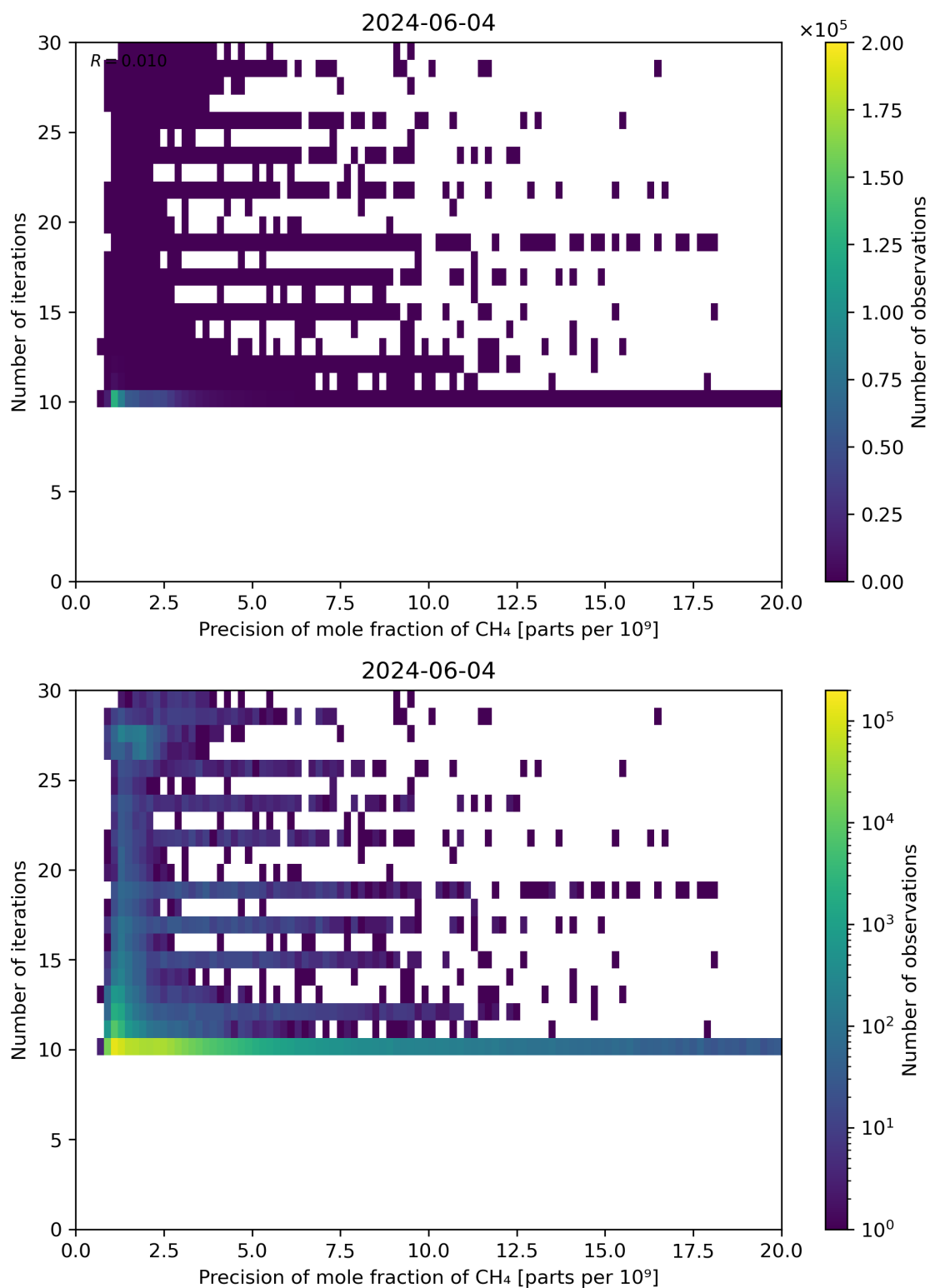
Figure 83: Scatter density plot of “Precision of mole fraction of CH 4 ” against “Number of iterations” for 2024-06-03 to 2024-06-05.
