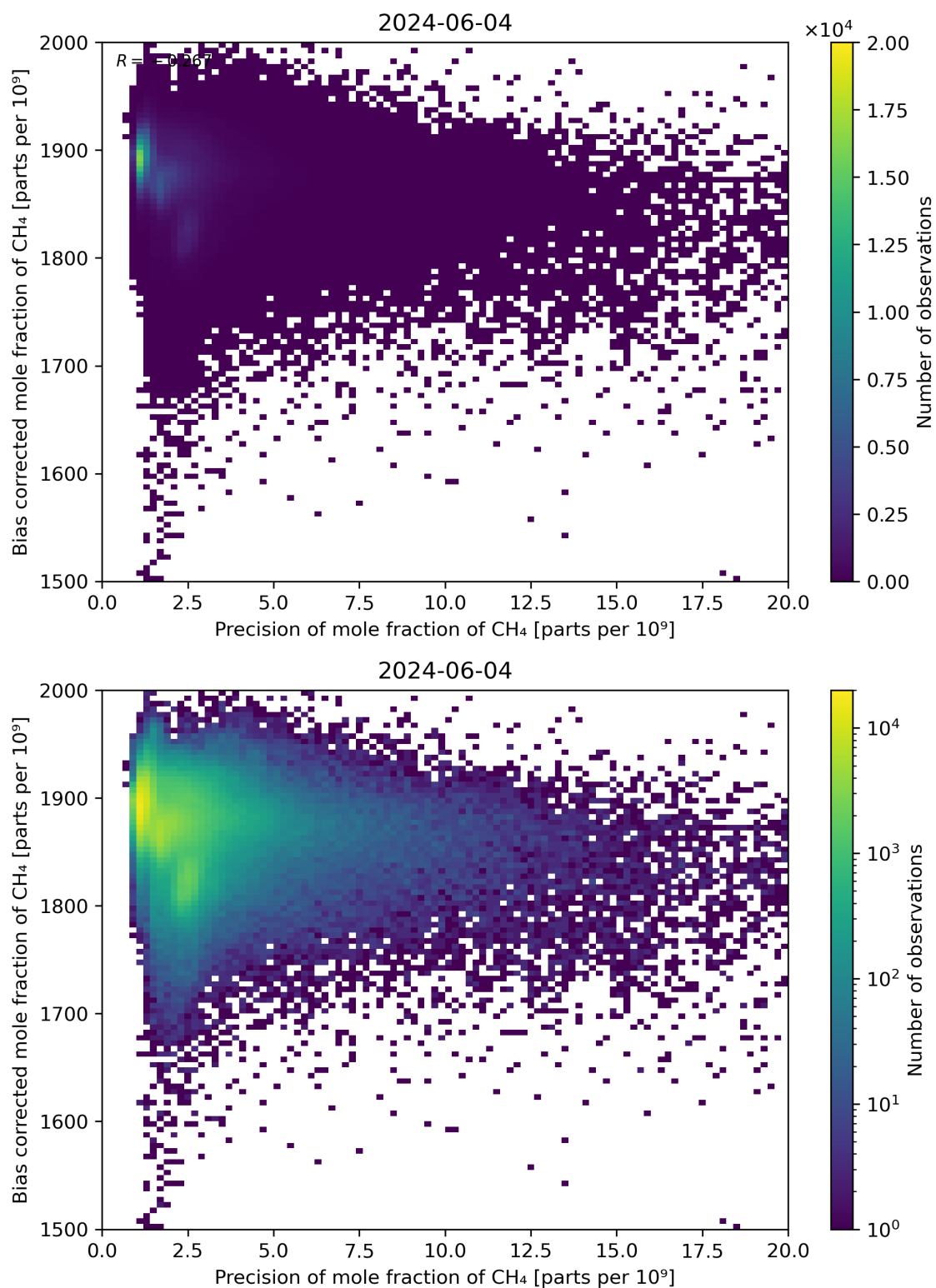
Figure 82: Scatter density plot of “Precision of mole fraction of \text{CH}_4 ” against “Bias corrected mole fraction of \text{CH}_4 ” for 2024-06-03 to 2024-06-05.
