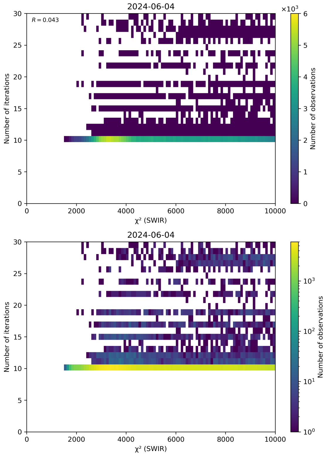
Figure 50: Scatter density plot of “ \chi^2 (SWIR)” against “Number of iterations” for 2024-06-03 to 2024-06-05.
