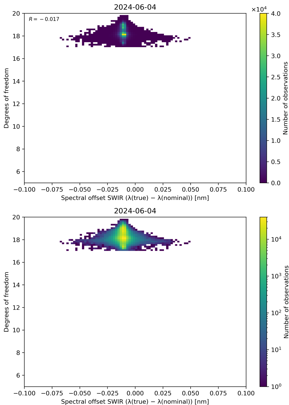
Figure 119: Scatter density plot of “Spectral offset SWIR ( \lambda(\text{true}) - \lambda(\text{nominal}) )” against “Degrees of freedom” for 2024-06-03 to 2024-06-05.
