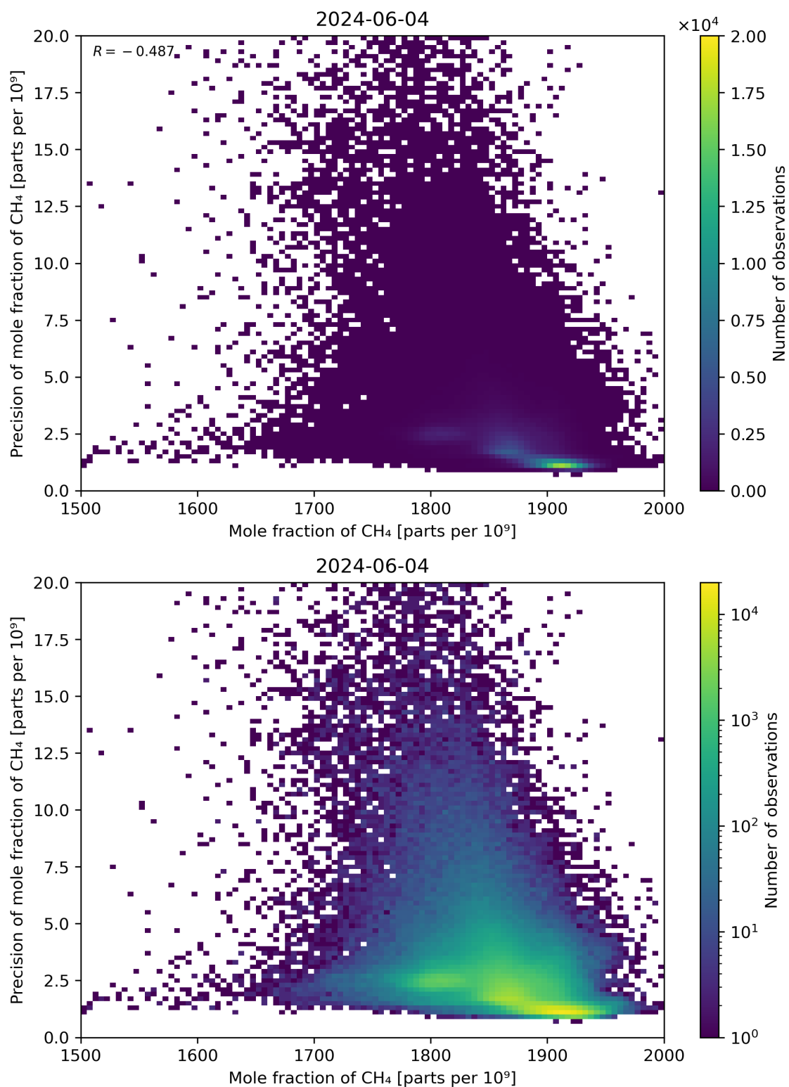
Figure 75: Scatter density plot of “Mole fraction of CH 4 ” against “Precision of mole fraction of CH 4 ” for 2024-06-03 to 2024-06-05.
