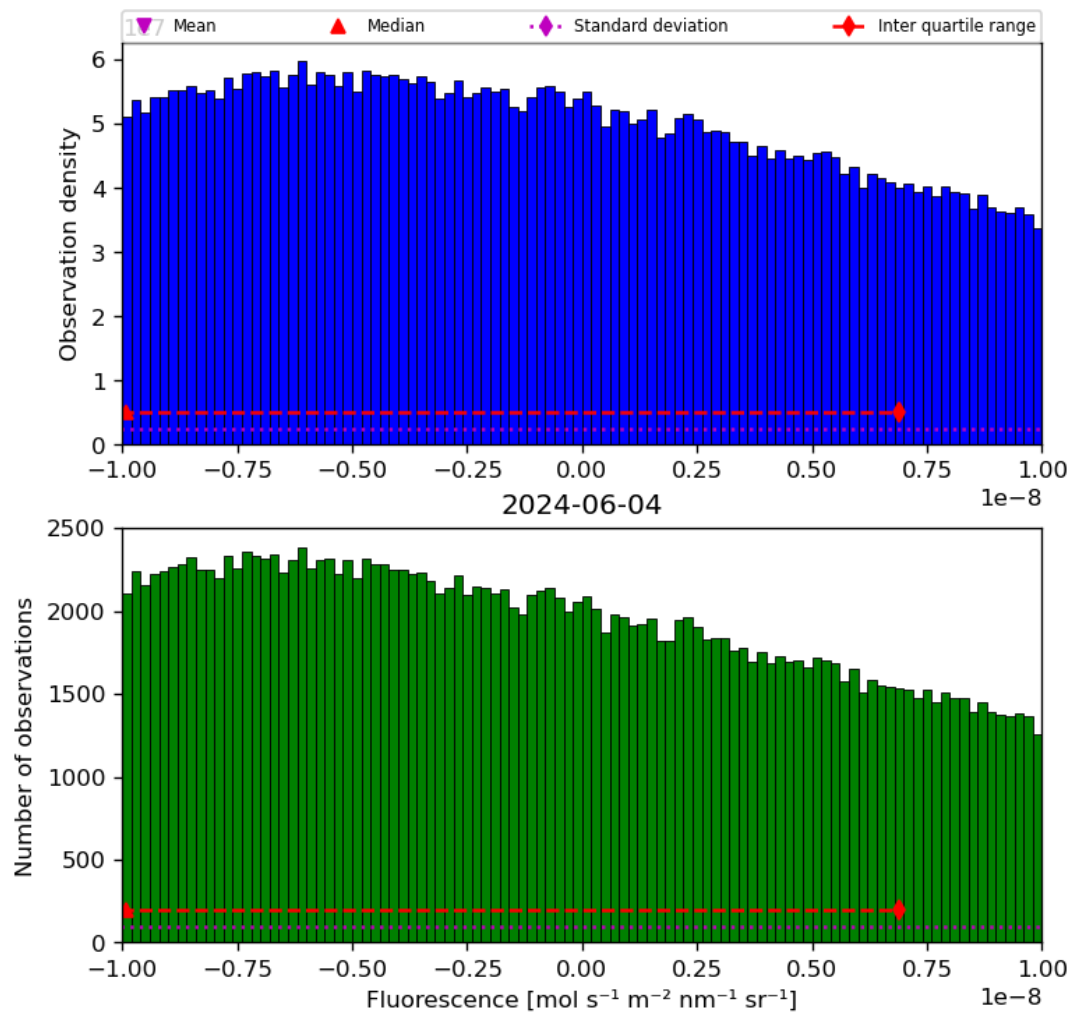
Figure 32: Histogram of “Fluorescence” for 2024-06-03 to 2024-06-05
