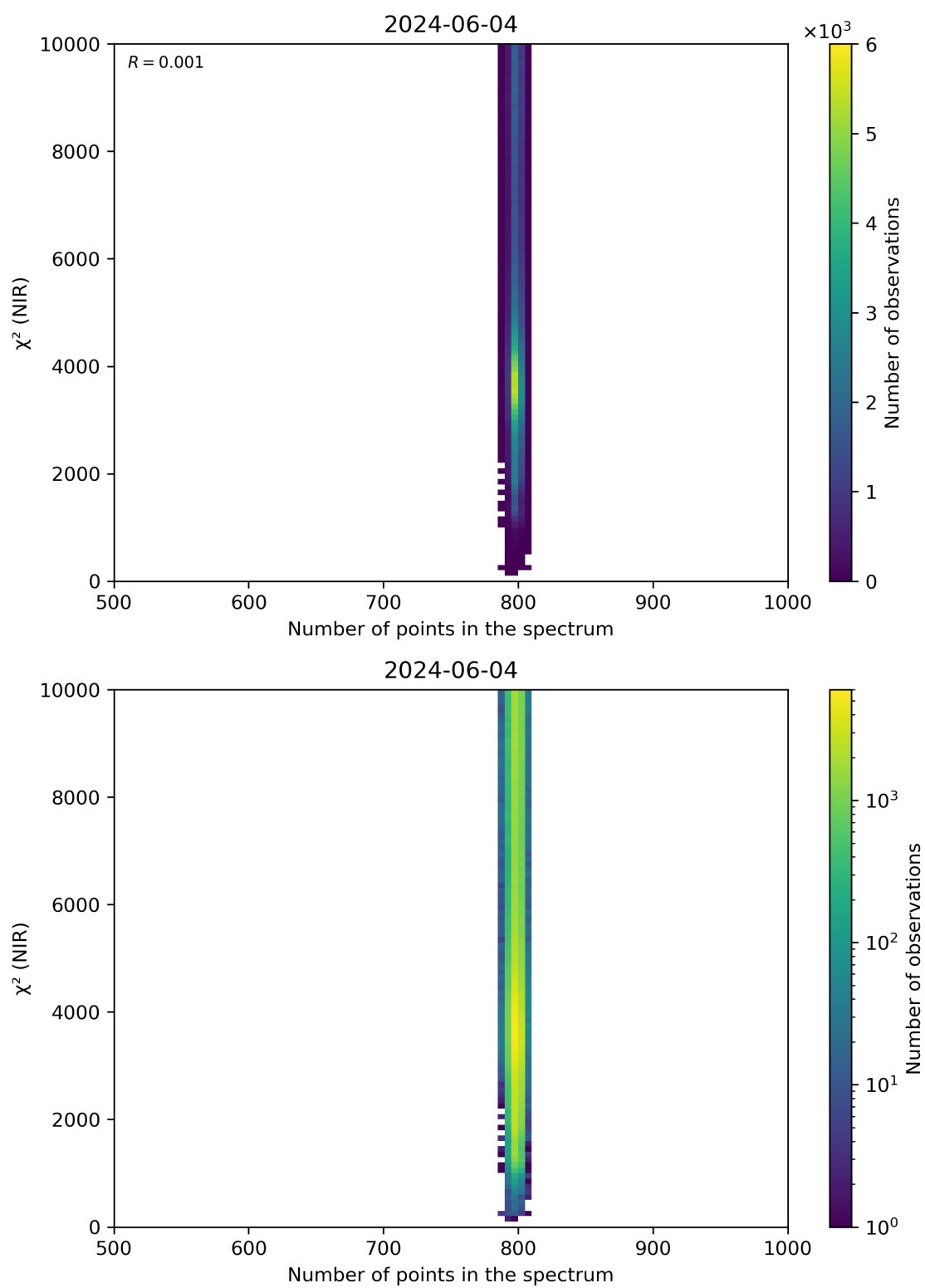
Figure 88: Scatter density plot of “Number of points in the spectrum” against “ \chi^2 (NIR)” for 2024-06-03 to 2024-06-05.
