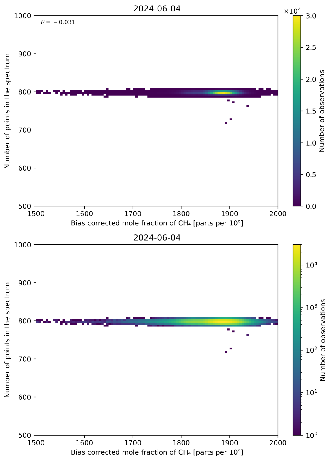
Figure 68: Scatter density plot of “Bias corrected mole fraction of CH 4 ” against “Number of points in the spectrum” for 2024-06-03 to 2024-06-05.
