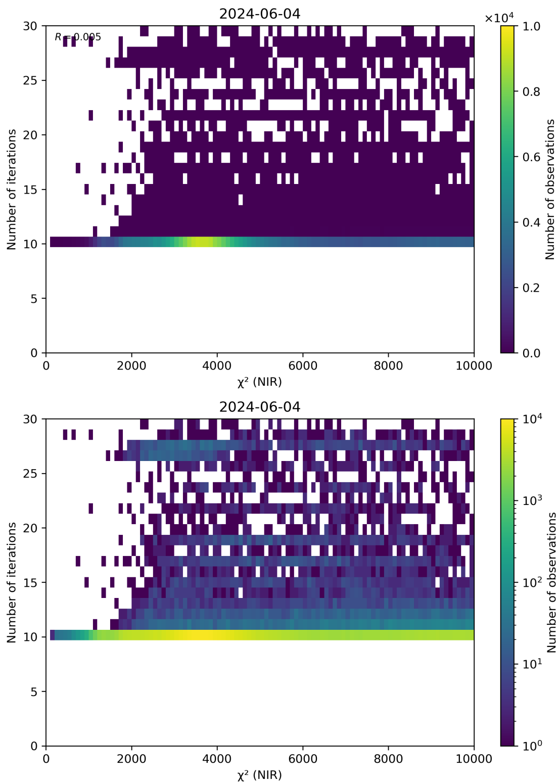
Figure 46: Scatter density plot of “ \chi^2 (NIR)” against “Number of iterations” for 2024-06-03 to 2024-06-05.
