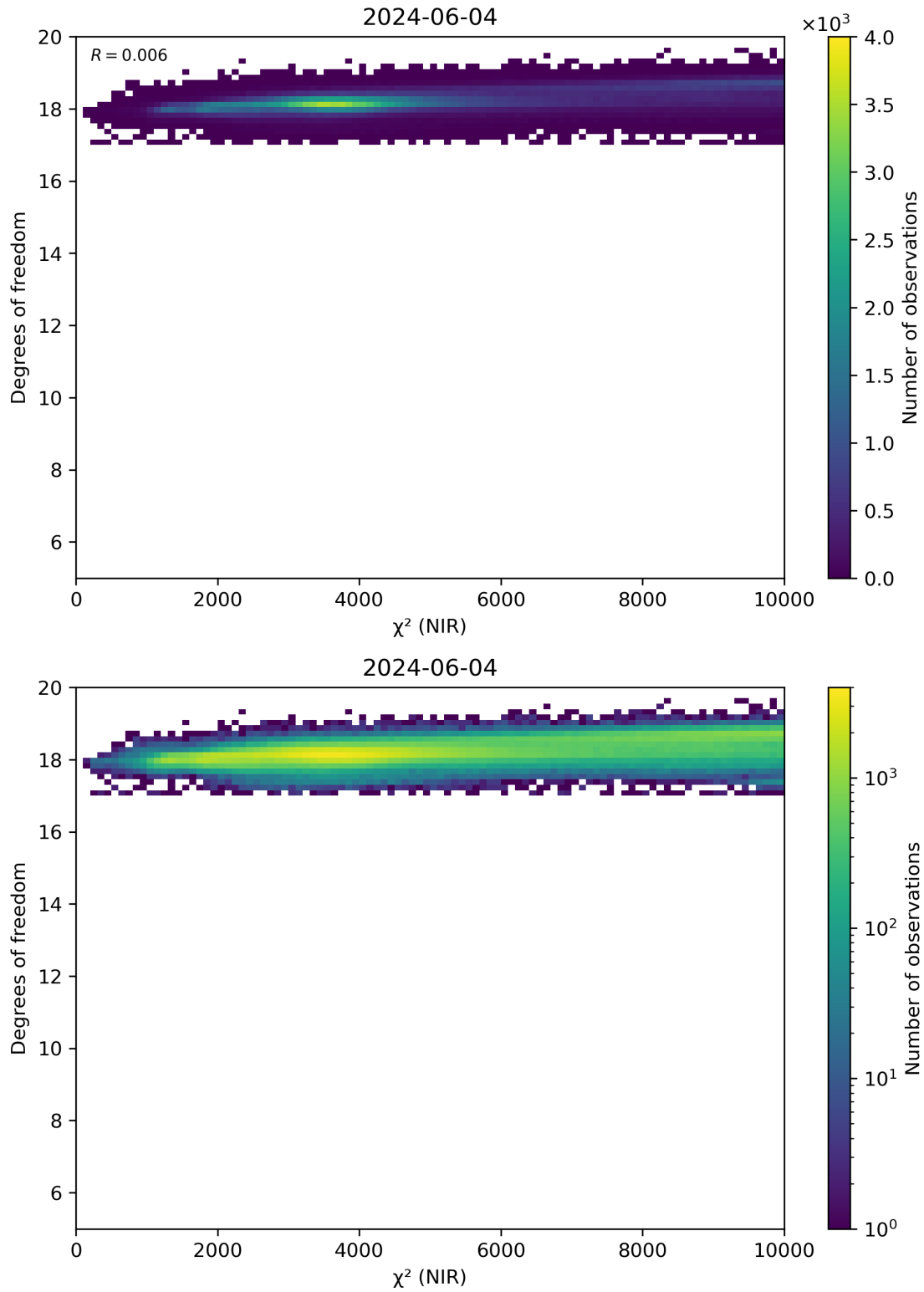
Figure 44: Scatter density plot of “ \chi^2 (NIR)” against “Degrees of freedom” for 2024-06-03 to 2024-06-05.
