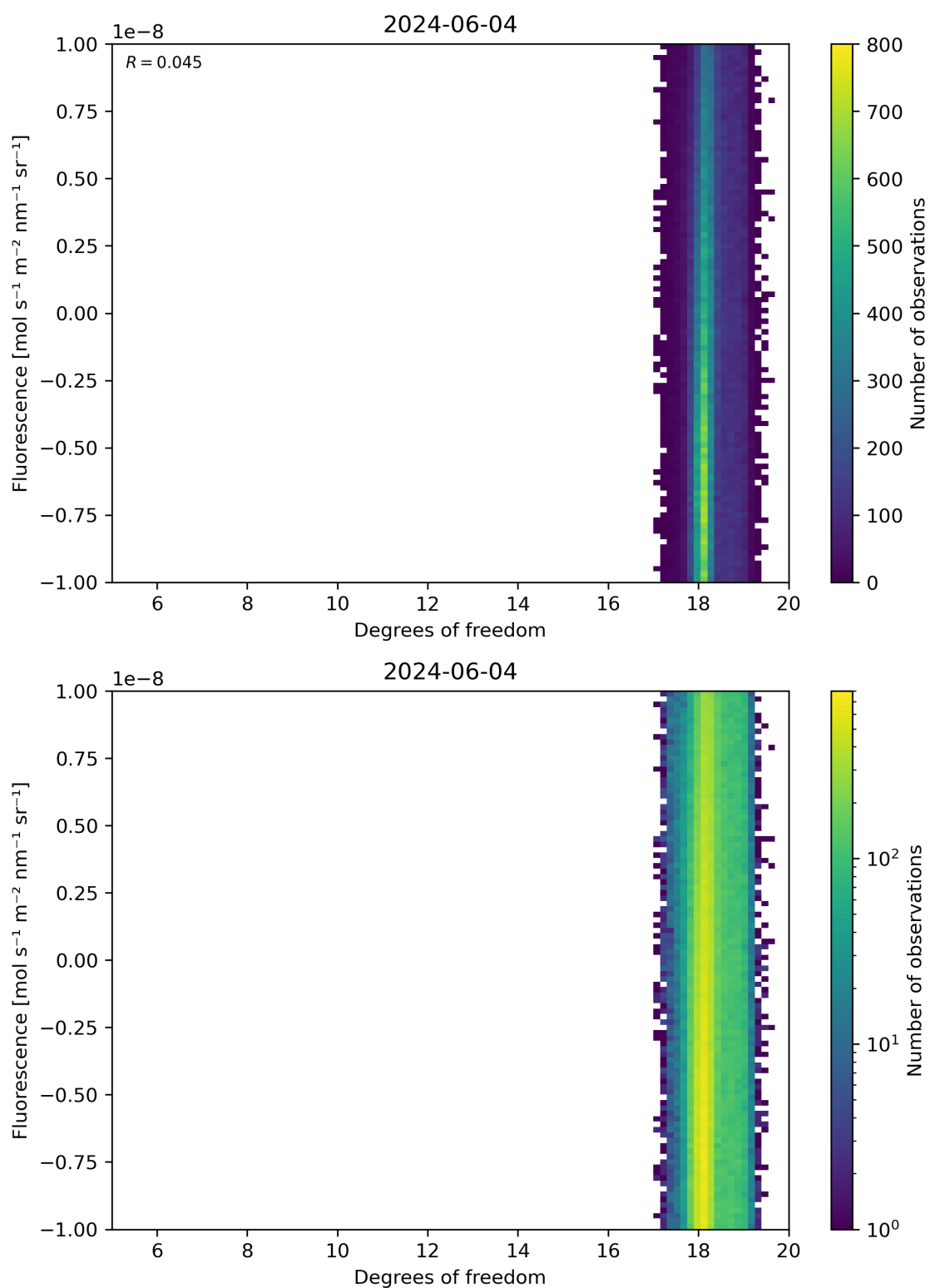
Figure 51: Scatter density plot of “Degrees of freedom” against “Fluorescence” for 2024-06-03 to 2024-06-05.
