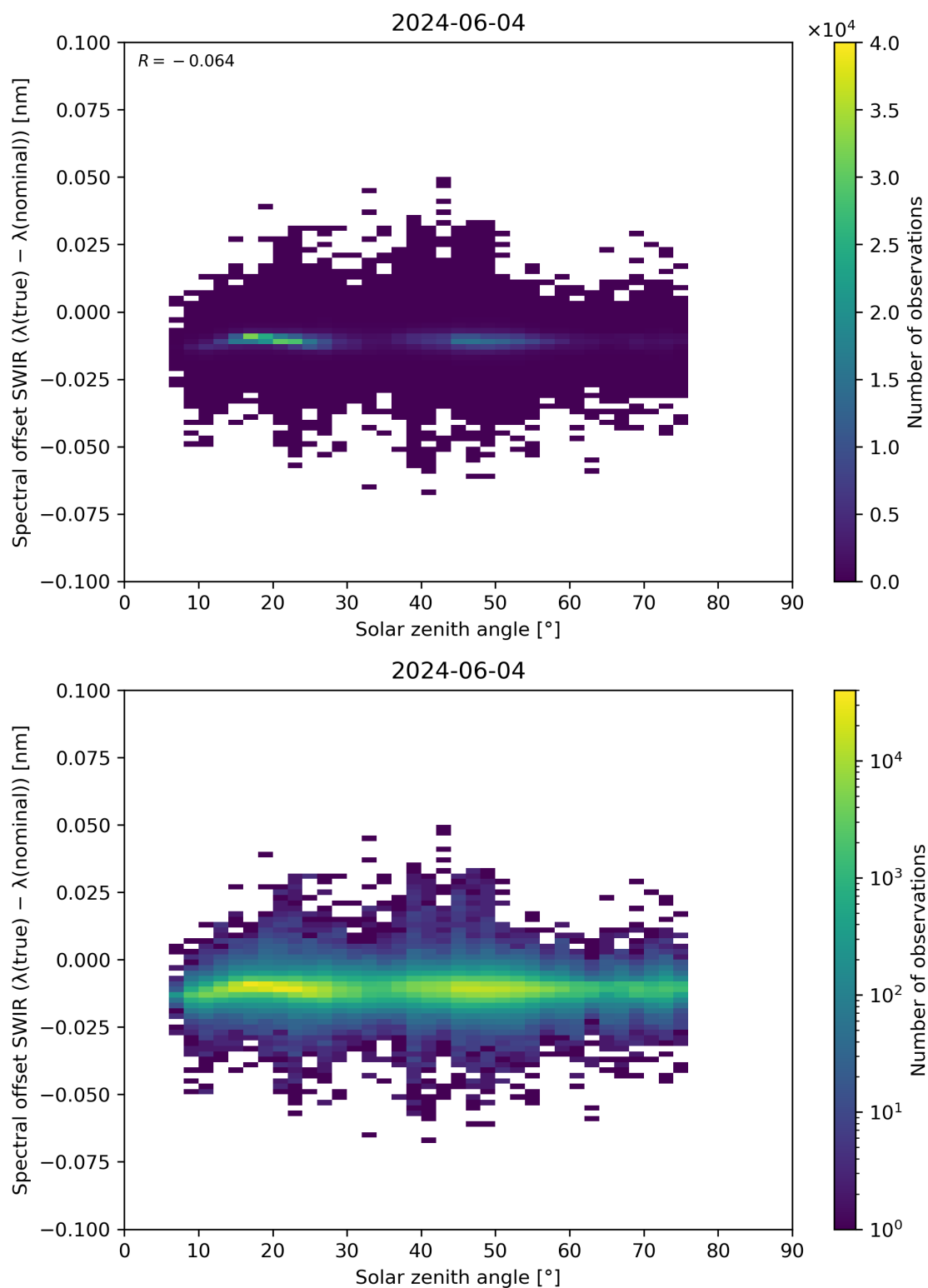
Figure 104: Scatter density plot of “Solar zenith angle” against “Spectral offset SWIR ( \lambda(\text{true}) - \lambda(\text{nominal}) )” for 2024-06-03 to 2024-06-05.
