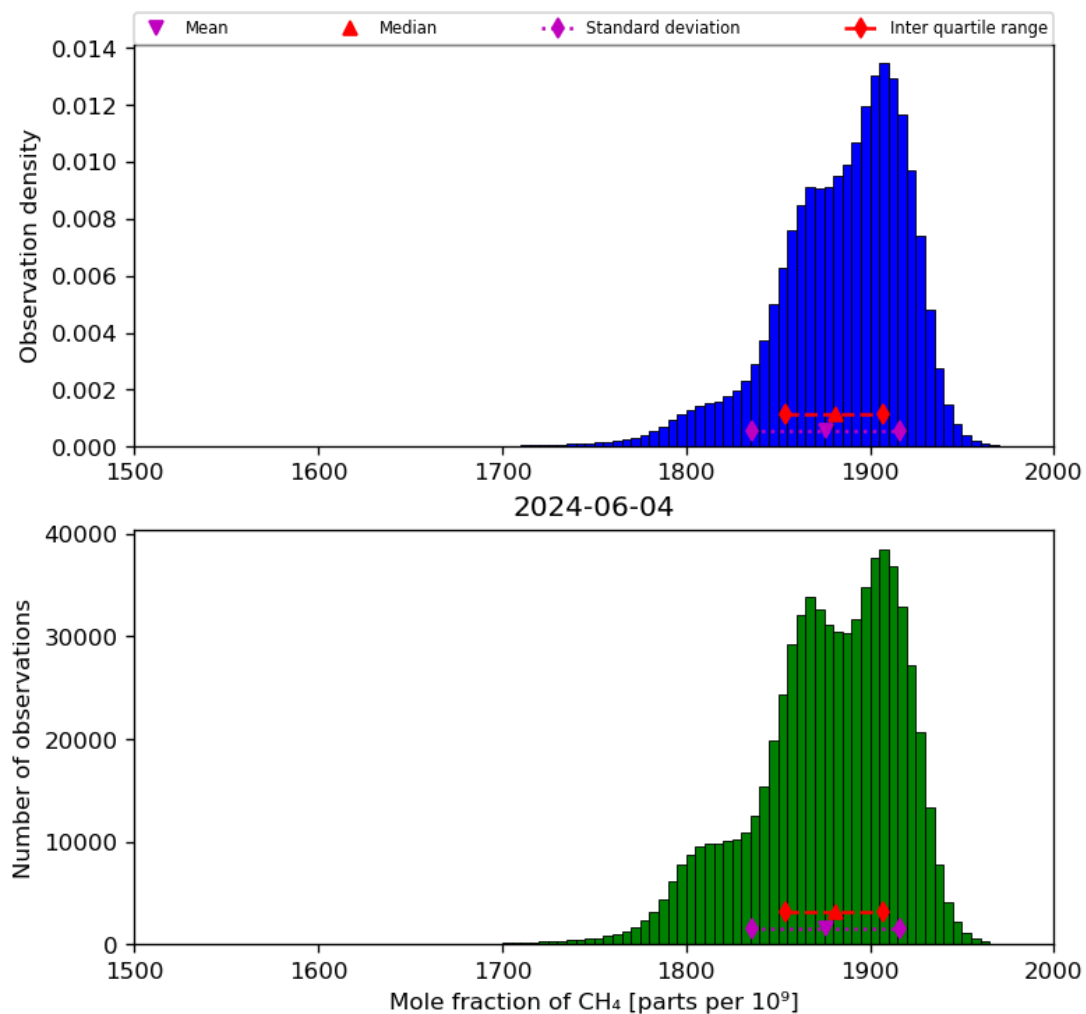
Figure 23: Histogram of “Mole fraction of CH 4 ” for 2024-06-03 to 2024-06-05
