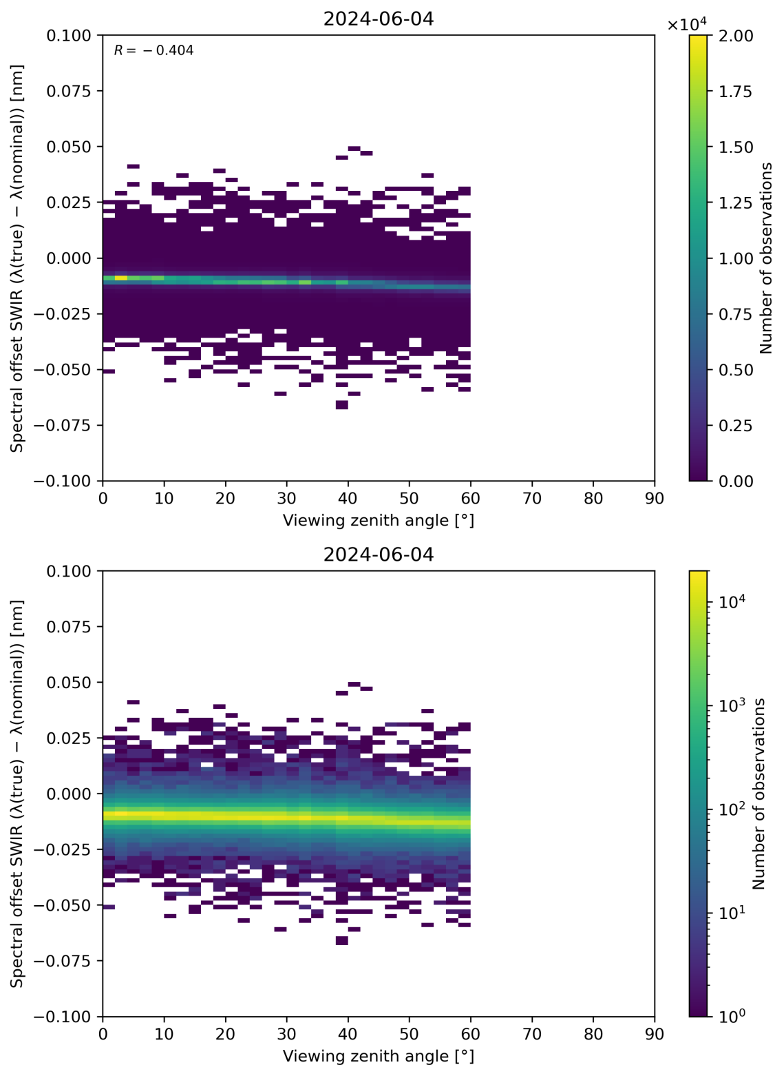
Figure 116: Scatter density plot of “Viewing zenith angle” against “Spectral offset SWIR ( \lambda(\text{true}) - \lambda(\text{nominal}) )” for 2024-06-03 to 2024-06-05.
