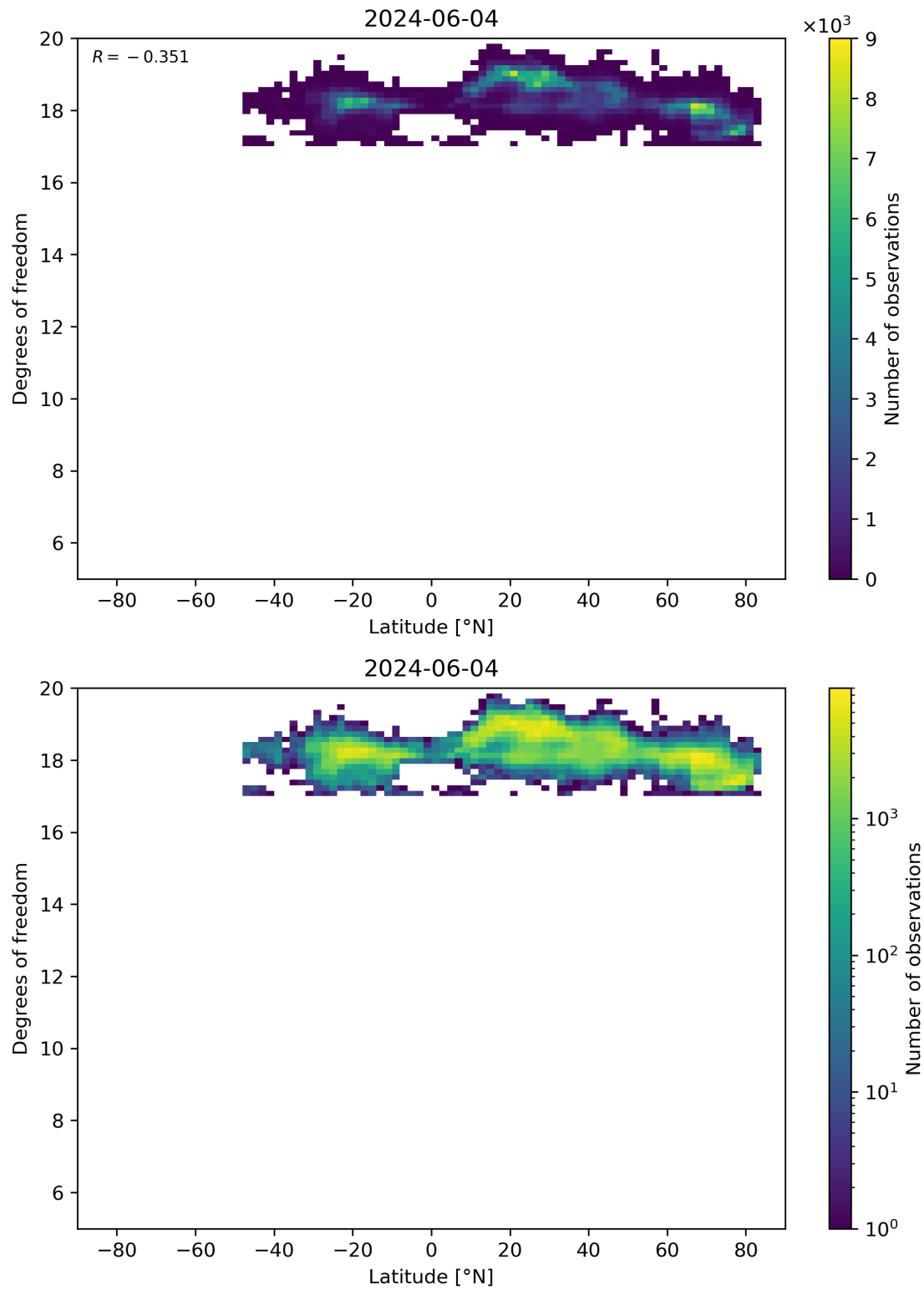
Figure 55: Scatter density plot of “Latitude” against “Degrees of freedom” for 2024-06-03 to 2024-06-05.
