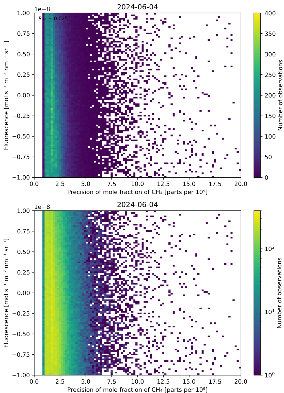
Figure 81: Scatter density plot of “Precision of mole fraction of \text{CH}_4 ” against “Fluorescence” for 2024-06-03 to 2024-06-05.
