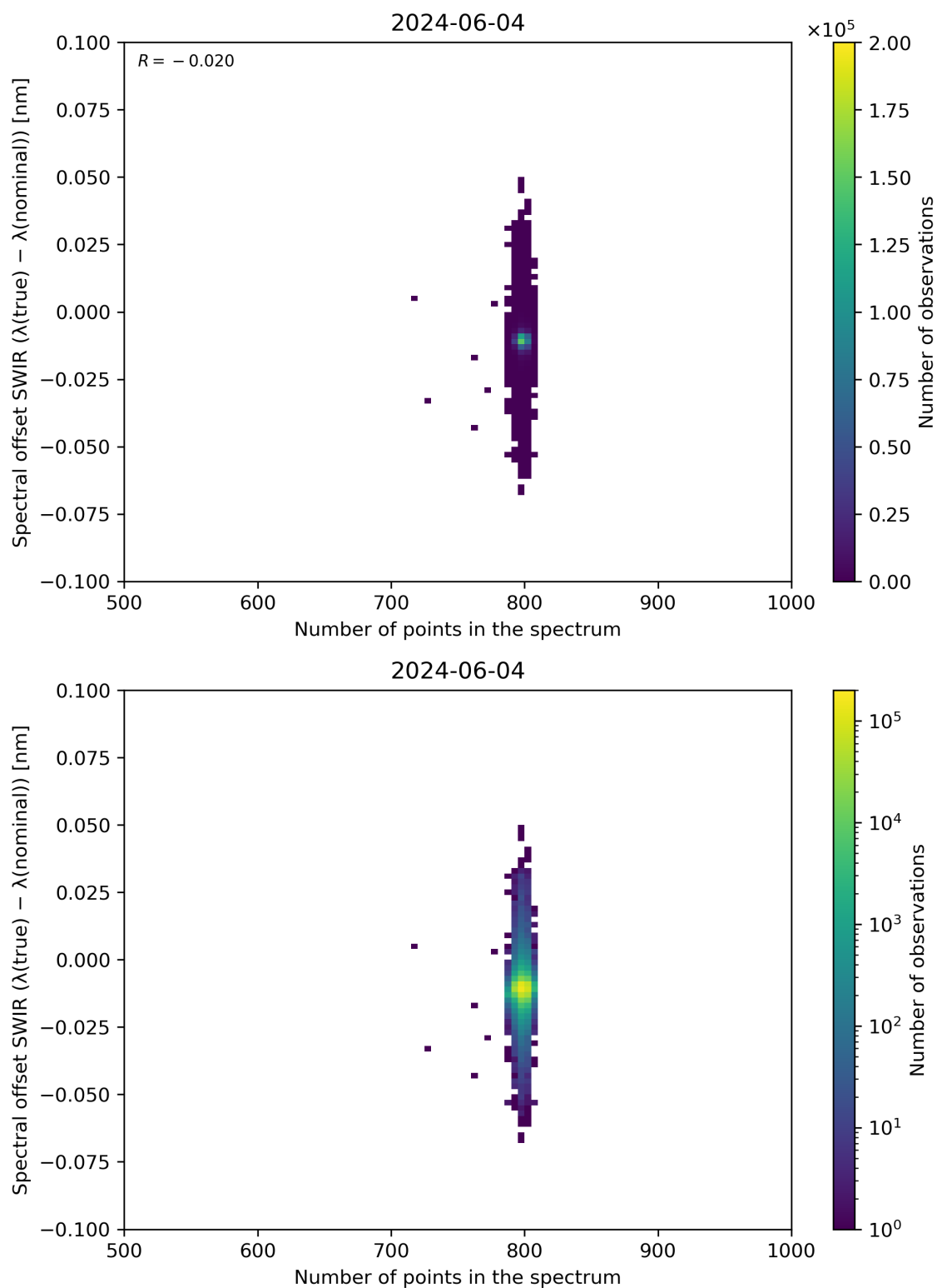
Figure 93: Scatter density plot of “Number of points in the spectrum” against “Spectral offset SWIR ( \lambda(\text{true}) - \lambda(\text{nominal}) )” for 2024-06-03 to 2024-06-05.
