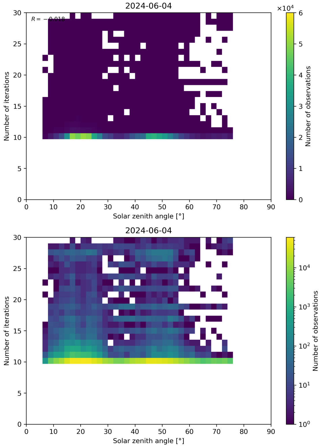
Figure 102: Scatter density plot of “Solar zenith angle” against “Number of iterations” for 2024-06-03 to 2024-06-05.
