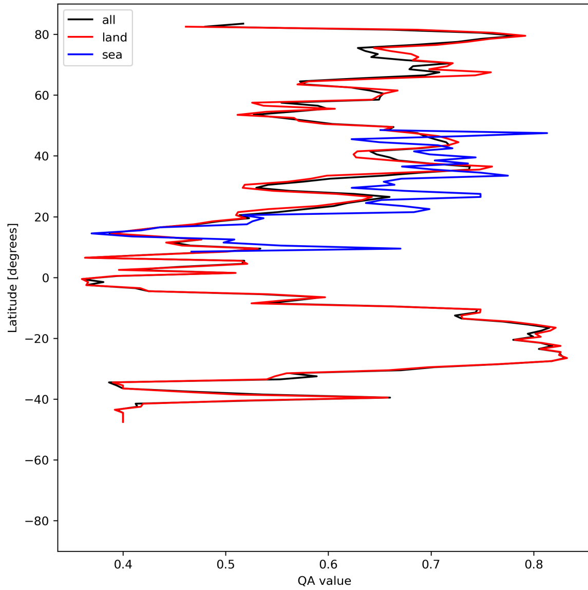
Figure 11: Zonal average of “QA value” for 2024-06-03 to 2024-06-05.
