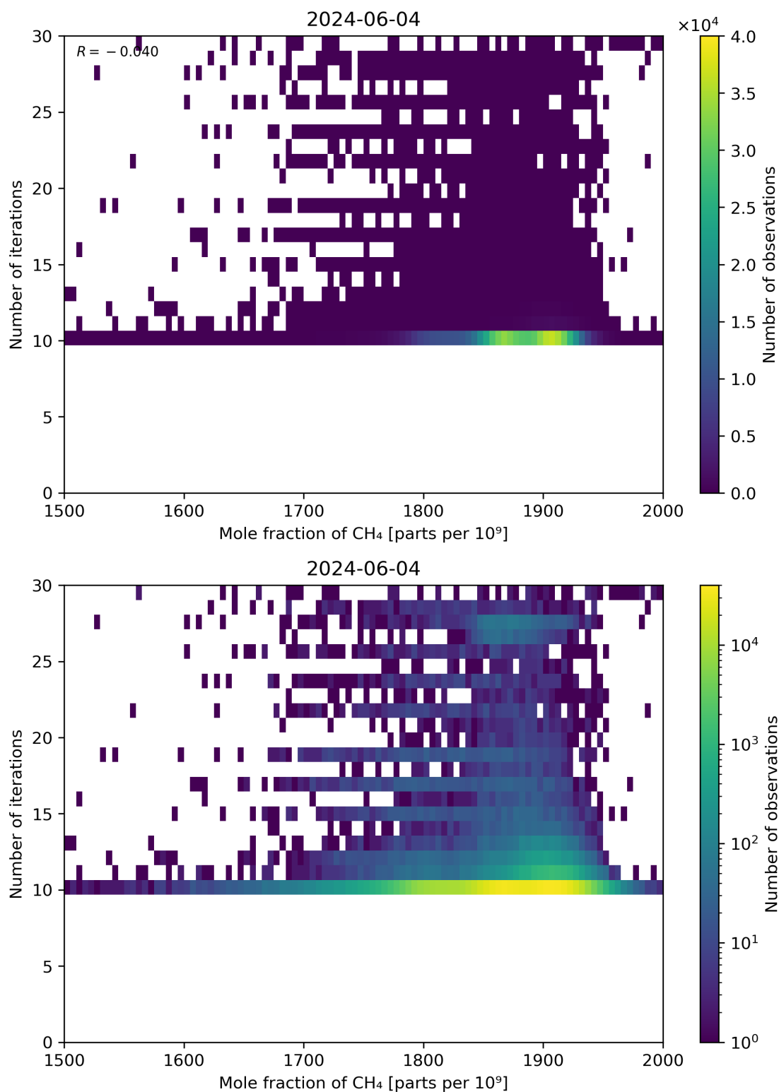
Figure 76: Scatter density plot of “Mole fraction of CH 4 ” against “Number of iterations” for 2024-06-03 to 2024-06-05.
