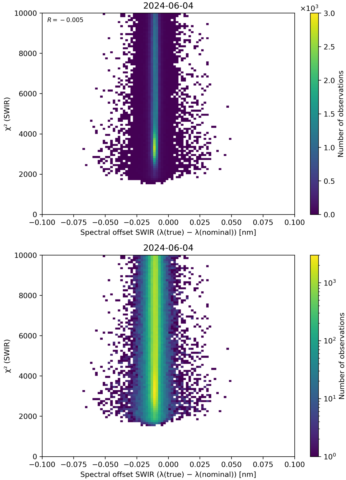
Figure 118: Scatter density plot of “Spectral offset SWIR ( \lambda(\text{true}) - \lambda(\text{nominal}) )” against “ \chi^2 (SWIR)” for 2024-06-03 to 2024-06-05.
