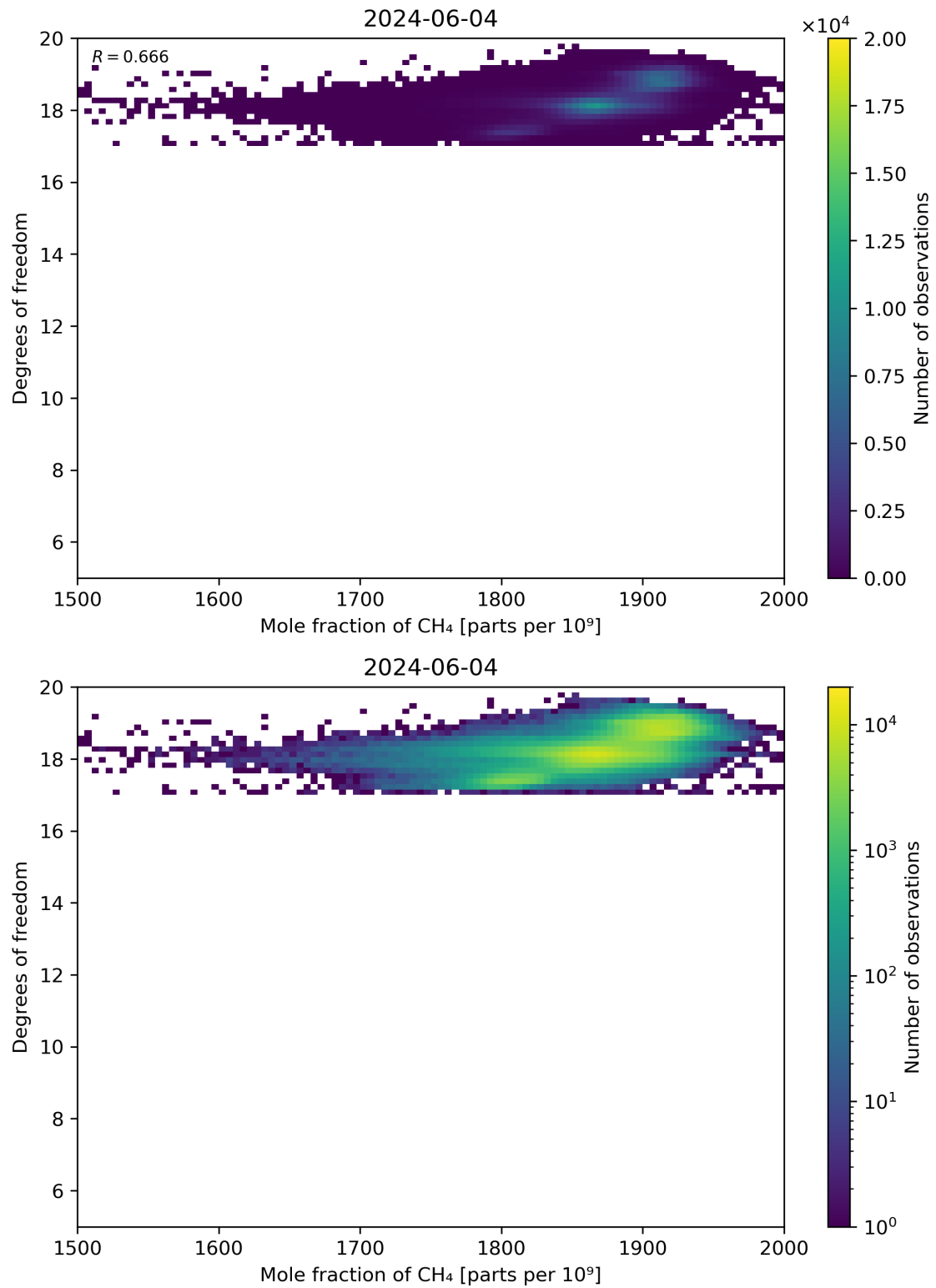
Figure 72: Scatter density plot of “Mole fraction of CH 4 ” against “Degrees of freedom” for 2024-06-03 to 2024-06-05.
