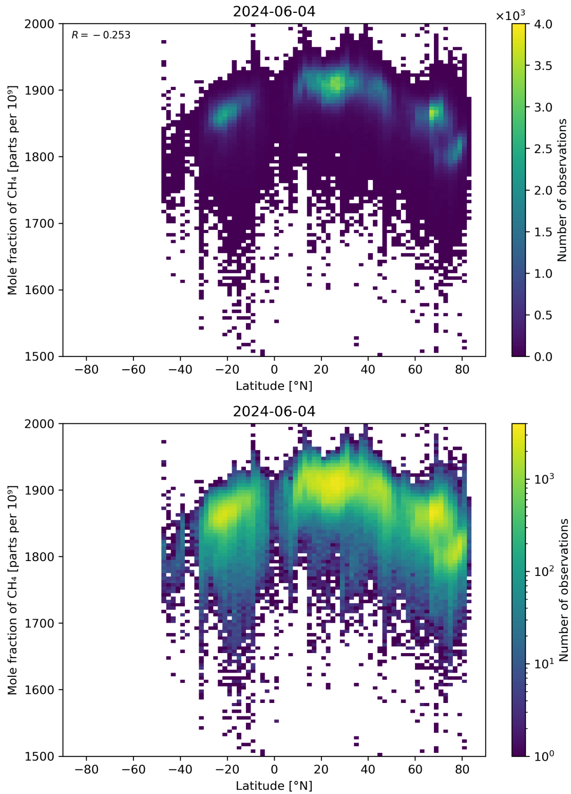
Figure 57: Scatter density plot of “Latitude” against “Mole fraction of CH 4 ” for 2024-06-03 to 2024-06-05.
