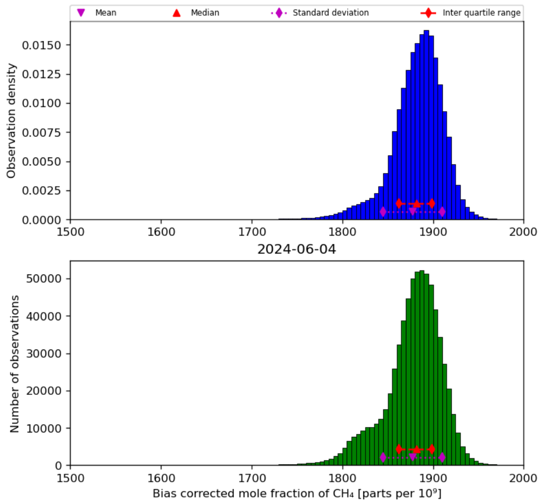
Figure 25: Histogram of “Bias corrected mole fraction of CH 4 ” for 2024-06-03 to 2024-06-05
