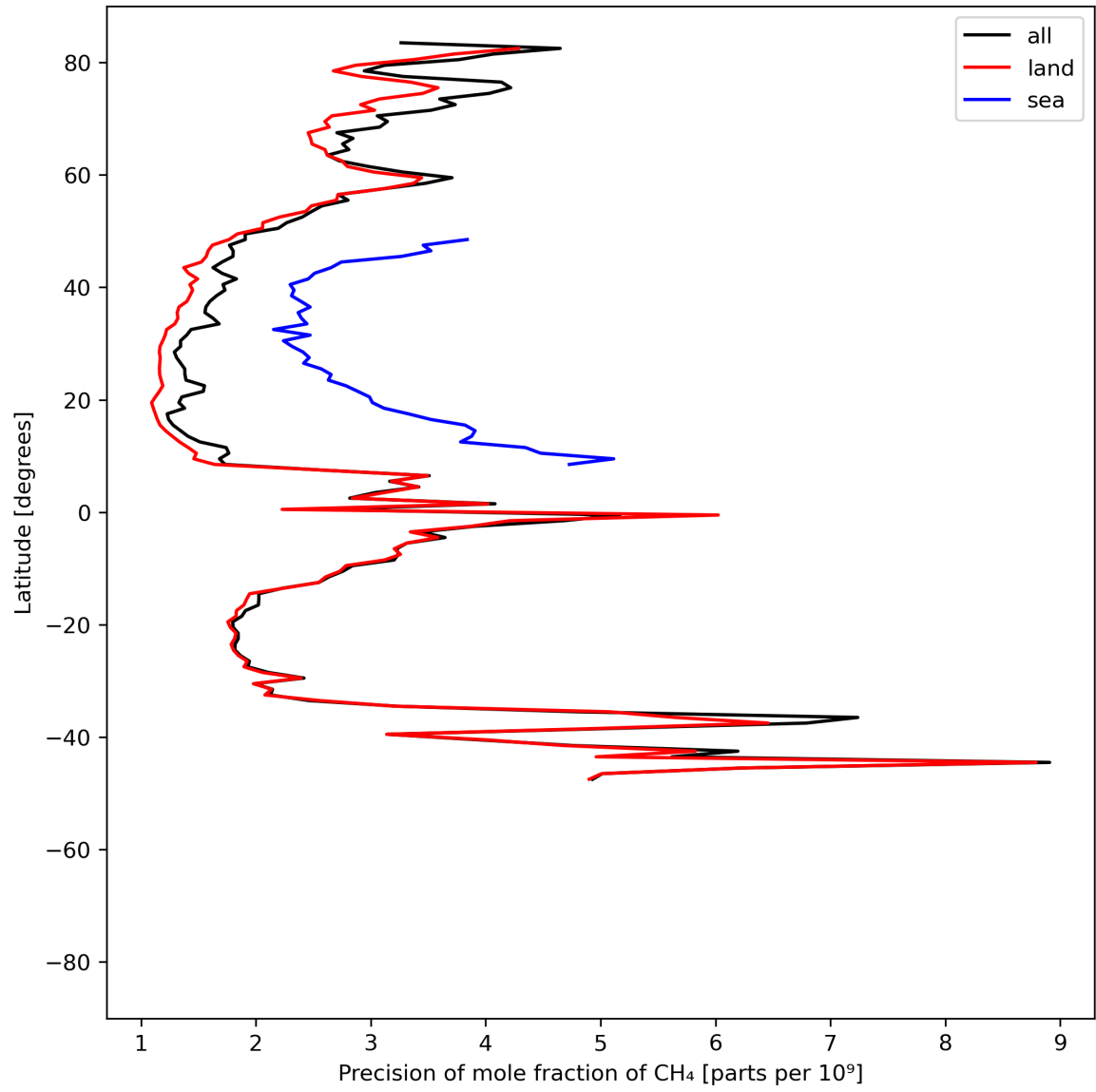
Figure 13: Zonal average of “Precision of mole fraction of CH 4 ” for 2024-06-03 to 2024-06-05.
