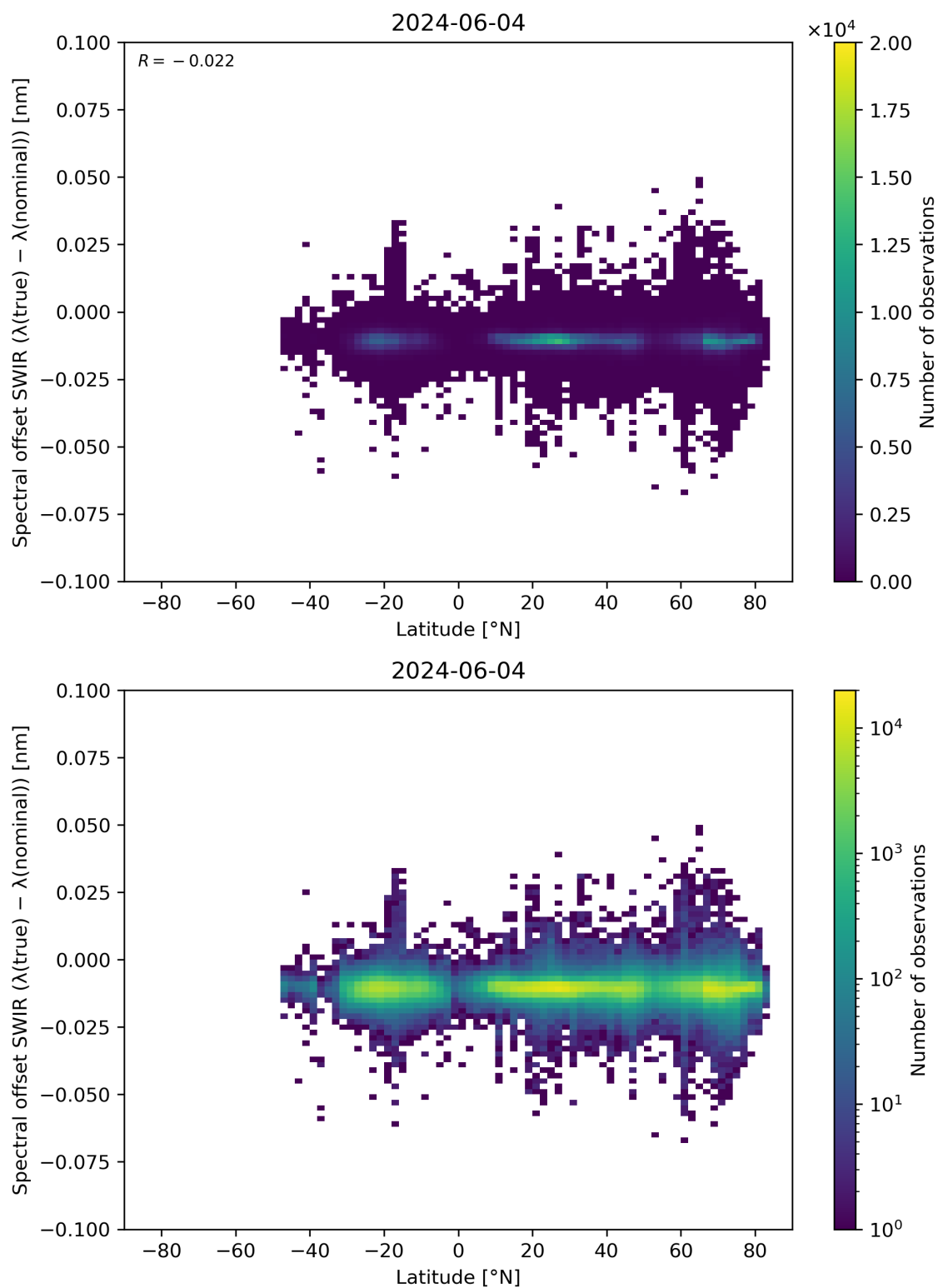
Figure 62: Scatter density plot of “Latitude” against “Spectral offset SWIR ( \lambda(\text{true}) - \lambda(\text{nominal}) )” for 2024-06-03 to 2024-06-05.
