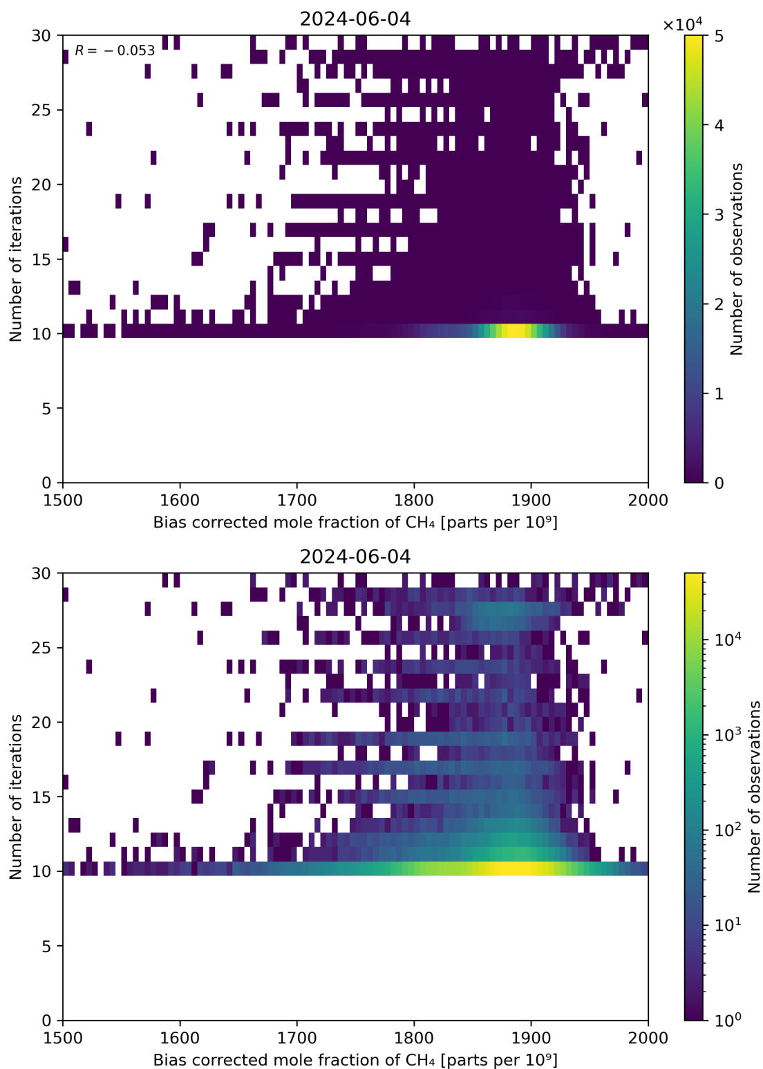
Figure 67: Scatter density plot of “Bias corrected mole fraction of CH 4 ” against “Number of iterations” for 2024-06-03 to 2024-06-05.
