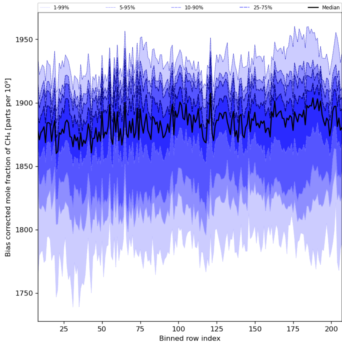
Figure 36: Along track statistics of “Bias corrected mole fraction of CH 4 ” for 2024-06-03 to 2024-06-05
