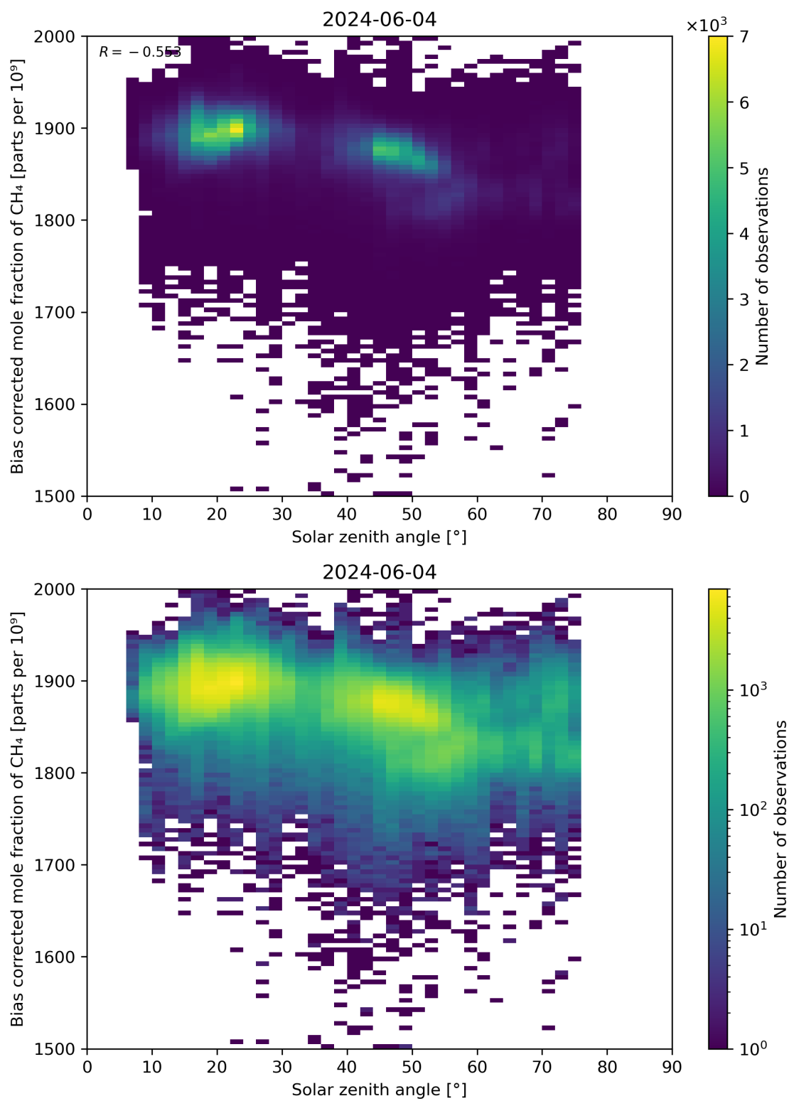
Figure 100: Scatter density plot of “Solar zenith angle” against “Bias corrected mole fraction of CH 4 ” for 2024-06-03 to 2024-06-05.
