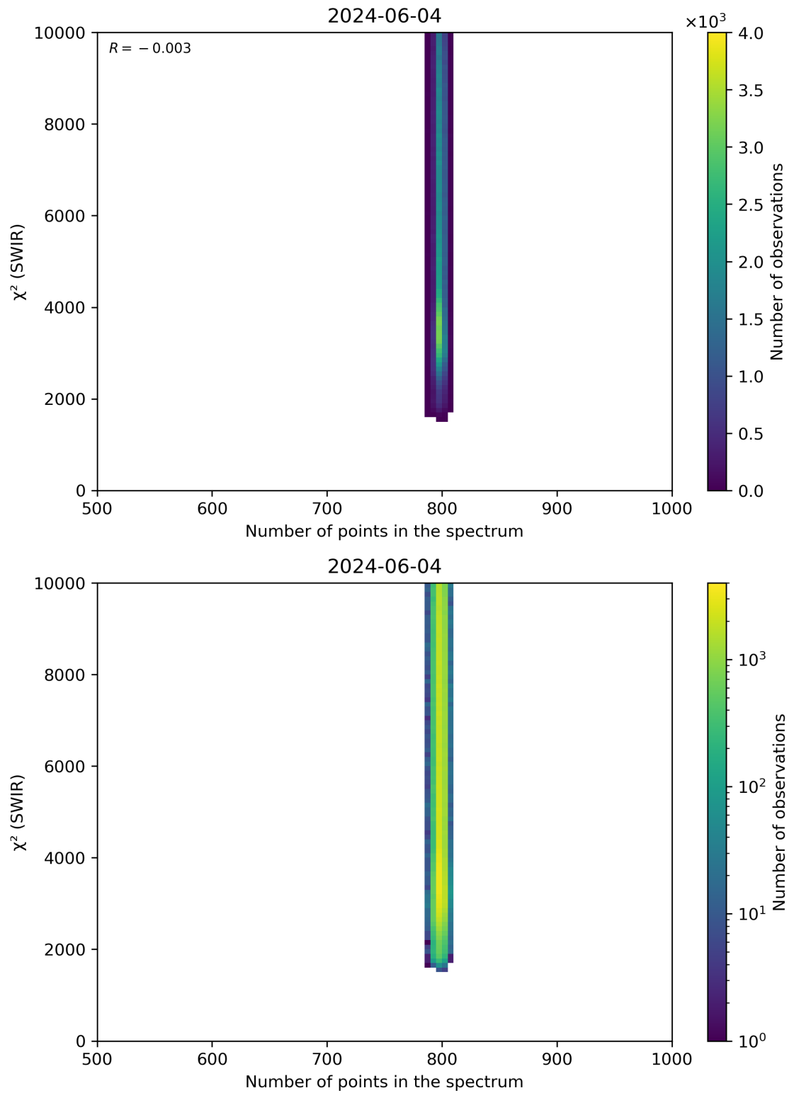
Figure 89: Scatter density plot of “Number of points in the spectrum” against “ \chi^2 (SWIR)” for 2024-06-03 to 2024-06-05.
