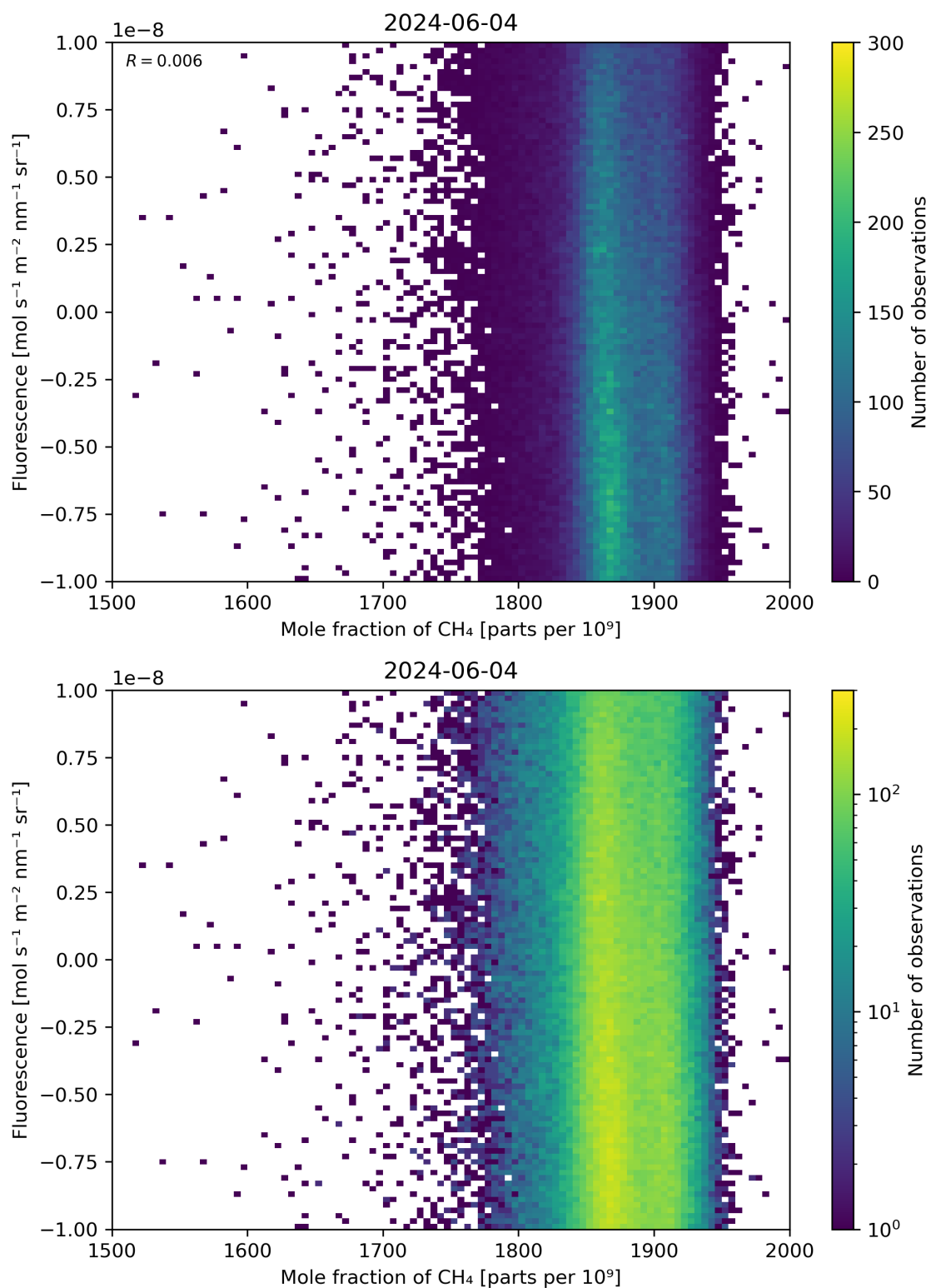
Figure 73: Scatter density plot of “Mole fraction of CH 4 ” against “Fluorescence” for 2024-06-03 to 2024-06-05.
