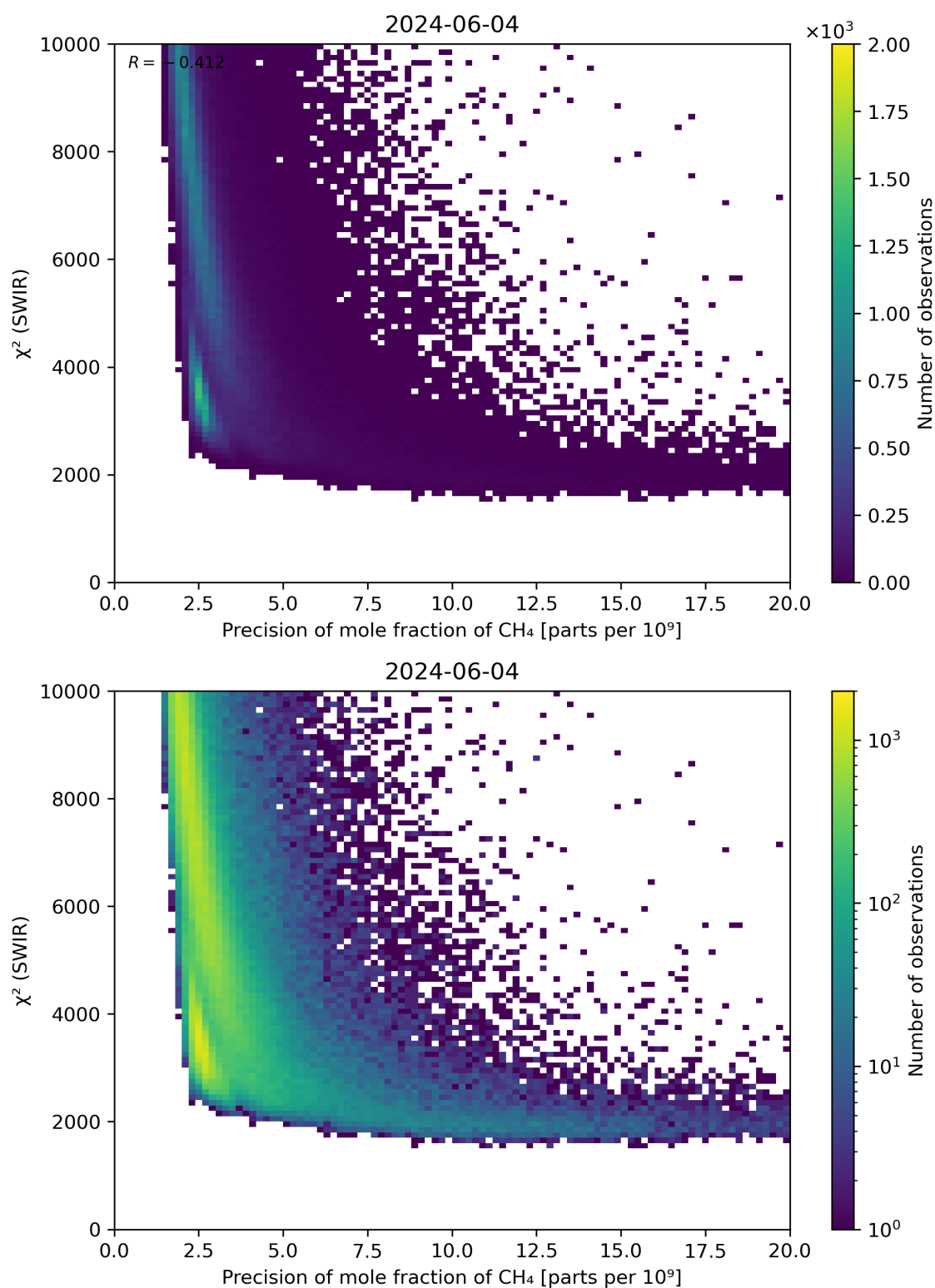
Figure 79: Scatter density plot of “Precision of mole fraction of \text{CH}_4 ” against “ \chi^2 (SWIR)” for 2024-06-03 to 2024-06-05.
