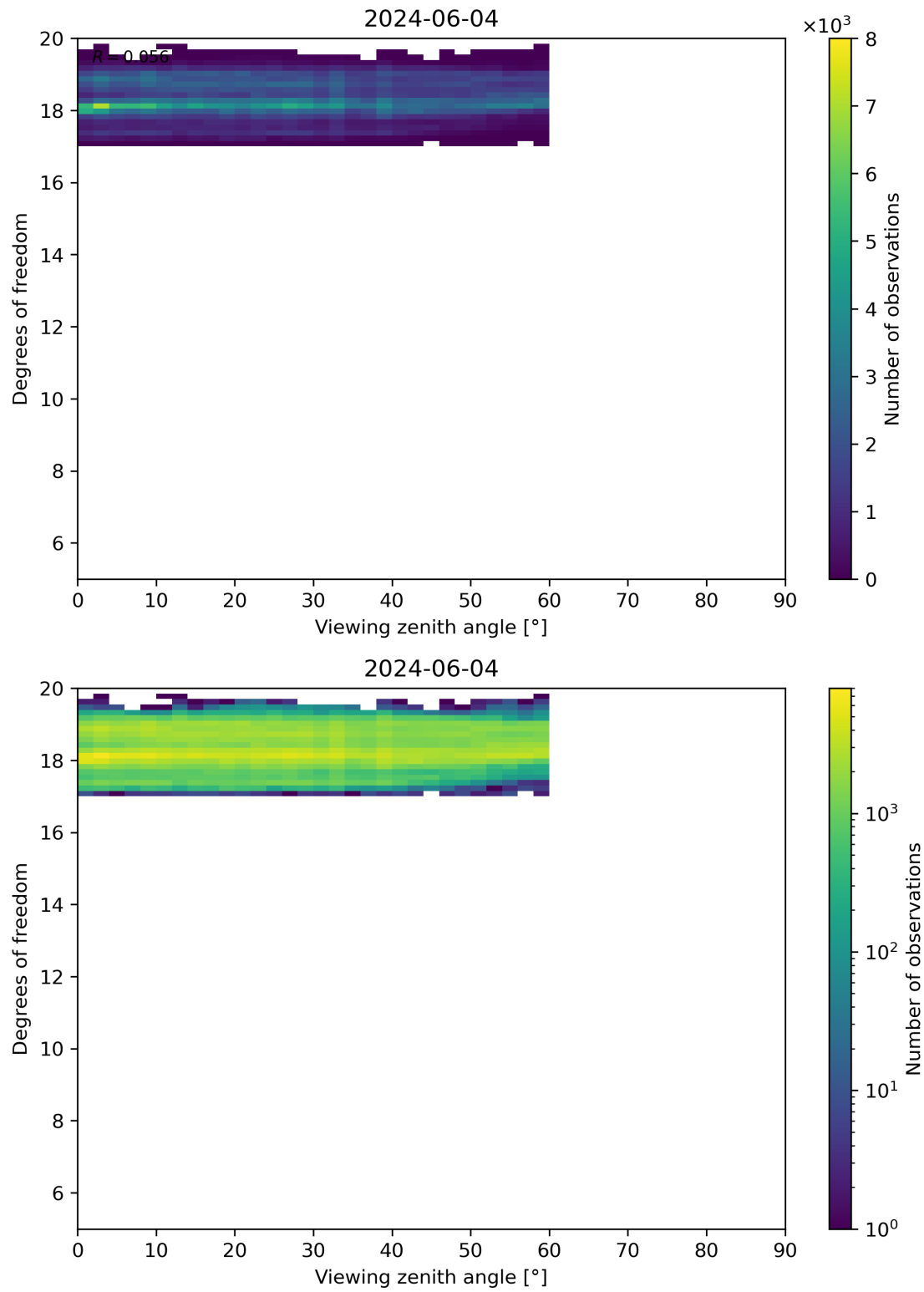
Figure 107: Scatter density plot of “Viewing zenith angle” against “Degrees of freedom” for 2024-06-03 to 2024-06-05.
