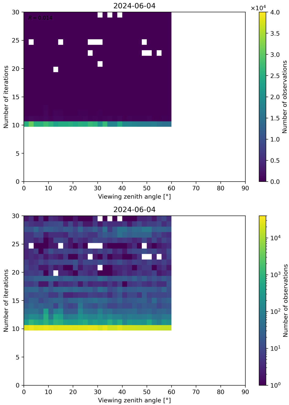
Figure 113: Scatter density plot of “Viewing zenith angle” against “Number of iterations” for 2024-06-03 to 2024-06-05.
