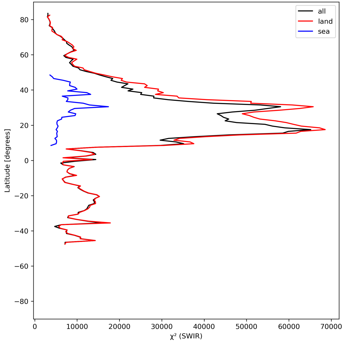
Figure 17: Zonal average of “ \chi^2 (SWIR)” for 2024-06-03 to 2024-06-05.
