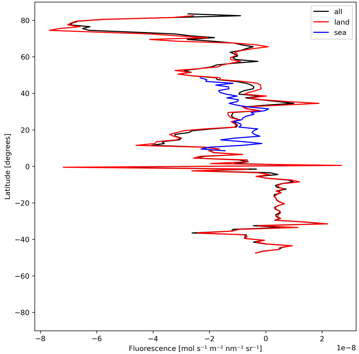
Figure 21: Zonal average of “Fluorescence” for 2024-06-03 to 2024-06-05.
