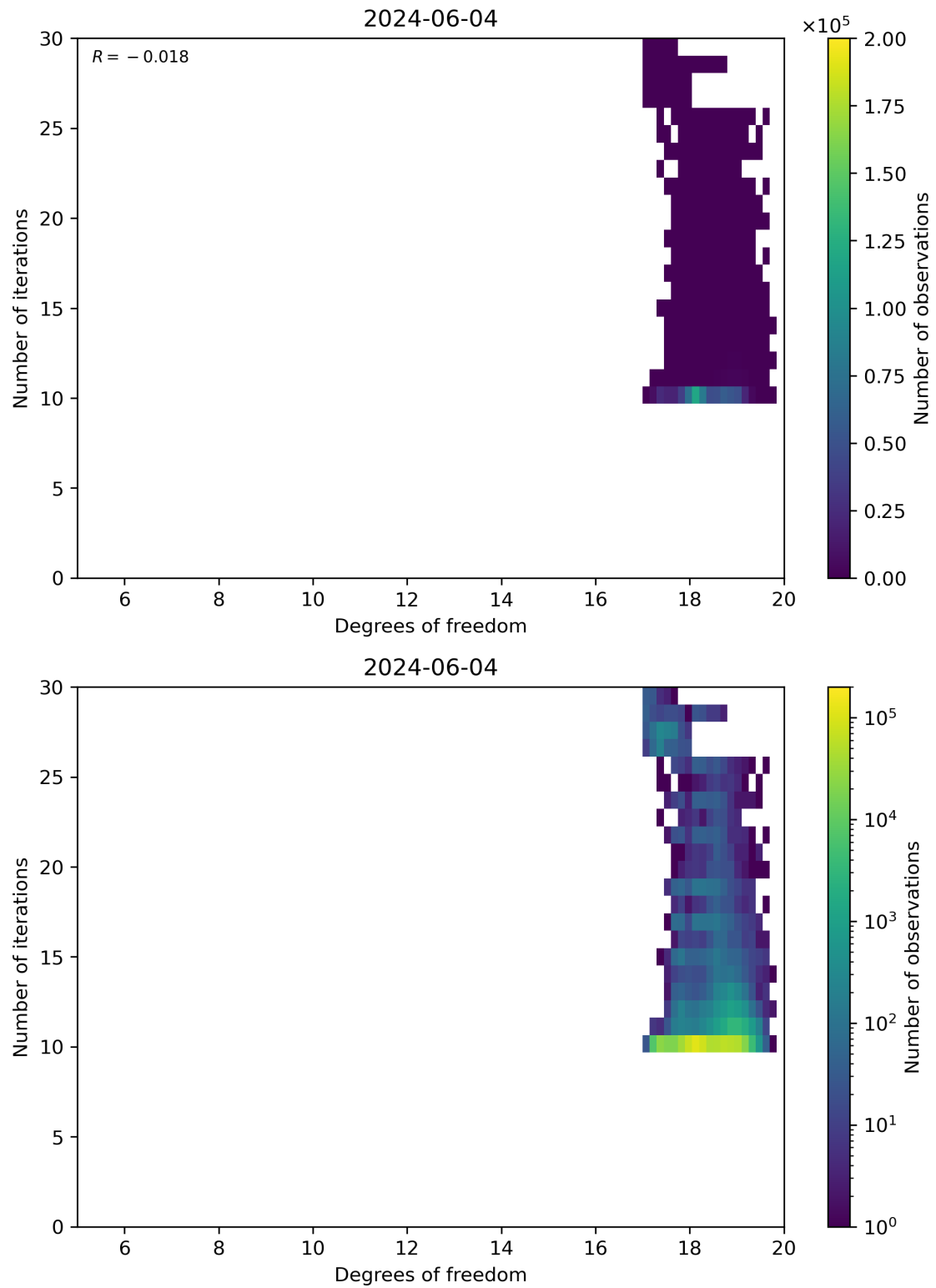
Figure 52: Scatter density plot of “Degrees of freedom” against “Number of iterations” for 2024-06-03 to 2024-06-05.
