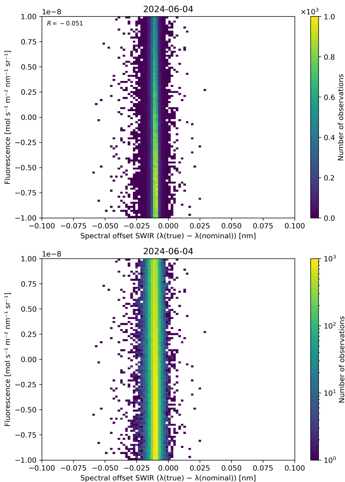
Figure 120: Scatter density plot of “Spectral offset SWIR ( \lambda(\text{true}) - \lambda(\text{nominal}) )” against “Fluorescence” for 2024-06-03 to 2024-06-05.
