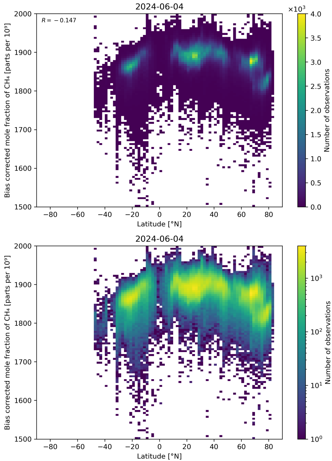
Figure 58: Scatter density plot of “Latitude” against “Bias corrected mole fraction of \text{CH}_4 ” for 2024-06-03 to 2024-06-05.
