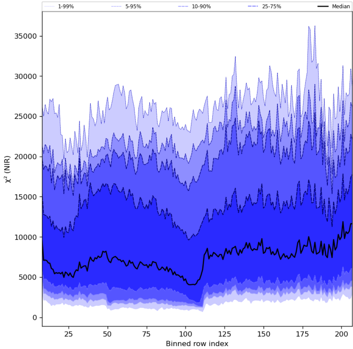
Figure 40: Along track statistics of " \chi^2 (NIR)" for 2024-06-06 to 2024-06-08
