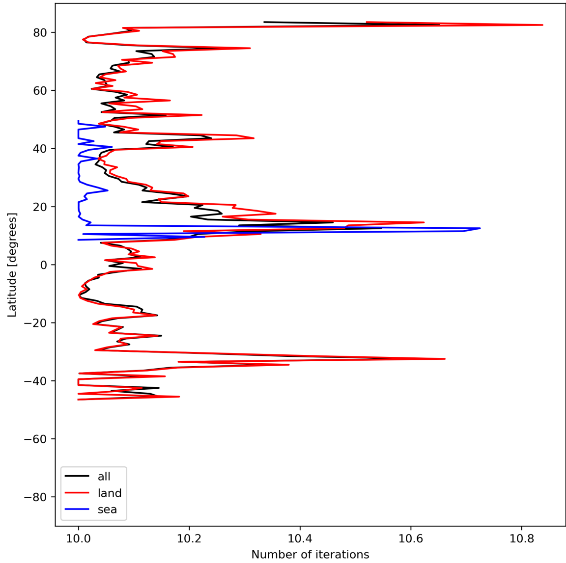
Figure 20: Zonal average of “Number of iterations” for 2024-06-06 to 2024-06-08.
