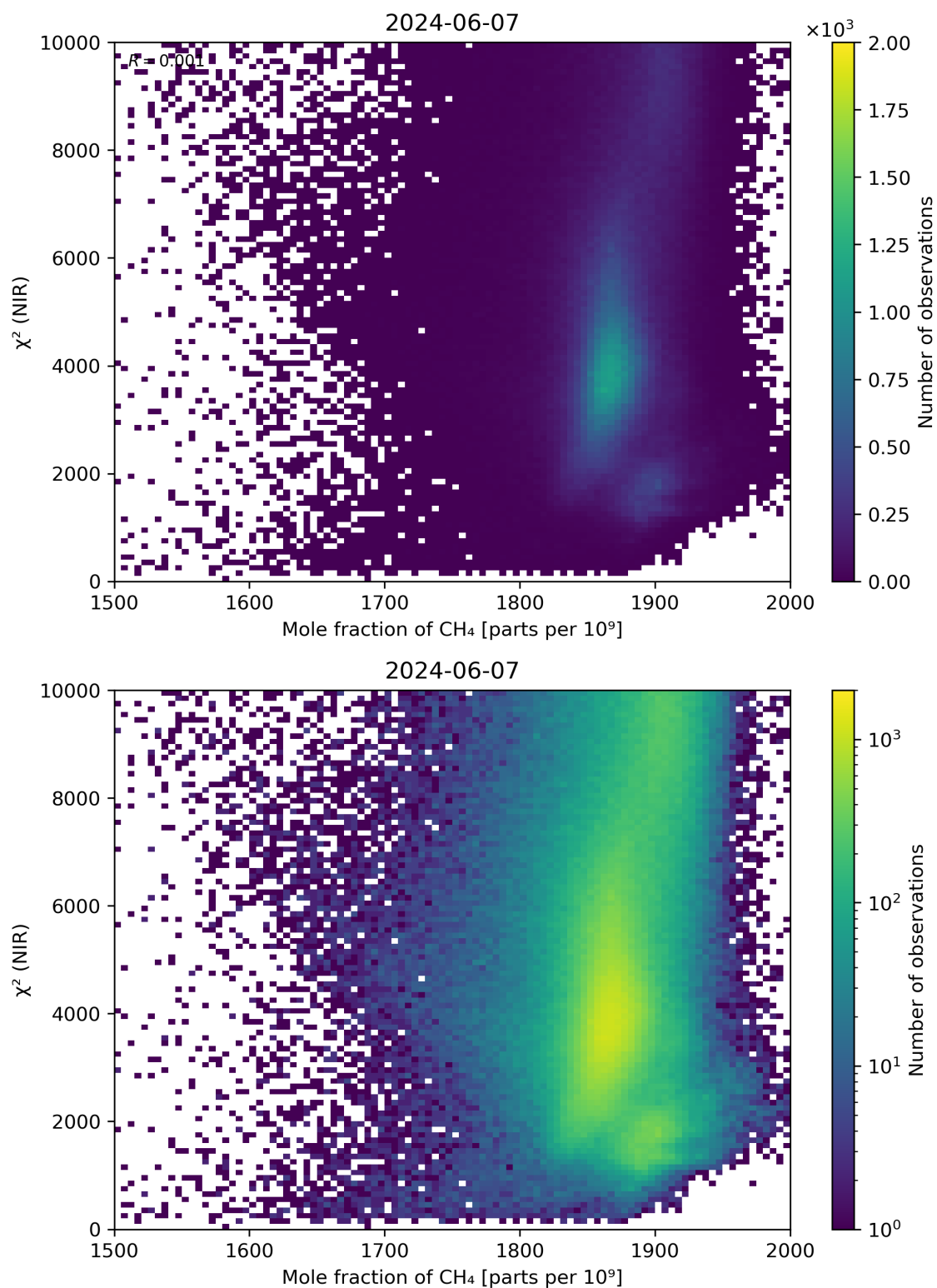
Figure 70: Scatter density plot of “Mole fraction of CH 4 ” against “ \chi^2 (NIR)” for 2024-06-06 to 2024-06-08.
