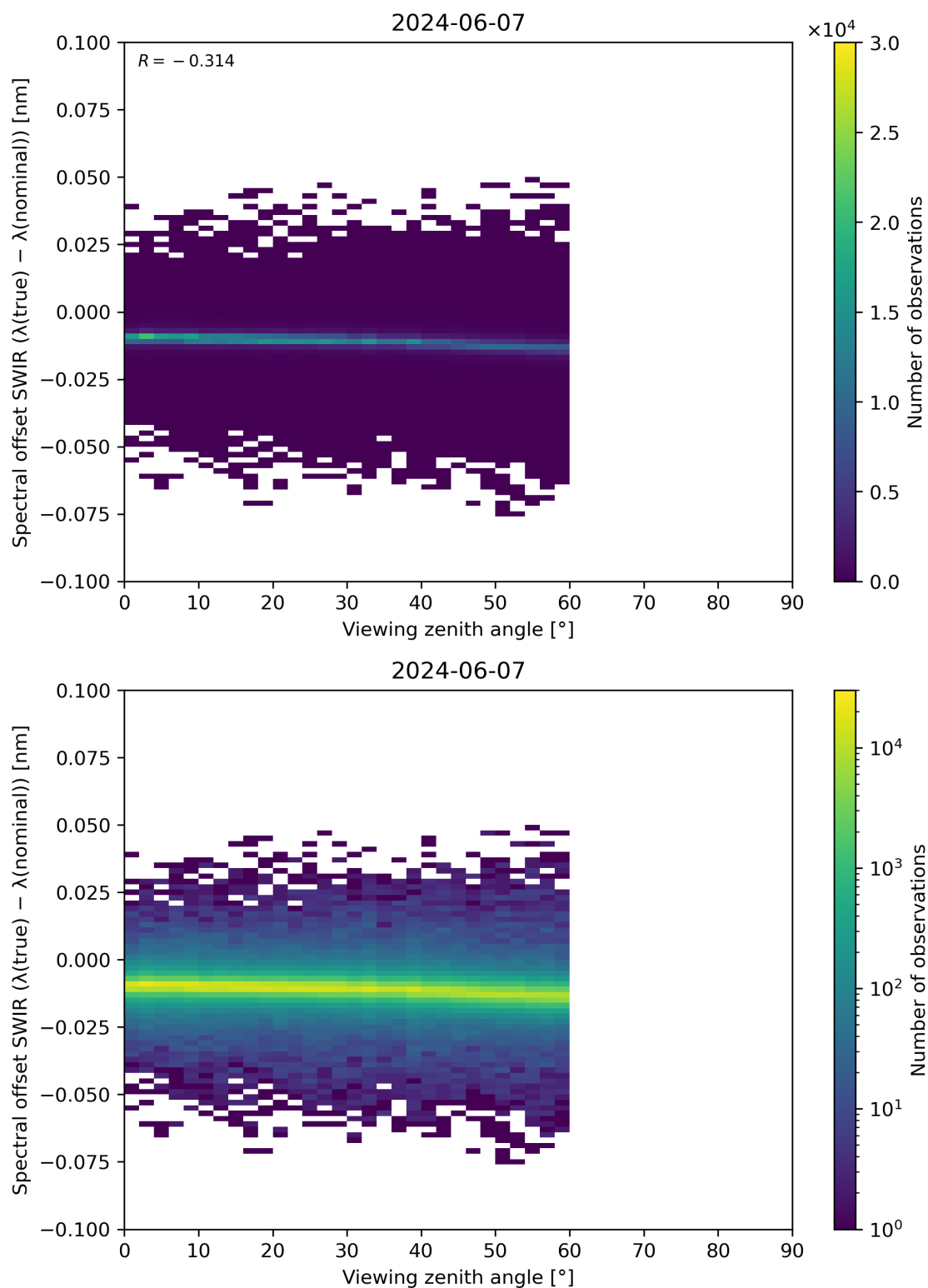
Figure 116: Scatter density plot of “Viewing zenith angle” against “Spectral offset SWIR ( \lambda(\text{true}) - \lambda(\text{nominal}) )” for 2024-06-06 to 2024-06-08.
