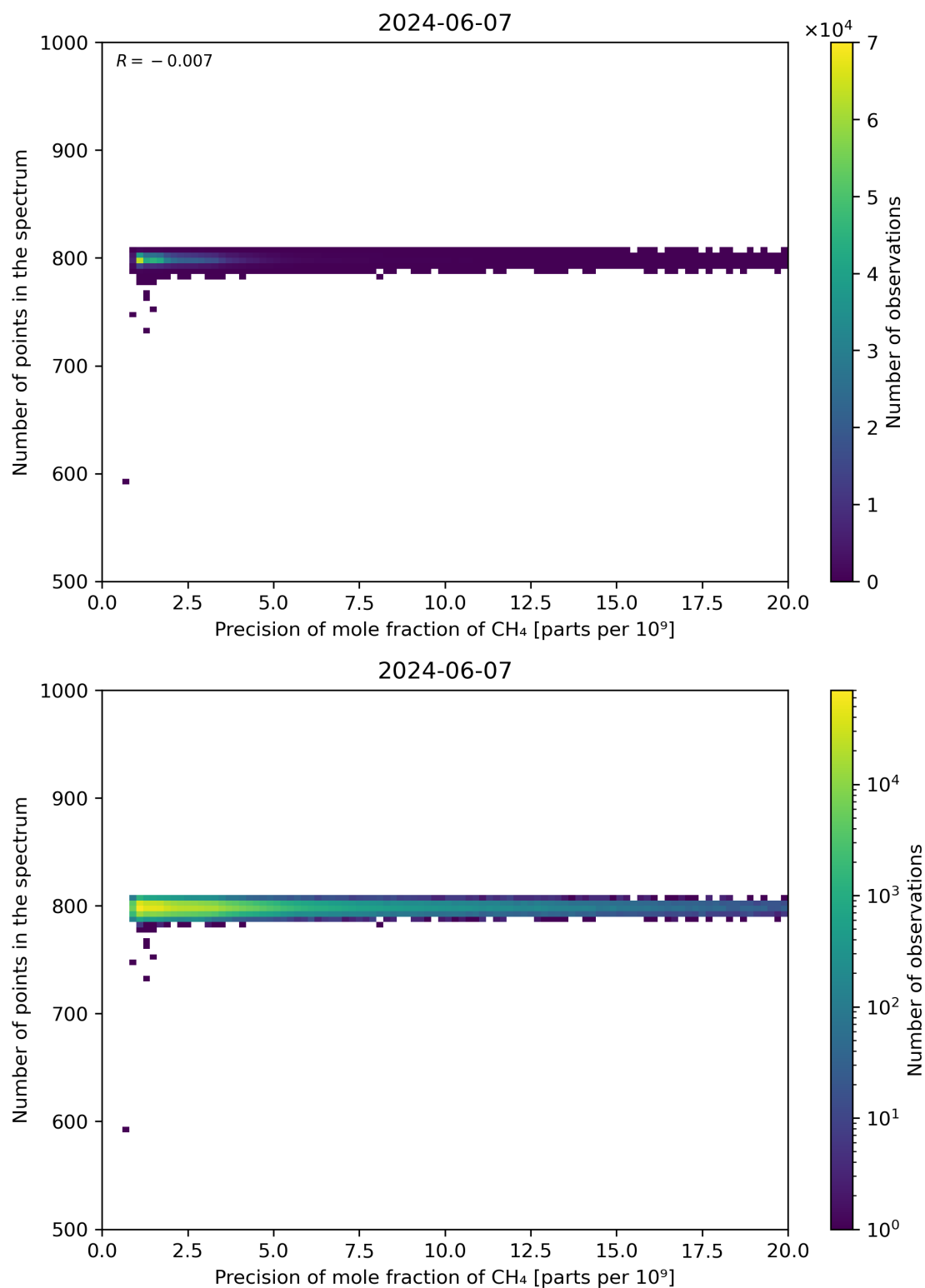
Figure 84: Scatter density plot of “Precision of mole fraction of CH 4 ” against “Number of points in the spectrum” for 2024-06-06 to 2024-06-08.
