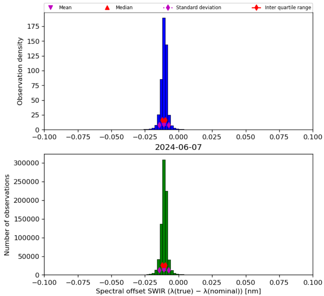
Figure 27: Histogram of “Spectral offset SWIR ( \lambda(\text{true}) - \lambda(\text{nominal}) )” for 2024-06-06 to 2024-06-08
