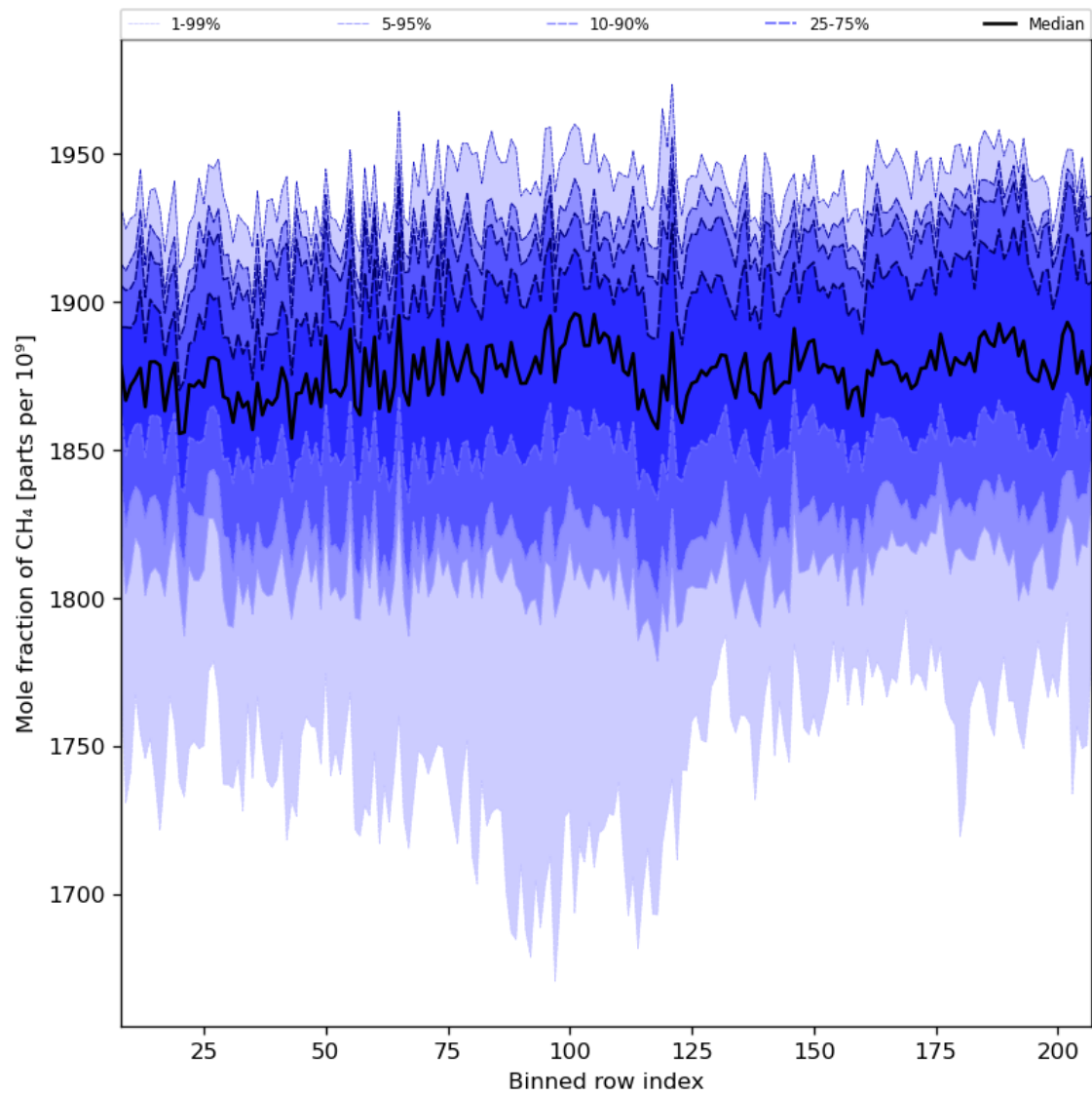
Figure 34: Along track statistics of “Mole fraction of CH 4 ” for 2024-06-06 to 2024-06-08
