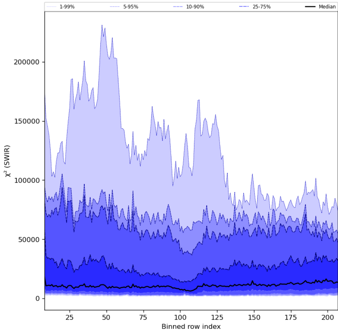
Figure 39: Along track statistics of “ \chi^2 (SWIR)” for 2024-06-06 to 2024-06-08
