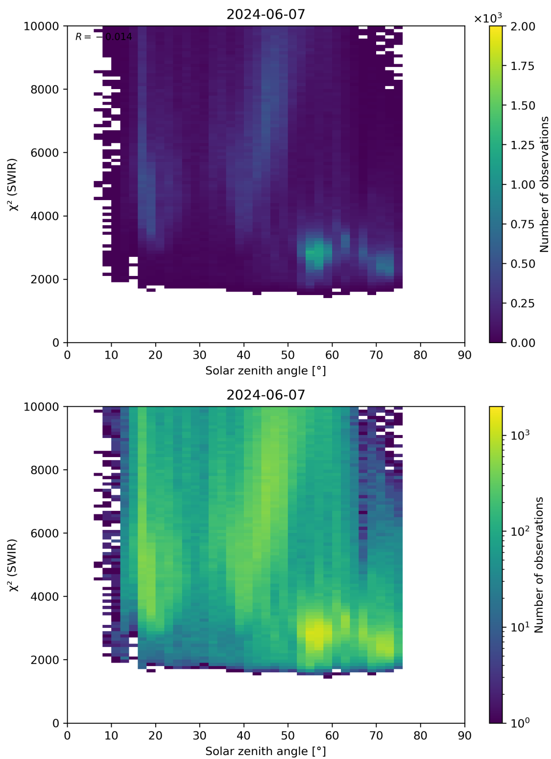
Figure 95: Scatter density plot of “Solar zenith angle” against “ \chi^2 (SWIR)” for 2024-06-06 to 2024-06-08.
