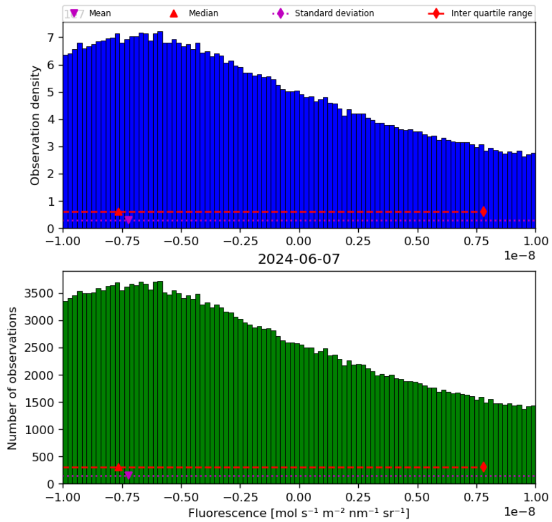
Figure 32: Histogram of “Fluorescence” for 2024-06-06 to 2024-06-08
