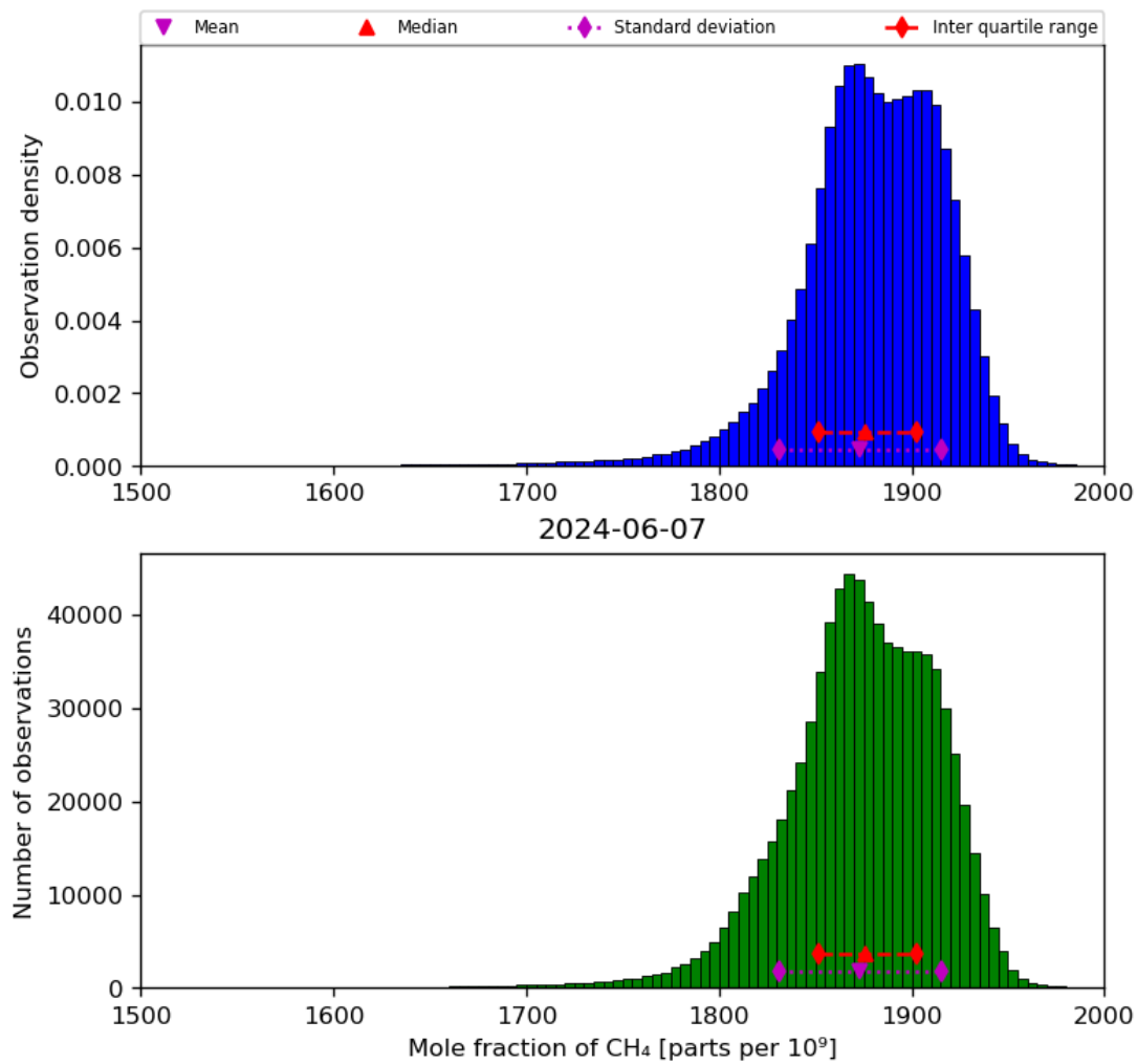
Figure 23: Histogram of “Mole fraction of CH 4 ” for 2024-06-06 to 2024-06-08
