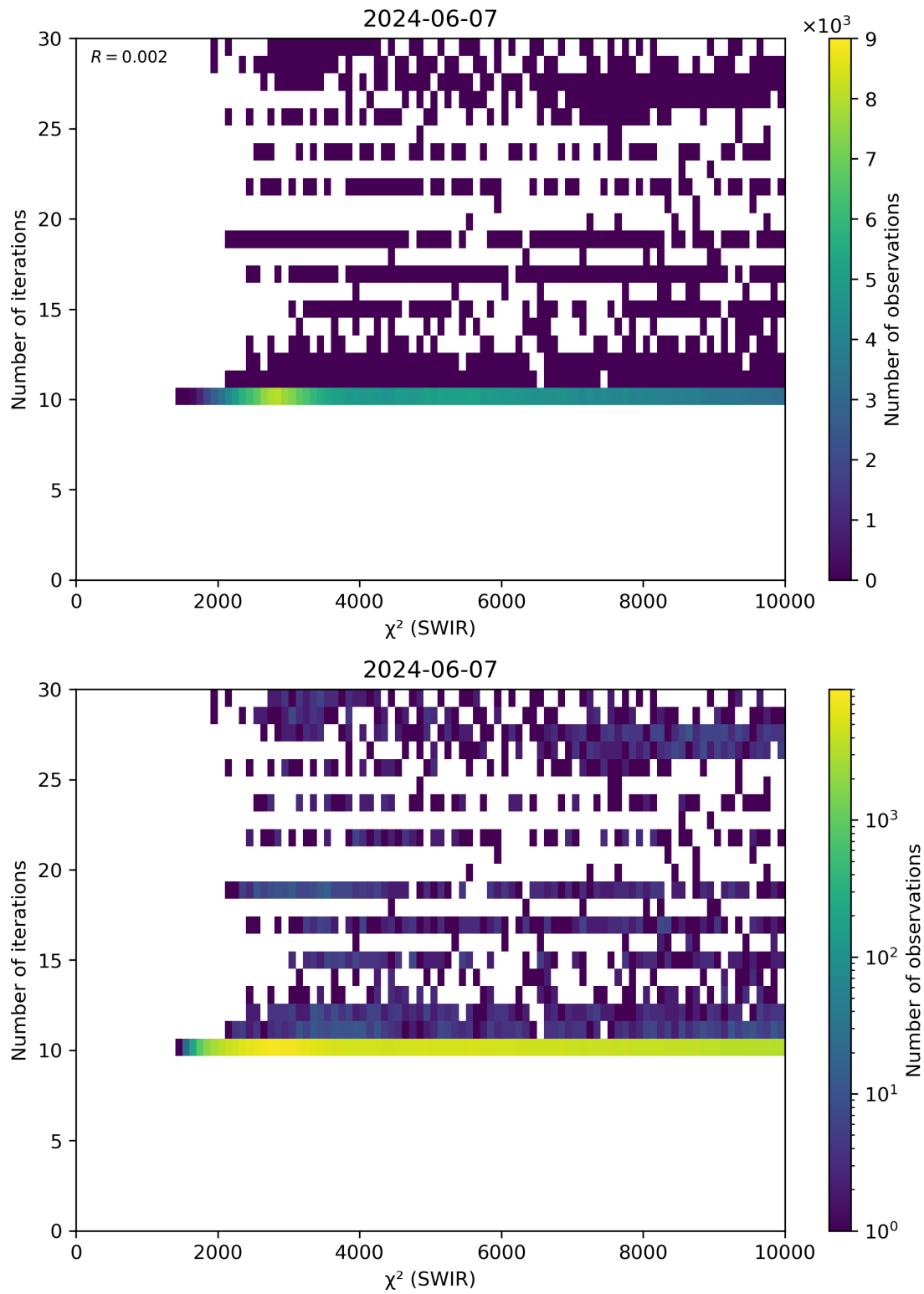
Figure 50: Scatter density plot of “ \chi^2 (SWIR)” against “Number of iterations” for 2024-06-06 to 2024-06-08.
