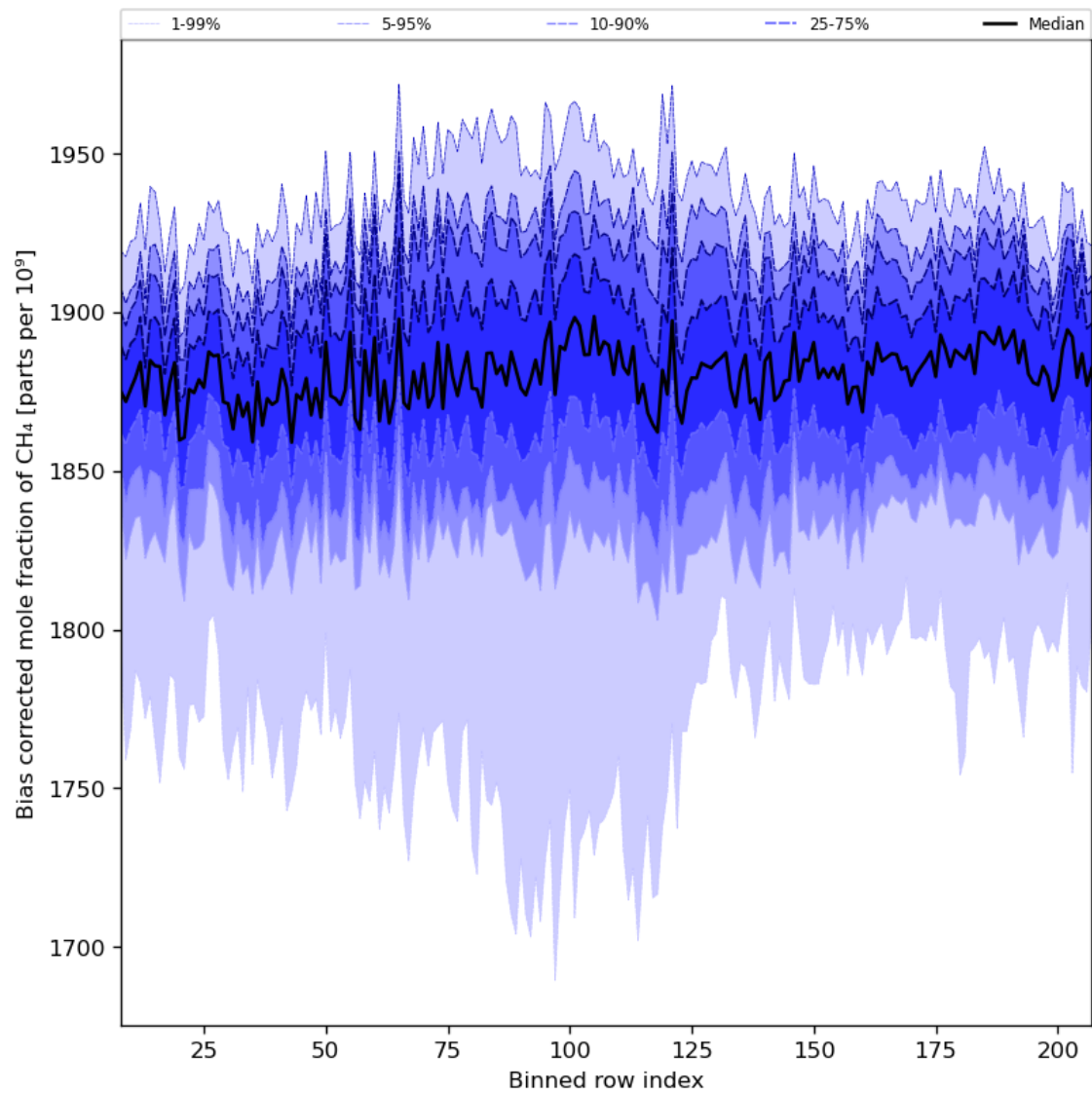
Figure 36: Along track statistics of “Bias corrected mole fraction of CH 4 ” for 2024-06-06 to 2024-06-08
