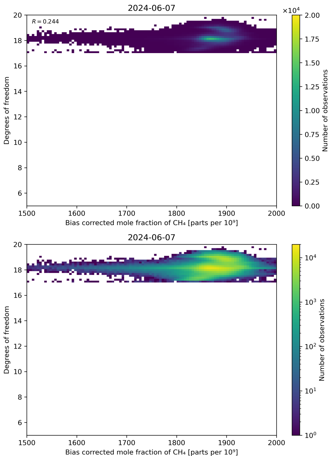
Figure 65: Scatter density plot of “Bias corrected mole fraction of CH 4 ” against “Degrees of freedom” for 2024-06-06 to 2024-06-08.
