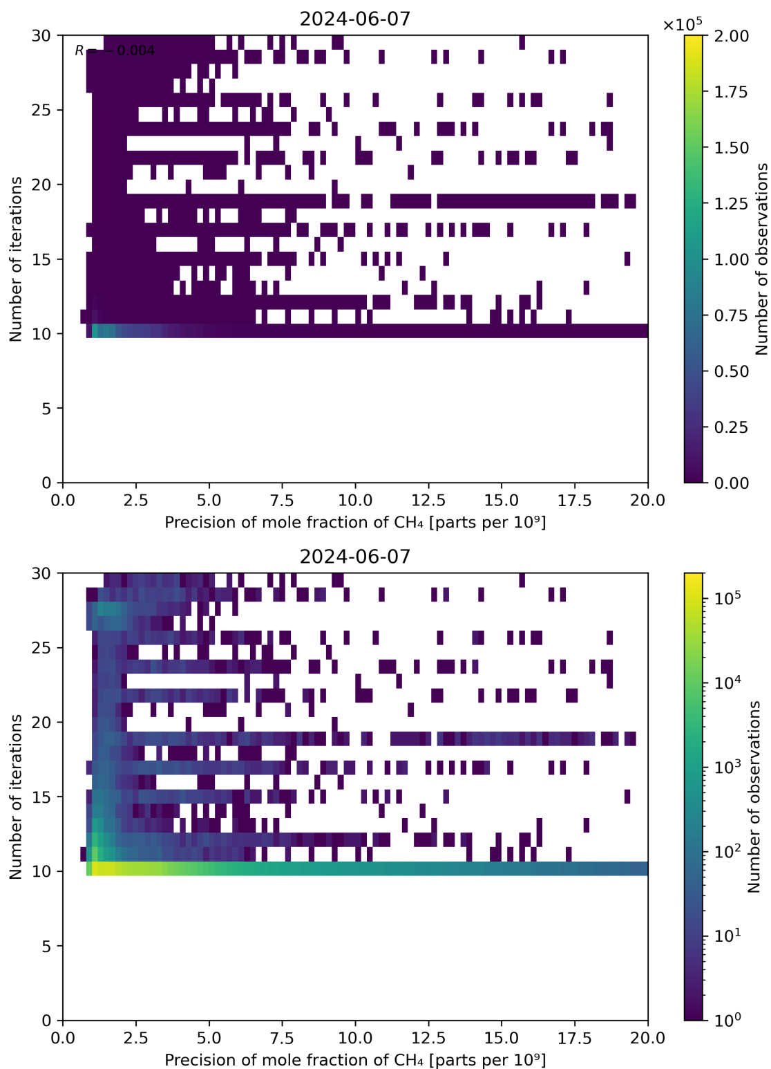
Figure 83: Scatter density plot of “Precision of mole fraction of CH 4 ” against “Number of iterations” for 2024-06-06 to 2024-06-08.
