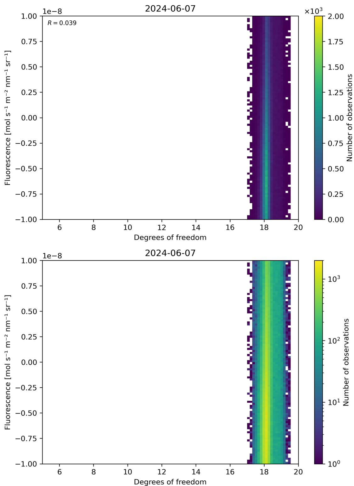
Figure 51: Scatter density plot of “Degrees of freedom” against “Fluorescence” for 2024-06-06 to 2024-06-08.
