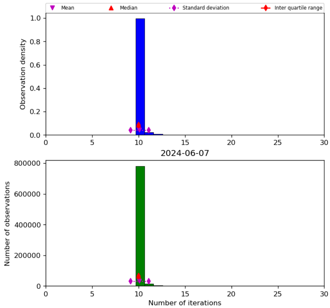
Figure 31: Histogram of “Number of iterations” for 2024-06-06 to 2024-06-08
