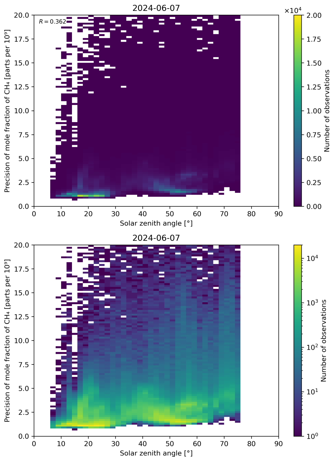
Figure 101: Scatter density plot of “Solar zenith angle” against “Precision of mole fraction of CH 4 ” for 2024-06-06 to 2024-06-08.
