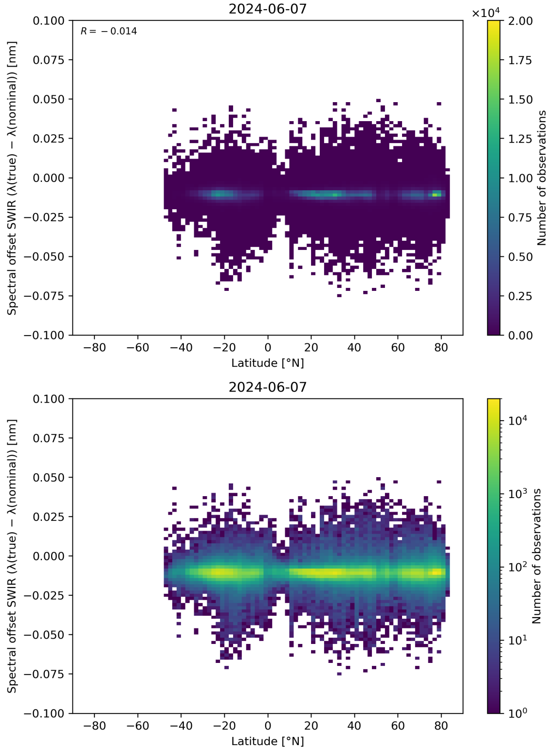
Figure 62: Scatter density plot of “Latitude” against “Spectral offset SWIR ( \lambda(\text{true}) - \lambda(\text{nominal}) )” for 2024-06-06 to 2024-06-08.
