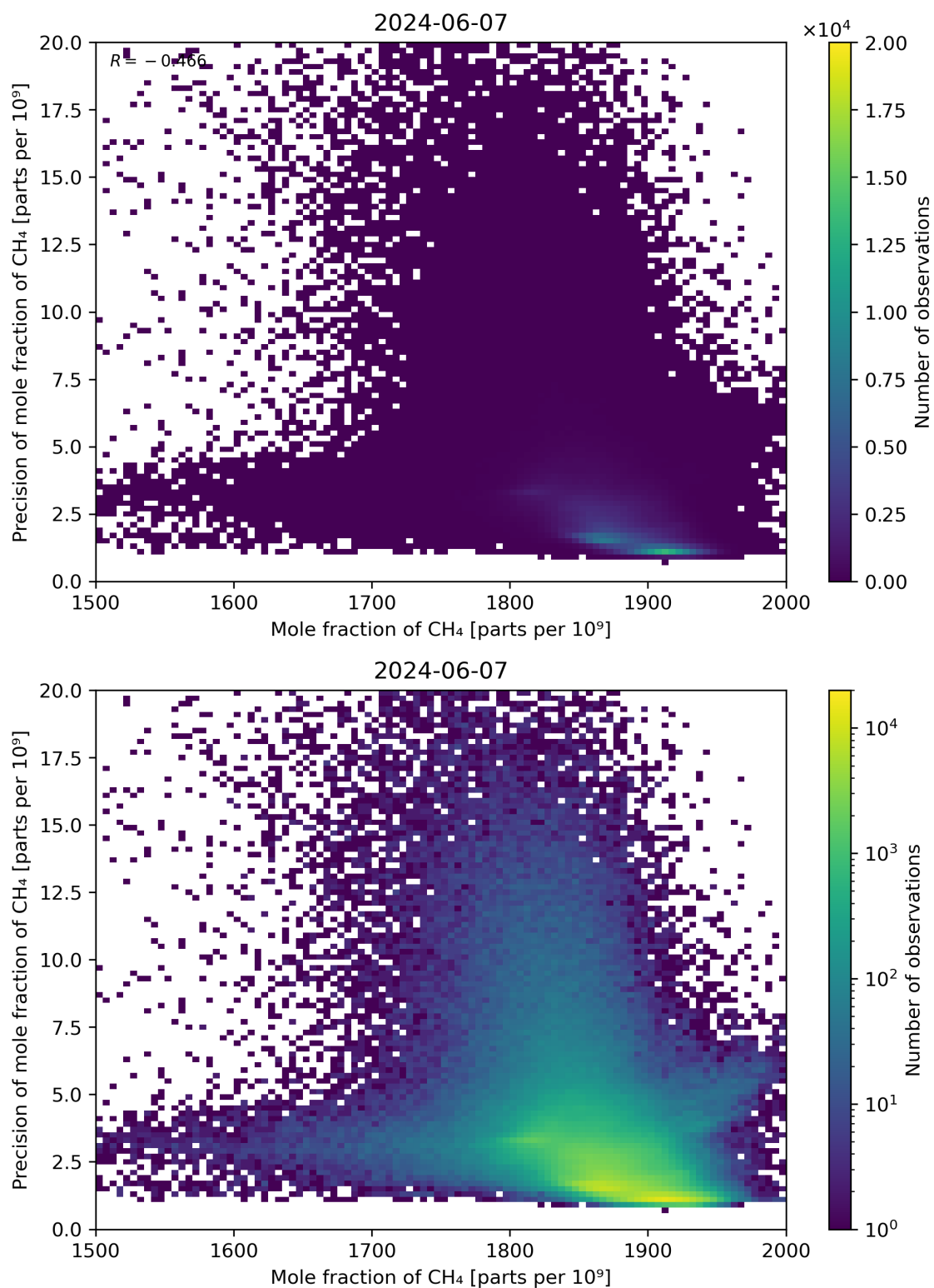
Figure 75: Scatter density plot of “Mole fraction of CH 4 ” against “Precision of mole fraction of CH 4 ” for 2024-06-06 to 2024-06-08.
