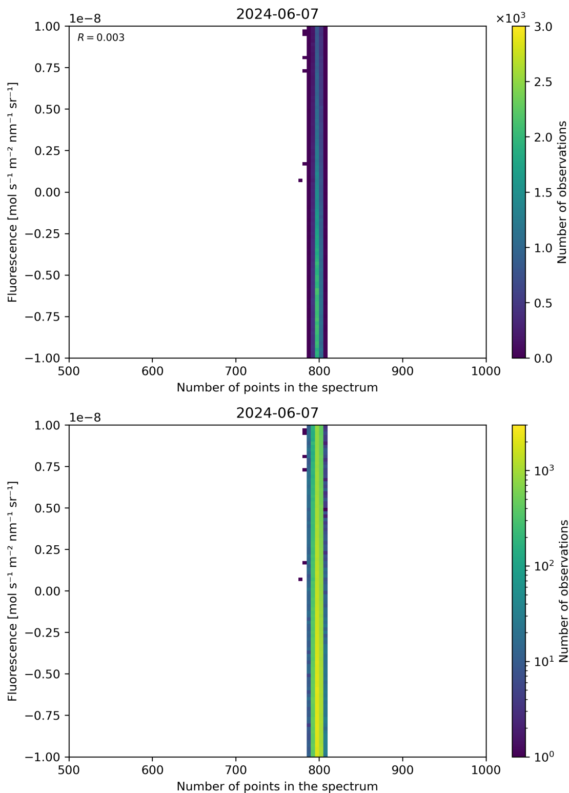
Figure 91: Scatter density plot of “Number of points in the spectrum” against “Fluorescence” for 2024-06-06 to 2024-06-08.
