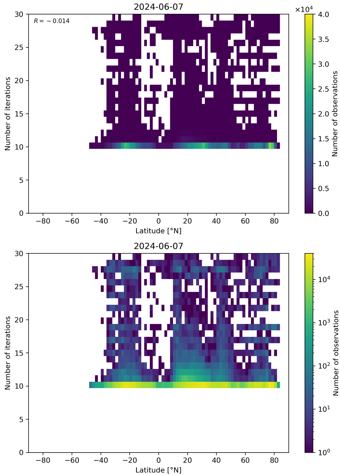
Figure 60: Scatter density plot of “Latitude” against “Number of iterations” for 2024-06-06 to 2024-06-08.
