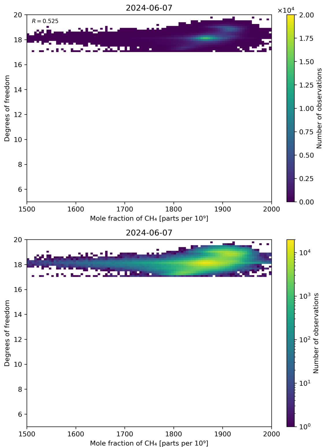
Figure 72: Scatter density plot of “Mole fraction of CH 4 ” against “Degrees of freedom” for 2024-06-06 to 2024-06-08.
