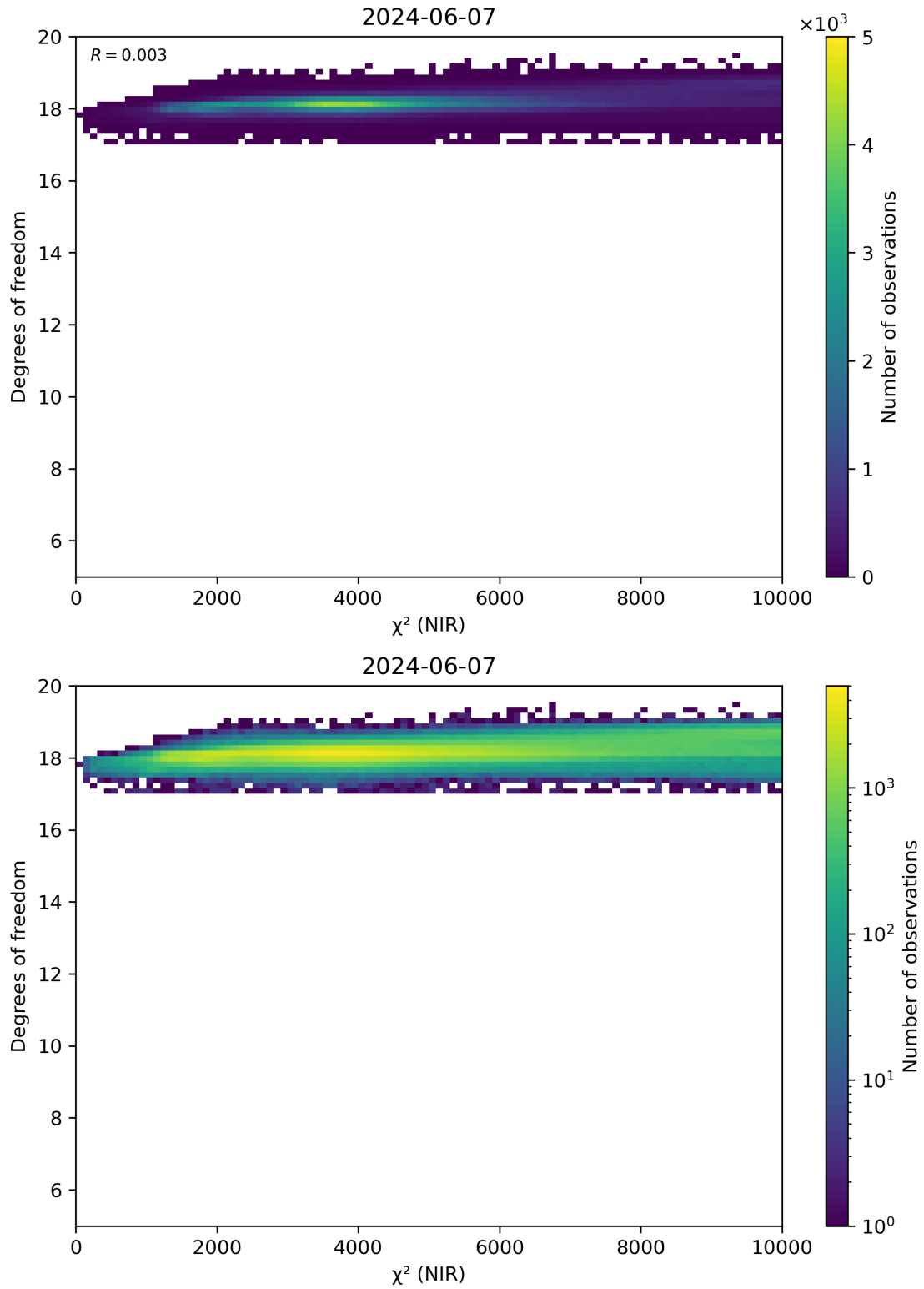
Figure 44: Scatter density plot of “ \chi^2 (NIR)” against “Degrees of freedom” for 2024-06-06 to 2024-06-08.
