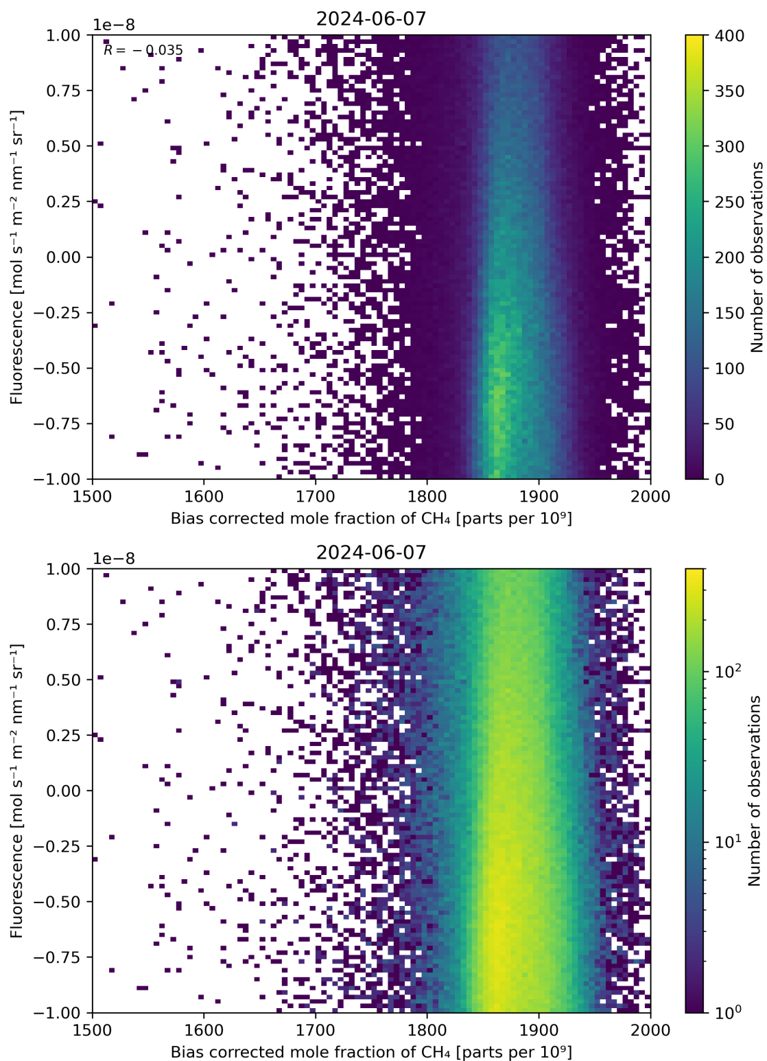
Figure 66: Scatter density plot of “Bias corrected mole fraction of \text{CH}_4 ” against “Fluorescence” for 2024-06-06 to 2024-06-08.
