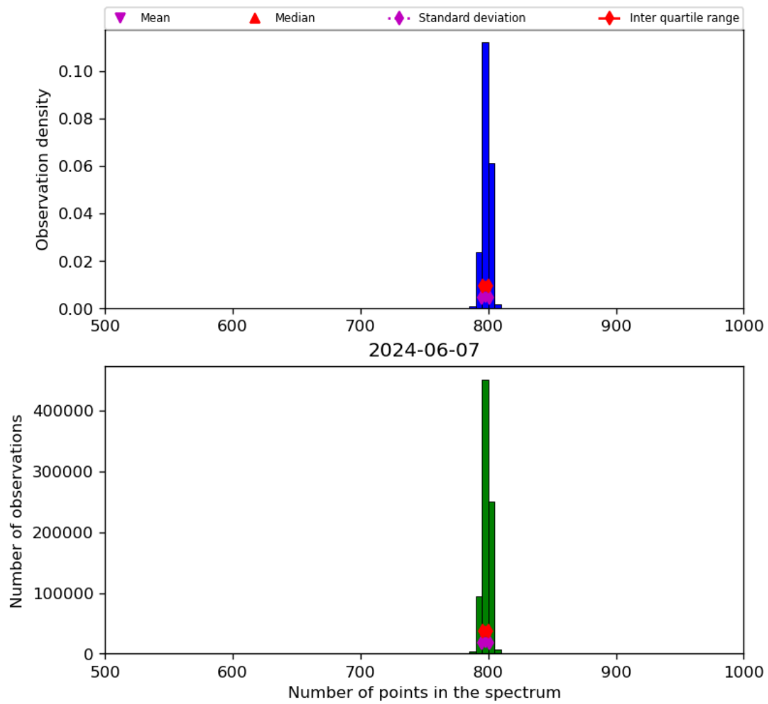
Figure 26: Histogram of “Number of points in the spectrum” for 2024-06-06 to 2024-06-08
