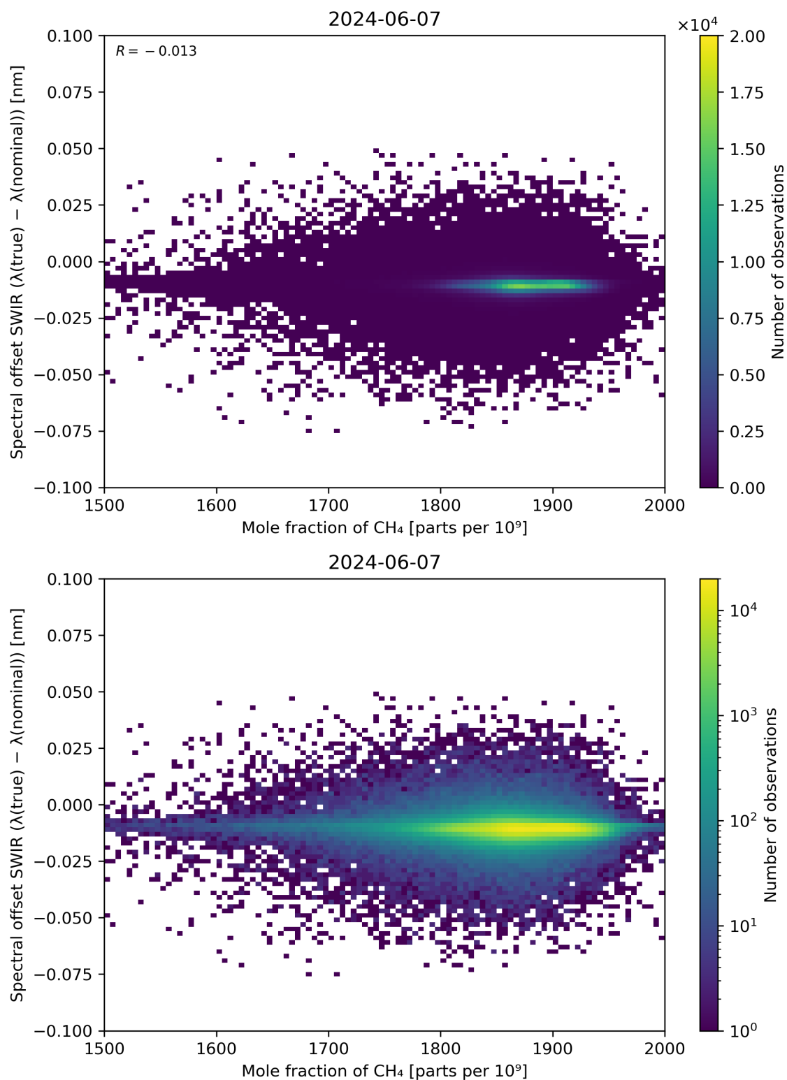
Figure 86: Scatter density plot of “Mole fraction of CH 4 ” against “Spectral offset SWIR ( \lambda(\text{true}) - \lambda(\text{nominal}) )” for 2024-06-06 to 2024-06-08.
