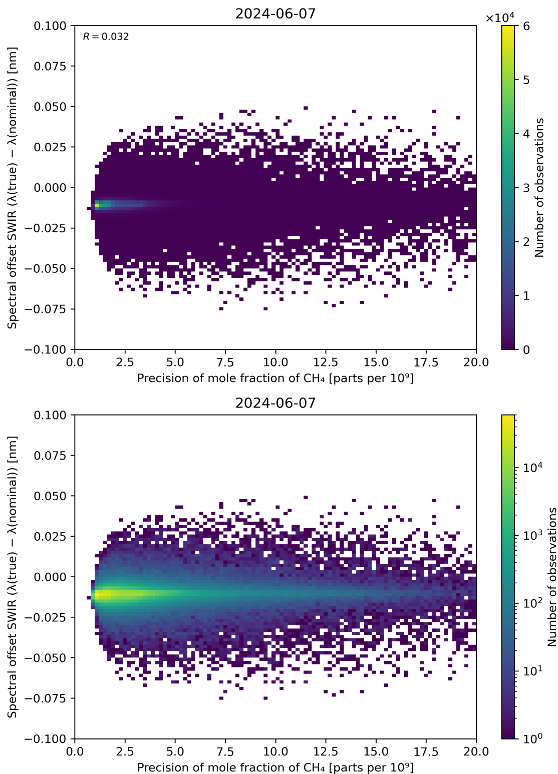
Figure 85: Scatter density plot of “Precision of mole fraction of \text{CH}_4 ” against “Spectral offset SWIR ( \lambda(\text{true}) - \lambda(\text{nominal}) )” for 2024-06-06 to 2024-06-08.
