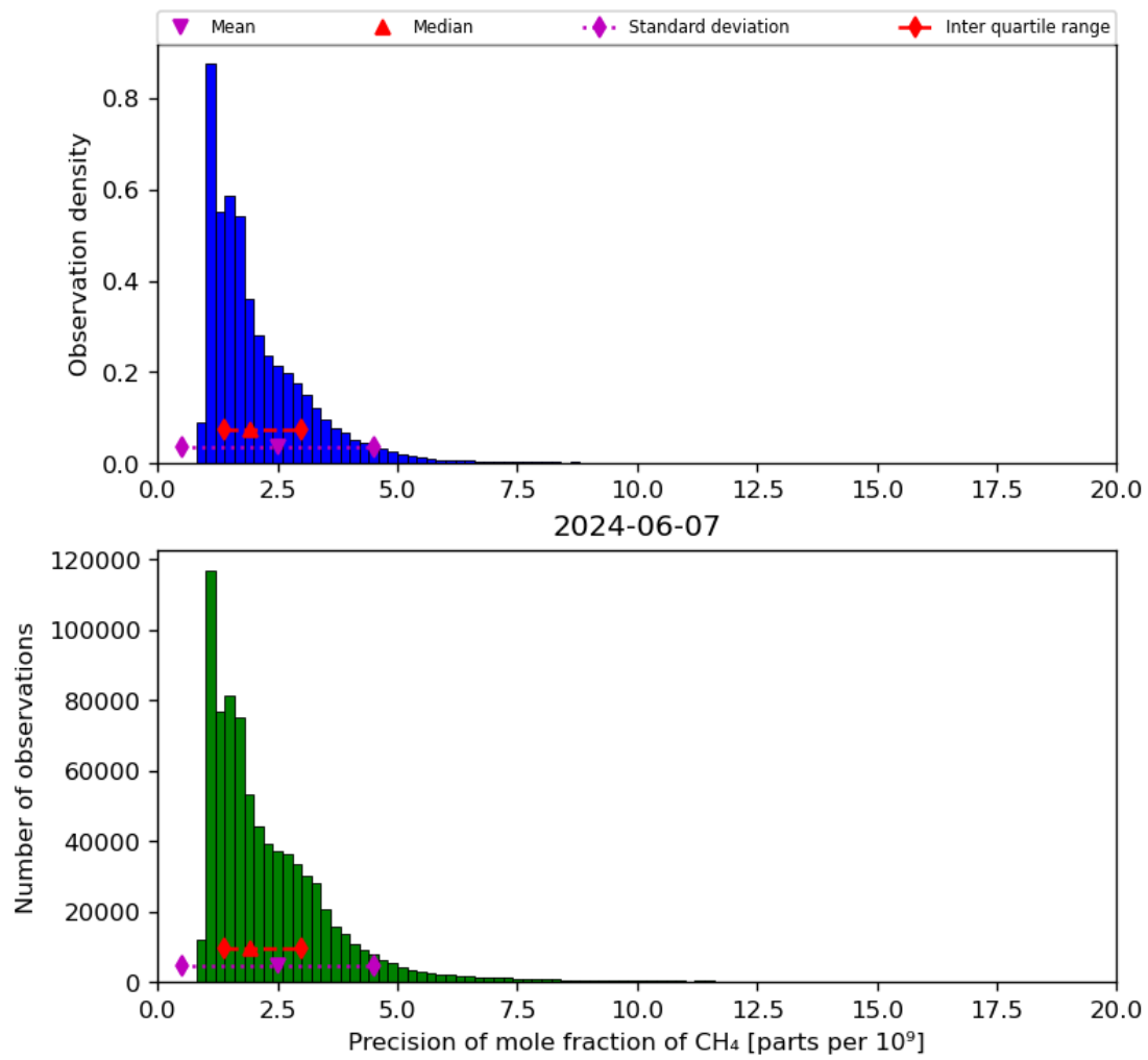
Figure 24: Histogram of “Precision of mole fraction of CH 4 ” for 2024-06-06 to 2024-06-08
