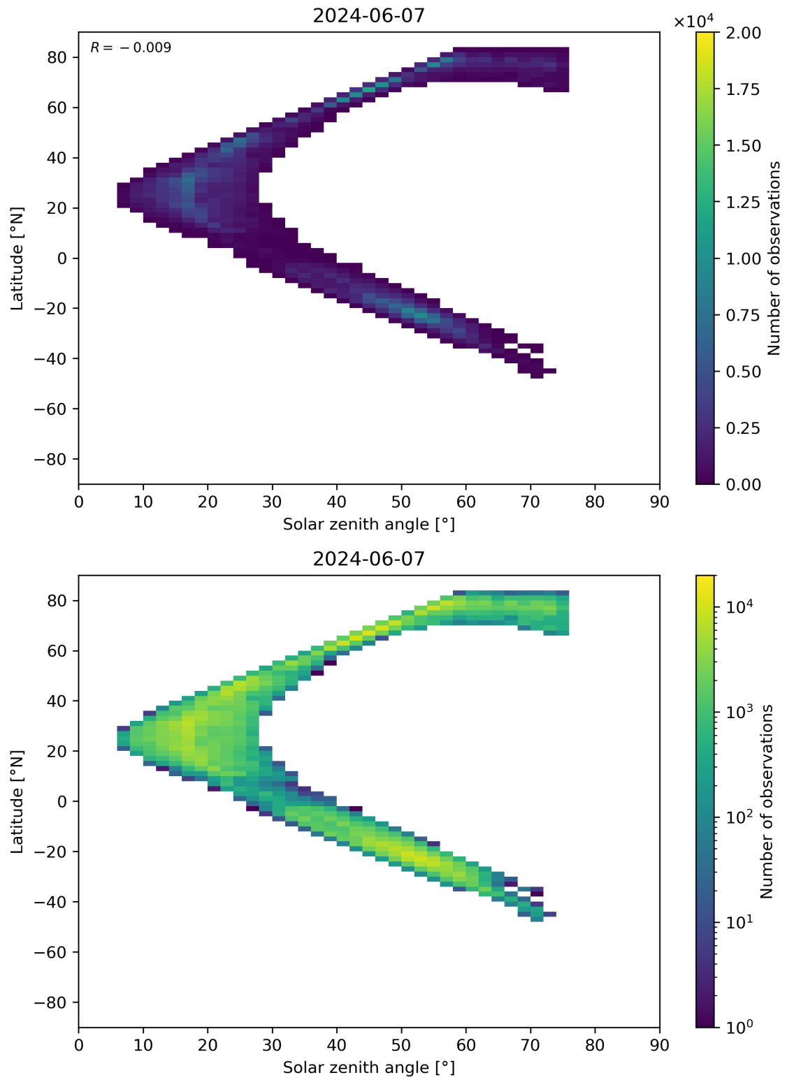
Figure 98: Scatter density plot of “Solar zenith angle” against “Latitude” for 2024-06-06 to 2024-06-08.
