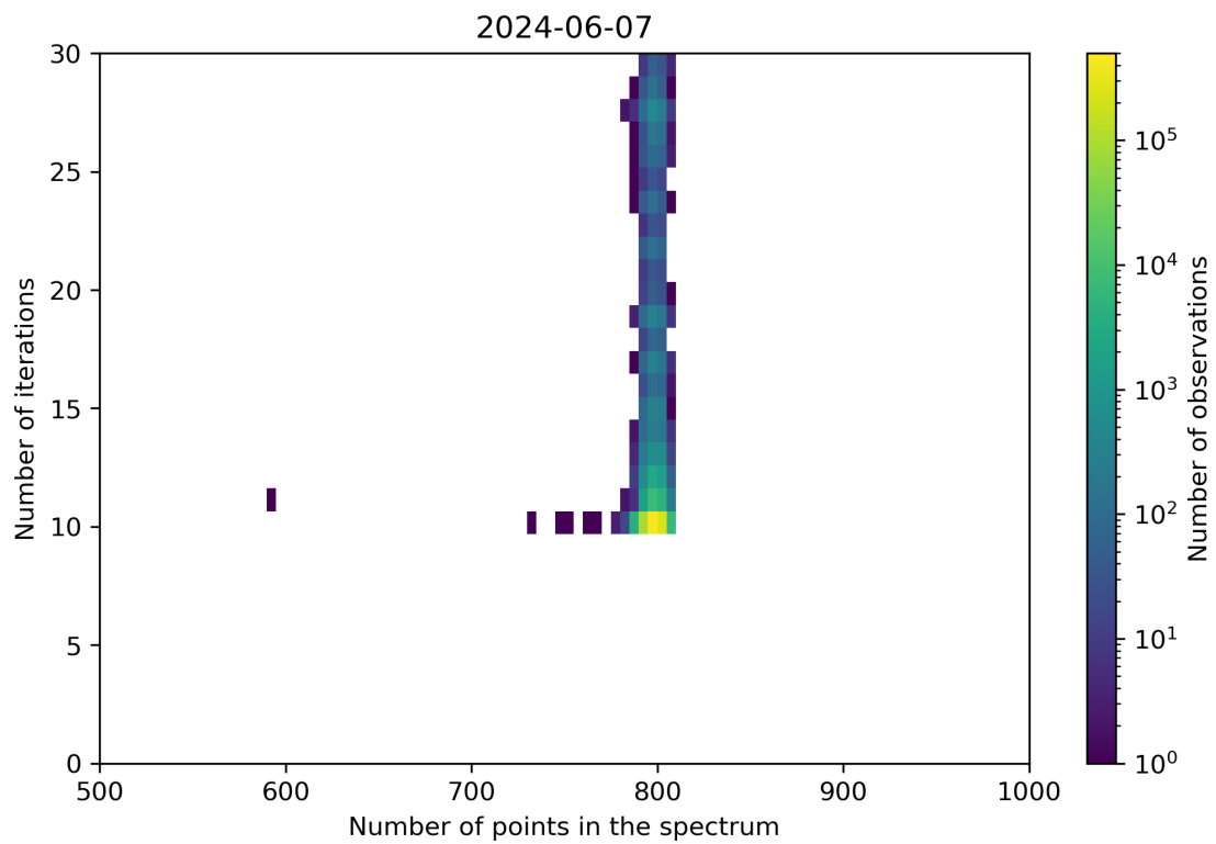
Figure 92: Scatter density plot of “Number of points in the spectrum” against “Number of iterations” for 2024-06-06 to 2024-06-08.
