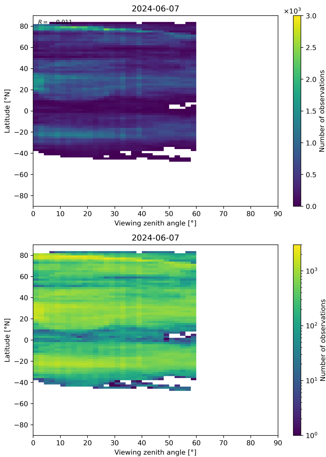
Figure 109: Scatter density plot of “Viewing zenith angle” against “Latitude” for 2024-06-06 to 2024-06-08.
