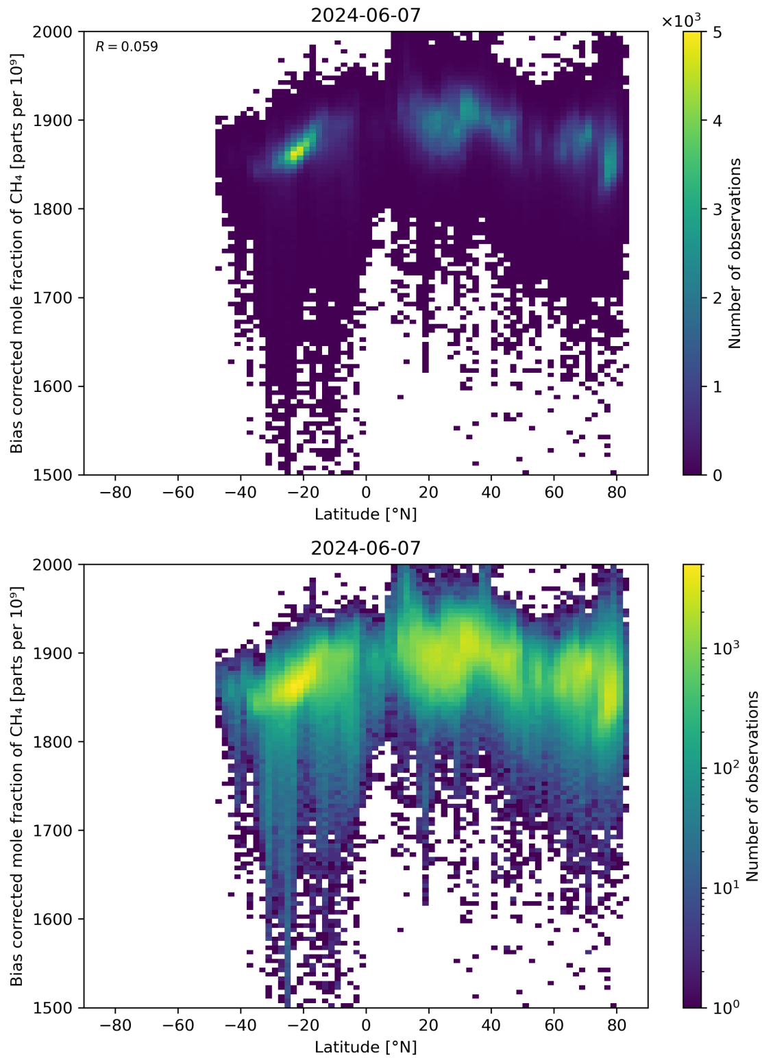
Figure 58: Scatter density plot of “Latitude” against “Bias corrected mole fraction of \text{CH}_4 ” for 2024-06-06 to 2024-06-08.
