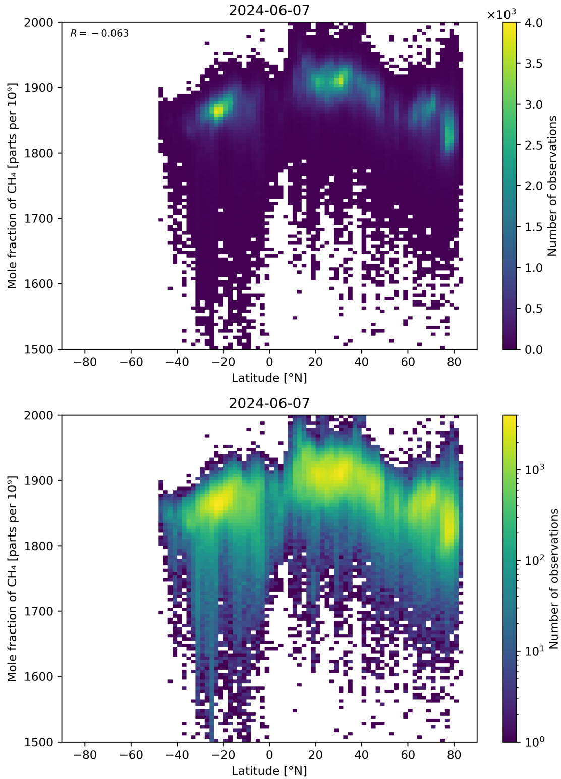
Figure 57: Scatter density plot of “Latitude” against “Mole fraction of \text{CH}_4 ” for 2024-06-06 to 2024-06-08.
