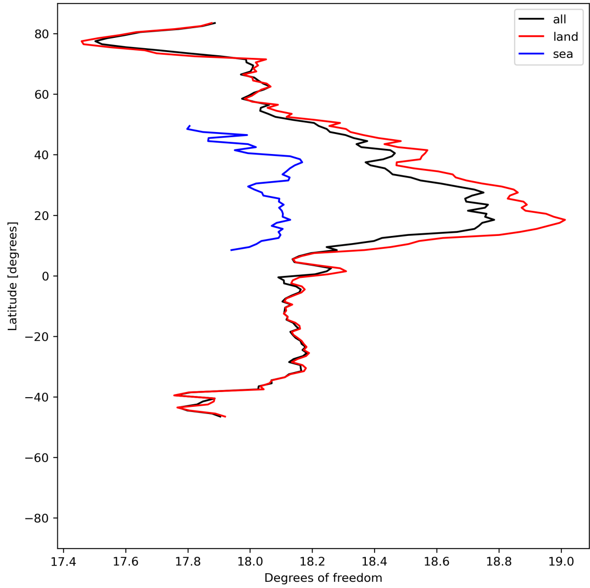
Figure 19: Zonal average of “Degrees of freedom” for 2024-06-06 to 2024-06-08.
