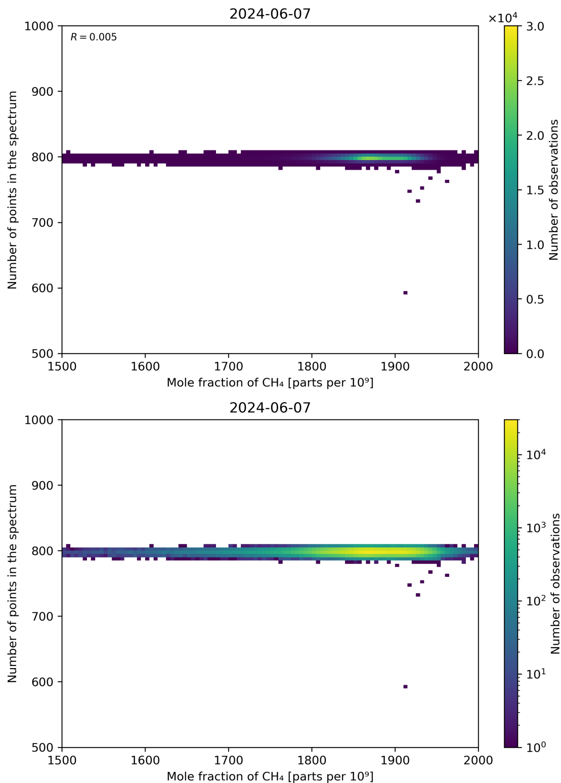
Figure 77: Scatter density plot of “Mole fraction of CH 4 ” against “Number of points in the spectrum” for 2024-06-06 to 2024-06-08.
