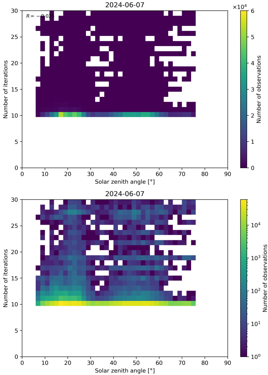
Figure 102: Scatter density plot of “Solar zenith angle” against “Number of iterations” for 2024-06-06 to 2024-06-08.
