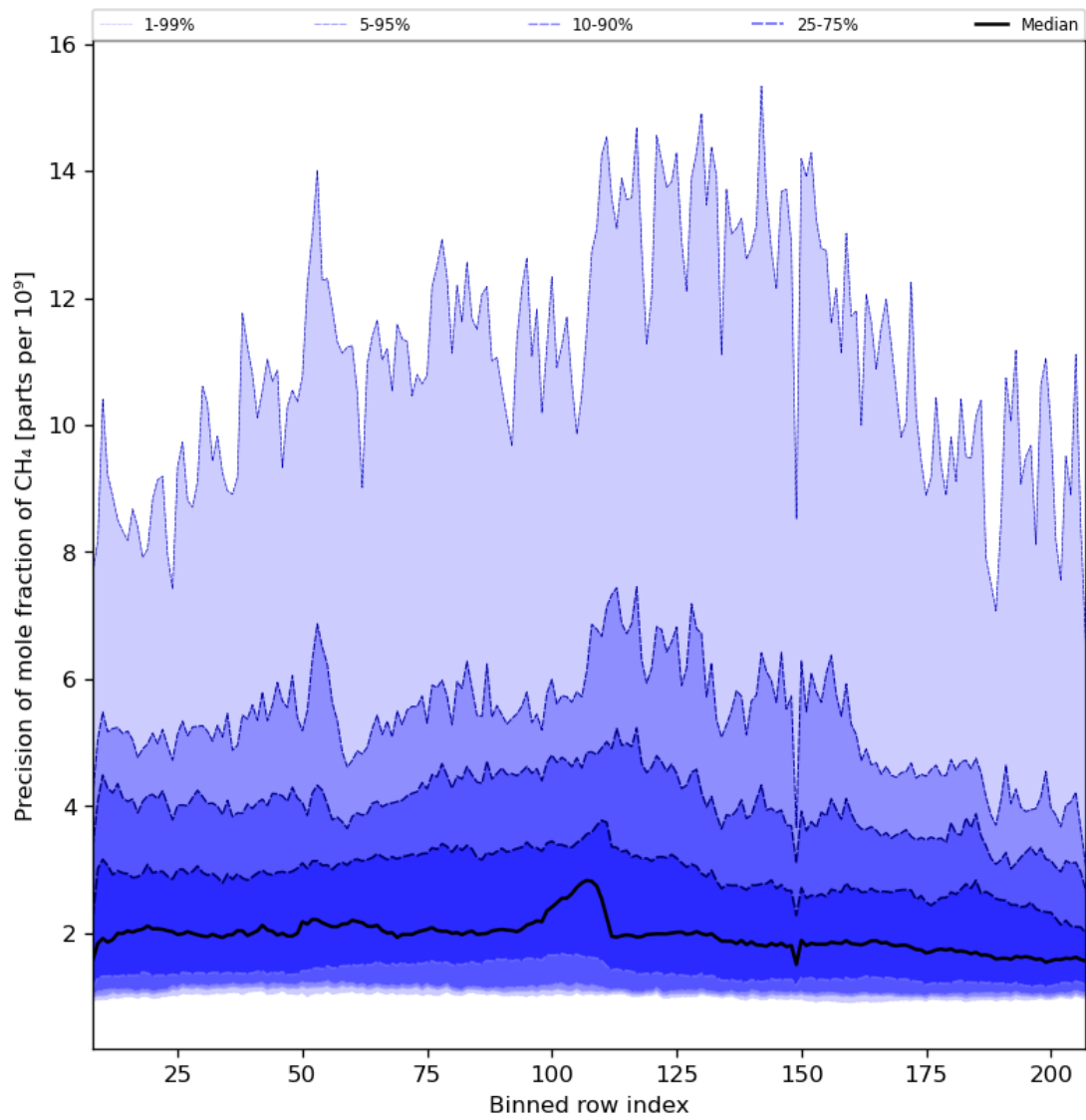
Figure 35: Along track statistics of “Precision of mole fraction of CH 4 ” for 2024-06-06 to 2024-06-08
