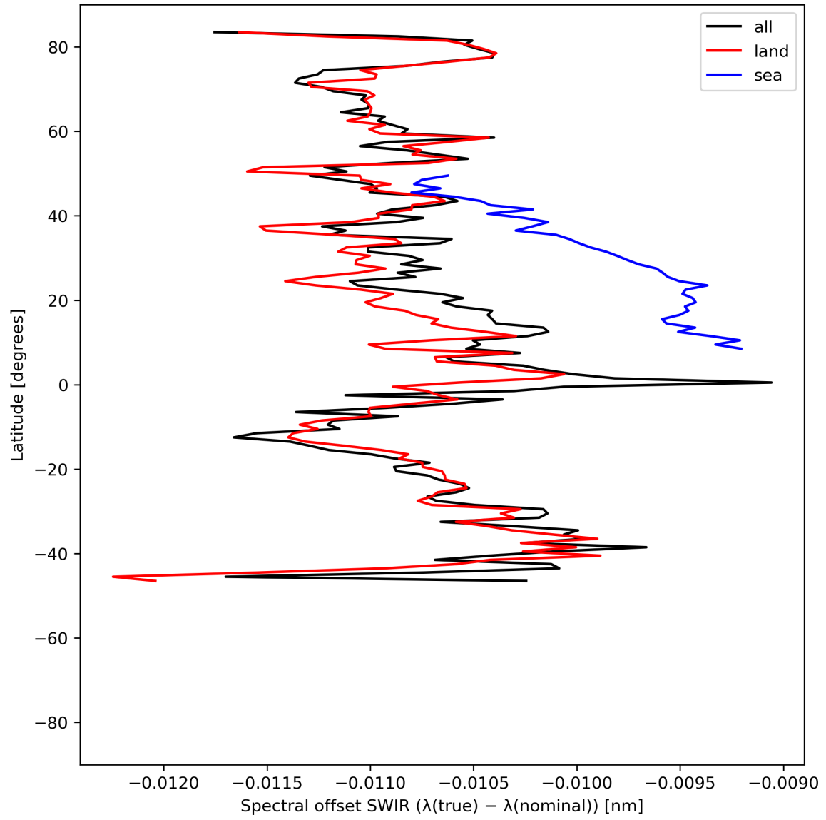
Figure 16: Zonal average of “Spectral offset SWIR ( \lambda(\text{true}) - \lambda(\text{nominal}) )” for 2024-06-06 to 2024-06-08.
