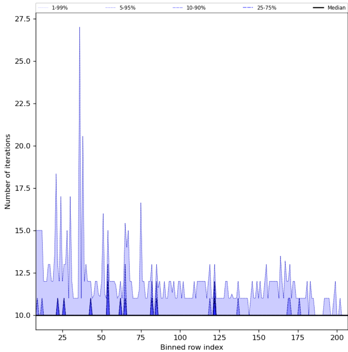
Figure 42: Along track statistics of “Number of iterations” for 2024-06-06 to 2024-06-08
