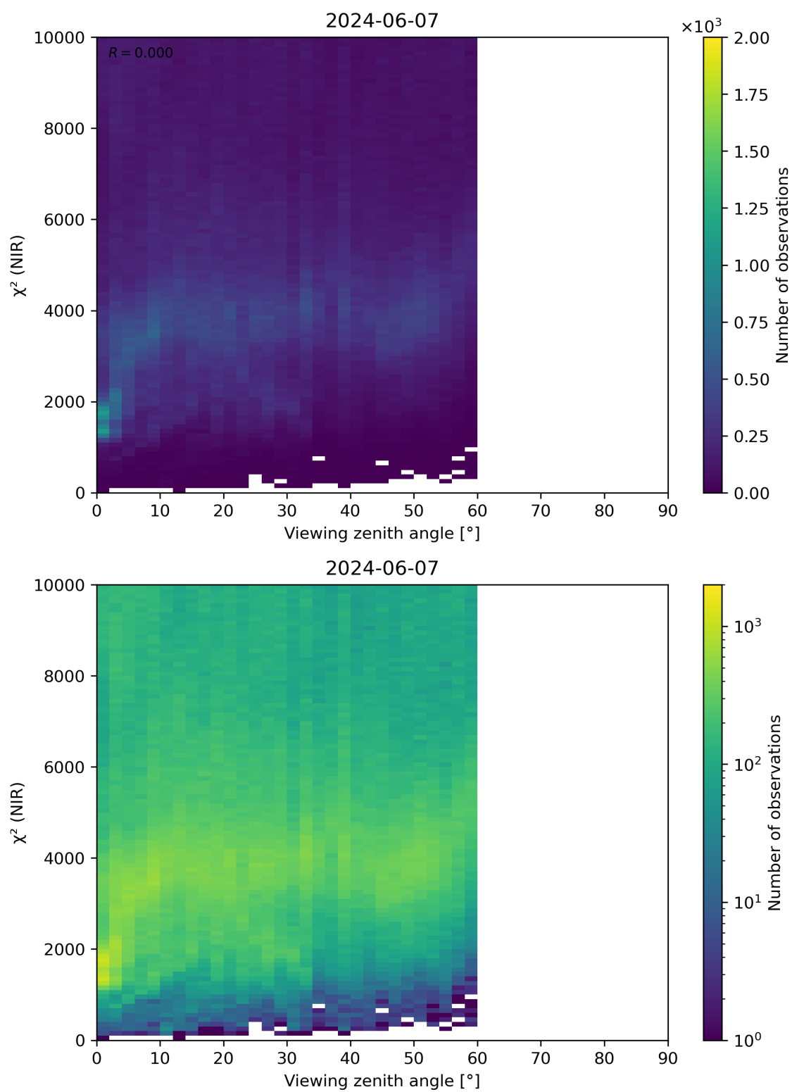
Figure 105: Scatter density plot of “Viewing zenith angle” against “ \chi^2 (NIR)” for 2024-06-06 to 2024-06-08.
