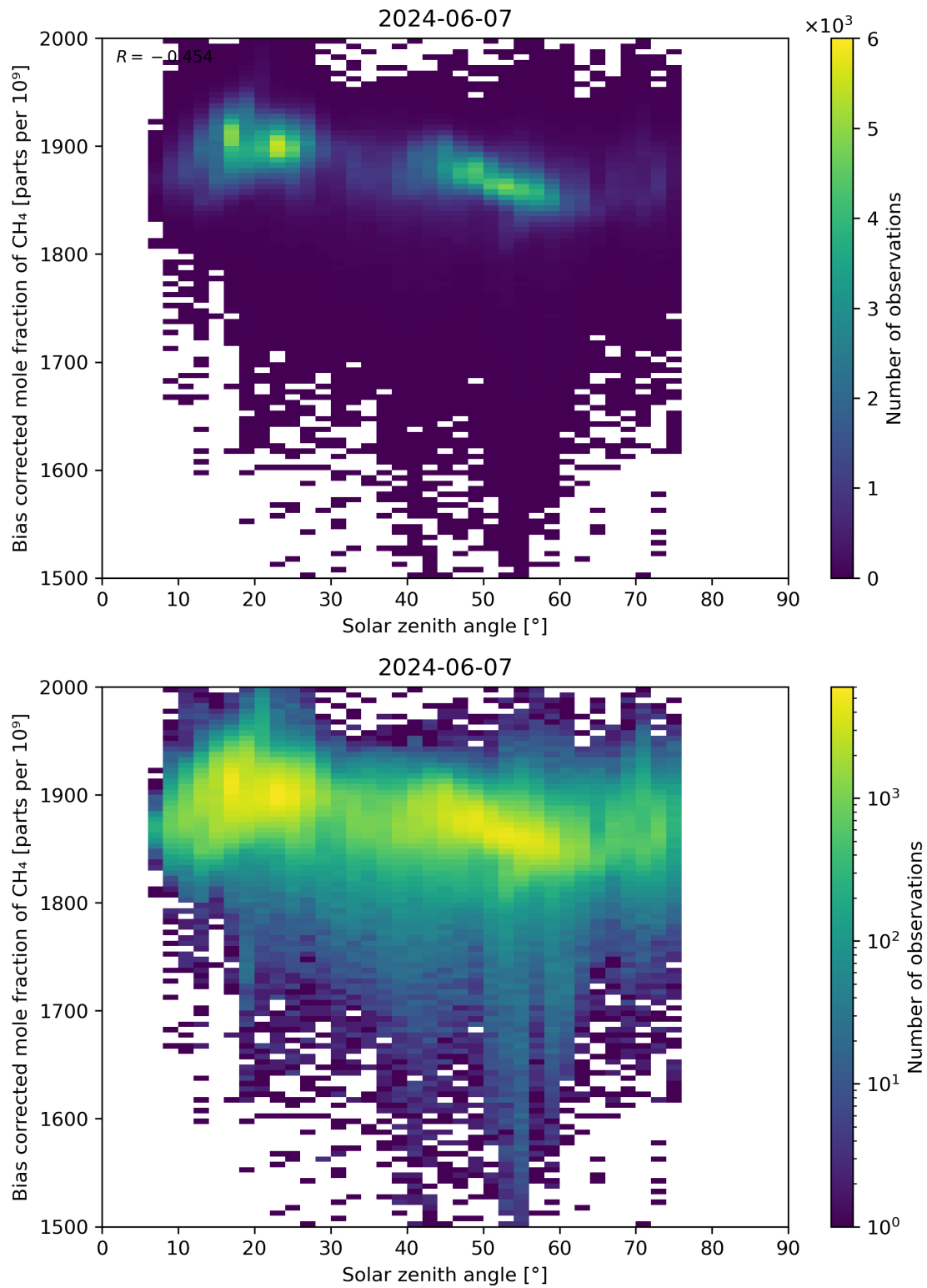
Figure 100: Scatter density plot of “Solar zenith angle” against “Bias corrected mole fraction of CH 4 ” for 2024-06-06 to 2024-06-08.
