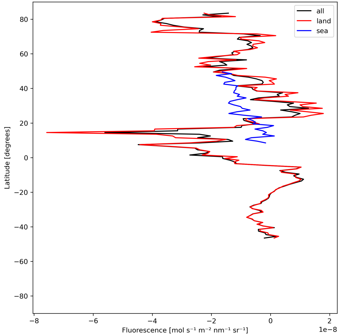
Figure 21: Zonal average of “Fluorescence” for 2024-06-06 to 2024-06-08.
