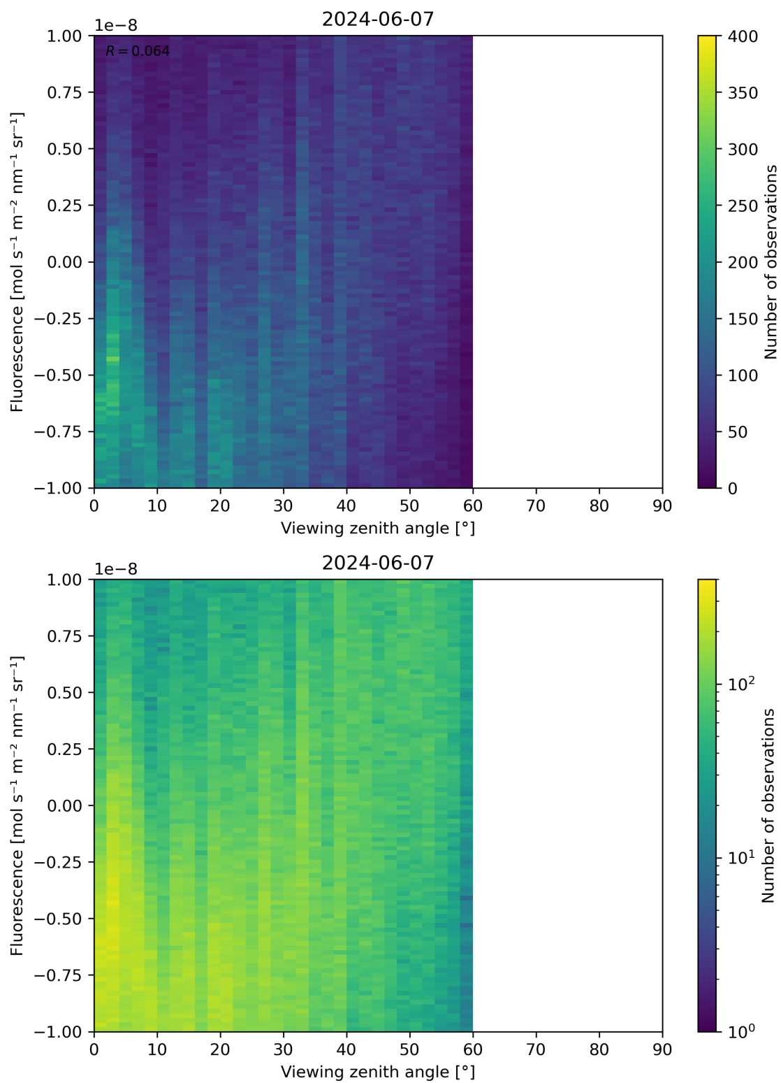
Figure 108: Scatter density plot of “Viewing zenith angle” against “Fluorescence” for 2024-06-06 to 2024-06-08.
