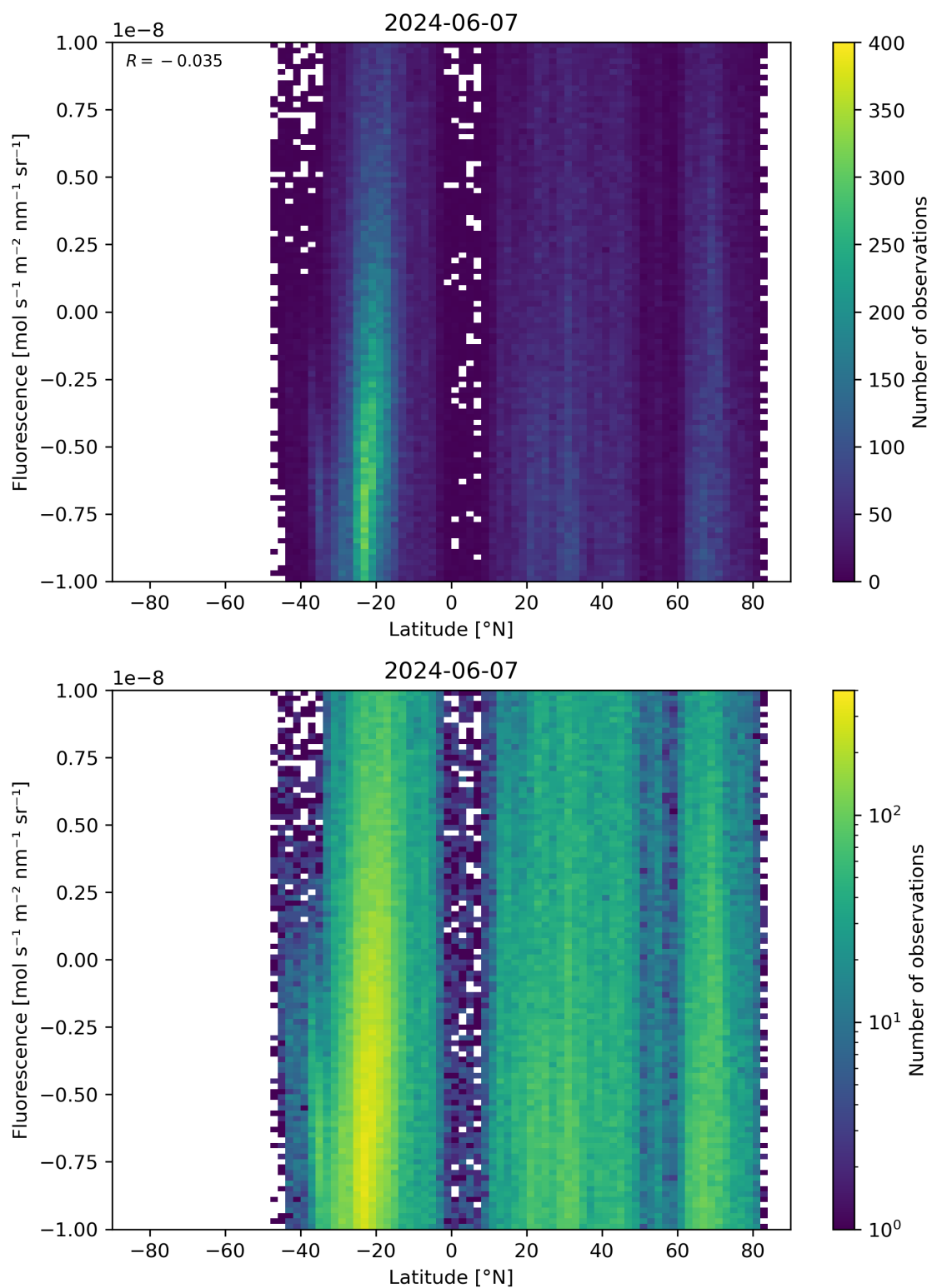
Figure 56: Scatter density plot of “Latitude” against “Fluorescence” for 2024-06-06 to 2024-06-08.
