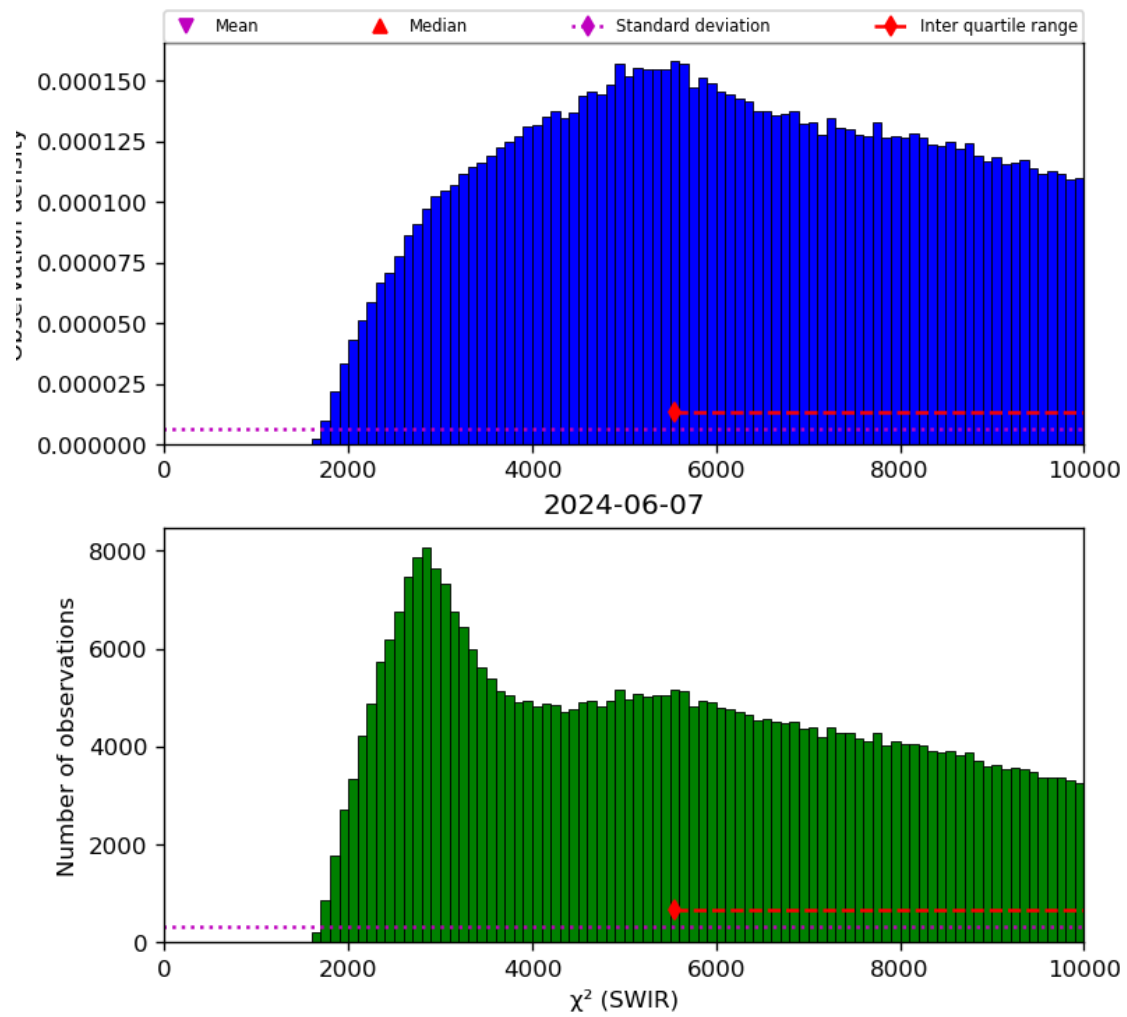
Figure 28: Histogram of “ \chi^2 (SWIR)” for 2024-06-06 to 2024-06-08
