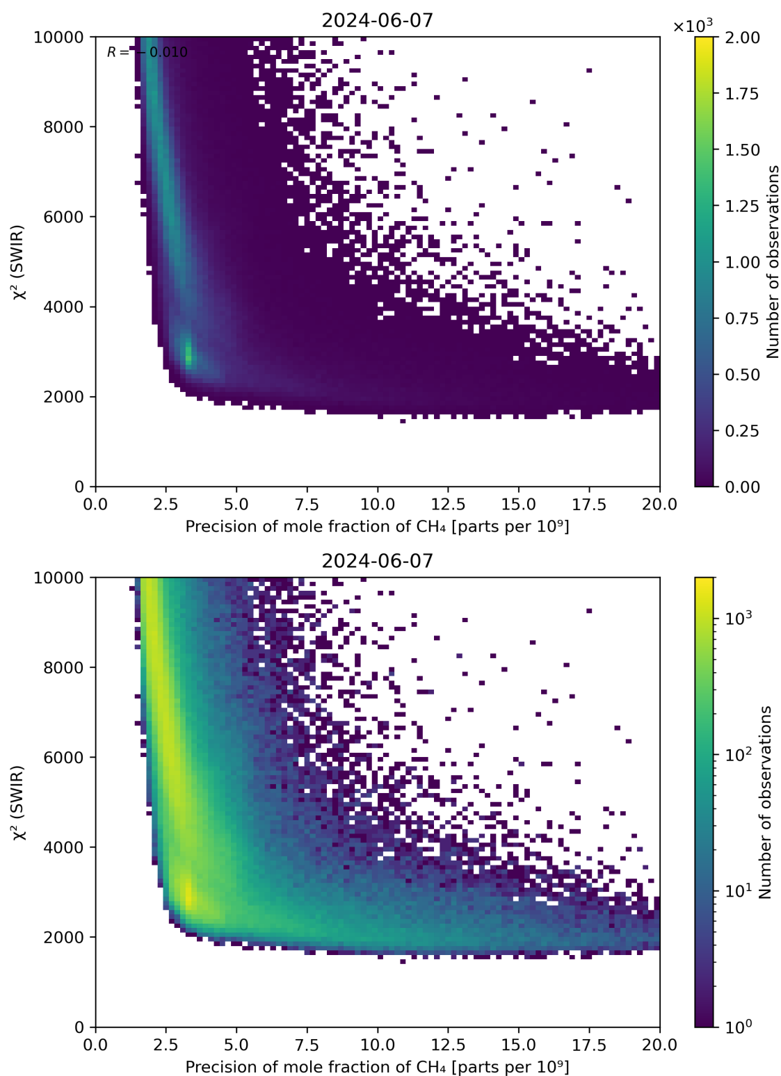
Figure 79: Scatter density plot of “Precision of mole fraction of CH 4 ” against “ \chi^2 (SWIR)” for 2024-06-06 to 2024-06-08.
