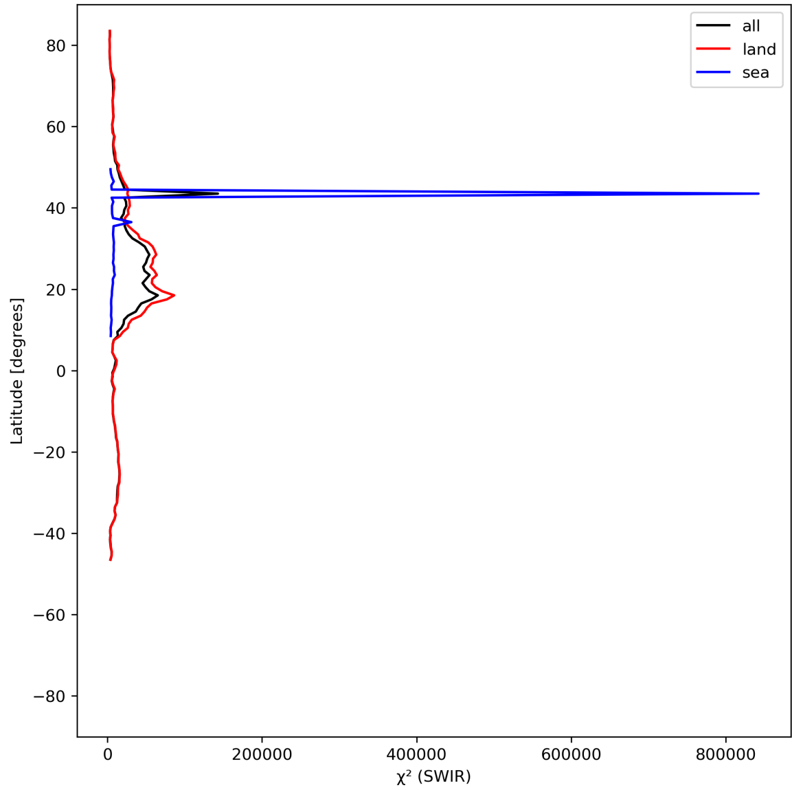
Figure 17: Zonal average of “ \chi^2 (SWIR)” for 2024-06-06 to 2024-06-08.
