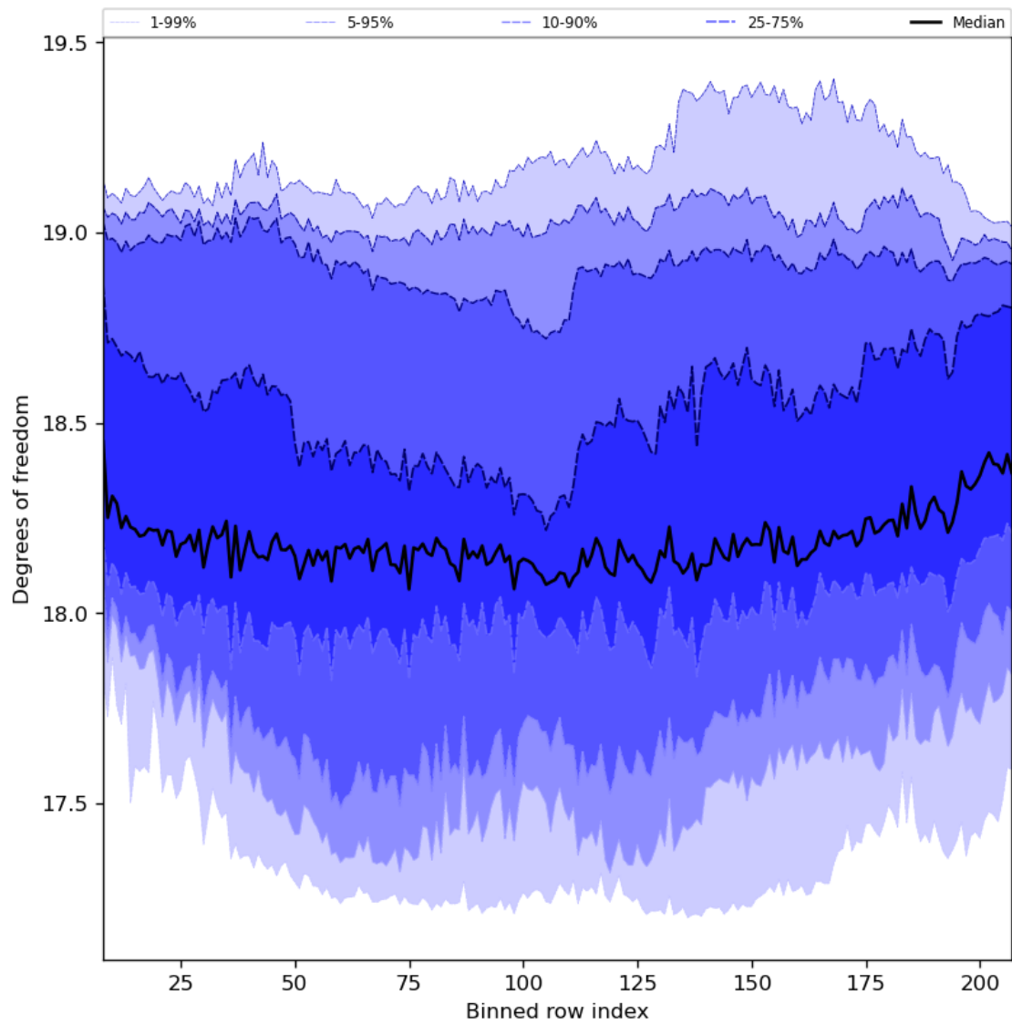
Figure 41: Along track statistics of “Degrees of freedom” for 2024-06-06 to 2024-06-08
