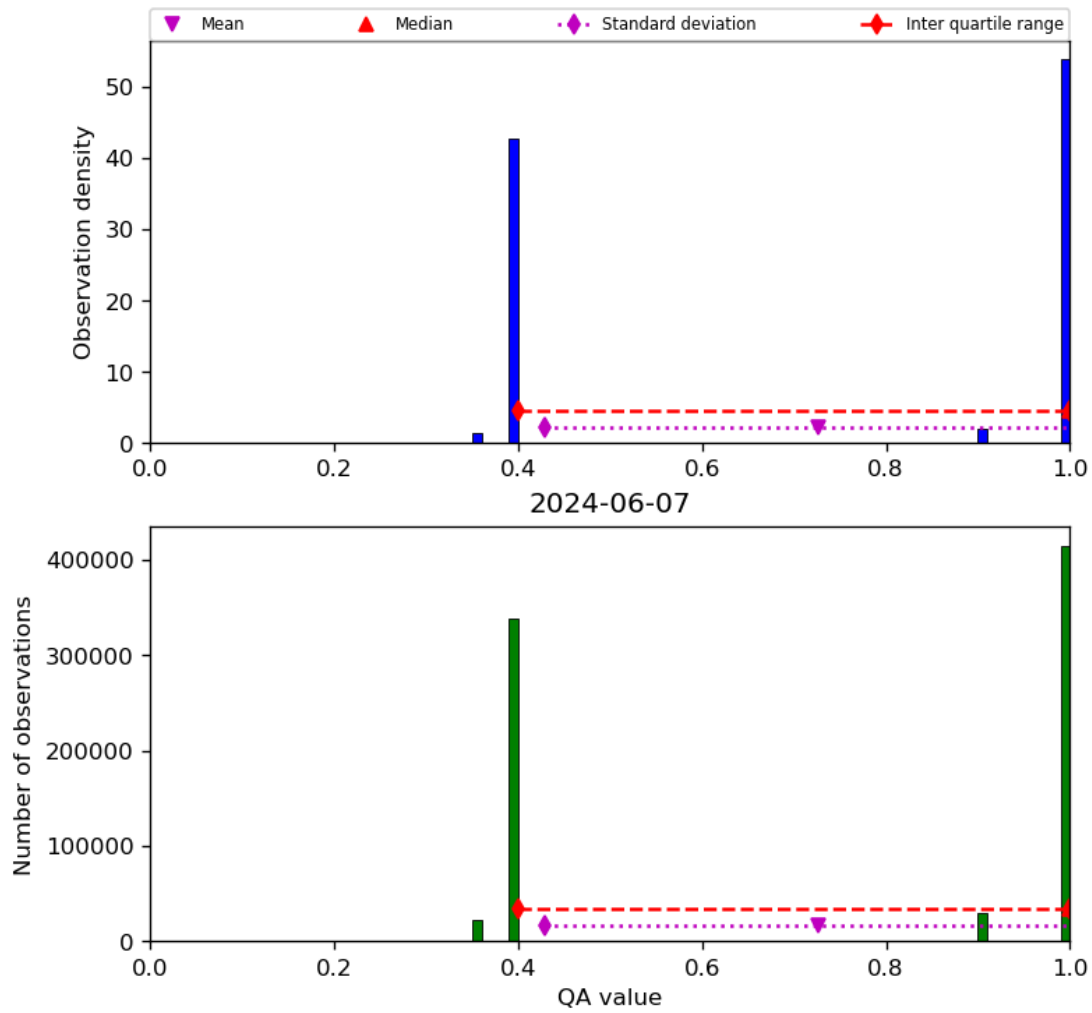
Figure 22: Histogram of “QA value” for 2024-06-06 to 2024-06-08
