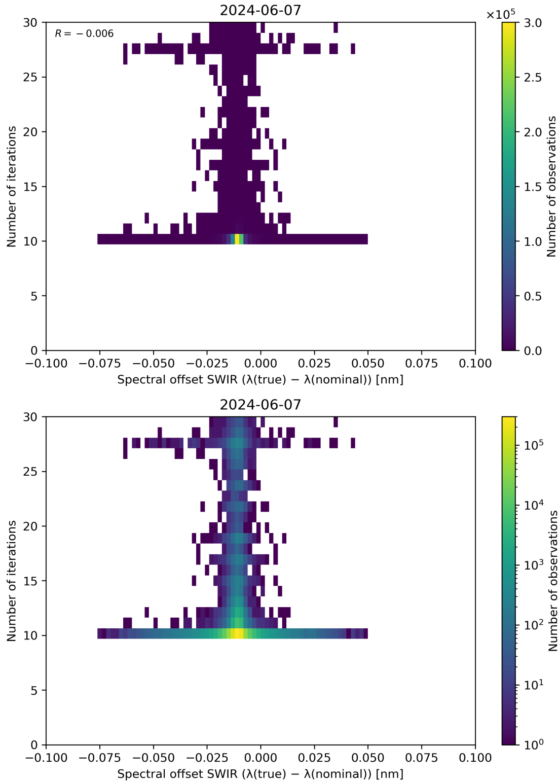
Figure 121: Scatter density plot of “Spectral offset SWIR ( \lambda(\text{true}) - \lambda(\text{nominal}) )” against “Number of iterations” for 2024-06-06 to 2024-06-08.
