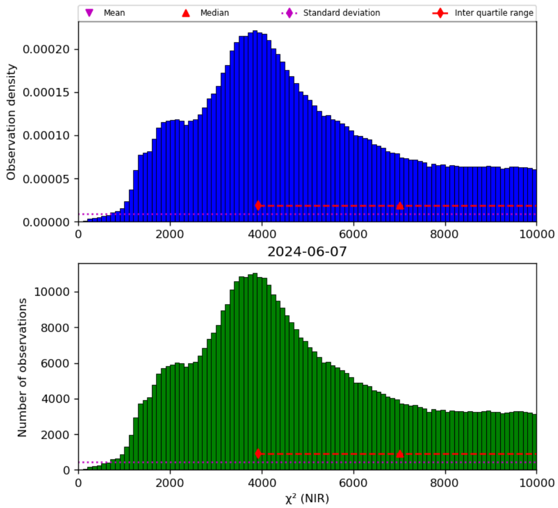
Figure 29: Histogram of “ \chi^2 (NIR)” for 2024-06-06 to 2024-06-08
