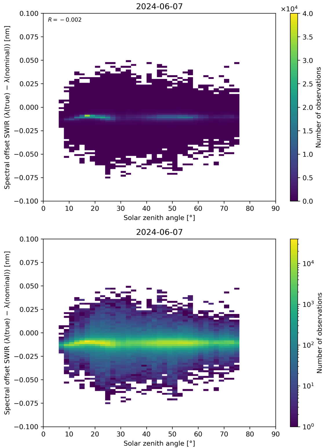
Figure 104: Scatter density plot of “Solar zenith angle” against “Spectral offset SWIR ( \lambda(\text{true}) - \lambda(\text{nominal}) )” for 2024-06-06 to 2024-06-08.
