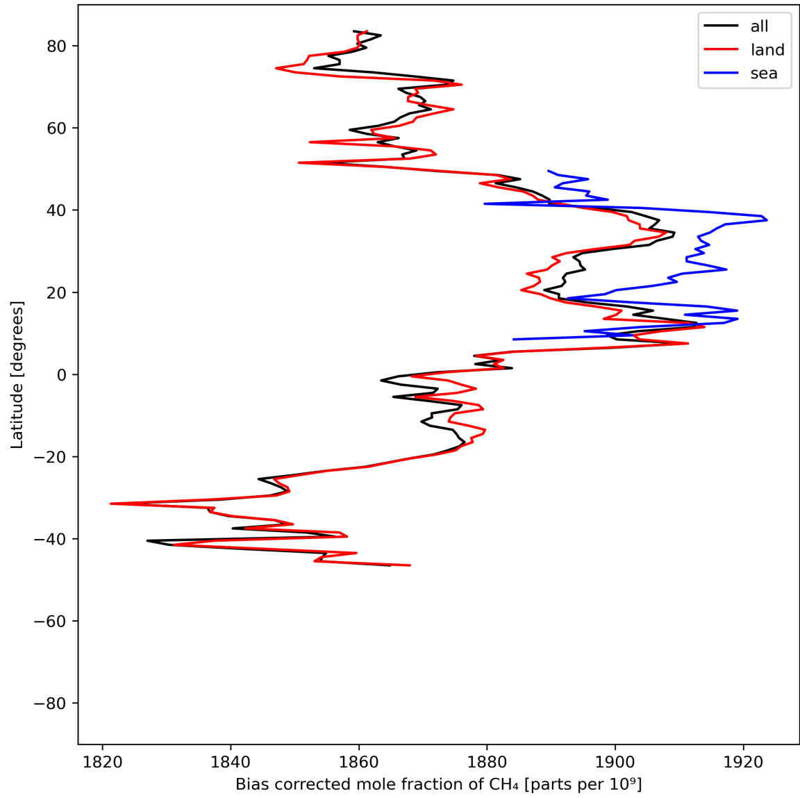
Figure 14: Zonal average of “Bias corrected mole fraction of CH 4 ” for 2024-06-06 to 2024-06-08.
