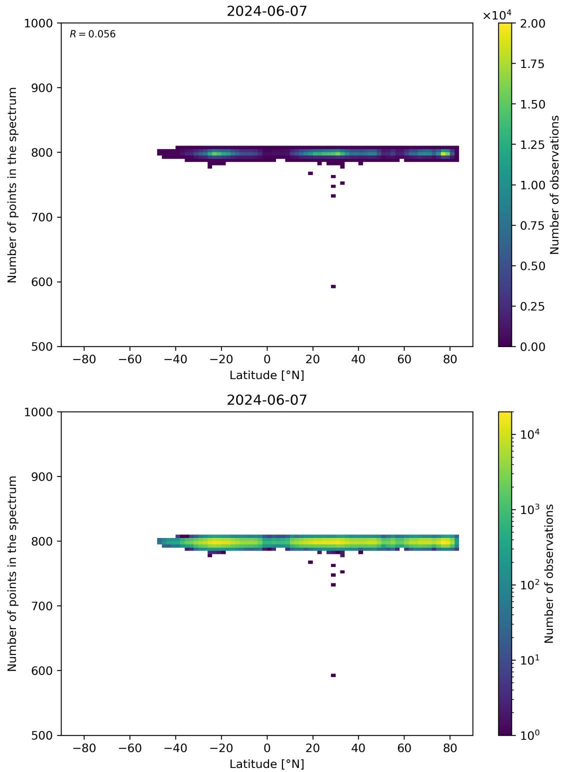
Figure 61: Scatter density plot of “Latitude” against “Number of points in the spectrum” for 2024-06-06 to 2024-06-08.
