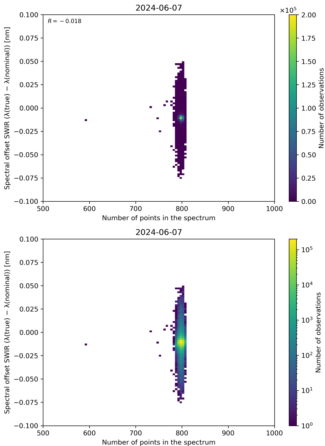
Figure 93: Scatter density plot of “Number of points in the spectrum” against “Spectral offset SWIR ( \lambda(\text{true}) - \lambda(\text{nominal}) )” for 2024-06-06 to 2024-06-08.
