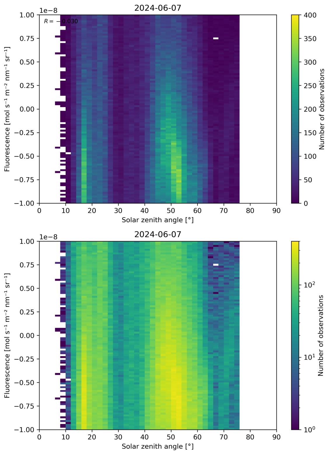
Figure 97: Scatter density plot of “Solar zenith angle” against “Fluorescence” for 2024-06-06 to 2024-06-08.
