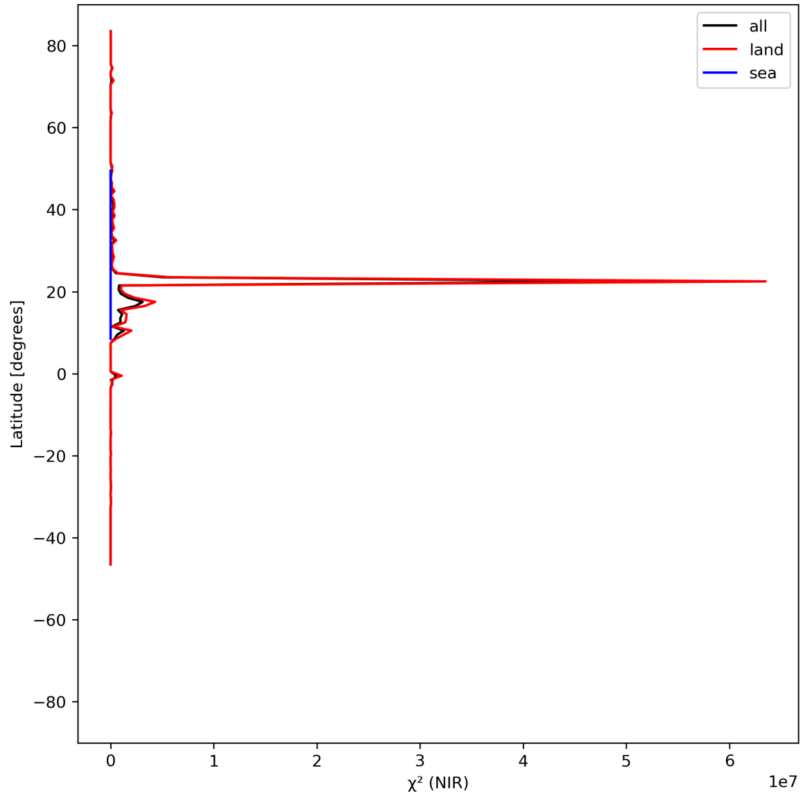
Figure 18: Zonal average of “ \chi^2 (NIR)” for 2024-06-06 to 2024-06-08.
