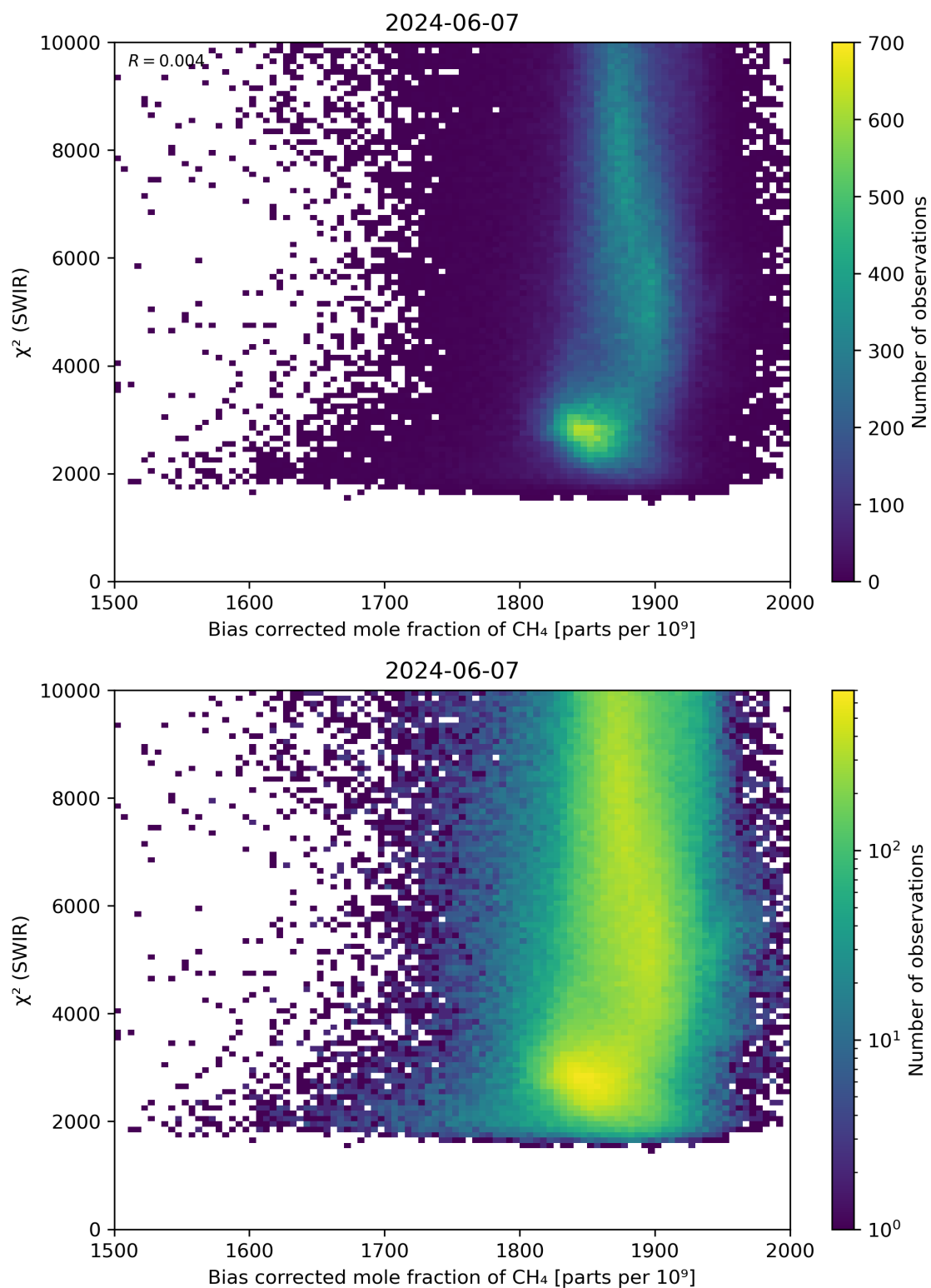
Figure 64: Scatter density plot of “Bias corrected mole fraction of \text{CH}_4 ” against “ \chi^2 (SWIR)” for 2024-06-06 to 2024-06-08.
