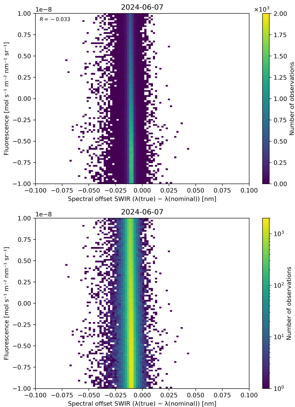
Figure 120: Scatter density plot of “Spectral offset SWIR ( \lambda(\text{true}) - \lambda(\text{nominal}) )” against “Fluorescence” for 2024-06-06 to 2024-06-08.
