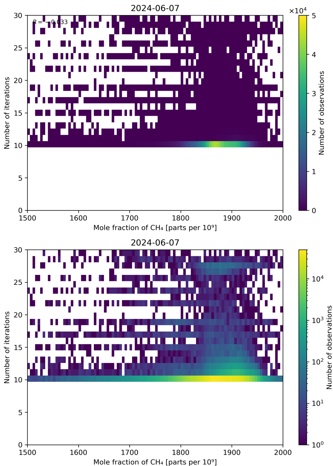
Figure 76: Scatter density plot of “Mole fraction of CH 4 ” against “Number of iterations” for 2024-06-06 to 2024-06-08.
