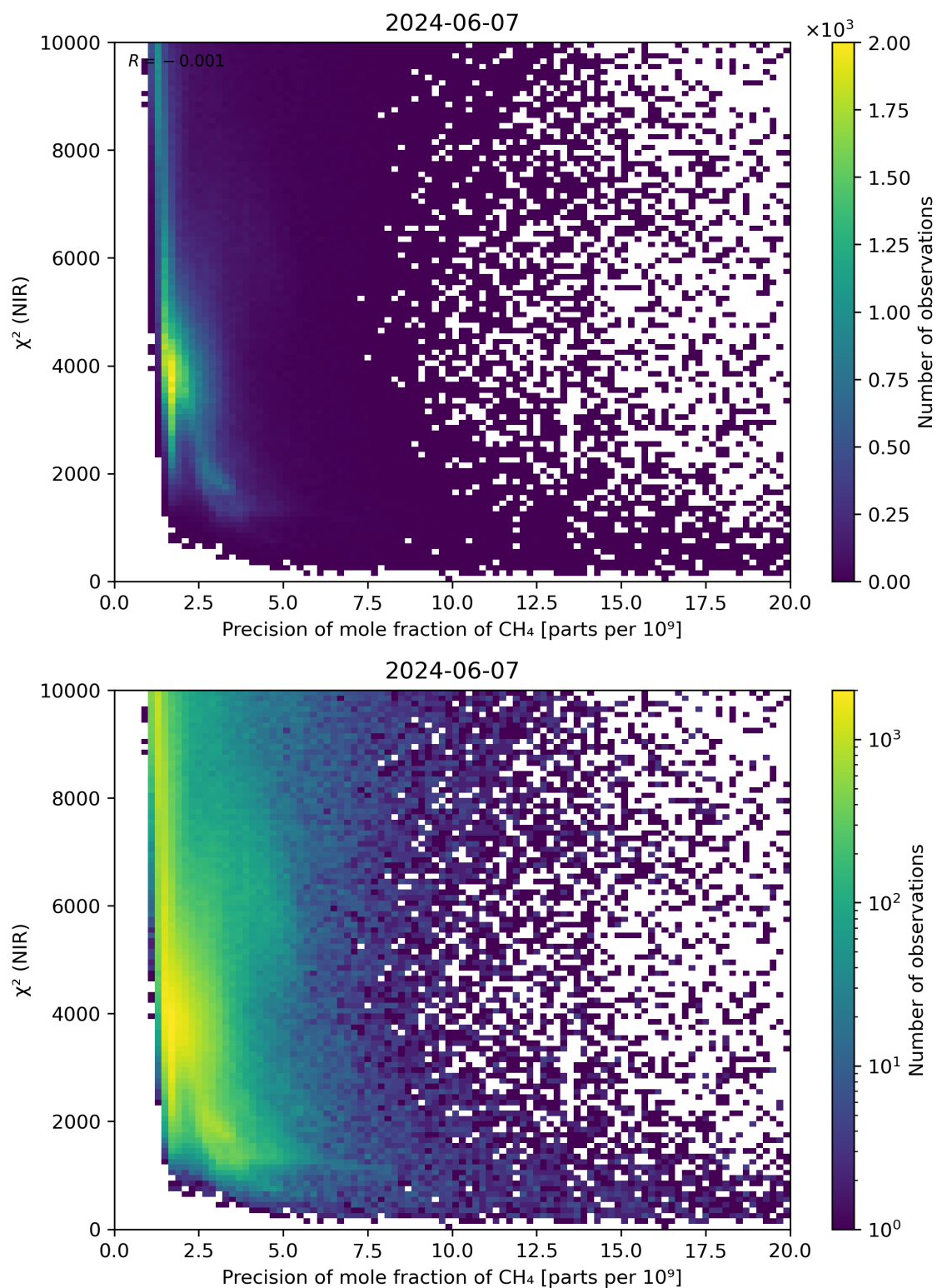
Figure 78: Scatter density plot of “Precision of mole fraction of \text{CH}_4 ” against “ \chi^2 (NIR)” for 2024-06-06 to 2024-06-08.
