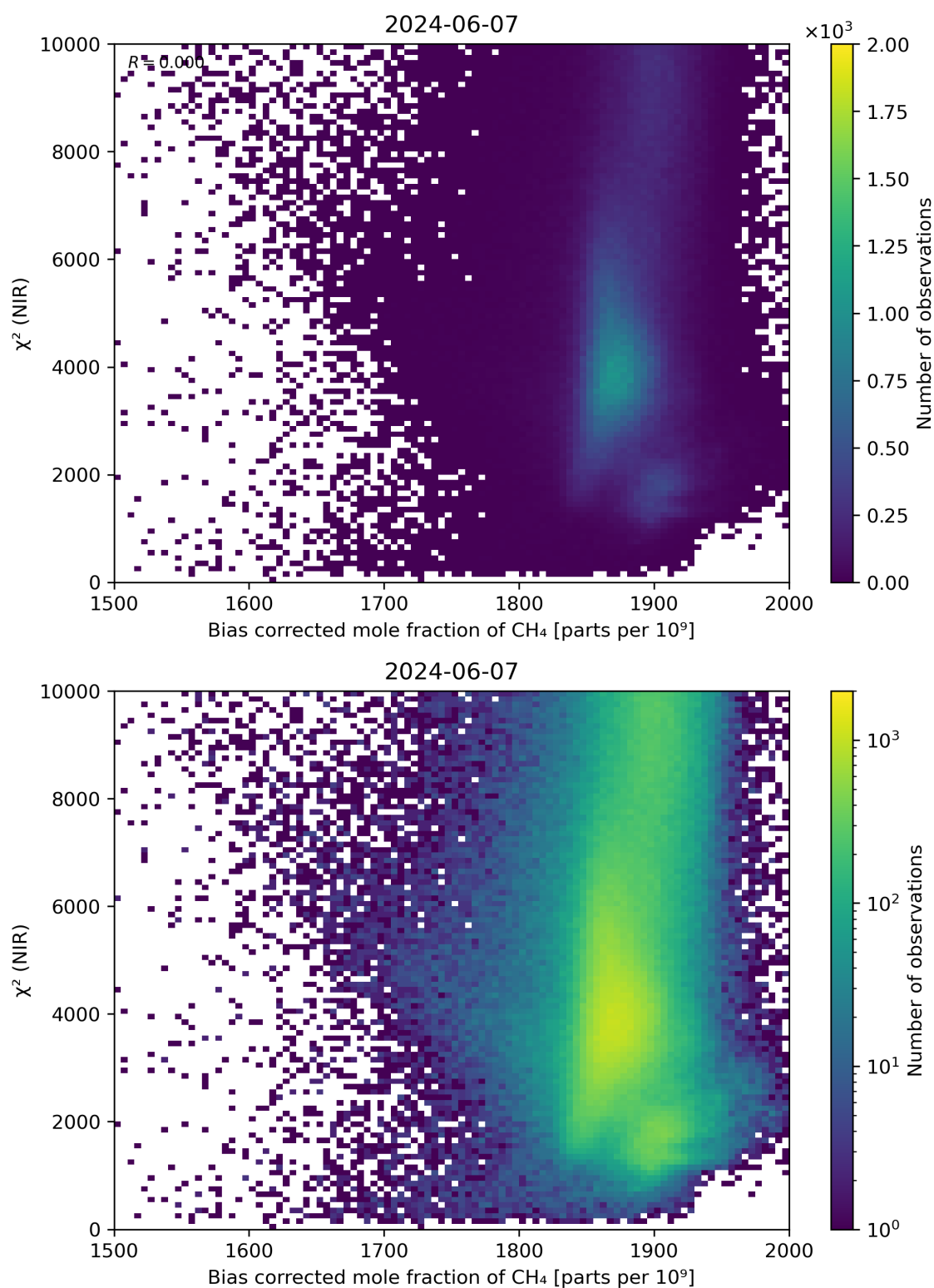
Figure 63: Scatter density plot of “Bias corrected mole fraction of CH 4 ” against “ \chi^2 (NIR)” for 2024-06-06 to 2024-06-08.
