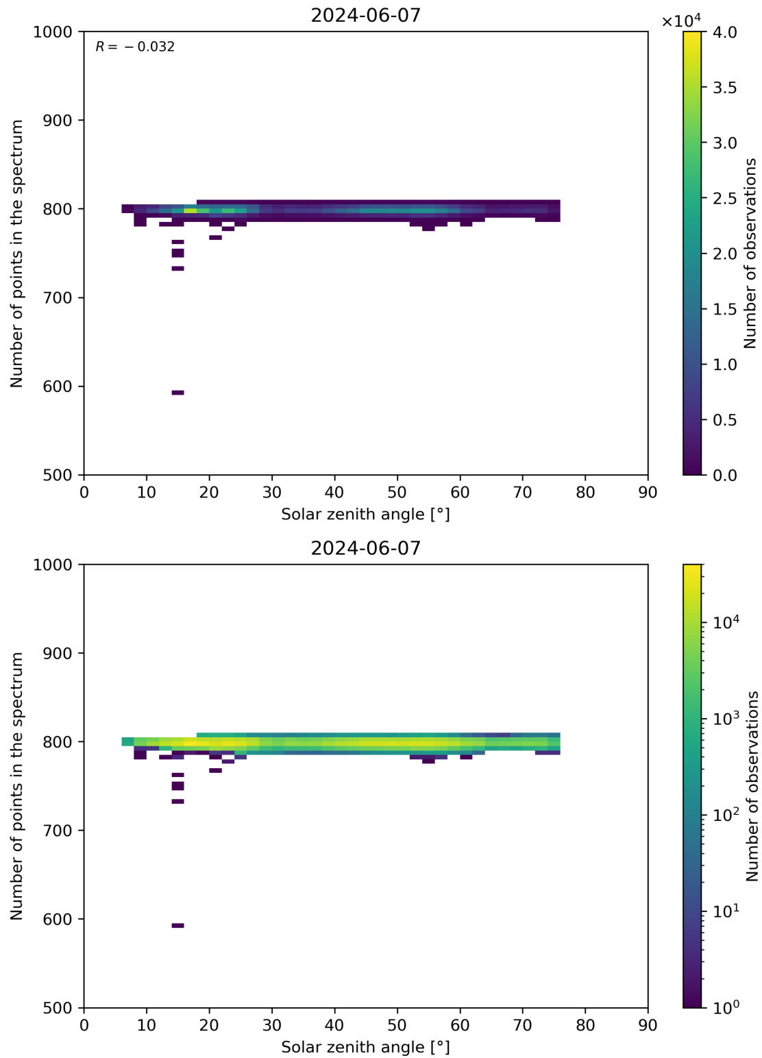
Figure 103: Scatter density plot of “Solar zenith angle” against “Number of points in the spectrum” for 2024-06-06 to 2024-06-08.
