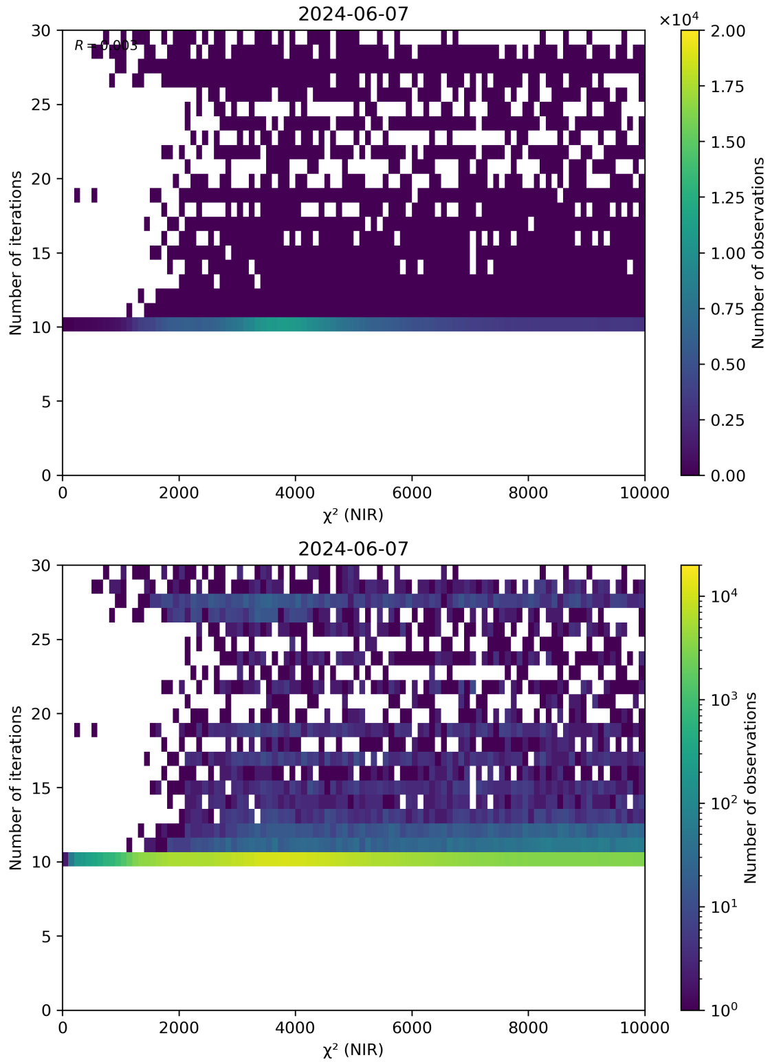
Figure 46: Scatter density plot of “ \chi^2 (NIR)” against “Number of iterations” for 2024-06-06 to 2024-06-08.
