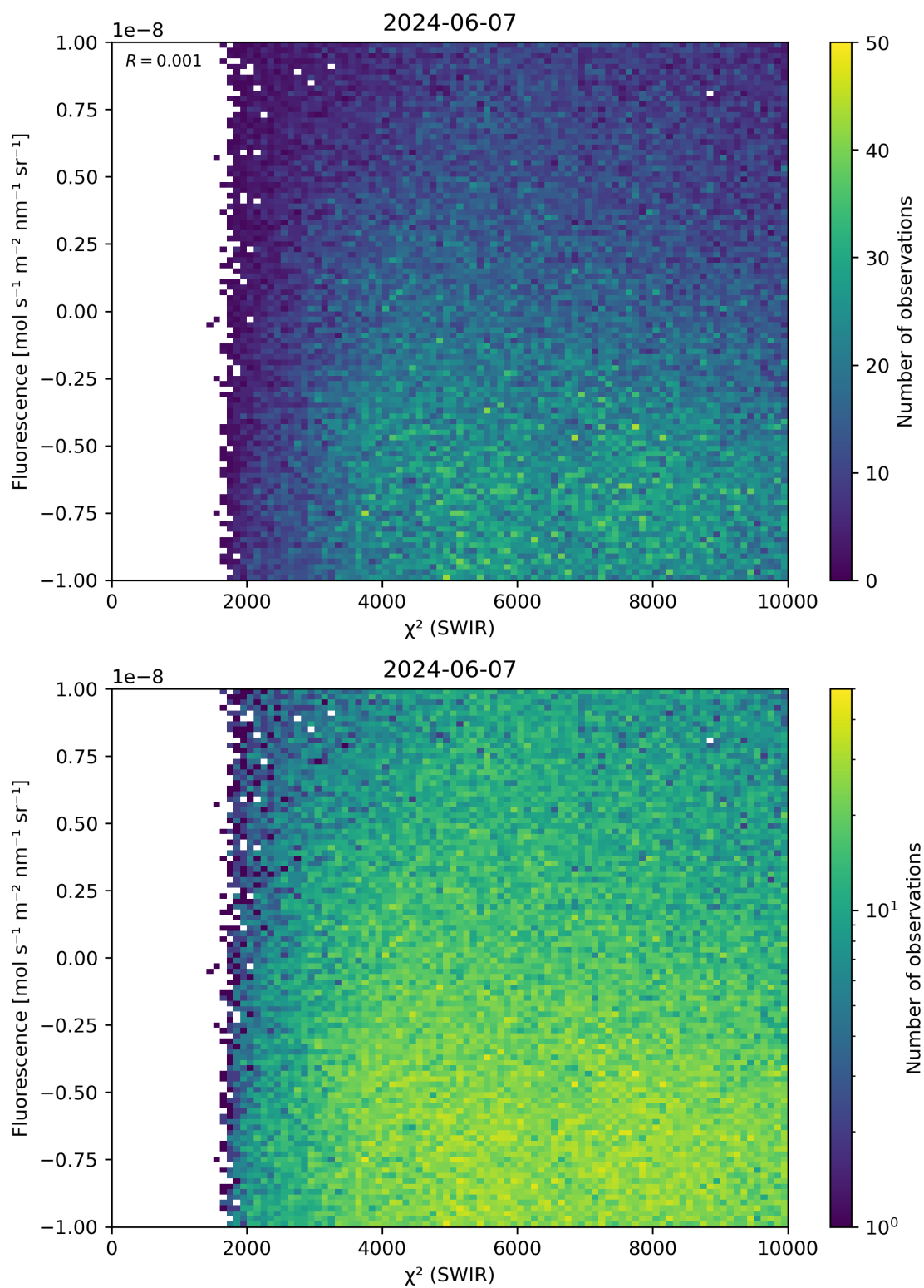
Figure 49: Scatter density plot of “ \chi^2 (SWIR)” against “Fluorescence” for 2024-06-06 to 2024-06-08.
