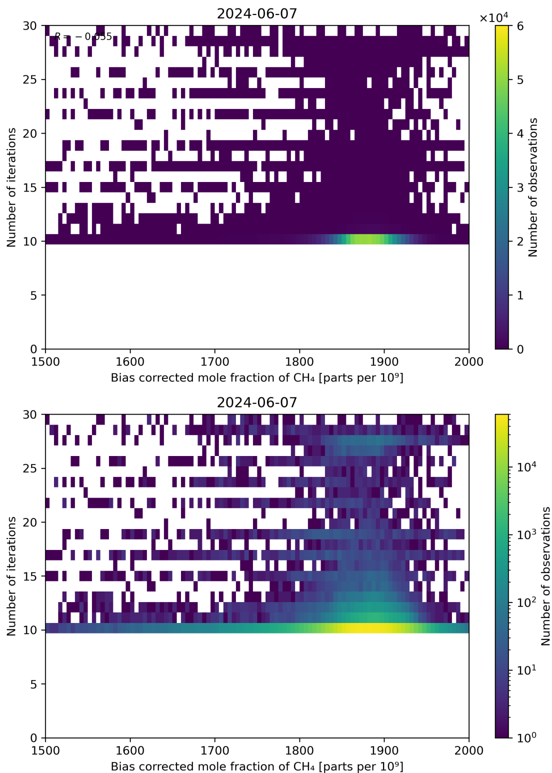
Figure 67: Scatter density plot of “Bias corrected mole fraction of CH 4 ” against “Number of iterations” for 2024-06-06 to 2024-06-08.
