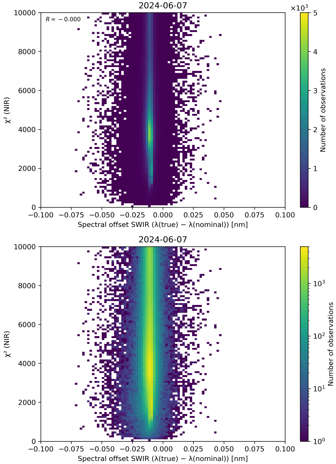
Figure 117: Scatter density plot of “Spectral offset SWIR ( \lambda(\text{true}) - \lambda(\text{nominal}) )” against “ \chi^2 (NIR)” for 2024-06-06 to 2024-06-08.
