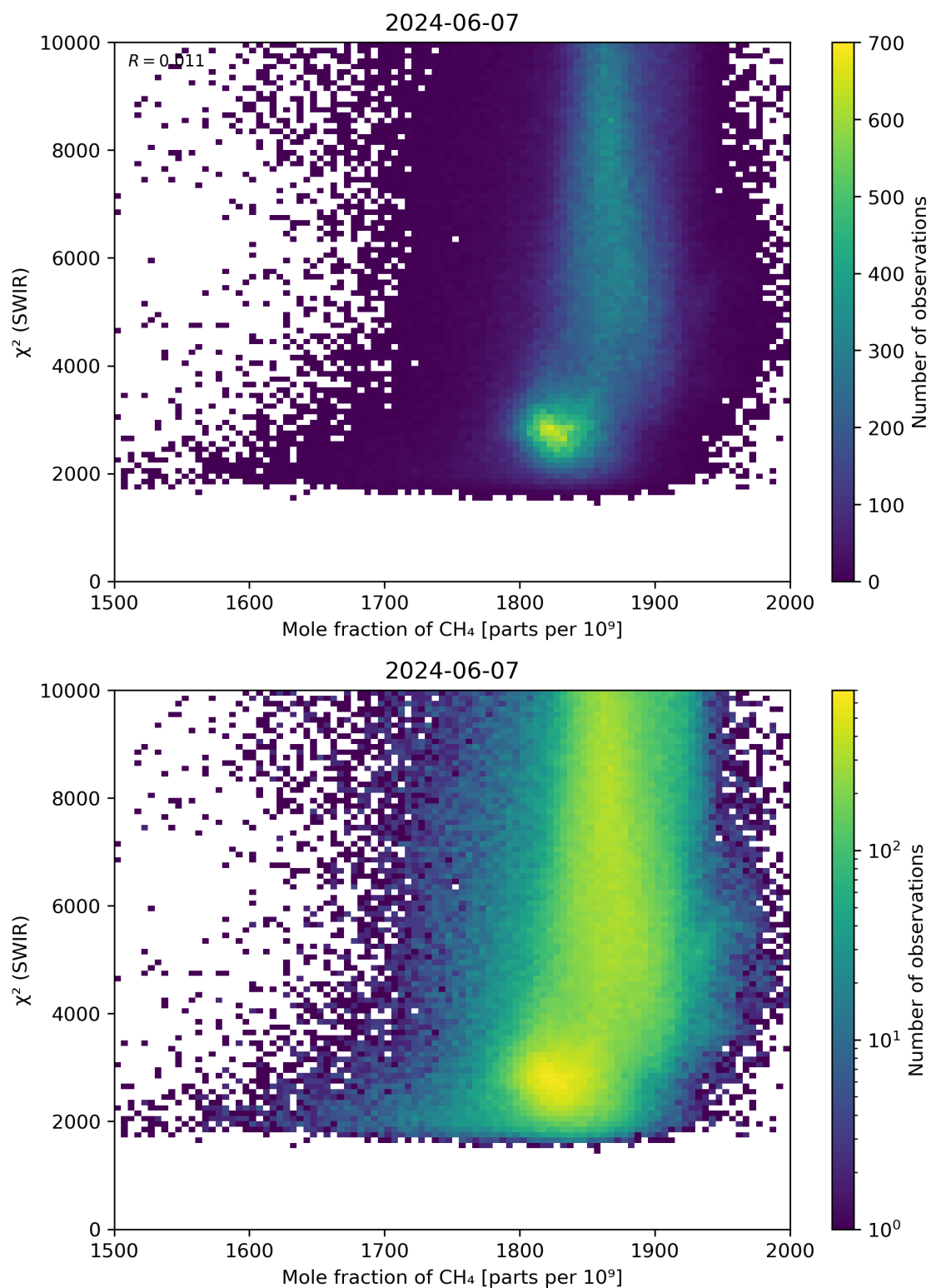
Figure 71: Scatter density plot of “Mole fraction of \text{CH}_4 ” against “ \chi^2 (SWIR)” for 2024-06-06 to 2024-06-08.
