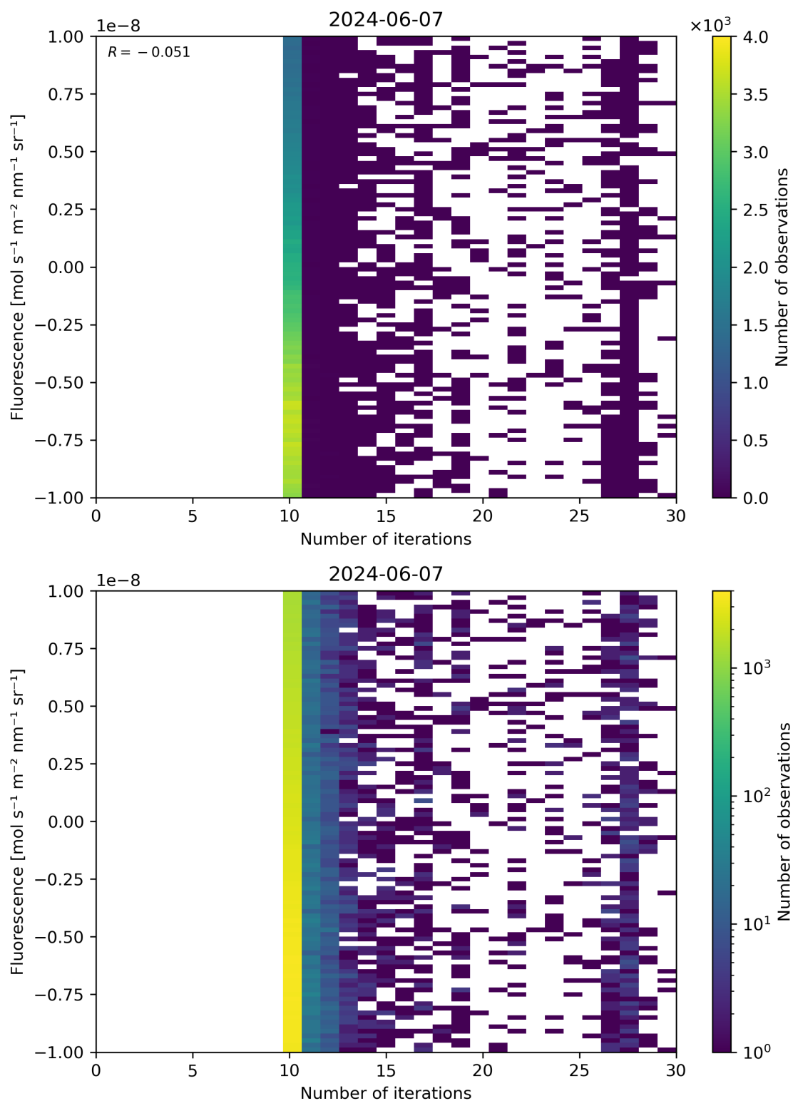
Figure 87: Scatter density plot of “Number of iterations” against “Fluorescence” for 2024-06-06 to 2024-06-08.
