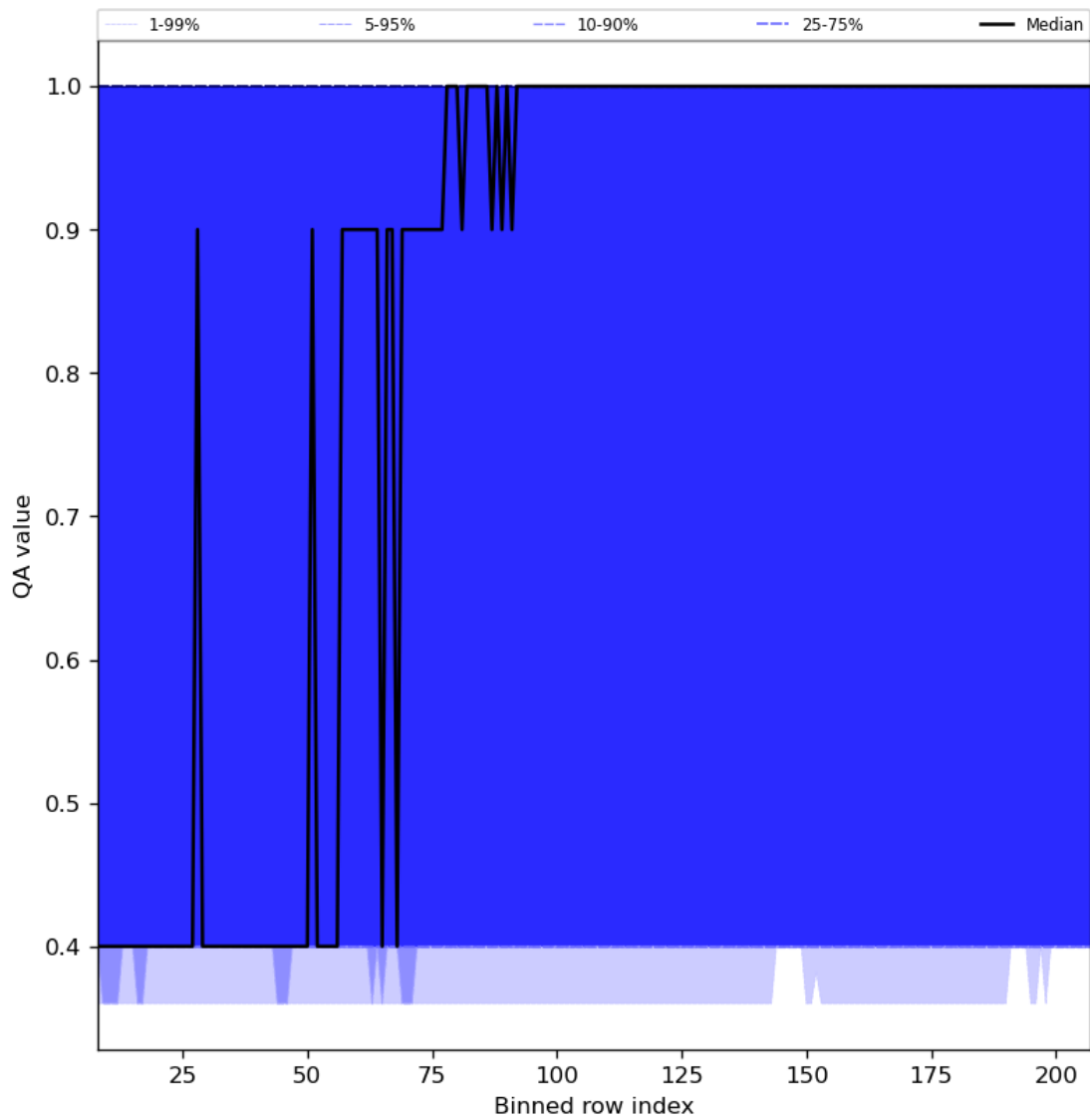
Figure 33: Along track statistics of “QA value” for 2024-06-06 to 2024-06-08
