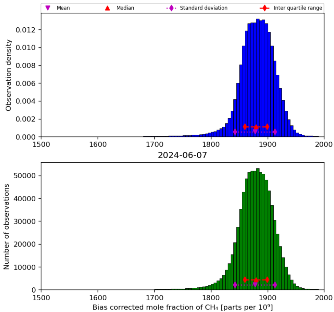
Figure 25: Histogram of “Bias corrected mole fraction of CH 4 ” for 2024-06-06 to 2024-06-08
