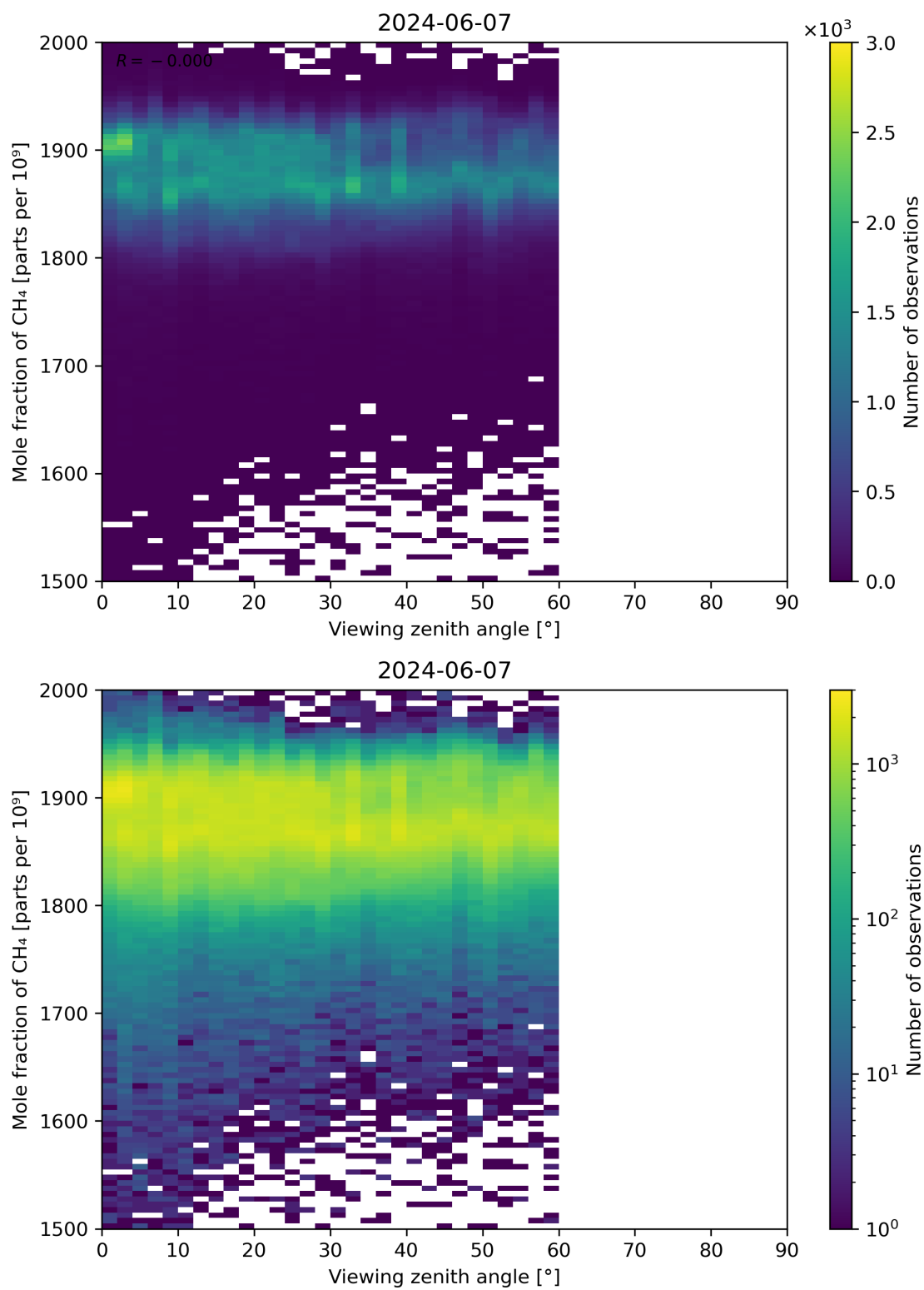
Figure 110: Scatter density plot of “Viewing zenith angle” against “Mole fraction of CH 4 ” for 2024-06-06 to 2024-06-08.
