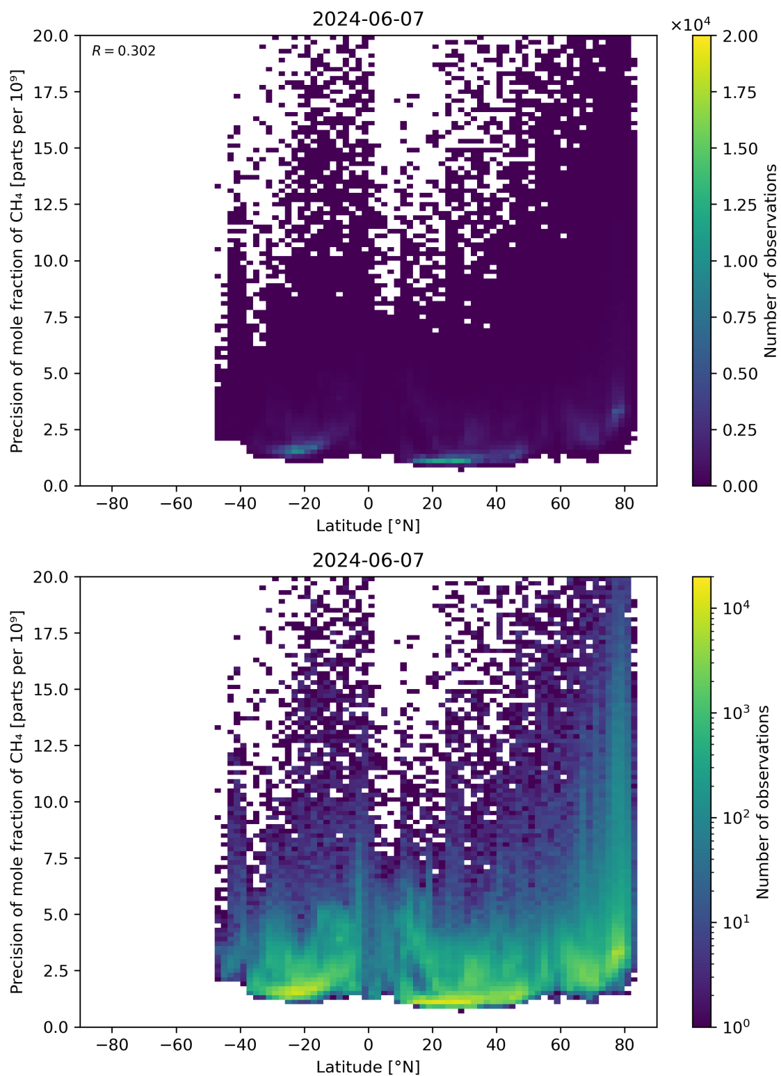
Figure 59: Scatter density plot of “Latitude” against “Precision of mole fraction of \text{CH}_4 ” for 2024-06-06 to 2024-06-08.
