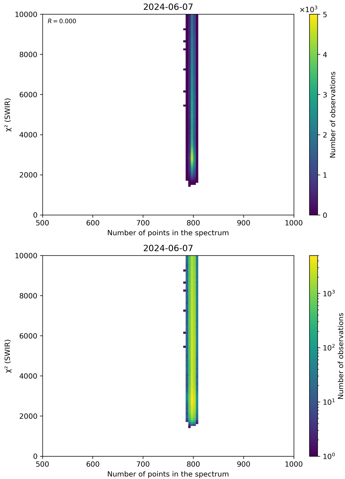
Figure 89: Scatter density plot of “Number of points in the spectrum” against “ \chi^2 (SWIR)” for 2024-06-06 to 2024-06-08.
