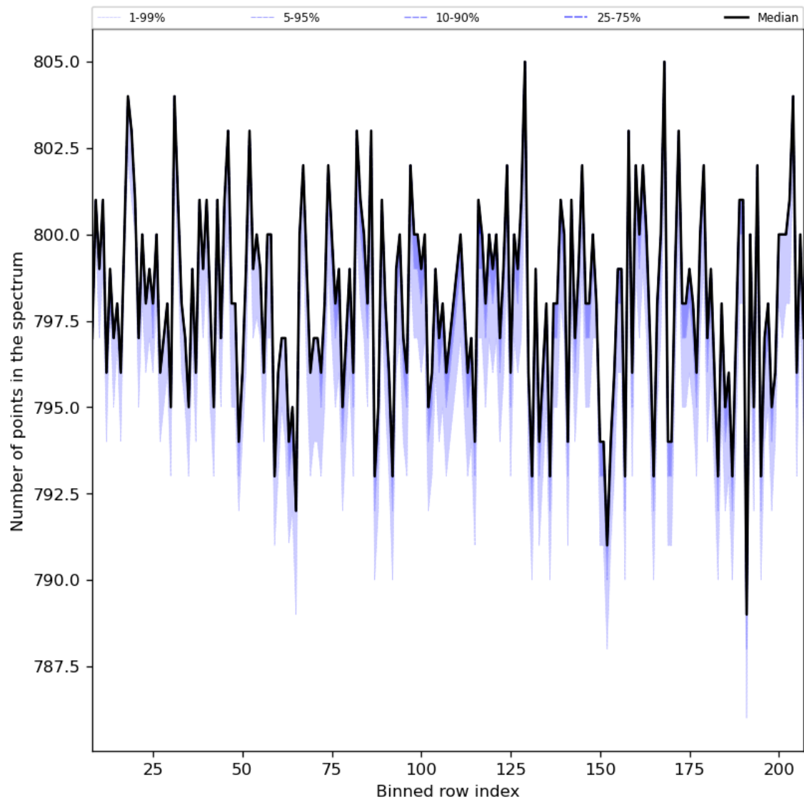
Figure 37: Along track statistics of “Number of points in the spectrum” for 2024-06-06 to 2024-06-08
