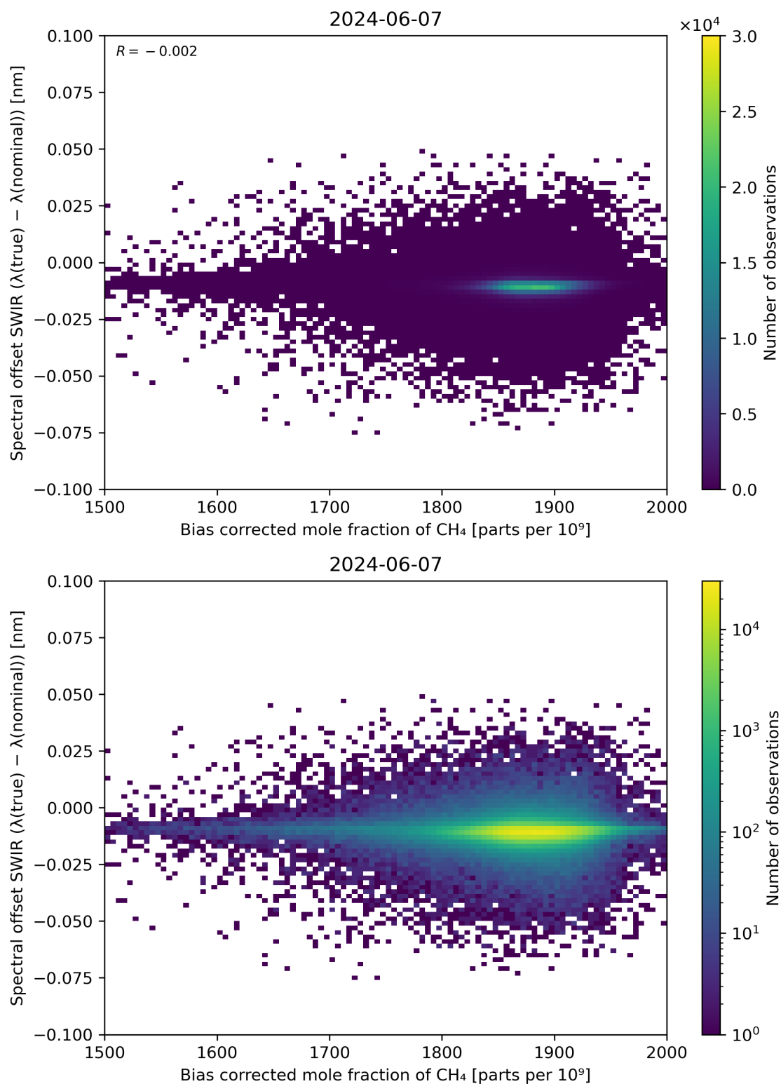
Figure 69: Scatter density plot of “Bias corrected mole fraction of \text{CH}_4 ” against “Spectral offset SWIR ( \lambda(\text{true}) - \lambda(\text{nominal}) )” for 2024-06-06 to 2024-06-08.
