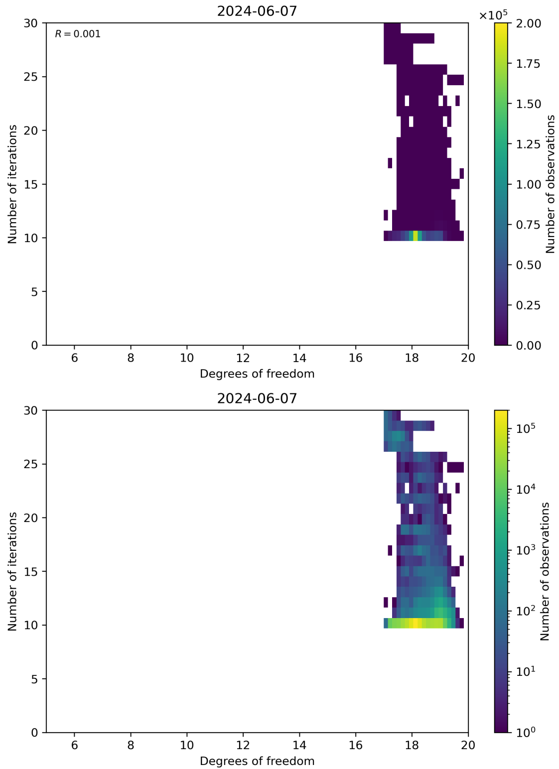
Figure 52: Scatter density plot of “Degrees of freedom” against “Number of iterations” for 2024-06-06 to 2024-06-08.
