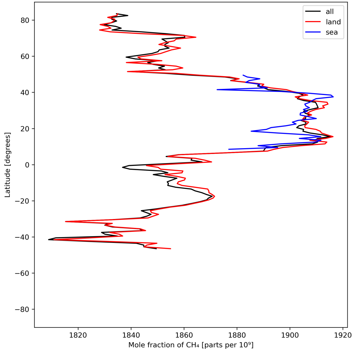
Figure 12: Zonal average of “Mole fraction of \text{CH}_4 ” for 2024-06-06 to 2024-06-08.
