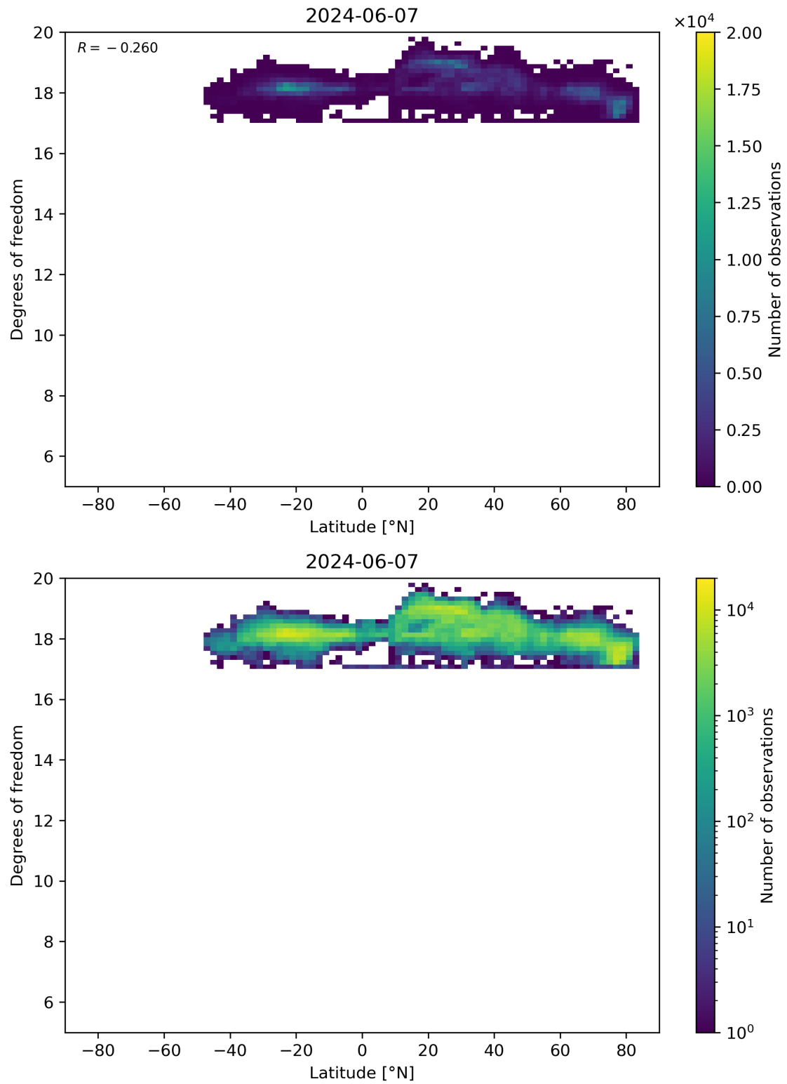
Figure 55: Scatter density plot of “Latitude” against “Degrees of freedom” for 2024-06-06 to 2024-06-08.
