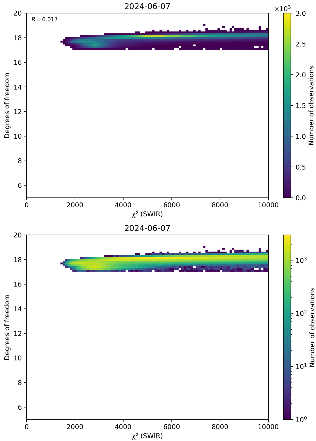
Figure 48: Scatter density plot of “ \chi^2 (SWIR)” against “Degrees of freedom” for 2024-06-06 to 2024-06-08.
