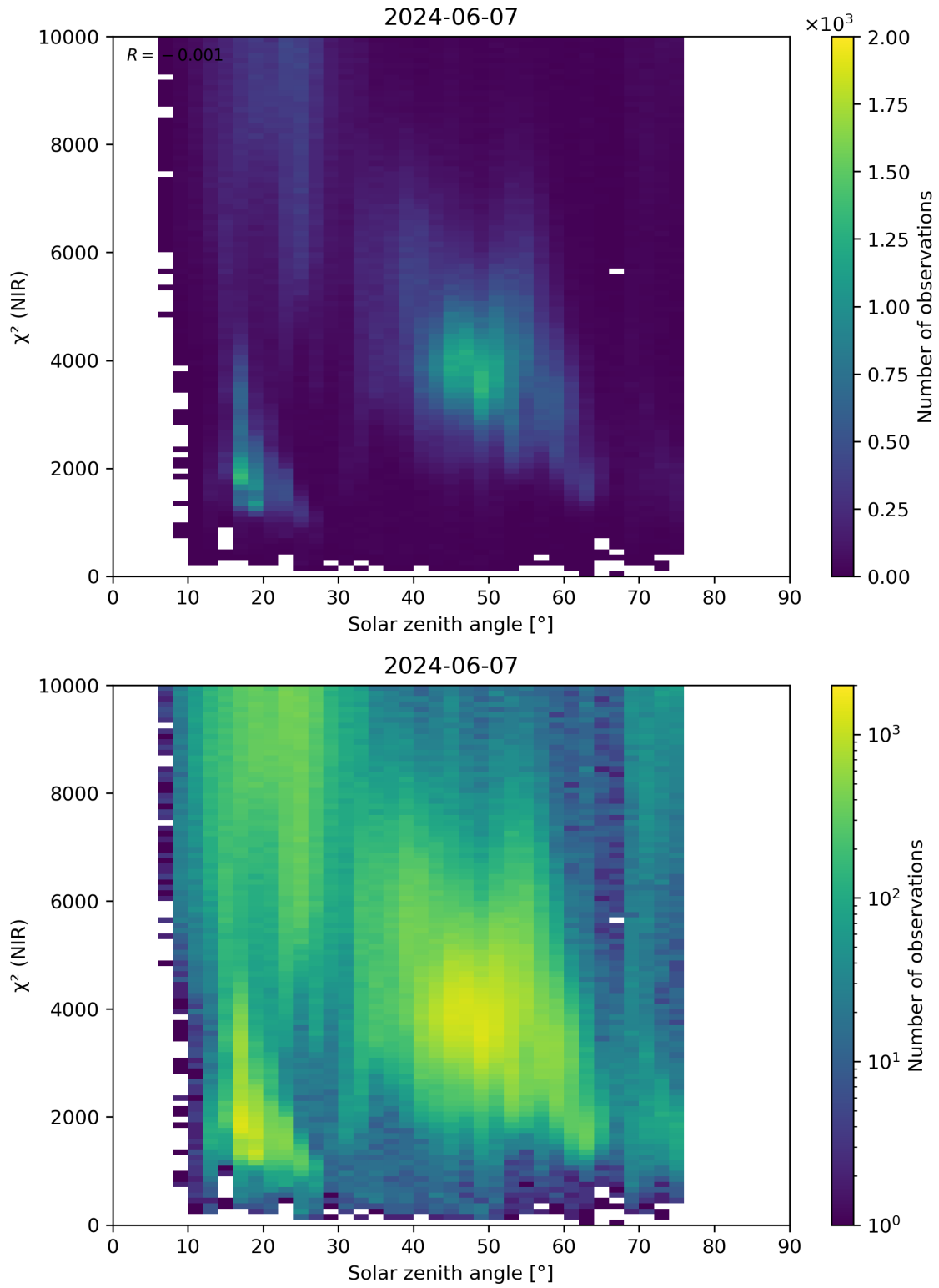
Figure 94: Scatter density plot of “Solar zenith angle” against “ \chi^2 (NIR)” for 2024-06-06 to 2024-06-08.
