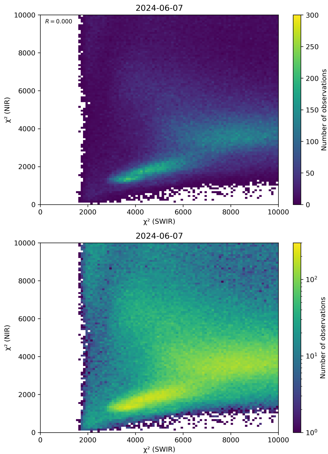
Figure 47: Scatter density plot of “ \chi^2 (SWIR)” against “ \chi^2 (NIR)” for 2024-06-06 to 2024-06-08.
