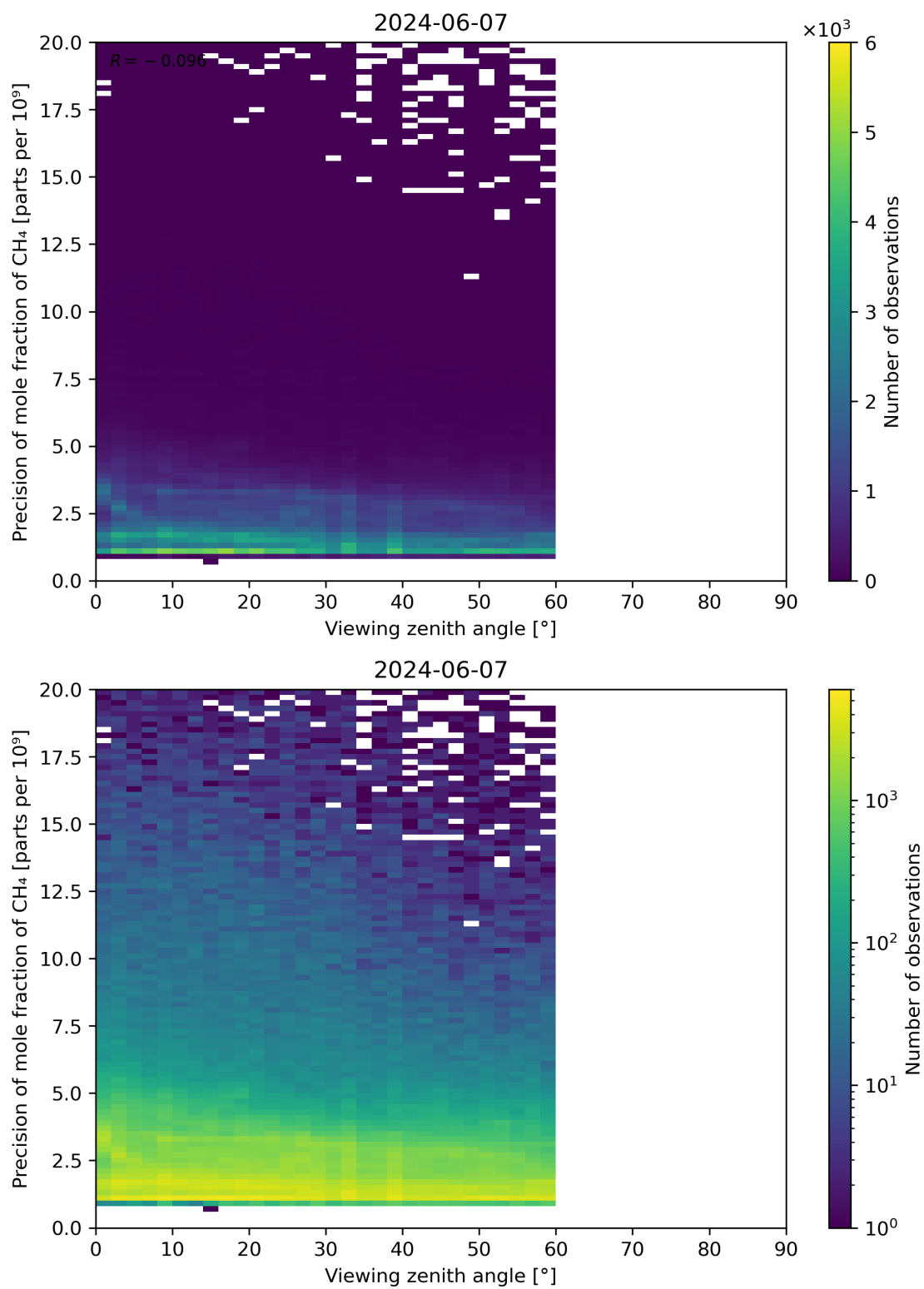
Figure 112: Scatter density plot of “Viewing zenith angle” against “Precision of mole fraction of CH 4 ” for 2024-06-06 to 2024-06-08.
