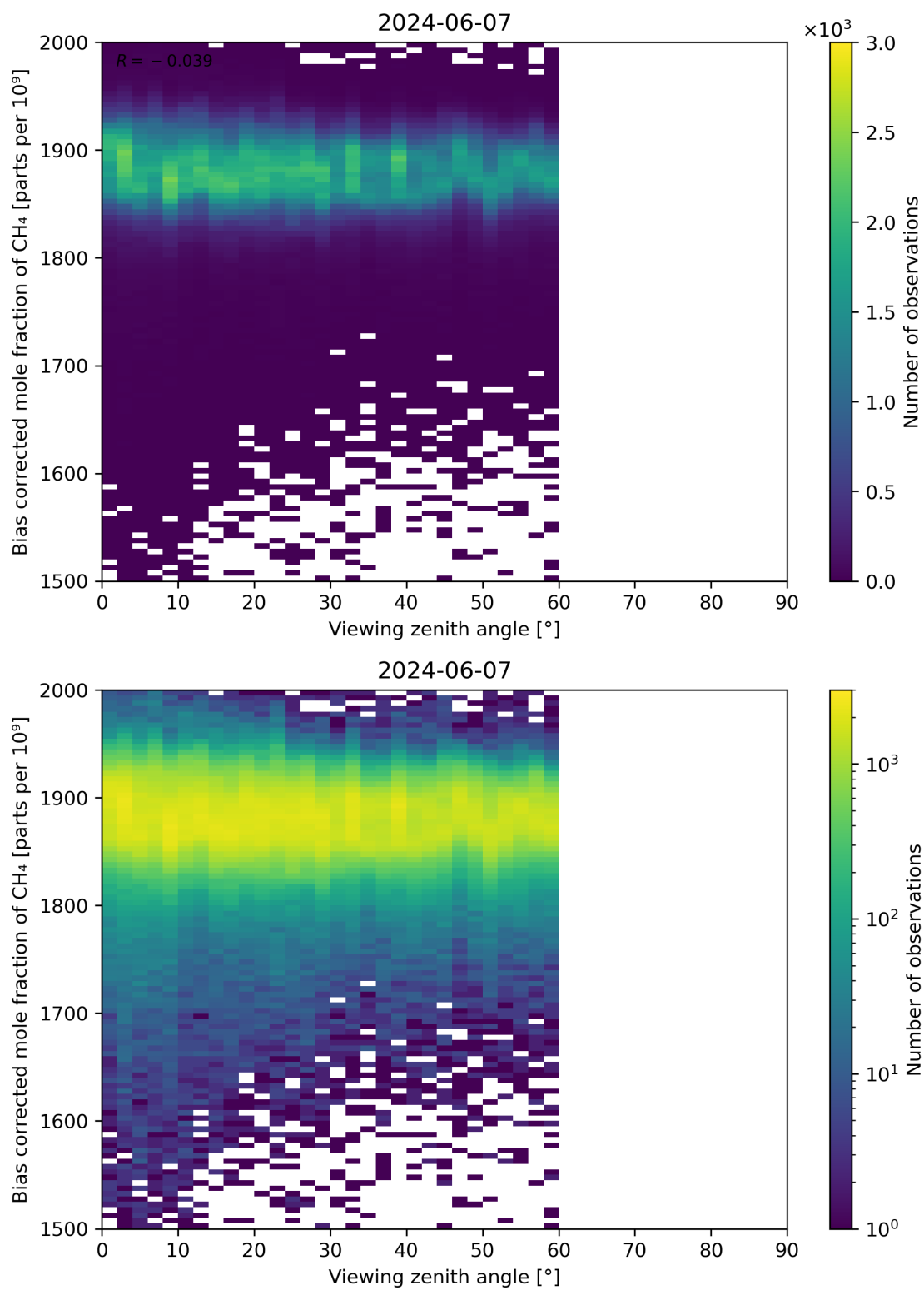
Figure 111: Scatter density plot of “Viewing zenith angle” against “Bias corrected mole fraction of CH 4 ” for 2024-06-06 to 2024-06-08.
