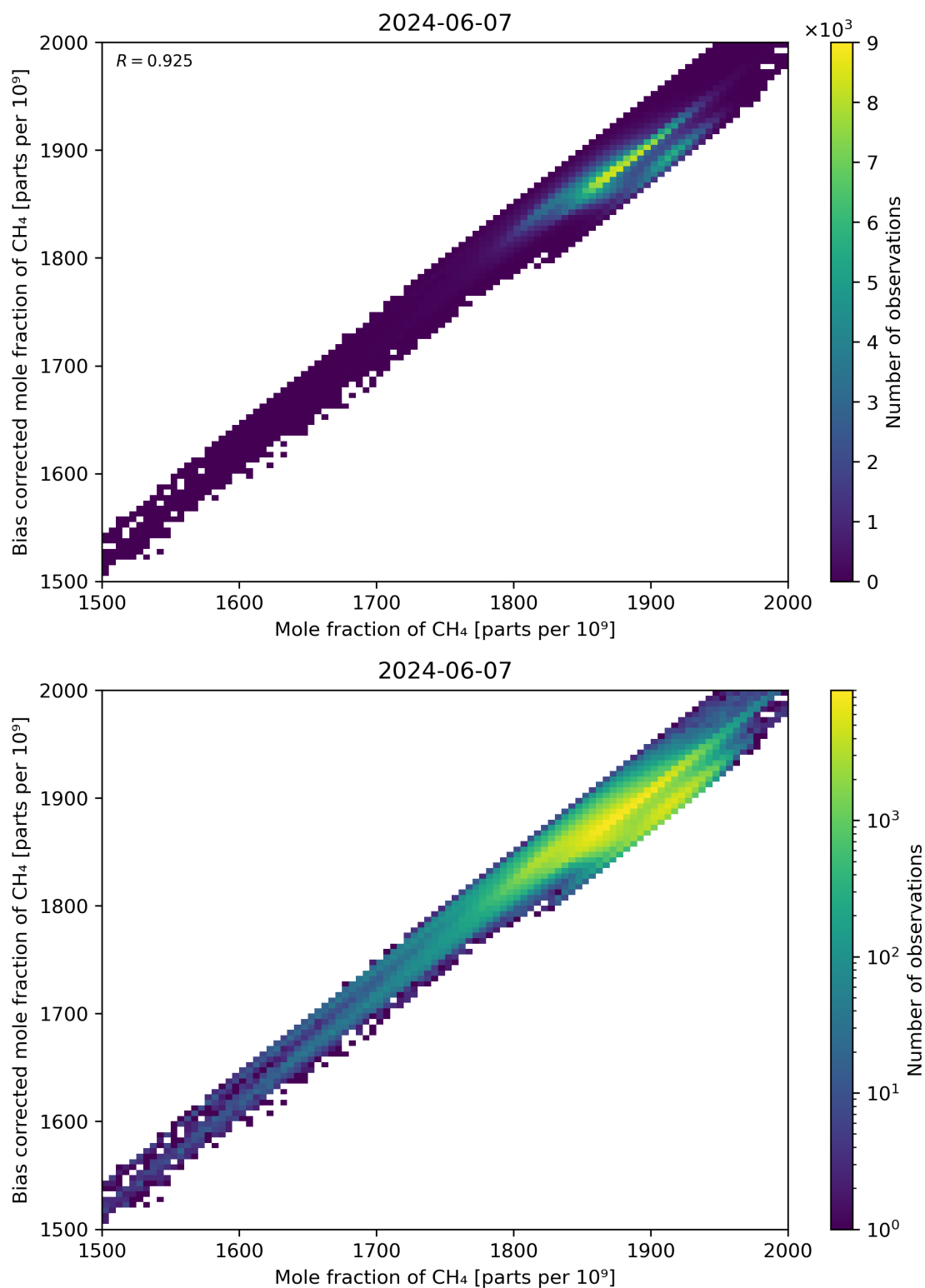
Figure 74: Scatter density plot of “Mole fraction of CH 4 ” against “Bias corrected mole fraction of CH 4 ” for 2024-06-06 to 2024-06-08.
