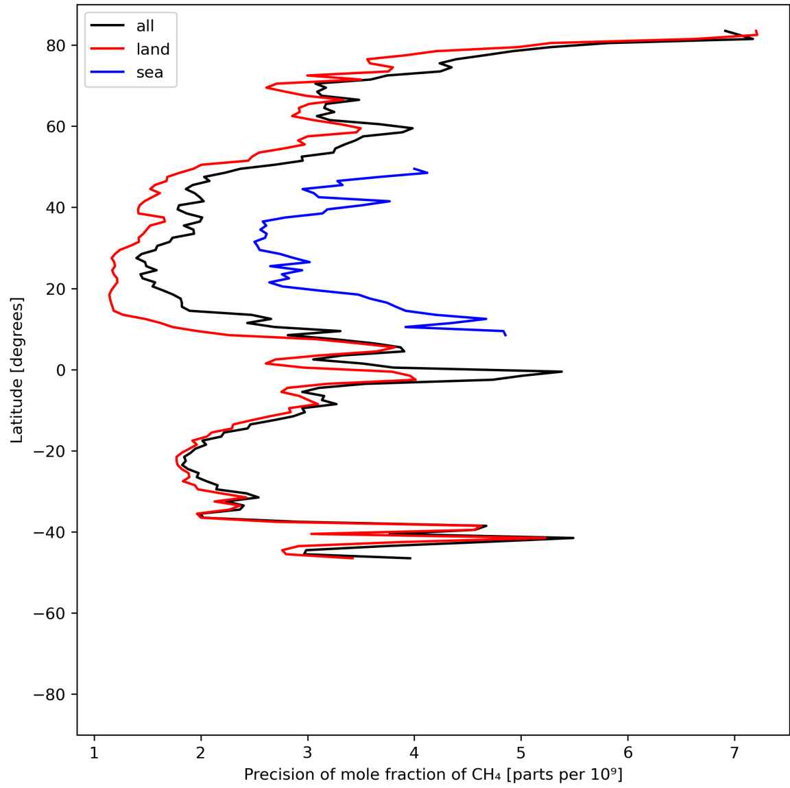
Figure 13: Zonal average of “Precision of mole fraction of CH 4 ” for 2024-06-06 to 2024-06-08.
