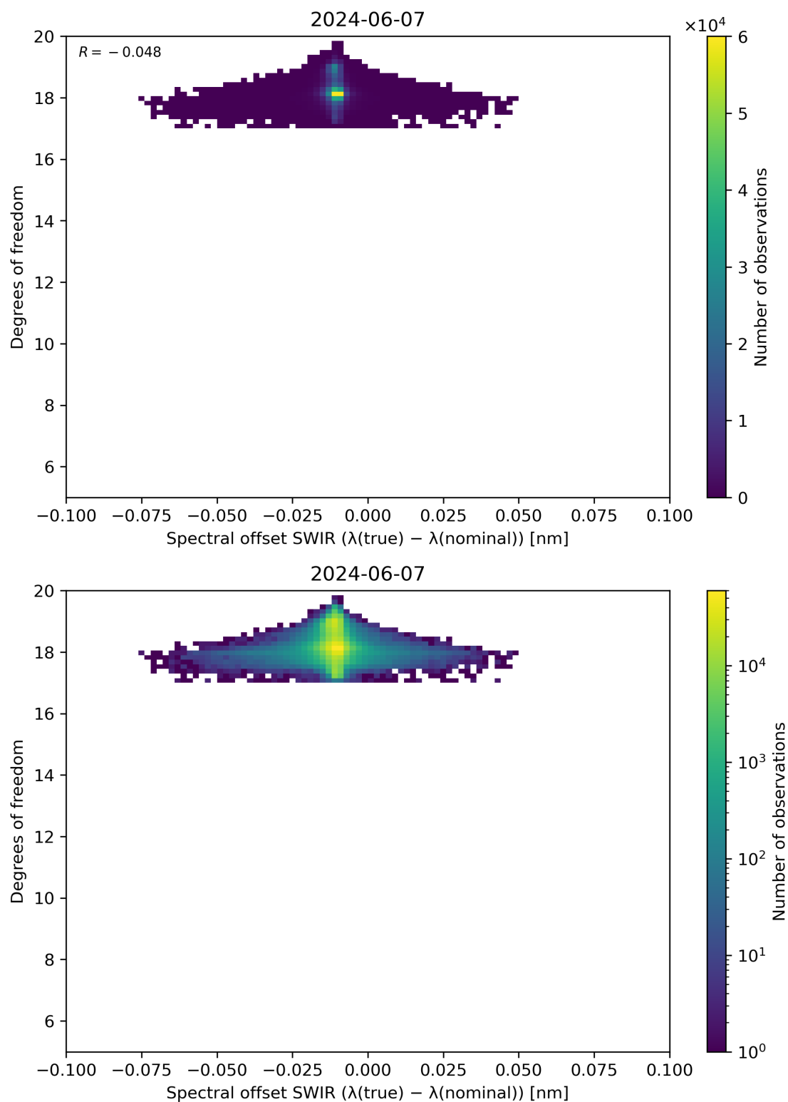
Figure 119: Scatter density plot of “Spectral offset SWIR ( \lambda(\text{true}) - \lambda(\text{nominal}) )” against “Degrees of freedom” for 2024-06-06 to 2024-06-08.
