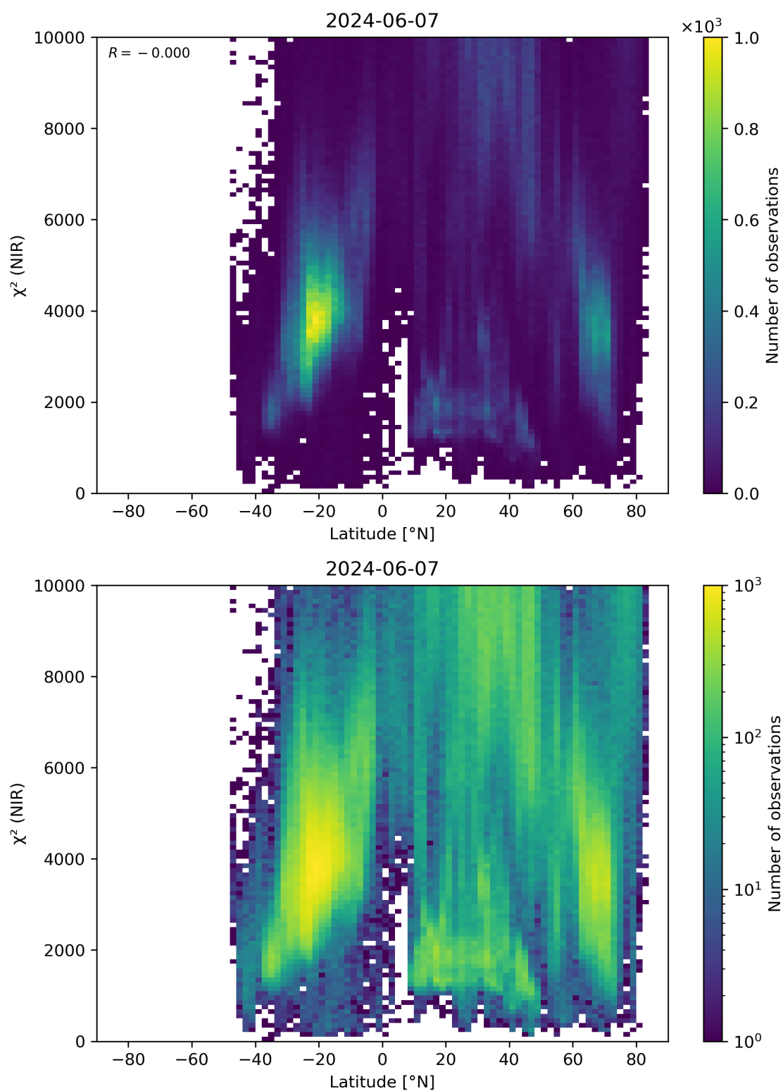
Figure 53: Scatter density plot of “Latitude” against “ \chi^2 (NIR)” for 2024-06-06 to 2024-06-08.
