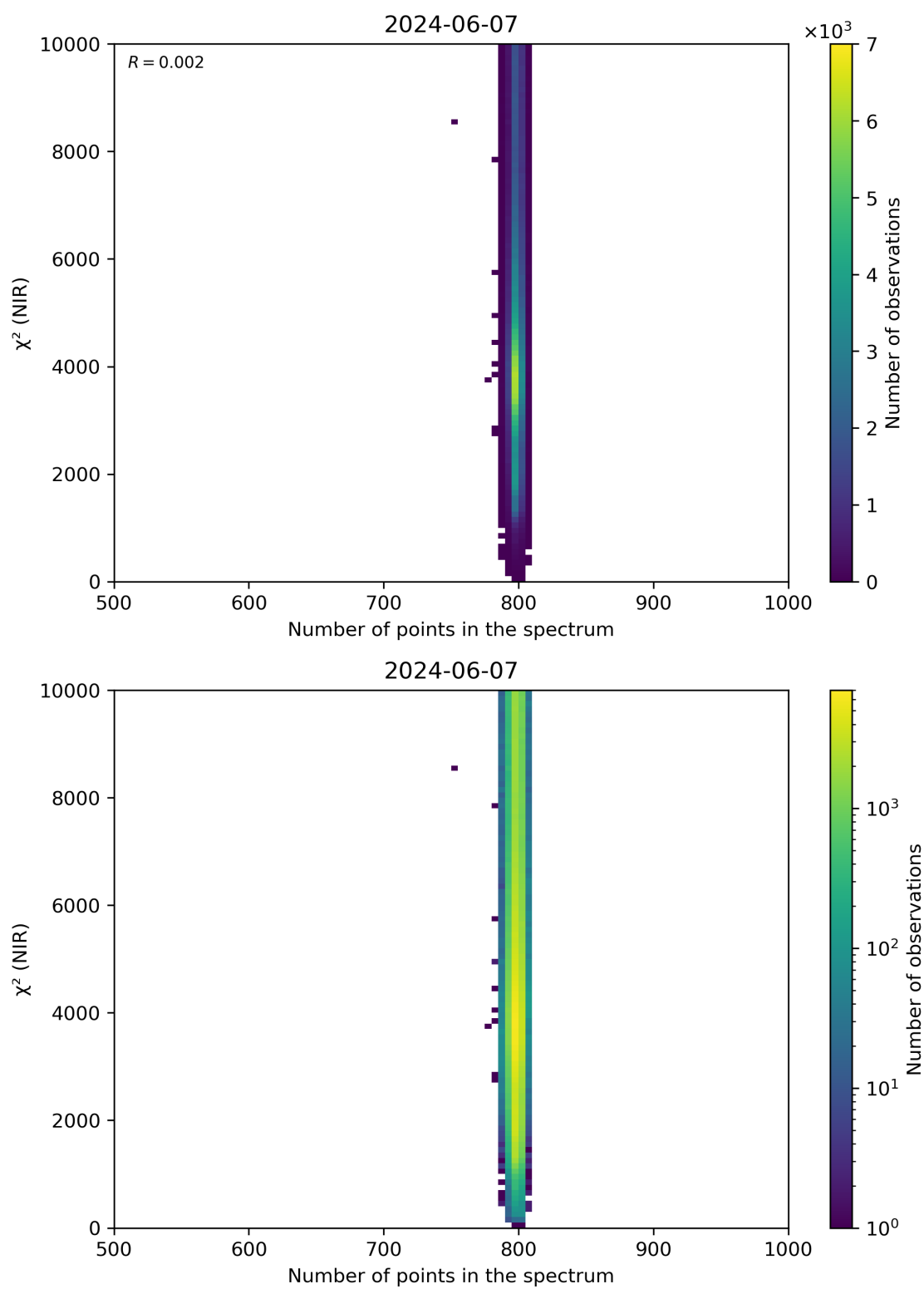
Figure 88: Scatter density plot of “Number of points in the spectrum” against “ \chi^2 (NIR)” for 2024-06-06 to 2024-06-08.
