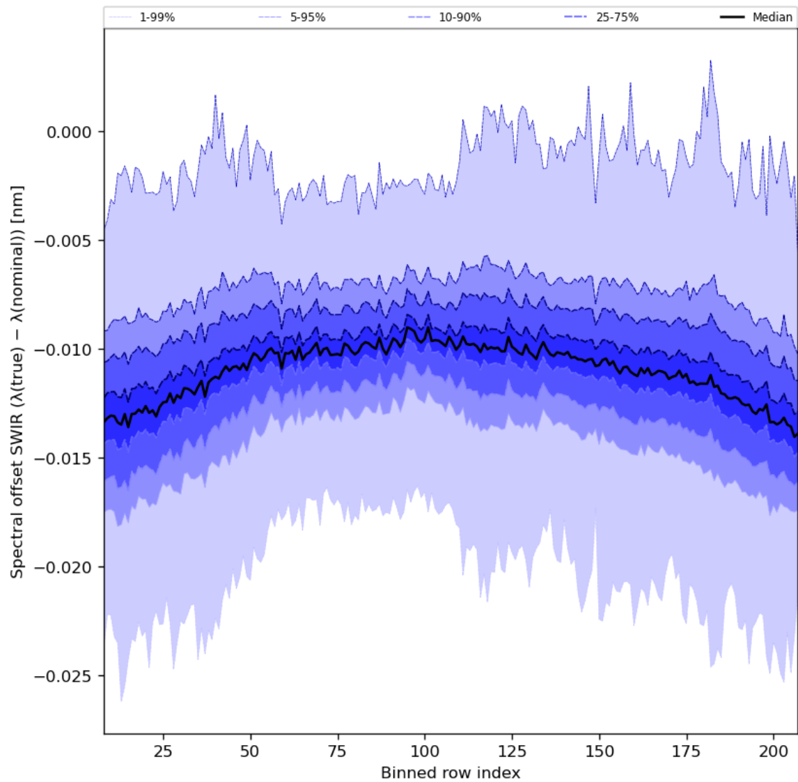
Figure 38: Along track statistics of “Spectral offset SWIR ( \lambda(\text{true}) - \lambda(\text{nominal}) )” for 2024-06-06 to 2024-06-08
