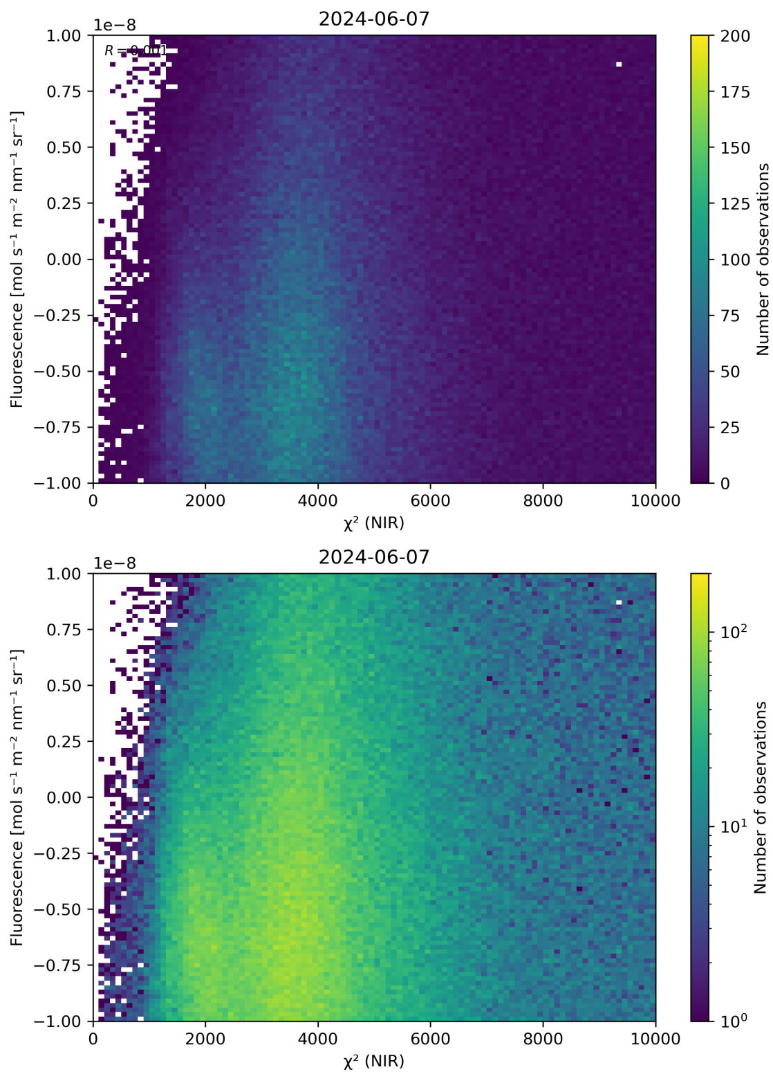
Figure 45: Scatter density plot of “ \chi^2 (NIR)” against “Fluorescence” for 2024-06-06 to 2024-06-08.
