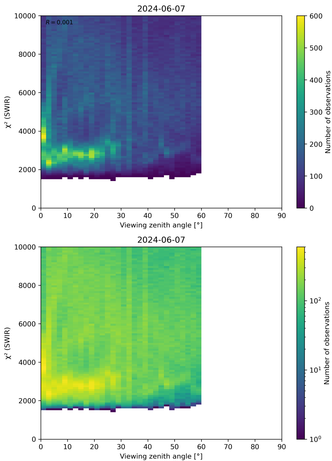
Figure 106: Scatter density plot of “Viewing zenith angle” against “ \chi^2 (SWIR)” for 2024-06-06 to 2024-06-08.
