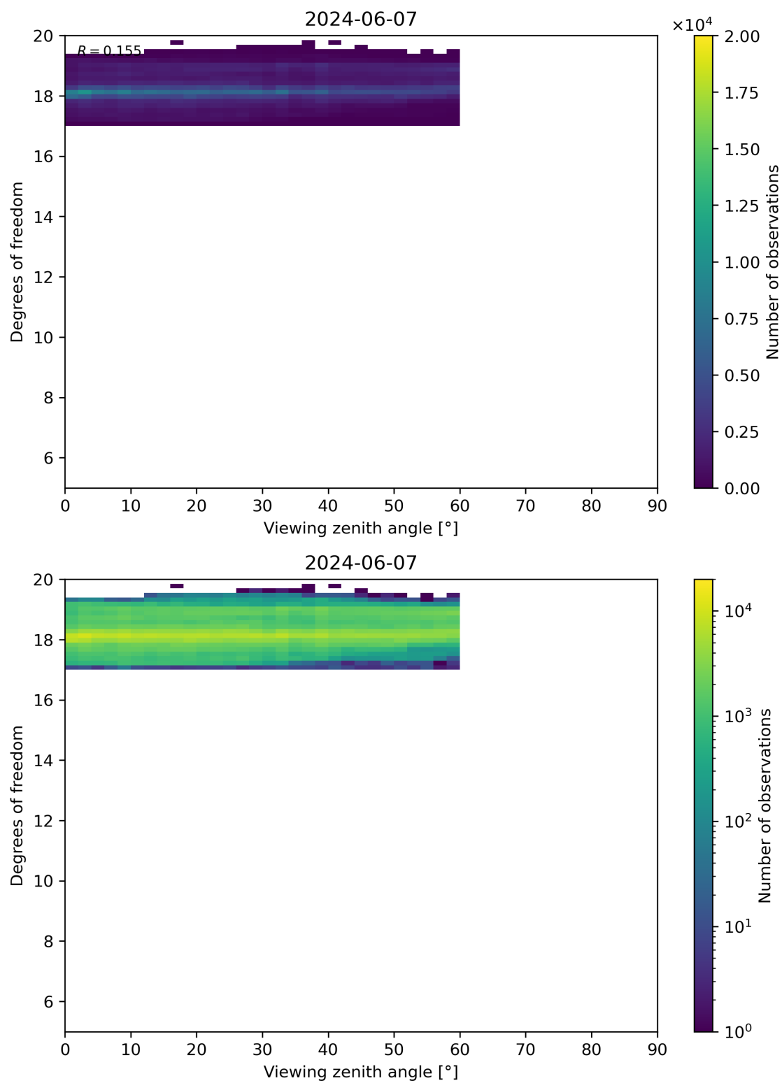
Figure 107: Scatter density plot of “Viewing zenith angle” against “Degrees of freedom” for 2024-06-06 to 2024-06-08.
