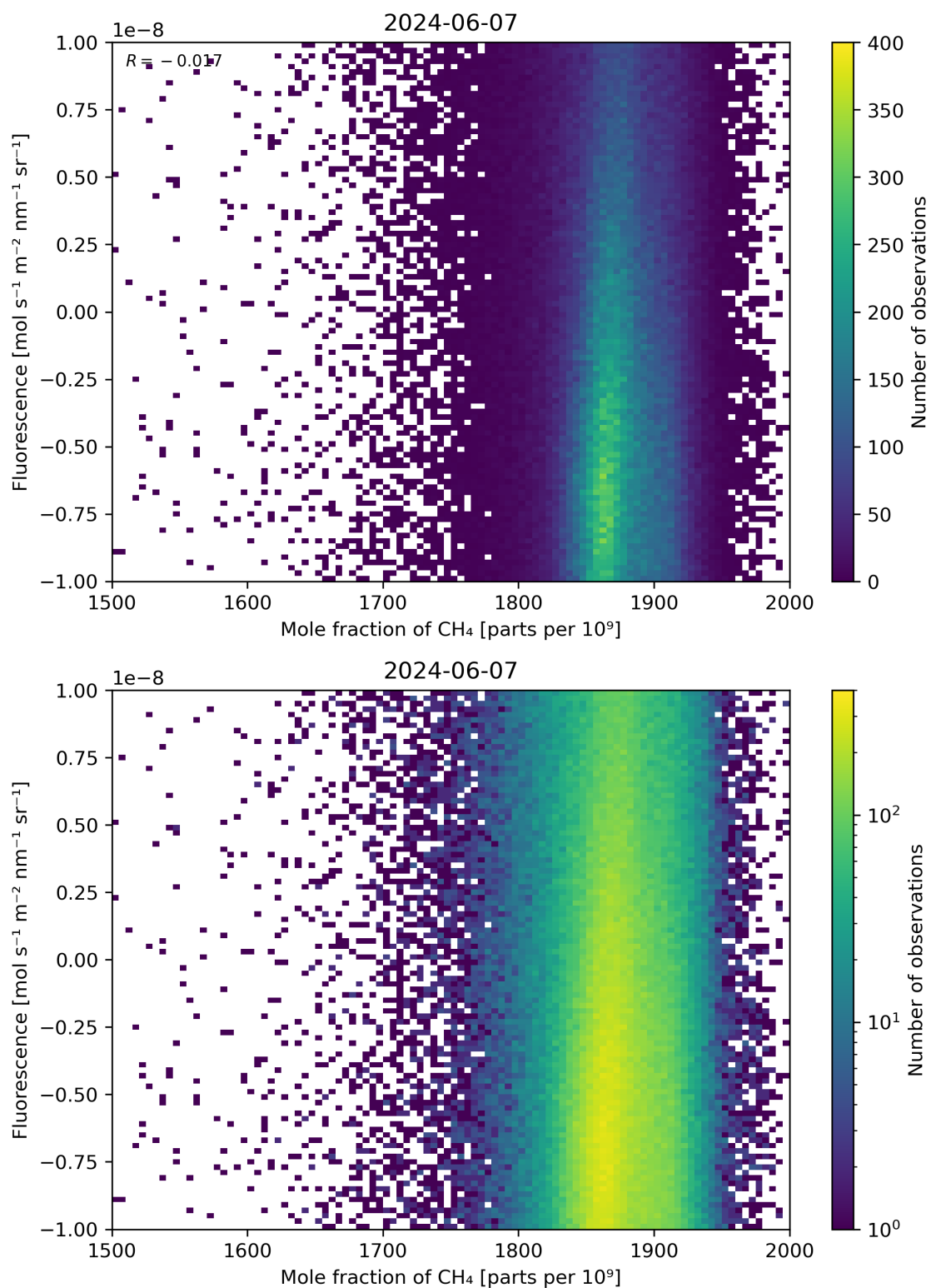
Figure 73: Scatter density plot of “Mole fraction of \text{CH}_4 ” against “Fluorescence” for 2024-06-06 to 2024-06-08.
