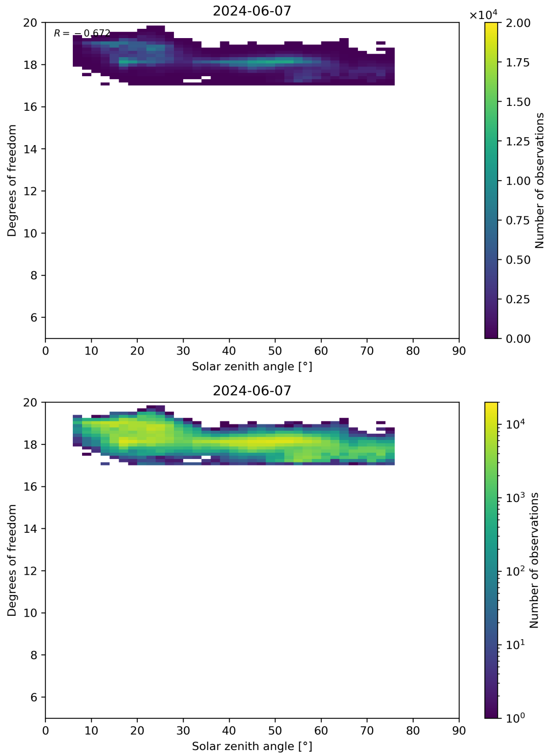
Figure 96: Scatter density plot of “Solar zenith angle” against “Degrees of freedom” for 2024-06-06 to 2024-06-08.
