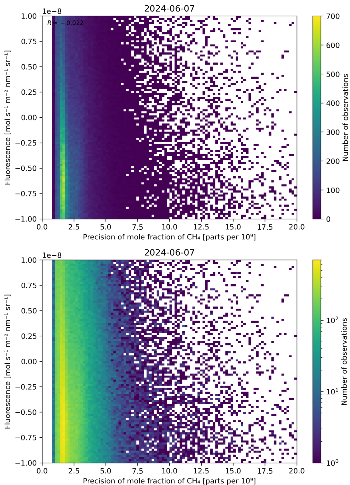
Figure 81: Scatter density plot of “Precision of mole fraction of CH 4 ” against “Fluorescence” for 2024-06-06 to 2024-06-08.
