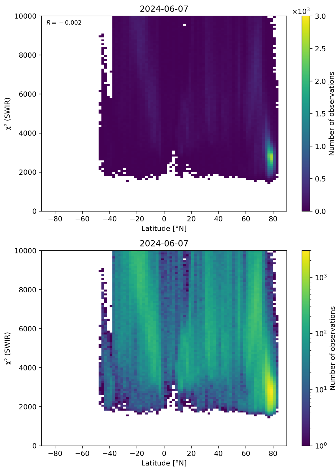
Figure 54: Scatter density plot of “Latitude” against “ \chi^2 (SWIR)” for 2024-06-06 to 2024-06-08.
