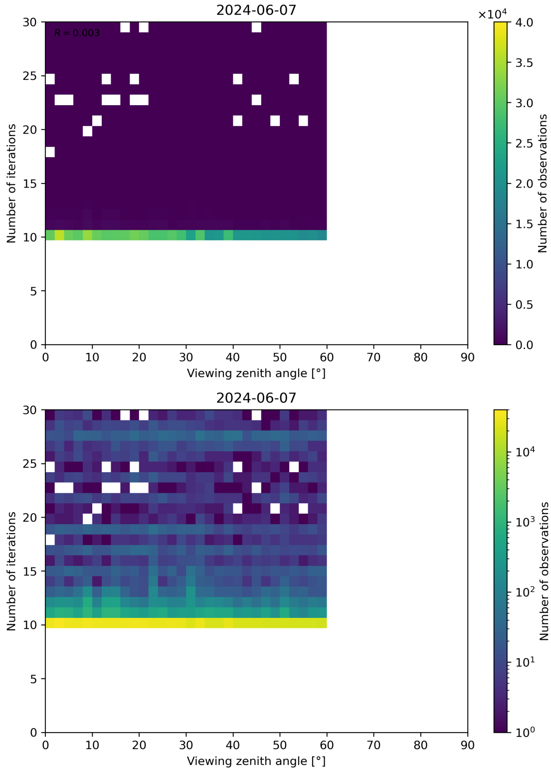
Figure 113: Scatter density plot of “Viewing zenith angle” against “Number of iterations” for 2024-06-06 to 2024-06-08.
