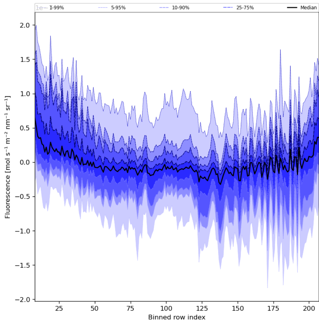
Figure 43: Along track statistics of “Fluorescence” for 2024-06-06 to 2024-06-08
