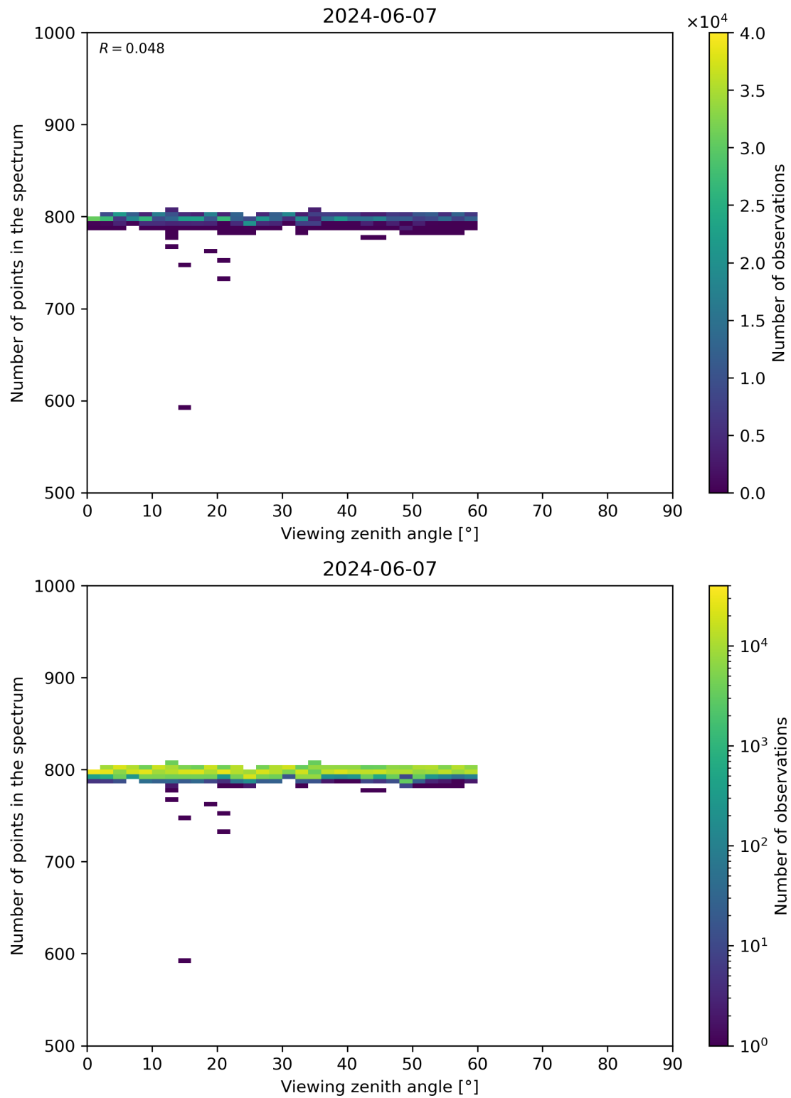
Figure 114: Scatter density plot of “Viewing zenith angle” against “Number of points in the spectrum” for 2024-06-06 to 2024-06-08.
