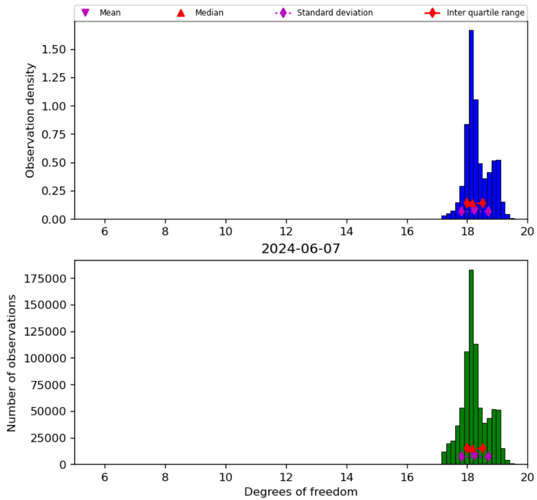
Figure 30: Histogram of “Degrees of freedom” for 2024-06-06 to 2024-06-08
