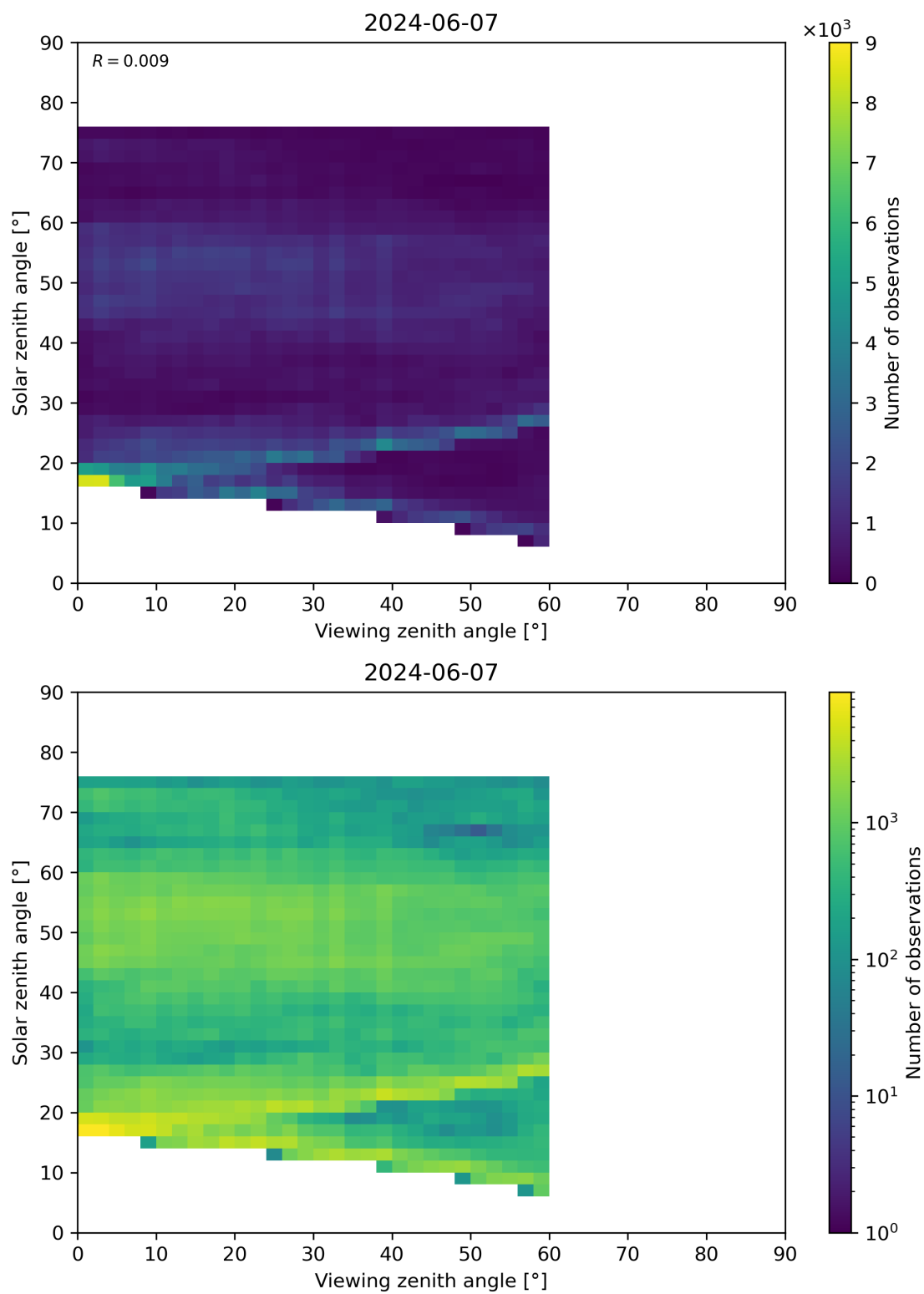
Figure 115: Scatter density plot of “Viewing zenith angle” against “Solar zenith angle” for 2024-06-06 to 2024-06-08.
