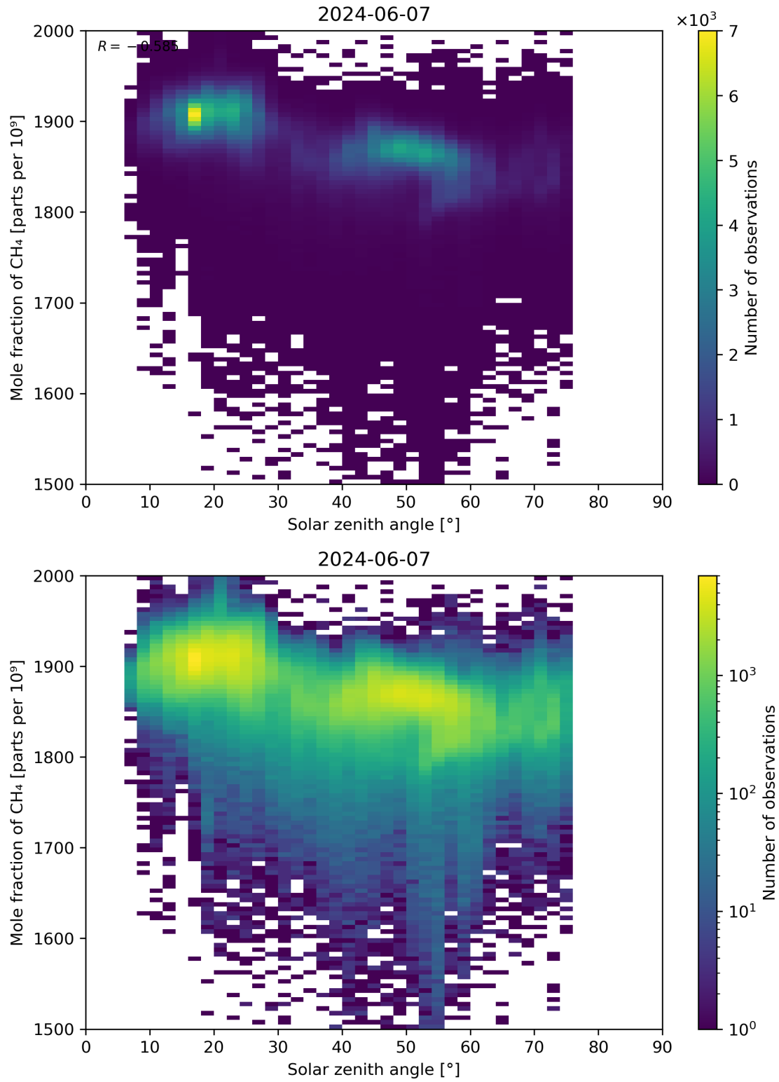
Figure 99: Scatter density plot of “Solar zenith angle” against “Mole fraction of CH 4 ” for 2024-06-06 to 2024-06-08.
