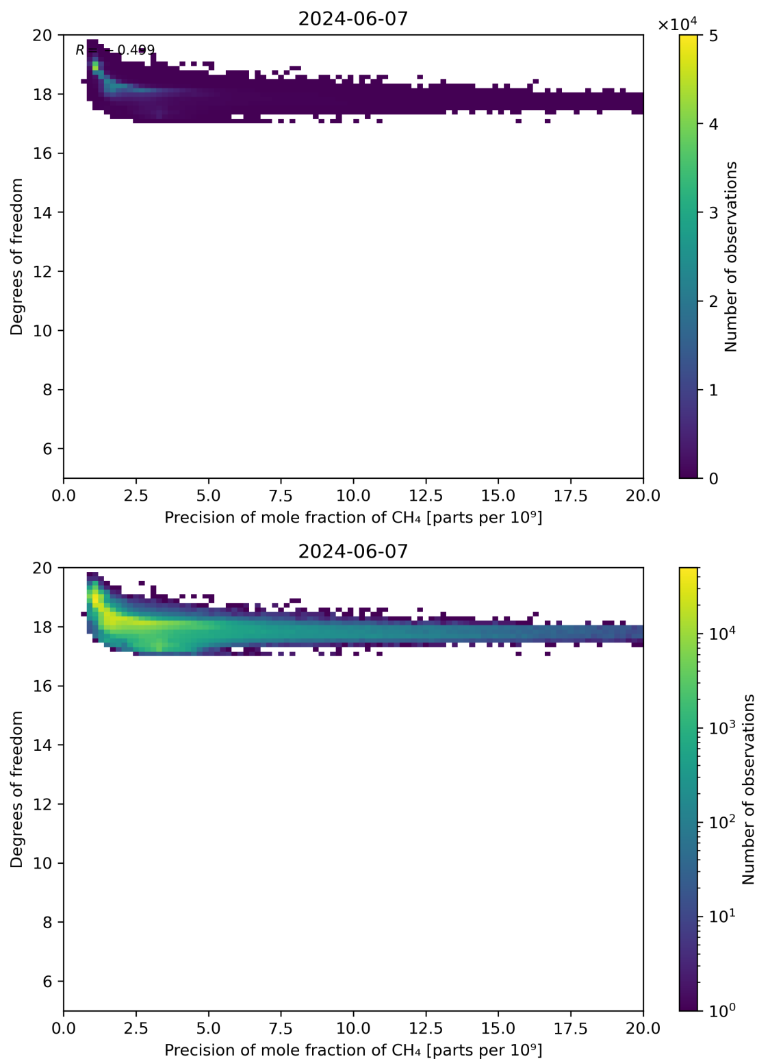
Figure 80: Scatter density plot of “Precision of mole fraction of CH 4 ” against “Degrees of freedom” for 2024-06-06 to 2024-06-08.
