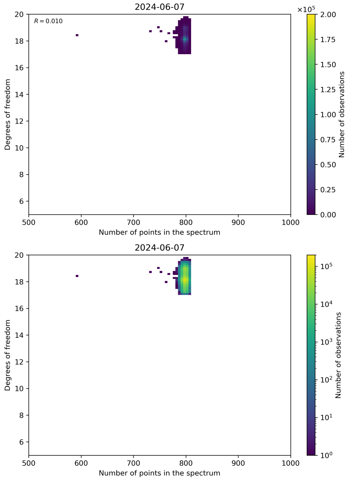
Figure 90: Scatter density plot of “Number of points in the spectrum” against “Degrees of freedom” for 2024-06-06 to 2024-06-08.
