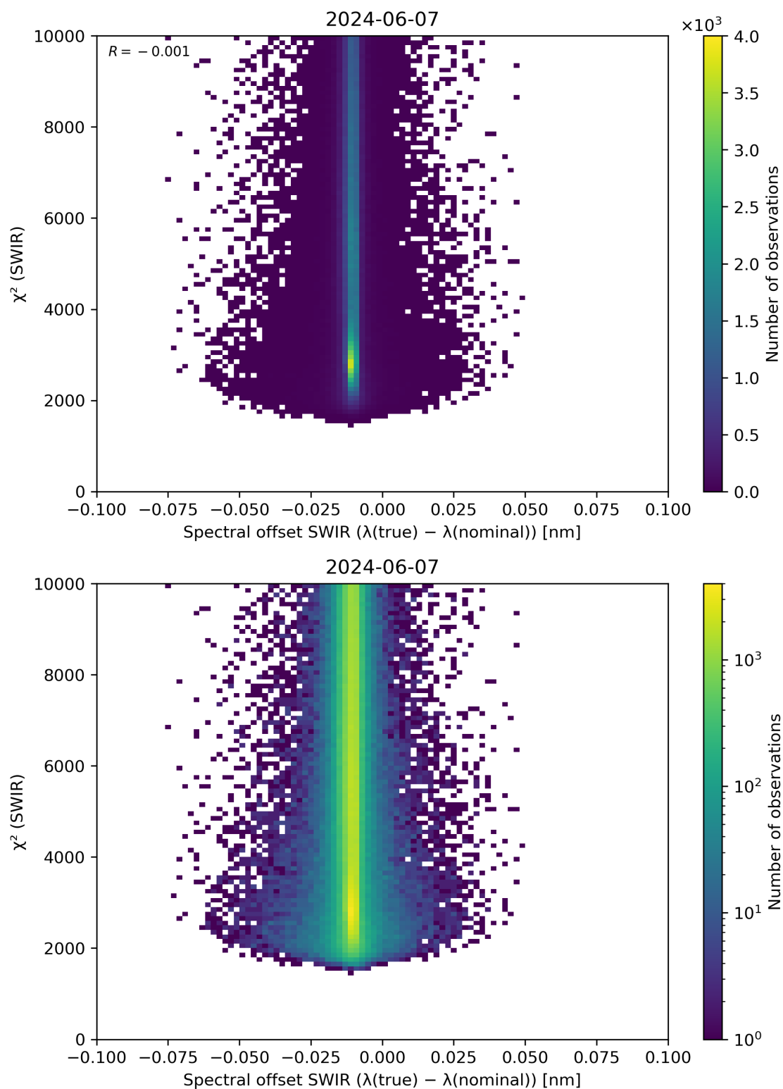
Figure 118: Scatter density plot of “Spectral offset SWIR ( \lambda(\text{true}) - \lambda(\text{nominal}) )” against “ \chi^2 (SWIR)” for 2024-06-06 to 2024-06-08.
