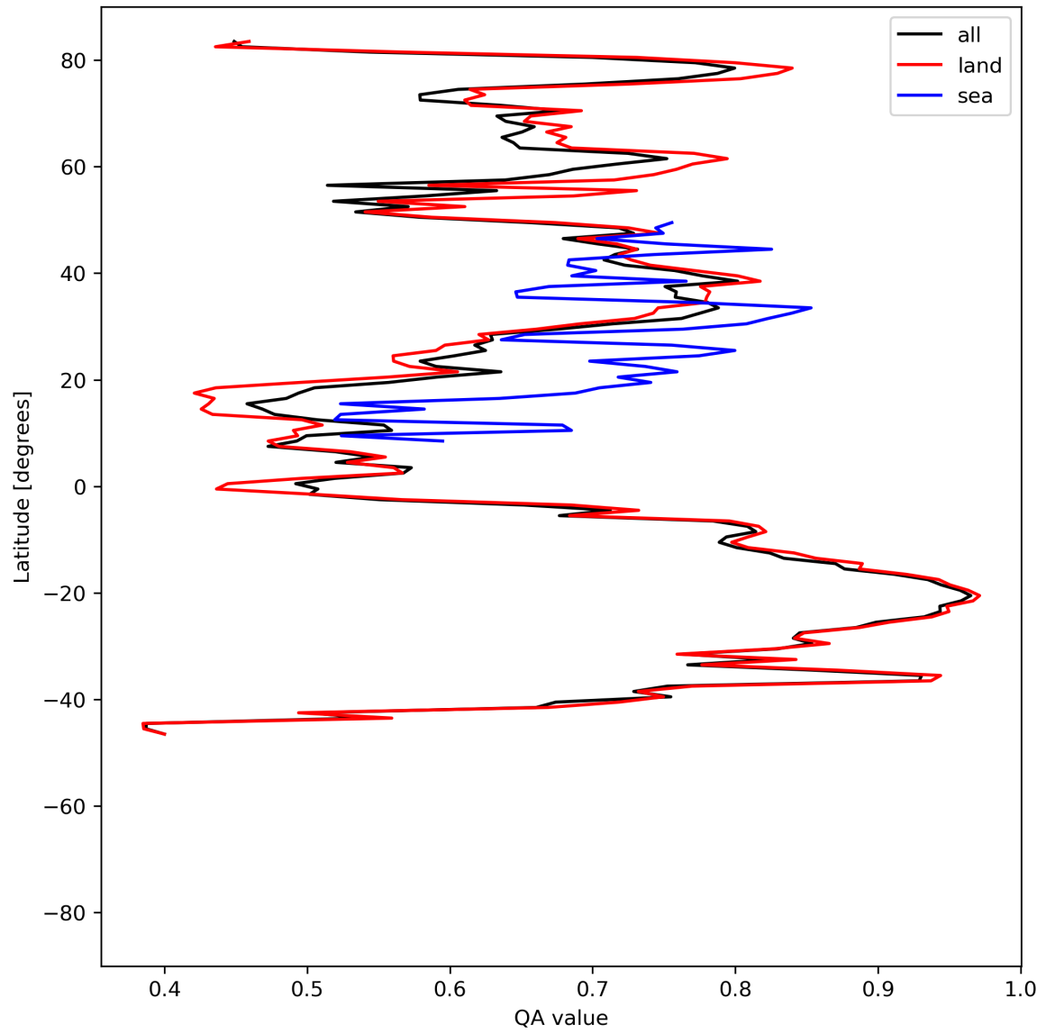
Figure 11: Zonal average of “QA value” for 2024-06-06 to 2024-06-08.
