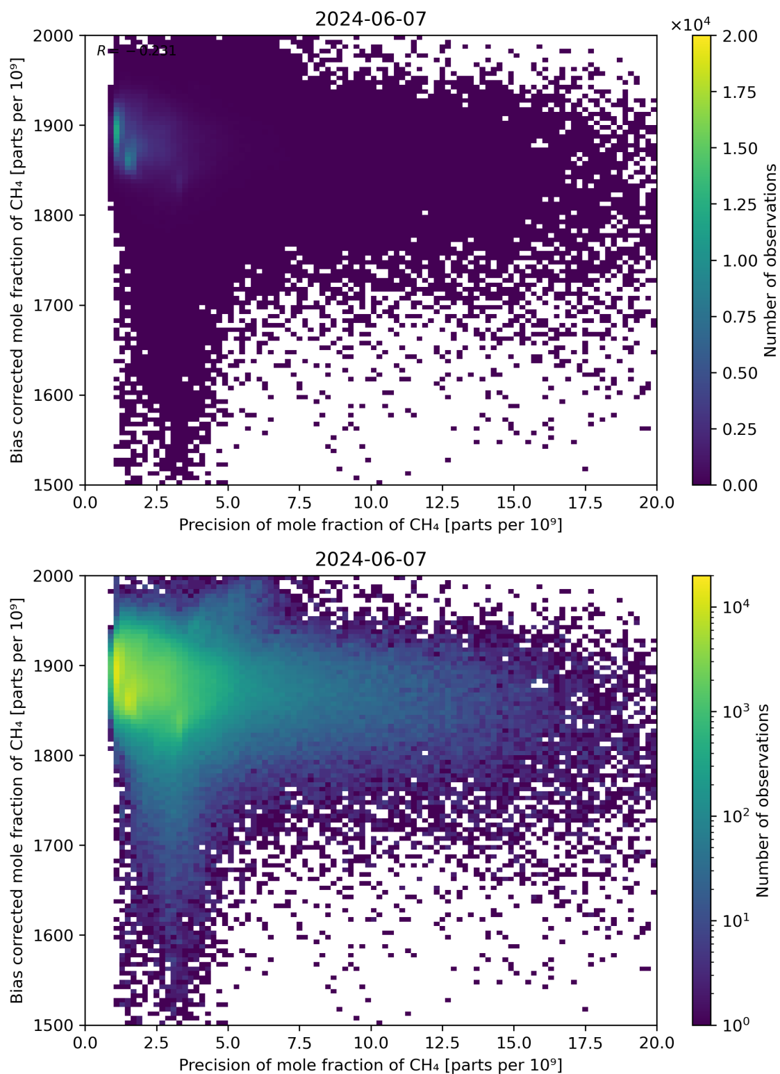
Figure 82: Scatter density plot of “Precision of mole fraction of CH 4 ” against “Bias corrected mole fraction of CH 4 ” for 2024-06-06 to 2024-06-08.
