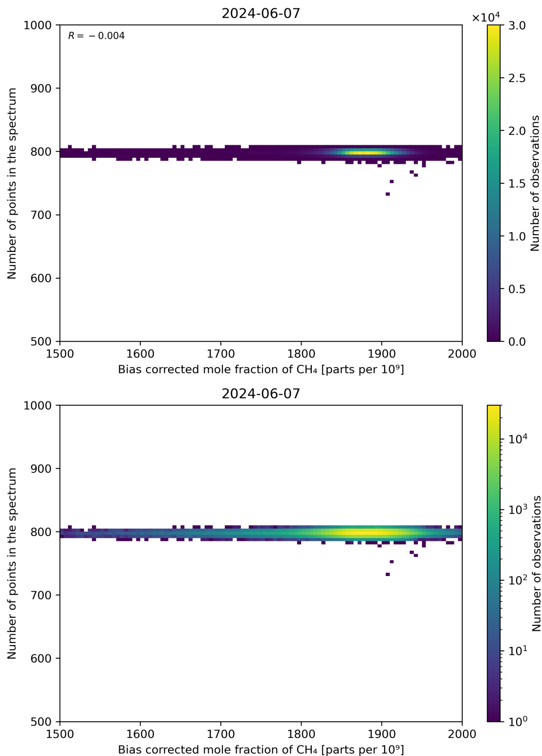
Figure 68: Scatter density plot of “Bias corrected mole fraction of CH 4 ” against “Number of points in the spectrum” for 2024-06-06 to 2024-06-08.
