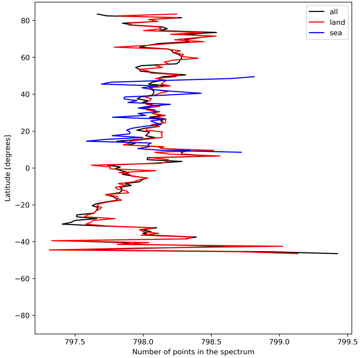
Figure 15: Zonal average of “Number of points in the spectrum” for 2024-06-06 to 2024-06-08.
