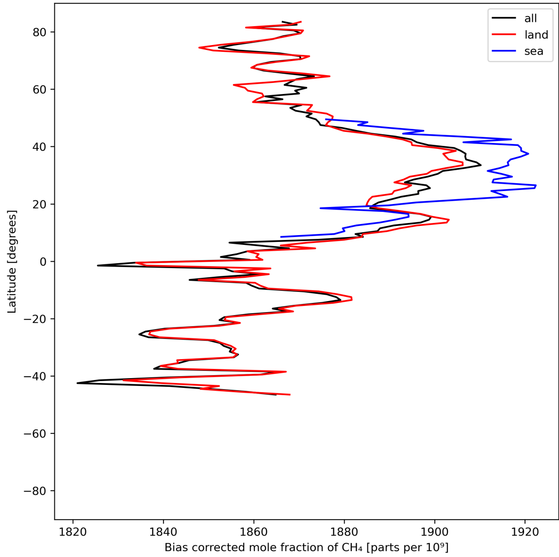
Figure 14: Zonal average of “Bias corrected mole fraction of CH 4 ” for 2024-06-08 to 2024-06-09.
