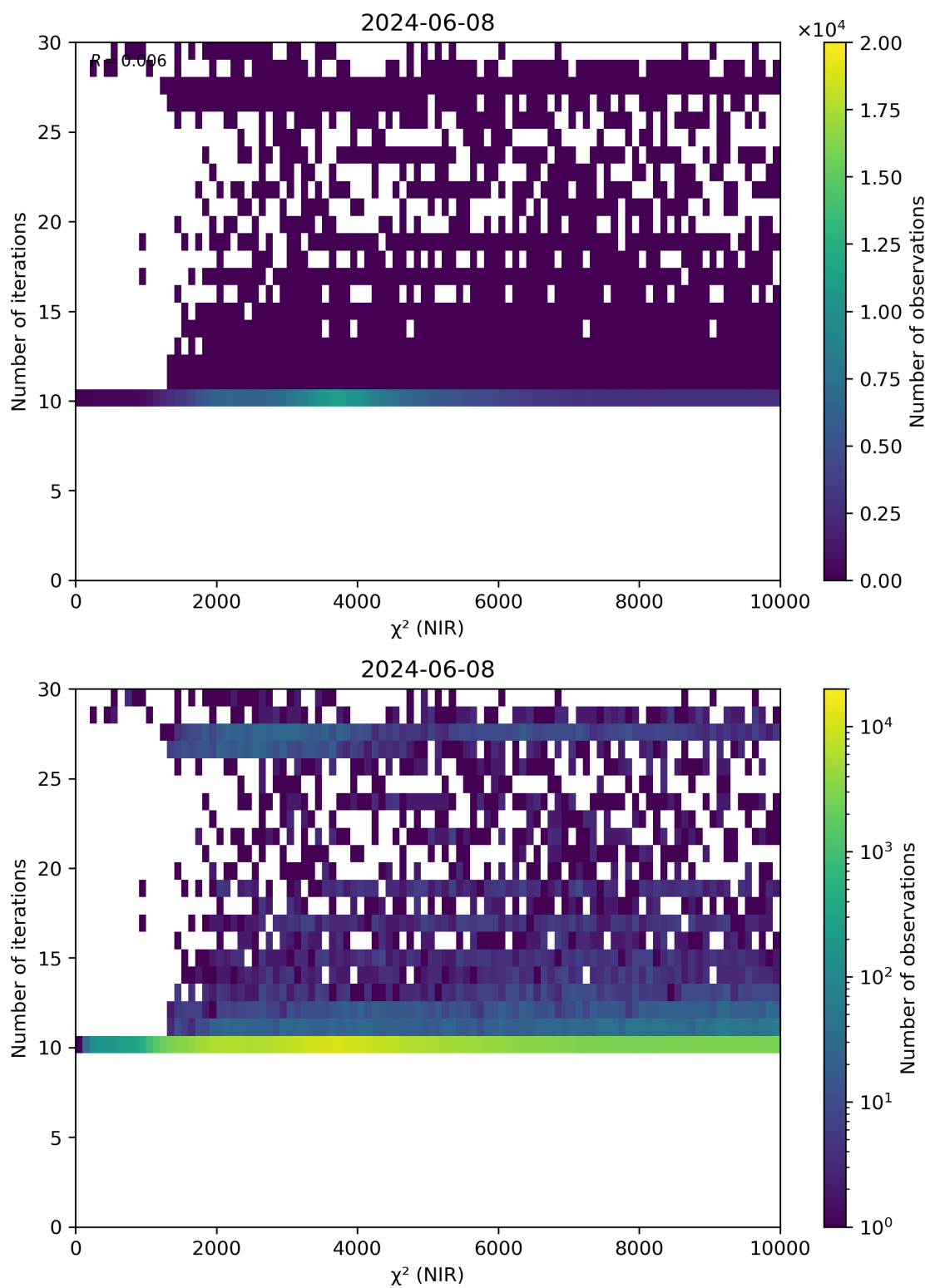
Figure 46: Scatter density plot of “ \chi^2 (NIR)” against “Number of iterations” for 2024-06-08 to 2024-06-09.
