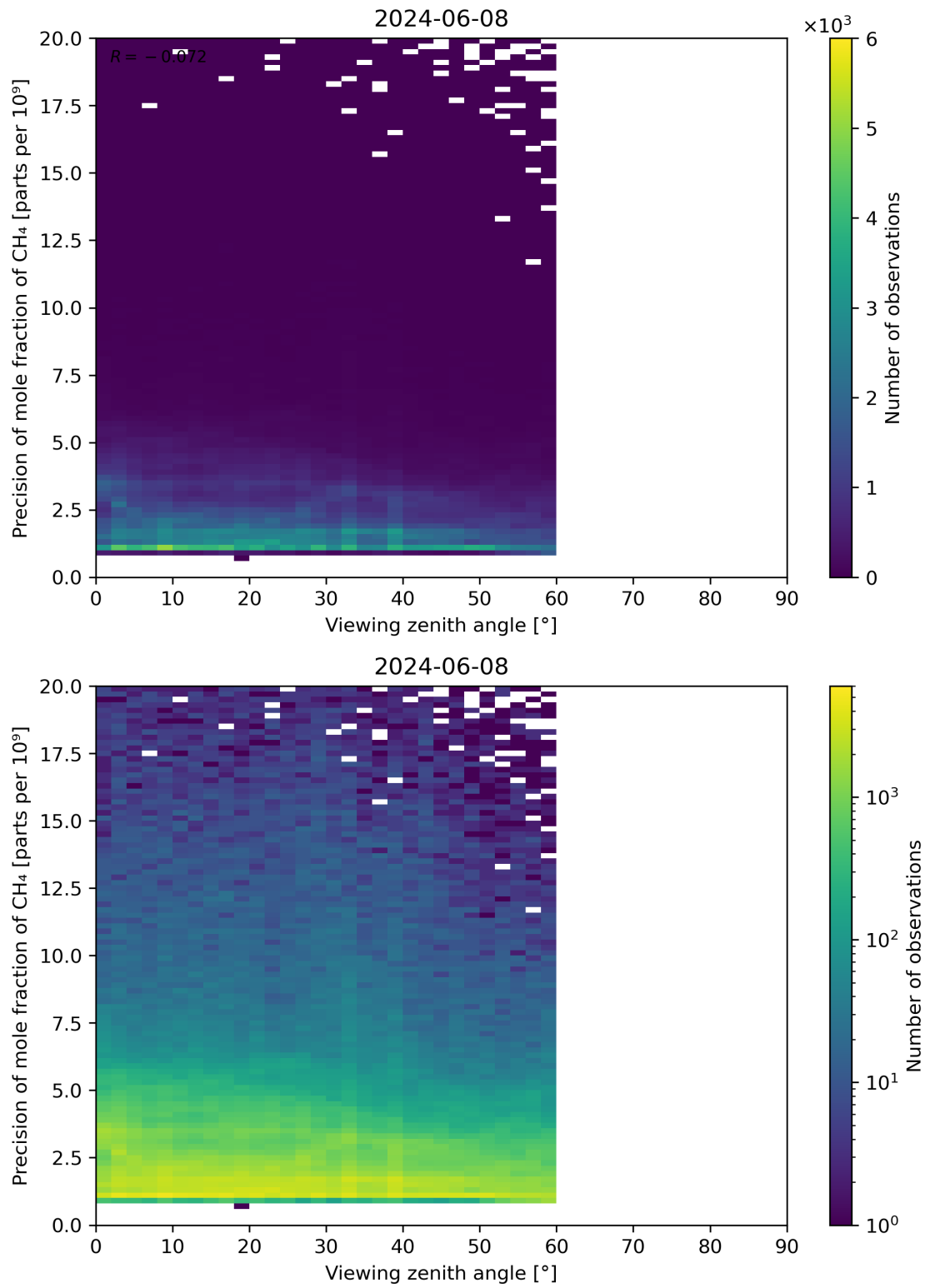
Figure 112: Scatter density plot of “Viewing zenith angle” against “Precision of mole fraction of CH 4 ” for 2024-06-08 to 2024-06-09.
