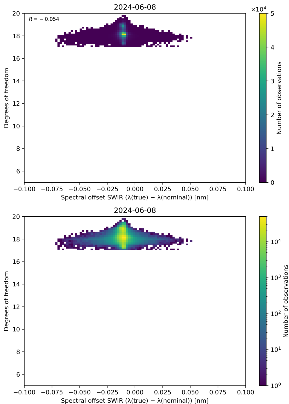
Figure 119: Scatter density plot of “Spectral offset SWIR ( \lambda(\text{true}) - \lambda(\text{nominal}) )” against “Degrees of freedom” for 2024-06-08 to 2024-06-09.
