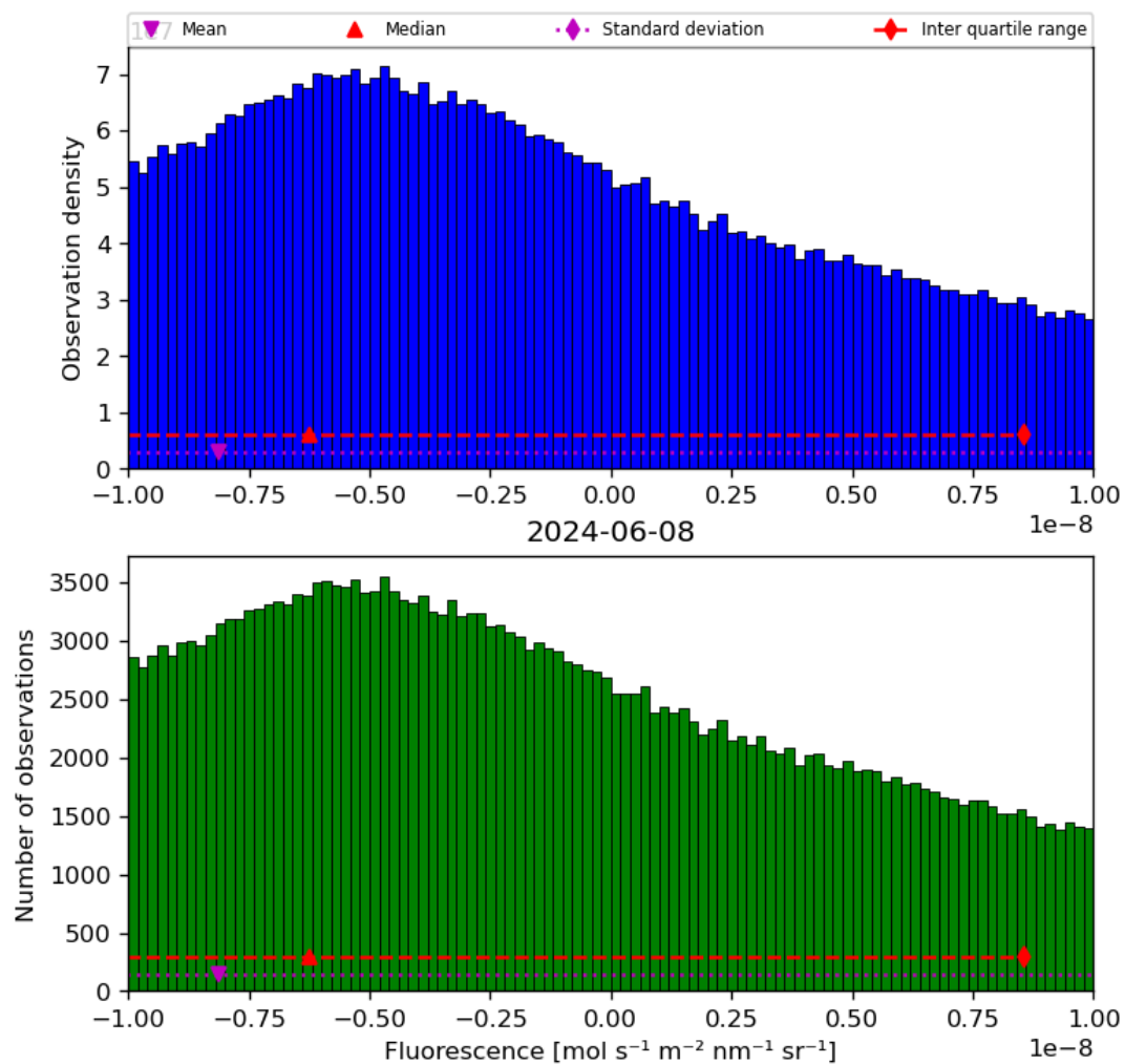
Figure 32: Histogram of “Fluorescence” for 2024-06-08 to 2024-06-09
