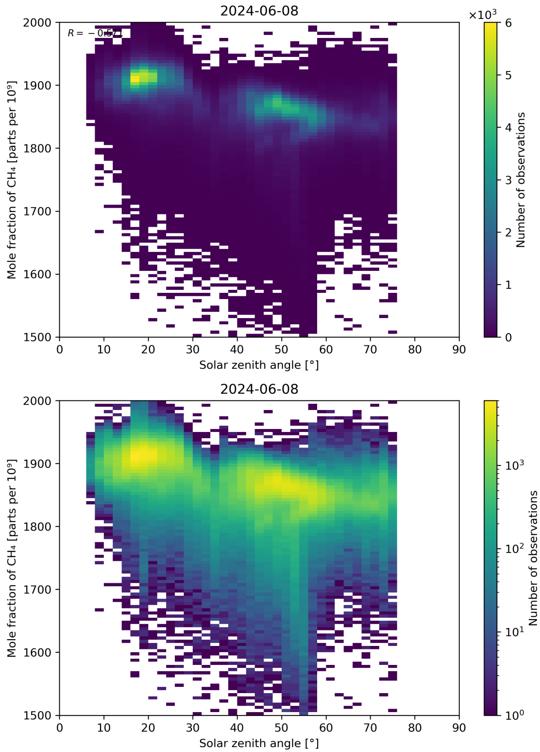
Figure 99: Scatter density plot of “Solar zenith angle” against “Mole fraction of CH 4 ” for 2024-06-08 to 2024-06-09.
