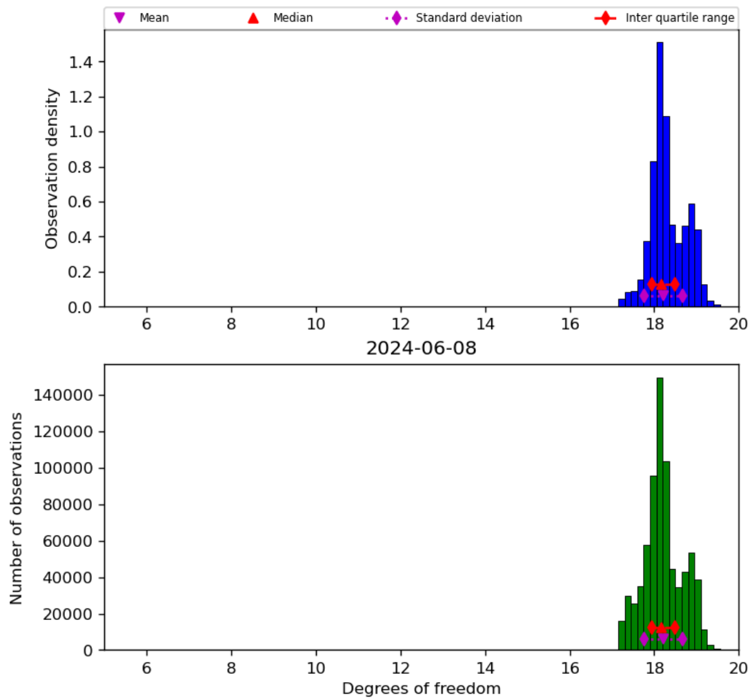
Figure 30: Histogram of “Degrees of freedom” for 2024-06-08 to 2024-06-09
