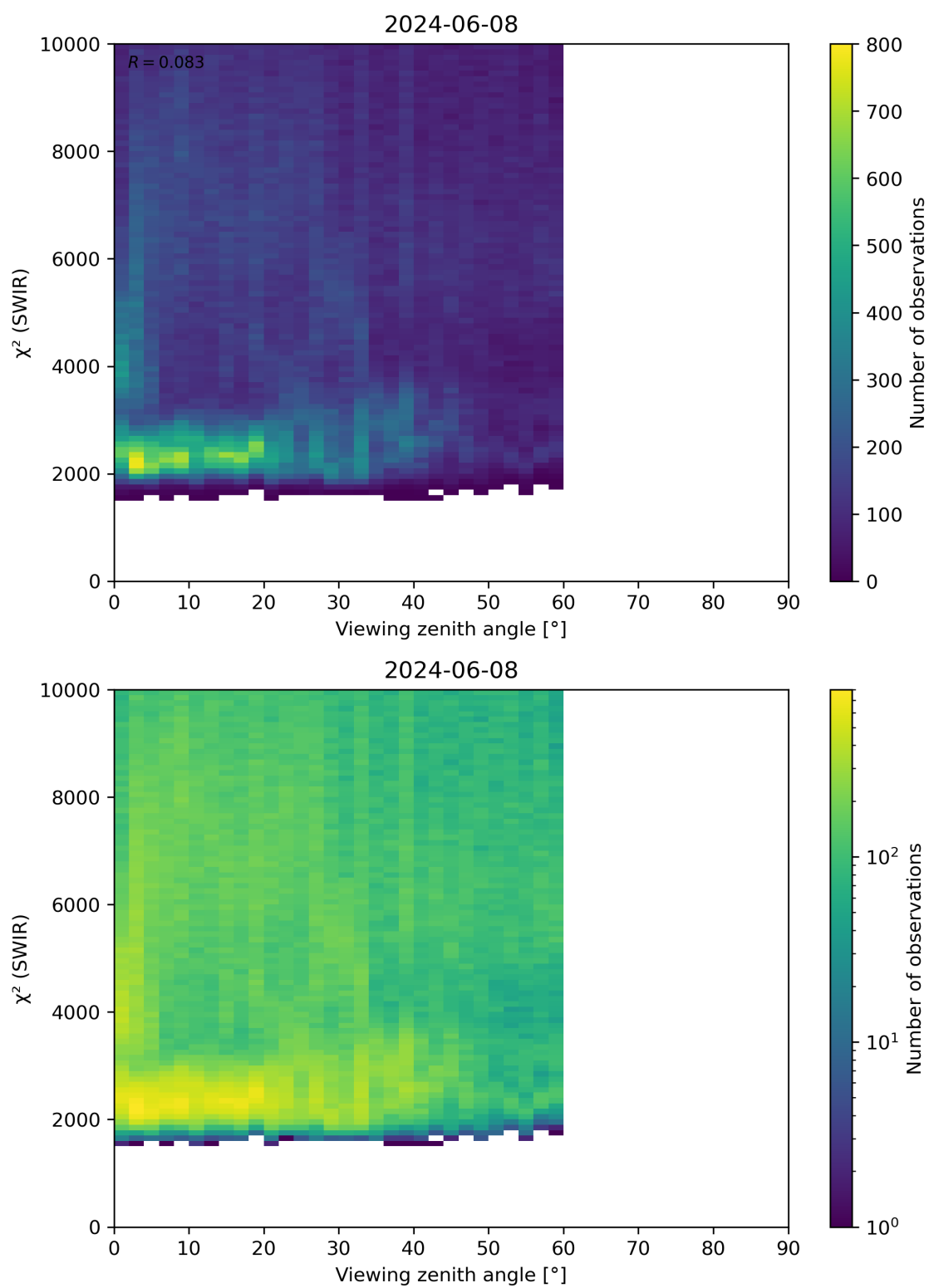
Figure 106: Scatter density plot of “Viewing zenith angle” against “ \chi^2 (SWIR)” for 2024-06-08 to 2024-06-09.
