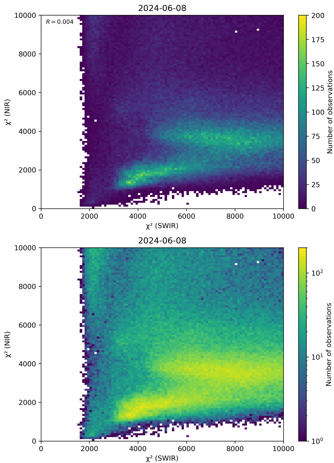
Figure 47: Scatter density plot of “ \chi^2 (SWIR)” against “ \chi^2 (NIR)” for 2024-06-08 to 2024-06-09.
