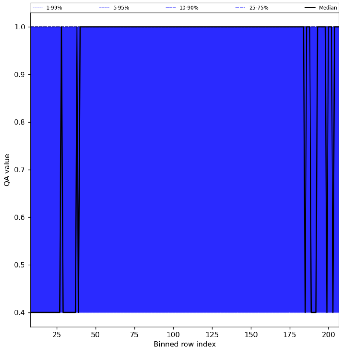
Figure 33: Along track statistics of “QA value” for 2024-06-08 to 2024-06-09
