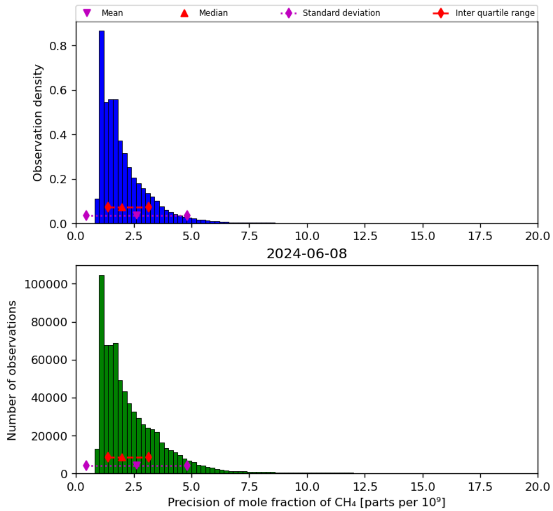
Figure 24: Histogram of “Precision of mole fraction of CH 4 ” for 2024-06-08 to 2024-06-09
