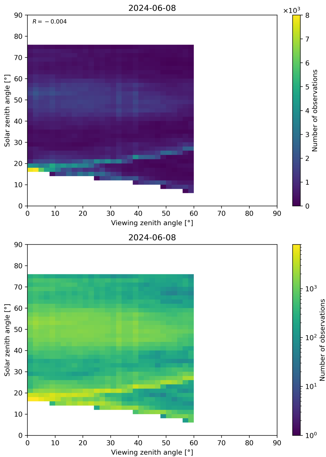
Figure 115: Scatter density plot of “Viewing zenith angle” against “Solar zenith angle” for 2024-06-08 to 2024-06-09.
