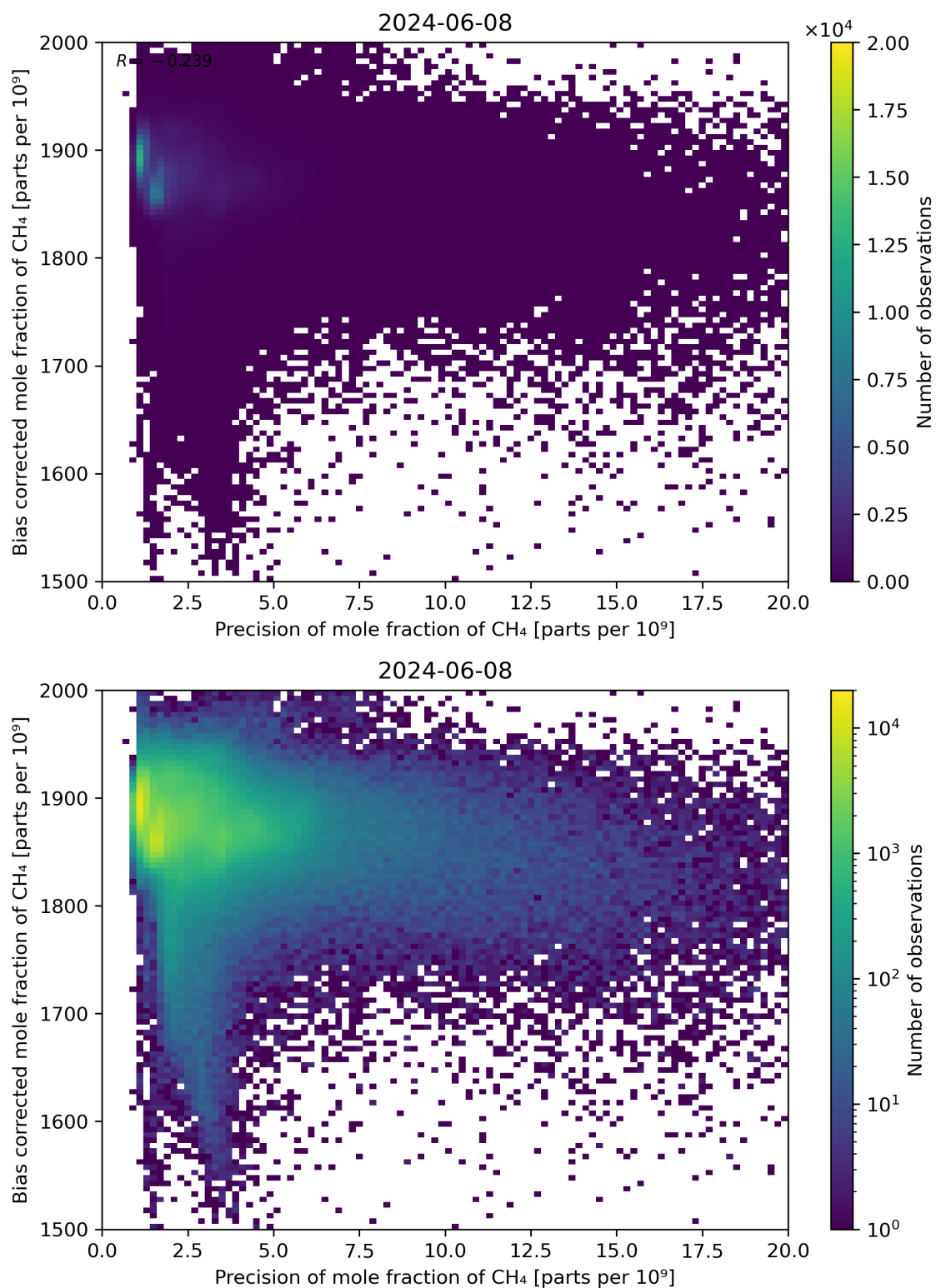
Figure 82: Scatter density plot of “Precision of mole fraction of CH 4 ” against “Bias corrected mole fraction of CH 4 ” for 2024-06-08 to 2024-06-09.
