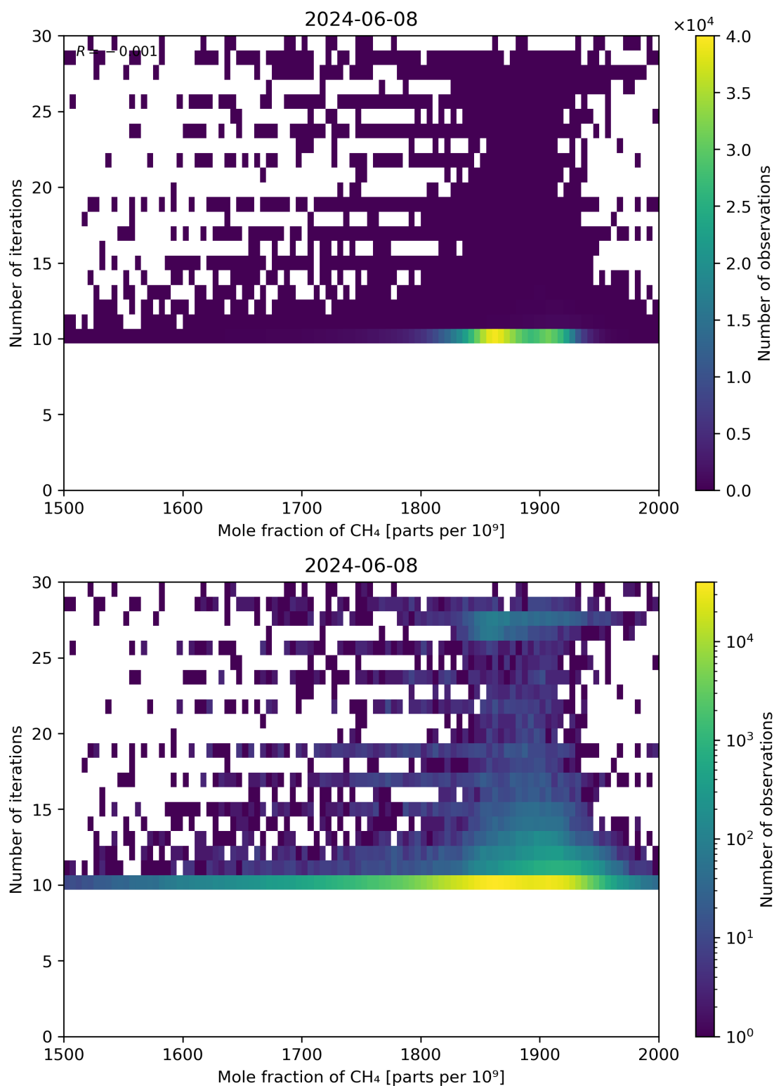
Figure 76: Scatter density plot of “Mole fraction of CH 4 ” against “Number of iterations” for 2024-06-08 to 2024-06-09.
