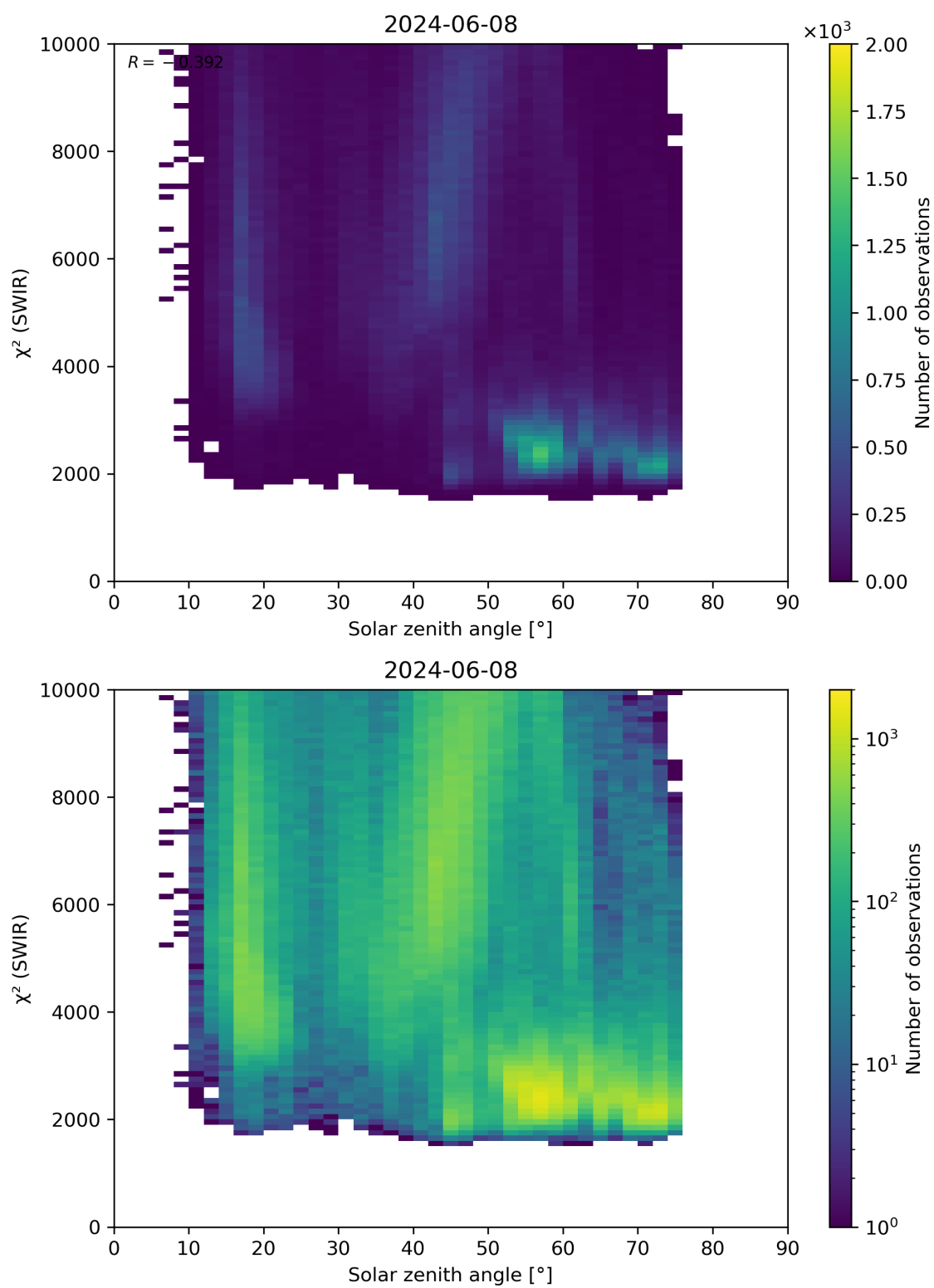
Figure 95: Scatter density plot of “Solar zenith angle” against “ \chi^2 (SWIR)” for 2024-06-08 to 2024-06-09.
