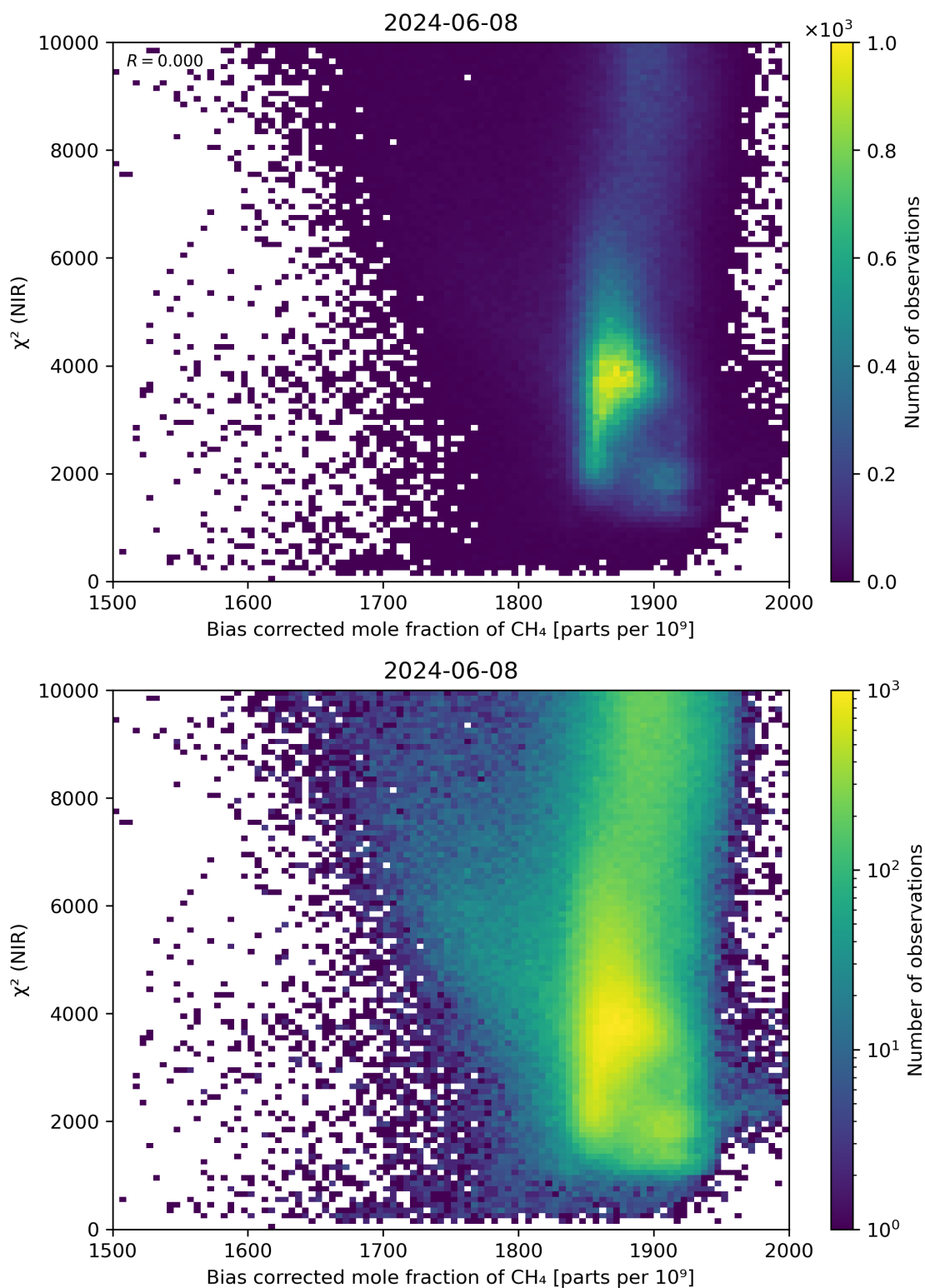
Figure 63: Scatter density plot of “Bias corrected mole fraction of CH 4 ” against “ \chi^2 (NIR)” for 2024-06-08 to 2024-06-09.
