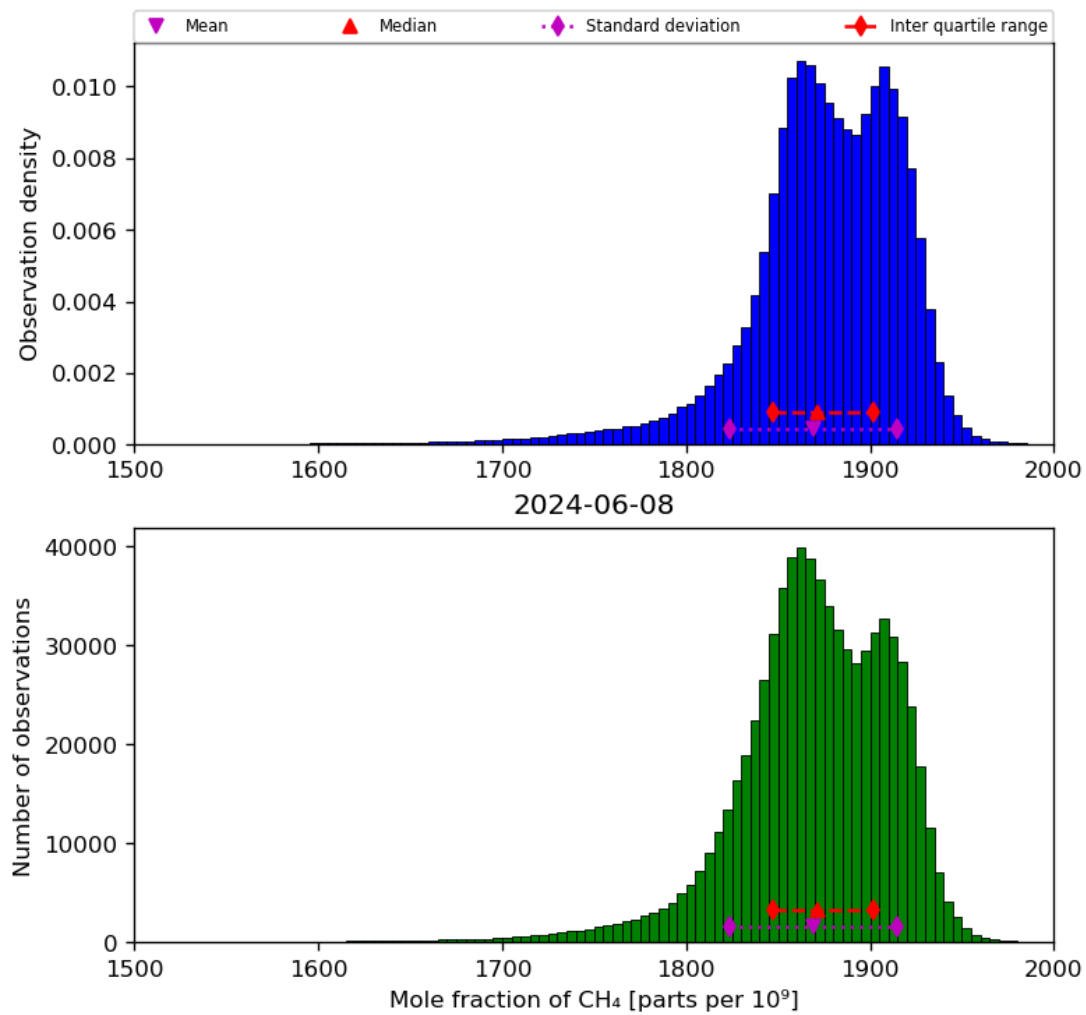
Figure 23: Histogram of “Mole fraction of CH 4 ” for 2024-06-08 to 2024-06-09
