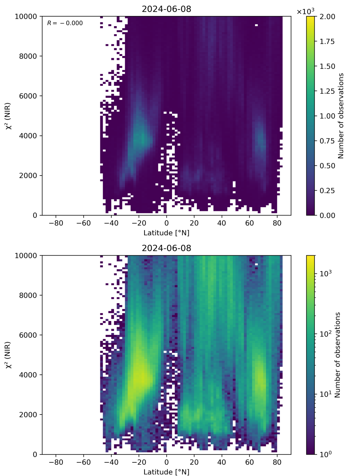
Figure 53: Scatter density plot of “Latitude” against “ \chi^2 (NIR)” for 2024-06-08 to 2024-06-09.
