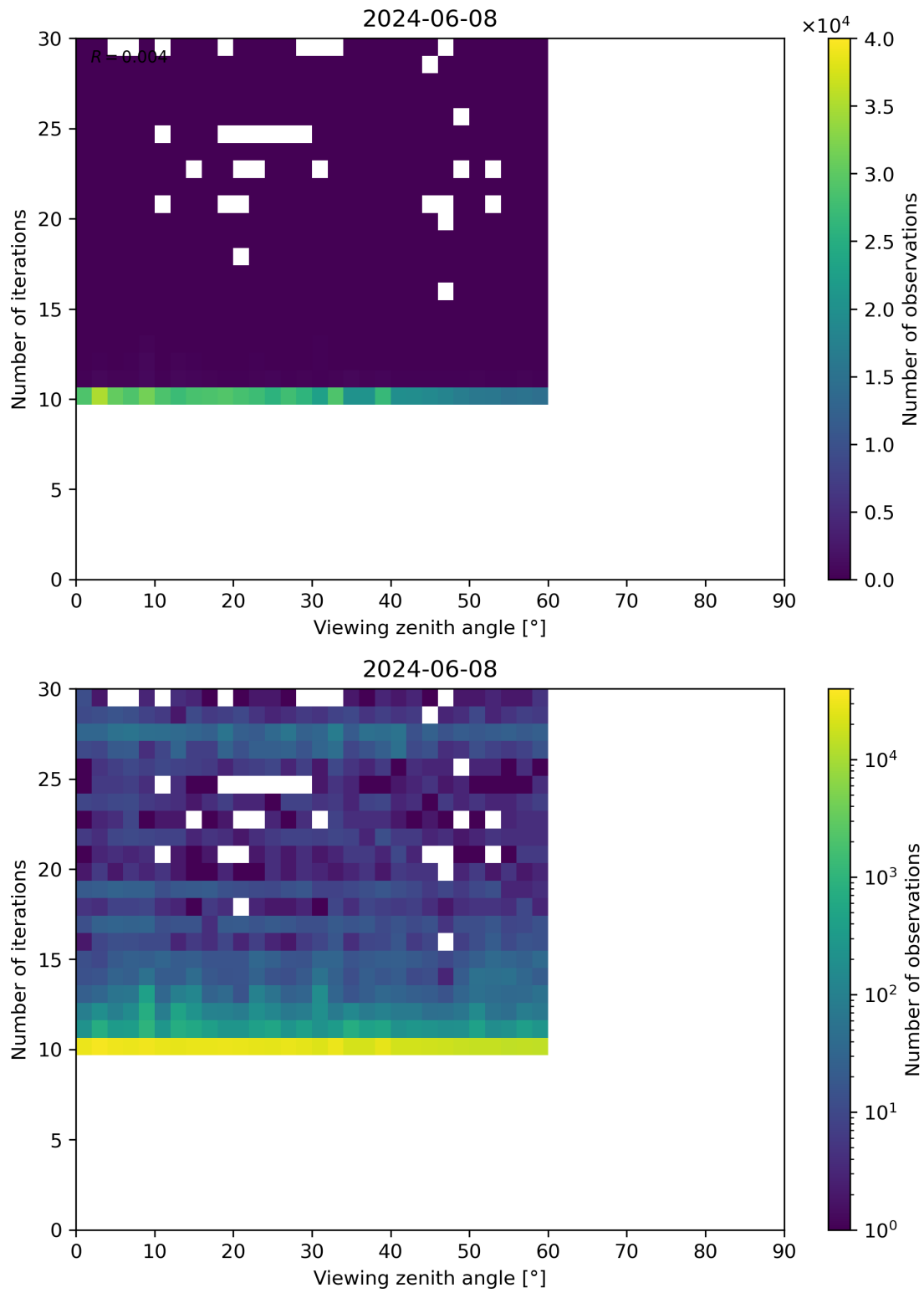
Figure 113: Scatter density plot of “Viewing zenith angle” against “Number of iterations” for 2024-06-08 to 2024-06-09.
