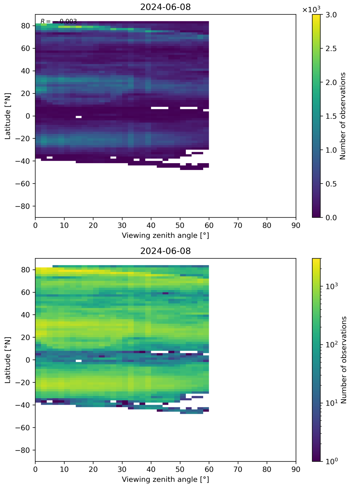
Figure 109: Scatter density plot of “Viewing zenith angle” against “Latitude” for 2024-06-08 to 2024-06-09.
