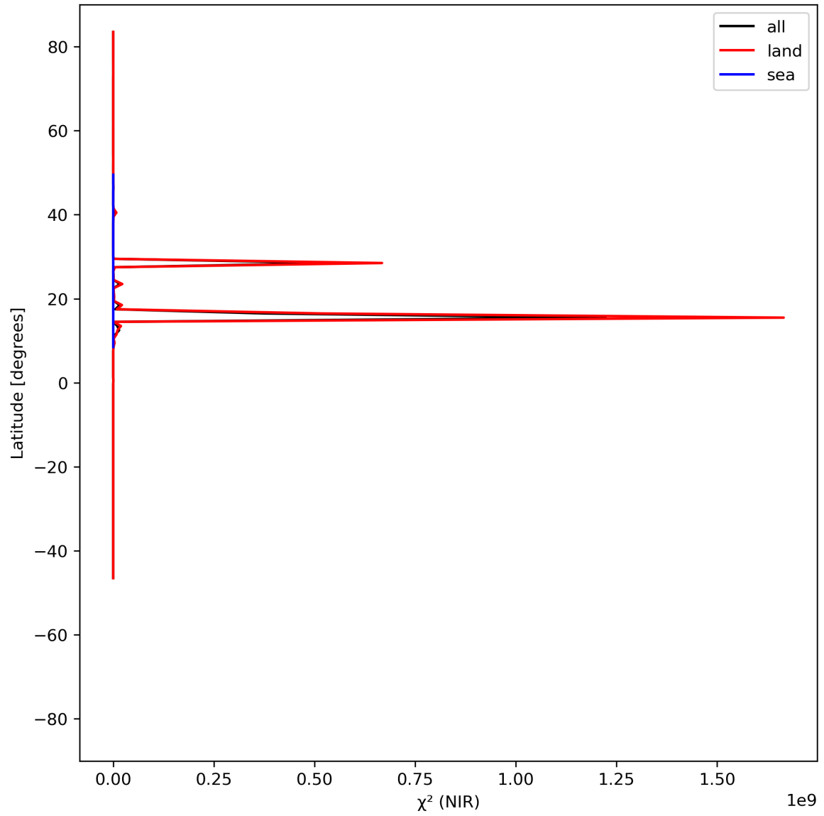
Figure 18: Zonal average of “ \chi^2 (NIR)” for 2024-06-08 to 2024-06-09.
