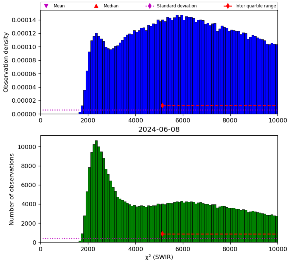
Figure 28: Histogram of “ \chi^2 (SWIR)” for 2024-06-08 to 2024-06-09
