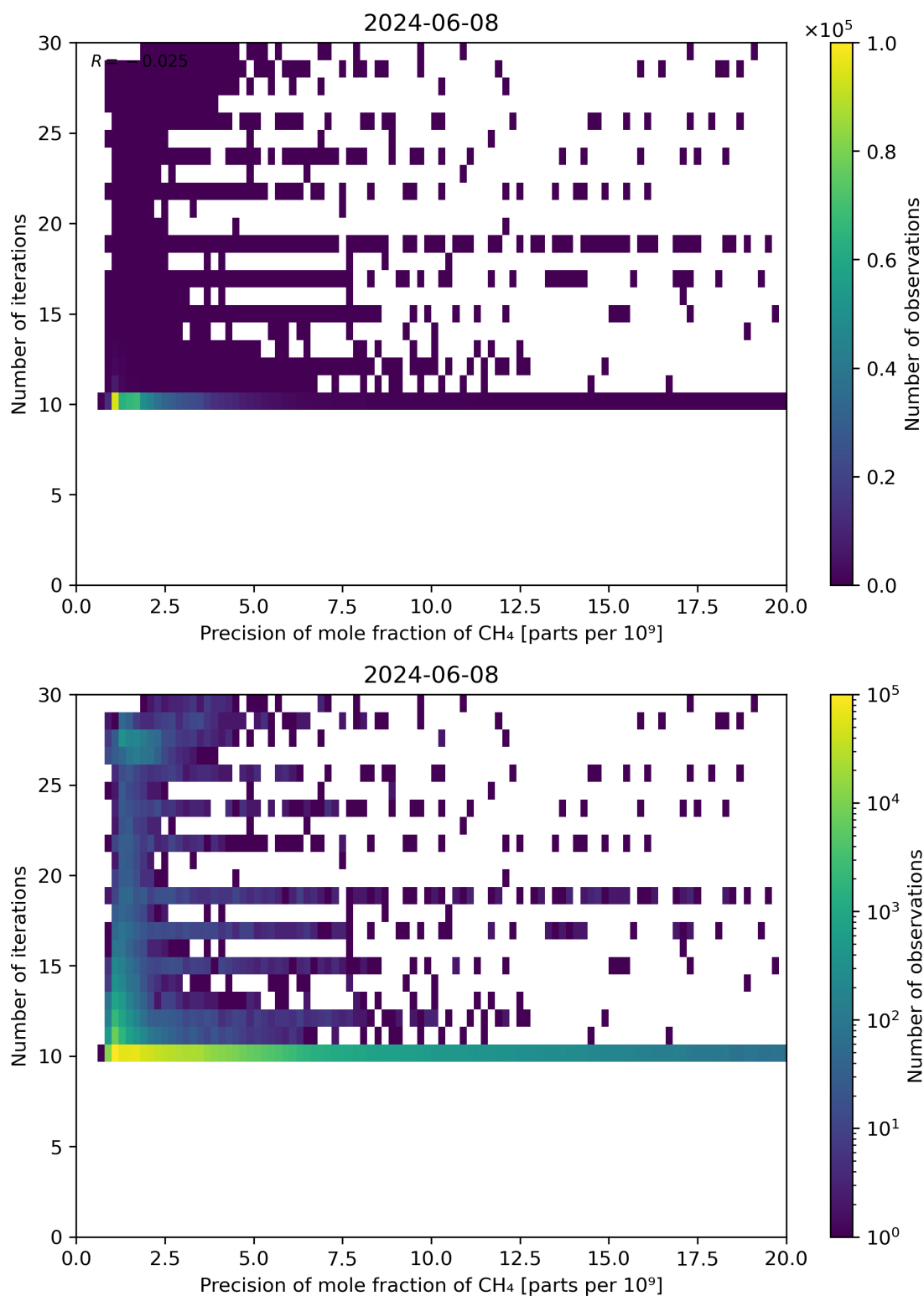
Figure 83: Scatter density plot of “Precision of mole fraction of CH 4 ” against “Number of iterations” for 2024-06-08 to 2024-06-09.
