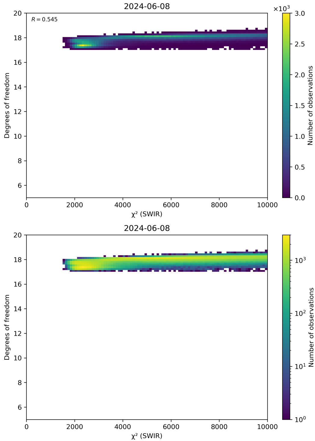
Figure 48: Scatter density plot of “ \chi^2 (SWIR)” against “Degrees of freedom” for 2024-06-08 to 2024-06-09.
