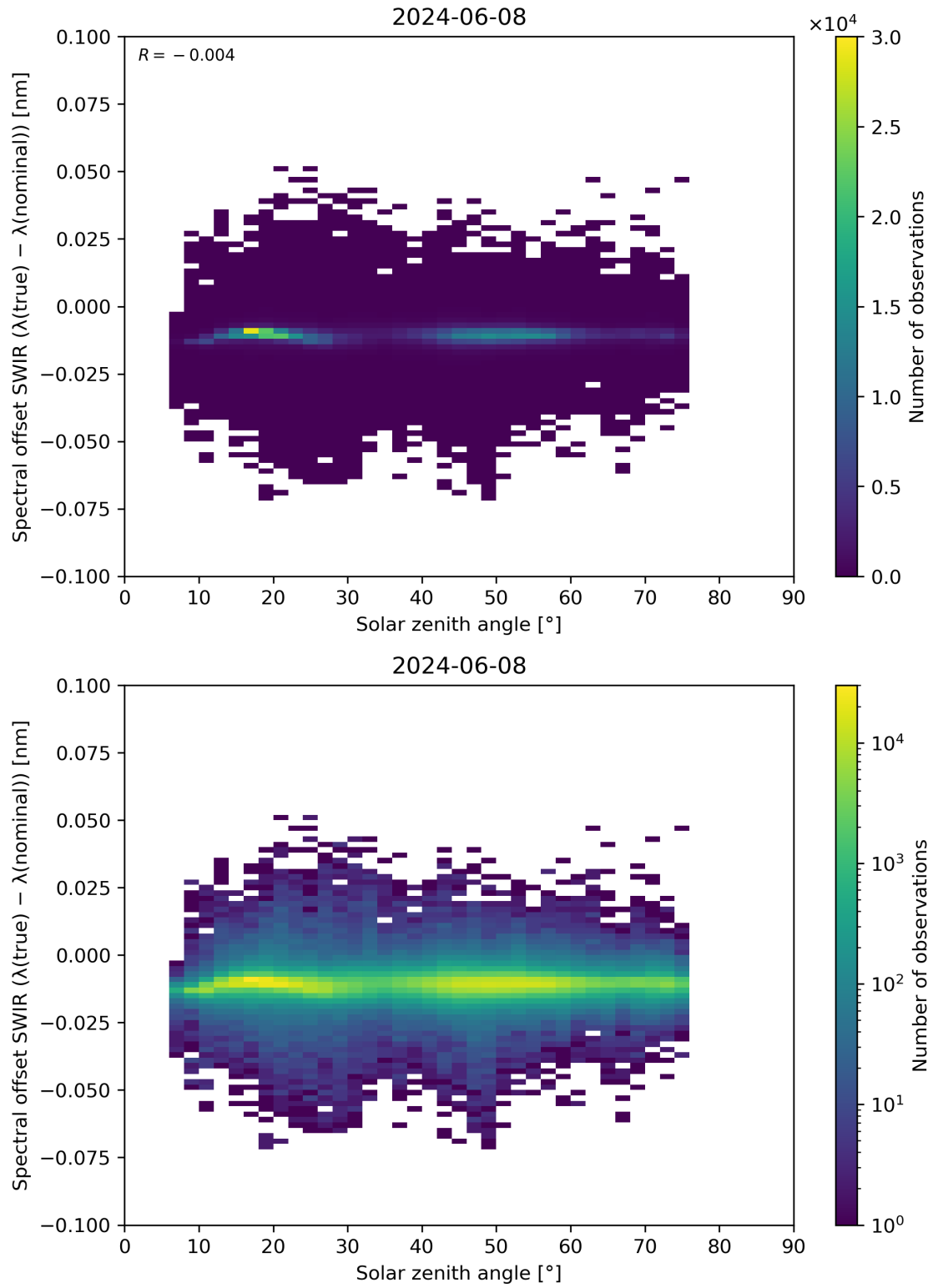
Figure 104: Scatter density plot of “Solar zenith angle” against “Spectral offset SWIR ( \lambda(\text{true}) - \lambda(\text{nominal}) )” for 2024-06-08 to 2024-06-09.
