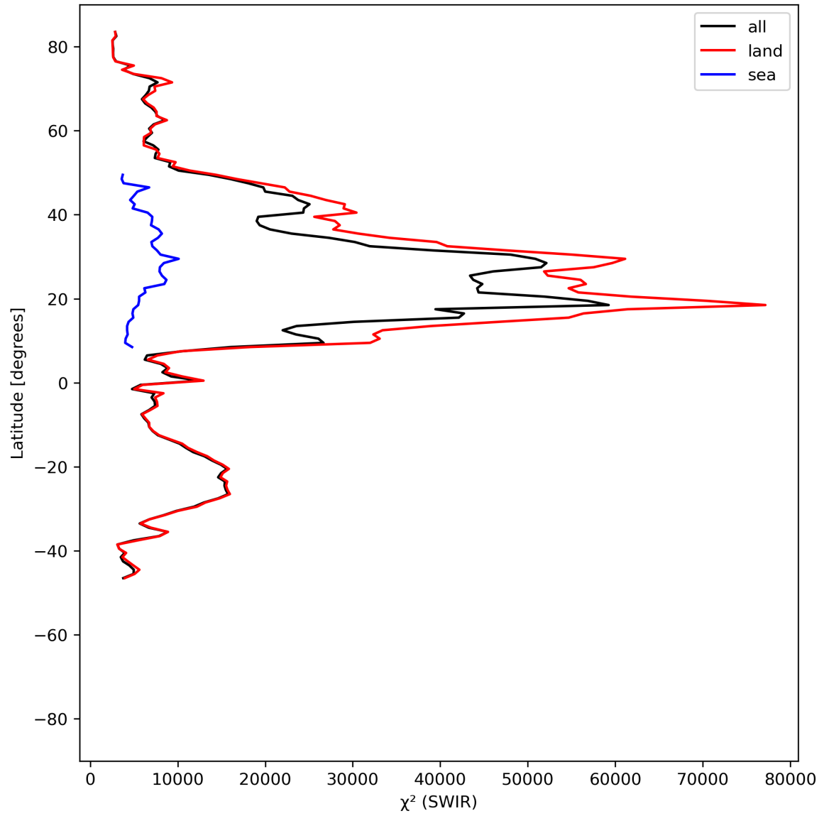
Figure 17: Zonal average of “ \chi^2 (SWIR)” for 2024-06-08 to 2024-06-09.
