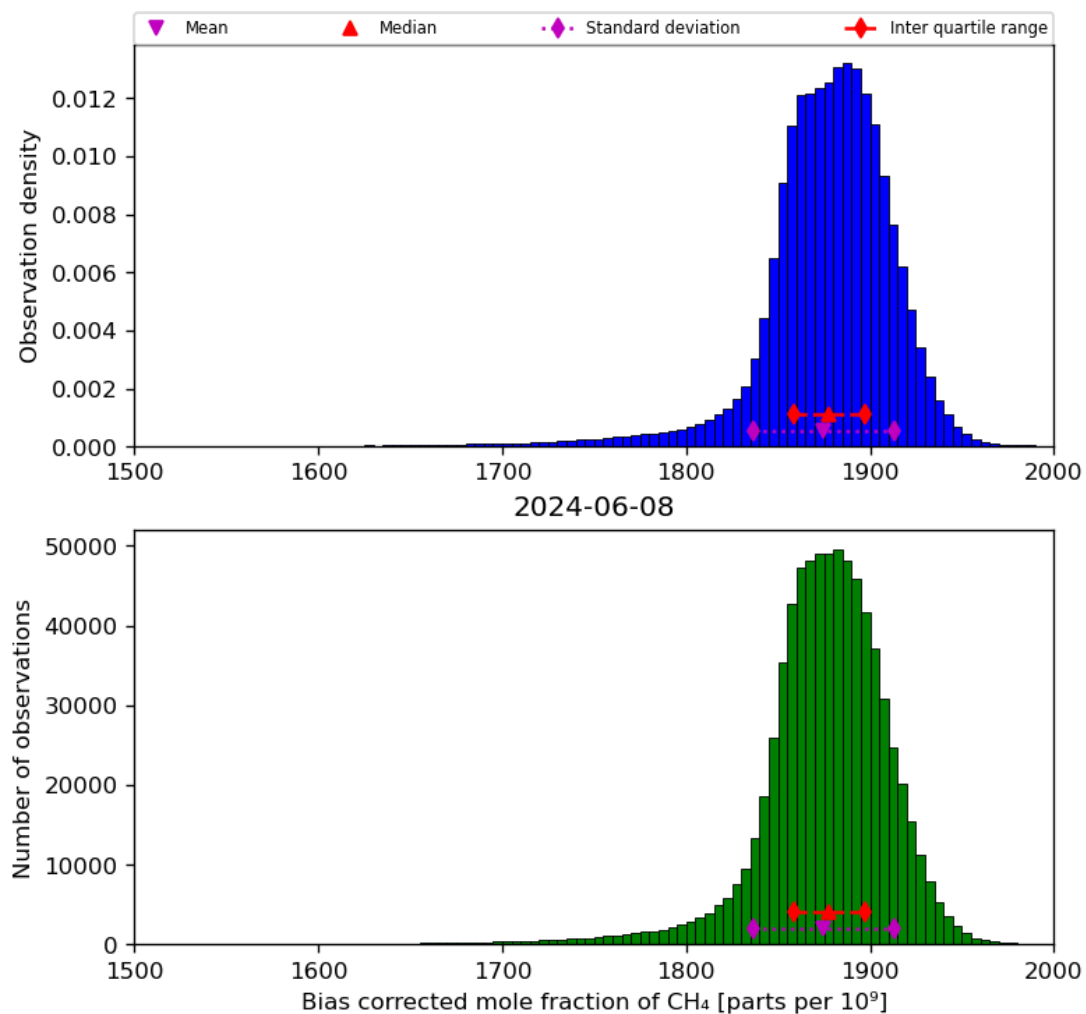
Figure 25: Histogram of “Bias corrected mole fraction of CH 4 ” for 2024-06-08 to 2024-06-09
