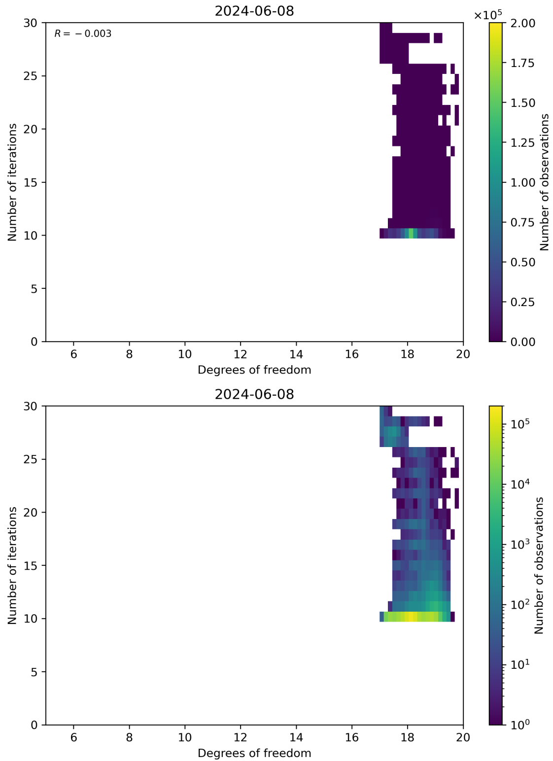
Figure 52: Scatter density plot of “Degrees of freedom” against “Number of iterations” for 2024-06-08 to 2024-06-09.
