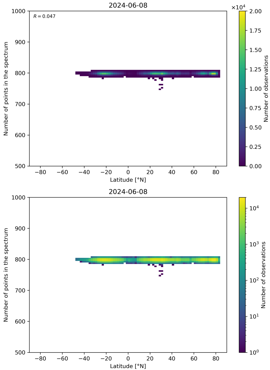
Figure 61: Scatter density plot of “Latitude” against “Number of points in the spectrum” for 2024-06-08 to 2024-06-09.
