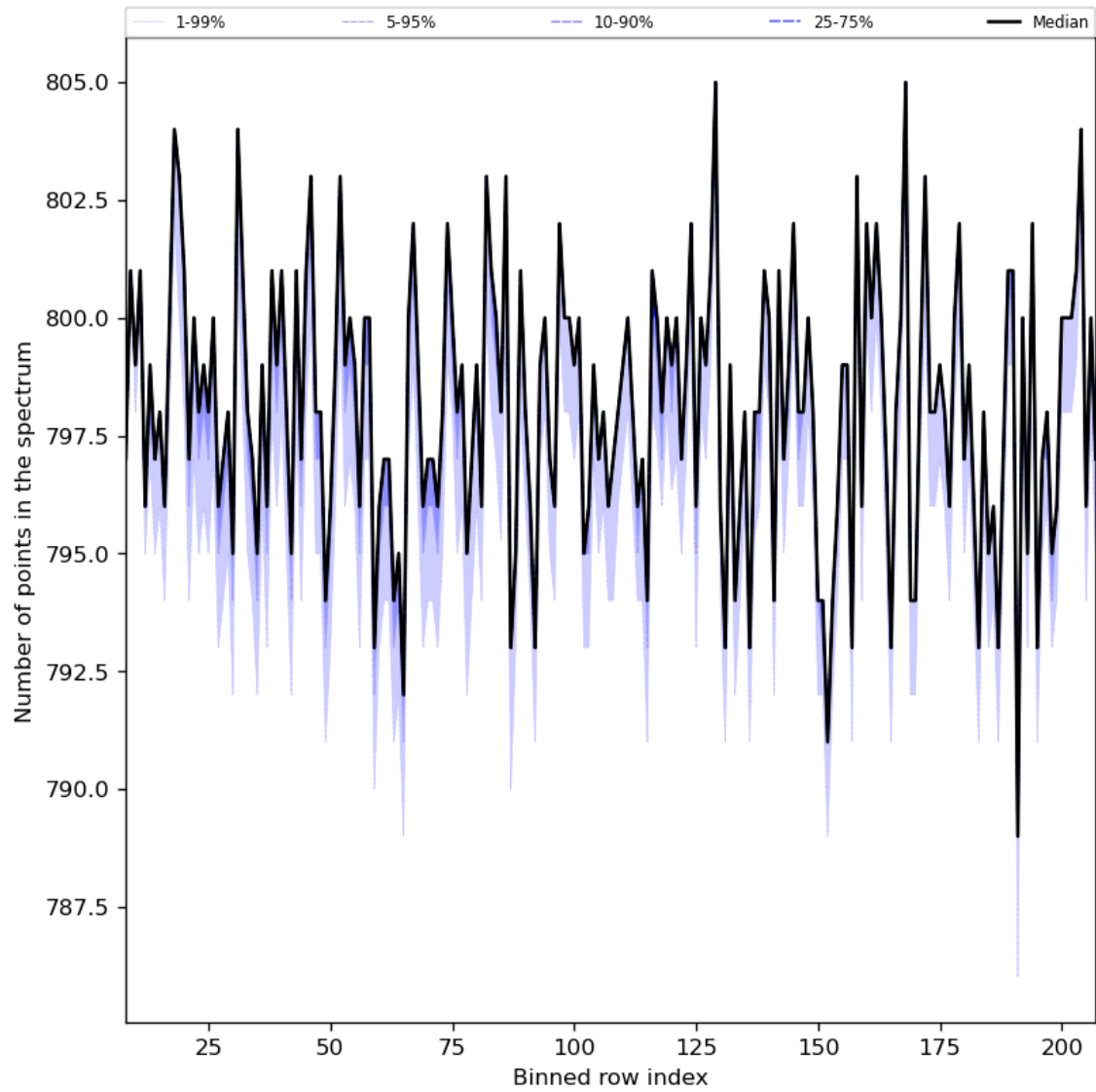
Figure 37: Along track statistics of “Number of points in the spectrum” for 2024-06-08 to 2024-06-09
