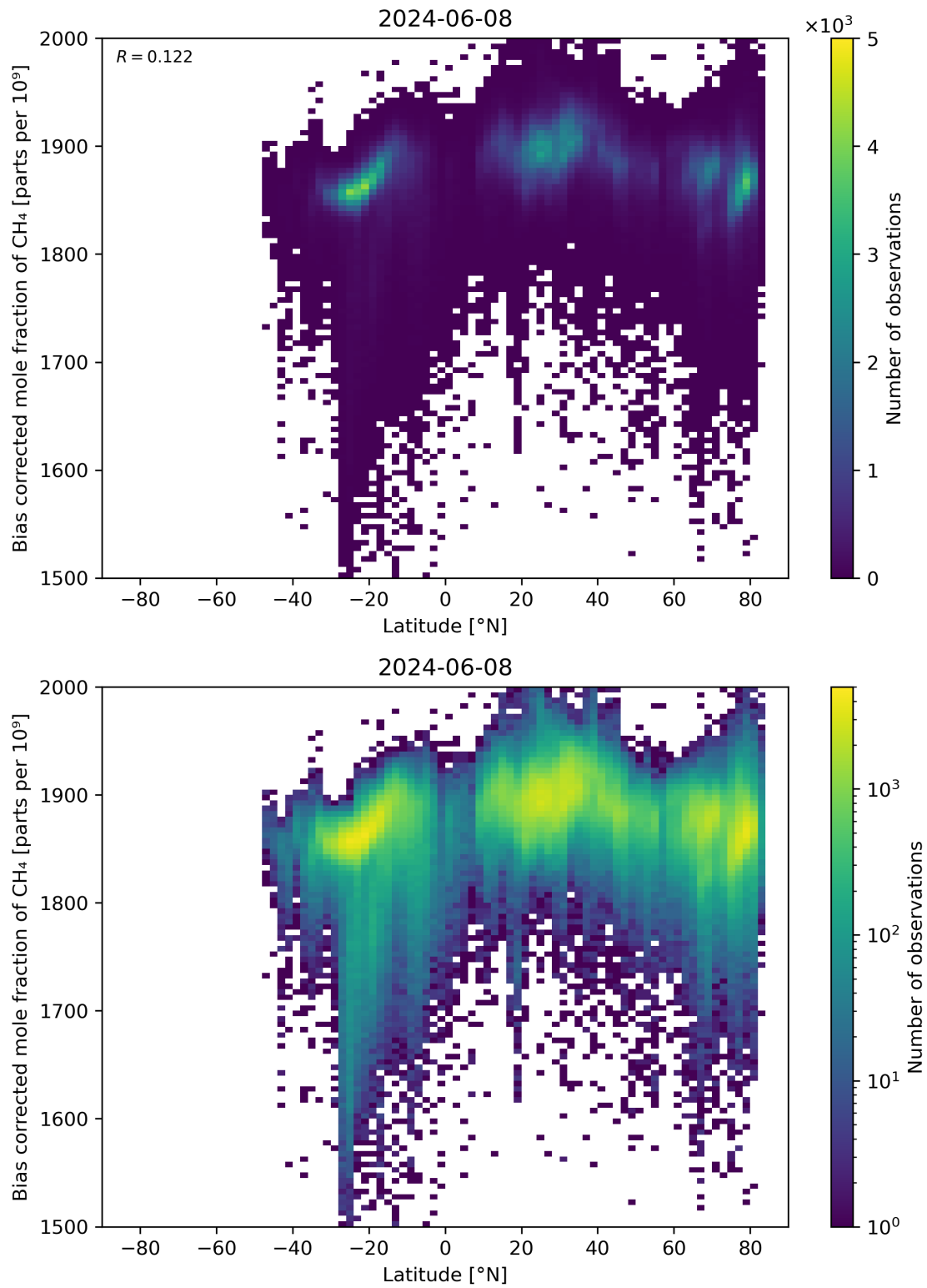
Figure 58: Scatter density plot of “Latitude” against “Bias corrected mole fraction of \text{CH}_4 ” for 2024-06-08 to 2024-06-09.
