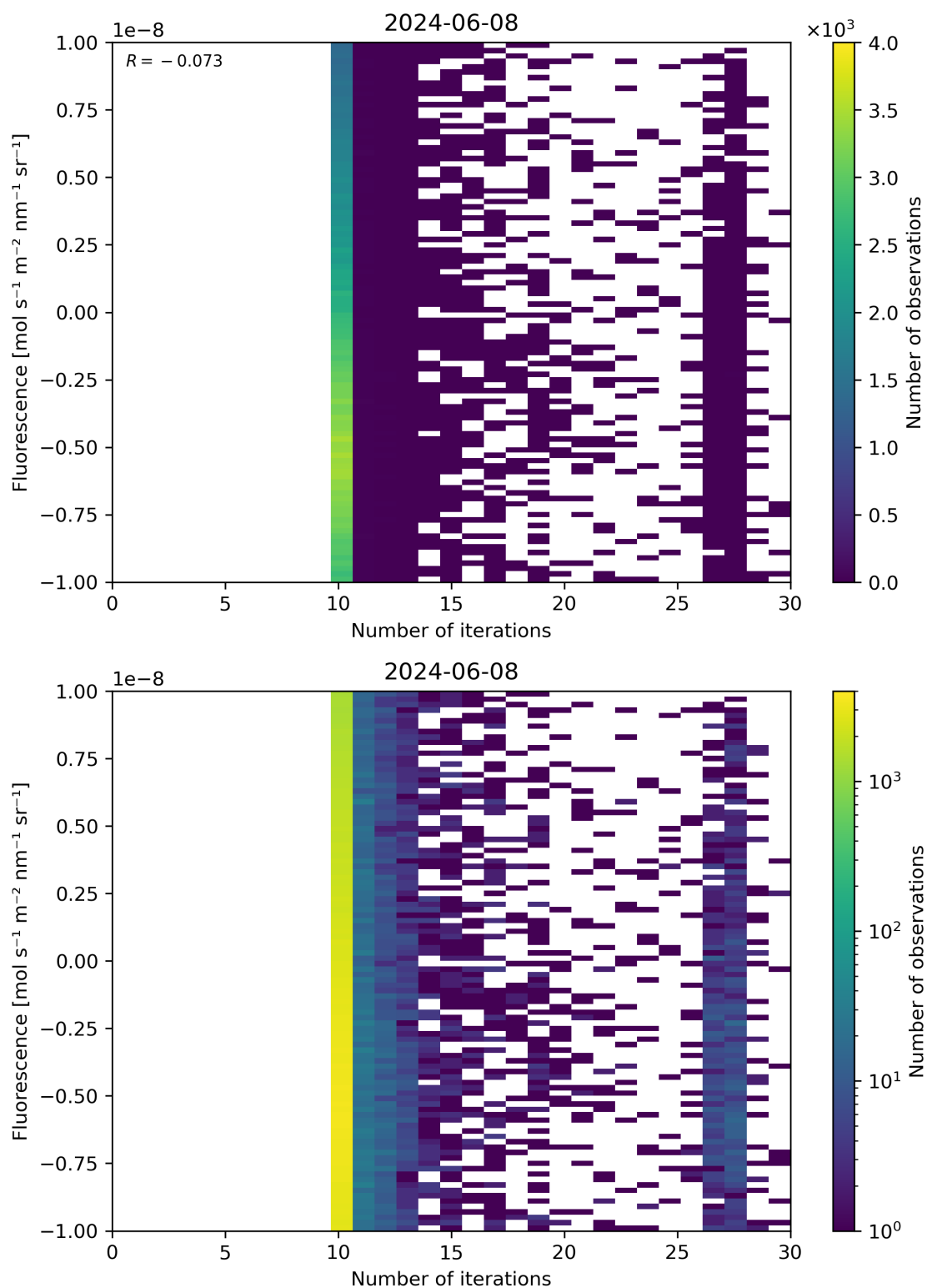
Figure 87: Scatter density plot of “Number of iterations” against “Fluorescence” for 2024-06-08 to 2024-06-09.
