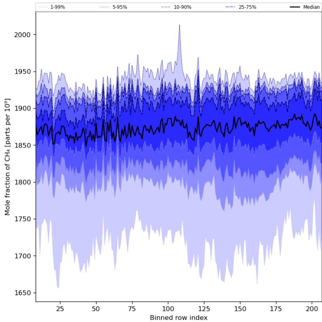
Figure 34: Along track statistics of “Mole fraction of CH 4 ” for 2024-06-08 to 2024-06-09
