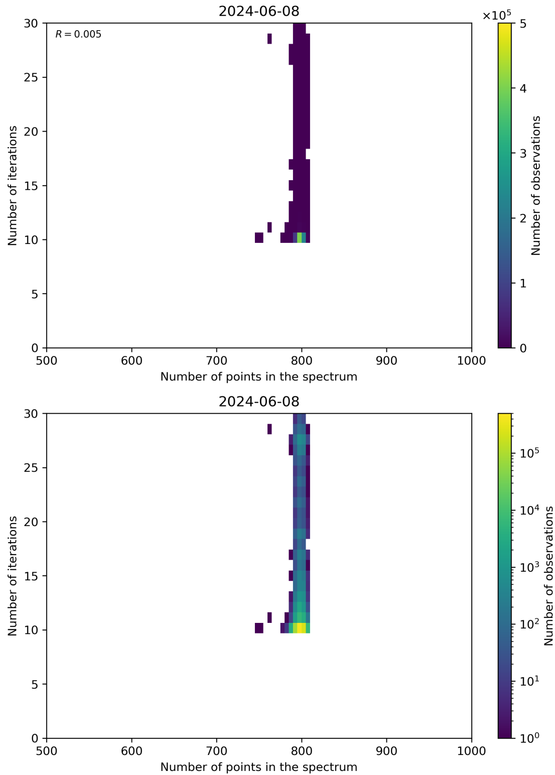
Figure 92: Scatter density plot of “Number of points in the spectrum” against “Number of iterations” for 2024-06-08 to 2024-06-09.
