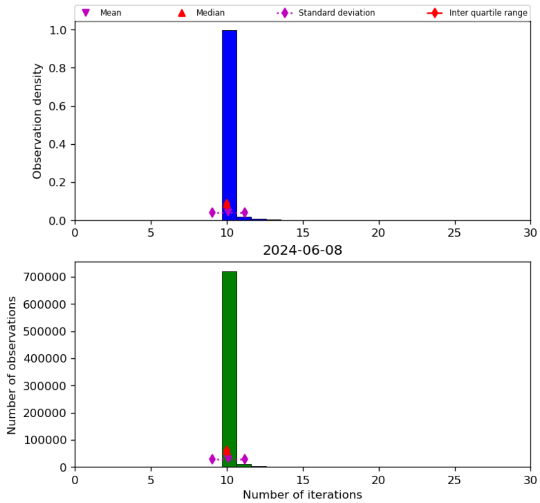
Figure 31: Histogram of “Number of iterations” for 2024-06-08 to 2024-06-09
