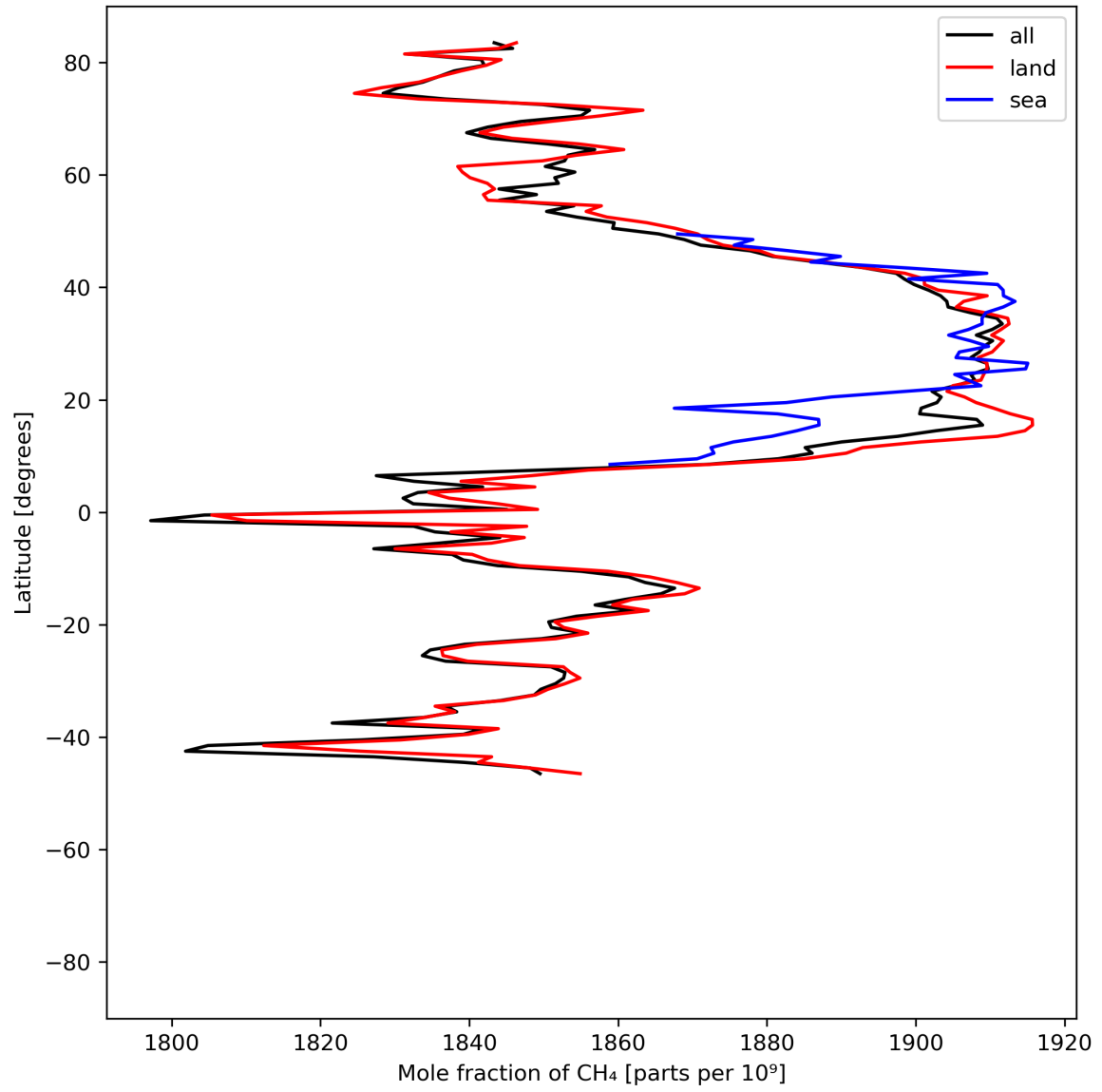
Figure 12: Zonal average of “Mole fraction of \text{CH}_4 ” for 2024-06-08 to 2024-06-09.
