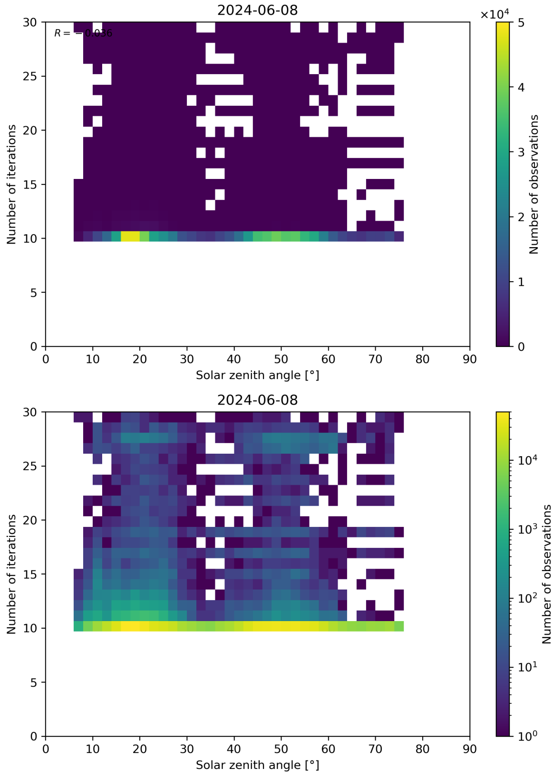
Figure 102: Scatter density plot of “Solar zenith angle” against “Number of iterations” for 2024-06-08 to 2024-06-09.
