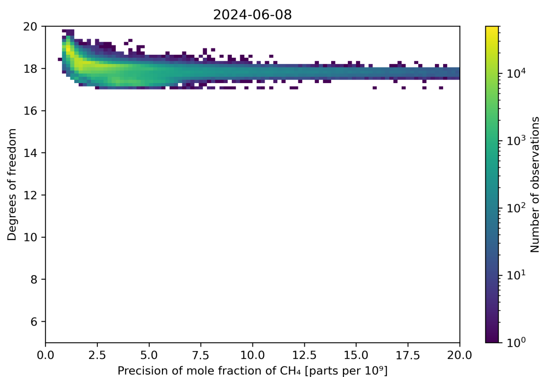
Figure 80: Scatter density plot of “Precision of mole fraction of CH 4 ” against “Degrees of freedom” for 2024-06-08 to 2024-06-09.
