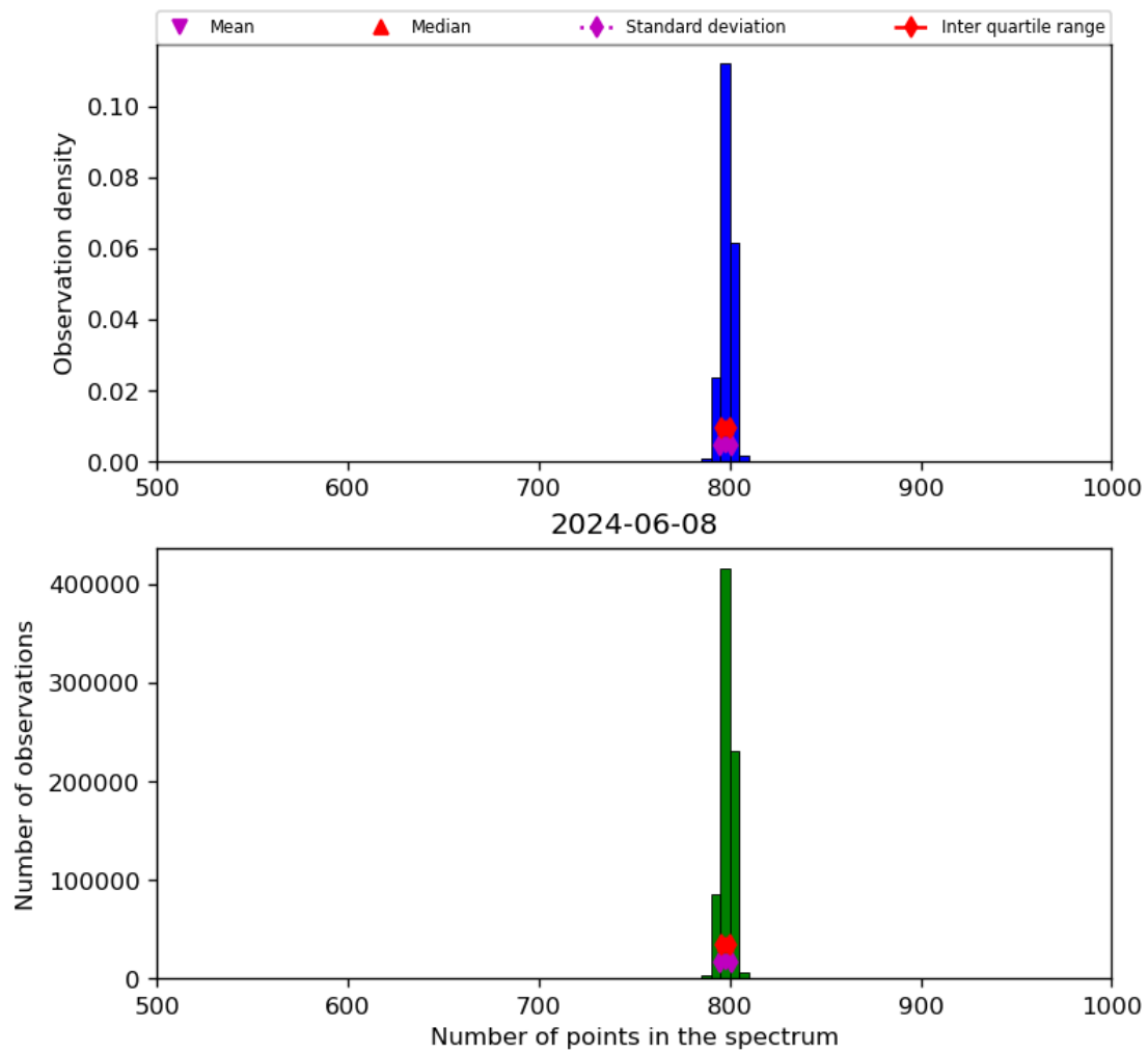
Figure 26: Histogram of “Number of points in the spectrum” for 2024-06-08 to 2024-06-09
