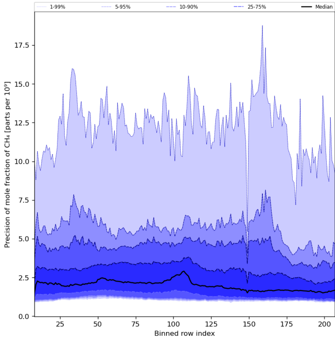
Figure 35: Along track statistics of “Precision of mole fraction of CH 4 ” for 2024-06-08 to 2024-06-09
