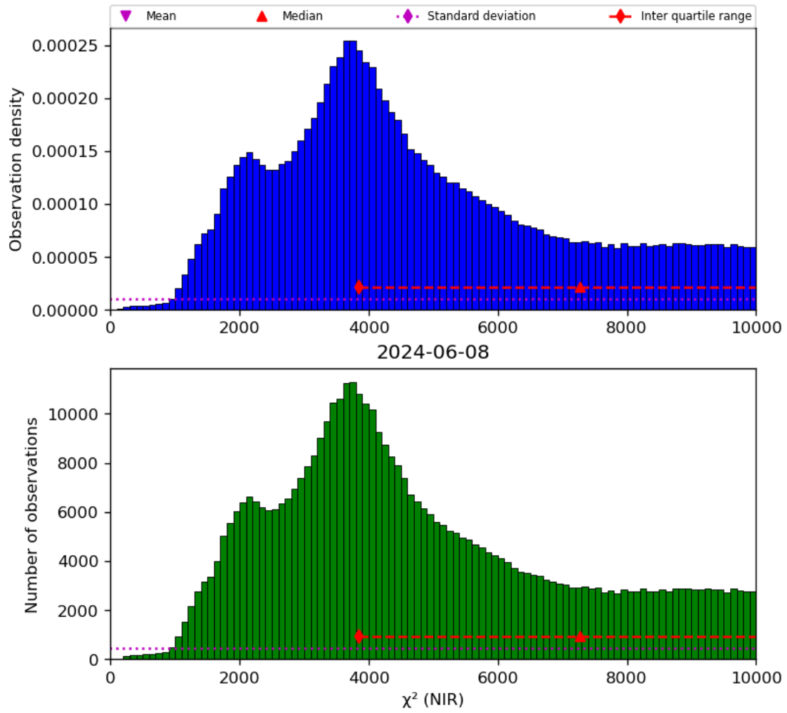
Figure 29: Histogram of " \chi^2 (NIR)" for 2024-06-08 to 2024-06-09
