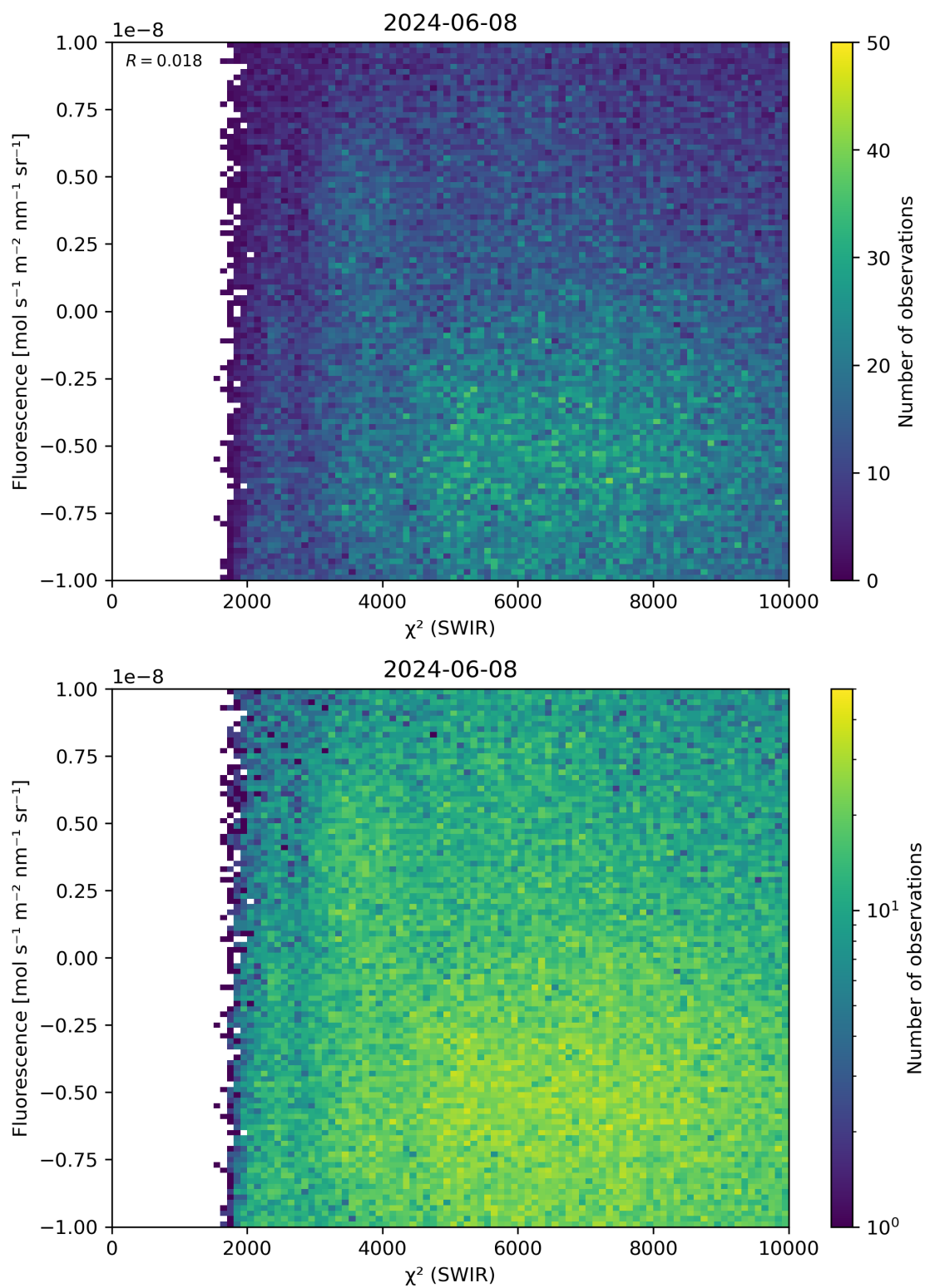
Figure 49: Scatter density plot of “ \chi^2 (SWIR)” against “Fluorescence” for 2024-06-08 to 2024-06-09.
