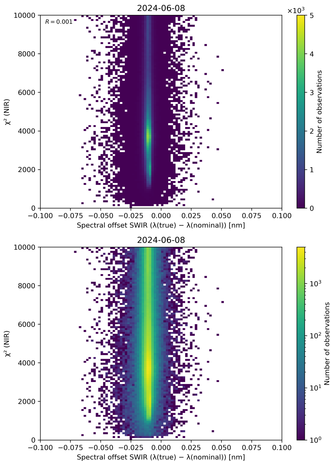
Figure 117: Scatter density plot of “Spectral offset SWIR ( \lambda(\text{true}) - \lambda(\text{nominal}) )” against “ \chi^2 (NIR)” for 2024-06-08 to 2024-06-09.
