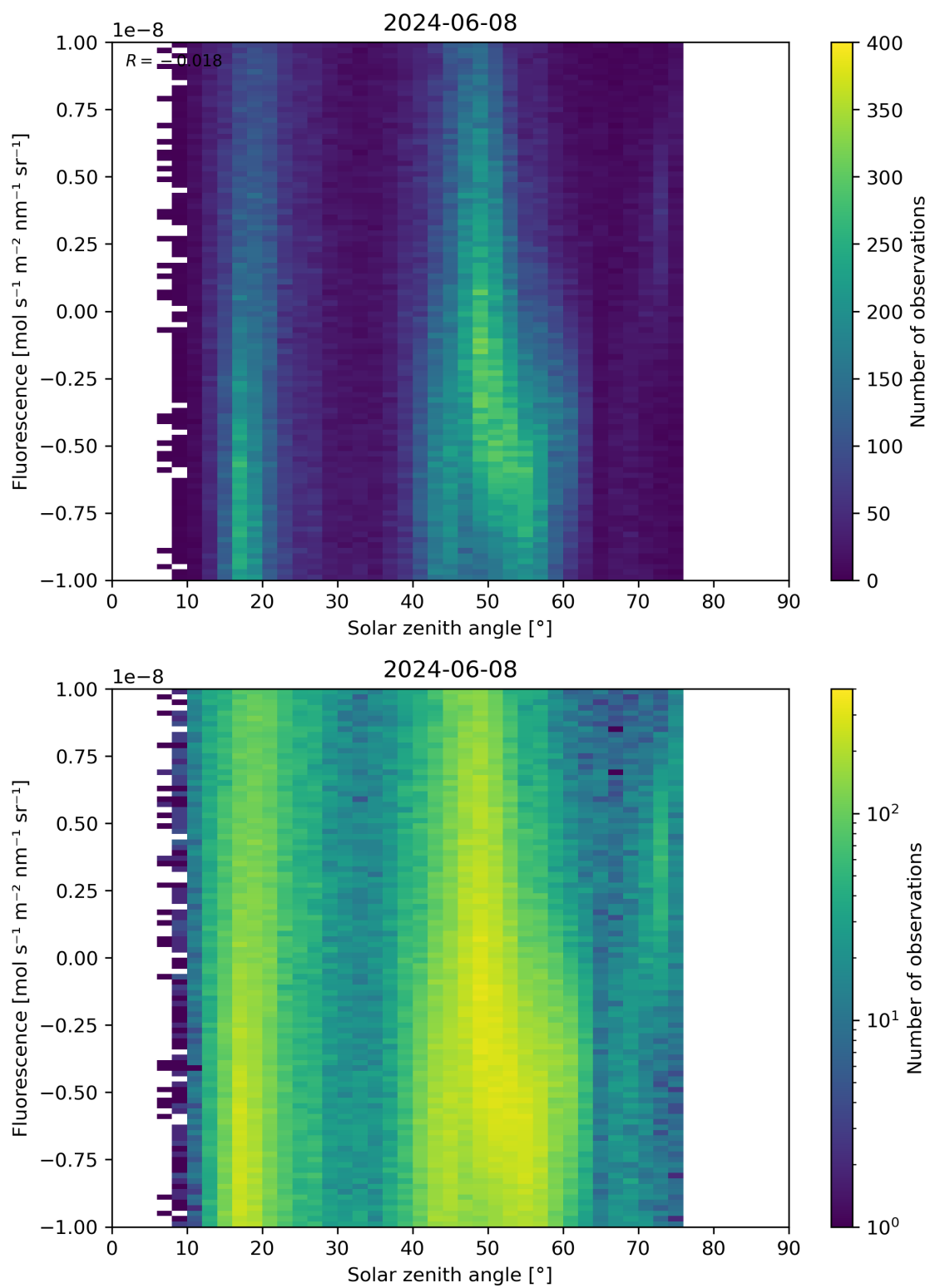
Figure 97: Scatter density plot of “Solar zenith angle” against “Fluorescence” for 2024-06-08 to 2024-06-09.
