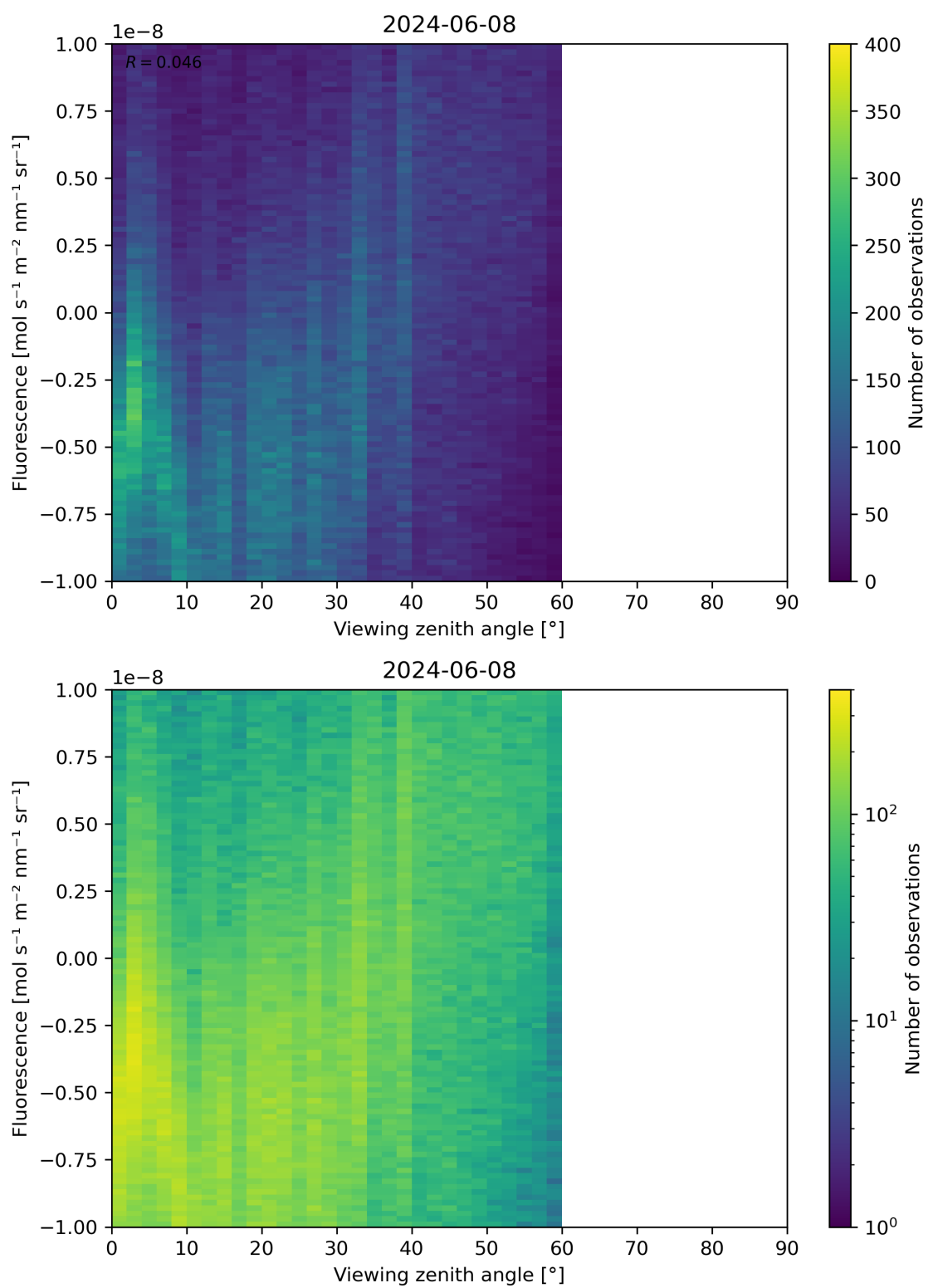
Figure 108: Scatter density plot of “Viewing zenith angle” against “Fluorescence” for 2024-06-08 to 2024-06-09.
