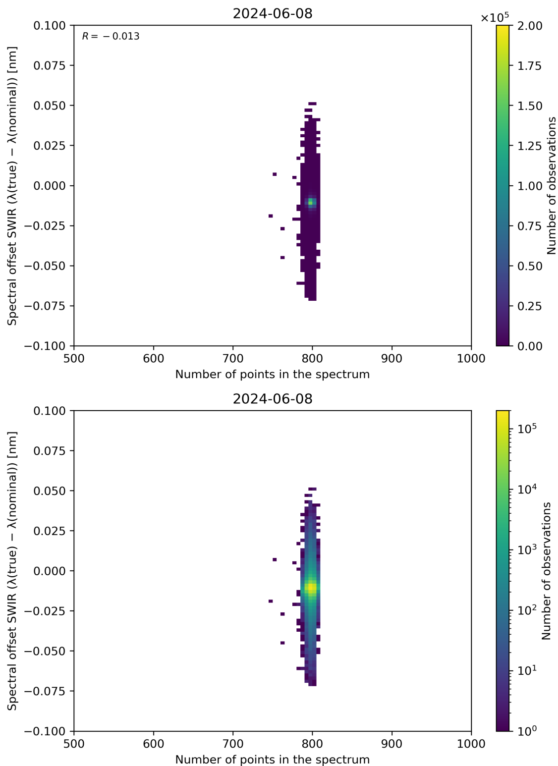
Figure 93: Scatter density plot of “Number of points in the spectrum” against “Spectral offset SWIR ( \lambda(\text{true}) - \lambda(\text{nominal}) )” for 2024-06-08 to 2024-06-09.
