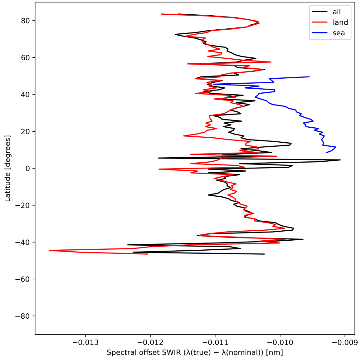
Figure 16: Zonal average of “Spectral offset SWIR ( \lambda(\text{true}) - \lambda(\text{nominal}) )” for 2024-06-08 to 2024-06-09.
