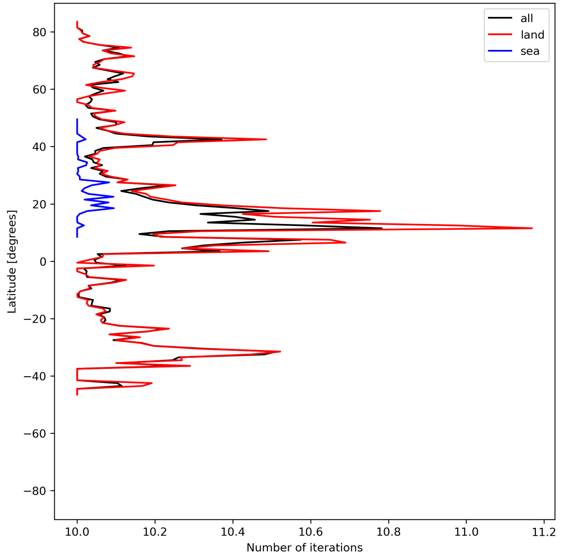
Figure 20: Zonal average of “Number of iterations” for 2024-06-08 to 2024-06-09.
