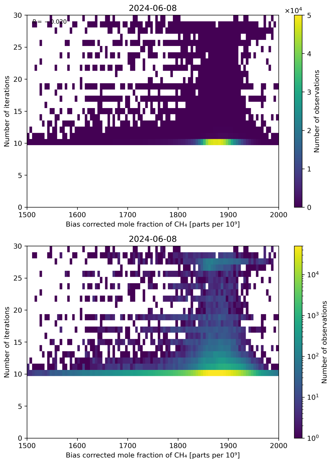
Figure 67: Scatter density plot of “Bias corrected mole fraction of CH 4 ” against “Number of iterations” for 2024-06-08 to 2024-06-09.
