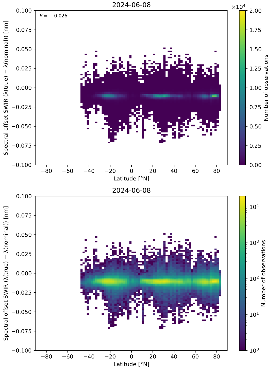
Figure 62: Scatter density plot of “Latitude” against “Spectral offset SWIR ( \lambda(\text{true}) - \lambda(\text{nominal}) )” for 2024-06-08 to 2024-06-09.
