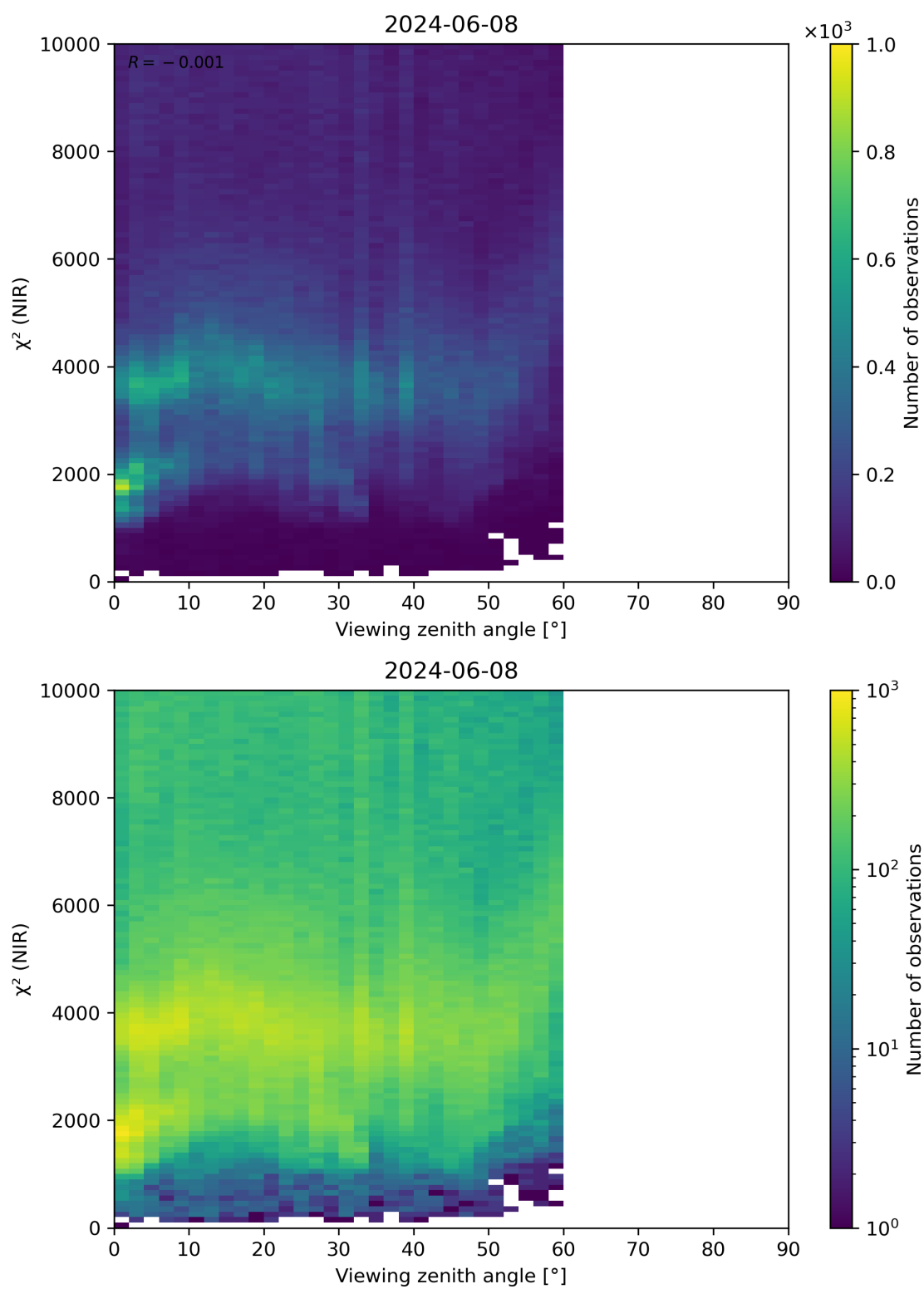
Figure 105: Scatter density plot of “Viewing zenith angle” against “ \chi^2 (NIR)” for 2024-06-08 to 2024-06-09.
