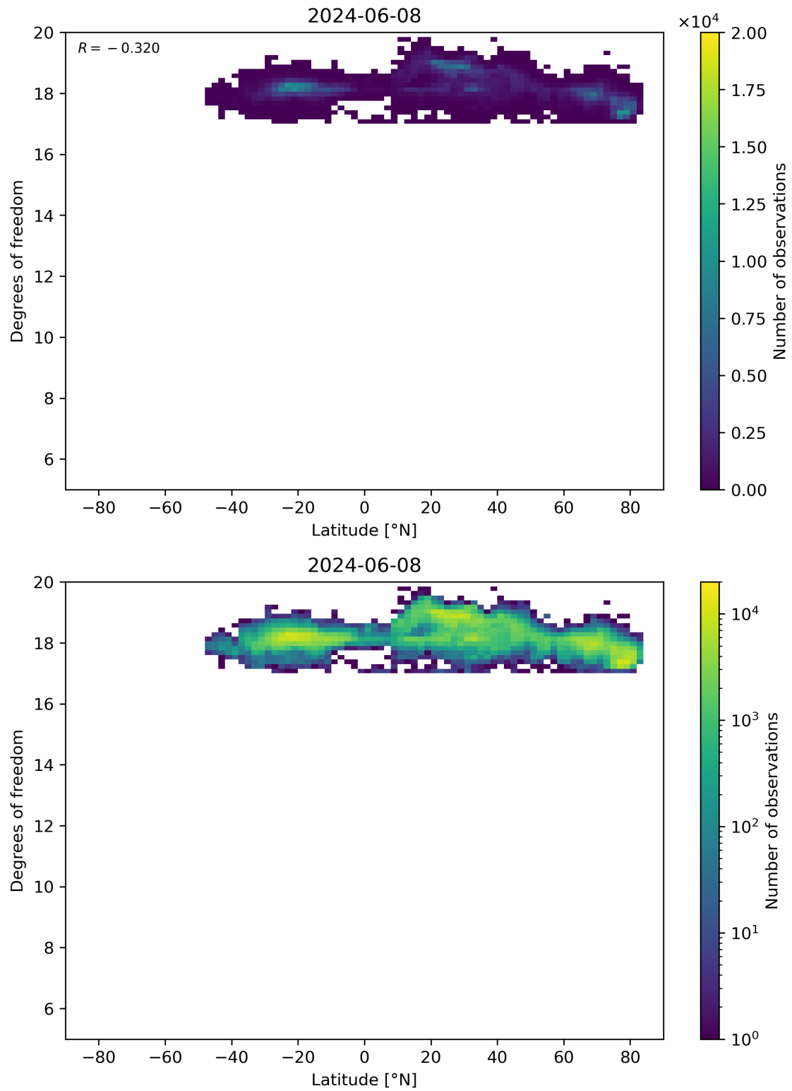
Figure 55: Scatter density plot of “Latitude” against “Degrees of freedom” for 2024-06-08 to 2024-06-09.
