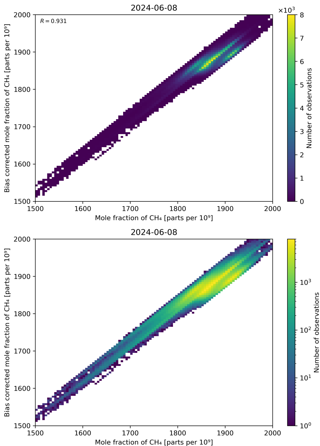
Figure 74: Scatter density plot of “Mole fraction of CH 4 ” against “Bias corrected mole fraction of CH 4 ” for 2024-06-08 to 2024-06-09.
