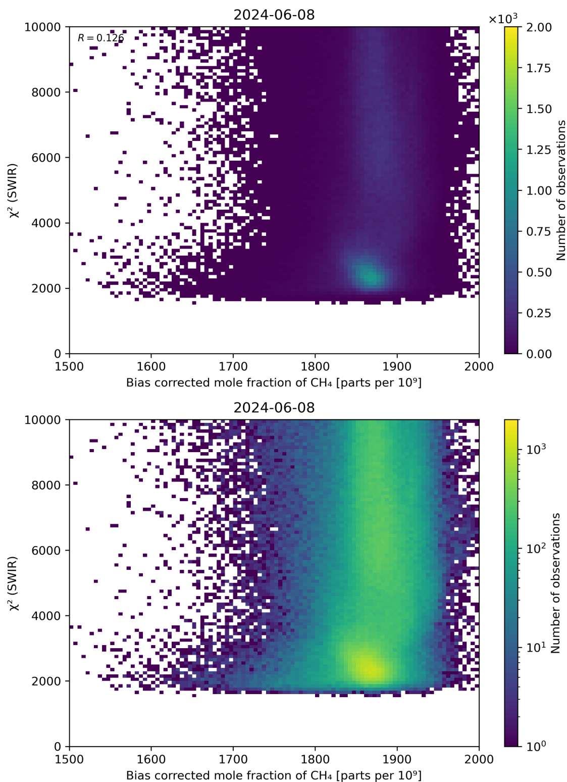
Figure 64: Scatter density plot of “Bias corrected mole fraction of \text{CH}_4 ” against “ \chi^2 (SWIR)” for 2024-06-08 to 2024-06-09.
