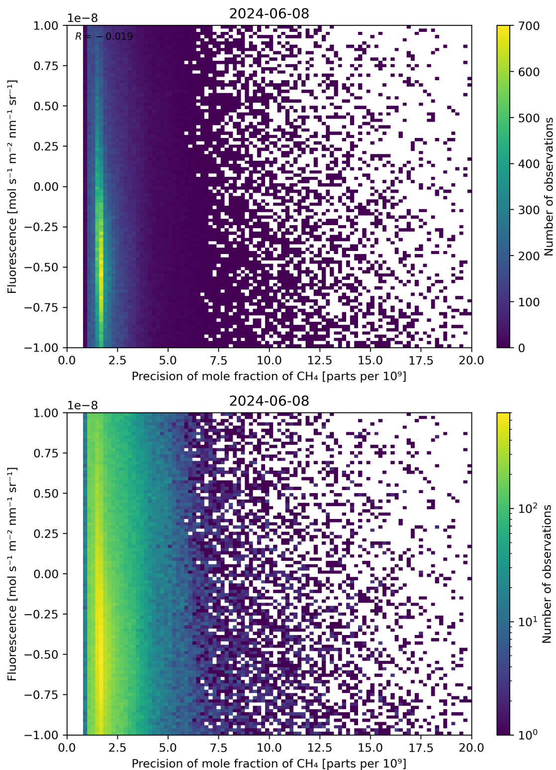
Figure 81: Scatter density plot of “Precision of mole fraction of CH 4 ” against “Fluorescence” for 2024-06-08 to 2024-06-09.
