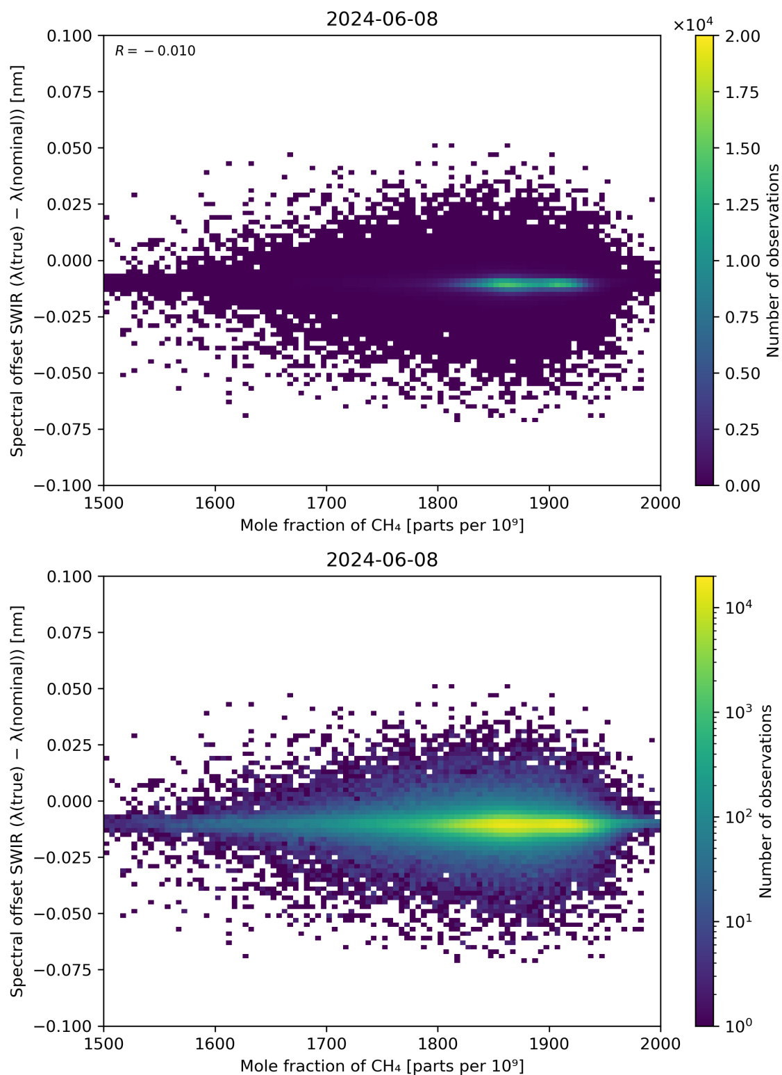
Figure 86: Scatter density plot of “Mole fraction of CH 4 ” against “Spectral offset SWIR ( \lambda(\text{true}) - \lambda(\text{nominal}) )” for 2024-06-08 to 2024-06-09.
