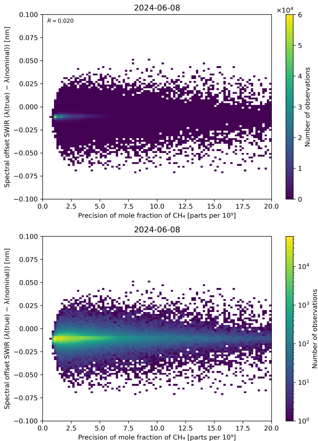
Figure 85: Scatter density plot of “Precision of mole fraction of CH 4 ” against “Spectral offset SWIR ( \lambda(\text{true}) - \lambda(\text{nominal}) )” for 2024-06-08 to 2024-06-09.
