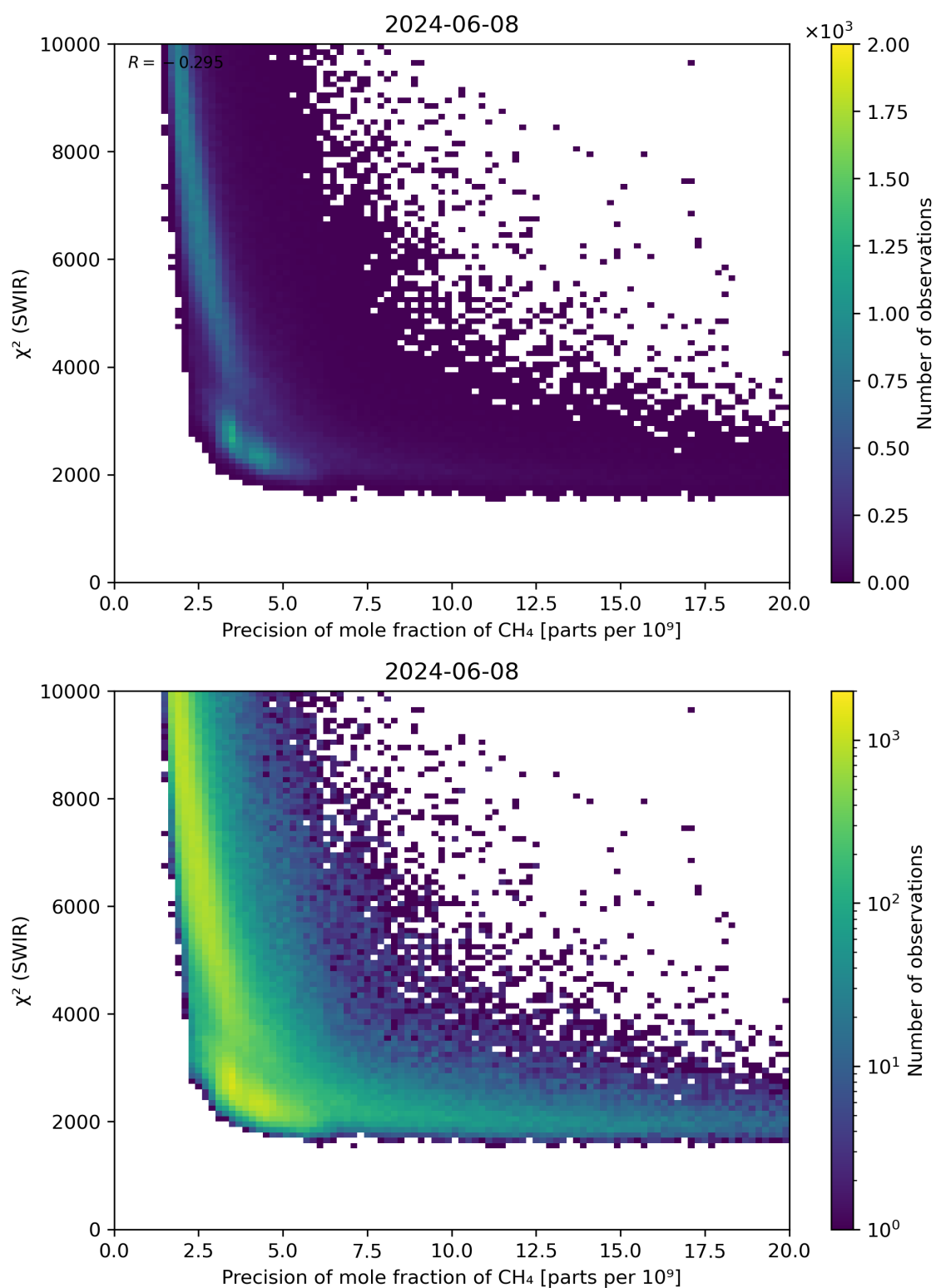
Figure 79: Scatter density plot of “Precision of mole fraction of CH 4 ” against “ \chi^2 (SWIR)” for 2024-06-08 to 2024-06-09.
