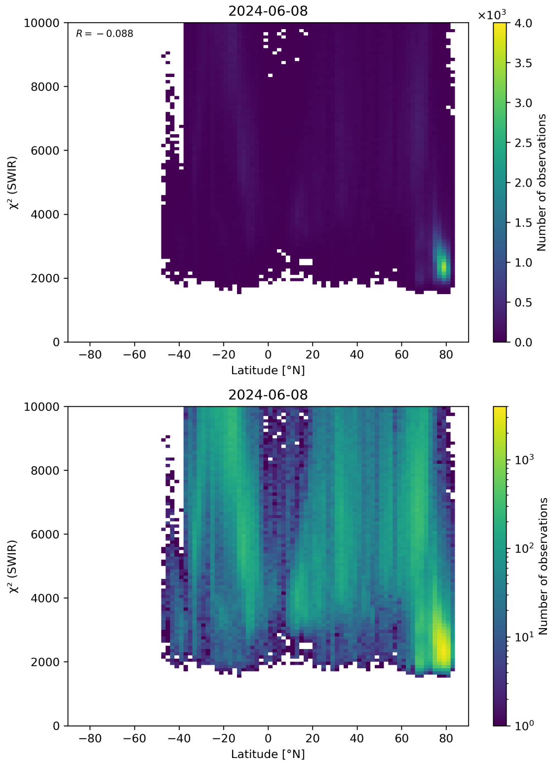
Figure 54: Scatter density plot of “Latitude” against “ \chi^2 (SWIR)” for 2024-06-08 to 2024-06-09.
