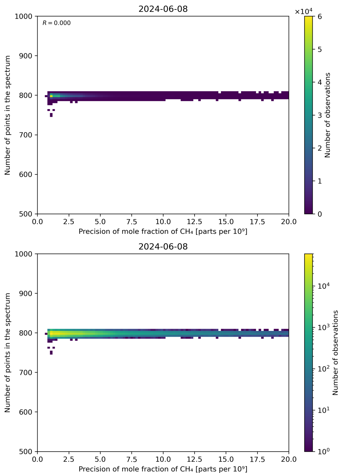
Figure 84: Scatter density plot of “Precision of mole fraction of CH 4 ” against “Number of points in the spectrum” for 2024-06-08 to 2024-06-09.
