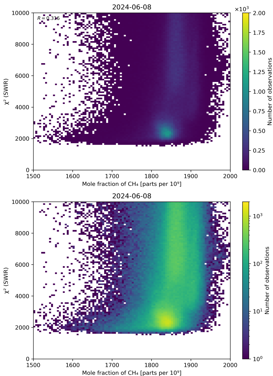
Figure 71: Scatter density plot of “Mole fraction of \text{CH}_4 ” against “ \chi^2 (SWIR)” for 2024-06-08 to 2024-06-09.
