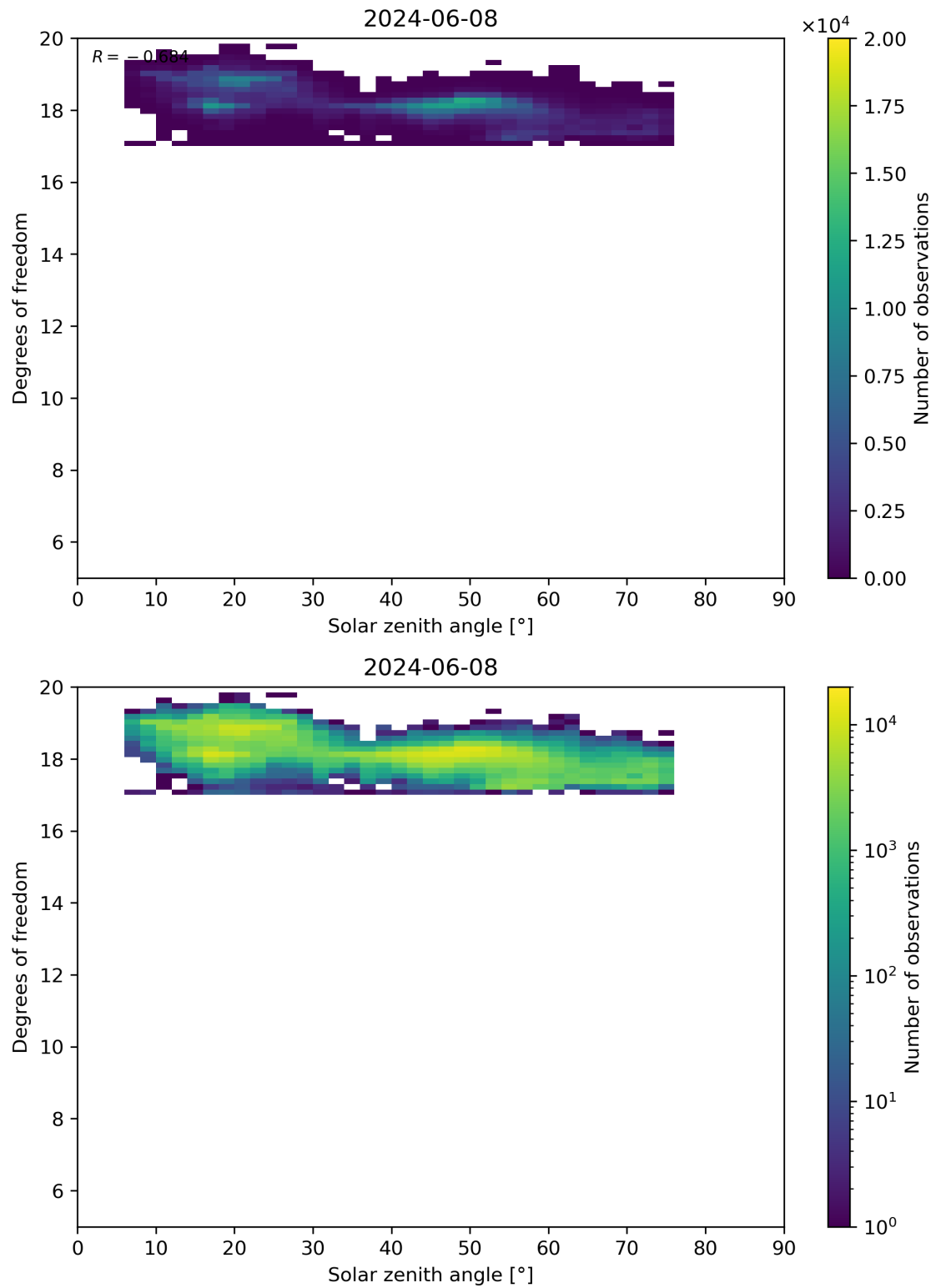
Figure 96: Scatter density plot of “Solar zenith angle” against “Degrees of freedom” for 2024-06-08 to 2024-06-09.
