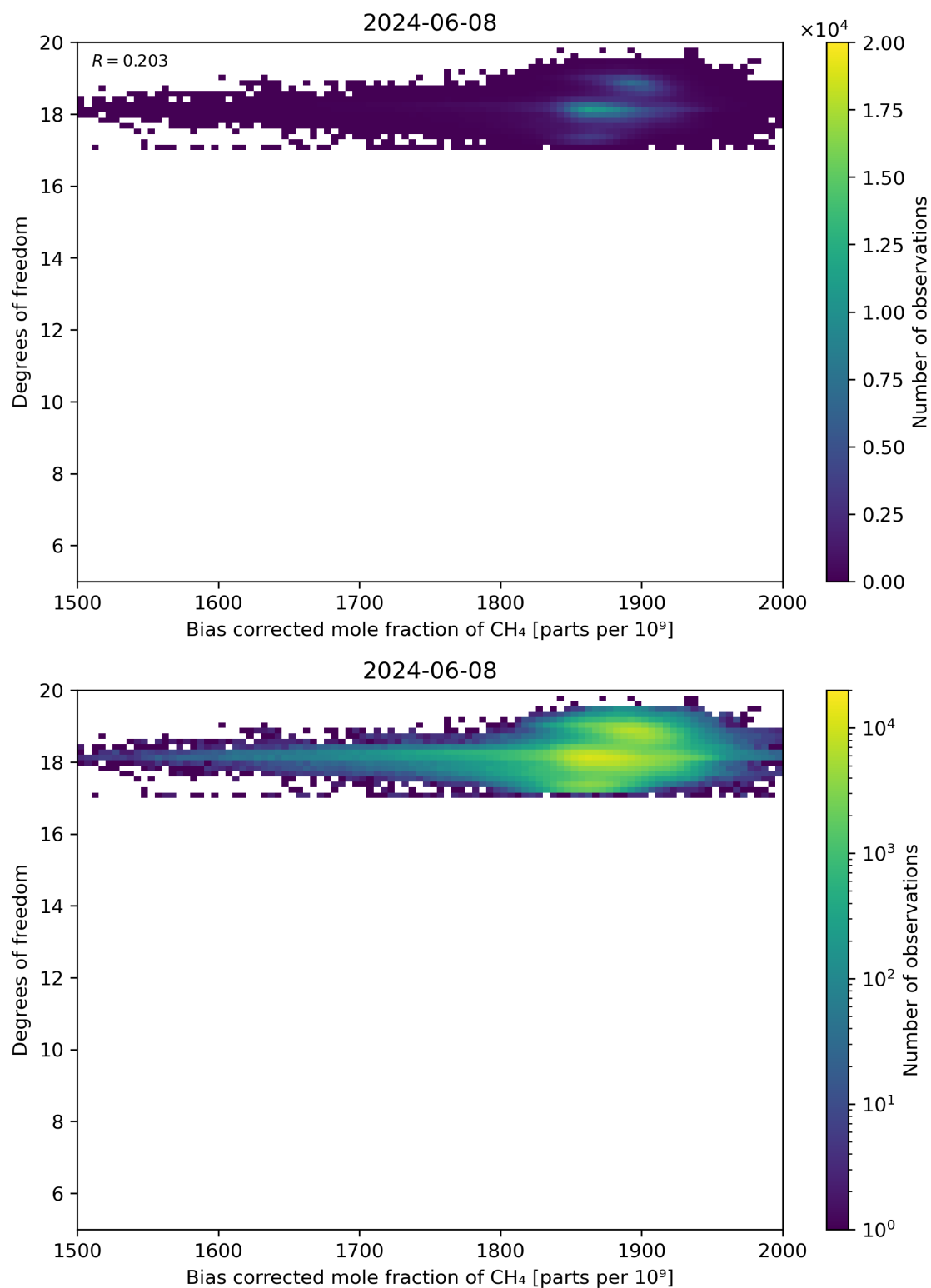
Figure 65: Scatter density plot of “Bias corrected mole fraction of CH 4 ” against “Degrees of freedom” for 2024-06-08 to 2024-06-09.
