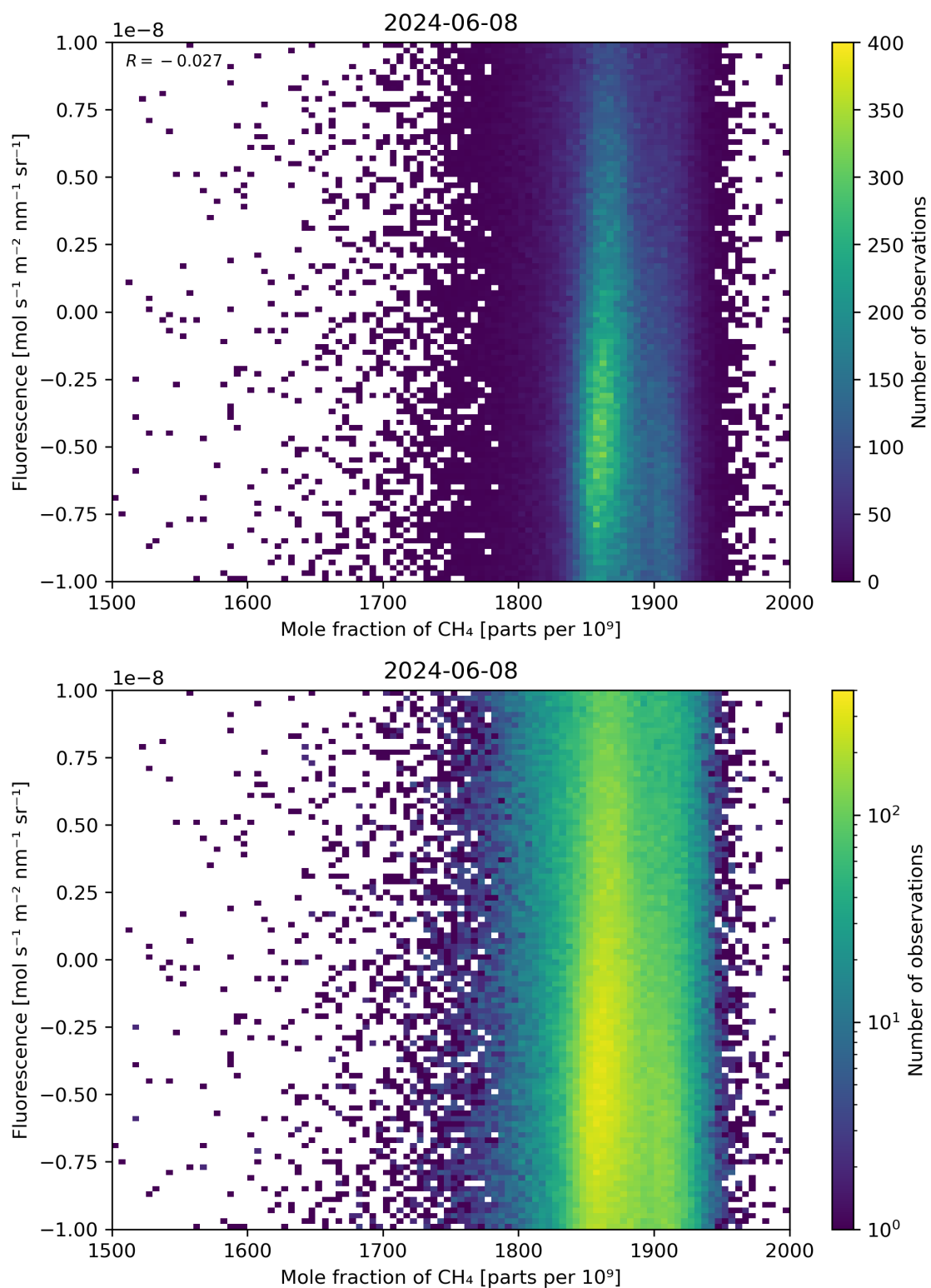
Figure 73: Scatter density plot of “Mole fraction of \text{CH}_4 ” against “Fluorescence” for 2024-06-08 to 2024-06-09.
