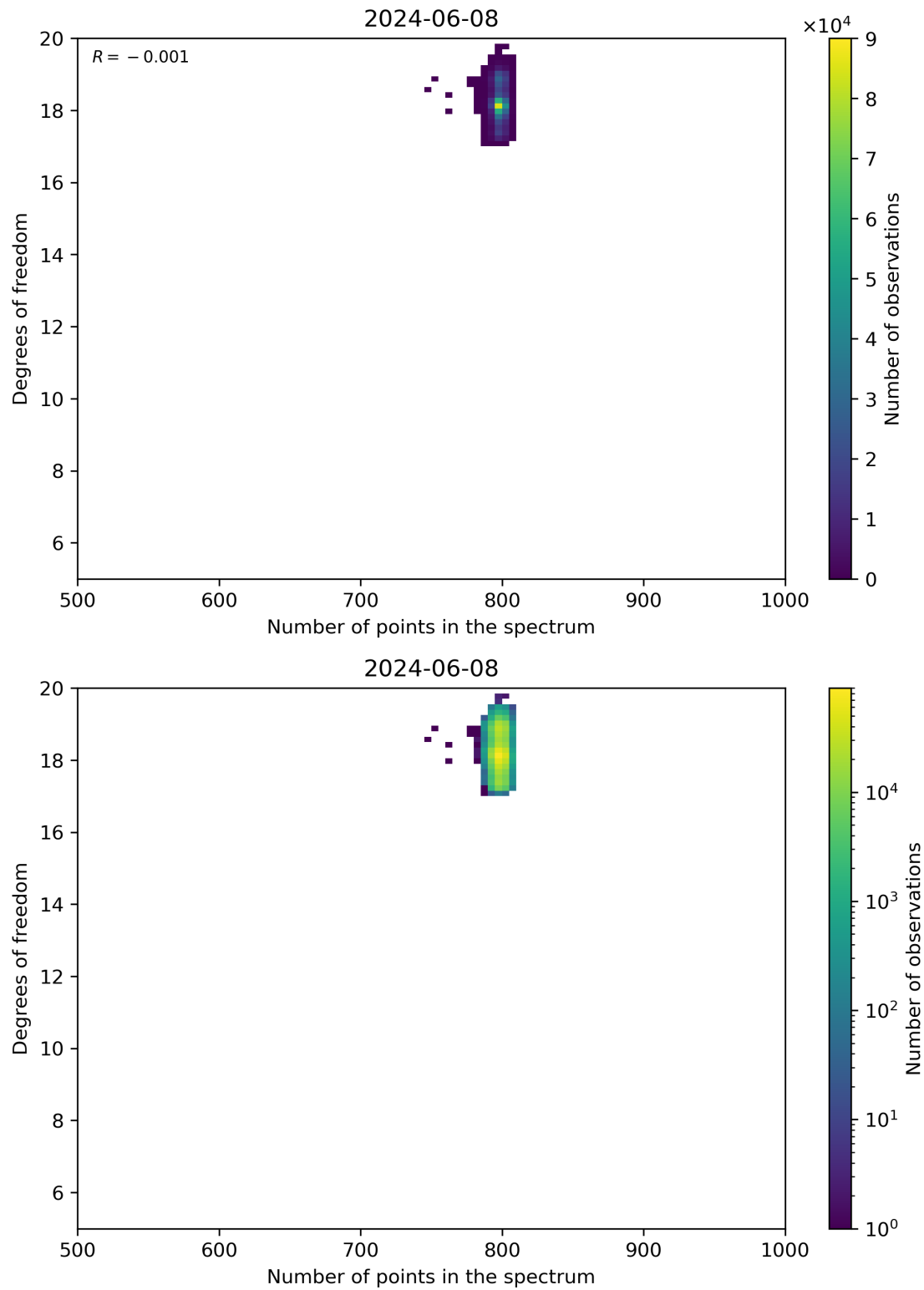
Figure 90: Scatter density plot of “Number of points in the spectrum” against “Degrees of freedom” for 2024-06-08 to 2024-06-09.
