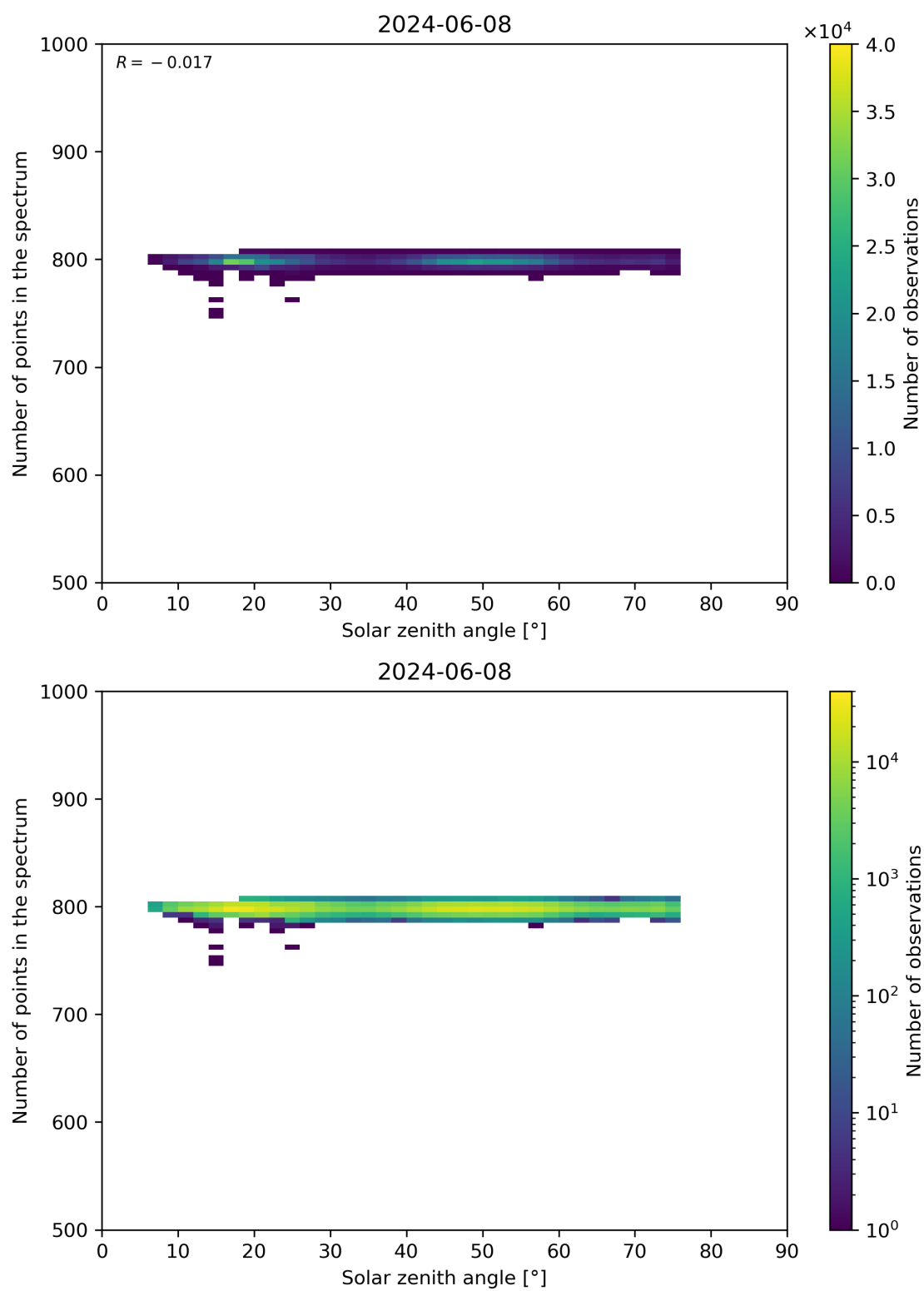
Figure 103: Scatter density plot of “Solar zenith angle” against “Number of points in the spectrum” for 2024-06-08 to 2024-06-09.
