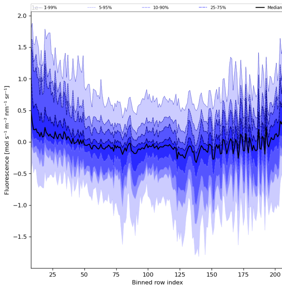
Figure 43: Along track statistics of “Fluorescence” for 2024-06-08 to 2024-06-09
