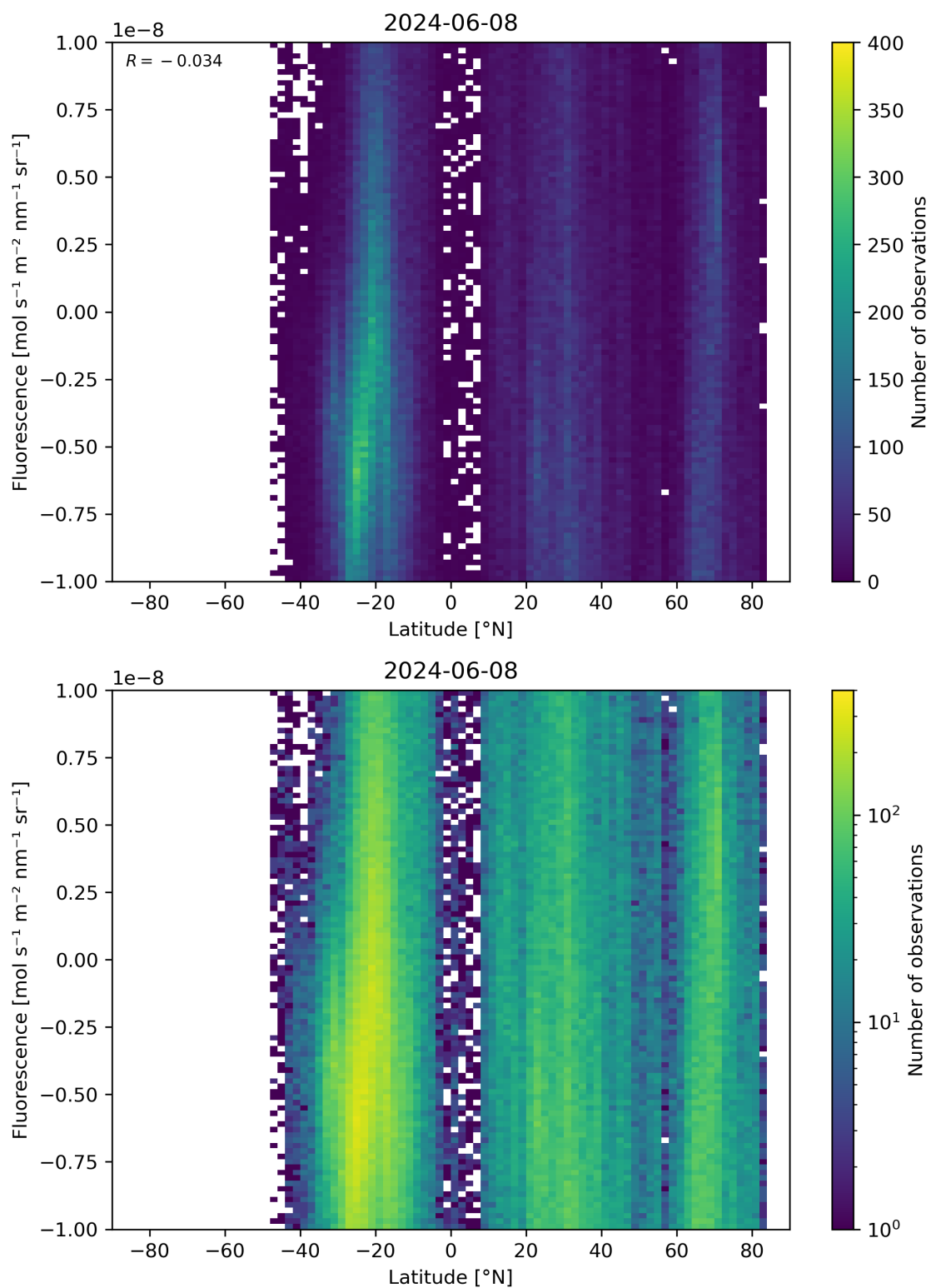
Figure 56: Scatter density plot of “Latitude” against “Fluorescence” for 2024-06-08 to 2024-06-09.
