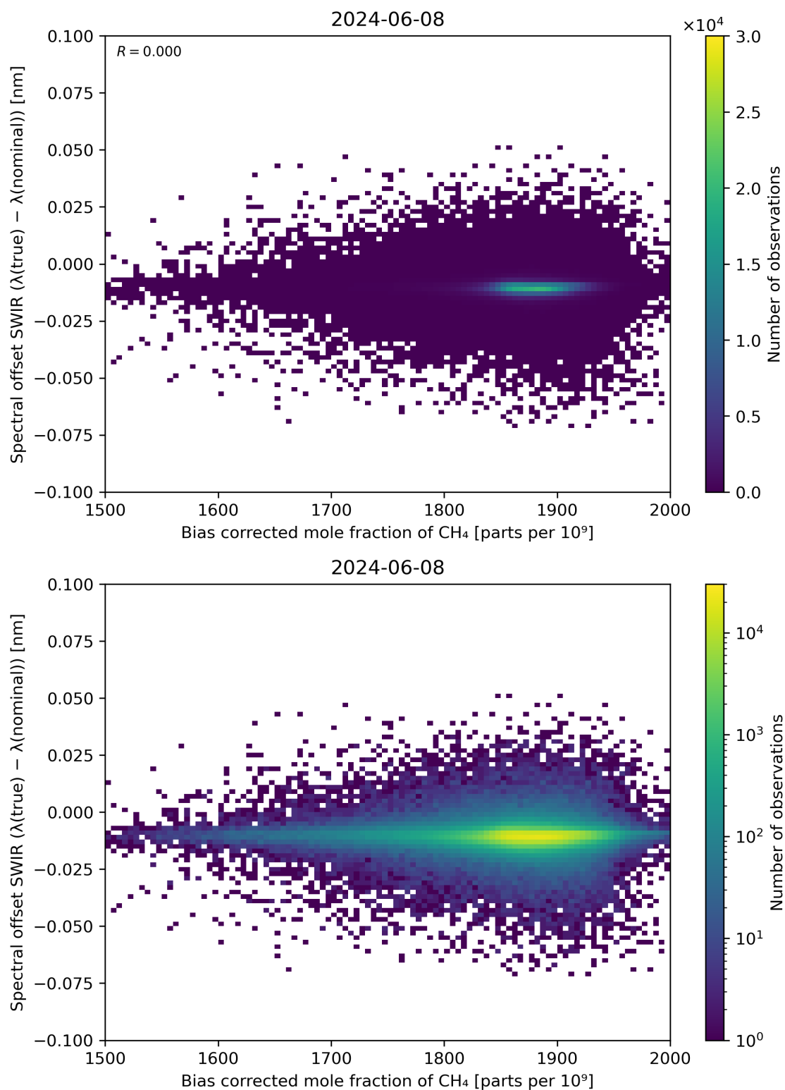
Figure 69: Scatter density plot of “Bias corrected mole fraction of \text{CH}_4 ” against “Spectral offset SWIR ( \lambda(\text{true}) - \lambda(\text{nominal}) )” for 2024-06-08 to 2024-06-09.
