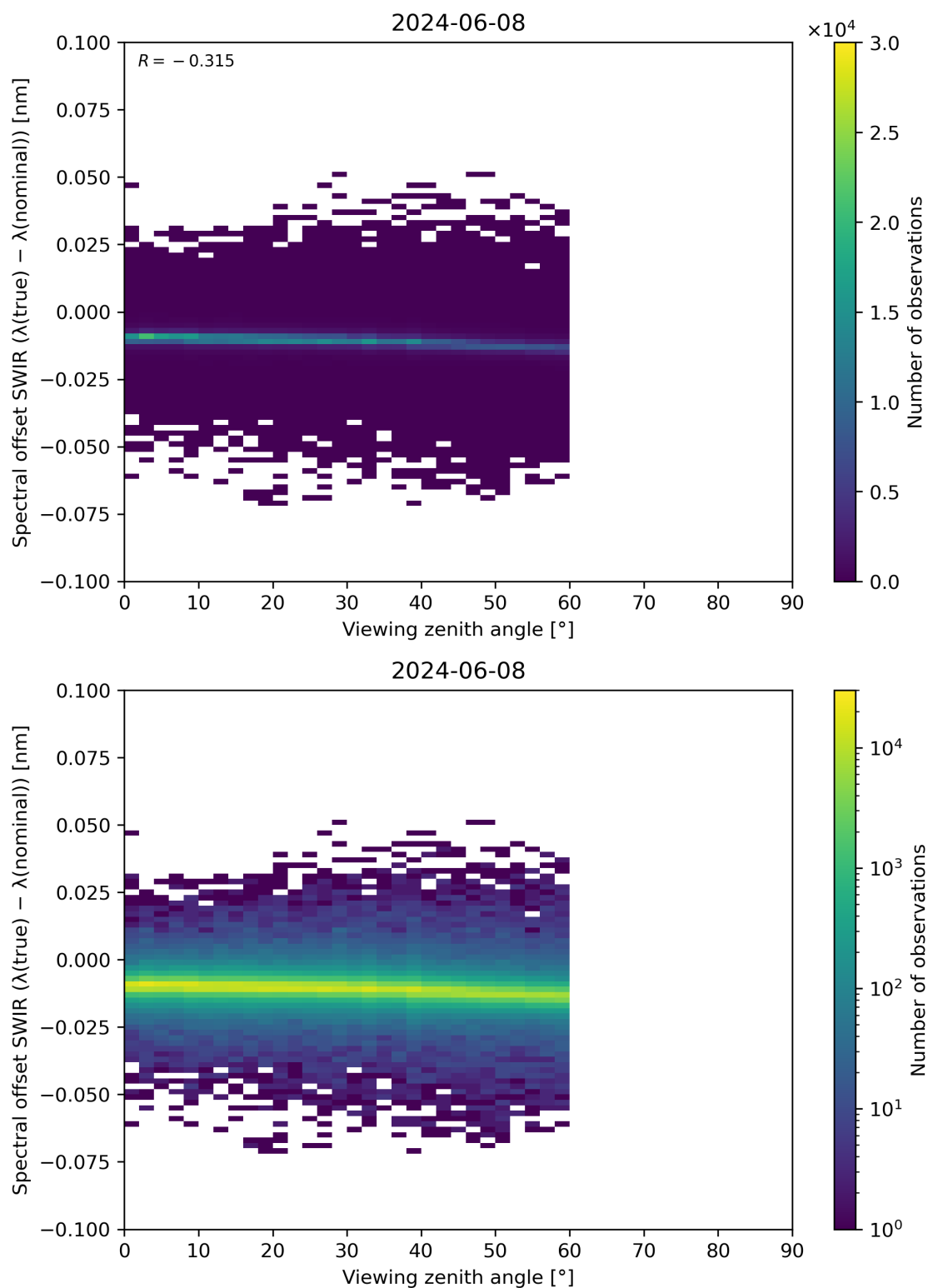
Figure 116: Scatter density plot of “Viewing zenith angle” against “Spectral offset SWIR ( \lambda(\text{true}) - \lambda(\text{nominal}) )” for 2024-06-08 to 2024-06-09.
