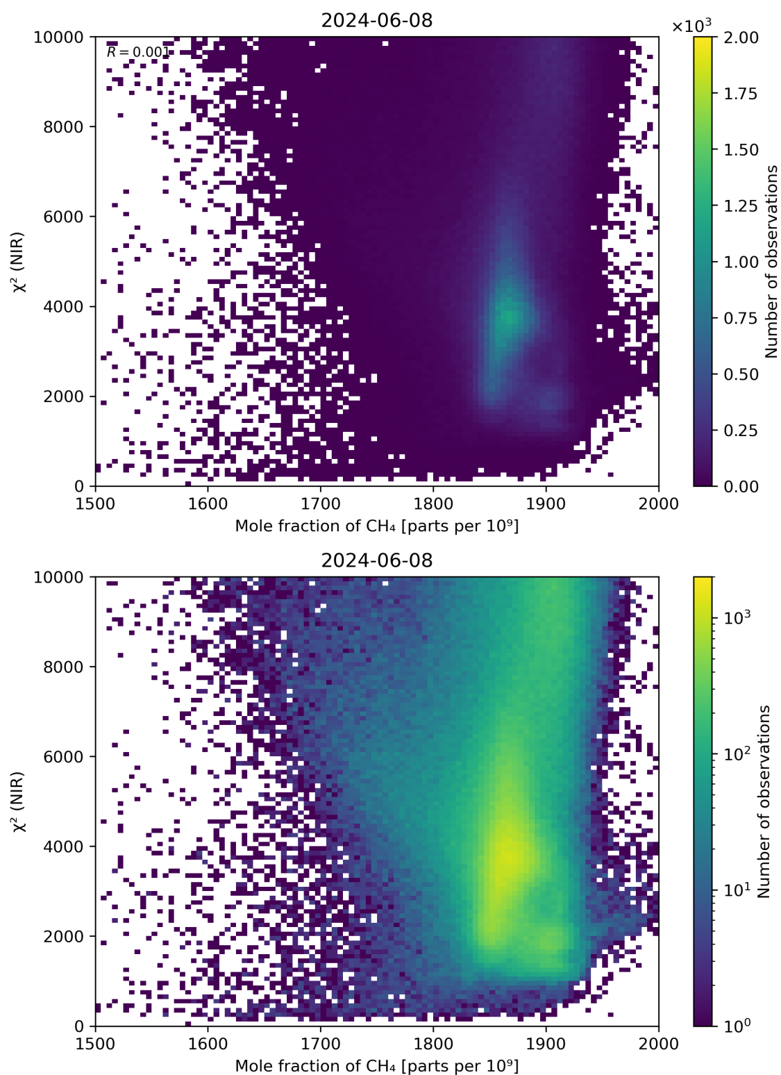
Figure 70: Scatter density plot of “Mole fraction of \text{CH}_4 ” against “ \chi^2 (NIR)” for 2024-06-08 to 2024-06-09.
