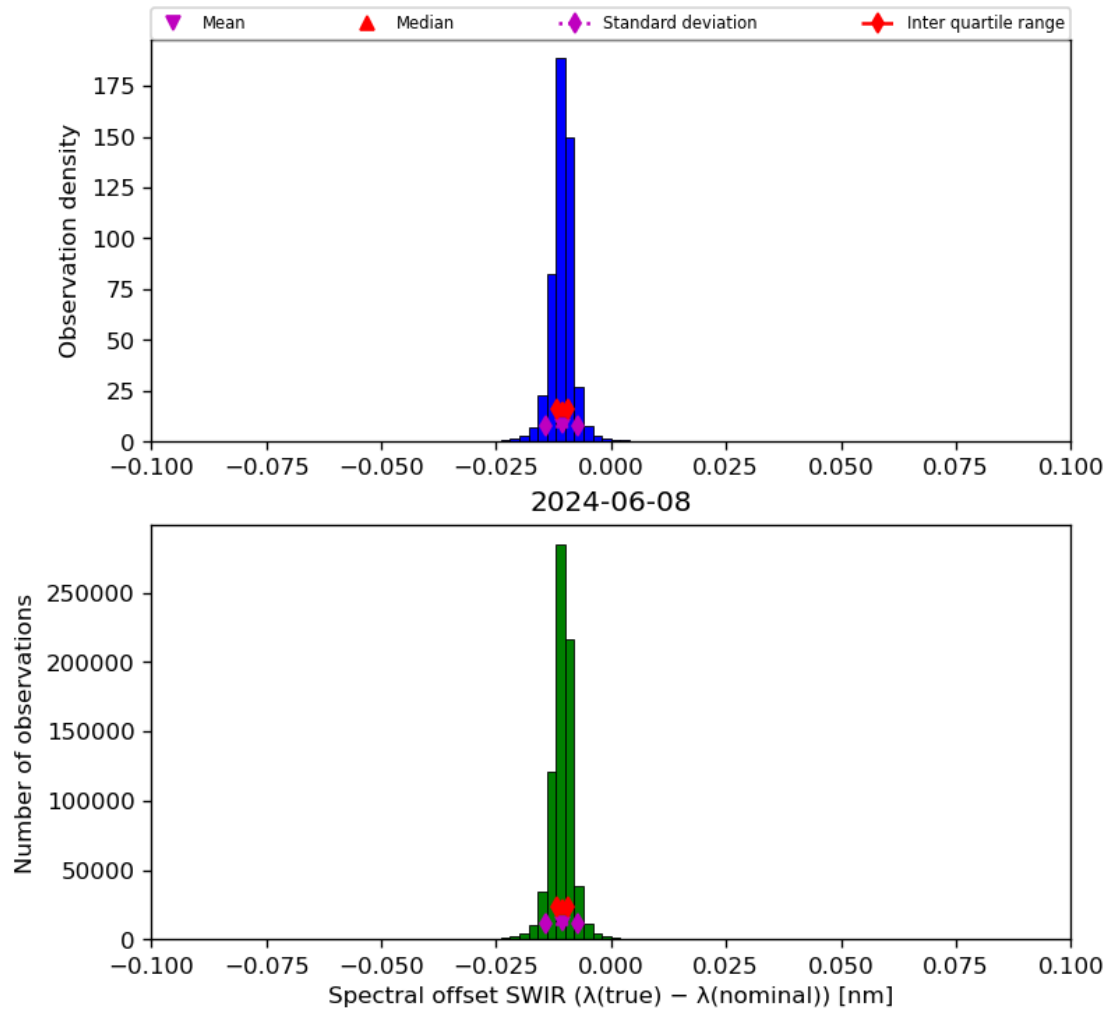
Figure 27: Histogram of “Spectral offset SWIR ( \lambda(\text{true}) - \lambda(\text{nominal}) )” for 2024-06-08 to 2024-06-09
