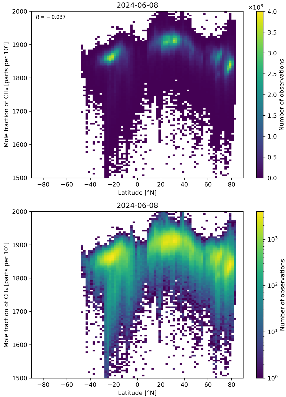
Figure 57: Scatter density plot of “Latitude” against “Mole fraction of CH 4 ” for 2024-06-08 to 2024-06-09.
