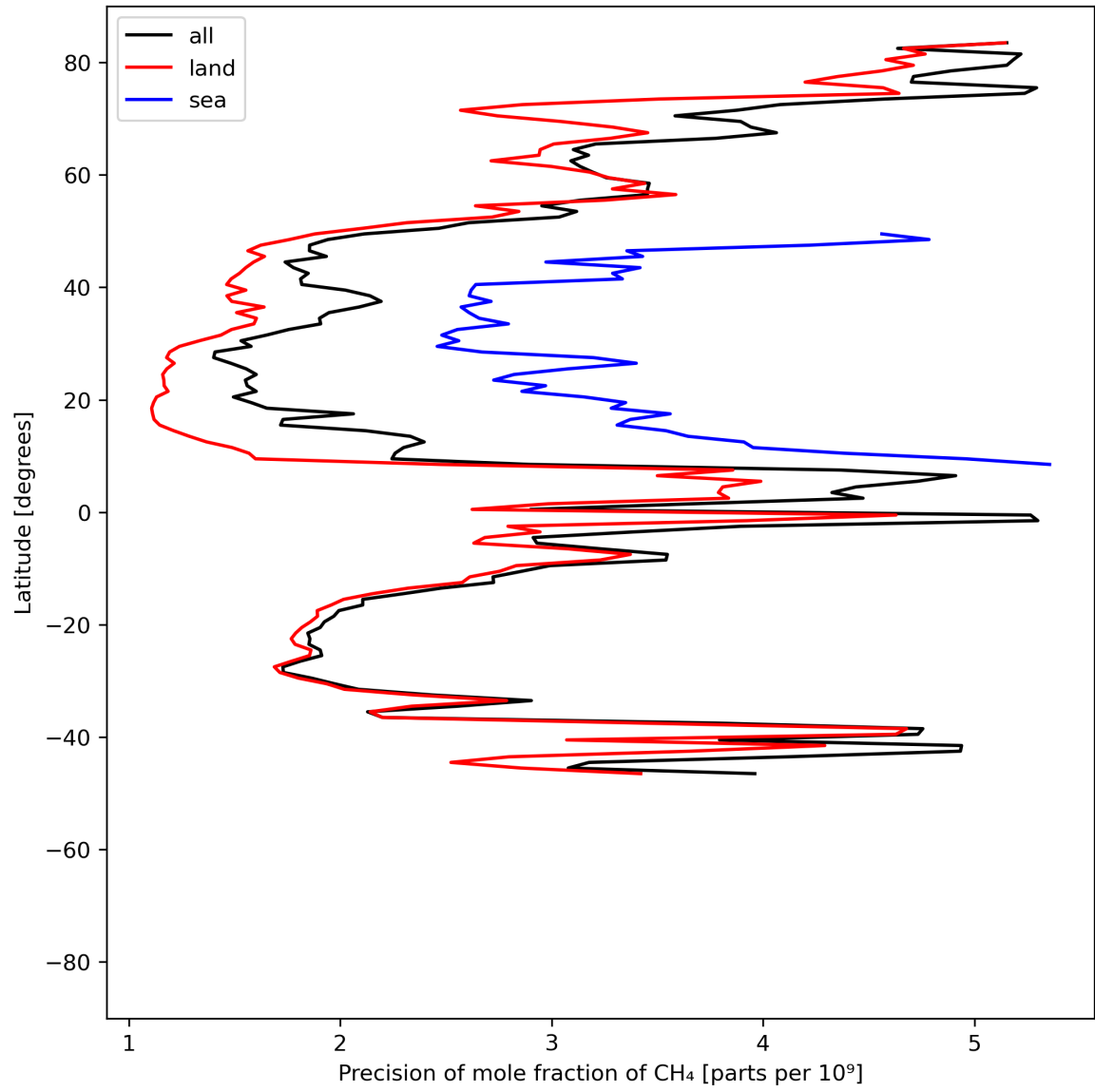
Figure 13: Zonal average of “Precision of mole fraction of CH 4 ” for 2024-06-08 to 2024-06-09.
