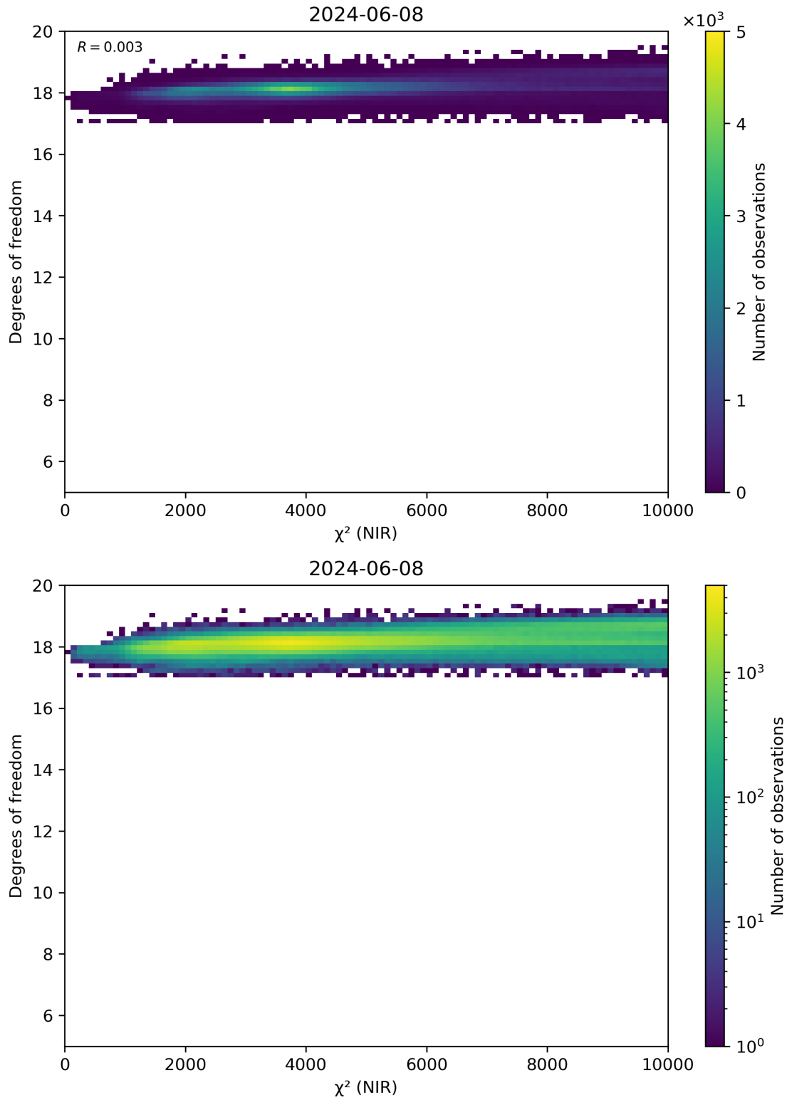
Figure 44: Scatter density plot of “ \chi^2 (NIR)” against “Degrees of freedom” for 2024-06-08 to 2024-06-09.
