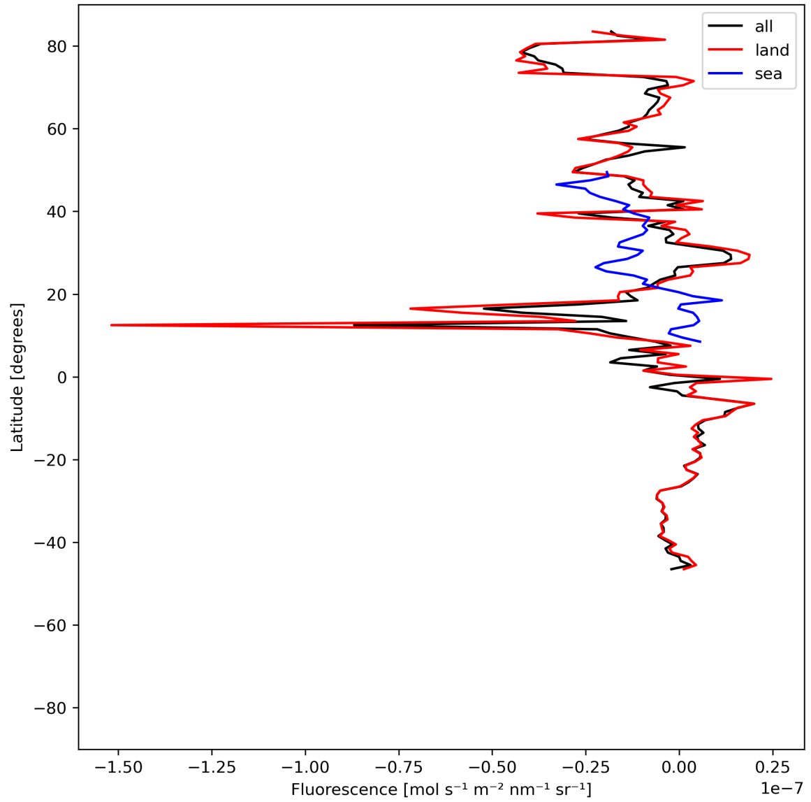
Figure 21: Zonal average of “Fluorescence” for 2024-06-08 to 2024-06-09.
