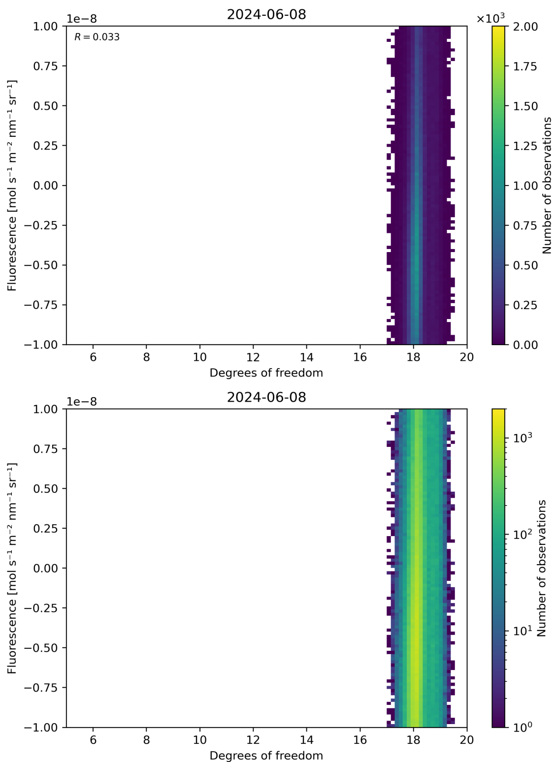
Figure 51: Scatter density plot of “Degrees of freedom” against “Fluorescence” for 2024-06-08 to 2024-06-09.
