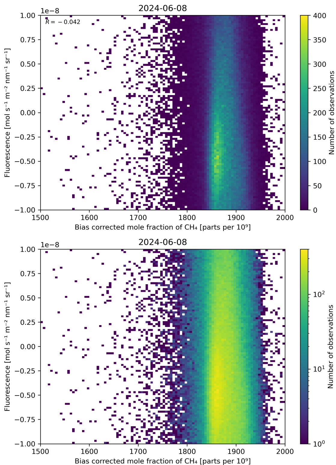
Figure 66: Scatter density plot of “Bias corrected mole fraction of \text{CH}_4 ” against “Fluorescence” for 2024-06-08 to 2024-06-09.
