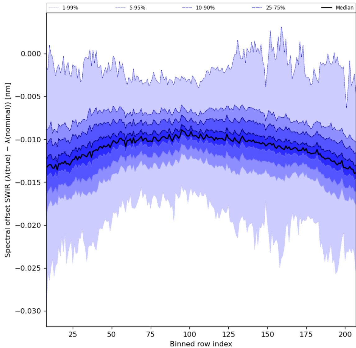
Figure 38: Along track statistics of “Spectral offset SWIR ( \lambda(\text{true}) - \lambda(\text{nominal}) )” for 2024-06-08 to 2024-06-09
