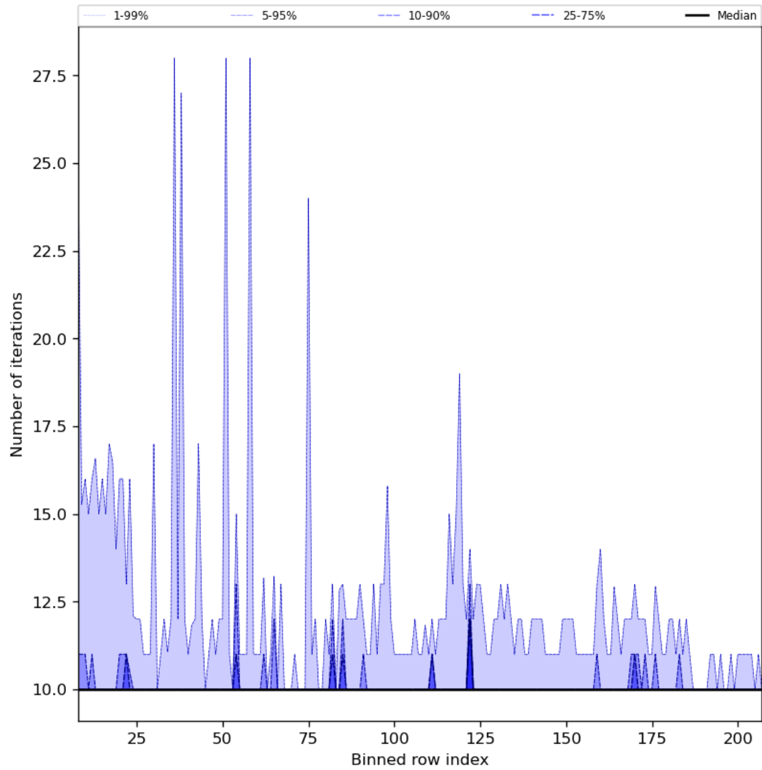
Figure 42: Along track statistics of “Number of iterations” for 2024-06-08 to 2024-06-09
