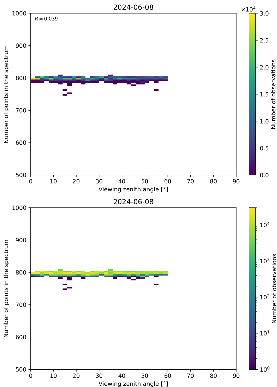
Figure 114: Scatter density plot of “Viewing zenith angle” against “Number of points in the spectrum” for 2024-06-08 to 2024-06-09.
