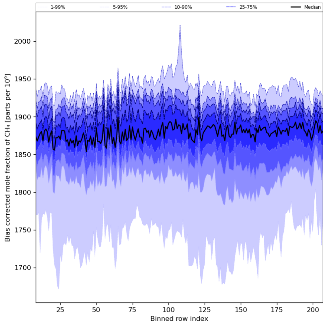
Figure 36: Along track statistics of “Bias corrected mole fraction of CH 4 ” for 2024-06-08 to 2024-06-09
