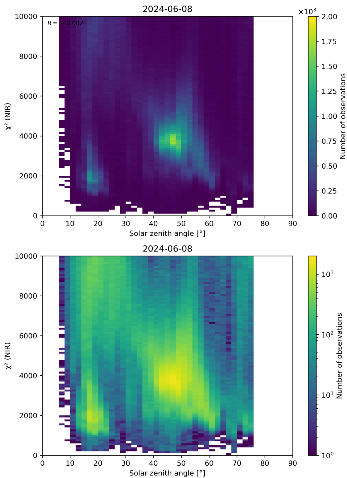
Figure 94: Scatter density plot of “Solar zenith angle” against “ \chi^2 (NIR)” for 2024-06-08 to 2024-06-09.
