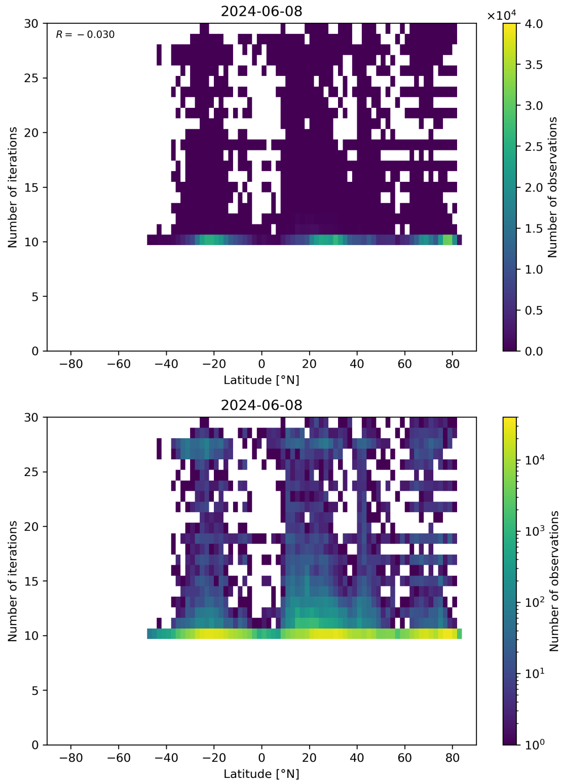
Figure 60: Scatter density plot of “Latitude” against “Number of iterations” for 2024-06-08 to 2024-06-09.
