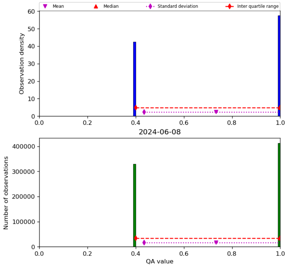
Figure 22: Histogram of “QA value” for 2024-06-08 to 2024-06-09
