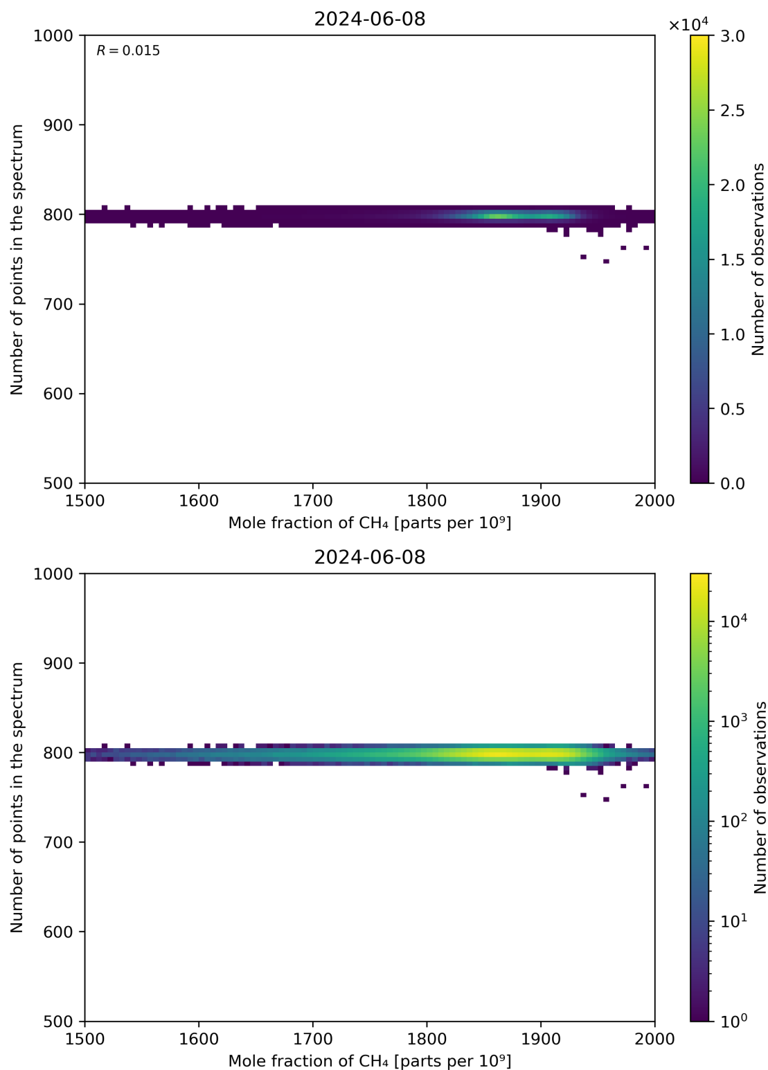
Figure 77: Scatter density plot of “Mole fraction of CH 4 ” against “Number of points in the spectrum” for 2024-06-08 to 2024-06-09.
