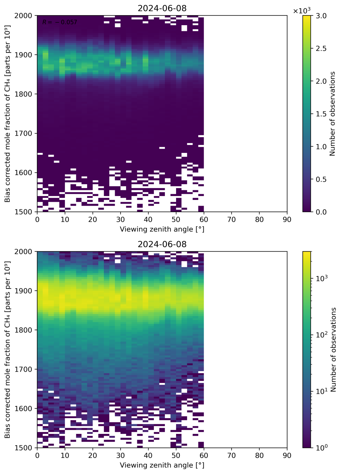
Figure 111: Scatter density plot of “Viewing zenith angle” against “Bias corrected mole fraction of CH 4 ” for 2024-06-08 to 2024-06-09.
