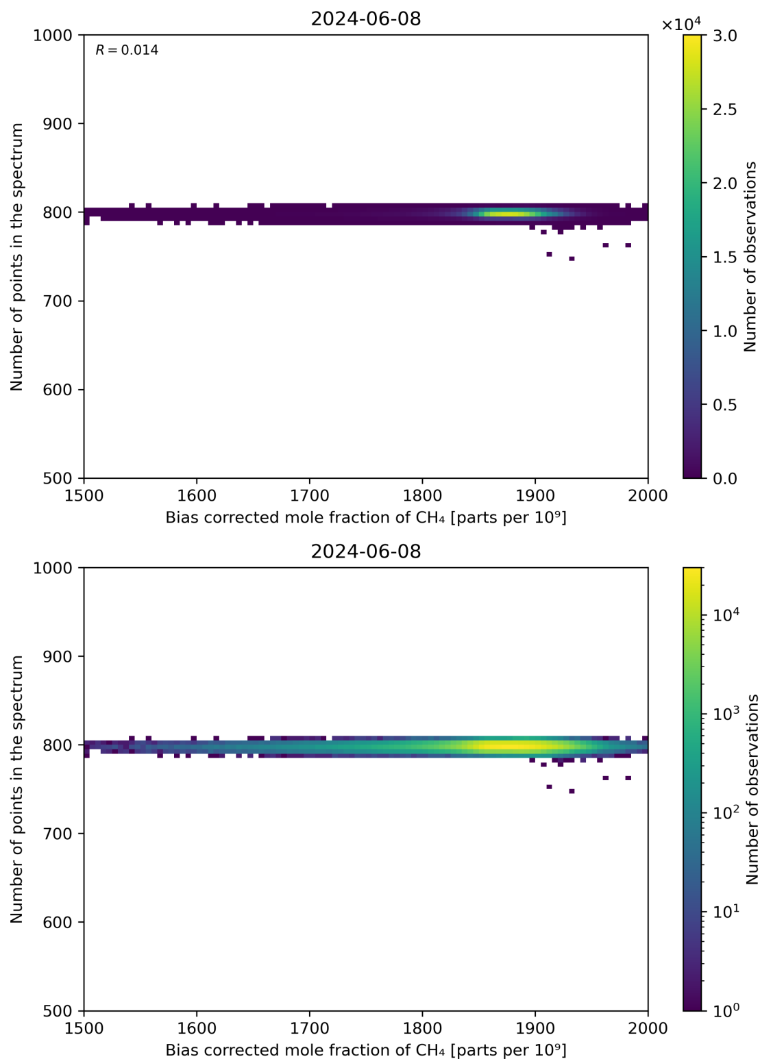
Figure 68: Scatter density plot of “Bias corrected mole fraction of CH 4 ” against “Number of points in the spectrum” for 2024-06-08 to 2024-06-09.
