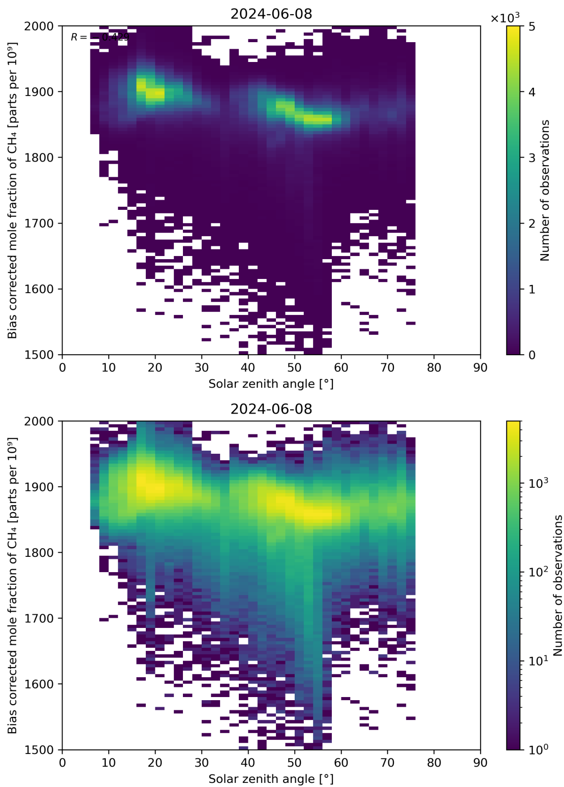
Figure 100: Scatter density plot of “Solar zenith angle” against “Bias corrected mole fraction of CH 4 ” for 2024-06-08 to 2024-06-09.
