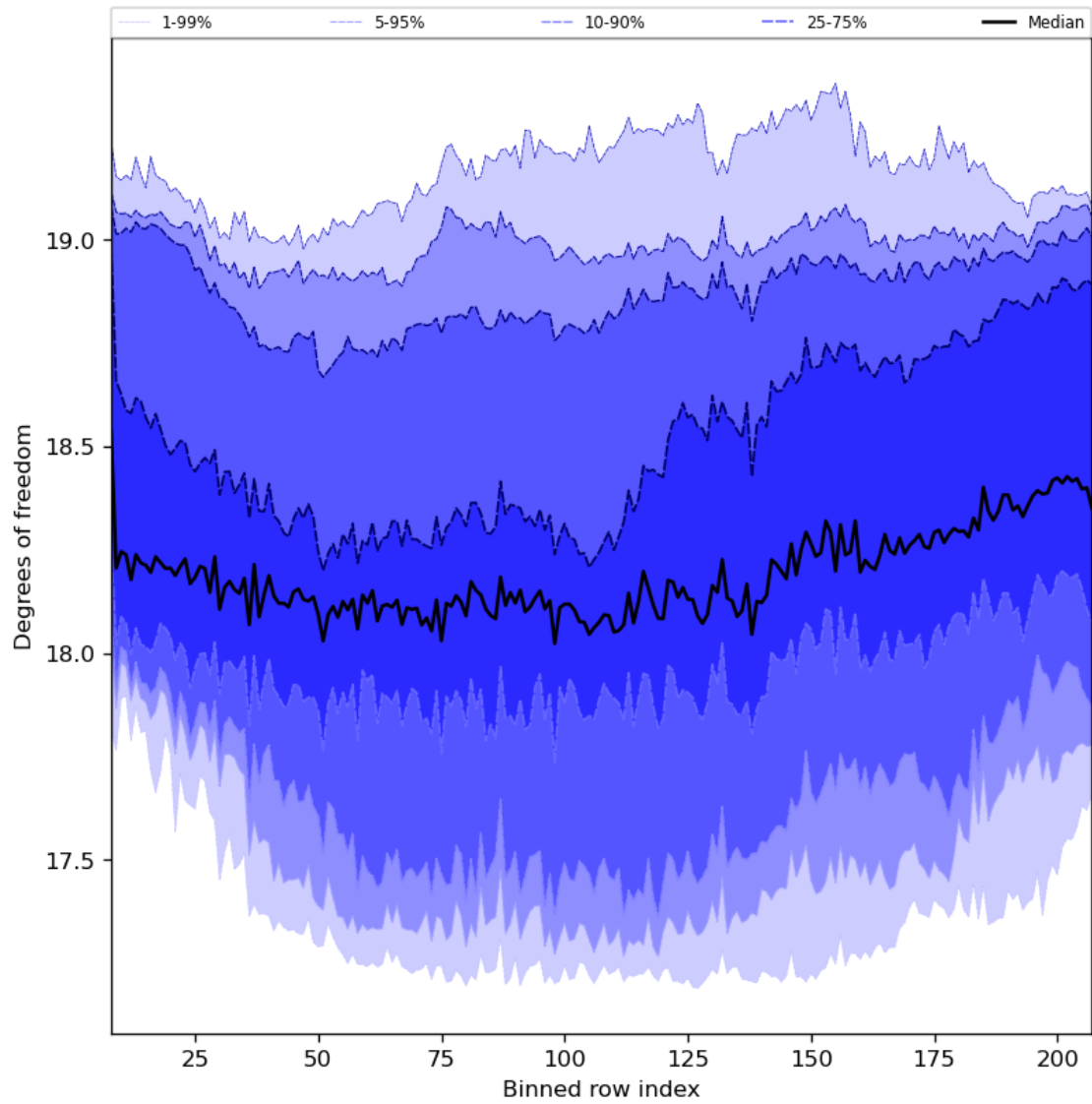
Figure 41: Along track statistics of “Degrees of freedom” for 2024-06-08 to 2024-06-09
