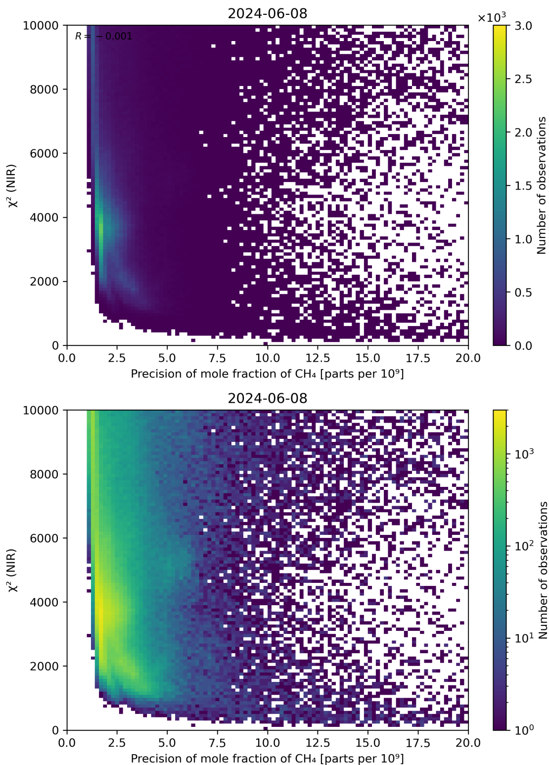
Figure 78: Scatter density plot of “Precision of mole fraction of CH 4 ” against “ \chi^2 (NIR)” for 2024-06-08 to 2024-06-09.
