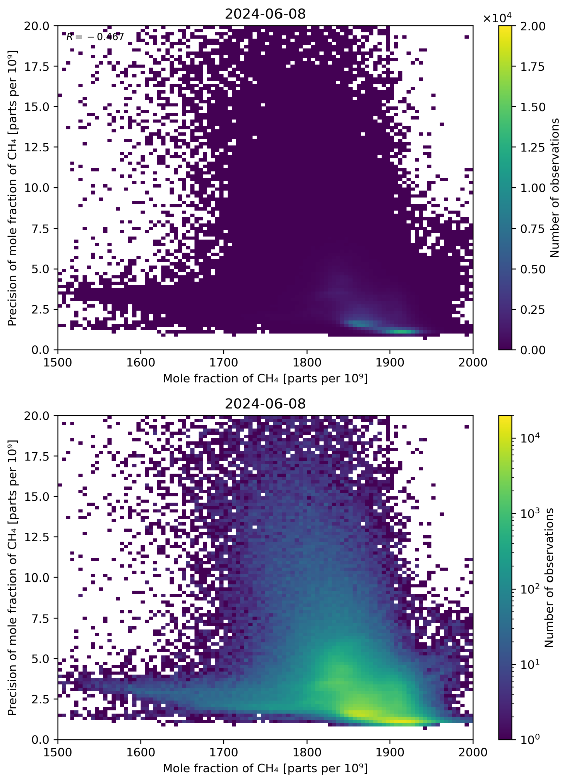
Figure 75: Scatter density plot of “Mole fraction of CH 4 ” against “Precision of mole fraction of CH 4 ” for 2024-06-08 to 2024-06-09.
