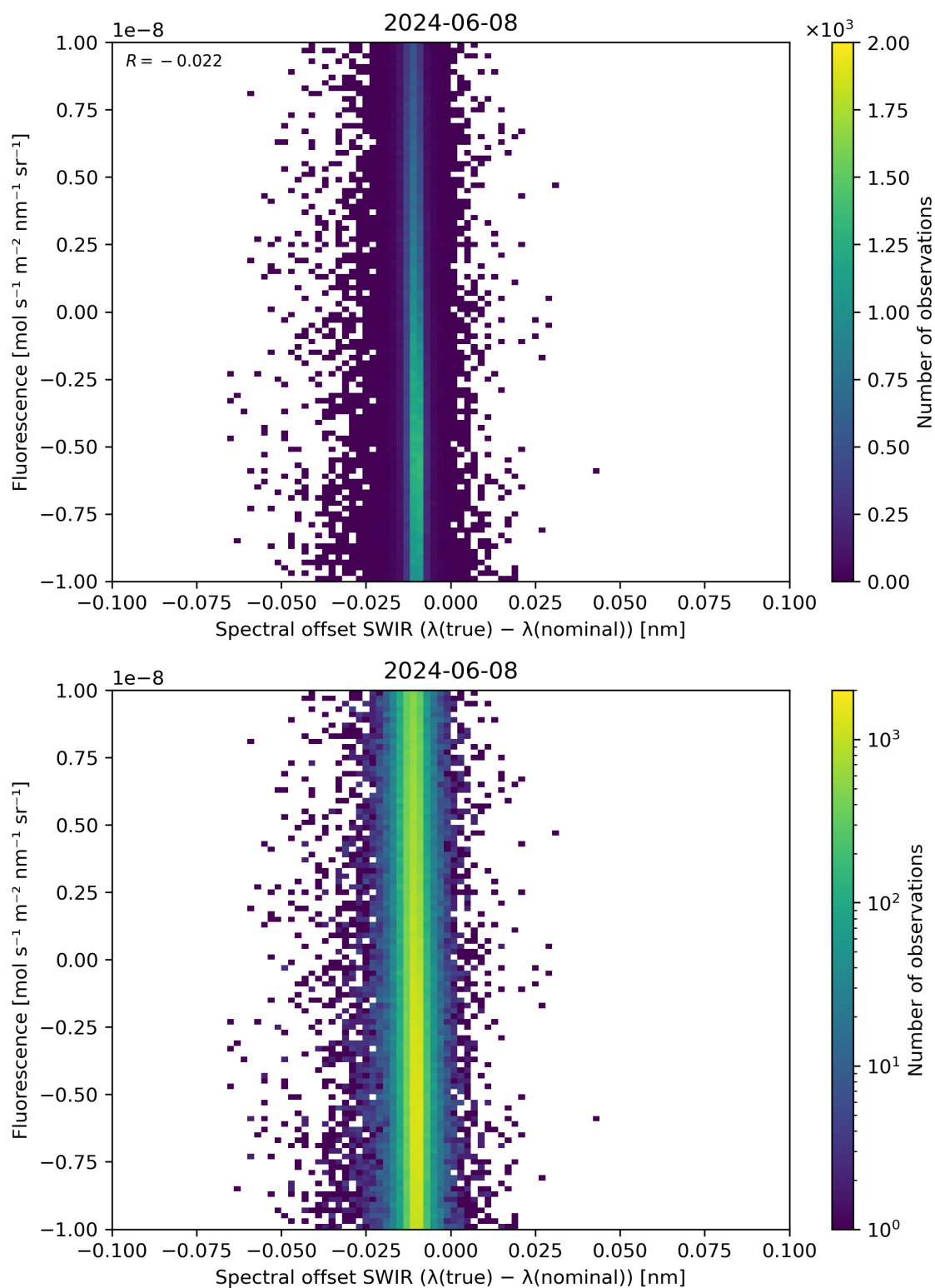
Figure 120: Scatter density plot of “Spectral offset SWIR ( \lambda(\text{true}) - \lambda(\text{nominal}) )” against “Fluorescence” for 2024-06-08 to 2024-06-09.
