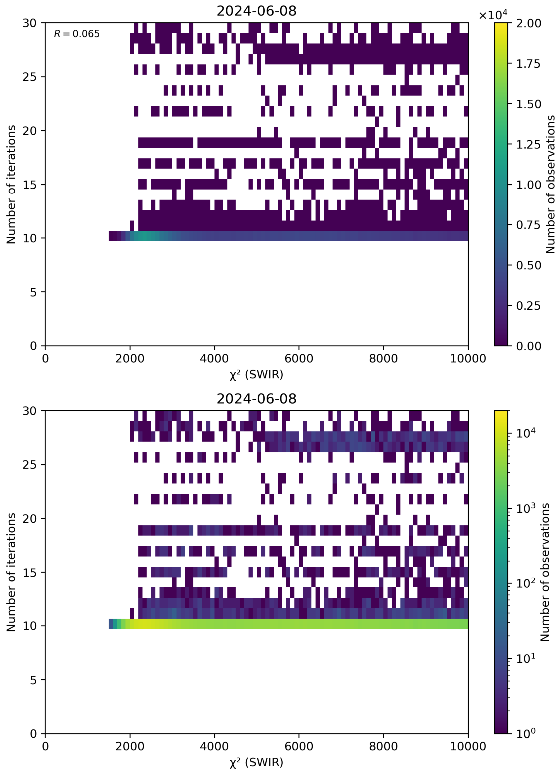
Figure 50: Scatter density plot of “ \chi^2 (SWIR)” against “Number of iterations” for 2024-06-08 to 2024-06-09.
