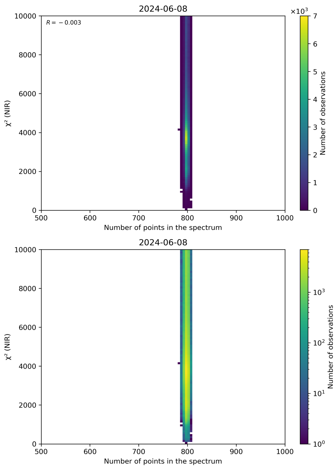
Figure 88: Scatter density plot of “Number of points in the spectrum” against “ \chi^2 (NIR)” for 2024-06-08 to 2024-06-09.
