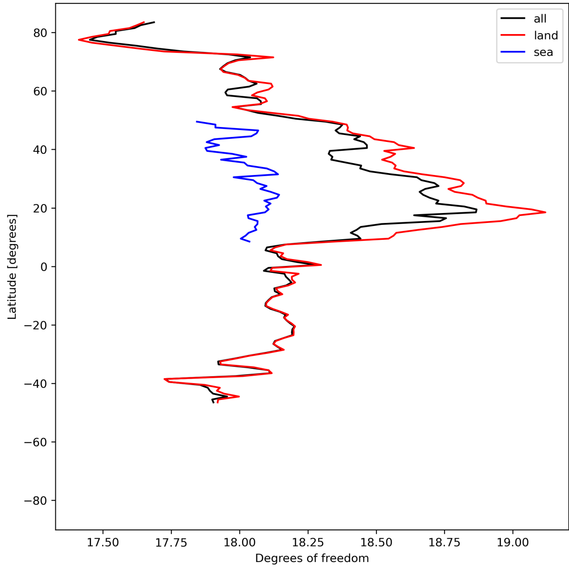
Figure 19: Zonal average of “Degrees of freedom” for 2024-06-08 to 2024-06-09.
