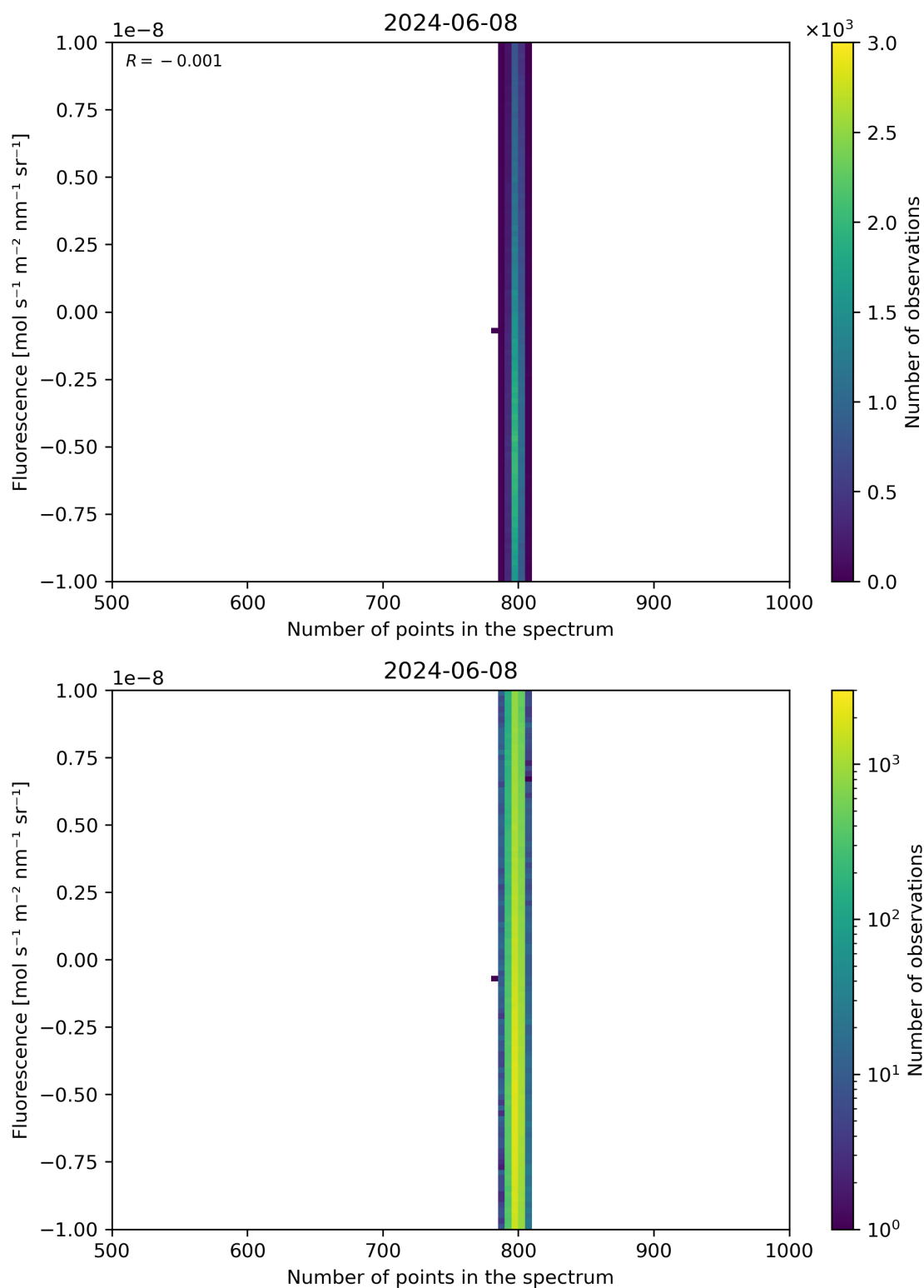
Figure 91: Scatter density plot of “Number of points in the spectrum” against “Fluorescence” for 2024-06-08 to 2024-06-09.
