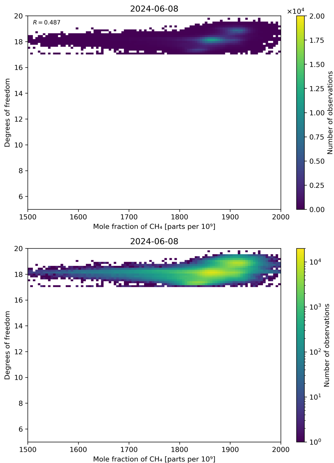
Figure 72: Scatter density plot of “Mole fraction of CH 4 ” against “Degrees of freedom” for 2024-06-08 to 2024-06-09.
