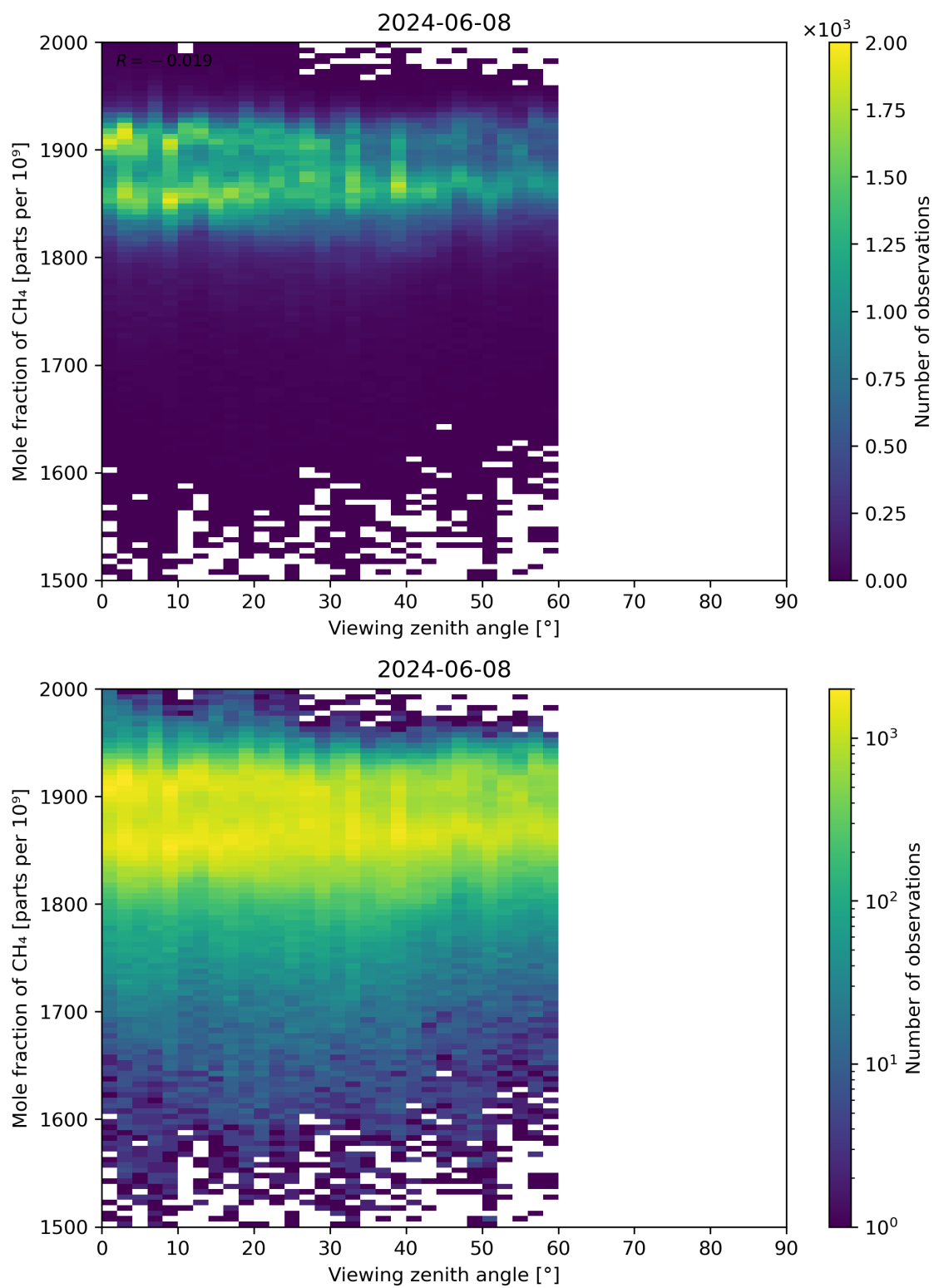
Figure 110: Scatter density plot of “Viewing zenith angle” against “Mole fraction of CH 4 ” for 2024-06-08 to 2024-06-09.
