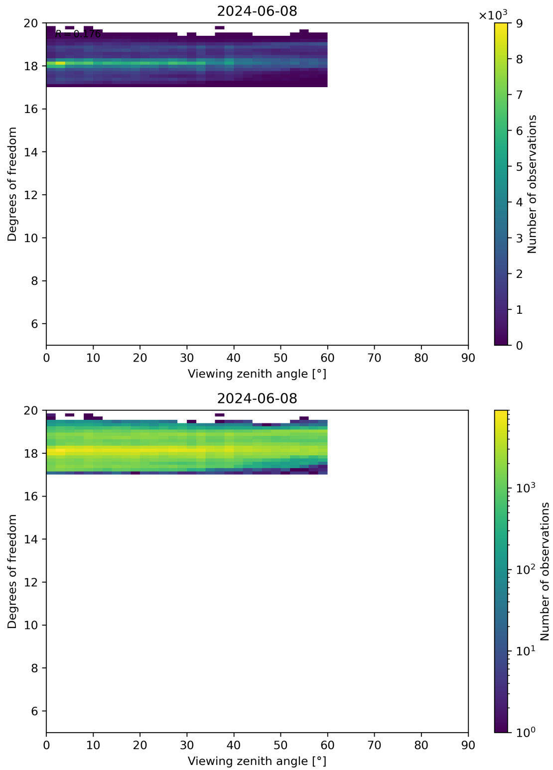
Figure 107: Scatter density plot of “Viewing zenith angle” against “Degrees of freedom” for 2024-06-08 to 2024-06-09.
