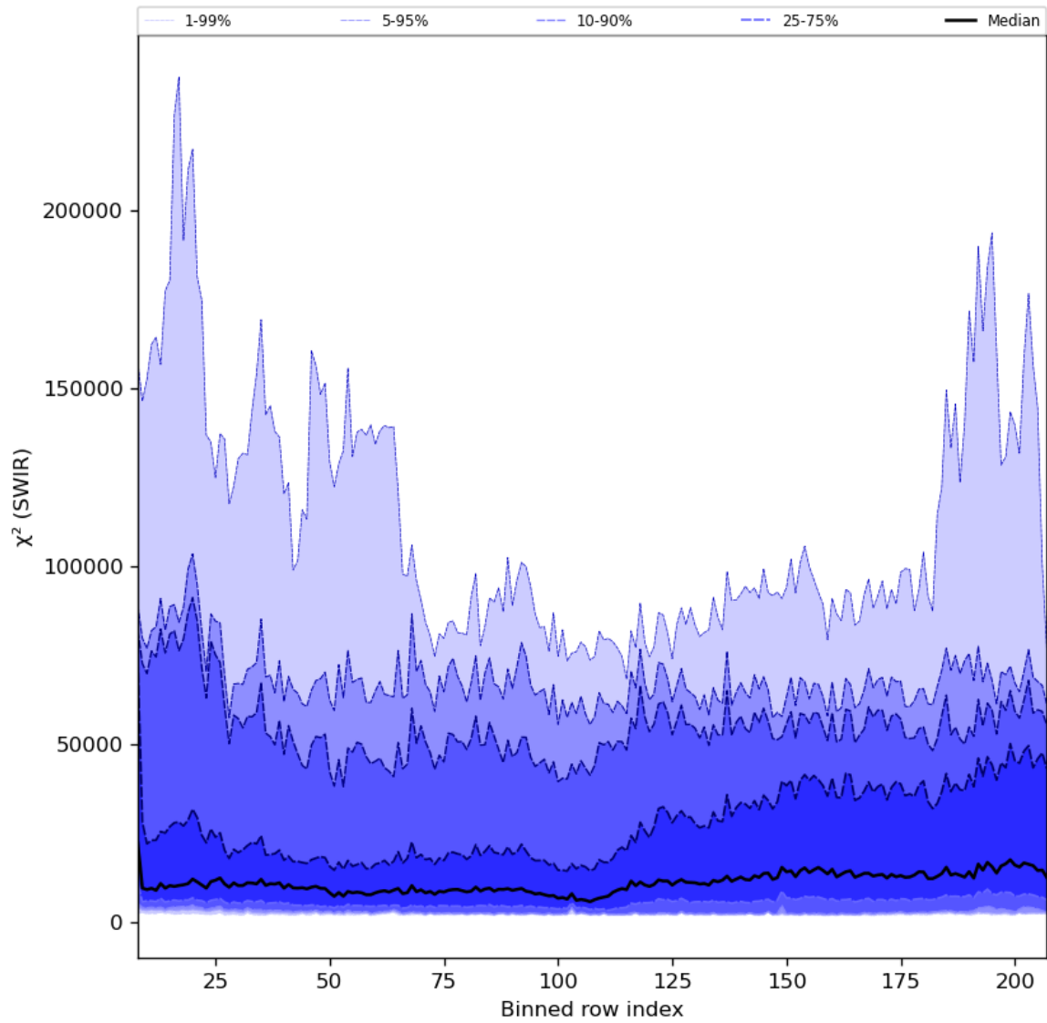
Figure 39: Along track statistics of " \chi^2 (SWIR)" for 2024-06-08 to 2024-06-09
