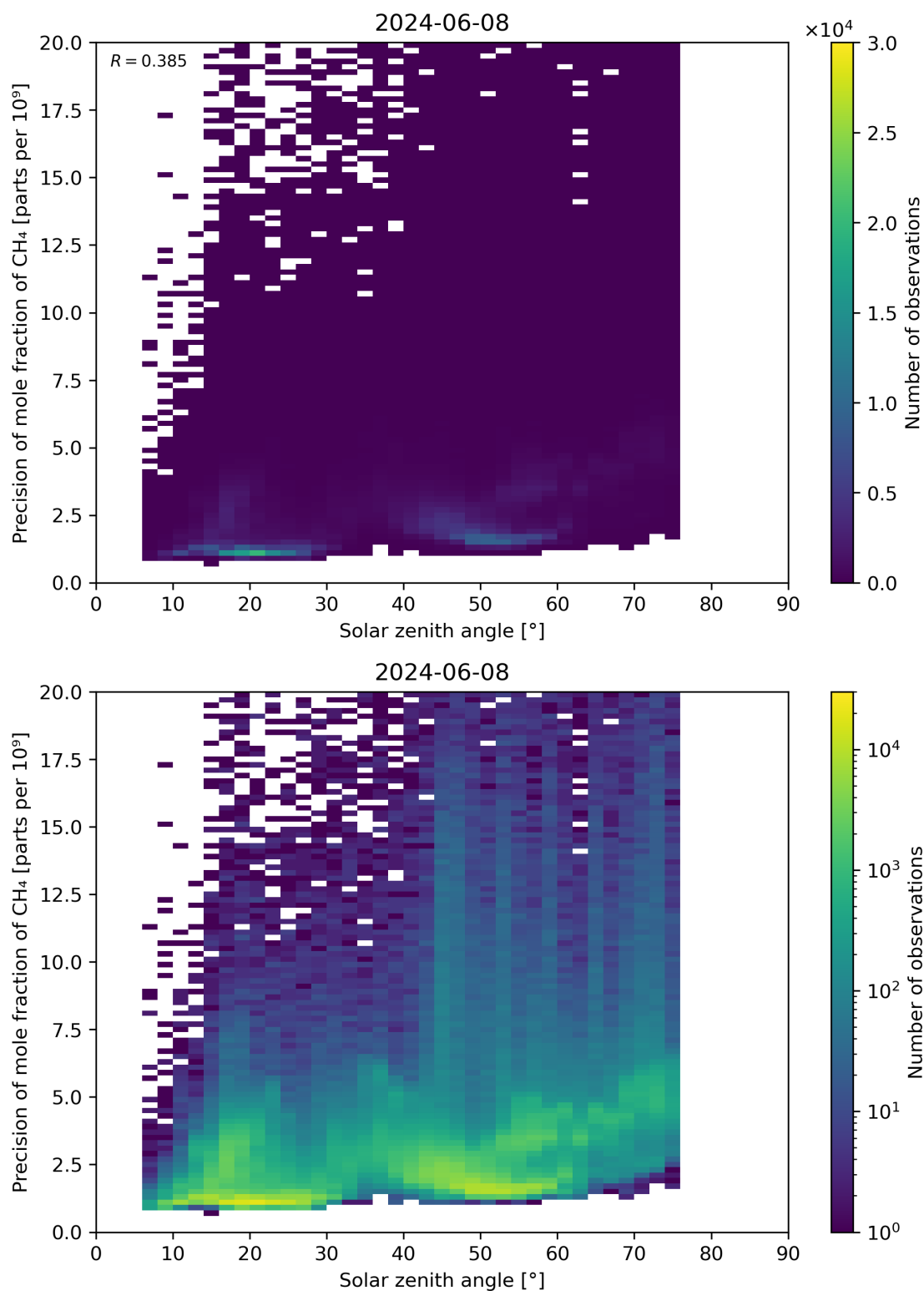
Figure 101: Scatter density plot of “Solar zenith angle” against “Precision of mole fraction of CH 4 ” for 2024-06-08 to 2024-06-09.
