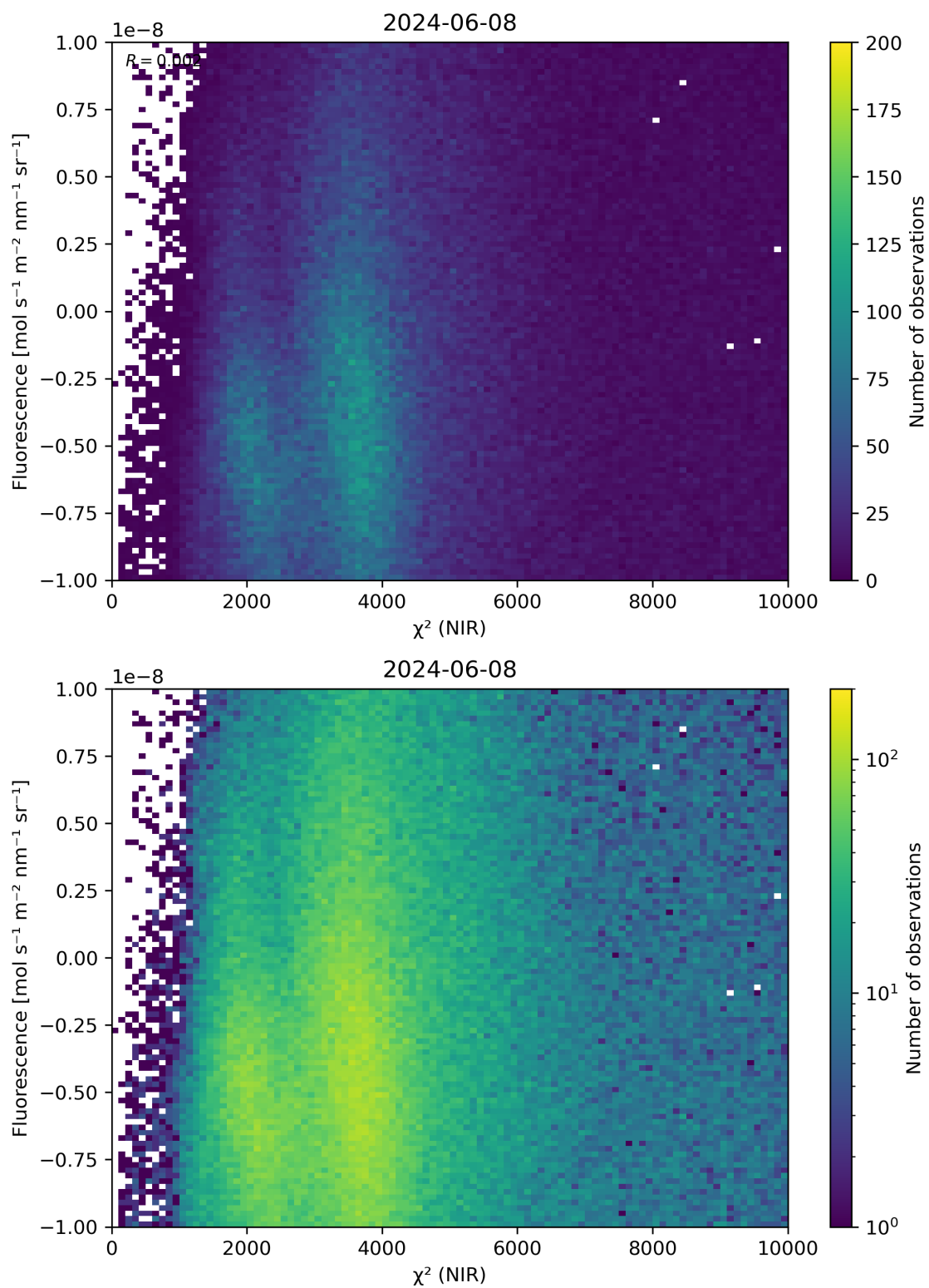
Figure 45: Scatter density plot of “ \chi^2 (NIR)” against “Fluorescence” for 2024-06-08 to 2024-06-09.
