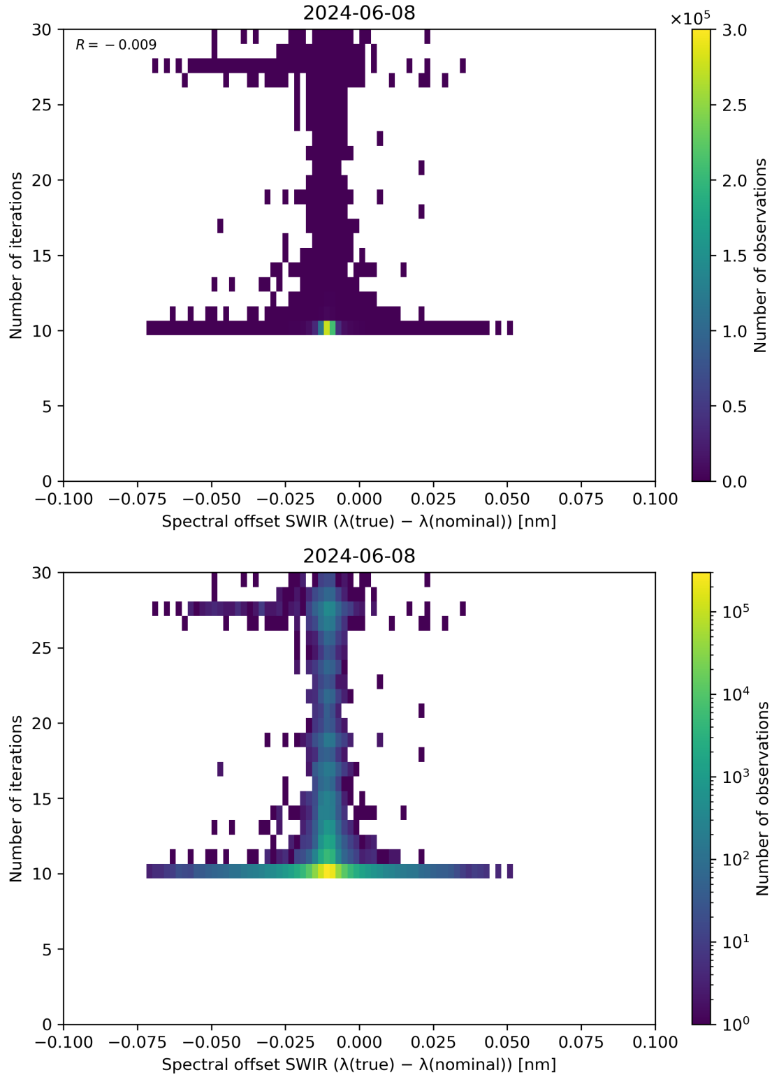
Figure 121: Scatter density plot of “Spectral offset SWIR ( \lambda(\text{true}) - \lambda(\text{nominal}) )” against “Number of iterations” for 2024-06-08 to 2024-06-09.
