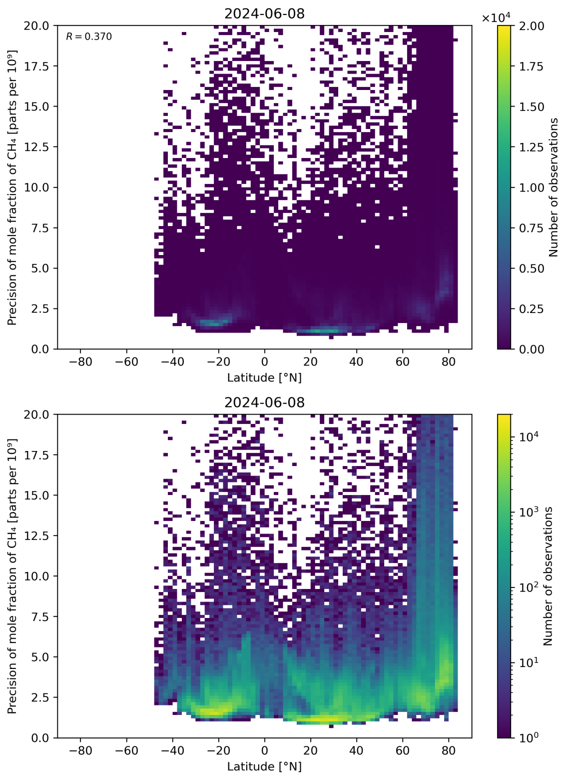
Figure 59: Scatter density plot of “Latitude” against “Precision of mole fraction of CH 4 ” for 2024-06-08 to 2024-06-09.
