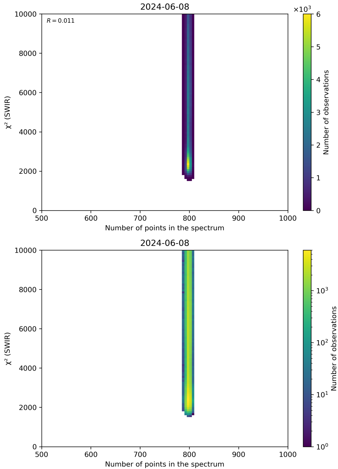
Figure 89: Scatter density plot of “Number of points in the spectrum” against “ \chi^2 (SWIR)” for 2024-06-08 to 2024-06-09.
