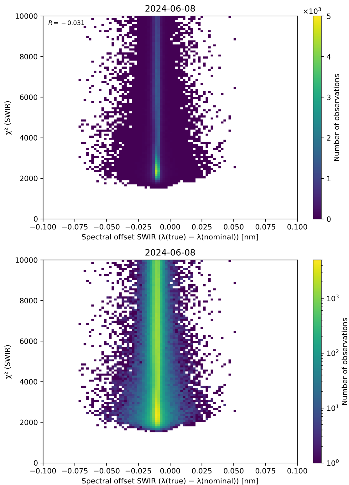
Figure 118: Scatter density plot of “Spectral offset SWIR ( \lambda(\text{true}) - \lambda(\text{nominal}) )” against “ \chi^2 (SWIR)” for 2024-06-08 to 2024-06-09.
