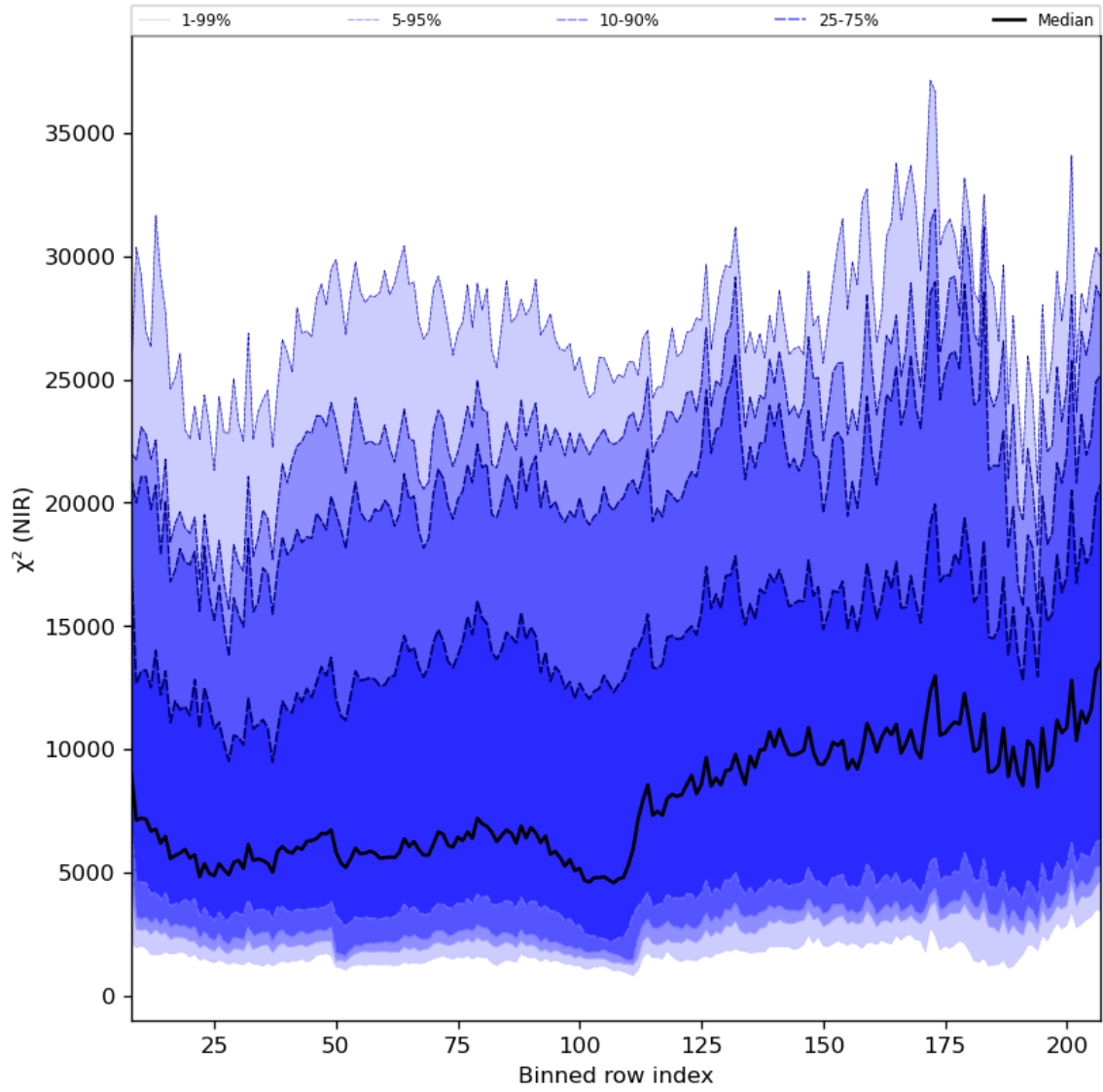
Figure 40: Along track statistics of “ \chi^2 (NIR)” for 2024-06-08 to 2024-06-09
