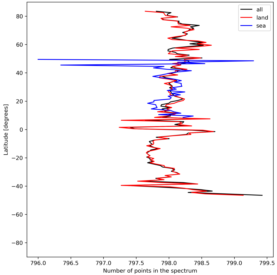
Figure 15: Zonal average of “Number of points in the spectrum” for 2024-06-08 to 2024-06-09.
