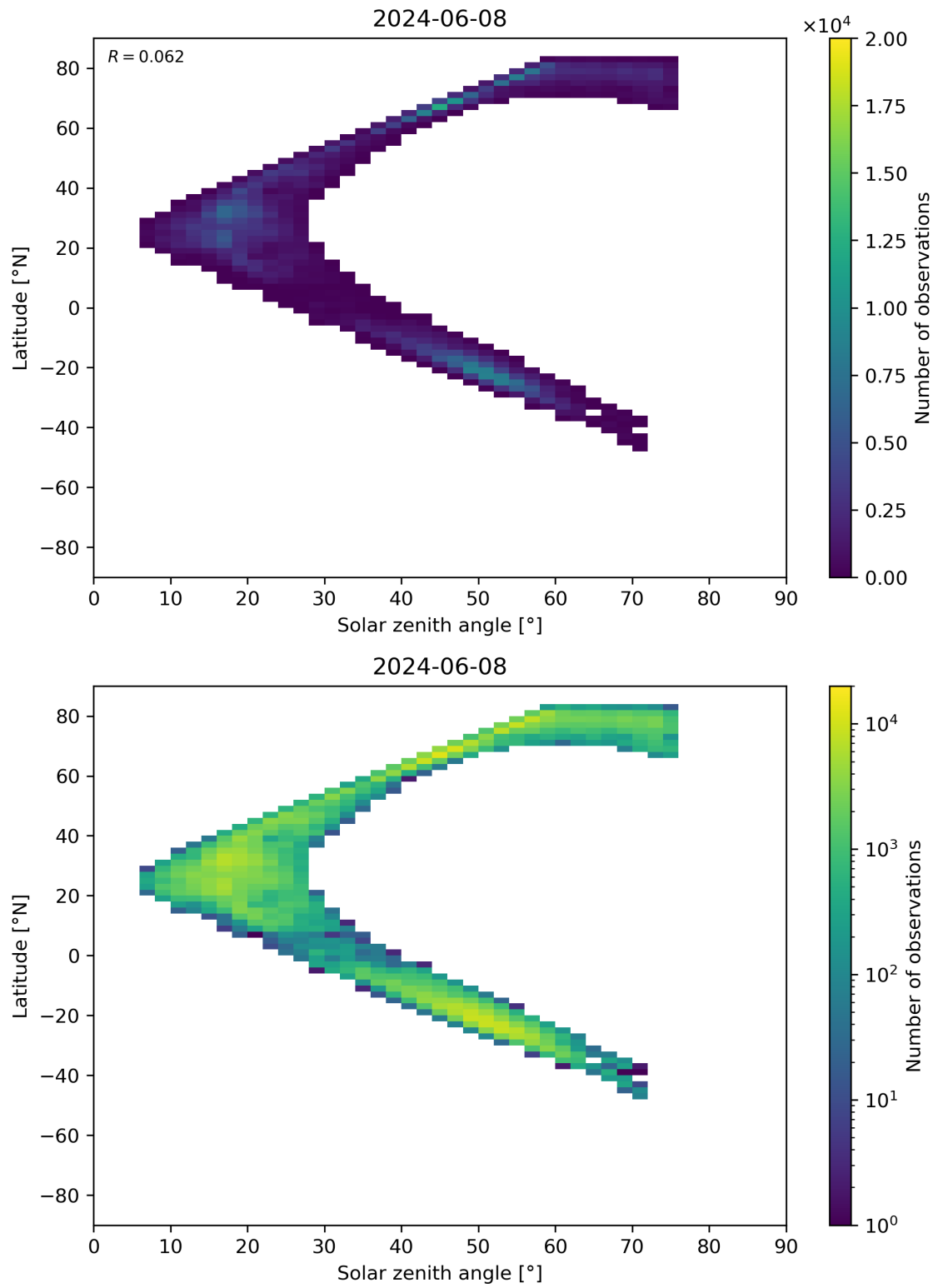
Figure 98: Scatter density plot of “Solar zenith angle” against “Latitude” for 2024-06-08 to 2024-06-09.
