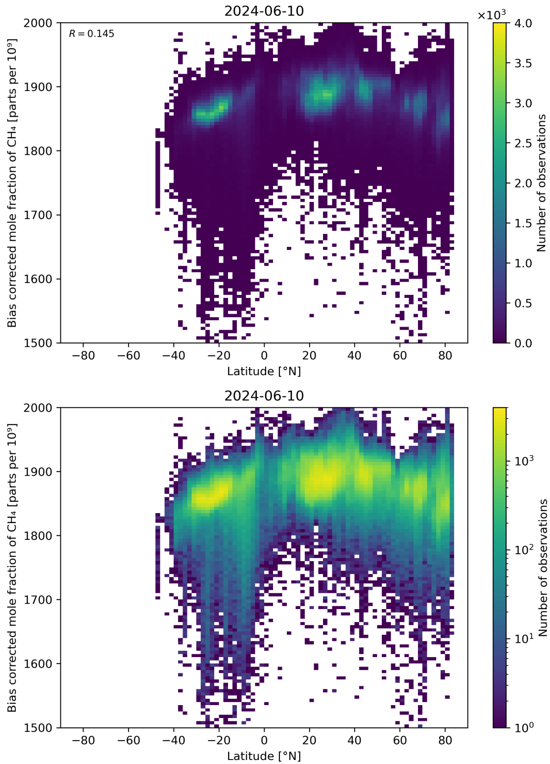
Figure 58: Scatter density plot of “Latitude” against “Bias corrected mole fraction of CH 4 ” for 2024-06-09 to 2024-06-11.
