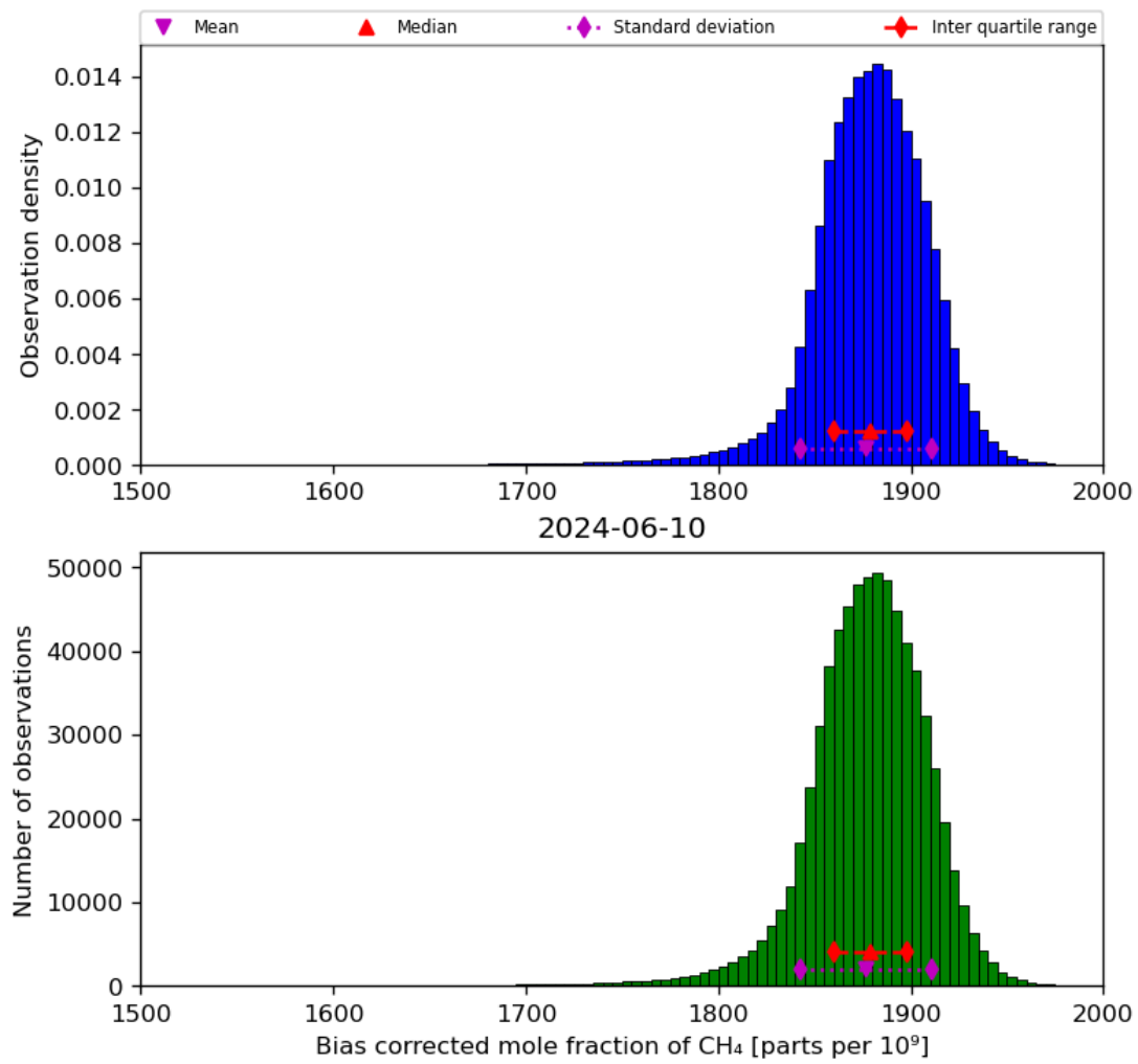
Figure 25: Histogram of “Bias corrected mole fraction of CH 4 ” for 2024-06-09 to 2024-06-11
