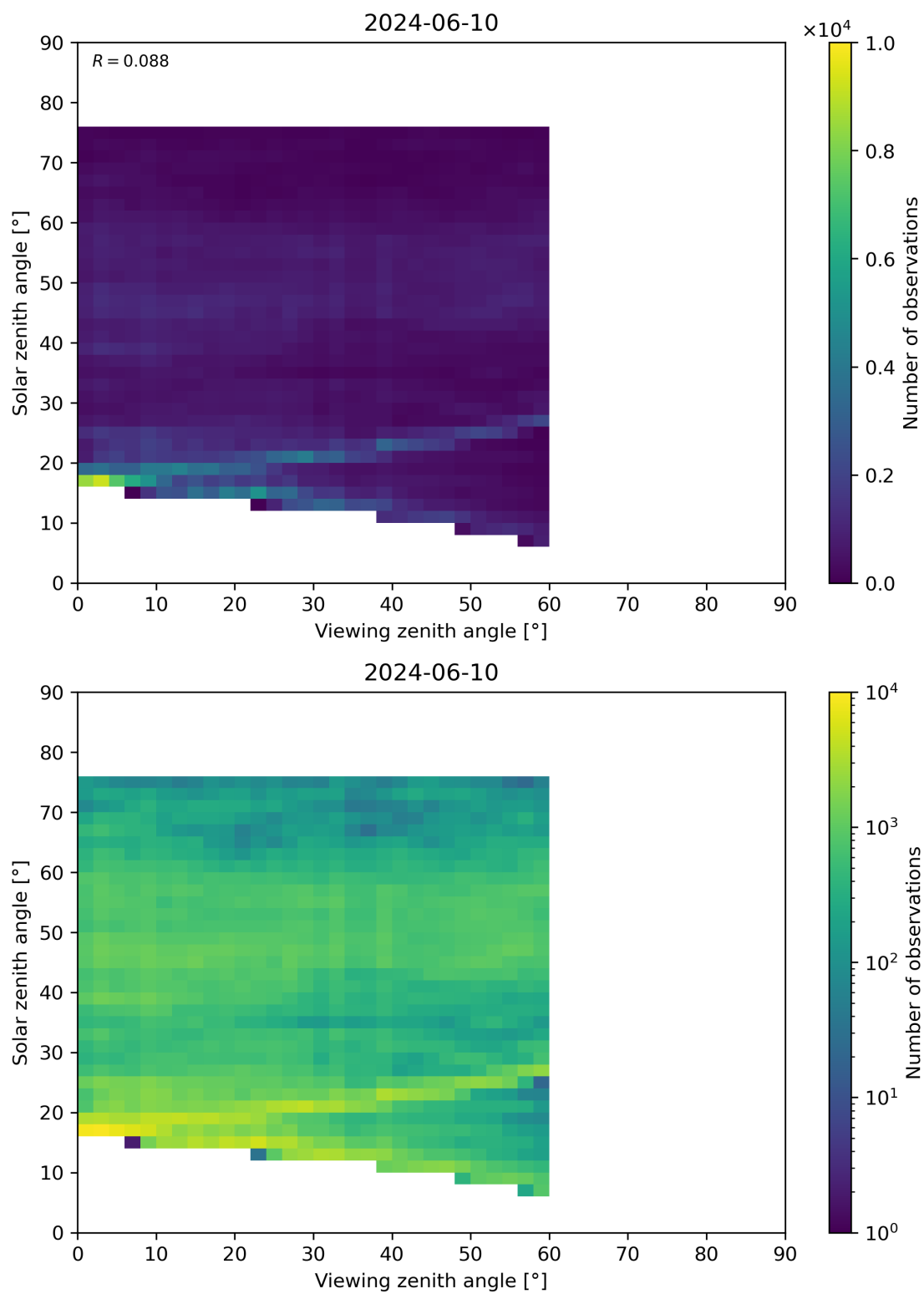
Figure 115: Scatter density plot of “Viewing zenith angle” against “Solar zenith angle” for 2024-06-09 to 2024-06-11.
