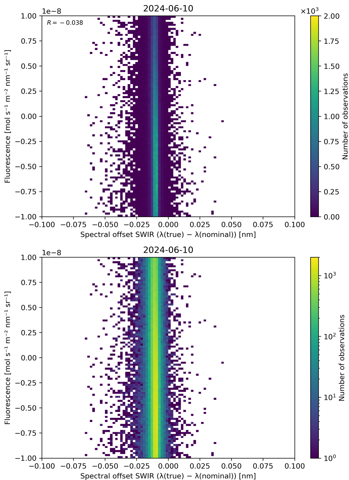
Figure 120: Scatter density plot of “Spectral offset SWIR ( \lambda(\text{true}) - \lambda(\text{nominal}) )” against “Fluorescence” for 2024-06-09 to 2024-06-11.
