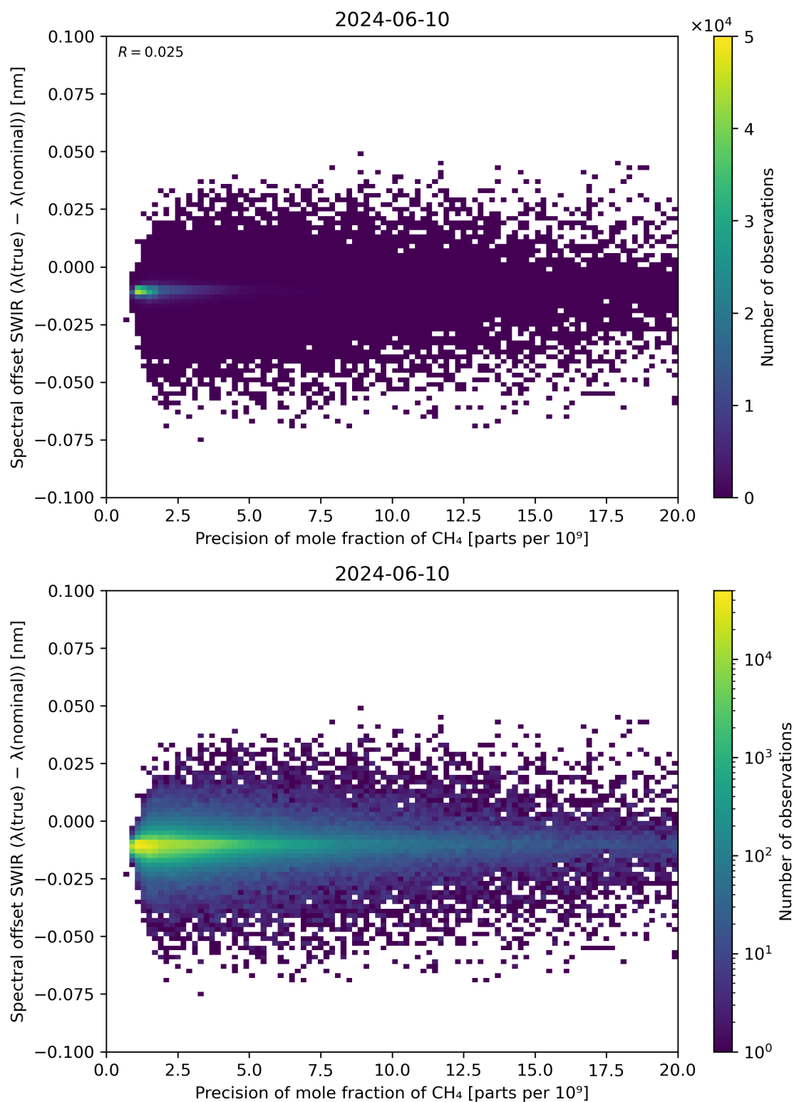
Figure 85: Scatter density plot of “Precision of mole fraction of \text{CH}_4 ” against “Spectral offset SWIR ( \lambda(\text{true}) - \lambda(\text{nominal}) )” for 2024-06-09 to 2024-06-11.
