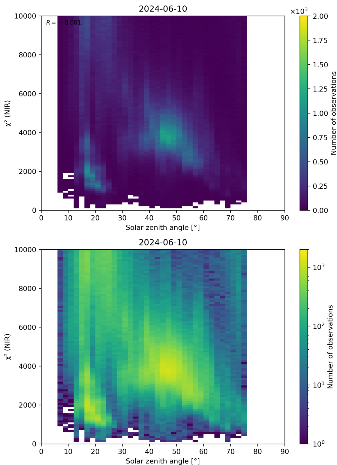
Figure 94: Scatter density plot of “Solar zenith angle” against “ \chi^2 (NIR)” for 2024-06-09 to 2024-06-11.
