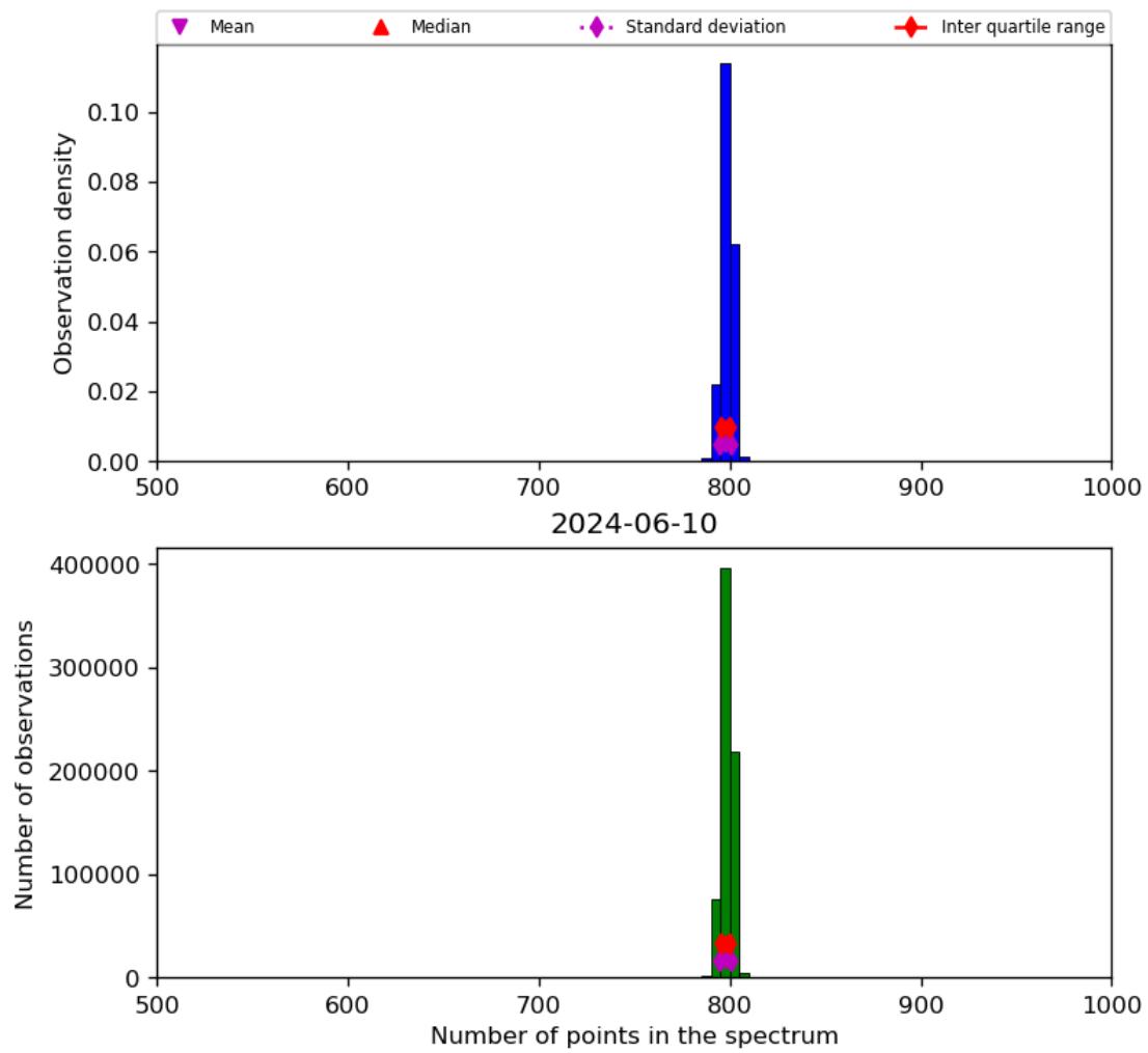
Figure 26: Histogram of “Number of points in the spectrum” for 2024-06-09 to 2024-06-11
