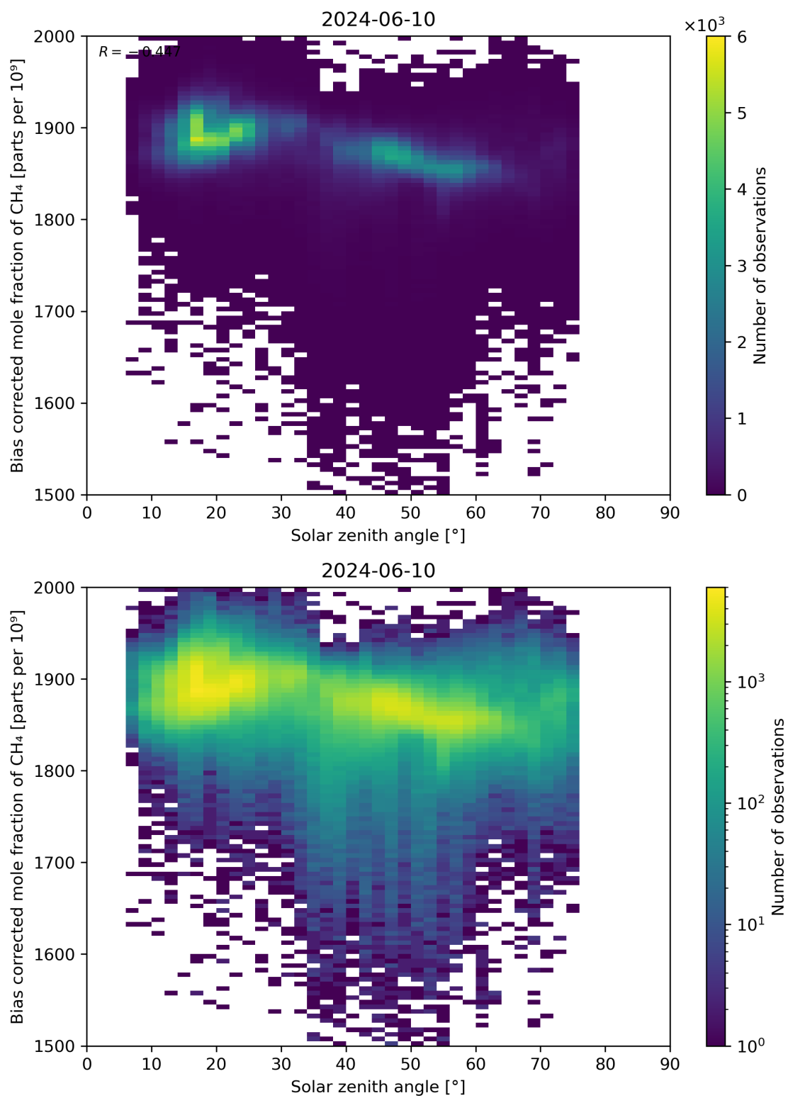
Figure 100: Scatter density plot of “Solar zenith angle” against “Bias corrected mole fraction of \text{CH}_4 ” for 2024-06-09 to 2024-06-11.
