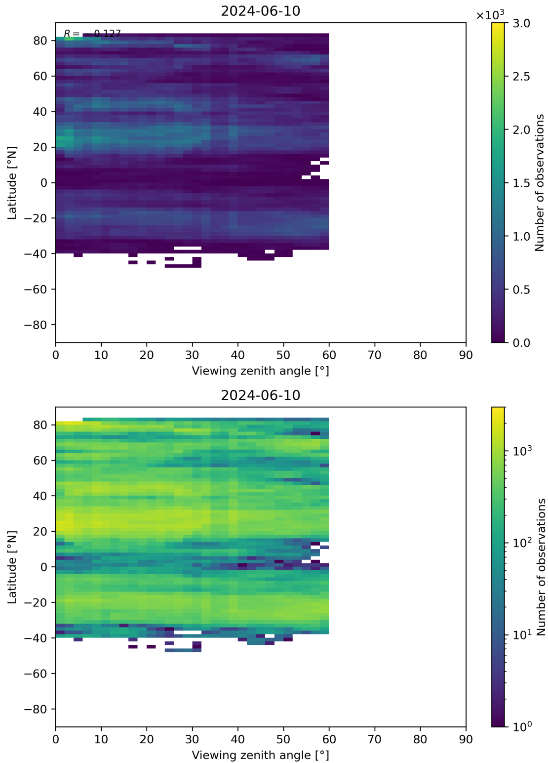
Figure 109: Scatter density plot of “Viewing zenith angle” against “Latitude” for 2024-06-09 to 2024-06-11.
