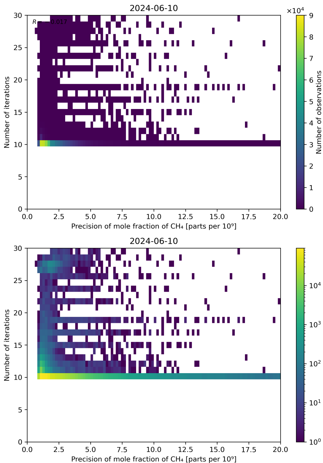
Figure 83: Scatter density plot of “Precision of mole fraction of CH 4 ” against “Number of iterations” for 2024-06-09 to 2024-06-11.
