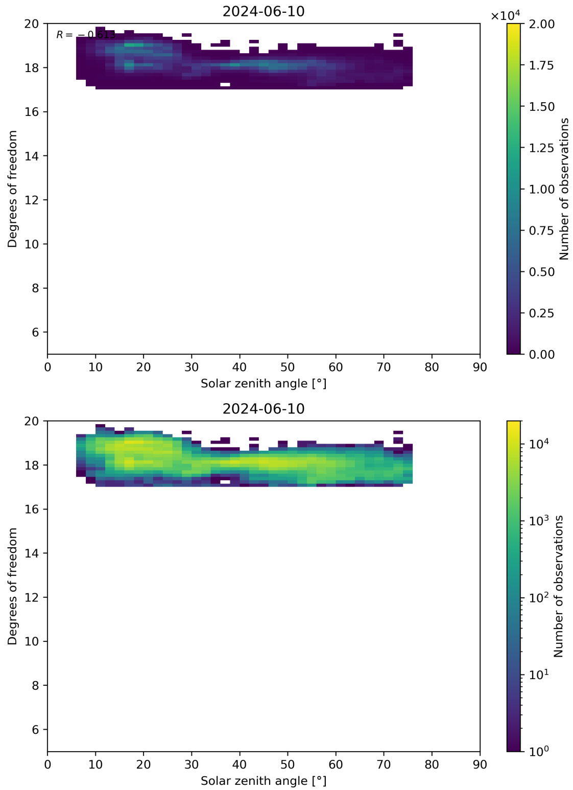
Figure 96: Scatter density plot of “Solar zenith angle” against “Degrees of freedom” for 2024-06-09 to 2024-06-11.
