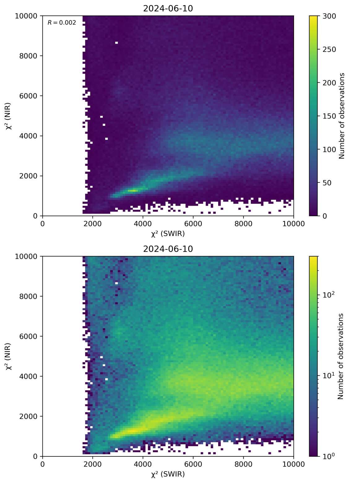
Figure 47: Scatter density plot of “ \chi^2 (SWIR)” against “ \chi^2 (NIR)” for 2024-06-09 to 2024-06-11.
