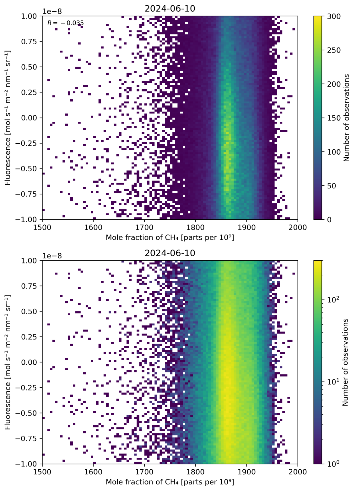
Figure 73: Scatter density plot of “Mole fraction of \text{CH}_4 ” against “Fluorescence” for 2024-06-09 to 2024-06-11.
