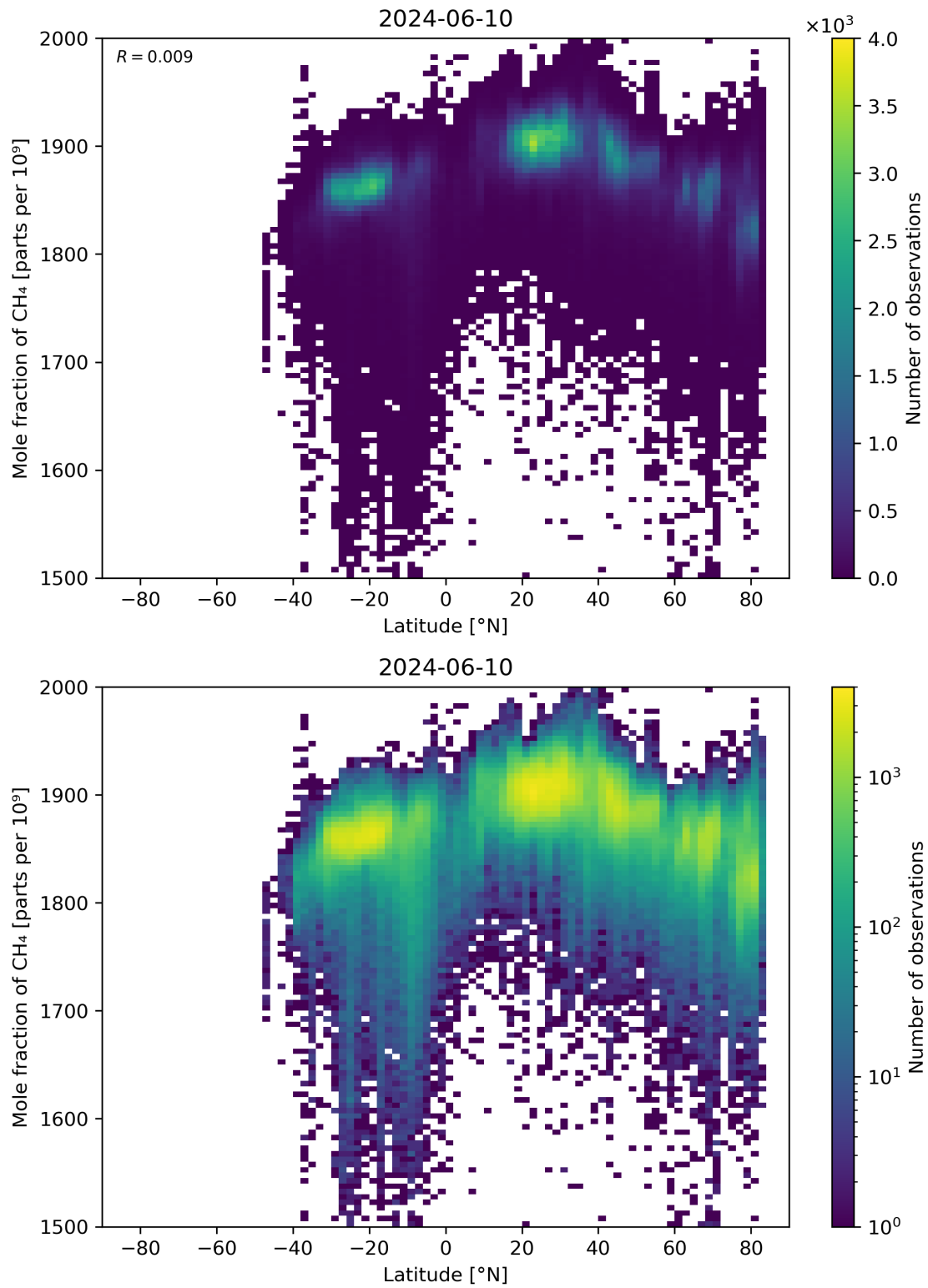
Figure 57: Scatter density plot of “Latitude” against “Mole fraction of \text{CH}_4 ” for 2024-06-09 to 2024-06-11.
