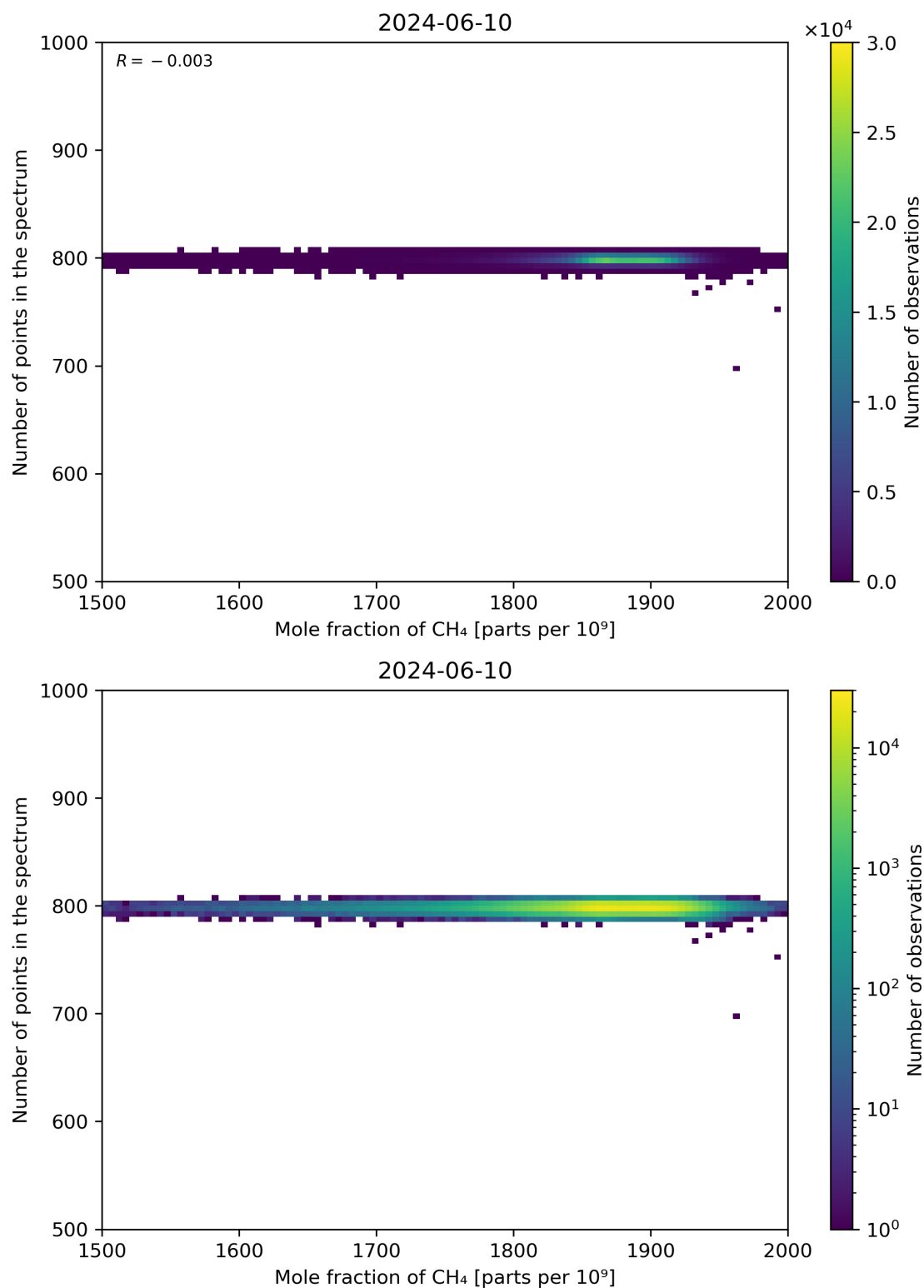
Figure 77: Scatter density plot of “Mole fraction of CH 4 ” against “Number of points in the spectrum” for 2024-06-09 to 2024-06-11.
