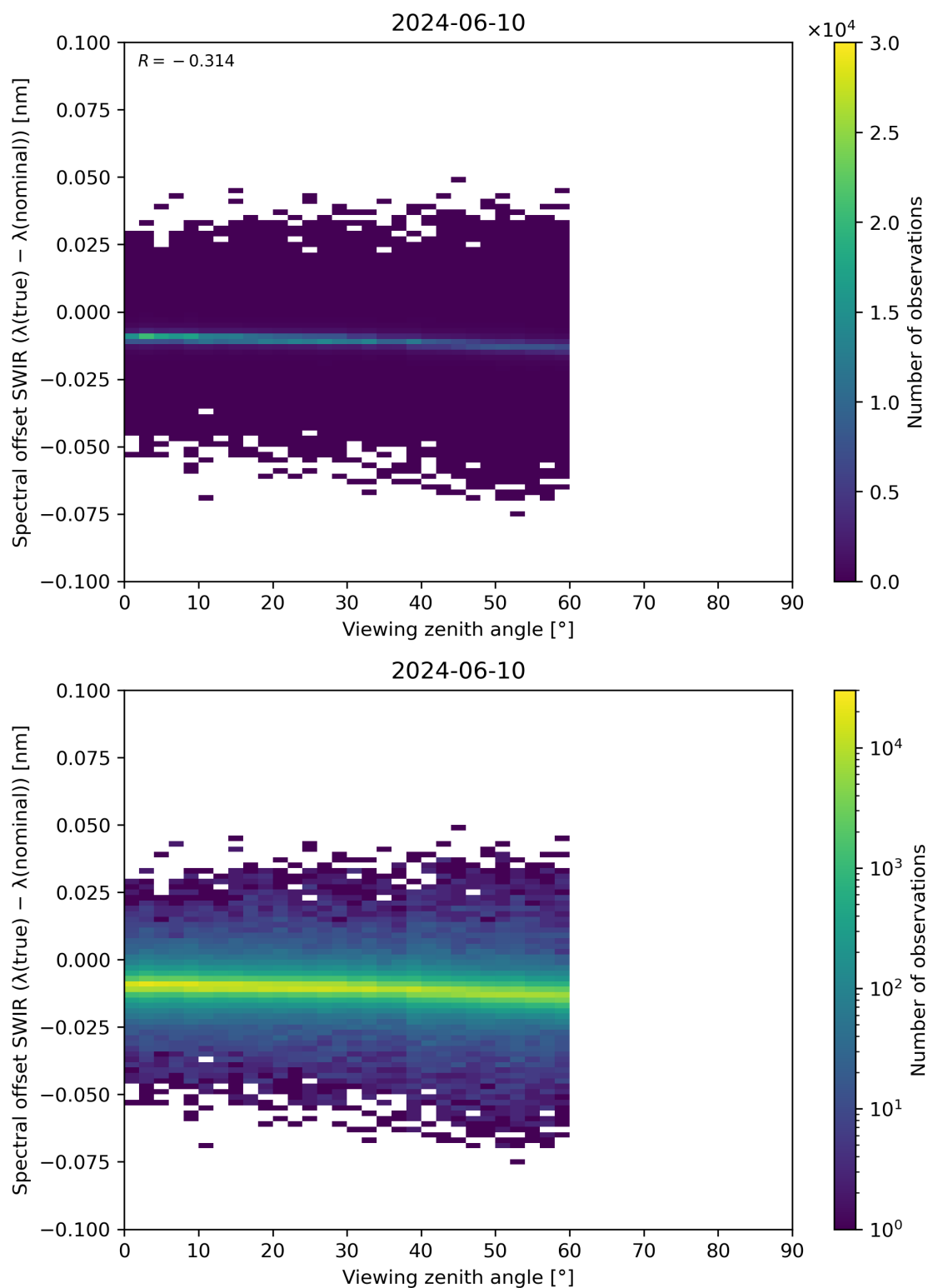
Figure 116: Scatter density plot of “Viewing zenith angle” against “Spectral offset SWIR ( \lambda(\text{true}) - \lambda(\text{nominal}) )” for 2024-06-09 to 2024-06-11.
