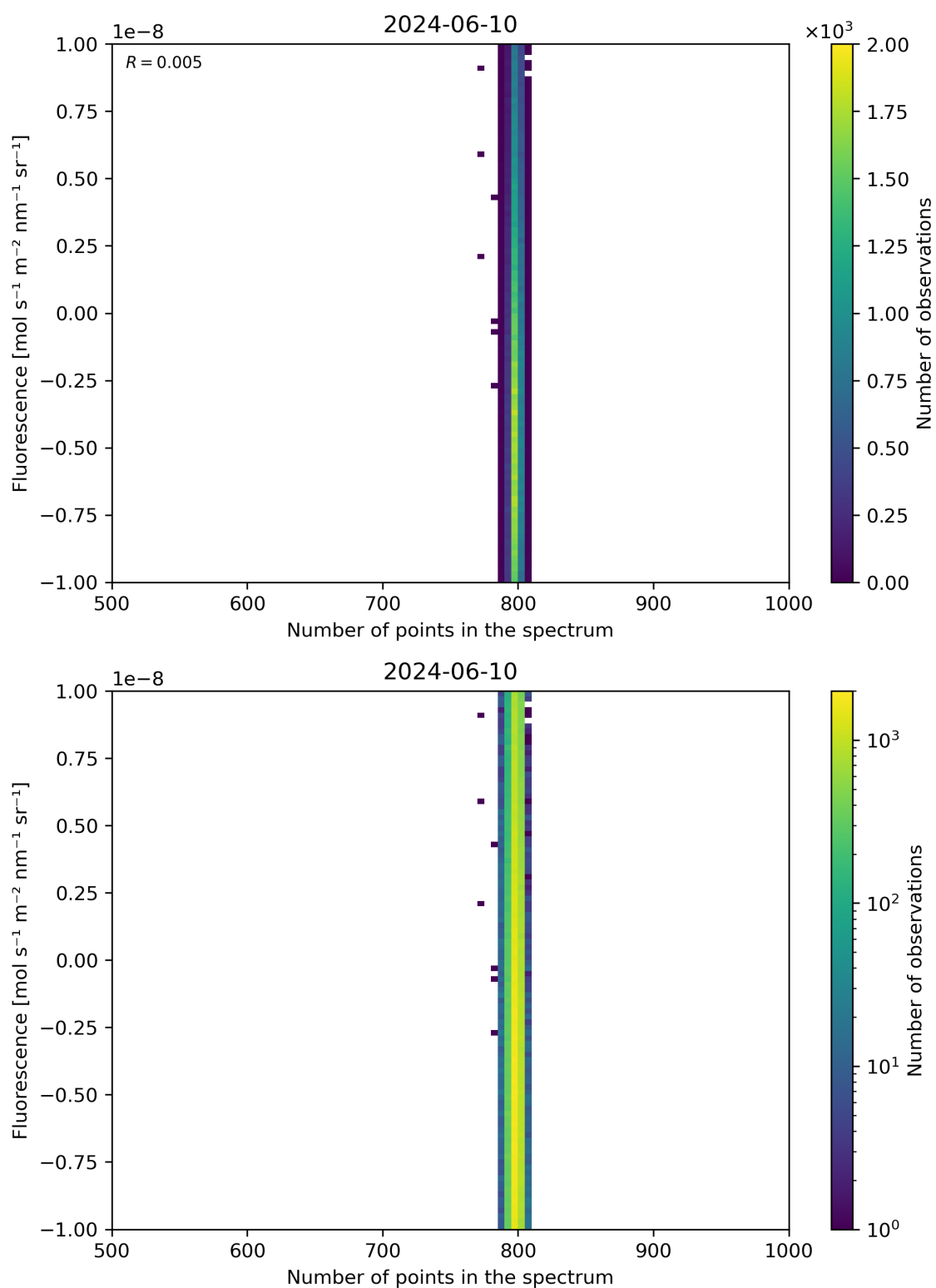
Figure 91: Scatter density plot of “Number of points in the spectrum” against “Fluorescence” for 2024-06-09 to 2024-06-11.
