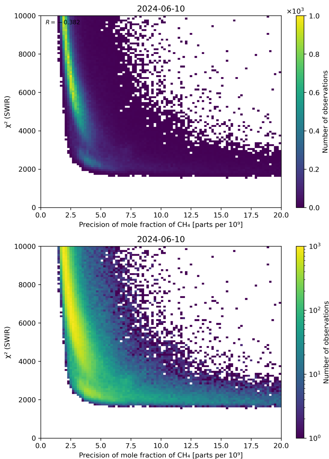
Figure 79: Scatter density plot of “Precision of mole fraction of \text{CH}_4 ” against “ \chi^2 (SWIR)” for 2024-06-09 to 2024-06-11.
