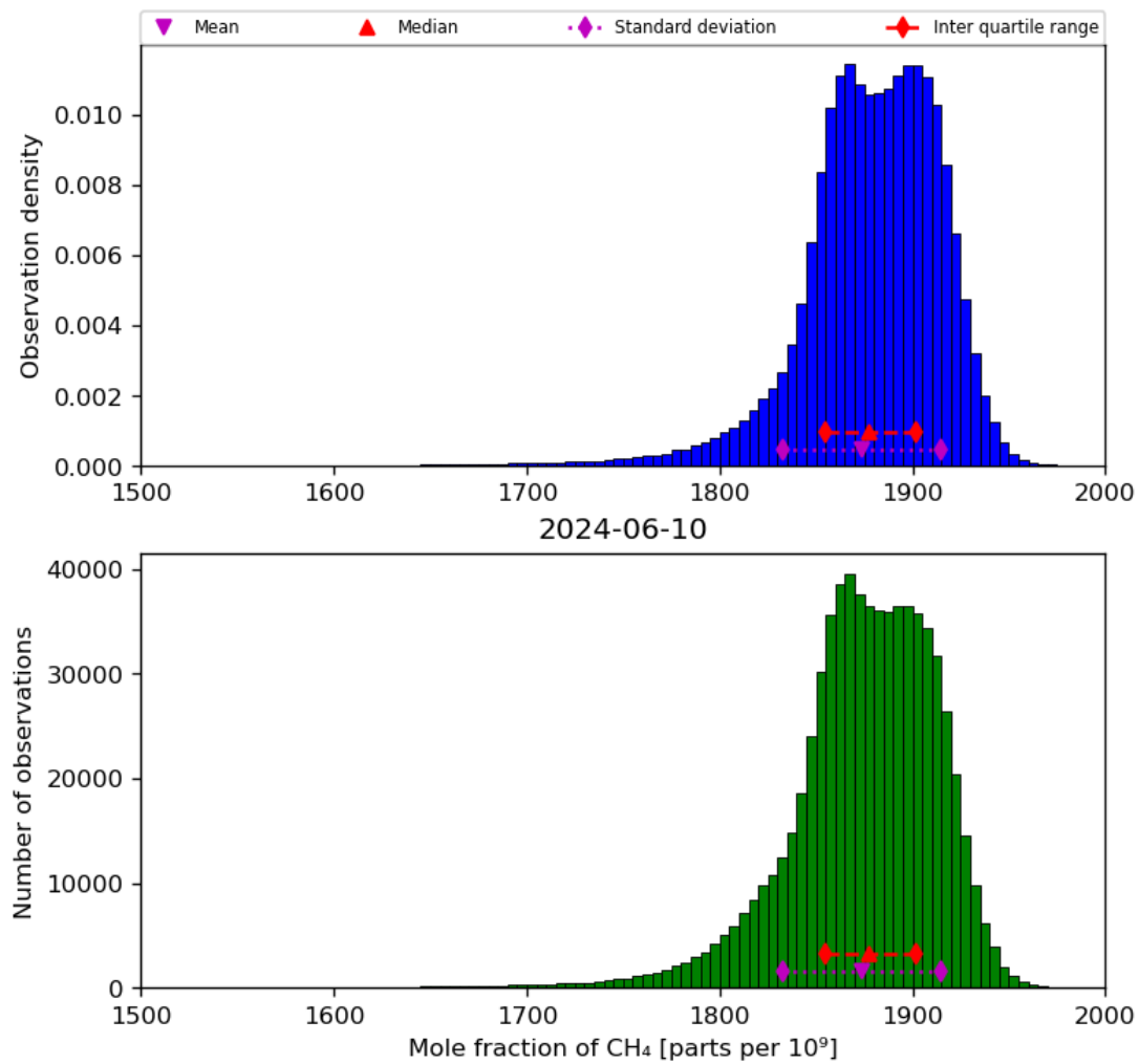
Figure 23: Histogram of “Mole fraction of CH 4 ” for 2024-06-09 to 2024-06-11
