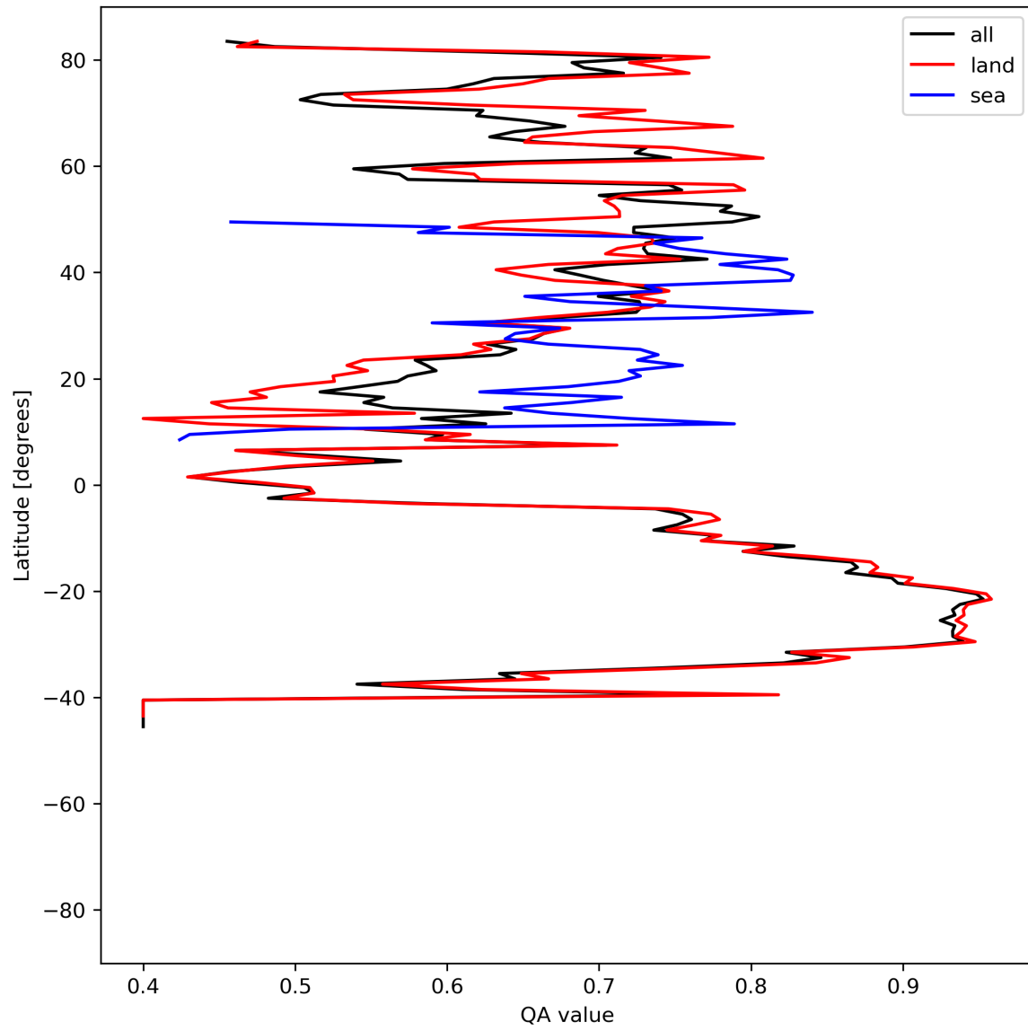
Figure 11: Zonal average of “QA value” for 2024-06-09 to 2024-06-11.
