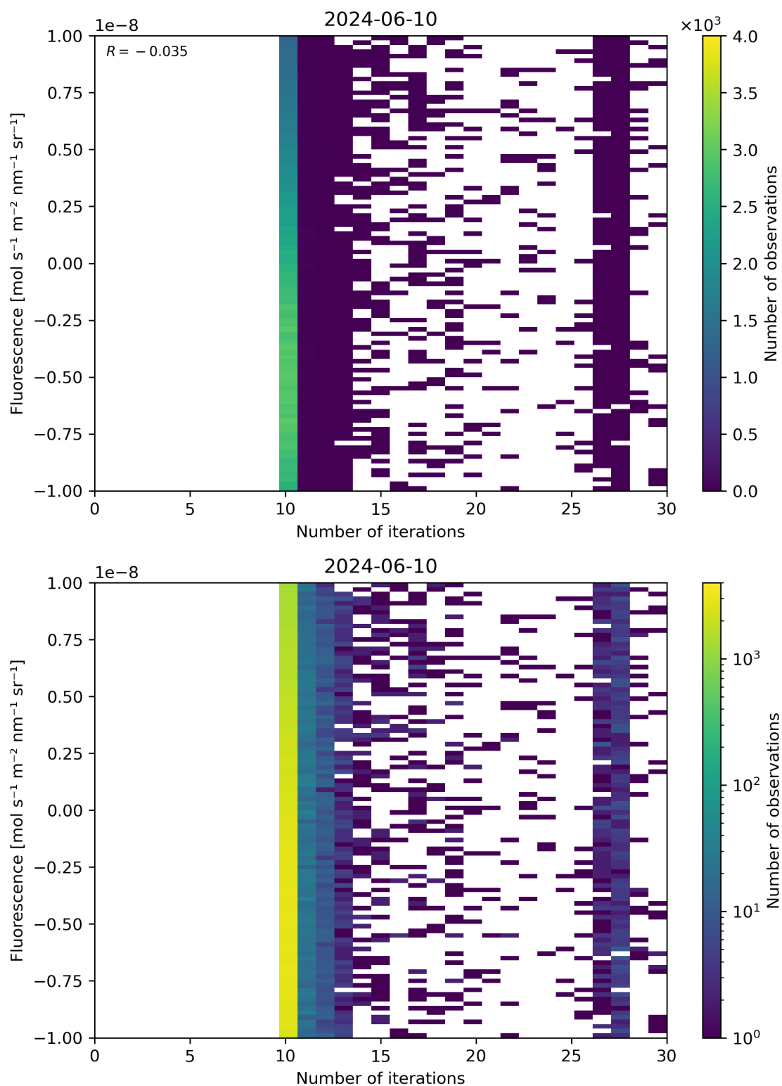
Figure 87: Scatter density plot of “Number of iterations” against “Fluorescence” for 2024-06-09 to 2024-06-11.
