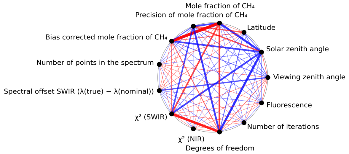
Figure 1: Map of correlation graph for 2024-06-09 to 2024-06-11.
