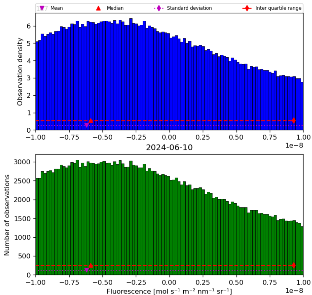
Figure 32: Histogram of “Fluorescence” for 2024-06-09 to 2024-06-11
