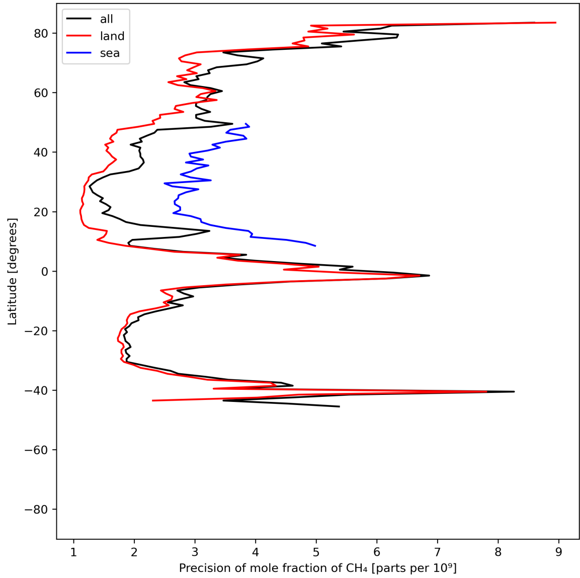
Figure 13: Zonal average of “Precision of mole fraction of CH 4 ” for 2024-06-09 to 2024-06-11.
