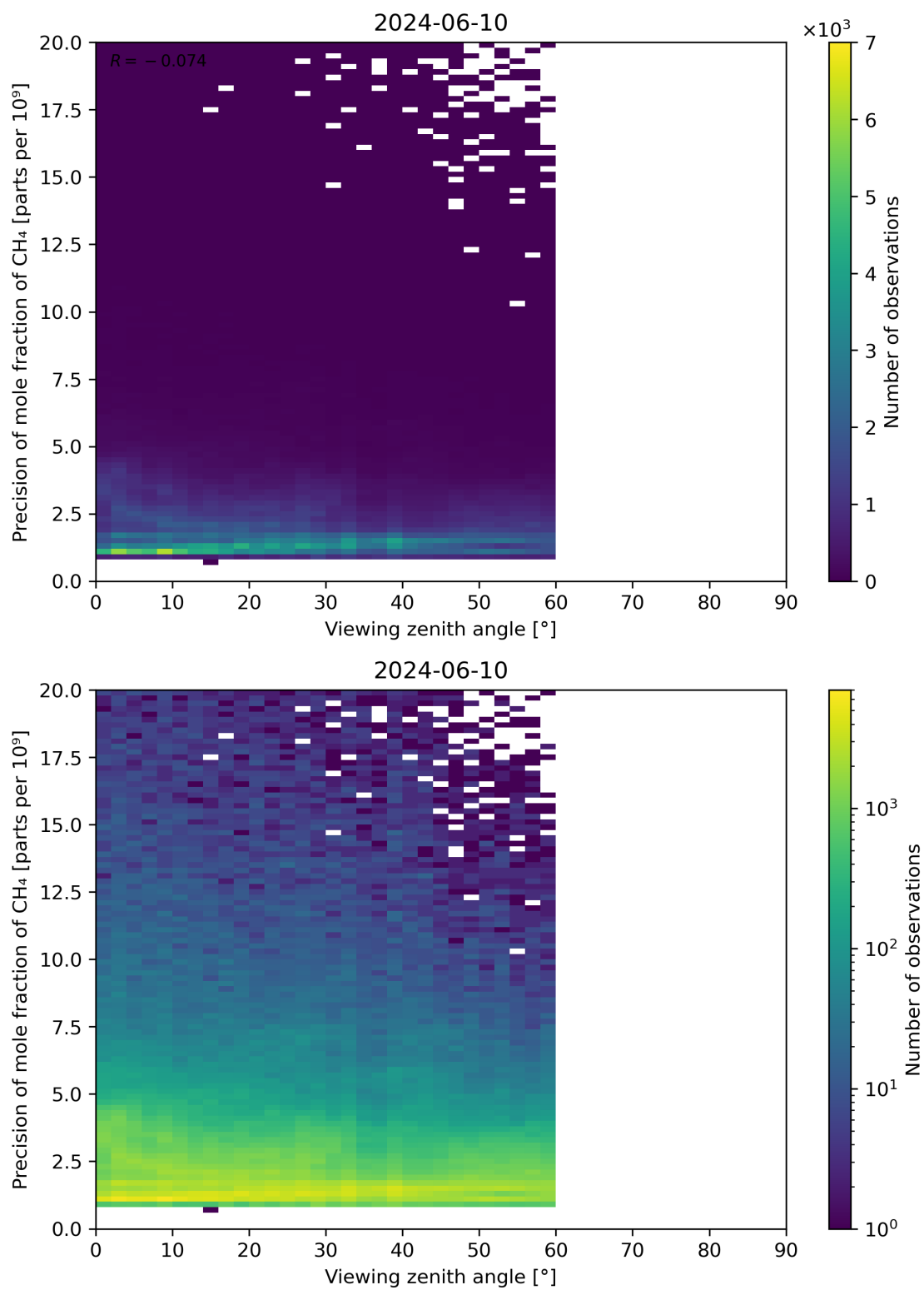
Figure 112: Scatter density plot of “Viewing zenith angle” against “Precision of mole fraction of CH 4 ” for 2024-06-09 to 2024-06-11.
