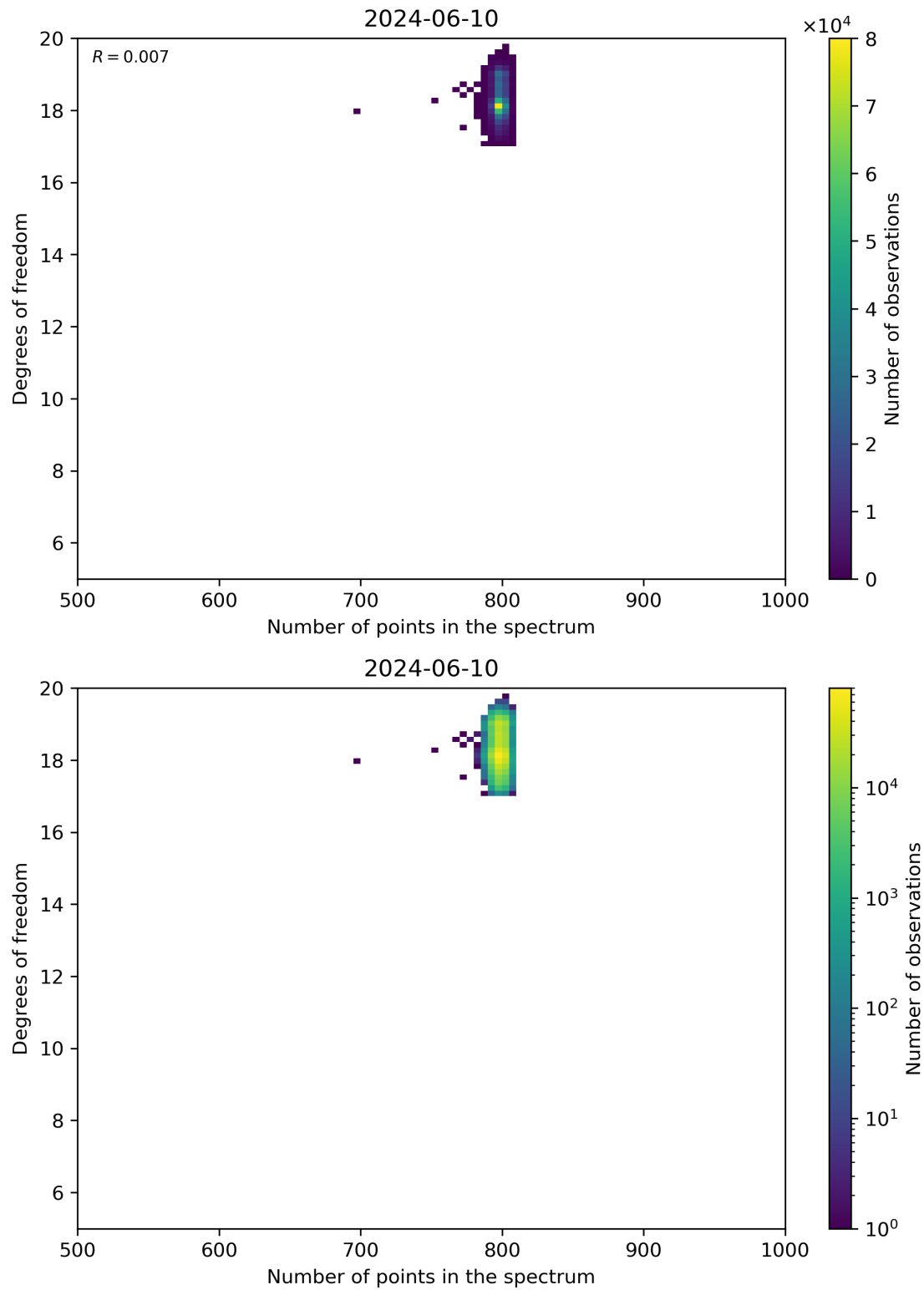
Figure 90: Scatter density plot of “Number of points in the spectrum” against “Degrees of freedom” for 2024-06-09 to 2024-06-11.
