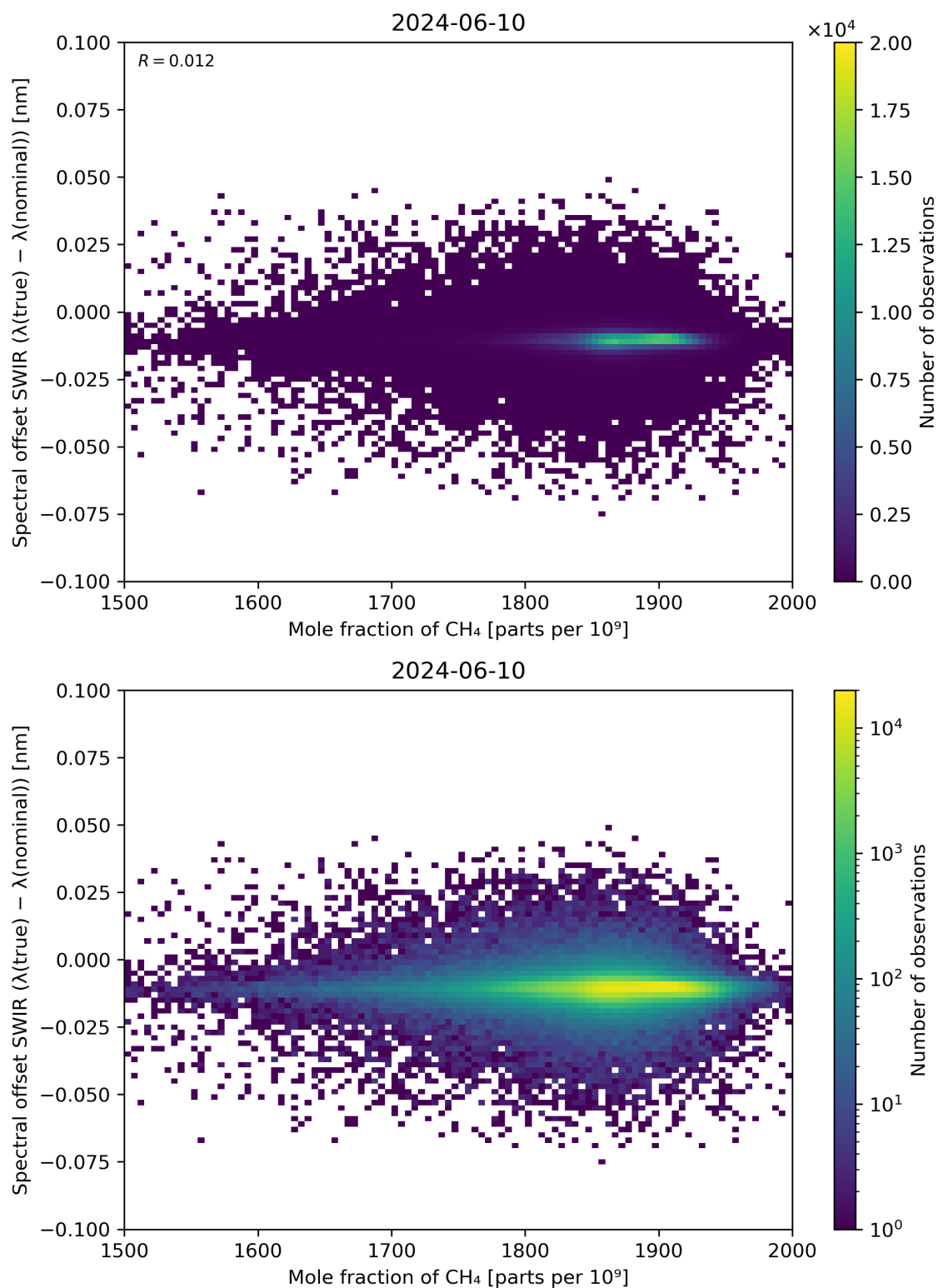
Figure 86: Scatter density plot of “Mole fraction of CH 4 ” against “Spectral offset SWIR ( \lambda(\text{true}) - \lambda(\text{nominal}) )” for 2024-06-09 to 2024-06-11.
