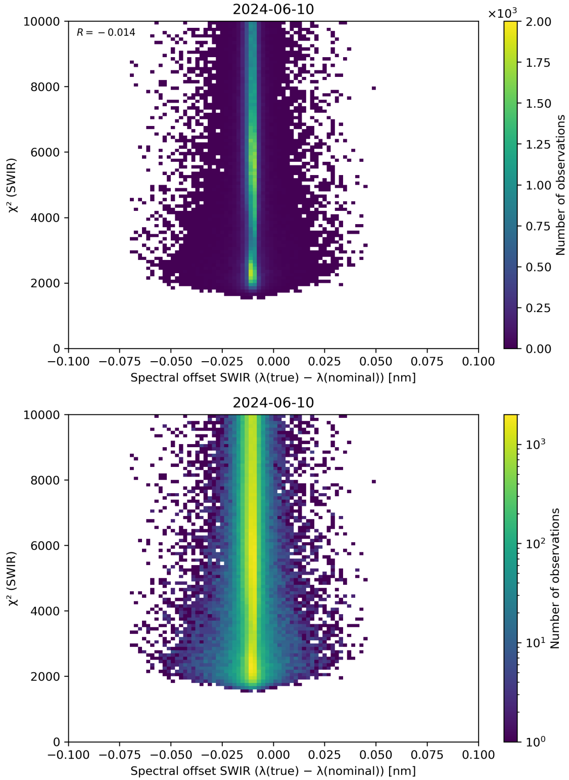
Figure 118: Scatter density plot of “Spectral offset SWIR ( \lambda(\text{true}) - \lambda(\text{nominal}) )” against “ \chi^2 (SWIR)” for 2024-06-09 to 2024-06-11.
