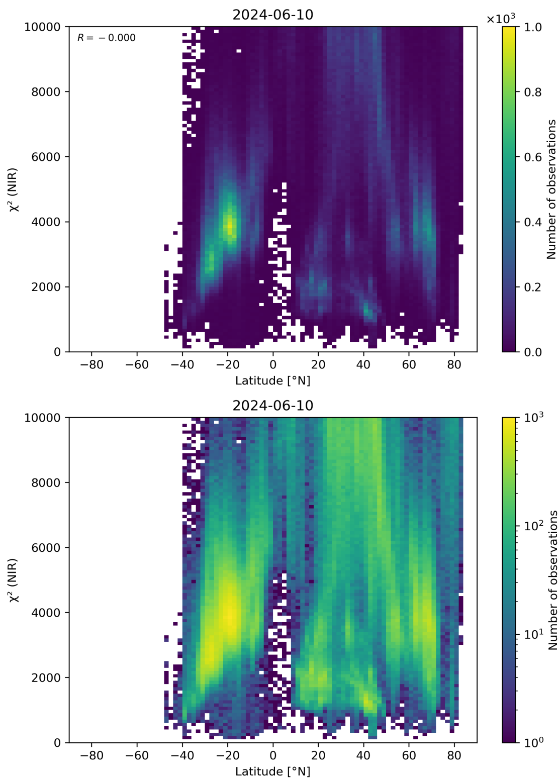
Figure 53: Scatter density plot of “Latitude” against “ \chi^2 (NIR)” for 2024-06-09 to 2024-06-11.
