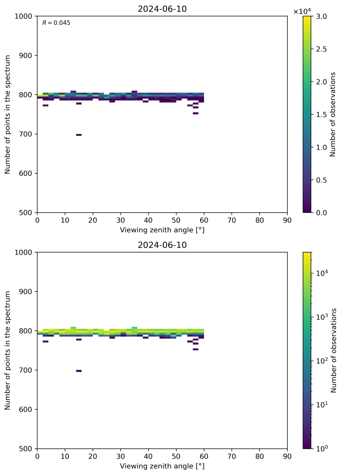
Figure 114: Scatter density plot of “Viewing zenith angle” against “Number of points in the spectrum” for 2024-06-09 to 2024-06-11.
