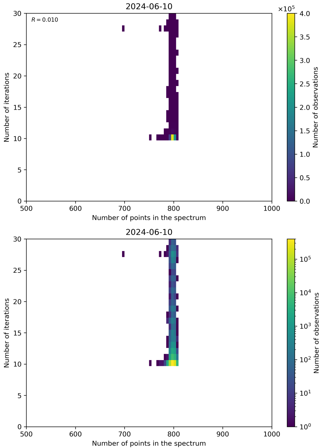
Figure 92: Scatter density plot of “Number of points in the spectrum” against “Number of iterations” for 2024-06-09 to 2024-06-11.
