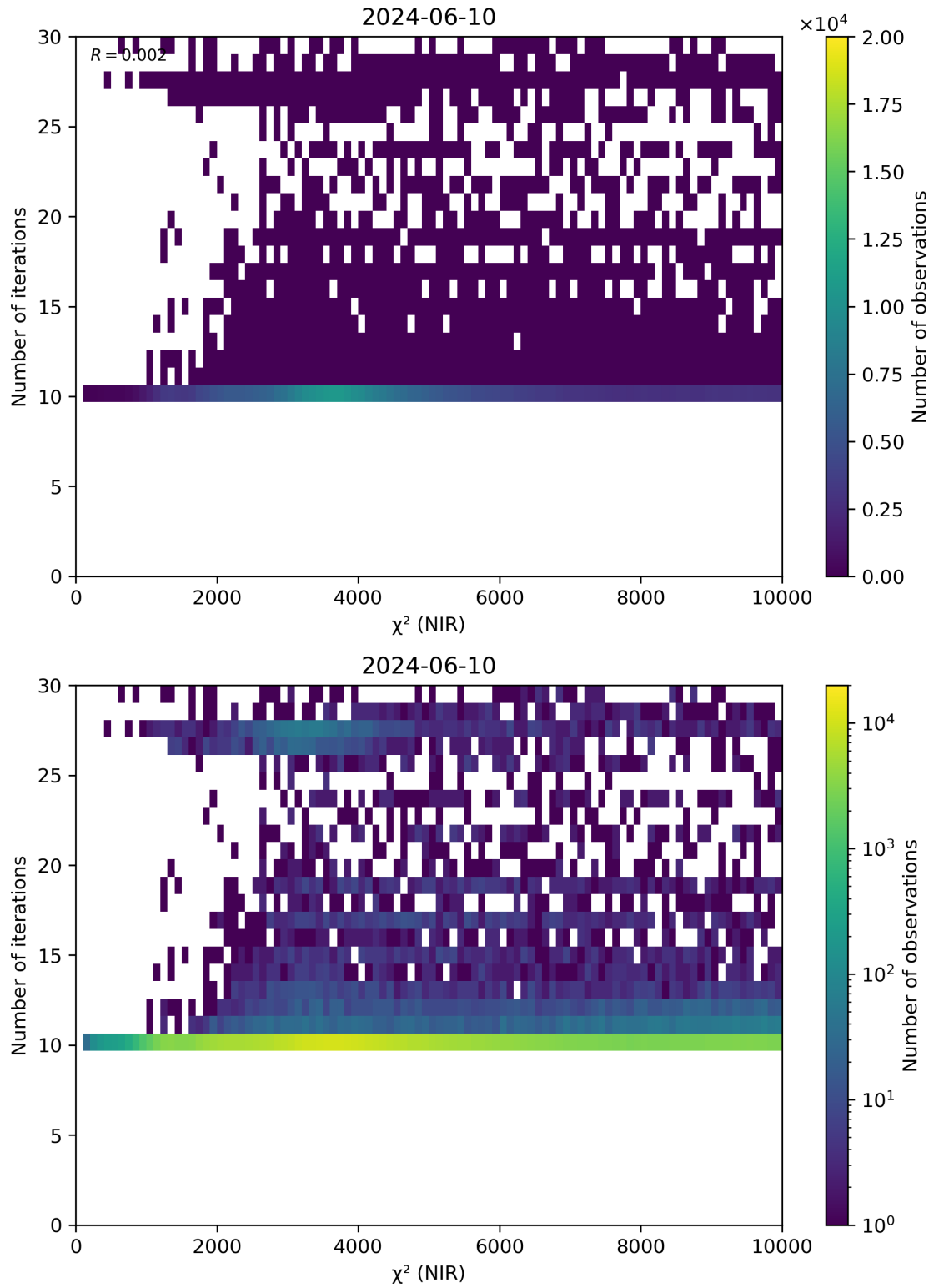
Figure 46: Scatter density plot of “ \chi^2 (NIR)” against “Number of iterations” for 2024-06-09 to 2024-06-11.
