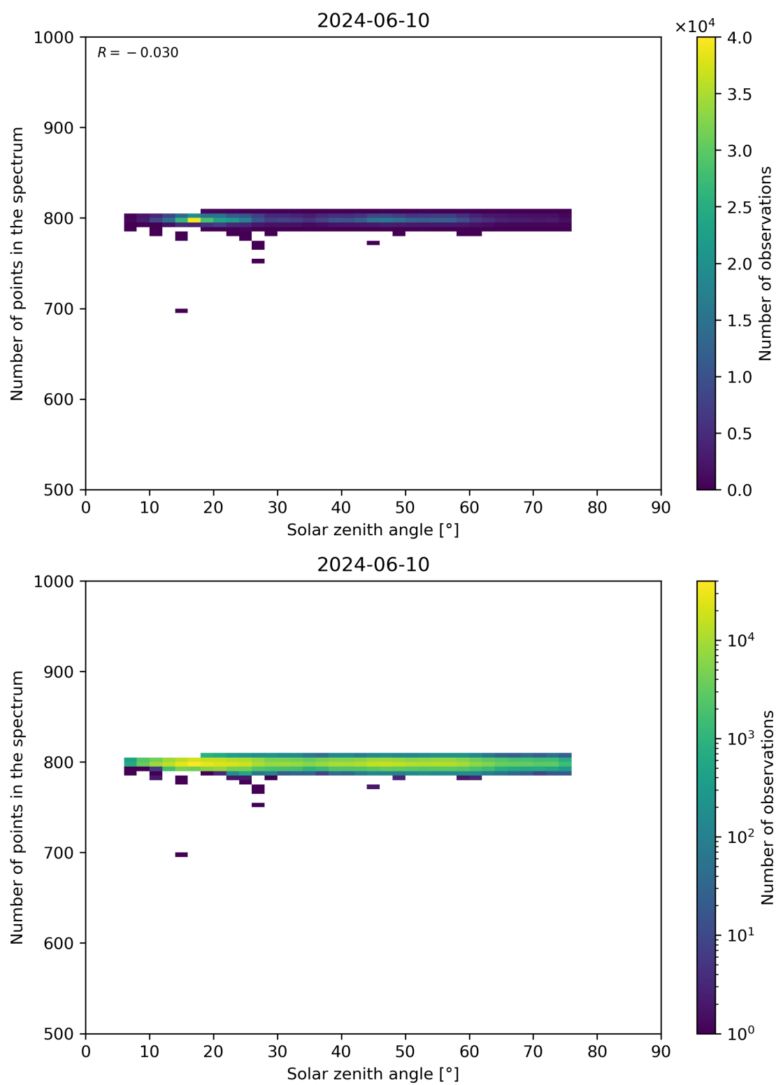
Figure 103: Scatter density plot of “Solar zenith angle” against “Number of points in the spectrum” for 2024-06-09 to 2024-06-11.
