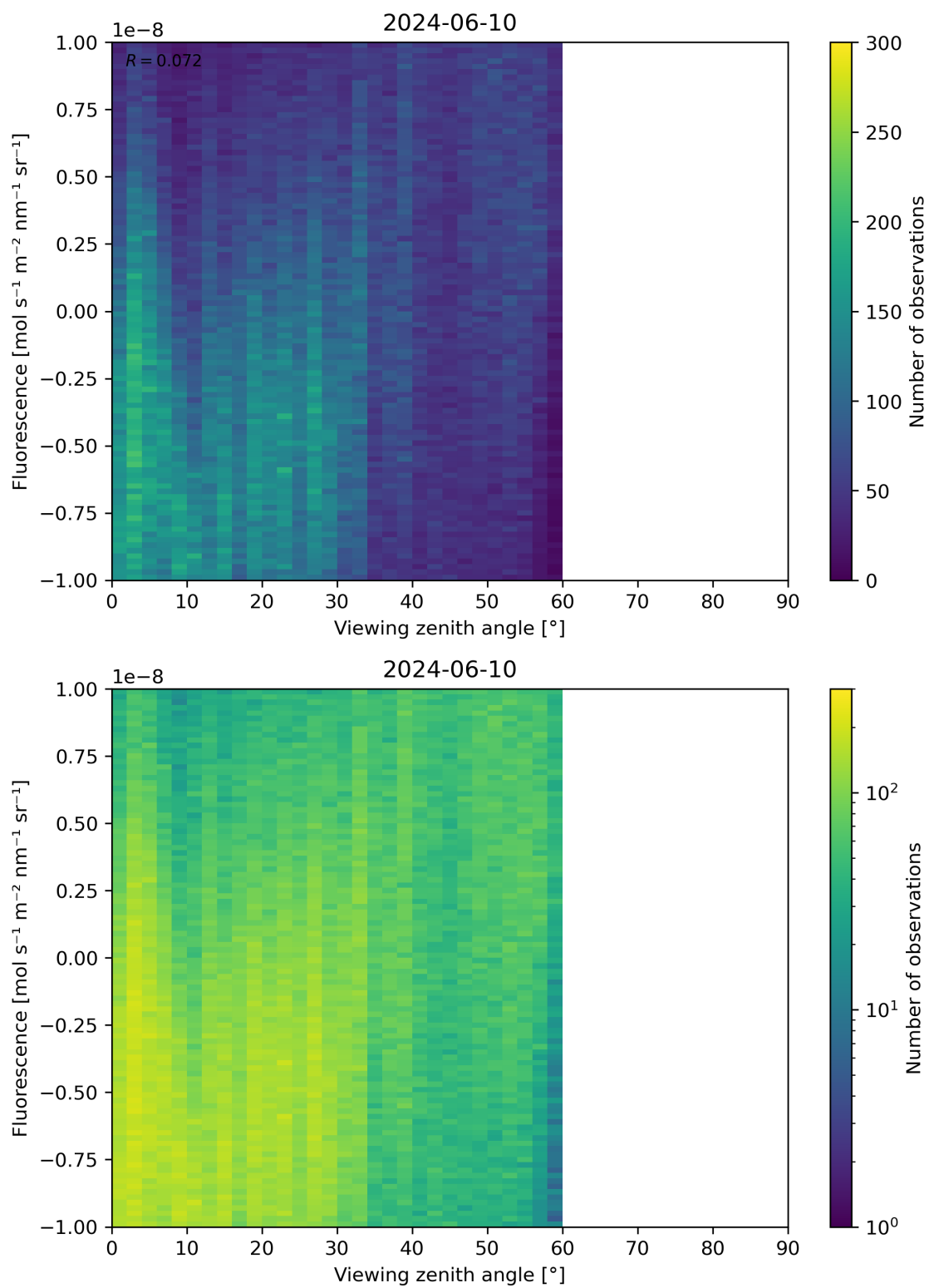
Figure 108: Scatter density plot of “Viewing zenith angle” against “Fluorescence” for 2024-06-09 to 2024-06-11.
