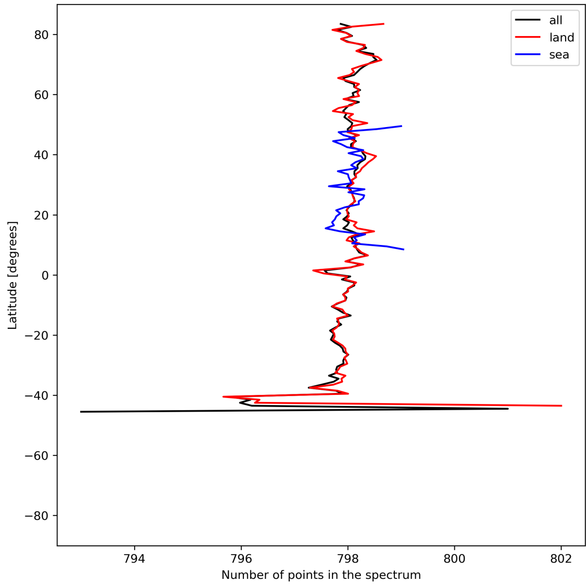
Figure 15: Zonal average of “Number of points in the spectrum” for 2024-06-09 to 2024-06-11.
