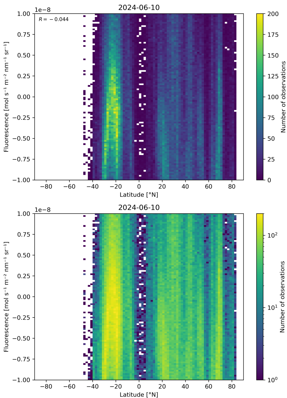
Figure 56: Scatter density plot of “Latitude” against “Fluorescence” for 2024-06-09 to 2024-06-11.
