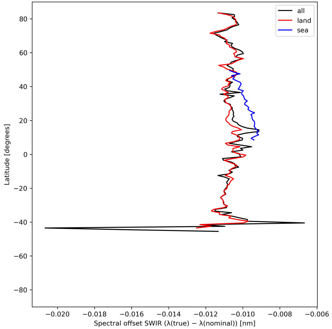
Figure 16: Zonal average of “Spectral offset SWIR ( \lambda(\text{true}) - \lambda(\text{nominal}) )” for 2024-06-09 to 2024-06-11.
