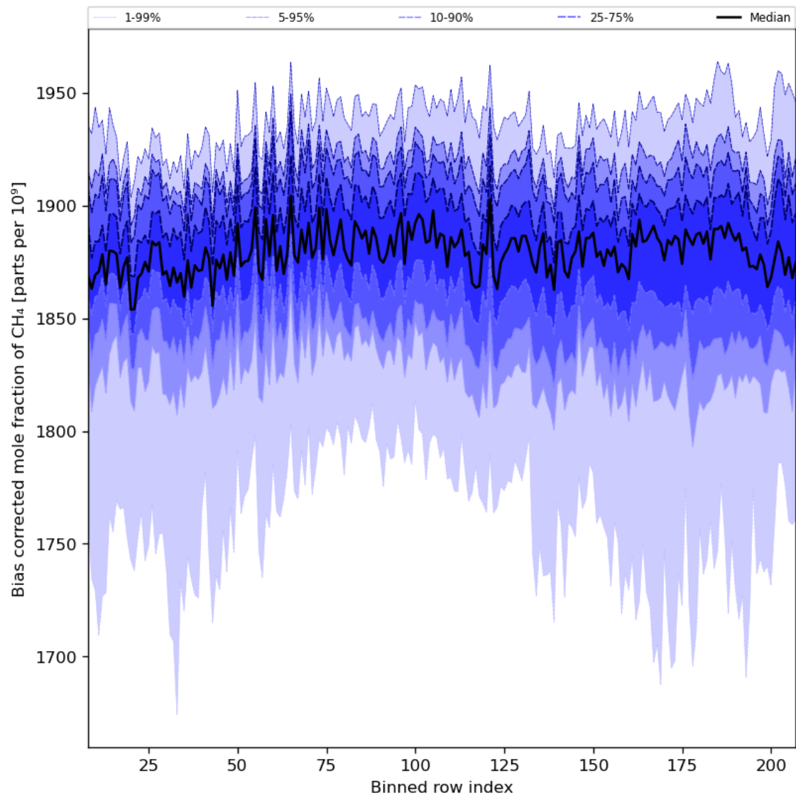
Figure 36: Along track statistics of “Bias corrected mole fraction of CH 4 ” for 2024-06-09 to 2024-06-11
