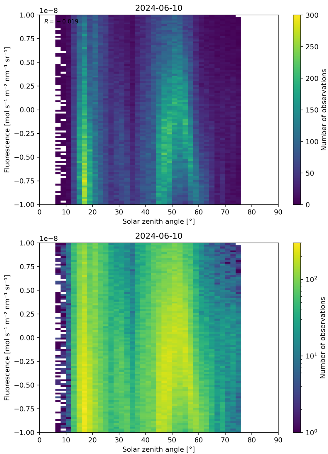
Figure 97: Scatter density plot of “Solar zenith angle” against “Fluorescence” for 2024-06-09 to 2024-06-11.
