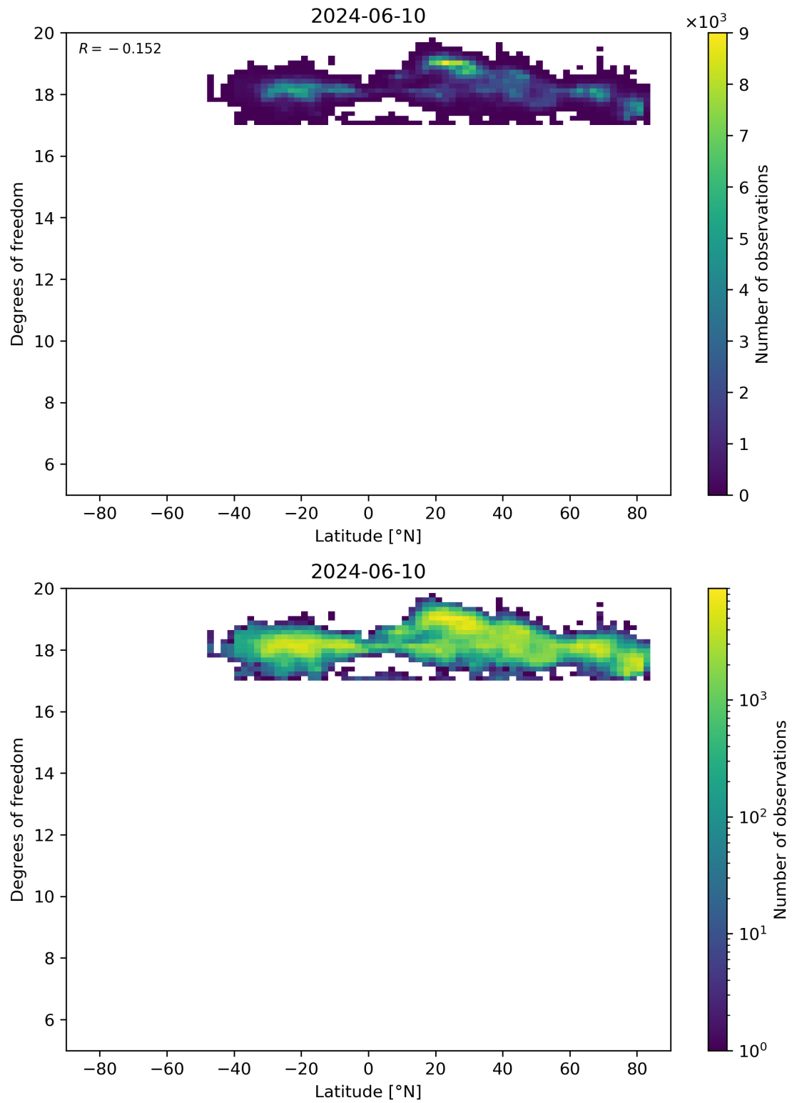
Figure 55: Scatter density plot of “Latitude” against “Degrees of freedom” for 2024-06-09 to 2024-06-11.
