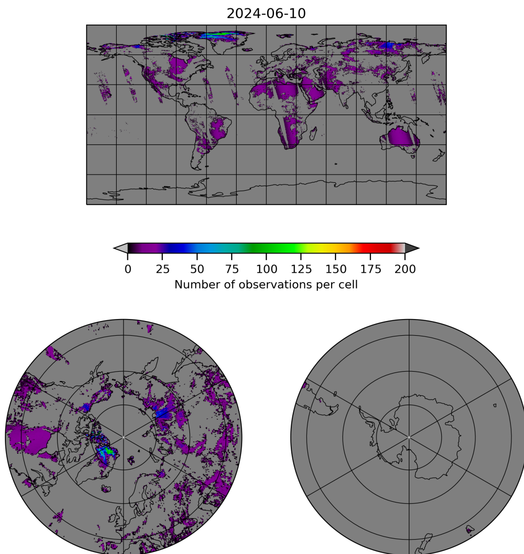
Figure 10: Map of the number of observations for 2024-06-09 to 2024-06-11
