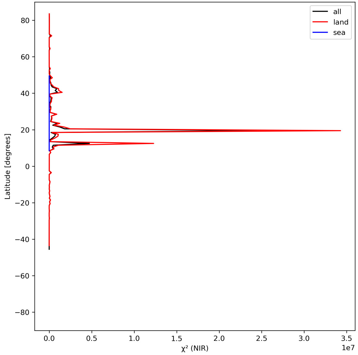
Figure 18: Zonal average of “ \chi^2 (NIR)” for 2024-06-09 to 2024-06-11.
