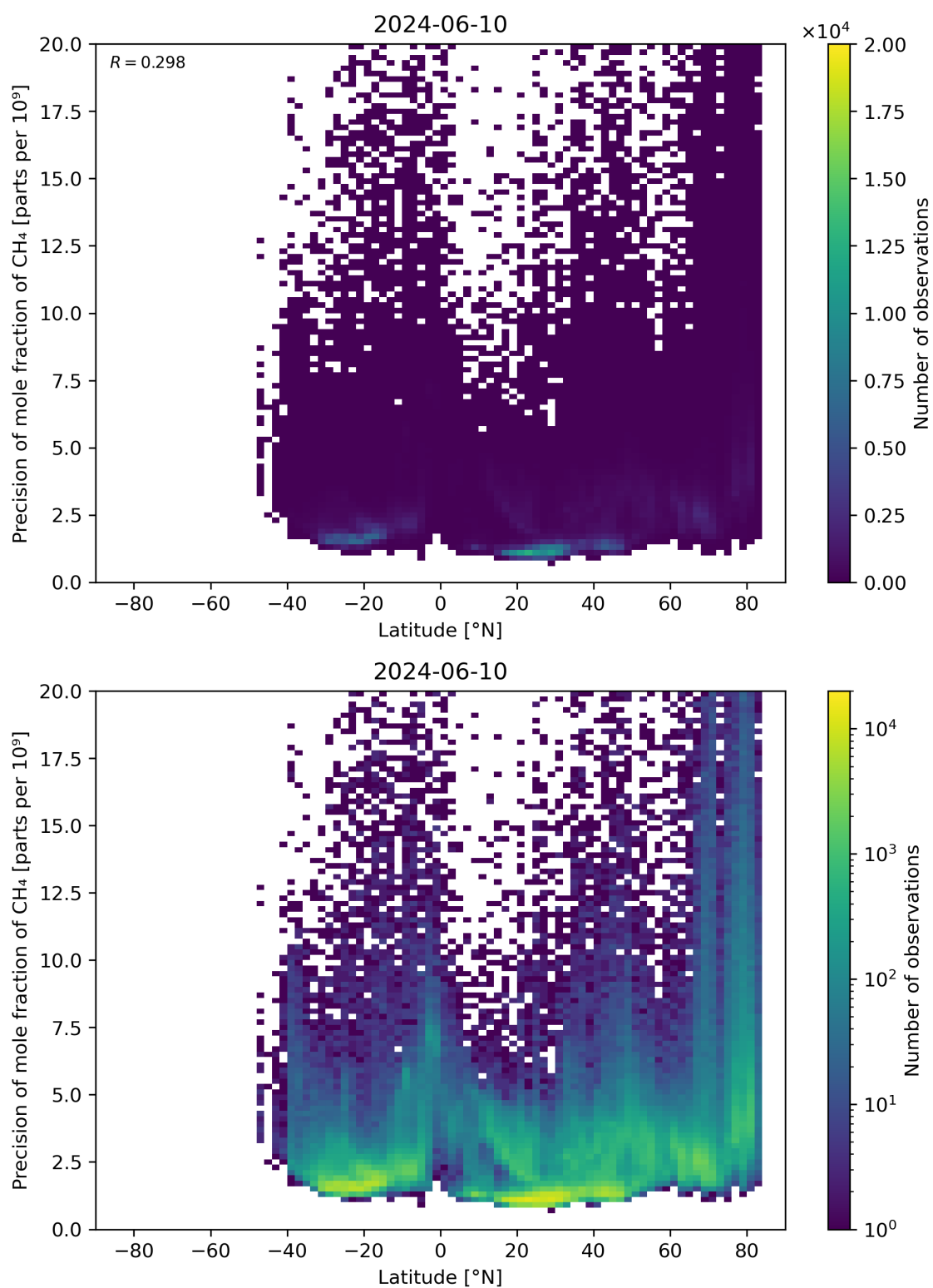
Figure 59: Scatter density plot of “Latitude” against “Precision of mole fraction of \text{CH}_4 ” for 2024-06-09 to 2024-06-11.
