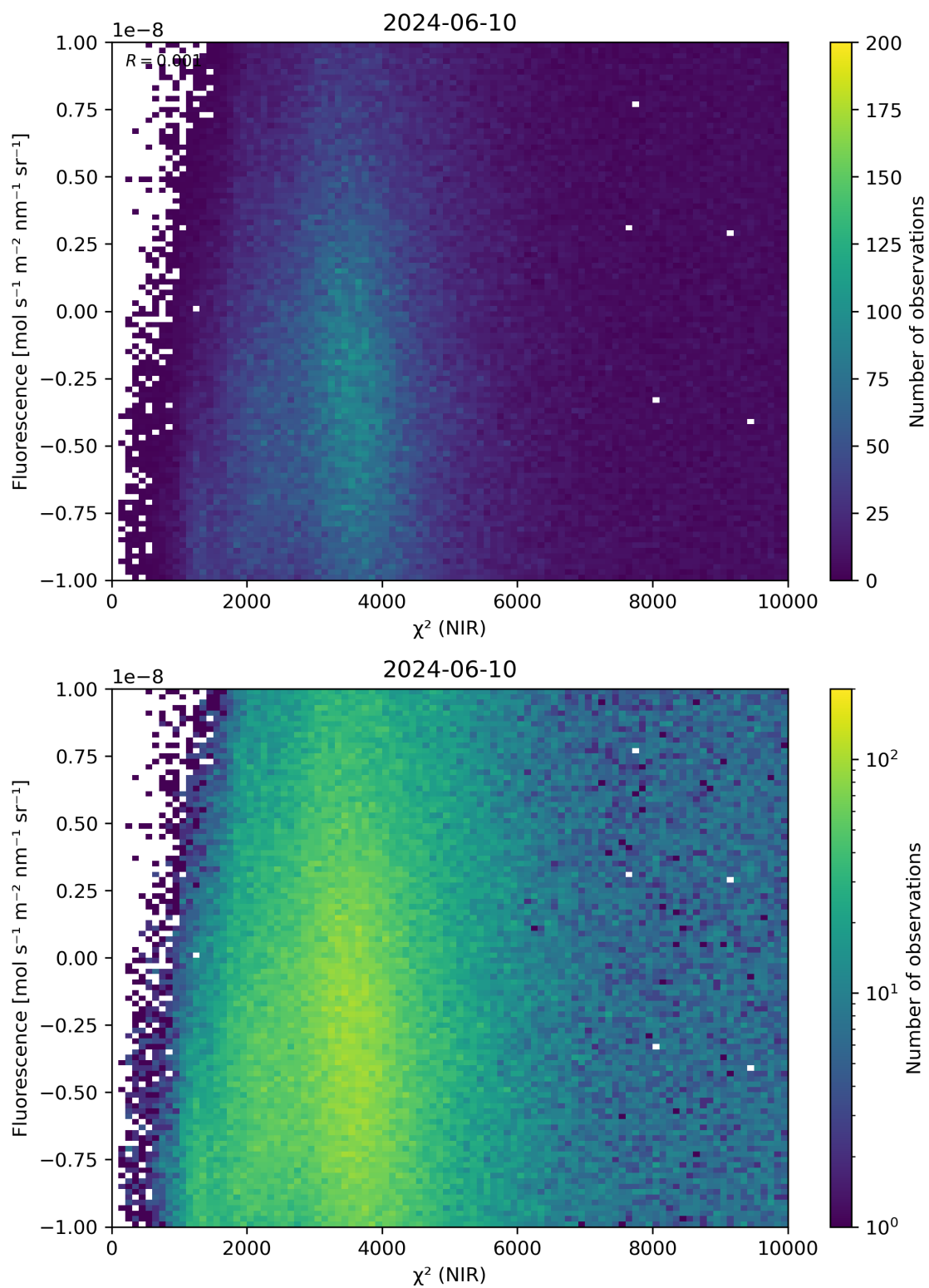
Figure 45: Scatter density plot of “ \chi^2 (NIR)” against “Fluorescence” for 2024-06-09 to 2024-06-11.
