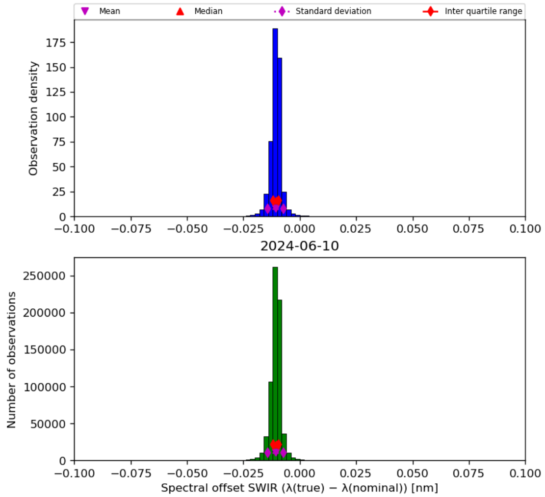
Figure 27: Histogram of “Spectral offset SWIR ( \lambda(\text{true}) - \lambda(\text{nominal}) )” for 2024-06-09 to 2024-06-11
