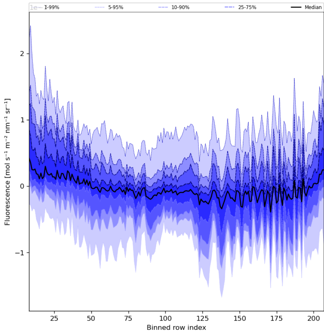
Figure 43: Along track statistics of “Fluorescence” for 2024-06-09 to 2024-06-11
