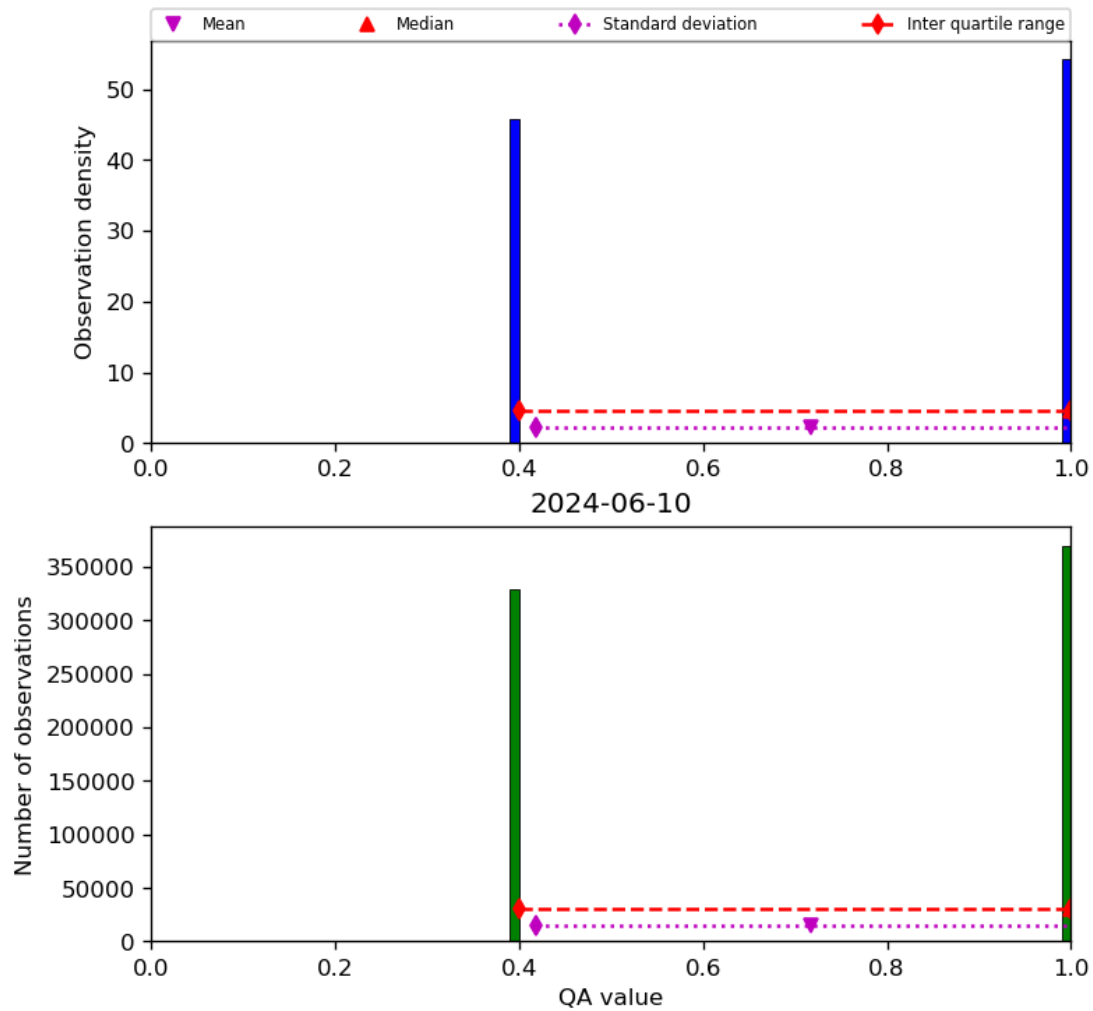
Figure 22: Histogram of “QA value” for 2024-06-09 to 2024-06-11
