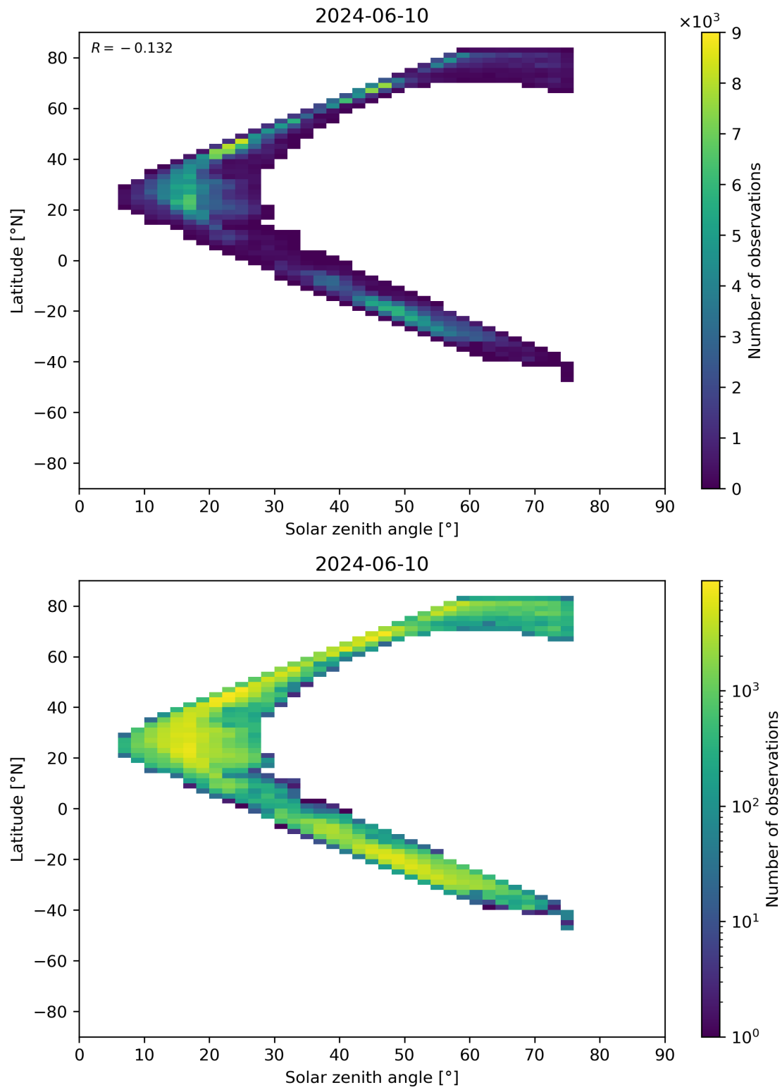
Figure 98: Scatter density plot of “Solar zenith angle” against “Latitude” for 2024-06-09 to 2024-06-11.
