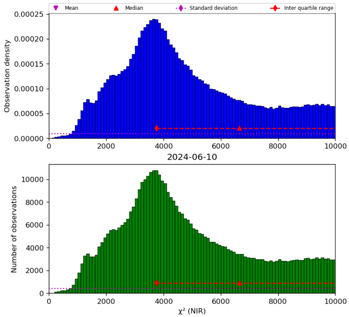
Figure 29: Histogram of “ \chi^2 (NIR)” for 2024-06-09 to 2024-06-11
