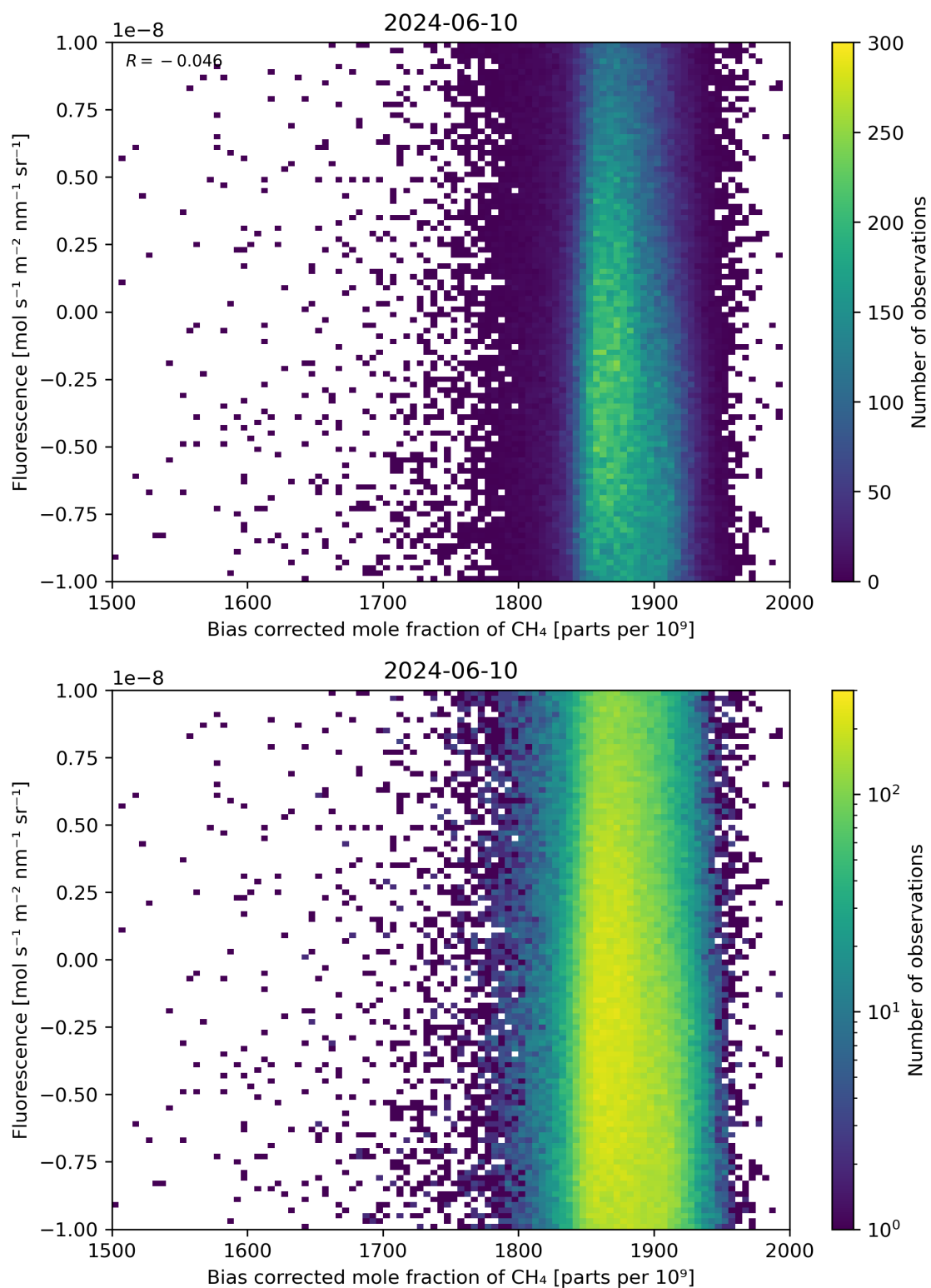
Figure 66: Scatter density plot of “Bias corrected mole fraction of \text{CH}_4 ” against “Fluorescence” for 2024-06-09 to 2024-06-11.
