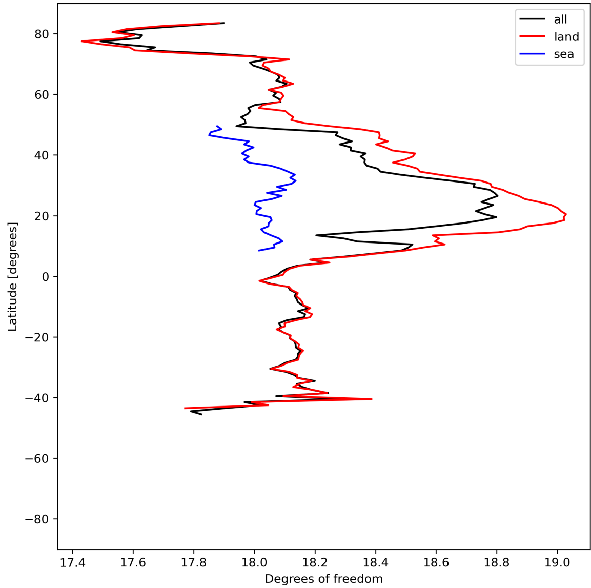
Figure 19: Zonal average of “Degrees of freedom” for 2024-06-09 to 2024-06-11.
