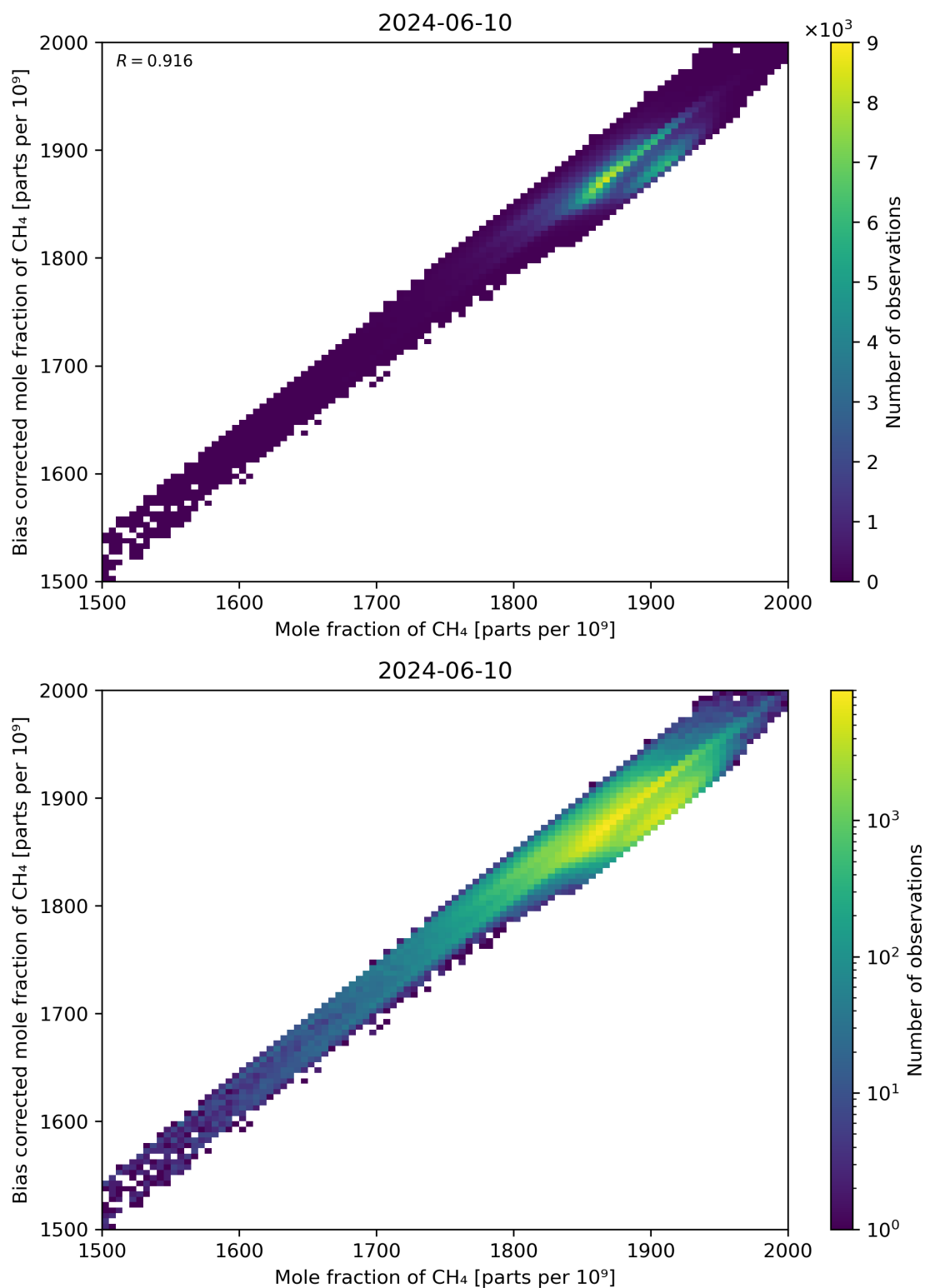
Figure 74: Scatter density plot of “Mole fraction of CH 4 ” against “Bias corrected mole fraction of CH 4 ” for 2024-06-09 to 2024-06-11.
