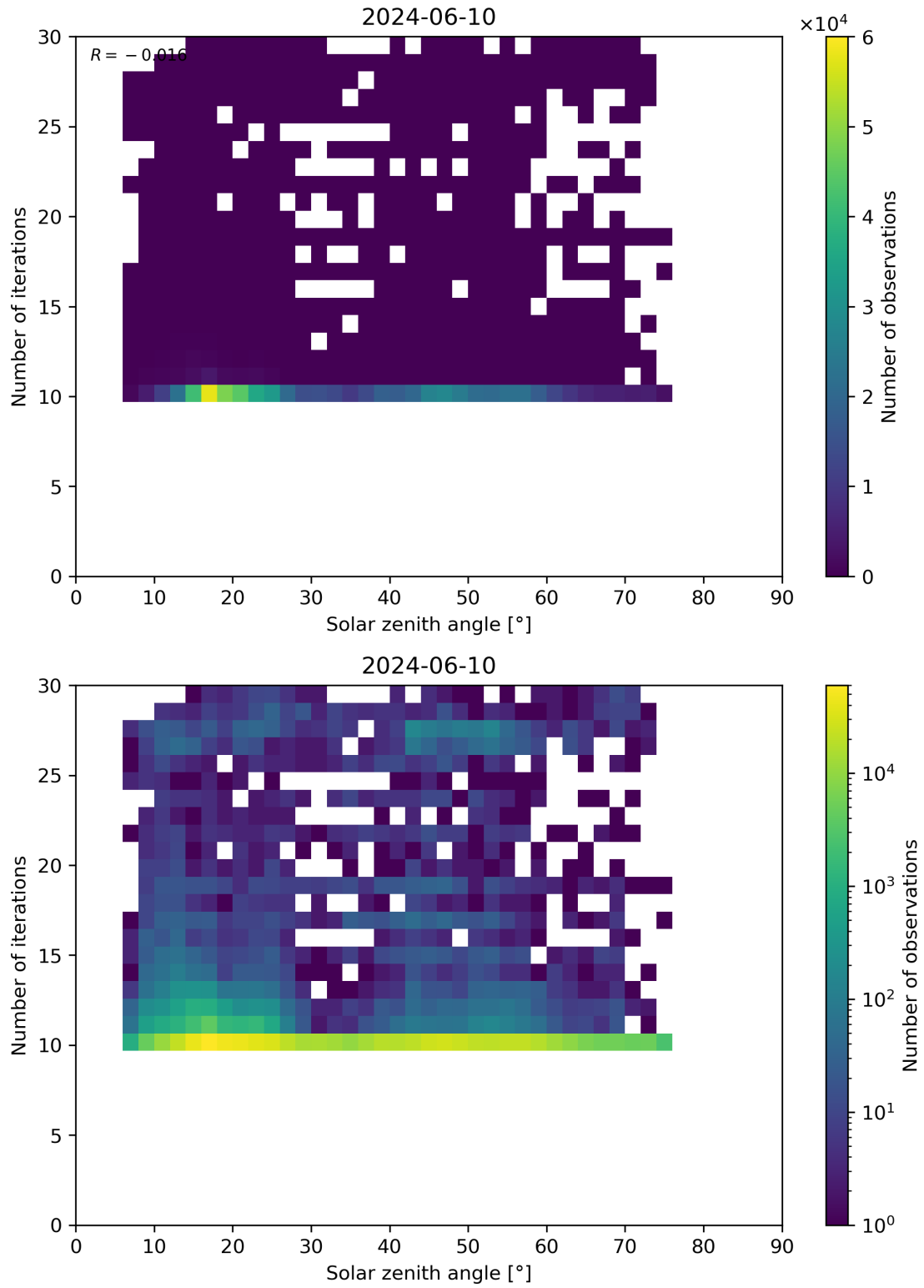
Figure 102: Scatter density plot of “Solar zenith angle” against “Number of iterations” for 2024-06-09 to 2024-06-11.
