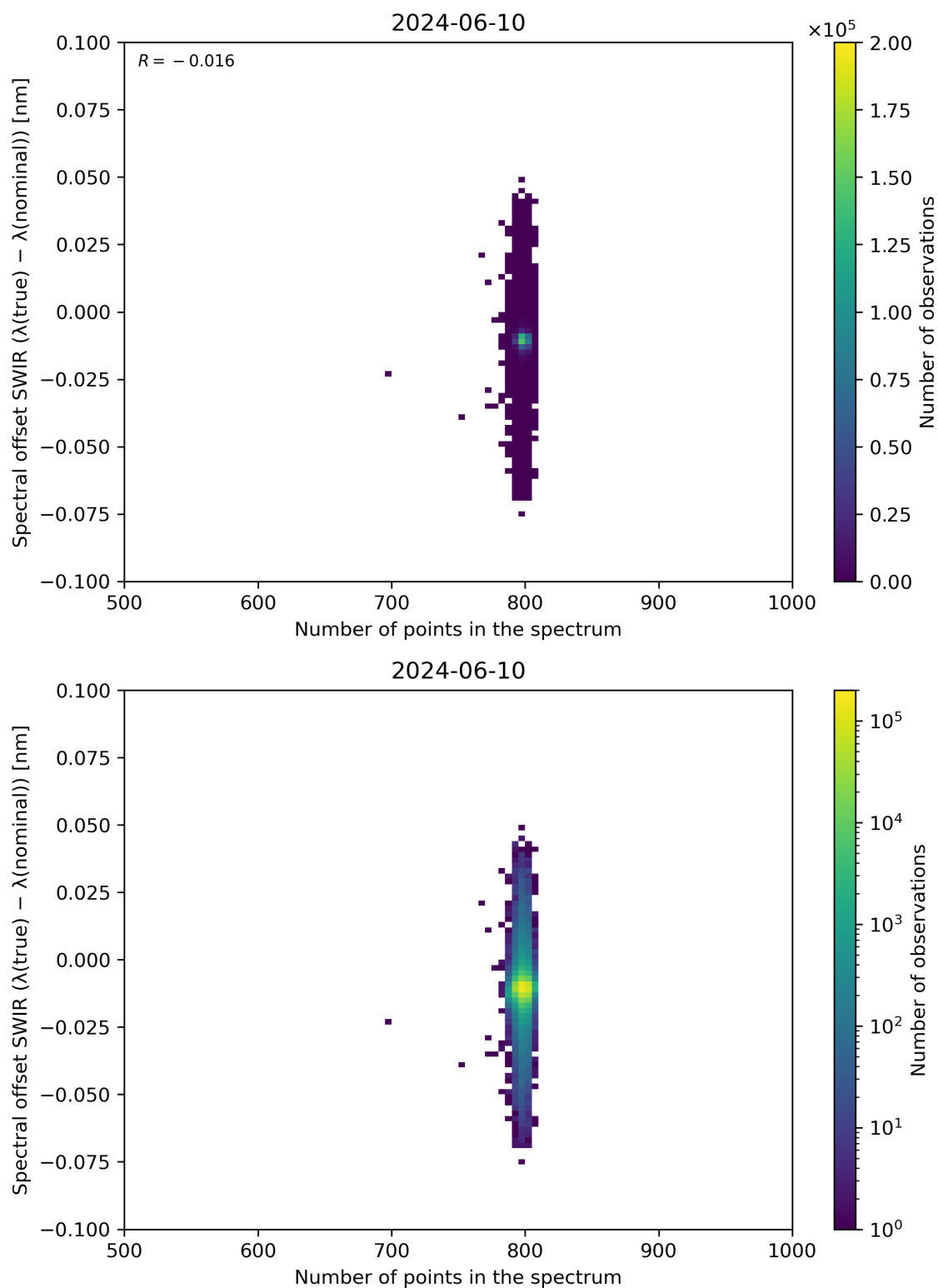
Figure 93: Scatter density plot of “Number of points in the spectrum” against “Spectral offset SWIR ( \lambda(\text{true}) - \lambda(\text{nominal}) )” for 2024-06-09 to 2024-06-11.
