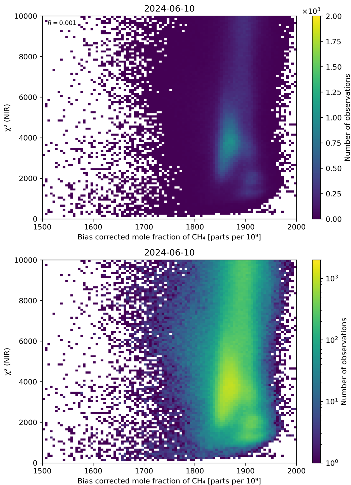
Figure 63: Scatter density plot of “Bias corrected mole fraction of CH 4 ” against “ \chi^2 (NIR)” for 2024-06-09 to 2024-06-11.
