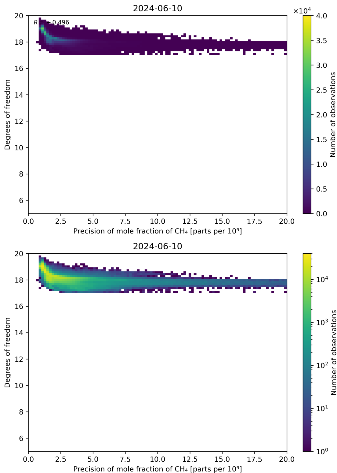
Figure 80: Scatter density plot of “Precision of mole fraction of CH 4 ” against “Degrees of freedom” for 2024-06-09 to 2024-06-11.
