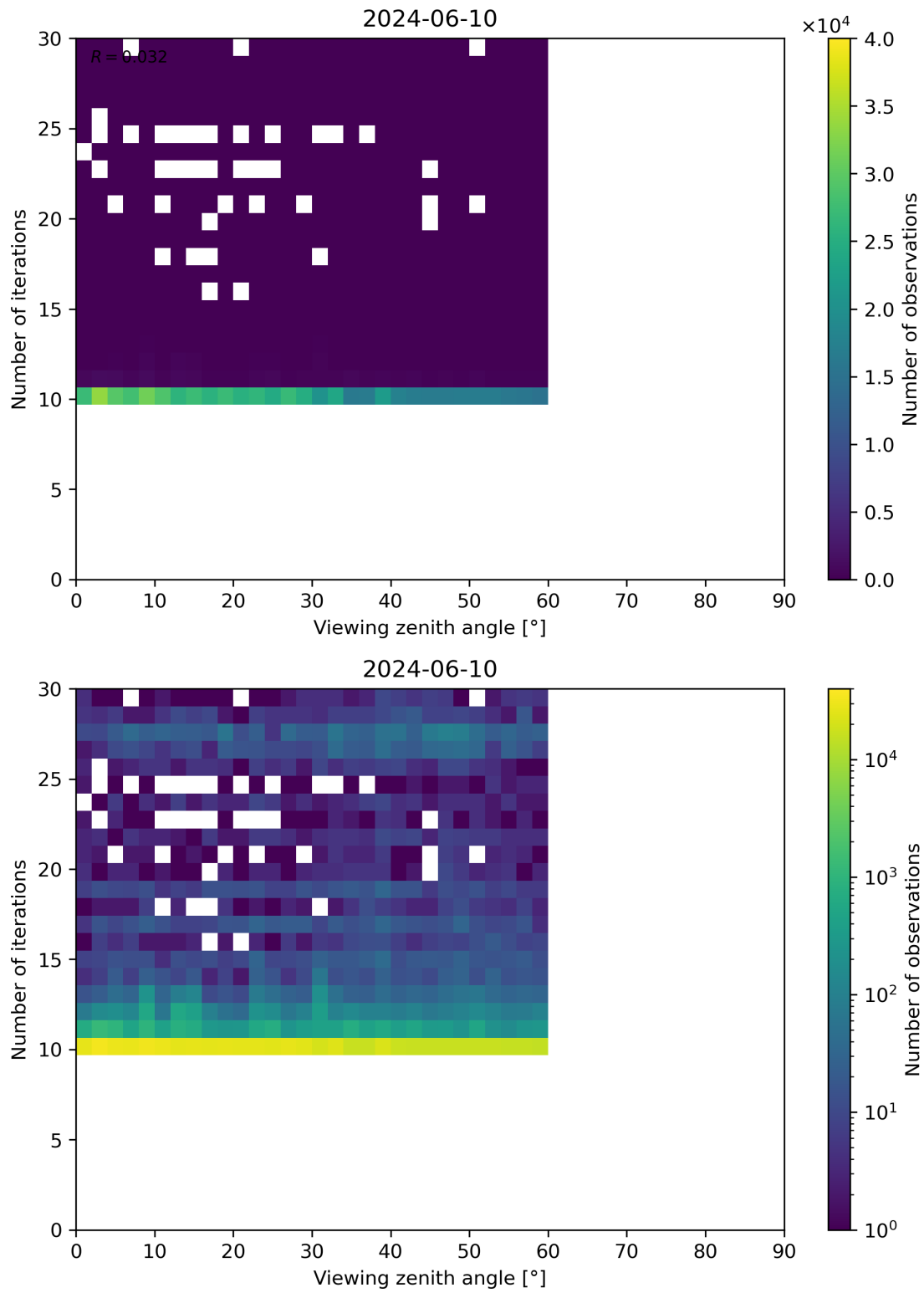
Figure 113: Scatter density plot of “Viewing zenith angle” against “Number of iterations” for 2024-06-09 to 2024-06-11.
