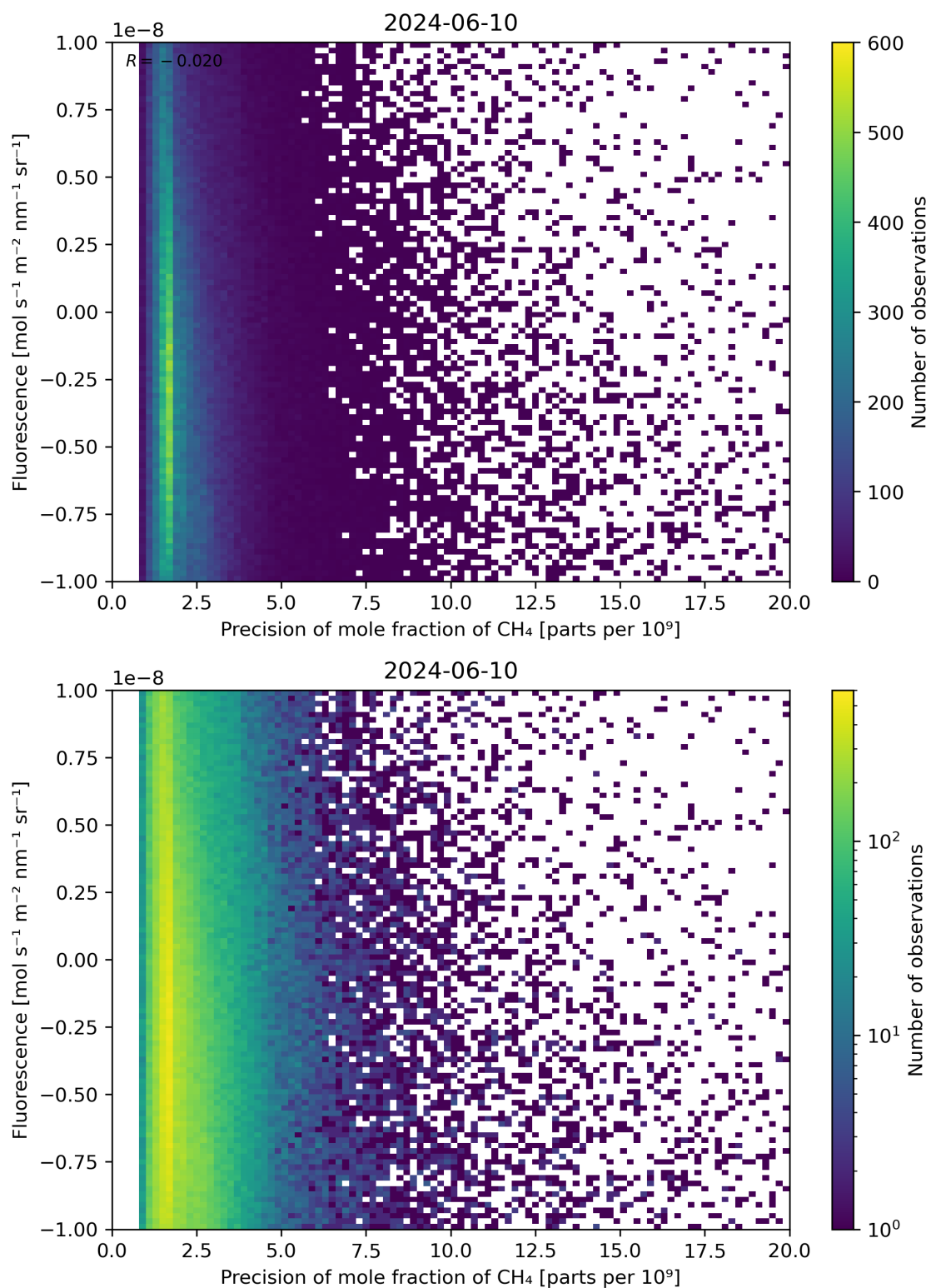
Figure 81: Scatter density plot of “Precision of mole fraction of \text{CH}_4 ” against “Fluorescence” for 2024-06-09 to 2024-06-11.
