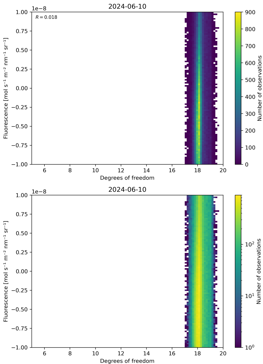
Figure 51: Scatter density plot of “Degrees of freedom” against “Fluorescence” for 2024-06-09 to 2024-06-11.
