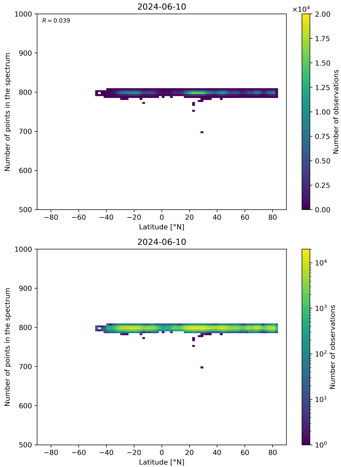
Figure 61: Scatter density plot of “Latitude” against “Number of points in the spectrum” for 2024-06-09 to 2024-06-11.
