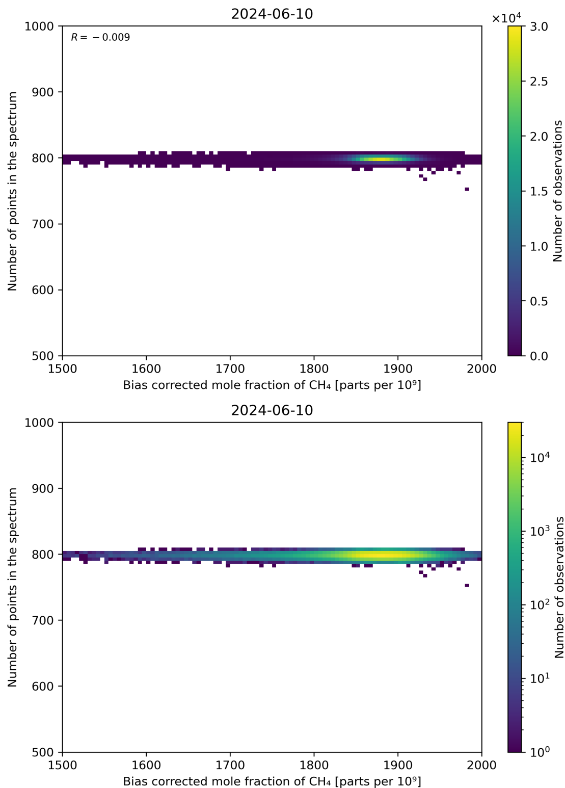
Figure 68: Scatter density plot of “Bias corrected mole fraction of CH 4 ” against “Number of points in the spectrum” for 2024-06-09 to 2024-06-11.
