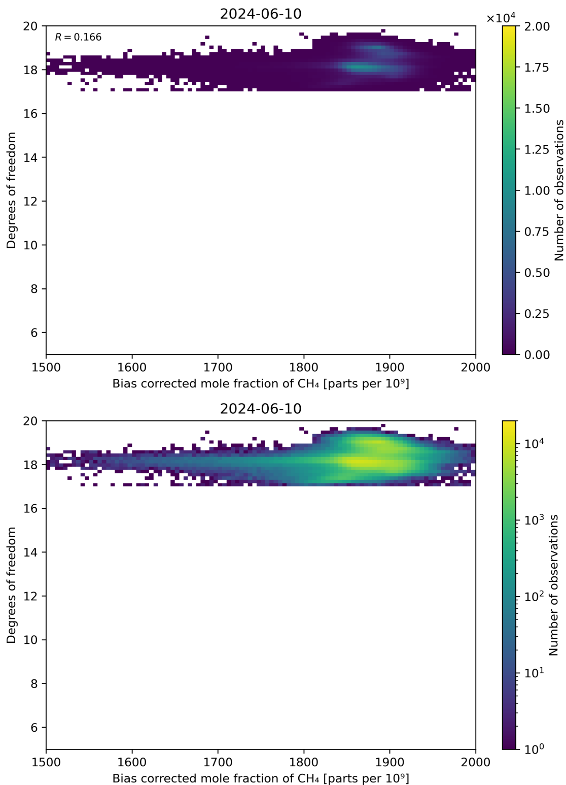
Figure 65: Scatter density plot of “Bias corrected mole fraction of CH 4 ” against “Degrees of freedom” for 2024-06-09 to 2024-06-11.
