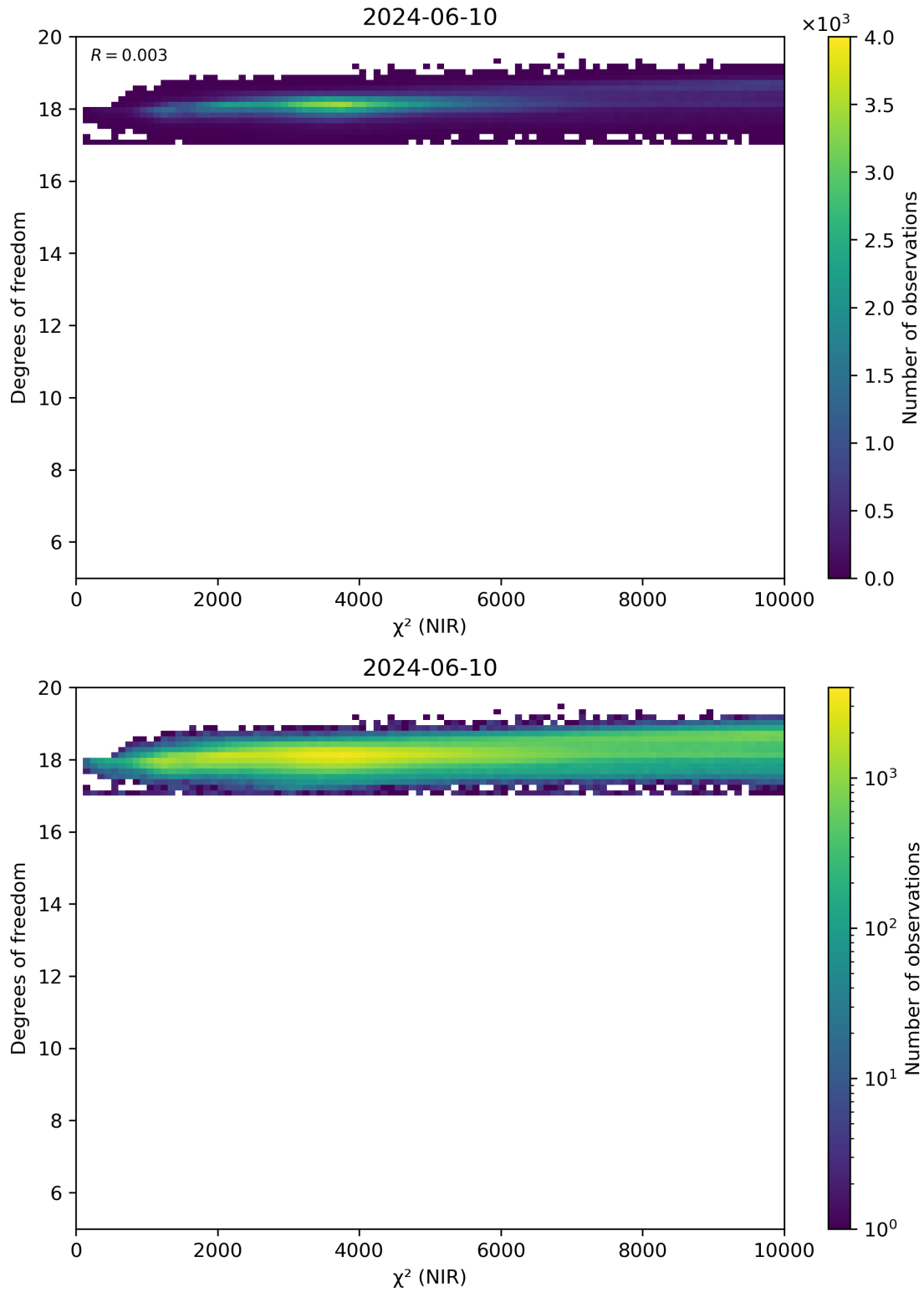
Figure 44: Scatter density plot of “ \chi^2 (NIR)” against “Degrees of freedom” for 2024-06-09 to 2024-06-11.
