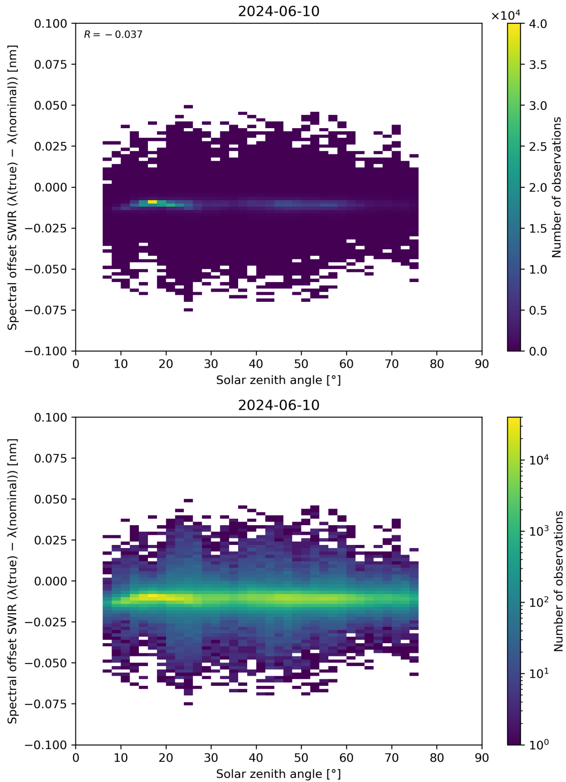
Figure 104: Scatter density plot of “Solar zenith angle” against “Spectral offset SWIR ( \lambda(\text{true}) - \lambda(\text{nominal}) )” for 2024-06-09 to 2024-06-11.
