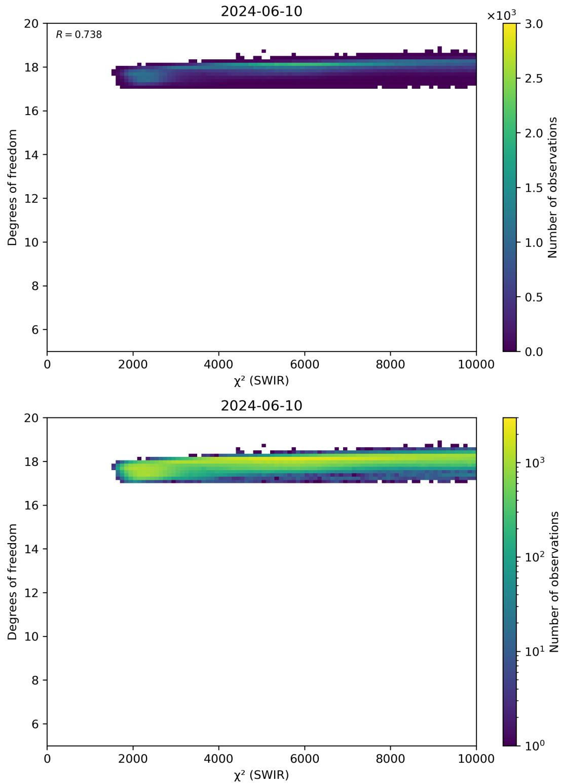
Figure 48: Scatter density plot of “ \chi^2 (SWIR)” against “Degrees of freedom” for 2024-06-09 to 2024-06-11.
