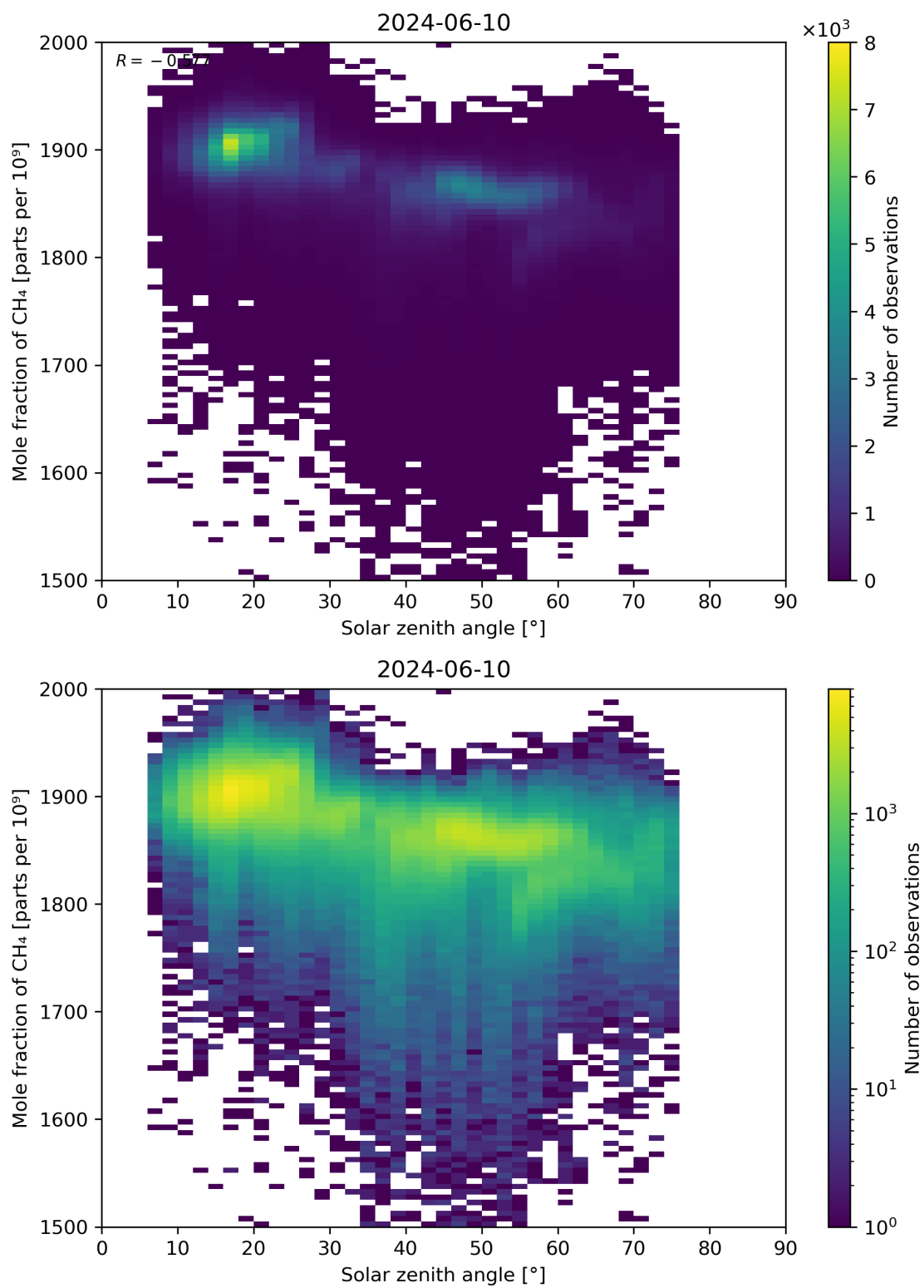
Figure 99: Scatter density plot of “Solar zenith angle” against “Mole fraction of CH 4 ” for 2024-06-09 to 2024-06-11.
