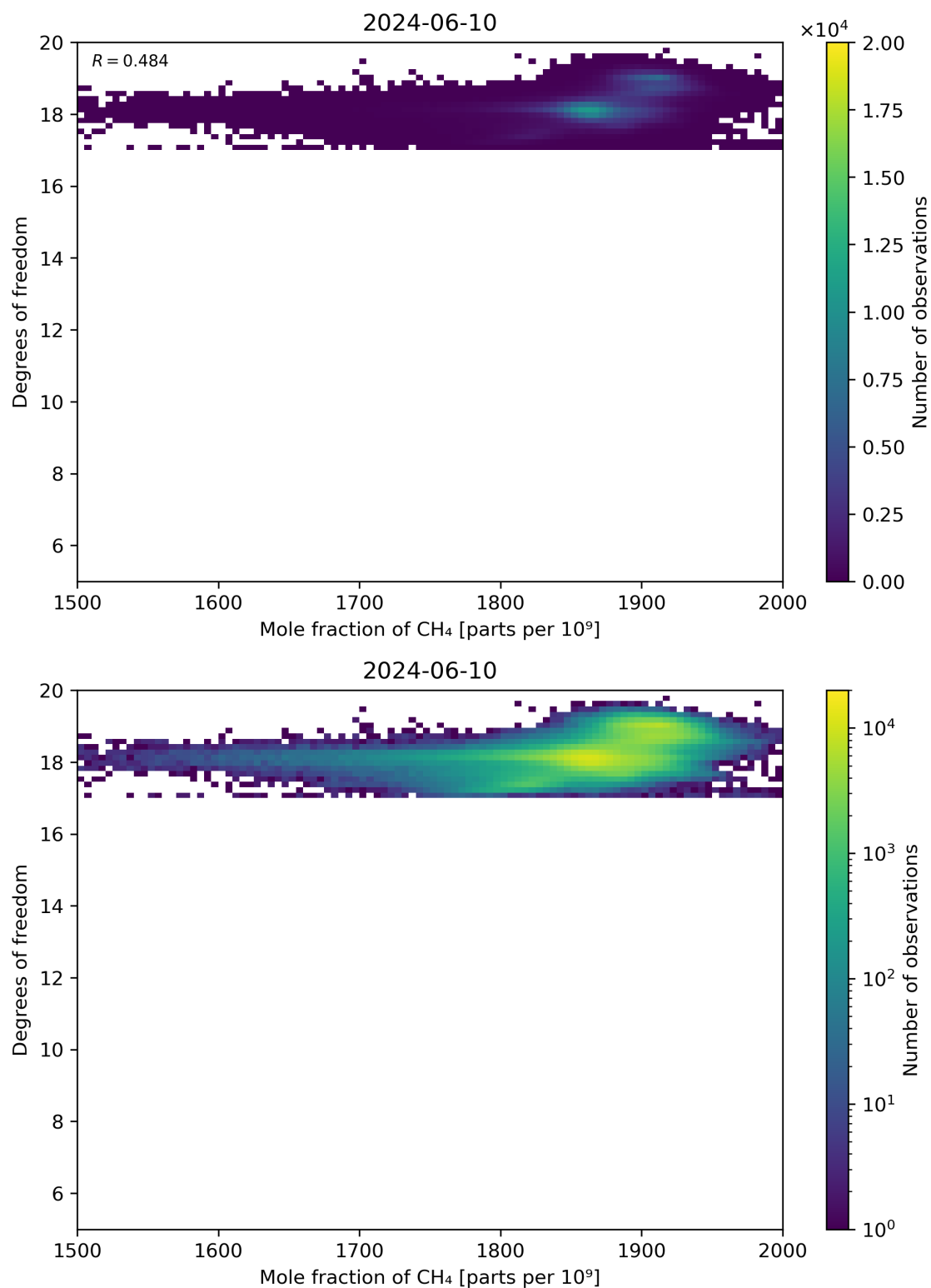
Figure 72: Scatter density plot of “Mole fraction of CH 4 ” against “Degrees of freedom” for 2024-06-09 to 2024-06-11.
