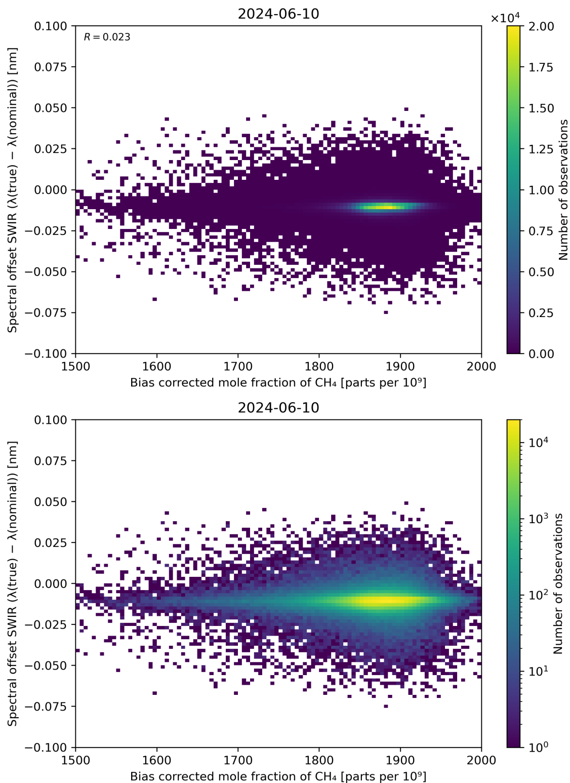
Figure 69: Scatter density plot of “Bias corrected mole fraction of \text{CH}_4 ” against “Spectral offset SWIR ( \lambda(\text{true}) - \lambda(\text{nominal}) )” for 2024-06-09 to 2024-06-11.
