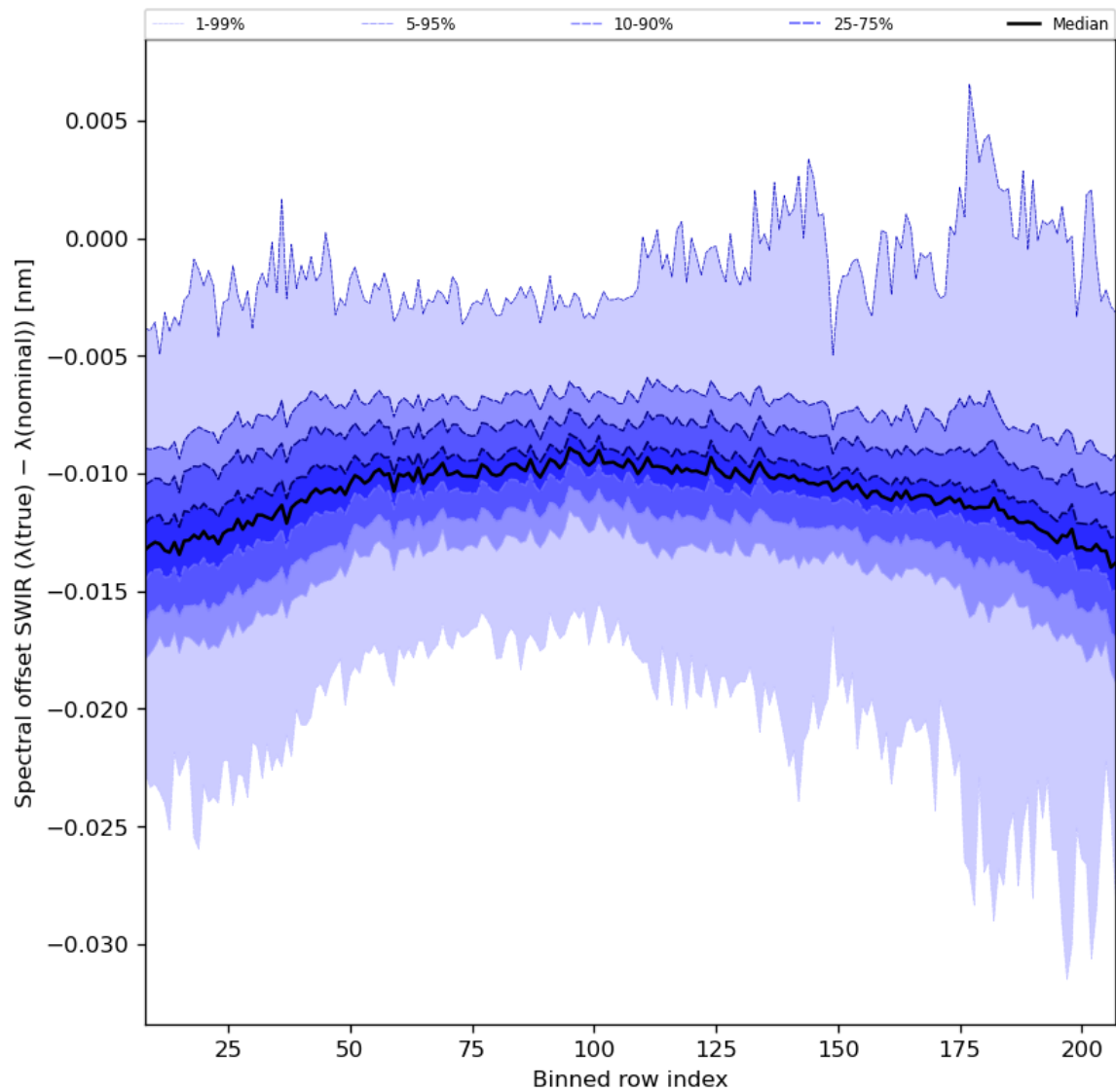
Figure 38: Along track statistics of “Spectral offset SWIR ( \lambda(\text{true}) - \lambda(\text{nominal}) )” for 2024-06-09 to 2024-06-11
