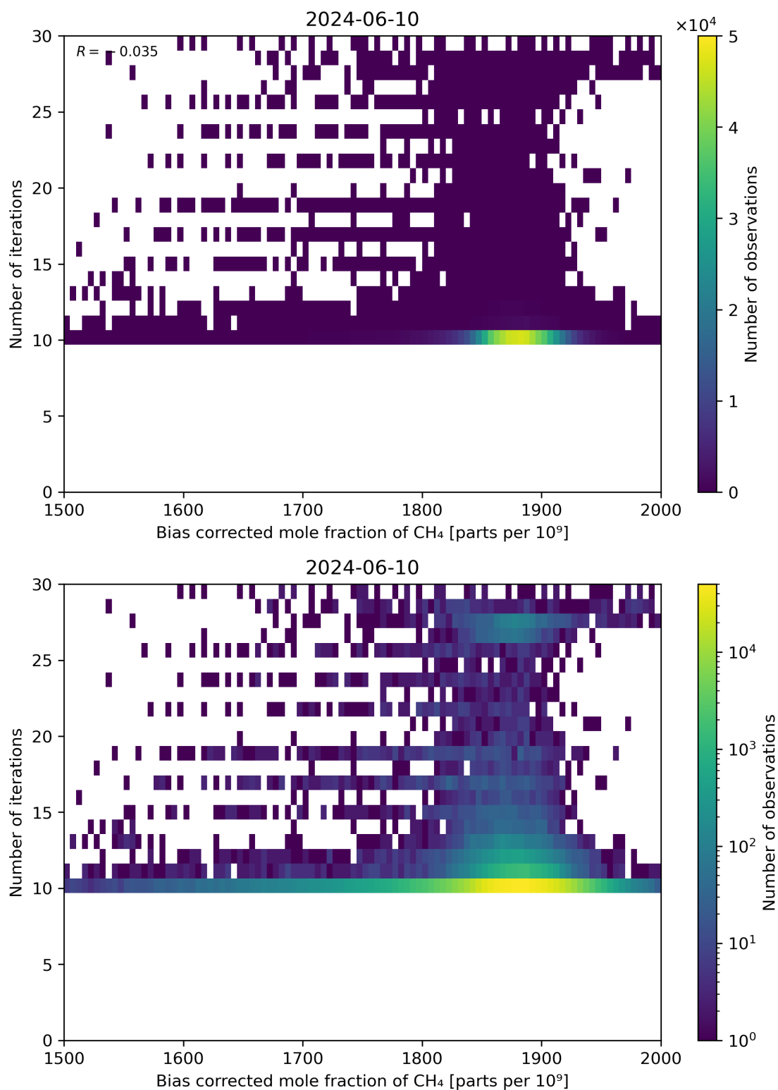
Figure 67: Scatter density plot of “Bias corrected mole fraction of \text{CH}_4 ” against “Number of iterations” for 2024-06-09 to 2024-06-11.
