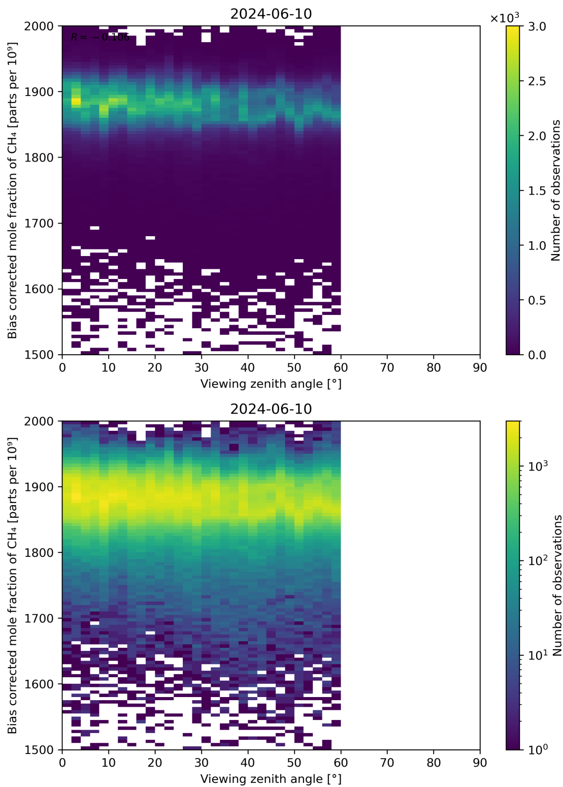
Figure 111: Scatter density plot of “Viewing zenith angle” against “Bias corrected mole fraction of CH 4 ” for 2024-06-09 to 2024-06-11.
