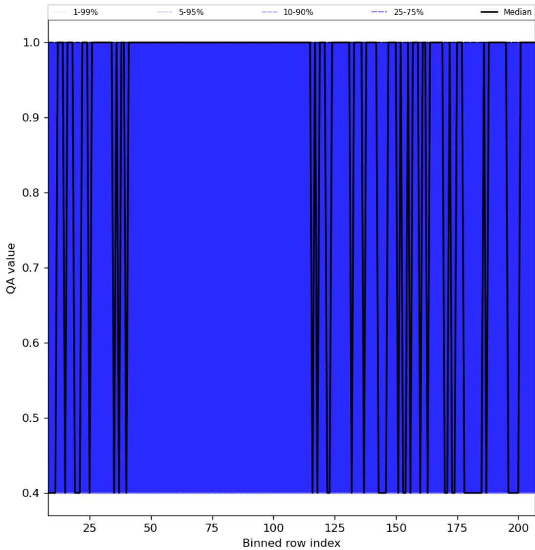
Figure 33: Along track statistics of “QA value” for 2024-06-09 to 2024-06-11
