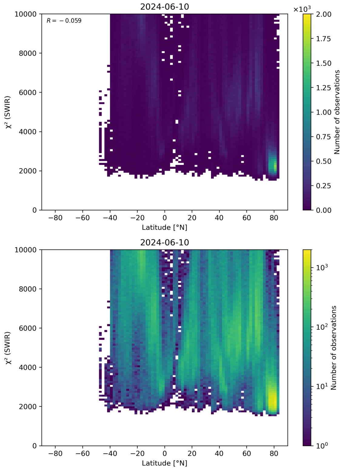
Figure 54: Scatter density plot of “Latitude” against “ \chi^2 (SWIR)” for 2024-06-09 to 2024-06-11.
