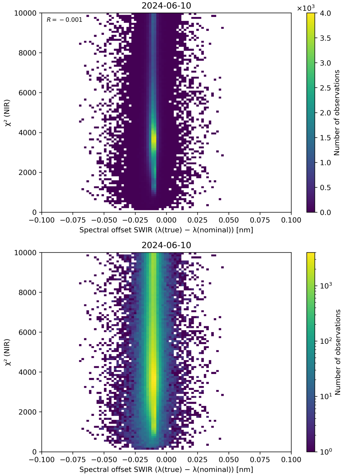
Figure 117: Scatter density plot of “Spectral offset SWIR ( \lambda(\text{true}) - \lambda(\text{nominal}) )” against “ \chi^2 (NIR)” for 2024-06-09 to 2024-06-11.
