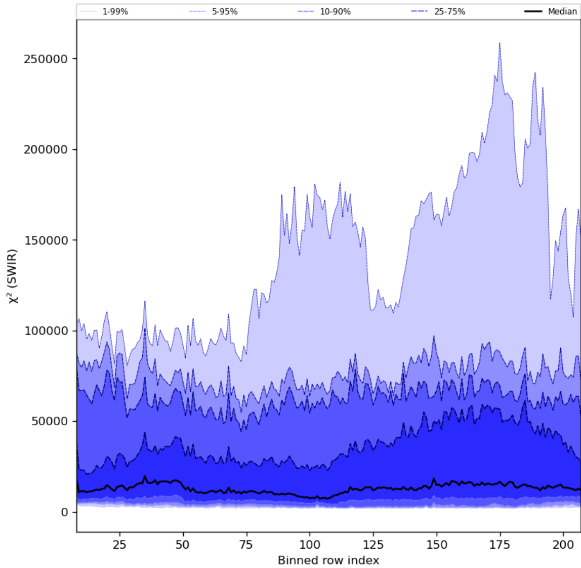
Figure 39: Along track statistics of “ \chi^2 (SWIR)” for 2024-06-09 to 2024-06-11
