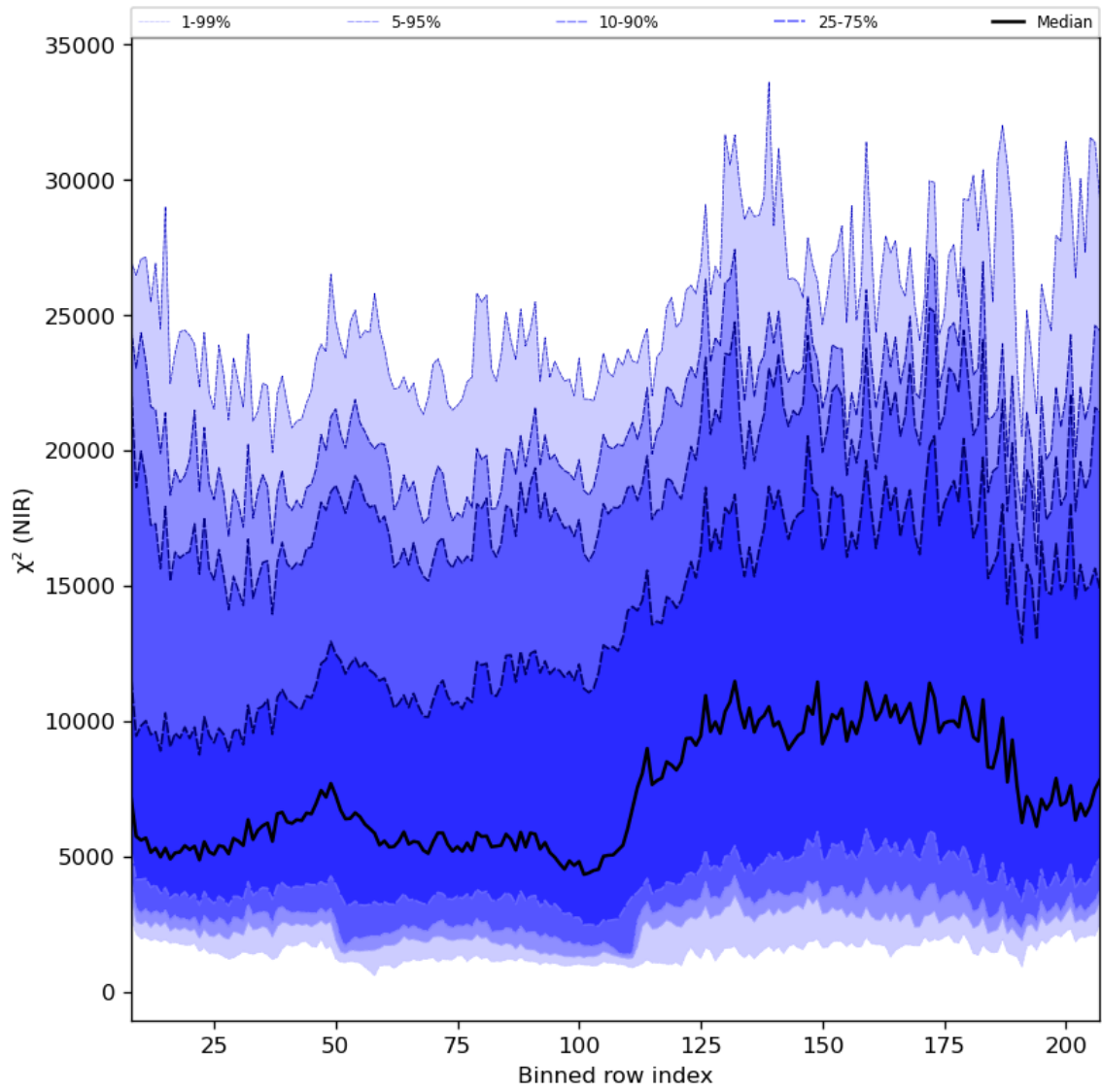
Figure 40: Along track statistics of “ \chi^2 (NIR)” for 2024-06-09 to 2024-06-11
