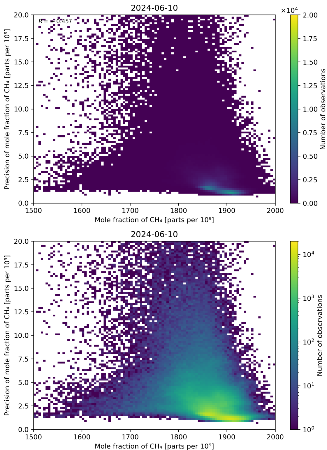
Figure 75: Scatter density plot of “Mole fraction of CH 4 ” against “Precision of mole fraction of CH 4 ” for 2024-06-09 to 2024-06-11.
