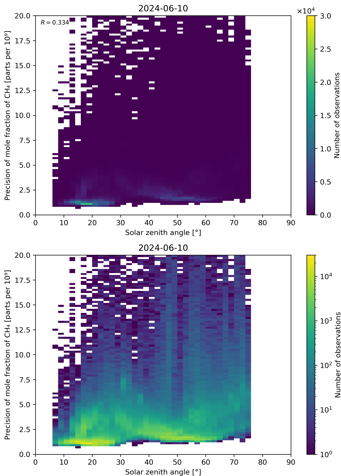
Figure 101: Scatter density plot of “Solar zenith angle” against “Precision of mole fraction of CH 4 ” for 2024-06-09 to 2024-06-11.
