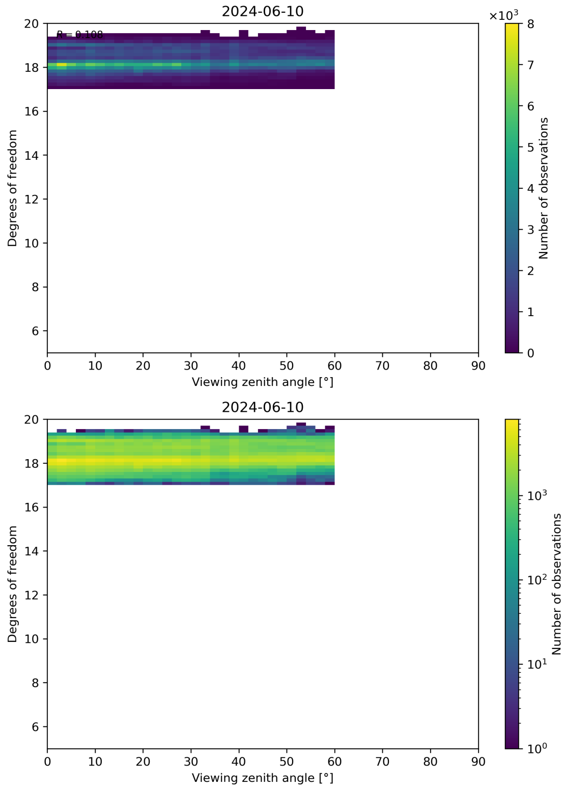
Figure 107: Scatter density plot of “Viewing zenith angle” against “Degrees of freedom” for 2024-06-09 to 2024-06-11.
