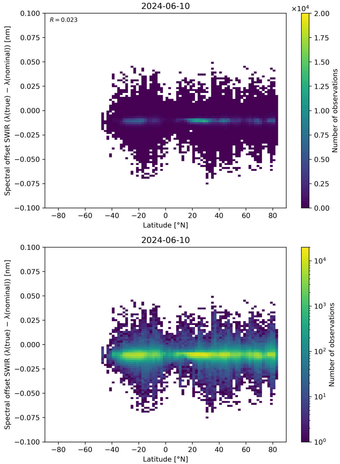
Figure 62: Scatter density plot of “Latitude” against “Spectral offset SWIR ( \lambda(\text{true}) - \lambda(\text{nominal}) )” for 2024-06-09 to 2024-06-11.
