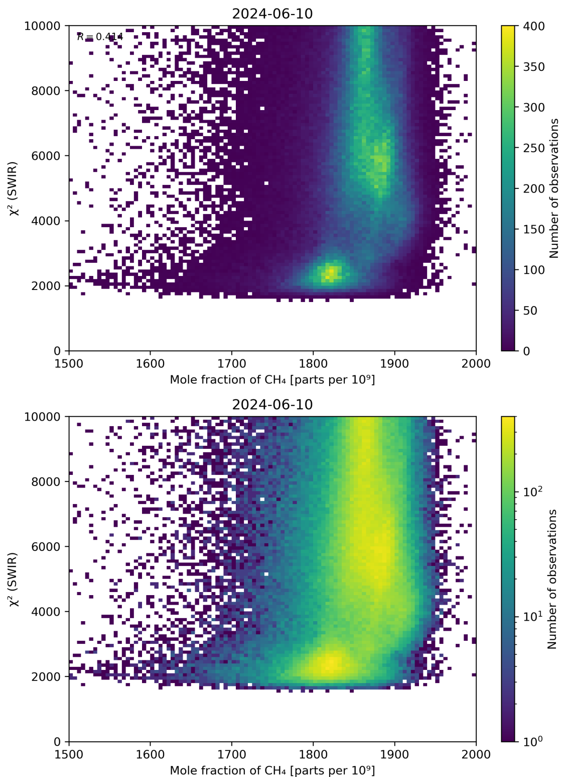
Figure 71: Scatter density plot of “Mole fraction of \text{CH}_4 ” against “ \chi^2 (SWIR)” for 2024-06-09 to 2024-06-11.
