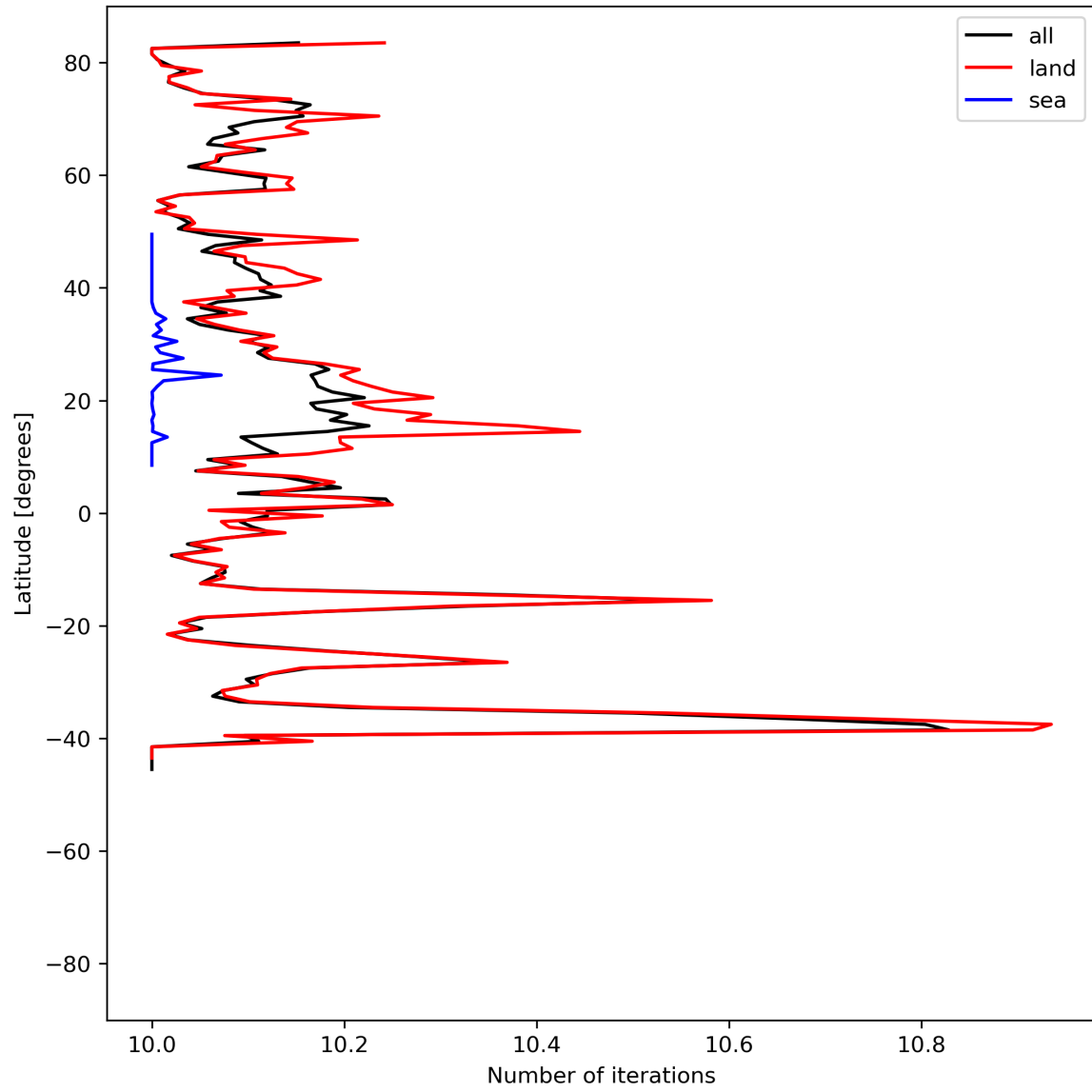
Figure 20: Zonal average of “Number of iterations” for 2024-06-09 to 2024-06-11.
