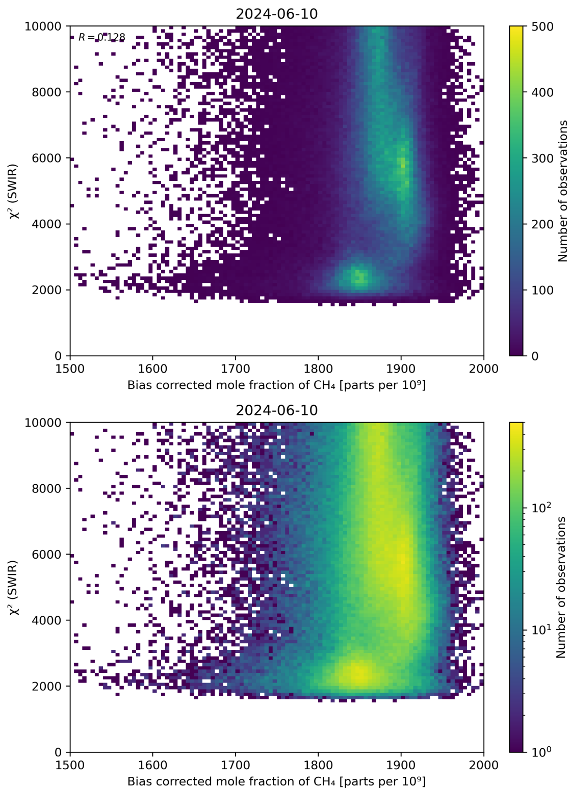
Figure 64: Scatter density plot of “Bias corrected mole fraction of CH 4 ” against “ \chi^2 (SWIR)” for 2024-06-09 to 2024-06-11.
