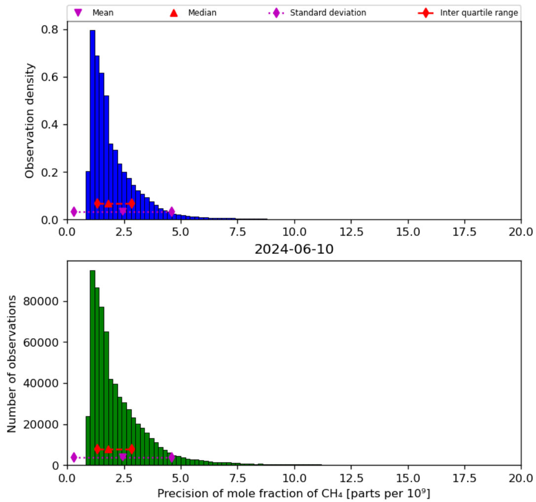
Figure 24: Histogram of “Precision of mole fraction of CH 4 ” for 2024-06-09 to 2024-06-11
