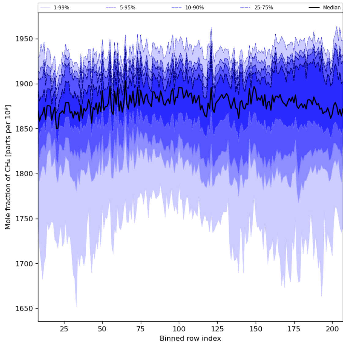
Figure 34: Along track statistics of “Mole fraction of CH 4 ” for 2024-06-09 to 2024-06-11
