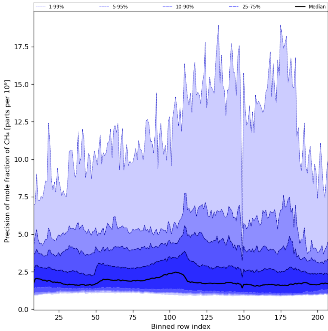
Figure 35: Along track statistics of “Precision of mole fraction of CH 4 ” for 2024-06-09 to 2024-06-11
