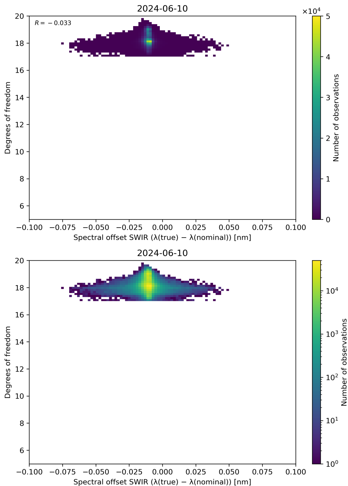
Figure 119: Scatter density plot of “Spectral offset SWIR ( \lambda(\text{true}) - \lambda(\text{nominal}) )” against “Degrees of freedom” for 2024-06-09 to 2024-06-11.
