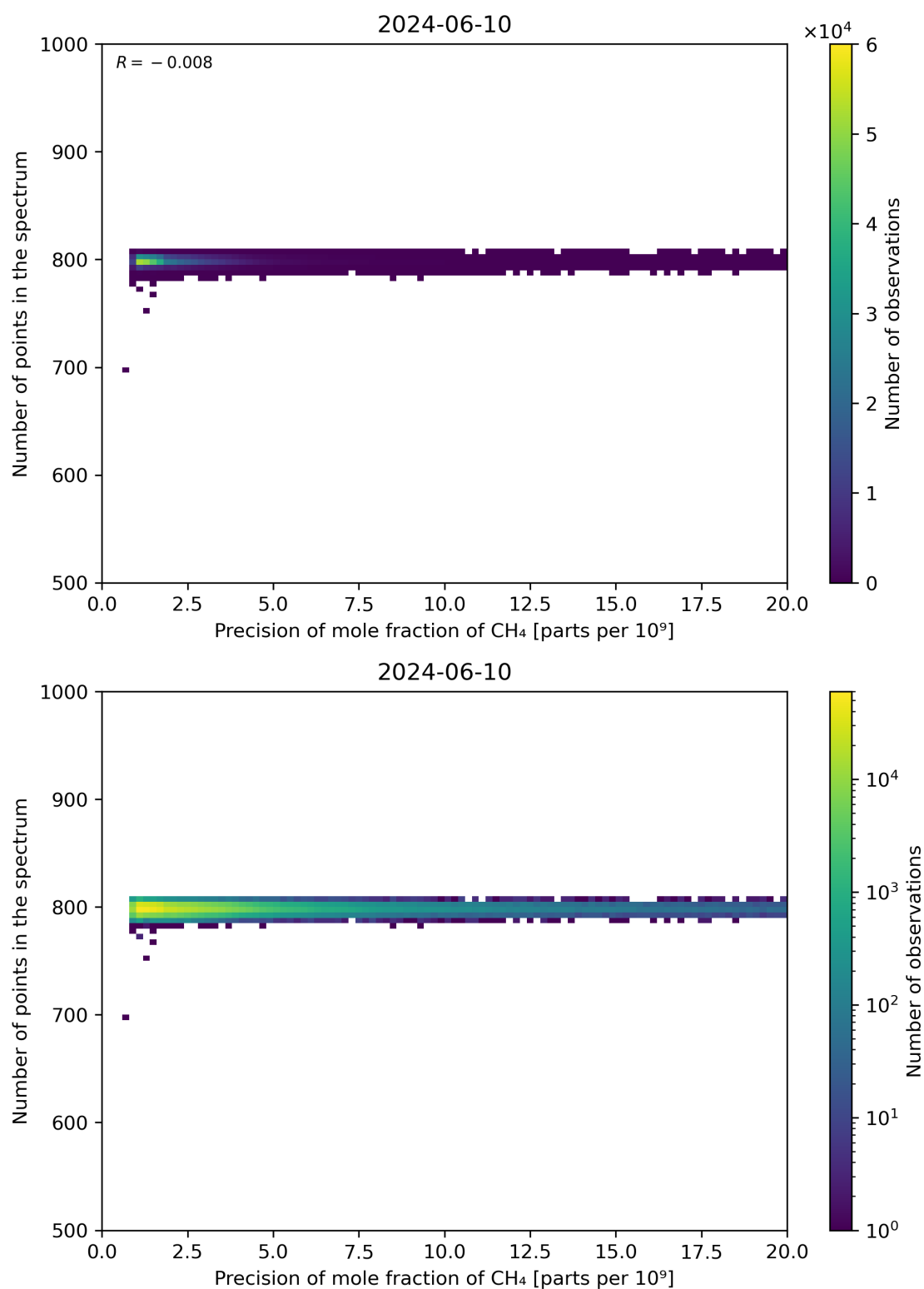
Figure 84: Scatter density plot of “Precision of mole fraction of CH 4 ” against “Number of points in the spectrum” for 2024-06-09 to 2024-06-11.
