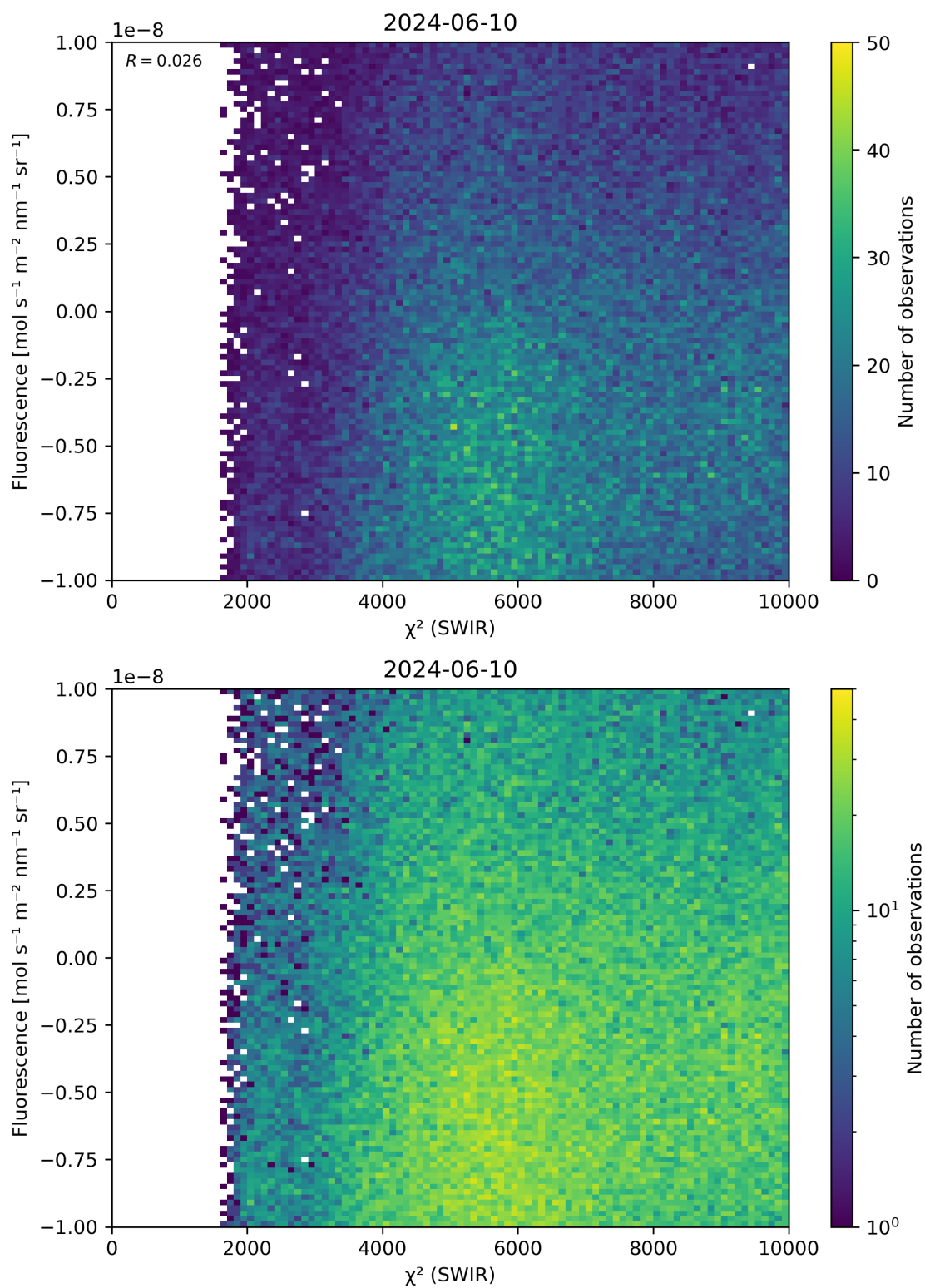
Figure 49: Scatter density plot of “ \chi^2 (SWIR)” against “Fluorescence” for 2024-06-09 to 2024-06-11.
