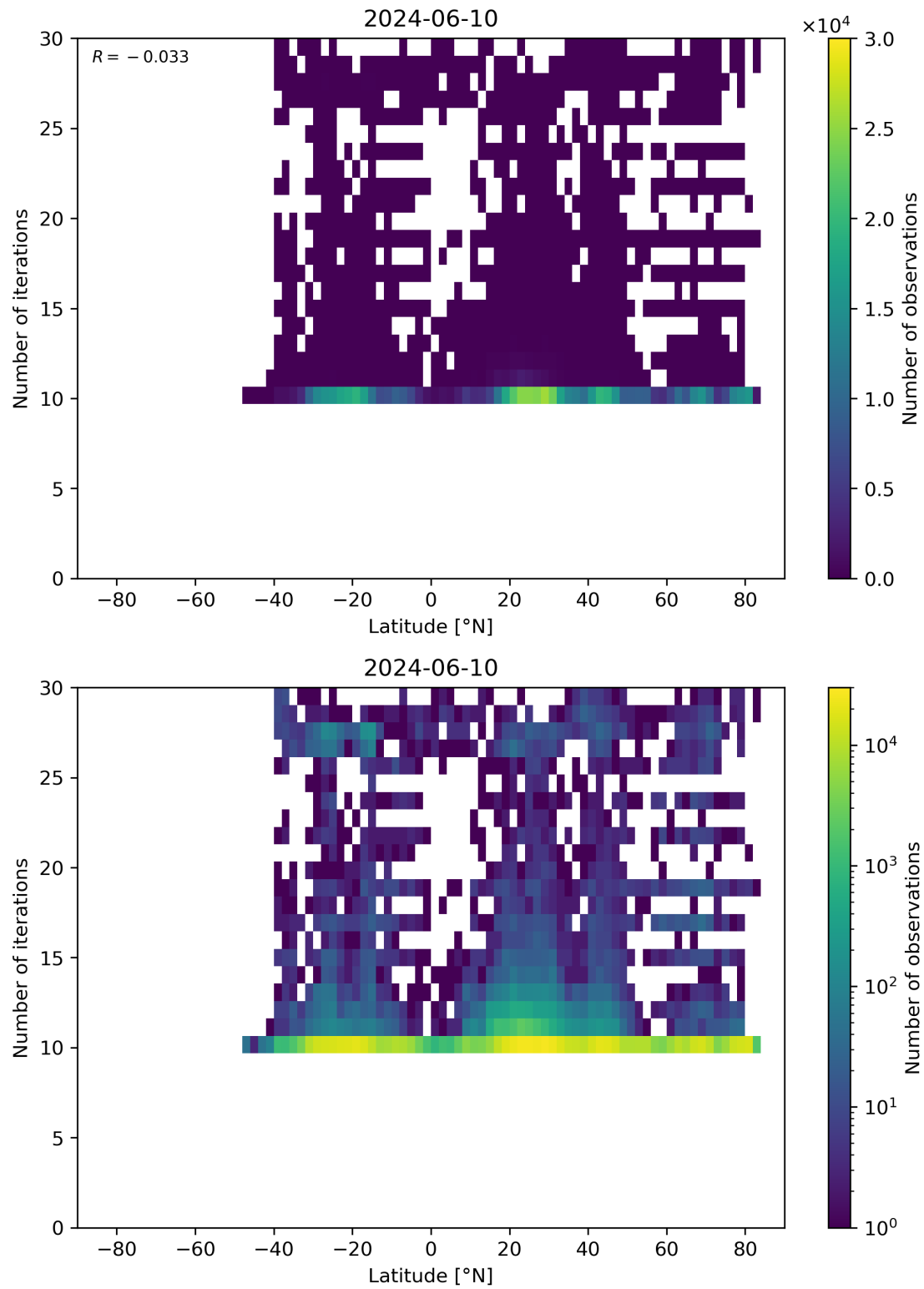
Figure 60: Scatter density plot of “Latitude” against “Number of iterations” for 2024-06-09 to 2024-06-11.
