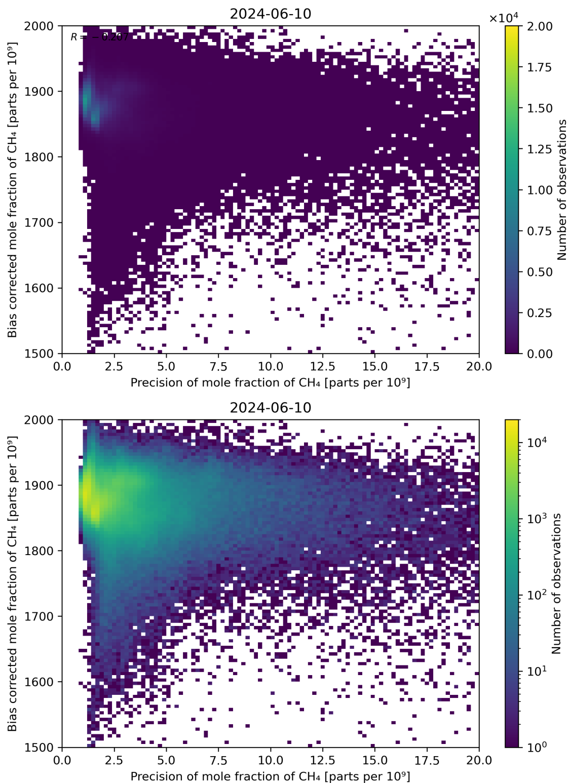
Figure 82: Scatter density plot of “Precision of mole fraction of CH 4 ” against “Bias corrected mole fraction of CH 4 ” for 2024-06-09 to 2024-06-11.
