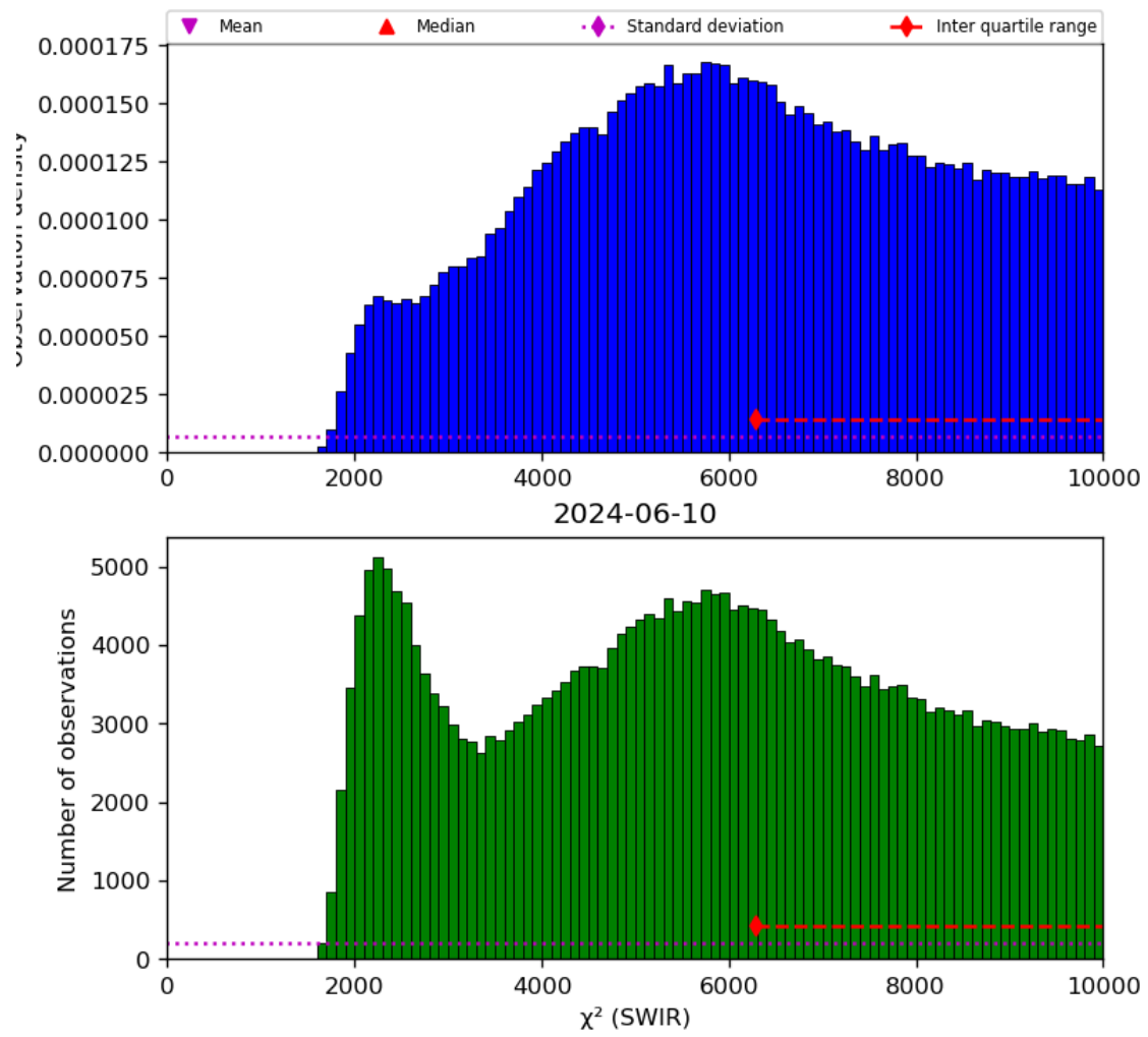
Figure 28: Histogram of “ \chi^2 (SWIR)” for 2024-06-09 to 2024-06-11
