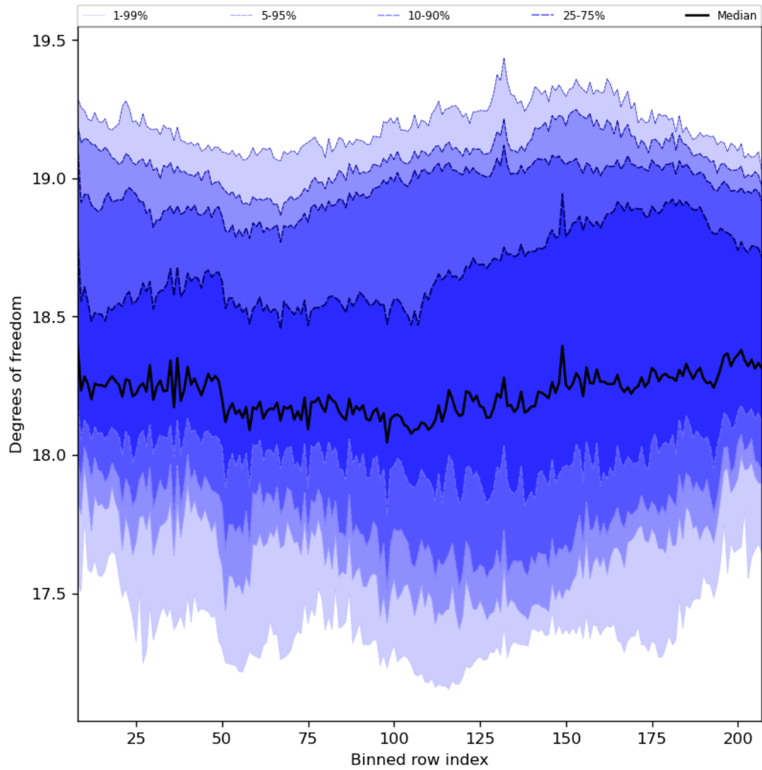
Figure 41: Along track statistics of “Degrees of freedom” for 2024-06-09 to 2024-06-11
