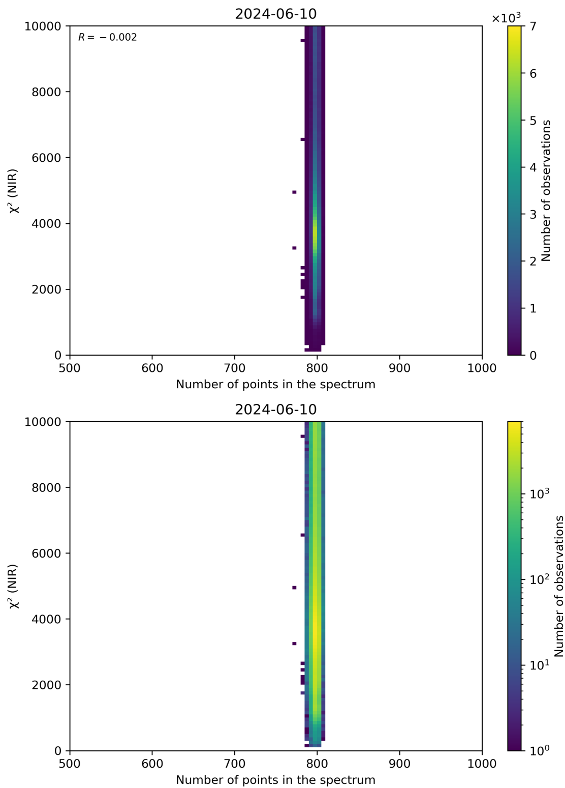
Figure 88: Scatter density plot of “Number of points in the spectrum” against “ \chi^2 (NIR)” for 2024-06-09 to 2024-06-11.
