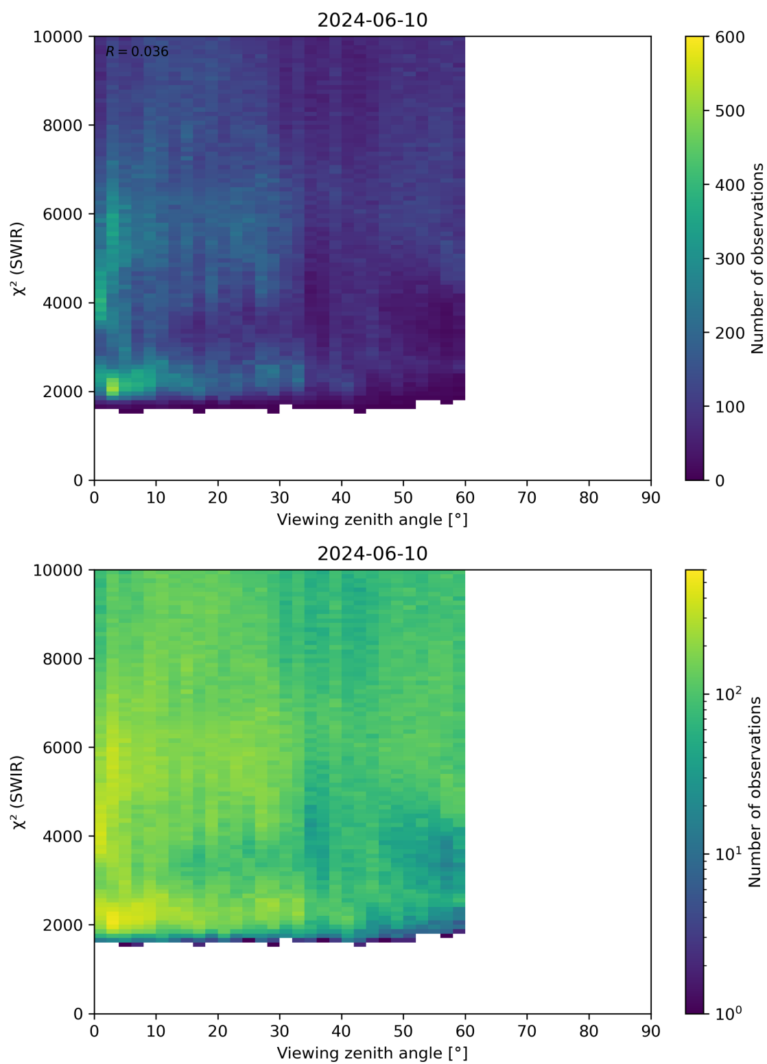
Figure 106: Scatter density plot of “Viewing zenith angle” against “ \chi^2 (SWIR)” for 2024-06-09 to 2024-06-11.
