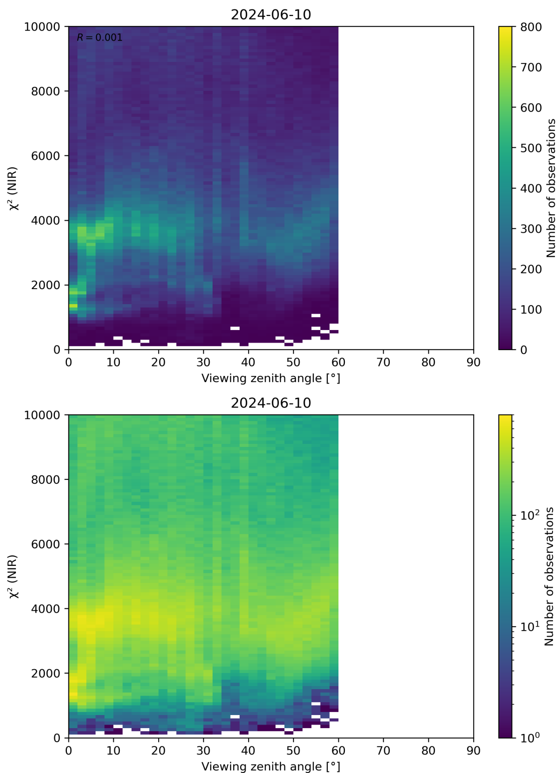
Figure 105: Scatter density plot of “Viewing zenith angle” against “ \chi^2 (NIR)” for 2024-06-09 to 2024-06-11.
