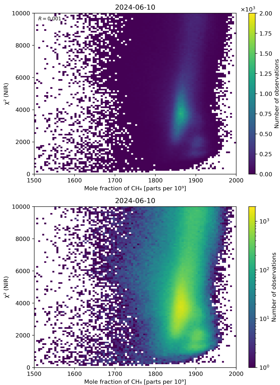
Figure 70: Scatter density plot of “Mole fraction of \text{CH}_4 ” against “ \chi^2 (NIR)” for 2024-06-09 to 2024-06-11.
