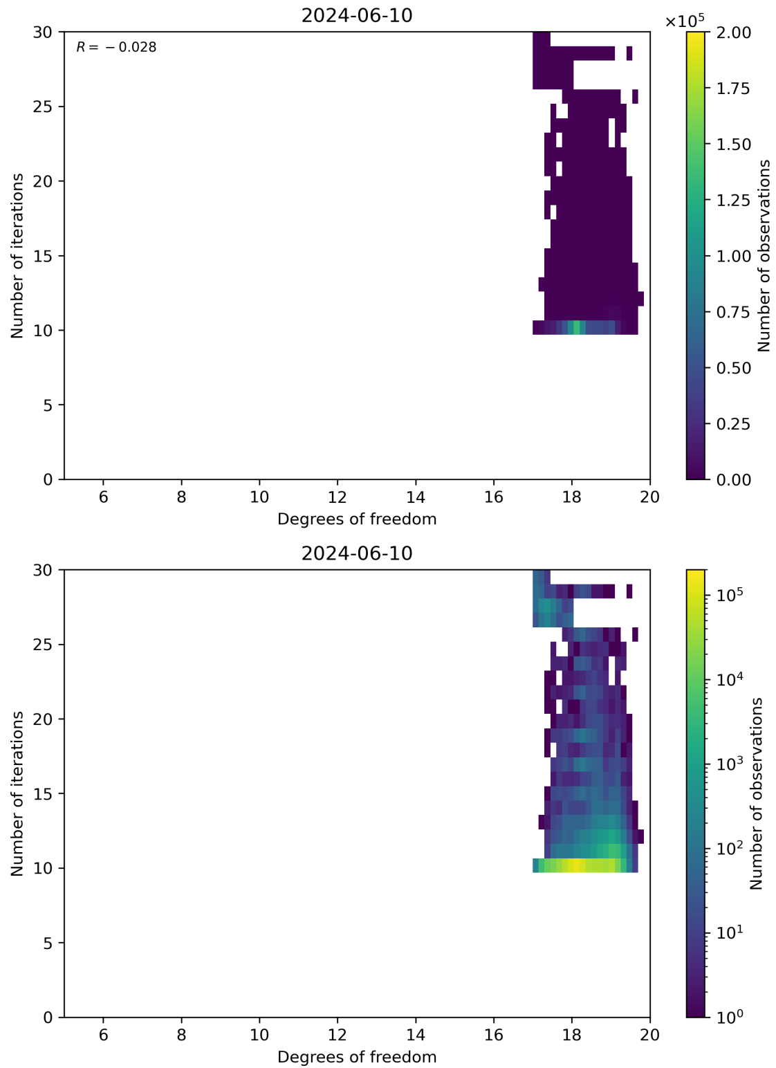
Figure 52: Scatter density plot of “Degrees of freedom” against “Number of iterations” for 2024-06-09 to 2024-06-11.
