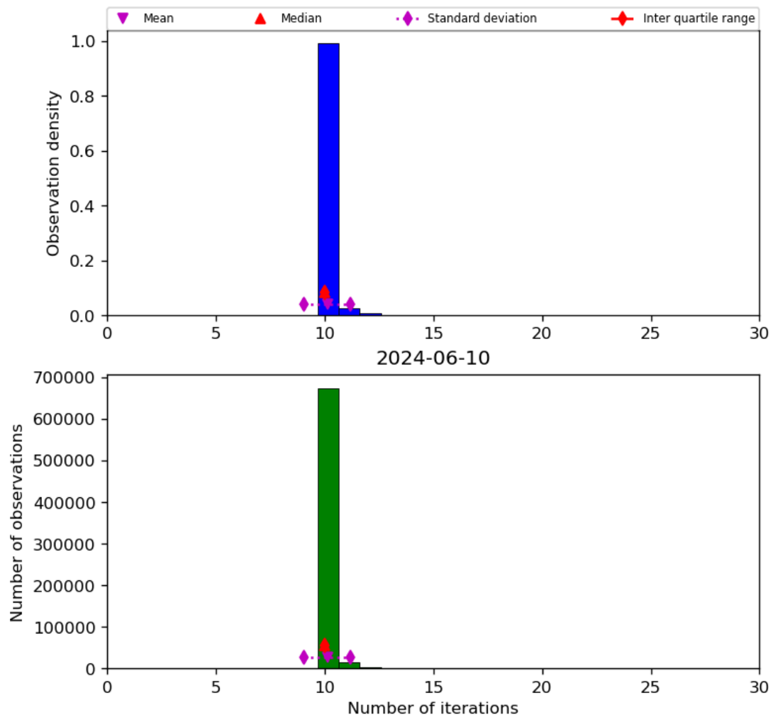
Figure 31: Histogram of “Number of iterations” for 2024-06-09 to 2024-06-11
