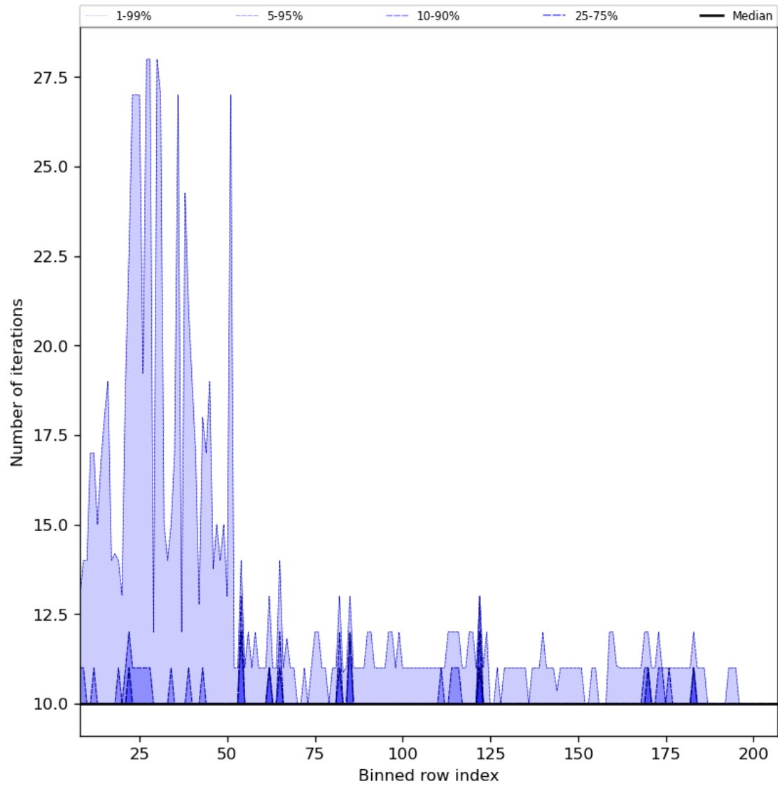
Figure 42: Along track statistics of “Number of iterations” for 2024-06-09 to 2024-06-11
