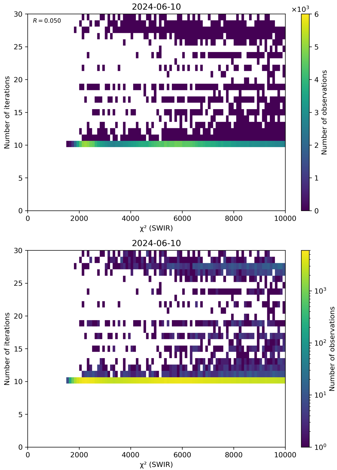
Figure 50: Scatter density plot of “ \chi^2 (SWIR)” against “Number of iterations” for 2024-06-09 to 2024-06-11.
