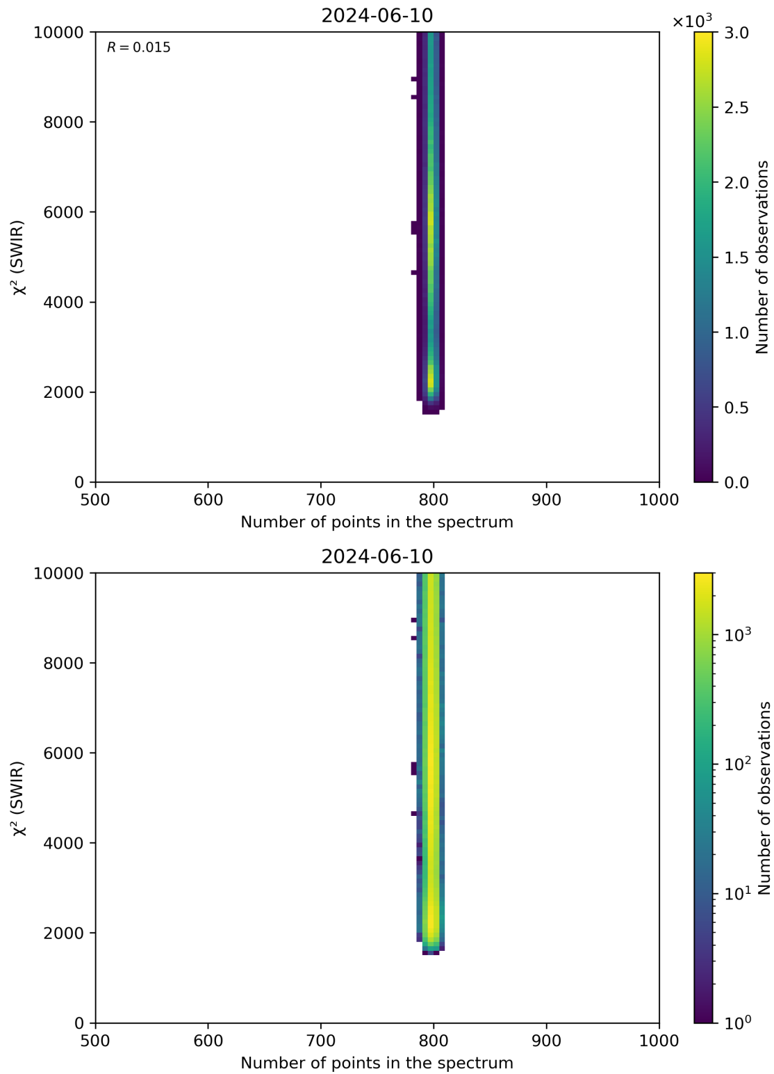
Figure 89: Scatter density plot of “Number of points in the spectrum” against “ \chi^2 (SWIR)” for 2024-06-09 to 2024-06-11.
