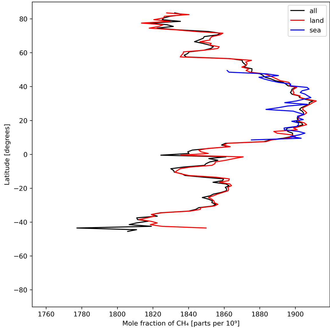
Figure 12: Zonal average of “Mole fraction of \text{CH}_4 ” for 2024-06-09 to 2024-06-11.
