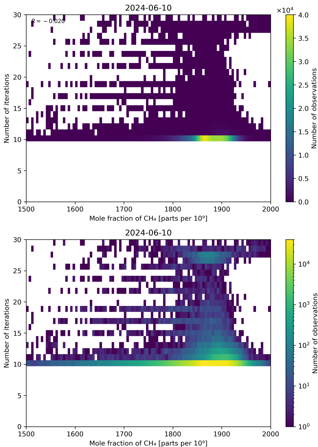
Figure 76: Scatter density plot of “Mole fraction of CH 4 ” against “Number of iterations” for 2024-06-09 to 2024-06-11.
