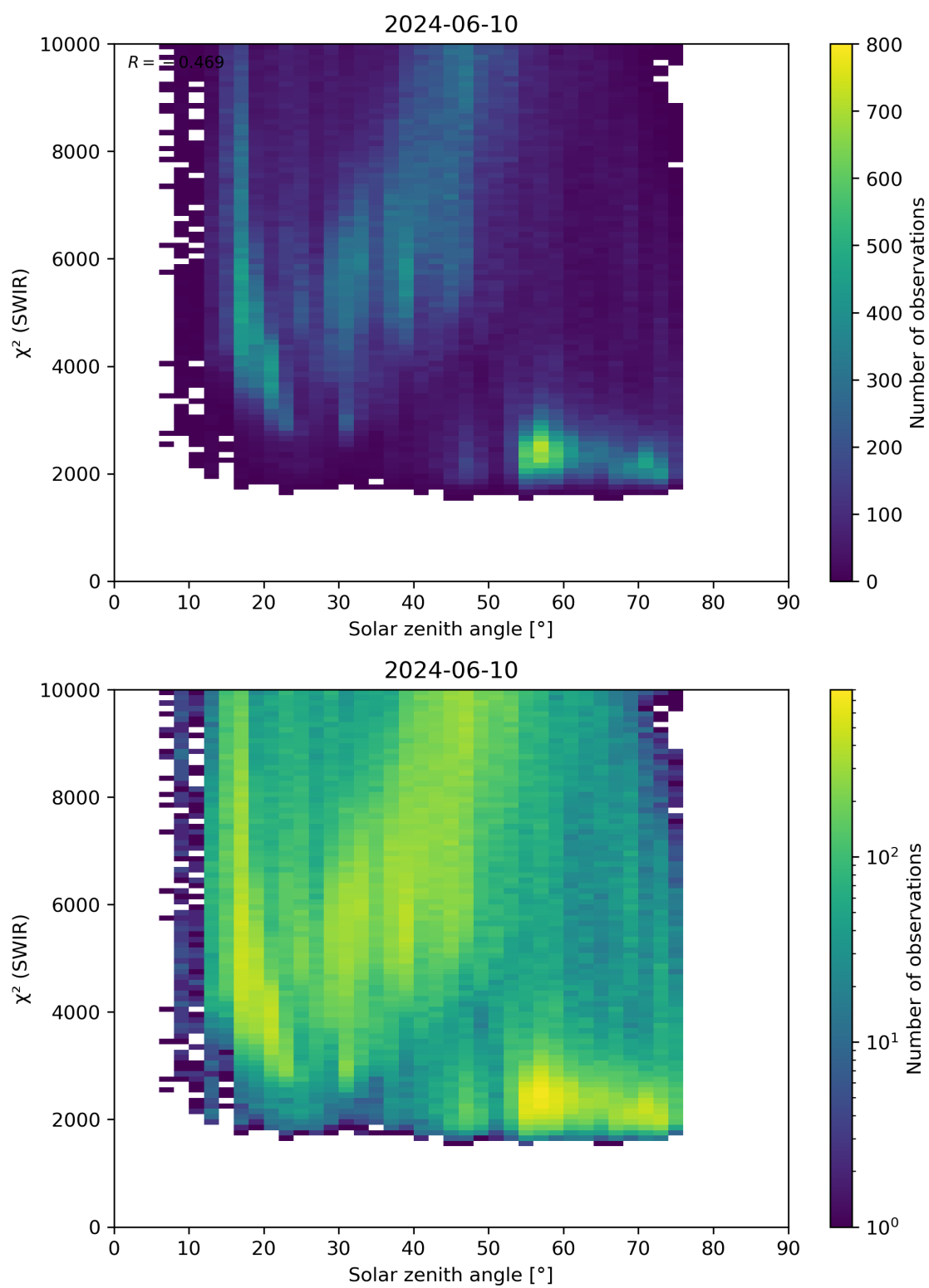
Figure 95: Scatter density plot of “Solar zenith angle” against “ \chi^2 (SWIR)” for 2024-06-09 to 2024-06-11.
