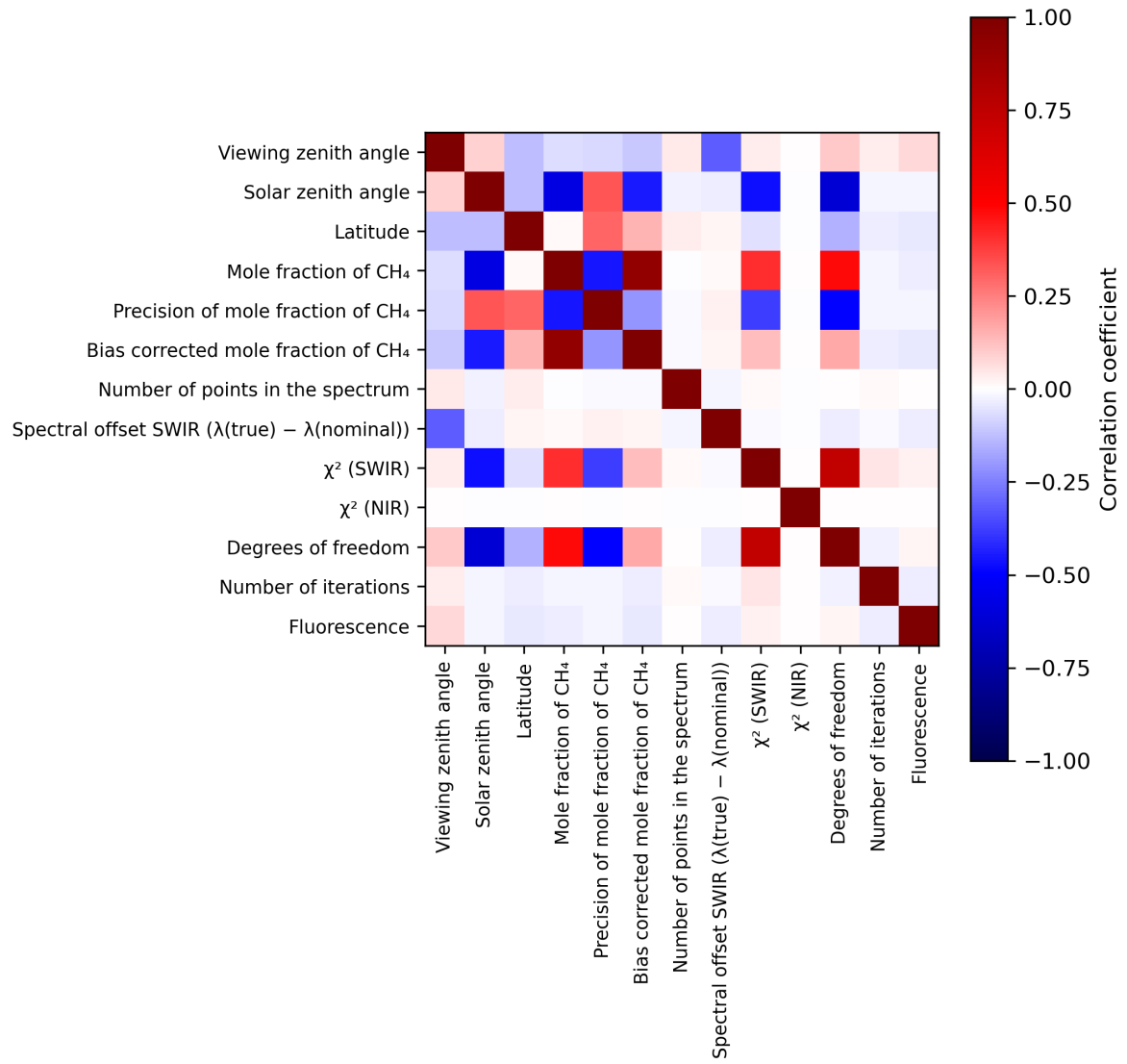
Figure 2: Map of correlation matrix for 2024-06-09 to 2024-06-11.
