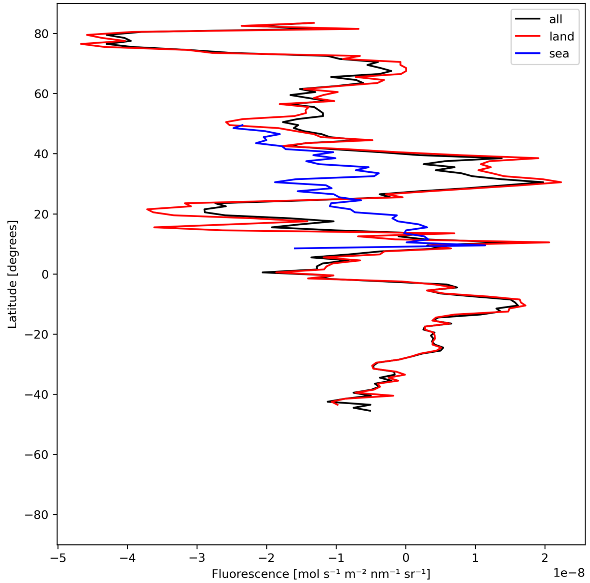
Figure 21: Zonal average of “Fluorescence” for 2024-06-09 to 2024-06-11.
