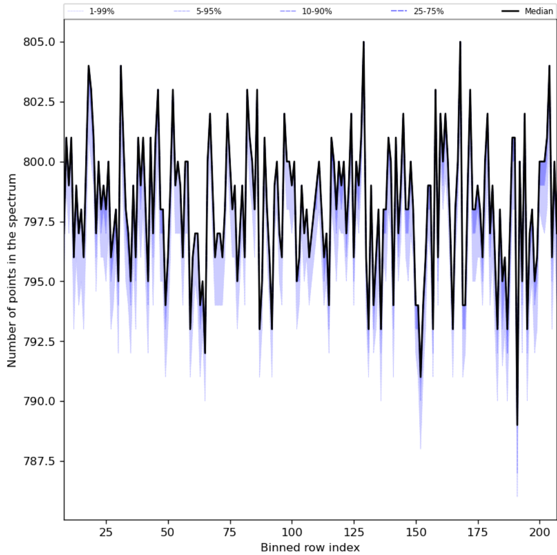
Figure 37: Along track statistics of “Number of points in the spectrum” for 2024-06-09 to 2024-06-11
