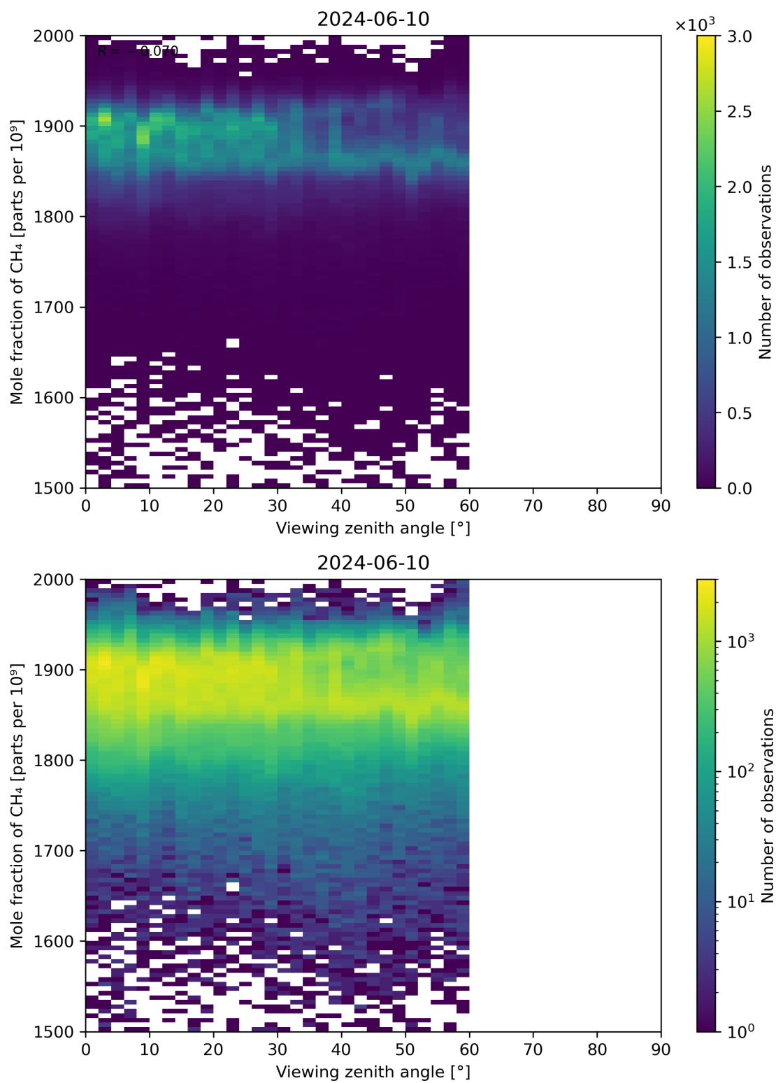
Figure 110: Scatter density plot of “Viewing zenith angle” against “Mole fraction of CH 4 ” for 2024-06-09 to 2024-06-11.
