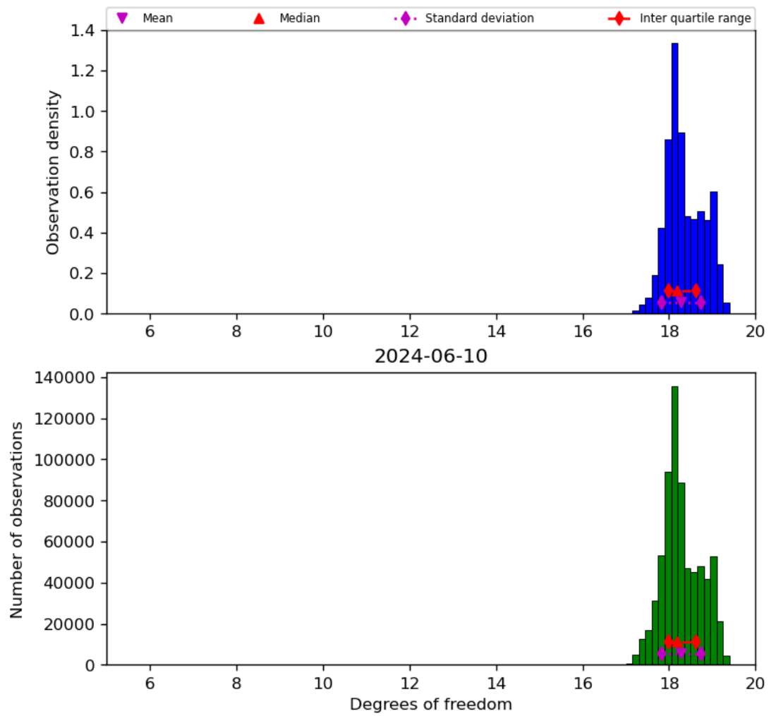
Figure 30: Histogram of “Degrees of freedom” for 2024-06-09 to 2024-06-11
