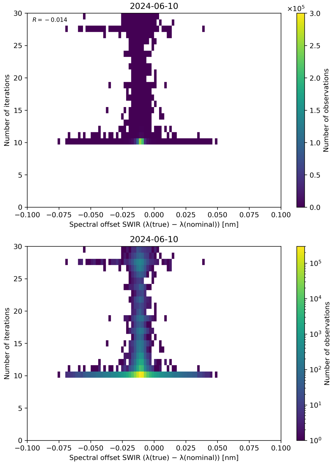
Figure 121: Scatter density plot of “Spectral offset SWIR ( \lambda(\text{true}) - \lambda(\text{nominal}) )” against “Number of iterations” for 2024-06-09 to 2024-06-11.
