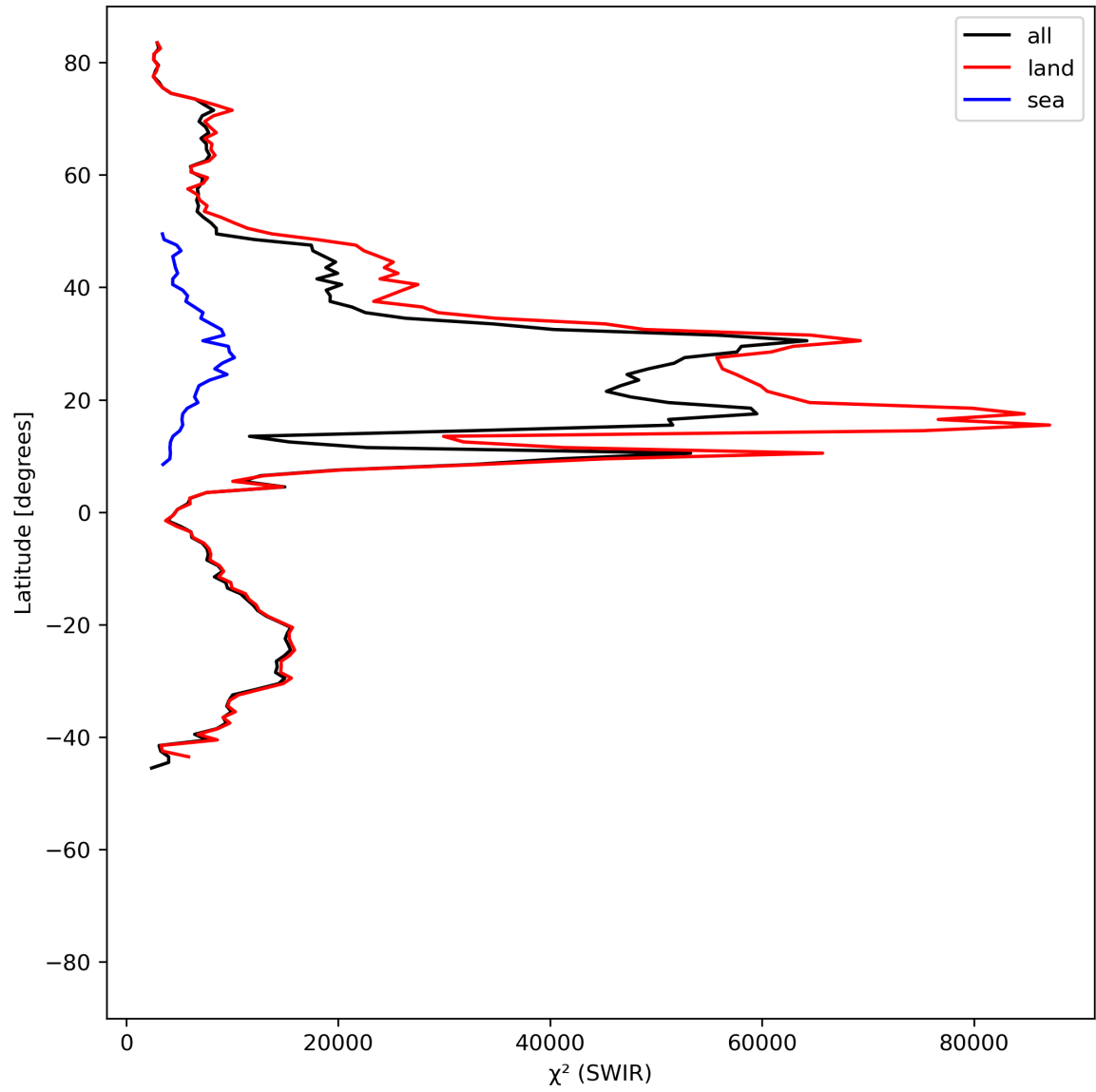
Figure 17: Zonal average of “ \chi^2 (SWIR)” for 2024-06-09 to 2024-06-11.
