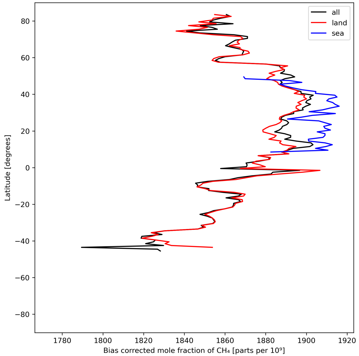
Figure 14: Zonal average of “Bias corrected mole fraction of CH 4 ” for 2024-06-09 to 2024-06-11.
