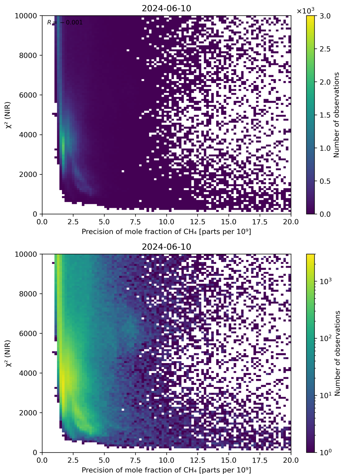
Figure 78: Scatter density plot of “Precision of mole fraction of CH 4 ” against “ \chi^2 (NIR)” for 2024-06-09 to 2024-06-11.
