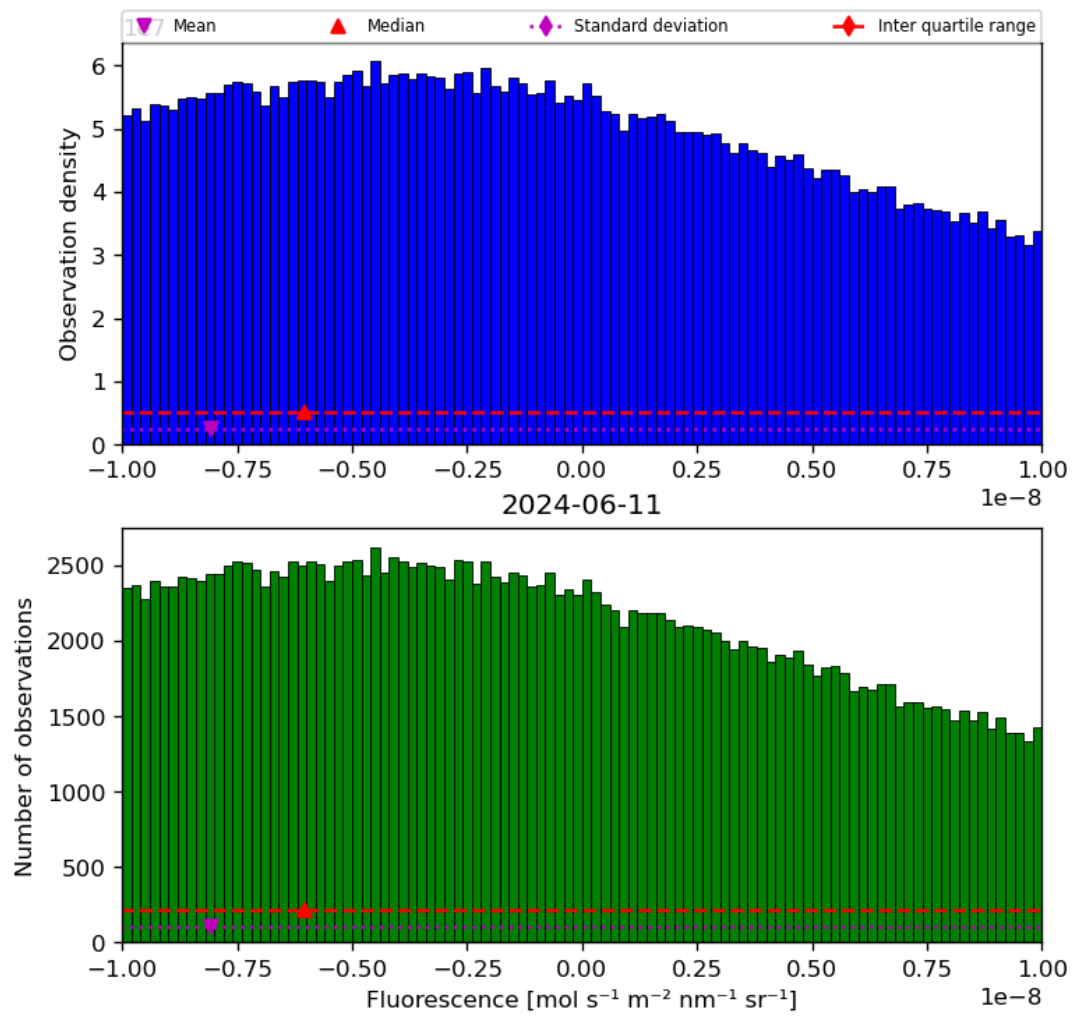
Figure 32: Histogram of “Fluorescence” for 2024-06-10 to 2024-06-12
