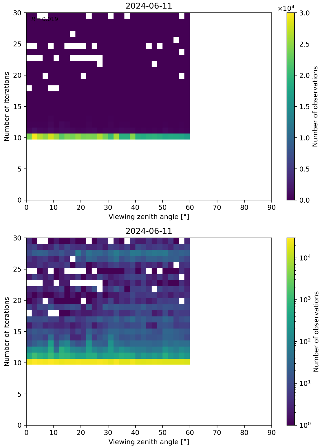
Figure 113: Scatter density plot of “Viewing zenith angle” against “Number of iterations” for 2024-06-10 to 2024-06-12.
