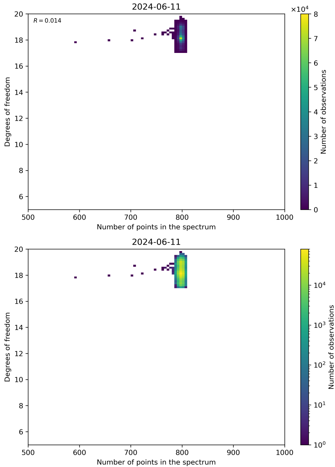
Figure 90: Scatter density plot of “Number of points in the spectrum” against “Degrees of freedom” for 2024-06-10 to 2024-06-12.
