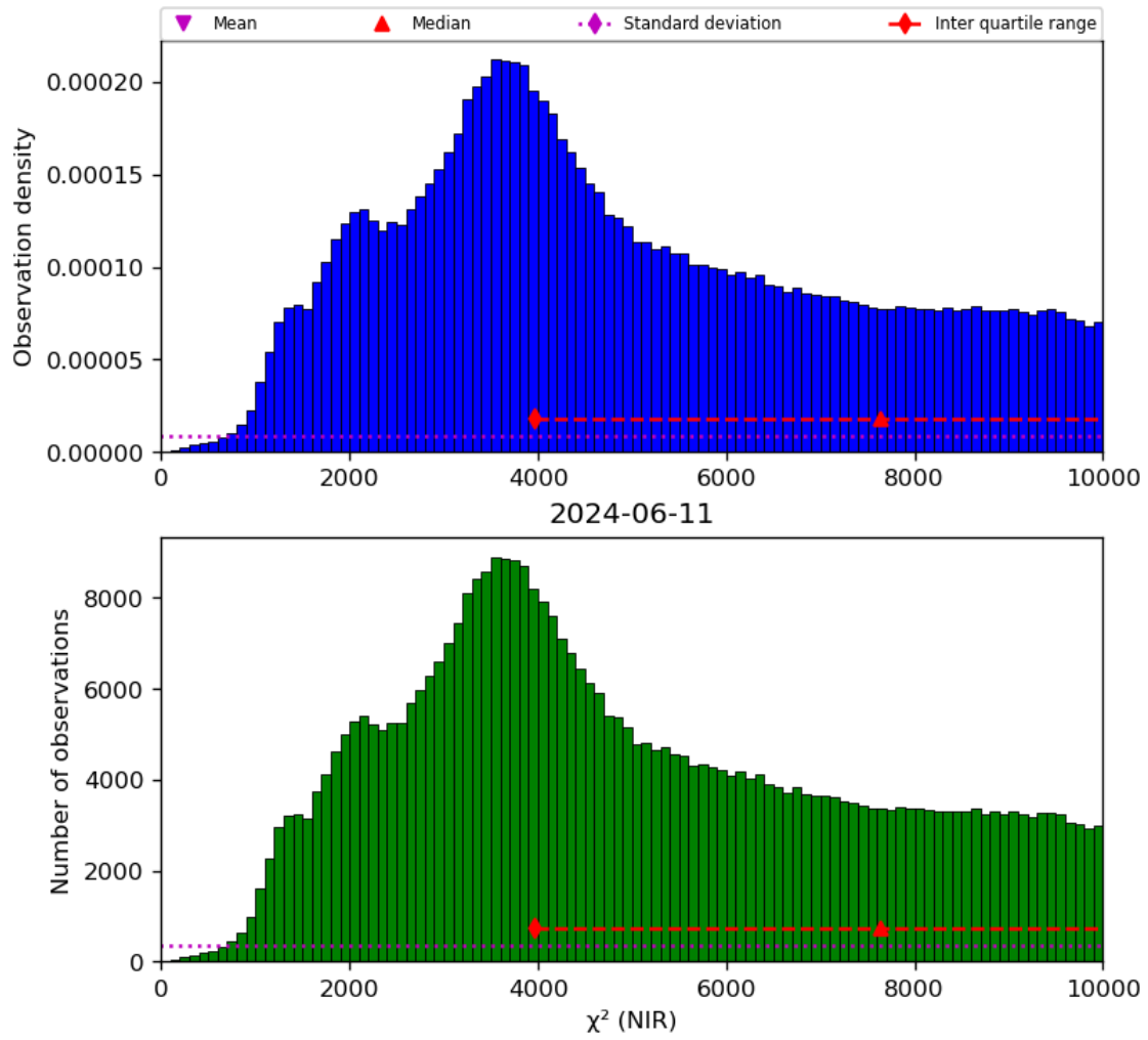
Figure 29: Histogram of “ \chi^2 (NIR)” for 2024-06-10 to 2024-06-12
