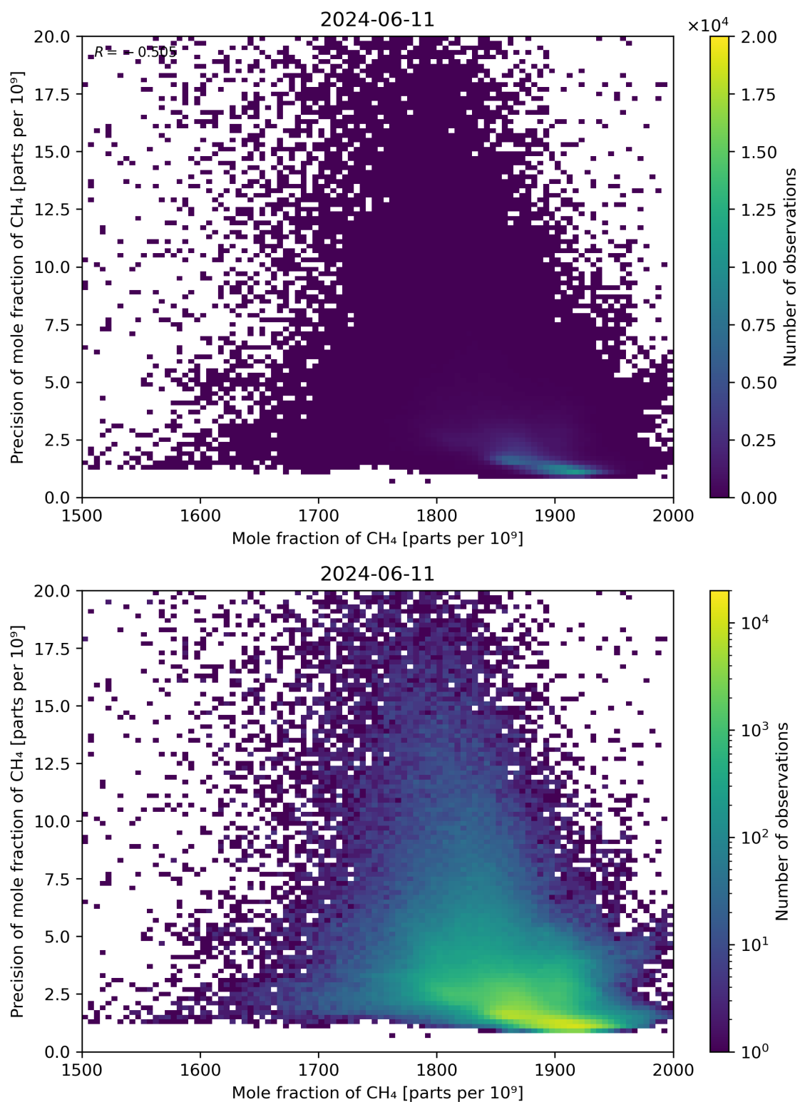
Figure 75: Scatter density plot of “Mole fraction of CH 4 ” against “Precision of mole fraction of CH 4 ” for 2024-06-10 to 2024-06-12.
