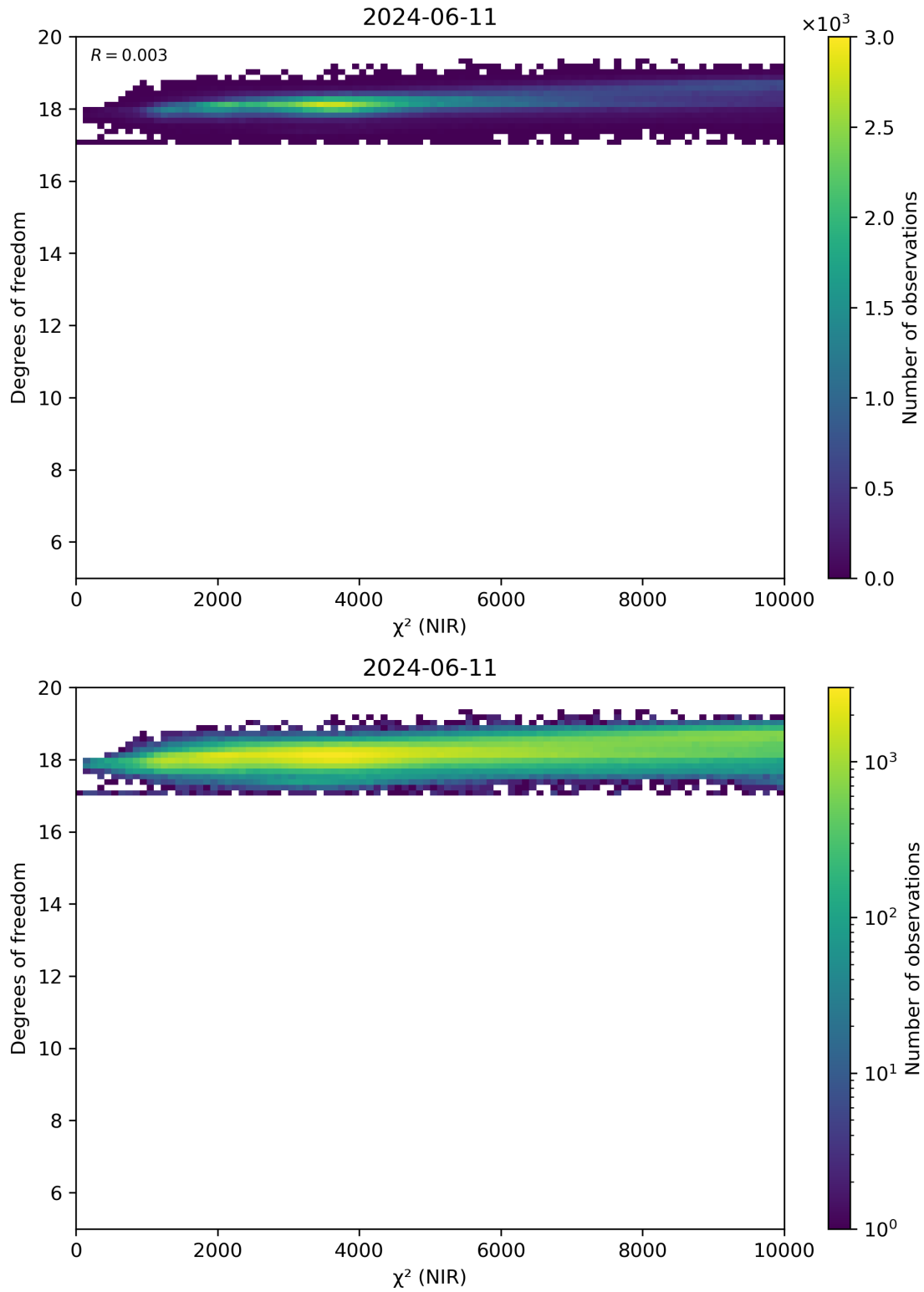
Figure 44: Scatter density plot of “ \chi^2 (NIR)” against “Degrees of freedom” for 2024-06-10 to 2024-06-12.
