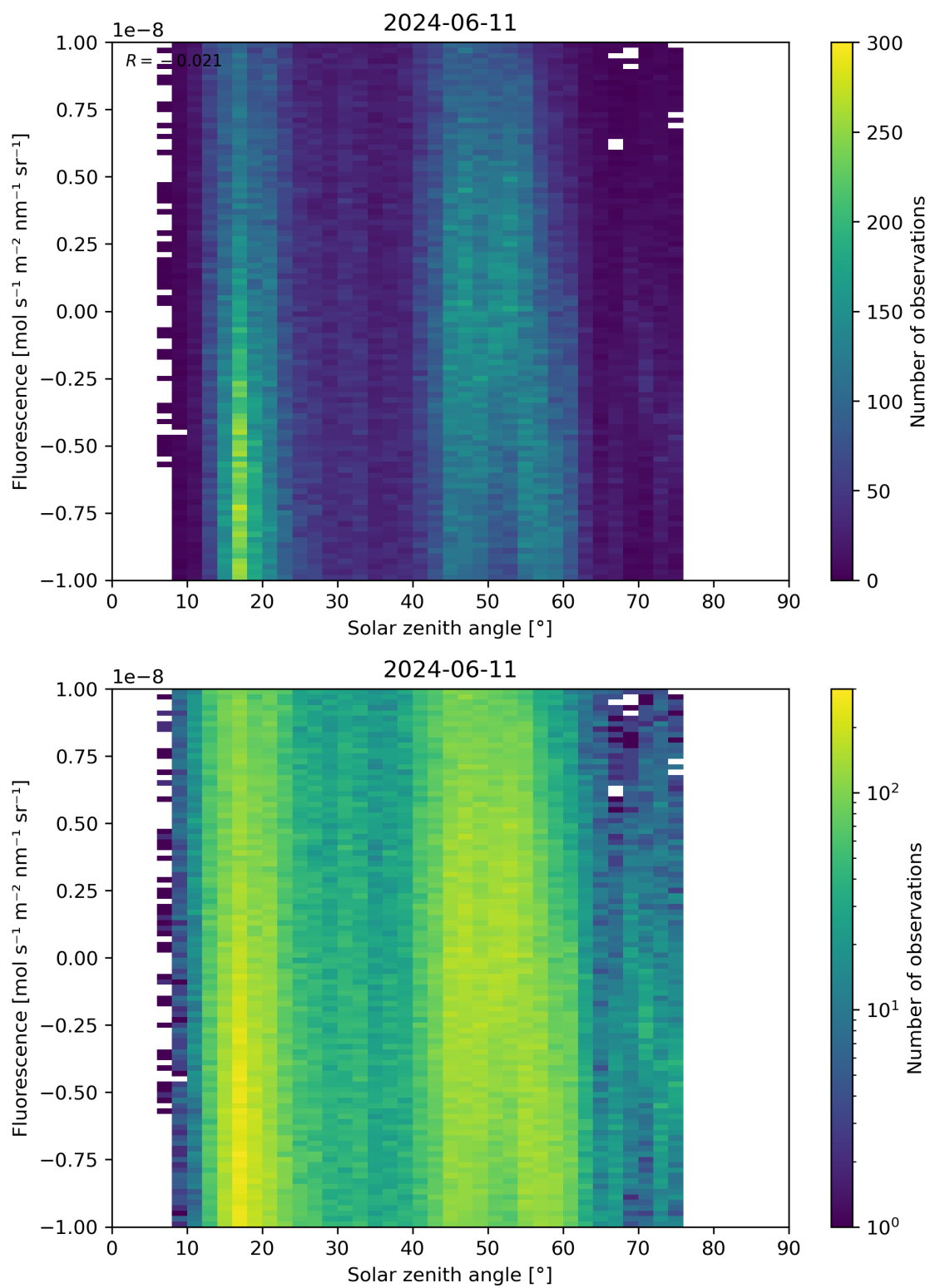
Figure 97: Scatter density plot of “Solar zenith angle” against “Fluorescence” for 2024-06-10 to 2024-06-12.
