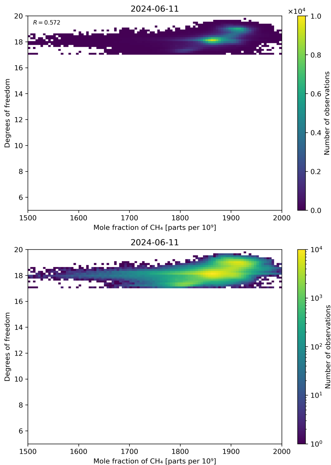
Figure 72: Scatter density plot of “Mole fraction of CH 4 ” against “Degrees of freedom” for 2024-06-10 to 2024-06-12.
