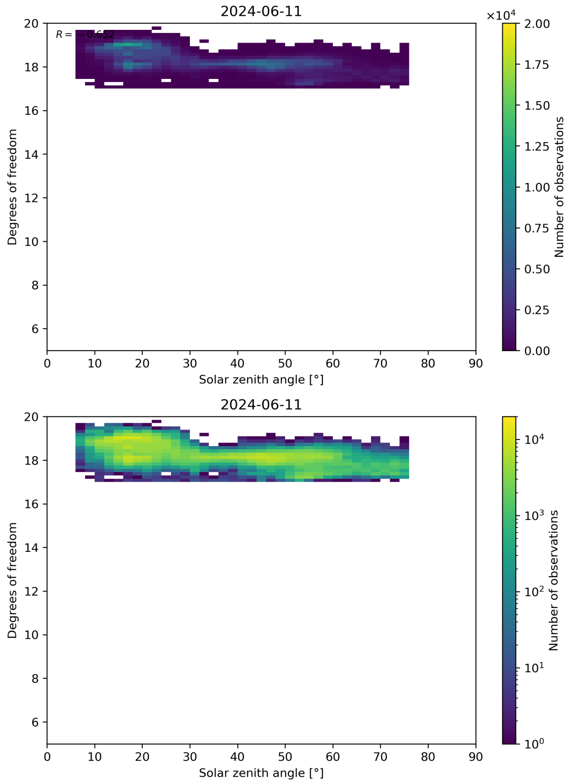
Figure 96: Scatter density plot of “Solar zenith angle” against “Degrees of freedom” for 2024-06-10 to 2024-06-12.
