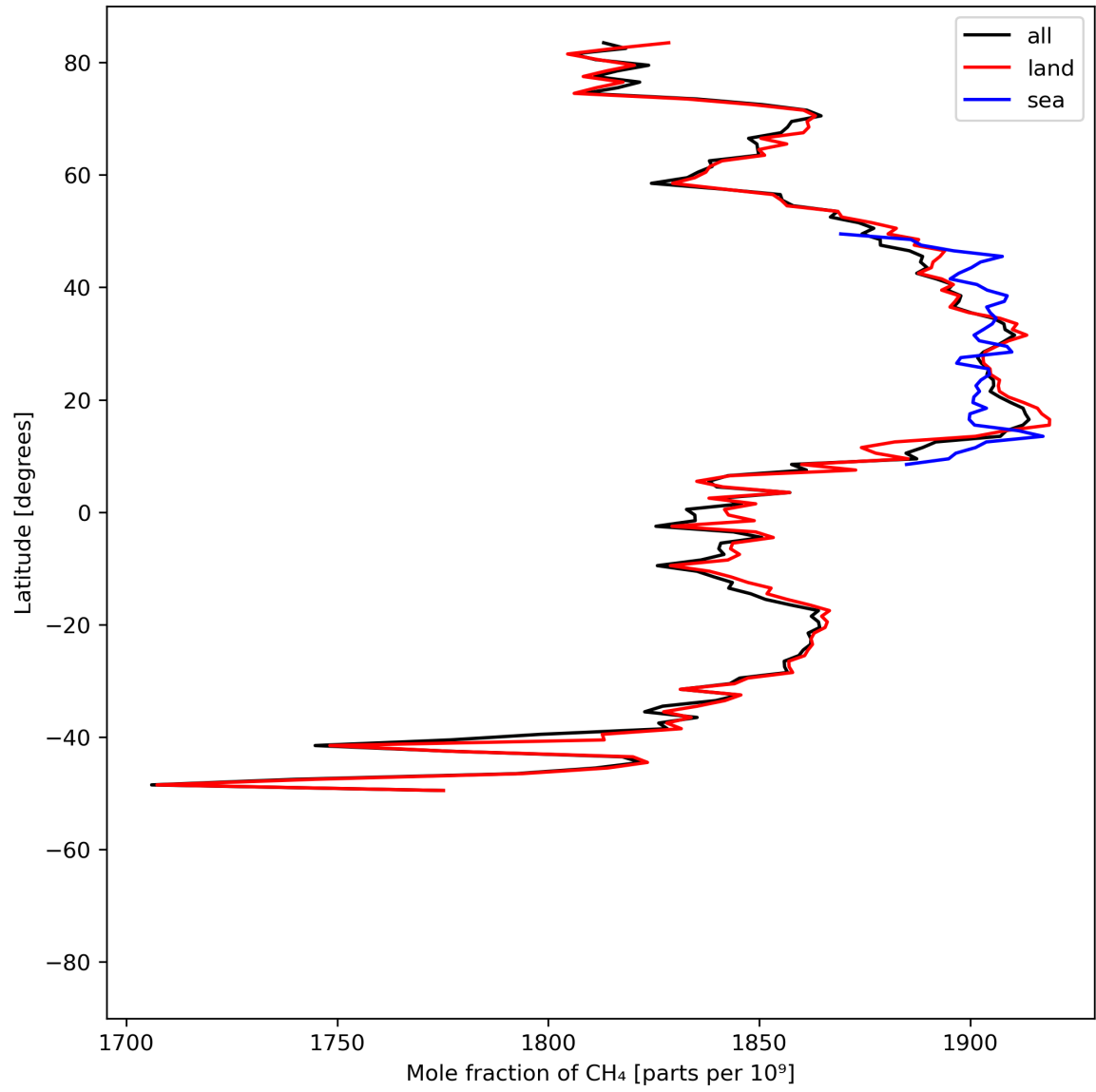
Figure 12: Zonal average of “Mole fraction of \text{CH}_4 ” for 2024-06-10 to 2024-06-12.
