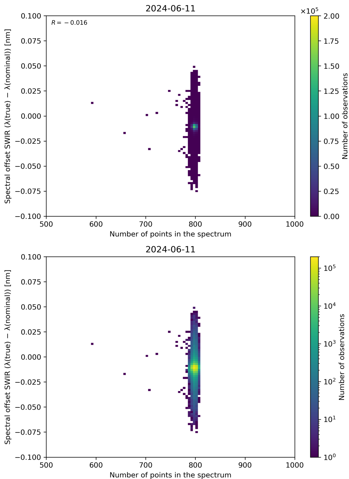
Figure 93: Scatter density plot of “Number of points in the spectrum” against “Spectral offset SWIR ( \lambda(\text{true}) - \lambda(\text{nominal}) )” for 2024-06-10 to 2024-06-12.
