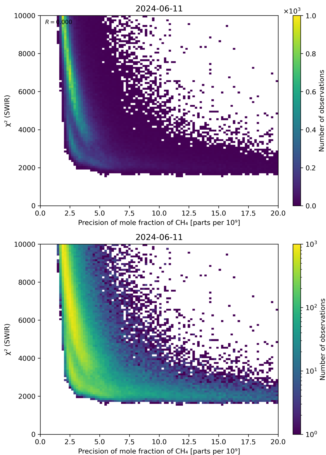
Figure 79: Scatter density plot of “Precision of mole fraction of CH 4 ” against “ \chi^2 (SWIR)” for 2024-06-10 to 2024-06-12.
