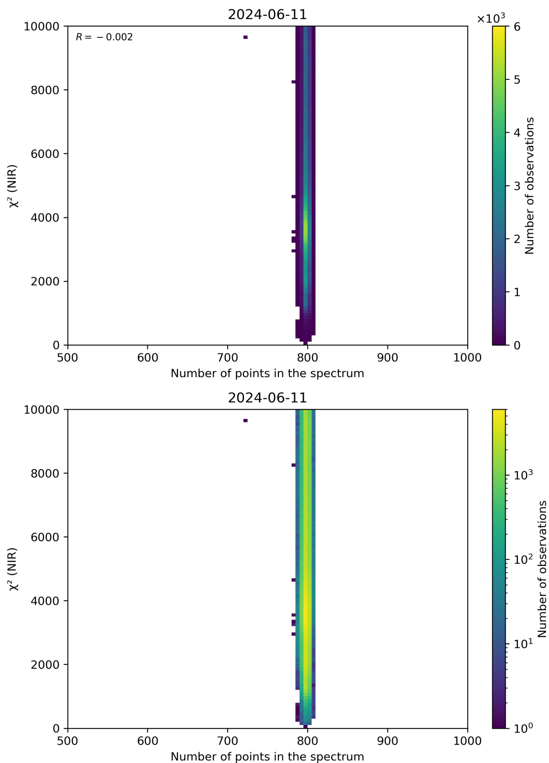
Figure 88: Scatter density plot of “Number of points in the spectrum” against “ \chi^2 (NIR)” for 2024-06-10 to 2024-06-12.
