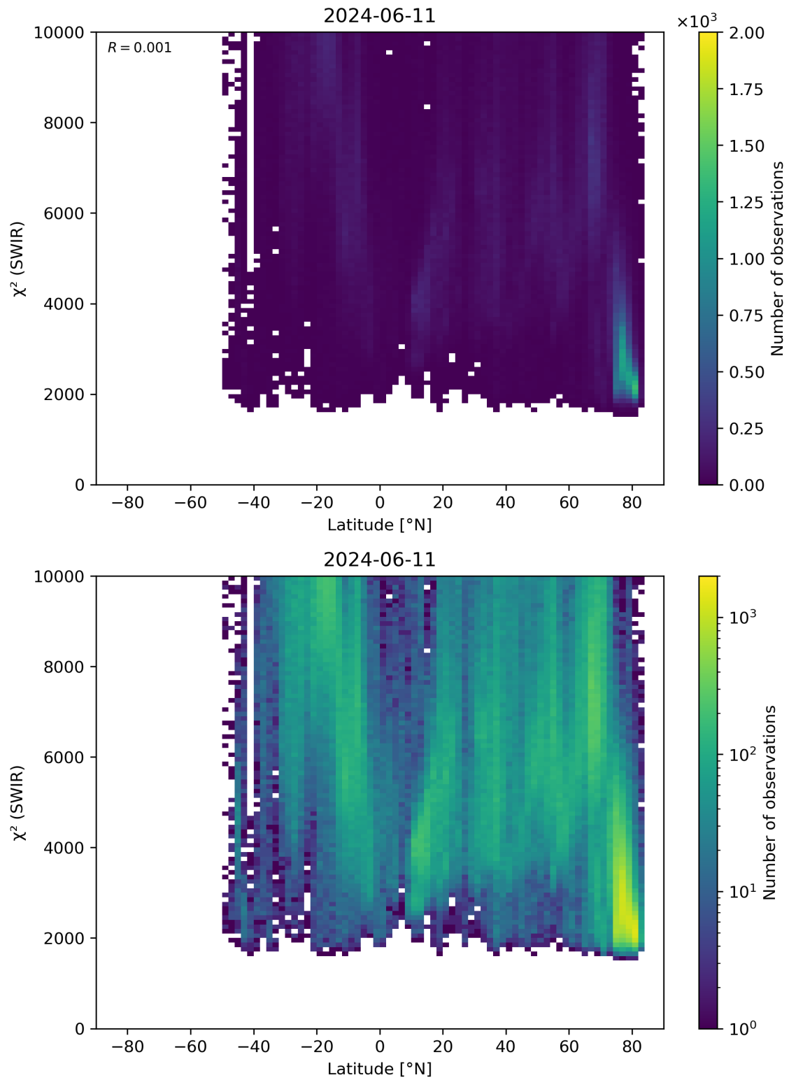
Figure 54: Scatter density plot of “Latitude” against “ \chi^2 (SWIR)” for 2024-06-10 to 2024-06-12.
