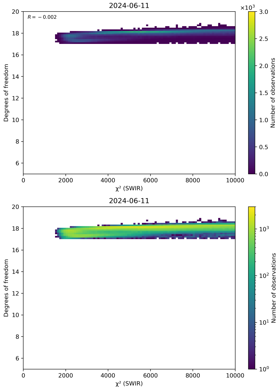
Figure 48: Scatter density plot of “ \chi^2 (SWIR)” against “Degrees of freedom” for 2024-06-10 to 2024-06-12.
