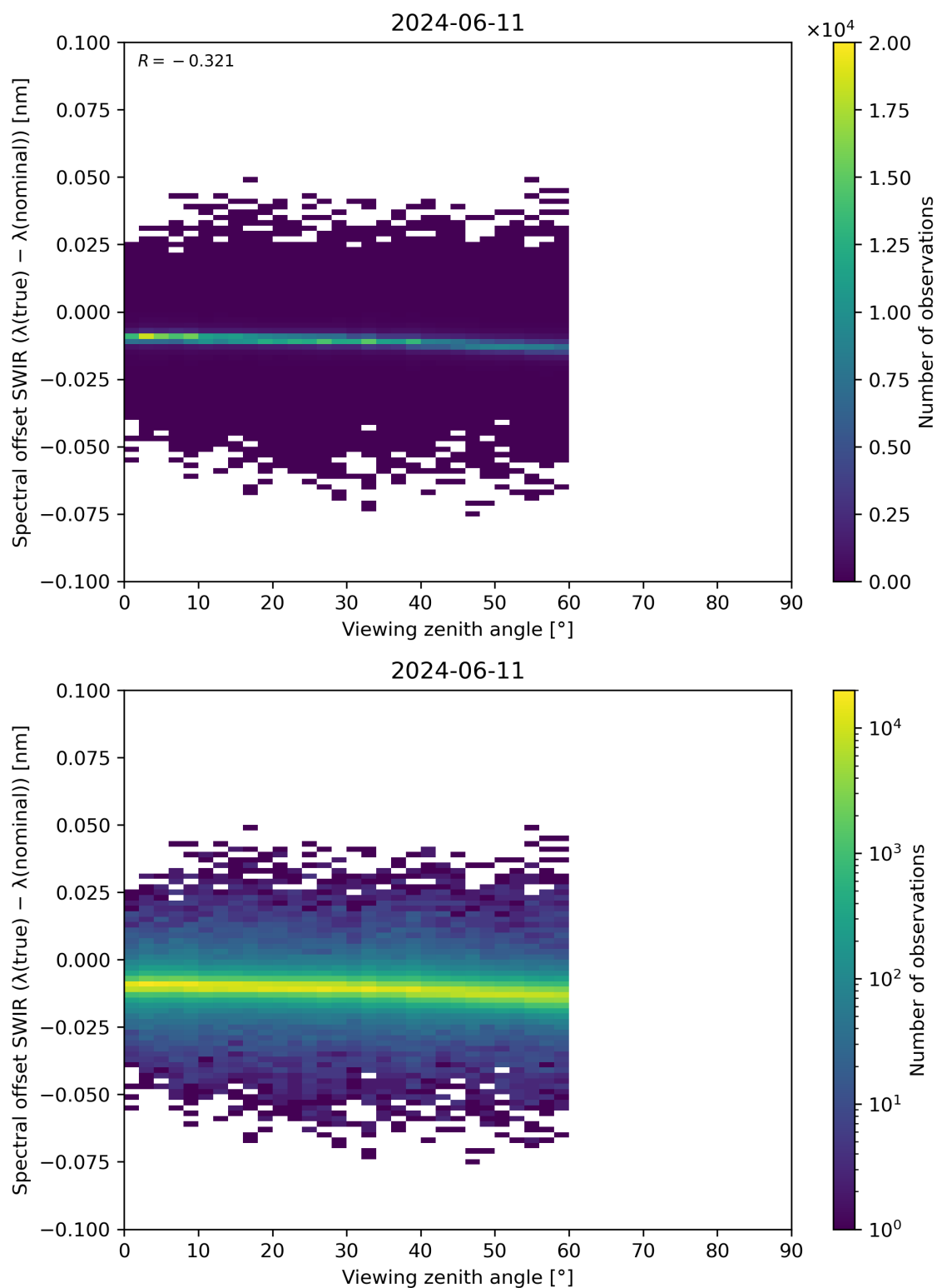
Figure 116: Scatter density plot of “Viewing zenith angle” against “Spectral offset SWIR ( \lambda(\text{true}) - \lambda(\text{nominal}) )” for 2024-06-10 to 2024-06-12.
