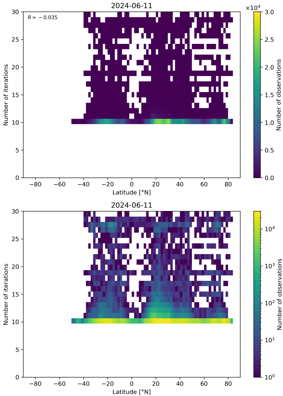
Figure 60: Scatter density plot of “Latitude” against “Number of iterations” for 2024-06-10 to 2024-06-12.
