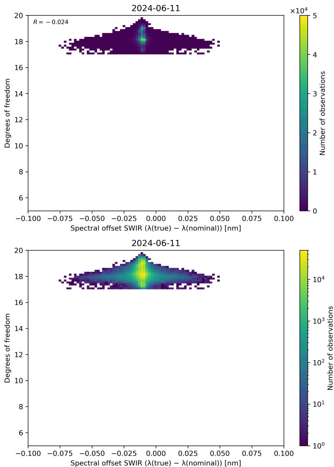
Figure 119: Scatter density plot of “Spectral offset SWIR ( \lambda(\text{true}) - \lambda(\text{nominal}) )” against “Degrees of freedom” for 2024-06-10 to 2024-06-12.
