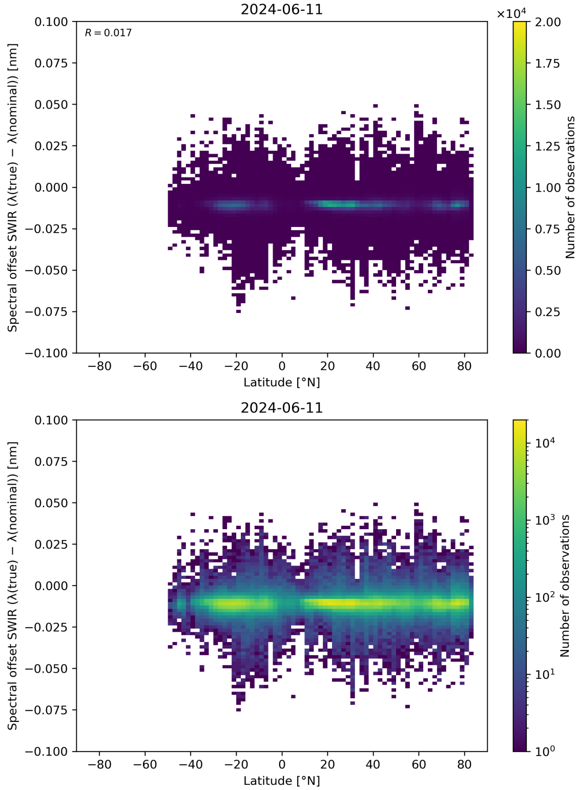
Figure 62: Scatter density plot of “Latitude” against “Spectral offset SWIR ( \lambda(\text{true}) - \lambda(\text{nominal}) )” for 2024-06-10 to 2024-06-12.
