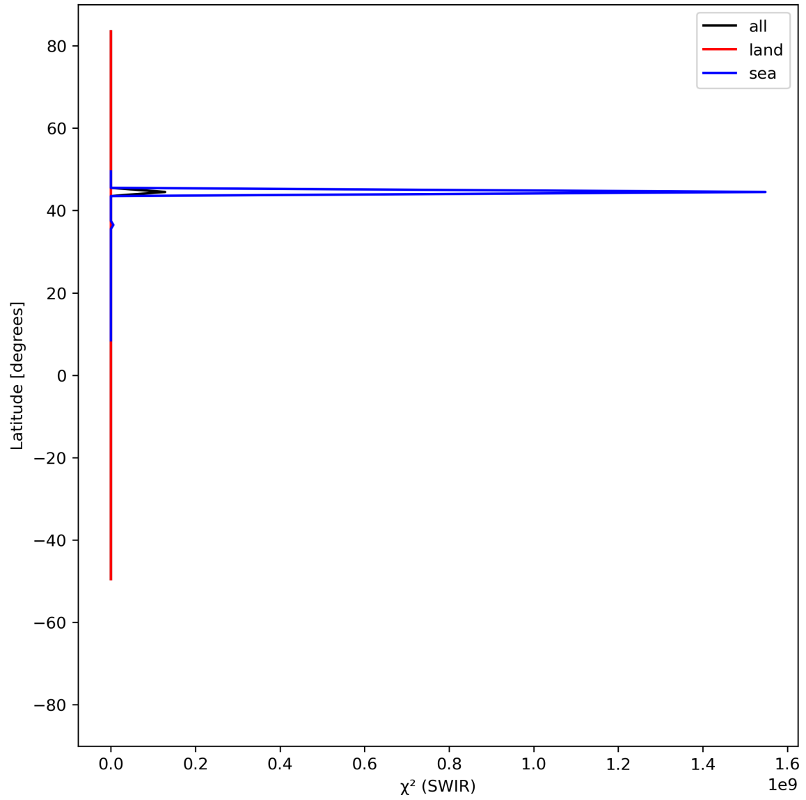
Figure 17: Zonal average of “ \chi^2 (SWIR)” for 2024-06-10 to 2024-06-12.
