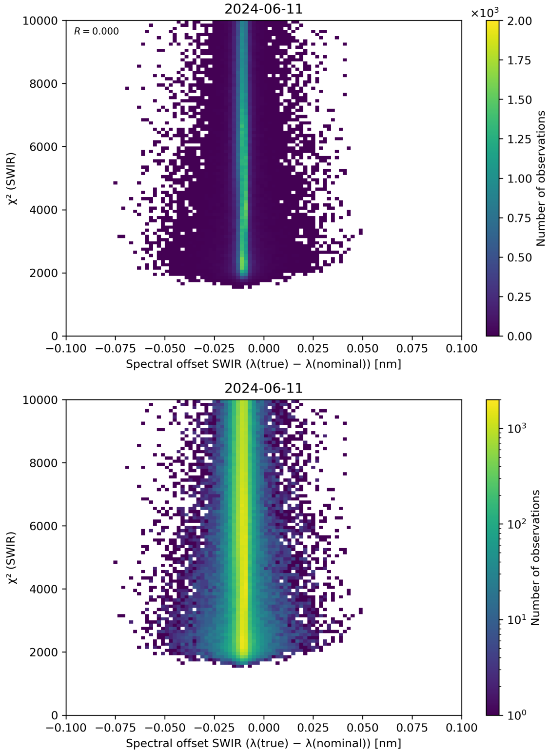
Figure 118: Scatter density plot of “Spectral offset SWIR ( \lambda(\text{true}) - \lambda(\text{nominal}) )” against “ \chi^2 (SWIR)” for 2024-06-10 to 2024-06-12.
