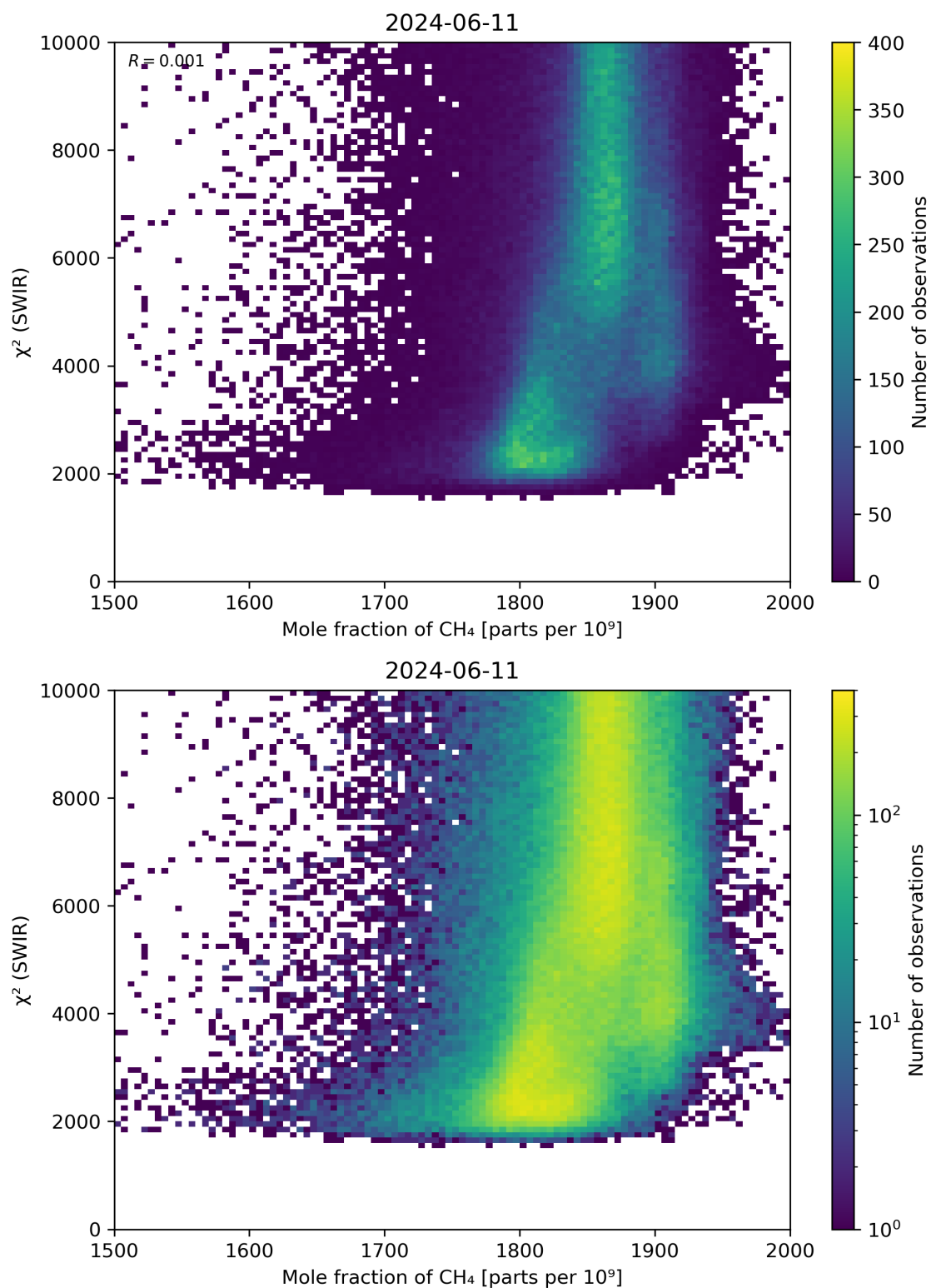
Figure 71: Scatter density plot of “Mole fraction of CH 4 ” against “ \chi^2 (SWIR)” for 2024-06-10 to 2024-06-12.
