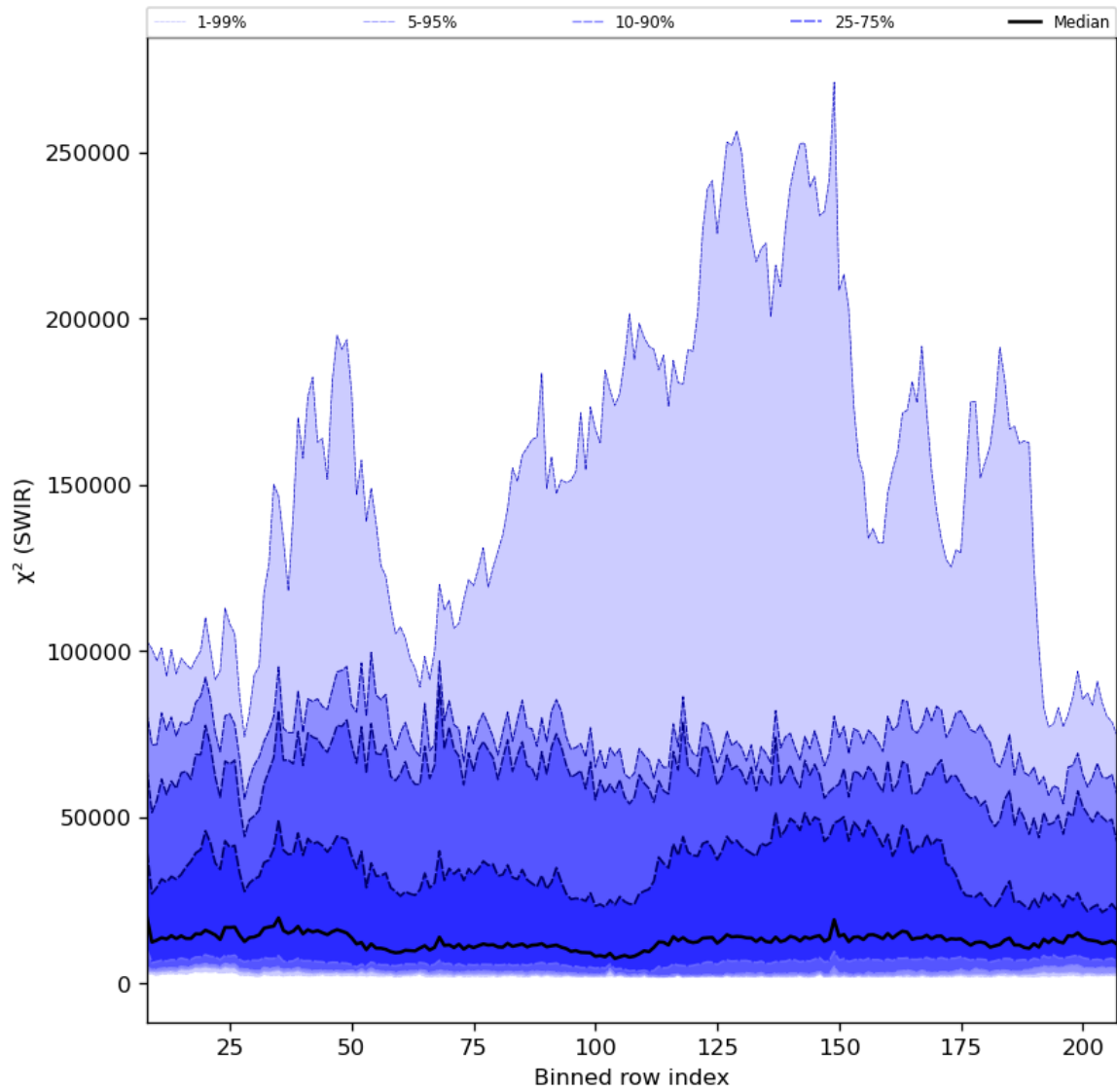
Figure 39: Along track statistics of " \chi^2 (SWIR)" for 2024-06-10 to 2024-06-12
