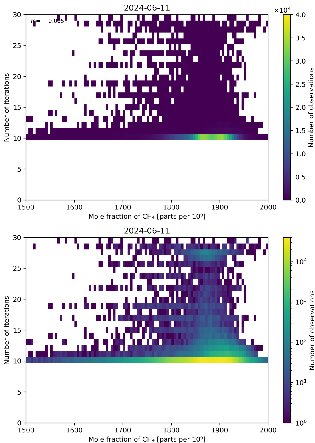
Figure 76: Scatter density plot of “Mole fraction of CH 4 ” against “Number of iterations” for 2024-06-10 to 2024-06-12.
