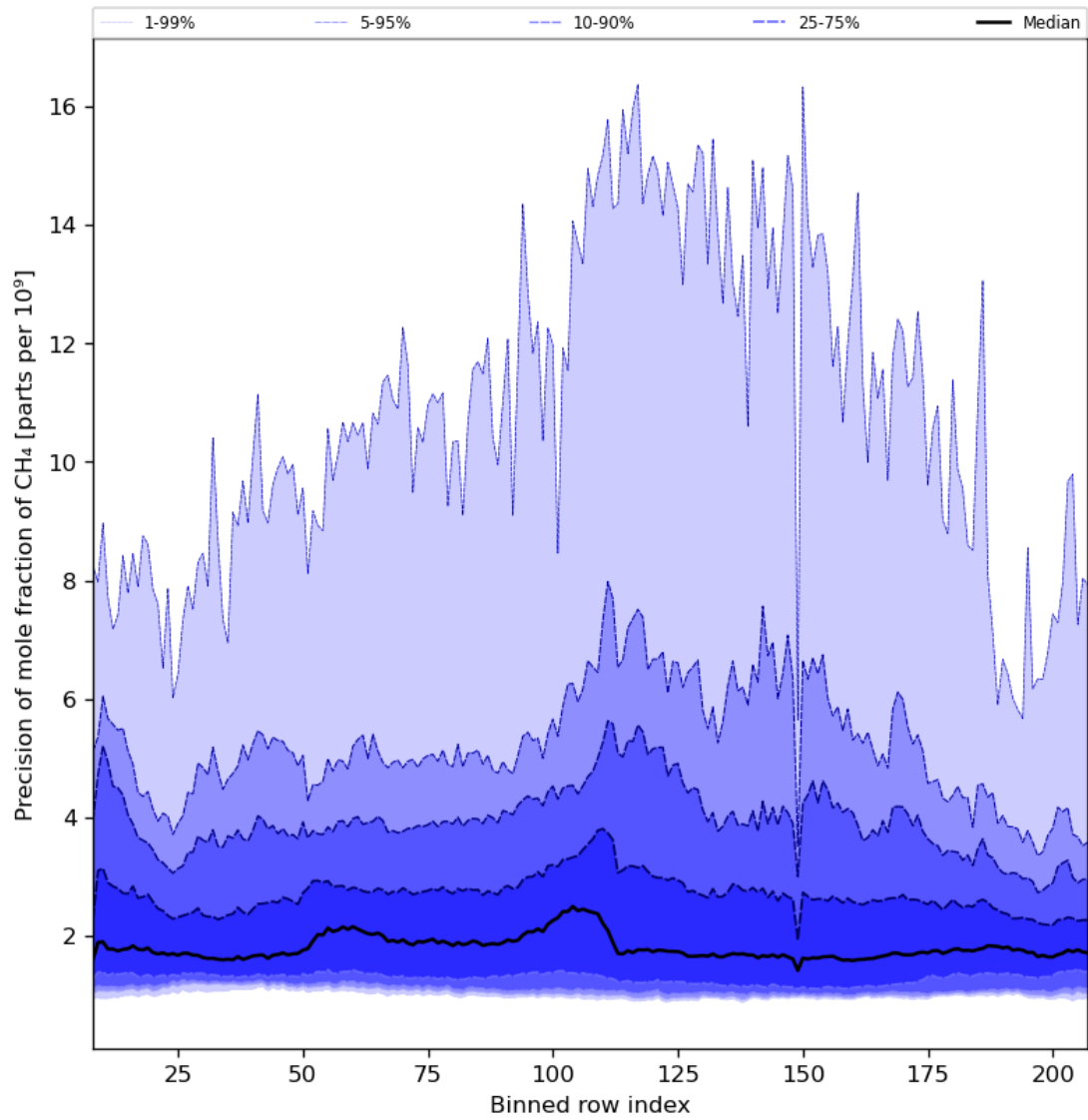
Figure 35: Along track statistics of “Precision of mole fraction of CH 4 ” for 2024-06-10 to 2024-06-12
