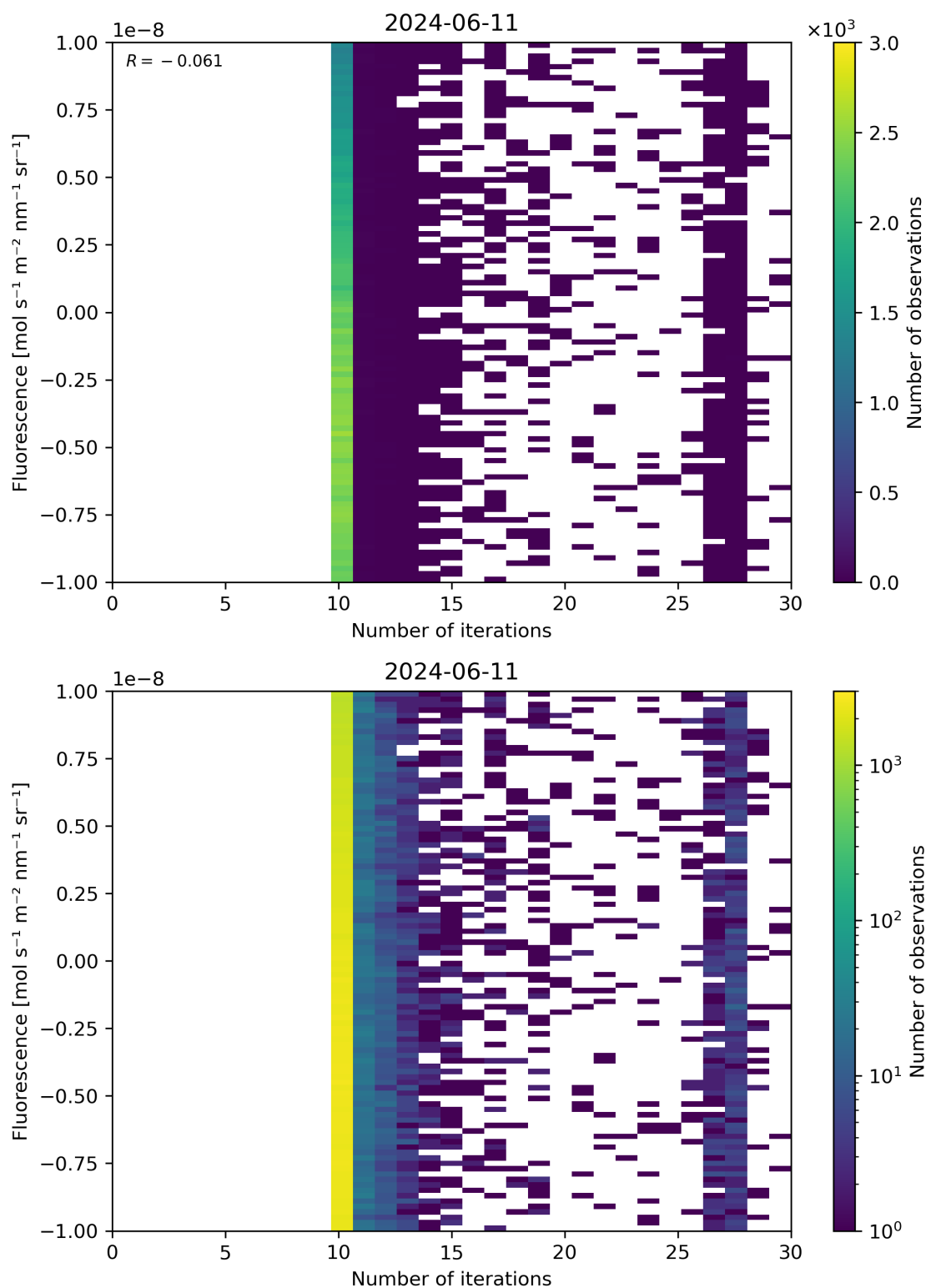
Figure 87: Scatter density plot of “Number of iterations” against “Fluorescence” for 2024-06-10 to 2024-06-12.
