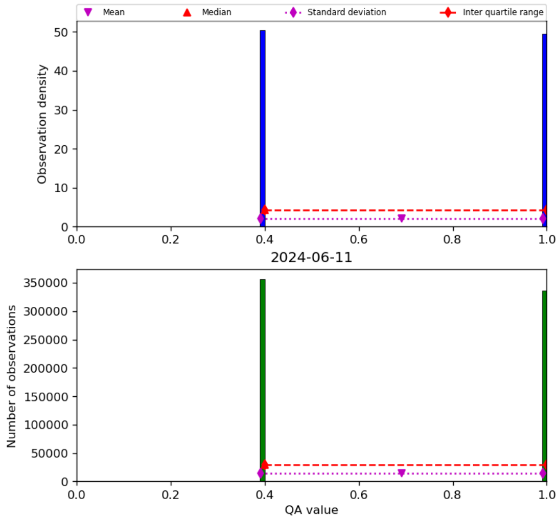
Figure 22: Histogram of “QA value” for 2024-06-10 to 2024-06-12
