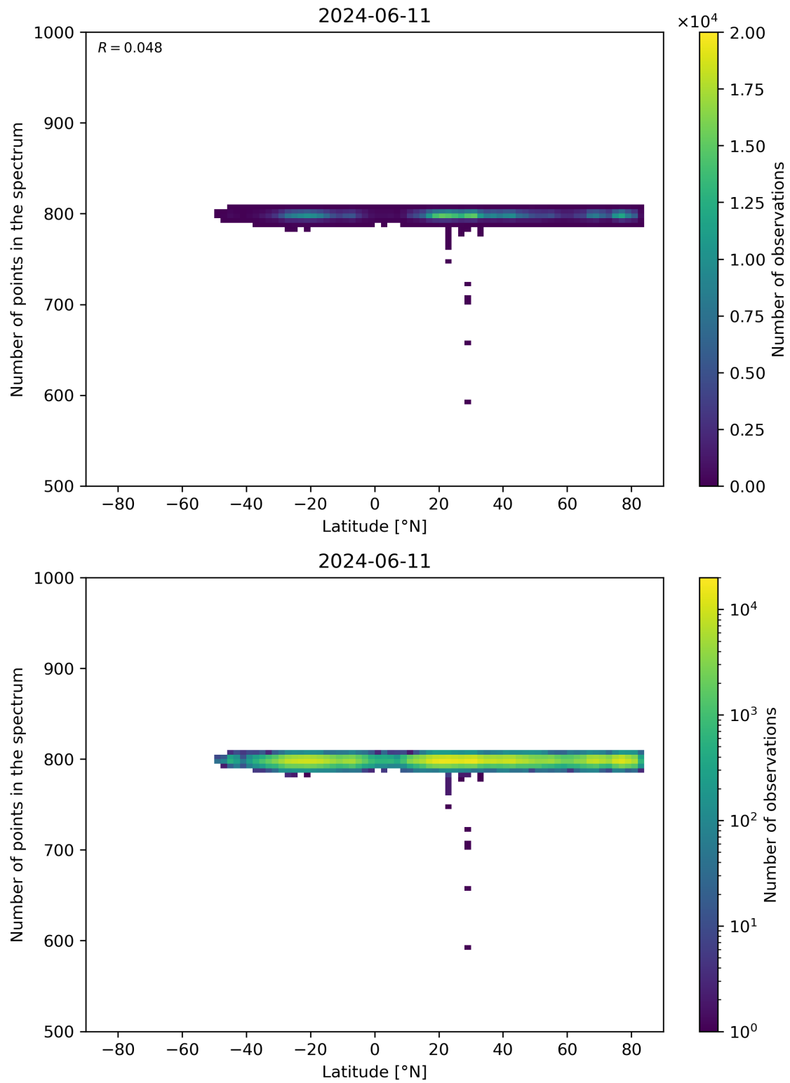
Figure 61: Scatter density plot of “Latitude” against “Number of points in the spectrum” for 2024-06-10 to 2024-06-12.
