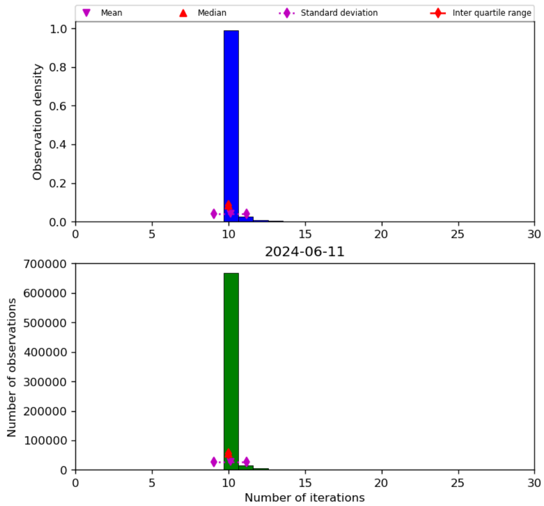
Figure 31: Histogram of “Number of iterations” for 2024-06-10 to 2024-06-12
