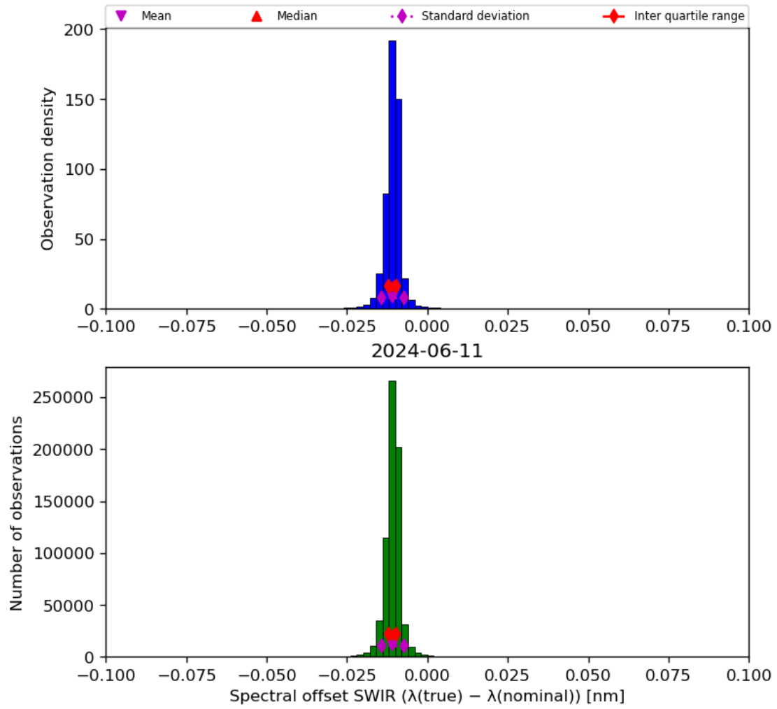
Figure 27: Histogram of “Spectral offset SWIR ( \lambda(\text{true}) - \lambda(\text{nominal}) )” for 2024-06-10 to 2024-06-12
