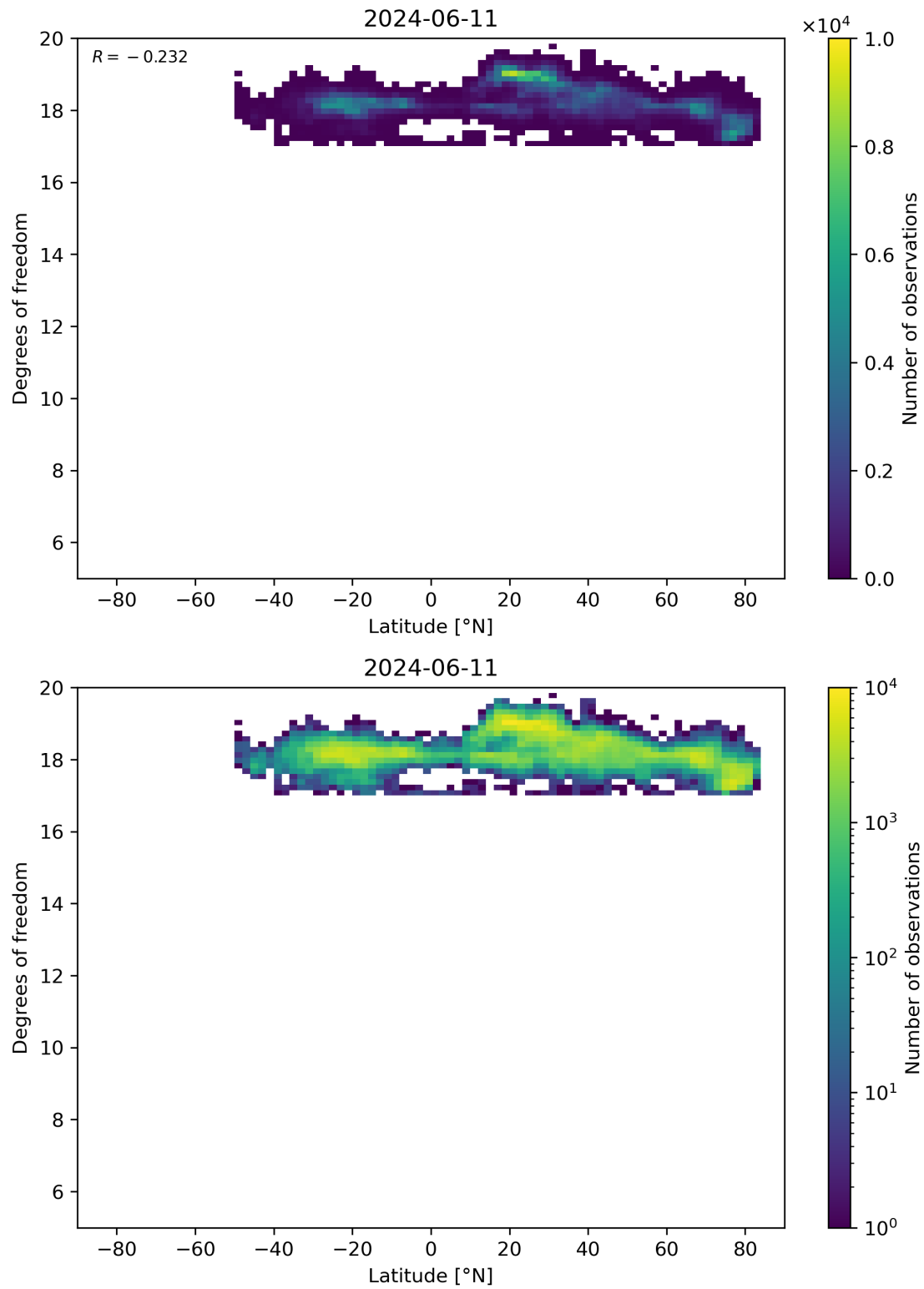
Figure 55: Scatter density plot of “Latitude” against “Degrees of freedom” for 2024-06-10 to 2024-06-12.
