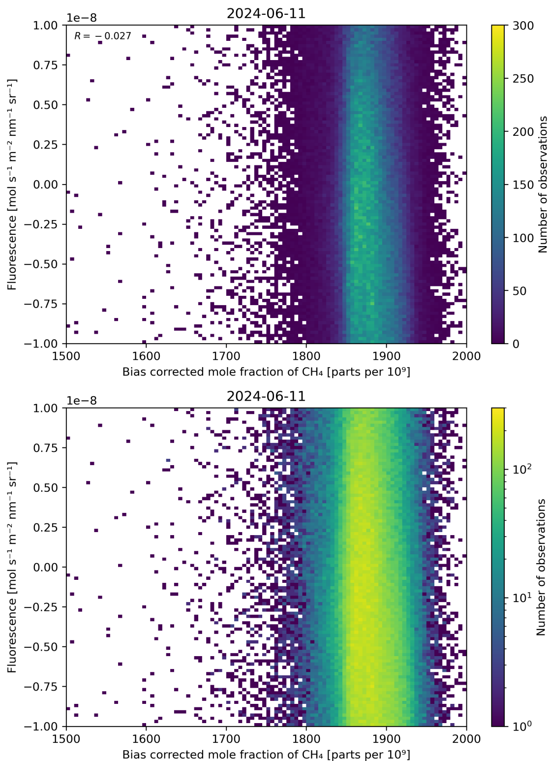
Figure 66: Scatter density plot of “Bias corrected mole fraction of \text{CH}_4 ” against “Fluorescence” for 2024-06-10 to 2024-06-12.
