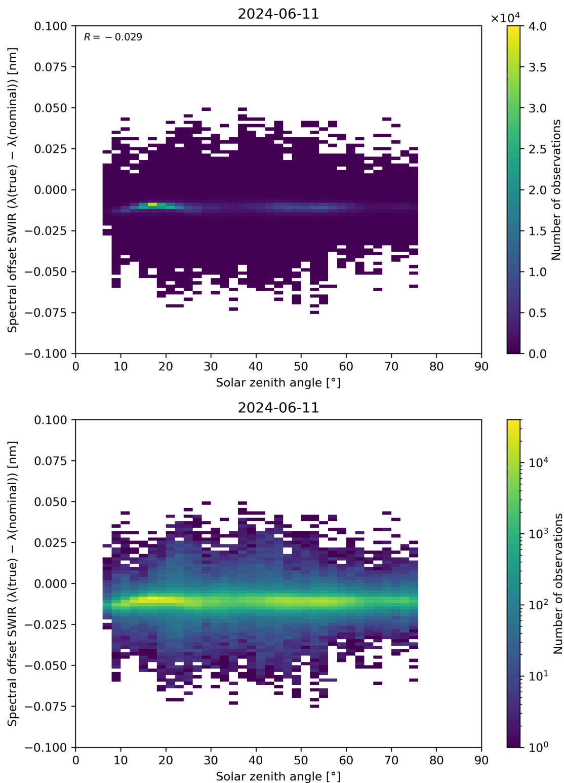
Figure 104: Scatter density plot of “Solar zenith angle” against “Spectral offset SWIR ( \lambda(\text{true}) - \lambda(\text{nominal}) )” for 2024-06-10 to 2024-06-12.
