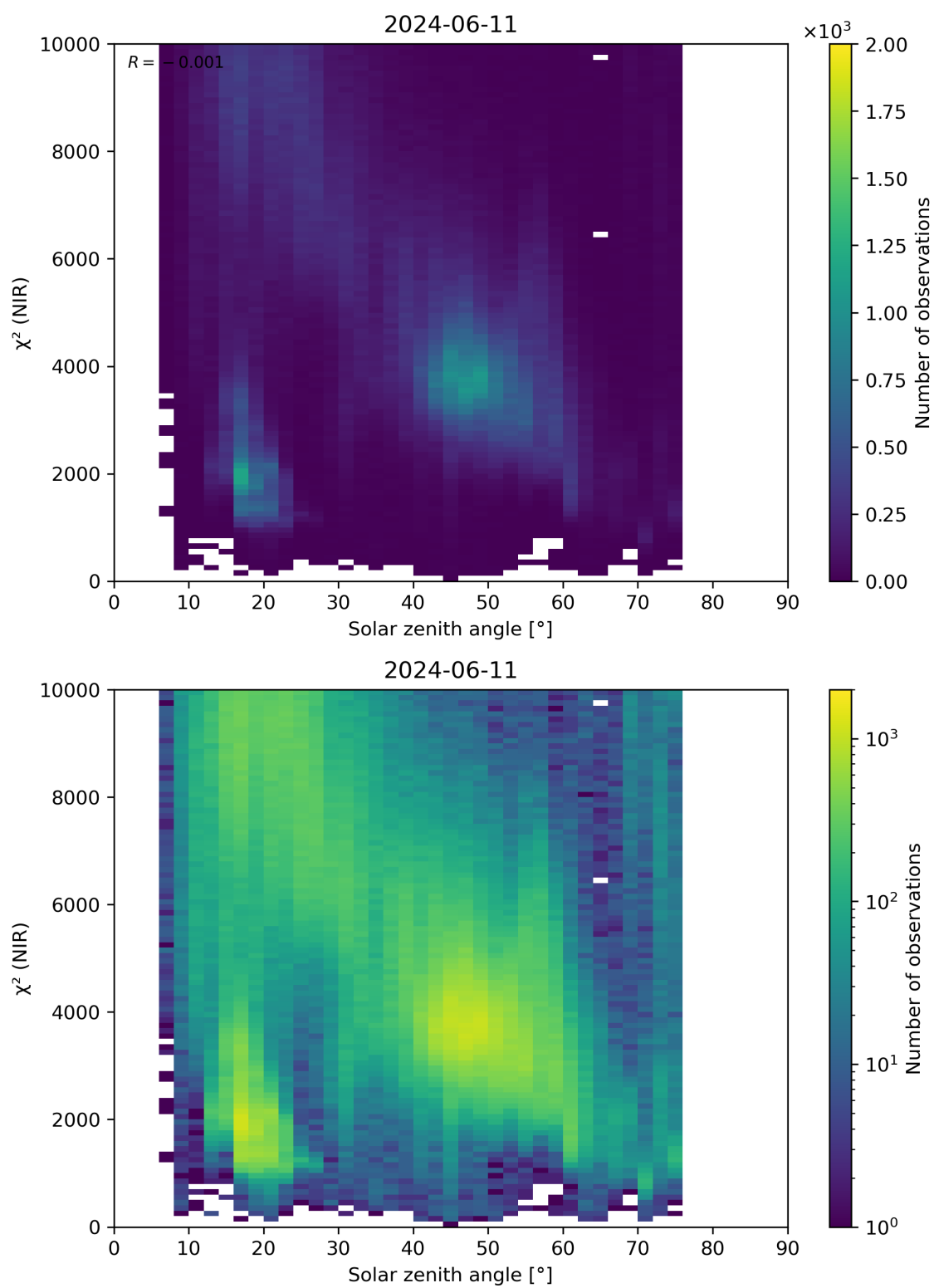
Figure 94: Scatter density plot of “Solar zenith angle” against “ \chi^2 (NIR)” for 2024-06-10 to 2024-06-12.
