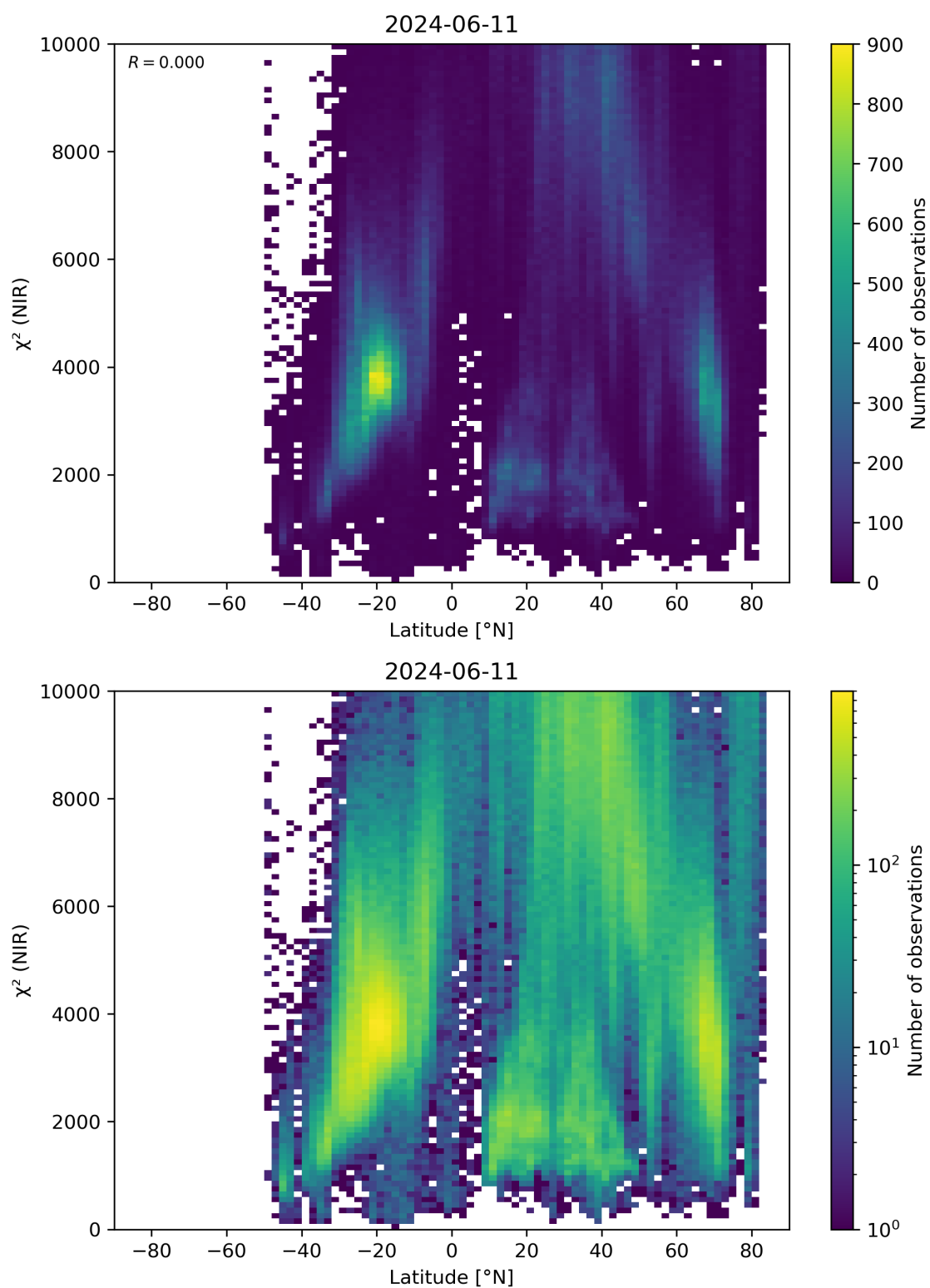
Figure 53: Scatter density plot of “Latitude” against “ \chi^2 (NIR)” for 2024-06-10 to 2024-06-12.
