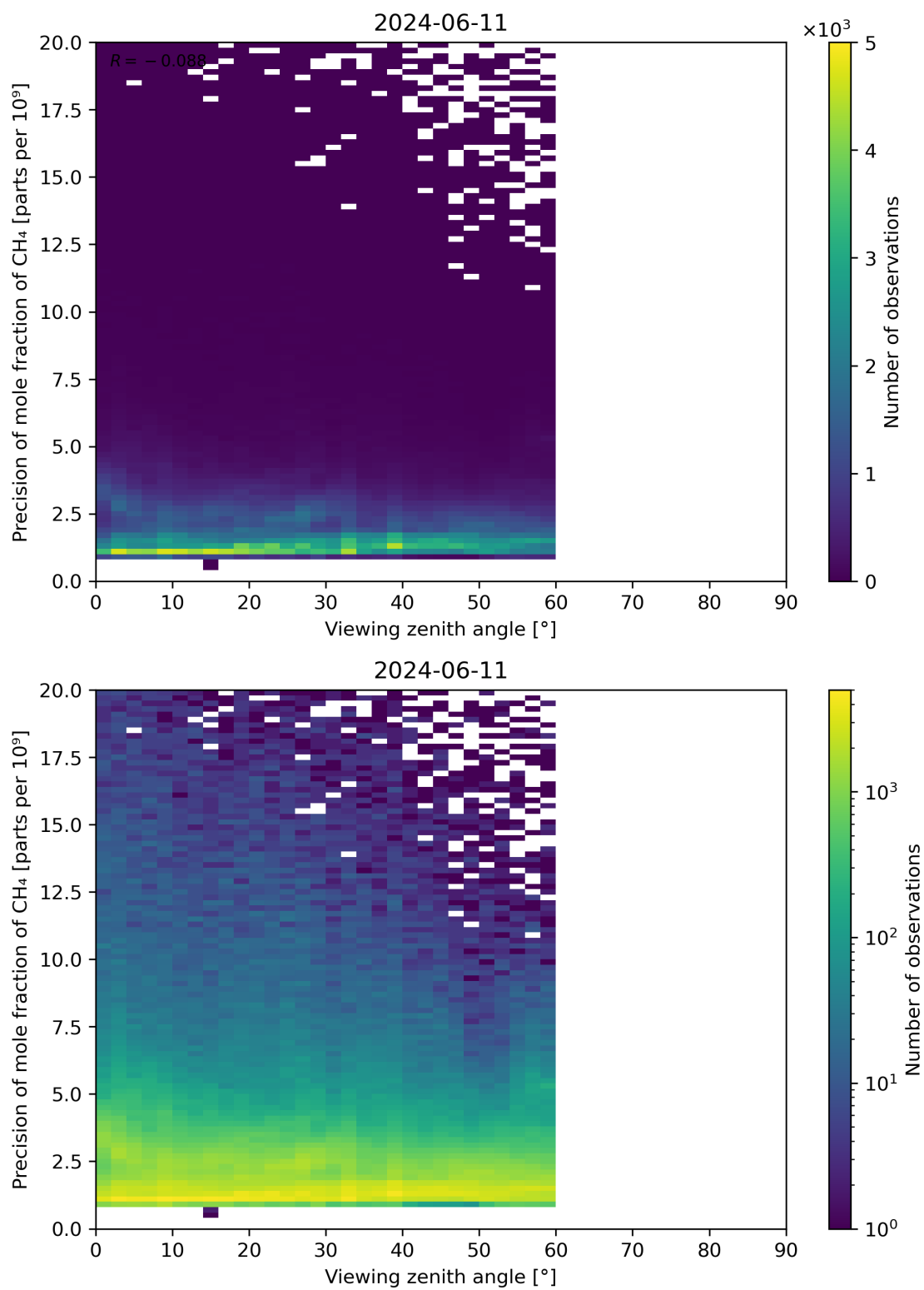
Figure 112: Scatter density plot of “Viewing zenith angle” against “Precision of mole fraction of CH 4 ” for 2024-06-10 to 2024-06-12.
