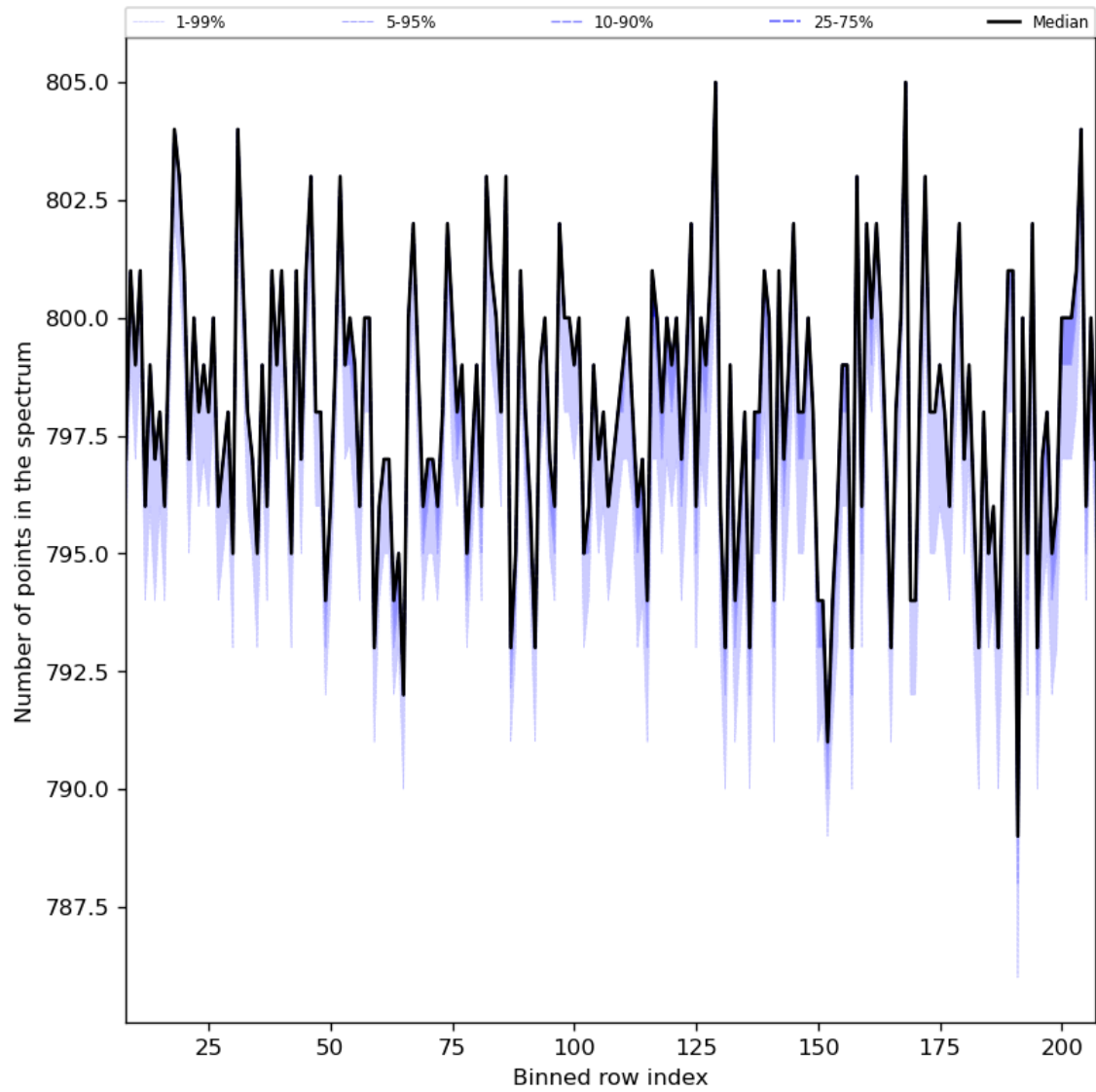
Figure 37: Along track statistics of “Number of points in the spectrum” for 2024-06-10 to 2024-06-12
