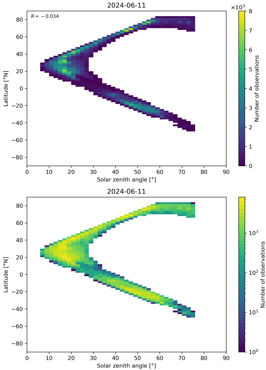
Figure 98: Scatter density plot of “Solar zenith angle” against “Latitude” for 2024-06-10 to 2024-06-12.
