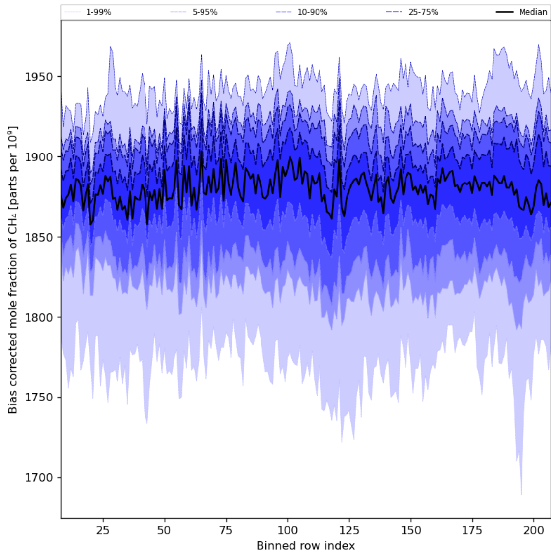
Figure 36: Along track statistics of “Bias corrected mole fraction of CH 4 ” for 2024-06-10 to 2024-06-12
