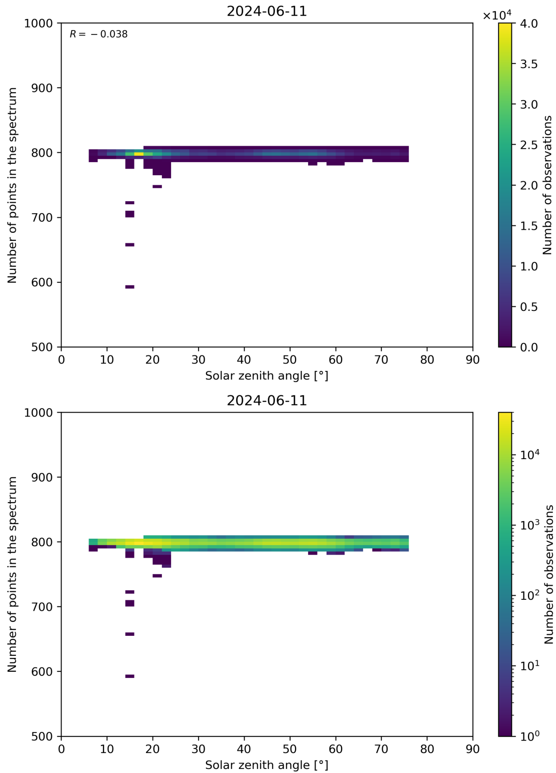
Figure 103: Scatter density plot of “Solar zenith angle” against “Number of points in the spectrum” for 2024-06-10 to 2024-06-12.
