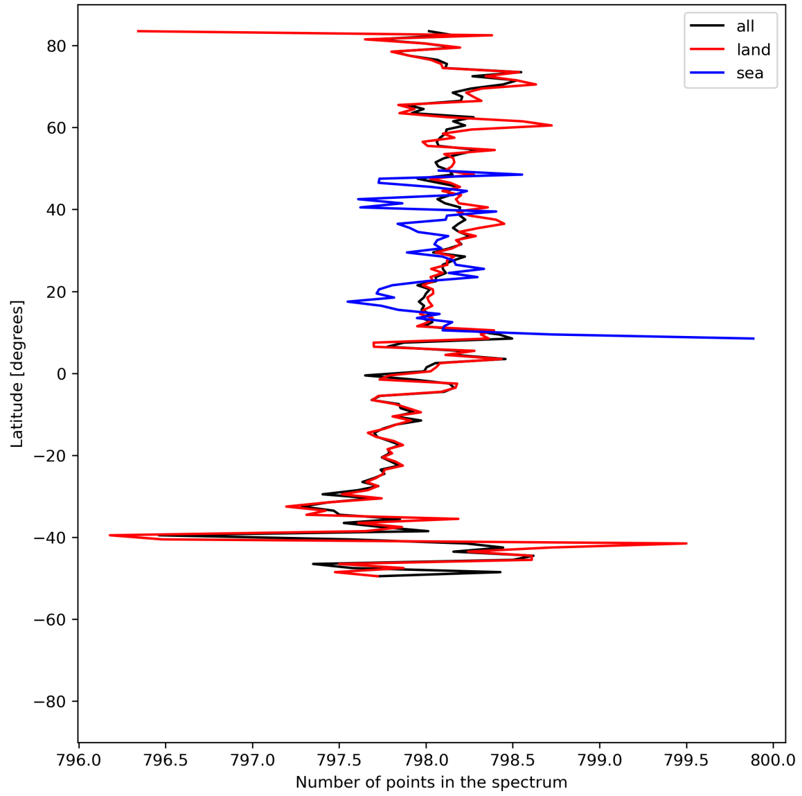
Figure 15: Zonal average of “Number of points in the spectrum” for 2024-06-10 to 2024-06-12.
