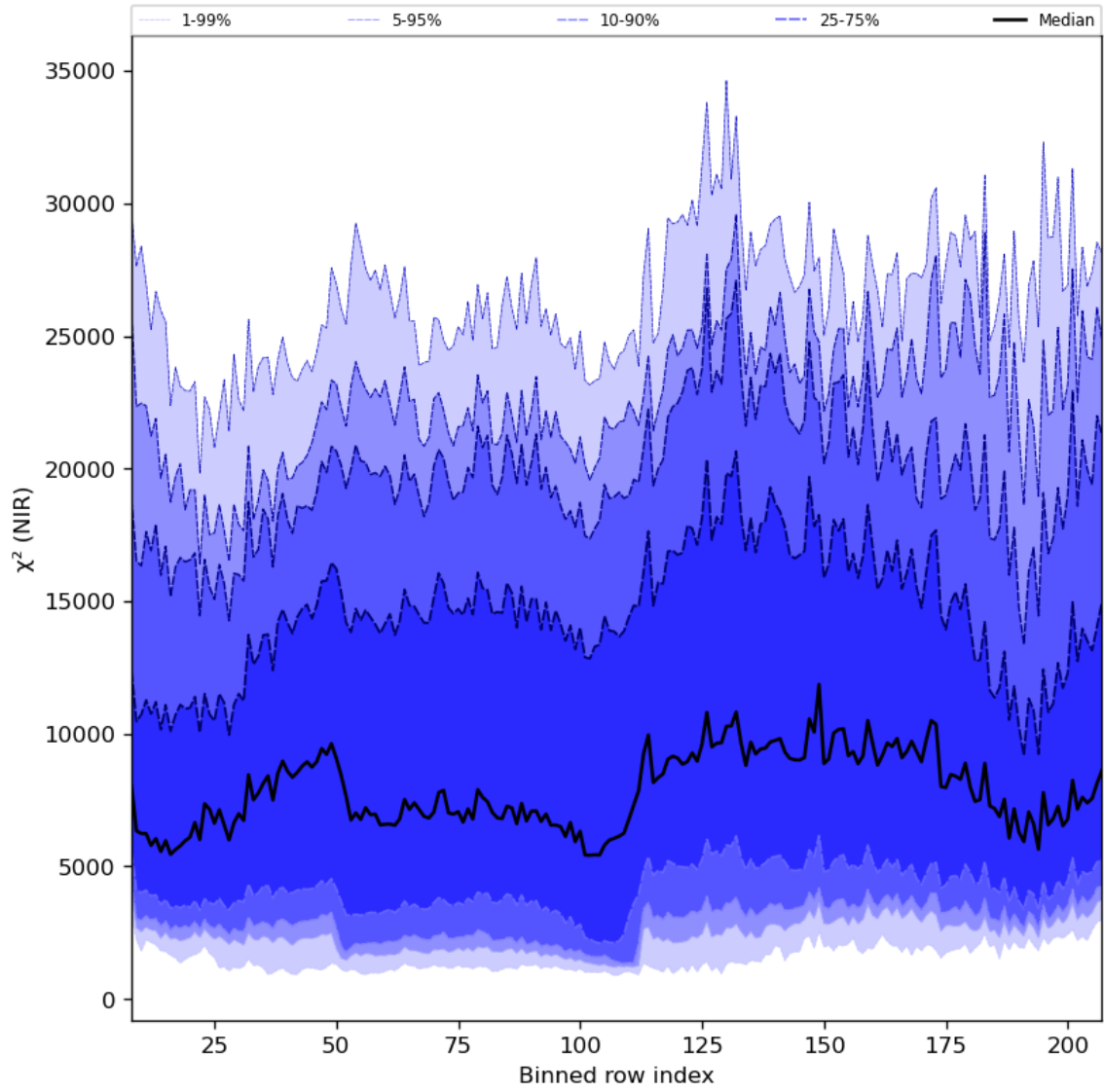
Figure 40: Along track statistics of “ \chi^2 (NIR)” for 2024-06-10 to 2024-06-12
