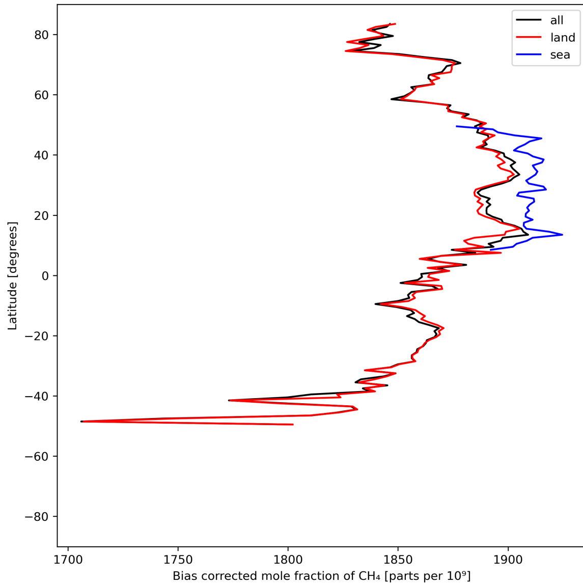
Figure 14: Zonal average of “Bias corrected mole fraction of CH 4 ” for 2024-06-10 to 2024-06-12.
