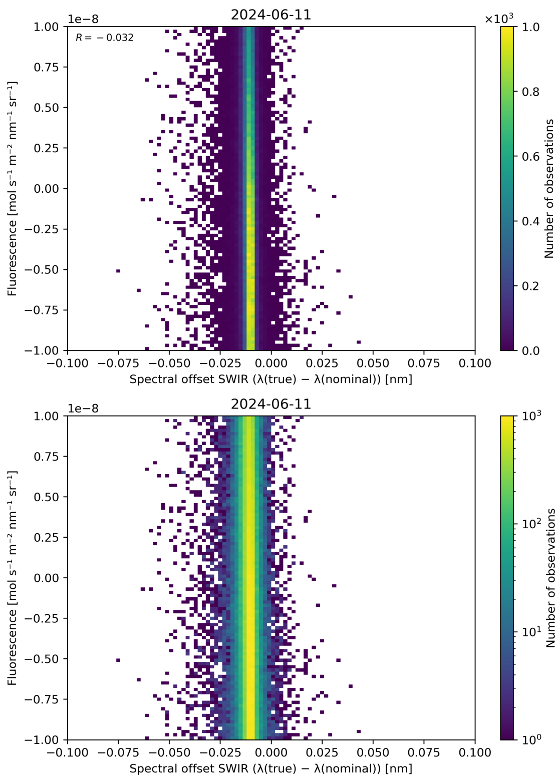
Figure 120: Scatter density plot of “Spectral offset SWIR ( \lambda(\text{true}) - \lambda(\text{nominal}) )” against “Fluorescence” for 2024-06-10 to 2024-06-12.
