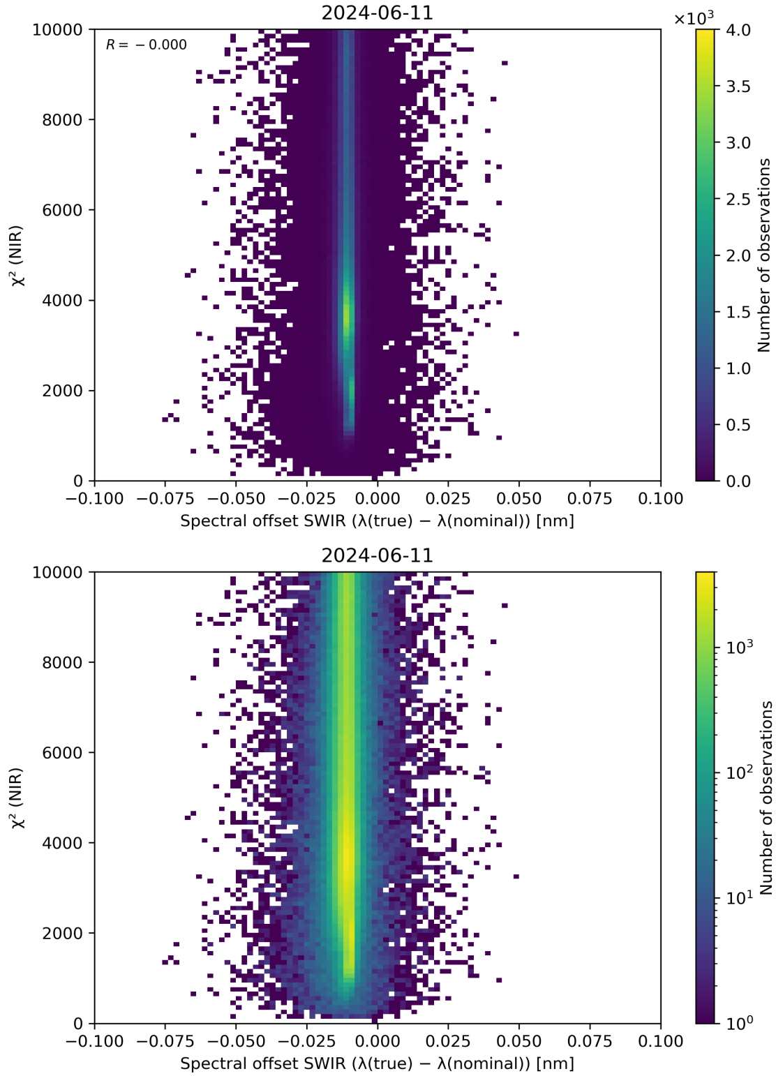
Figure 117: Scatter density plot of “Spectral offset SWIR ( \lambda(\text{true}) - \lambda(\text{nominal}) )” against “ \chi^2 (NIR)” for 2024-06-10 to 2024-06-12.
