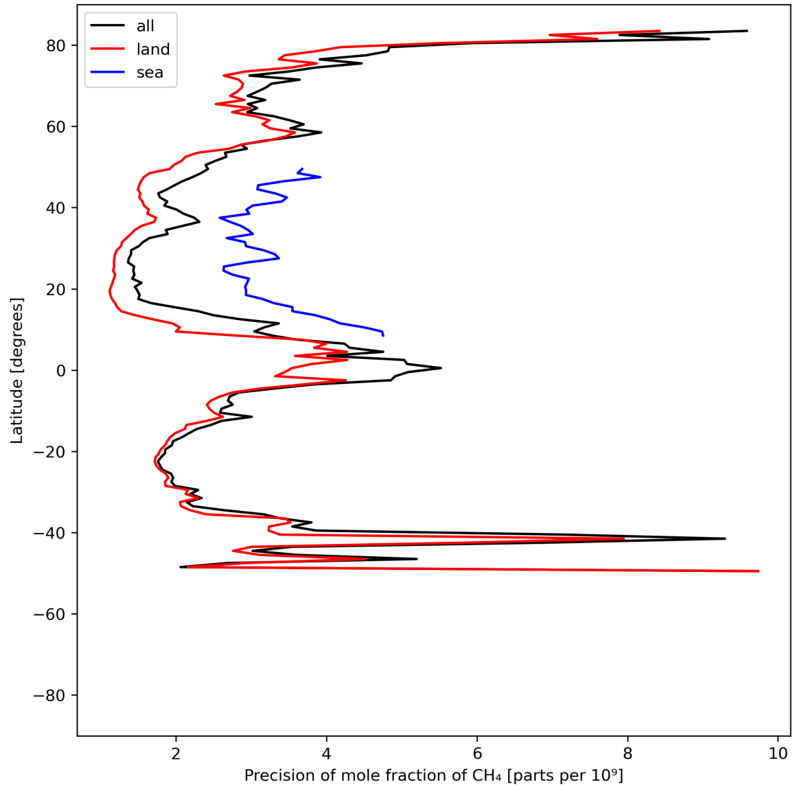
Figure 13: Zonal average of “Precision of mole fraction of CH 4 ” for 2024-06-10 to 2024-06-12.
