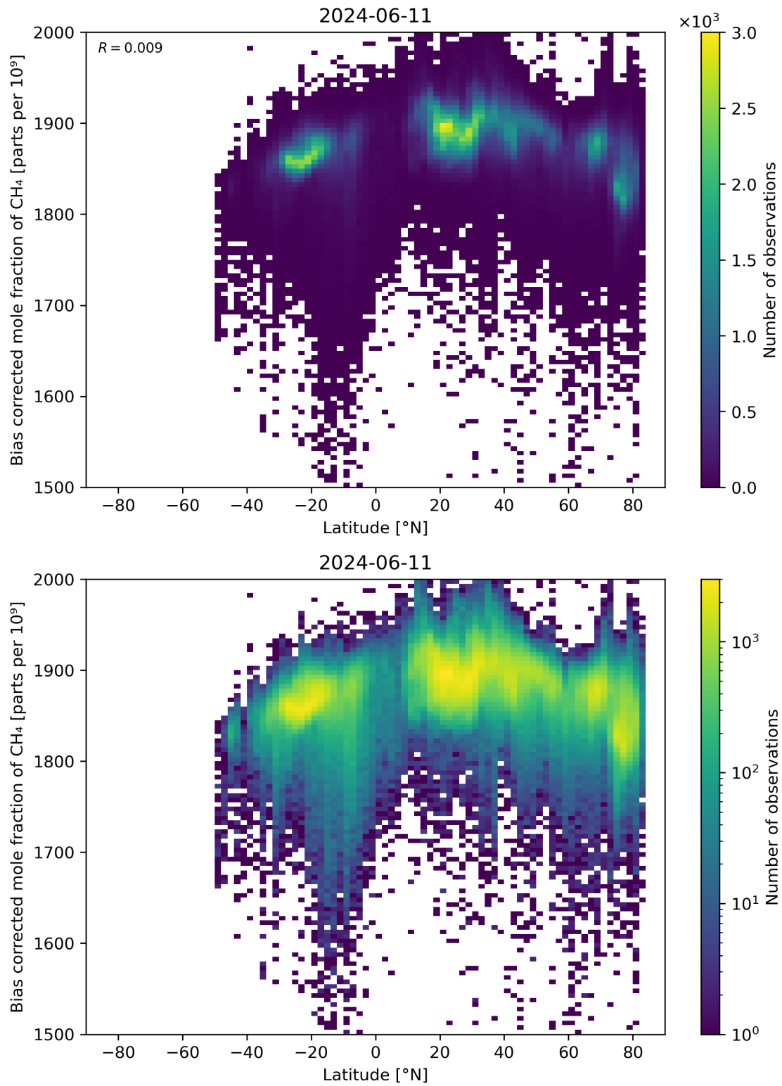
Figure 58: Scatter density plot of “Latitude” against “Bias corrected mole fraction of CH 4 ” for 2024-06-10 to 2024-06-12.
