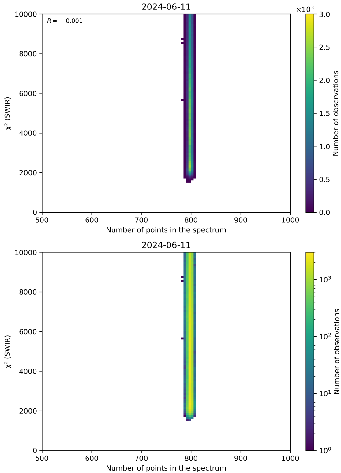
Figure 89: Scatter density plot of “Number of points in the spectrum” against “ \chi^2 (SWIR)” for 2024-06-10 to 2024-06-12.
