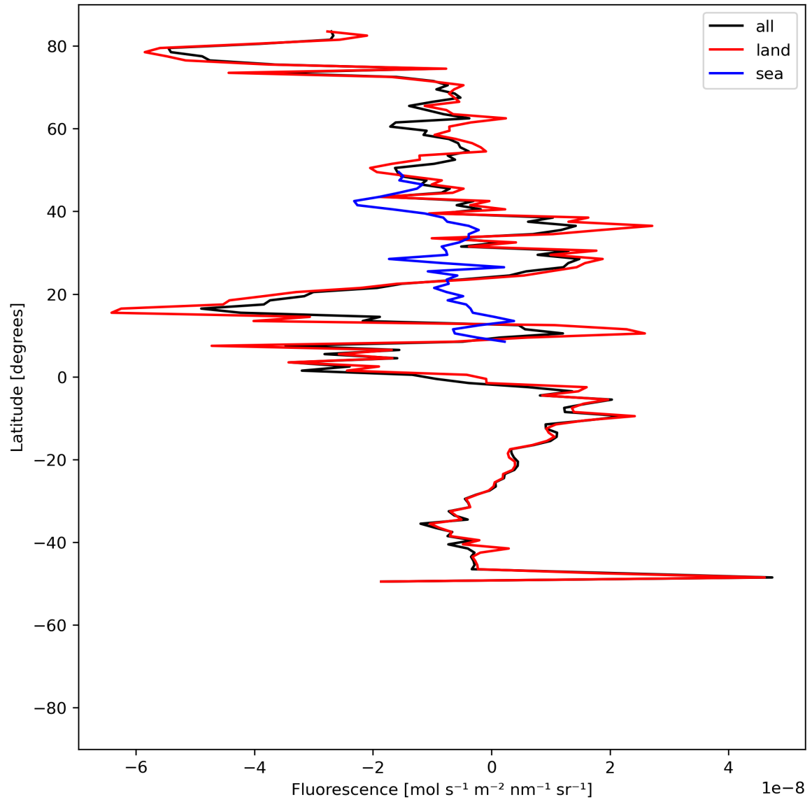
Figure 21: Zonal average of “Fluorescence” for 2024-06-10 to 2024-06-12.
