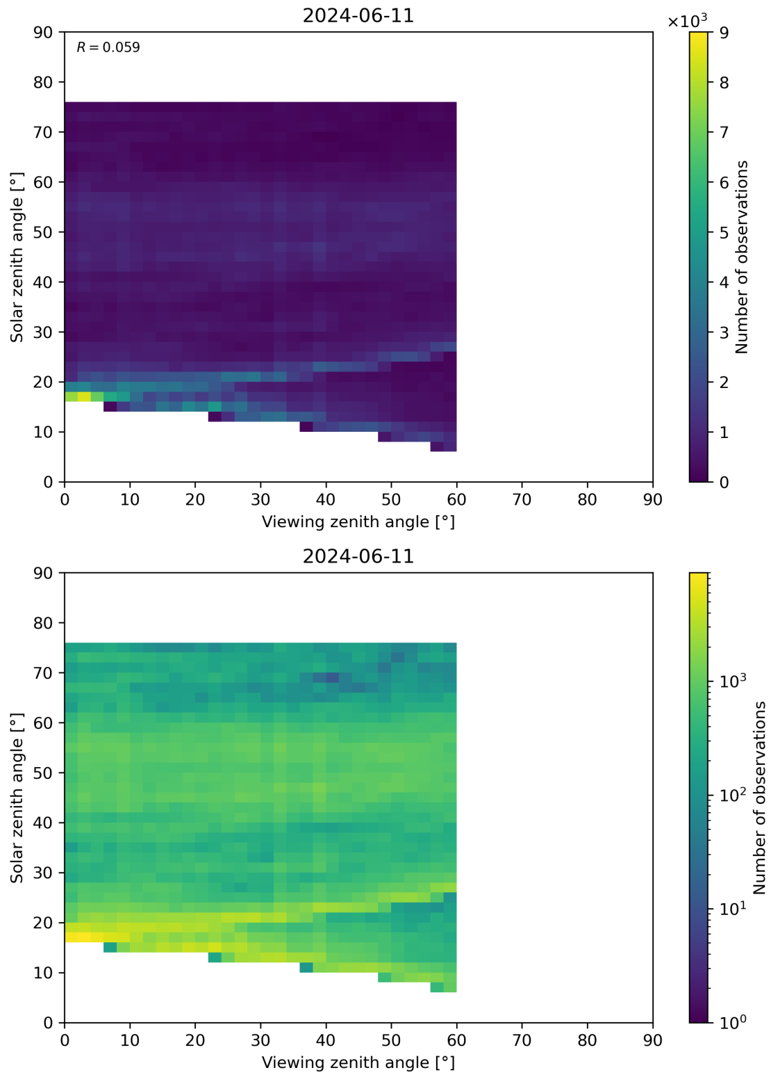
Figure 115: Scatter density plot of “Viewing zenith angle” against “Solar zenith angle” for 2024-06-10 to 2024-06-12.
