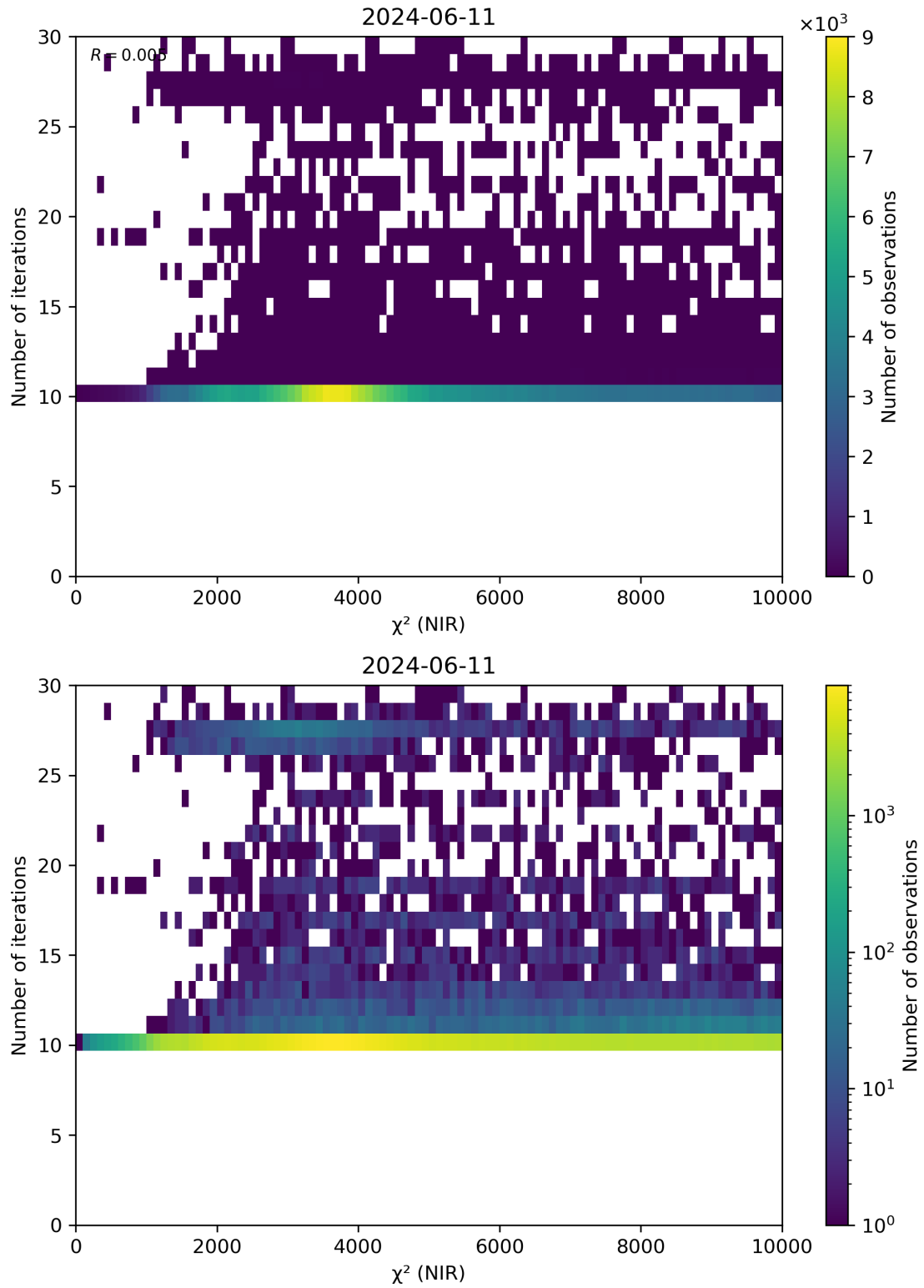
Figure 46: Scatter density plot of “ \chi^2 (NIR)” against “Number of iterations” for 2024-06-10 to 2024-06-12.
