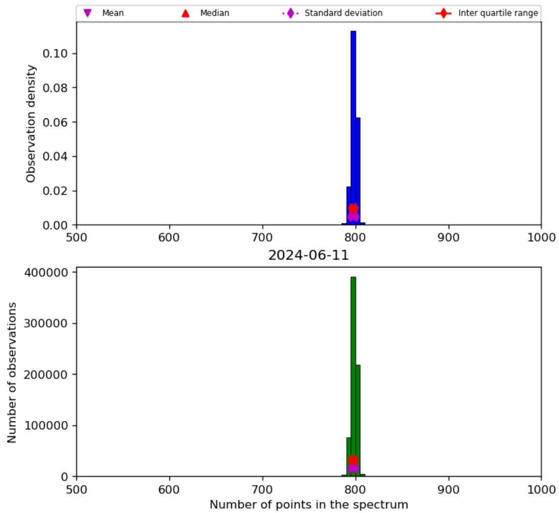
Figure 26: Histogram of “Number of points in the spectrum” for 2024-06-10 to 2024-06-12
