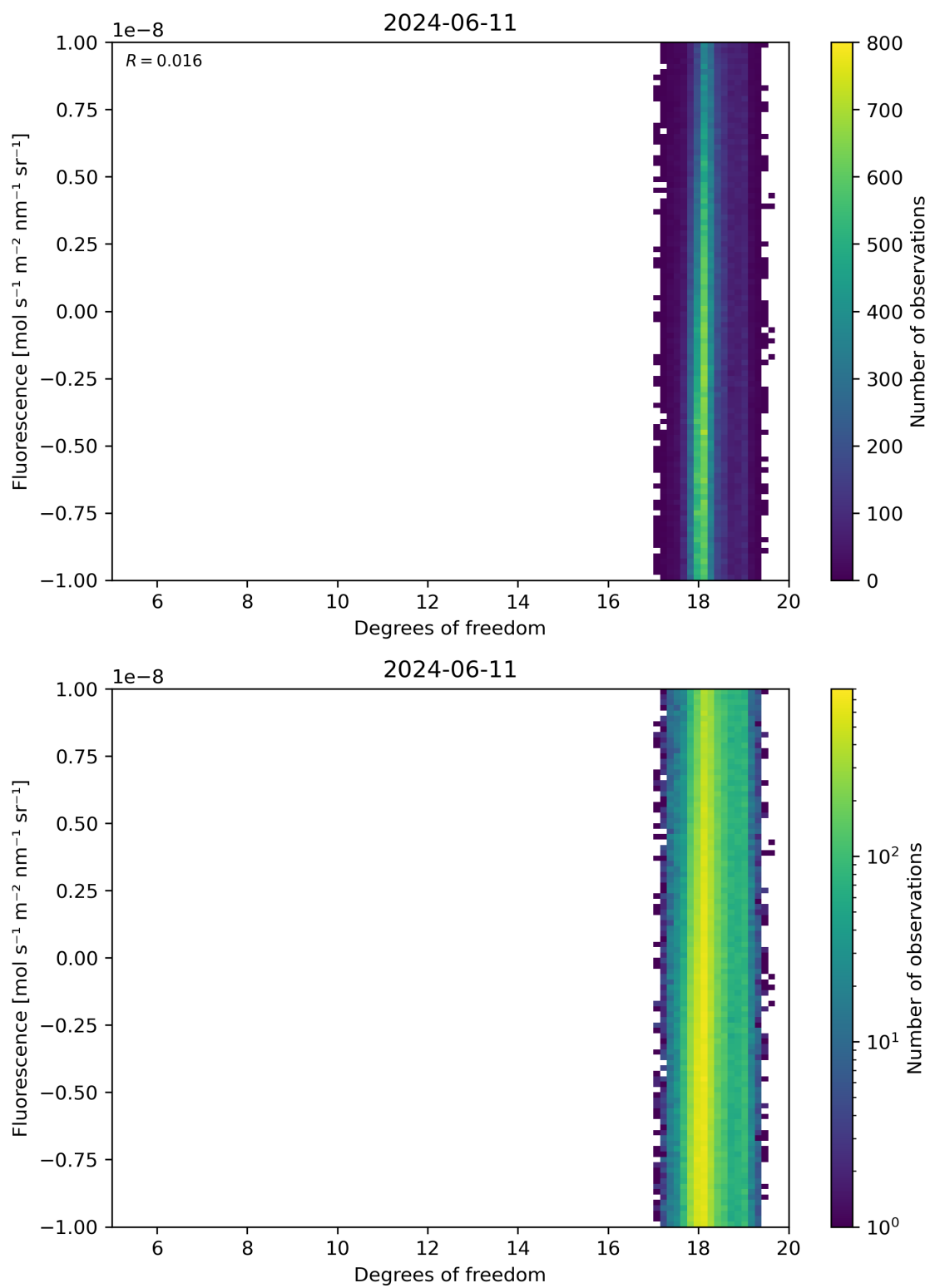
Figure 51: Scatter density plot of “Degrees of freedom” against “Fluorescence” for 2024-06-10 to 2024-06-12.
