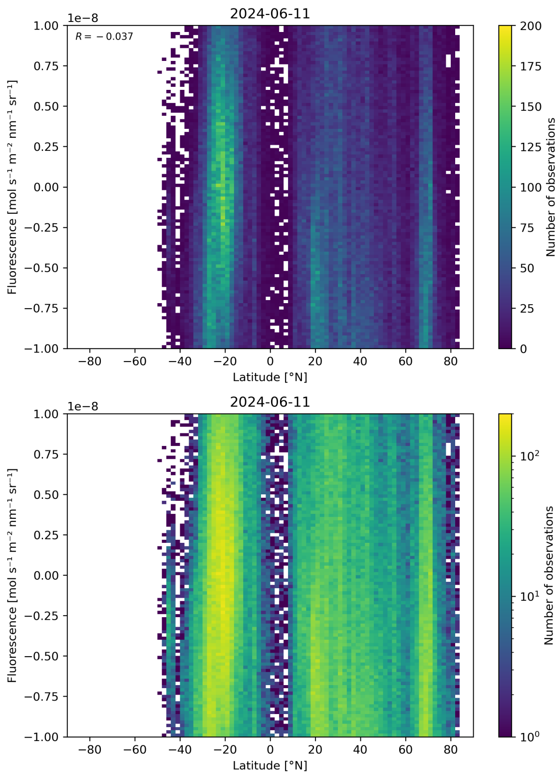
Figure 56: Scatter density plot of “Latitude” against “Fluorescence” for 2024-06-10 to 2024-06-12.
