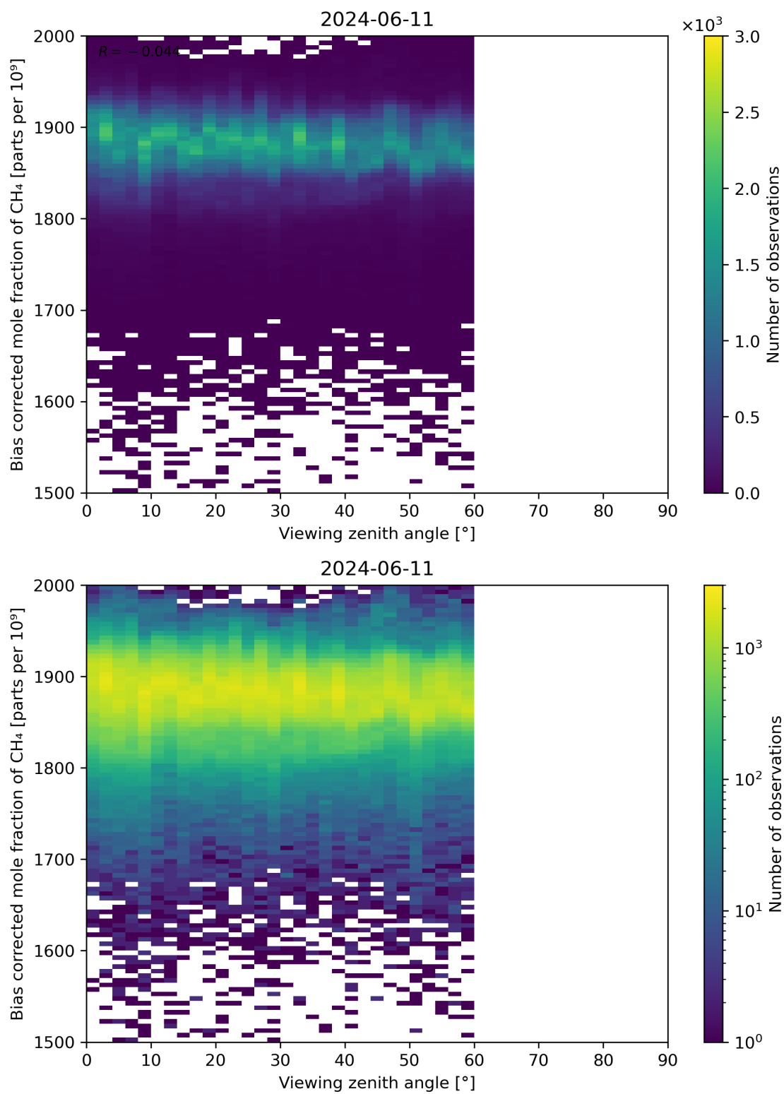
Figure 111: Scatter density plot of “Viewing zenith angle” against “Bias corrected mole fraction of CH 4 ” for 2024-06-10 to 2024-06-12.
