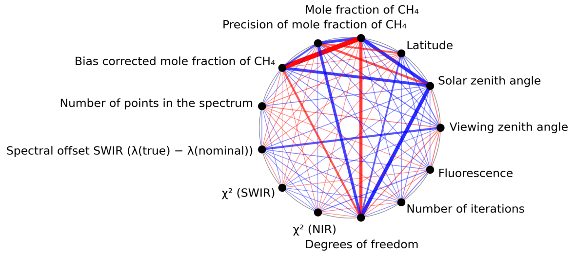
Figure 1: Map of correlation graph for 2024-06-10 to 2024-06-12.
