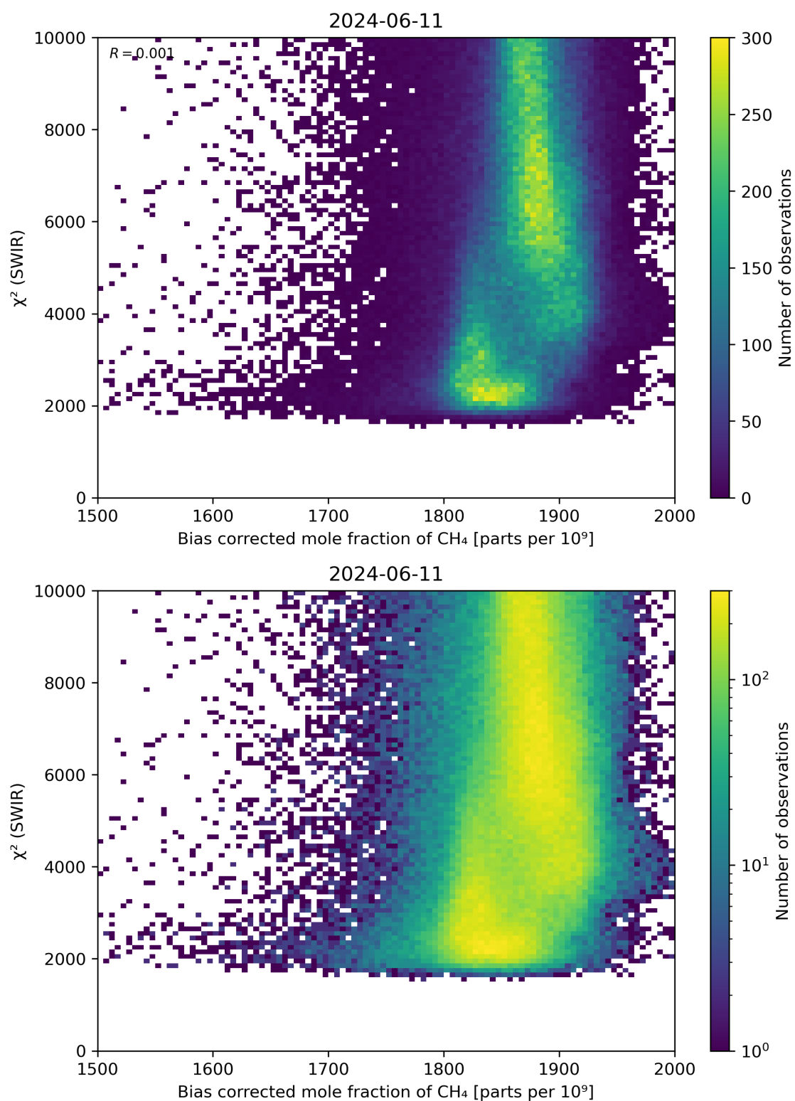
Figure 64: Scatter density plot of “Bias corrected mole fraction of \text{CH}_4 ” against “ \chi^2 (SWIR)” for 2024-06-10 to 2024-06-12.
