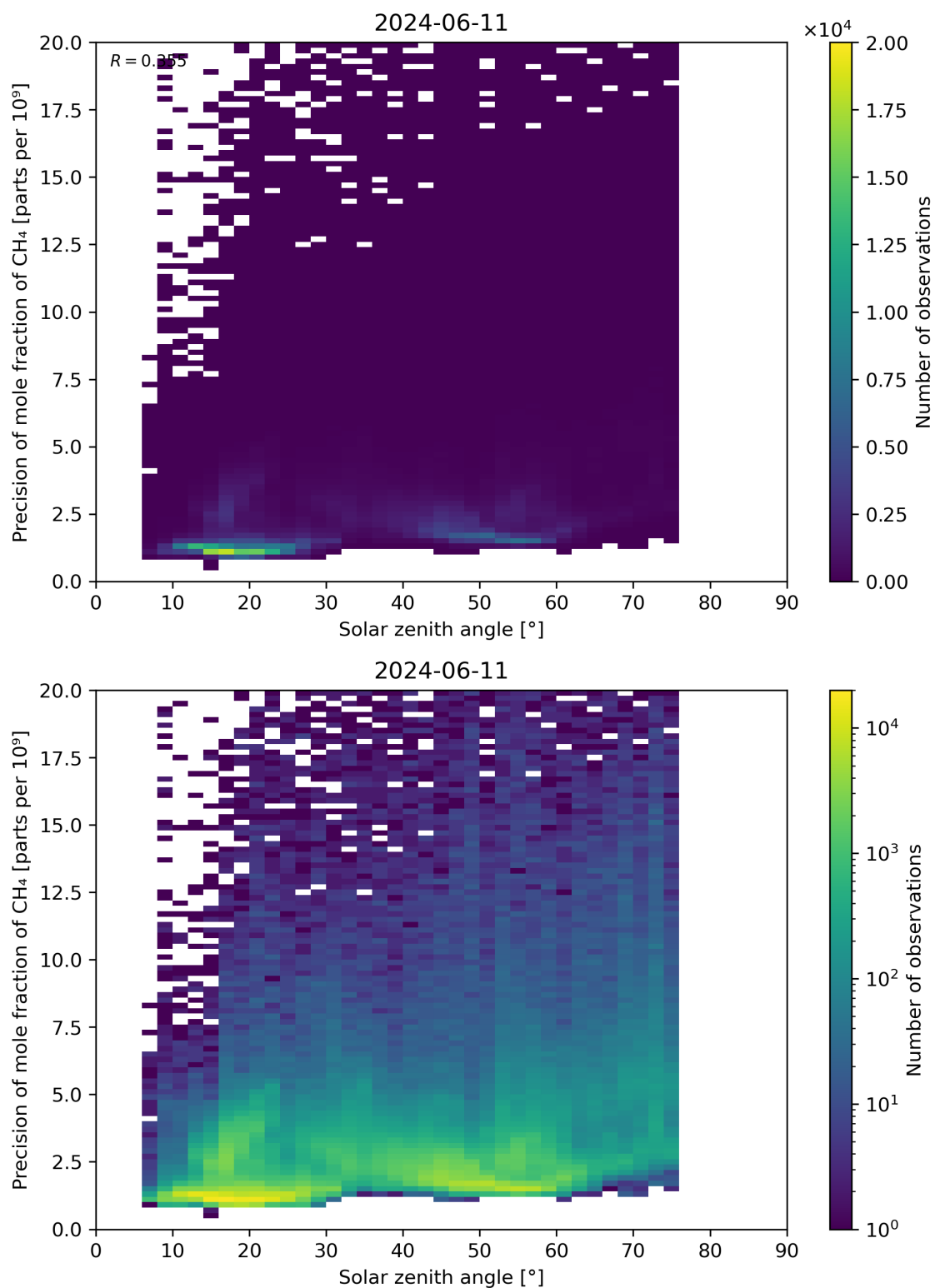
Figure 101: Scatter density plot of “Solar zenith angle” against “Precision of mole fraction of CH 4 ” for 2024-06-10 to 2024-06-12.
