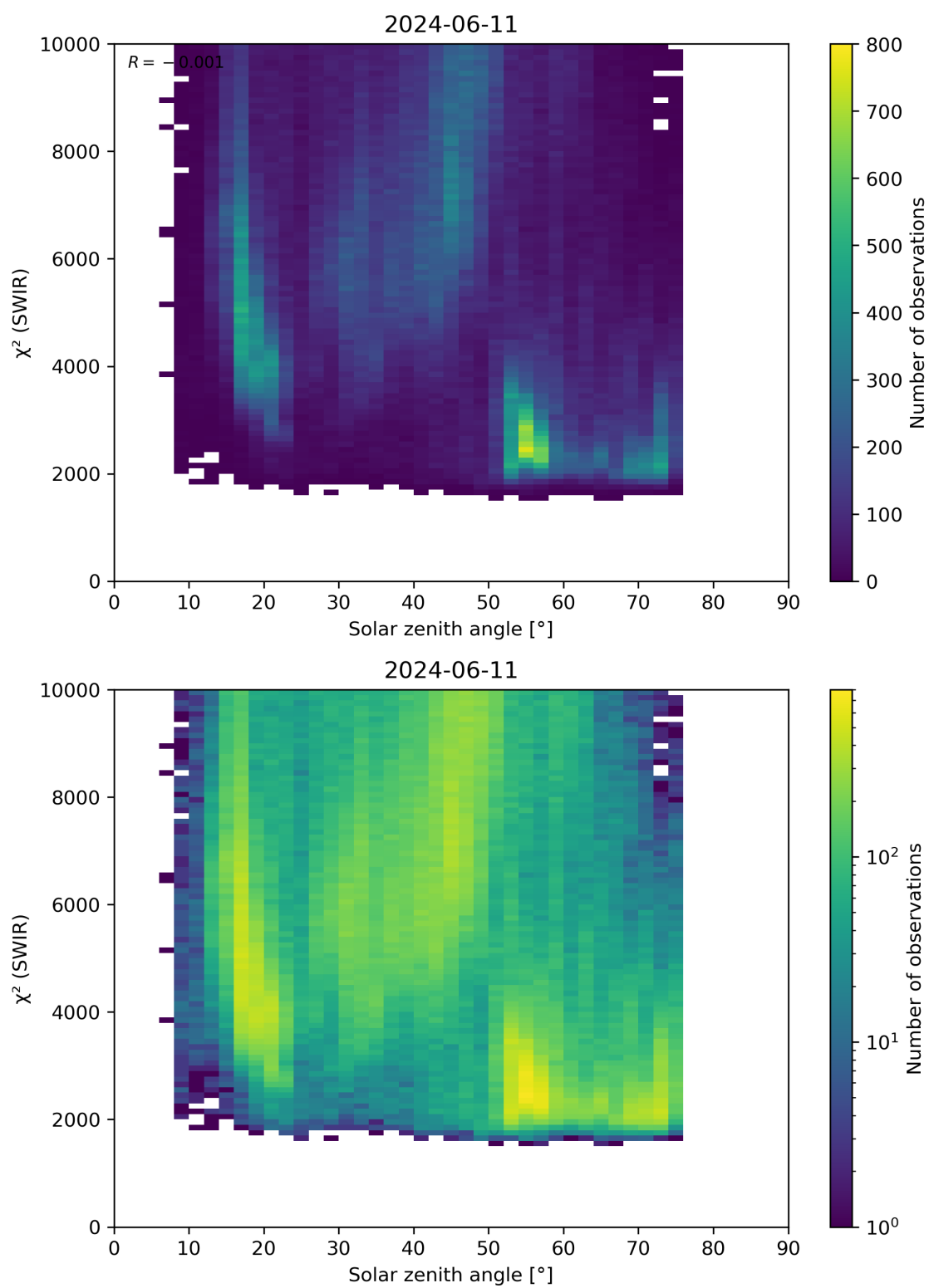
Figure 95: Scatter density plot of “Solar zenith angle” against “ \chi^2 (SWIR)” for 2024-06-10 to 2024-06-12.
