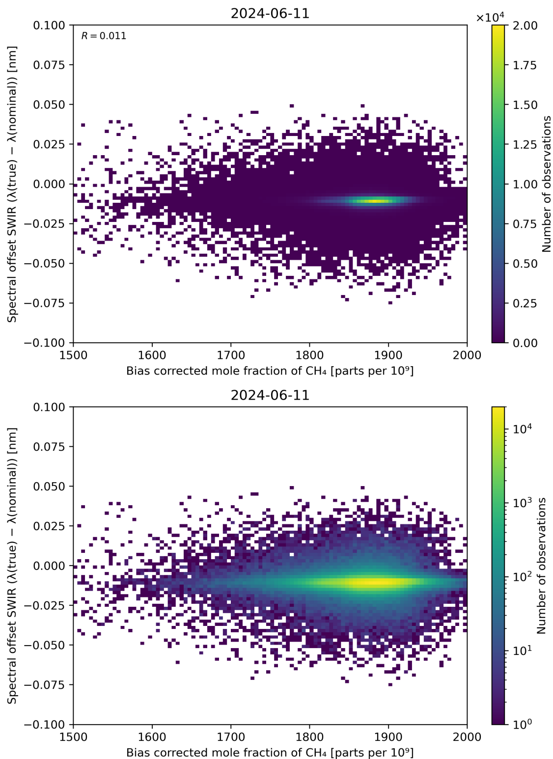
Figure 69: Scatter density plot of “Bias corrected mole fraction of \text{CH}_4 ” against “Spectral offset SWIR ( \lambda(\text{true}) - \lambda(\text{nominal}) )” for 2024-06-10 to 2024-06-12.
