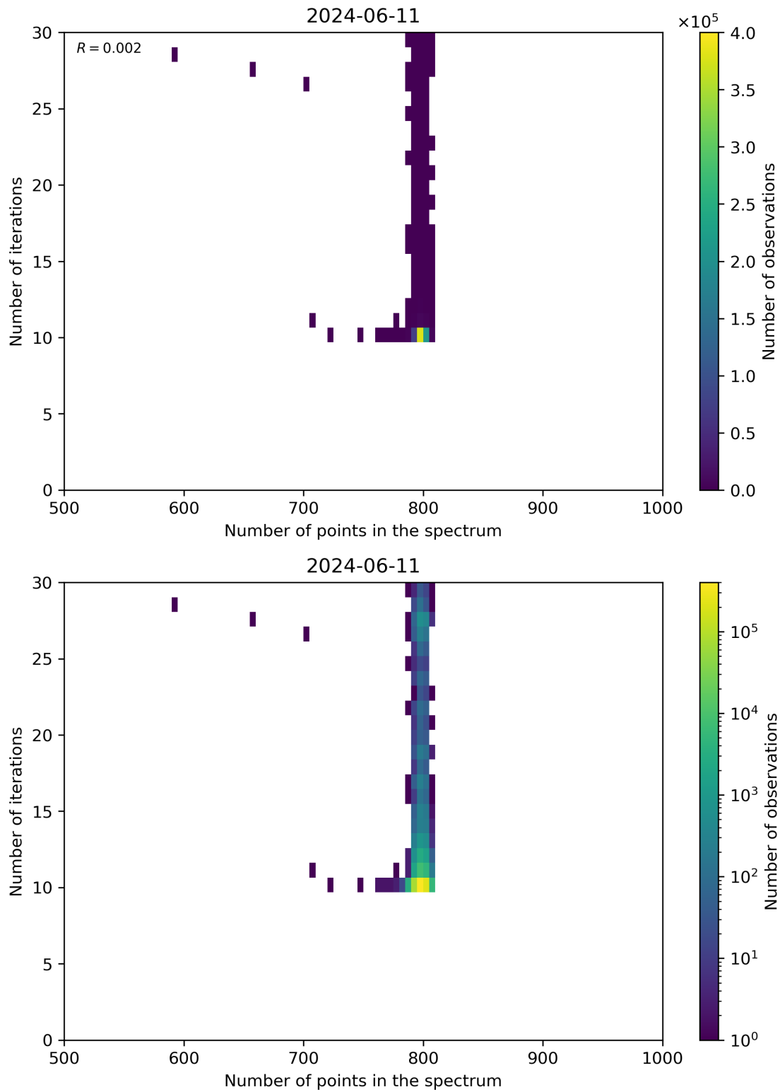
Figure 92: Scatter density plot of “Number of points in the spectrum” against “Number of iterations” for 2024-06-10 to 2024-06-12.
