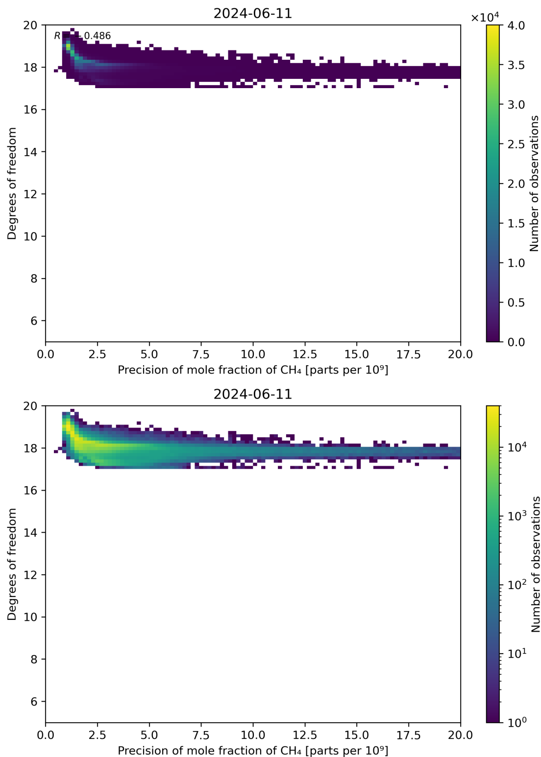
Figure 80: Scatter density plot of “Precision of mole fraction of CH 4 ” against “Degrees of freedom” for 2024-06-10 to 2024-06-12.
