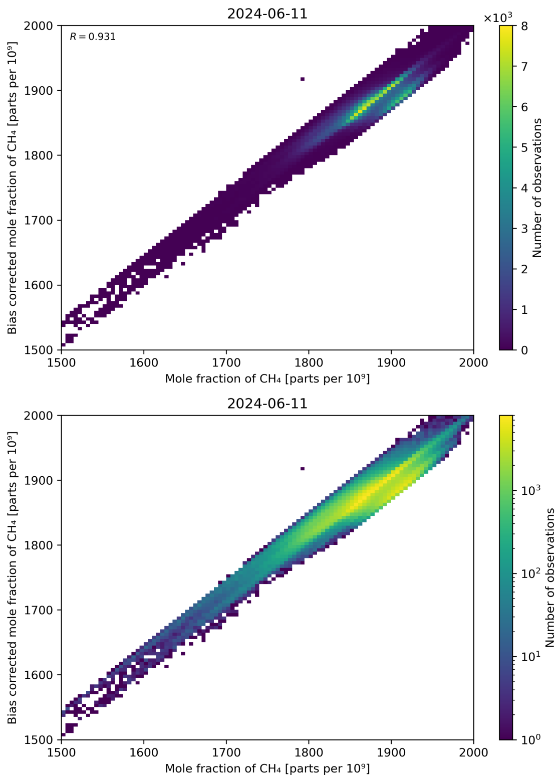
Figure 74: Scatter density plot of “Mole fraction of CH 4 ” against “Bias corrected mole fraction of CH 4 ” for 2024-06-10 to 2024-06-12.
