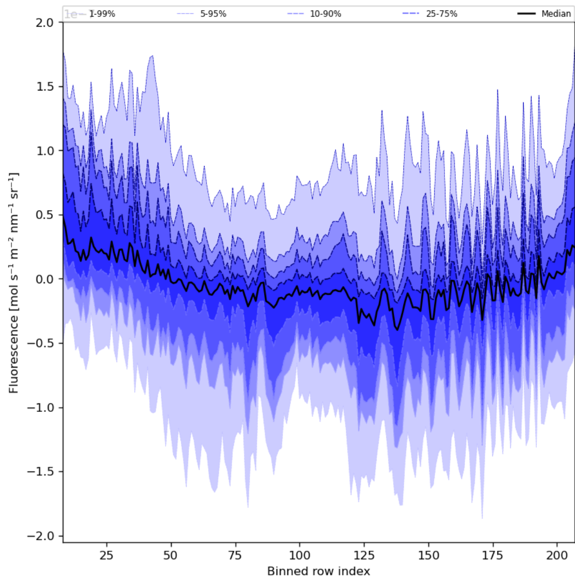
Figure 43: Along track statistics of “Fluorescence” for 2024-06-10 to 2024-06-12
