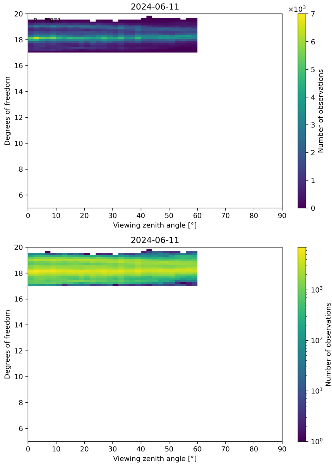
Figure 107: Scatter density plot of “Viewing zenith angle” against “Degrees of freedom” for 2024-06-10 to 2024-06-12.
