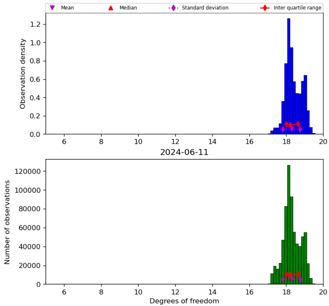
Figure 30: Histogram of “Degrees of freedom” for 2024-06-10 to 2024-06-12
