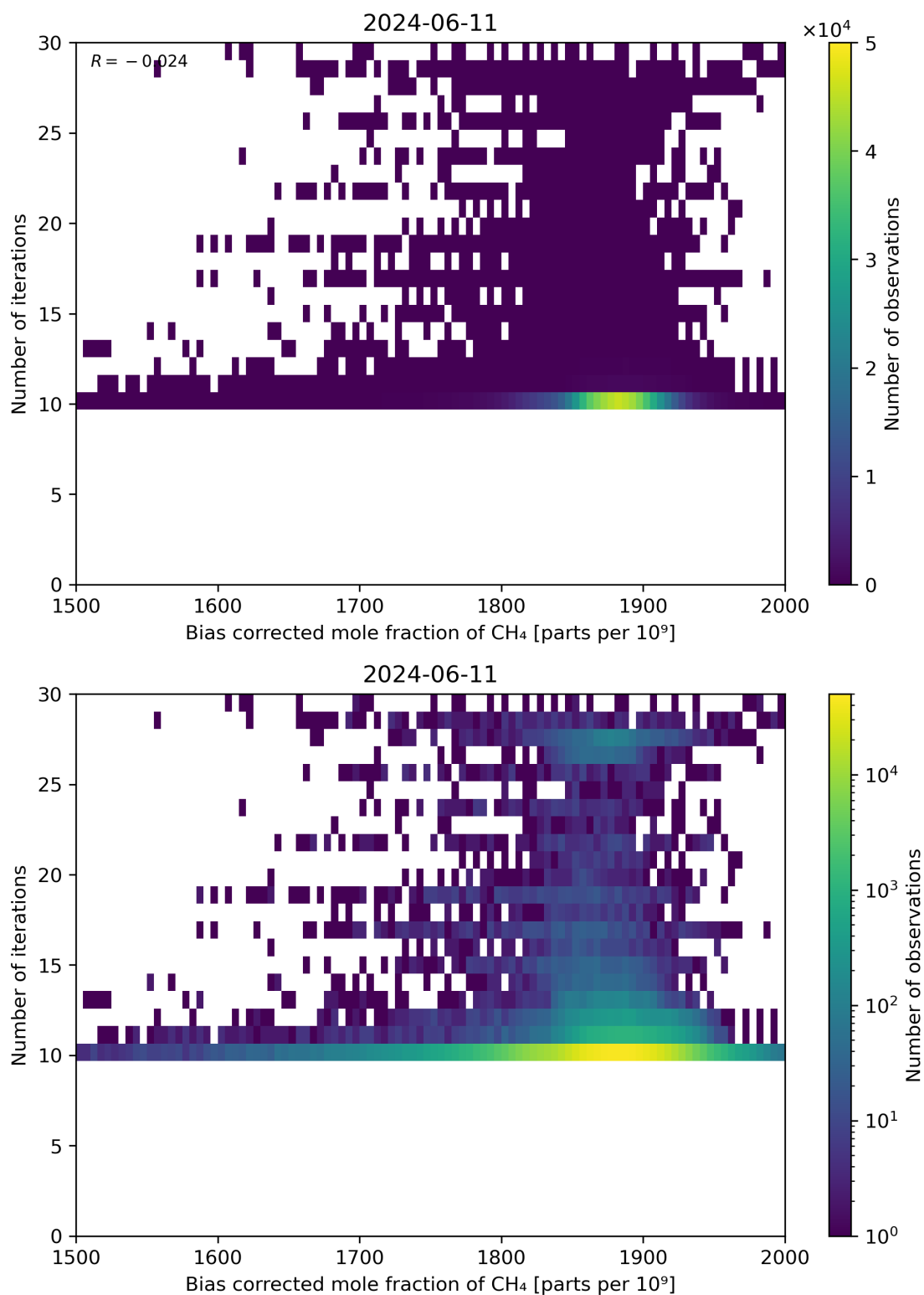
Figure 67: Scatter density plot of “Bias corrected mole fraction of CH 4 ” against “Number of iterations” for 2024-06-10 to 2024-06-12.
