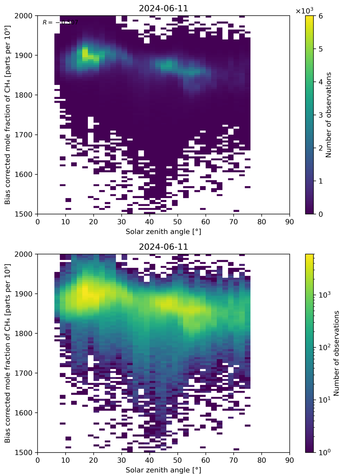
Figure 100: Scatter density plot of “Solar zenith angle” against “Bias corrected mole fraction of CH 4 ” for 2024-06-10 to 2024-06-12.
