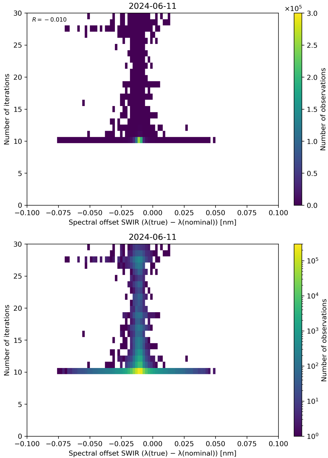
Figure 121: Scatter density plot of “Spectral offset SWIR ( \lambda(\text{true}) - \lambda(\text{nominal}) )” against “Number of iterations” for 2024-06-10 to 2024-06-12.
