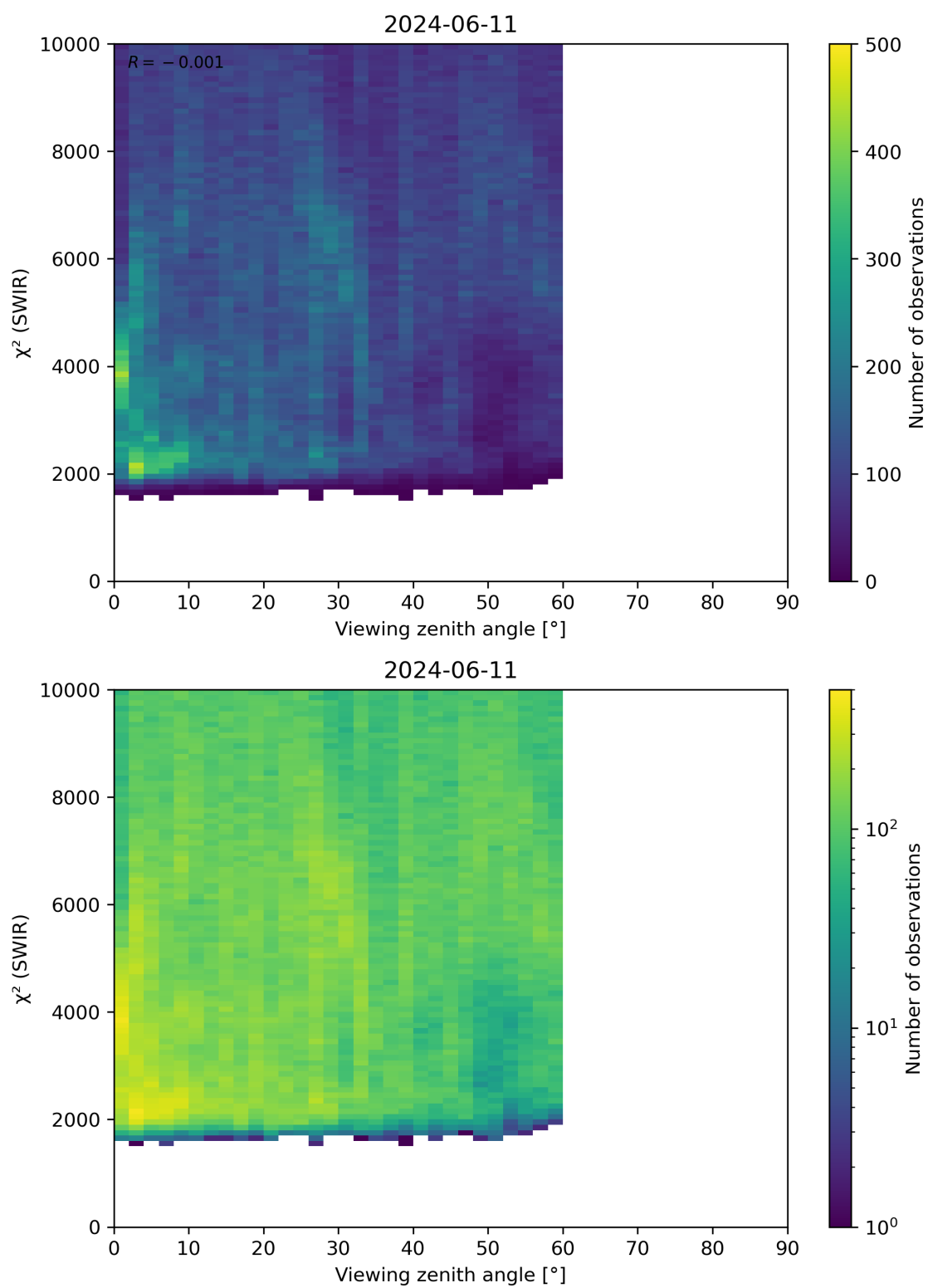
Figure 106: Scatter density plot of “Viewing zenith angle” against “ \chi^2 (SWIR)” for 2024-06-10 to 2024-06-12.
