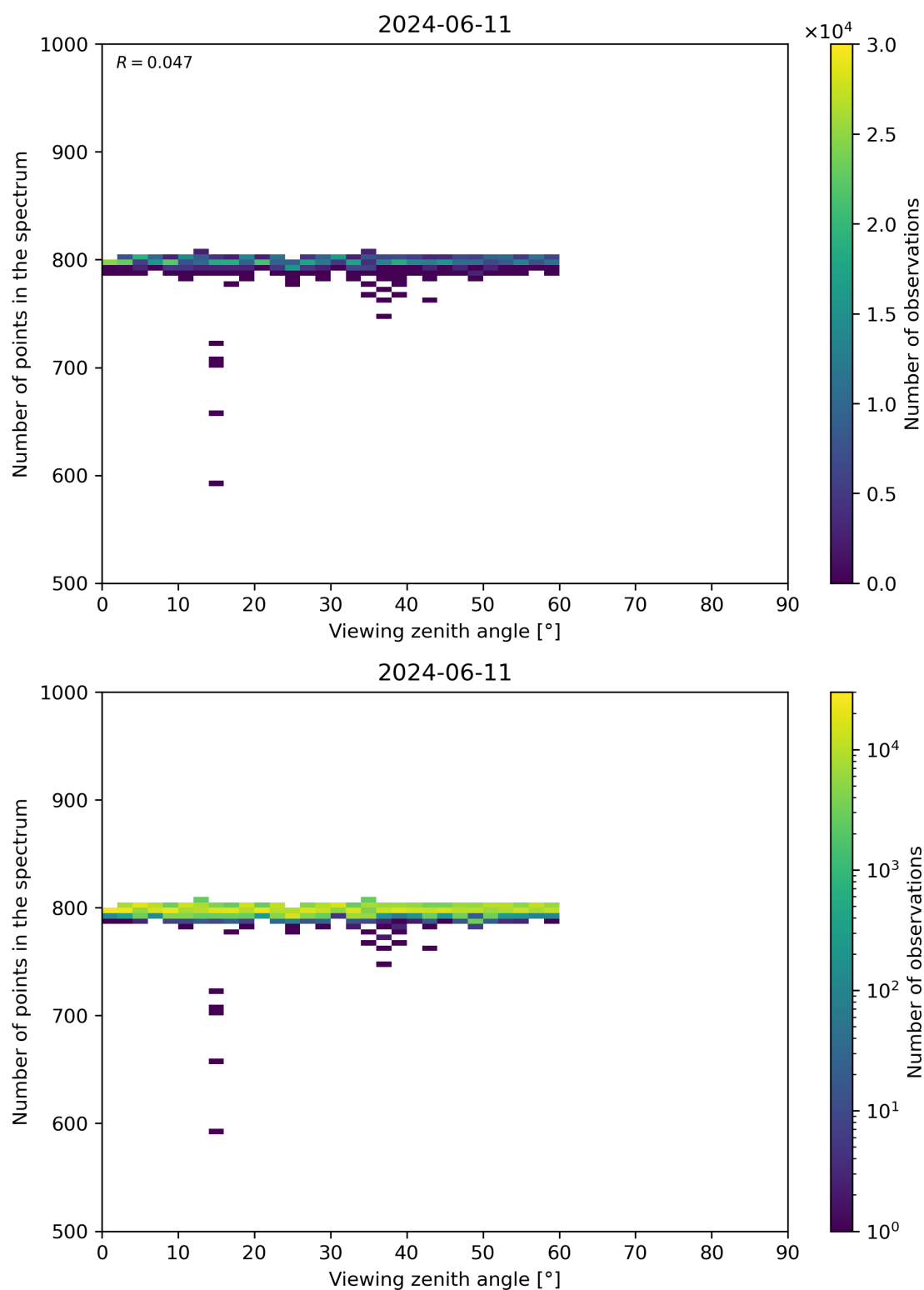
Figure 114: Scatter density plot of “Viewing zenith angle” against “Number of points in the spectrum” for 2024-06-10 to 2024-06-12.
