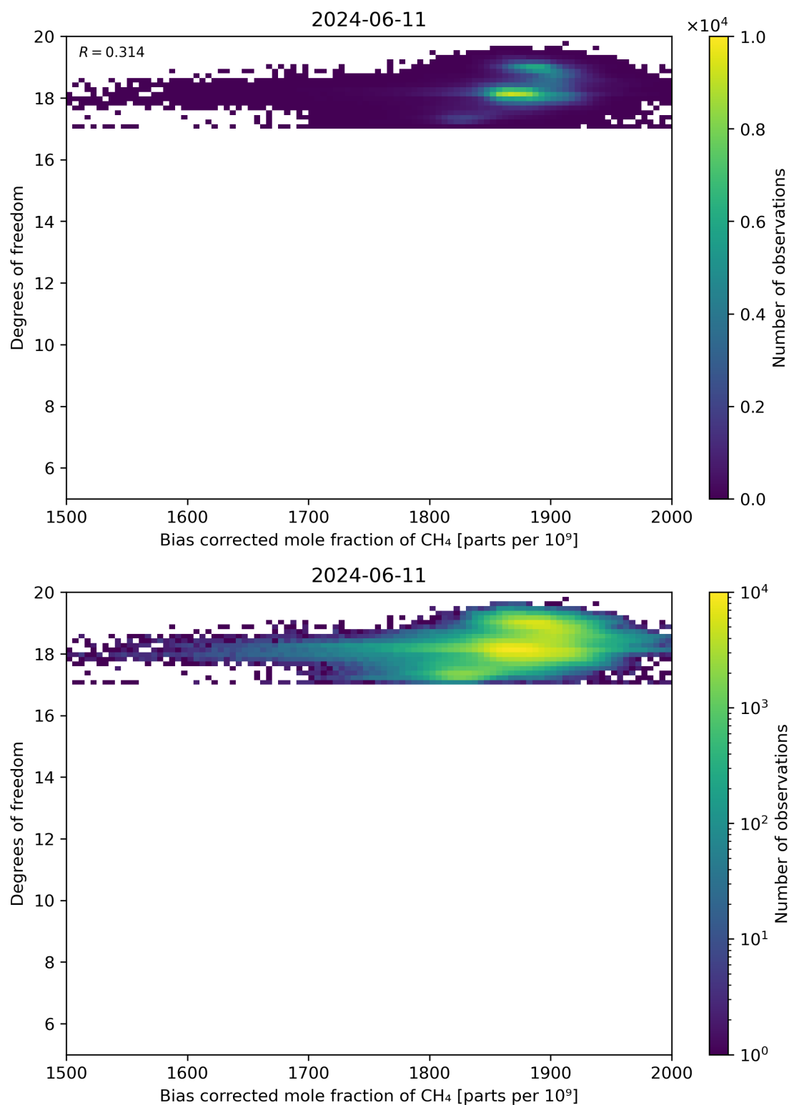
Figure 65: Scatter density plot of “Bias corrected mole fraction of CH 4 ” against “Degrees of freedom” for 2024-06-10 to 2024-06-12.
