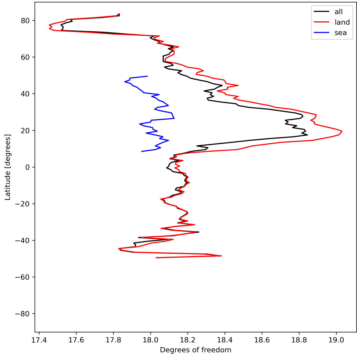
Figure 19: Zonal average of “Degrees of freedom” for 2024-06-10 to 2024-06-12.
