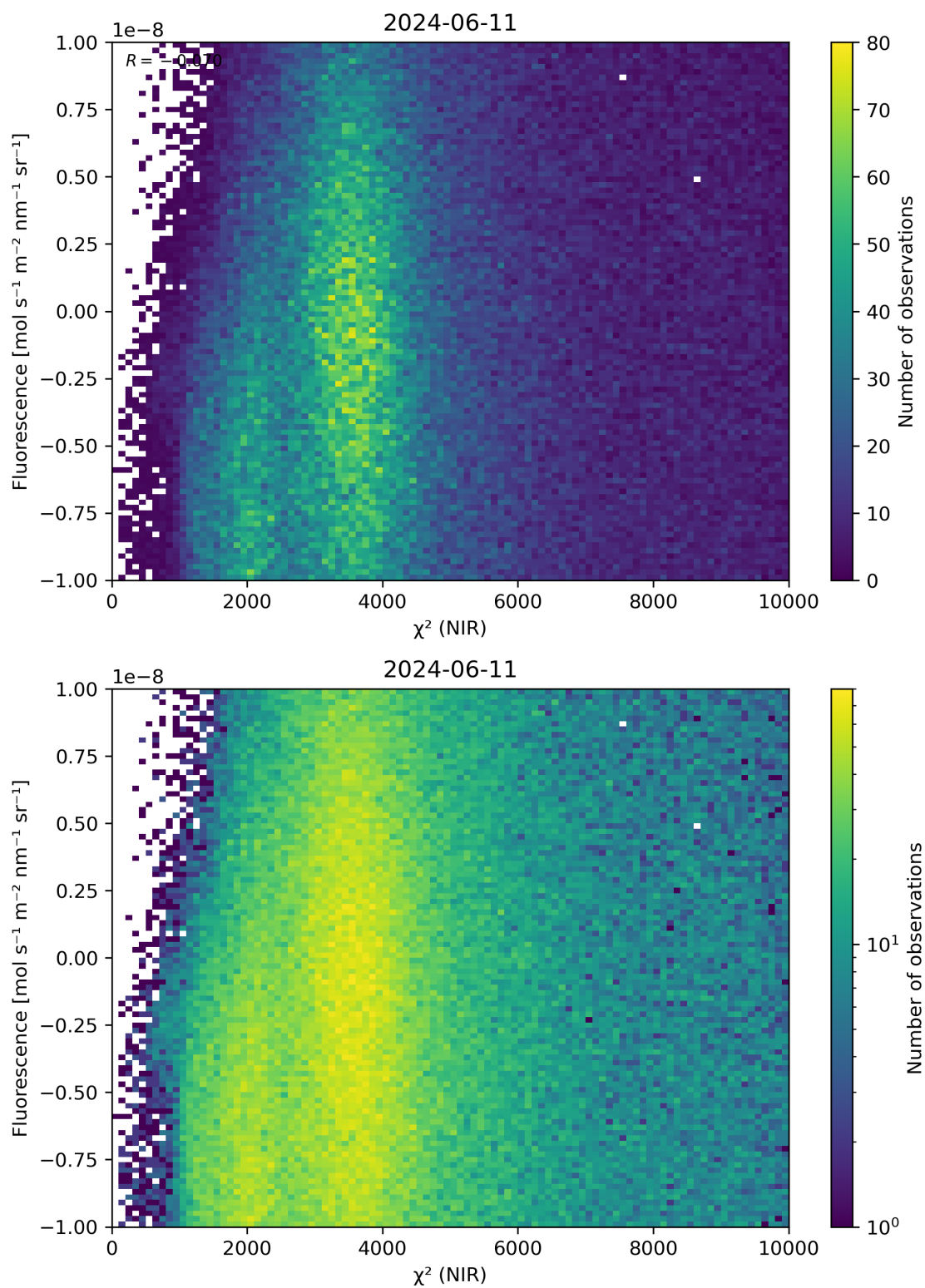
Figure 45: Scatter density plot of “ \chi^2 (NIR)” against “Fluorescence” for 2024-06-10 to 2024-06-12.
