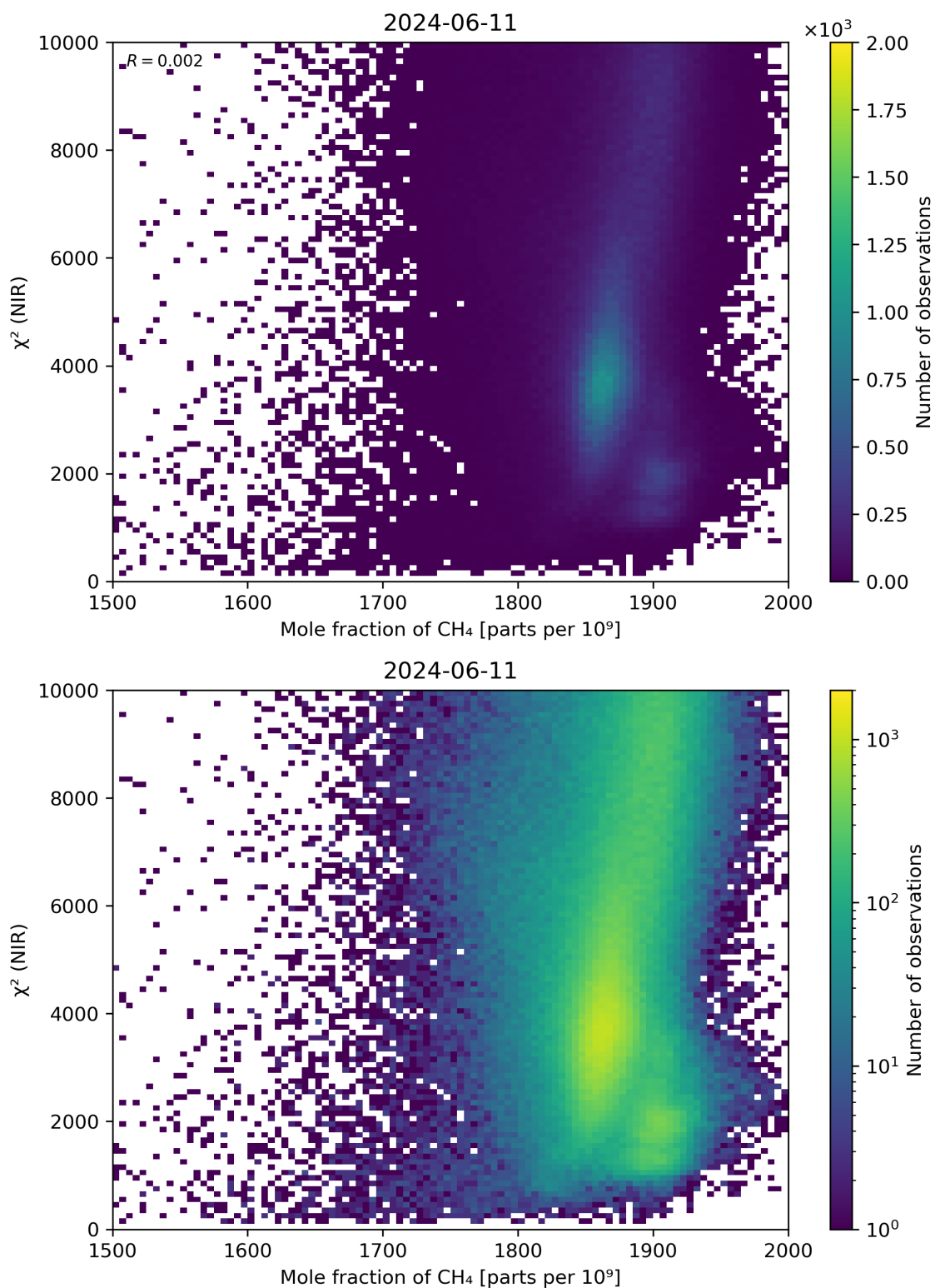
Figure 70: Scatter density plot of “Mole fraction of \text{CH}_4 ” against “ \chi^2 (NIR)” for 2024-06-10 to 2024-06-12.
