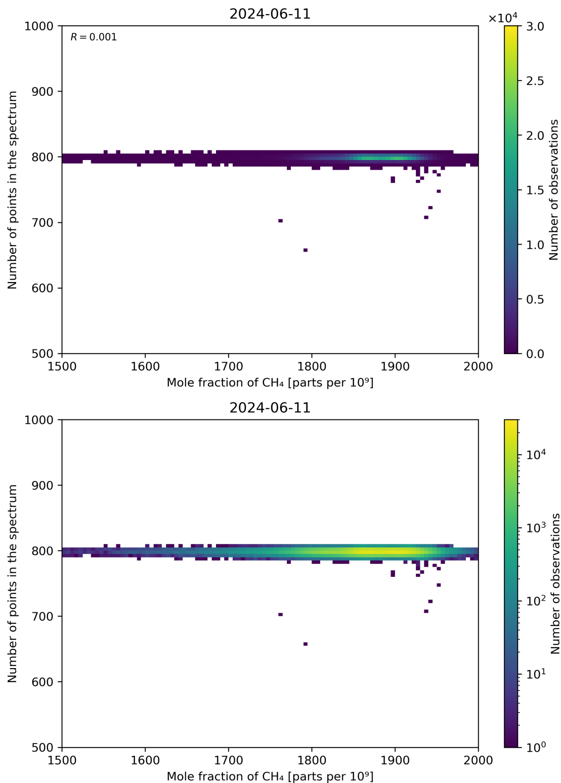
Figure 77: Scatter density plot of “Mole fraction of CH 4 ” against “Number of points in the spectrum” for 2024-06-10 to 2024-06-12.
