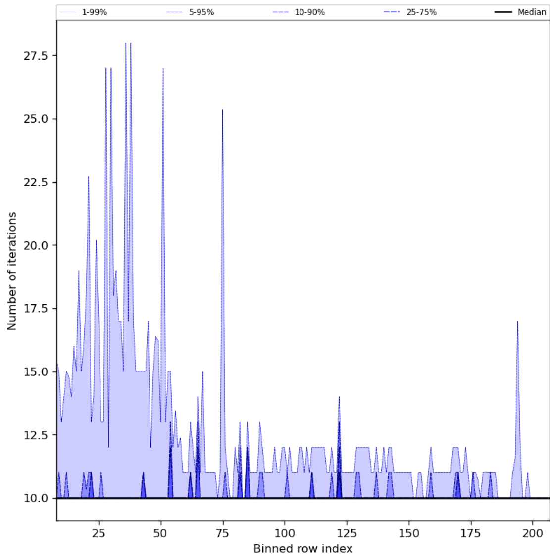
Figure 42: Along track statistics of “Number of iterations” for 2024-06-10 to 2024-06-12
