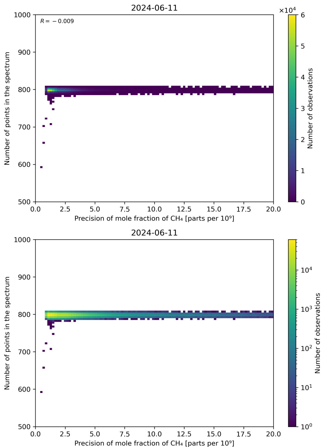
Figure 84: Scatter density plot of “Precision of mole fraction of CH 4 ” against “Number of points in the spectrum” for 2024-06-10 to 2024-06-12.
