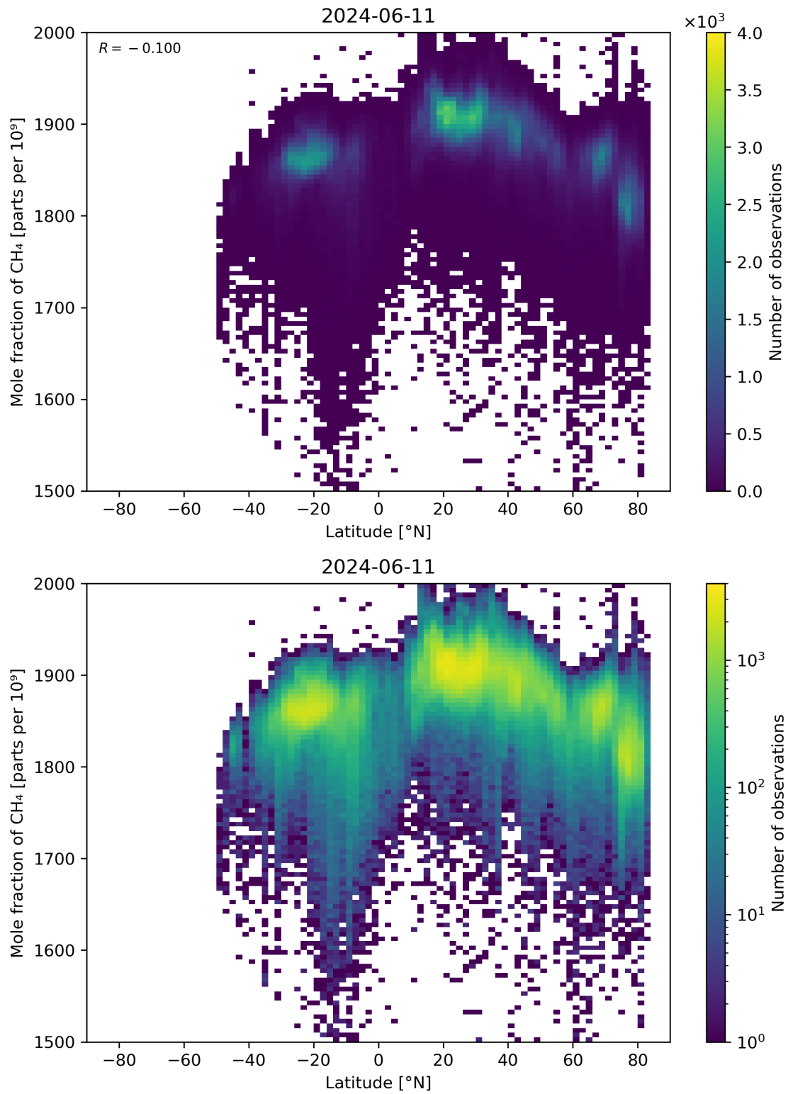
Figure 57: Scatter density plot of “Latitude” against “Mole fraction of \text{CH}_4 ” for 2024-06-10 to 2024-06-12.
