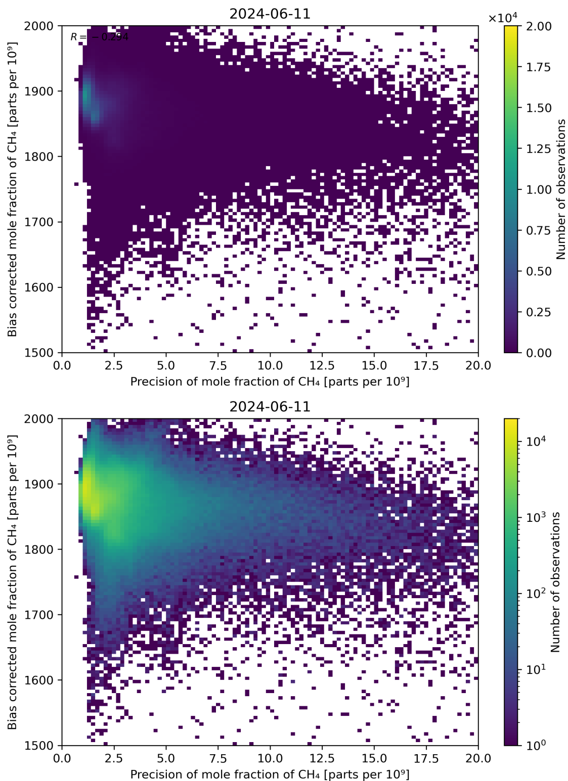
Figure 82: Scatter density plot of “Precision of mole fraction of CH 4 ” against “Bias corrected mole fraction of CH 4 ” for 2024-06-10 to 2024-06-12.
