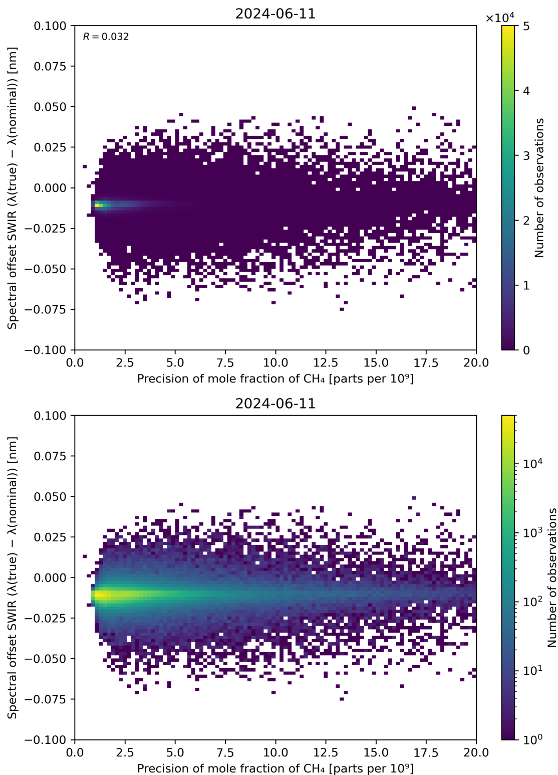
Figure 85: Scatter density plot of “Precision of mole fraction of \text{CH}_4 ” against “Spectral offset SWIR ( \lambda(\text{true}) - \lambda(\text{nominal}) )” for 2024-06-10 to 2024-06-12.
