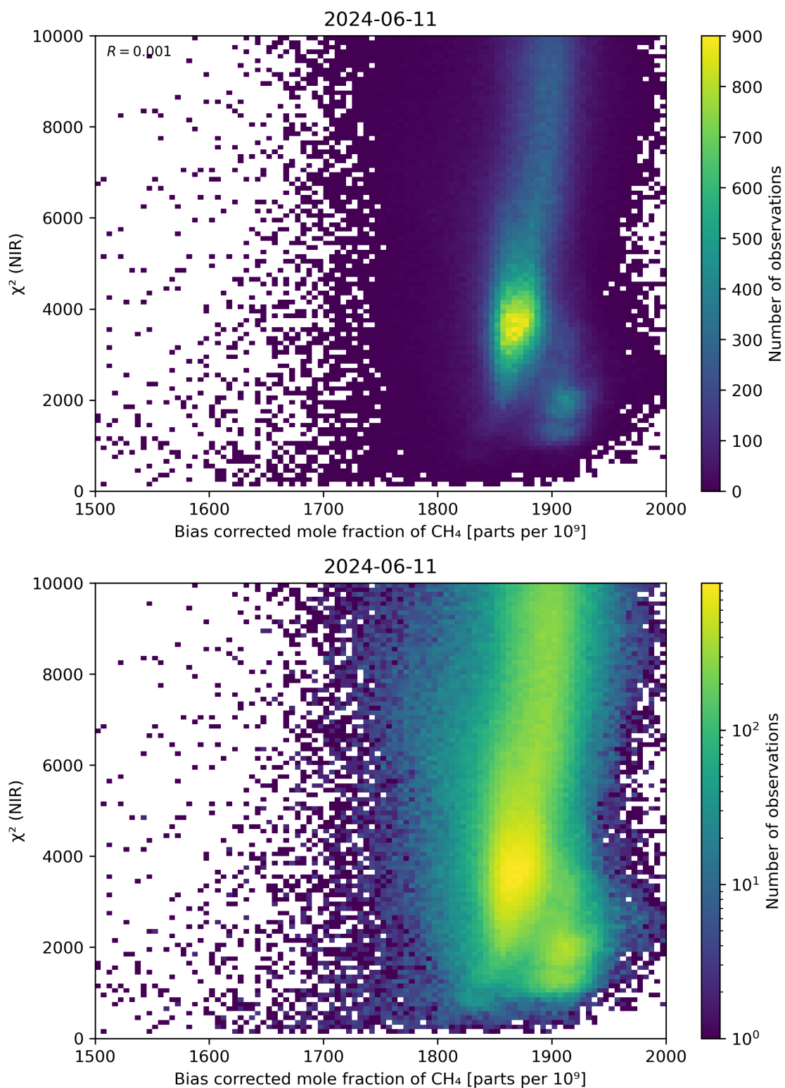
Figure 63: Scatter density plot of “Bias corrected mole fraction of CH 4 ” against “ \chi^2 (NIR)” for 2024-06-10 to 2024-06-12.
