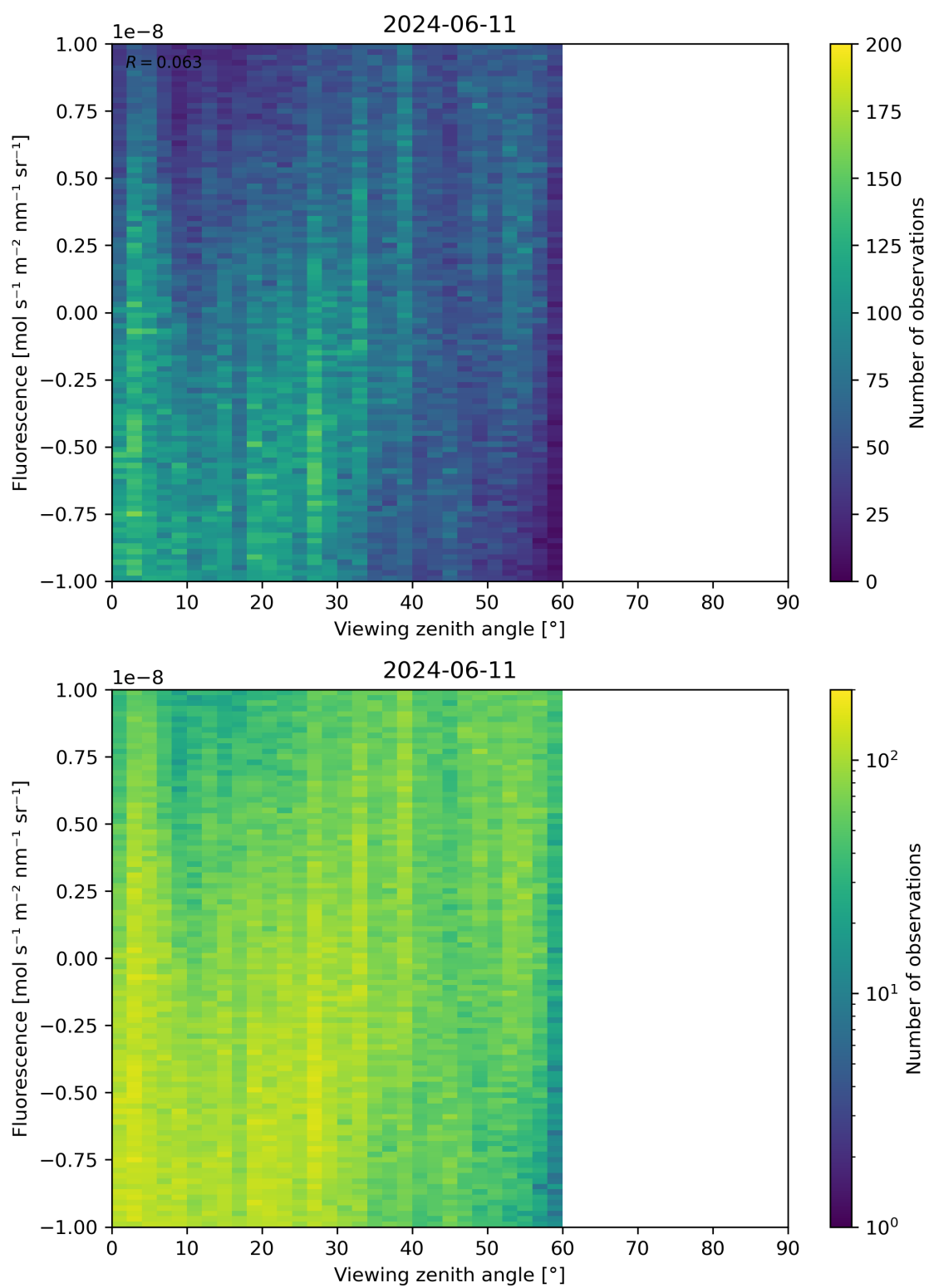
Figure 108: Scatter density plot of “Viewing zenith angle” against “Fluorescence” for 2024-06-10 to 2024-06-12.
