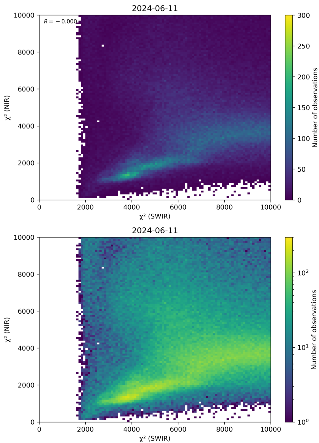
Figure 47: Scatter density plot of “ \chi^2 (SWIR)” against “ \chi^2 (NIR)” for 2024-06-10 to 2024-06-12.
