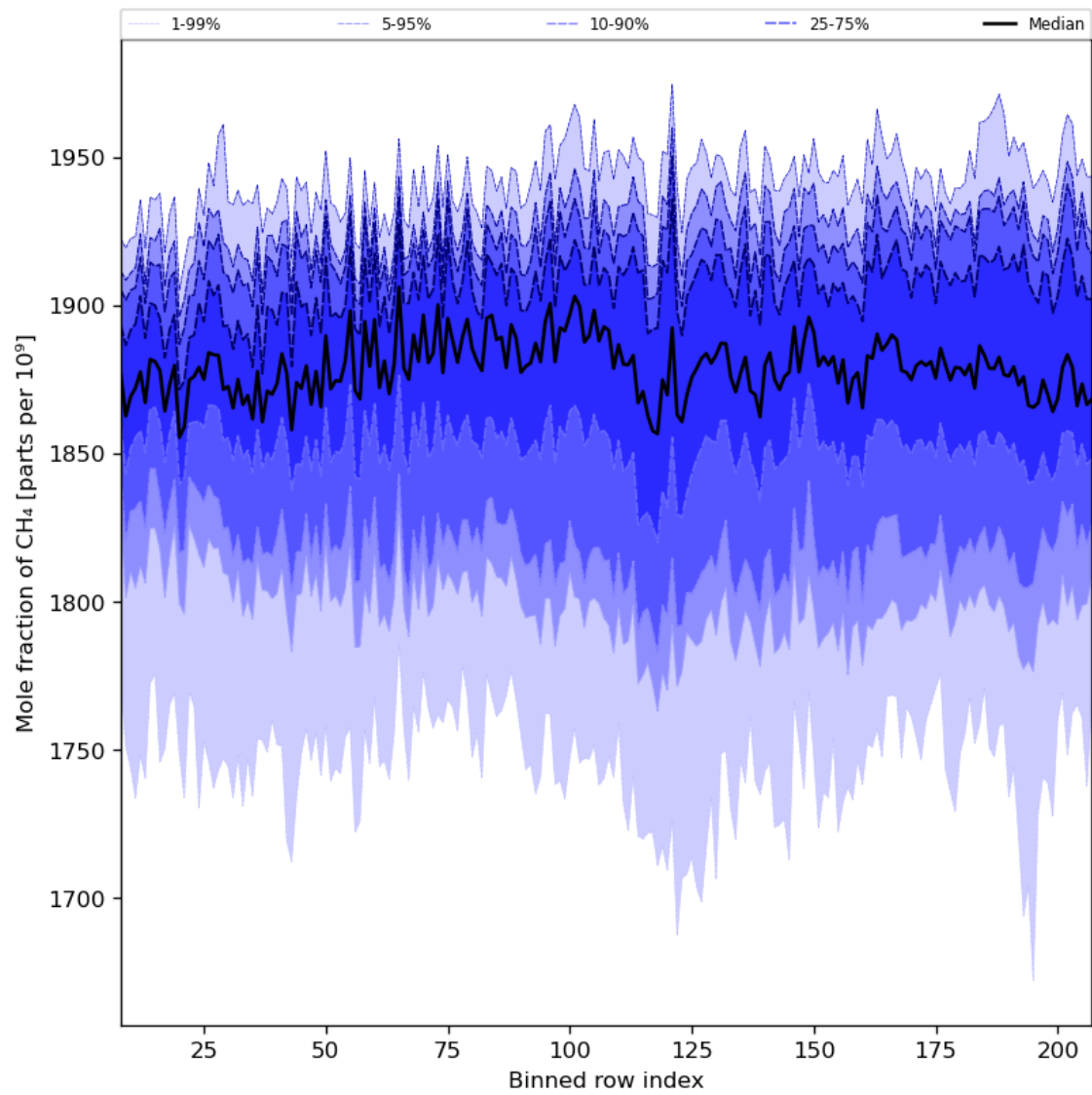
Figure 34: Along track statistics of “Mole fraction of CH 4 ” for 2024-06-10 to 2024-06-12
