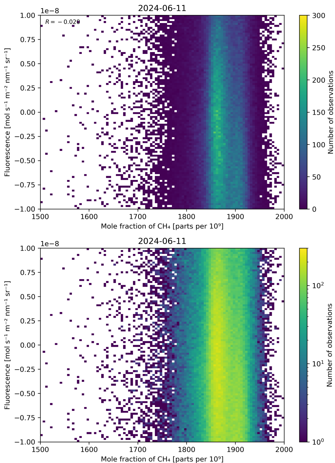
Figure 73: Scatter density plot of “Mole fraction of \text{CH}_4 ” against “Fluorescence” for 2024-06-10 to 2024-06-12.
