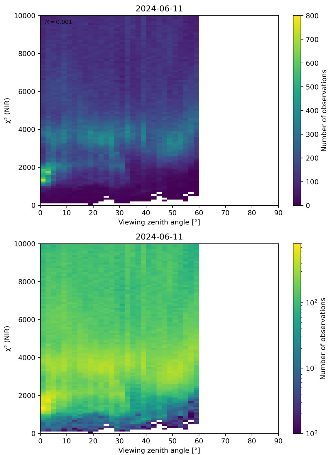
Figure 105: Scatter density plot of “Viewing zenith angle” against “ \chi^2 (NIR)” for 2024-06-10 to 2024-06-12.
