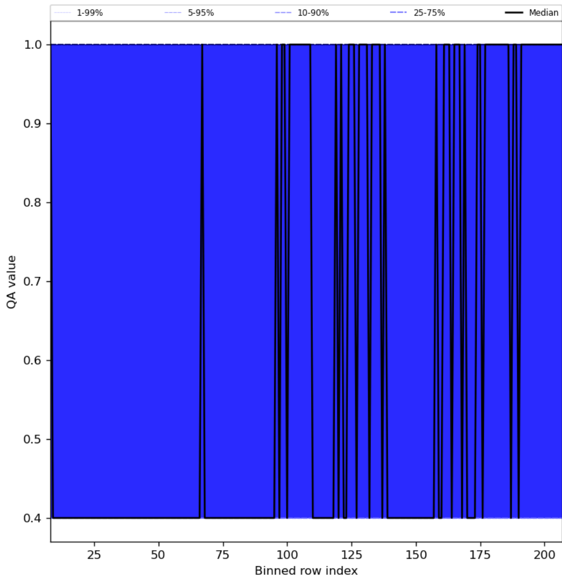
Figure 33: Along track statistics of “QA value” for 2024-06-10 to 2024-06-12
