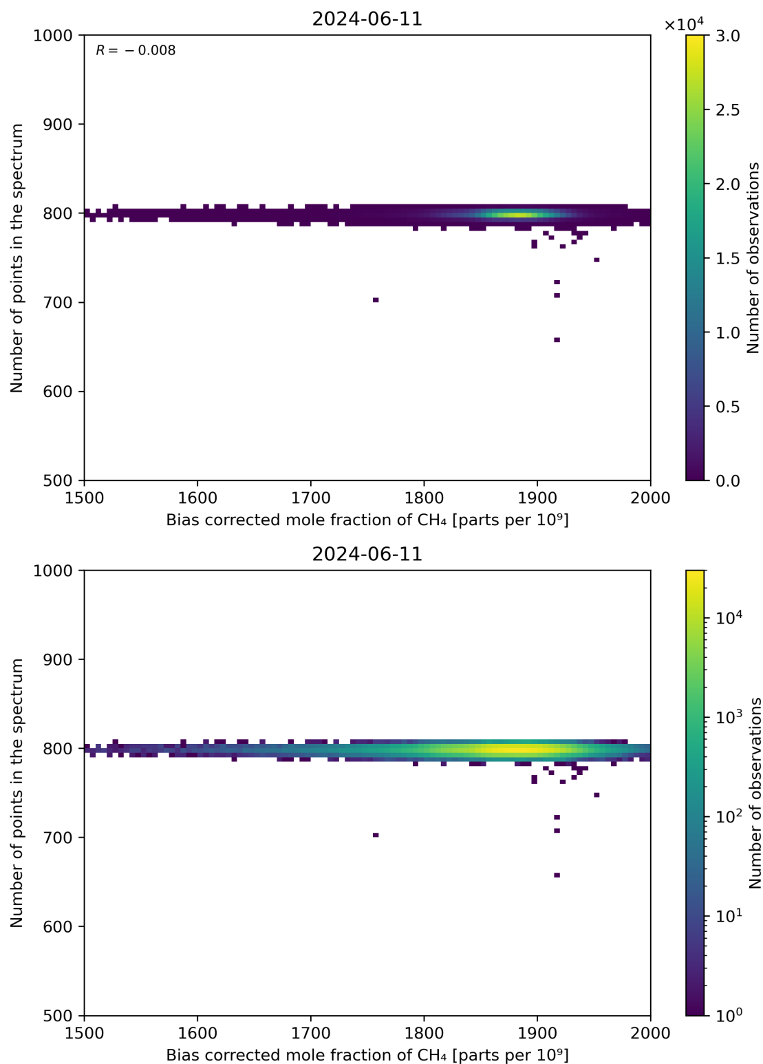
Figure 68: Scatter density plot of “Bias corrected mole fraction of CH 4 ” against “Number of points in the spectrum” for 2024-06-10 to 2024-06-12.
