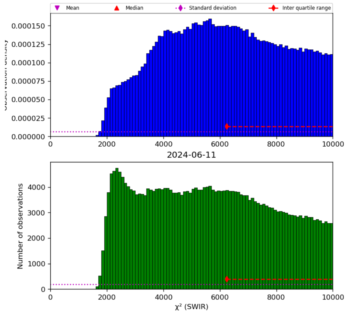
Figure 28: Histogram of “ \chi^2 (SWIR)” for 2024-06-10 to 2024-06-12
