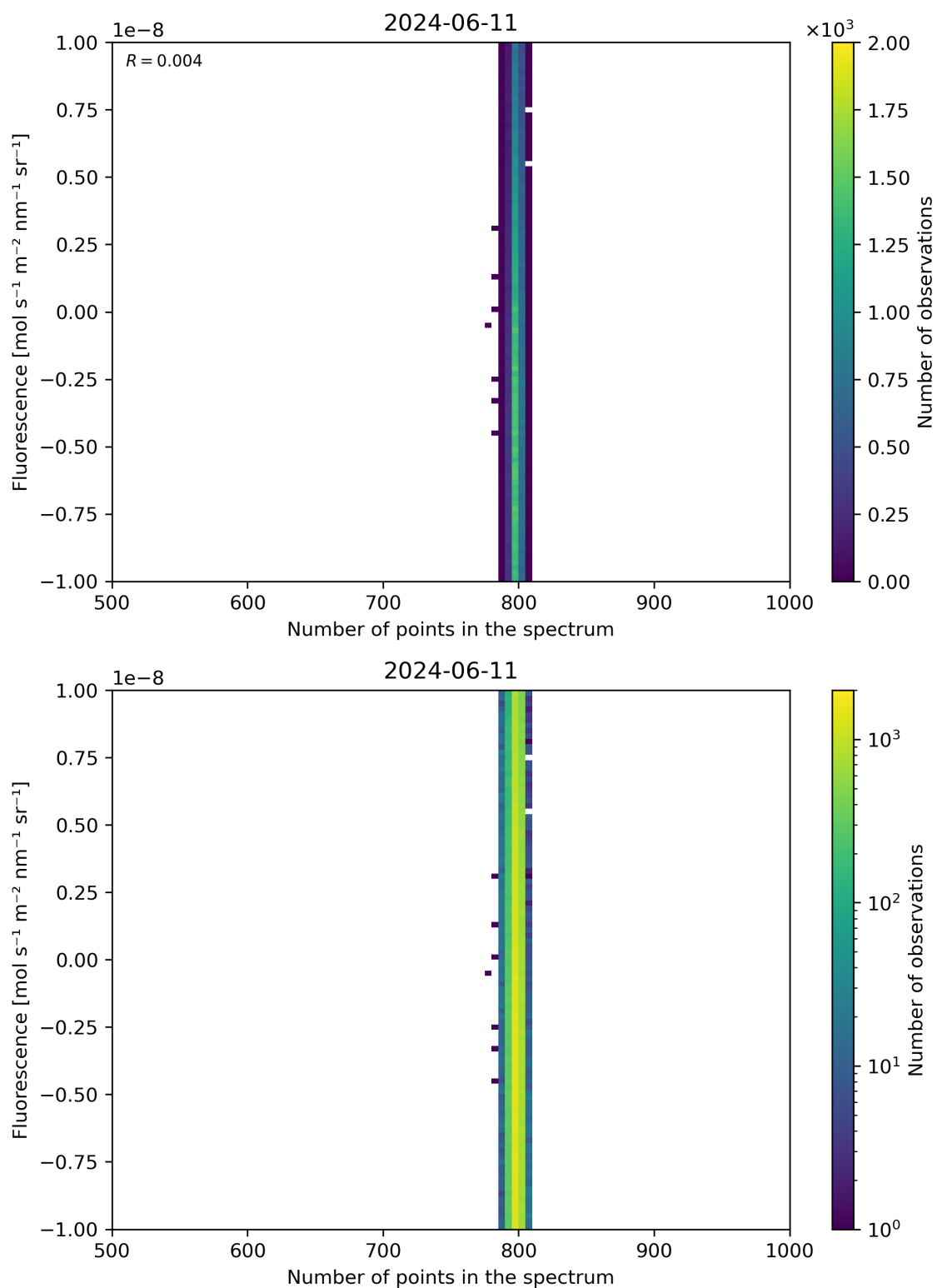
Figure 91: Scatter density plot of “Number of points in the spectrum” against “Fluorescence” for 2024-06-10 to 2024-06-12.
