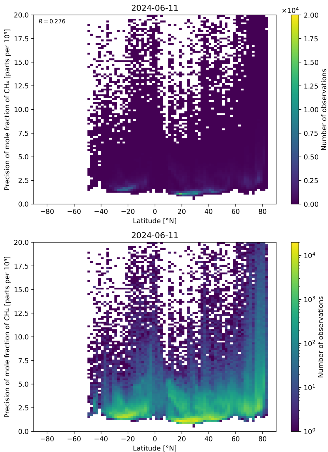
Figure 59: Scatter density plot of “Latitude” against “Precision of mole fraction of \text{CH}_4 ” for 2024-06-10 to 2024-06-12.
