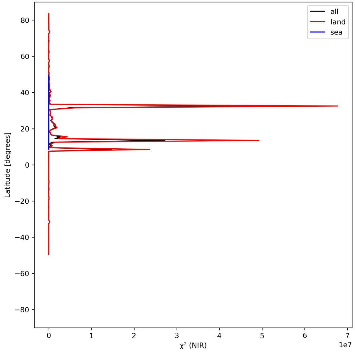
Figure 18: Zonal average of “ \chi^2 (NIR)” for 2024-06-10 to 2024-06-12.
