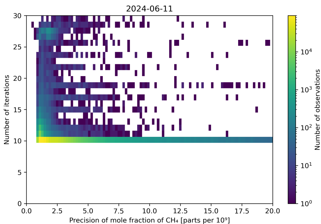
Figure 83: Scatter density plot of “Precision of mole fraction of CH 4 ” against “Number of iterations” for 2024-06-10 to 2024-06-12.
