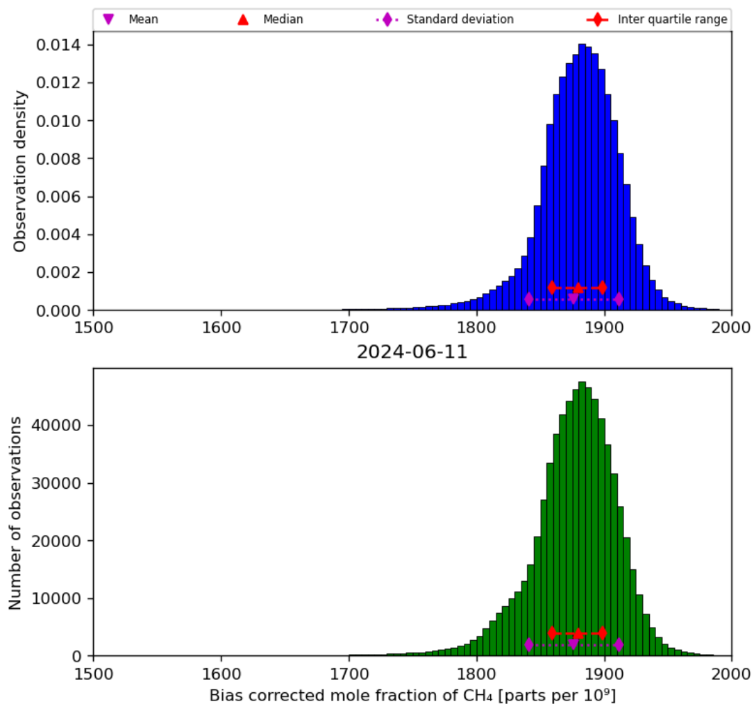
Figure 25: Histogram of “Bias corrected mole fraction of CH 4 ” for 2024-06-10 to 2024-06-12
