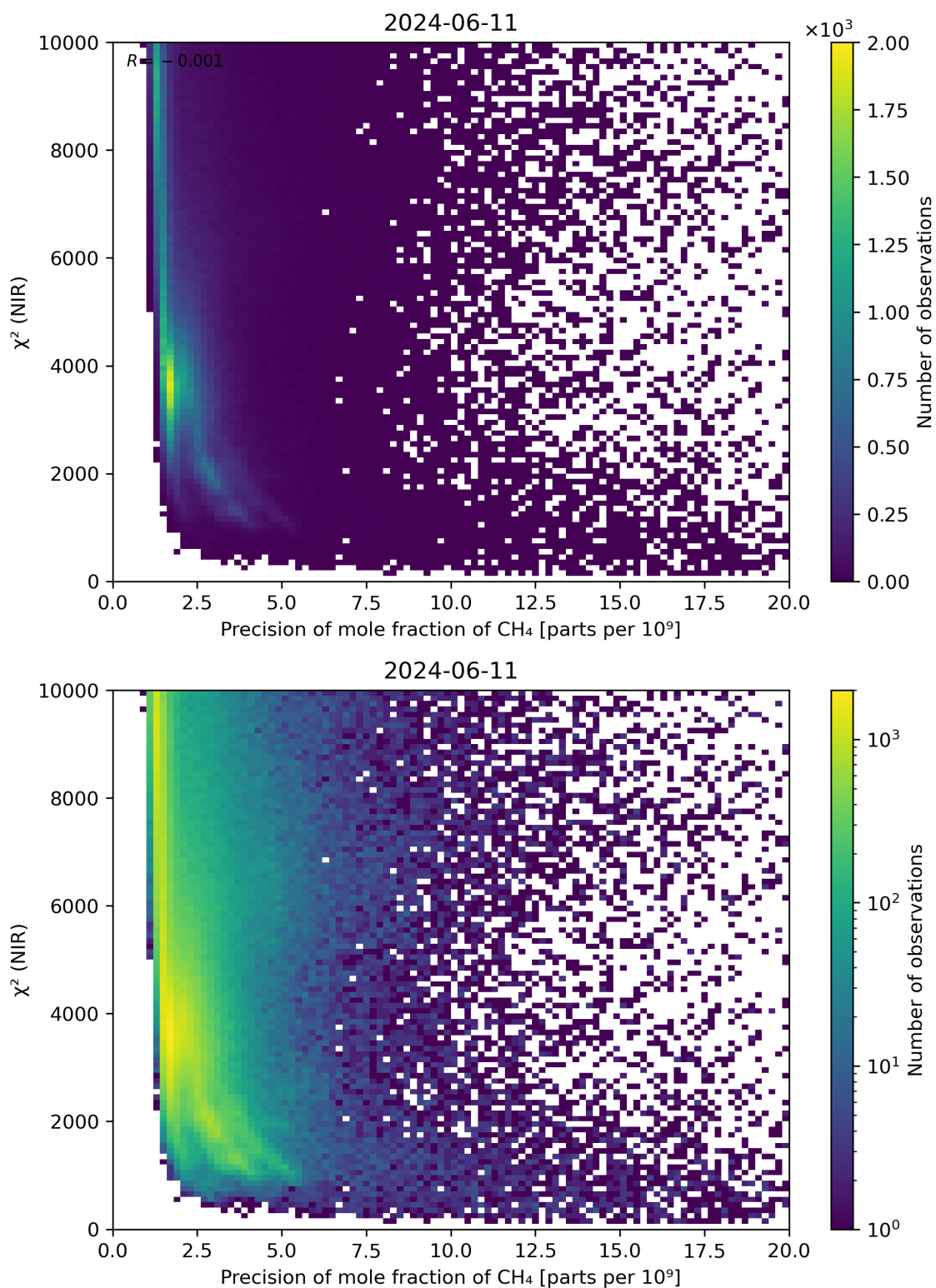
Figure 78: Scatter density plot of “Precision of mole fraction of CH 4 ” against “ \chi^2 (NIR)” for 2024-06-10 to 2024-06-12.
