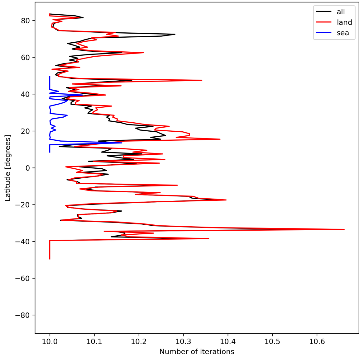
Figure 20: Zonal average of “Number of iterations” for 2024-06-10 to 2024-06-12.
