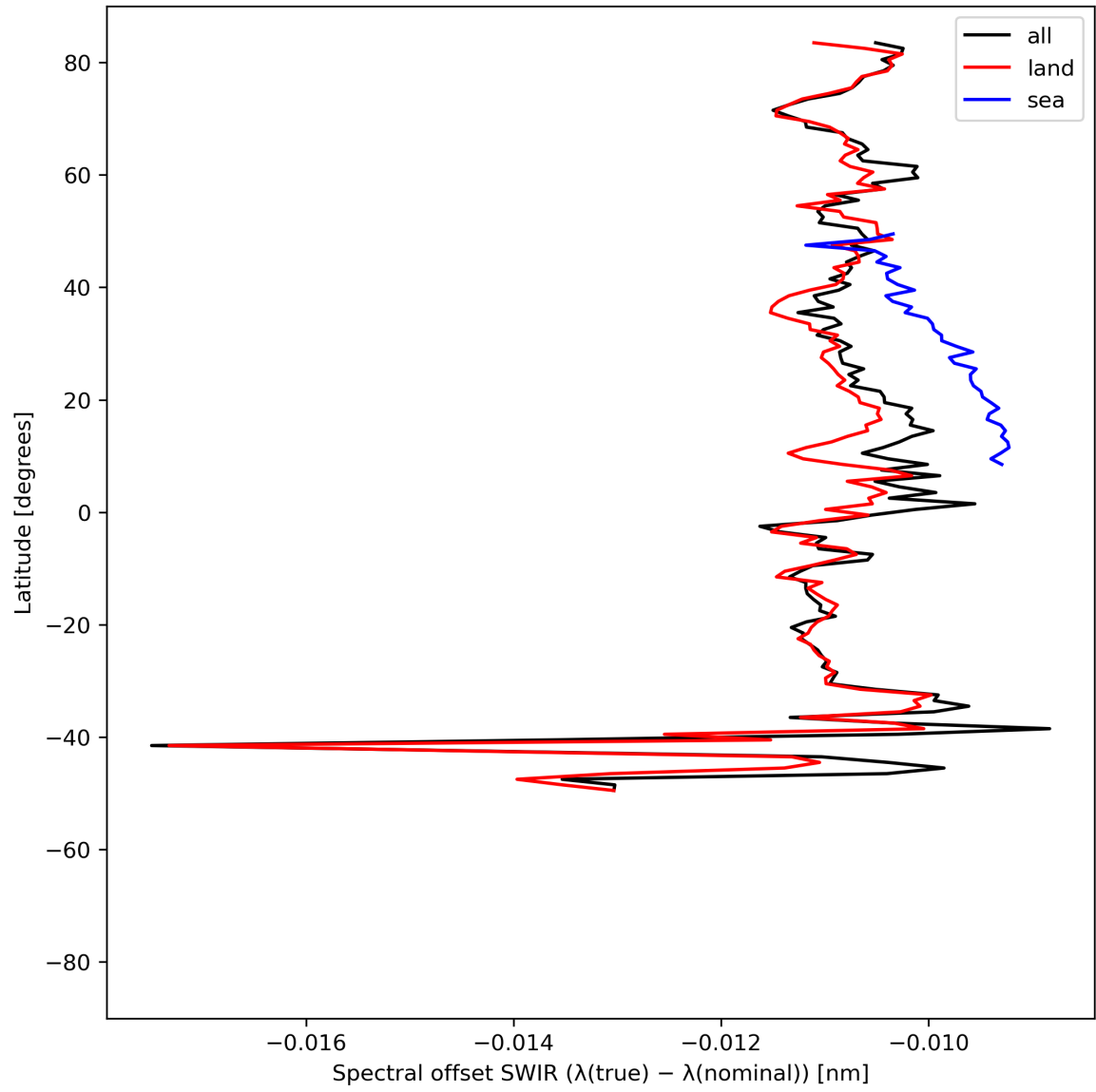
Figure 16: Zonal average of “Spectral offset SWIR ( \lambda(\text{true}) - \lambda(\text{nominal}) )” for 2024-06-10 to 2024-06-12.
