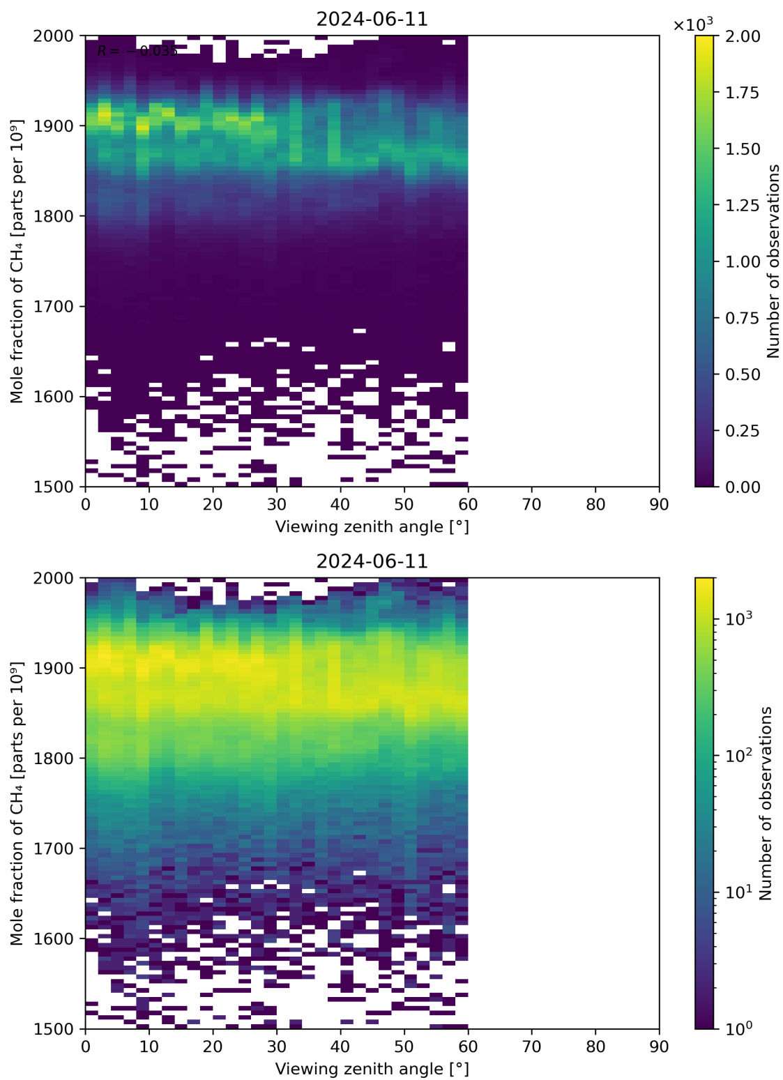
Figure 110: Scatter density plot of “Viewing zenith angle” against “Mole fraction of CH 4 ” for 2024-06-10 to 2024-06-12.
