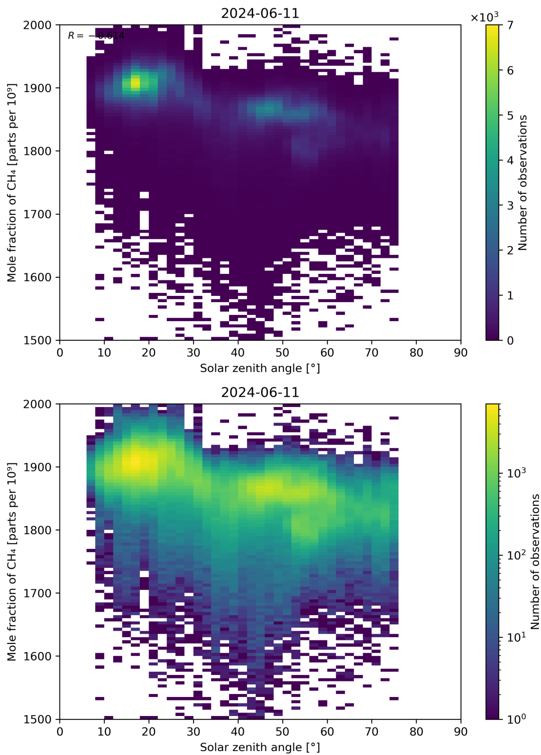
Figure 99: Scatter density plot of “Solar zenith angle” against “Mole fraction of CH 4 ” for 2024-06-10 to 2024-06-12.
