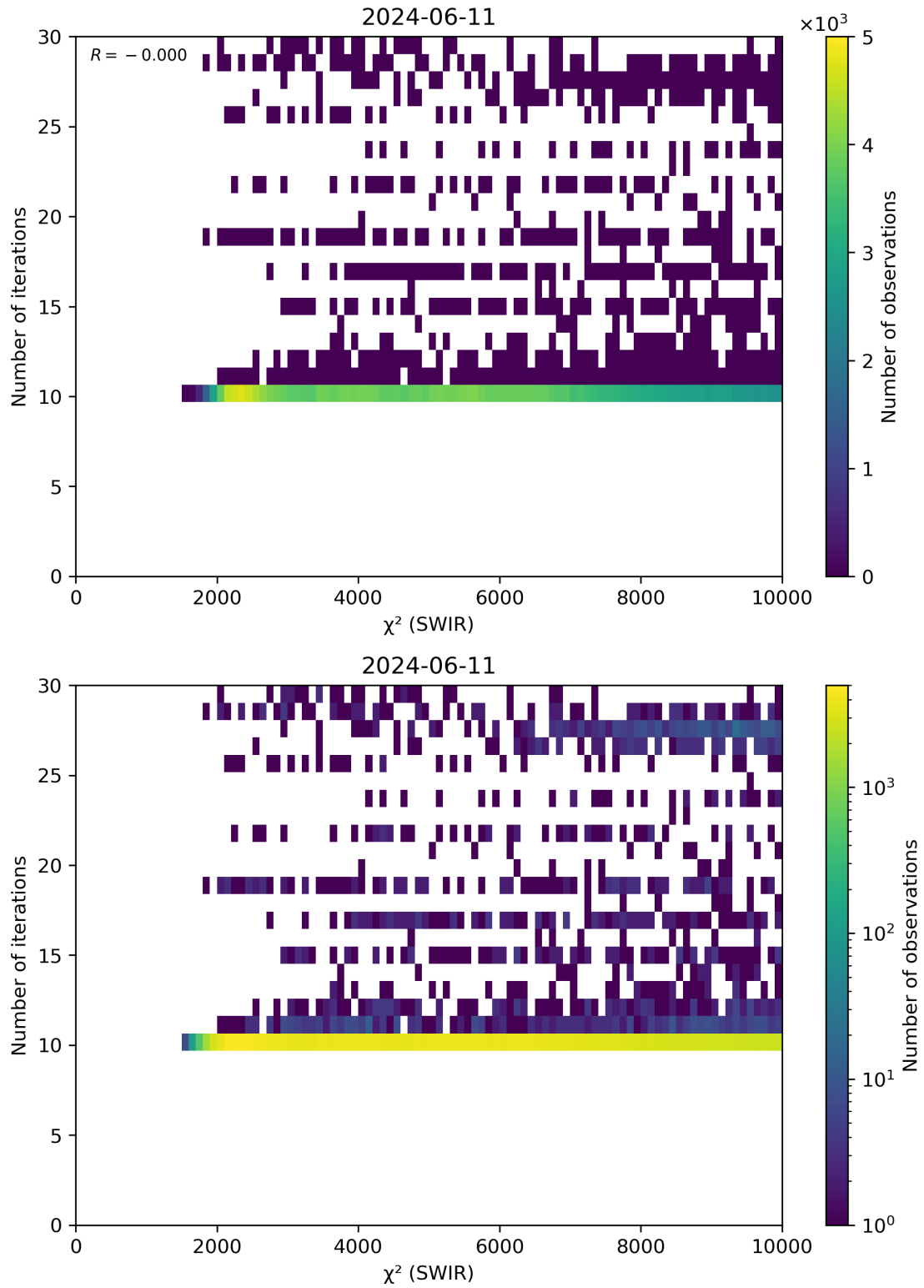
Figure 50: Scatter density plot of “ \chi^2 (SWIR)” against “Number of iterations” for 2024-06-10 to 2024-06-12.
