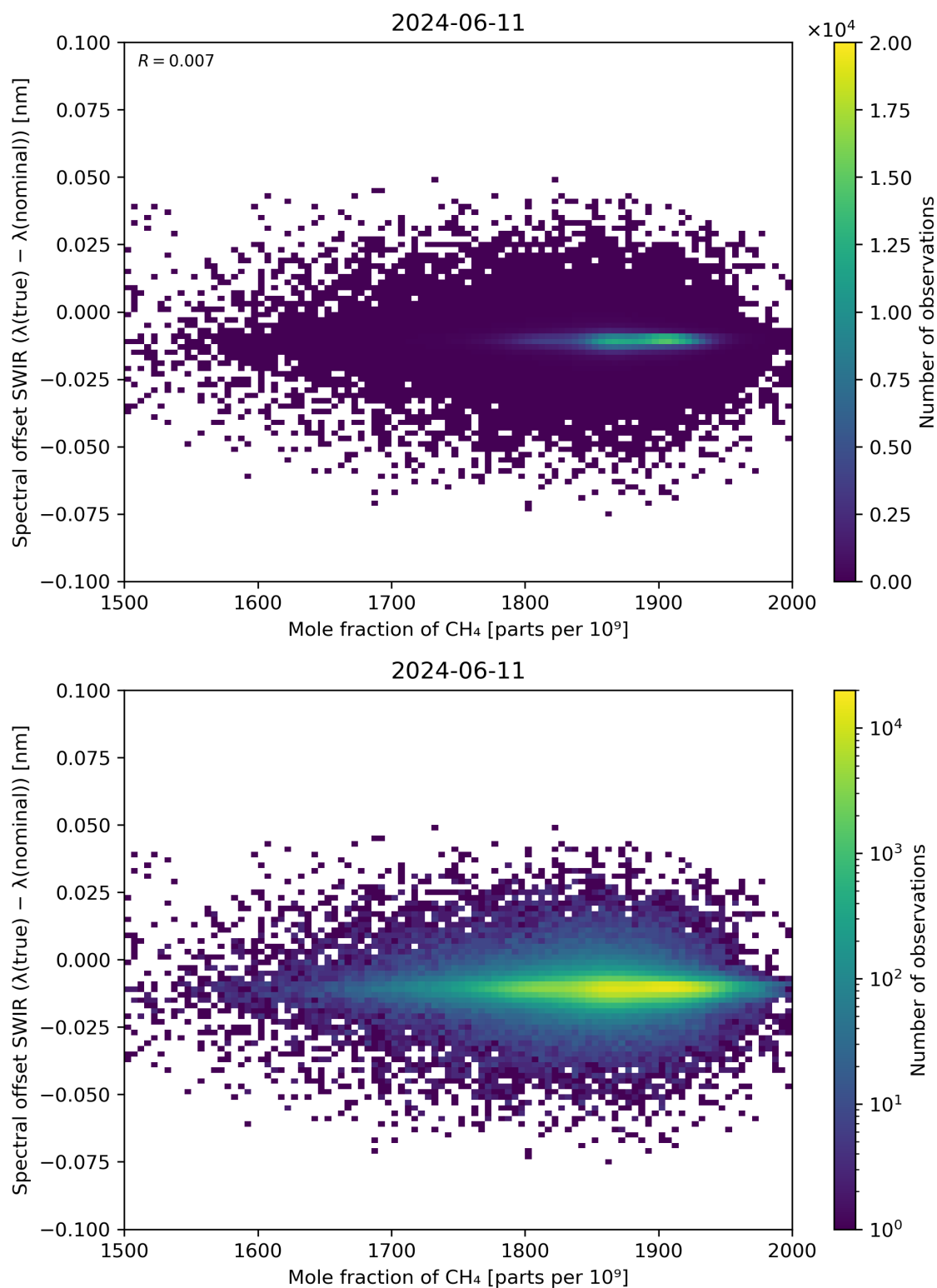
Figure 86: Scatter density plot of “Mole fraction of CH 4 ” against “Spectral offset SWIR ( \lambda(\text{true}) - \lambda(\text{nominal}) )” for 2024-06-10 to 2024-06-12.
