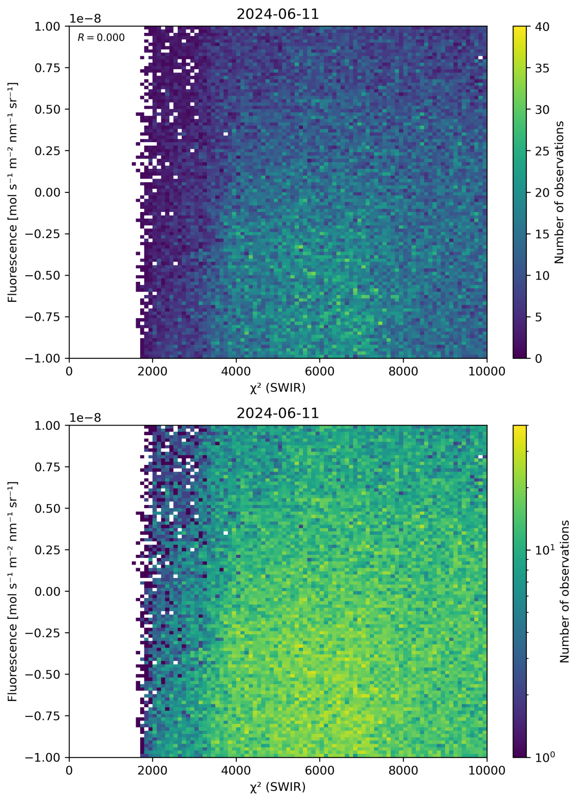
Figure 49: Scatter density plot of “ \chi^2 (SWIR)” against “Fluorescence” for 2024-06-10 to 2024-06-12.
