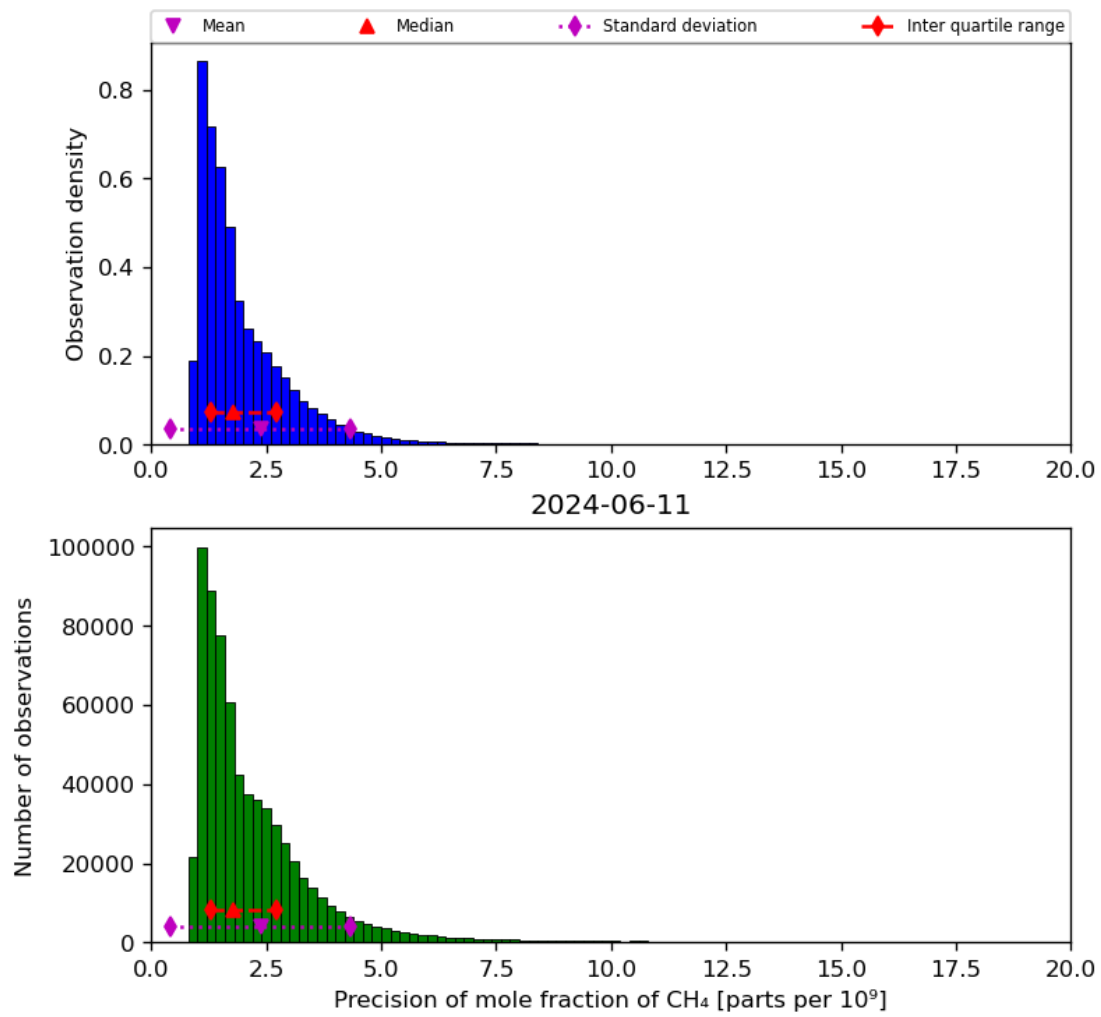
Figure 24: Histogram of “Precision of mole fraction of CH 4 ” for 2024-06-10 to 2024-06-12
