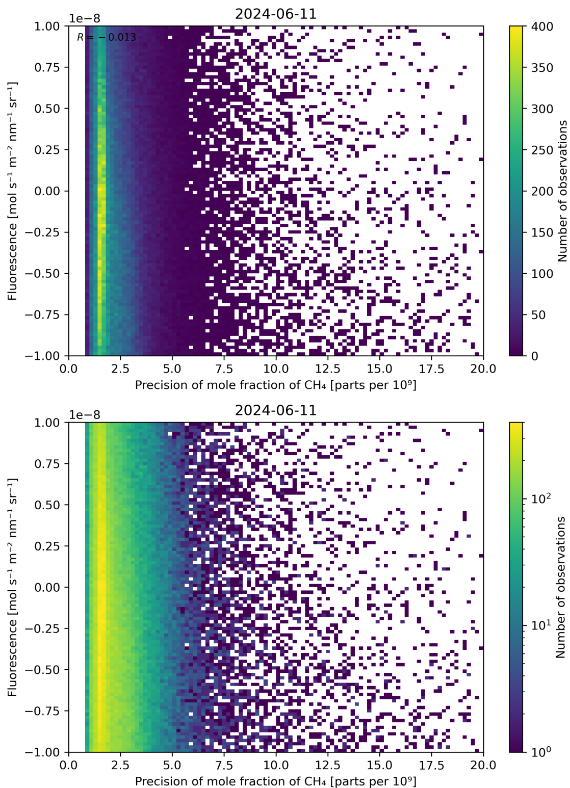
Figure 81: Scatter density plot of “Precision of mole fraction of \text{CH}_4 ” against “Fluorescence” for 2024-06-10 to 2024-06-12.
