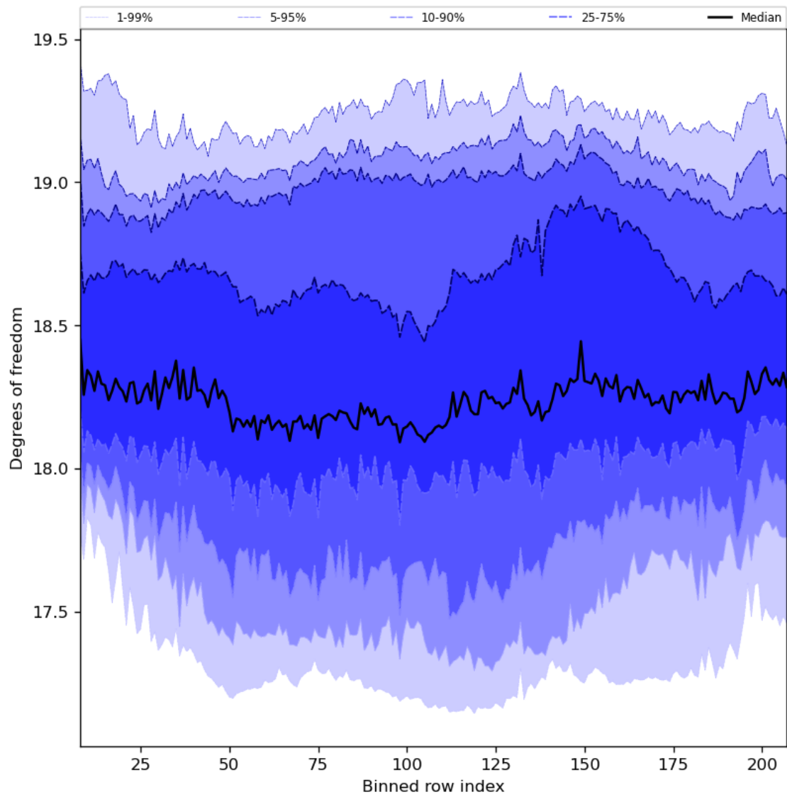
Figure 41: Along track statistics of “Degrees of freedom” for 2024-06-10 to 2024-06-12
