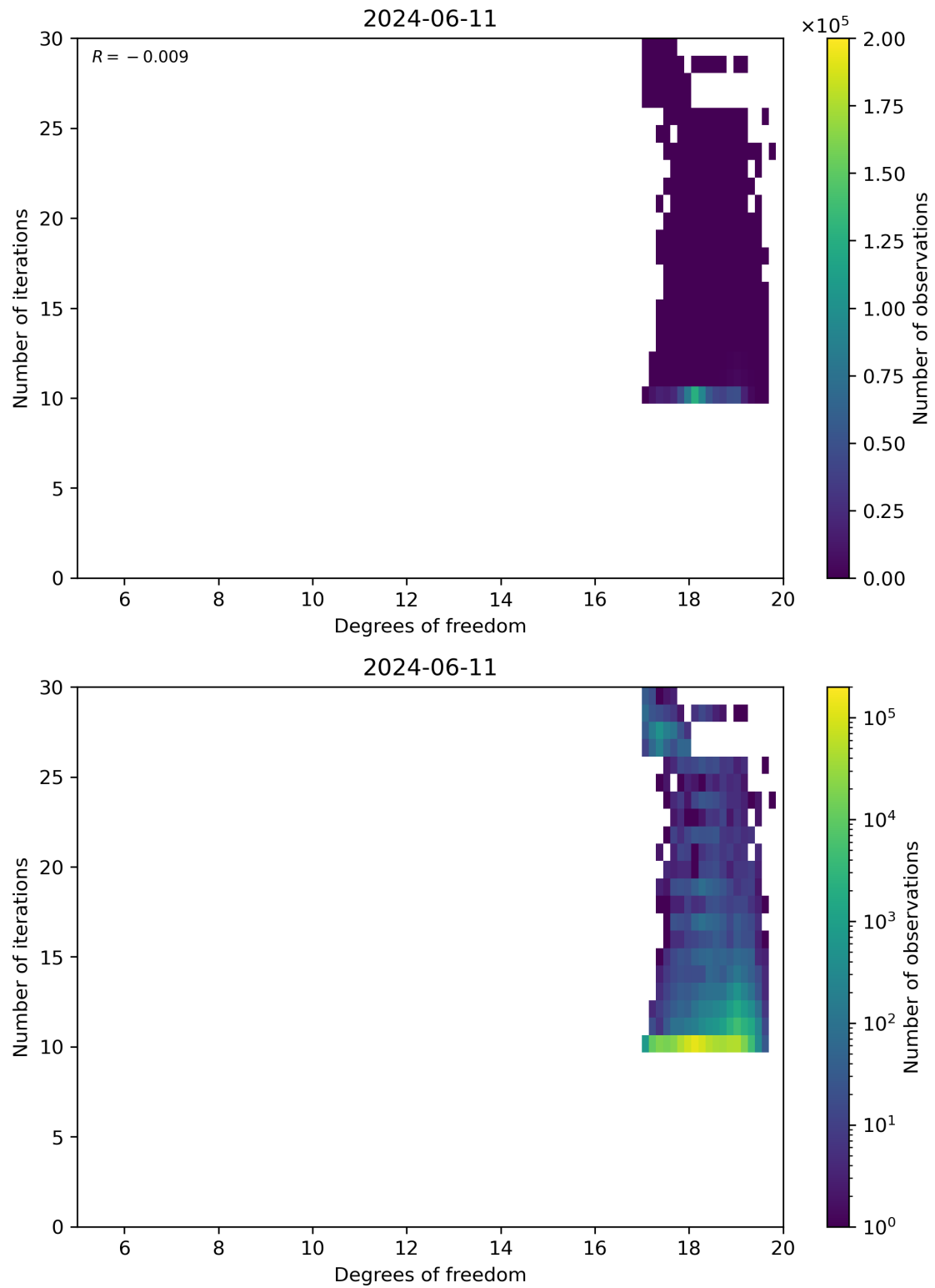
Figure 52: Scatter density plot of “Degrees of freedom” against “Number of iterations” for 2024-06-10 to 2024-06-12.
