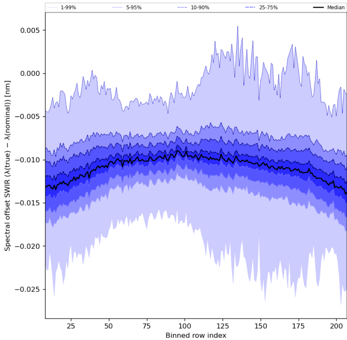
Figure 38: Along track statistics of “Spectral offset SWIR ( \lambda(\text{true}) - \lambda(\text{nominal}) )” for 2024-06-10 to 2024-06-12
