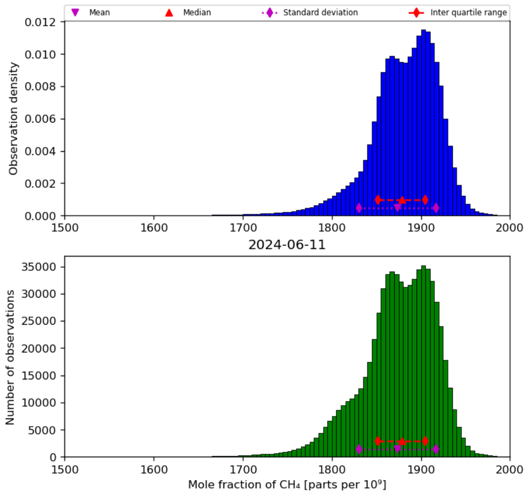
Figure 23: Histogram of “Mole fraction of CH 4 ” for 2024-06-10 to 2024-06-12
