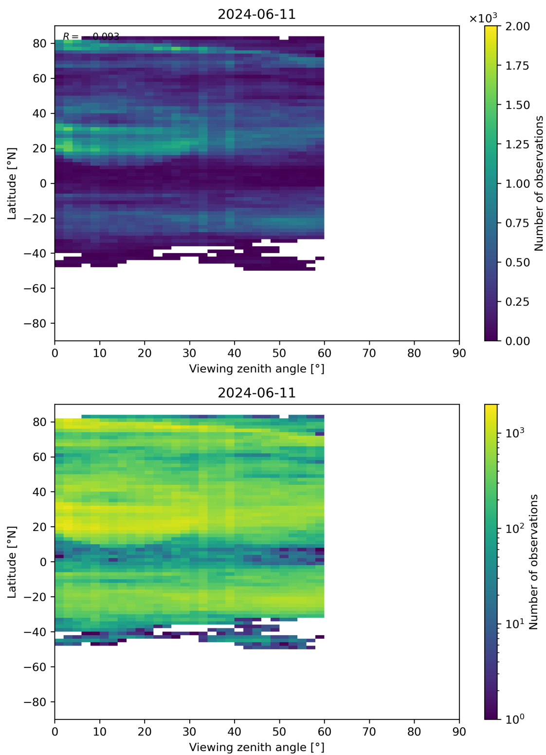
Figure 109: Scatter density plot of “Viewing zenith angle” against “Latitude” for 2024-06-10 to 2024-06-12.
