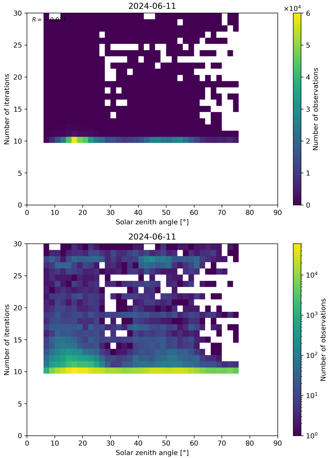
Figure 102: Scatter density plot of “Solar zenith angle” against “Number of iterations” for 2024-06-10 to 2024-06-12.
