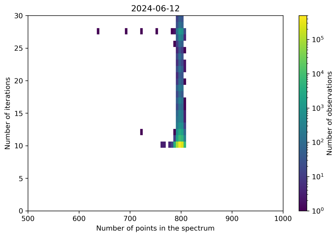
Figure 92: Scatter density plot of “Number of points in the spectrum” against “Number of iterations” for 2024-06-11 to 2024-06-13.
