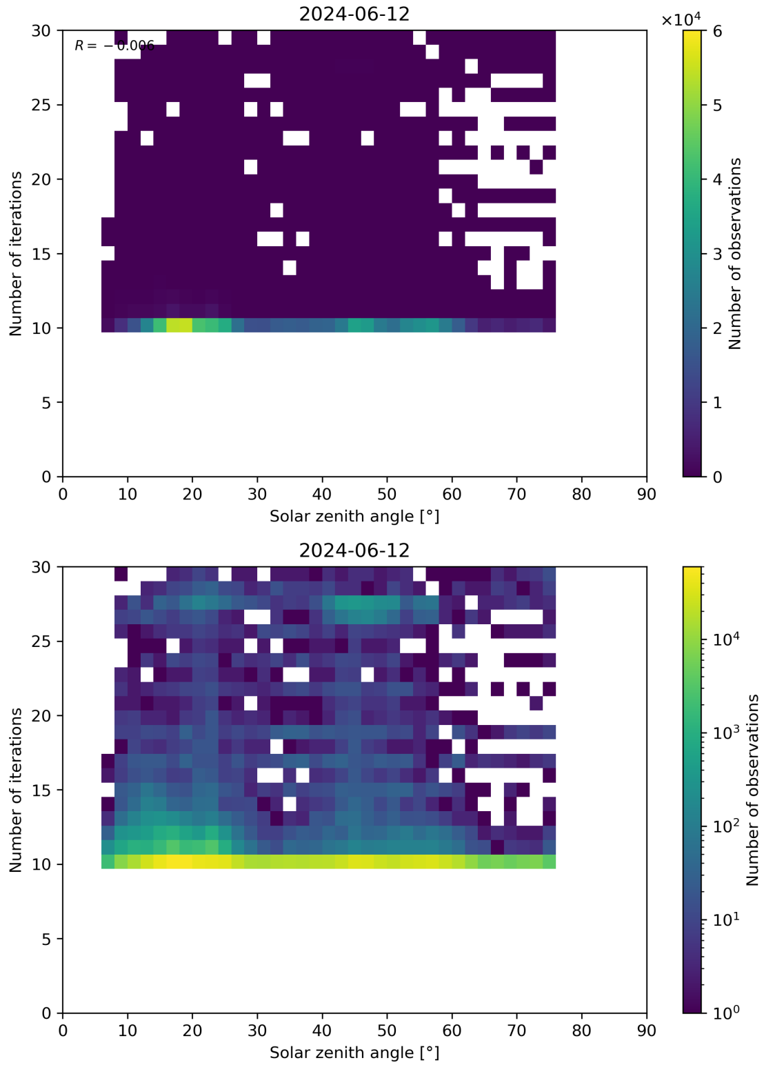
Figure 102: Scatter density plot of “Solar zenith angle” against “Number of iterations” for 2024-06-11 to 2024-06-13.
