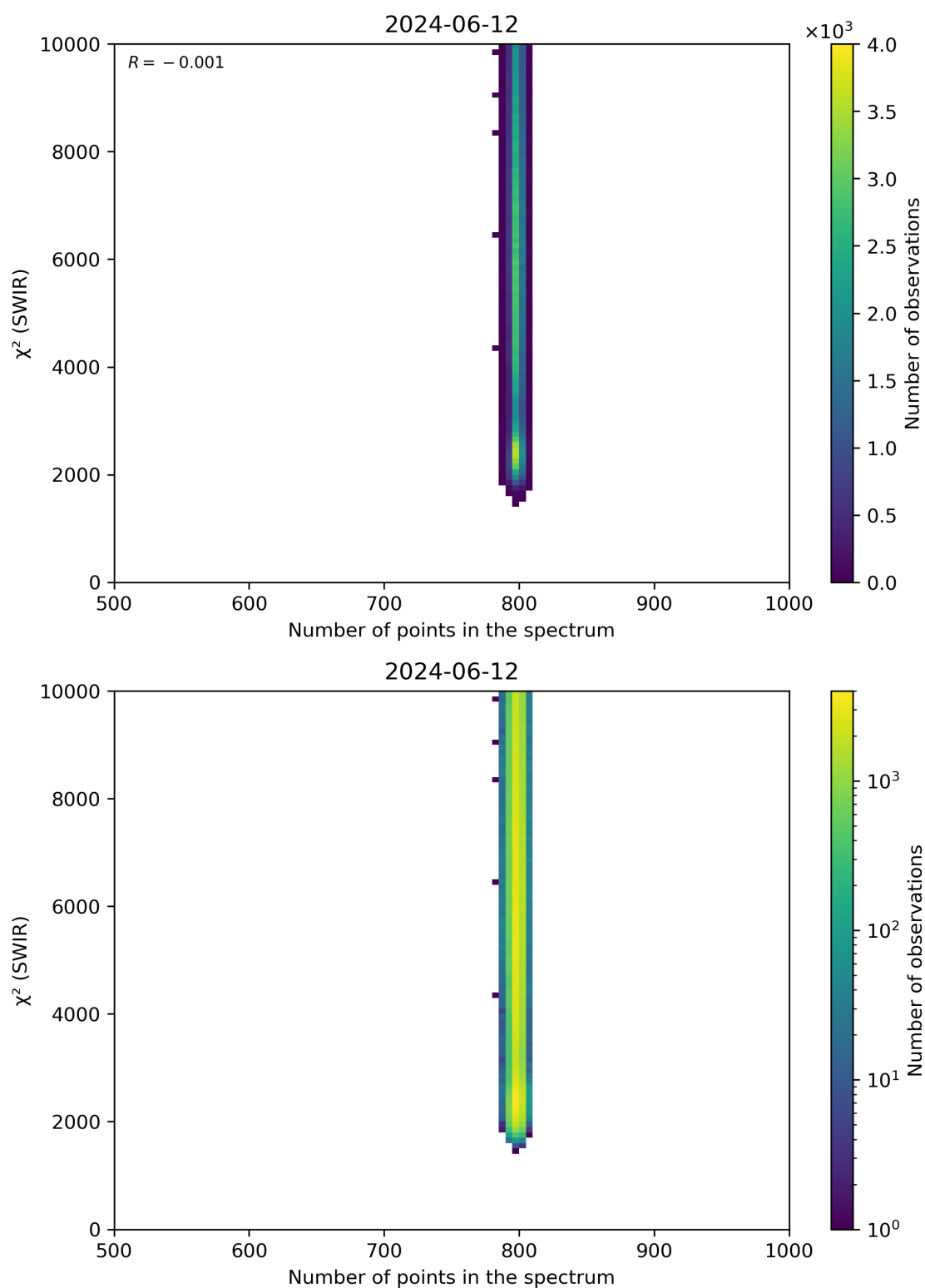
Figure 89: Scatter density plot of “Number of points in the spectrum” against “ \chi^2 (SWIR)” for 2024-06-11 to 2024-06-13.
