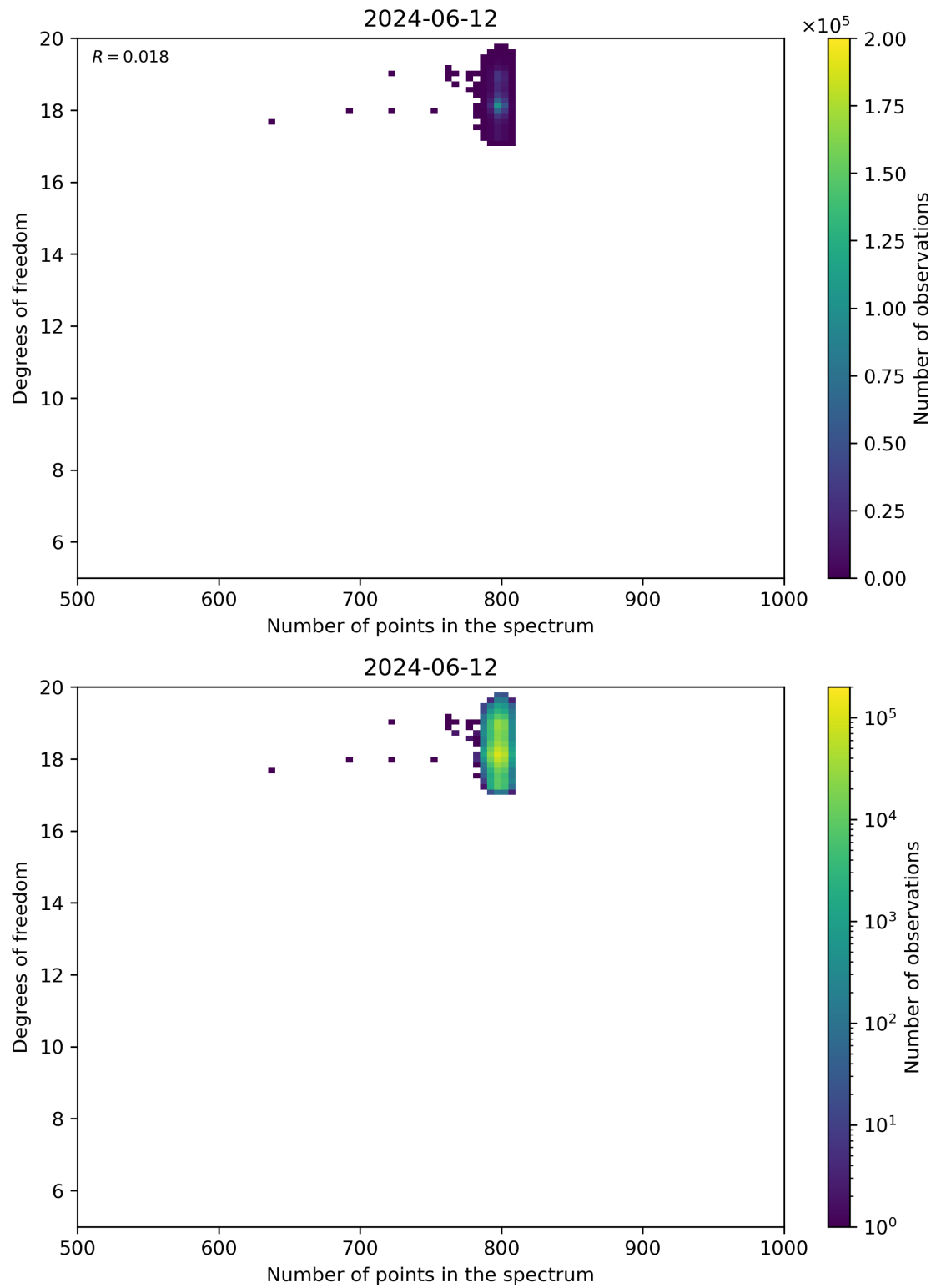
Figure 90: Scatter density plot of “Number of points in the spectrum” against “Degrees of freedom” for 2024-06-11 to 2024-06-13.
