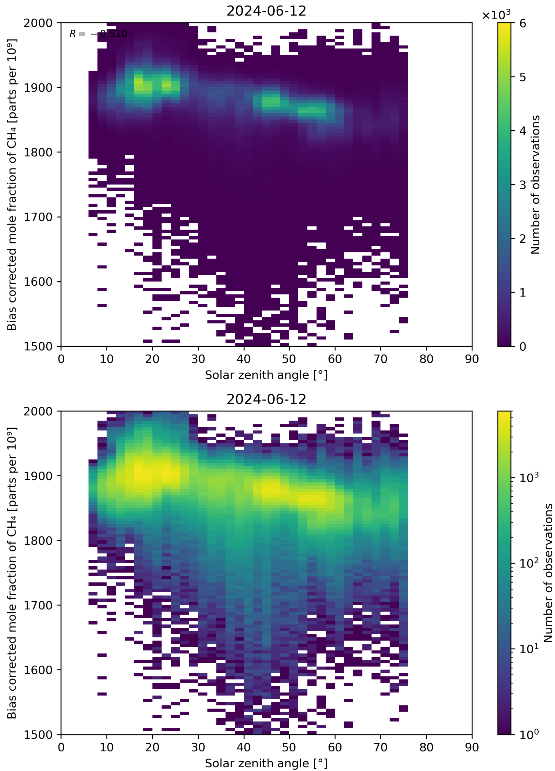
Figure 100: Scatter density plot of “Solar zenith angle” against “Bias corrected mole fraction of CH 4 ” for 2024-06-11 to 2024-06-13.
