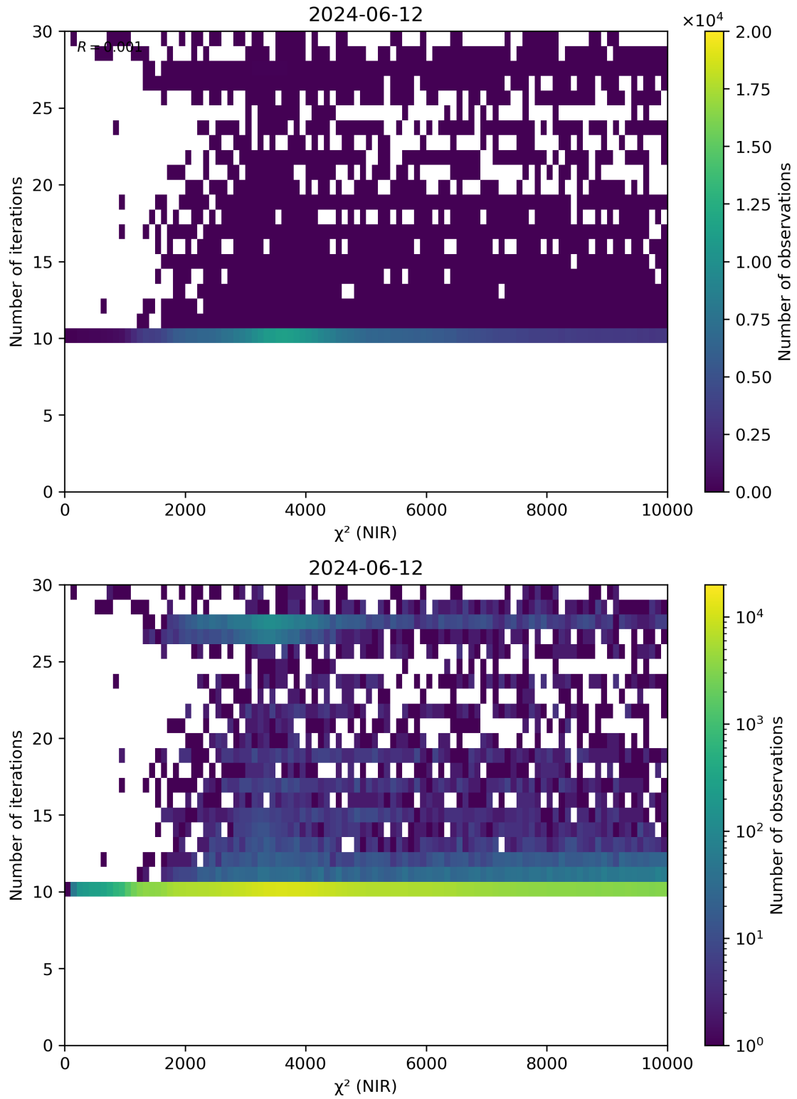
Figure 46: Scatter density plot of “ \chi^2 (NIR)” against “Number of iterations” for 2024-06-11 to 2024-06-13.
