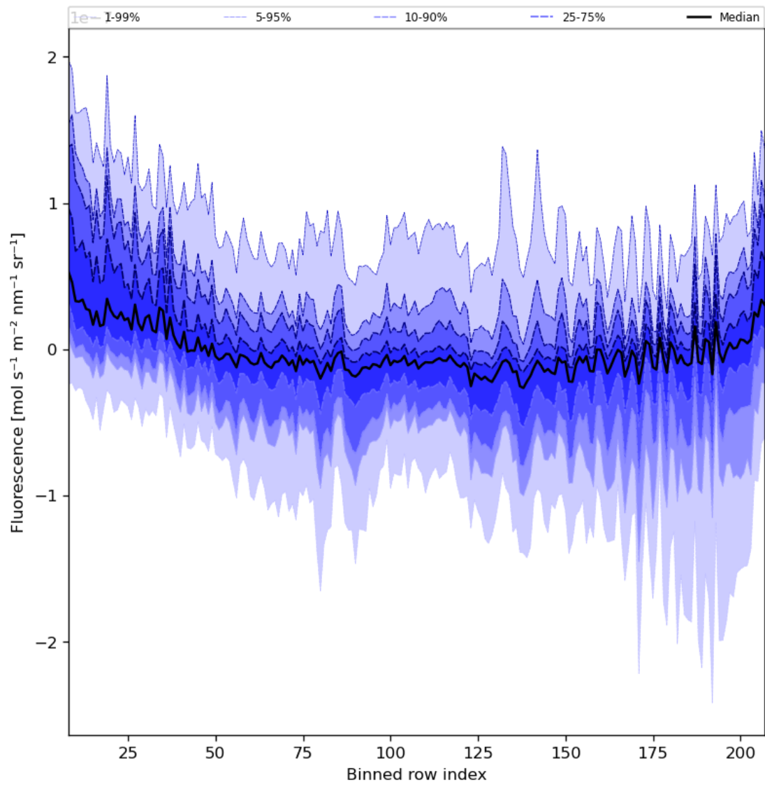
Figure 43: Along track statistics of “Fluorescence” for 2024-06-11 to 2024-06-13
