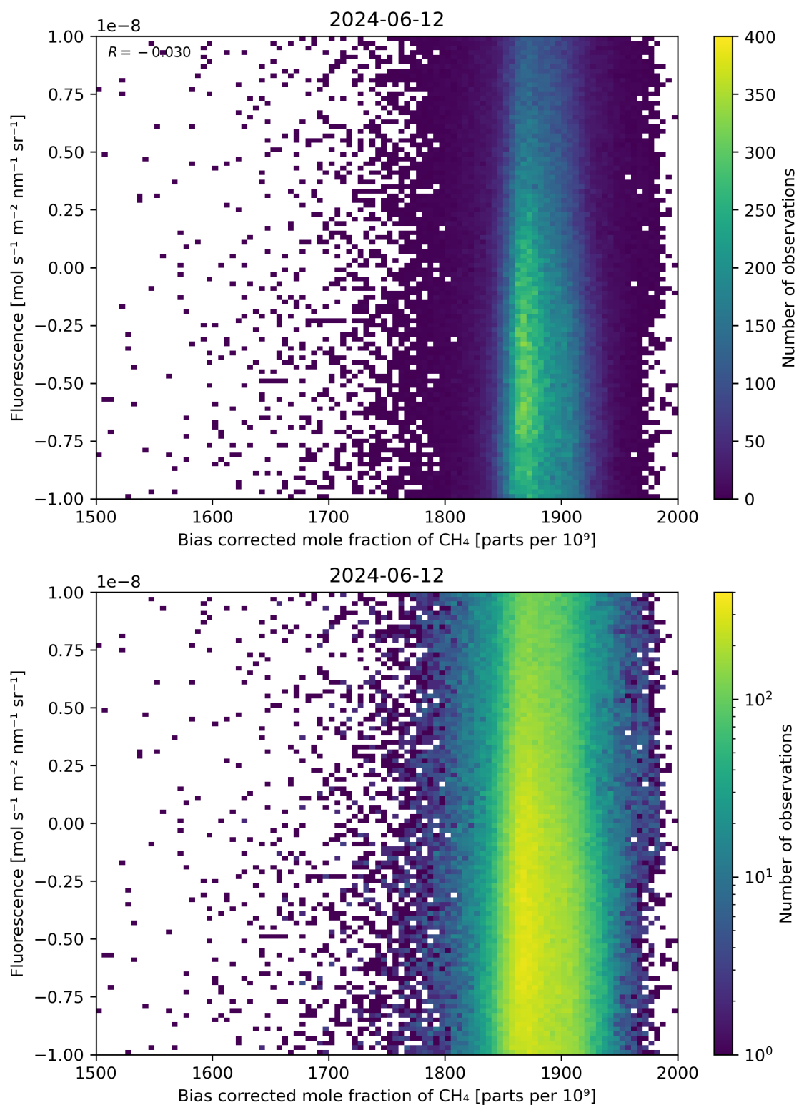
Figure 66: Scatter density plot of “Bias corrected mole fraction of \text{CH}_4 ” against “Fluorescence” for 2024-06-11 to 2024-06-13.
