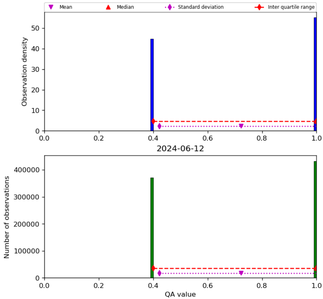
Figure 22: Histogram of “QA value” for 2024-06-11 to 2024-06-13
