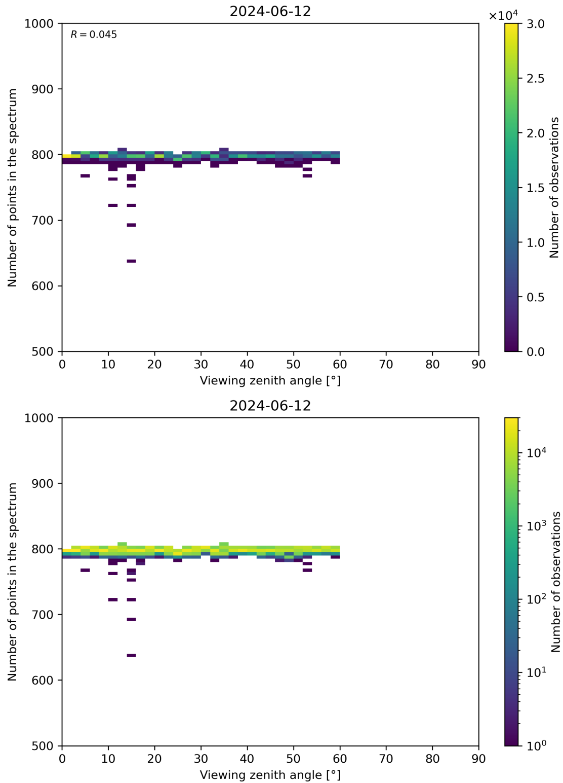
Figure 114: Scatter density plot of “Viewing zenith angle” against “Number of points in the spectrum” for 2024-06-11 to 2024-06-13.
