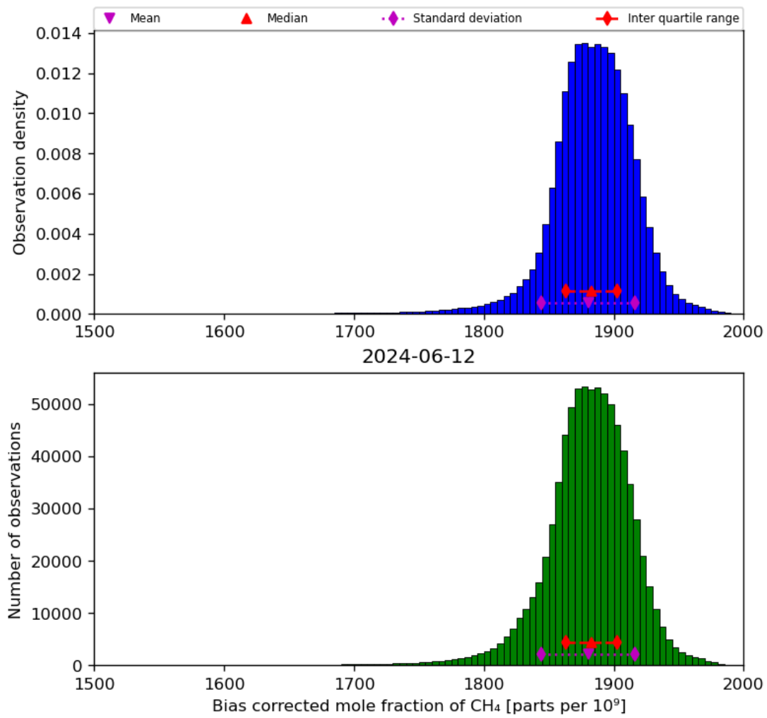
Figure 25: Histogram of “Bias corrected mole fraction of CH 4 ” for 2024-06-11 to 2024-06-13
