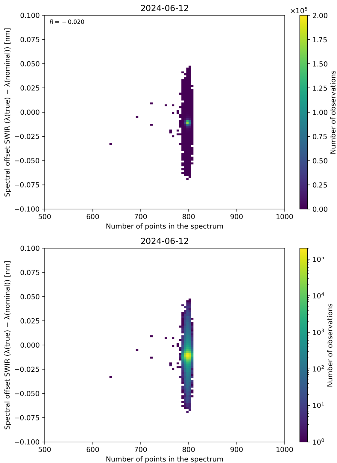
Figure 93: Scatter density plot of “Number of points in the spectrum” against “Spectral offset SWIR ( \lambda(\text{true}) - \lambda(\text{nominal}) )” for 2024-06-11 to 2024-06-13.
