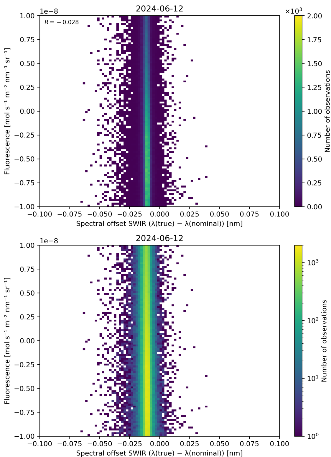
Figure 120: Scatter density plot of “Spectral offset SWIR ( \lambda(\text{true}) - \lambda(\text{nominal}) )” against “Fluorescence” for 2024-06-11 to 2024-06-13.
