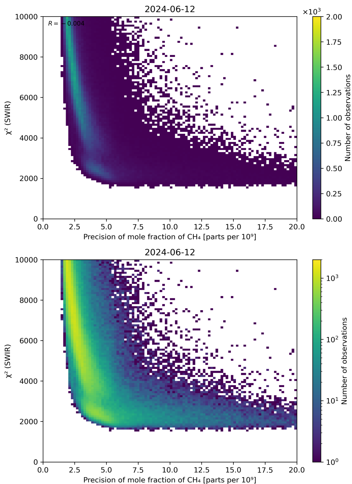
Figure 79: Scatter density plot of “Precision of mole fraction of CH 4 ” against “ \chi^2 (SWIR)” for 2024-06-11 to 2024-06-13.
