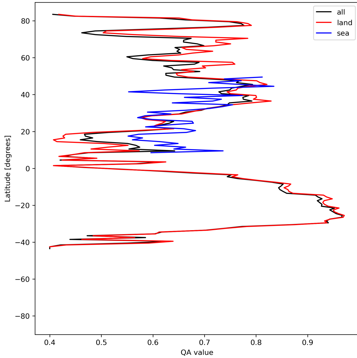
Figure 11: Zonal average of “QA value” for 2024-06-11 to 2024-06-13.
