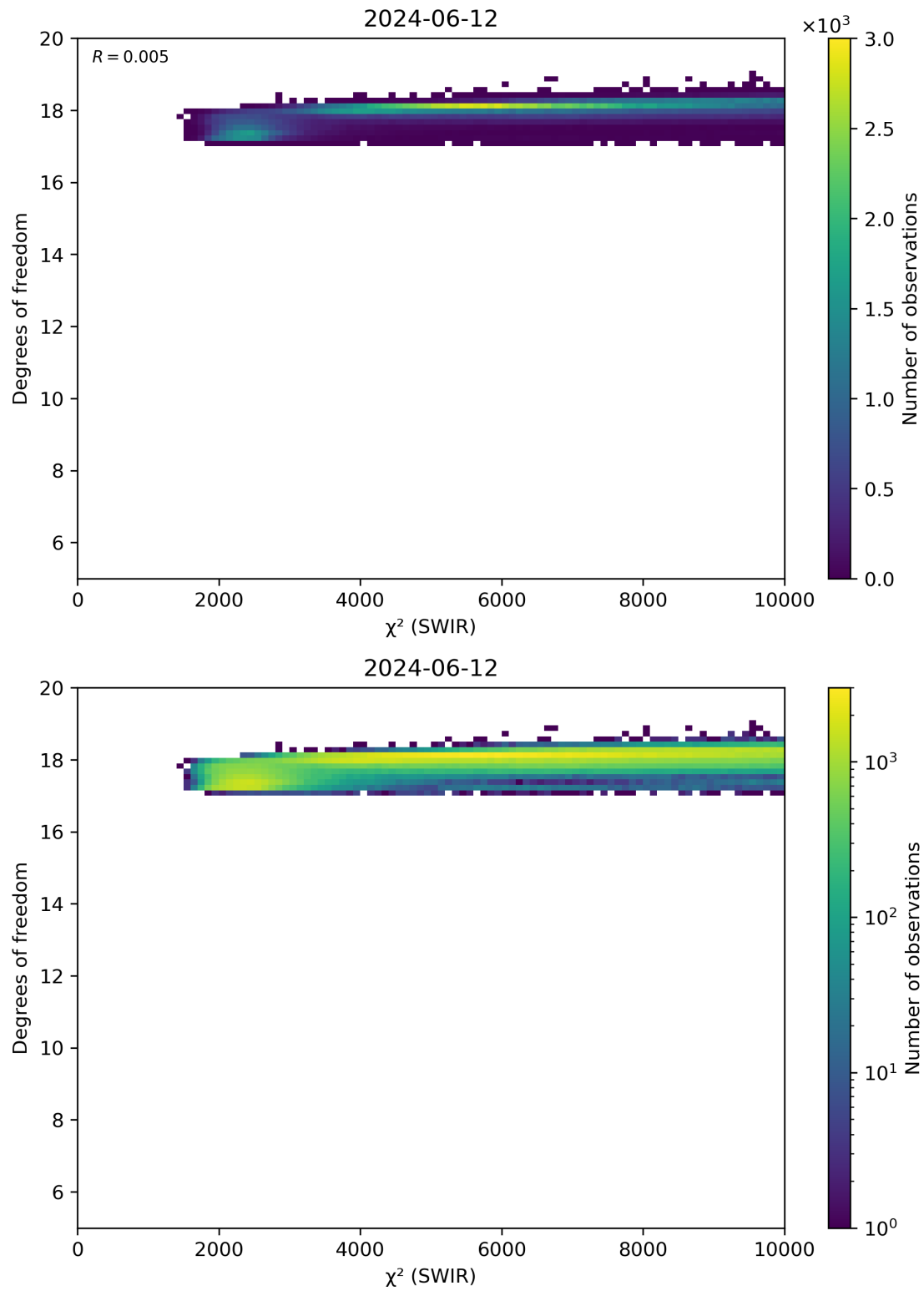
Figure 48: Scatter density plot of “ \chi^2 (SWIR)” against “Degrees of freedom” for 2024-06-11 to 2024-06-13.
