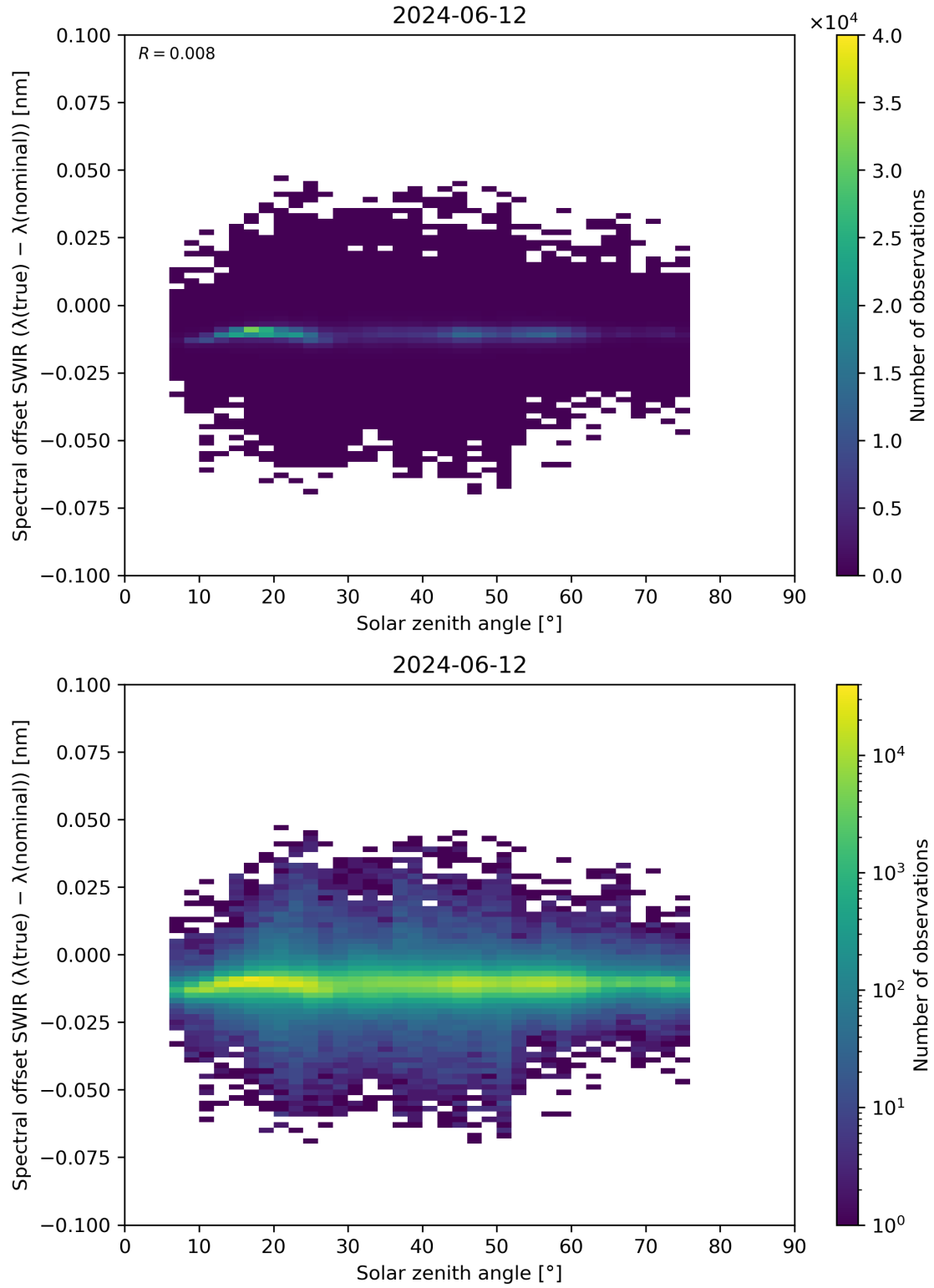
Figure 104: Scatter density plot of “Solar zenith angle” against “Spectral offset SWIR ( \lambda(\text{true}) - \lambda(\text{nominal}) )” for 2024-06-11 to 2024-06-13.
