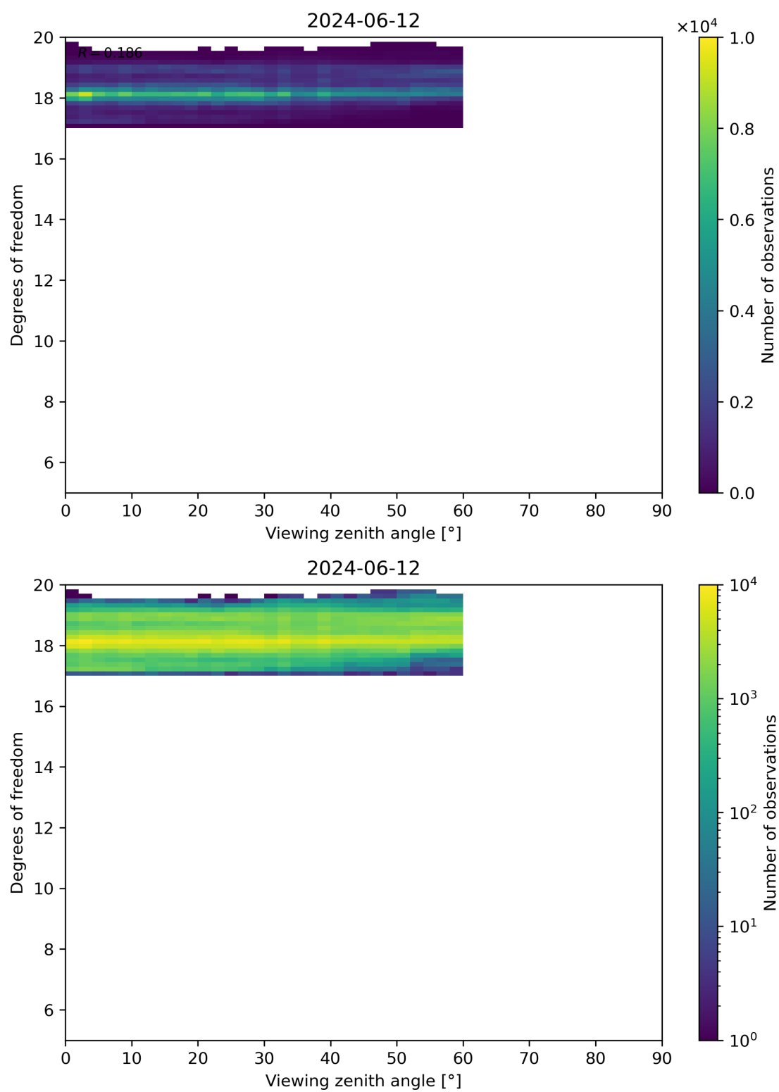
Figure 107: Scatter density plot of “Viewing zenith angle” against “Degrees of freedom” for 2024-06-11 to 2024-06-13.
