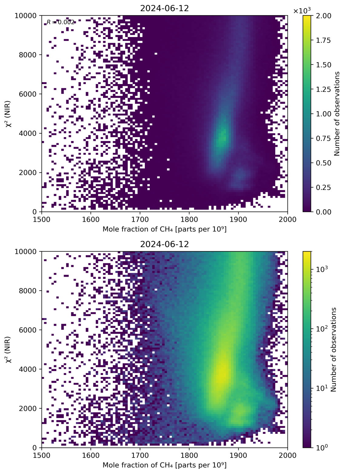
Figure 70: Scatter density plot of “Mole fraction of CH 4 ” against “ \chi^2 (NIR)” for 2024-06-11 to 2024-06-13.
