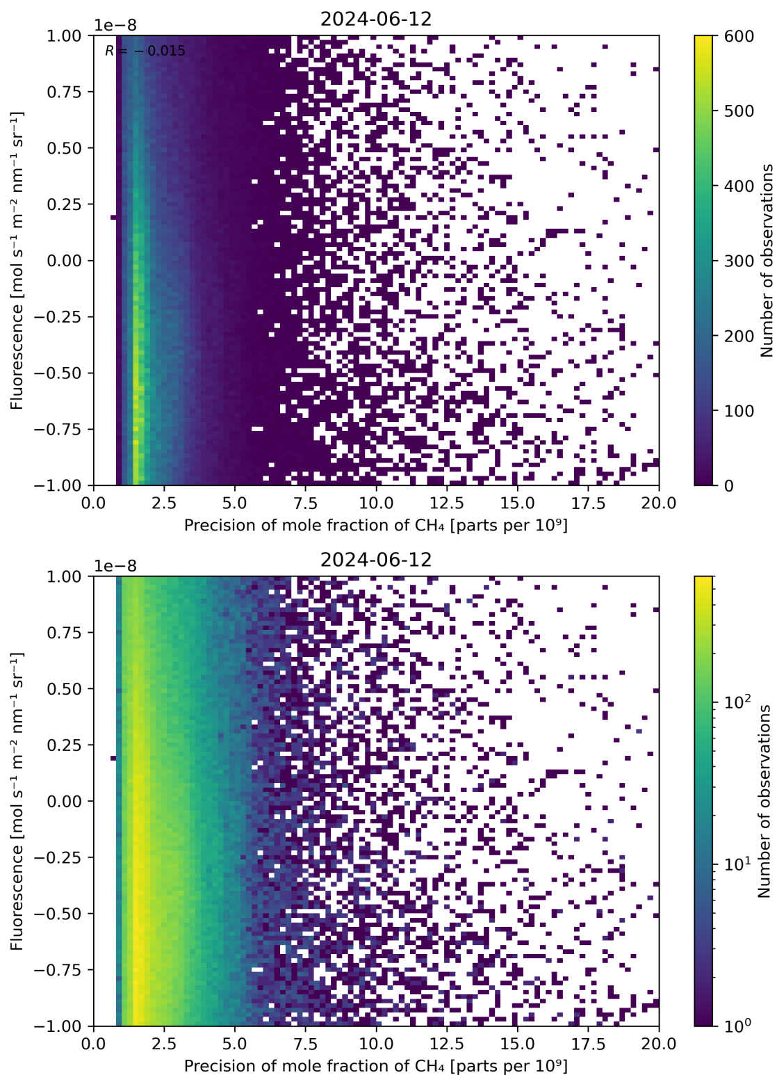
Figure 81: Scatter density plot of “Precision of mole fraction of CH 4 ” against “Fluorescence” for 2024-06-11 to 2024-06-13.
