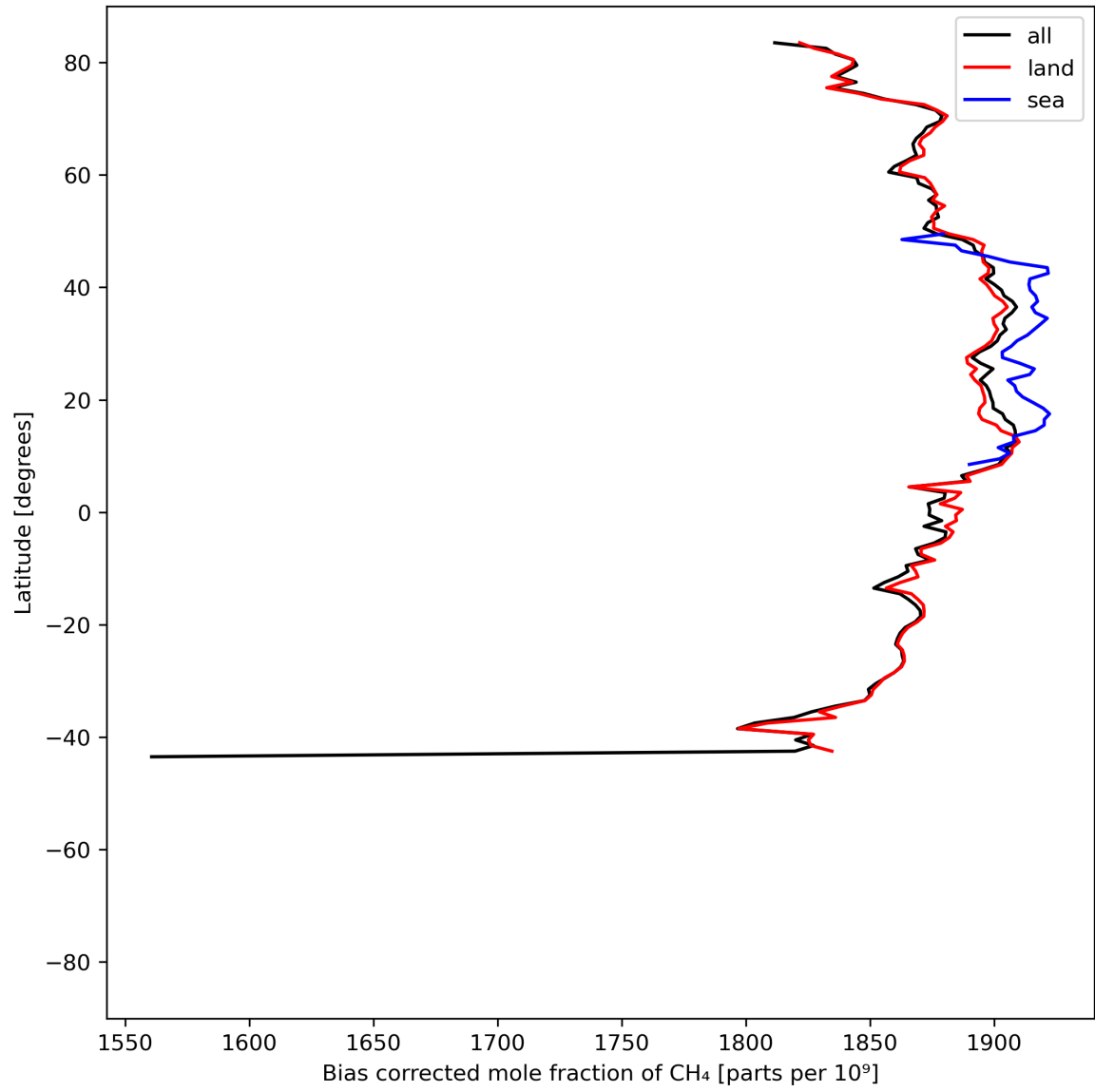
Figure 14: Zonal average of “Bias corrected mole fraction of CH 4 ” for 2024-06-11 to 2024-06-13.
