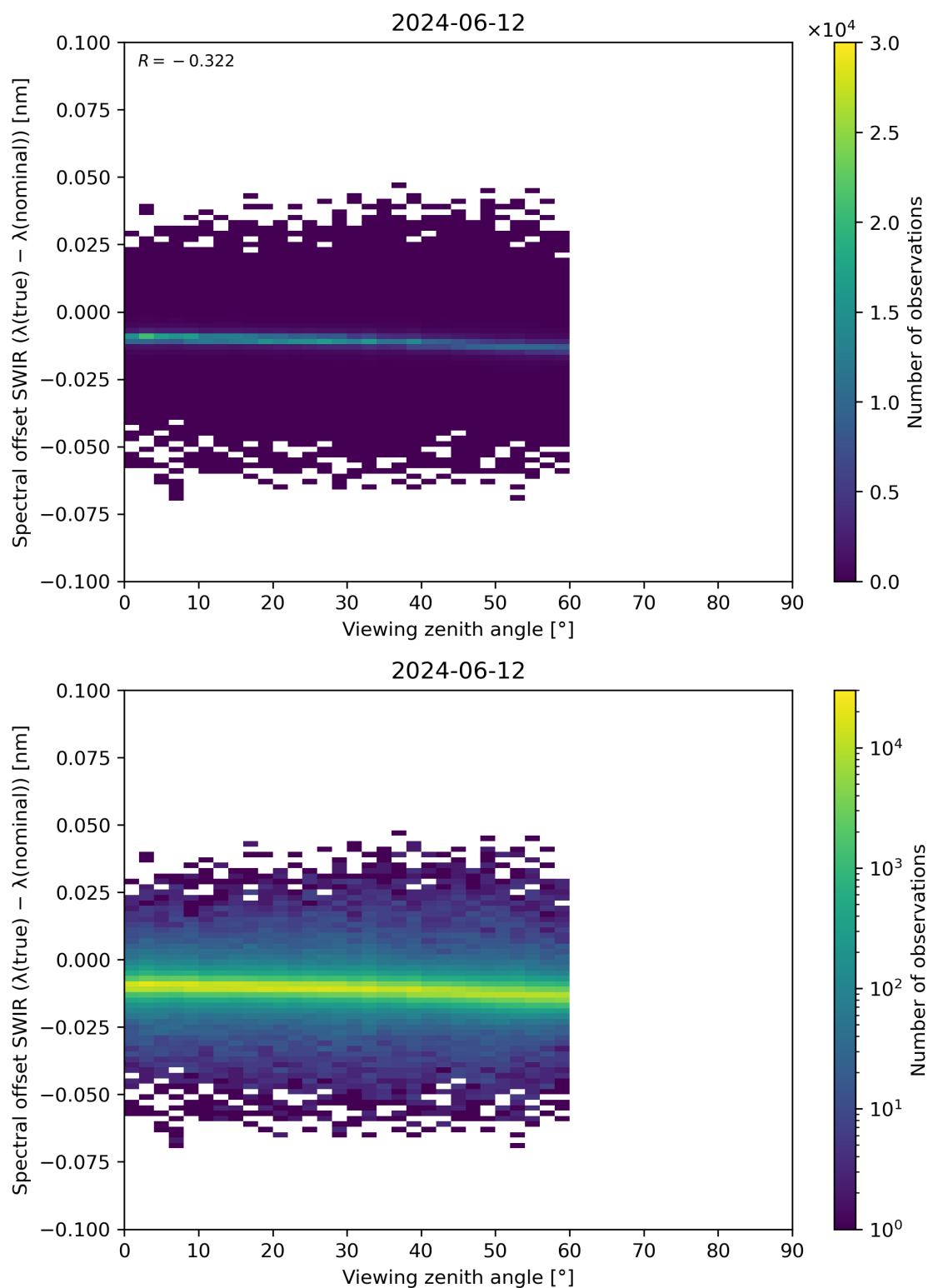
Figure 116: Scatter density plot of “Viewing zenith angle” against “Spectral offset SWIR ( \lambda(\text{true}) - \lambda(\text{nominal}) )” for 2024-06-11 to 2024-06-13.
