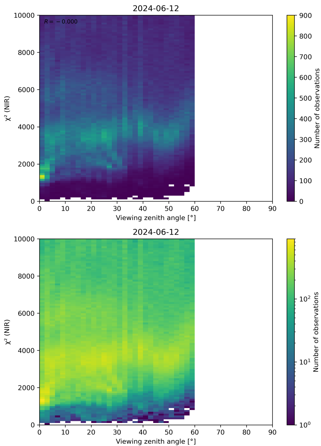
Figure 105: Scatter density plot of “Viewing zenith angle” against “ \chi^2 (NIR)” for 2024-06-11 to 2024-06-13.
