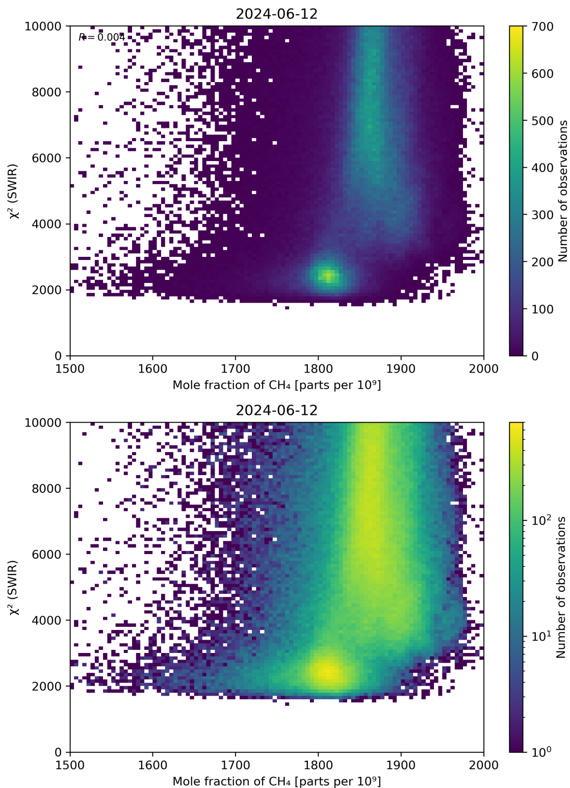
Figure 71: Scatter density plot of “Mole fraction of CH 4 ” against “ \chi^2 (SWIR)” for 2024-06-11 to 2024-06-13.
