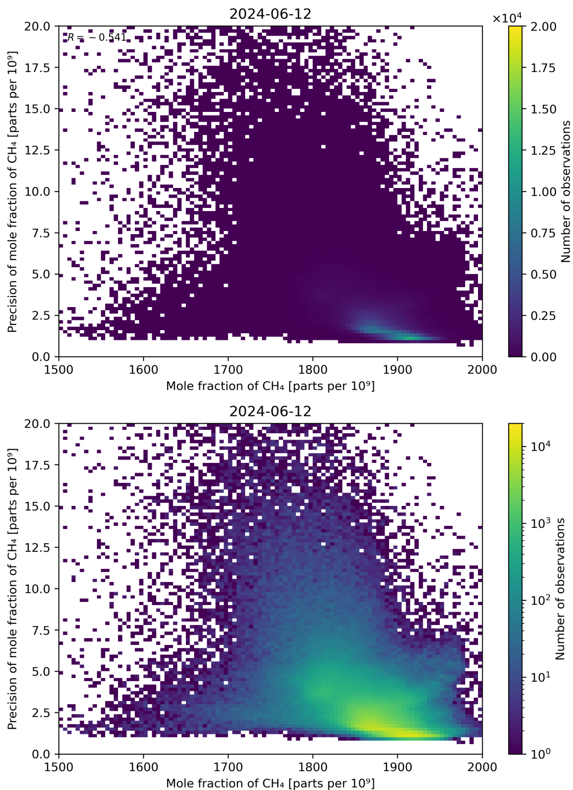
Figure 75: Scatter density plot of “Mole fraction of CH 4 ” against “Precision of mole fraction of CH 4 ” for 2024-06-11 to 2024-06-13.
