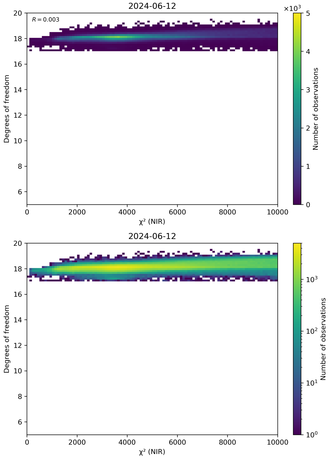
Figure 44: Scatter density plot of “ \chi^2 (NIR)” against “Degrees of freedom” for 2024-06-11 to 2024-06-13.
