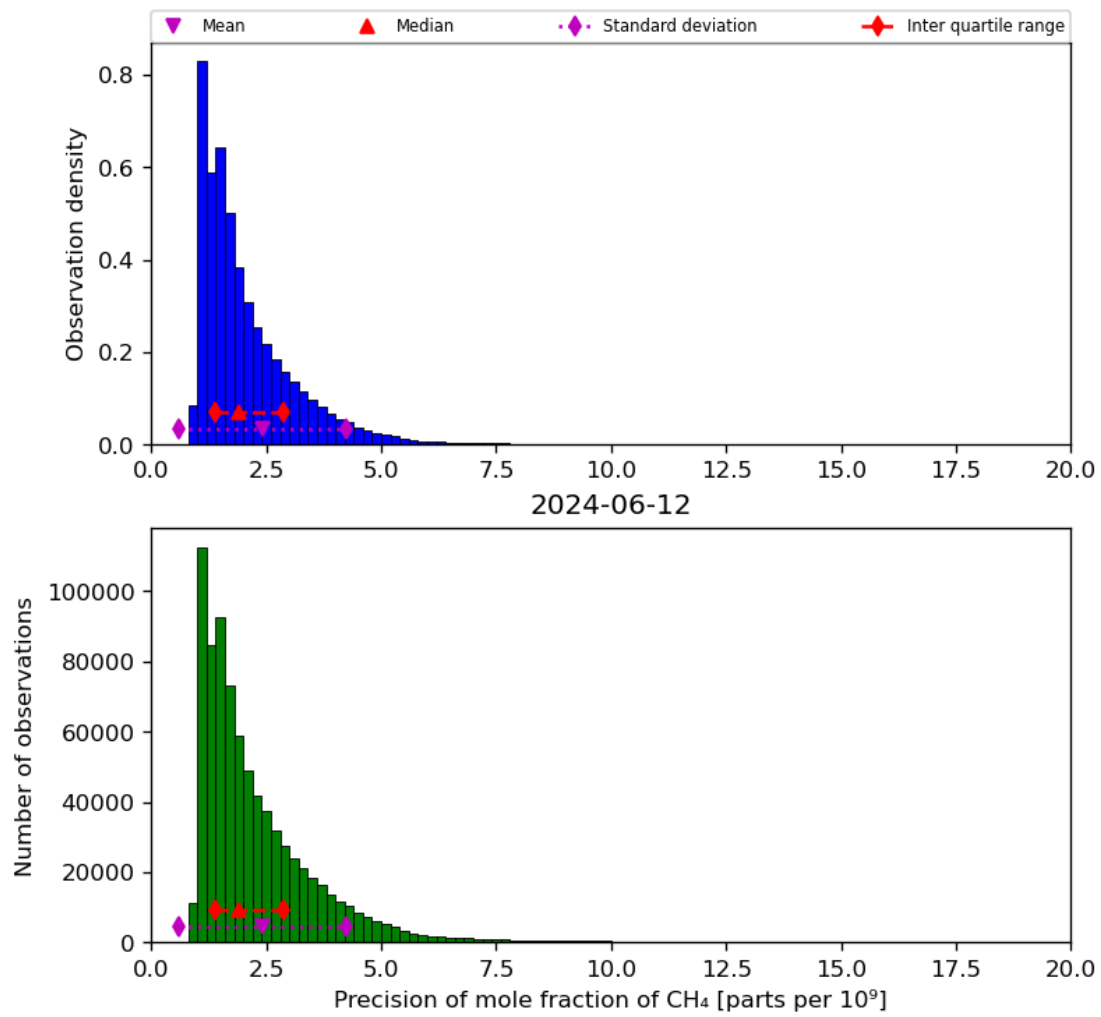
Figure 24: Histogram of “Precision of mole fraction of CH 4 ” for 2024-06-11 to 2024-06-13
