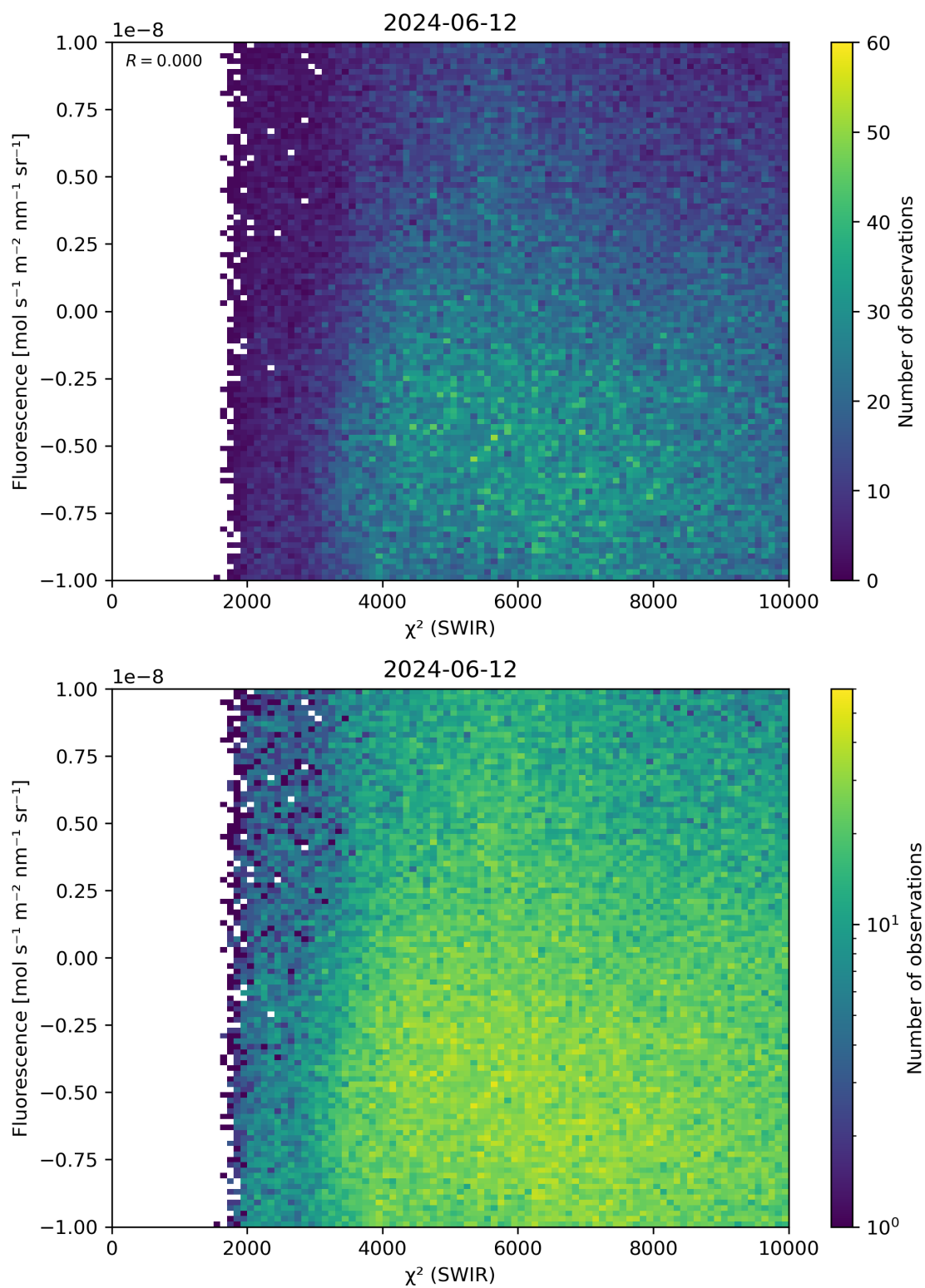
Figure 49: Scatter density plot of “ \chi^2 (SWIR)” against “Fluorescence” for 2024-06-11 to 2024-06-13.
