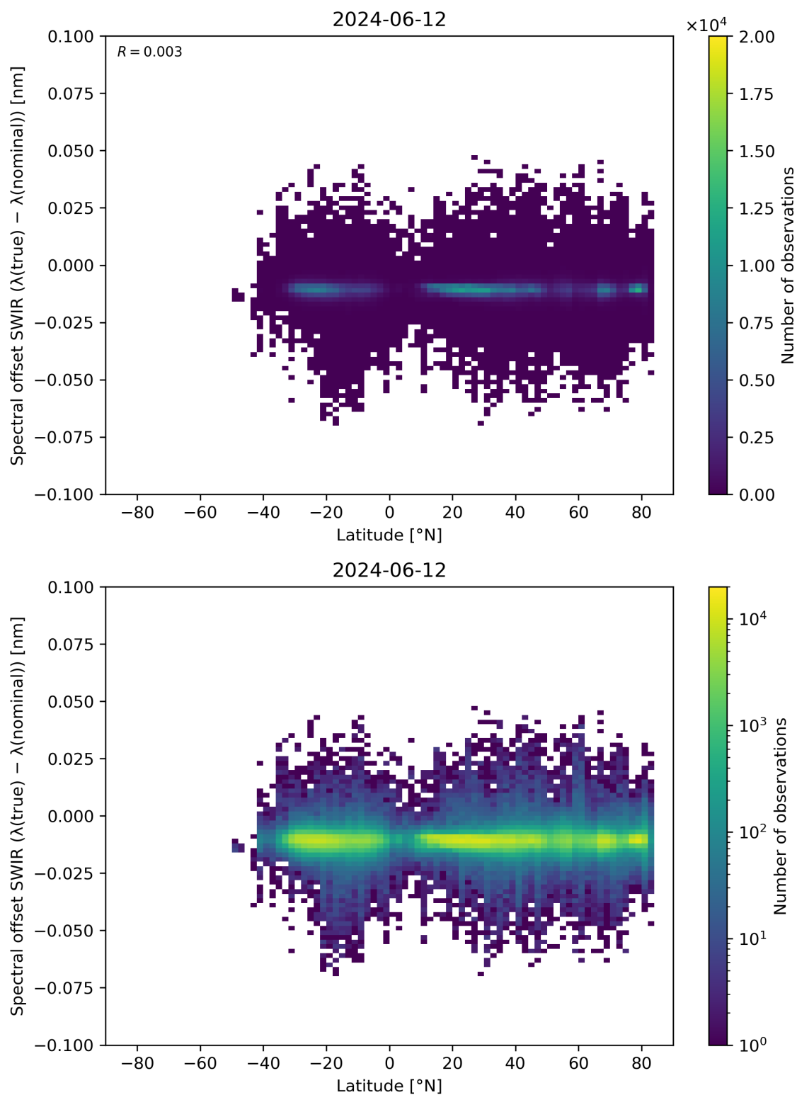
Figure 62: Scatter density plot of “Latitude” against “Spectral offset SWIR ( \lambda(\text{true}) - \lambda(\text{nominal}) )” for 2024-06-11 to 2024-06-13.
