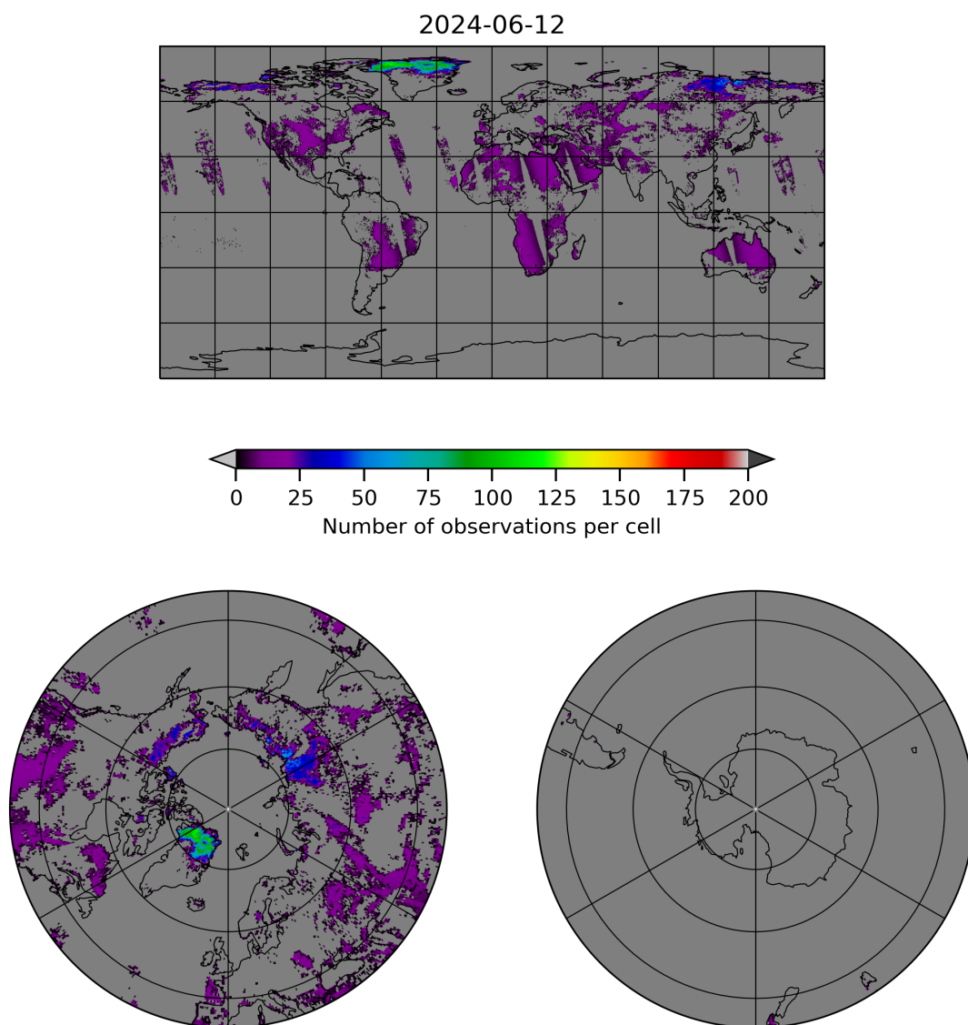
Figure 10: Map of the number of observations for 2024-06-11 to 2024-06-13
