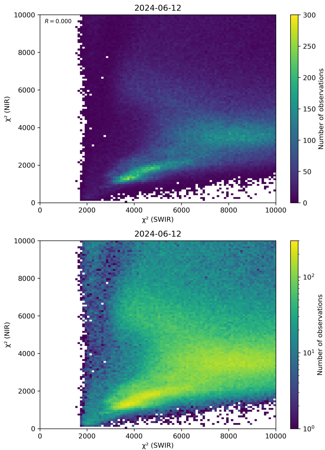
Figure 47: Scatter density plot of “ \chi^2 (SWIR)” against “ \chi^2 (NIR)” for 2024-06-11 to 2024-06-13.
