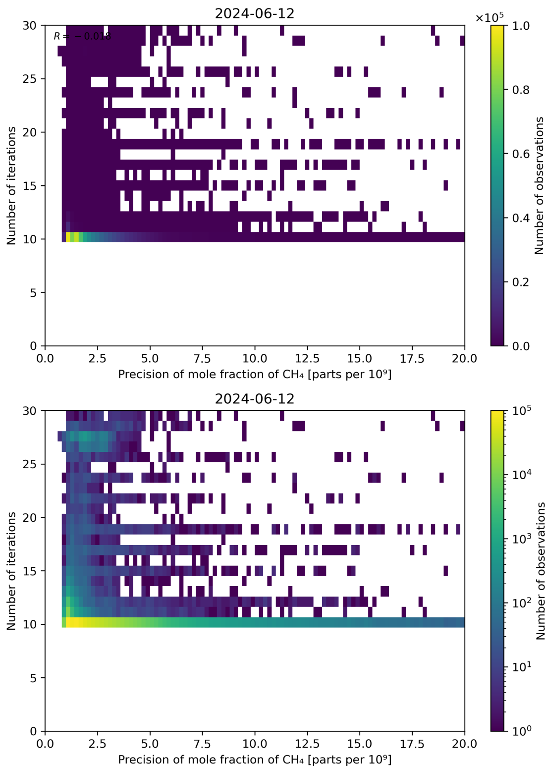
Figure 83: Scatter density plot of “Precision of mole fraction of CH 4 ” against “Number of iterations” for 2024-06-11 to 2024-06-13.
