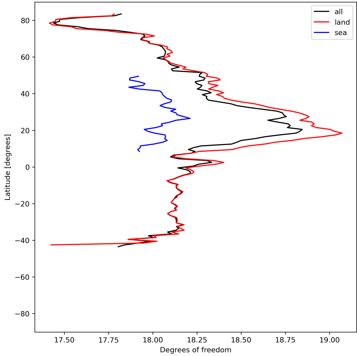
Figure 19: Zonal average of “Degrees of freedom” for 2024-06-11 to 2024-06-13.
