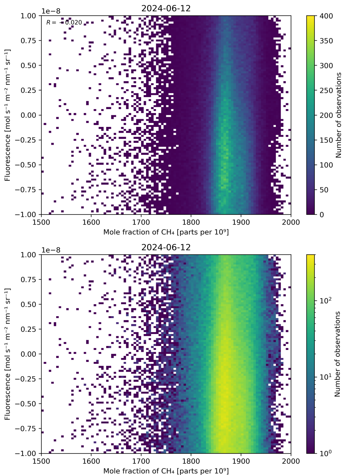
Figure 73: Scatter density plot of “Mole fraction of \text{CH}_4 ” against “Fluorescence” for 2024-06-11 to 2024-06-13.
