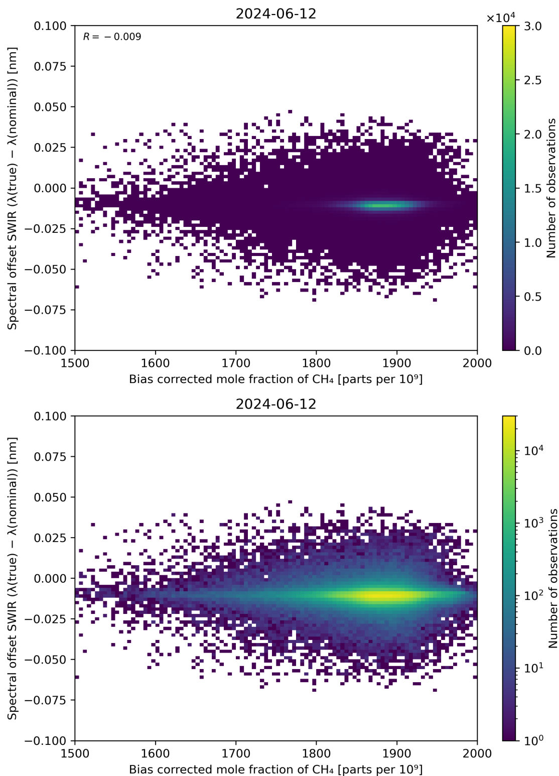
Figure 69: Scatter density plot of “Bias corrected mole fraction of \text{CH}_4 ” against “Spectral offset SWIR ( \lambda(\text{true}) - \lambda(\text{nominal}) )” for 2024-06-11 to 2024-06-13.
