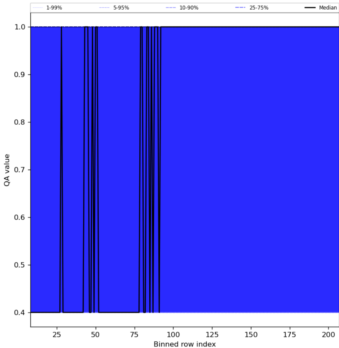
Figure 33: Along track statistics of “QA value” for 2024-06-11 to 2024-06-13
