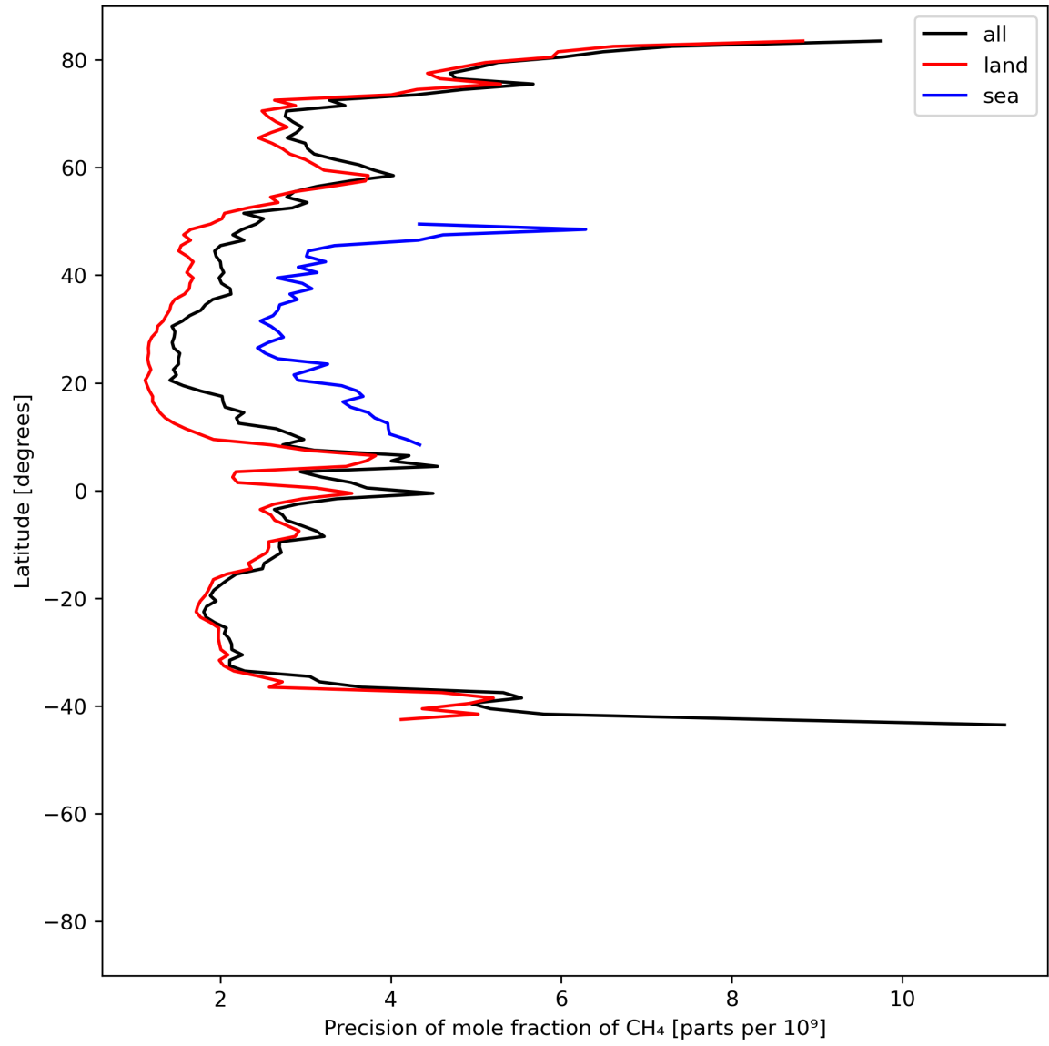
Figure 13: Zonal average of “Precision of mole fraction of CH 4 ” for 2024-06-11 to 2024-06-13.
