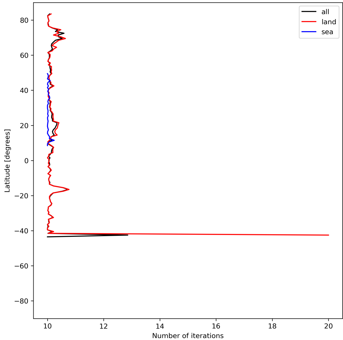
Figure 20: Zonal average of “Number of iterations” for 2024-06-11 to 2024-06-13.
