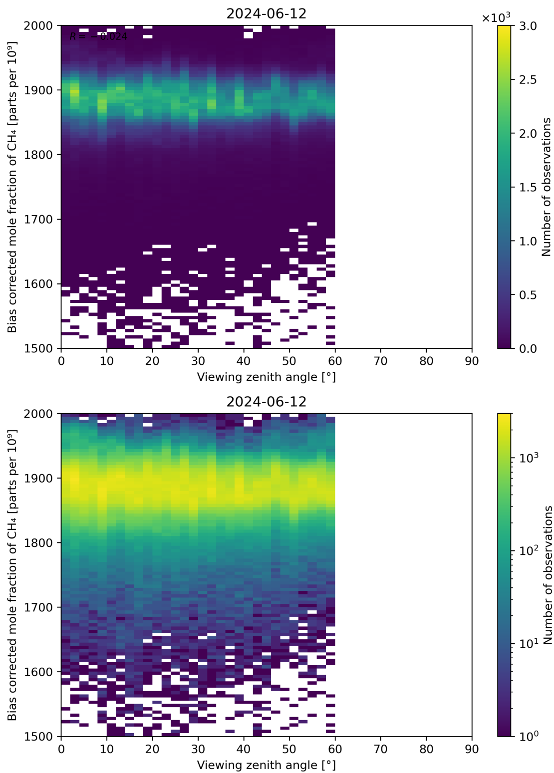
Figure 111: Scatter density plot of “Viewing zenith angle” against “Bias corrected mole fraction of CH 4 ” for 2024-06-11 to 2024-06-13.
