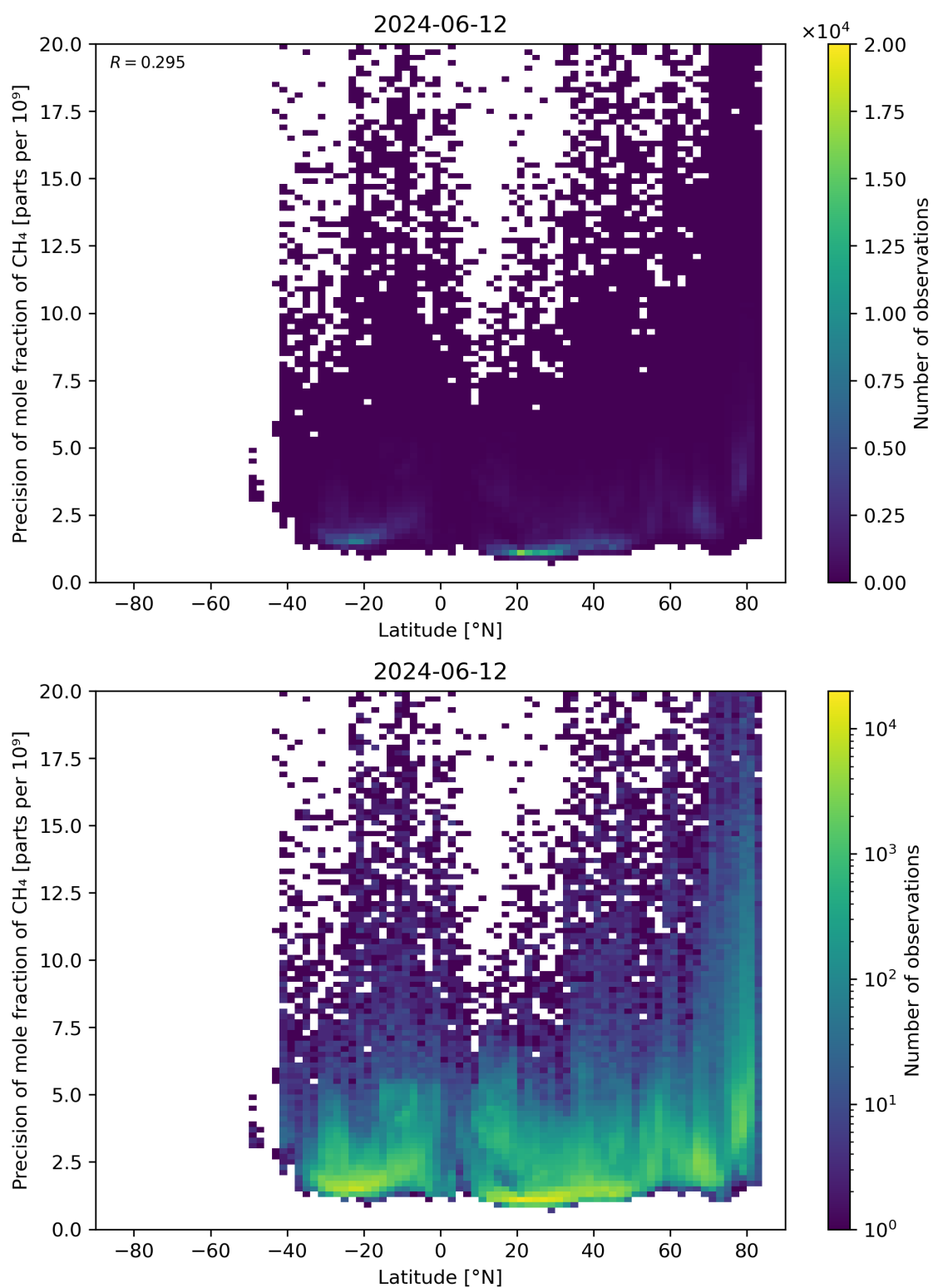
Figure 59: Scatter density plot of “Latitude” against “Precision of mole fraction of \text{CH}_4 ” for 2024-06-11 to 2024-06-13.
