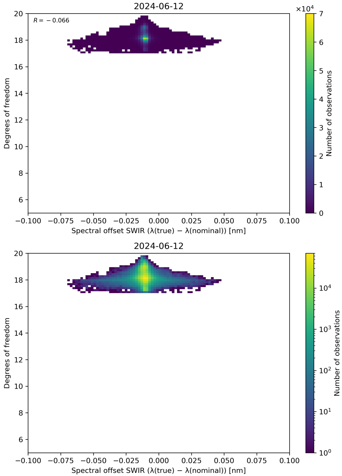
Figure 119: Scatter density plot of “Spectral offset SWIR ( \lambda(\text{true}) - \lambda(\text{nominal}) )” against “Degrees of freedom” for 2024-06-11 to 2024-06-13.
