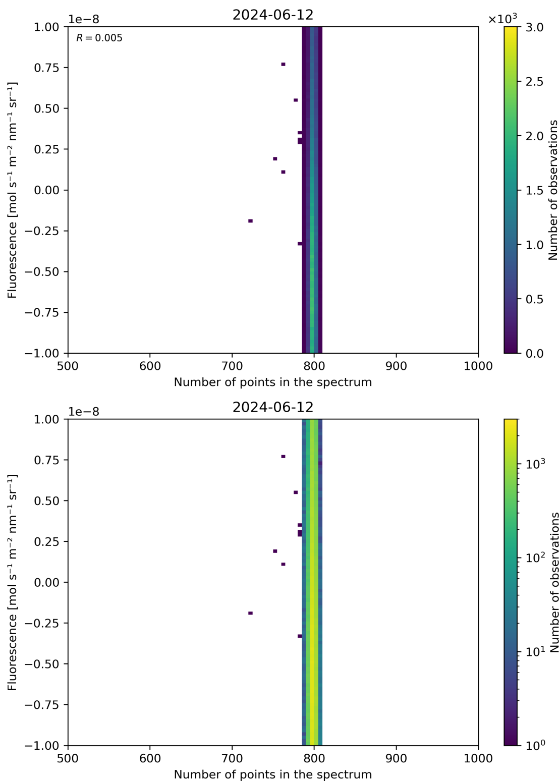
Figure 91: Scatter density plot of “Number of points in the spectrum” against “Fluorescence” for 2024-06-11 to 2024-06-13.
