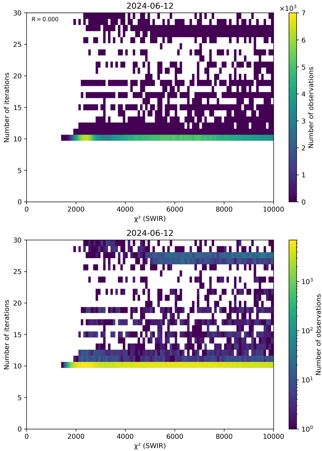
Figure 50: Scatter density plot of “ \chi^2 (SWIR)” against “Number of iterations” for 2024-06-11 to 2024-06-13.
