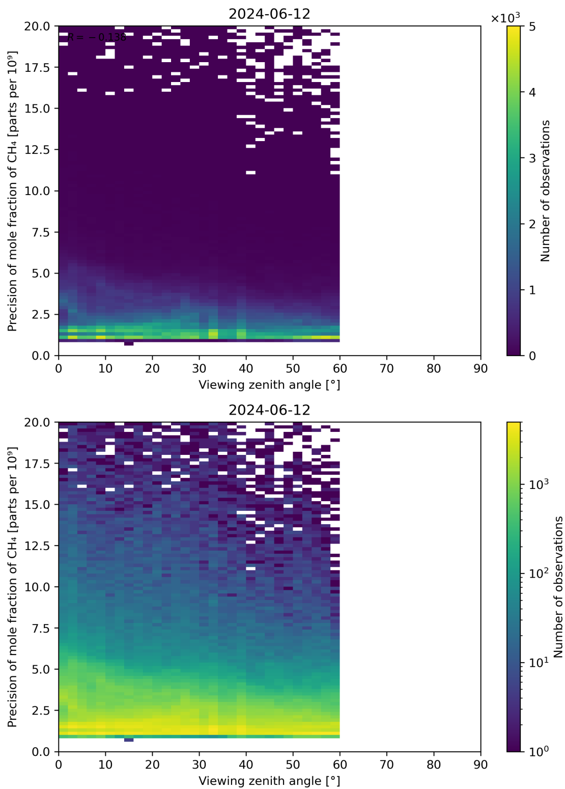
Figure 112: Scatter density plot of “Viewing zenith angle” against “Precision of mole fraction of CH 4 ” for 2024-06-11 to 2024-06-13.
