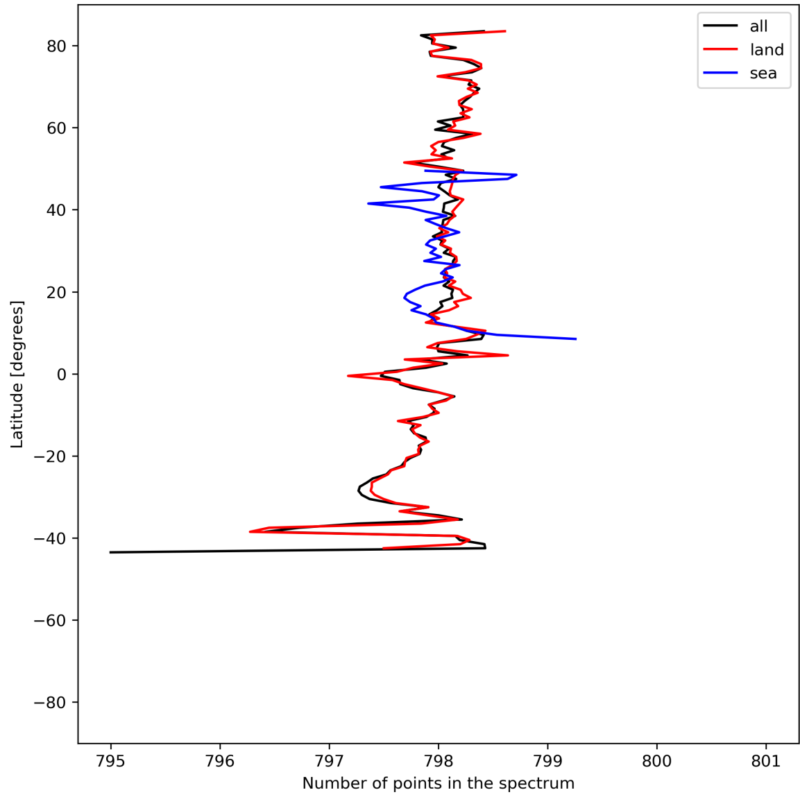
Figure 15: Zonal average of “Number of points in the spectrum” for 2024-06-11 to 2024-06-13.
