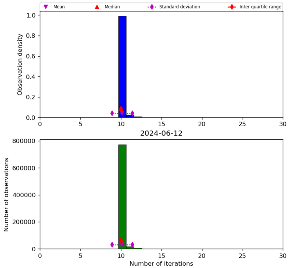
Figure 31: Histogram of “Number of iterations” for 2024-06-11 to 2024-06-13
