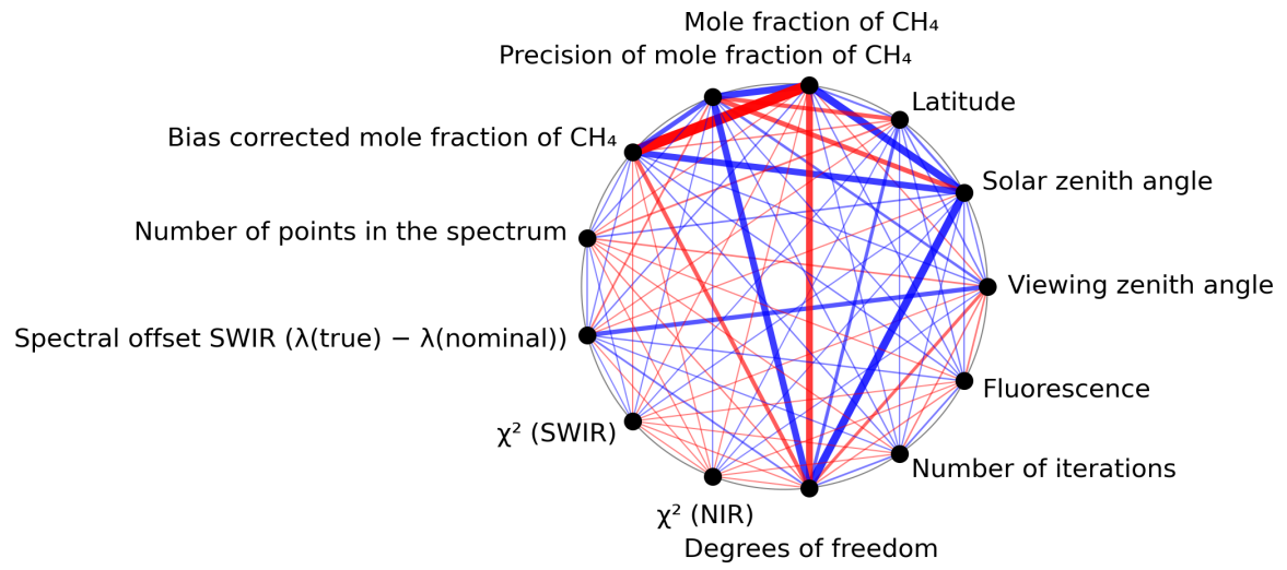
Figure 1: Map of correlation graph for 2024-06-11 to 2024-06-13.
