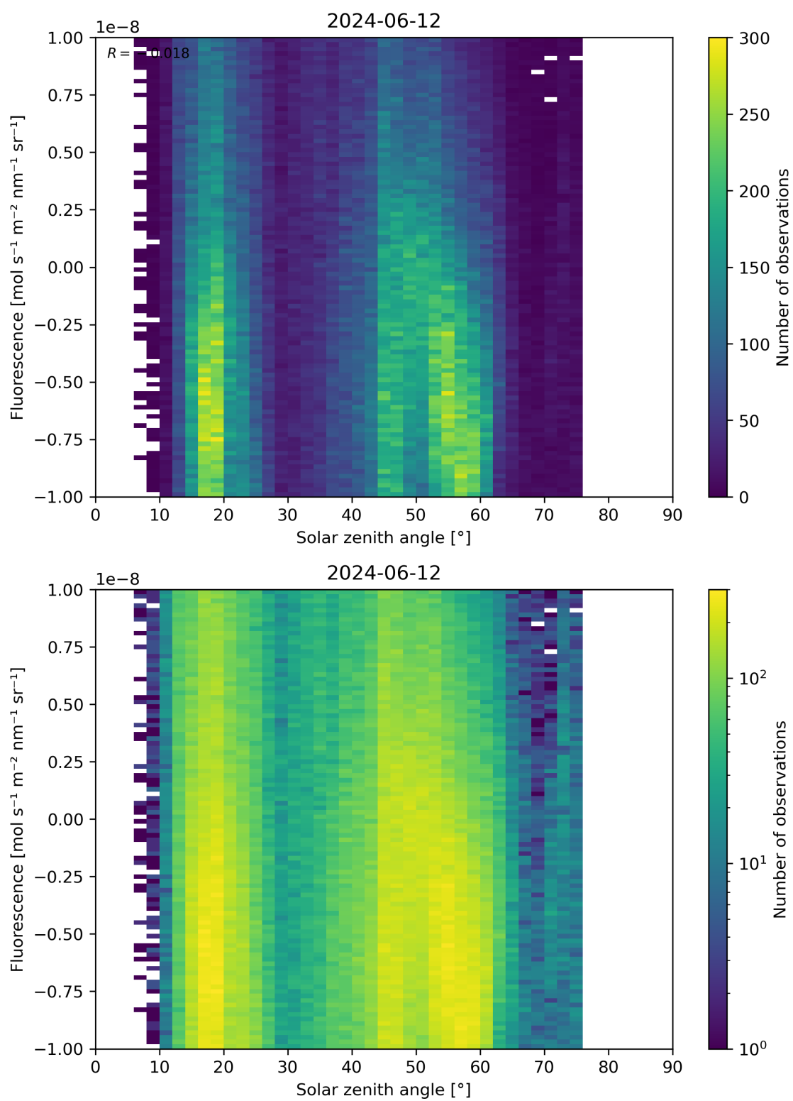
Figure 97: Scatter density plot of “Solar zenith angle” against “Fluorescence” for 2024-06-11 to 2024-06-13.
