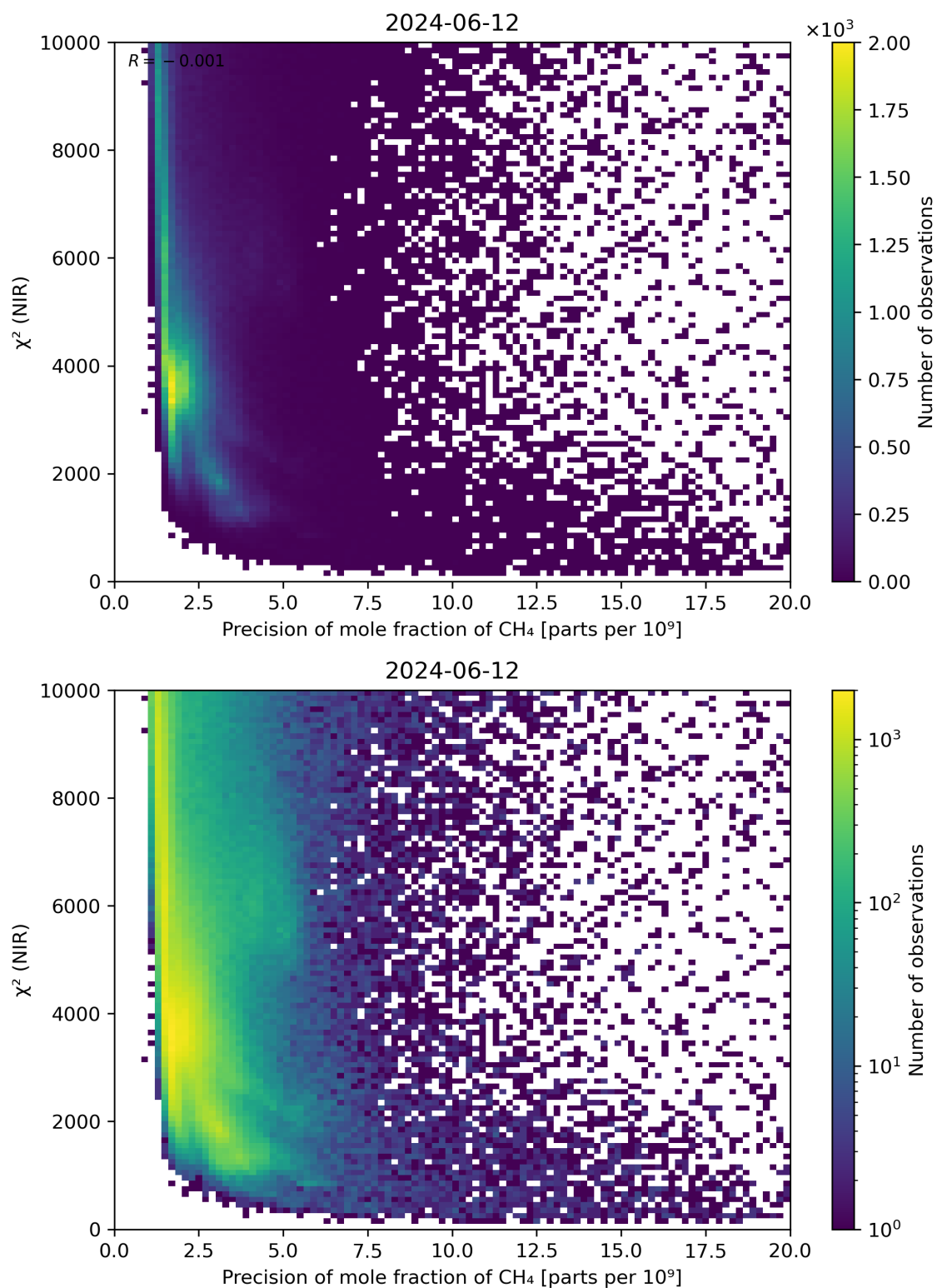
Figure 78: Scatter density plot of “Precision of mole fraction of \text{CH}_4 ” against “ \chi^2 (NIR)” for 2024-06-11 to 2024-06-13.
