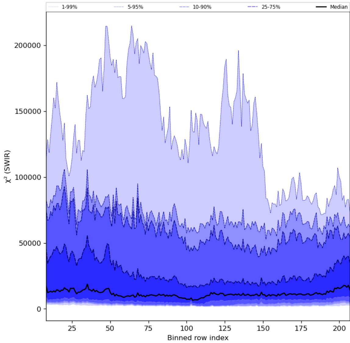
Figure 39: Along track statistics of “ \chi^2 (SWIR)” for 2024-06-11 to 2024-06-13
