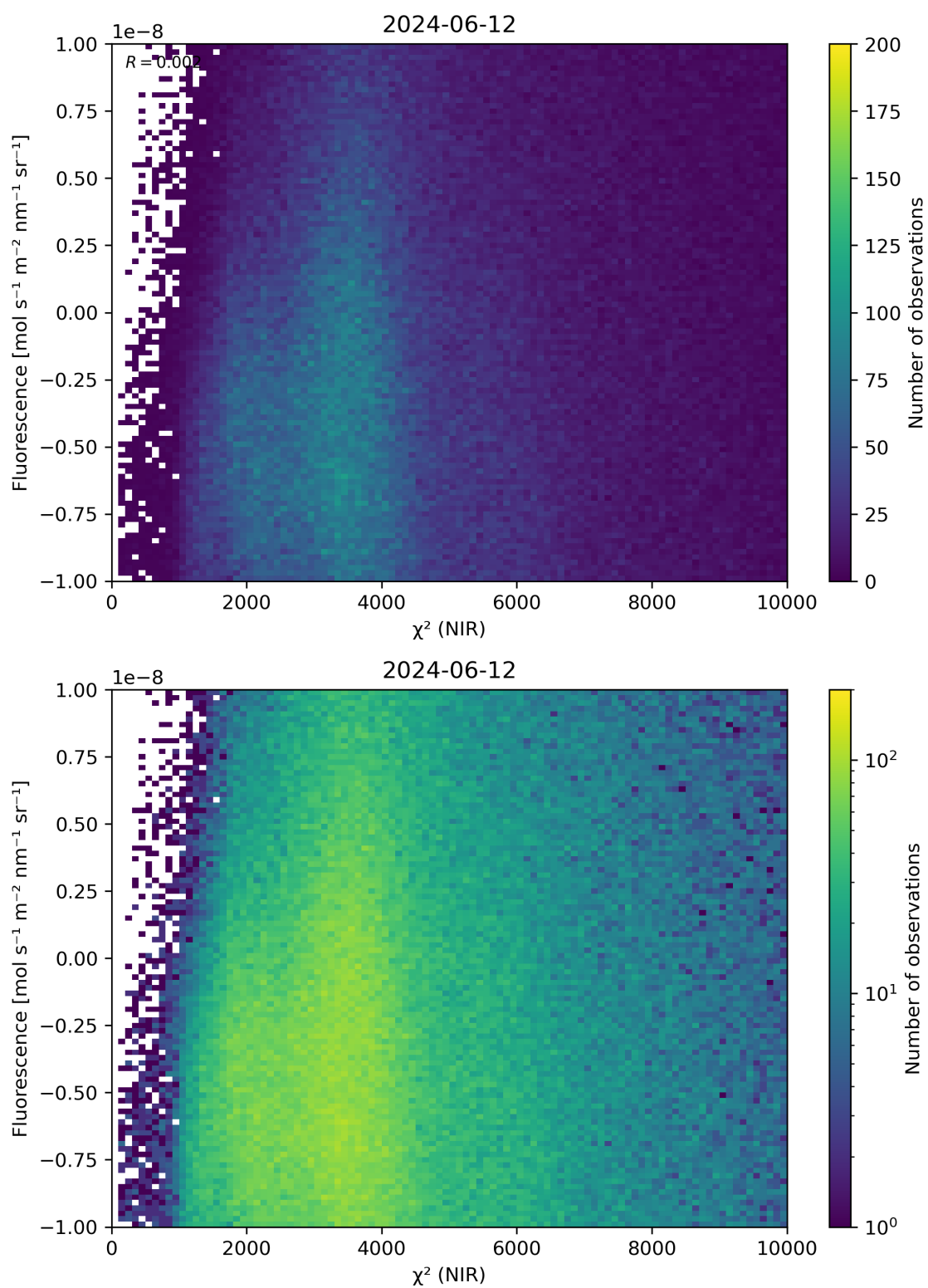
Figure 45: Scatter density plot of “ \chi^2 (NIR)” against “Fluorescence” for 2024-06-11 to 2024-06-13.
