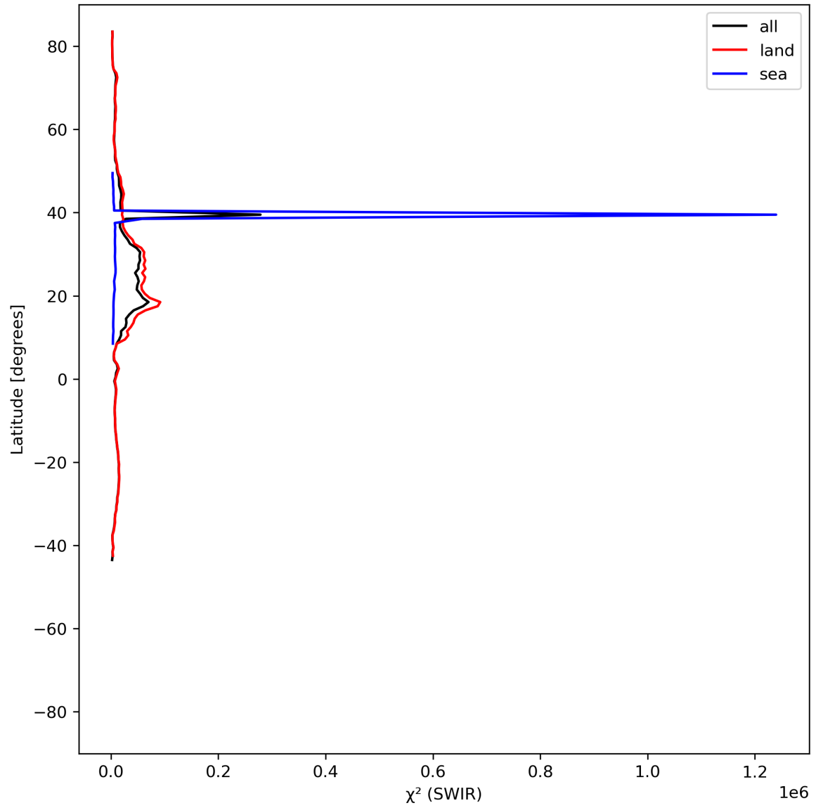
Figure 17: Zonal average of “ \chi^2 (SWIR)” for 2024-06-11 to 2024-06-13.
