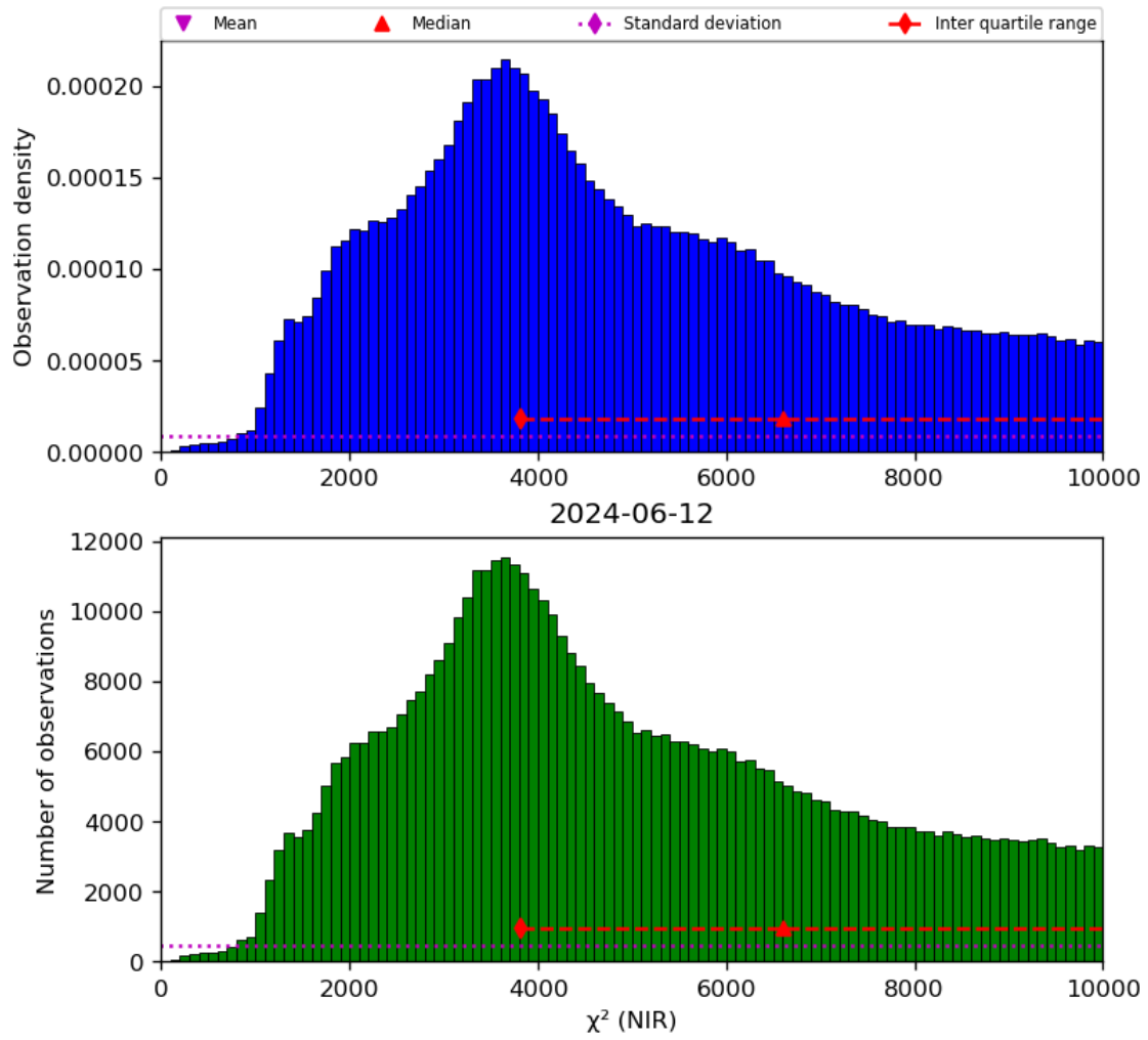
Figure 29: Histogram of “ \chi^2 (NIR)” for 2024-06-11 to 2024-06-13
