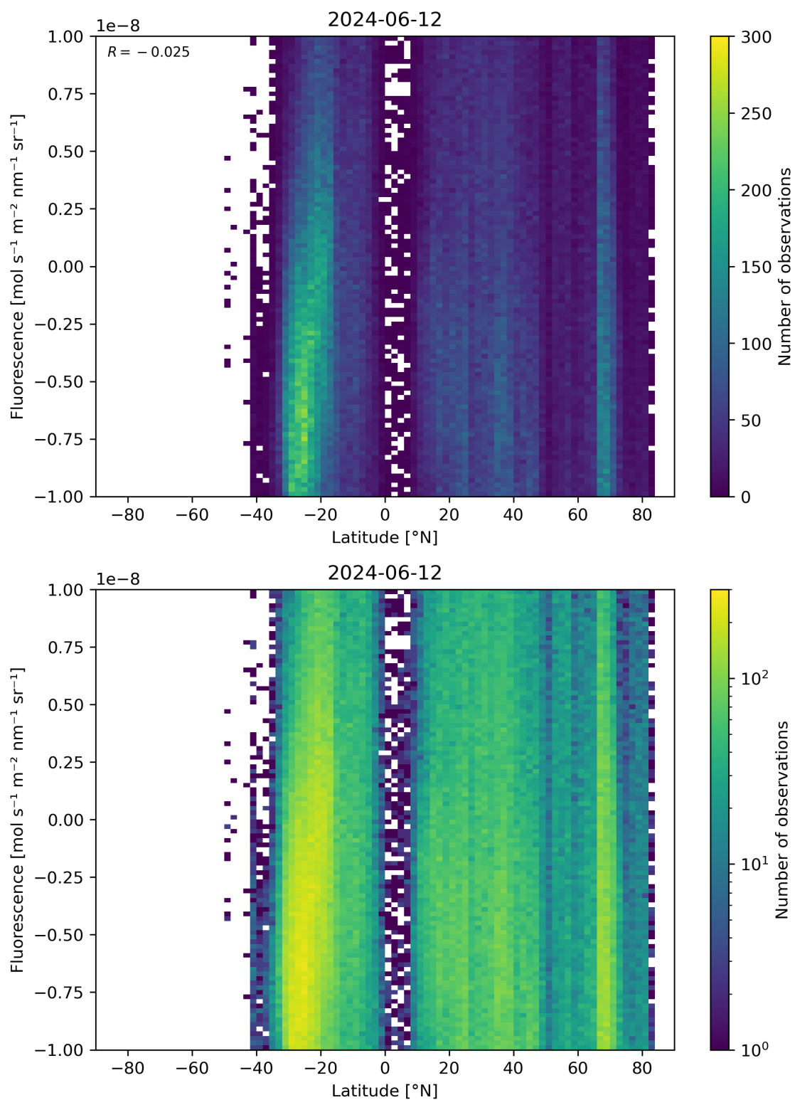
Figure 56: Scatter density plot of “Latitude” against “Fluorescence” for 2024-06-11 to 2024-06-13.
