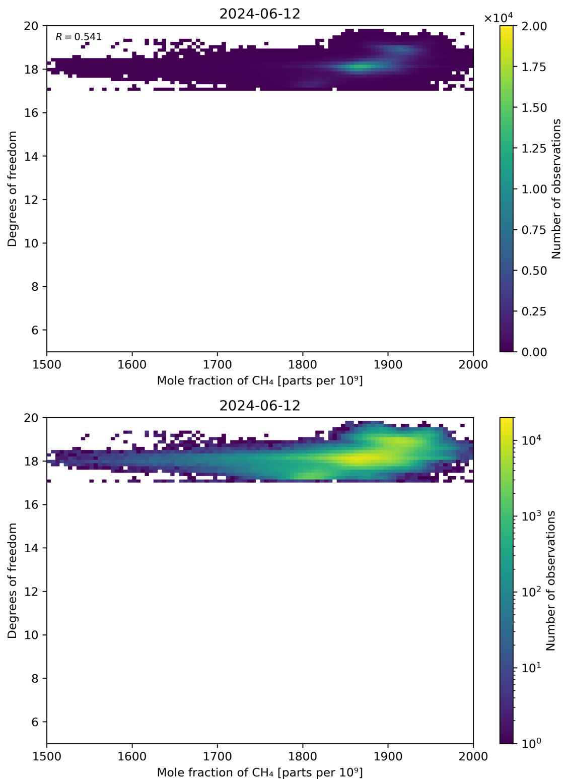
Figure 72: Scatter density plot of “Mole fraction of CH 4 ” against “Degrees of freedom” for 2024-06-11 to 2024-06-13.
