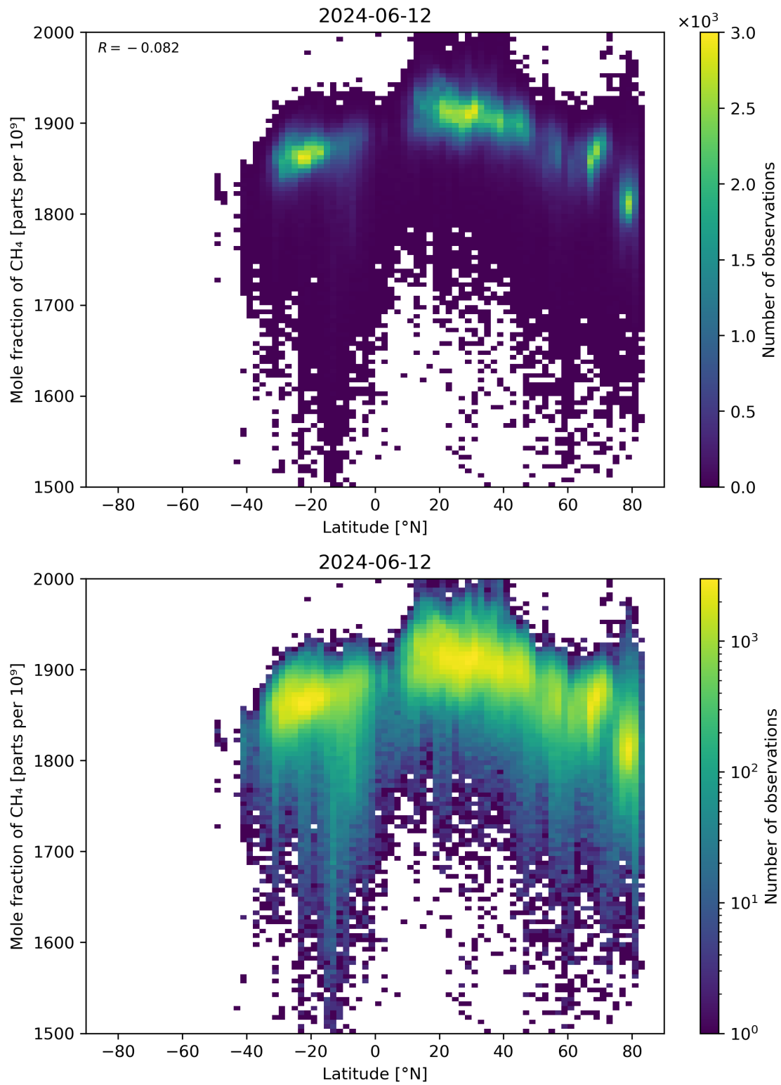
Figure 57: Scatter density plot of “Latitude” against “Mole fraction of \text{CH}_4 ” for 2024-06-11 to 2024-06-13.
