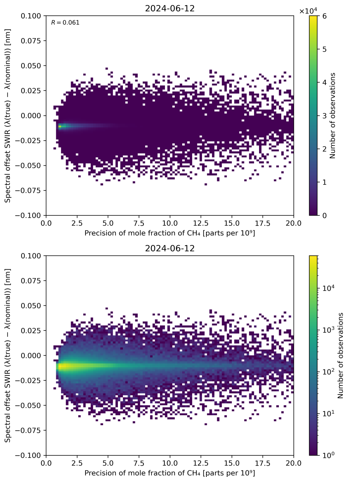
Figure 85: Scatter density plot of “Precision of mole fraction of CH 4 ” against “Spectral offset SWIR ( \lambda(\text{true}) - \lambda(\text{nominal}) )” for 2024-06-11 to 2024-06-13.
