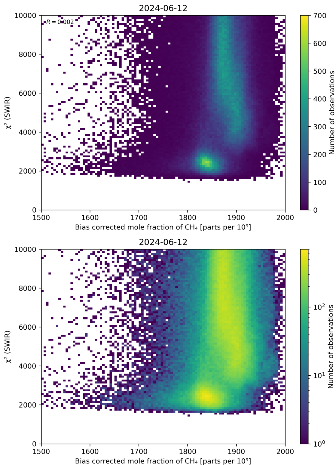
Figure 64: Scatter density plot of “Bias corrected mole fraction of CH 4 ” against “ \chi^2 (SWIR)” for 2024-06-11 to 2024-06-13.
