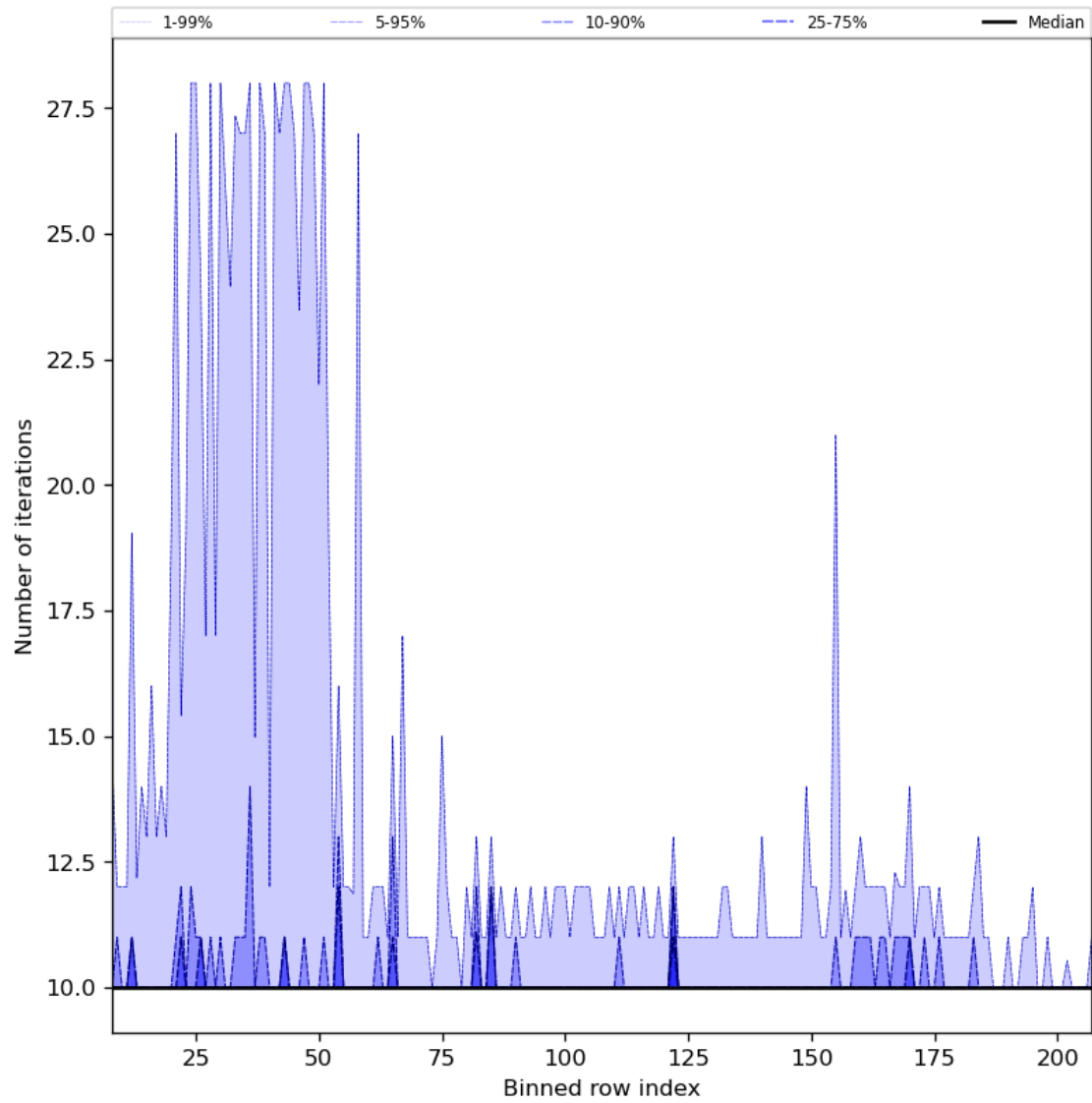
Figure 42: Along track statistics of “Number of iterations” for 2024-06-11 to 2024-06-13
