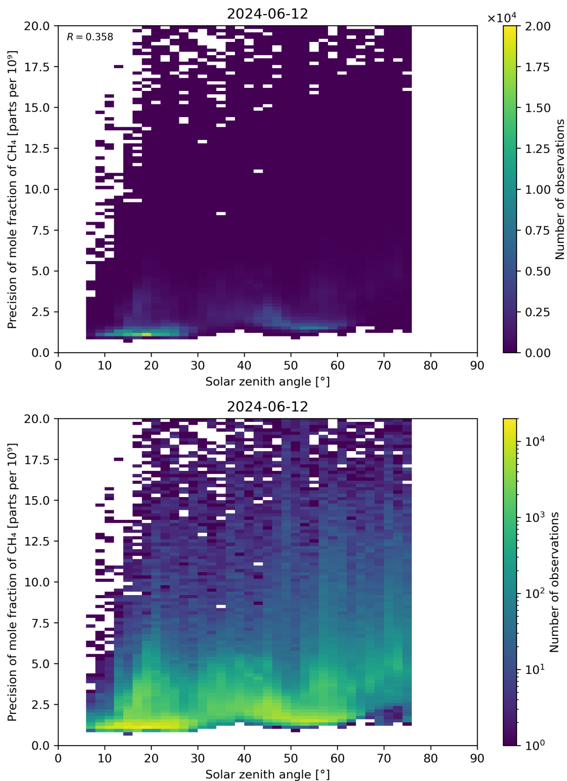
Figure 101: Scatter density plot of “Solar zenith angle” against “Precision of mole fraction of CH 4 ” for 2024-06-11 to 2024-06-13.
