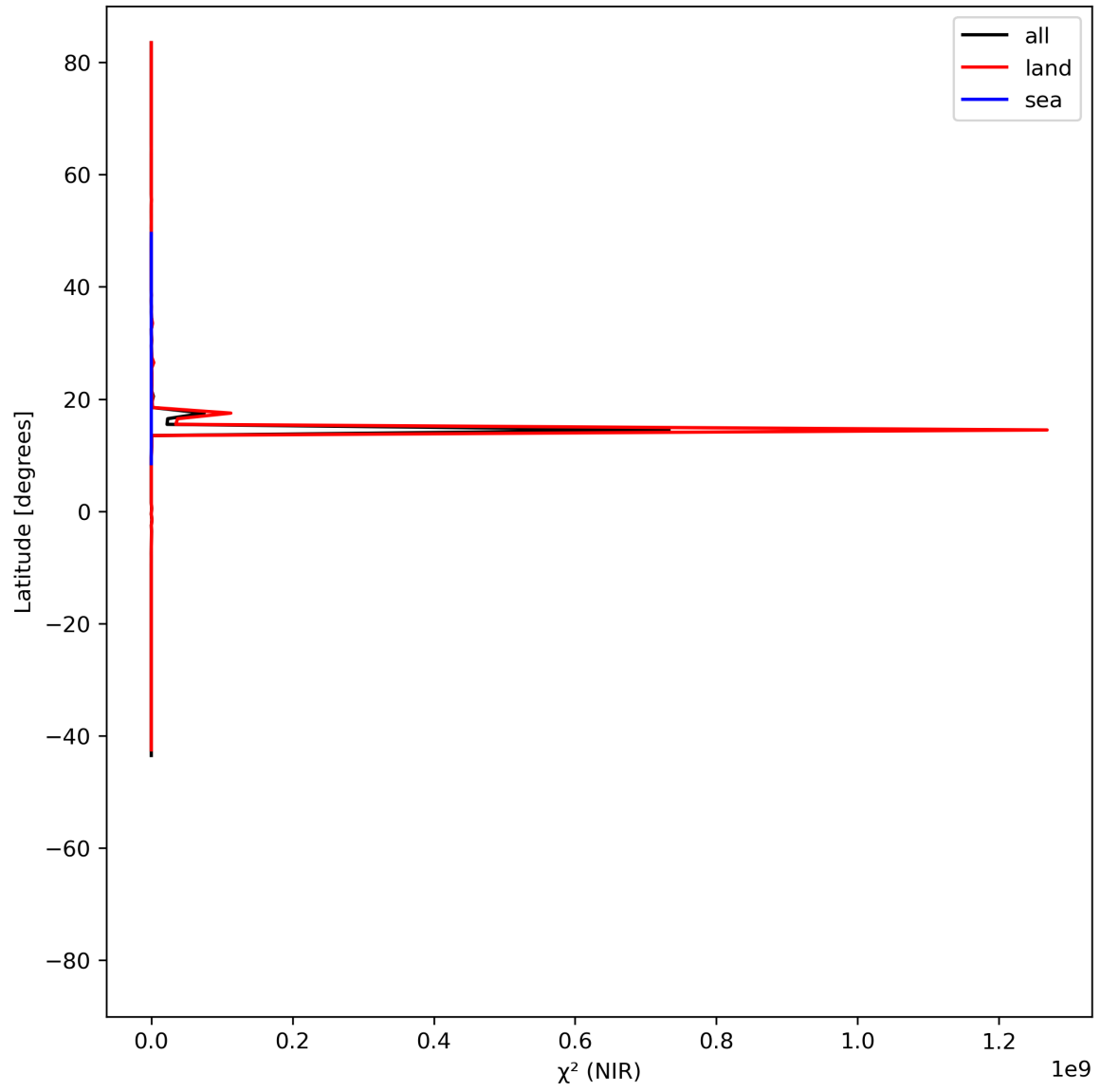
Figure 18: Zonal average of “ \chi^2 (NIR)” for 2024-06-11 to 2024-06-13.
