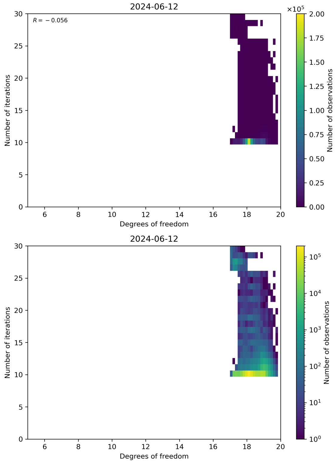
Figure 52: Scatter density plot of “Degrees of freedom” against “Number of iterations” for 2024-06-11 to 2024-06-13.
