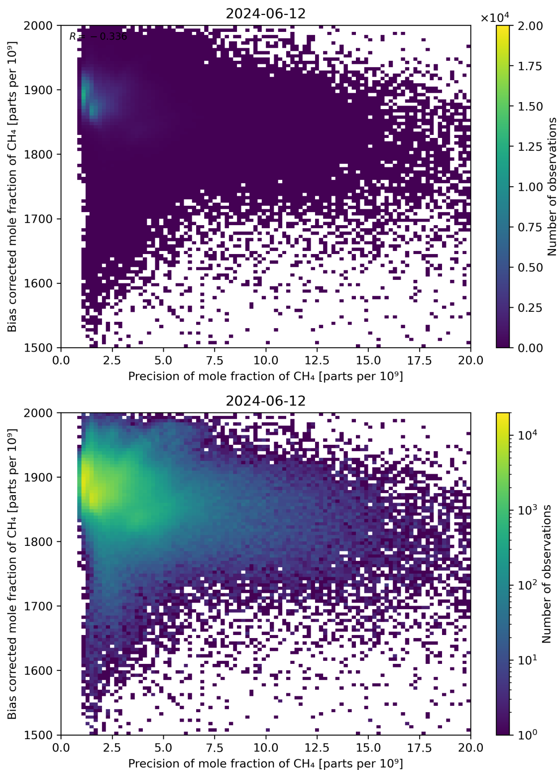
Figure 82: Scatter density plot of “Precision of mole fraction of CH 4 ” against “Bias corrected mole fraction of CH 4 ” for 2024-06-11 to 2024-06-13.
