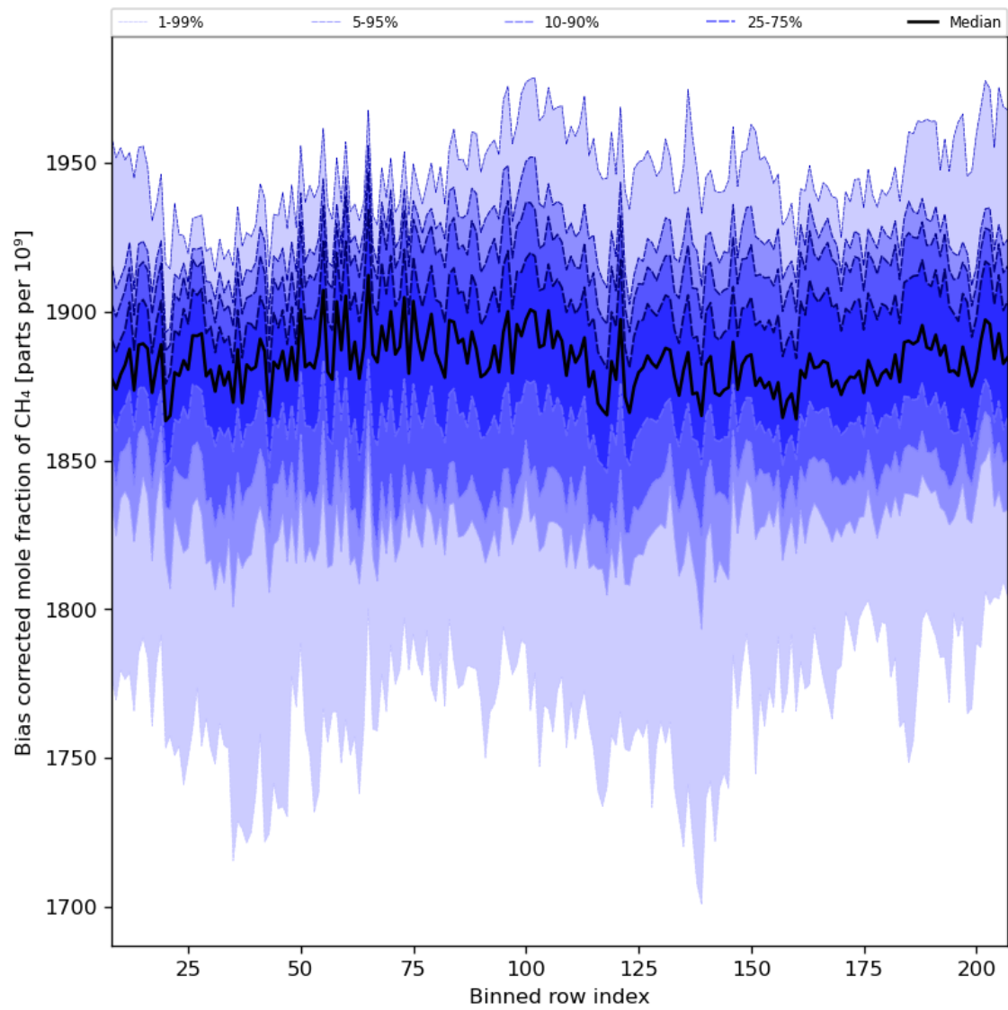
Figure 36: Along track statistics of “Bias corrected mole fraction of CH 4 ” for 2024-06-11 to 2024-06-13
