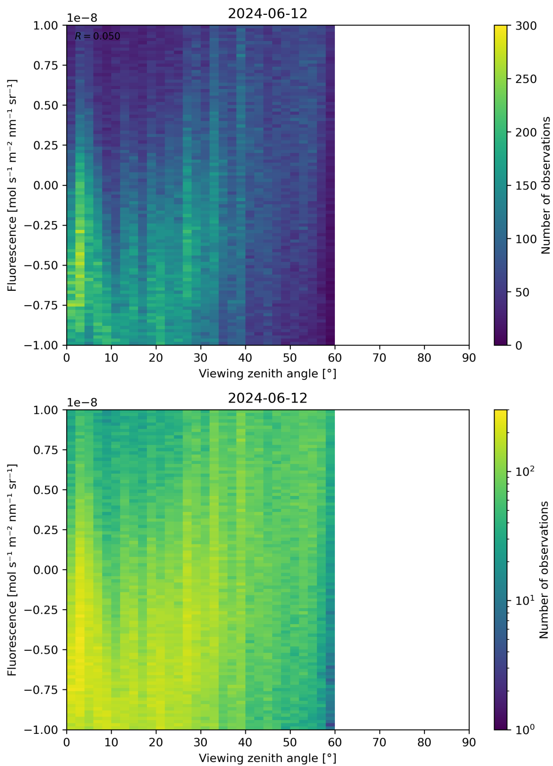
Figure 108: Scatter density plot of “Viewing zenith angle” against “Fluorescence” for 2024-06-11 to 2024-06-13.
