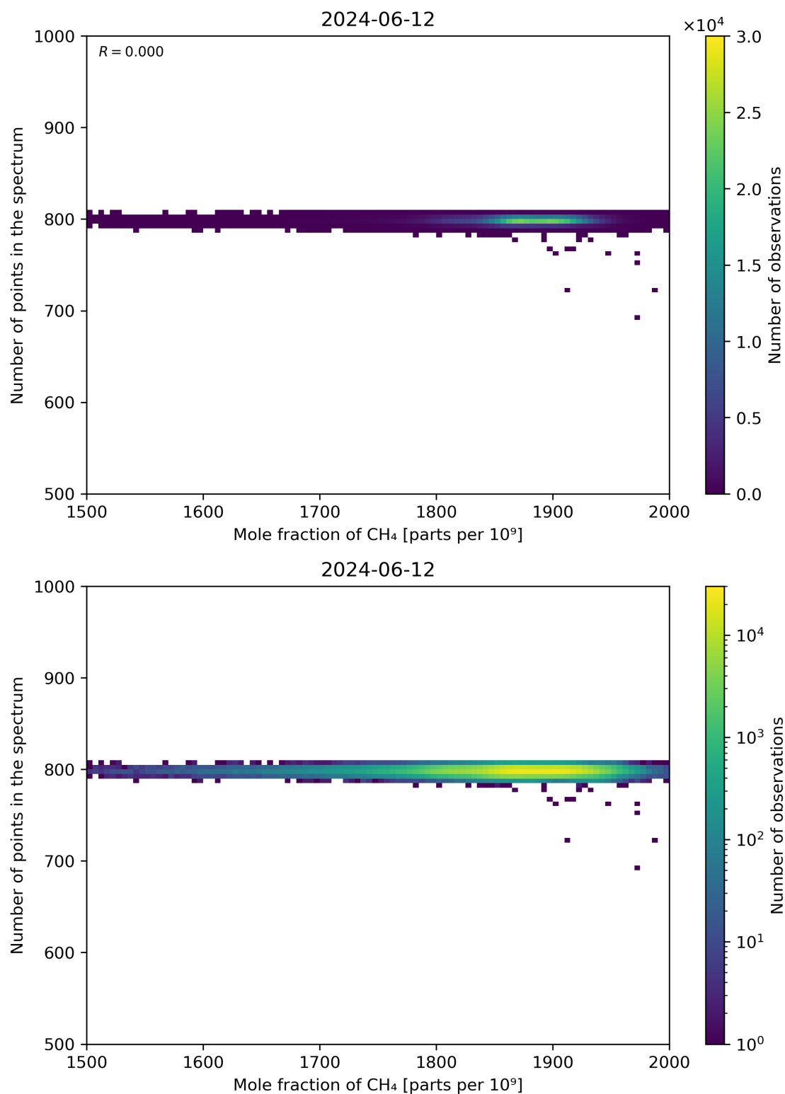
Figure 77: Scatter density plot of “Mole fraction of CH 4 ” against “Number of points in the spectrum” for 2024-06-11 to 2024-06-13.
