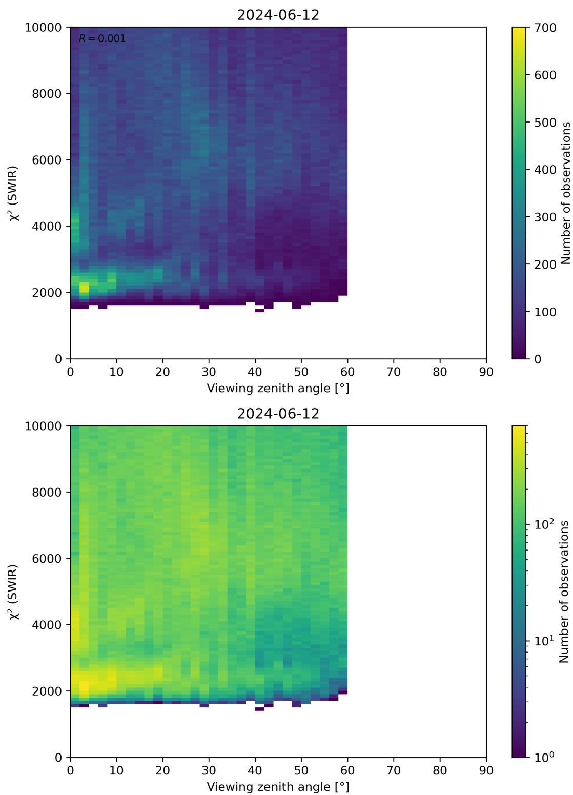
Figure 106: Scatter density plot of “Viewing zenith angle” against “ \chi^2 (SWIR)” for 2024-06-11 to 2024-06-13.
