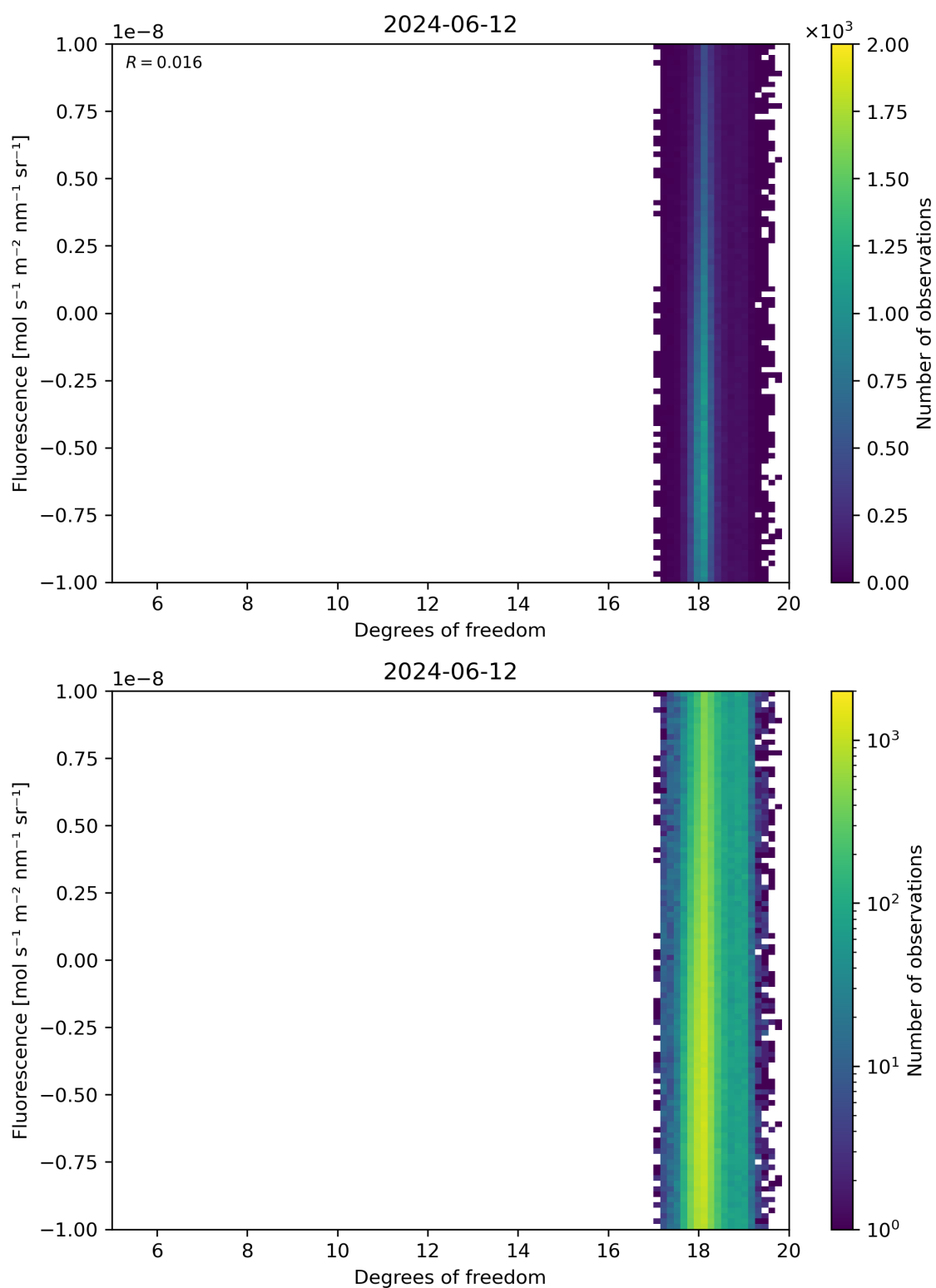
Figure 51: Scatter density plot of “Degrees of freedom” against “Fluorescence” for 2024-06-11 to 2024-06-13.
