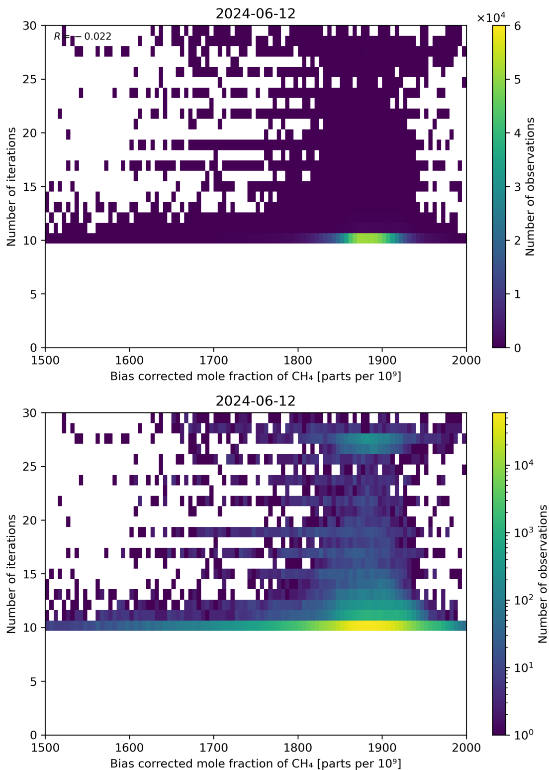
Figure 67: Scatter density plot of “Bias corrected mole fraction of CH 4 ” against “Number of iterations” for 2024-06-11 to 2024-06-13.
