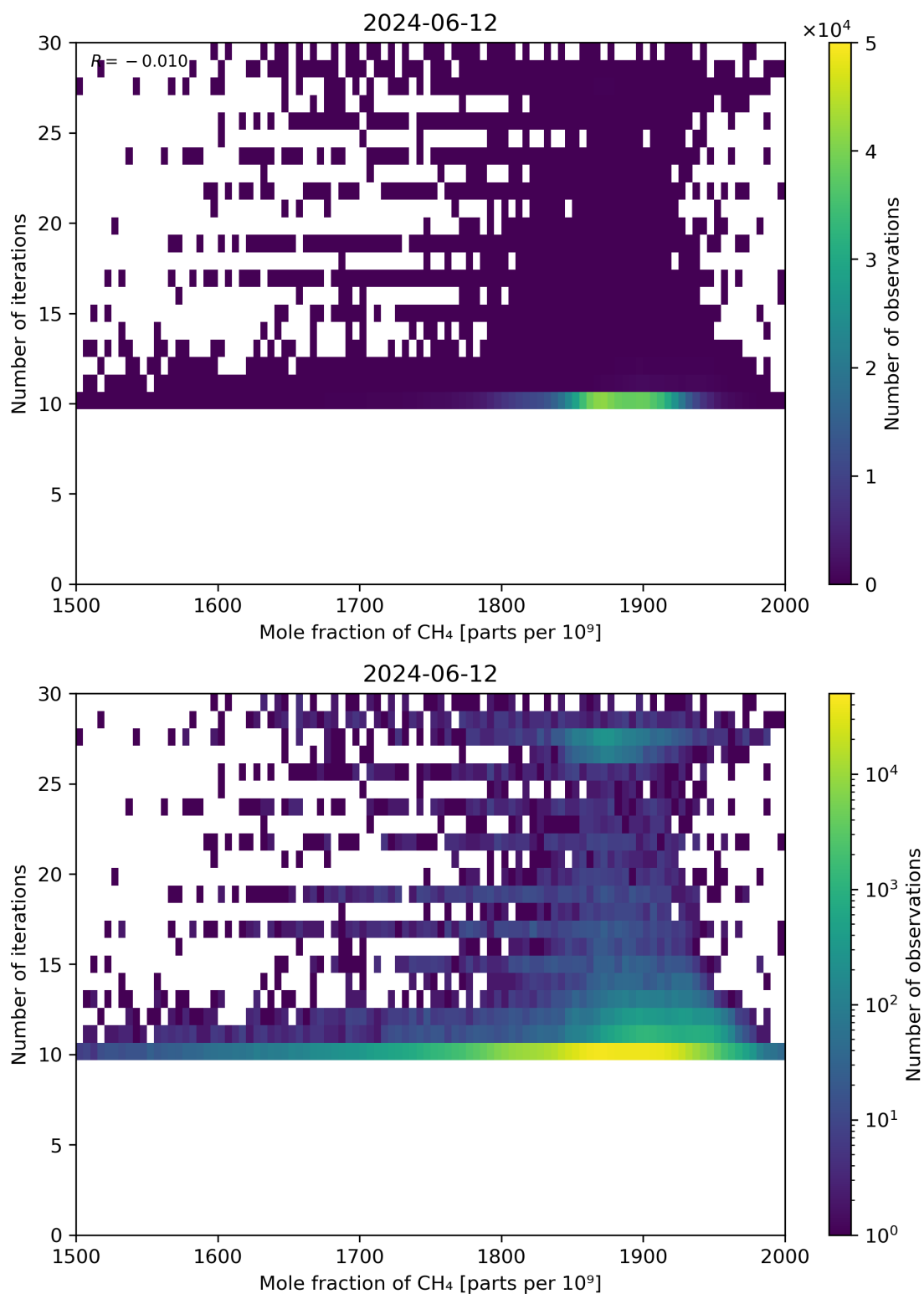
Figure 76: Scatter density plot of “Mole fraction of CH 4 ” against “Number of iterations” for 2024-06-11 to 2024-06-13.
