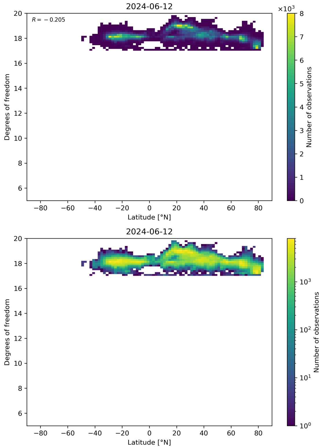
Figure 55: Scatter density plot of “Latitude” against “Degrees of freedom” for 2024-06-11 to 2024-06-13.
