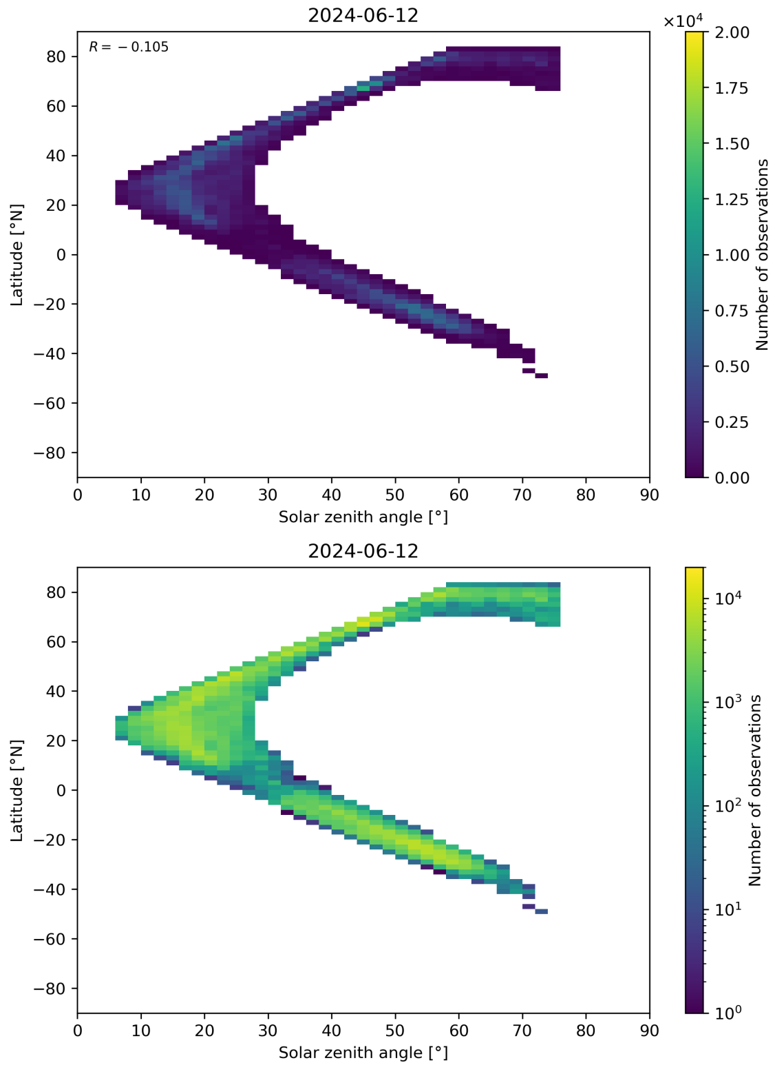
Figure 98: Scatter density plot of “Solar zenith angle” against “Latitude” for 2024-06-11 to 2024-06-13.
