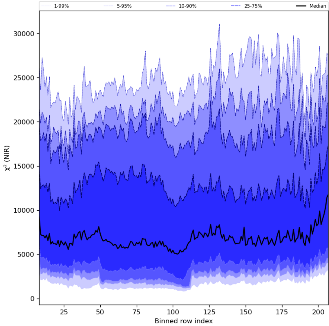
Figure 40: Along track statistics of “ \chi^2 (NIR)” for 2024-06-11 to 2024-06-13
