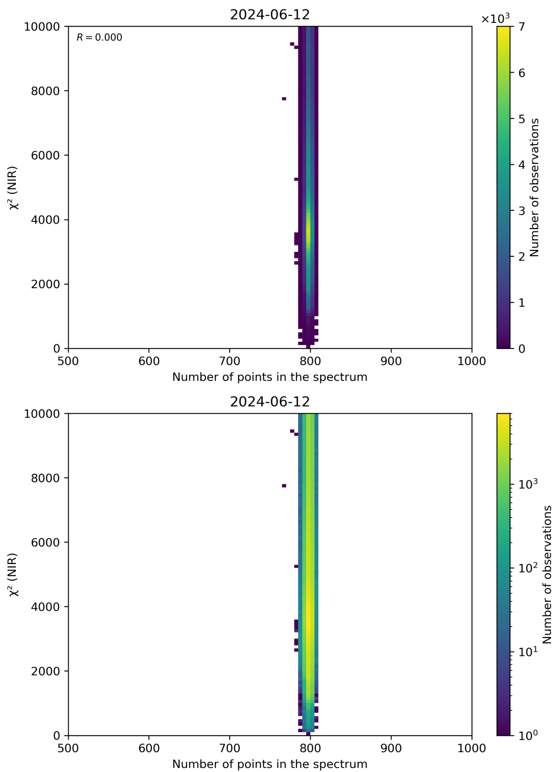
Figure 88: Scatter density plot of “Number of points in the spectrum” against “ \chi^2 (NIR)” for 2024-06-11 to 2024-06-13.
