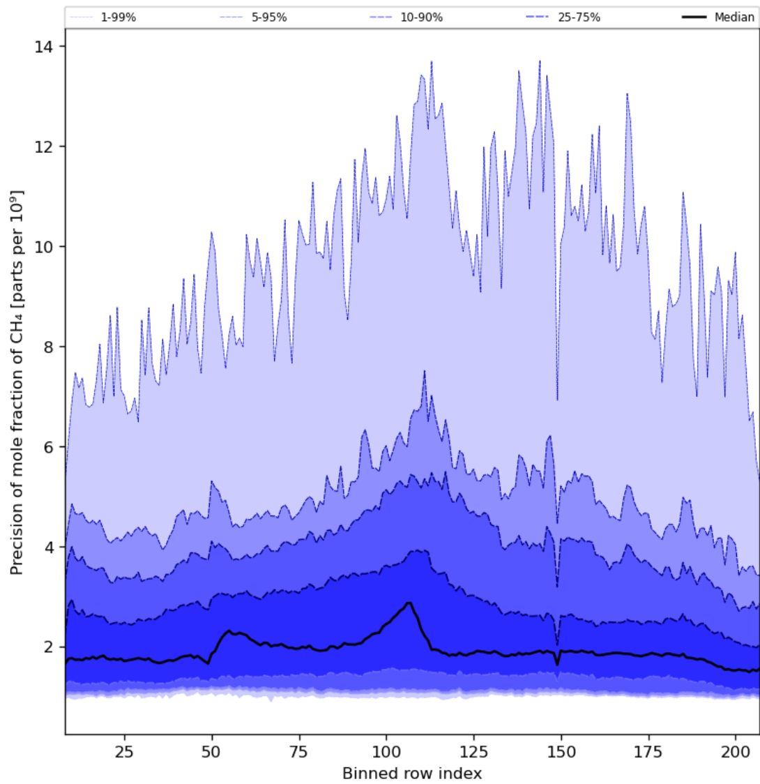
Figure 35: Along track statistics of “Precision of mole fraction of CH 4 ” for 2024-06-11 to 2024-06-13
