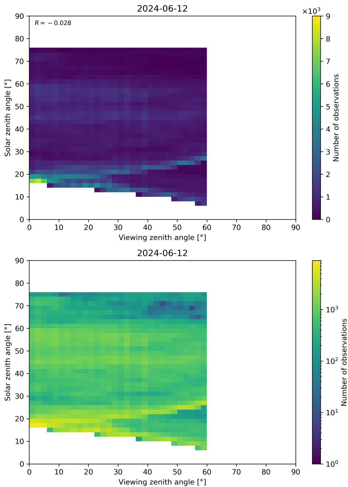
Figure 115: Scatter density plot of “Viewing zenith angle” against “Solar zenith angle” for 2024-06-11 to 2024-06-13.
