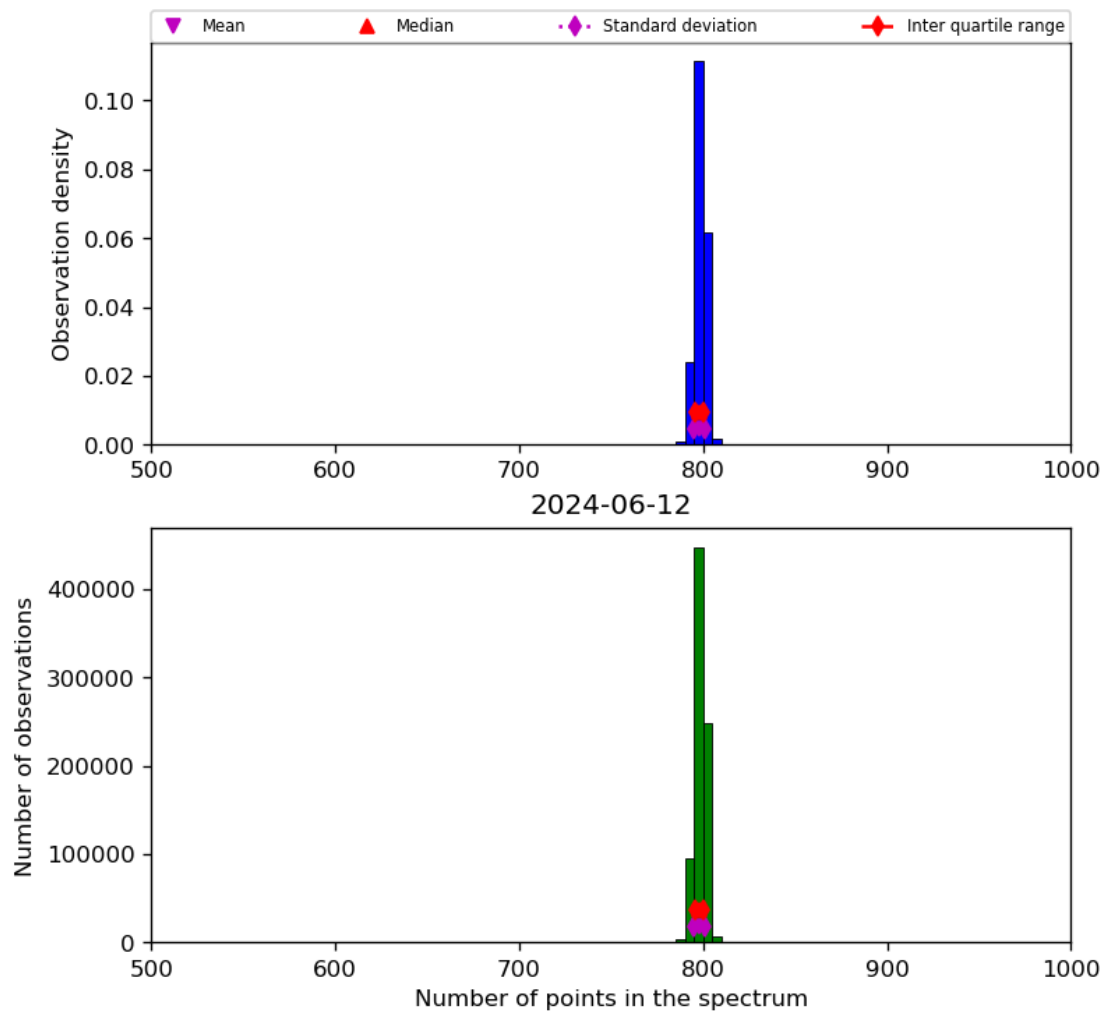
Figure 26: Histogram of “Number of points in the spectrum” for 2024-06-11 to 2024-06-13
