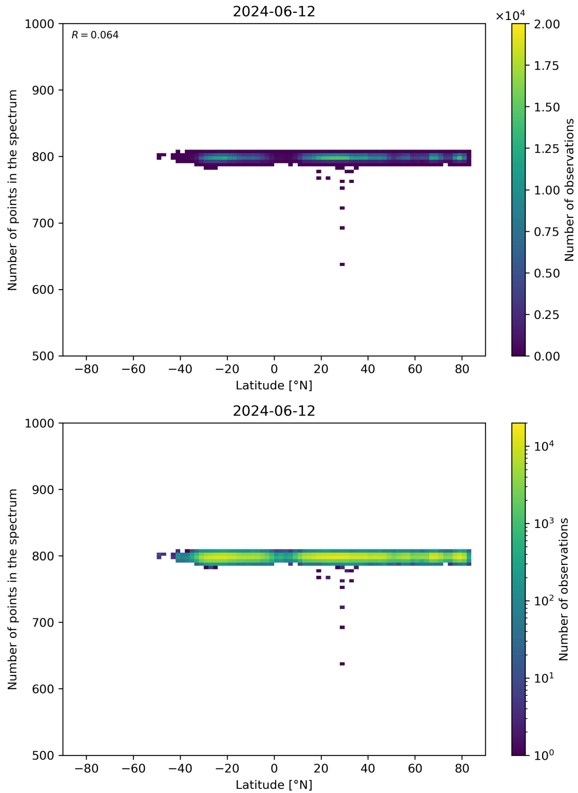
Figure 61: Scatter density plot of “Latitude” against “Number of points in the spectrum” for 2024-06-11 to 2024-06-13.
