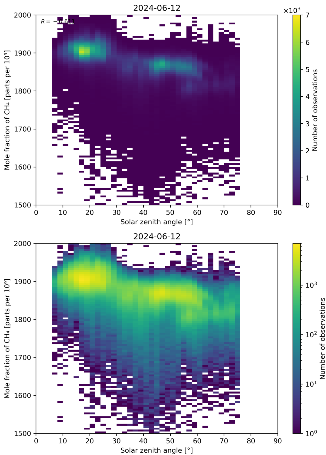
Figure 99: Scatter density plot of “Solar zenith angle” against “Mole fraction of \text{CH}_4 ” for 2024-06-11 to 2024-06-13.
