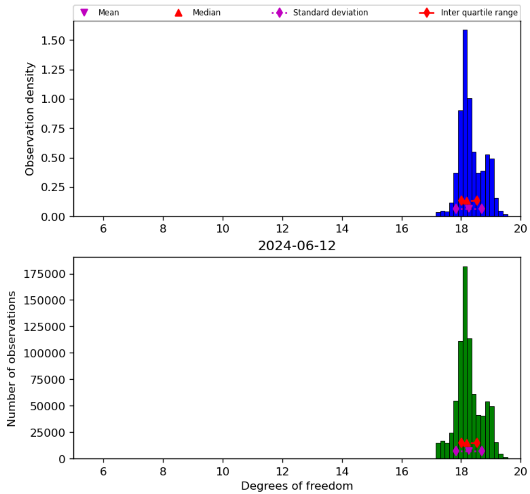
Figure 30: Histogram of “Degrees of freedom” for 2024-06-11 to 2024-06-13
