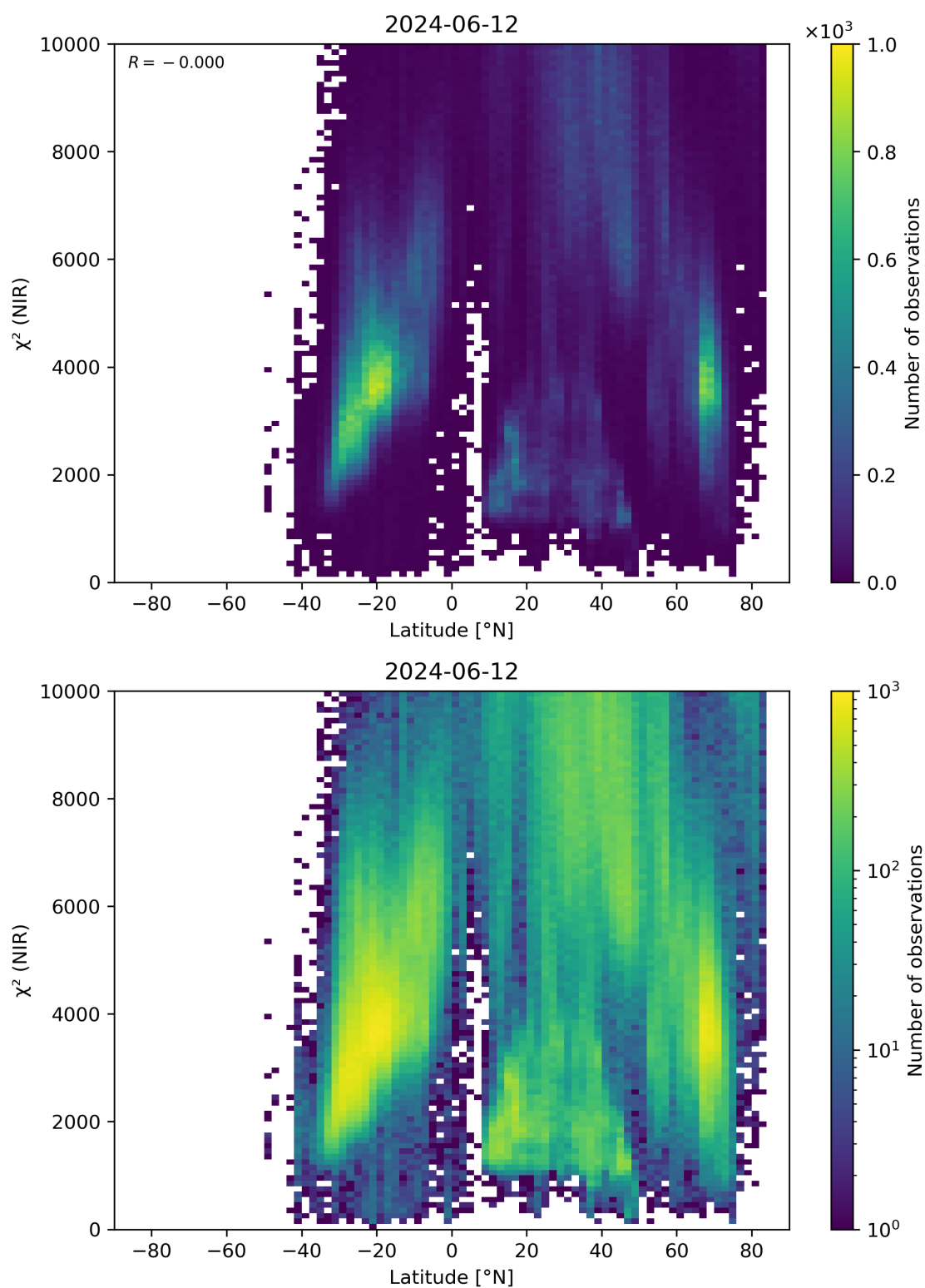
Figure 53: Scatter density plot of “Latitude” against “ \chi^2 (NIR)” for 2024-06-11 to 2024-06-13.
