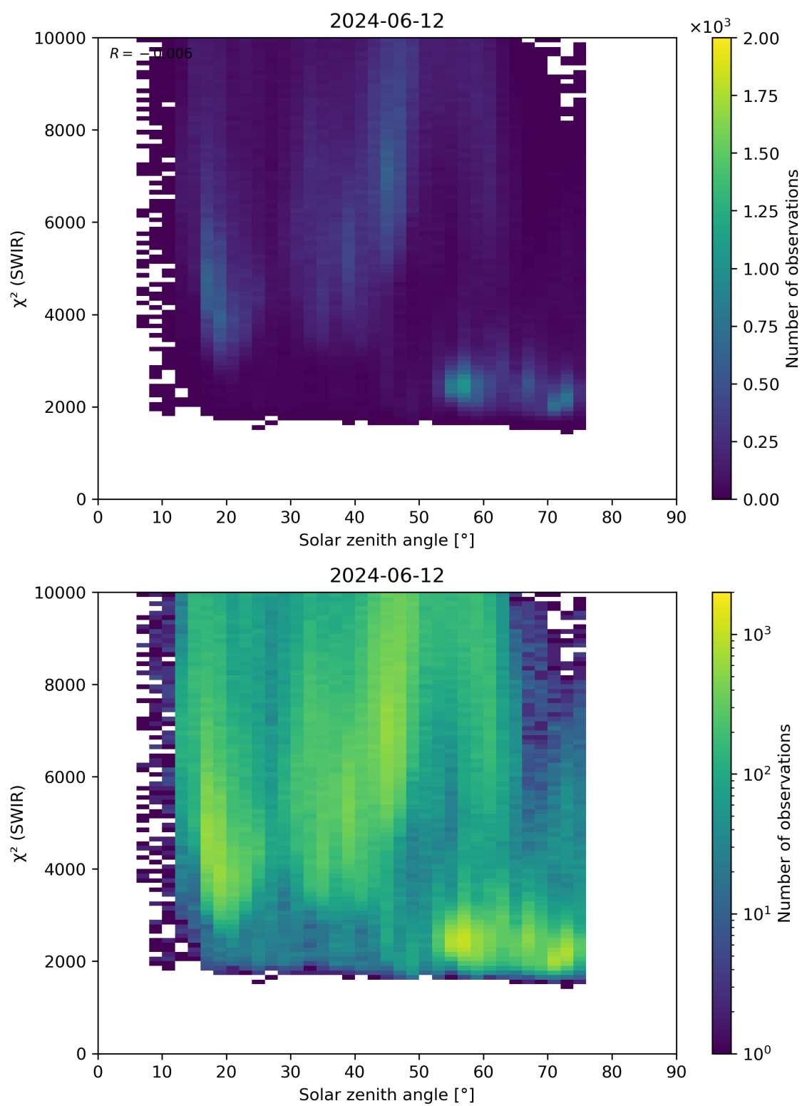
Figure 95: Scatter density plot of “Solar zenith angle” against “ \chi^2 (SWIR)” for 2024-06-11 to 2024-06-13.
