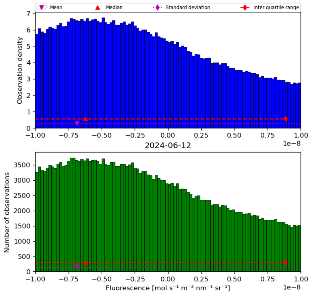
Figure 32: Histogram of “Fluorescence” for 2024-06-11 to 2024-06-13
