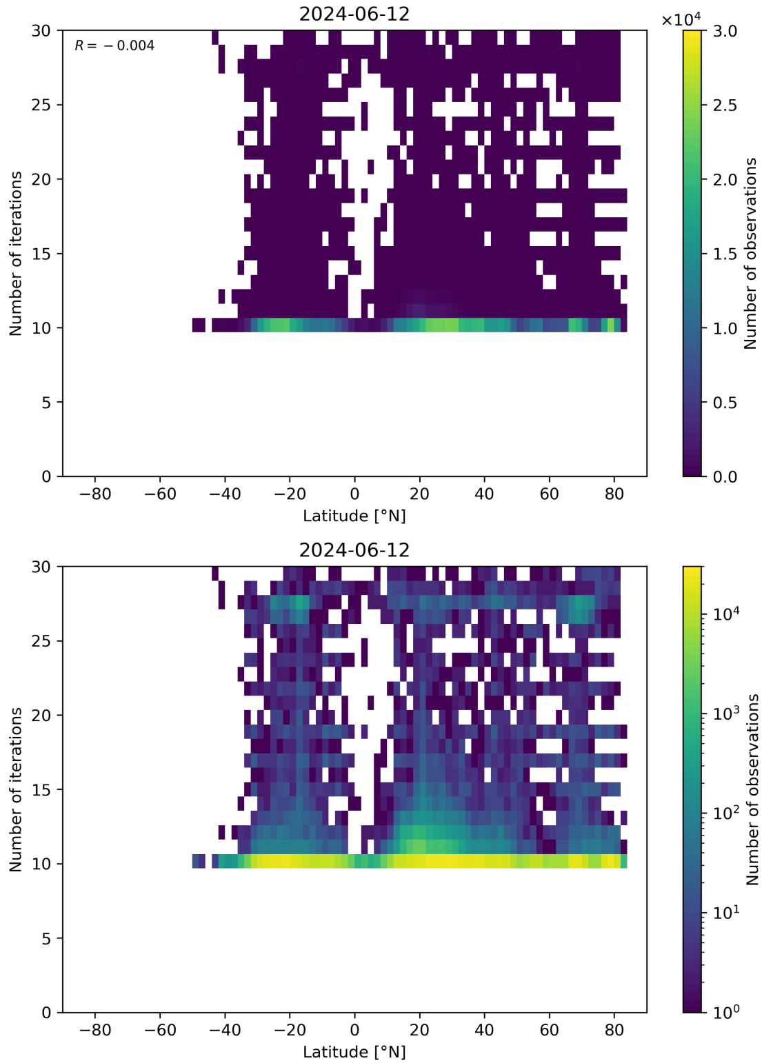
Figure 60: Scatter density plot of “Latitude” against “Number of iterations” for 2024-06-11 to 2024-06-13.
