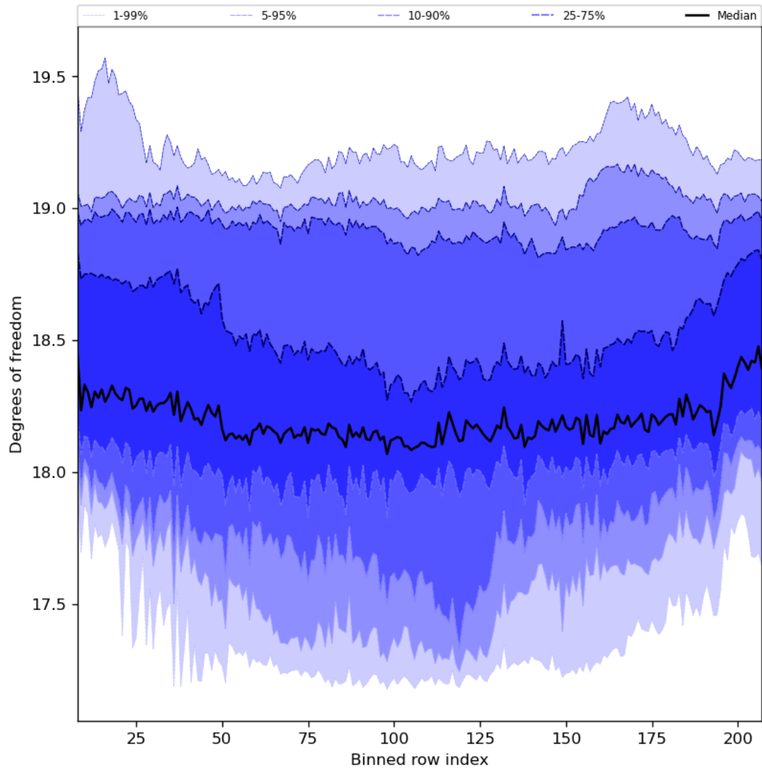
Figure 41: Along track statistics of “Degrees of freedom” for 2024-06-11 to 2024-06-13
