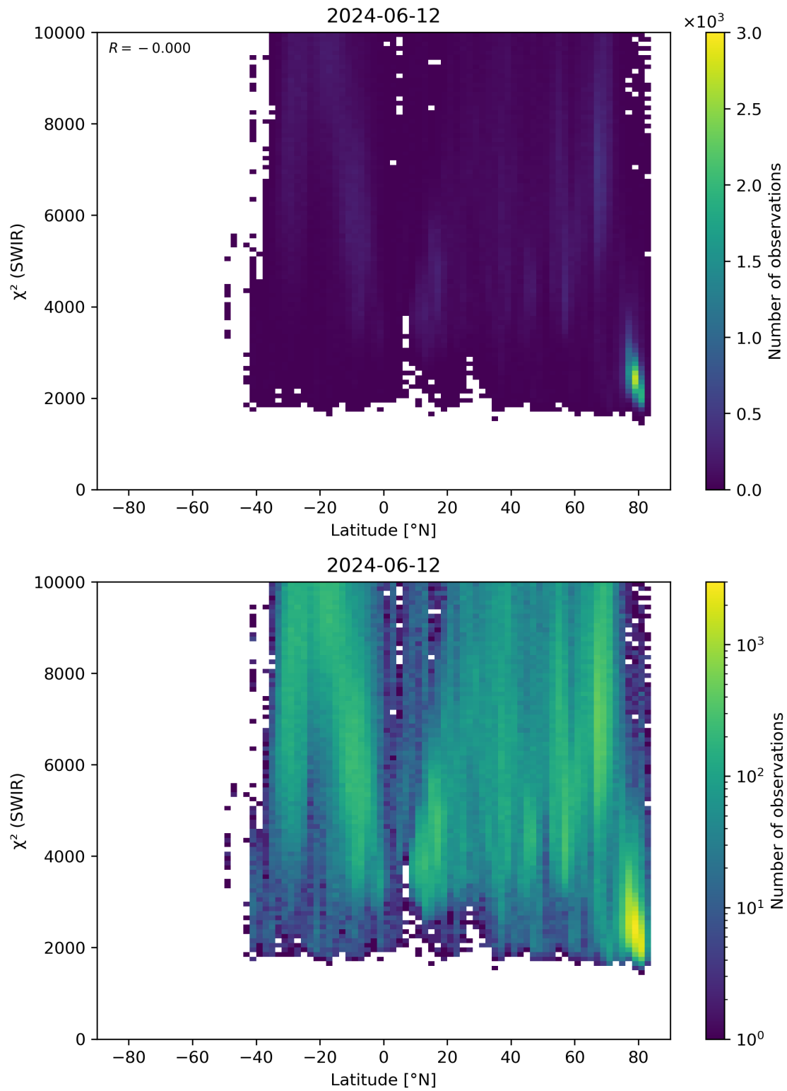
Figure 54: Scatter density plot of “Latitude” against “ \chi^2 (SWIR)” for 2024-06-11 to 2024-06-13.
