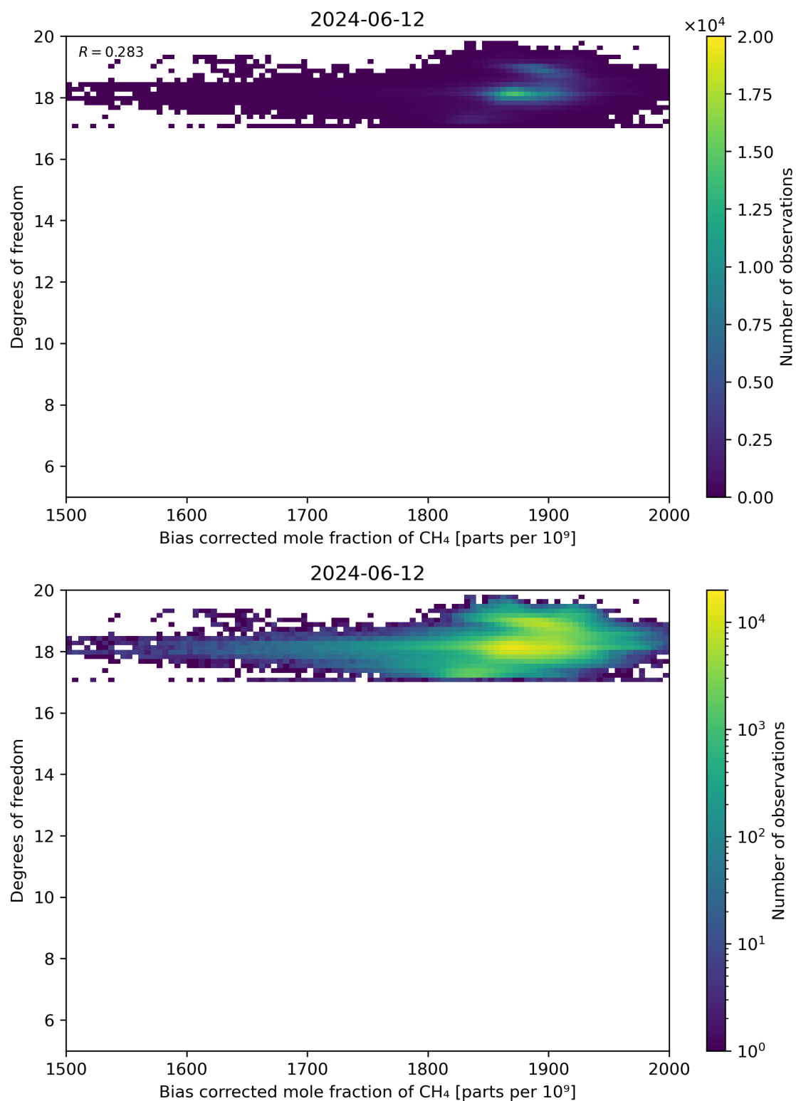
Figure 65: Scatter density plot of “Bias corrected mole fraction of CH 4 ” against “Degrees of freedom” for 2024-06-11 to 2024-06-13.
