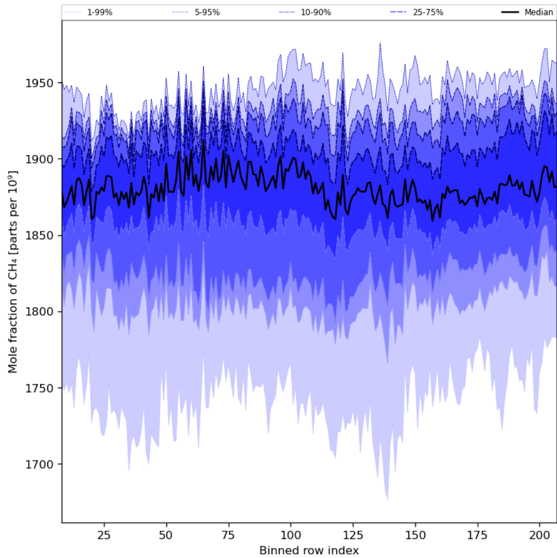
Figure 34: Along track statistics of “Mole fraction of CH 4 ” for 2024-06-11 to 2024-06-13
