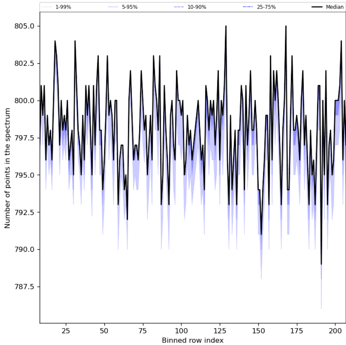
Figure 37: Along track statistics of “Number of points in the spectrum” for 2024-06-11 to 2024-06-13
