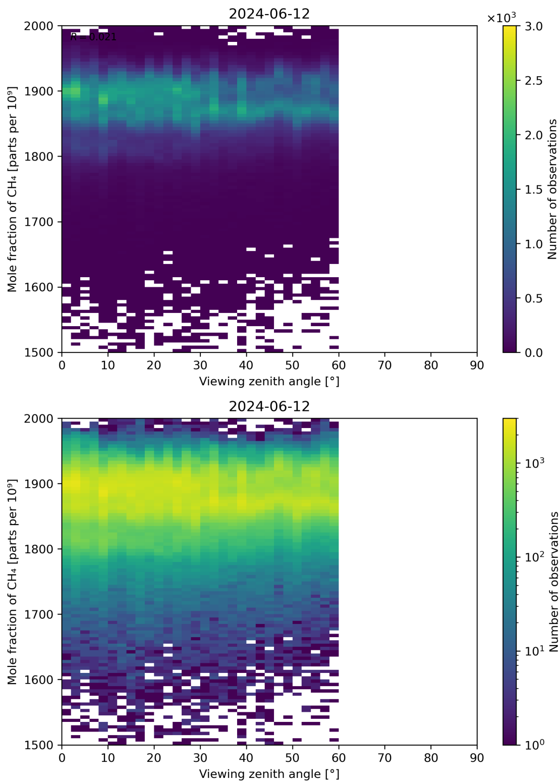
Figure 110: Scatter density plot of “Viewing zenith angle” against “Mole fraction of CH 4 ” for 2024-06-11 to 2024-06-13.
