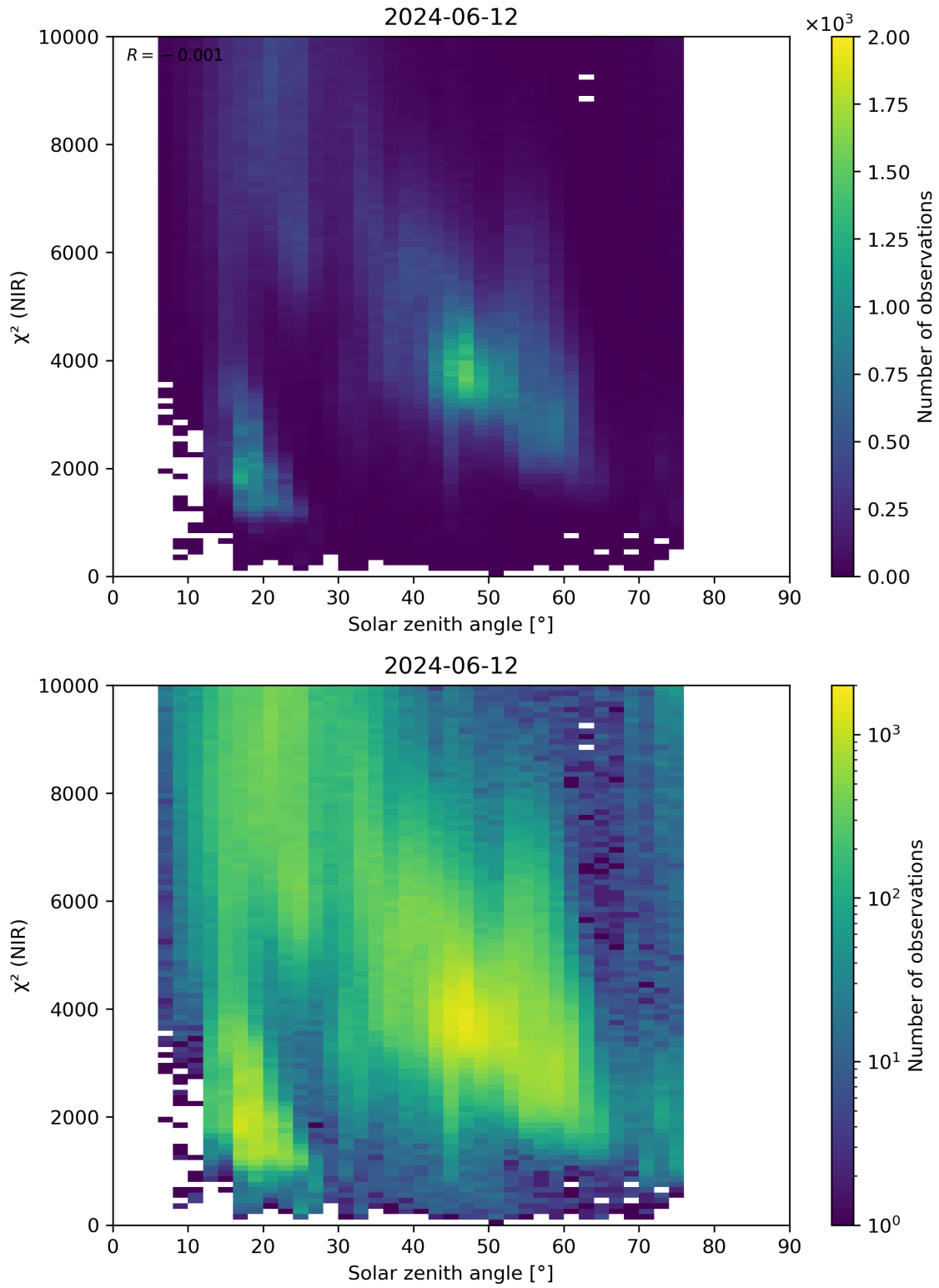
Figure 94: Scatter density plot of “Solar zenith angle” against “ \chi^2 (NIR)” for 2024-06-11 to 2024-06-13.
