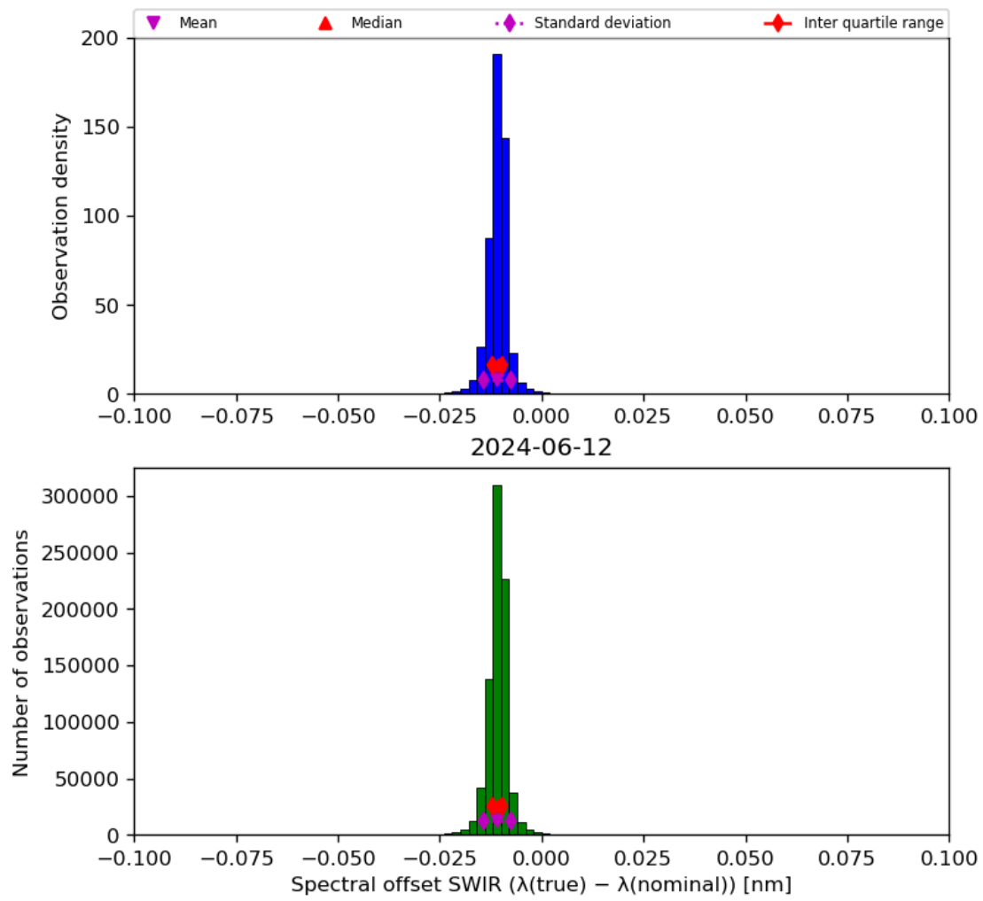
Figure 27: Histogram of “Spectral offset SWIR ( \lambda(\text{true}) - \lambda(\text{nominal}) )” for 2024-06-11 to 2024-06-13
