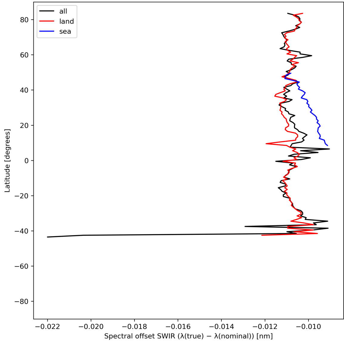
Figure 16: Zonal average of “Spectral offset SWIR ( \lambda(\text{true}) - \lambda(\text{nominal}) )” for 2024-06-11 to 2024-06-13.
