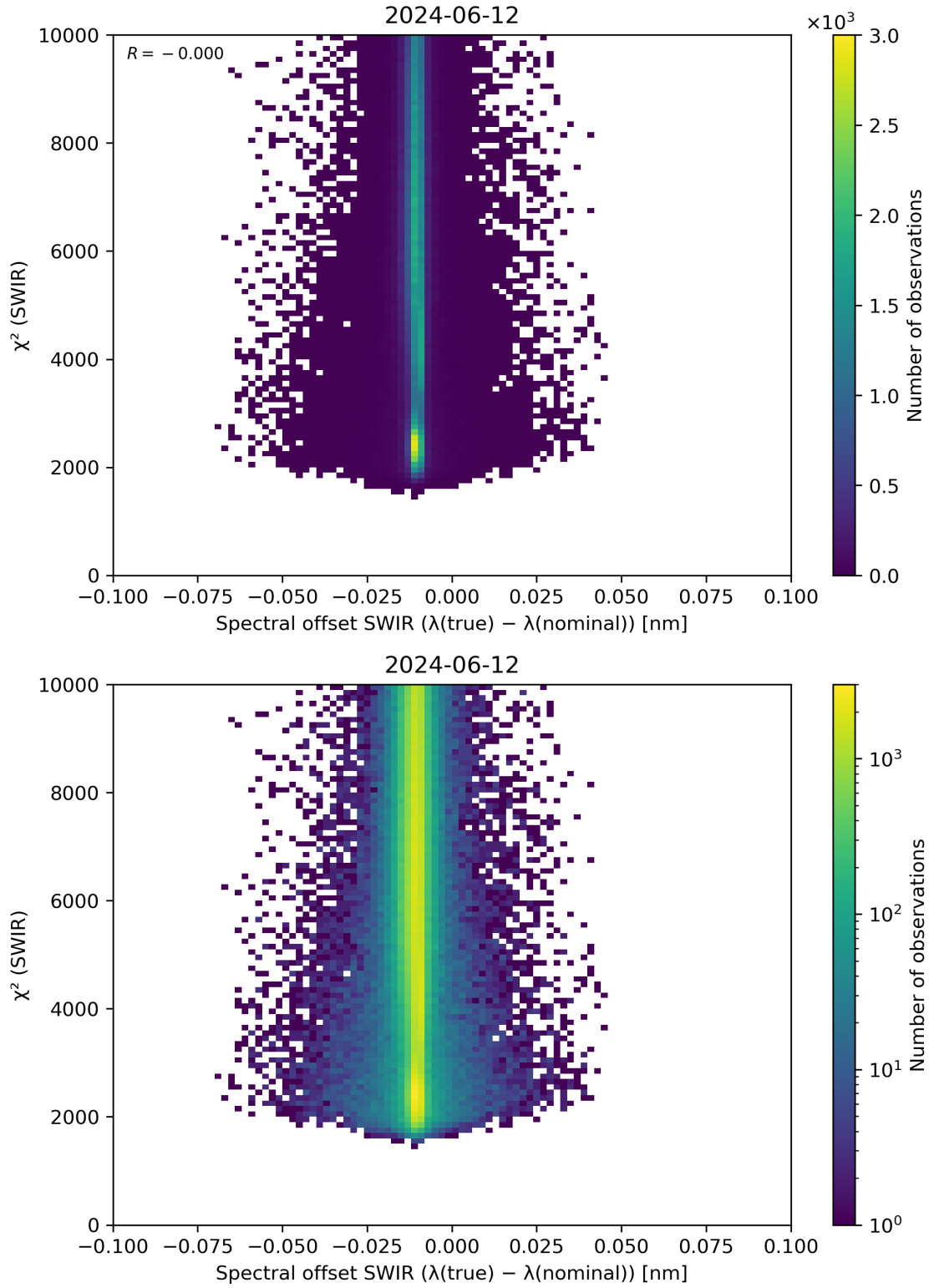
Figure 118: Scatter density plot of “Spectral offset SWIR ( \lambda(\text{true}) - \lambda(\text{nominal}) )” against “ \chi^2 (SWIR)” for 2024-06-11 to 2024-06-13.
