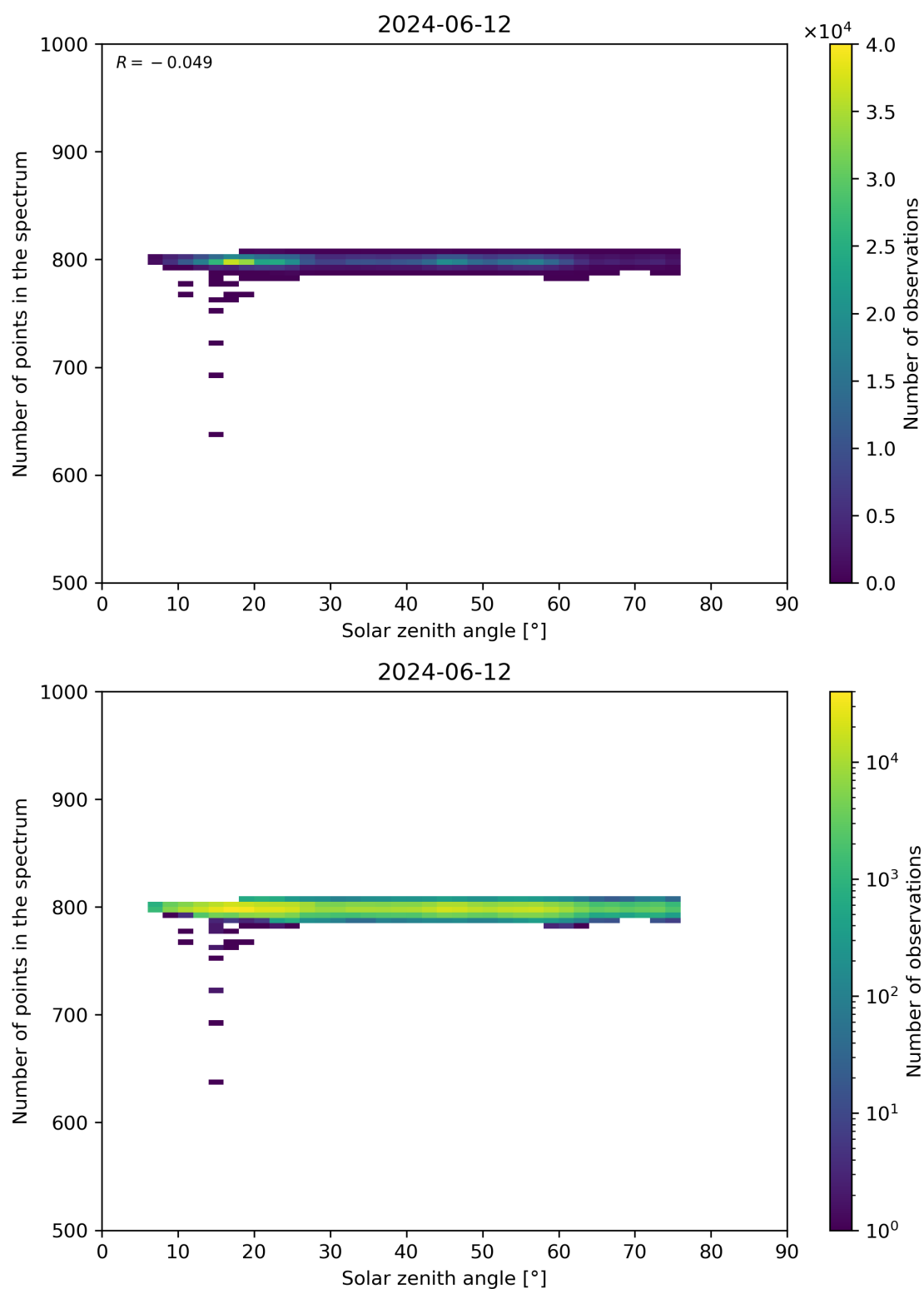
Figure 103: Scatter density plot of “Solar zenith angle” against “Number of points in the spectrum” for 2024-06-11 to 2024-06-13.
