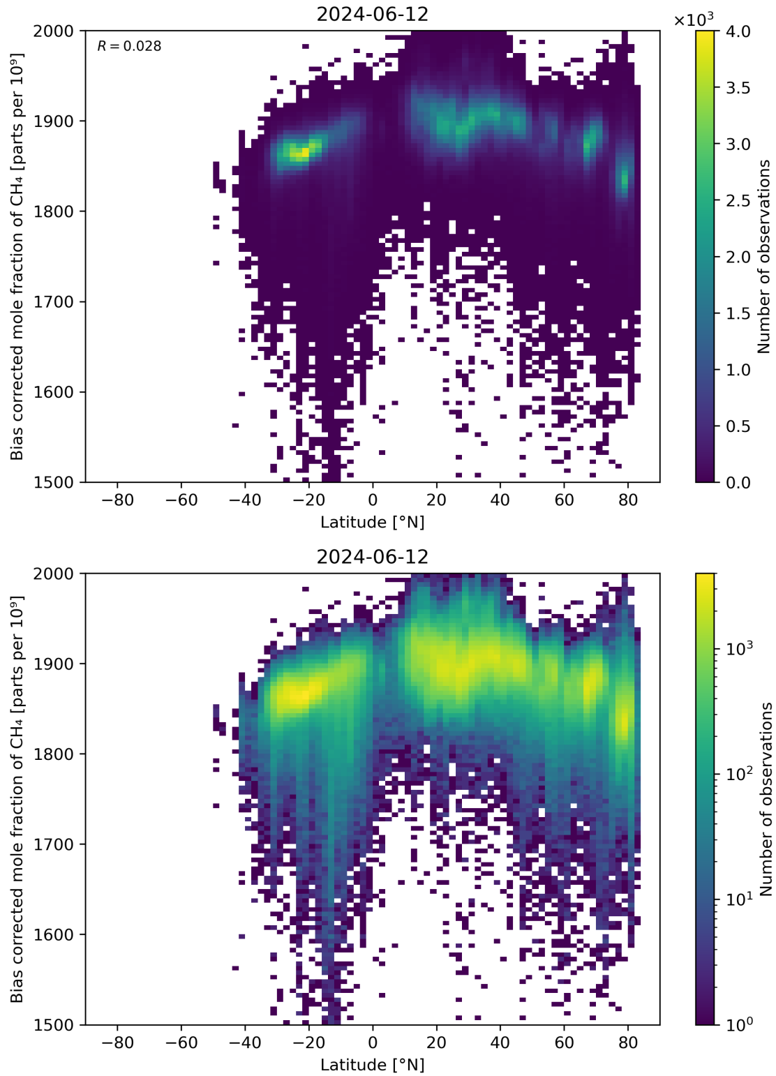
Figure 58: Scatter density plot of “Latitude” against “Bias corrected mole fraction of CH 4 ” for 2024-06-11 to 2024-06-13.
