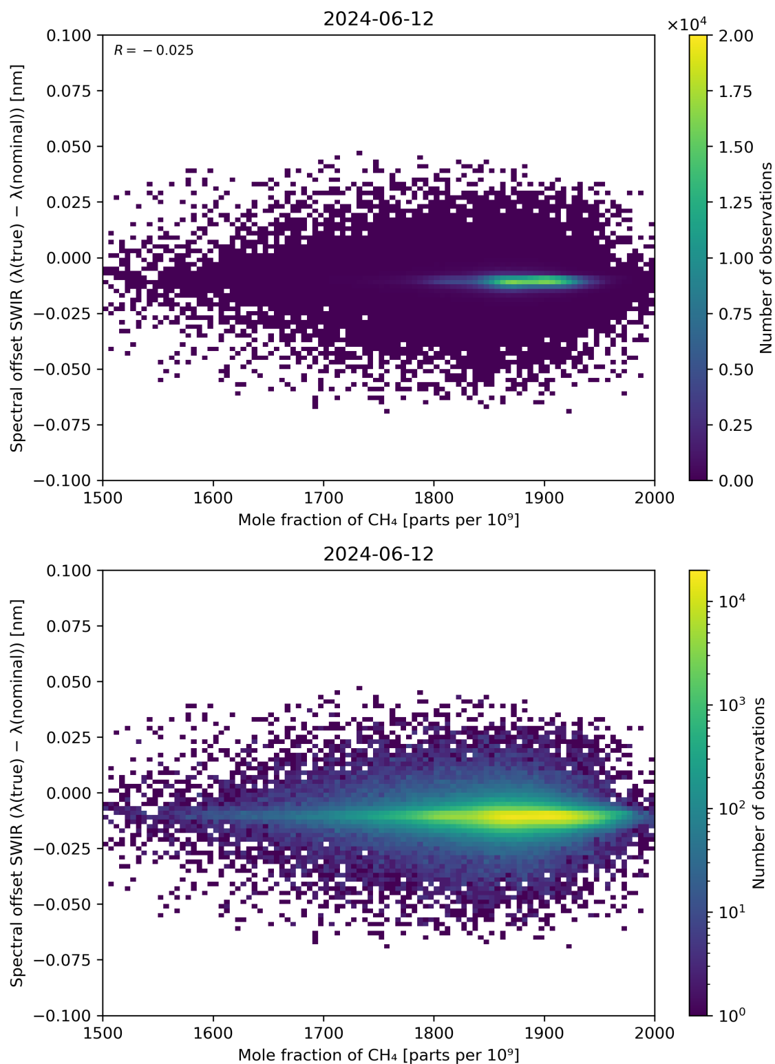
Figure 86: Scatter density plot of “Mole fraction of CH 4 ” against “Spectral offset SWIR ( \lambda(\text{true}) - \lambda(\text{nominal}) )” for 2024-06-11 to 2024-06-13.
