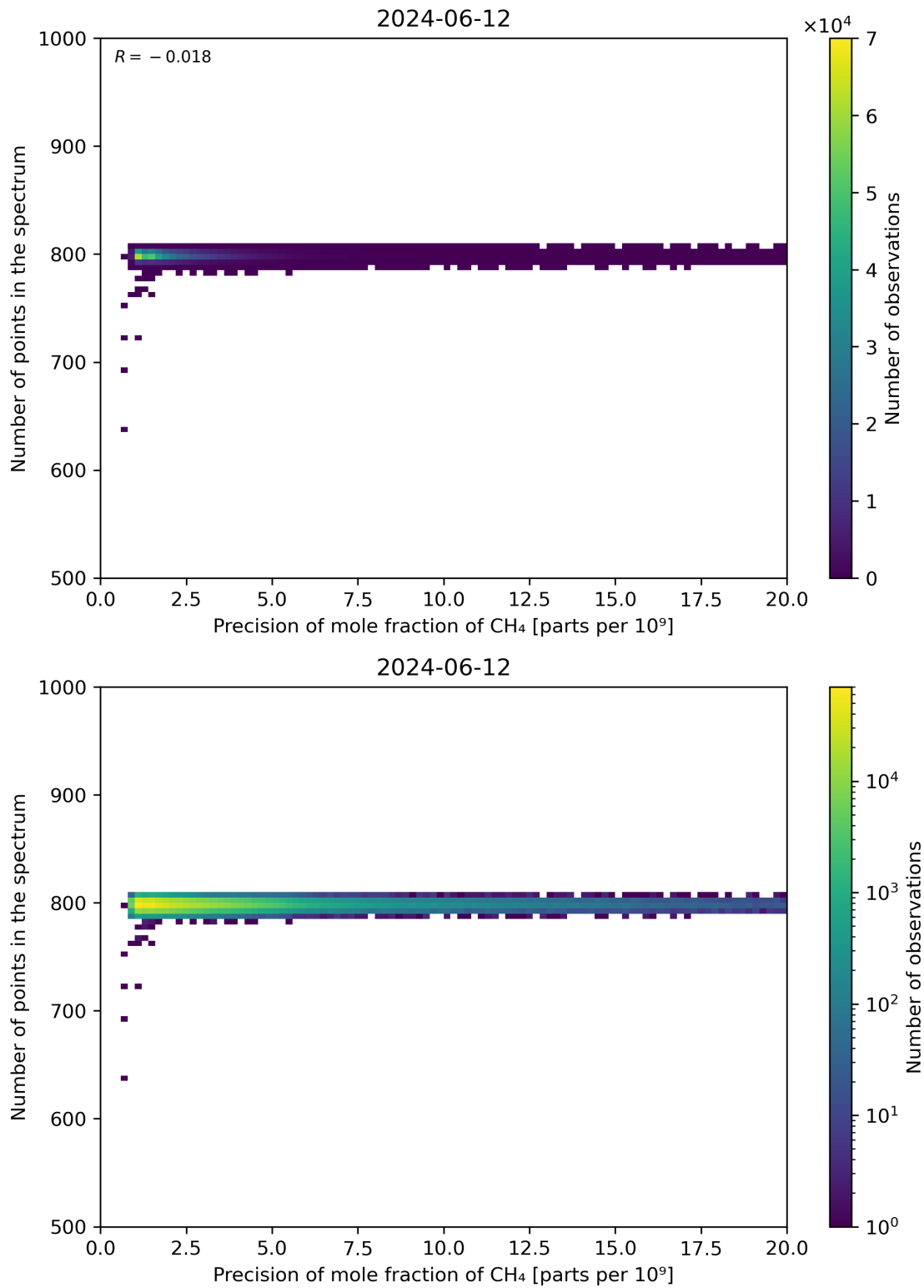
Figure 84: Scatter density plot of “Precision of mole fraction of CH 4 ” against “Number of points in the spectrum” for 2024-06-11 to 2024-06-13.
