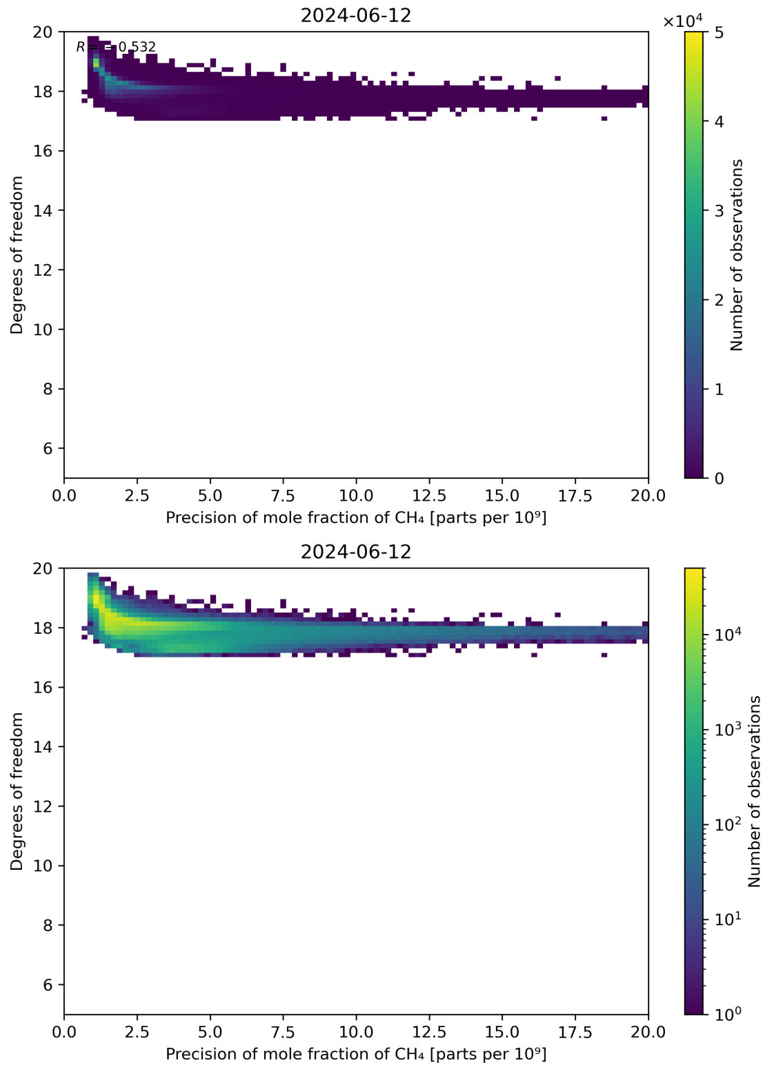
Figure 80: Scatter density plot of “Precision of mole fraction of CH 4 ” against “Degrees of freedom” for 2024-06-11 to 2024-06-13.
