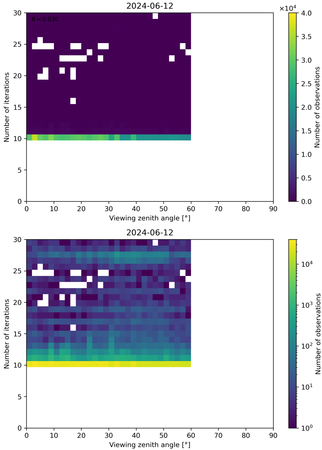
Figure 113: Scatter density plot of “Viewing zenith angle” against “Number of iterations” for 2024-06-11 to 2024-06-13.
