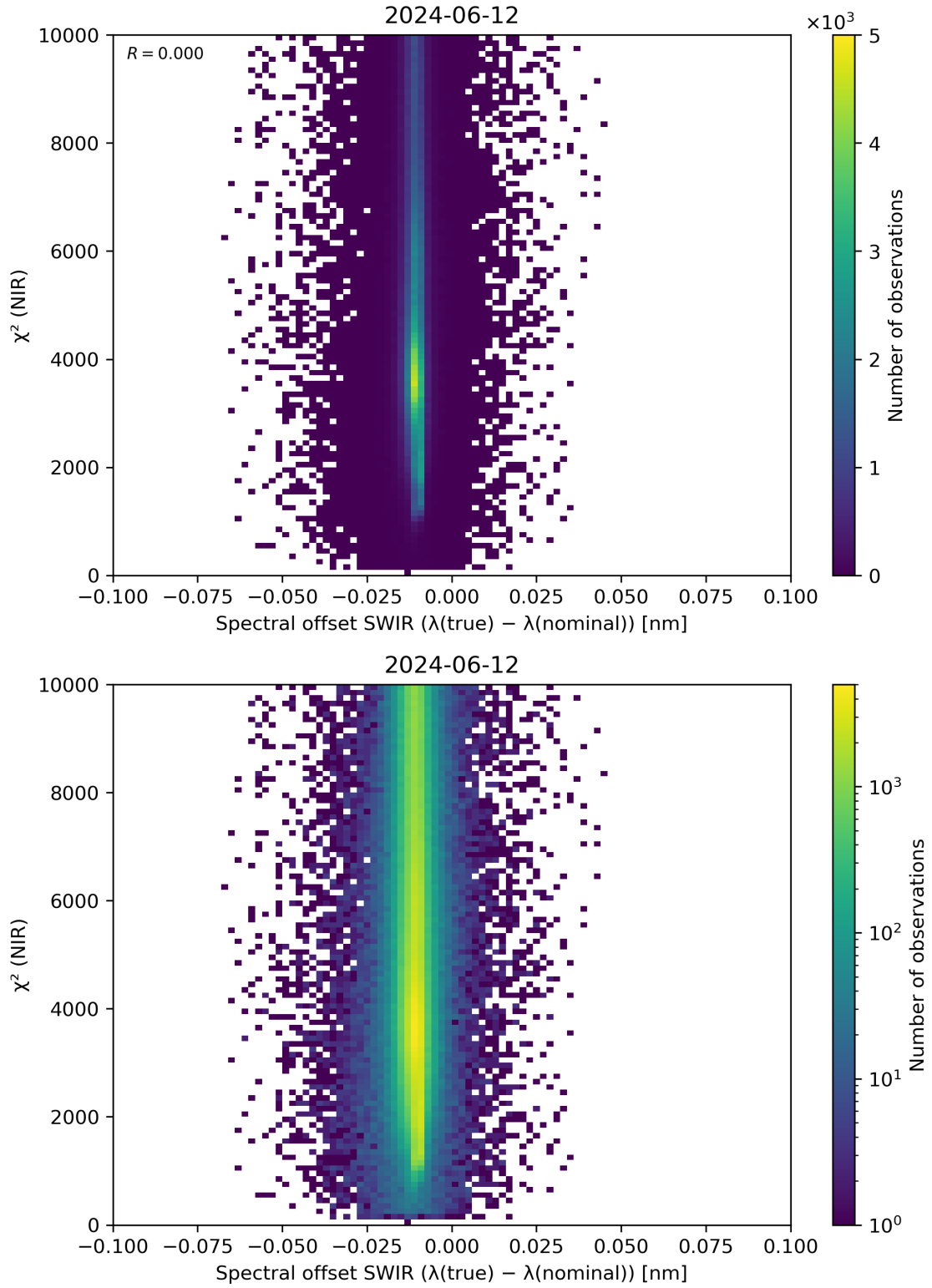
Figure 117: Scatter density plot of “Spectral offset SWIR ( \lambda(\text{true}) - \lambda(\text{nominal}) )” against “ \chi^2 (NIR)” for 2024-06-11 to 2024-06-13.
