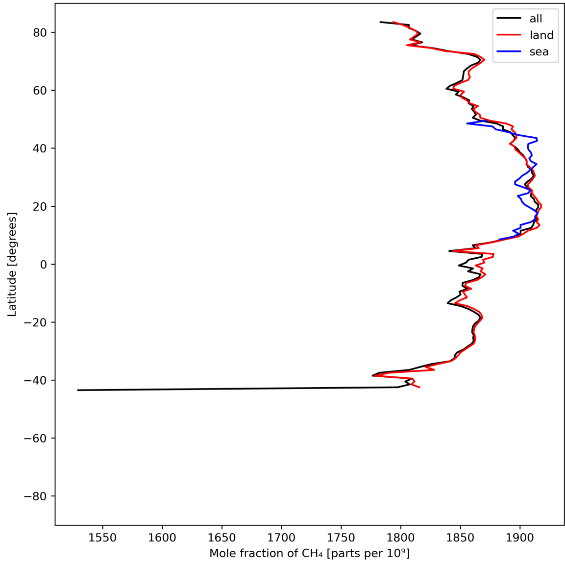
Figure 12: Zonal average of “Mole fraction of \text{CH}_4 ” for 2024-06-11 to 2024-06-13.
