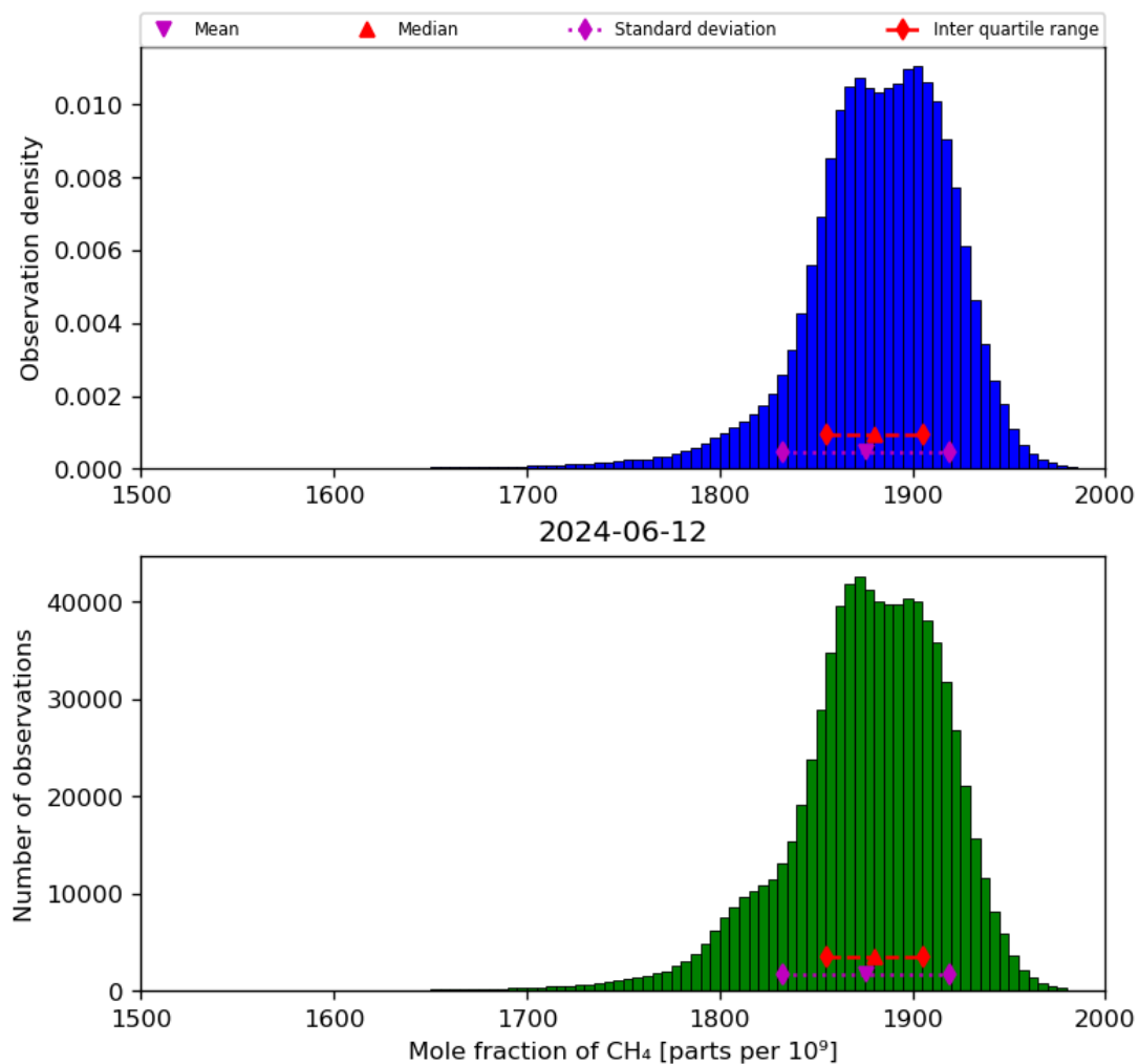
Figure 23: Histogram of “Mole fraction of CH 4 ” for 2024-06-11 to 2024-06-13
