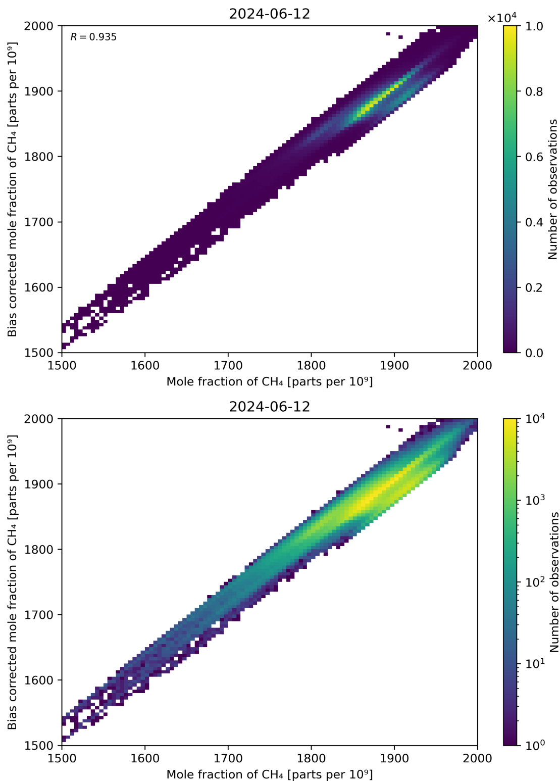
Figure 74: Scatter density plot of “Mole fraction of CH 4 ” against “Bias corrected mole fraction of CH 4 ” for 2024-06-11 to 2024-06-13.
