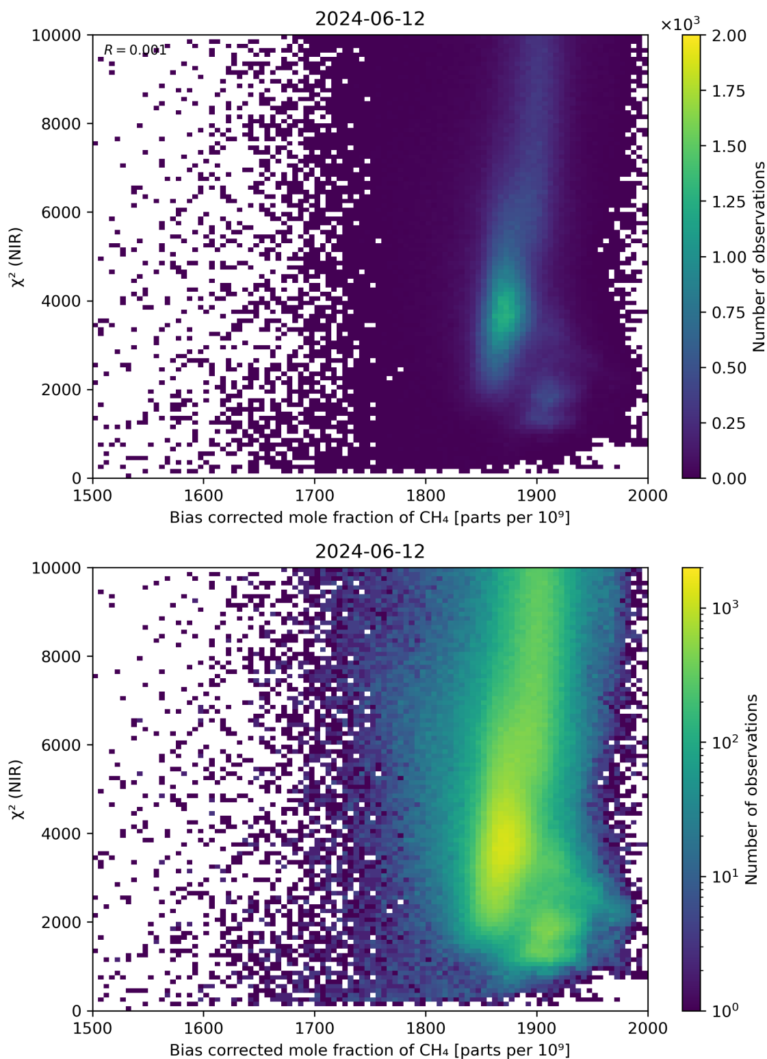
Figure 63: Scatter density plot of “Bias corrected mole fraction of \text{CH}_4 ” against “ \chi^2 (NIR)” for 2024-06-11 to 2024-06-13.
