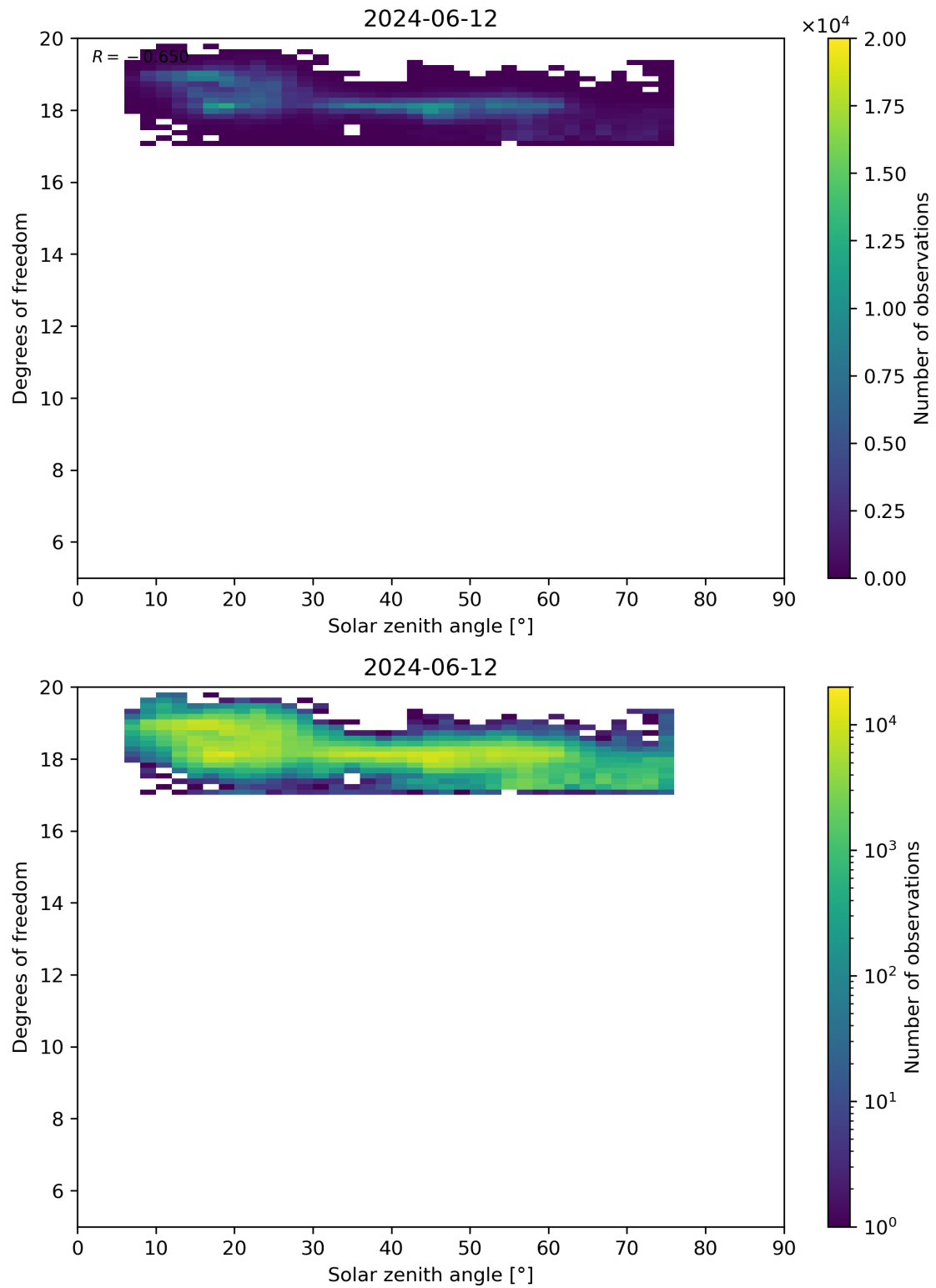
Figure 96: Scatter density plot of “Solar zenith angle” against “Degrees of freedom” for 2024-06-11 to 2024-06-13.
