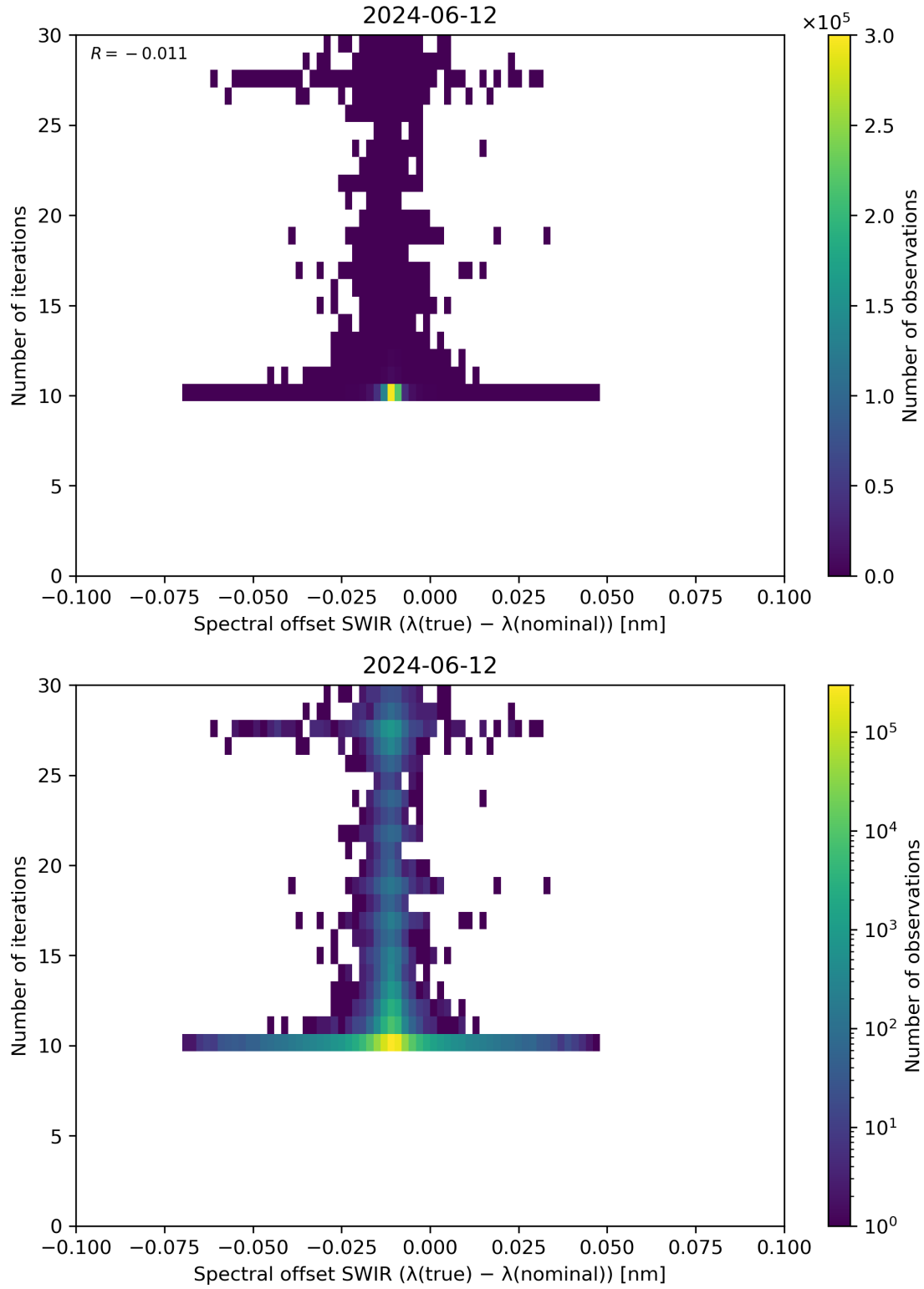
Figure 121: Scatter density plot of “Spectral offset SWIR ( \lambda(\text{true}) - \lambda(\text{nominal}) )” against “Number of iterations” for 2024-06-11 to 2024-06-13.
