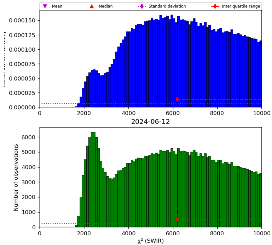
Figure 28: Histogram of “ \chi^2 (SWIR)” for 2024-06-11 to 2024-06-13
