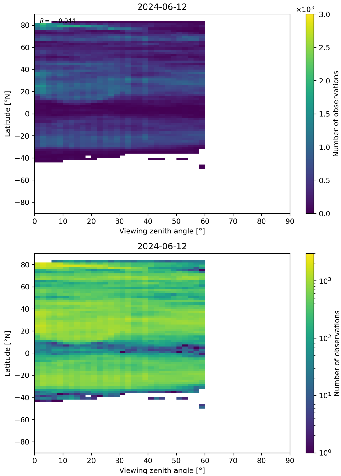
Figure 109: Scatter density plot of “Viewing zenith angle” against “Latitude” for 2024-06-11 to 2024-06-13.
