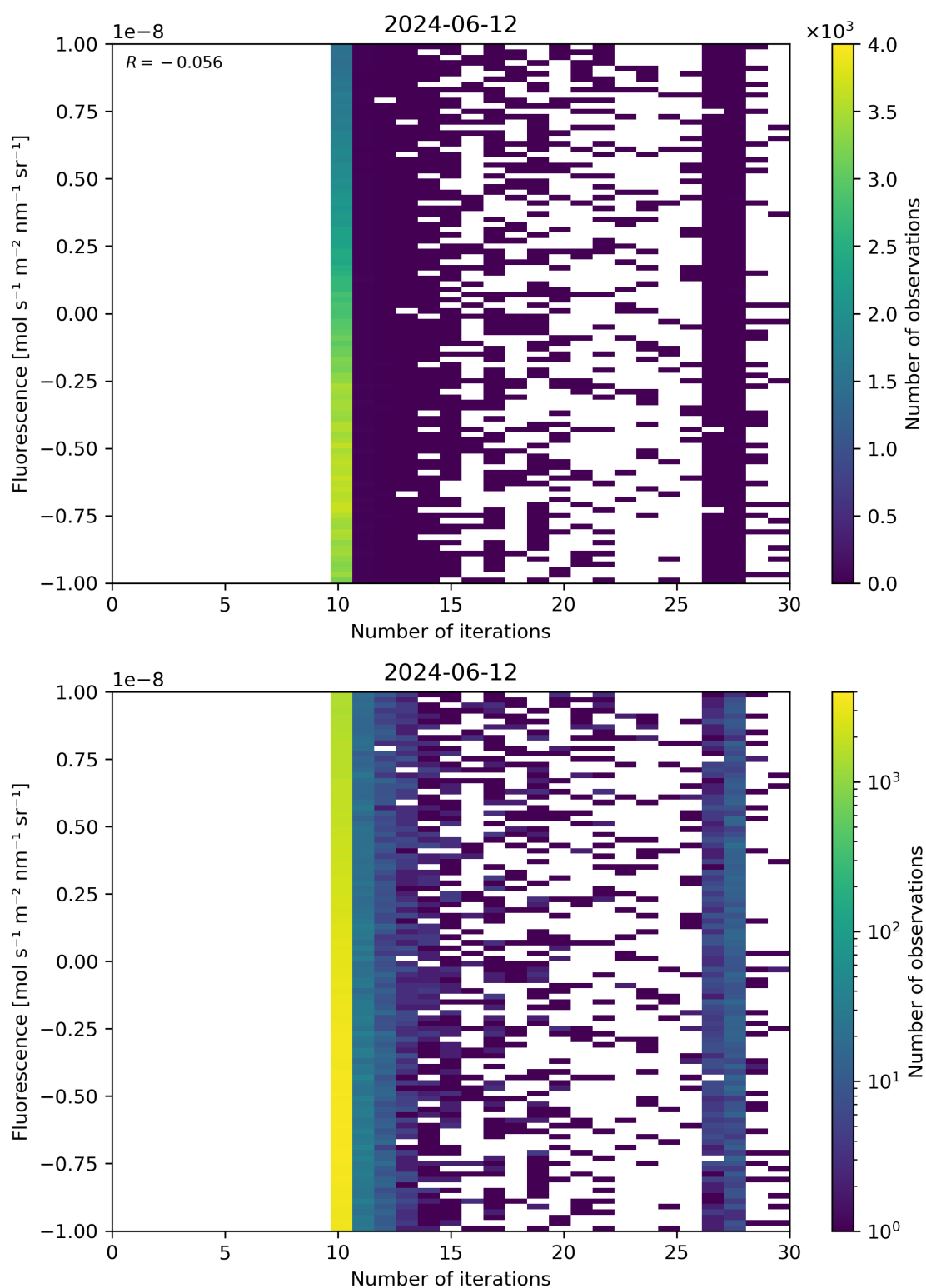
Figure 87: Scatter density plot of “Number of iterations” against “Fluorescence” for 2024-06-11 to 2024-06-13.
