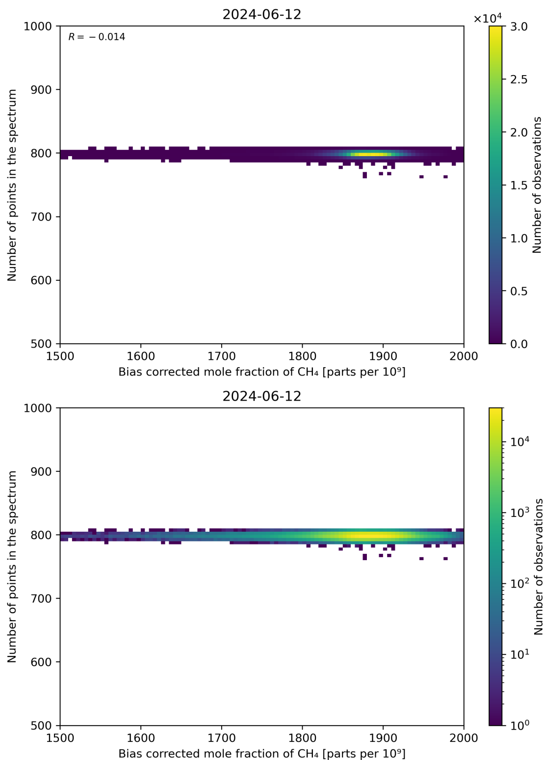
Figure 68: Scatter density plot of “Bias corrected mole fraction of CH 4 ” against “Number of points in the spectrum” for 2024-06-11 to 2024-06-13.
