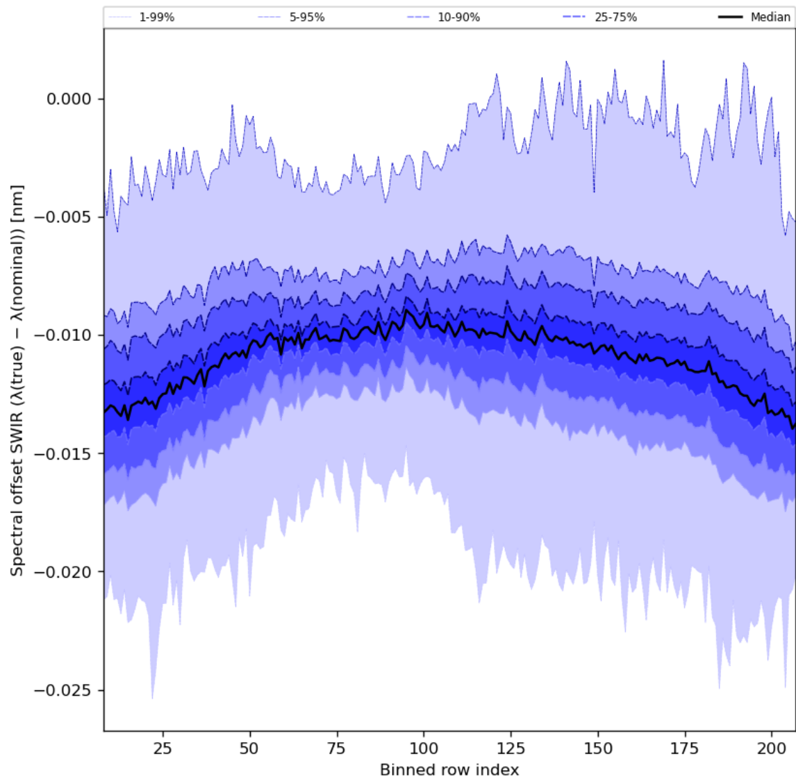
Figure 38: Along track statistics of “Spectral offset SWIR ( \lambda(\text{true}) - \lambda(\text{nominal}) )” for 2024-06-11 to 2024-06-13
