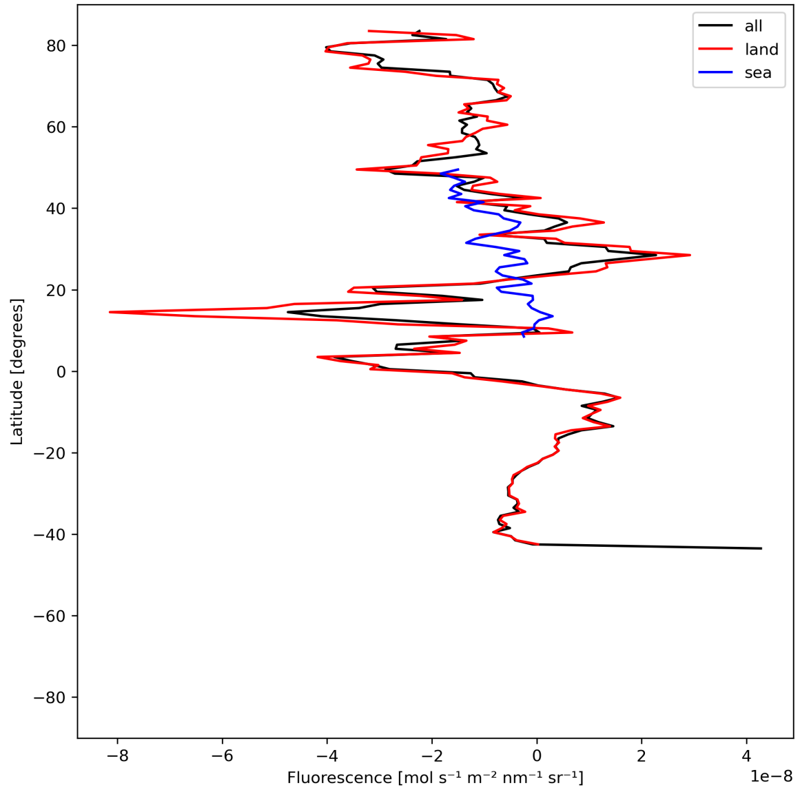
Figure 21: Zonal average of “Fluorescence” for 2024-06-11 to 2024-06-13.
