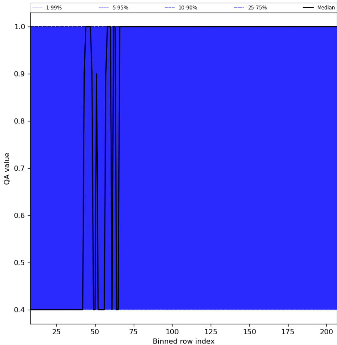
Figure 33: Along track statistics of “QA value” for 2024-06-13 to 2024-06-14
