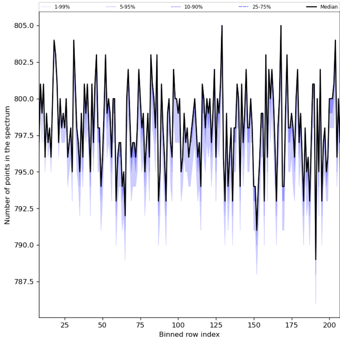
Figure 37: Along track statistics of “Number of points in the spectrum” for 2024-06-13 to 2024-06-14
