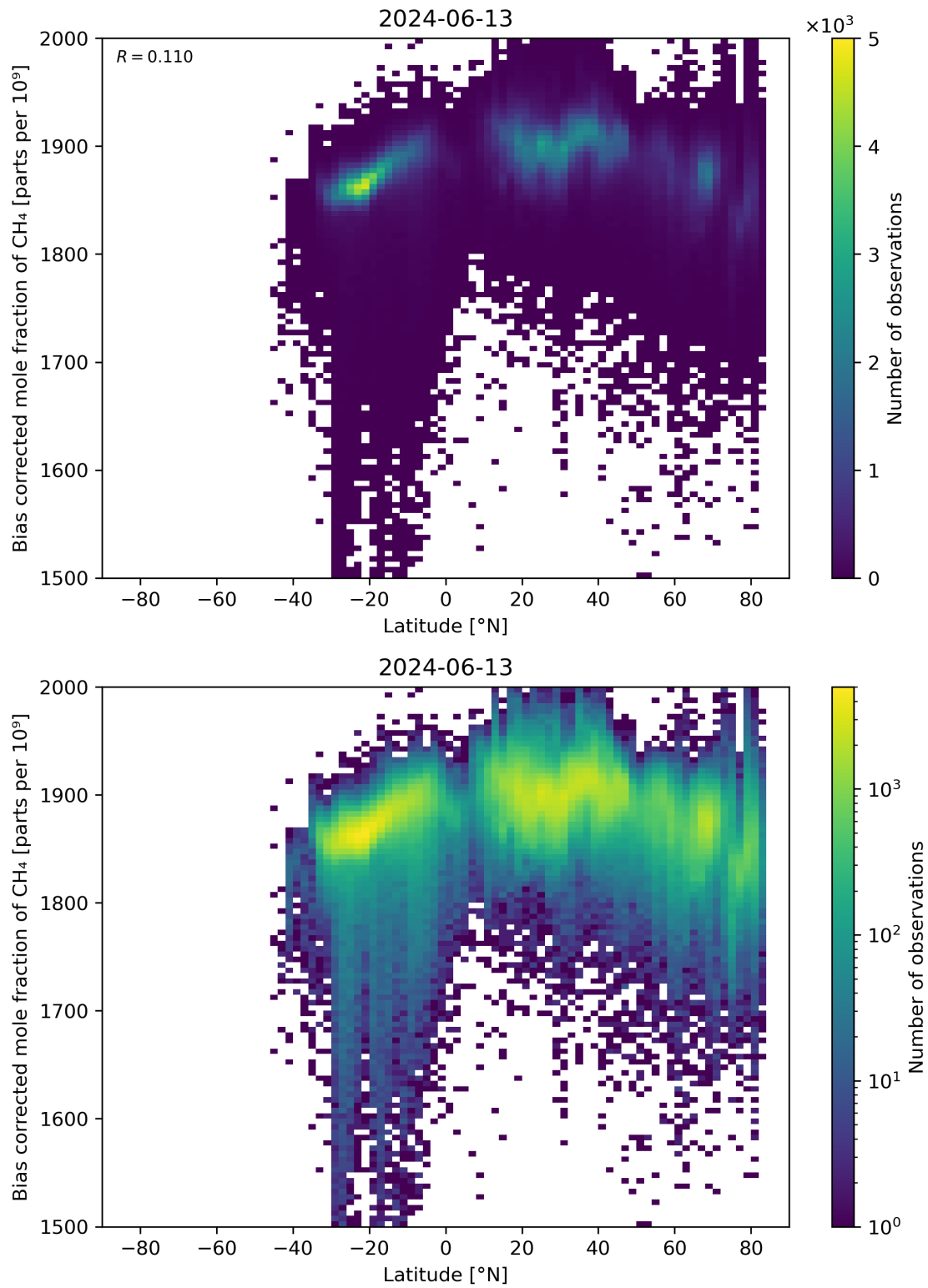
Figure 58: Scatter density plot of “Latitude” against “Bias corrected mole fraction of \text{CH}_4 ” for 2024-06-13 to 2024-06-14.
