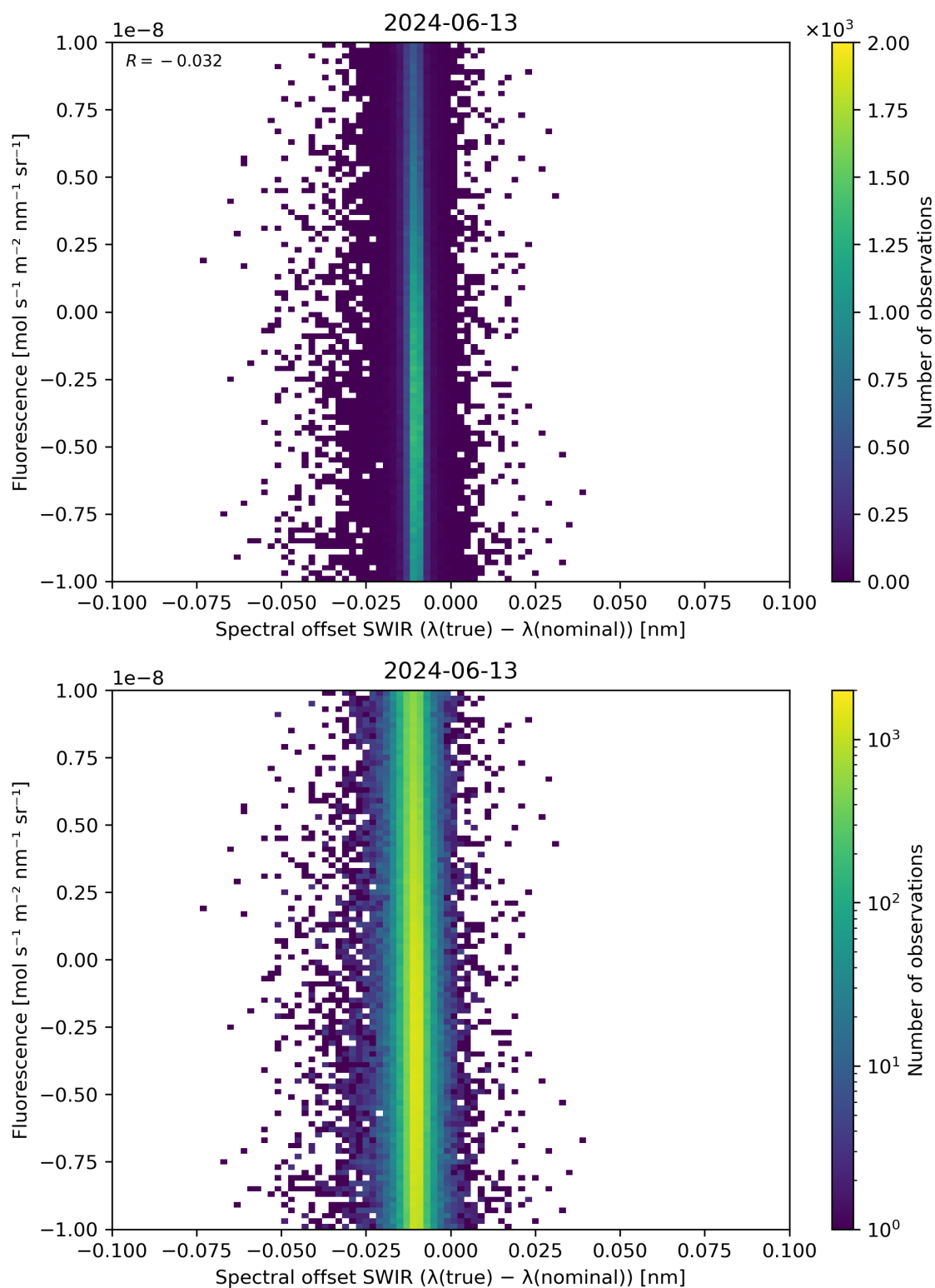
Figure 120: Scatter density plot of “Spectral offset SWIR ( \lambda(\text{true}) - \lambda(\text{nominal}) )” against “Fluorescence” for 2024-06-13 to 2024-06-14.
