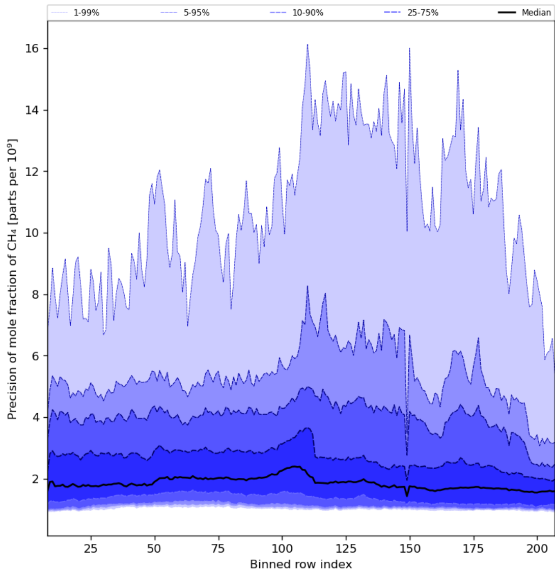
Figure 35: Along track statistics of “Precision of mole fraction of CH 4 ” for 2024-06-13 to 2024-06-14
