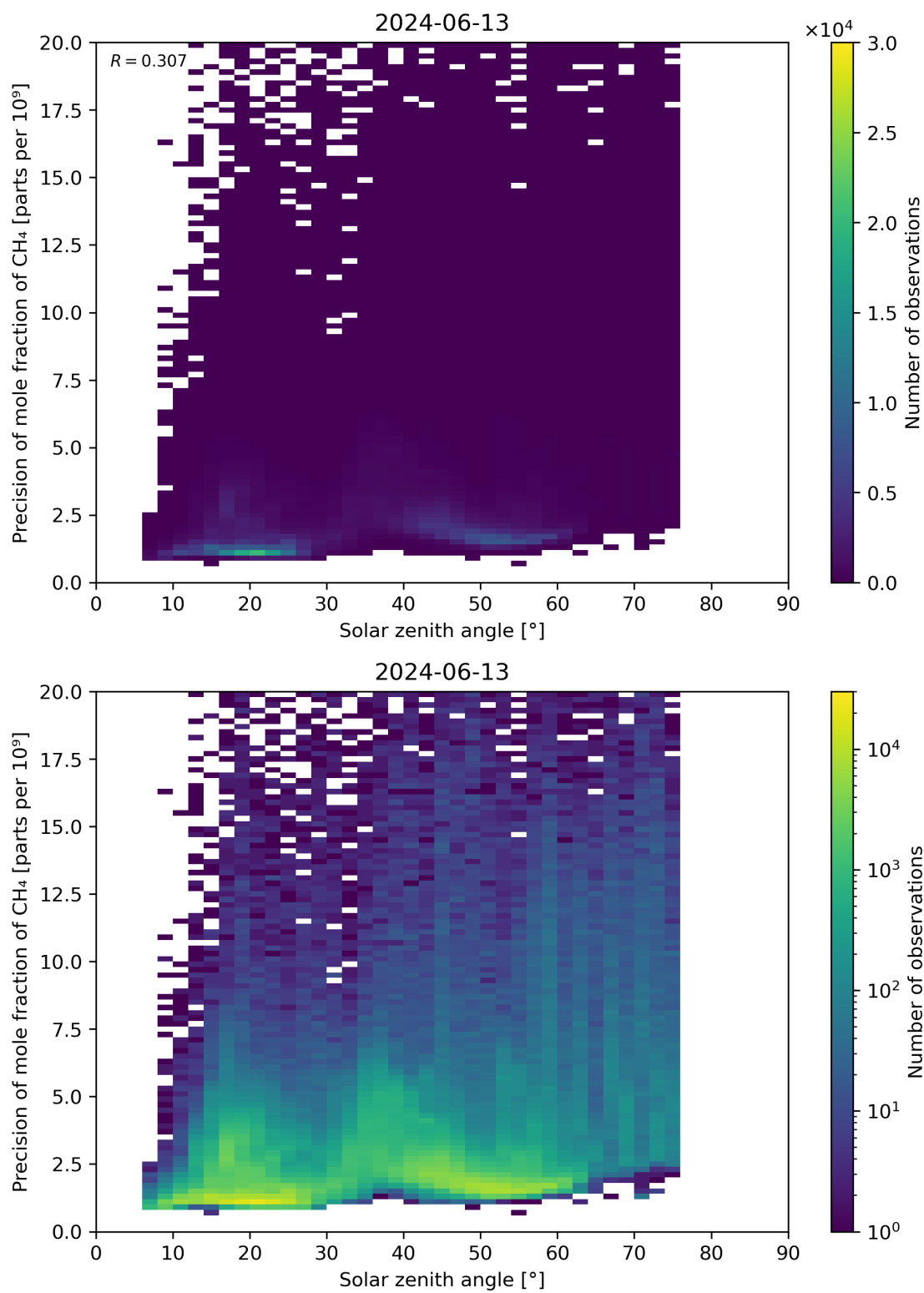
Figure 101: Scatter density plot of “Solar zenith angle” against “Precision of mole fraction of CH 4 ” for 2024-06-13 to 2024-06-14.
