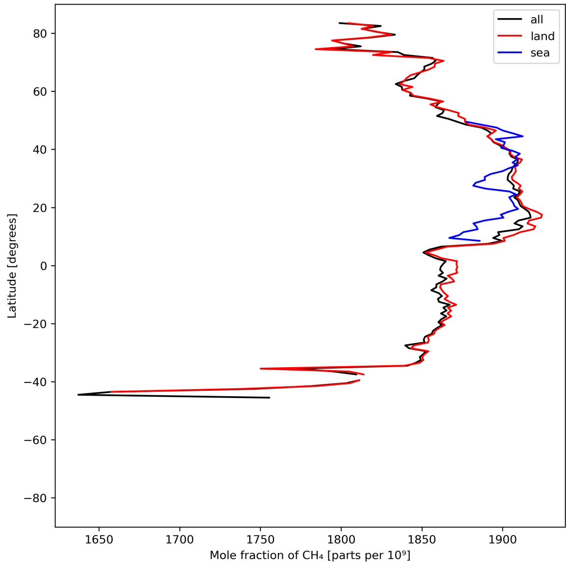
Figure 12: Zonal average of “Mole fraction of CH 4 ” for 2024-06-13 to 2024-06-14.
