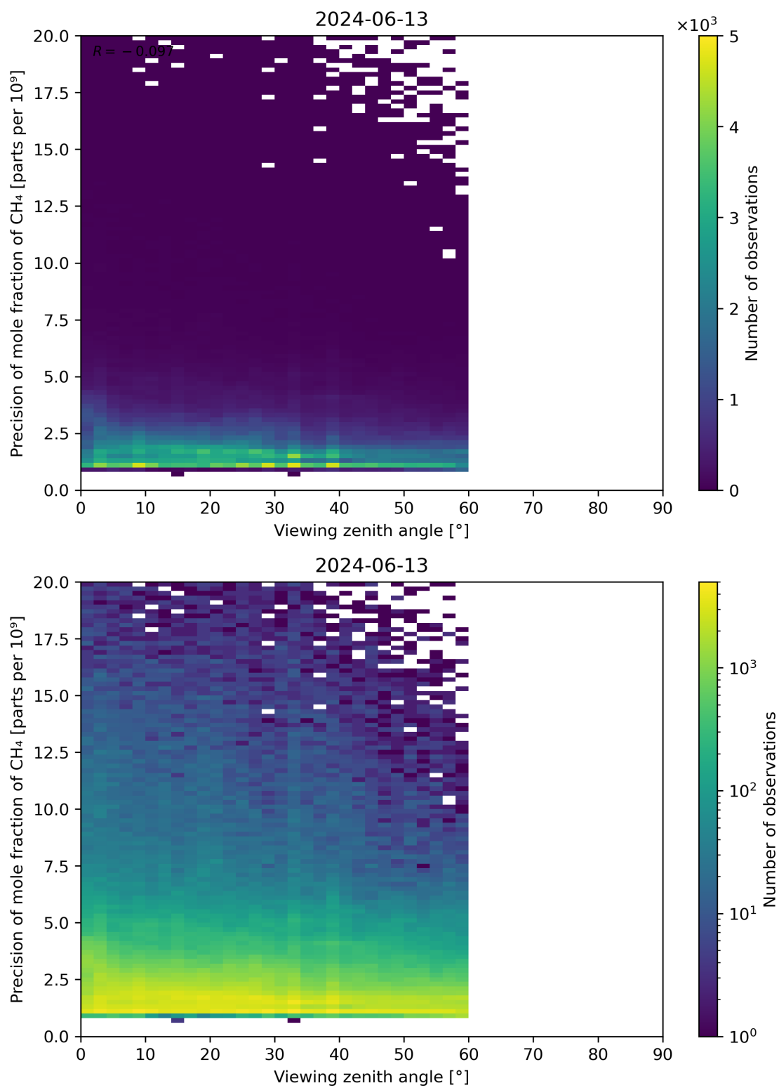
Figure 112: Scatter density plot of “Viewing zenith angle” against “Precision of mole fraction of CH 4 ” for 2024-06-13 to 2024-06-14.
