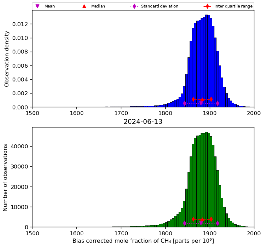
Figure 25: Histogram of “Bias corrected mole fraction of CH 4 ” for 2024-06-13 to 2024-06-14
