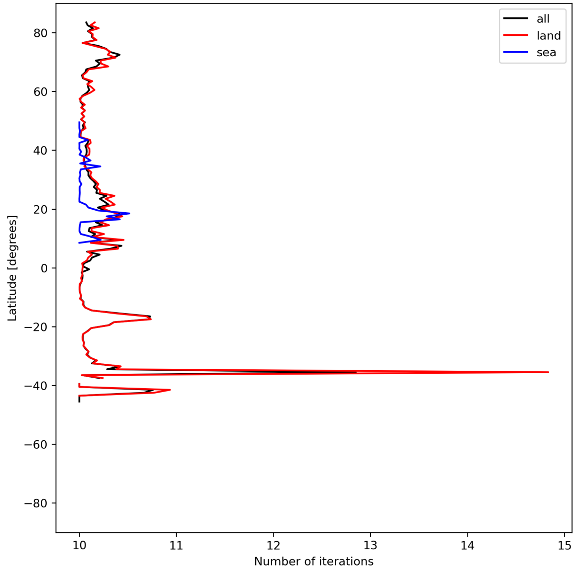
Figure 20: Zonal average of “Number of iterations” for 2024-06-13 to 2024-06-14.
