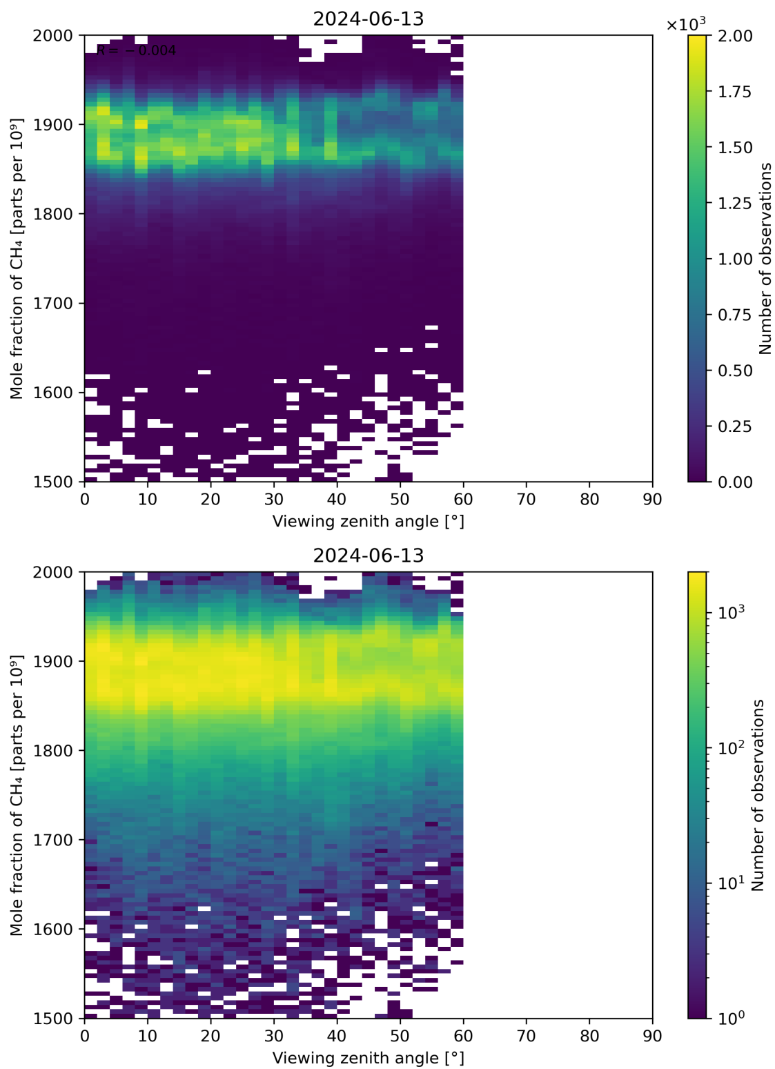
Figure 110: Scatter density plot of “Viewing zenith angle” against “Mole fraction of CH 4 ” for 2024-06-13 to 2024-06-14.
