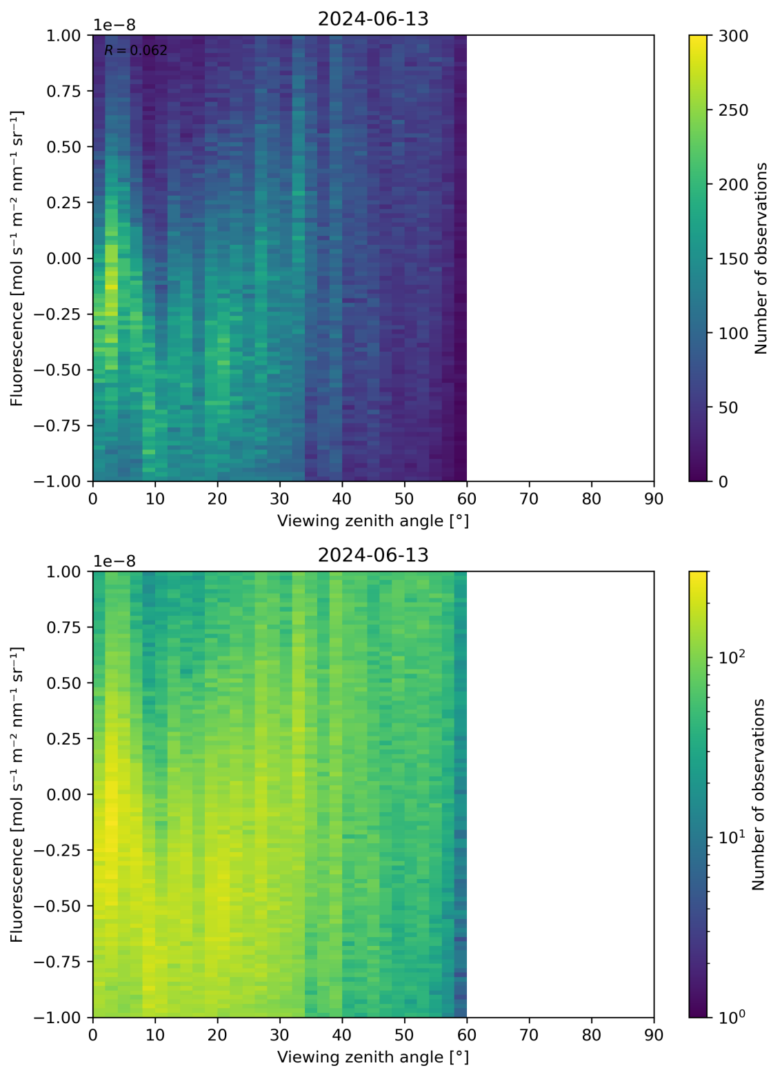
Figure 108: Scatter density plot of “Viewing zenith angle” against “Fluorescence” for 2024-06-13 to 2024-06-14.
