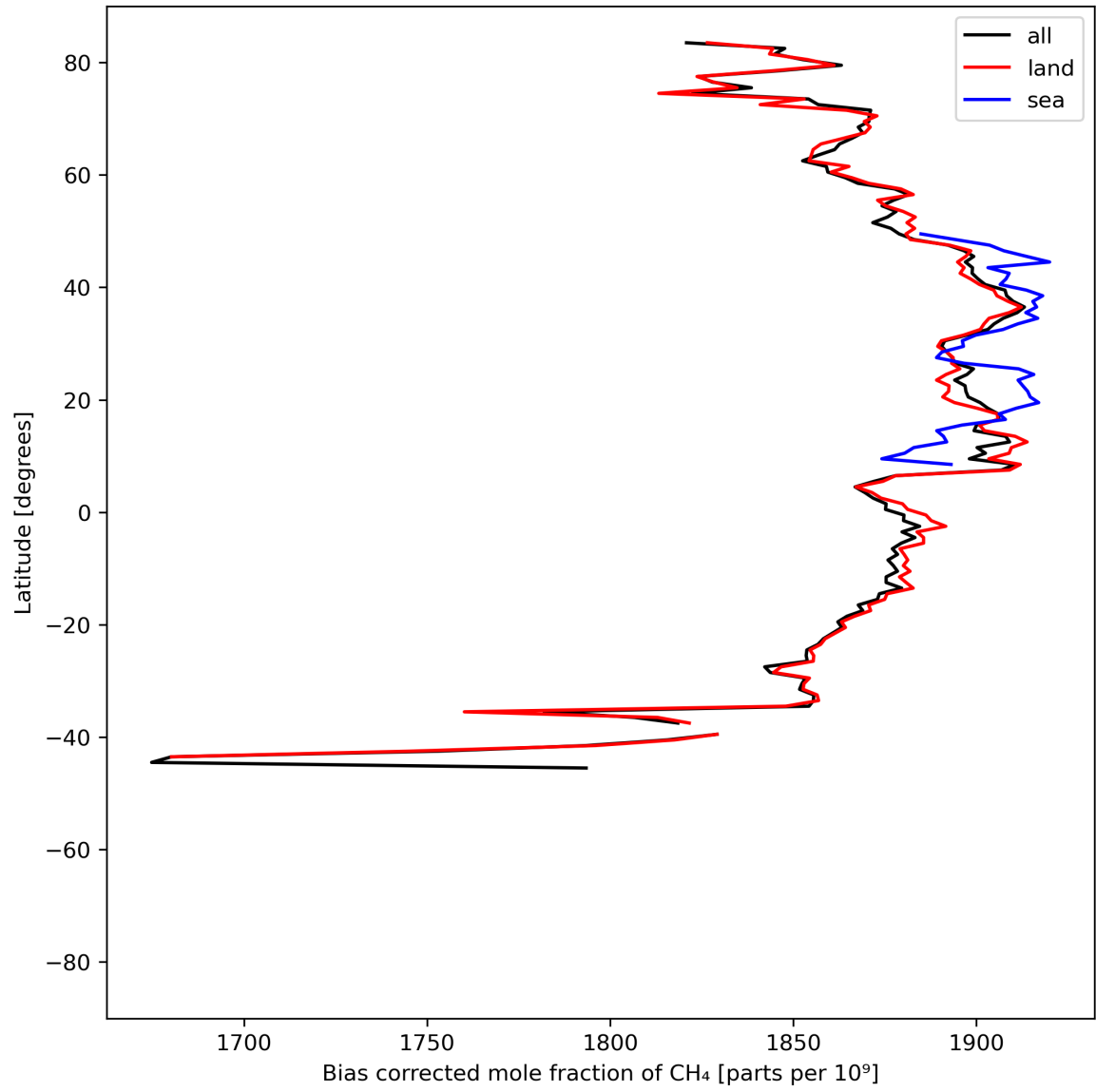
Figure 14: Zonal average of “Bias corrected mole fraction of CH 4 ” for 2024-06-13 to 2024-06-14.
