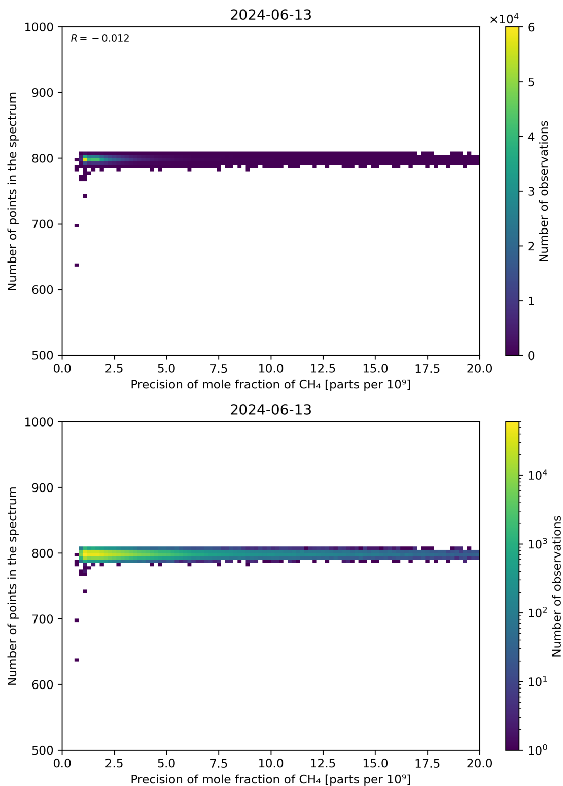
Figure 84: Scatter density plot of “Precision of mole fraction of CH 4 ” against “Number of points in the spectrum” for 2024-06-13 to 2024-06-14.
