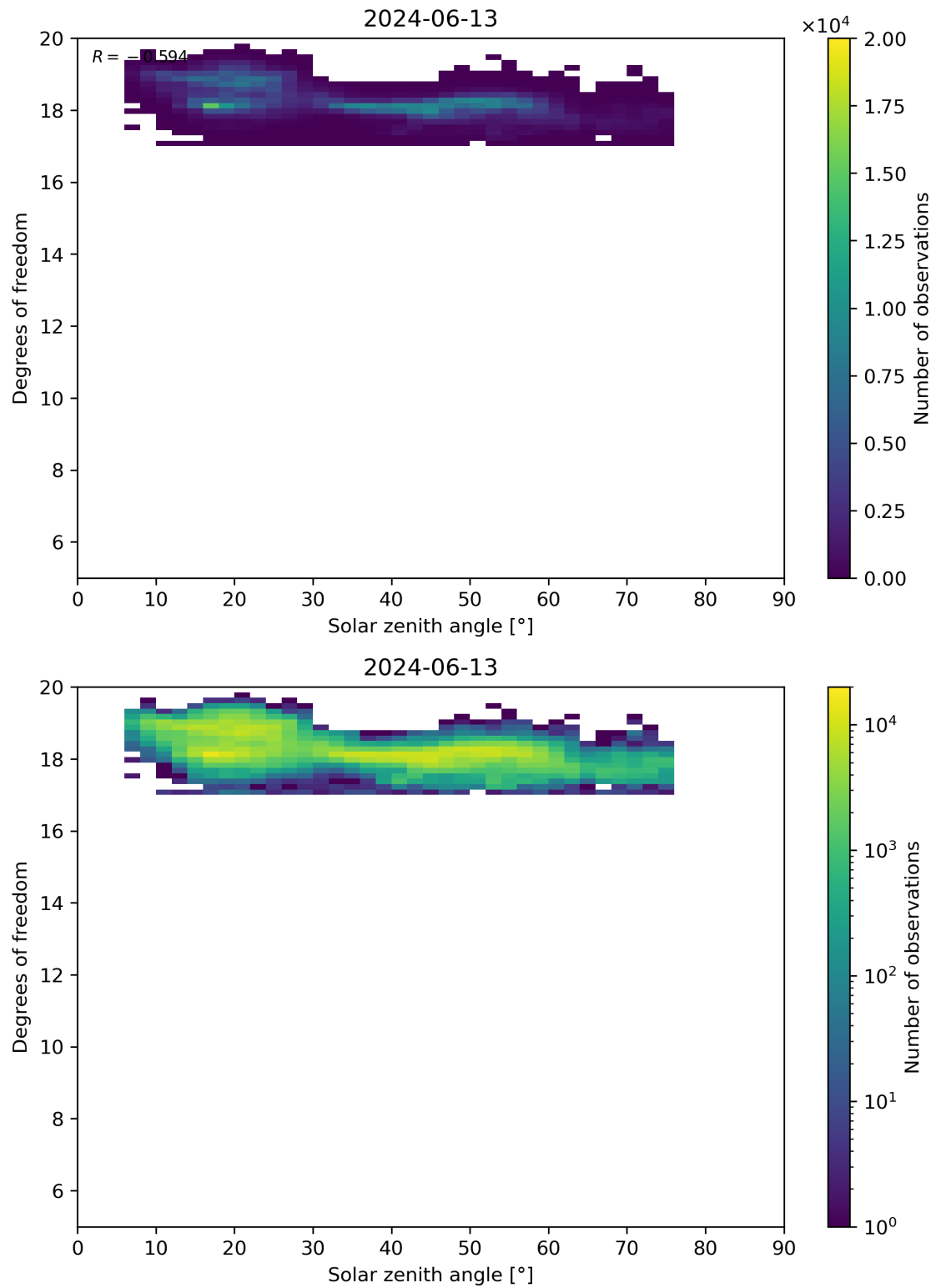
Figure 96: Scatter density plot of “Solar zenith angle” against “Degrees of freedom” for 2024-06-13 to 2024-06-14.
