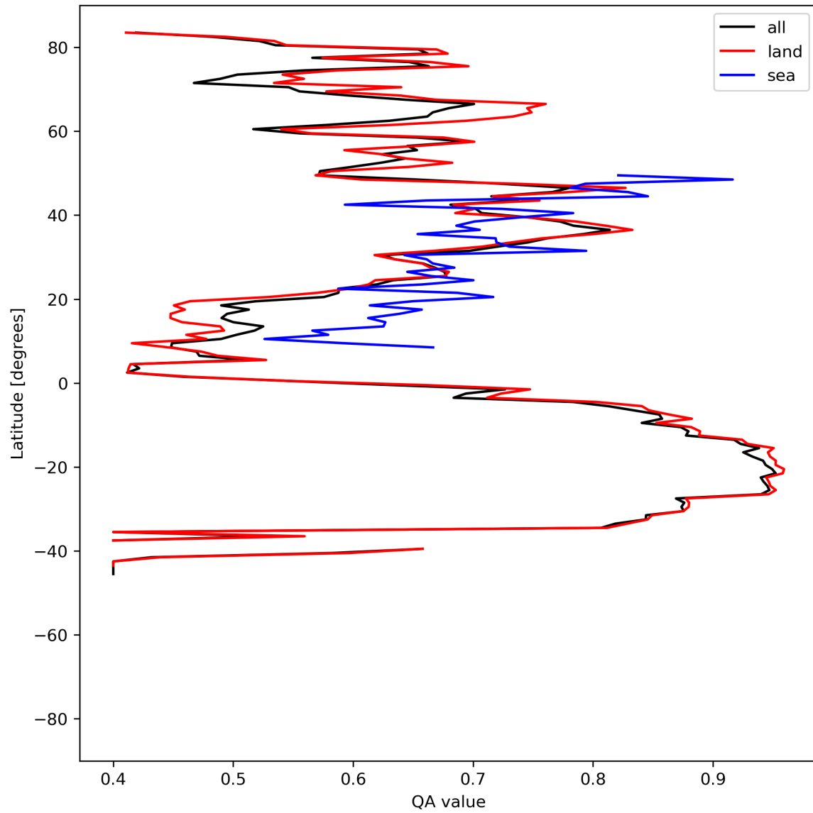
Figure 11: Zonal average of “QA value” for 2024-06-13 to 2024-06-14.
