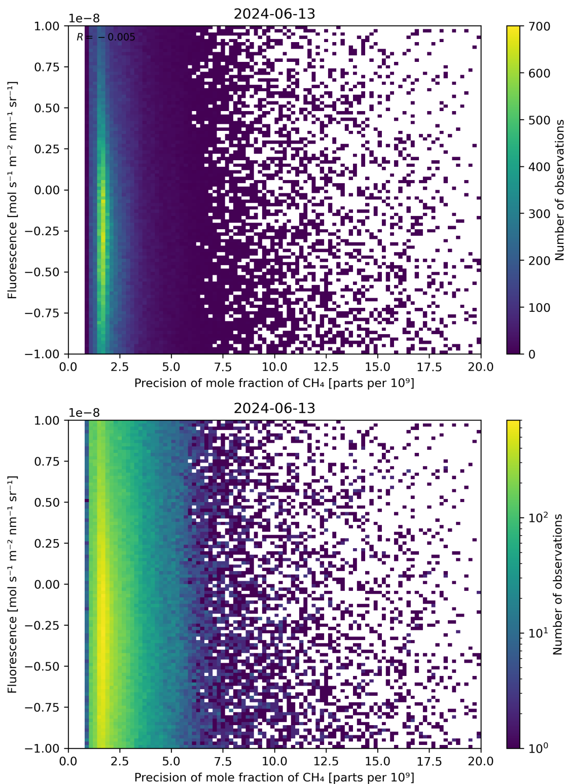
Figure 81: Scatter density plot of “Precision of mole fraction of CH 4 ” against “Fluorescence” for 2024-06-13 to 2024-06-14.
