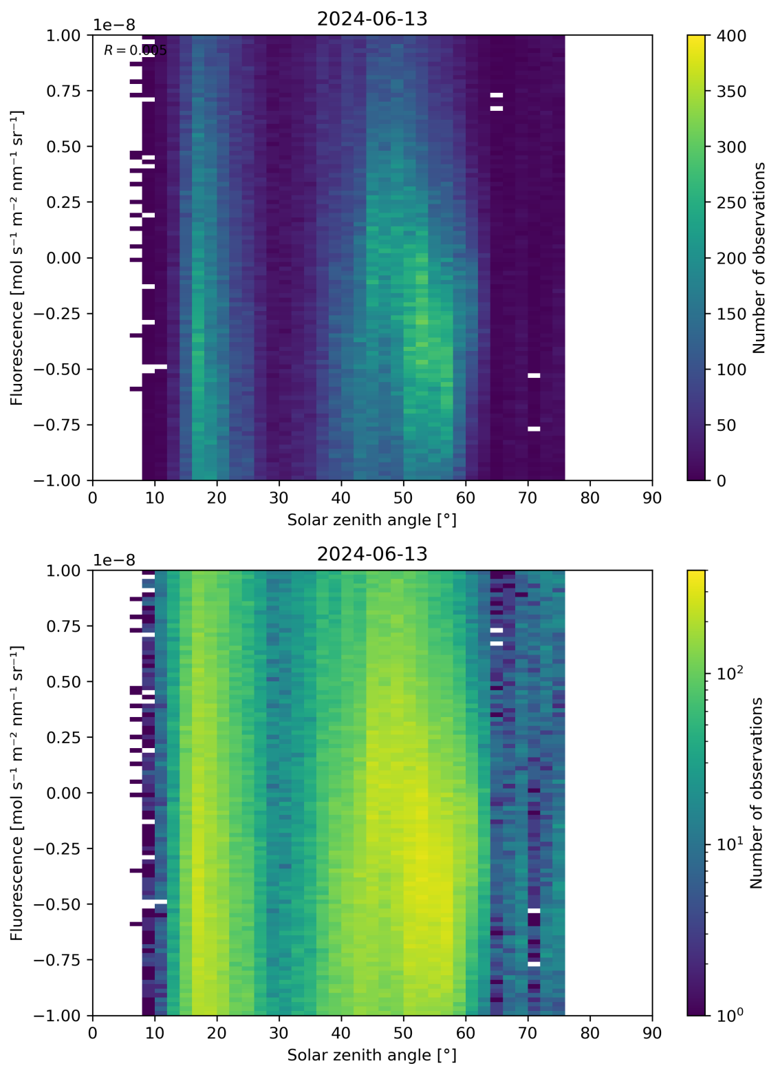
Figure 97: Scatter density plot of “Solar zenith angle” against “Fluorescence” for 2024-06-13 to 2024-06-14.
