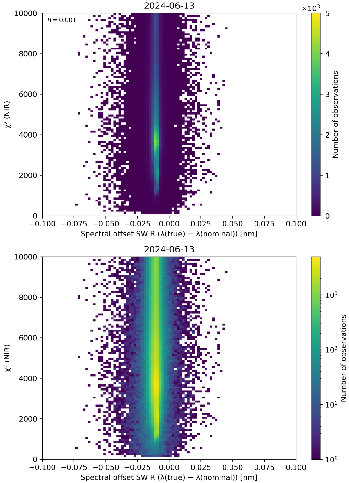
Figure 117: Scatter density plot of “Spectral offset SWIR ( \lambda(\text{true}) - \lambda(\text{nominal}) )” against “ \chi^2 (NIR)” for 2024-06-13 to 2024-06-14.
