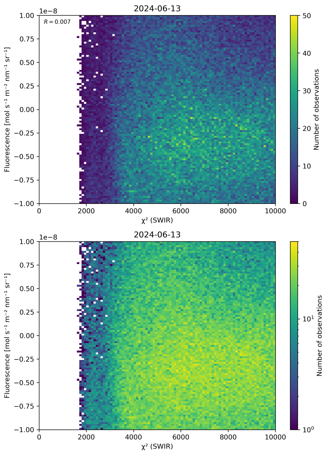
Figure 49: Scatter density plot of “ \chi^2 (SWIR)” against “Fluorescence” for 2024-06-13 to 2024-06-14.
