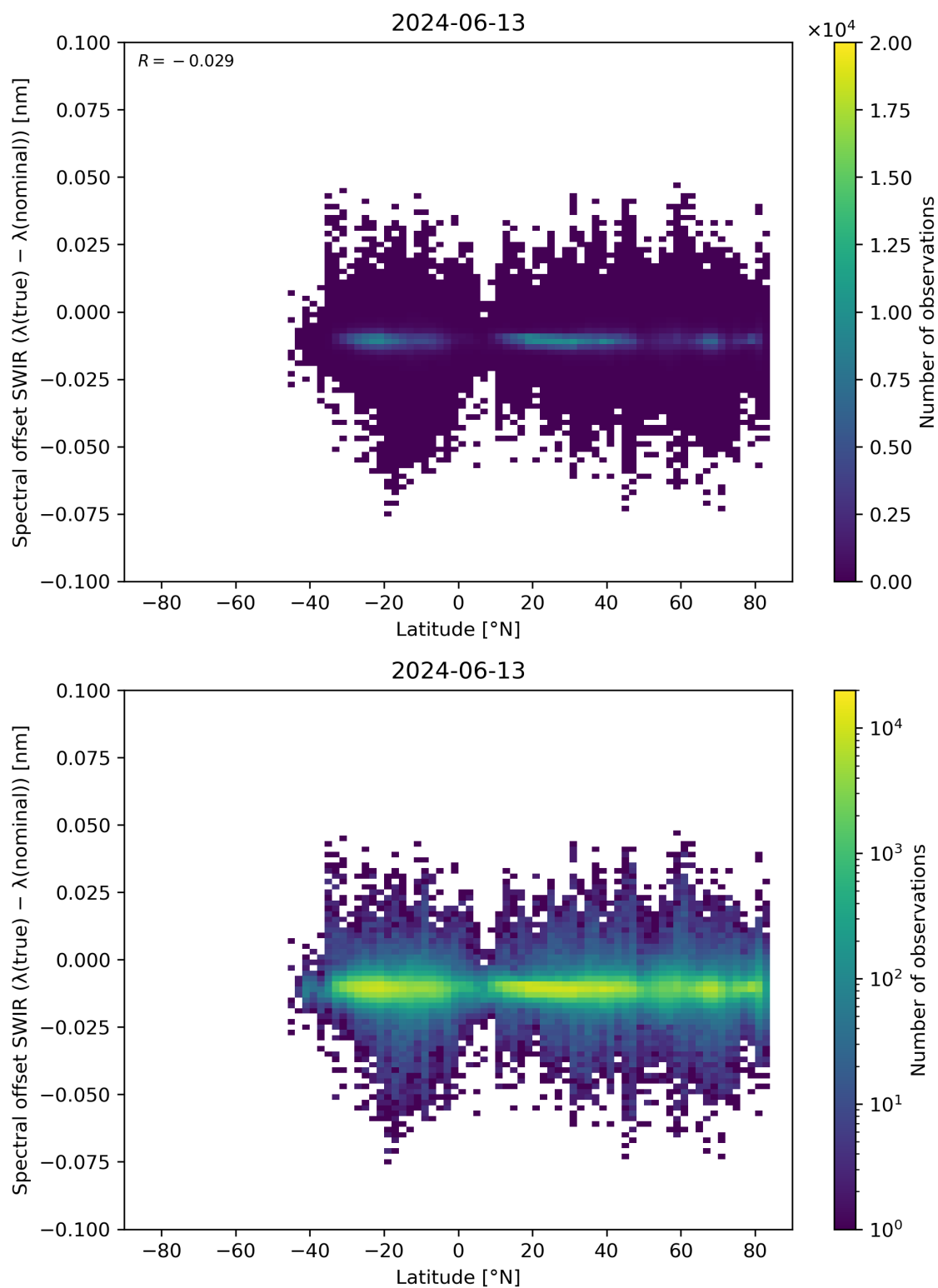
Figure 62: Scatter density plot of “Latitude” against “Spectral offset SWIR ( \lambda(\text{true}) - \lambda(\text{nominal}) )” for 2024-06-13 to 2024-06-14.
