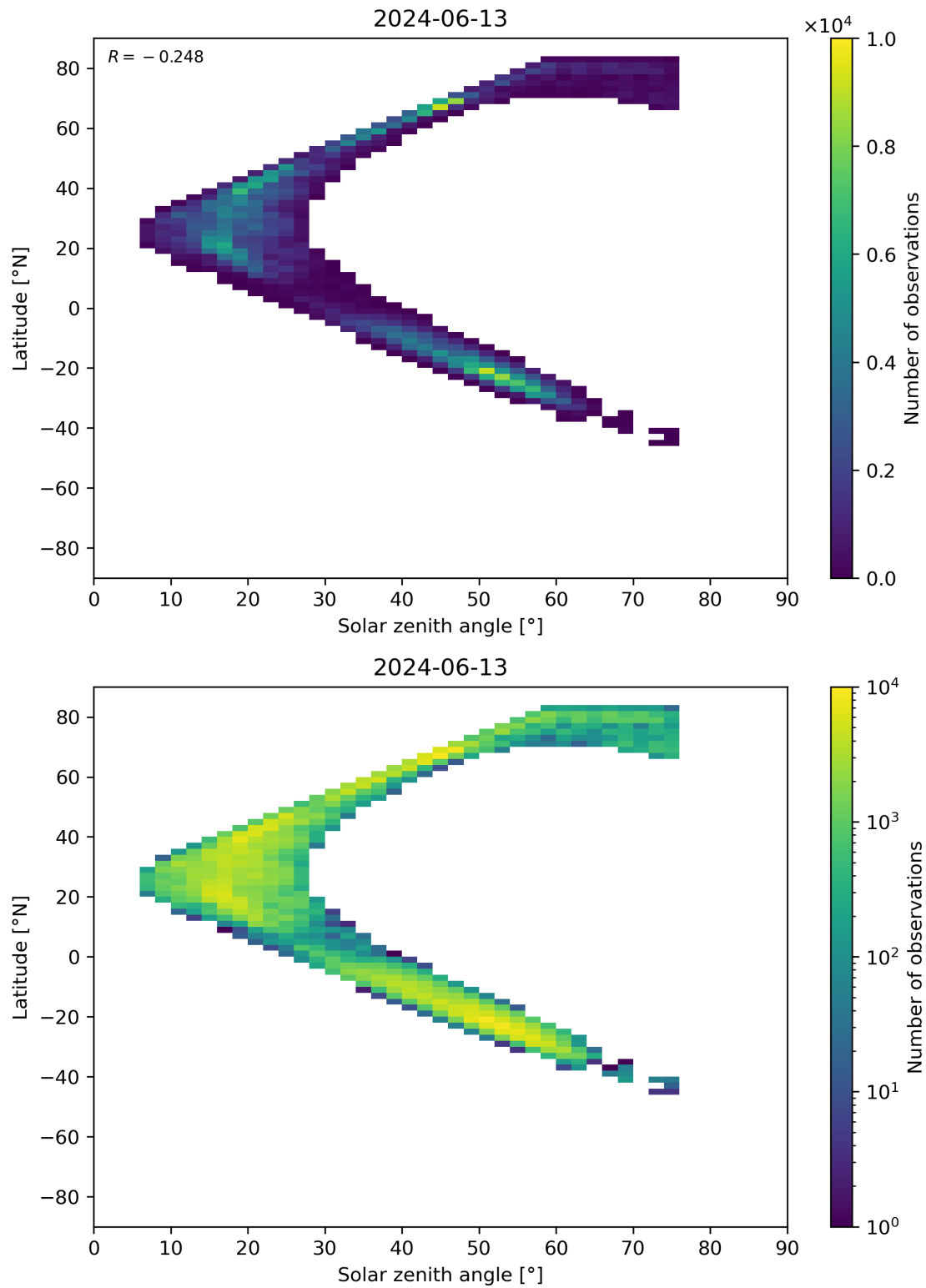
Figure 98: Scatter density plot of “Solar zenith angle” against “Latitude” for 2024-06-13 to 2024-06-14.
