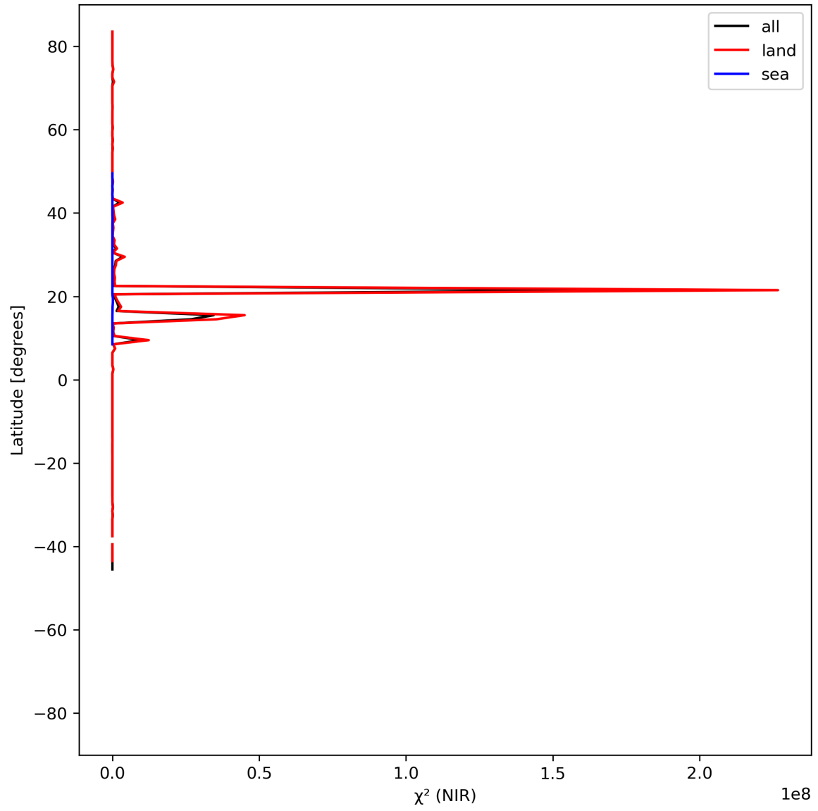
Figure 18: Zonal average of “ \chi^2 (NIR)” for 2024-06-13 to 2024-06-14.
