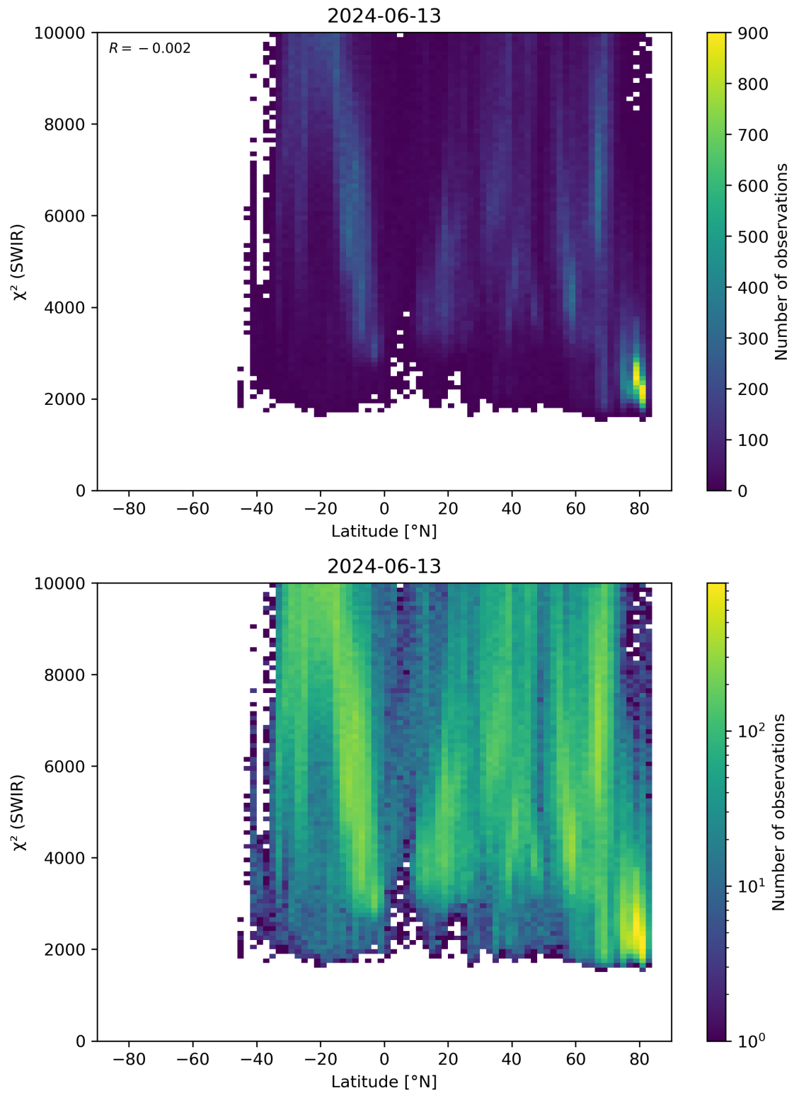
Figure 54: Scatter density plot of “Latitude” against “ \chi^2 (SWIR)” for 2024-06-13 to 2024-06-14.
