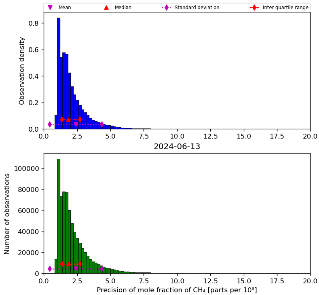
Figure 24: Histogram of “Precision of mole fraction of CH 4 ” for 2024-06-13 to 2024-06-14
