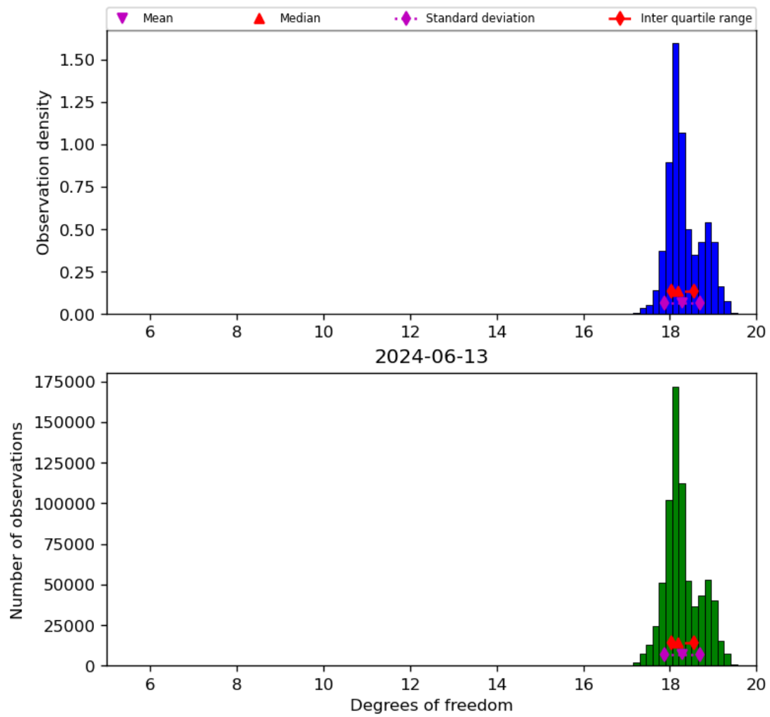
Figure 30: Histogram of “Degrees of freedom” for 2024-06-13 to 2024-06-14
