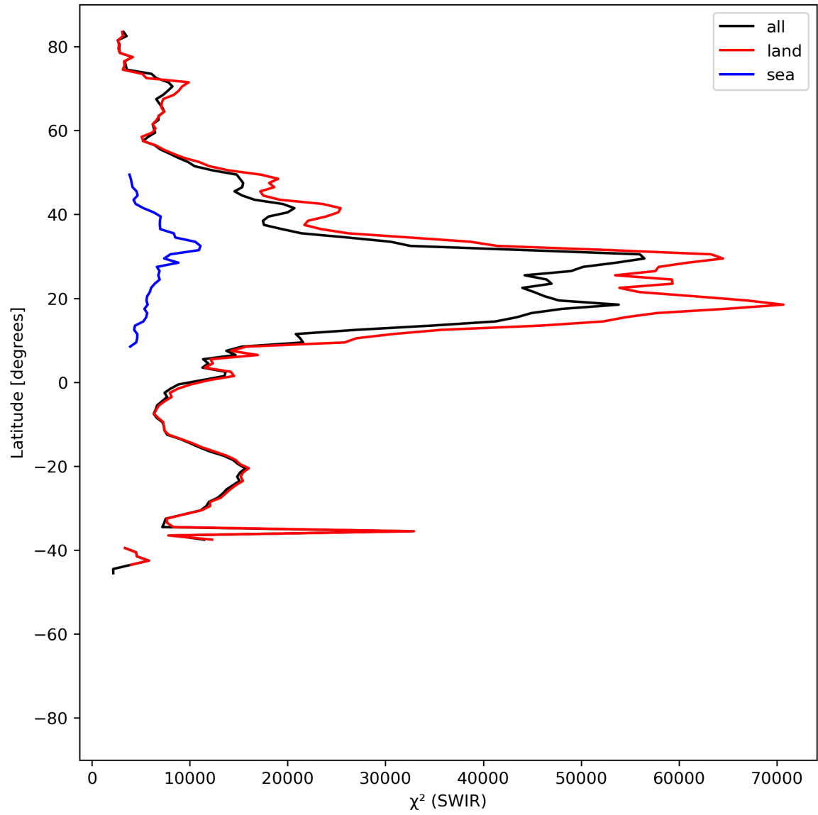
Figure 17: Zonal average of “ \chi^2 (SWIR)” for 2024-06-13 to 2024-06-14.
