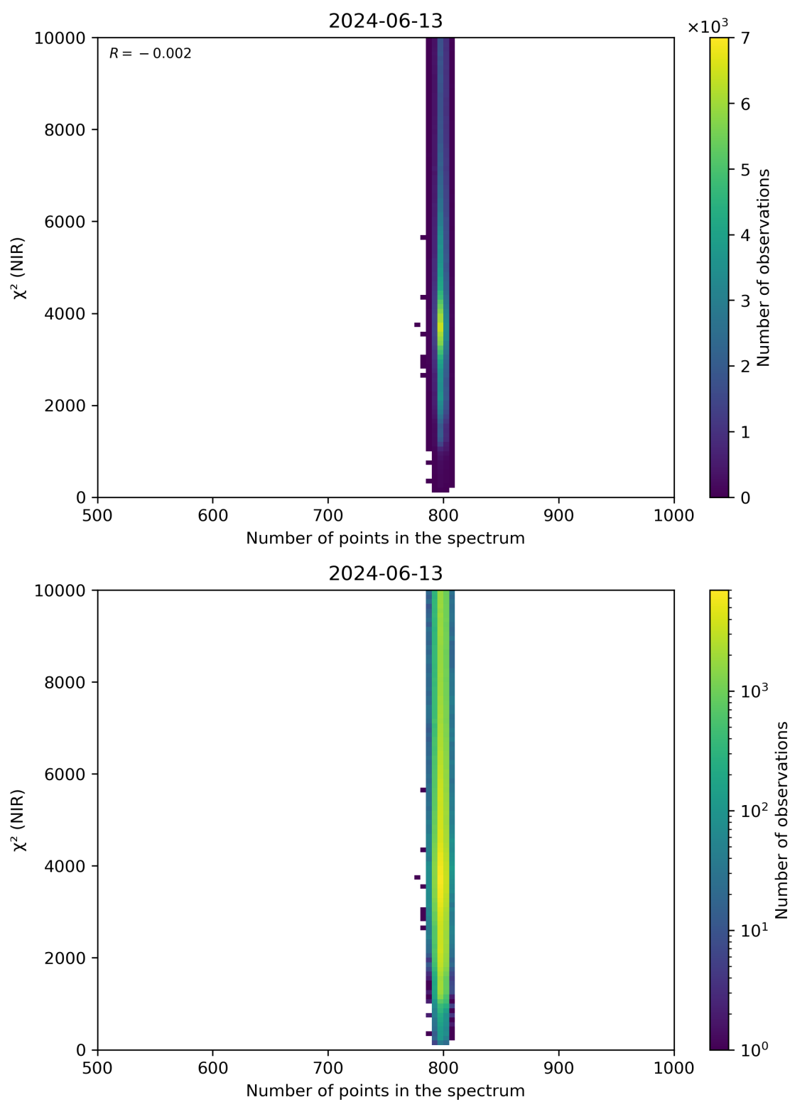
Figure 88: Scatter density plot of “Number of points in the spectrum” against “ \chi^2 (NIR)” for 2024-06-13 to 2024-06-14.
