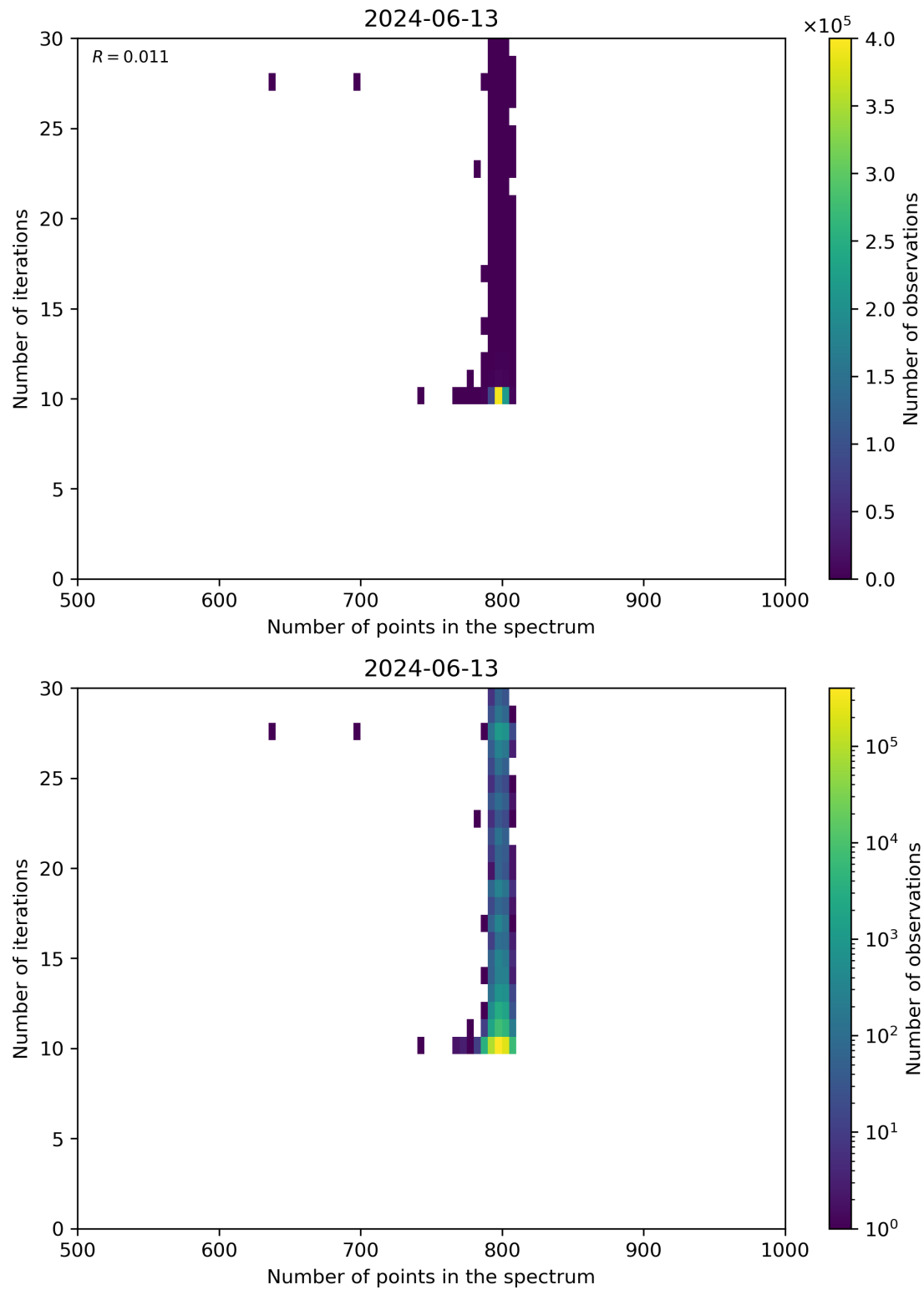
Figure 92: Scatter density plot of “Number of points in the spectrum” against “Number of iterations” for 2024-06-13 to 2024-06-14.
