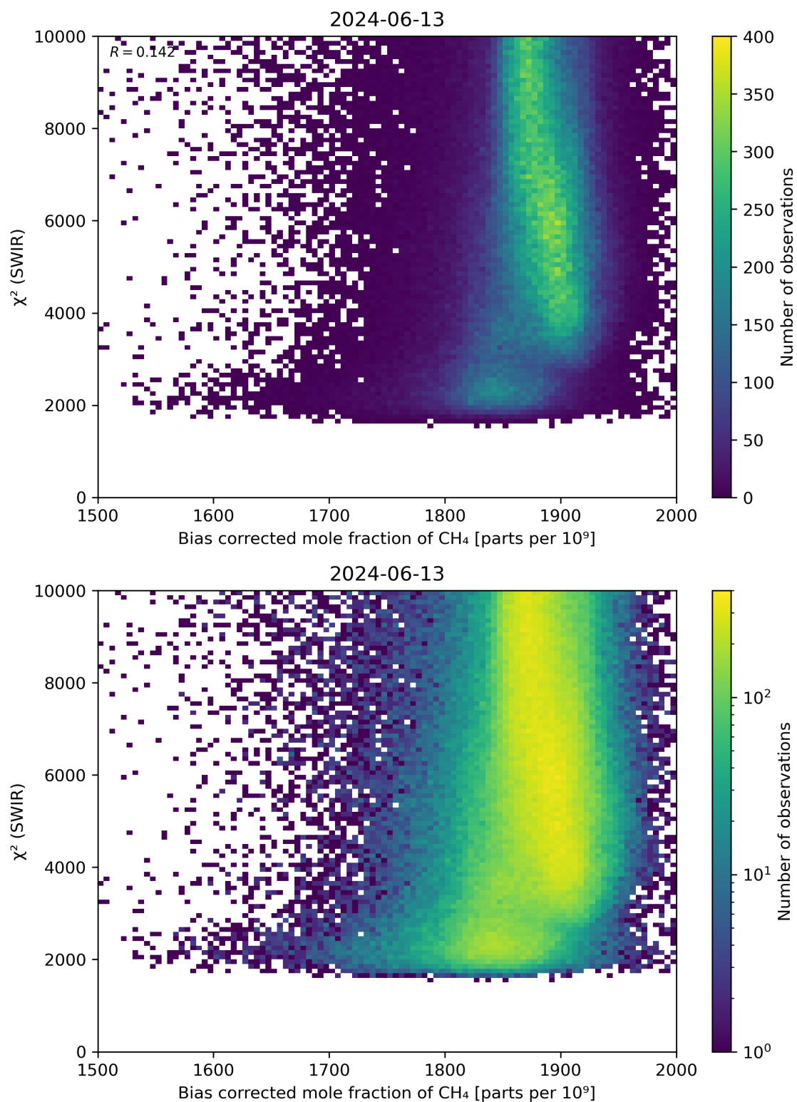
Figure 64: Scatter density plot of “Bias corrected mole fraction of \text{CH}_4 ” against “ \chi^2 (SWIR)” for 2024-06-13 to 2024-06-14.
