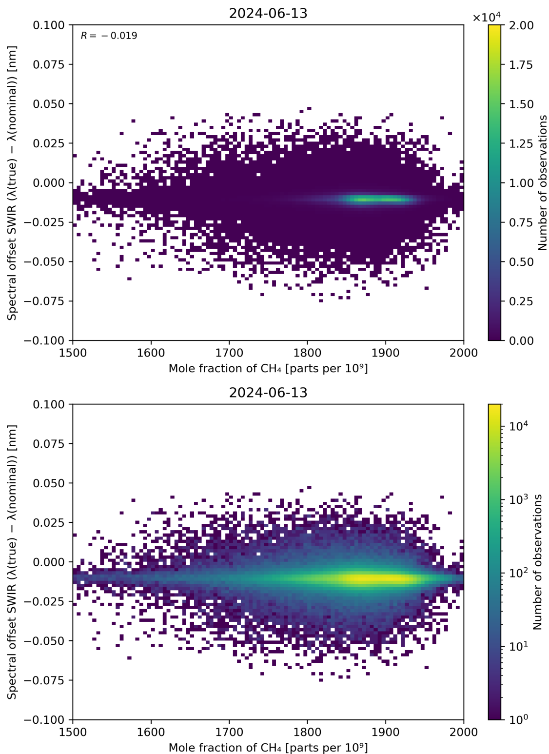
Figure 86: Scatter density plot of “Mole fraction of CH 4 ” against “Spectral offset SWIR ( \lambda(\text{true}) - \lambda(\text{nominal}) )” for 2024-06-13 to 2024-06-14.
