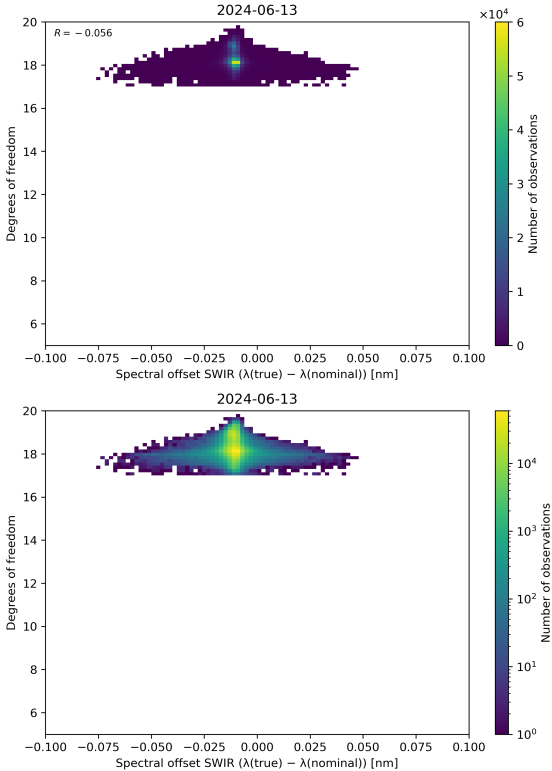
Figure 119: Scatter density plot of “Spectral offset SWIR ( \lambda(\text{true}) - \lambda(\text{nominal}) )” against “Degrees of freedom” for 2024-06-13 to 2024-06-14.
