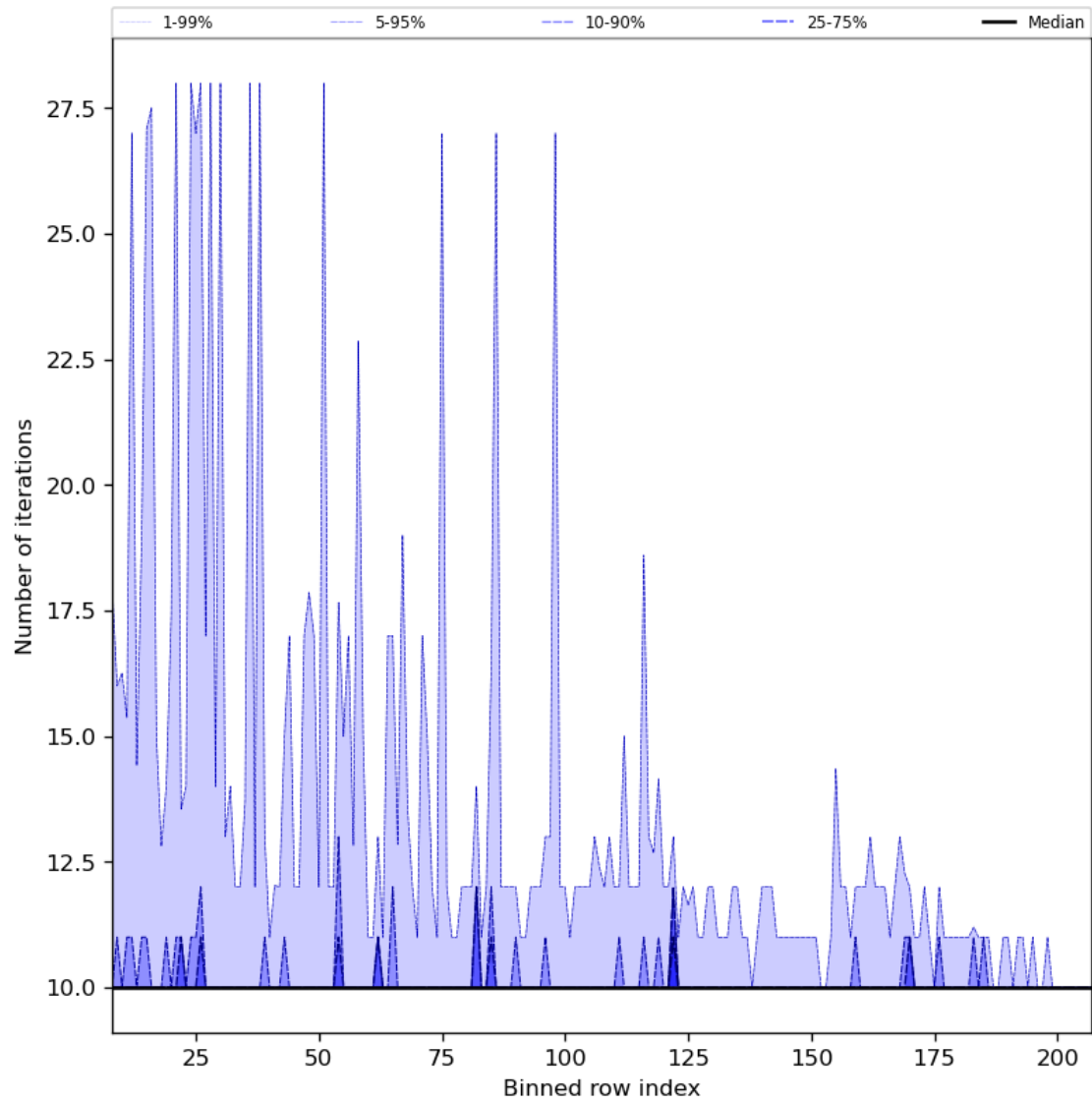
Figure 42: Along track statistics of “Number of iterations” for 2024-06-13 to 2024-06-14
