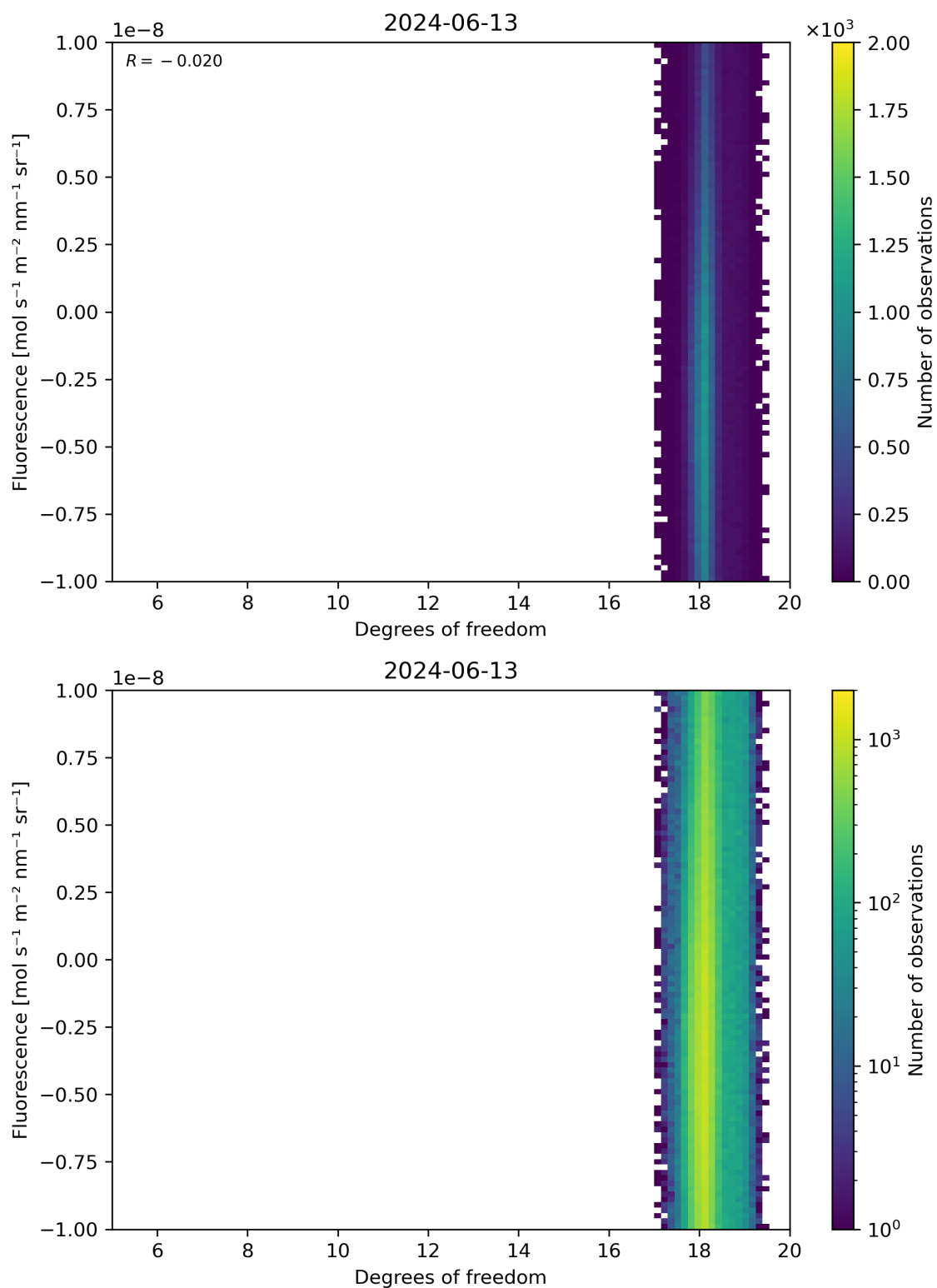
Figure 51: Scatter density plot of “Degrees of freedom” against “Fluorescence” for 2024-06-13 to 2024-06-14.
