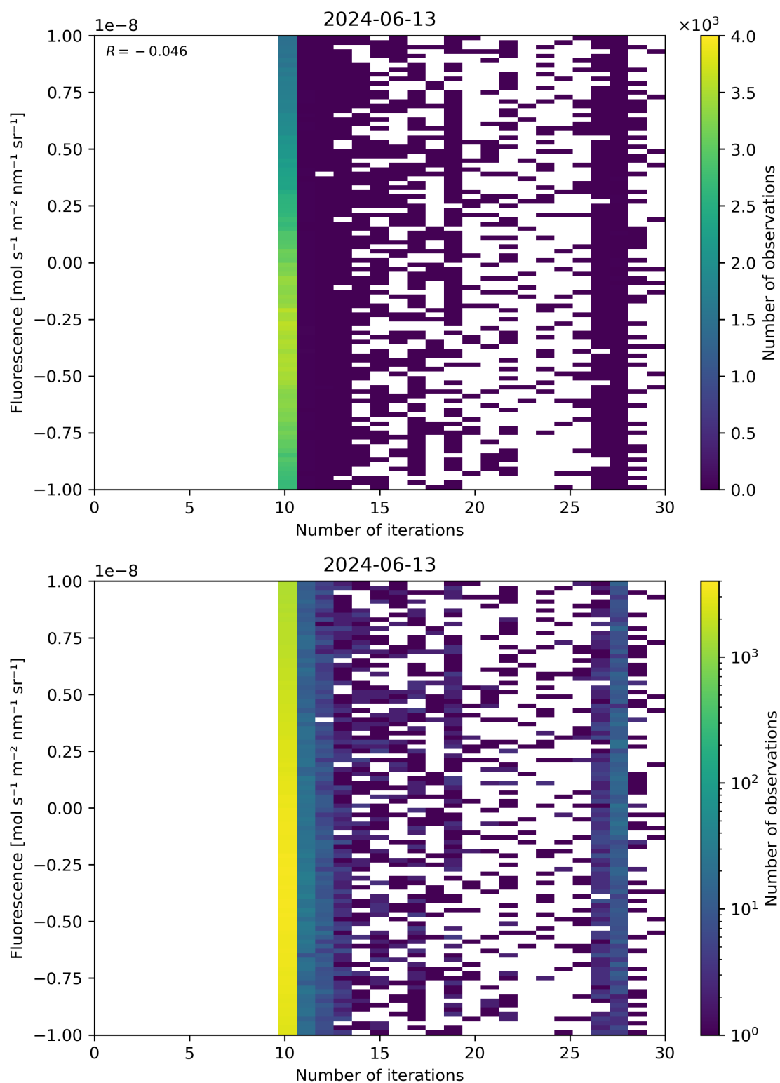
Figure 87: Scatter density plot of “Number of iterations” against “Fluorescence” for 2024-06-13 to 2024-06-14.
