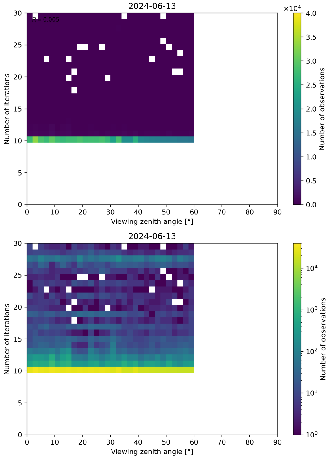
Figure 113: Scatter density plot of “Viewing zenith angle” against “Number of iterations” for 2024-06-13 to 2024-06-14.
