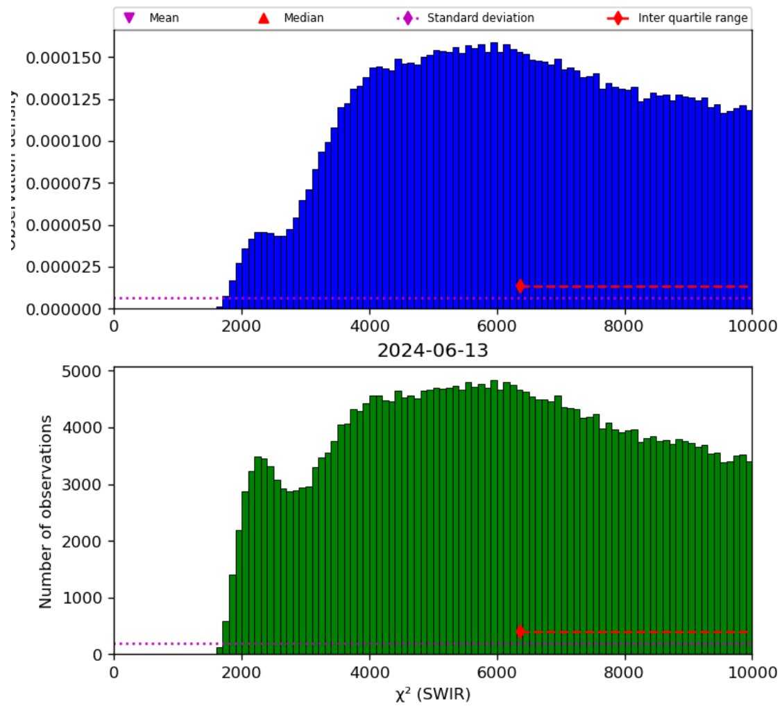
Figure 28: Histogram of “ \chi^2 (SWIR)” for 2024-06-13 to 2024-06-14
