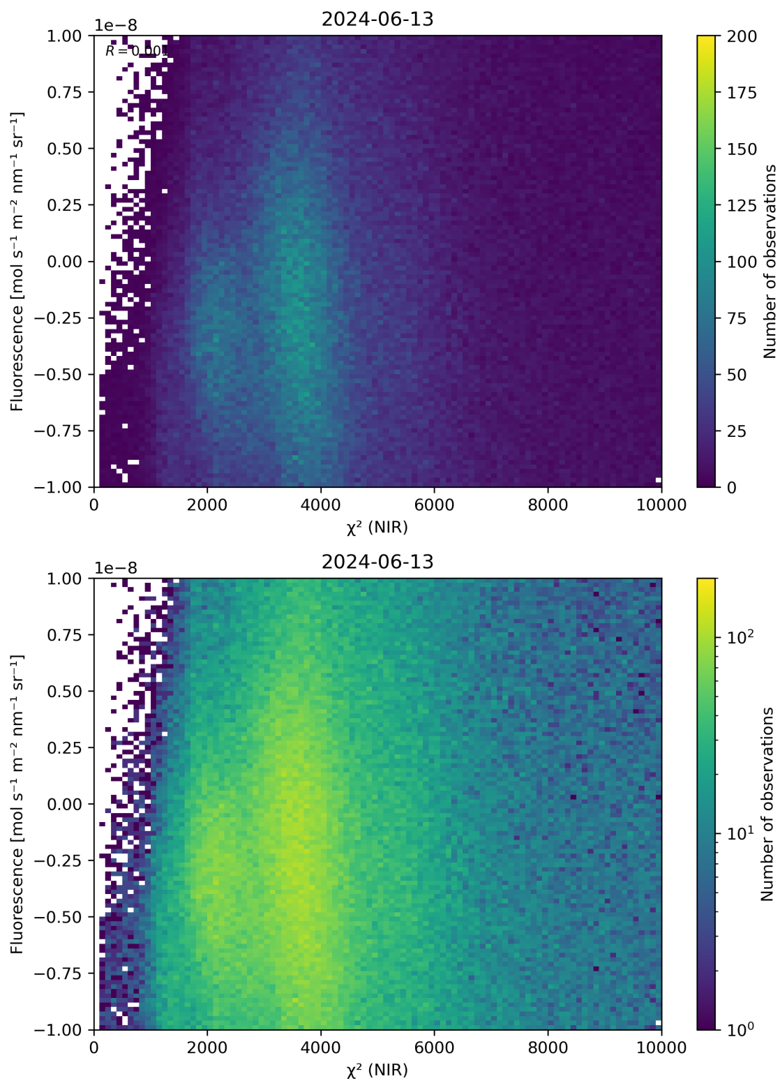
Figure 45: Scatter density plot of “ \chi^2 (NIR)” against “Fluorescence” for 2024-06-13 to 2024-06-14.
