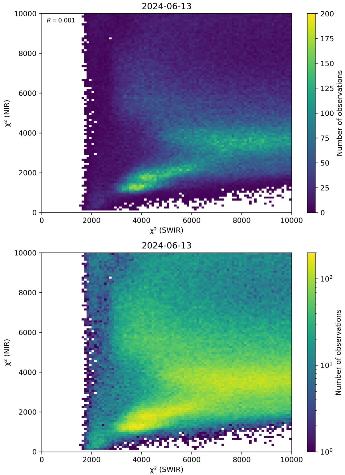
Figure 47: Scatter density plot of “ \chi^2 (SWIR)” against “ \chi^2 (NIR)” for 2024-06-13 to 2024-06-14.
