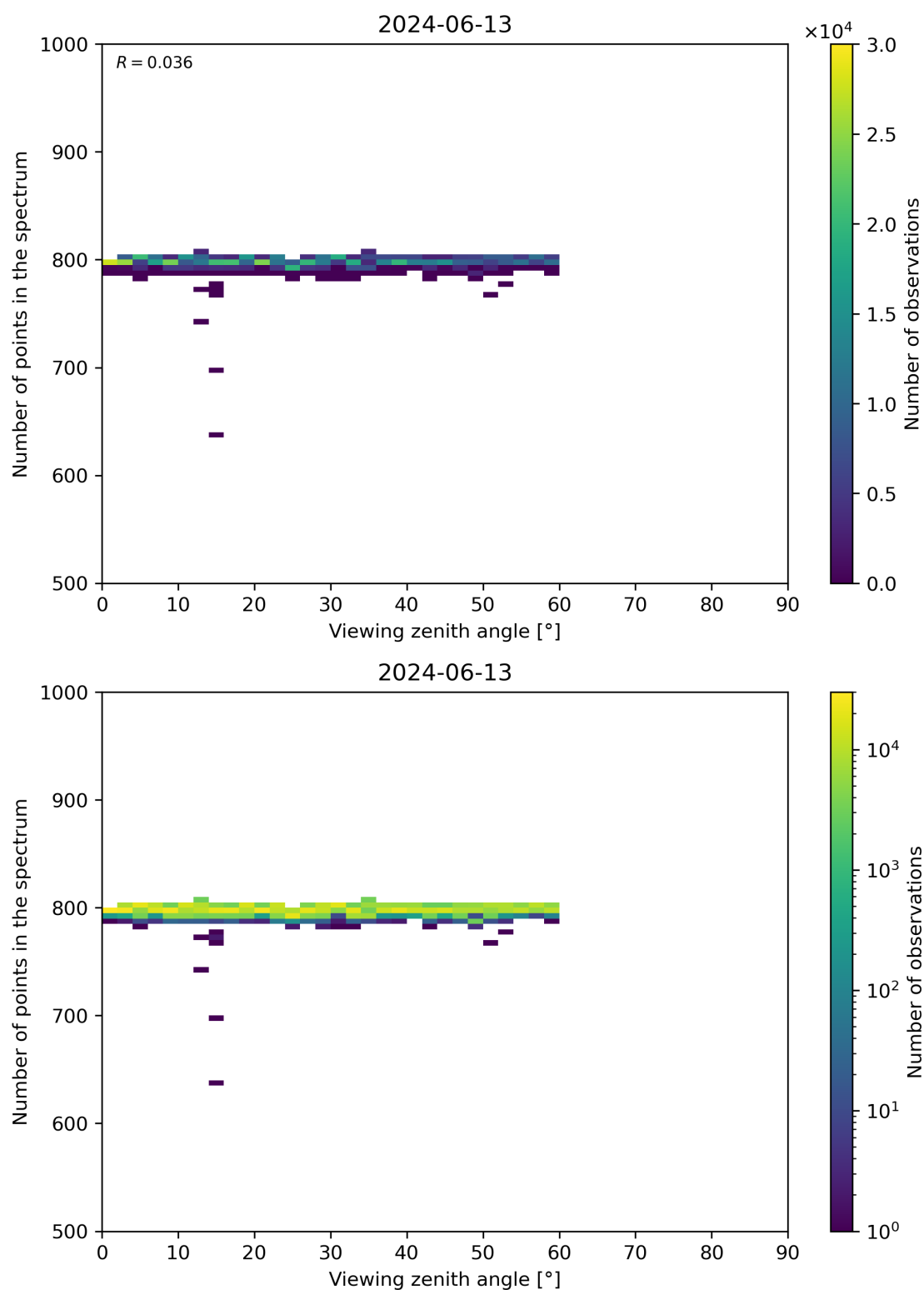
Figure 114: Scatter density plot of “Viewing zenith angle” against “Number of points in the spectrum” for 2024-06-13 to 2024-06-14.
