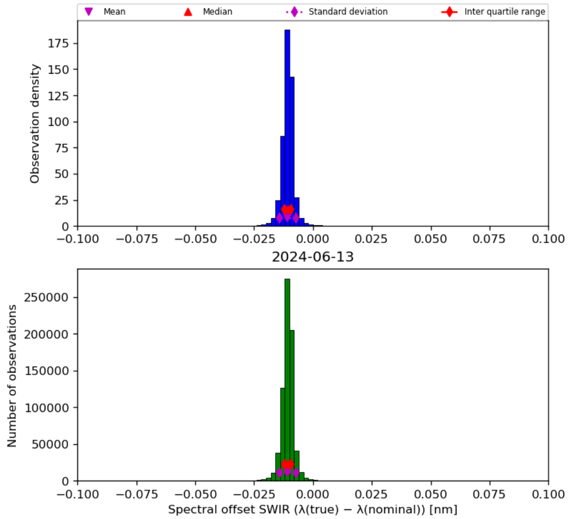
Figure 27: Histogram of “Spectral offset SWIR ( \lambda(\text{true}) - \lambda(\text{nominal}) )” for 2024-06-13 to 2024-06-14
