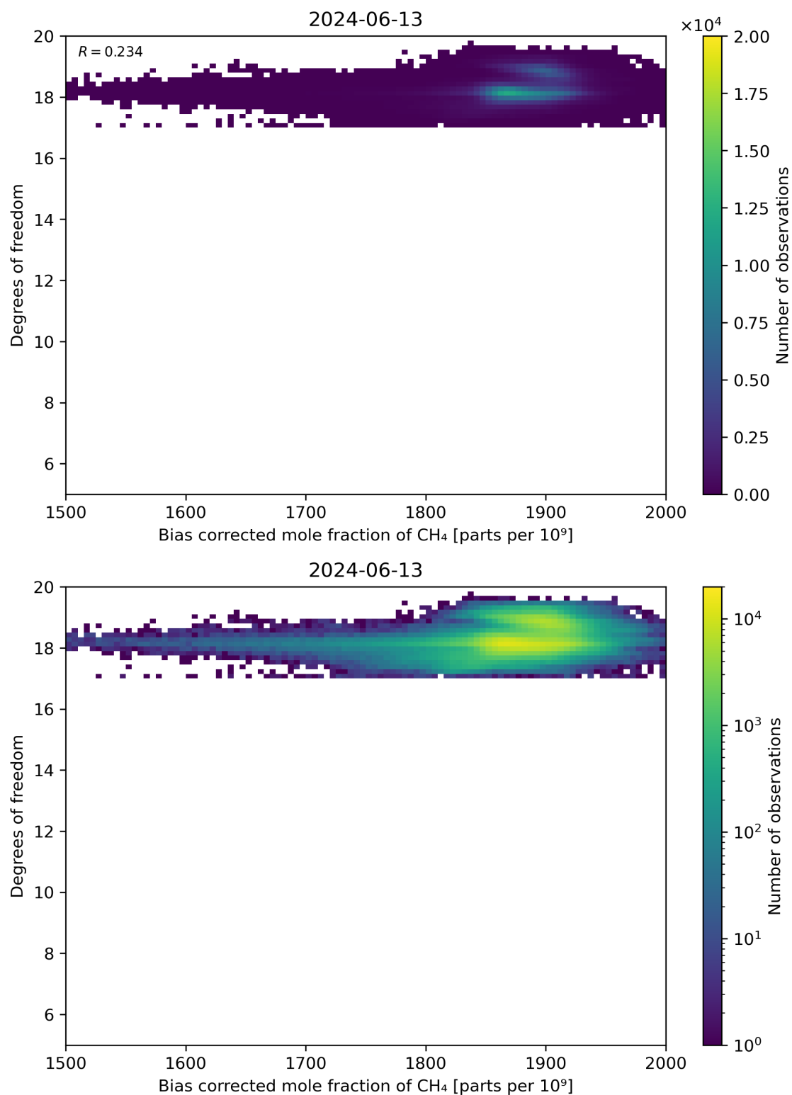
Figure 65: Scatter density plot of “Bias corrected mole fraction of CH 4 ” against “Degrees of freedom” for 2024-06-13 to 2024-06-14.
