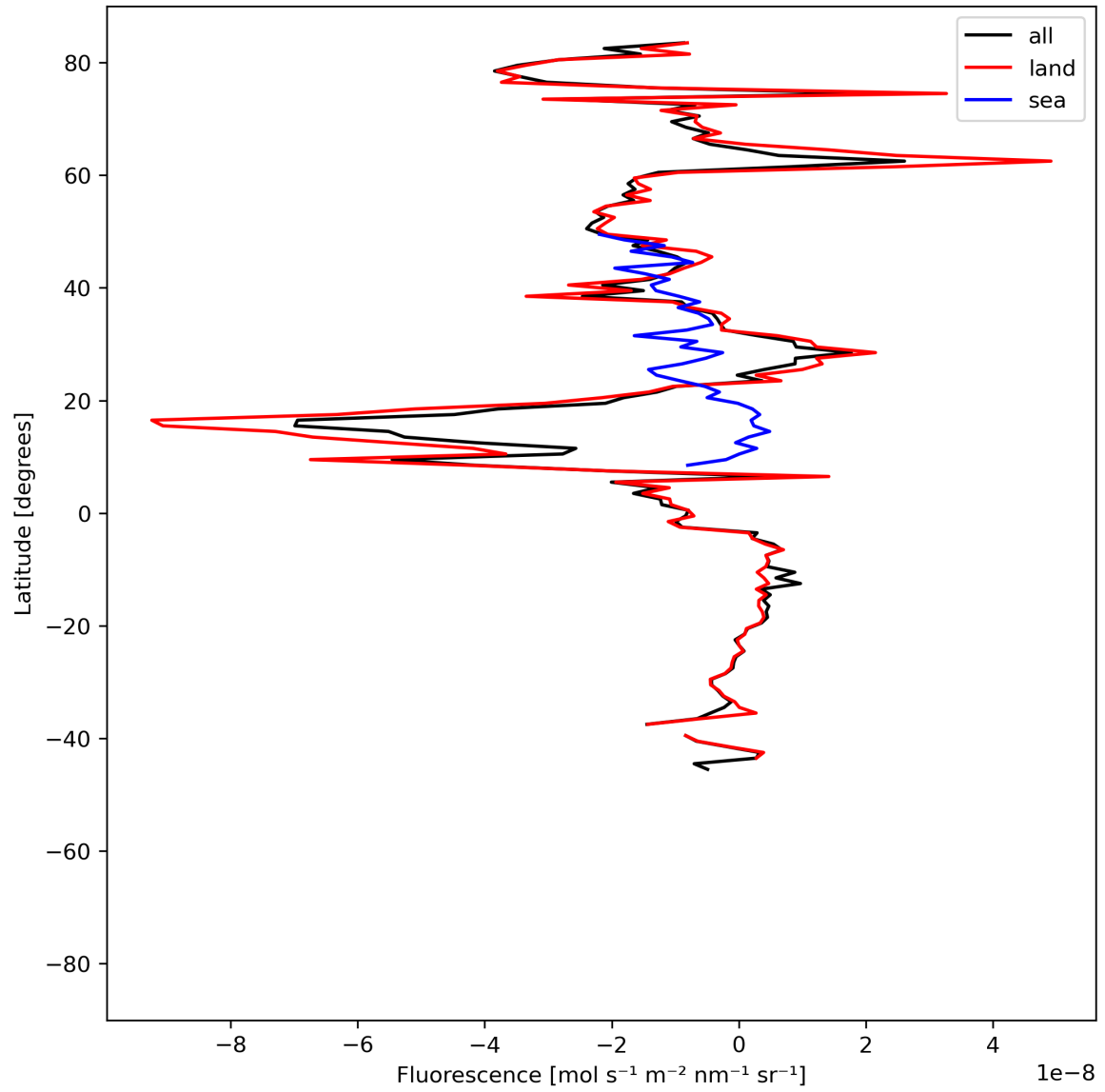
Figure 21: Zonal average of “Fluorescence” for 2024-06-13 to 2024-06-14.
