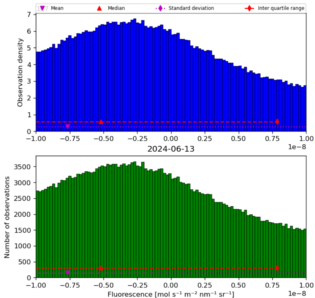
Figure 32: Histogram of “Fluorescence” for 2024-06-13 to 2024-06-14
