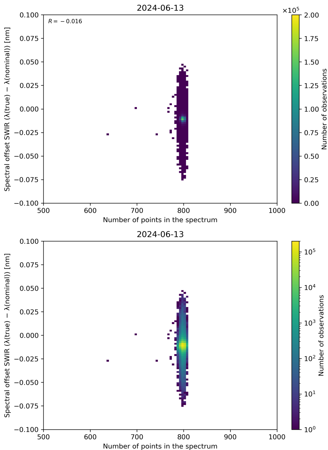
Figure 93: Scatter density plot of “Number of points in the spectrum” against “Spectral offset SWIR ( \lambda(\text{true}) - \lambda(\text{nominal}) )” for 2024-06-13 to 2024-06-14.
