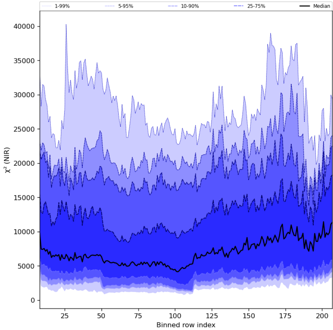
Figure 40: Along track statistics of " \chi^2 (NIR)" for 2024-06-13 to 2024-06-14
