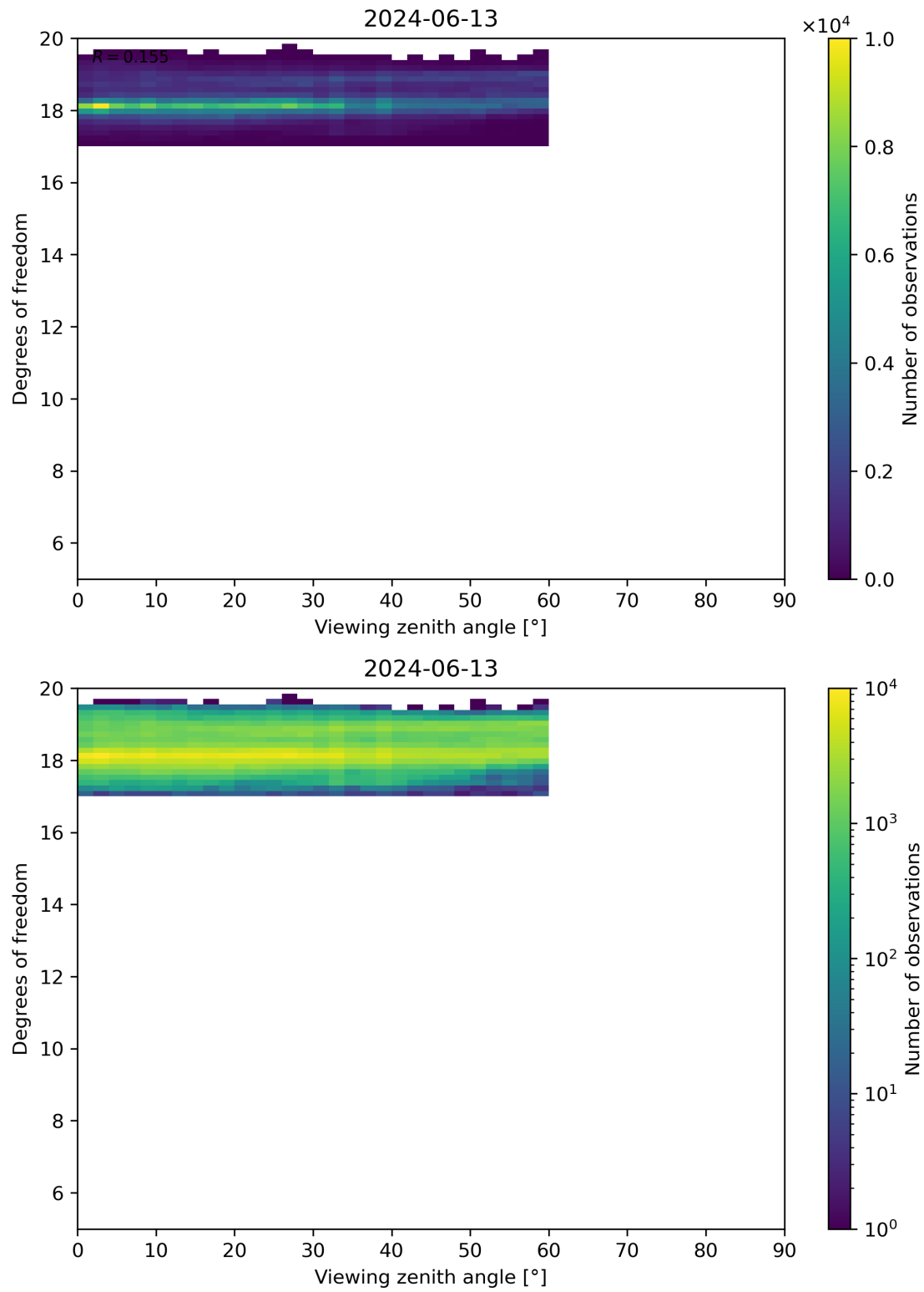
Figure 107: Scatter density plot of “Viewing zenith angle” against “Degrees of freedom” for 2024-06-13 to 2024-06-14.
