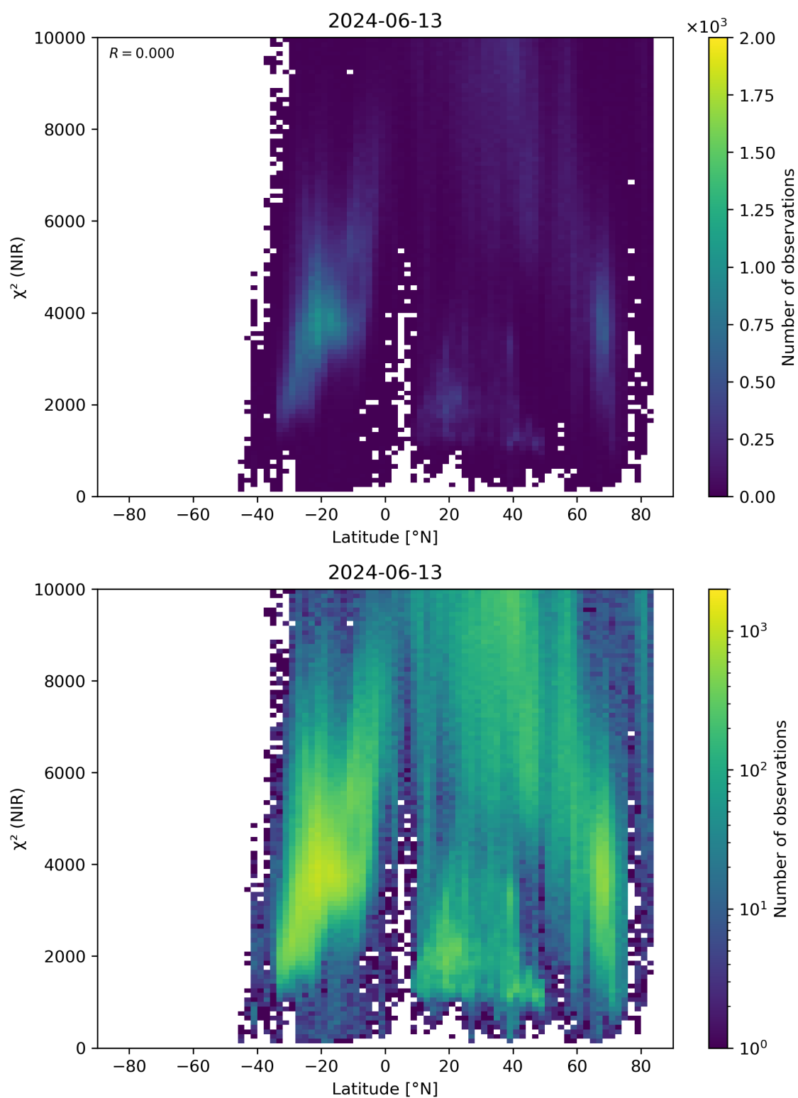
Figure 53: Scatter density plot of “Latitude” against “ \chi^2 (NIR)” for 2024-06-13 to 2024-06-14.
