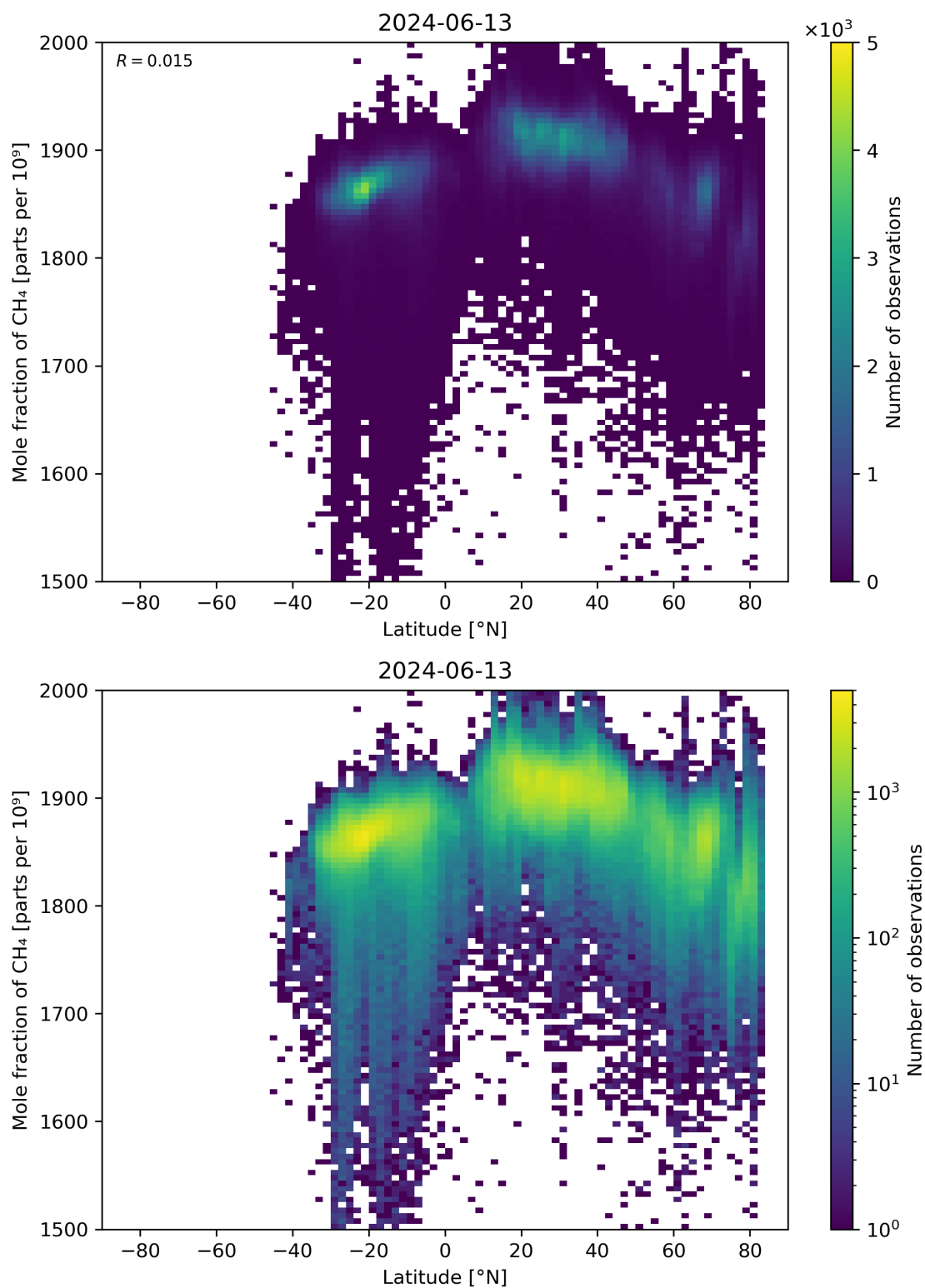
Figure 57: Scatter density plot of “Latitude” against “Mole fraction of CH 4 ” for 2024-06-13 to 2024-06-14.
