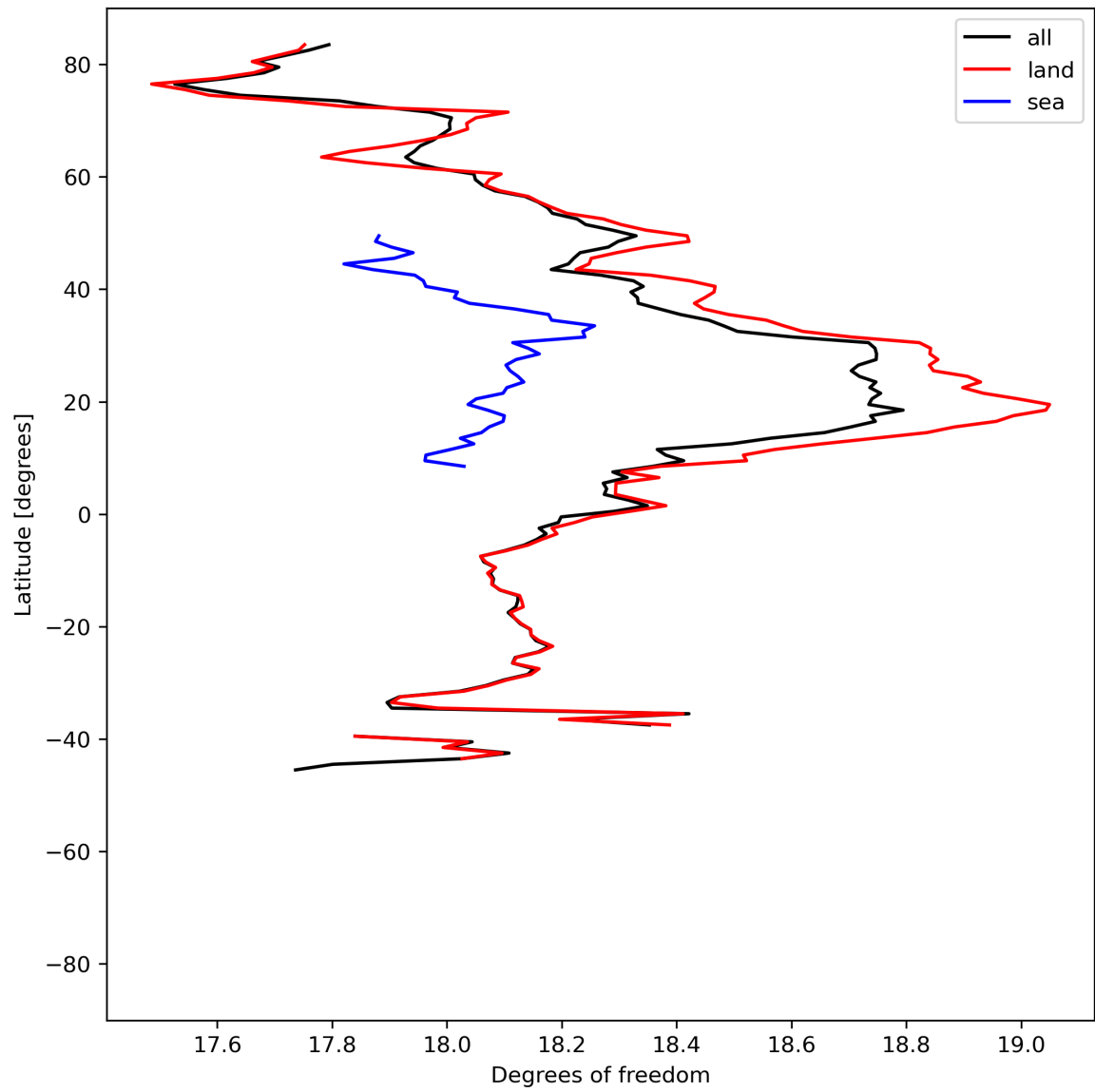
Figure 19: Zonal average of “Degrees of freedom” for 2024-06-13 to 2024-06-14.
