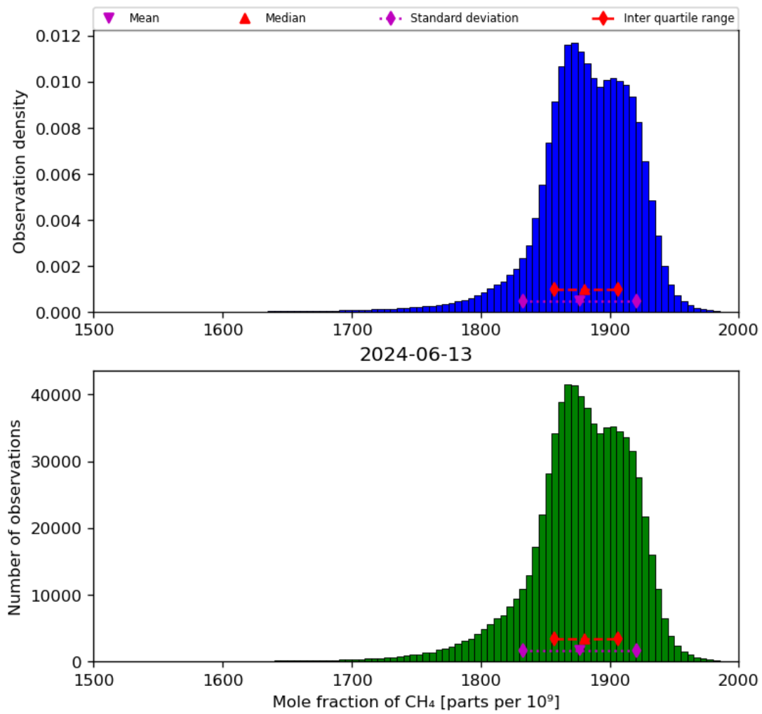
Figure 23: Histogram of “Mole fraction of CH 4 ” for 2024-06-13 to 2024-06-14
