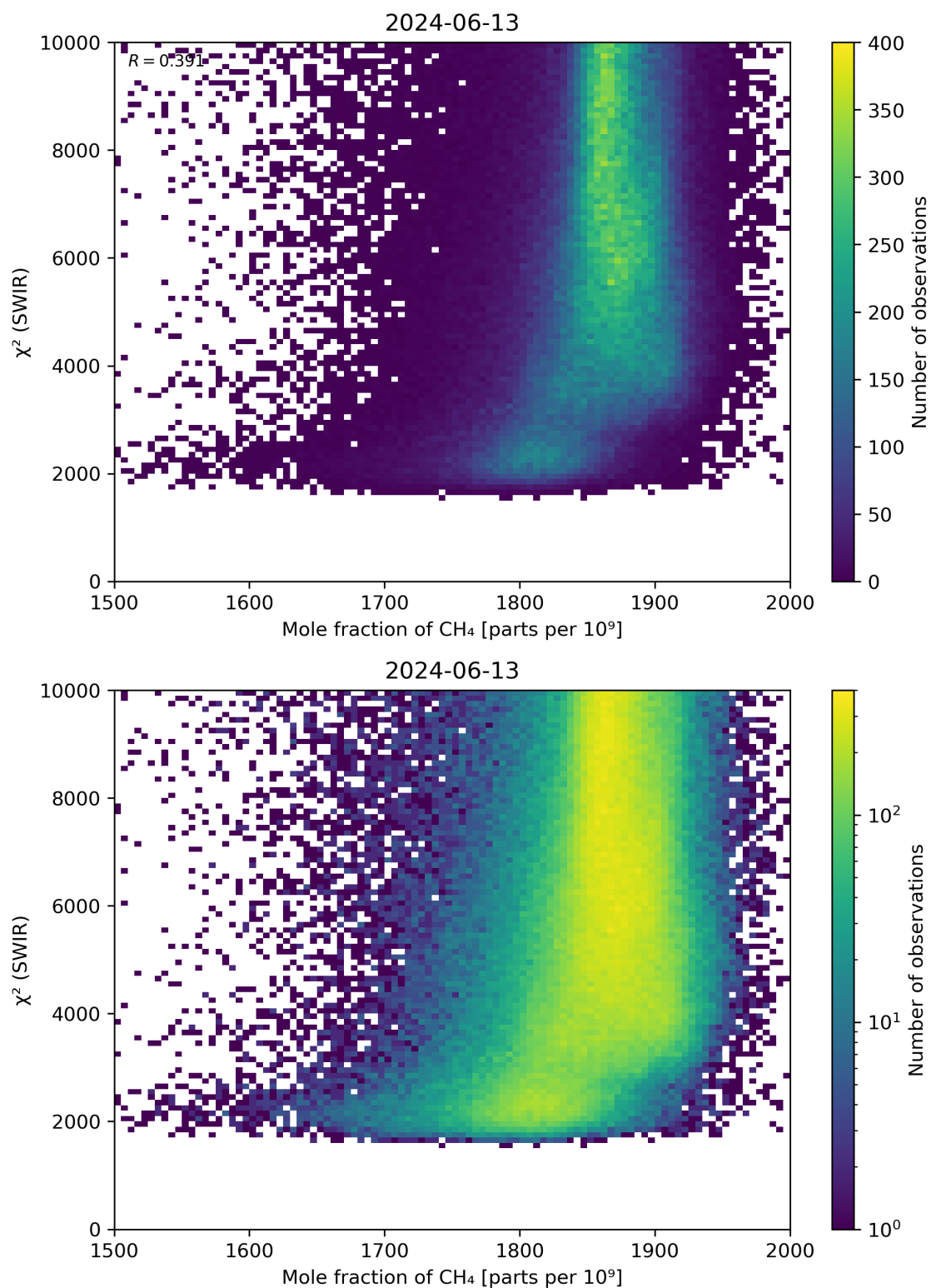
Figure 71: Scatter density plot of “Mole fraction of CH 4 ” against “ \chi^2 (SWIR)” for 2024-06-13 to 2024-06-14.
