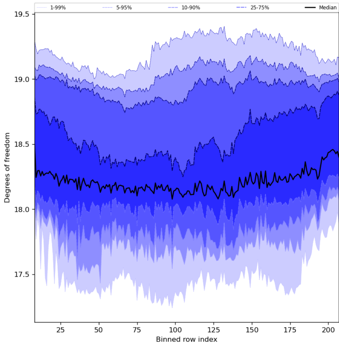
Figure 41: Along track statistics of “Degrees of freedom” for 2024-06-13 to 2024-06-14
