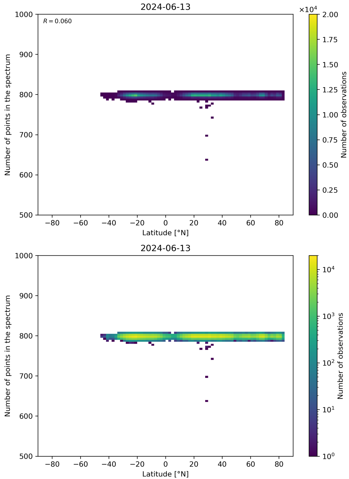
Figure 61: Scatter density plot of “Latitude” against “Number of points in the spectrum” for 2024-06-13 to 2024-06-14.
