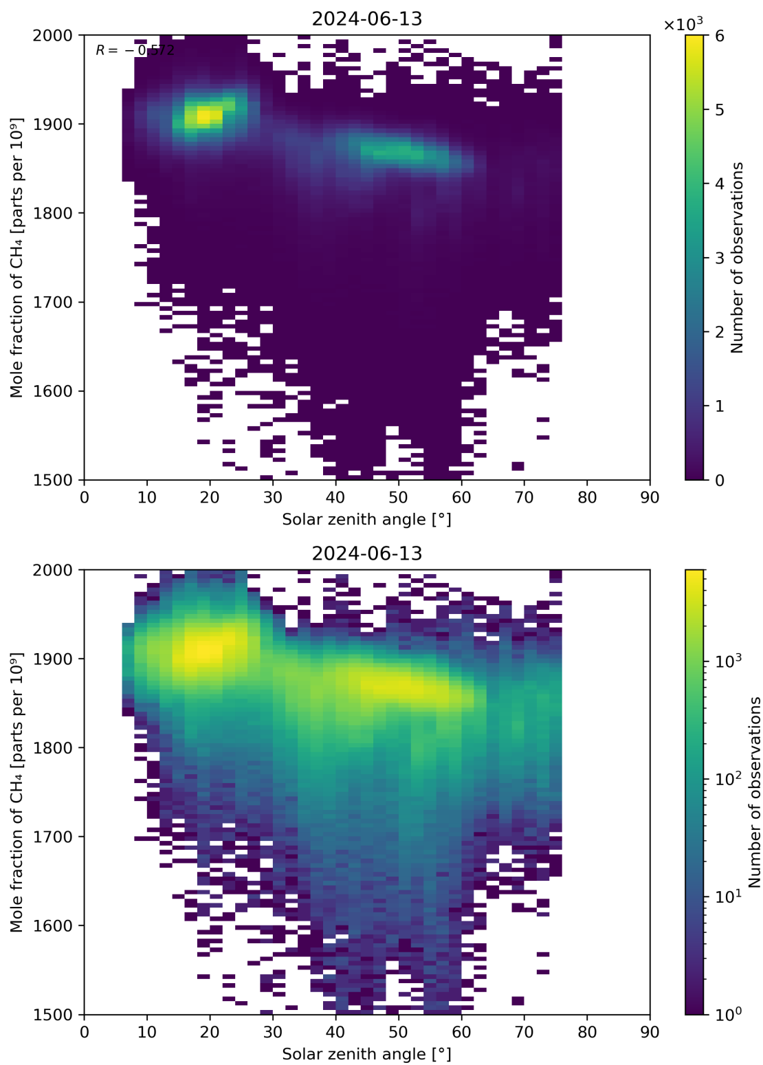
Figure 99: Scatter density plot of “Solar zenith angle” against “Mole fraction of CH 4 ” for 2024-06-13 to 2024-06-14.
