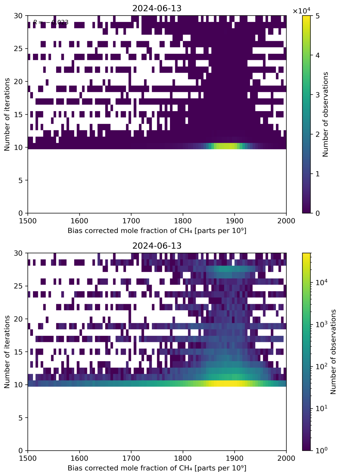
Figure 67: Scatter density plot of “Bias corrected mole fraction of \text{CH}_4 ” against “Number of iterations” for 2024-06-13 to 2024-06-14.
