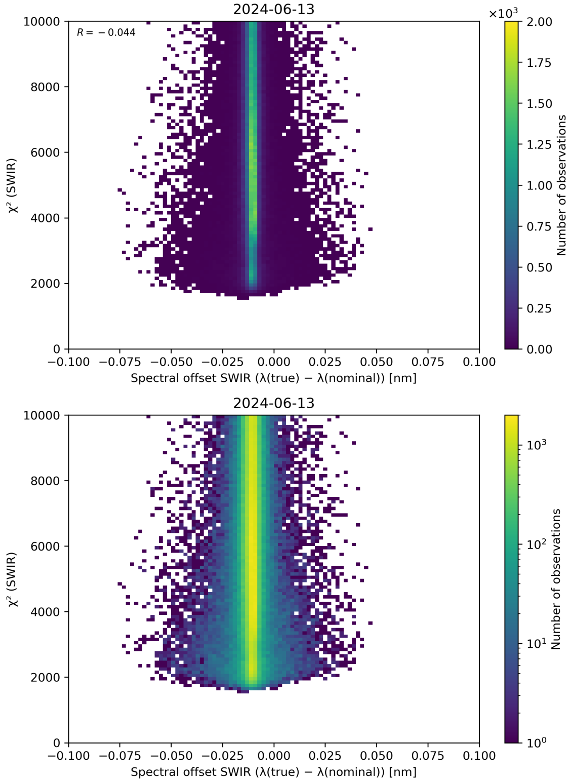
Figure 118: Scatter density plot of “Spectral offset SWIR ( \lambda(\text{true}) - \lambda(\text{nominal}) )” against “ \chi^2 (SWIR)” for 2024-06-13 to 2024-06-14.
