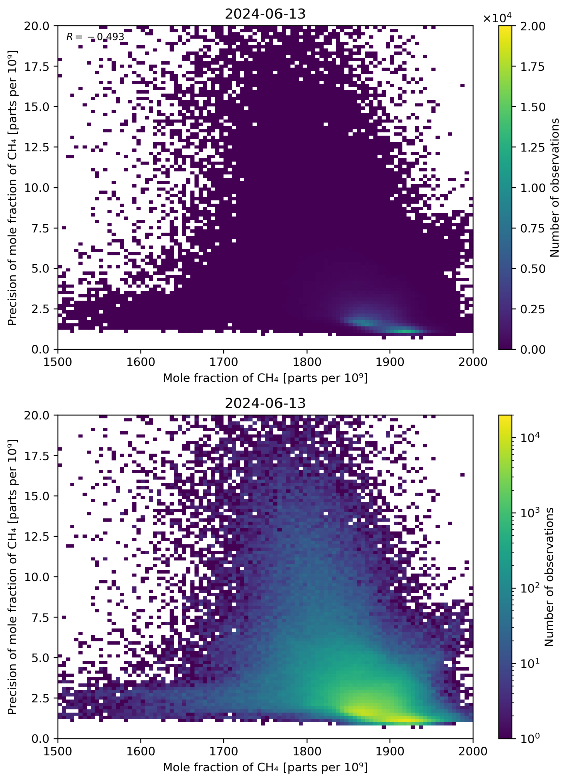
Figure 75: Scatter density plot of “Mole fraction of CH 4 ” against “Precision of mole fraction of CH 4 ” for 2024-06-13 to 2024-06-14.
