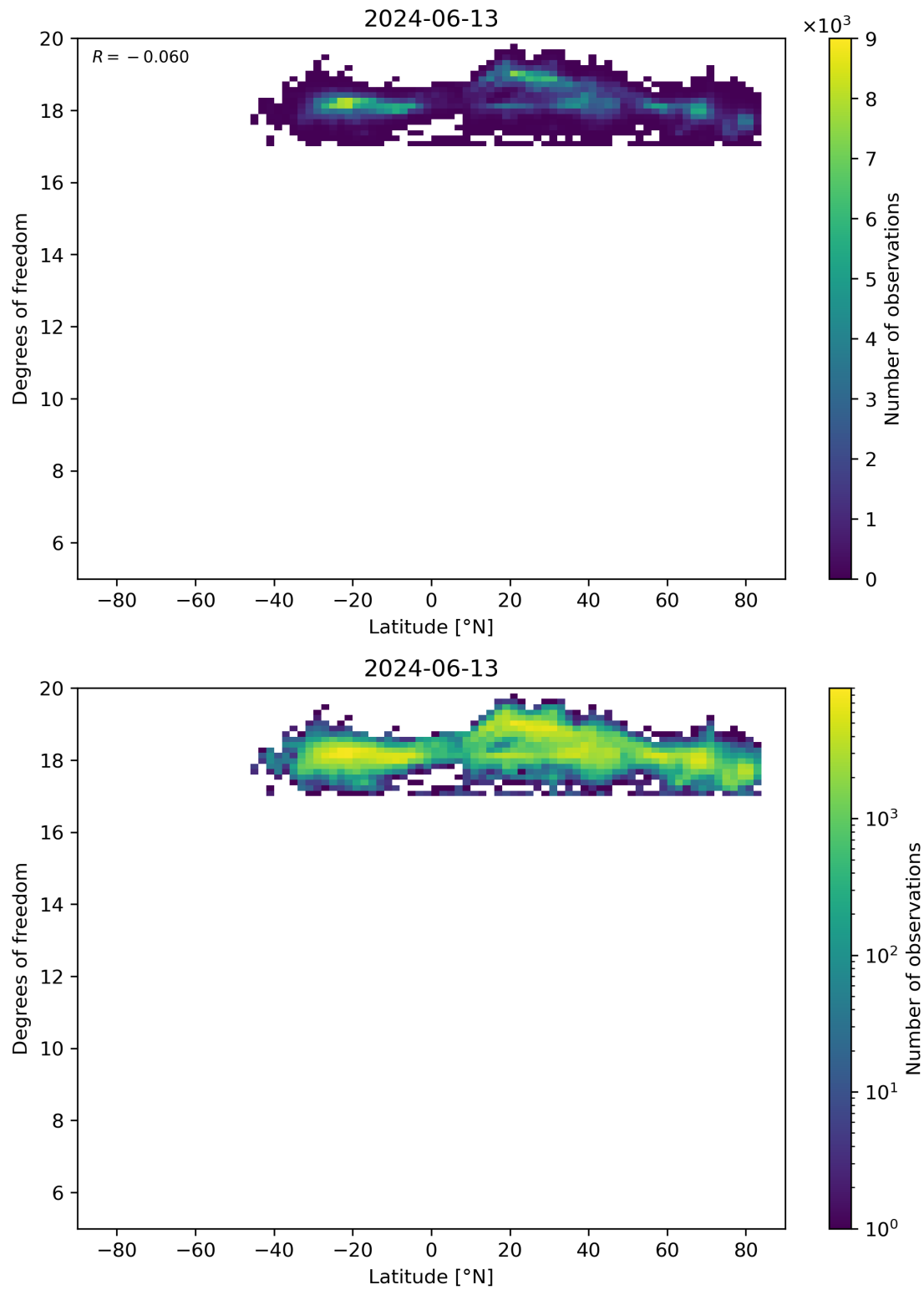
Figure 55: Scatter density plot of “Latitude” against “Degrees of freedom” for 2024-06-13 to 2024-06-14.
