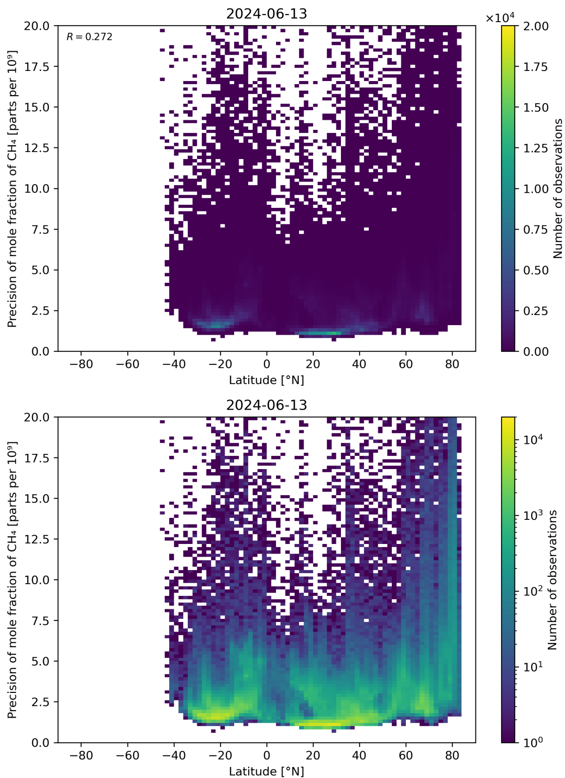
Figure 59: Scatter density plot of “Latitude” against “Precision of mole fraction of \text{CH}_4 ” for 2024-06-13 to 2024-06-14.
