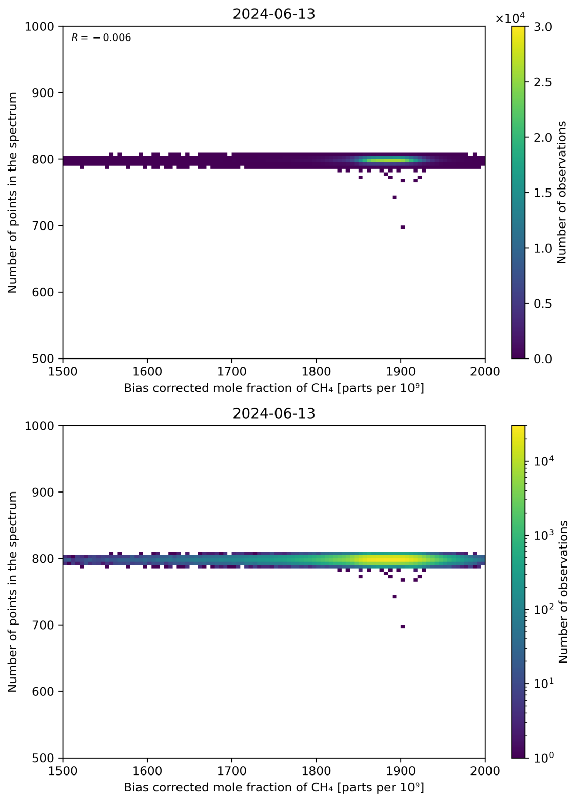
Figure 68: Scatter density plot of “Bias corrected mole fraction of CH 4 ” against “Number of points in the spectrum” for 2024-06-13 to 2024-06-14.
