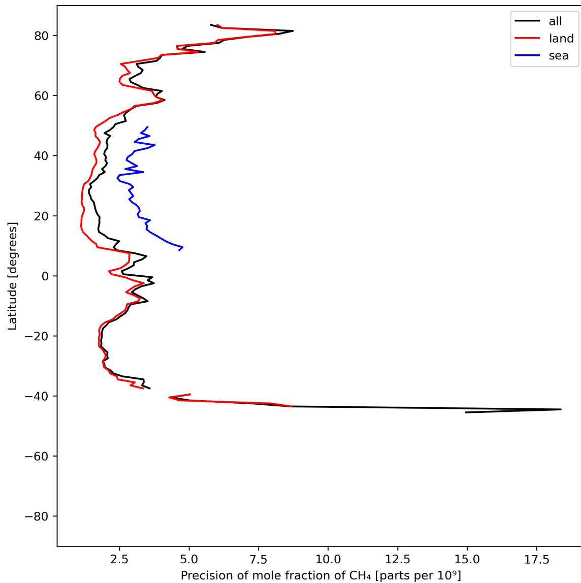
Figure 13: Zonal average of “Precision of mole fraction of \text{CH}_4 ” for 2024-06-13 to 2024-06-14.
