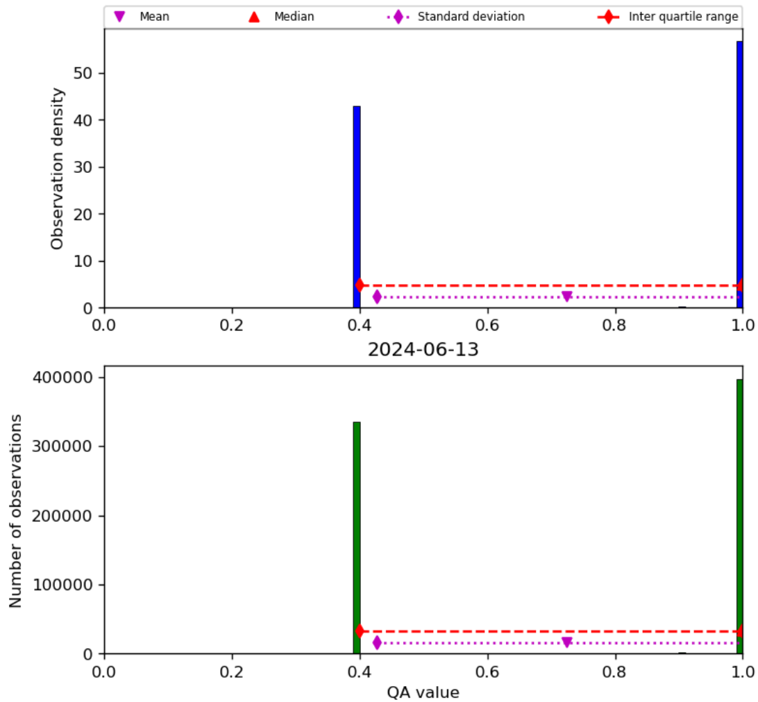
Figure 22: Histogram of “QA value” for 2024-06-13 to 2024-06-14
