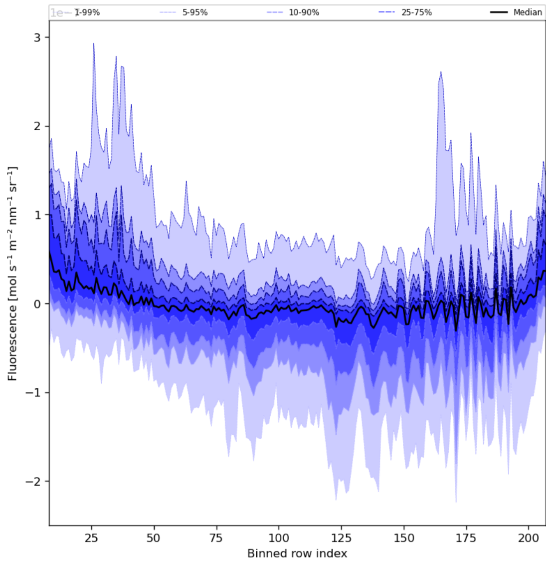
Figure 43: Along track statistics of “Fluorescence” for 2024-06-13 to 2024-06-14
