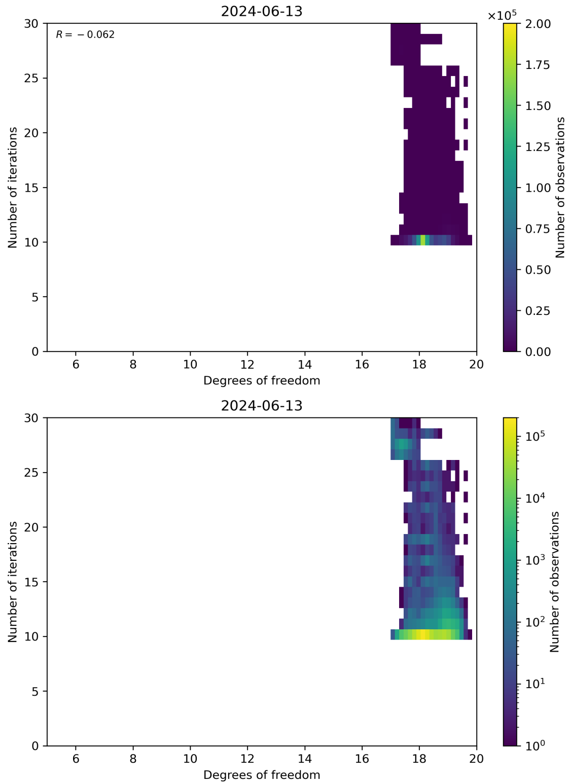
Figure 52: Scatter density plot of “Degrees of freedom” against “Number of iterations” for 2024-06-13 to 2024-06-14.
