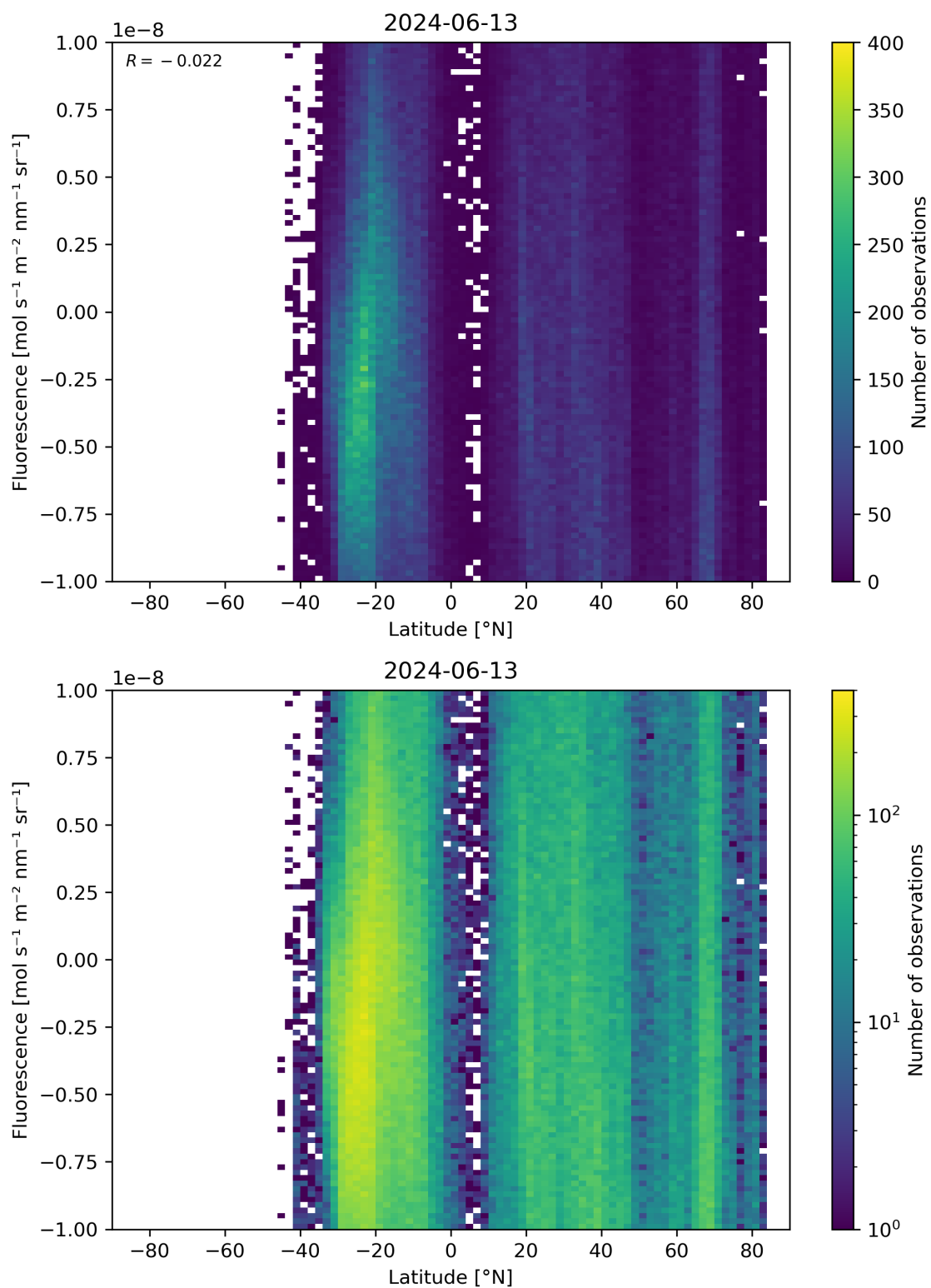
Figure 56: Scatter density plot of “Latitude” against “Fluorescence” for 2024-06-13 to 2024-06-14.
