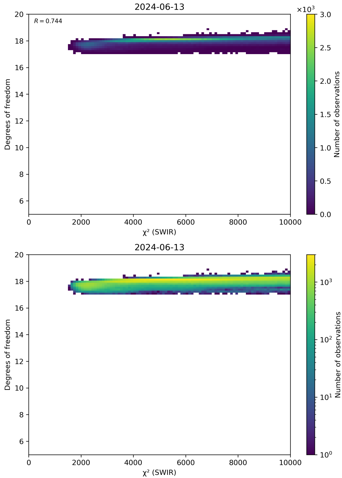
Figure 48: Scatter density plot of “ \chi^2 (SWIR)” against “Degrees of freedom” for 2024-06-13 to 2024-06-14.
