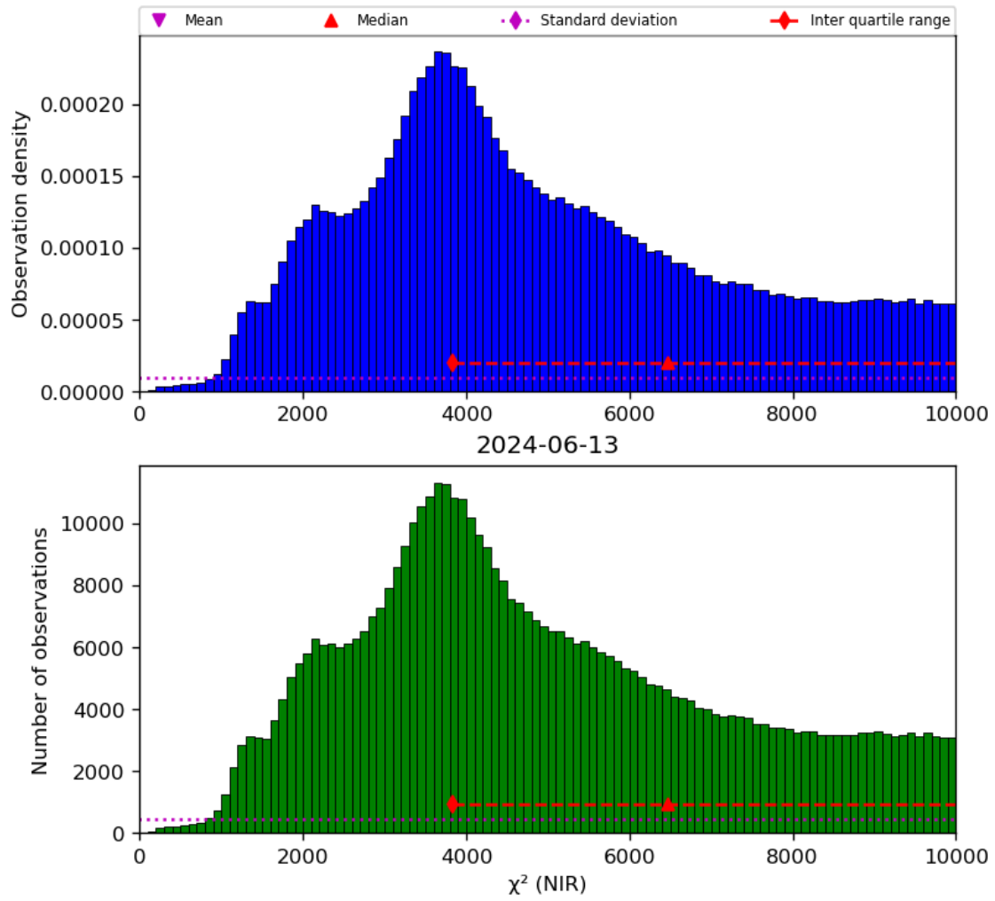
Figure 29: Histogram of “ \chi^2 (NIR)” for 2024-06-13 to 2024-06-14
