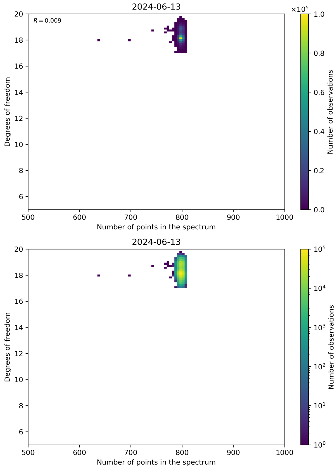
Figure 90: Scatter density plot of “Number of points in the spectrum” against “Degrees of freedom” for 2024-06-13 to 2024-06-14.
