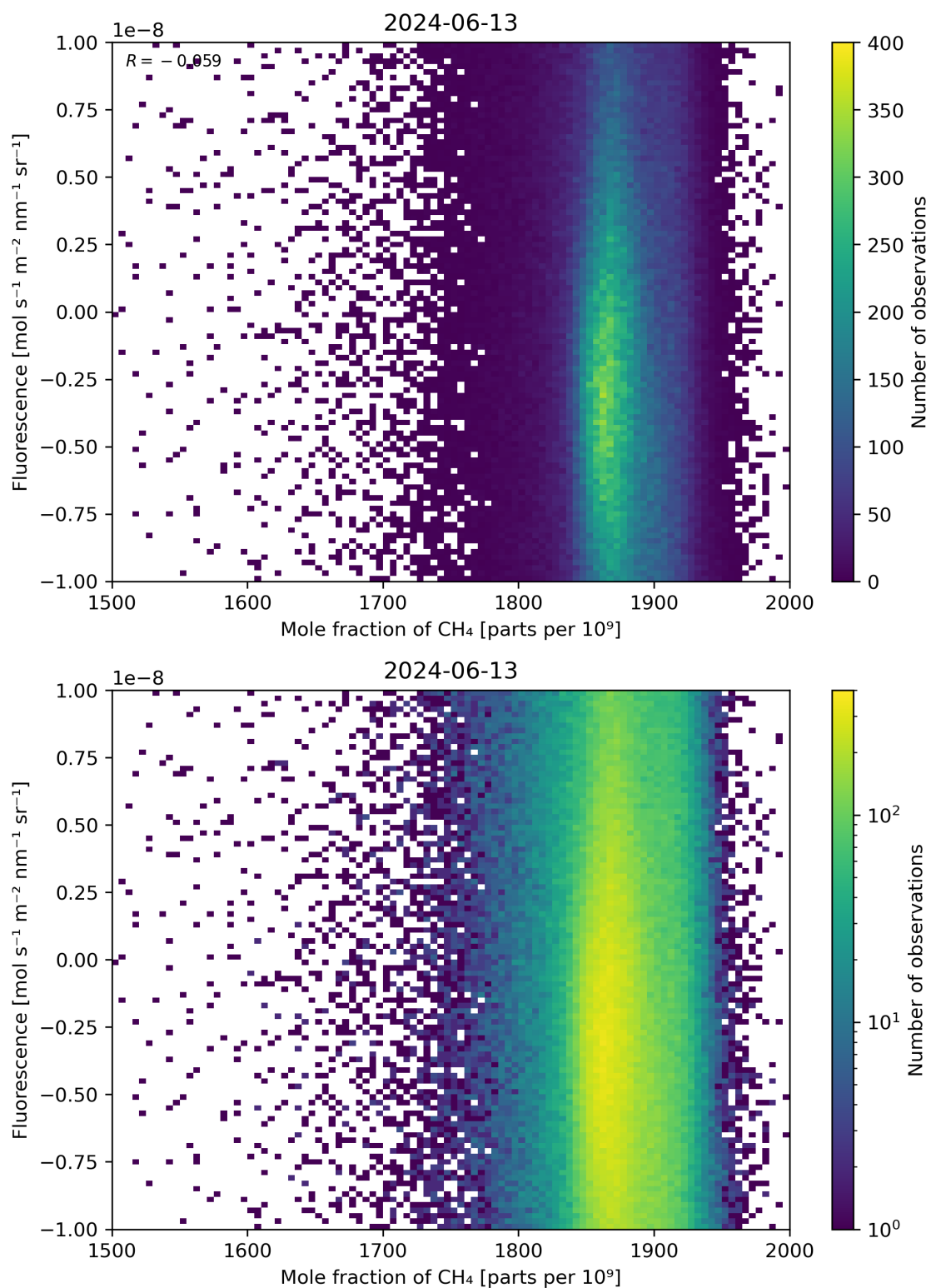
Figure 73: Scatter density plot of “Mole fraction of \text{CH}_4 ” against “Fluorescence” for 2024-06-13 to 2024-06-14.
