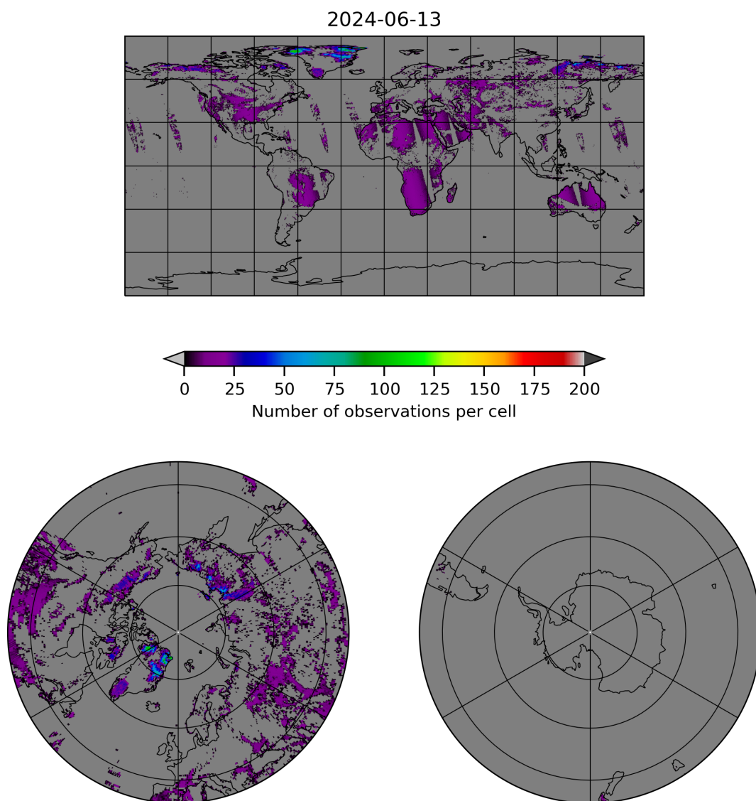
Figure 10: Map of the number of observations for 2024-06-13 to 2024-06-14
