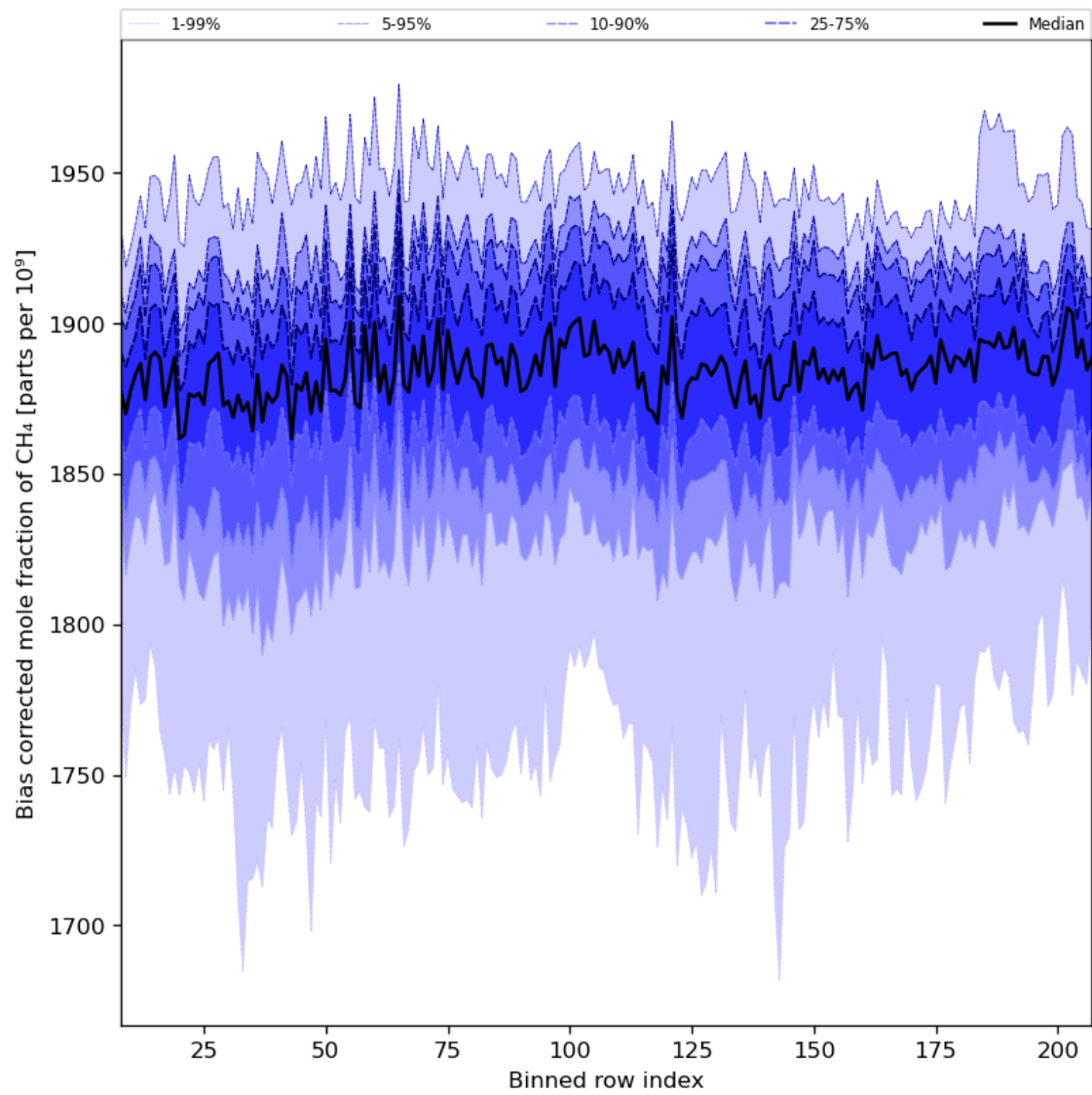
Figure 36: Along track statistics of “Bias corrected mole fraction of CH 4 ” for 2024-06-13 to 2024-06-14
