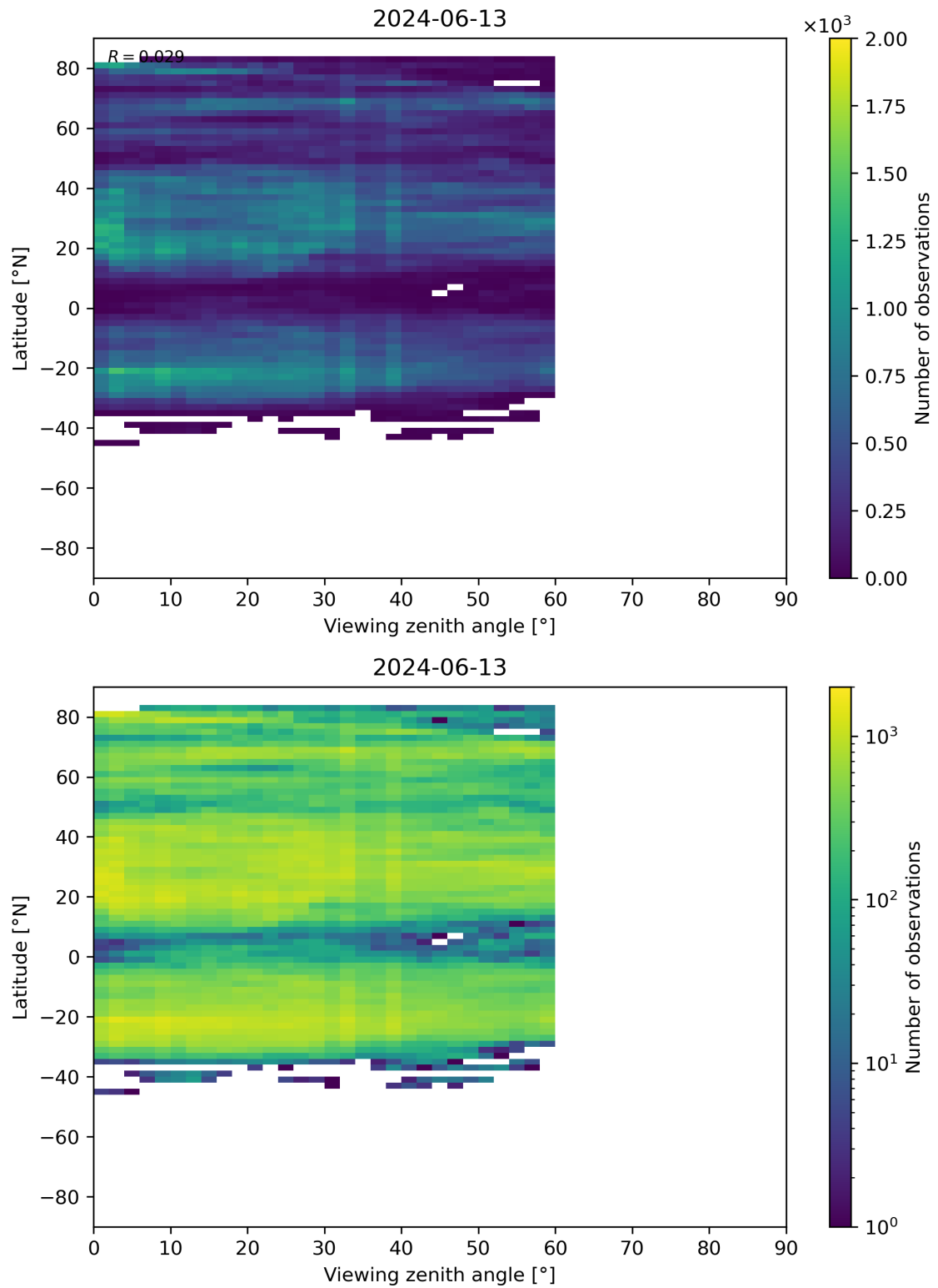
Figure 109: Scatter density plot of “Viewing zenith angle” against “Latitude” for 2024-06-13 to 2024-06-14.
