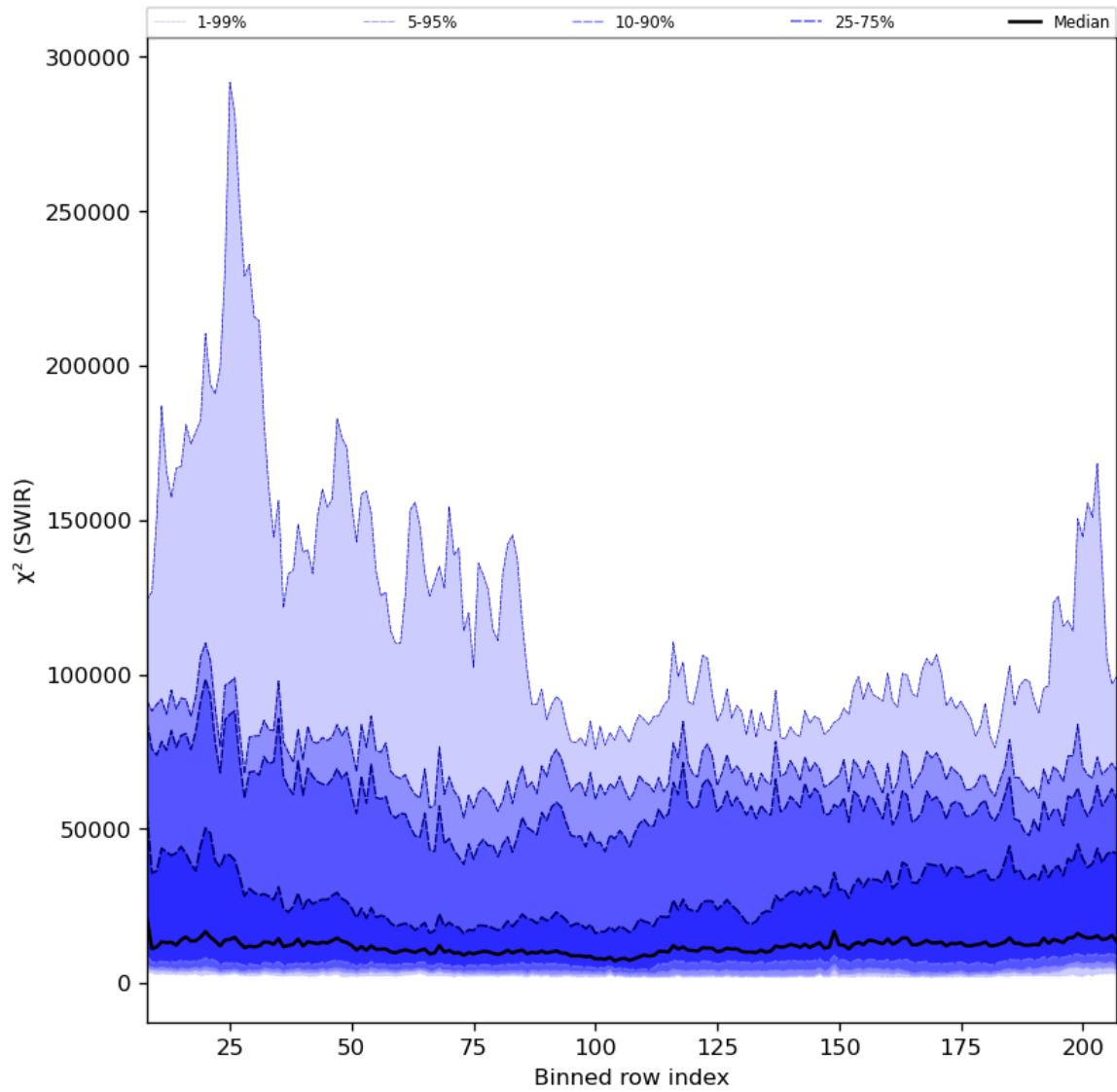
Figure 39: Along track statistics of " \chi^2 (SWIR)" for 2024-06-13 to 2024-06-14
