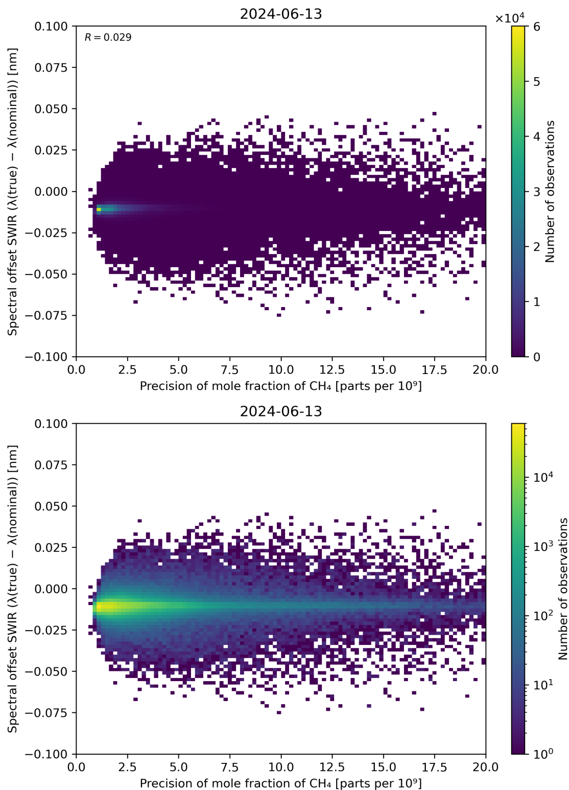
Figure 85: Scatter density plot of “Precision of mole fraction of CH 4 ” against “Spectral offset SWIR ( \lambda(\text{true}) - \lambda(\text{nominal}) )” for 2024-06-13 to 2024-06-14.
