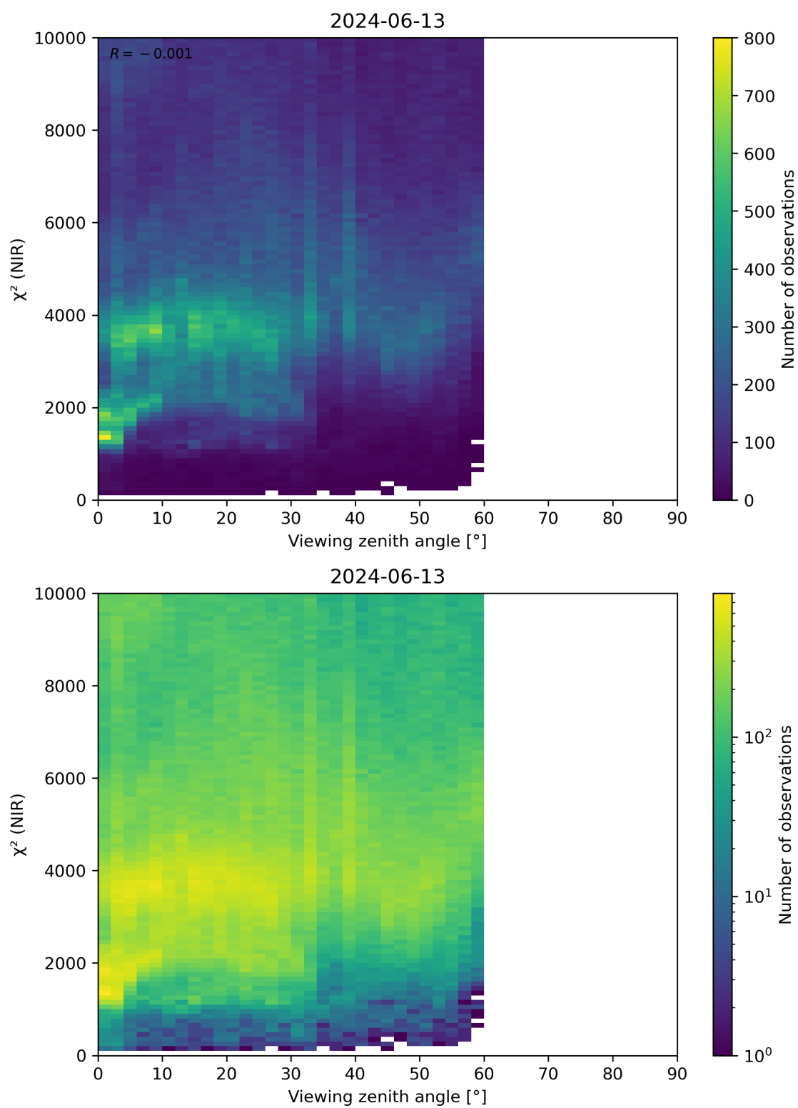
Figure 105: Scatter density plot of “Viewing zenith angle” against “ \chi^2 (NIR)” for 2024-06-13 to 2024-06-14.
