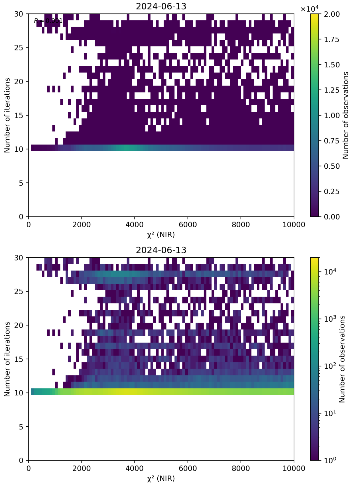
Figure 46: Scatter density plot of “ \chi^2 (NIR)” against “Number of iterations” for 2024-06-13 to 2024-06-14.
