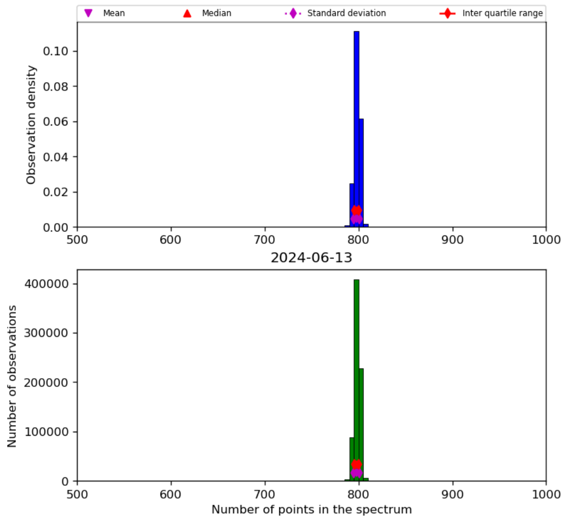
Figure 26: Histogram of “Number of points in the spectrum” for 2024-06-13 to 2024-06-14
