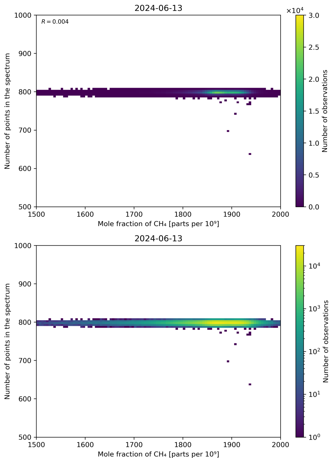
Figure 77: Scatter density plot of “Mole fraction of CH 4 ” against “Number of points in the spectrum” for 2024-06-13 to 2024-06-14.
