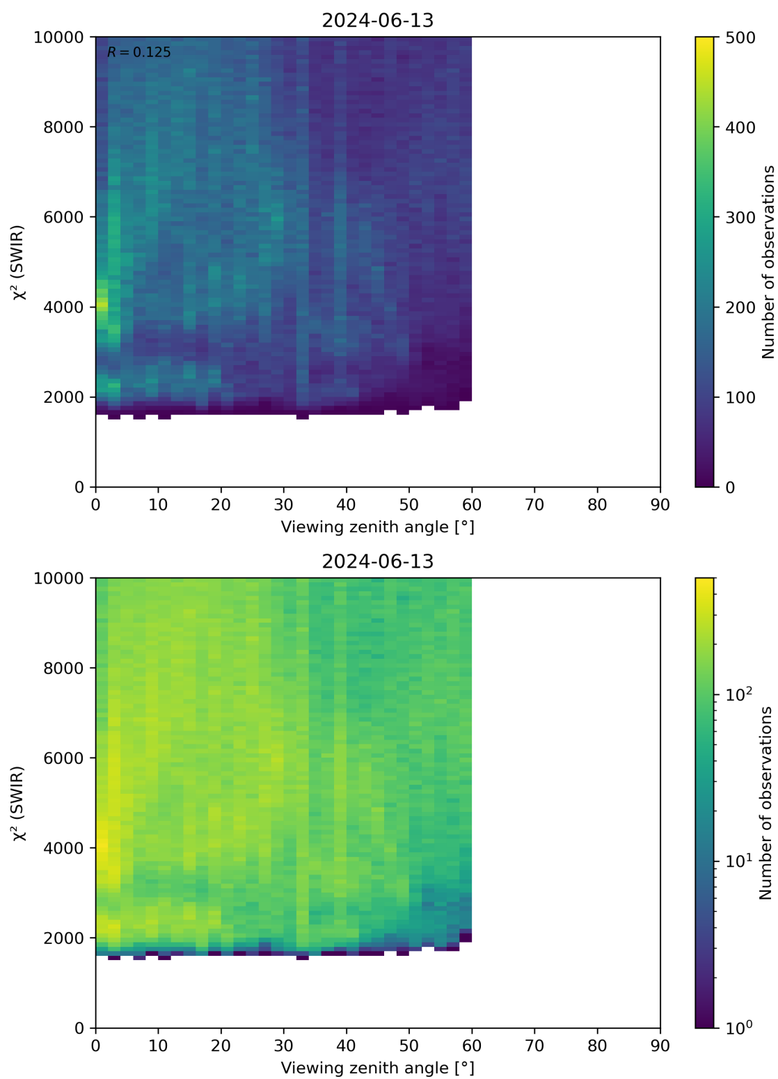
Figure 106: Scatter density plot of “Viewing zenith angle” against “ \chi^2 (SWIR)” for 2024-06-13 to 2024-06-14.
