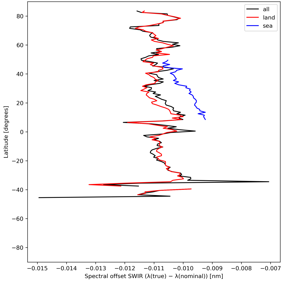
Figure 16: Zonal average of “Spectral offset SWIR ( \lambda(\text{true}) - \lambda(\text{nominal}) )” for 2024-06-13 to 2024-06-14.
