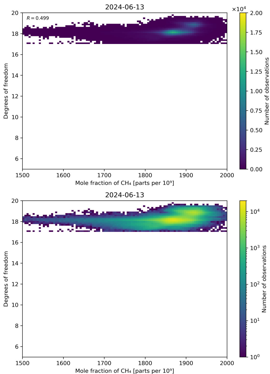
Figure 72: Scatter density plot of “Mole fraction of CH 4 ” against “Degrees of freedom” for 2024-06-13 to 2024-06-14.
