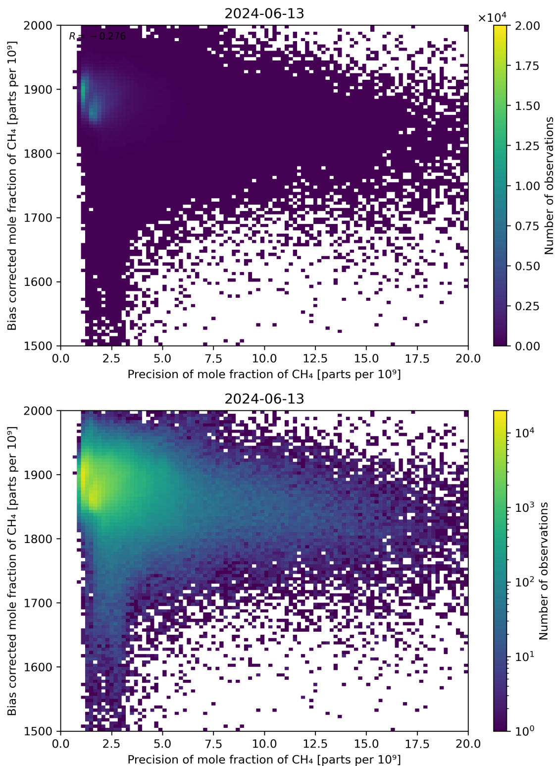
Figure 82: Scatter density plot of “Precision of mole fraction of CH 4 ” against “Bias corrected mole fraction of CH 4 ” for 2024-06-13 to 2024-06-14.
