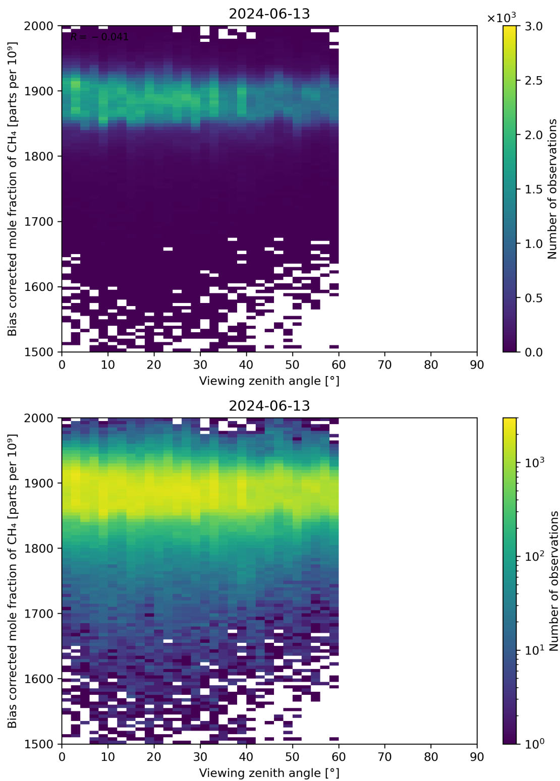
Figure 111: Scatter density plot of “Viewing zenith angle” against “Bias corrected mole fraction of CH 4 ” for 2024-06-13 to 2024-06-14.
