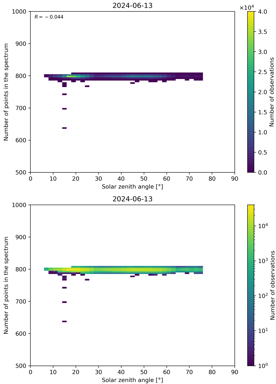
Figure 103: Scatter density plot of “Solar zenith angle” against “Number of points in the spectrum” for 2024-06-13 to 2024-06-14.
