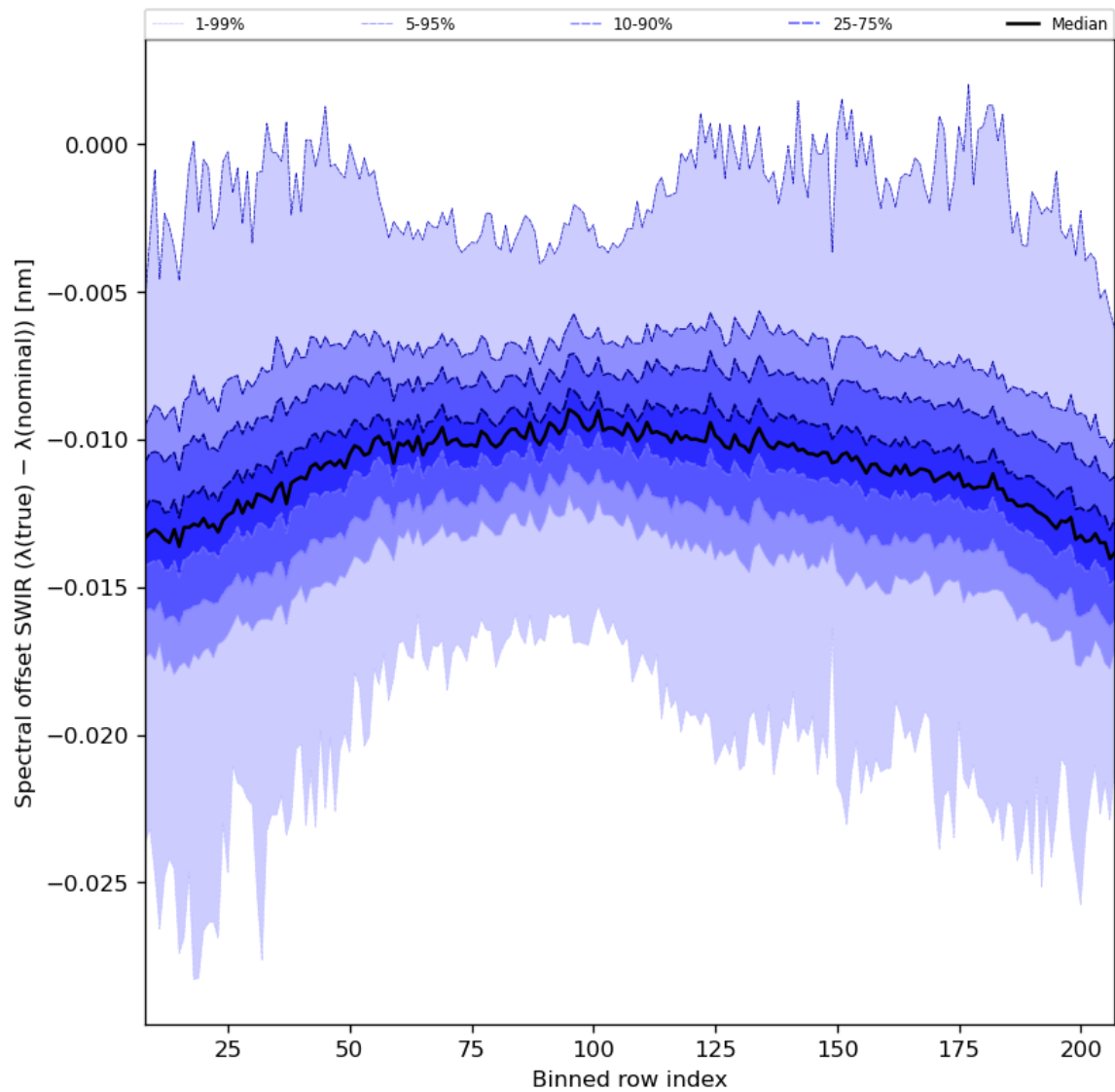
Figure 38: Along track statistics of “Spectral offset SWIR ( \lambda(\text{true}) - \lambda(\text{nominal}) )” for 2024-06-13 to 2024-06-14
