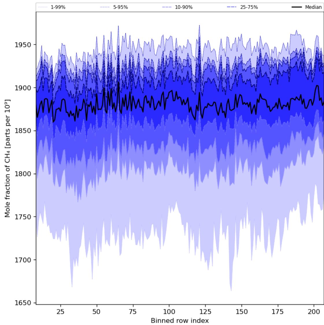
Figure 34: Along track statistics of “Mole fraction of CH 4 ” for 2024-06-13 to 2024-06-14
