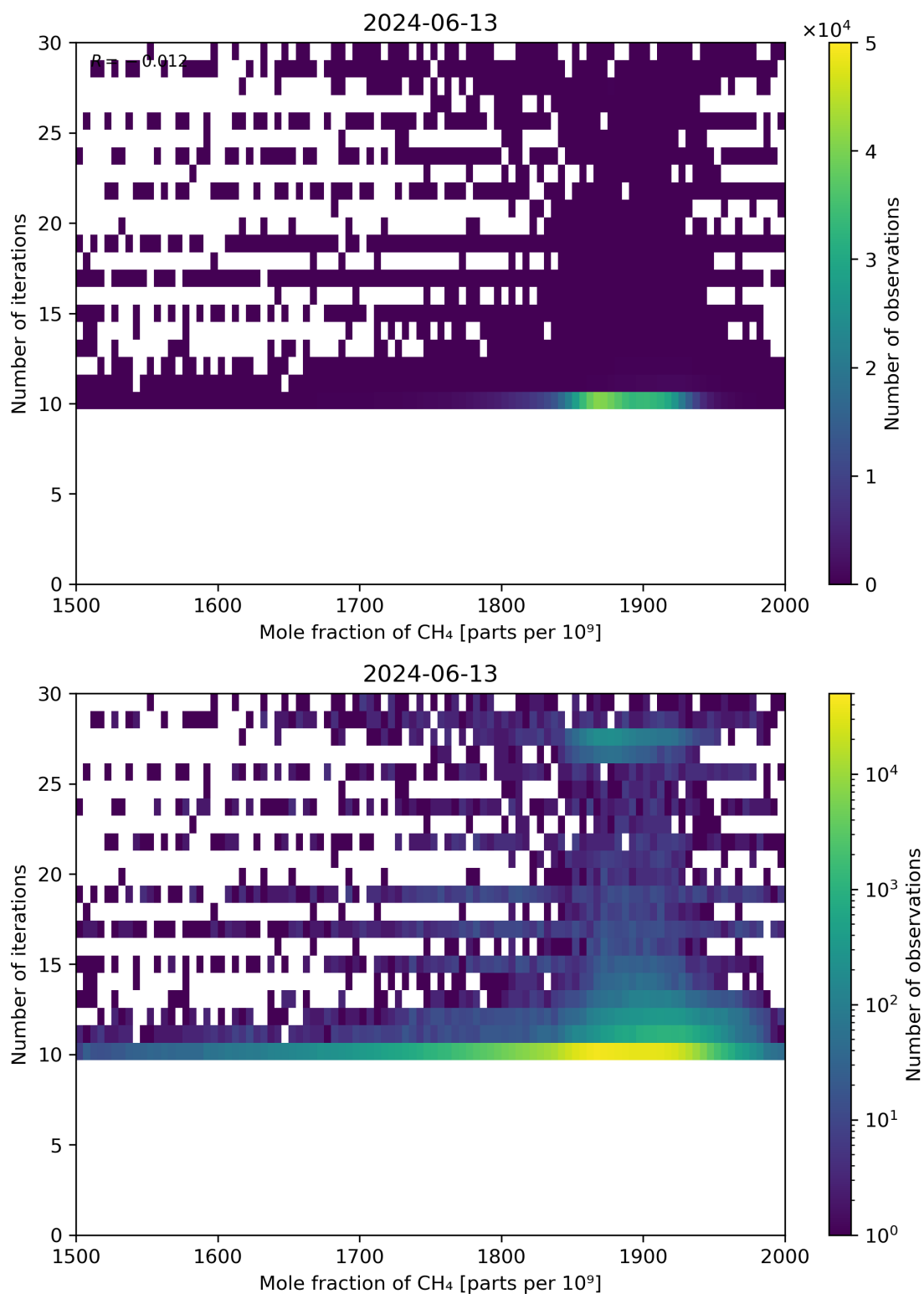
Figure 76: Scatter density plot of “Mole fraction of CH 4 ” against “Number of iterations” for 2024-06-13 to 2024-06-14.
