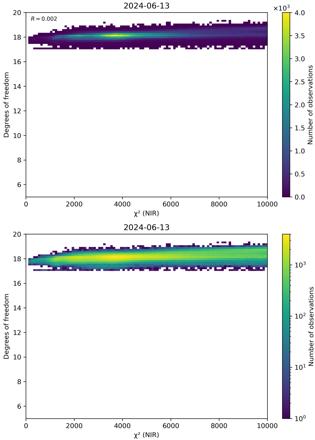
Figure 44: Scatter density plot of “ \chi^2 (NIR)” against “Degrees of freedom” for 2024-06-13 to 2024-06-14.
