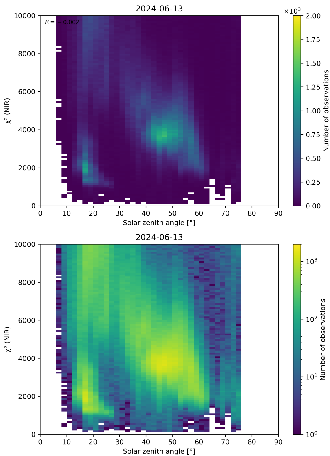
Figure 94: Scatter density plot of “Solar zenith angle” against “ \chi^2 (NIR)” for 2024-06-13 to 2024-06-14.
