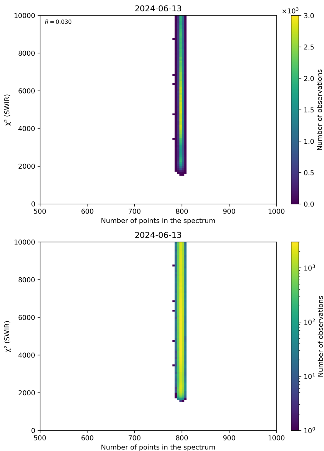
Figure 89: Scatter density plot of “Number of points in the spectrum” against “ \chi^2 (SWIR)” for 2024-06-13 to 2024-06-14.
