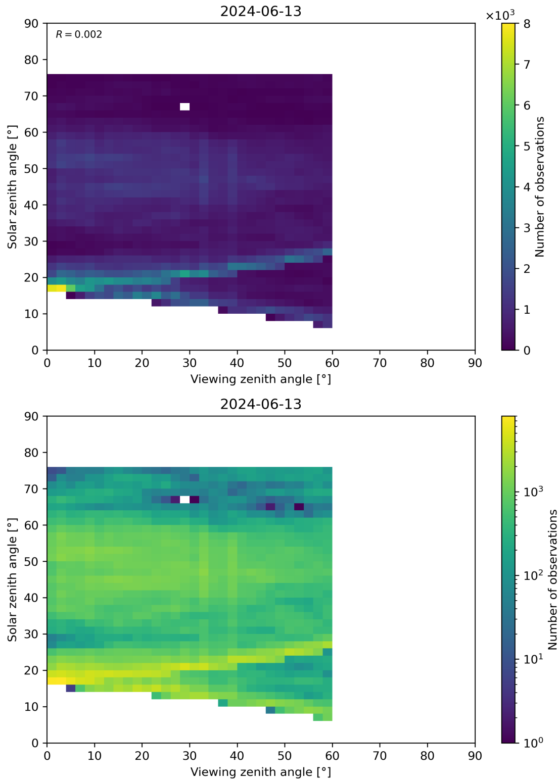
Figure 115: Scatter density plot of “Viewing zenith angle” against “Solar zenith angle” for 2024-06-13 to 2024-06-14.
