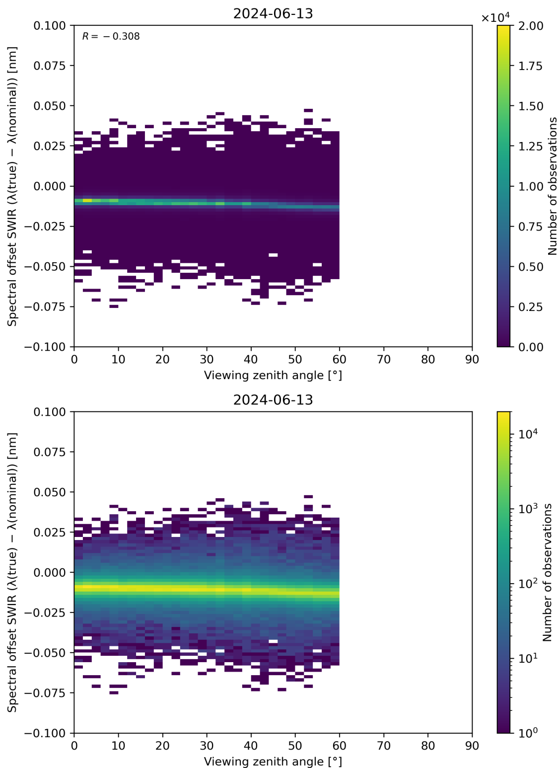
Figure 116: Scatter density plot of “Viewing zenith angle” against “Spectral offset SWIR ( \lambda(\text{true}) - \lambda(\text{nominal}) )” for 2024-06-13 to 2024-06-14.
