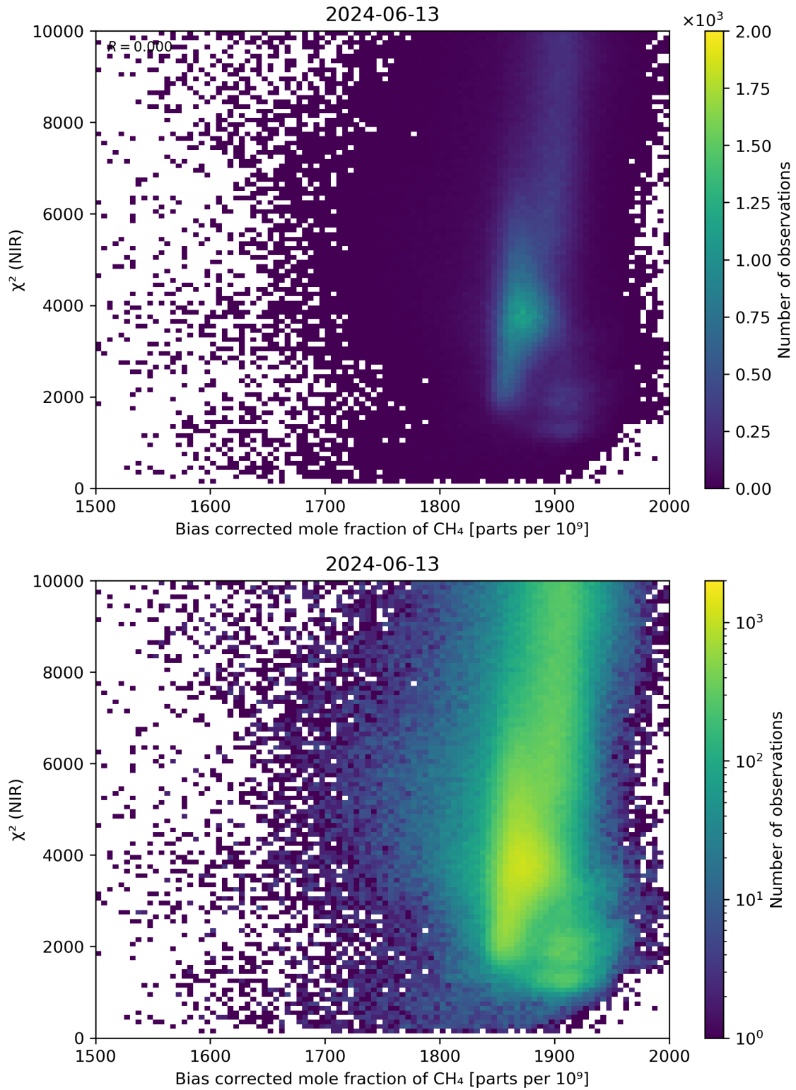
Figure 63: Scatter density plot of “Bias corrected mole fraction of CH 4 ” against “ \chi^2 (NIR)” for 2024-06-13 to 2024-06-14.
