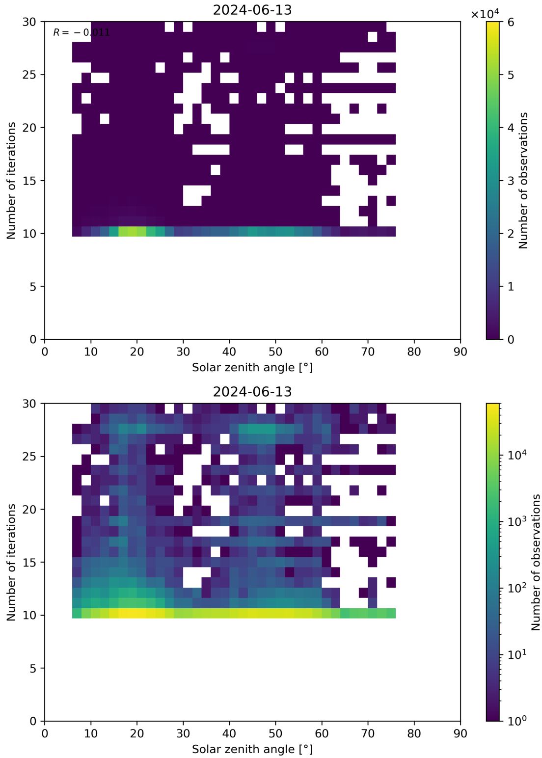
Figure 102: Scatter density plot of “Solar zenith angle” against “Number of iterations” for 2024-06-13 to 2024-06-14.
