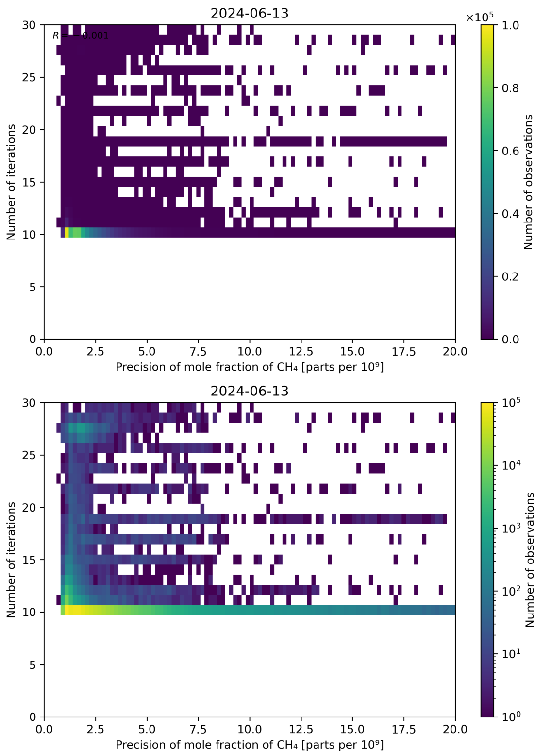
Figure 83: Scatter density plot of “Precision of mole fraction of CH 4 ” against “Number of iterations” for 2024-06-13 to 2024-06-14.
