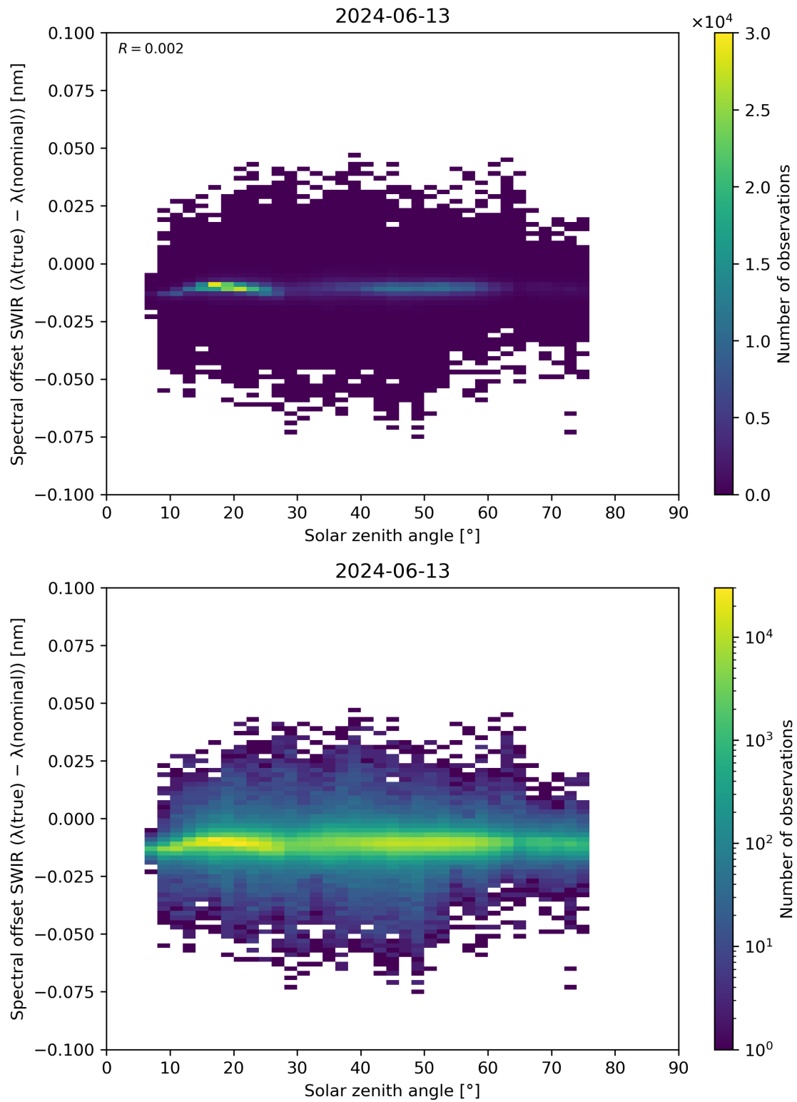
Figure 104: Scatter density plot of “Solar zenith angle” against “Spectral offset SWIR ( \lambda(\text{true}) - \lambda(\text{nominal}) )” for 2024-06-13 to 2024-06-14.
