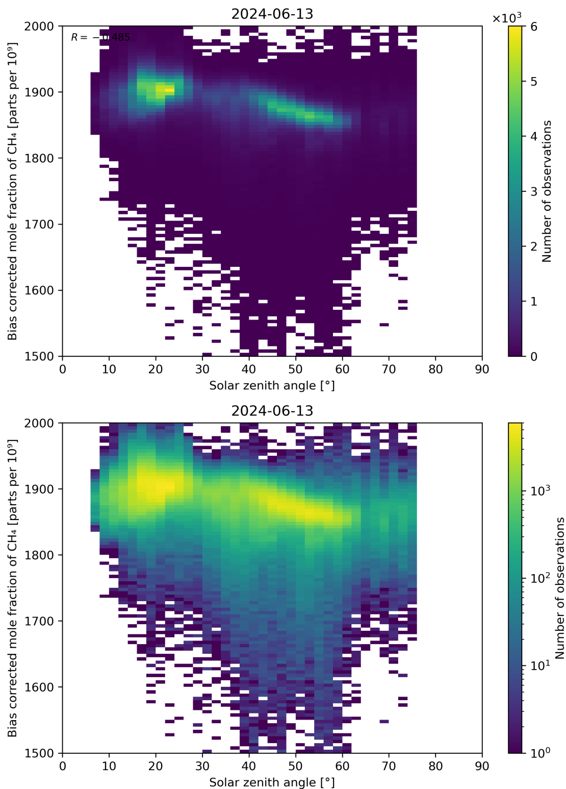
Figure 100: Scatter density plot of “Solar zenith angle” against “Bias corrected mole fraction of CH 4 ” for 2024-06-13 to 2024-06-14.
