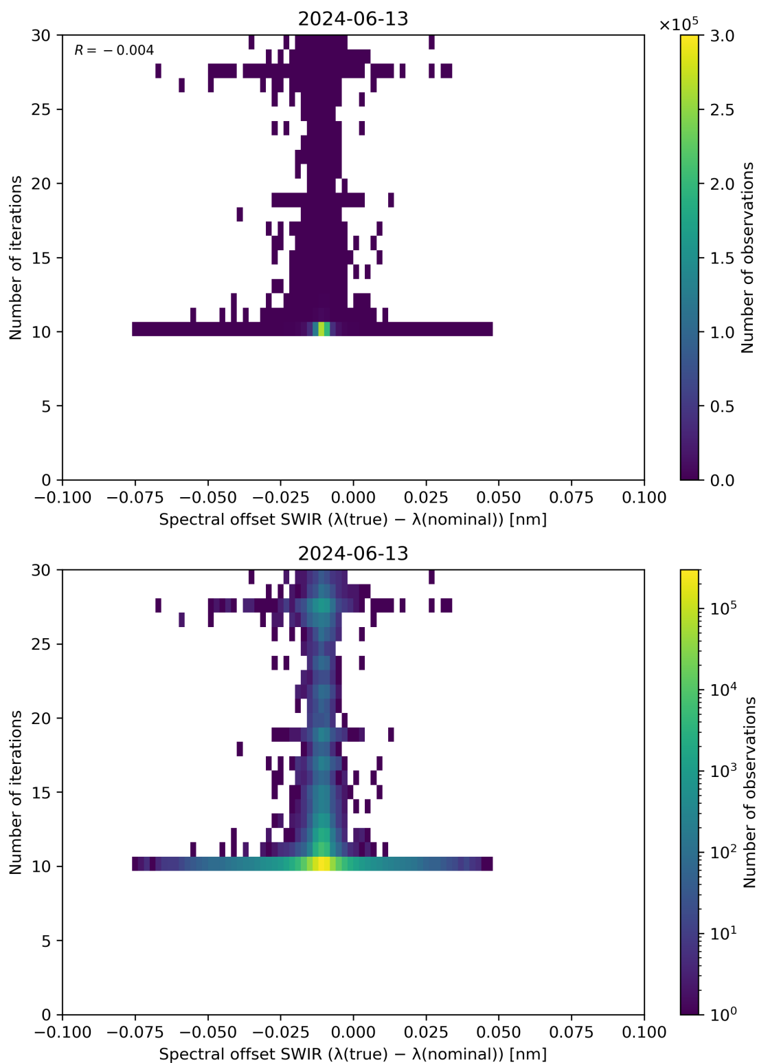
Figure 121: Scatter density plot of “Spectral offset SWIR ( \lambda(\text{true}) - \lambda(\text{nominal}) )” against “Number of iterations” for 2024-06-13 to 2024-06-14.
