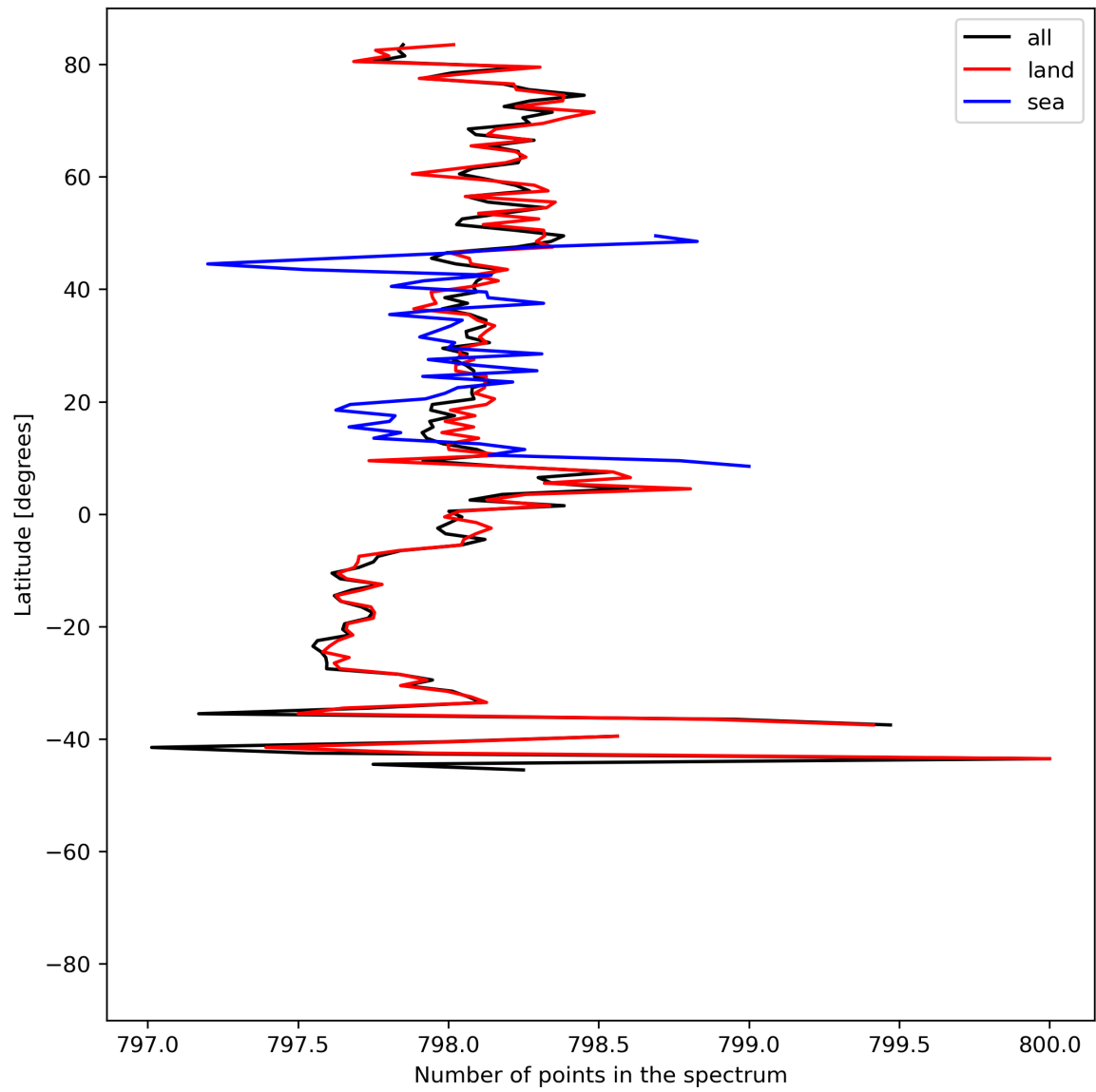
Figure 15: Zonal average of “Number of points in the spectrum” for 2024-06-13 to 2024-06-14.
