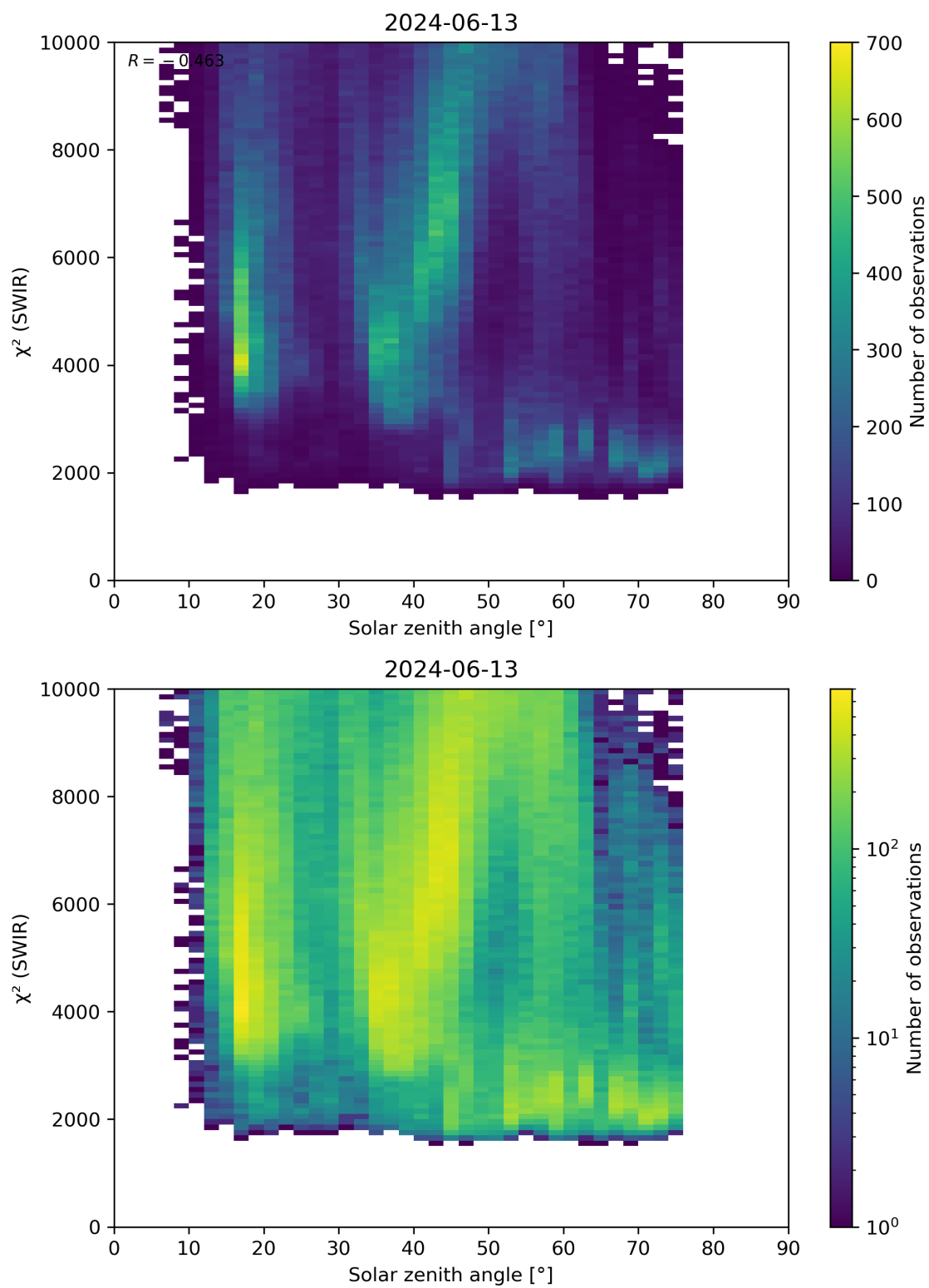
Figure 95: Scatter density plot of “Solar zenith angle” against “ \chi^2 (SWIR)” for 2024-06-13 to 2024-06-14.
