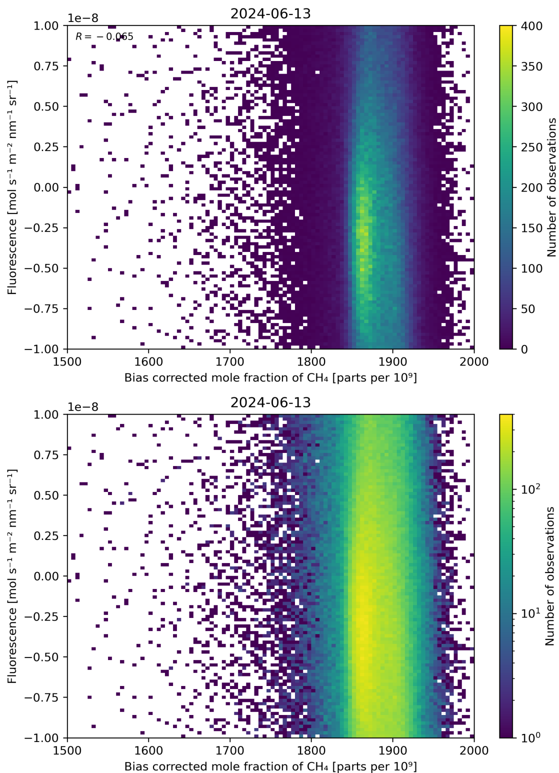
Figure 66: Scatter density plot of “Bias corrected mole fraction of \text{CH}_4 ” against “Fluorescence” for 2024-06-13 to 2024-06-14.
