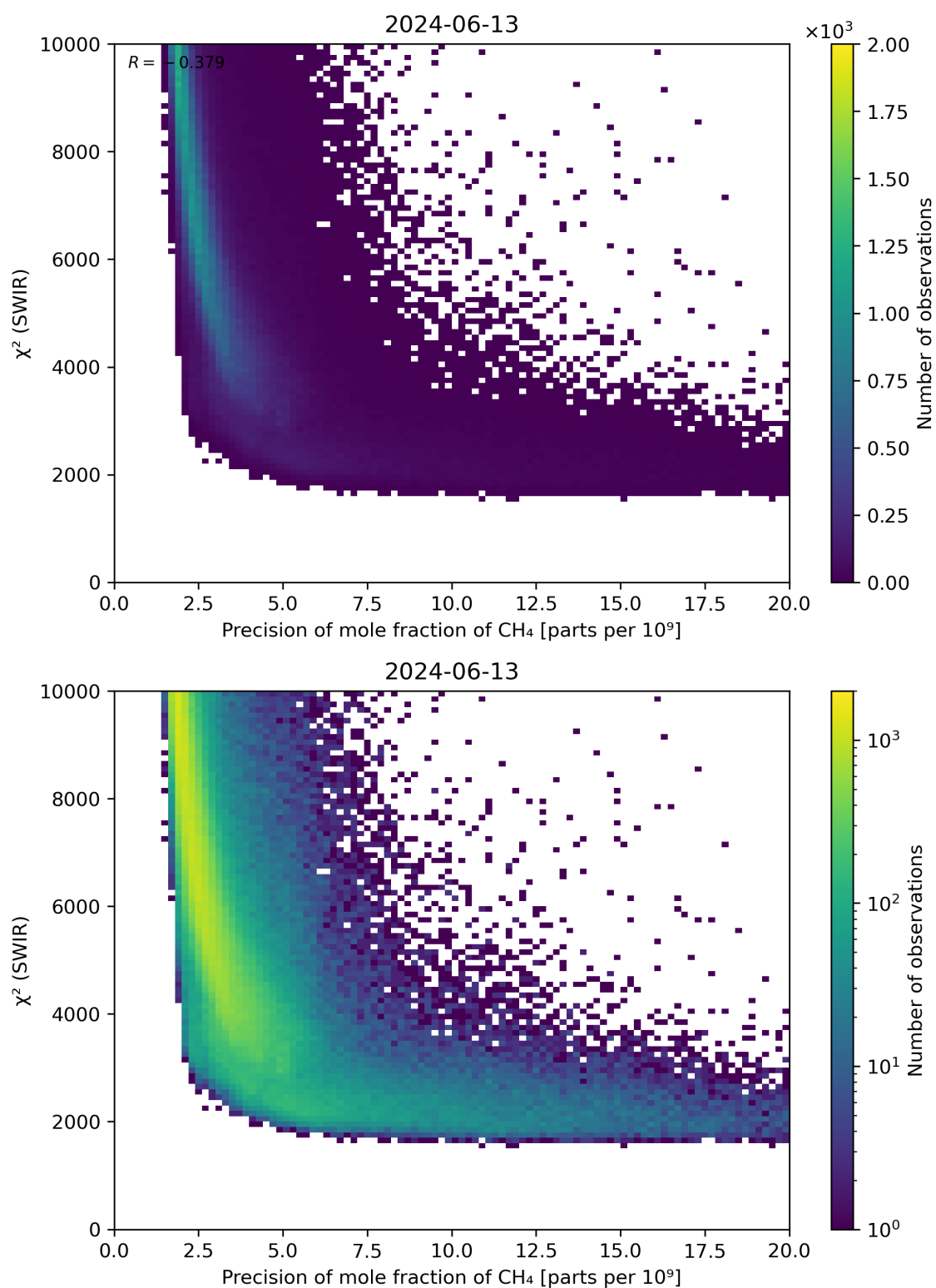
Figure 79: Scatter density plot of “Precision of mole fraction of \text{CH}_4 ” against “ \chi^2 (SWIR)” for 2024-06-13 to 2024-06-14.
