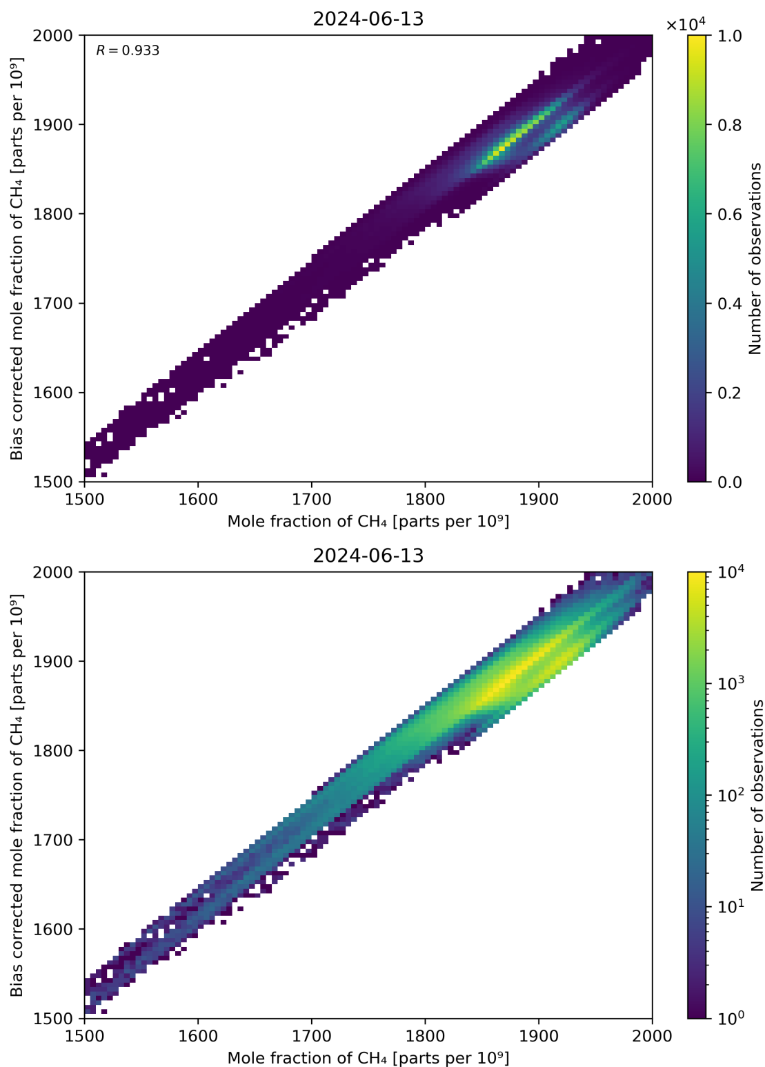
Figure 74: Scatter density plot of “Mole fraction of CH 4 ” against “Bias corrected mole fraction of CH 4 ” for 2024-06-13 to 2024-06-14.
