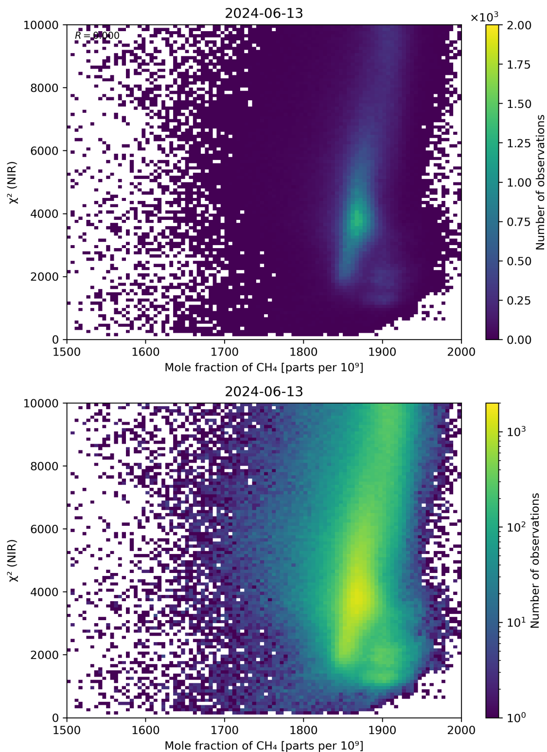
Figure 70: Scatter density plot of “Mole fraction of \text{CH}_4 ” against “ \chi^2 (NIR)” for 2024-06-13 to 2024-06-14.
