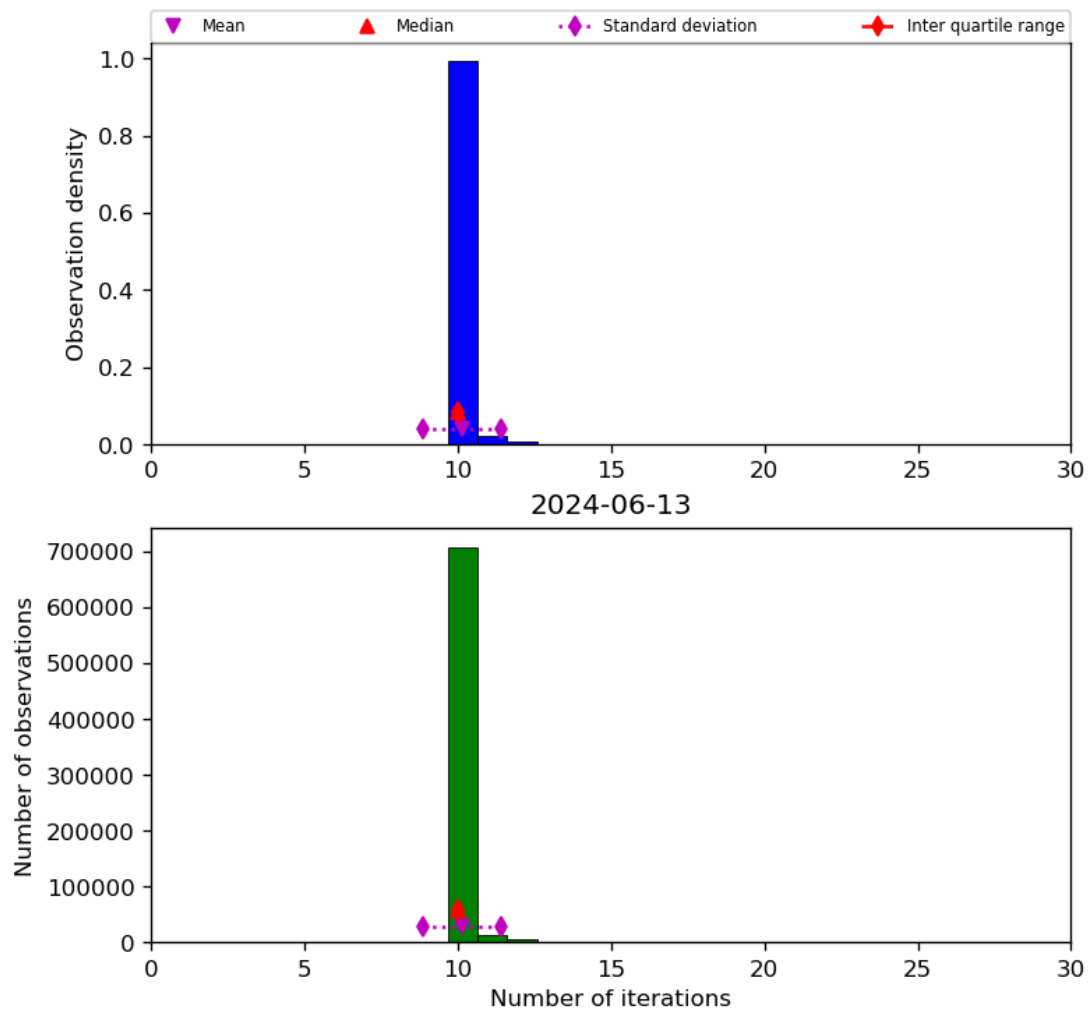
Figure 31: Histogram of “Number of iterations” for 2024-06-13 to 2024-06-14
