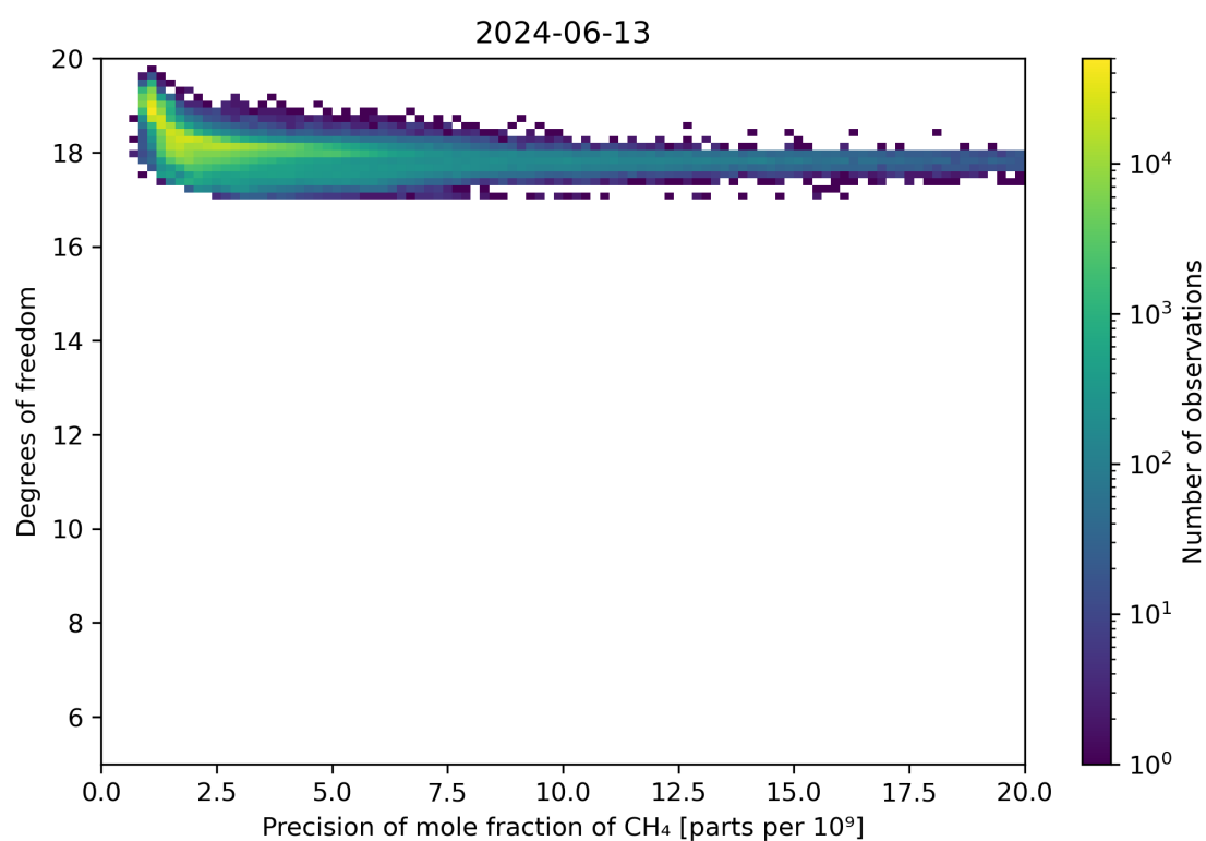
Figure 80: Scatter density plot of “Precision of mole fraction of CH 4 ” against “Degrees of freedom” for 2024-06-13 to 2024-06-14.
