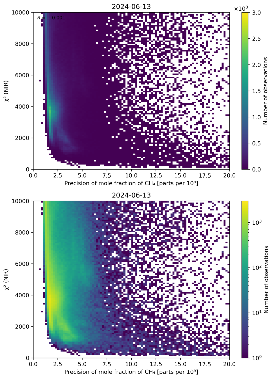
Figure 78: Scatter density plot of “Precision of mole fraction of CH 4 ” against “ \chi^2 (NIR)” for 2024-06-13 to 2024-06-14.
