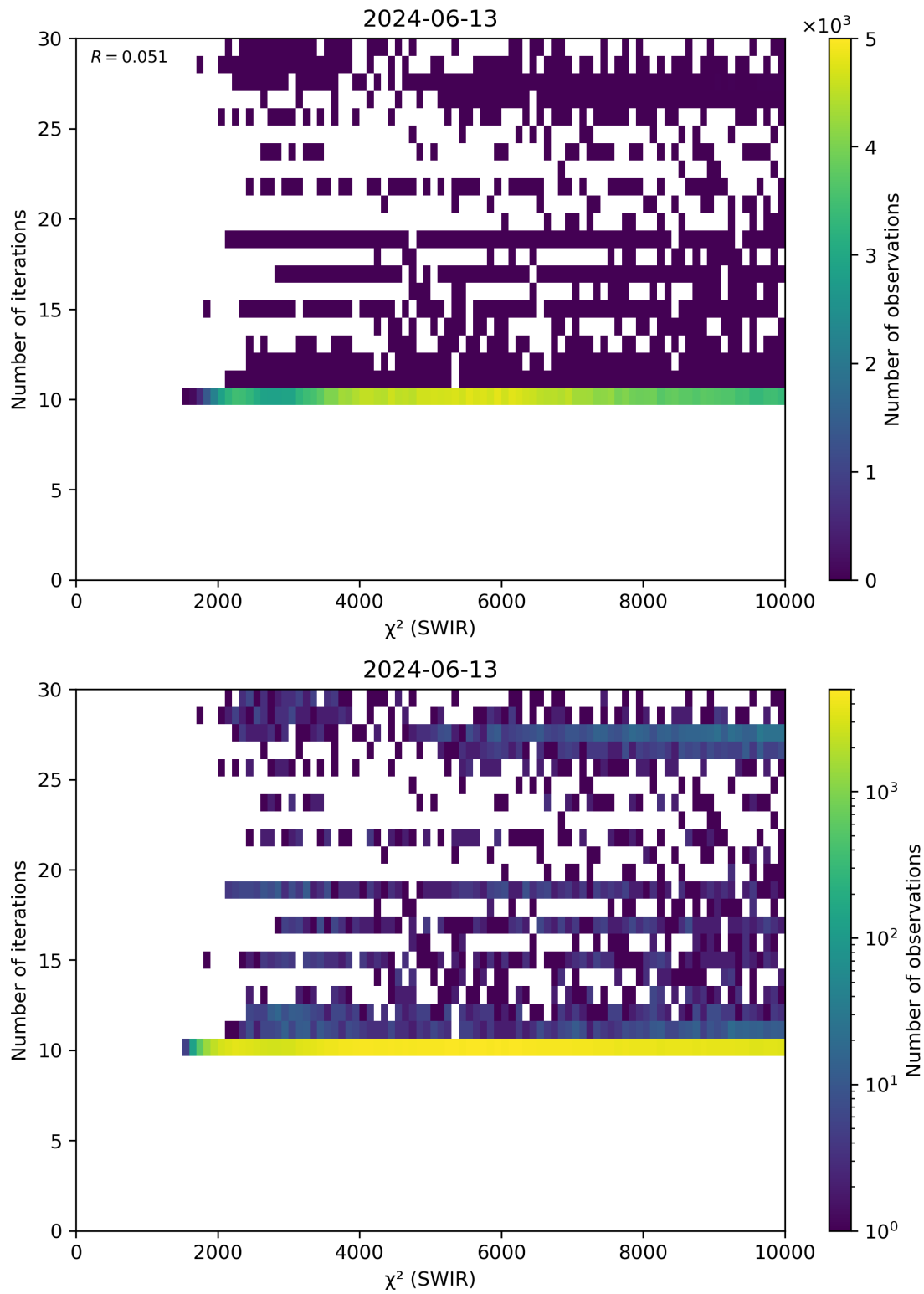
Figure 50: Scatter density plot of “ \chi^2 (SWIR)” against “Number of iterations” for 2024-06-13 to 2024-06-14.
