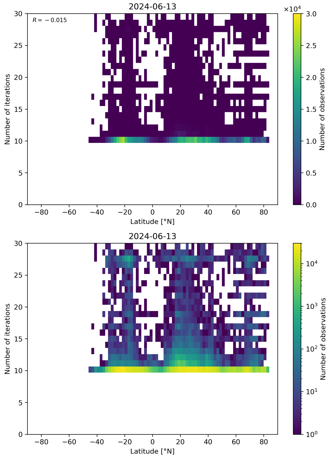
Figure 60: Scatter density plot of “Latitude” against “Number of iterations” for 2024-06-13 to 2024-06-14.
