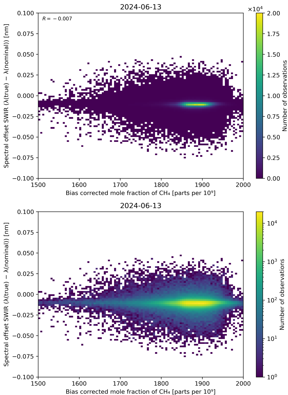
Figure 69: Scatter density plot of “Bias corrected mole fraction of \text{CH}_4 ” against “Spectral offset SWIR ( \lambda(\text{true}) - \lambda(\text{nominal}) )” for 2024-06-13 to 2024-06-14.
