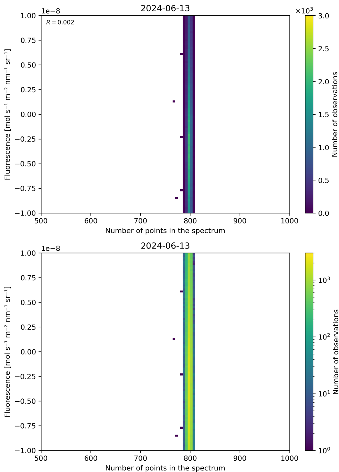
Figure 91: Scatter density plot of “Number of points in the spectrum” against “Fluorescence” for 2024-06-13 to 2024-06-14.
