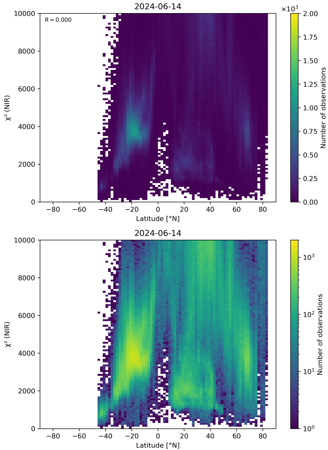
Figure 53: Scatter density plot of “Latitude” against “ \chi^2 (NIR)” for 2024-06-13 to 2024-06-15.
