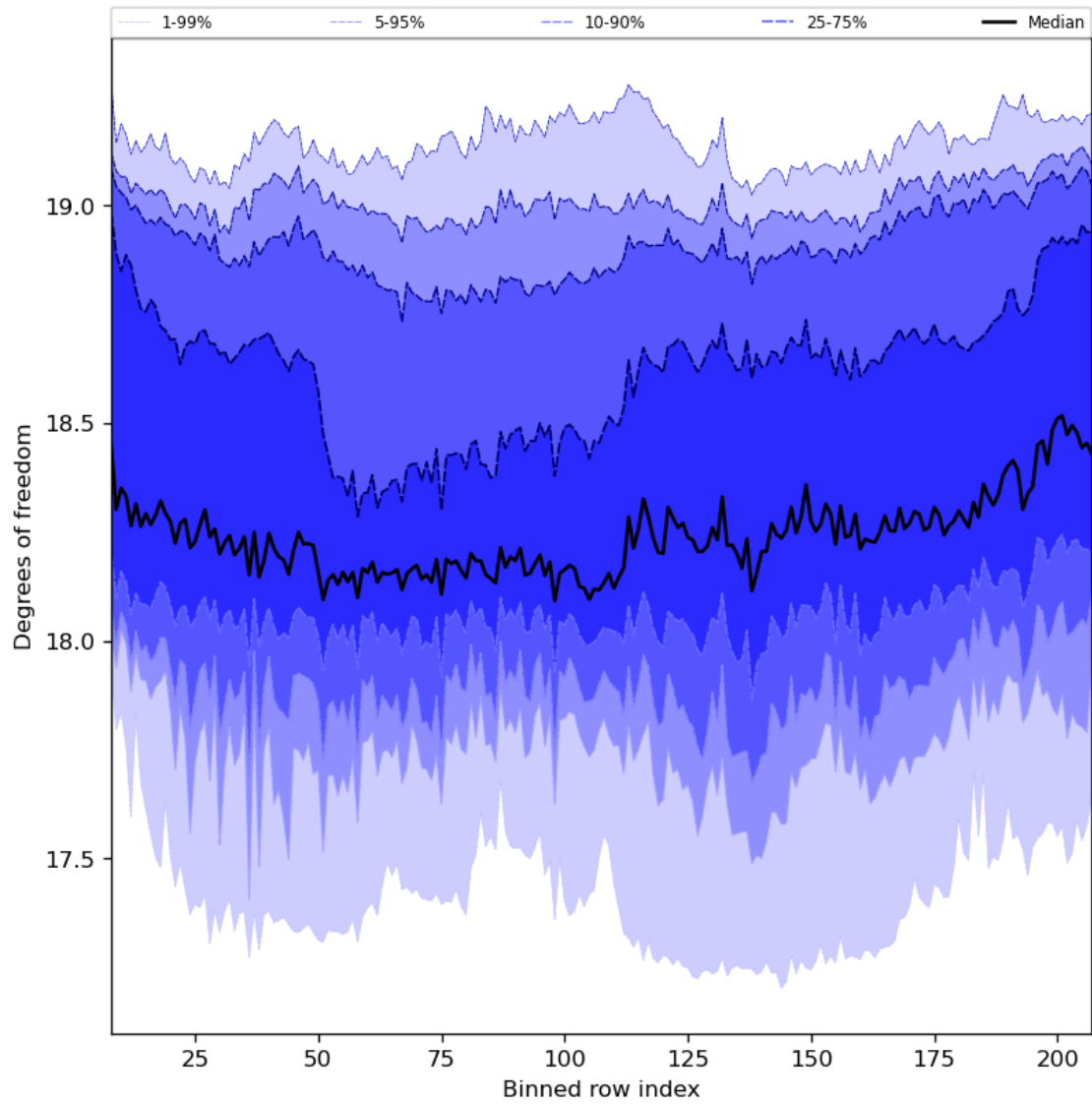
Figure 41: Along track statistics of “Degrees of freedom” for 2024-06-13 to 2024-06-15
