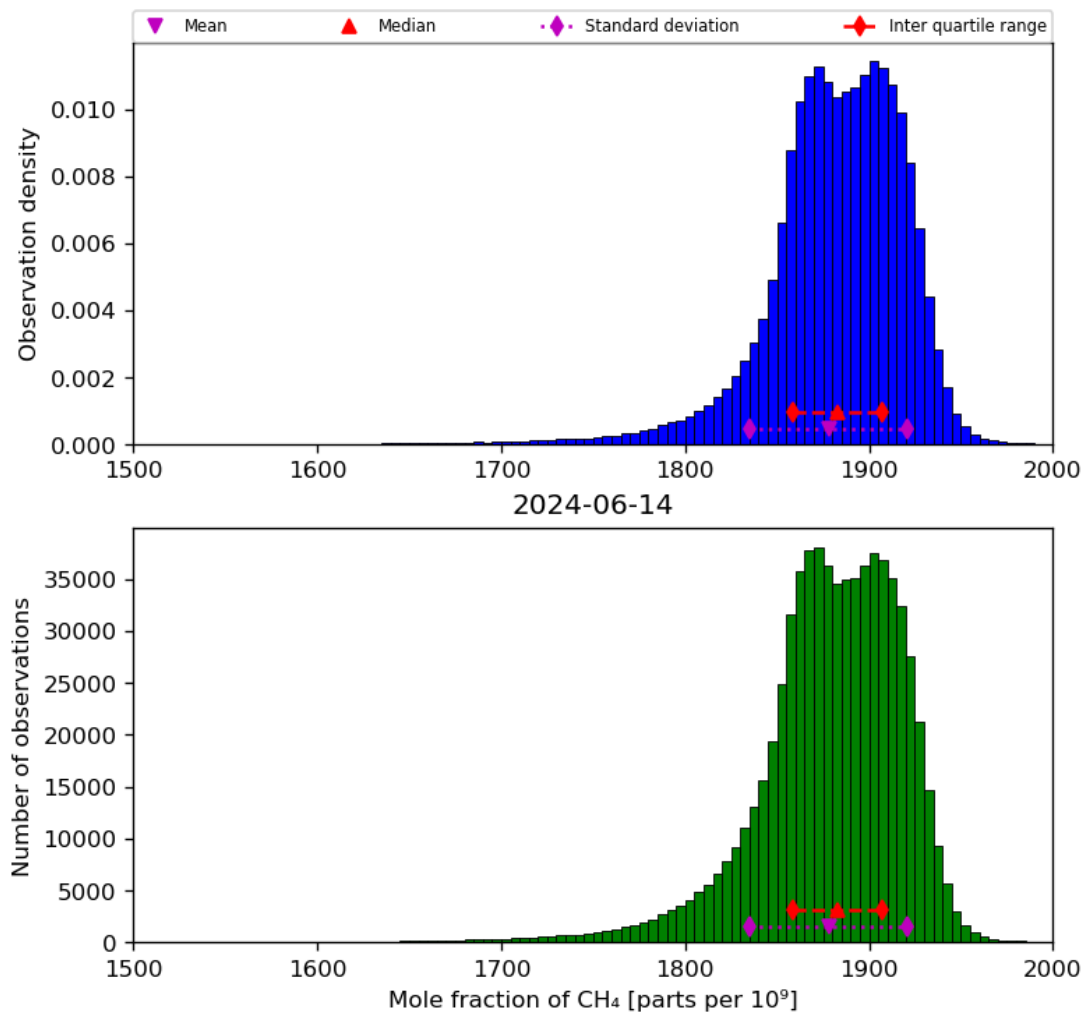
Figure 23: Histogram of “Mole fraction of CH 4 ” for 2024-06-13 to 2024-06-15
