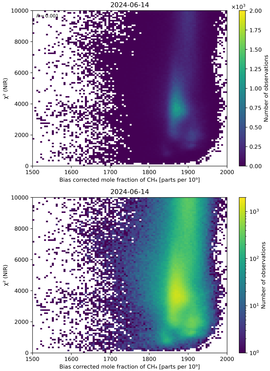
Figure 63: Scatter density plot of “Bias corrected mole fraction of CH 4 ” against “ \chi^2 (NIR)” for 2024-06-13 to 2024-06-15.
