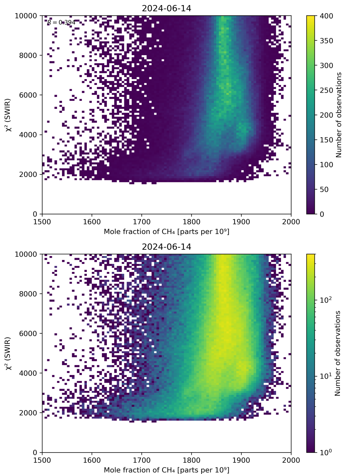
Figure 71: Scatter density plot of “Mole fraction of \text{CH}_4 ” against “ \chi^2 (SWIR)” for 2024-06-13 to 2024-06-15.
