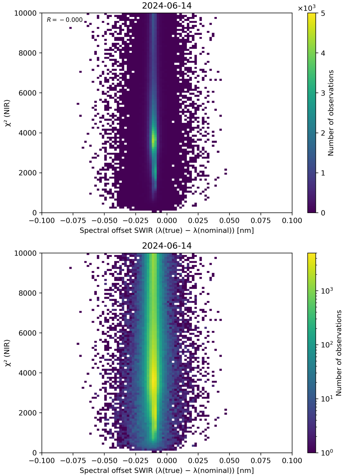
Figure 117: Scatter density plot of “Spectral offset SWIR ( \lambda(\text{true}) - \lambda(\text{nominal}) )” against “ \chi^2 (NIR)” for 2024-06-13 to 2024-06-15.
