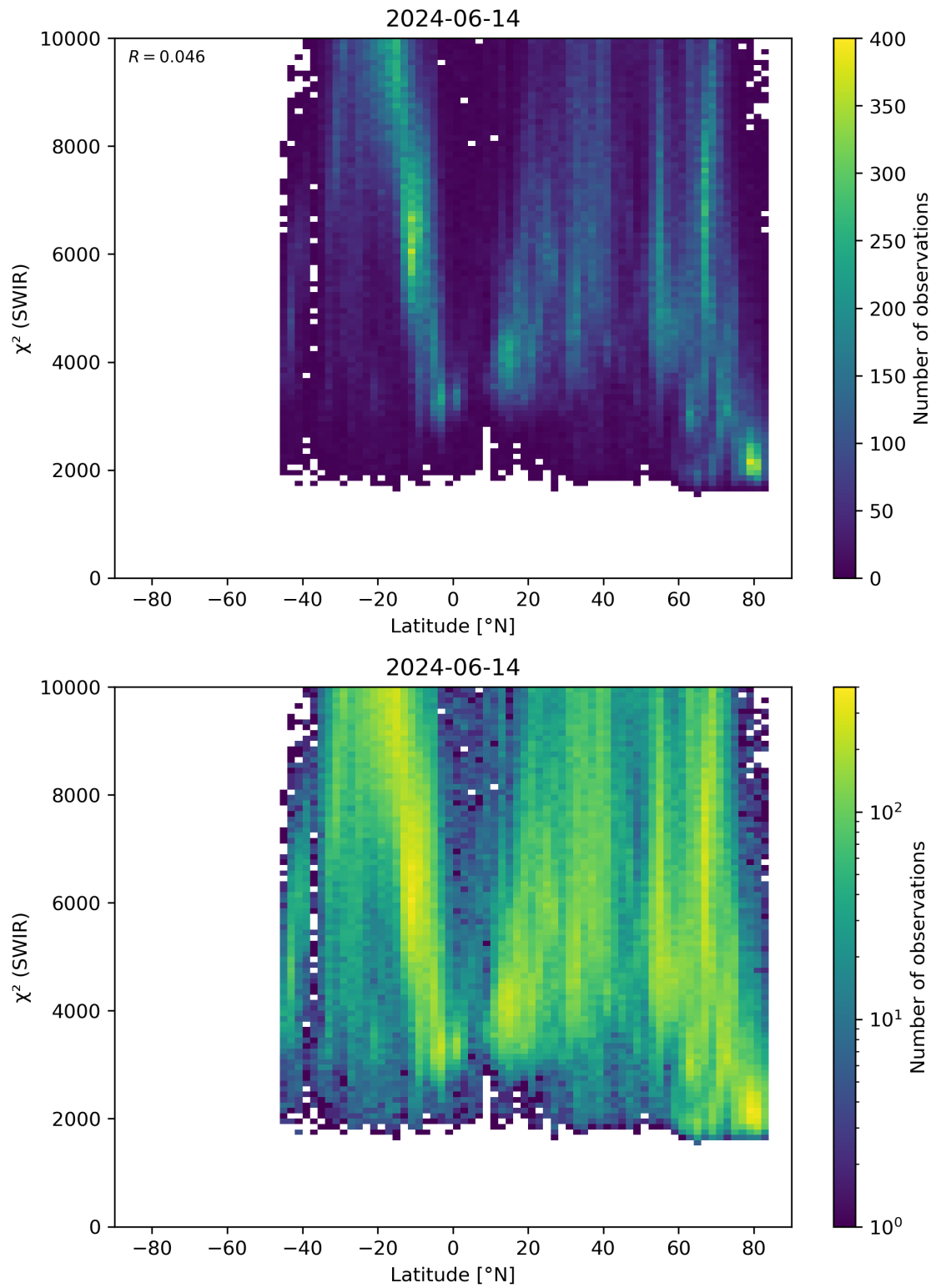
Figure 54: Scatter density plot of “Latitude” against “ \chi^2 (SWIR)” for 2024-06-13 to 2024-06-15.
