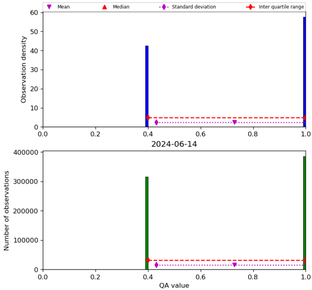
Figure 22: Histogram of “QA value” for 2024-06-13 to 2024-06-15
