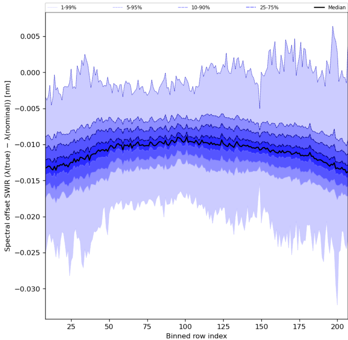
Figure 38: Along track statistics of “Spectral offset SWIR ( \lambda(\text{true}) - \lambda(\text{nominal}) )” for 2024-06-13 to 2024-06-15
