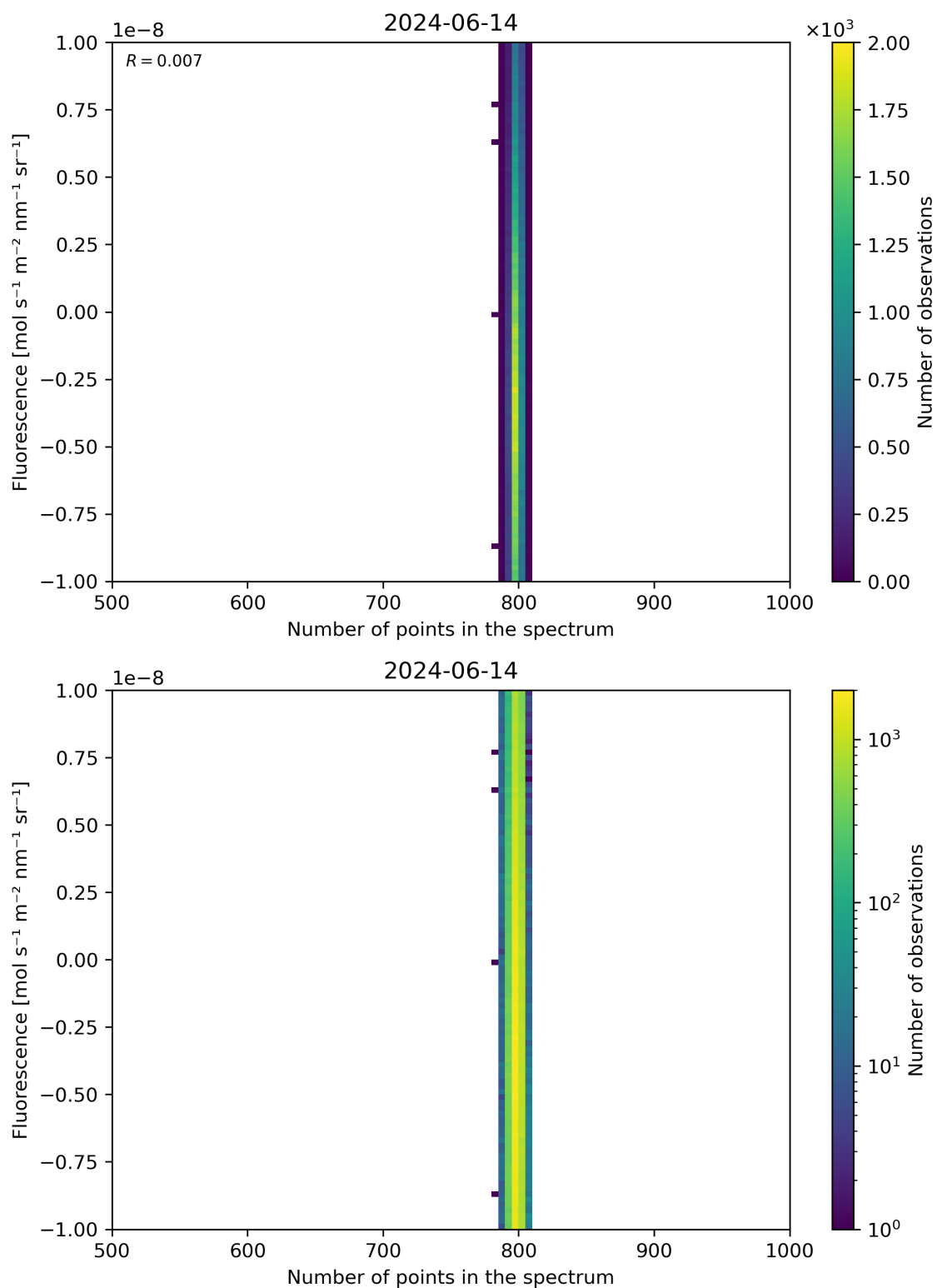
Figure 91: Scatter density plot of “Number of points in the spectrum” against “Fluorescence” for 2024-06-13 to 2024-06-15.
