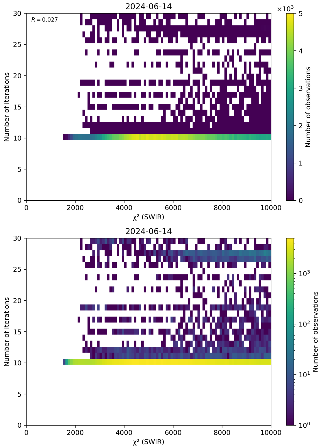
Figure 50: Scatter density plot of “ \chi^2 (SWIR)” against “Number of iterations” for 2024-06-13 to 2024-06-15.
