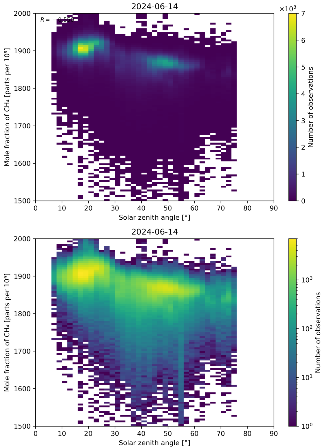
Figure 99: Scatter density plot of “Solar zenith angle” against “Mole fraction of CH 4 ” for 2024-06-13 to 2024-06-15.
