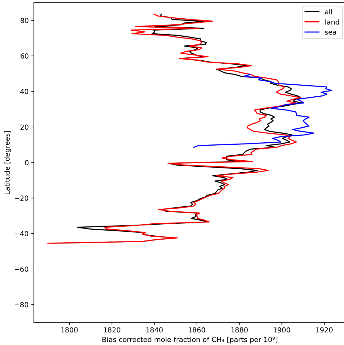
Figure 14: Zonal average of “Bias corrected mole fraction of CH 4 ” for 2024-06-13 to 2024-06-15.
