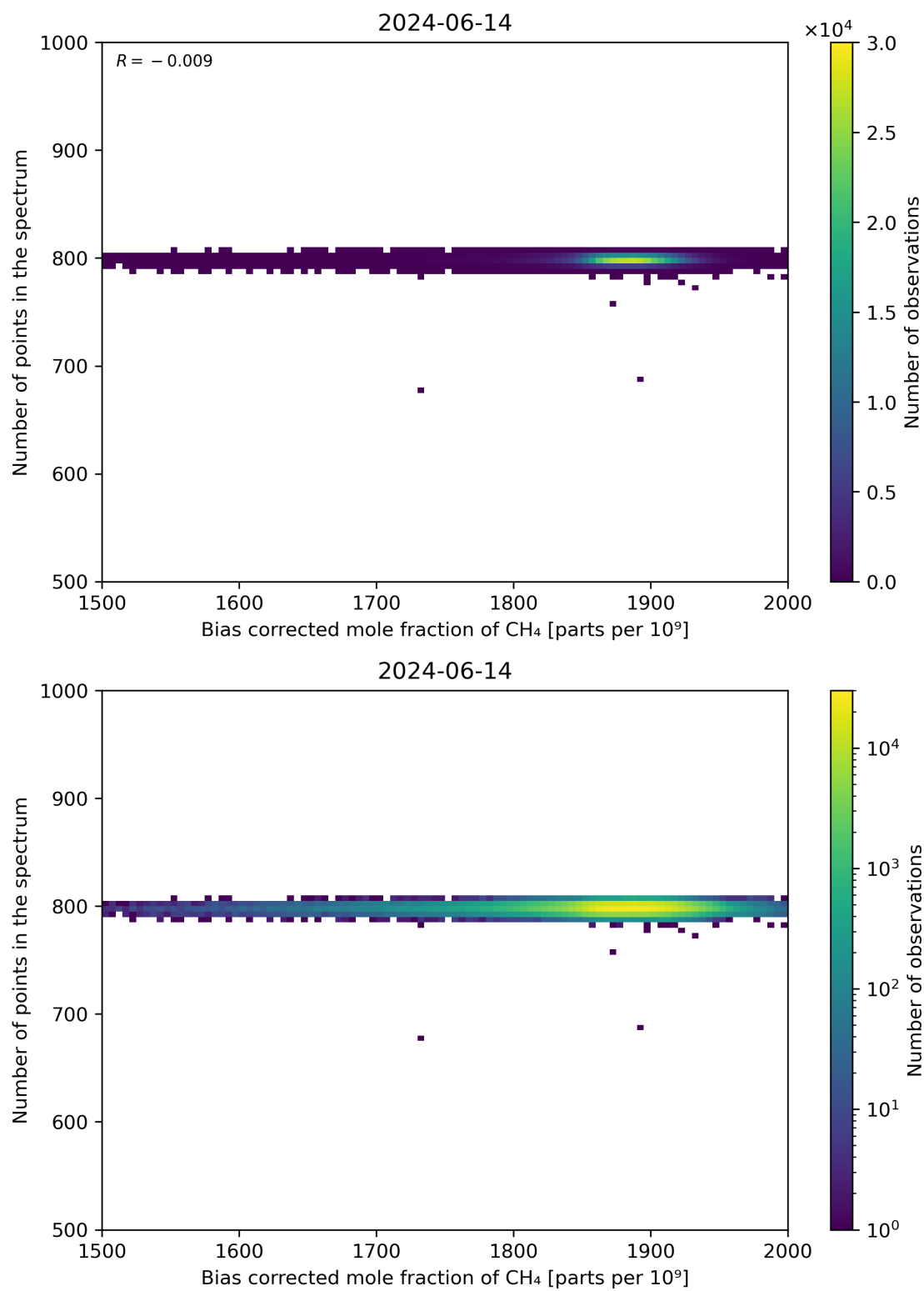
Figure 68: Scatter density plot of “Bias corrected mole fraction of CH 4 ” against “Number of points in the spectrum” for 2024-06-13 to 2024-06-15.
