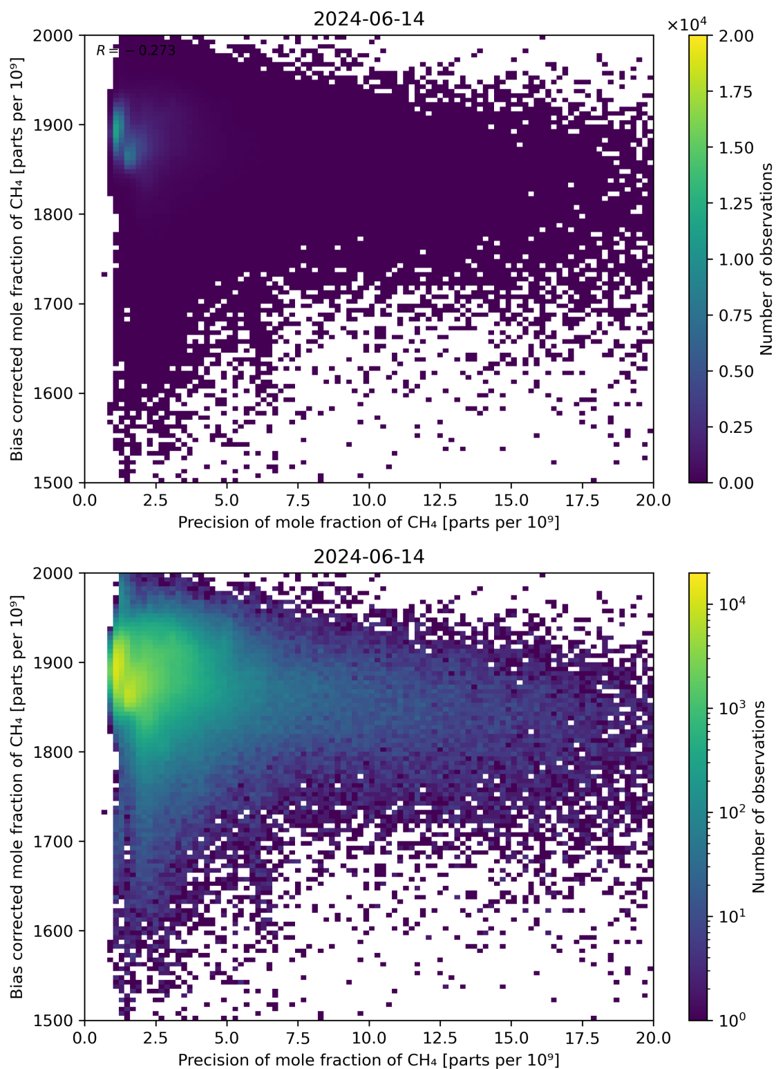
Figure 82: Scatter density plot of “Precision of mole fraction of CH 4 ” against “Bias corrected mole fraction of CH 4 ” for 2024-06-13 to 2024-06-15.
