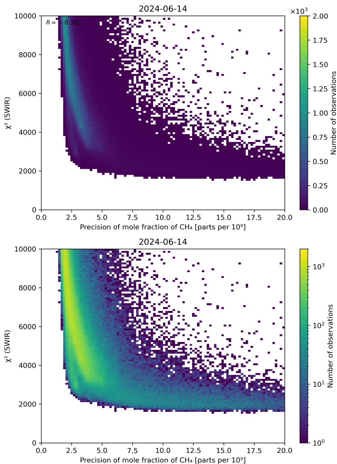
Figure 79: Scatter density plot of “Precision of mole fraction of \text{CH}_4 ” against “ \chi^2 (SWIR)” for 2024-06-13 to 2024-06-15.
