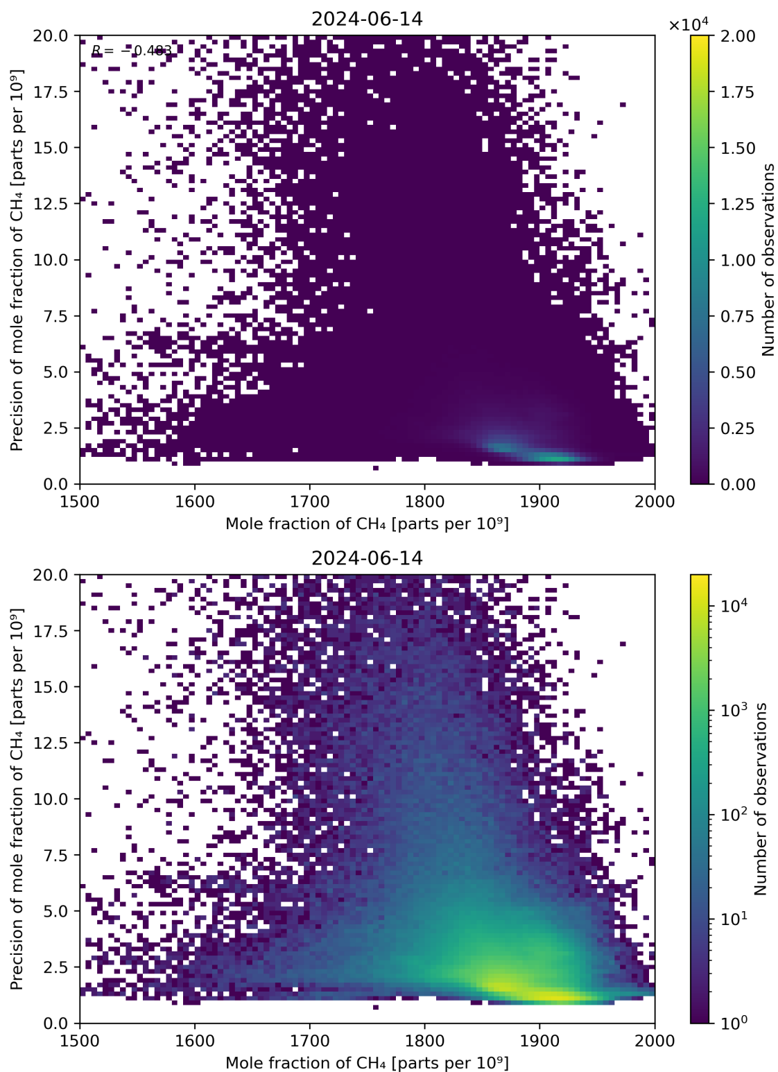
Figure 75: Scatter density plot of “Mole fraction of CH 4 ” against “Precision of mole fraction of CH 4 ” for 2024-06-13 to 2024-06-15.
