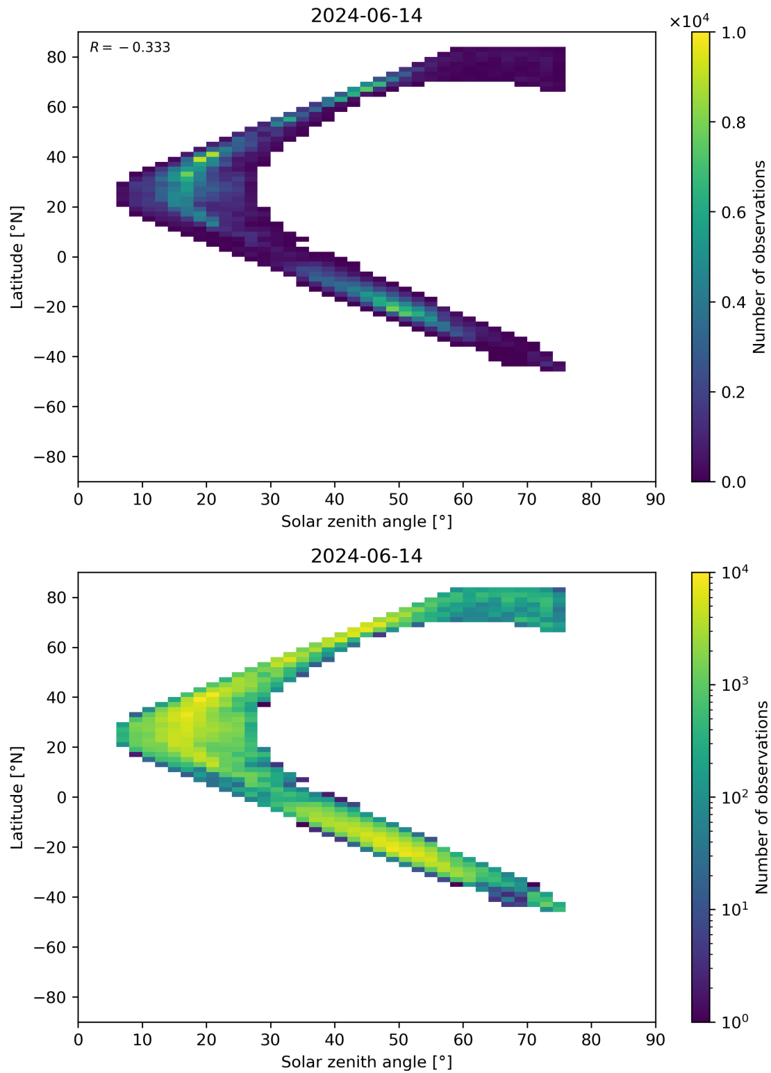
Figure 98: Scatter density plot of “Solar zenith angle” against “Latitude” for 2024-06-13 to 2024-06-15.
