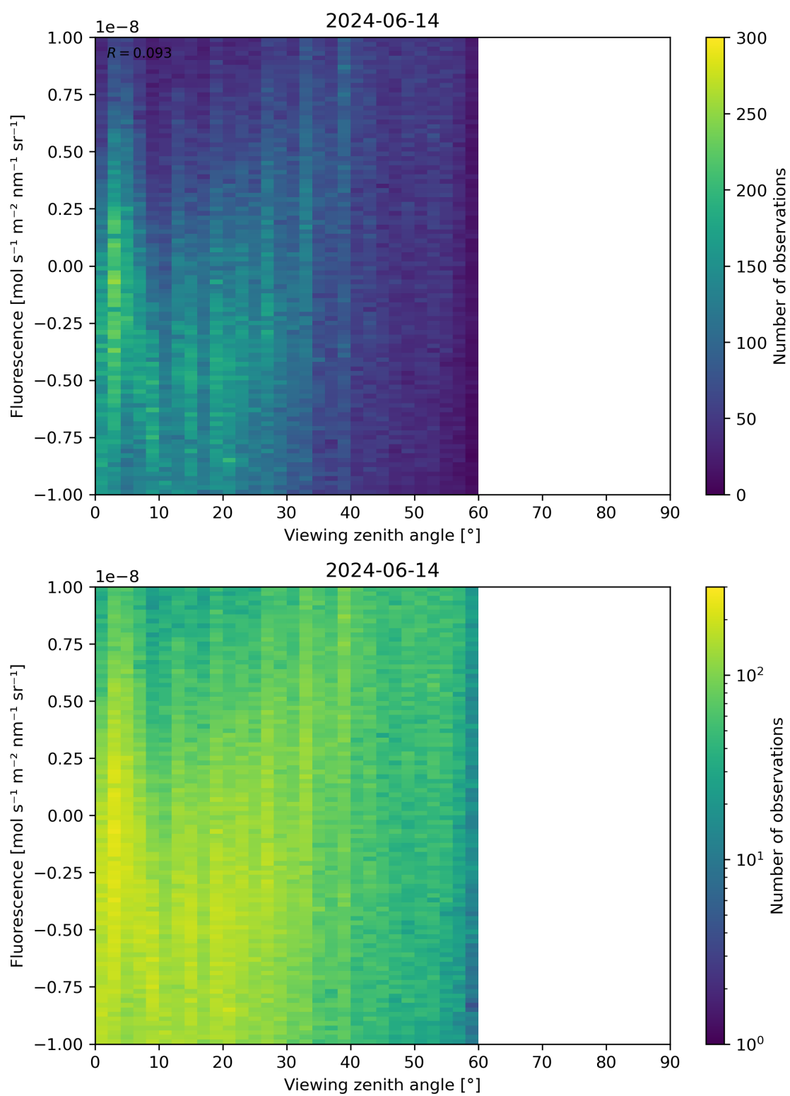
Figure 108: Scatter density plot of “Viewing zenith angle” against “Fluorescence” for 2024-06-13 to 2024-06-15.
