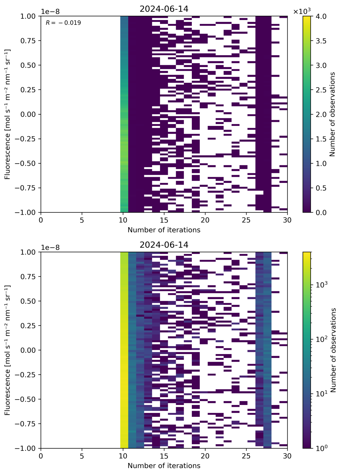
Figure 87: Scatter density plot of “Number of iterations” against “Fluorescence” for 2024-06-13 to 2024-06-15.
