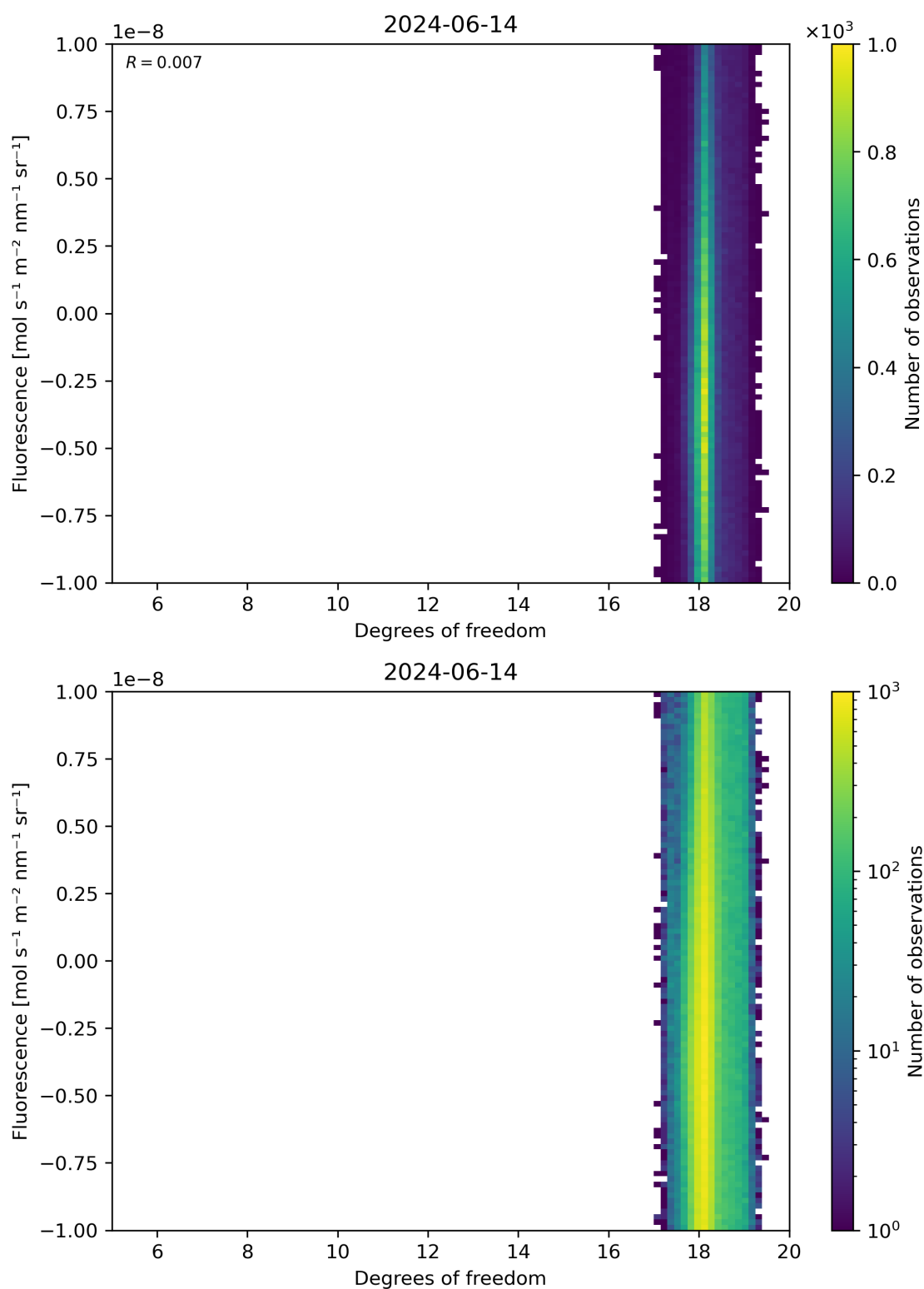
Figure 51: Scatter density plot of “Degrees of freedom” against “Fluorescence” for 2024-06-13 to 2024-06-15.
