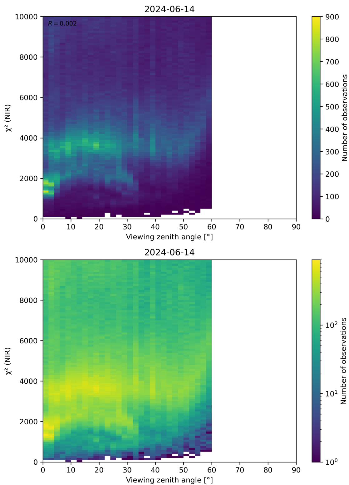
Figure 105: Scatter density plot of “Viewing zenith angle” against “ \chi^2 (NIR)” for 2024-06-13 to 2024-06-15.
