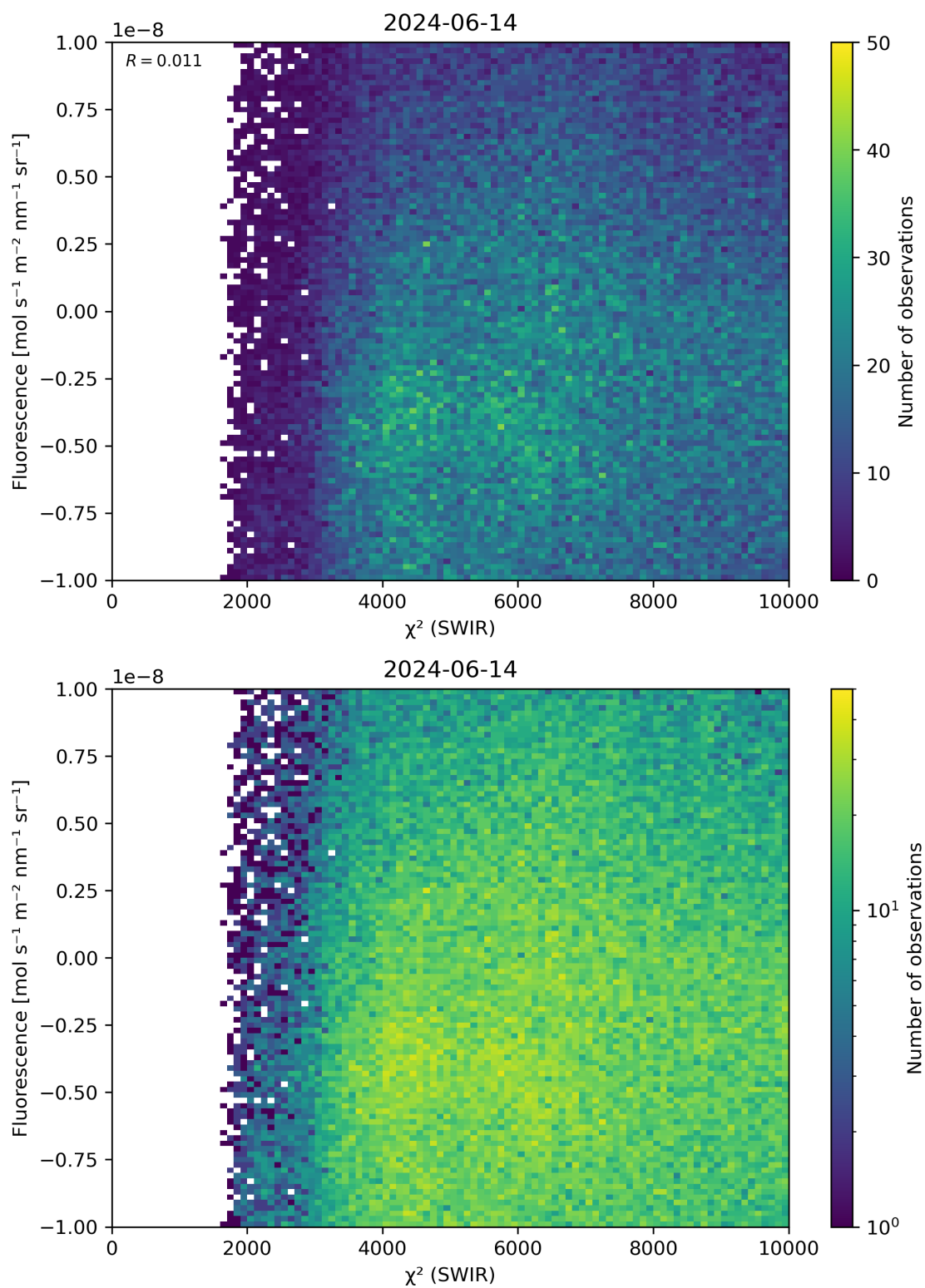
Figure 49: Scatter density plot of “ \chi^2 (SWIR)” against “Fluorescence” for 2024-06-13 to 2024-06-15.
