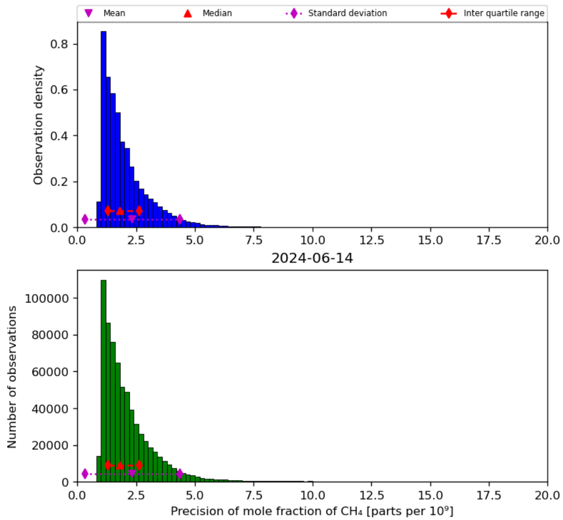
Figure 24: Histogram of “Precision of mole fraction of CH 4 ” for 2024-06-13 to 2024-06-15
