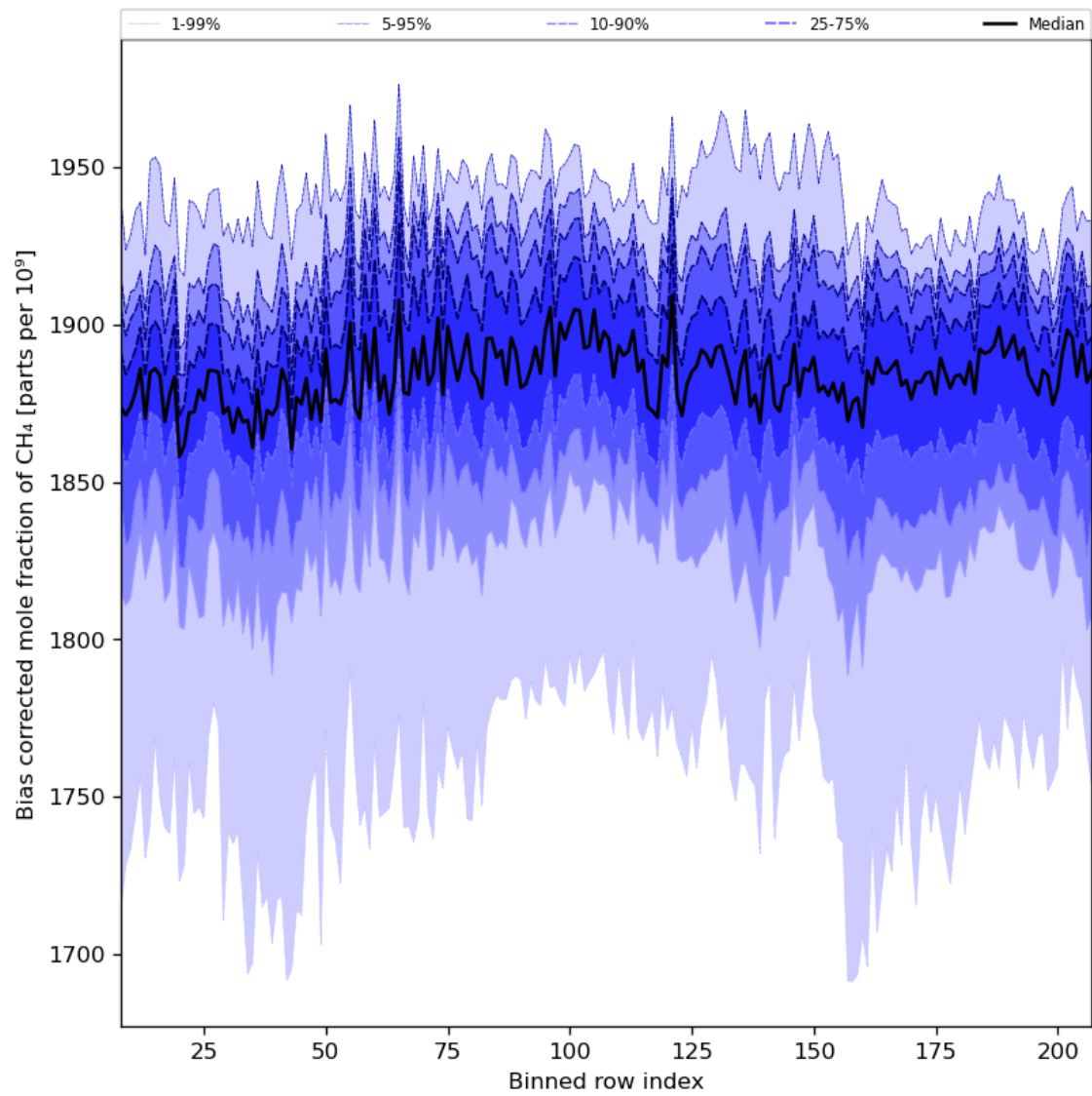
Figure 36: Along track statistics of “Bias corrected mole fraction of CH 4 ” for 2024-06-13 to 2024-06-15
