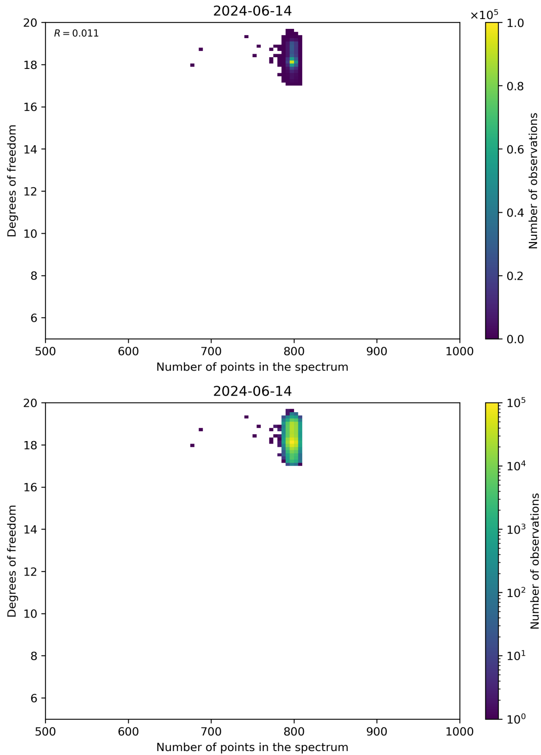
Figure 90: Scatter density plot of “Number of points in the spectrum” against “Degrees of freedom” for 2024-06-13 to 2024-06-15.
