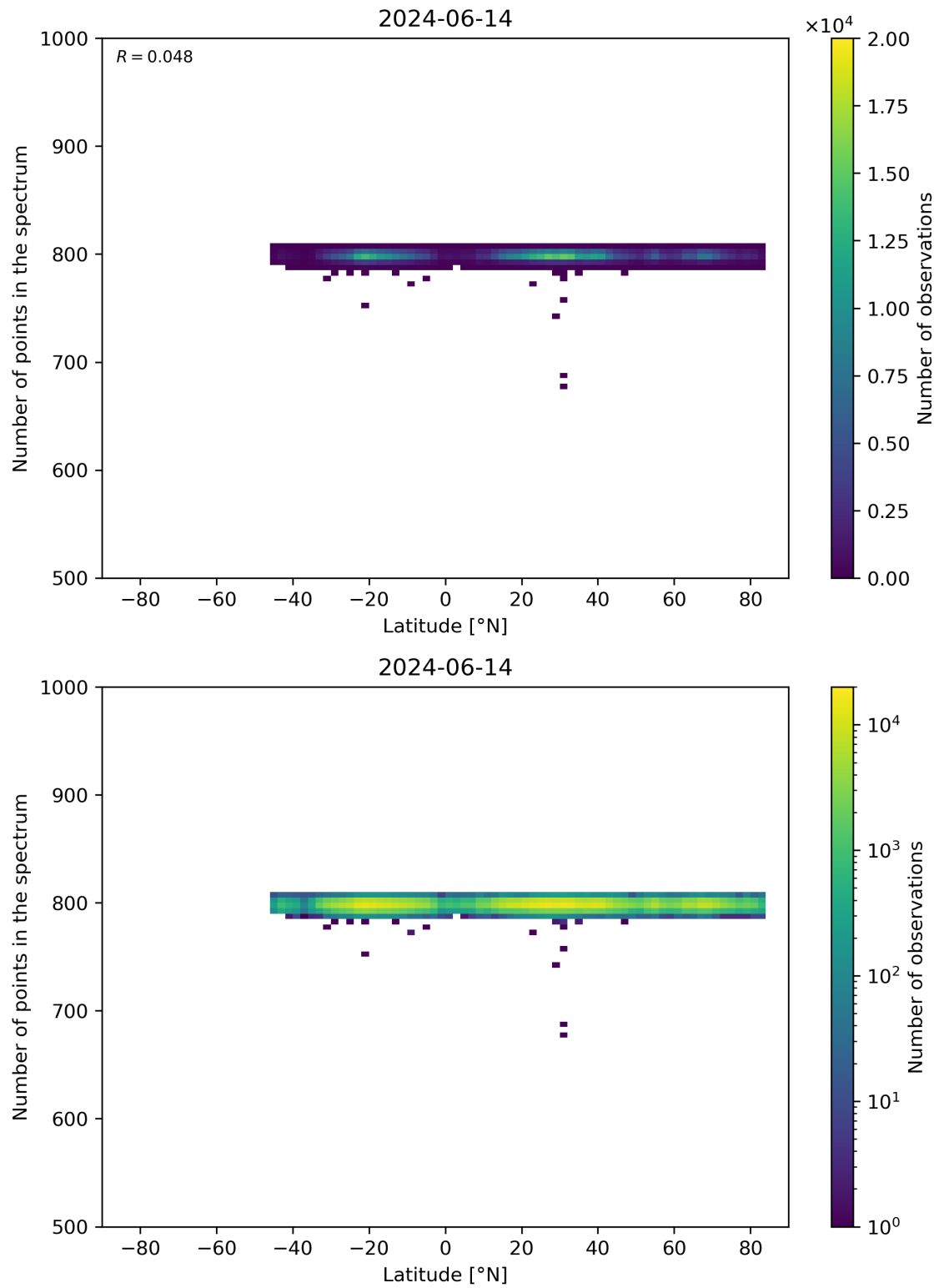
Figure 61: Scatter density plot of “Latitude” against “Number of points in the spectrum” for 2024-06-13 to 2024-06-15.
