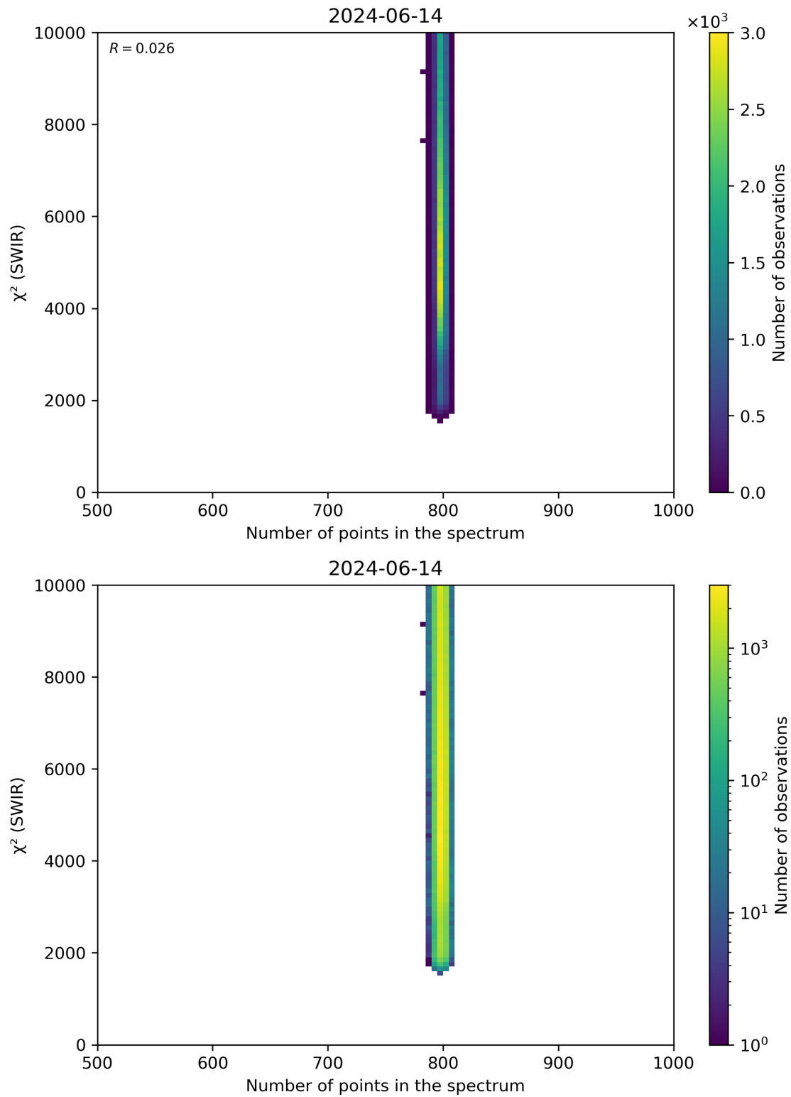
Figure 89: Scatter density plot of “Number of points in the spectrum” against “ \chi^2 (SWIR)” for 2024-06-13 to 2024-06-15.
