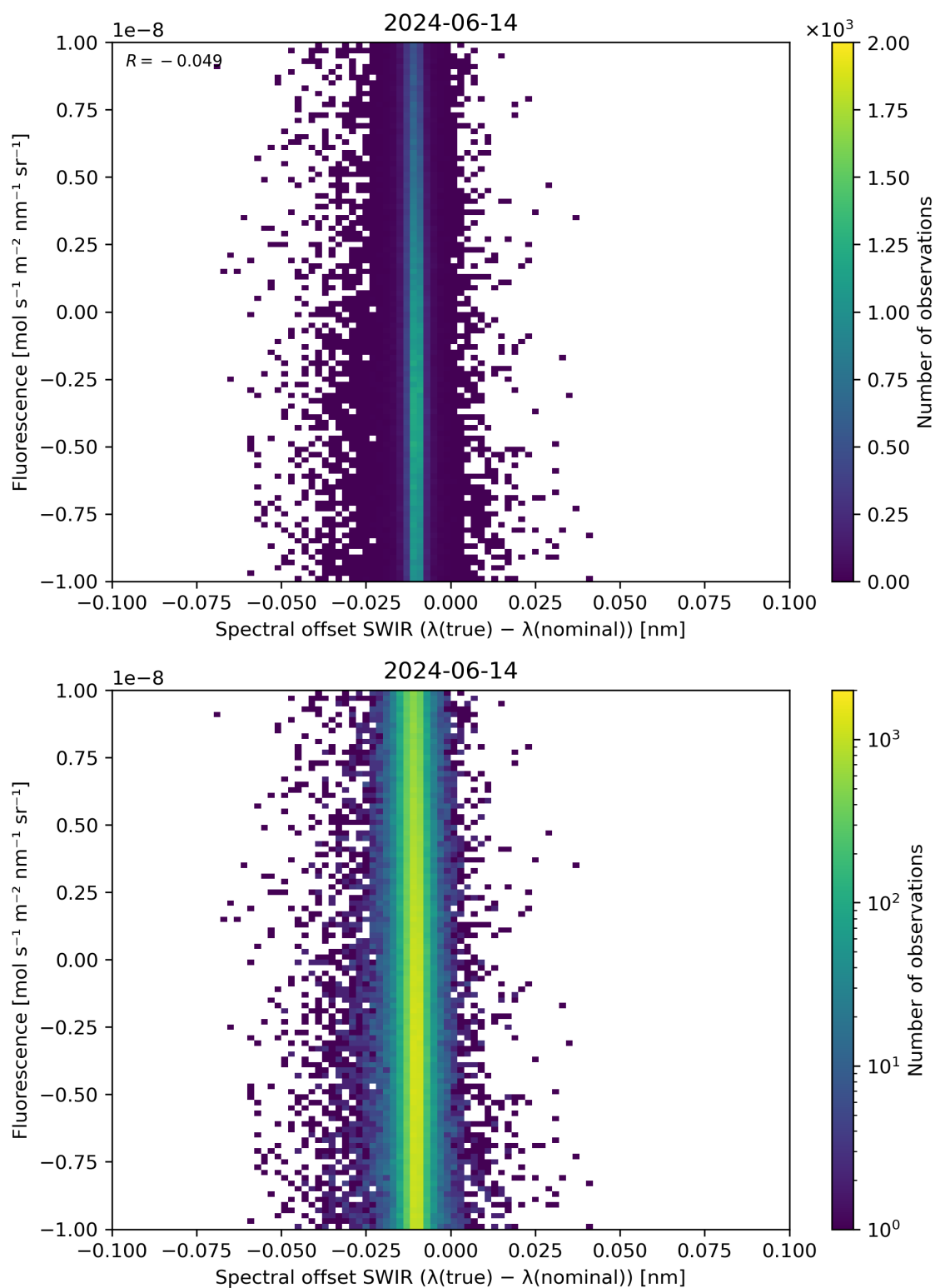
Figure 120: Scatter density plot of “Spectral offset SWIR ( \lambda(\text{true}) - \lambda(\text{nominal}) )” against “Fluorescence” for 2024-06-13 to 2024-06-15.
