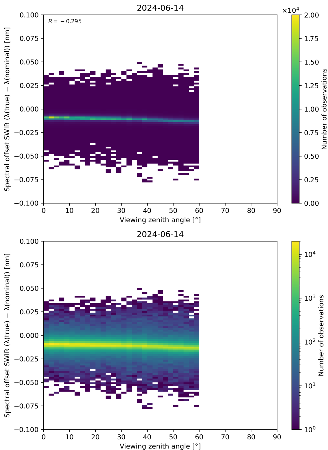
Figure 116: Scatter density plot of “Viewing zenith angle” against “Spectral offset SWIR ( \lambda(\text{true}) - \lambda(\text{nominal}) )” for 2024-06-13 to 2024-06-15.
