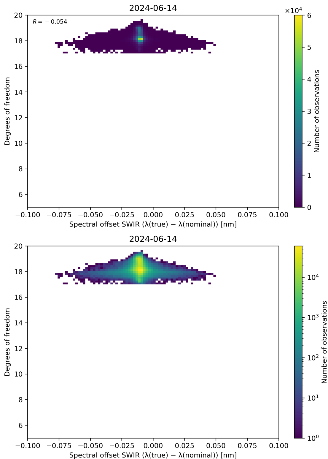
Figure 119: Scatter density plot of “Spectral offset SWIR ( \lambda(\text{true}) - \lambda(\text{nominal}) )” against “Degrees of freedom” for 2024-06-13 to 2024-06-15.
