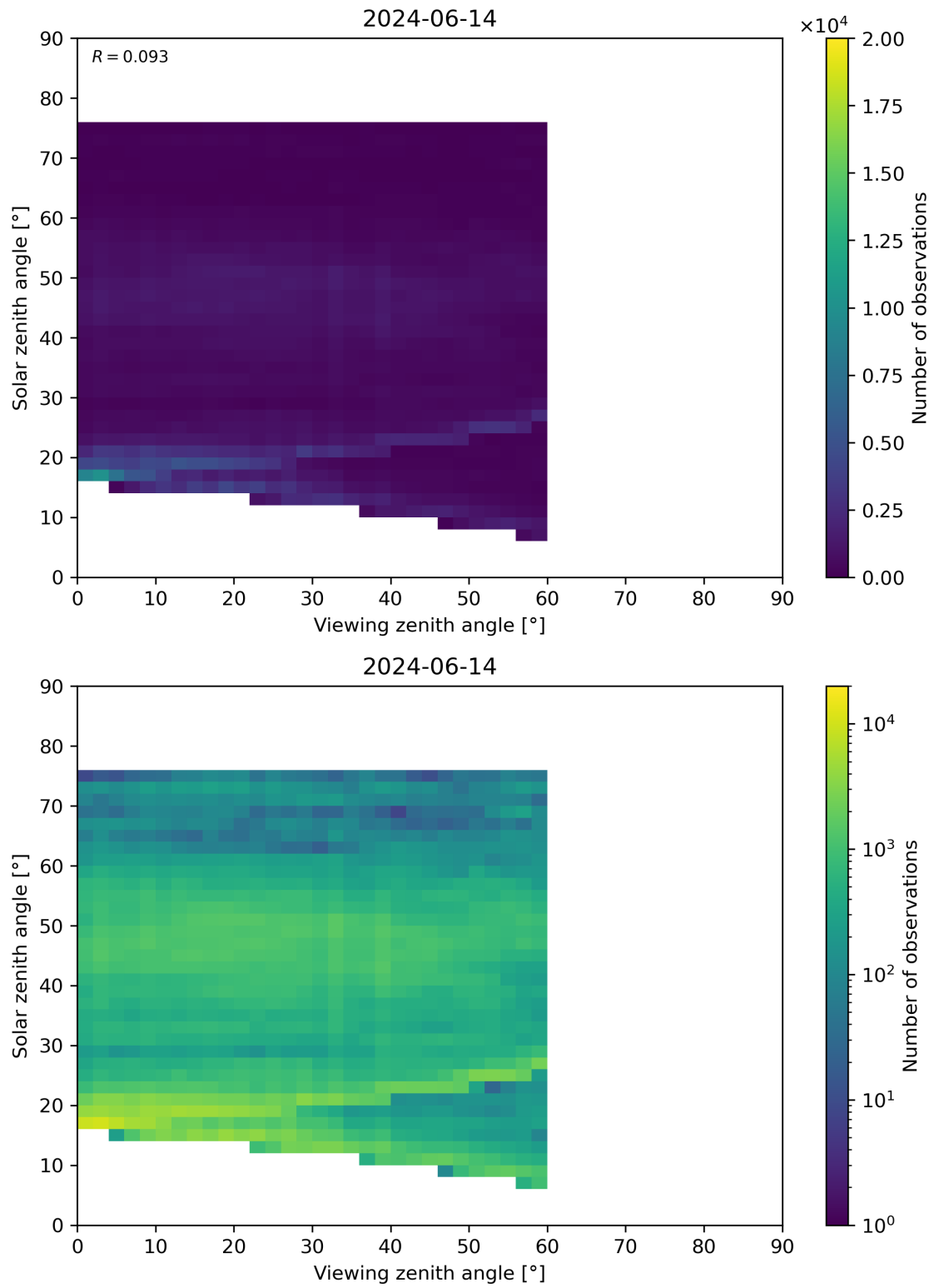
Figure 115: Scatter density plot of “Viewing zenith angle” against “Solar zenith angle” for 2024-06-13 to 2024-06-15.
