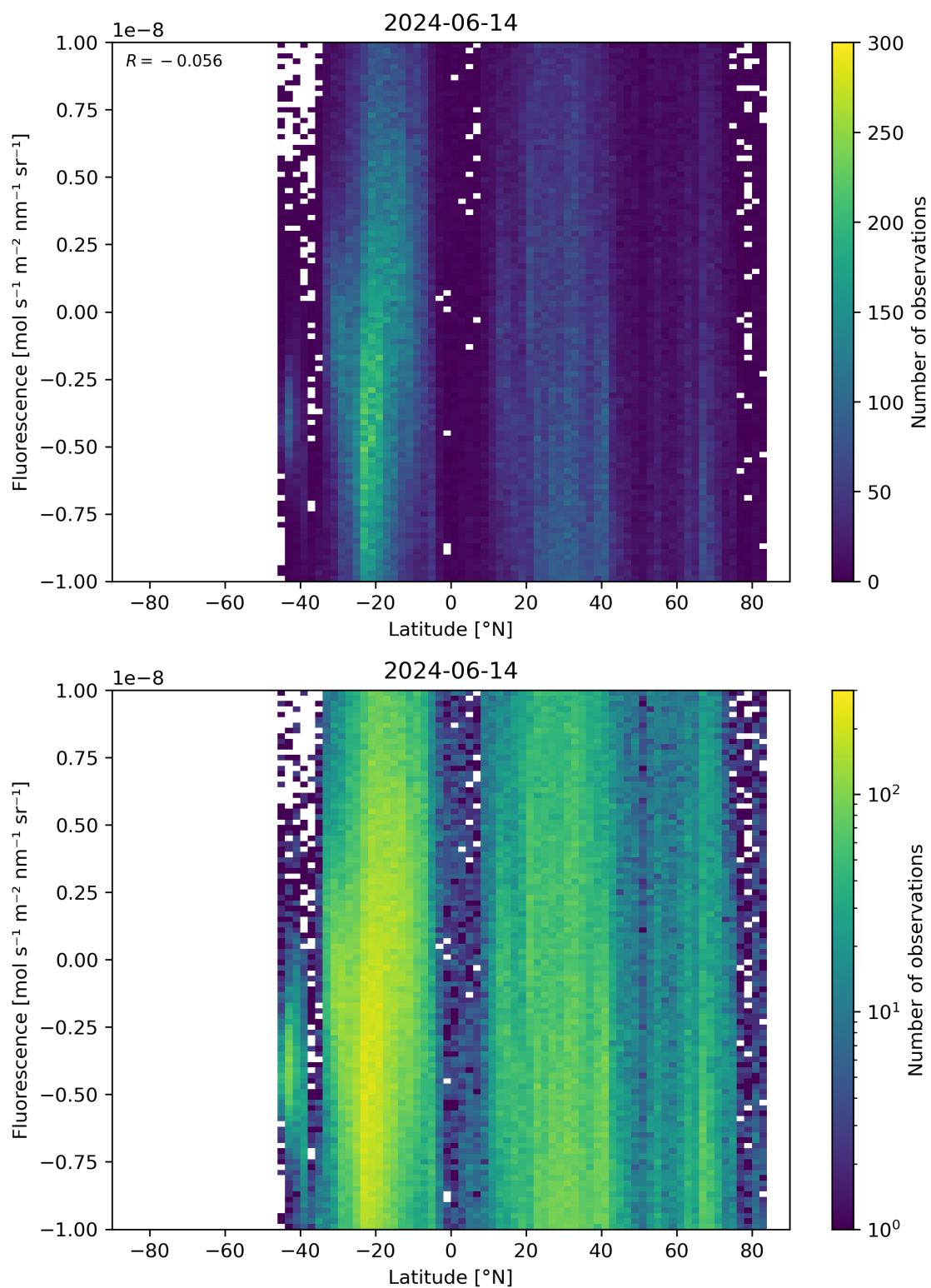
Figure 56: Scatter density plot of “Latitude” against “Fluorescence” for 2024-06-13 to 2024-06-15.
