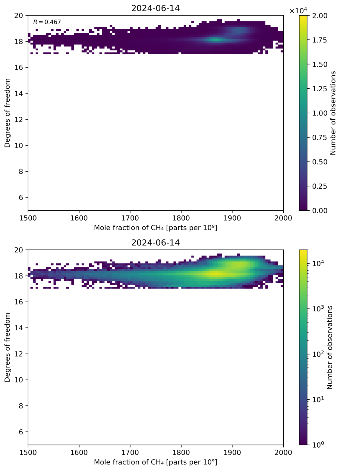
Figure 72: Scatter density plot of “Mole fraction of CH 4 ” against “Degrees of freedom” for 2024-06-13 to 2024-06-15.
