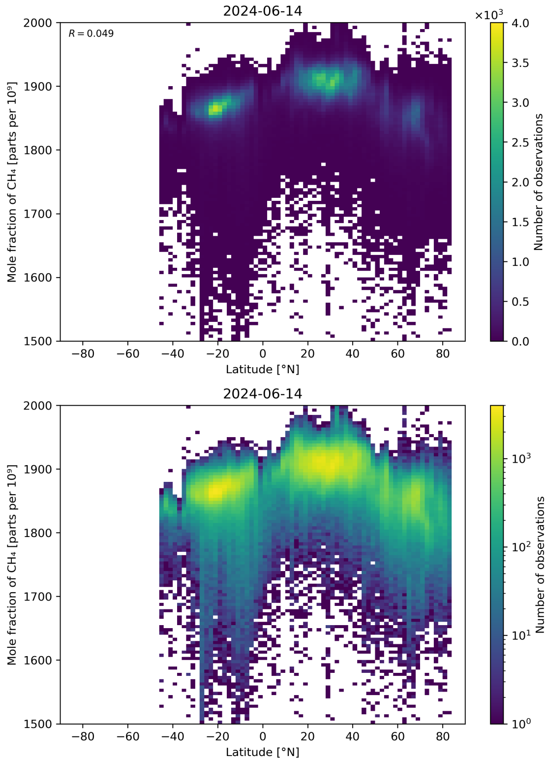
Figure 57: Scatter density plot of “Latitude” against “Mole fraction of \text{CH}_4 ” for 2024-06-13 to 2024-06-15.
