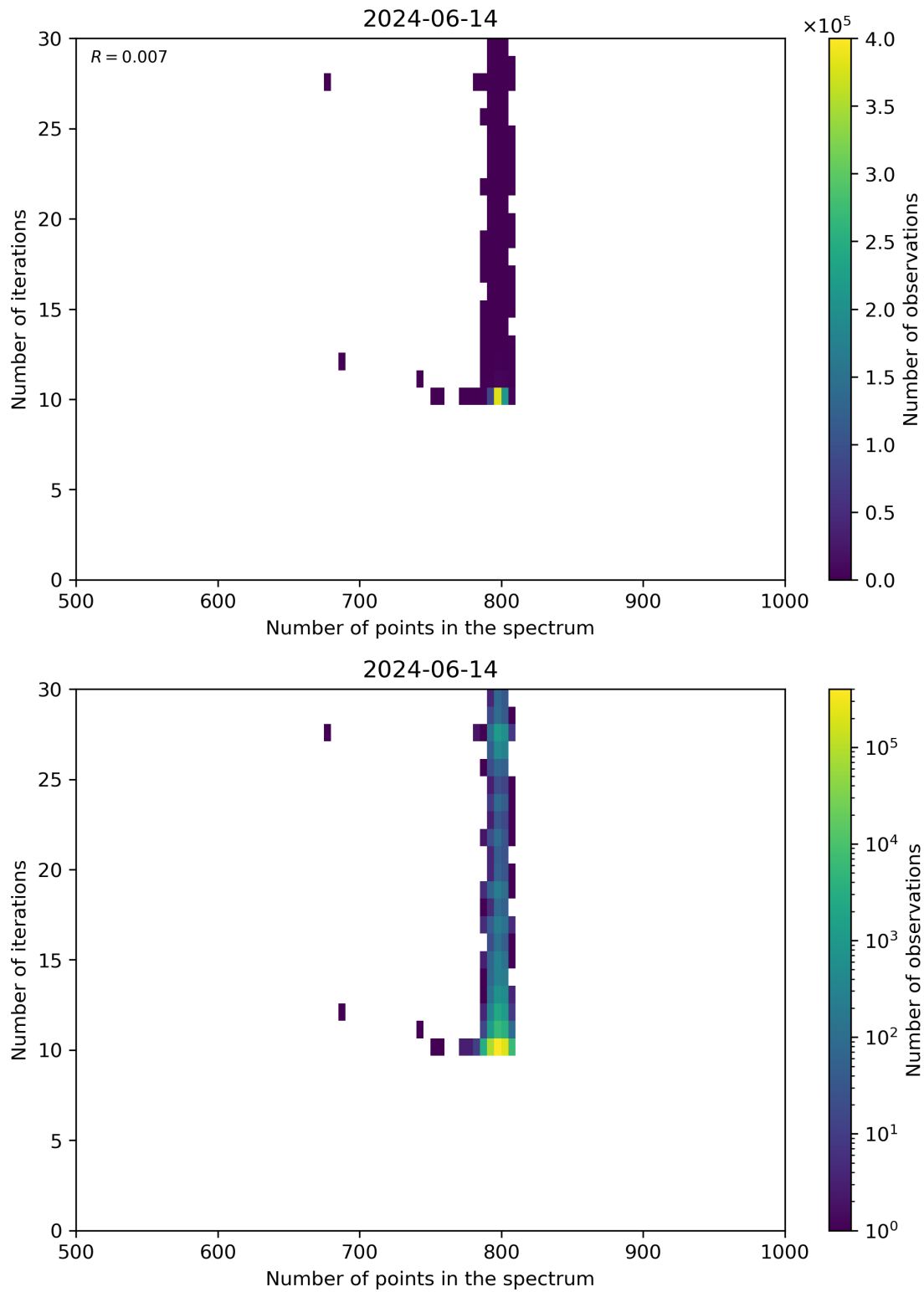
Figure 92: Scatter density plot of “Number of points in the spectrum” against “Number of iterations” for 2024-06-13 to 2024-06-15.
