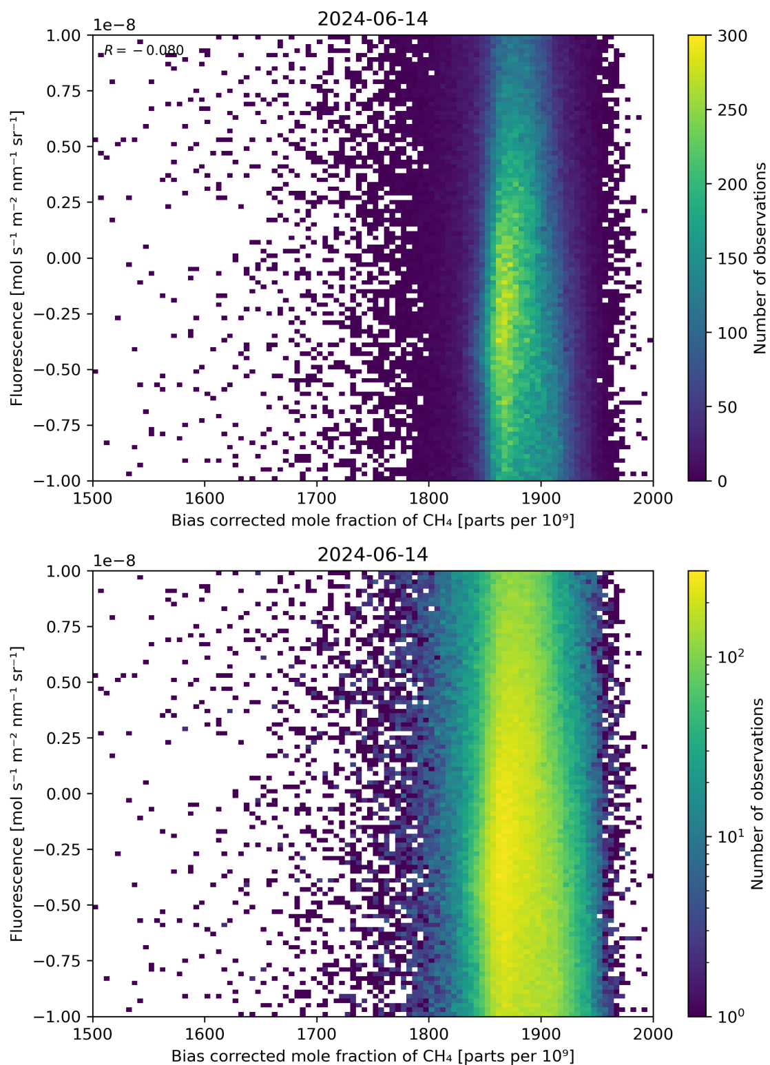
Figure 66: Scatter density plot of “Bias corrected mole fraction of \text{CH}_4 ” against “Fluorescence” for 2024-06-13 to 2024-06-15.
