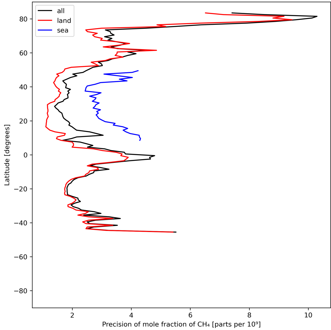
Figure 13: Zonal average of “Precision of mole fraction of CH 4 ” for 2024-06-13 to 2024-06-15.
