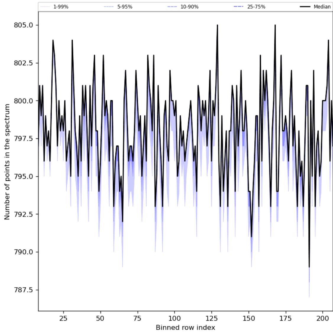
Figure 37: Along track statistics of “Number of points in the spectrum” for 2024-06-13 to 2024-06-15
