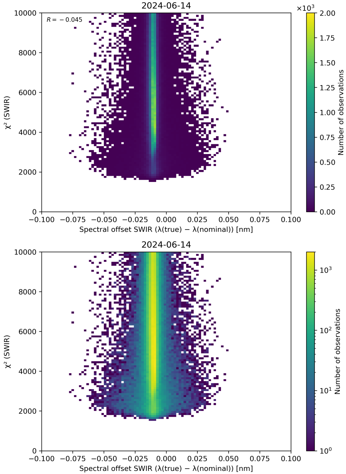
Figure 118: Scatter density plot of “Spectral offset SWIR ( \lambda(\text{true}) - \lambda(\text{nominal}) )” against “ \chi^2 (SWIR)” for 2024-06-13 to 2024-06-15.
