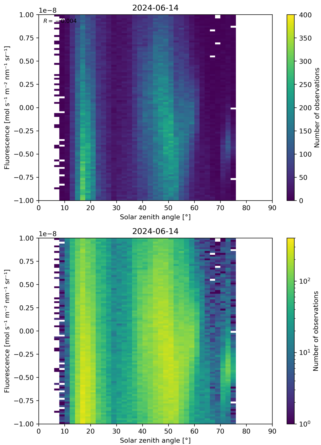
Figure 97: Scatter density plot of “Solar zenith angle” against “Fluorescence” for 2024-06-13 to 2024-06-15.
