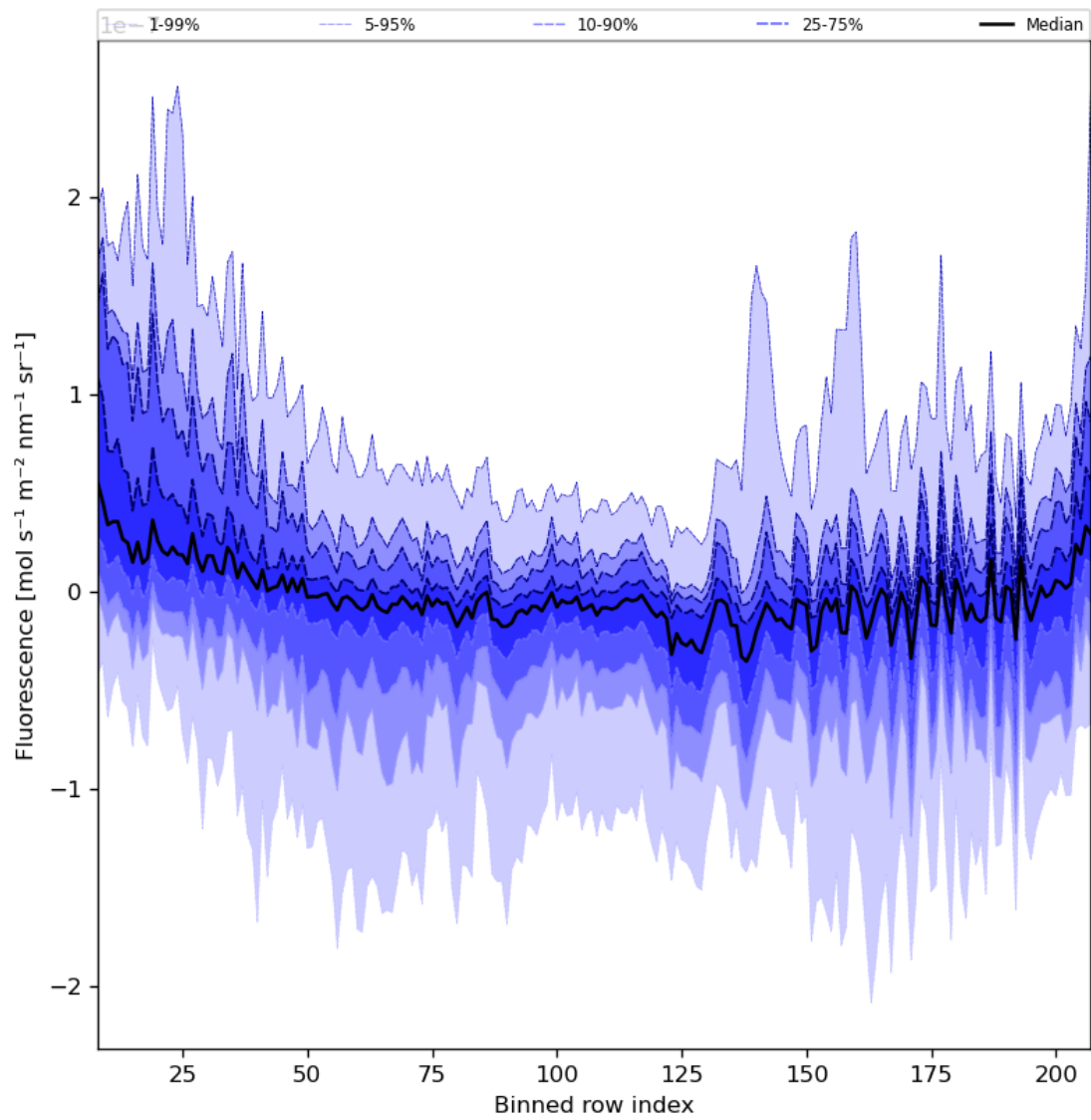
Figure 43: Along track statistics of “Fluorescence” for 2024-06-13 to 2024-06-15
