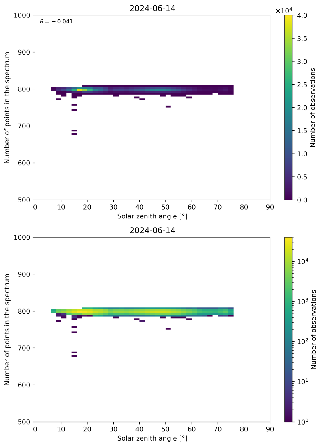
Figure 103: Scatter density plot of “Solar zenith angle” against “Number of points in the spectrum” for 2024-06-13 to 2024-06-15.
