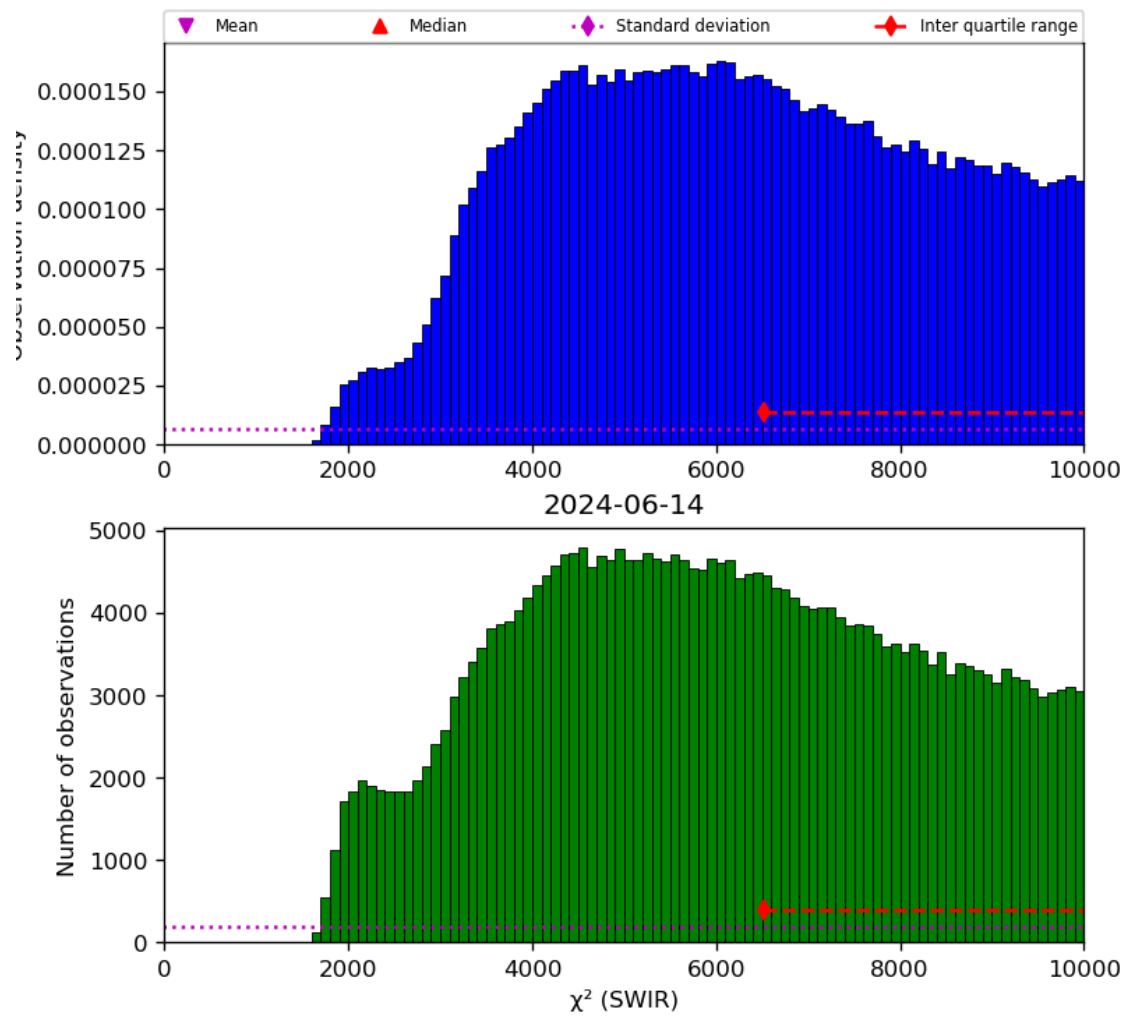
Figure 28: Histogram of “ \chi^2 (SWIR)” for 2024-06-13 to 2024-06-15
