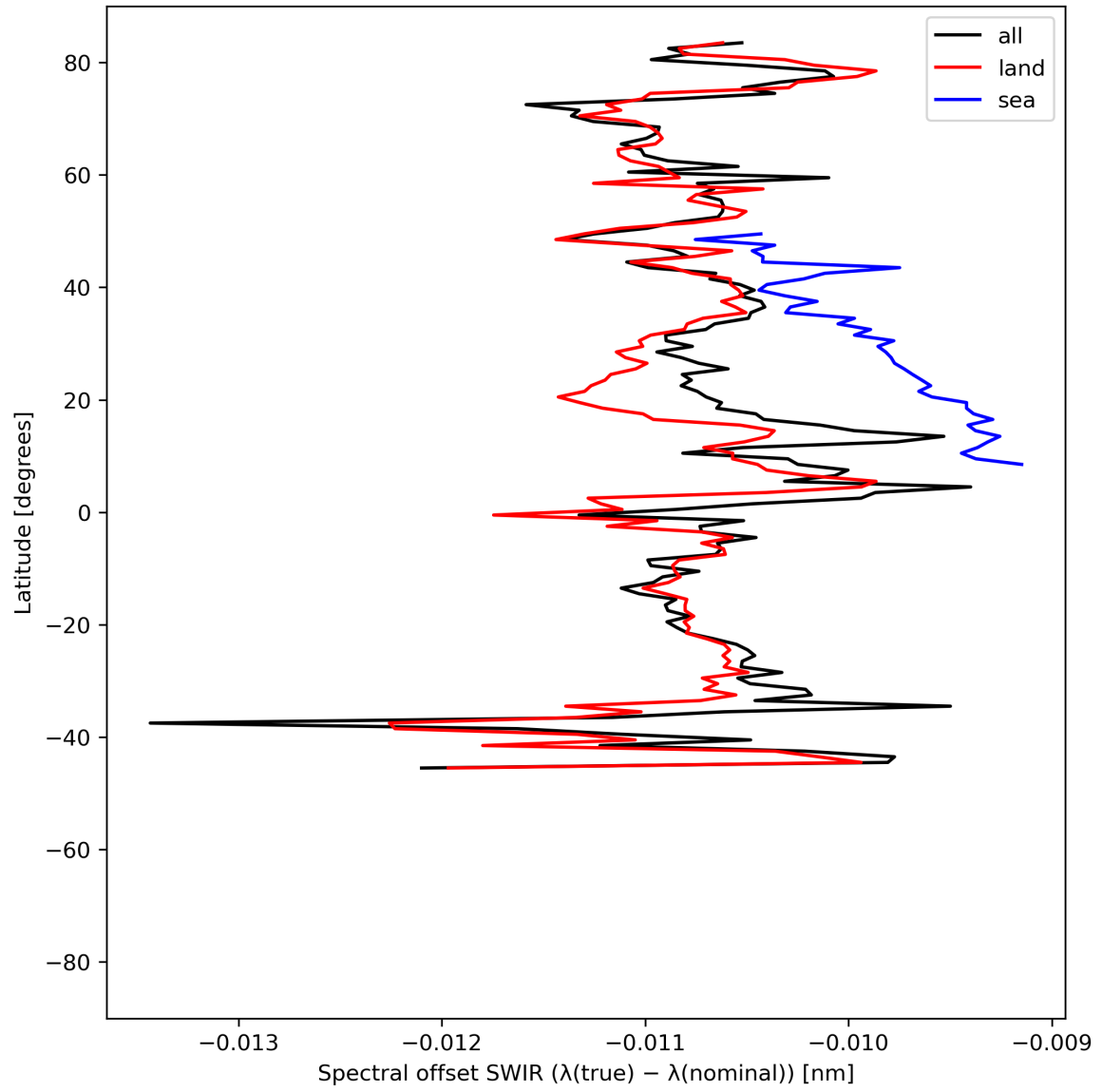
Figure 16: Zonal average of “Spectral offset SWIR ( \lambda(\text{true}) - \lambda(\text{nominal}) )” for 2024-06-13 to 2024-06-15.
