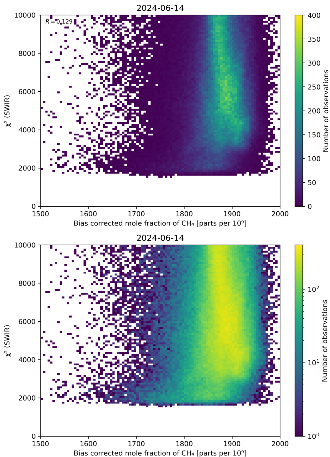
Figure 64: Scatter density plot of “Bias corrected mole fraction of \text{CH}_4 ” against “ \chi^2 (SWIR)” for 2024-06-13 to 2024-06-15.
