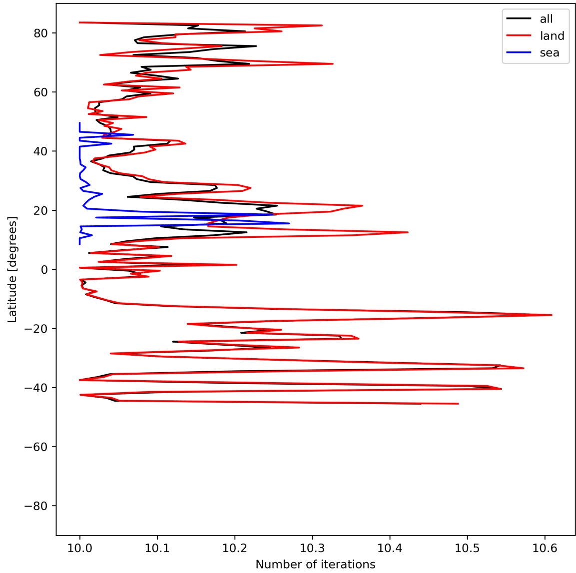
Figure 20: Zonal average of “Number of iterations” for 2024-06-13 to 2024-06-15.
