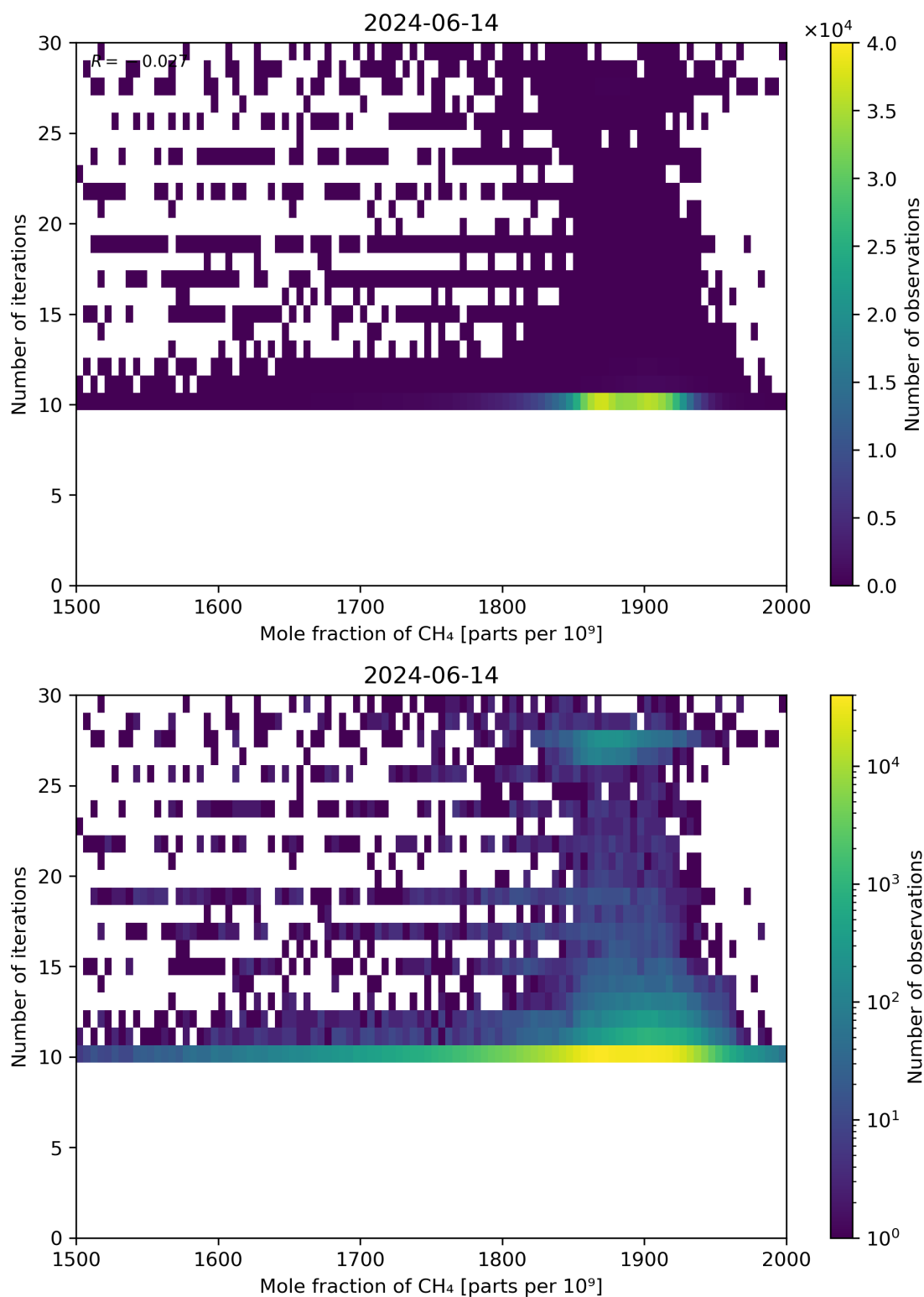
Figure 76: Scatter density plot of “Mole fraction of CH 4 ” against “Number of iterations” for 2024-06-13 to 2024-06-15.
