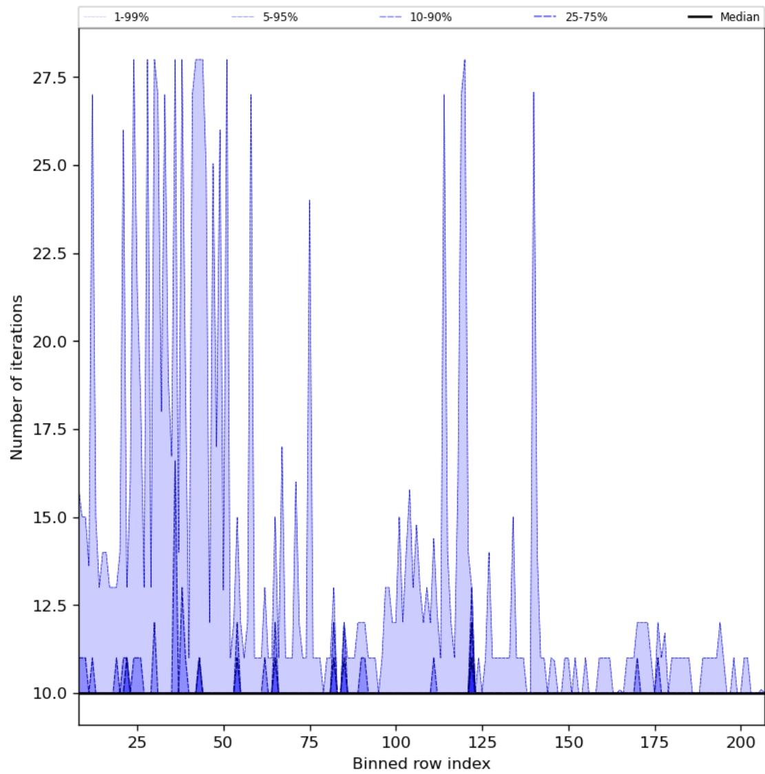
Figure 42: Along track statistics of “Number of iterations” for 2024-06-13 to 2024-06-15
