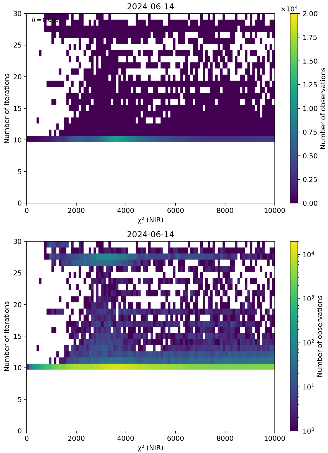
Figure 46: Scatter density plot of “ \chi^2 (NIR)” against “Number of iterations” for 2024-06-13 to 2024-06-15.
