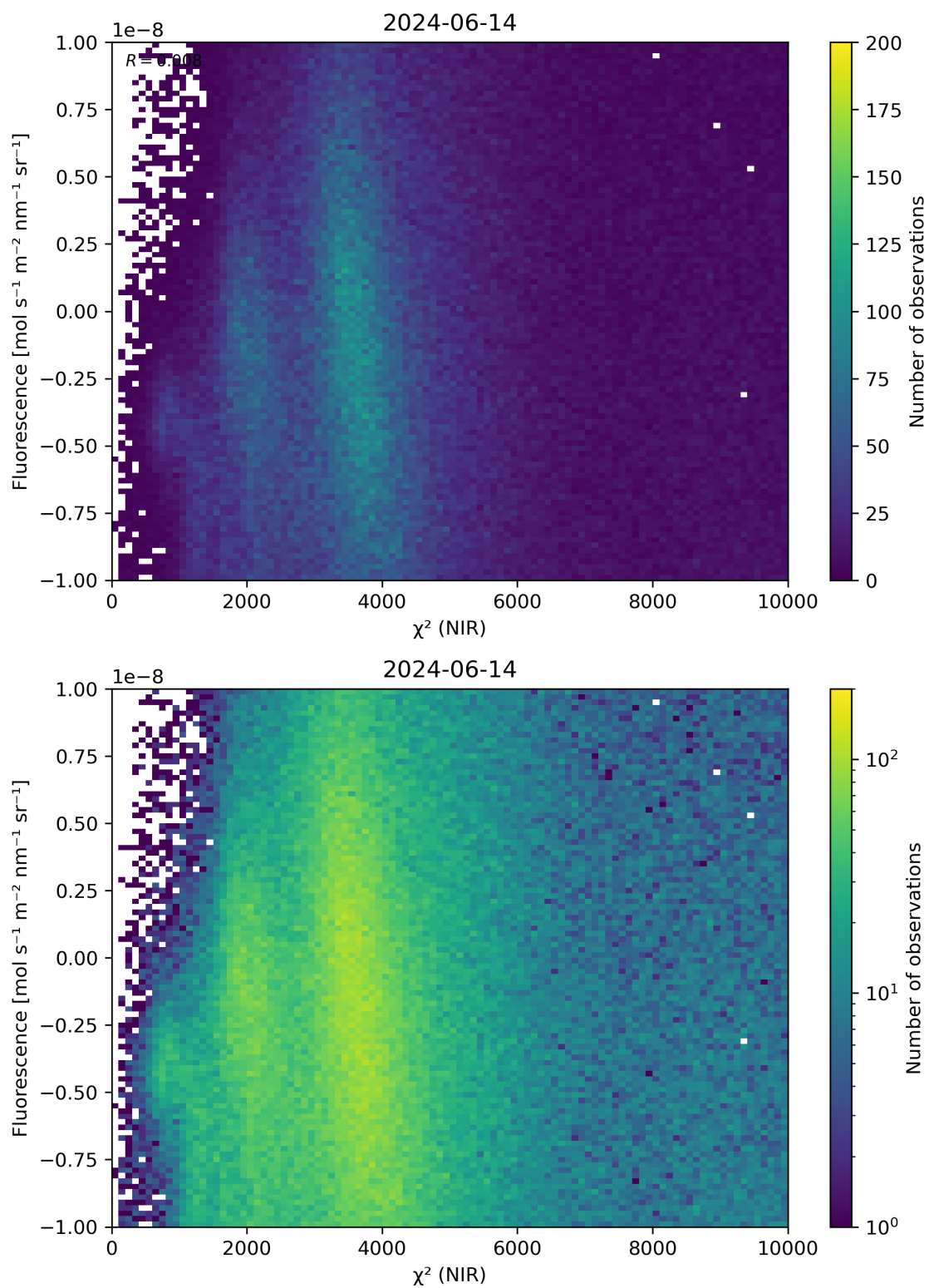
Figure 45: Scatter density plot of “ \chi^2 (NIR)” against “Fluorescence” for 2024-06-13 to 2024-06-15.
