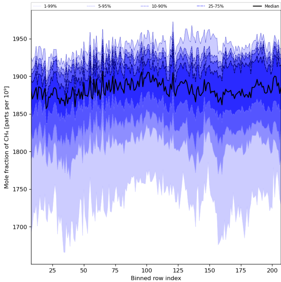
Figure 34: Along track statistics of “Mole fraction of CH 4 ” for 2024-06-13 to 2024-06-15
