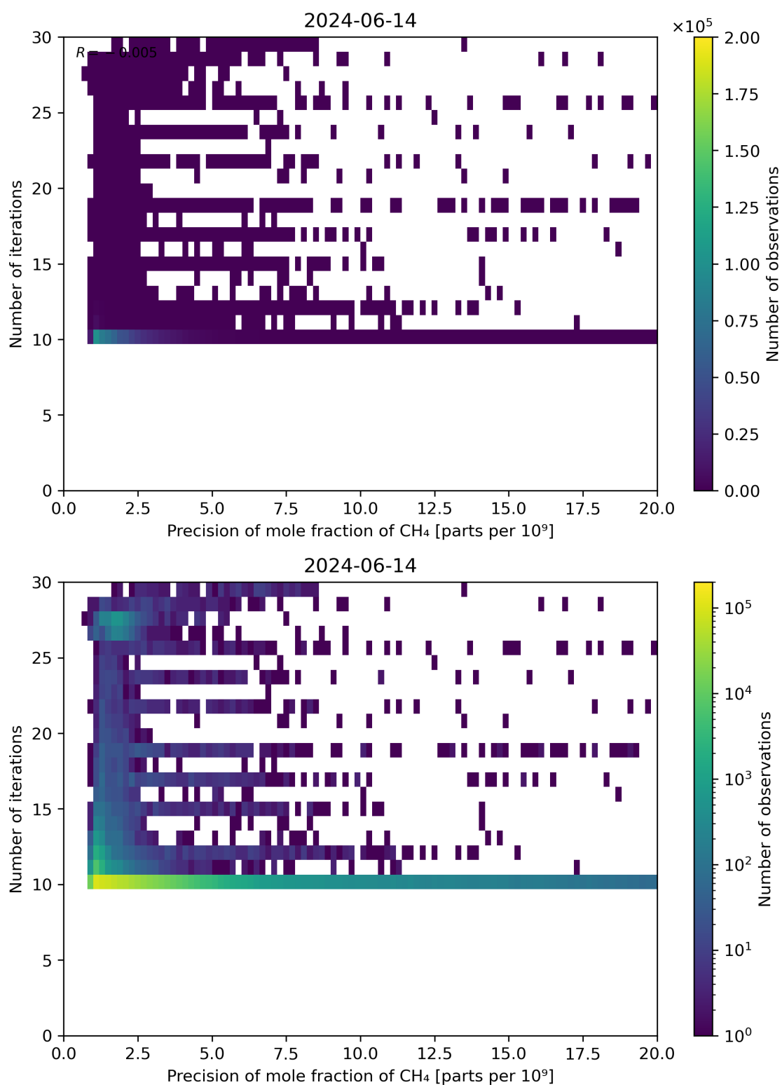
Figure 83: Scatter density plot of “Precision of mole fraction of CH 4 ” against “Number of iterations” for 2024-06-13 to 2024-06-15.
