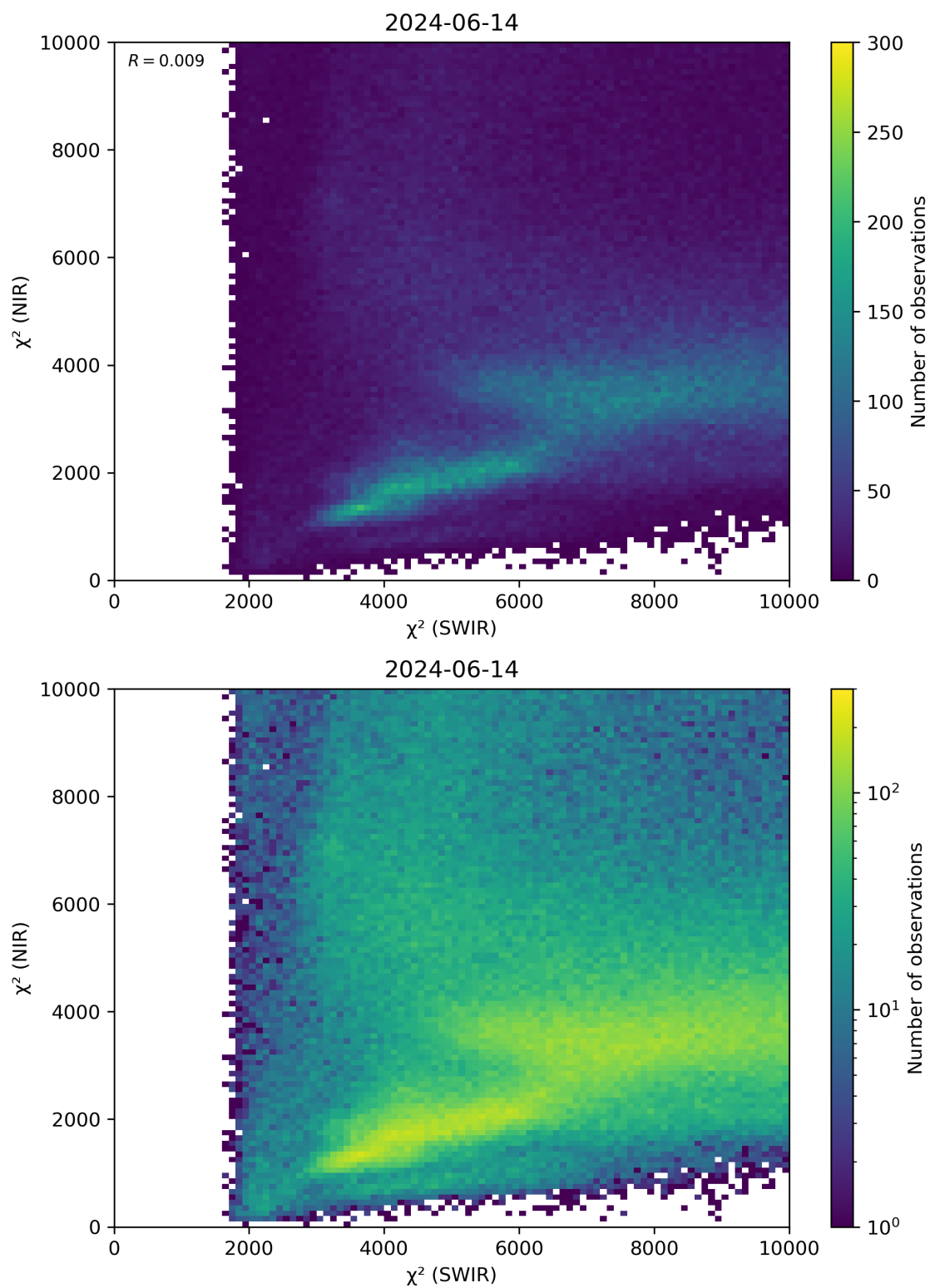
Figure 47: Scatter density plot of “ \chi^2 (SWIR)” against “ \chi^2 (NIR)” for 2024-06-13 to 2024-06-15.
