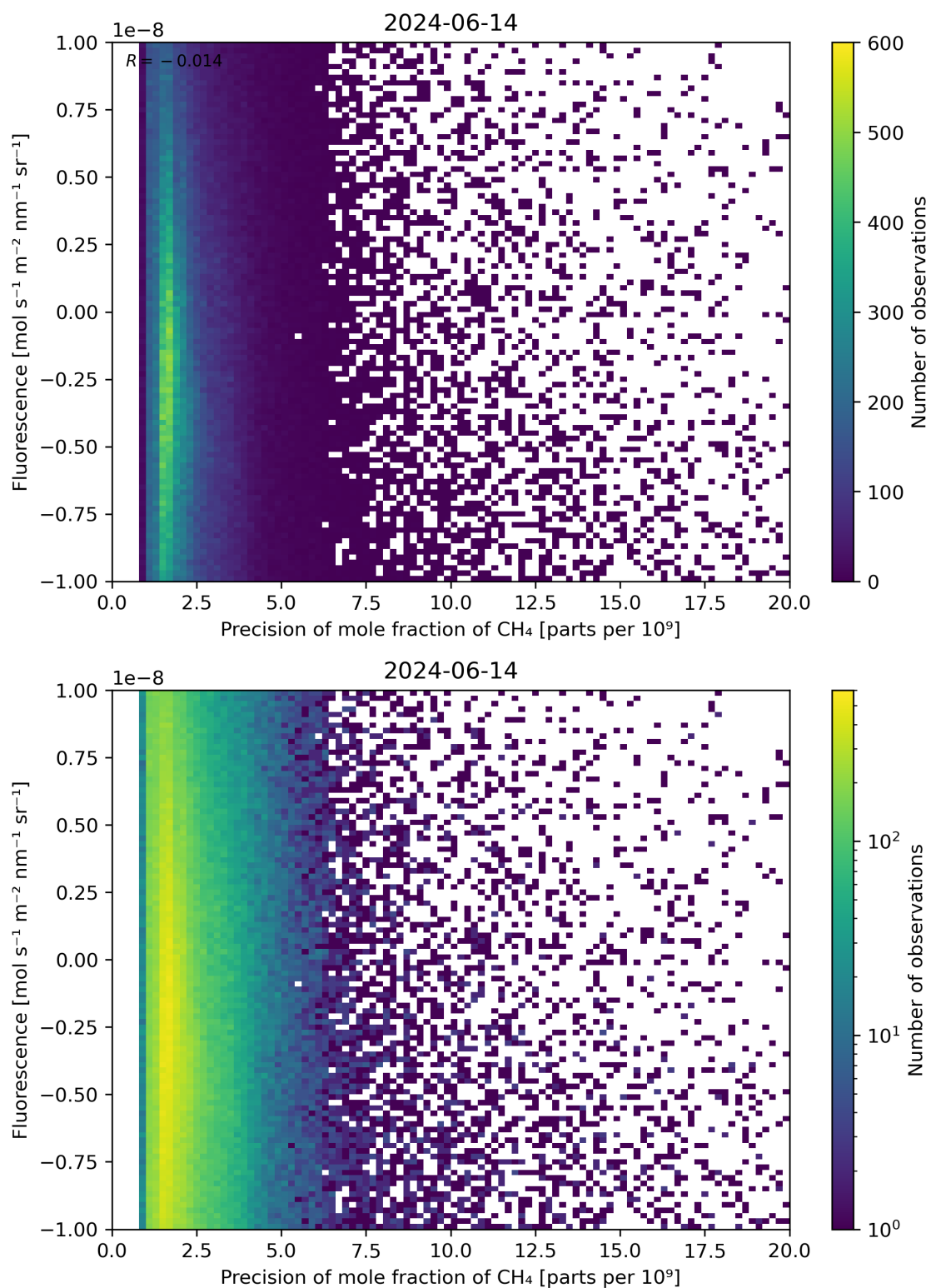
Figure 81: Scatter density plot of “Precision of mole fraction of \text{CH}_4 ” against “Fluorescence” for 2024-06-13 to 2024-06-15.
