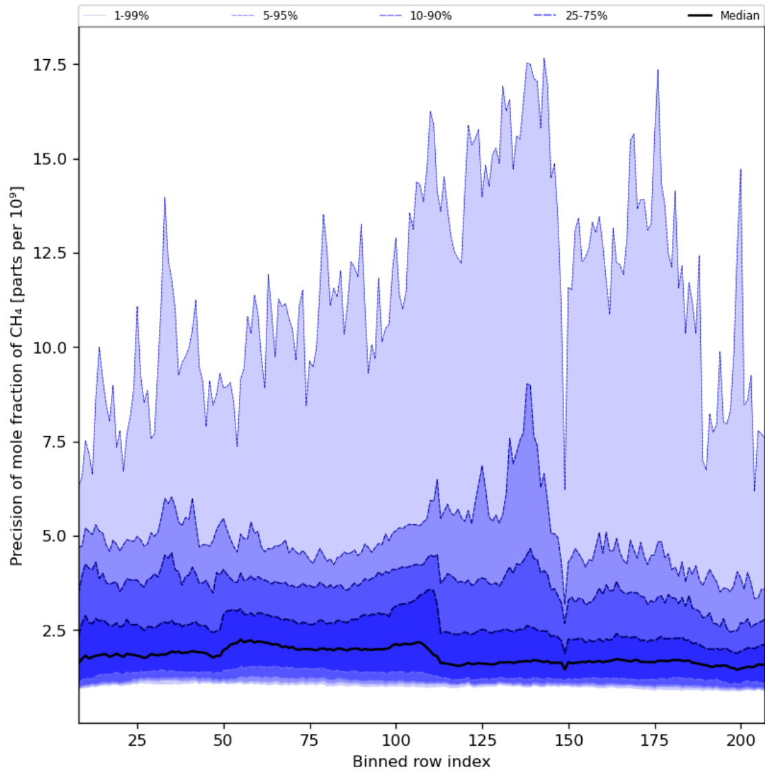
Figure 35: Along track statistics of “Precision of mole fraction of CH 4 ” for 2024-06-13 to 2024-06-15
