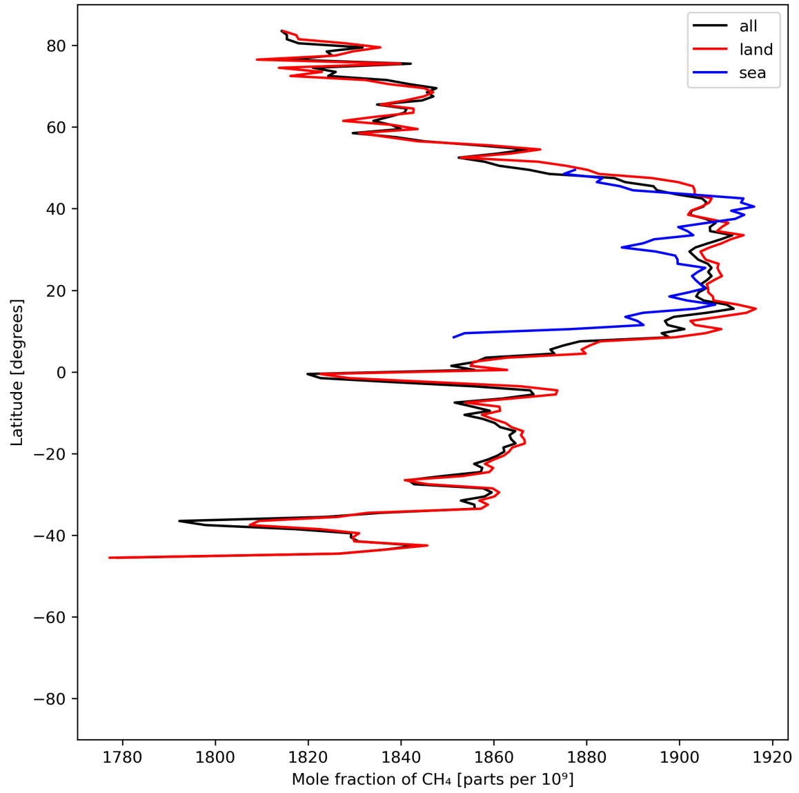
Figure 12: Zonal average of “Mole fraction of CH 4 ” for 2024-06-13 to 2024-06-15.
