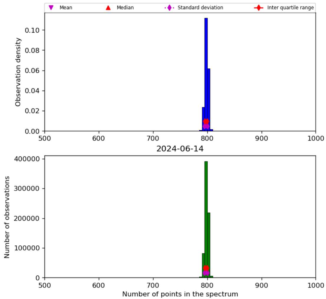
Figure 26: Histogram of “Number of points in the spectrum” for 2024-06-13 to 2024-06-15
