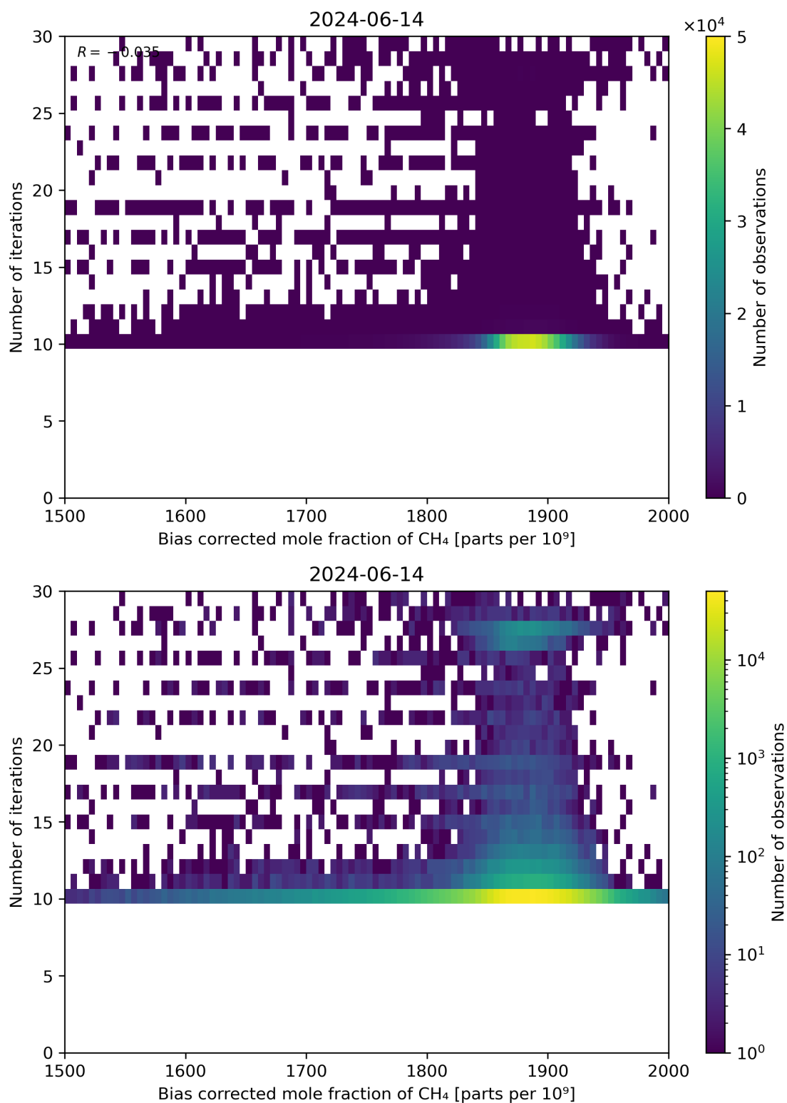
Figure 67: Scatter density plot of “Bias corrected mole fraction of CH 4 ” against “Number of iterations” for 2024-06-13 to 2024-06-15.
