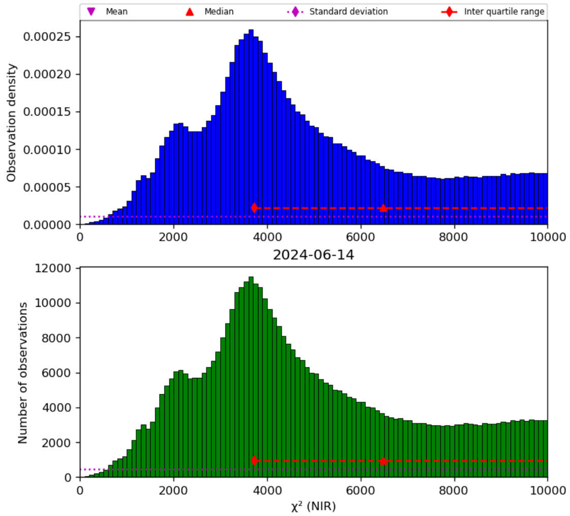
Figure 29: Histogram of “ \chi^2 (NIR)” for 2024-06-13 to 2024-06-15
