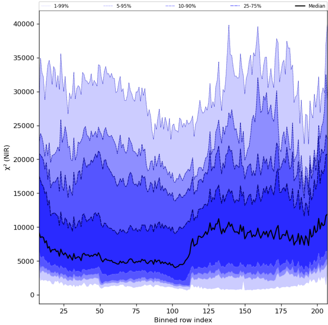
Figure 40: Along track statistics of “ \chi^2 (NIR)” for 2024-06-13 to 2024-06-15
