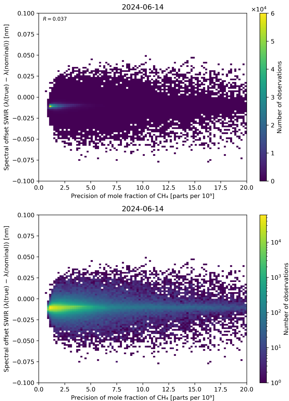
Figure 85: Scatter density plot of “Precision of mole fraction of CH 4 ” against “Spectral offset SWIR ( \lambda(\text{true}) - \lambda(\text{nominal}) )” for 2024-06-13 to 2024-06-15.
