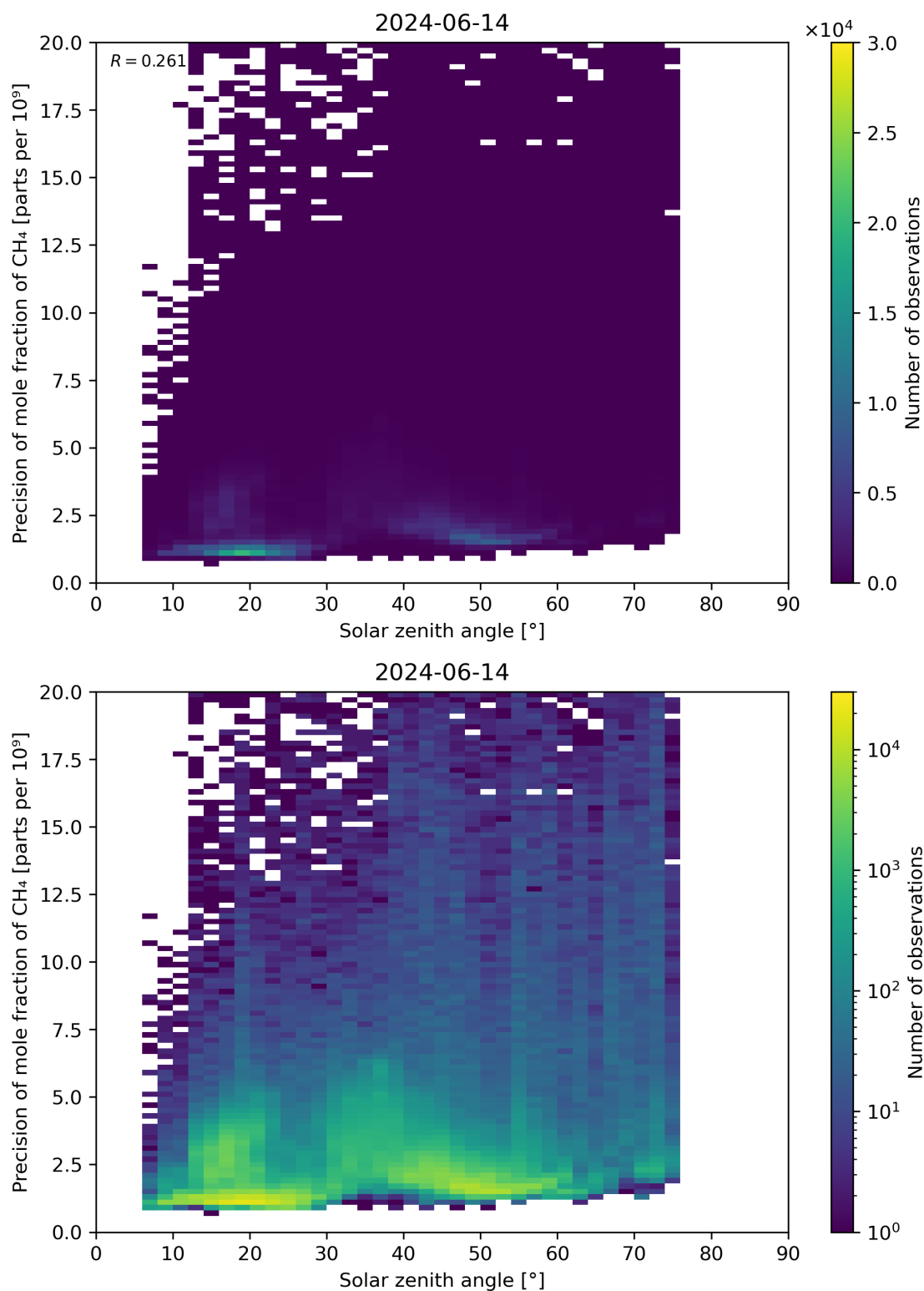
Figure 101: Scatter density plot of “Solar zenith angle” against “Precision of mole fraction of CH 4 ” for 2024-06-13 to 2024-06-15.
