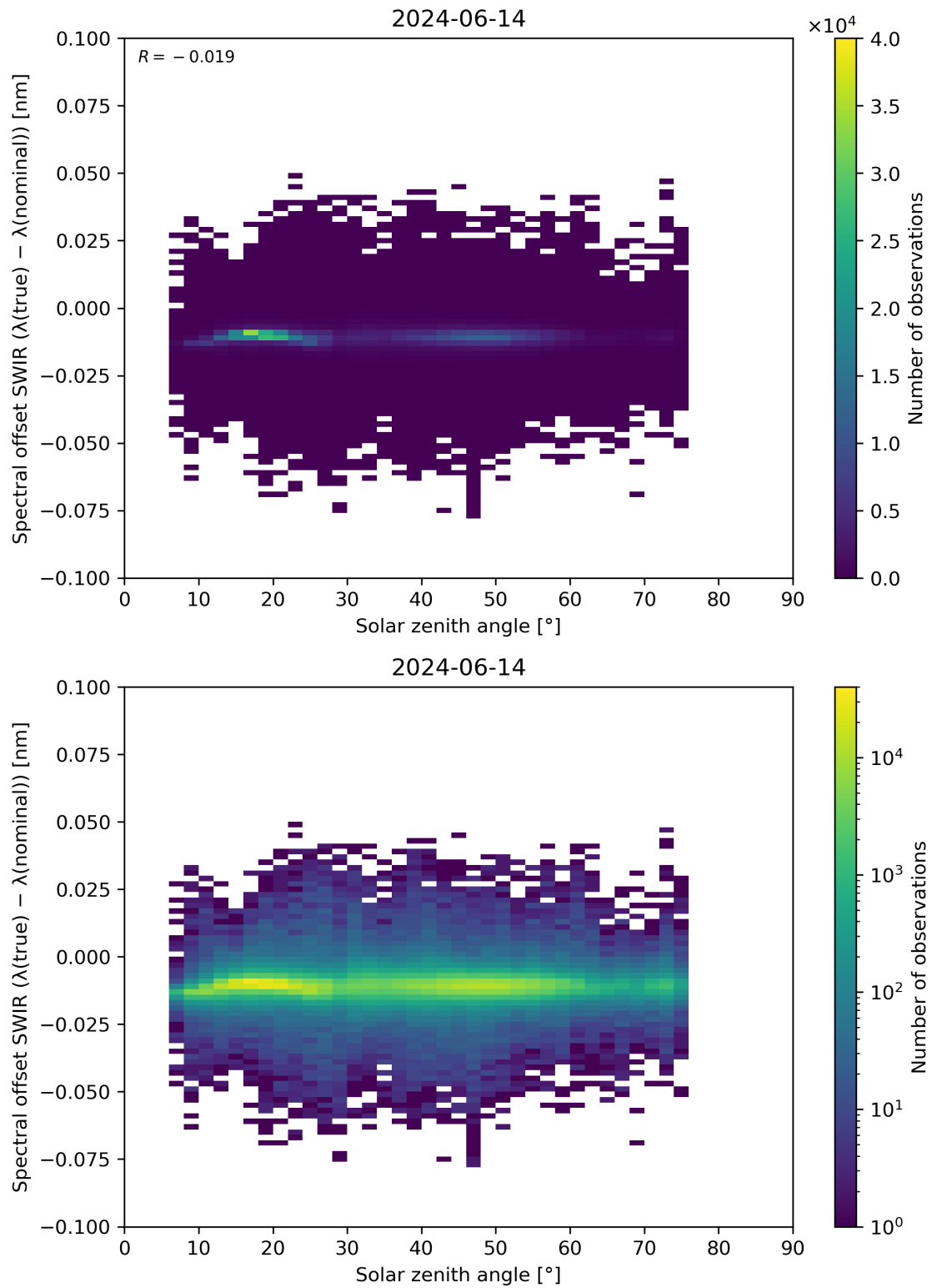
Figure 104: Scatter density plot of “Solar zenith angle” against “Spectral offset SWIR ( \lambda(\text{true}) - \lambda(\text{nominal}) )” for 2024-06-13 to 2024-06-15.
