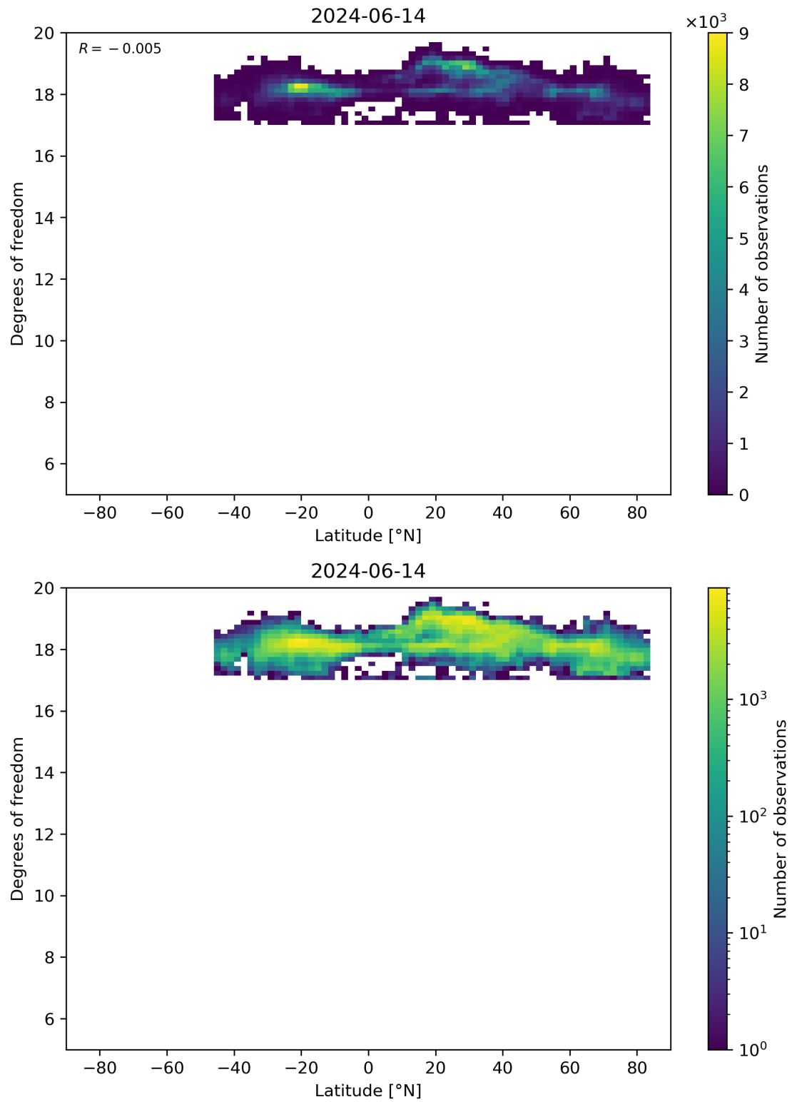
Figure 55: Scatter density plot of “Latitude” against “Degrees of freedom” for 2024-06-13 to 2024-06-15.
