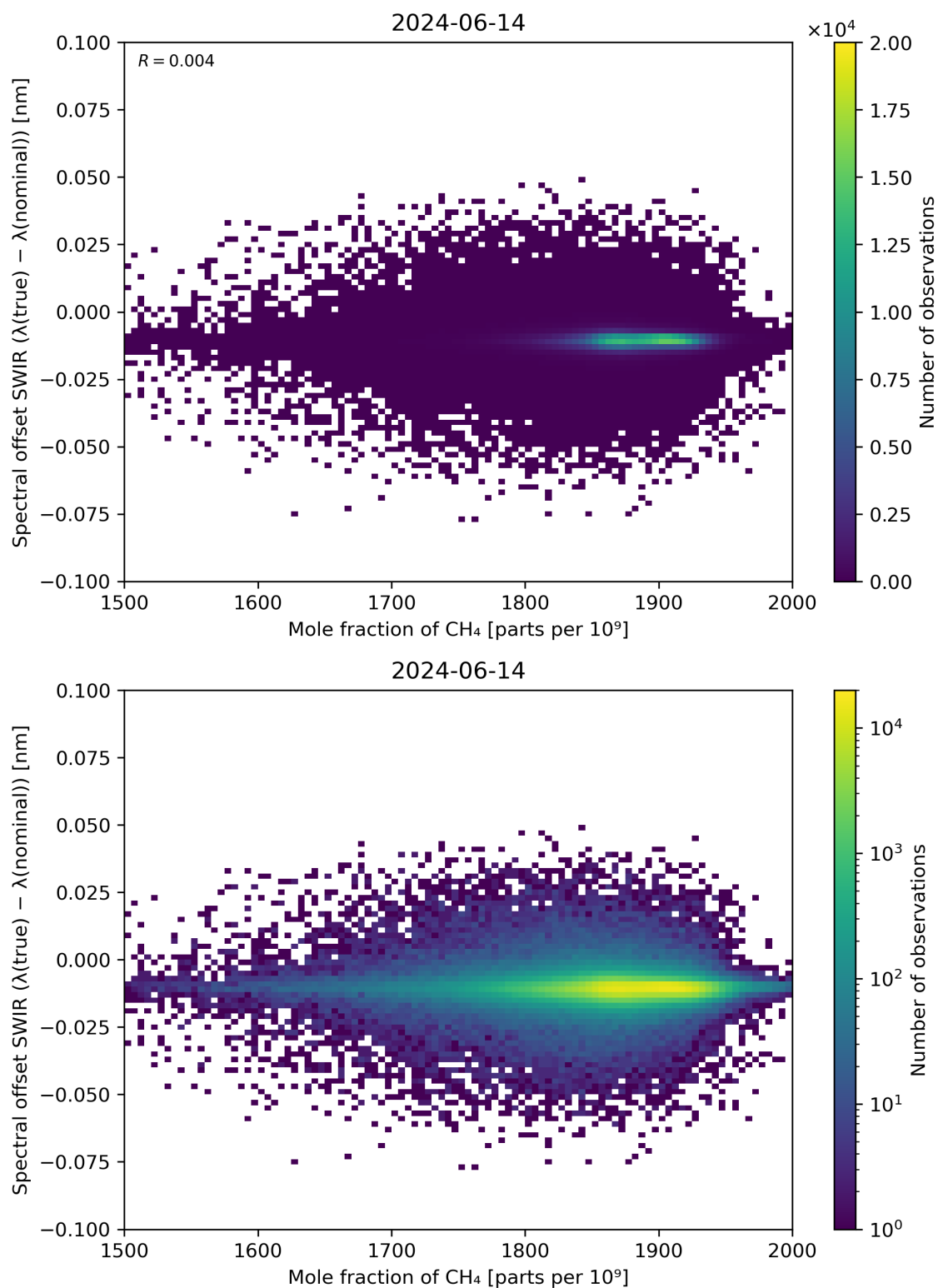
Figure 86: Scatter density plot of “Mole fraction of CH 4 ” against “Spectral offset SWIR ( \lambda(\text{true}) - \lambda(\text{nominal}) )” for 2024-06-13 to 2024-06-15.
