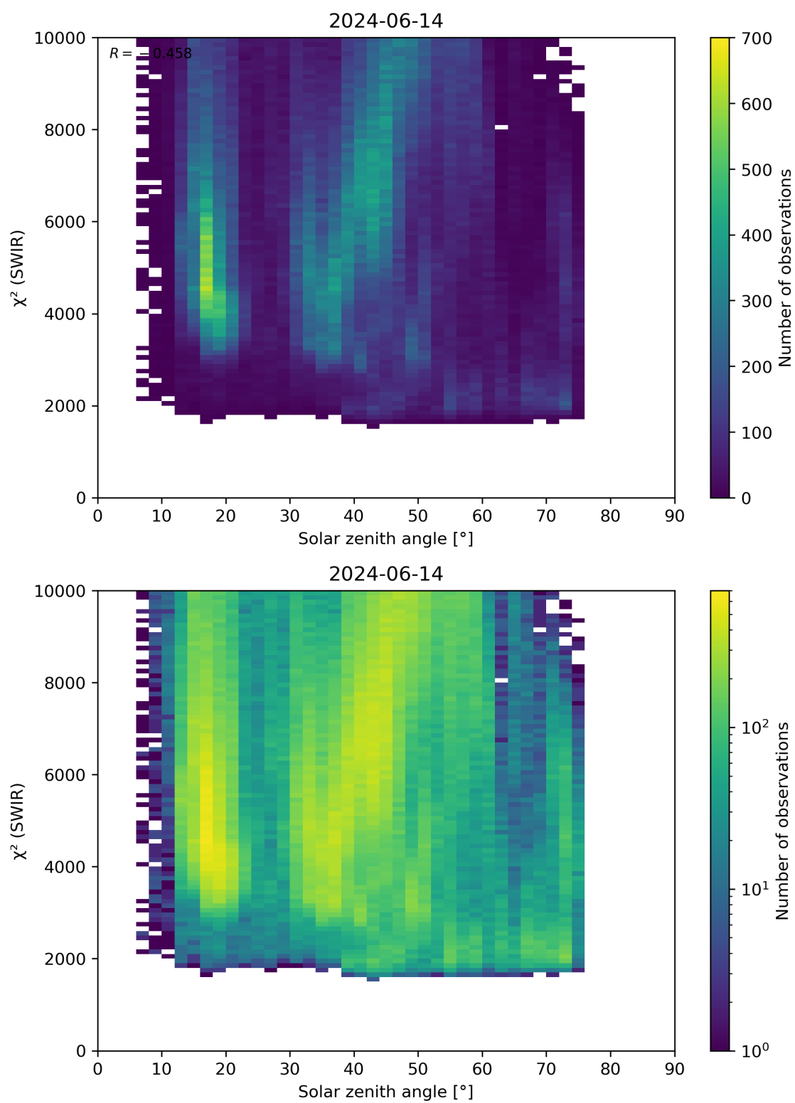
Figure 95: Scatter density plot of “Solar zenith angle” against “ \chi^2 (SWIR)” for 2024-06-13 to 2024-06-15.
