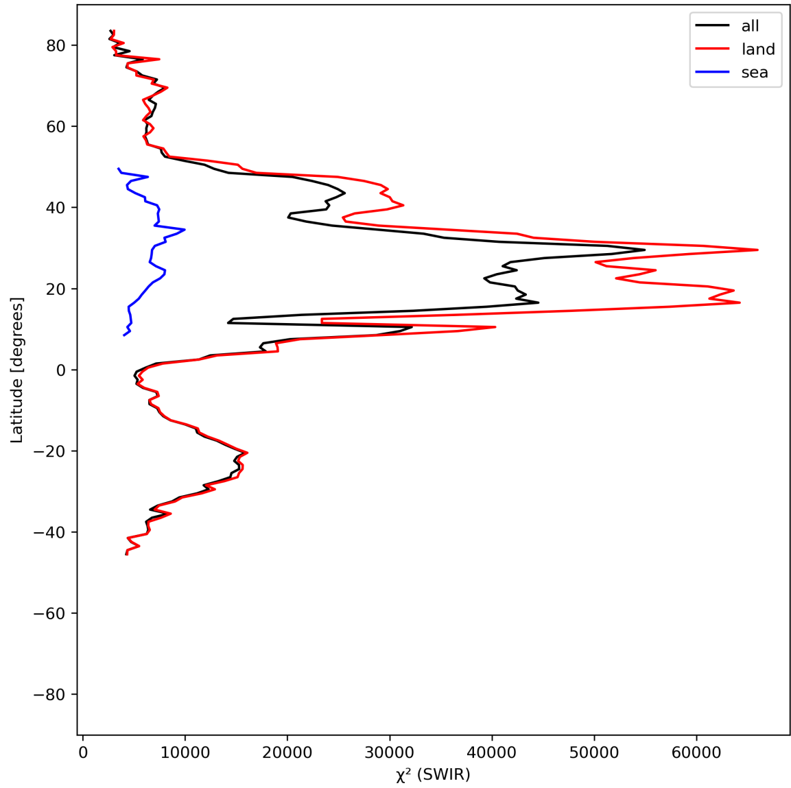
Figure 17: Zonal average of “ \chi^2 (SWIR)” for 2024-06-13 to 2024-06-15.
