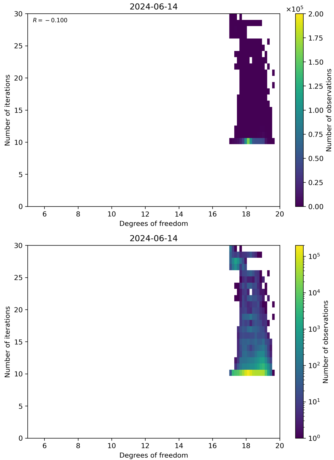
Figure 52: Scatter density plot of “Degrees of freedom” against “Number of iterations” for 2024-06-13 to 2024-06-15.
