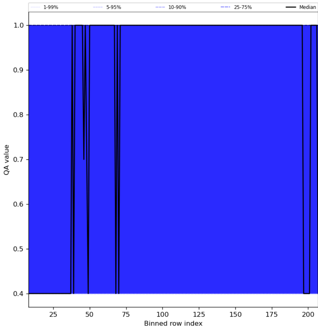
Figure 33: Along track statistics of “QA value” for 2024-06-13 to 2024-06-15
