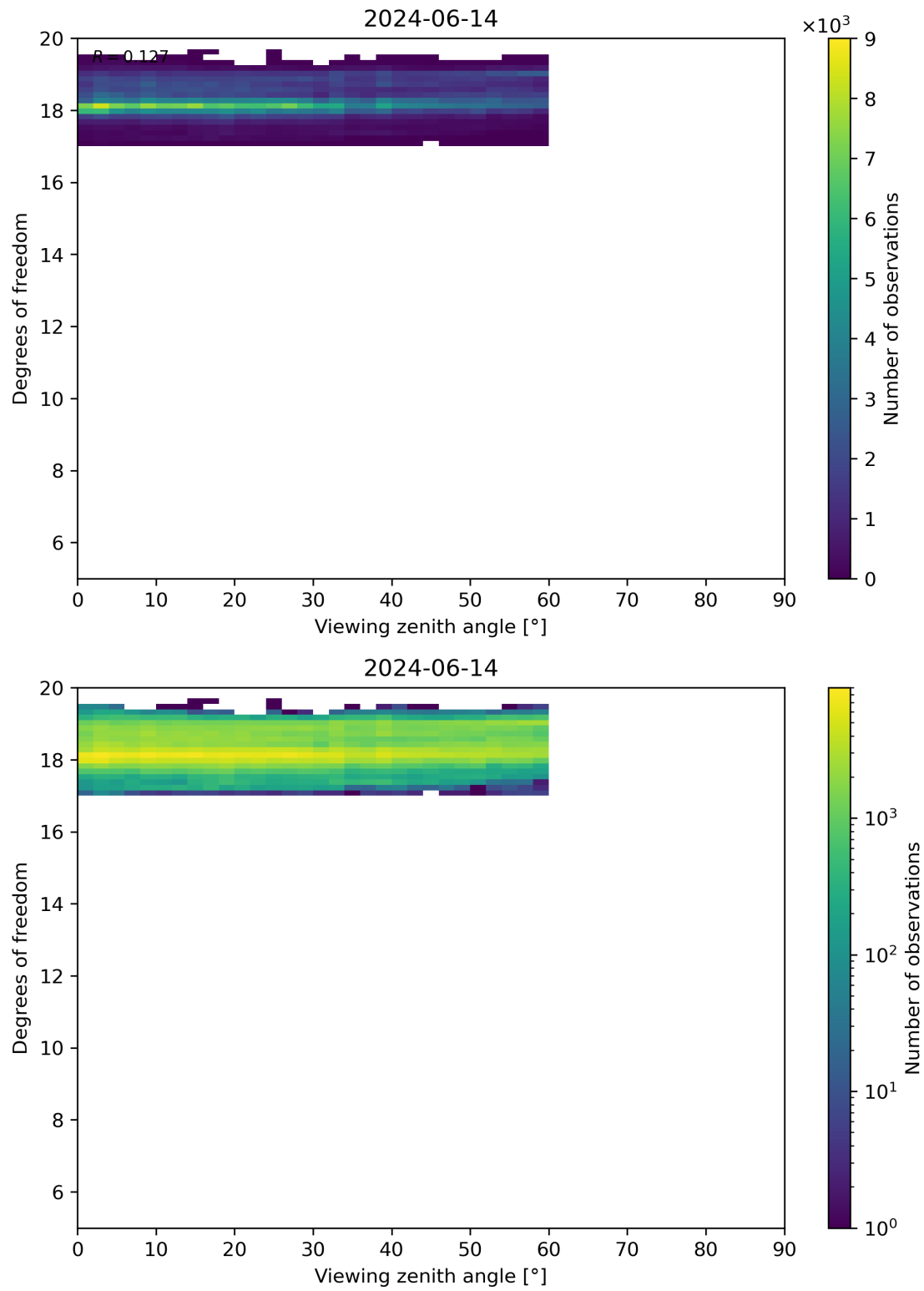
Figure 107: Scatter density plot of “Viewing zenith angle” against “Degrees of freedom” for 2024-06-13 to 2024-06-15.
