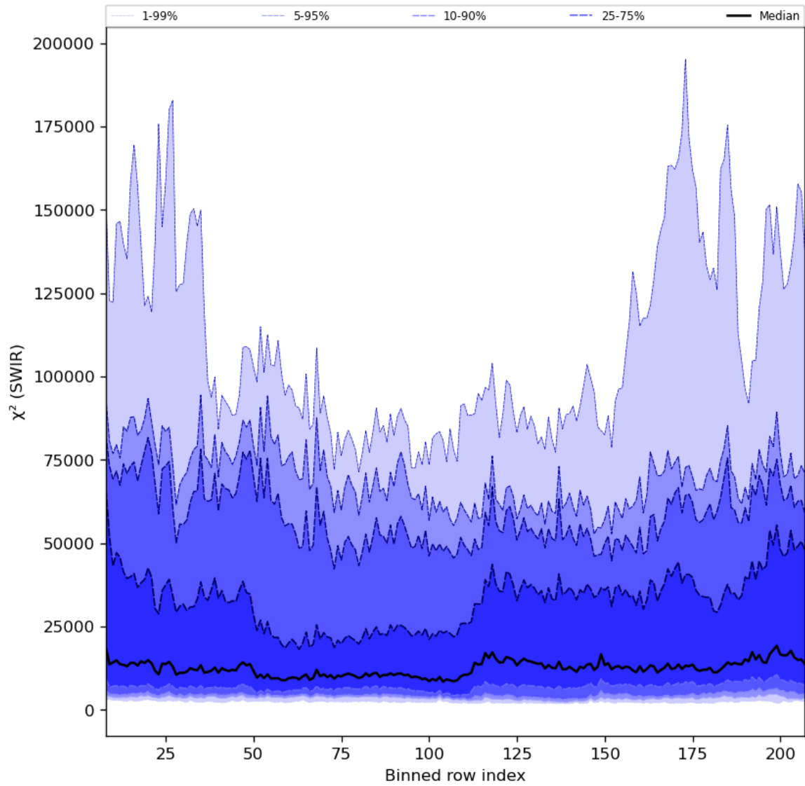
Figure 39: Along track statistics of " \chi^2 (SWIR)" for 2024-06-13 to 2024-06-15
