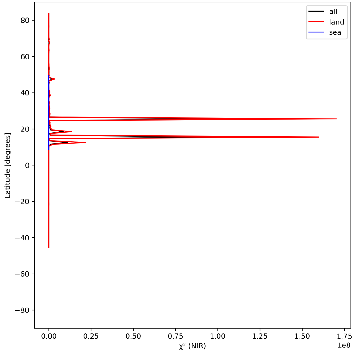
Figure 18: Zonal average of “ \chi^2 (NIR)” for 2024-06-13 to 2024-06-15.
