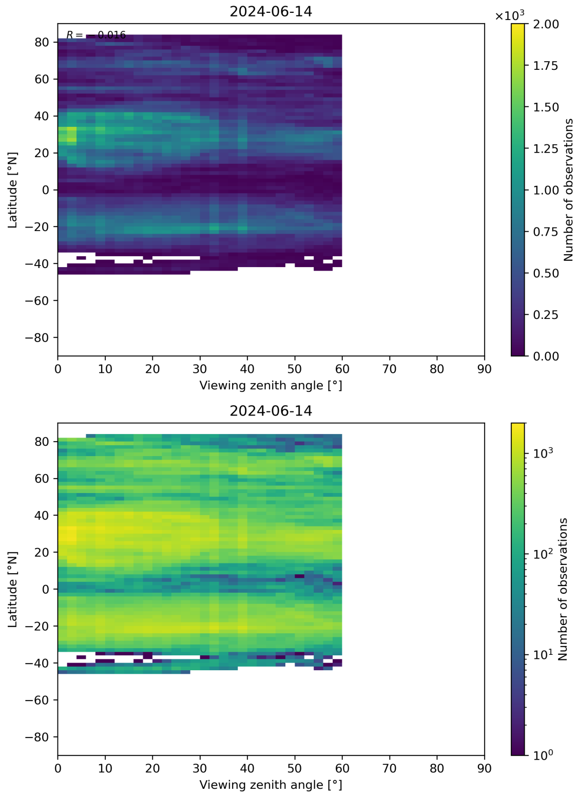
Figure 109: Scatter density plot of “Viewing zenith angle” against “Latitude” for 2024-06-13 to 2024-06-15.
