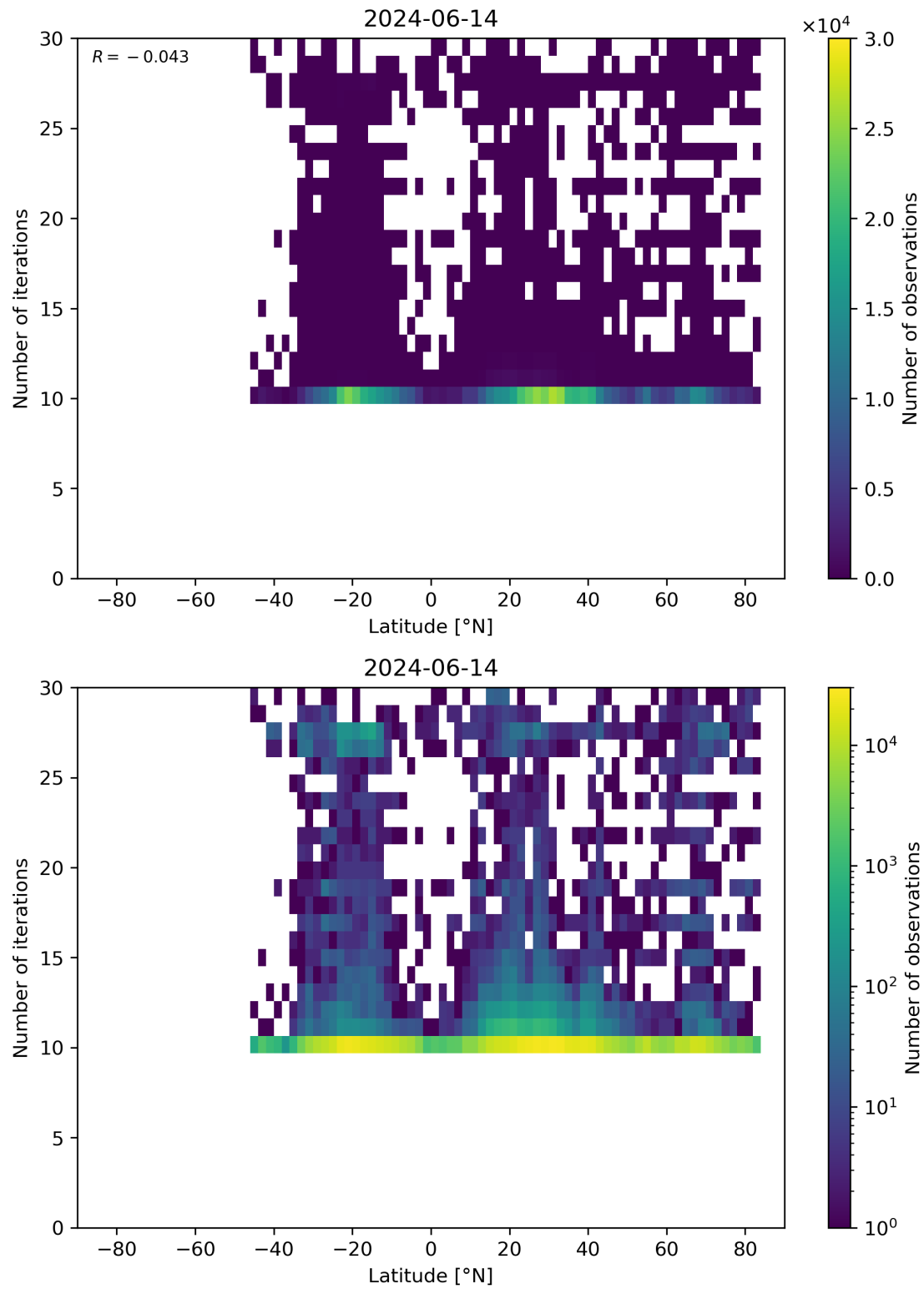
Figure 60: Scatter density plot of “Latitude” against “Number of iterations” for 2024-06-13 to 2024-06-15.
