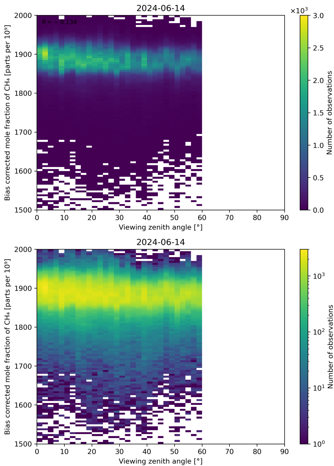
Figure 111: Scatter density plot of “Viewing zenith angle” against “Bias corrected mole fraction of CH 4 ” for 2024-06-13 to 2024-06-15.
