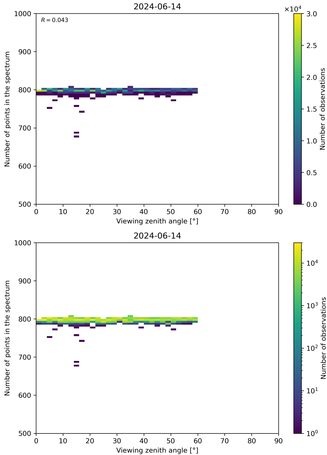
Figure 114: Scatter density plot of “Viewing zenith angle” against “Number of points in the spectrum” for 2024-06-13 to 2024-06-15.
