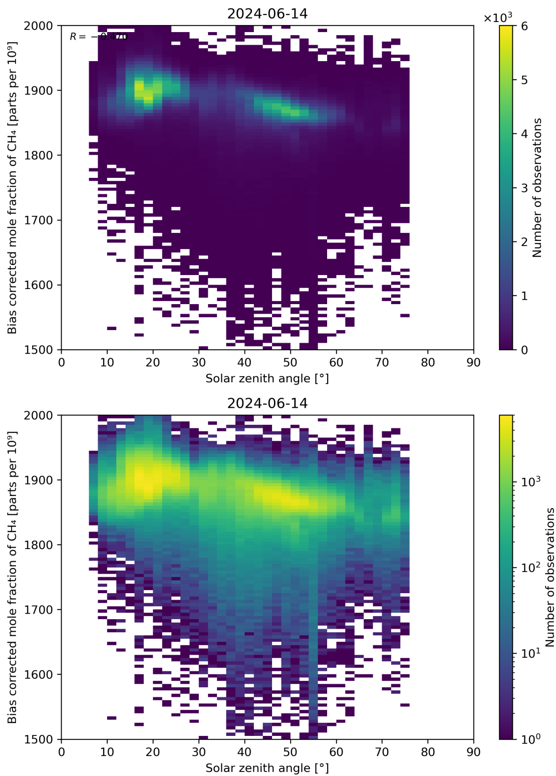
Figure 100: Scatter density plot of “Solar zenith angle” against “Bias corrected mole fraction of CH 4 ” for 2024-06-13 to 2024-06-15.
