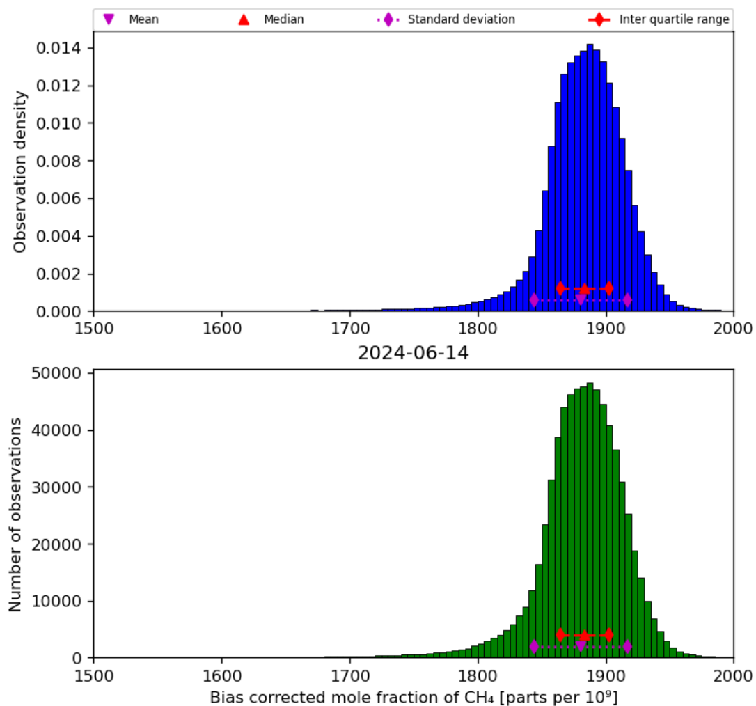
Figure 25: Histogram of “Bias corrected mole fraction of CH 4 ” for 2024-06-13 to 2024-06-15
