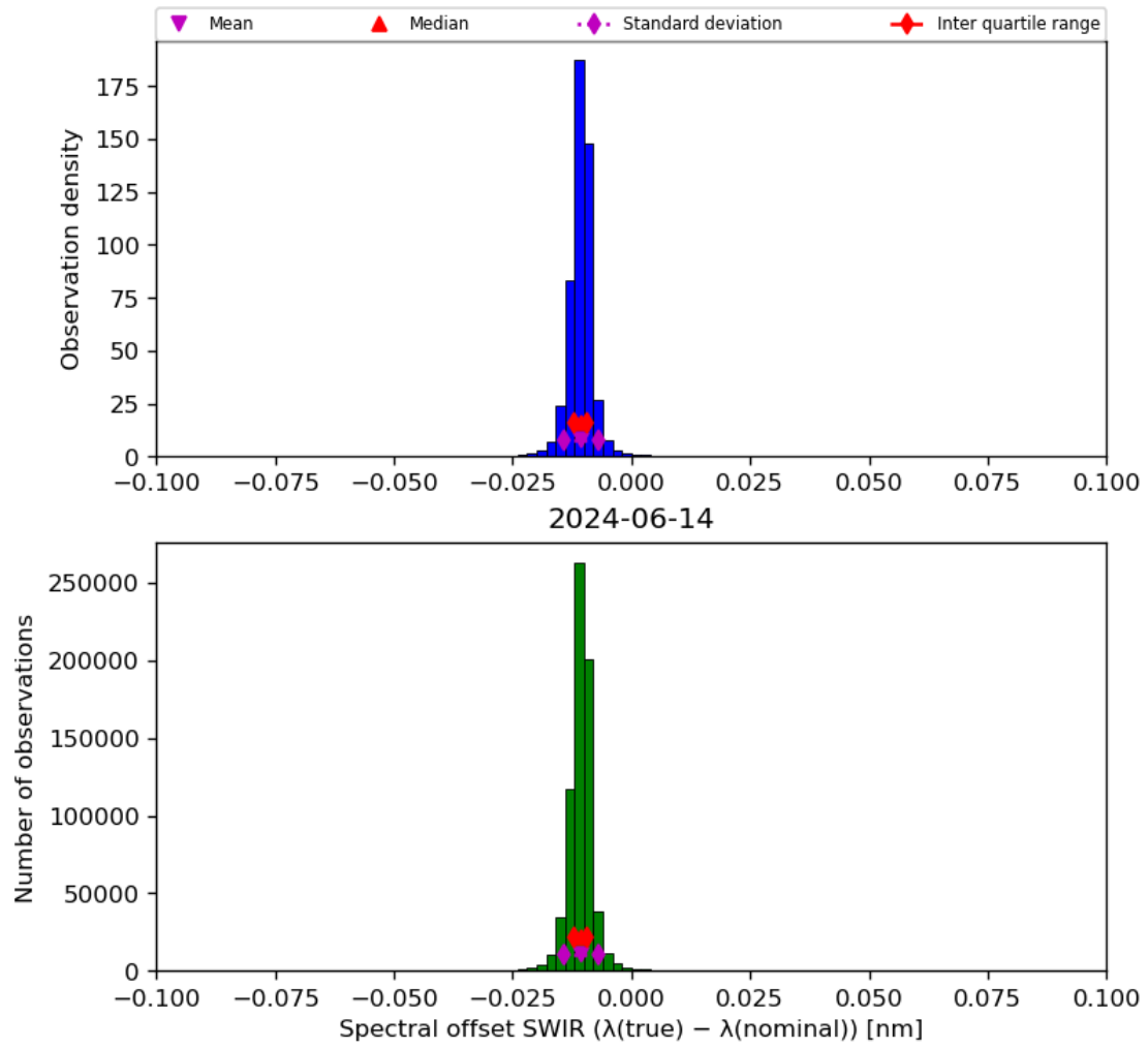
Figure 27: Histogram of “Spectral offset SWIR ( \lambda(\text{true}) - \lambda(\text{nominal}) )” for 2024-06-13 to 2024-06-15
