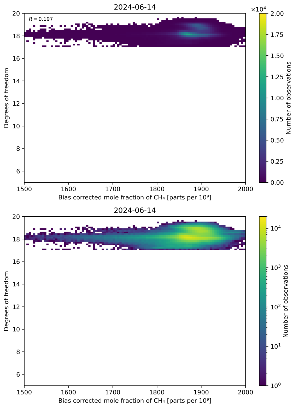
Figure 65: Scatter density plot of “Bias corrected mole fraction of CH 4 ” against “Degrees of freedom” for 2024-06-13 to 2024-06-15.
