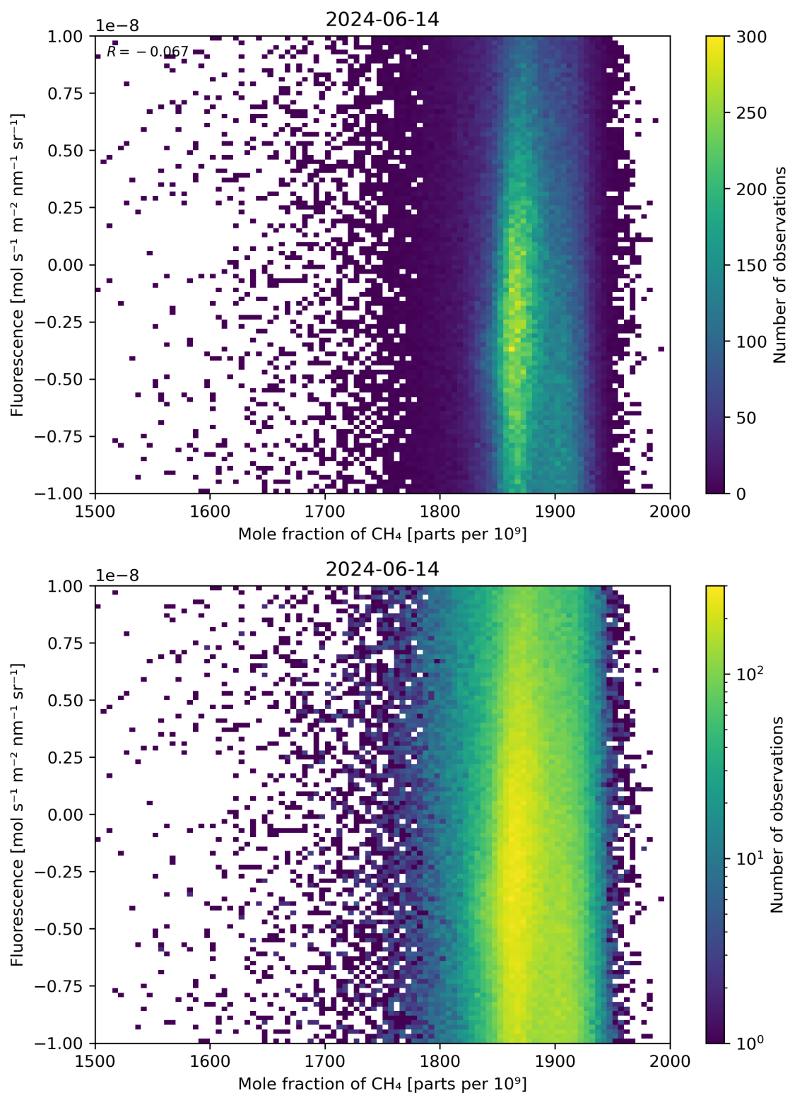
Figure 73: Scatter density plot of “Mole fraction of \text{CH}_4 ” against “Fluorescence” for 2024-06-13 to 2024-06-15.
