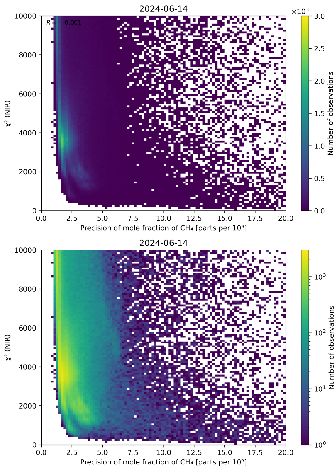
Figure 78: Scatter density plot of “Precision of mole fraction of CH 4 ” against “ \chi^2 (NIR)” for 2024-06-13 to 2024-06-15.
