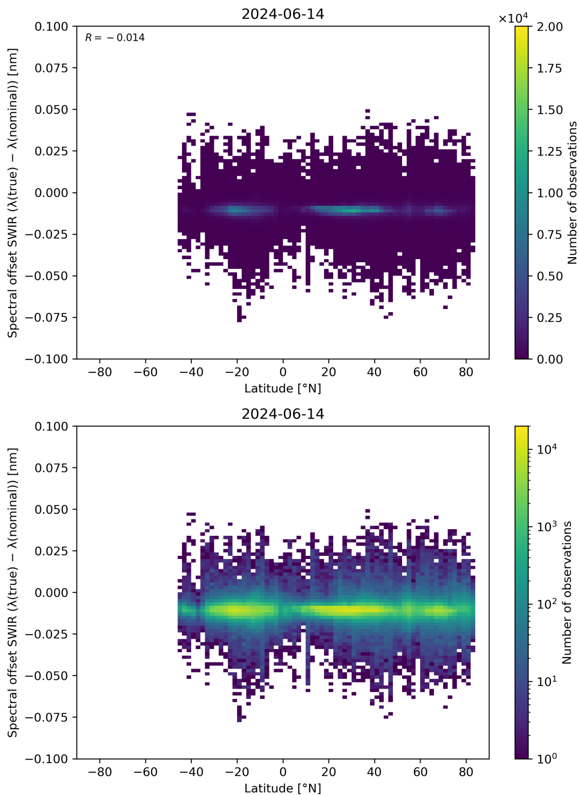
Figure 62: Scatter density plot of “Latitude” against “Spectral offset SWIR ( \lambda(\text{true}) - \lambda(\text{nominal}) )” for 2024-06-13 to 2024-06-15.
