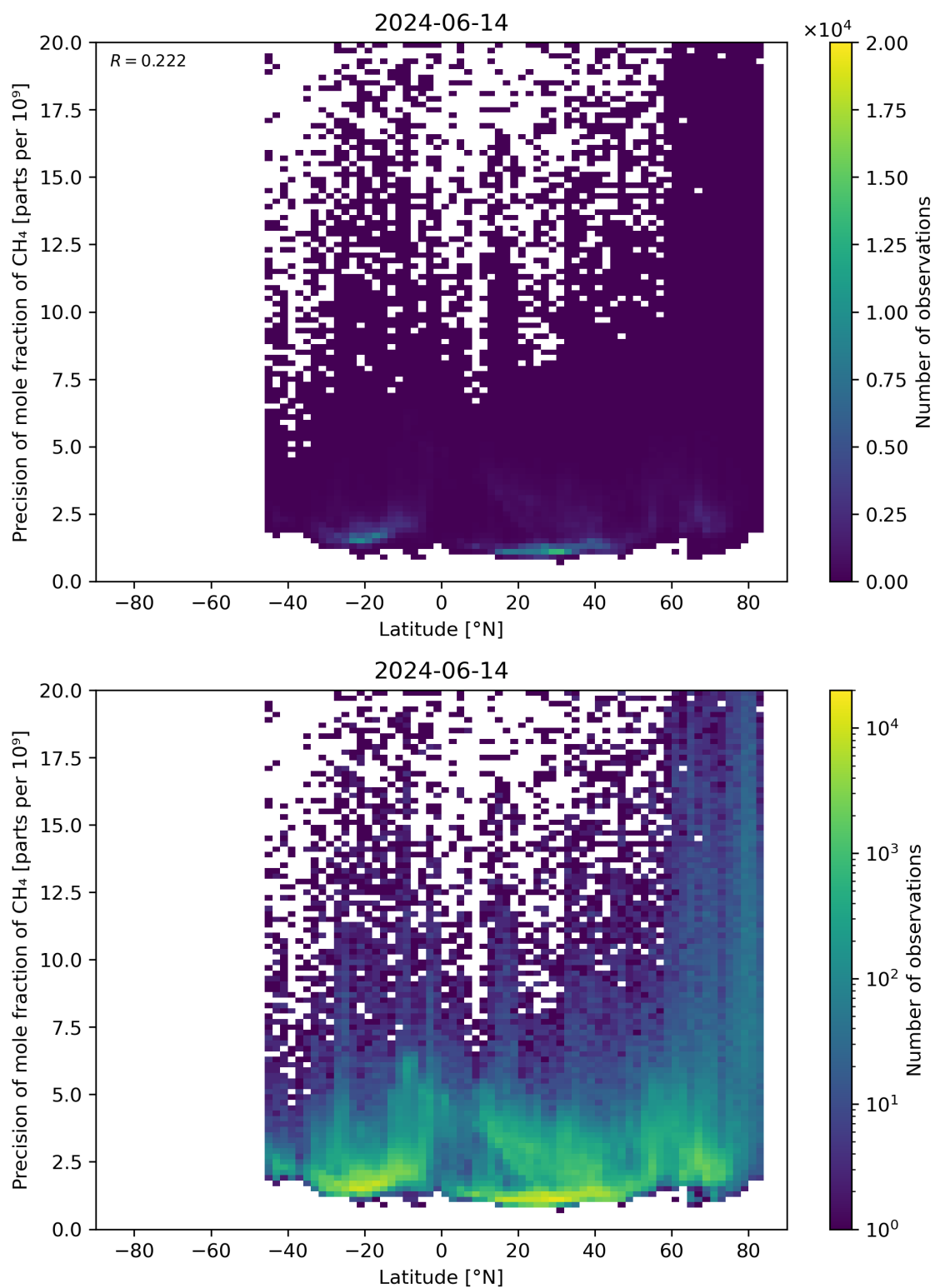
Figure 59: Scatter density plot of “Latitude” against “Precision of mole fraction of \text{CH}_4 ” for 2024-06-13 to 2024-06-15.
