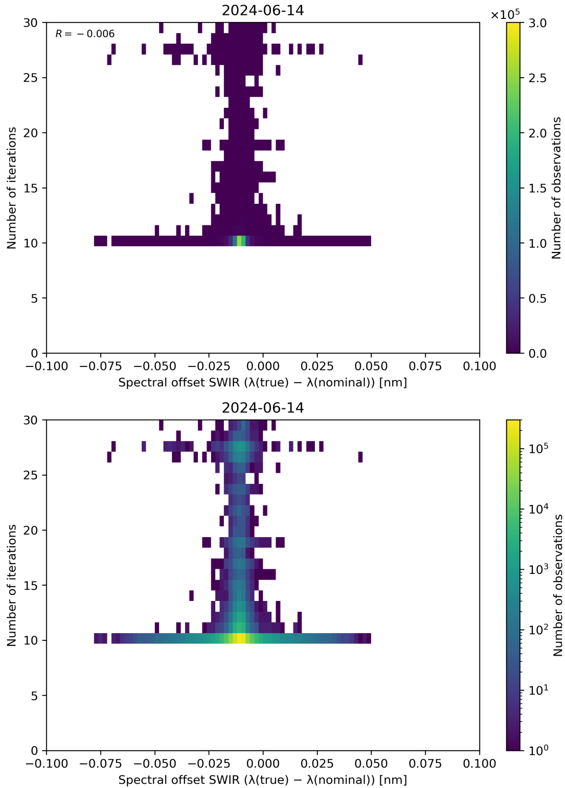
Figure 121: Scatter density plot of “Spectral offset SWIR ( \lambda(\text{true}) - \lambda(\text{nominal}) )” against “Number of iterations” for 2024-06-13 to 2024-06-15.
