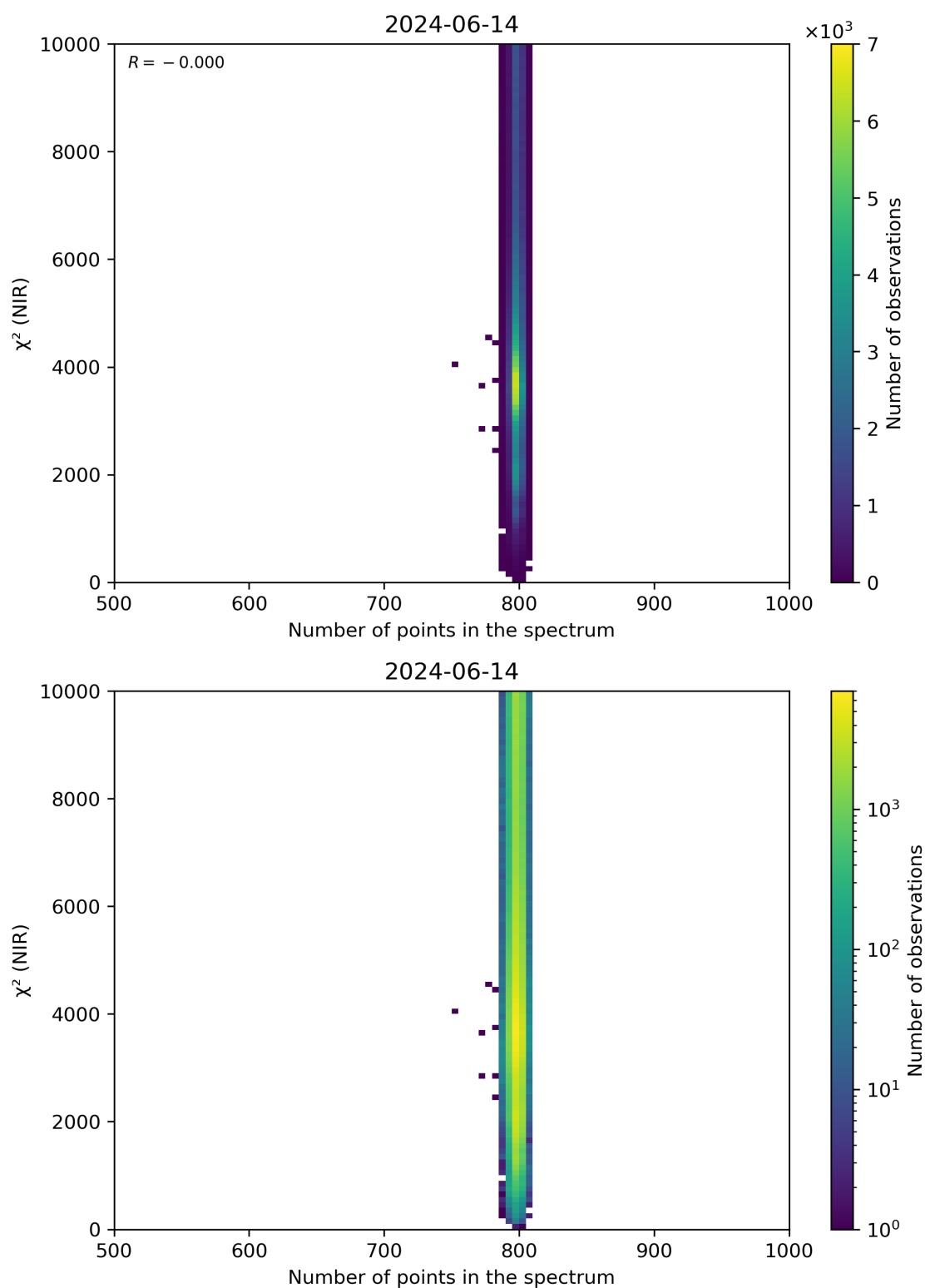
Figure 88: Scatter density plot of “Number of points in the spectrum” against “ \chi^2 (NIR)” for 2024-06-13 to 2024-06-15.
