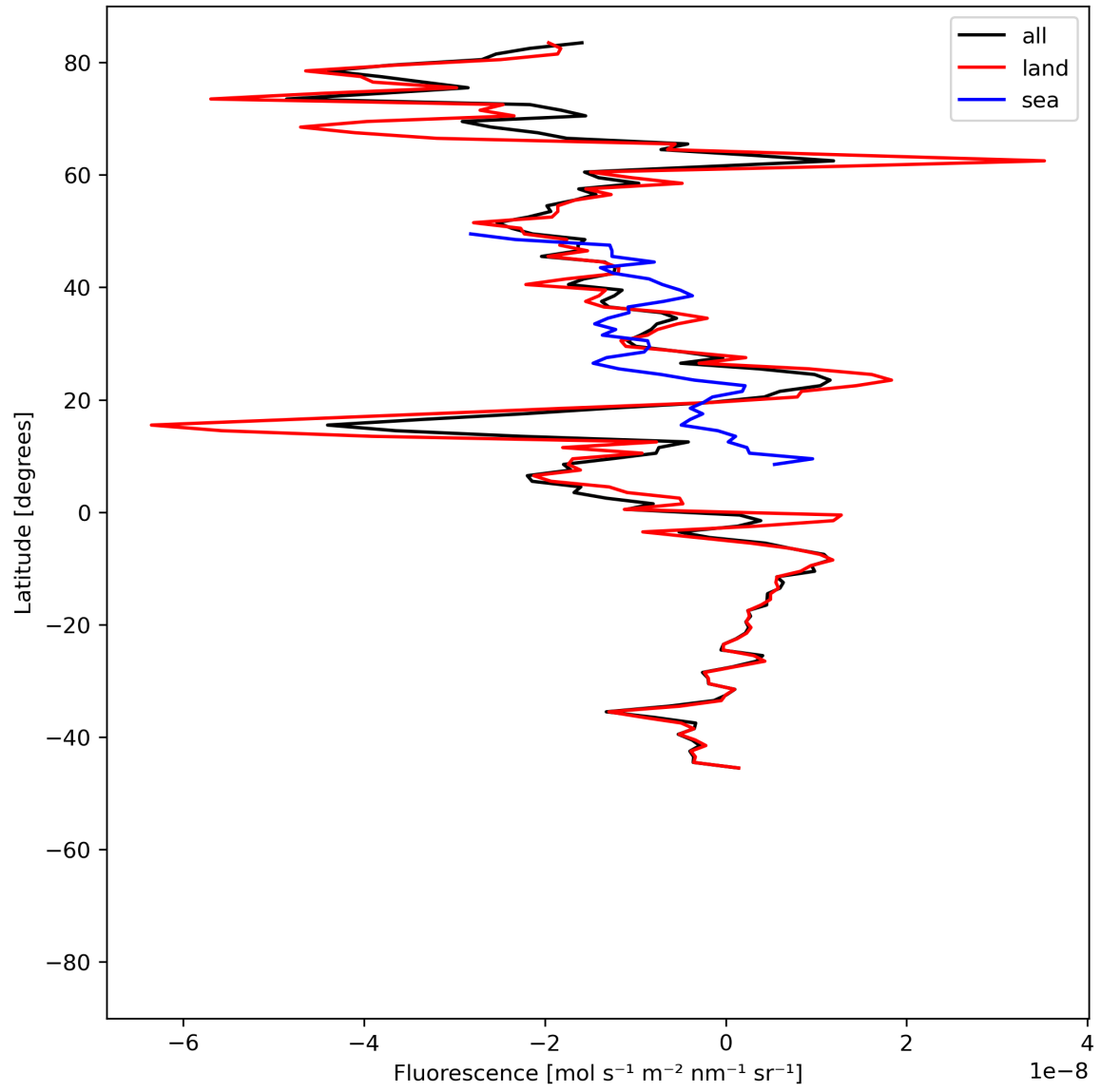
Figure 21: Zonal average of “Fluorescence” for 2024-06-13 to 2024-06-15.
