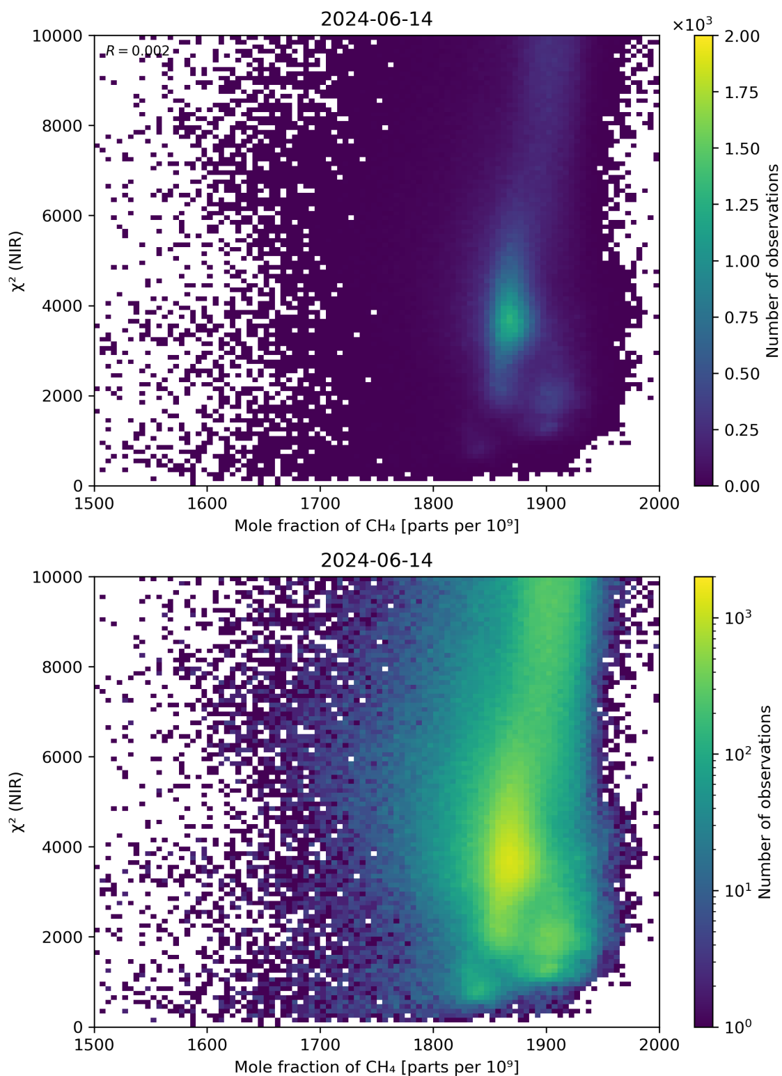
Figure 70: Scatter density plot of “Mole fraction of \text{CH}_4 ” against “ \chi^2 (NIR)” for 2024-06-13 to 2024-06-15.
