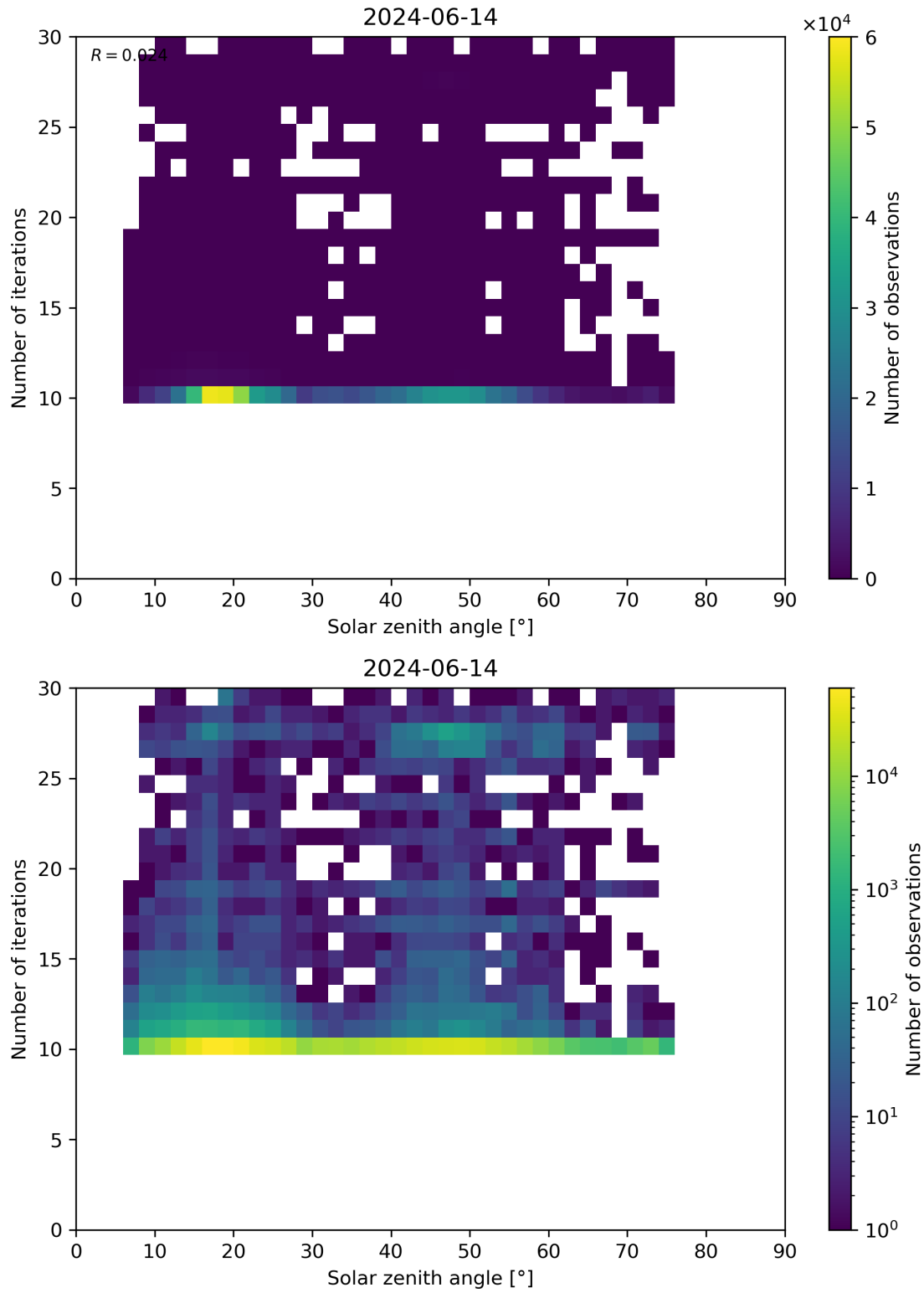
Figure 102: Scatter density plot of “Solar zenith angle” against “Number of iterations” for 2024-06-13 to 2024-06-15.
