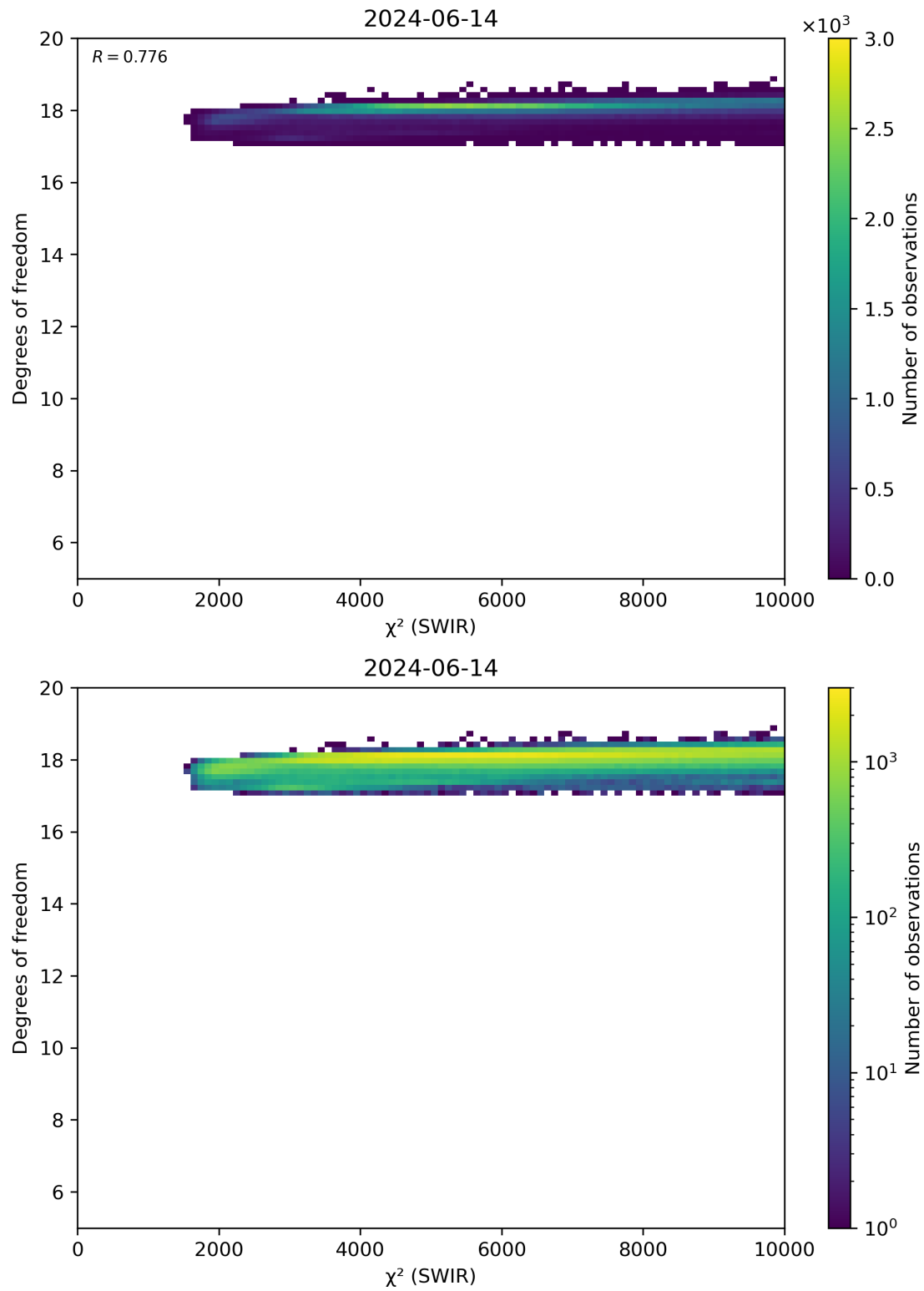
Figure 48: Scatter density plot of “ \chi^2 (SWIR)” against “Degrees of freedom” for 2024-06-13 to 2024-06-15.
