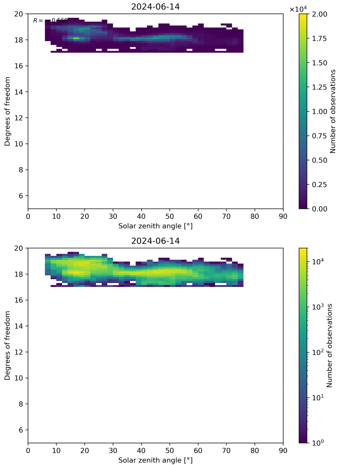
Figure 96: Scatter density plot of “Solar zenith angle” against “Degrees of freedom” for 2024-06-13 to 2024-06-15.
