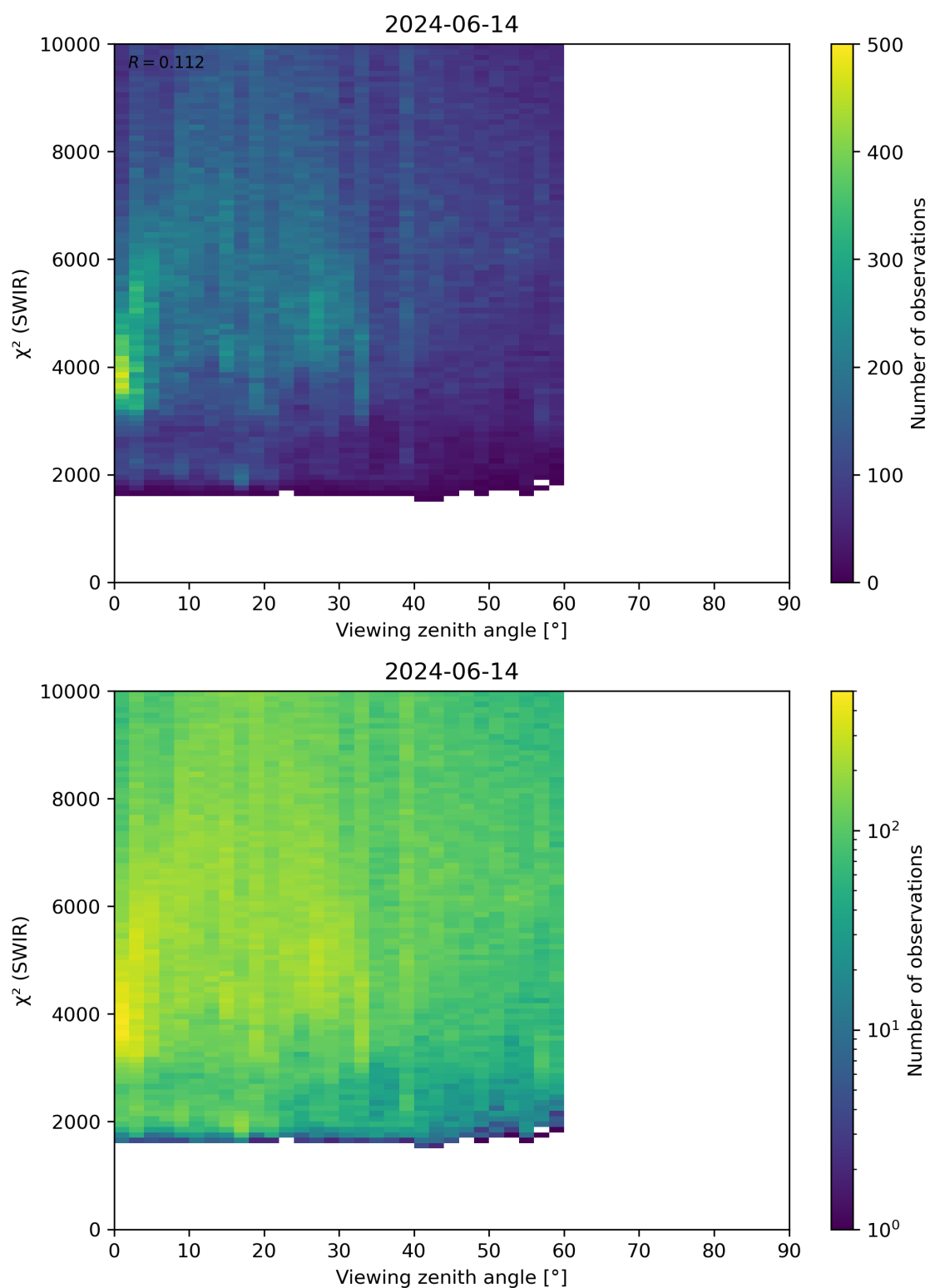
Figure 106: Scatter density plot of “Viewing zenith angle” against “ \chi^2 (SWIR)” for 2024-06-13 to 2024-06-15.
