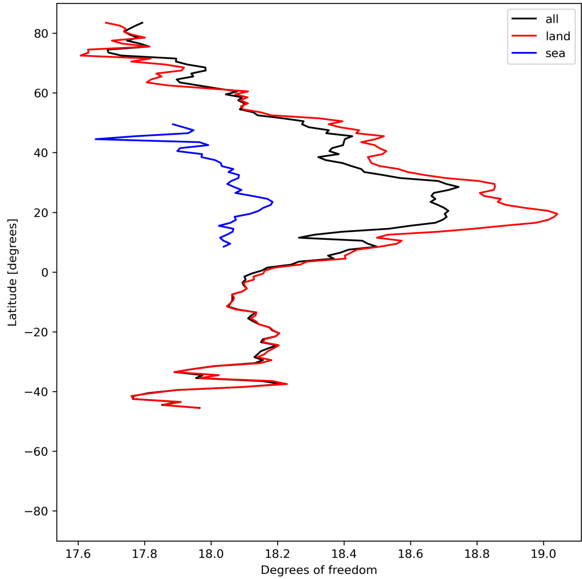
Figure 19: Zonal average of “Degrees of freedom” for 2024-06-13 to 2024-06-15.
