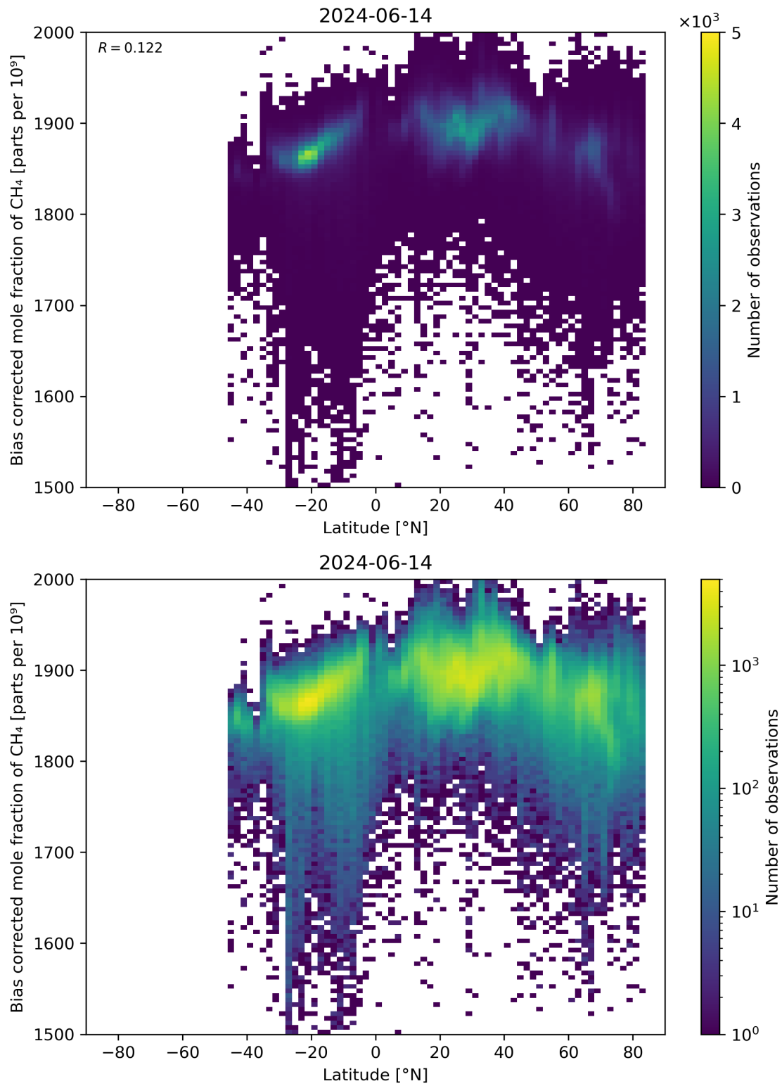
Figure 58: Scatter density plot of “Latitude” against “Bias corrected mole fraction of \text{CH}_4 ” for 2024-06-13 to 2024-06-15.
