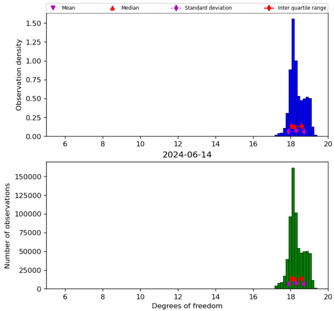
Figure 30: Histogram of “Degrees of freedom” for 2024-06-13 to 2024-06-15
