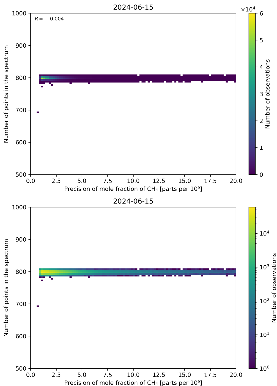
Figure 84: Scatter density plot of “Precision of mole fraction of CH 4 ” against “Number of points in the spectrum” for 2024-06-14 to 2024-06-16.
