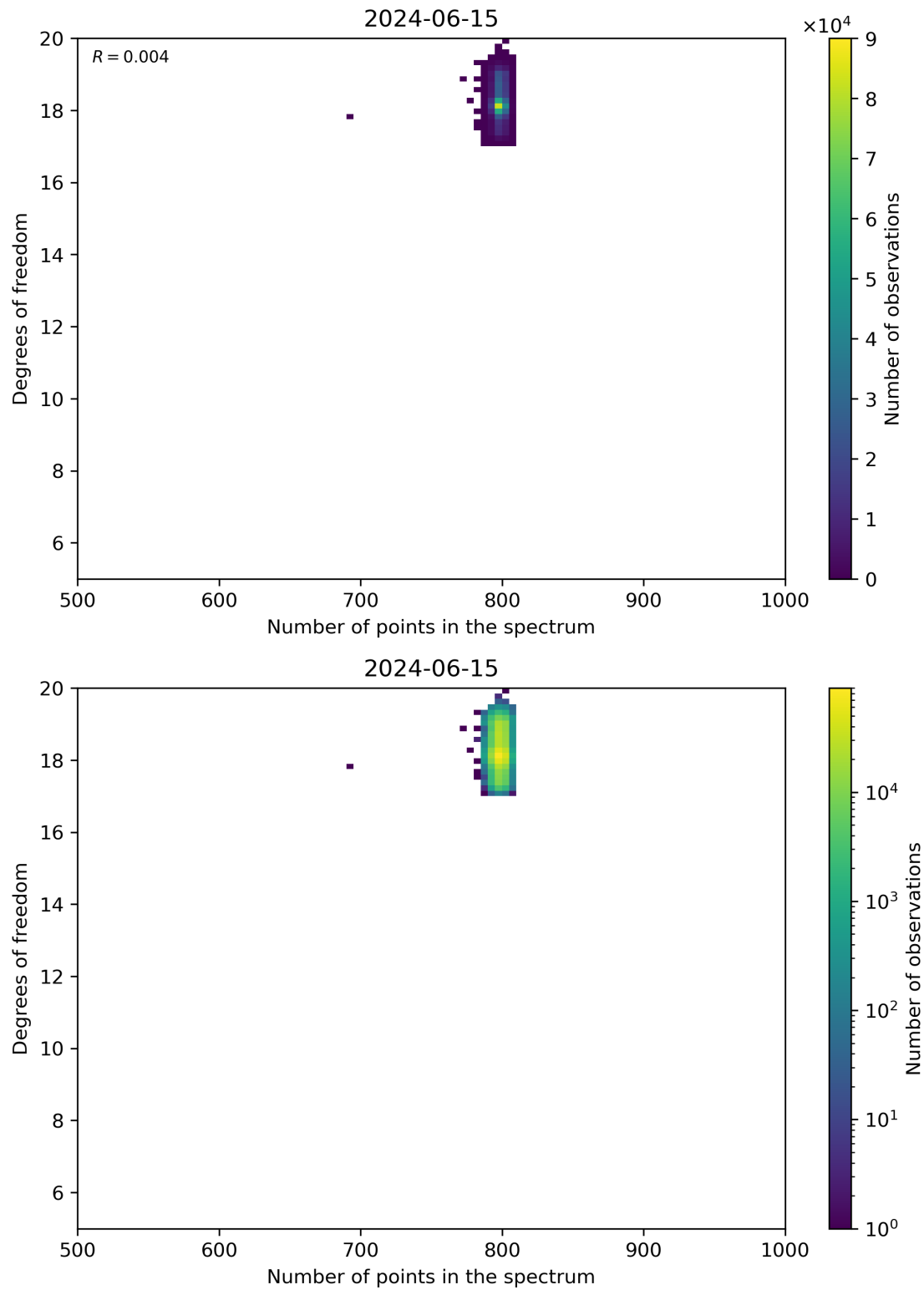
Figure 90: Scatter density plot of “Number of points in the spectrum” against “Degrees of freedom” for 2024-06-14 to 2024-06-16.
