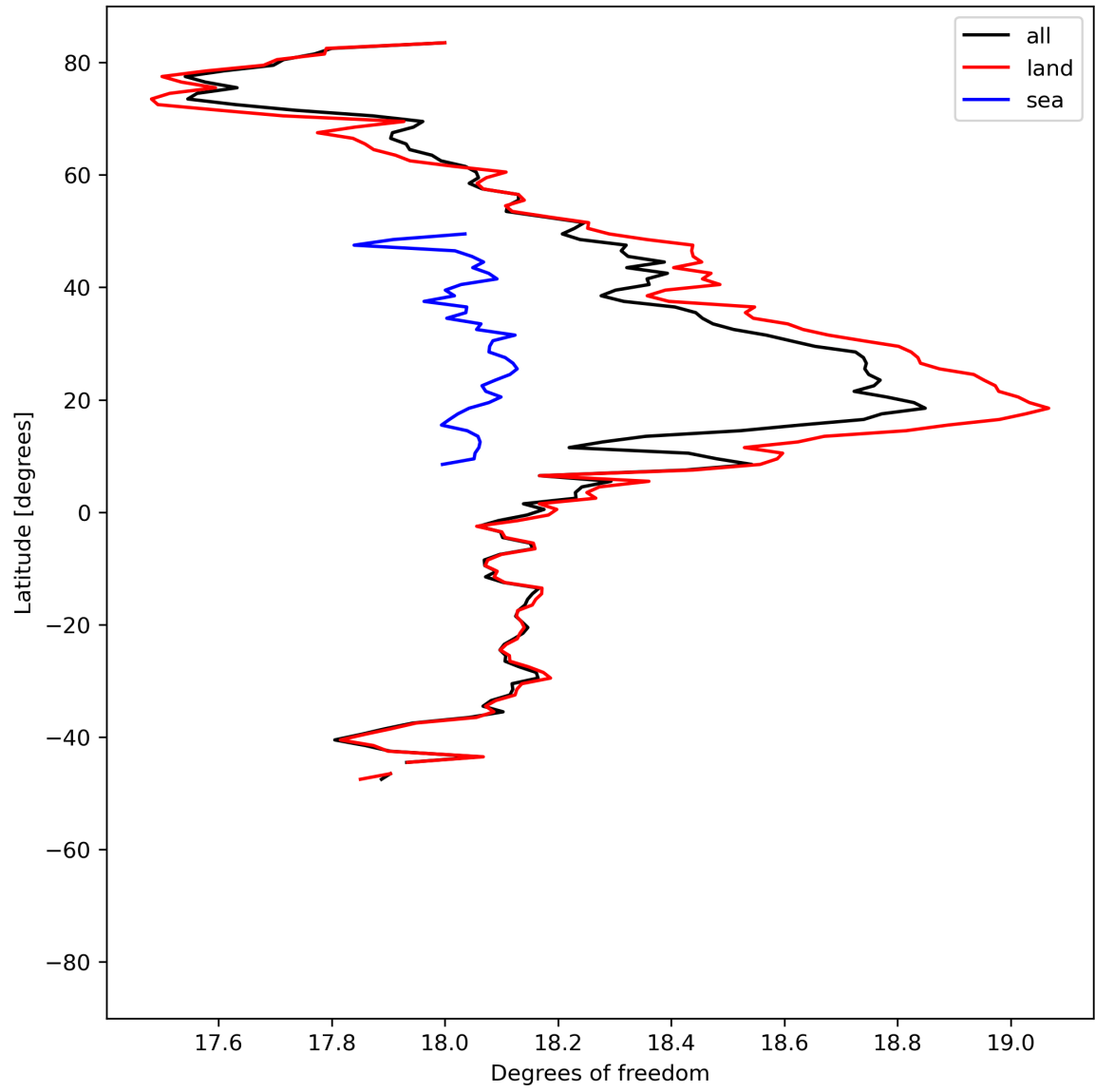
Figure 19: Zonal average of “Degrees of freedom” for 2024-06-14 to 2024-06-16.
