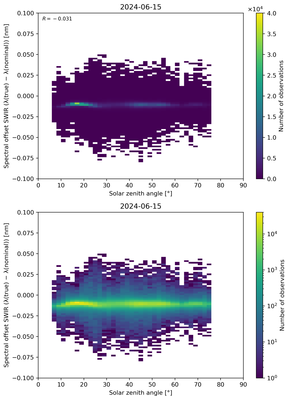
Figure 104: Scatter density plot of “Solar zenith angle” against “Spectral offset SWIR ( \lambda(\text{true}) - \lambda(\text{nominal}) )” for 2024-06-14 to 2024-06-16.
