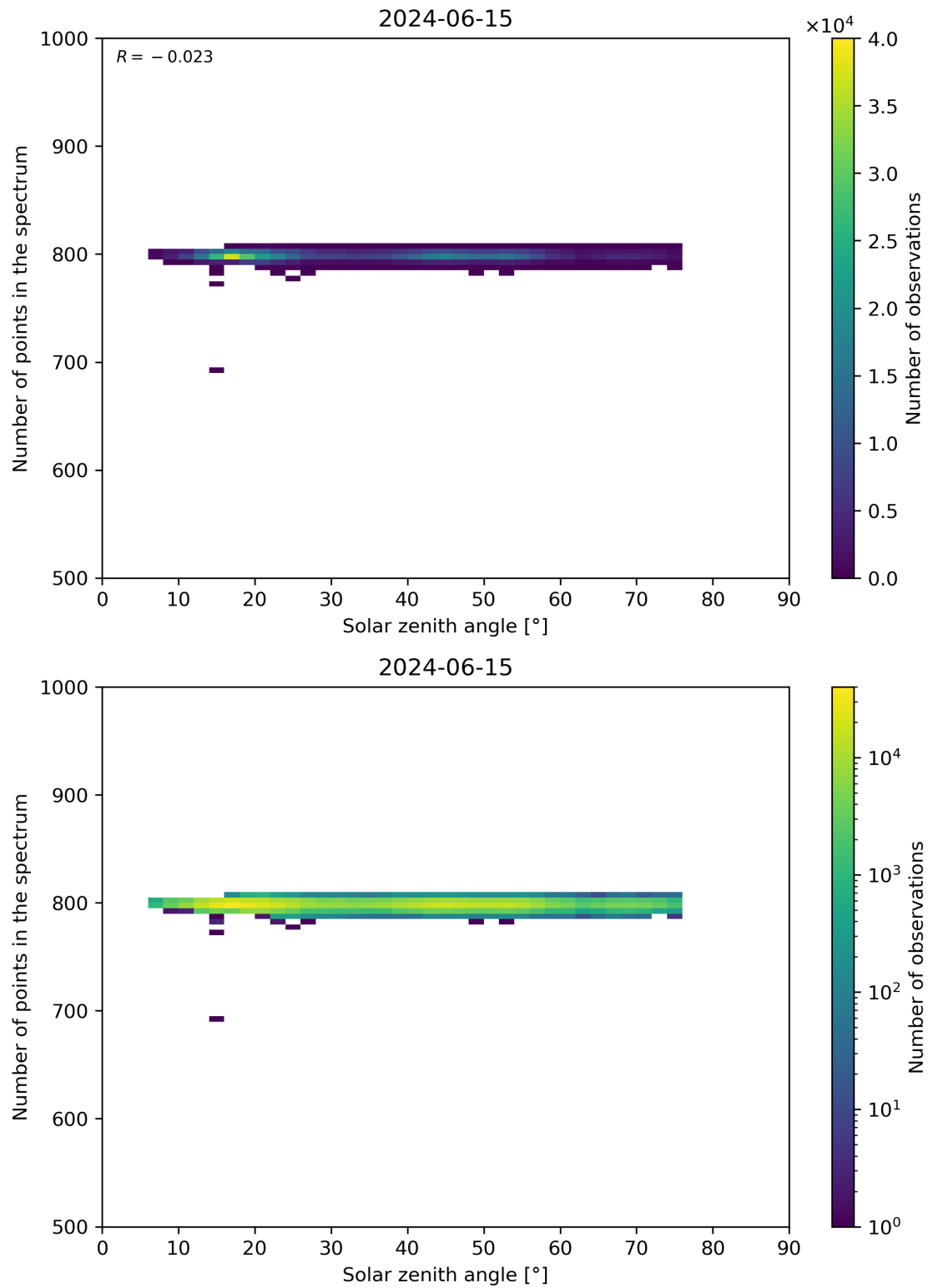
Figure 103: Scatter density plot of “Solar zenith angle” against “Number of points in the spectrum” for 2024-06-14 to 2024-06-16.
