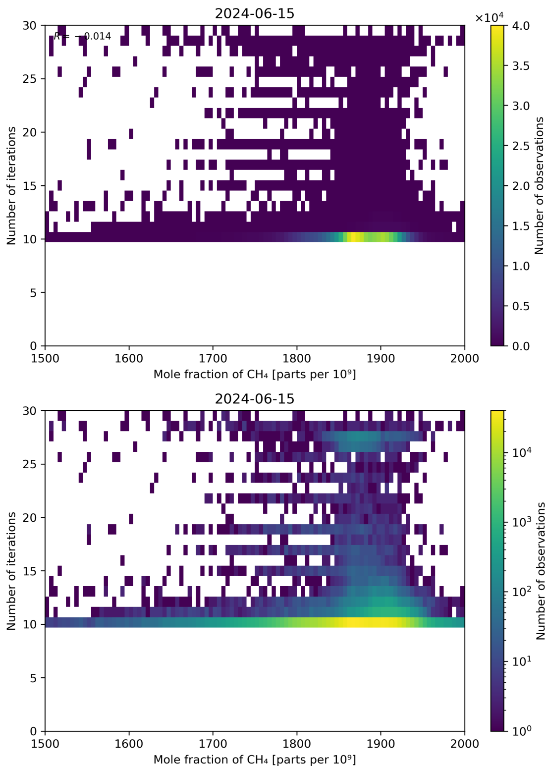
Figure 76: Scatter density plot of “Mole fraction of CH 4 ” against “Number of iterations” for 2024-06-14 to 2024-06-16.
