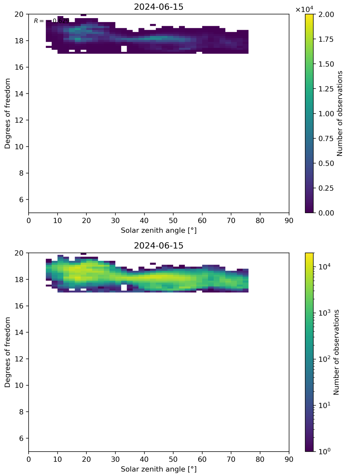
Figure 96: Scatter density plot of “Solar zenith angle” against “Degrees of freedom” for 2024-06-14 to 2024-06-16.
