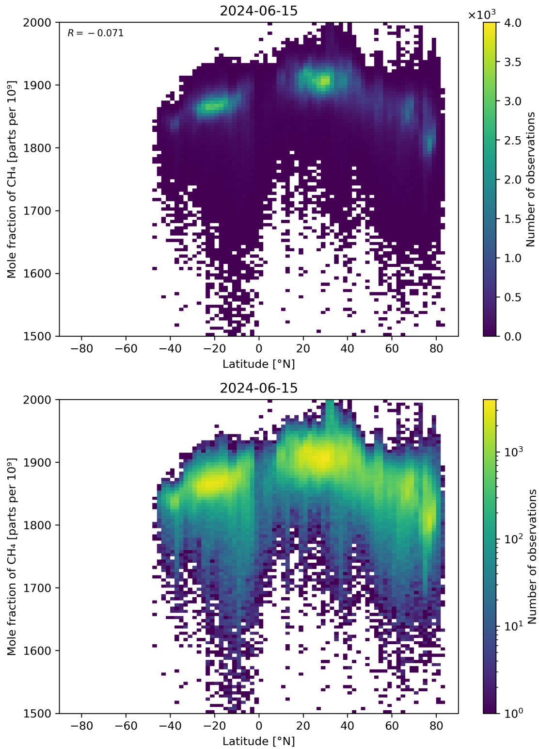
Figure 57: Scatter density plot of “Latitude” against “Mole fraction of \text{CH}_4 ” for 2024-06-14 to 2024-06-16.
