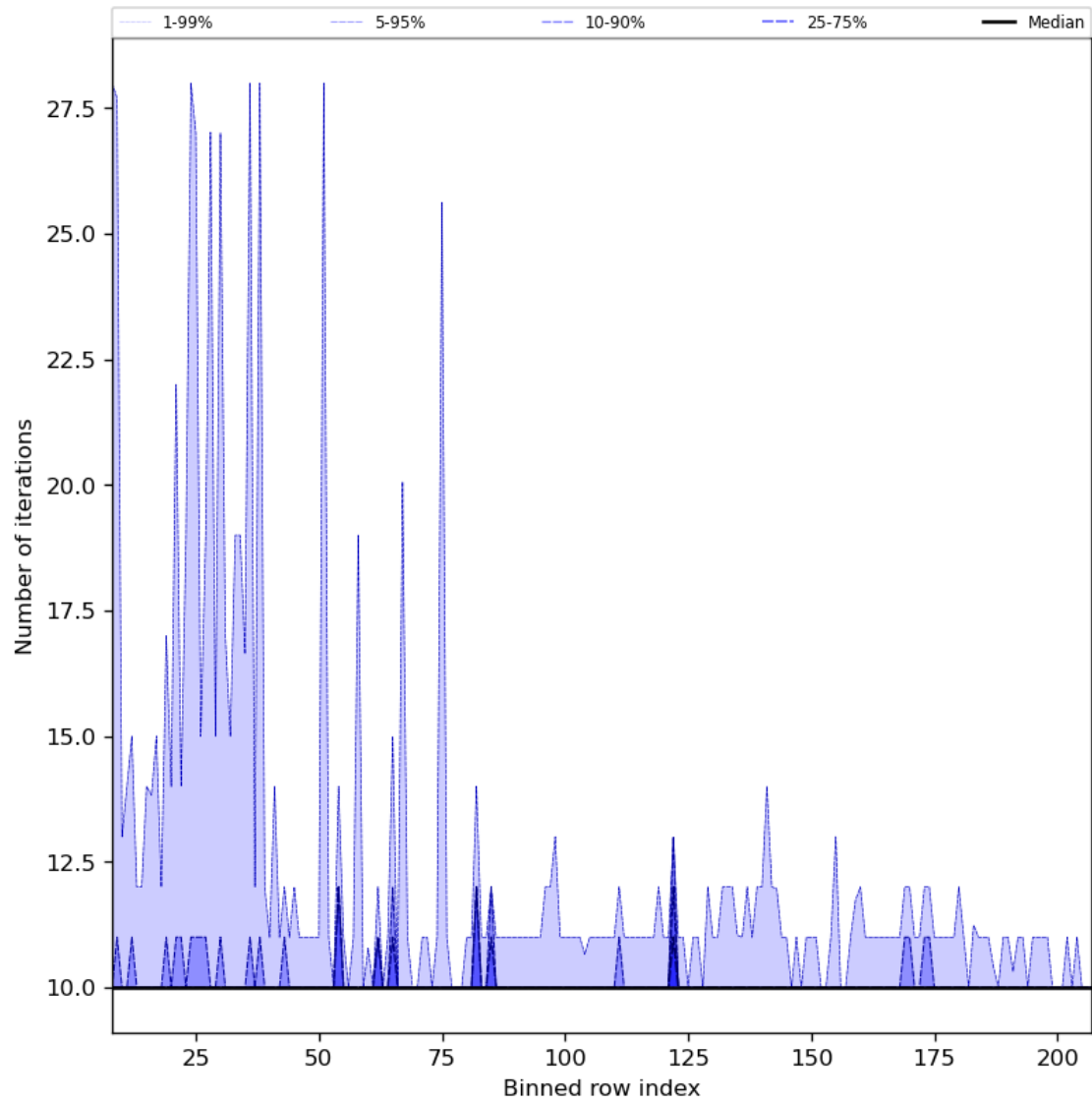
Figure 42: Along track statistics of “Number of iterations” for 2024-06-14 to 2024-06-16
