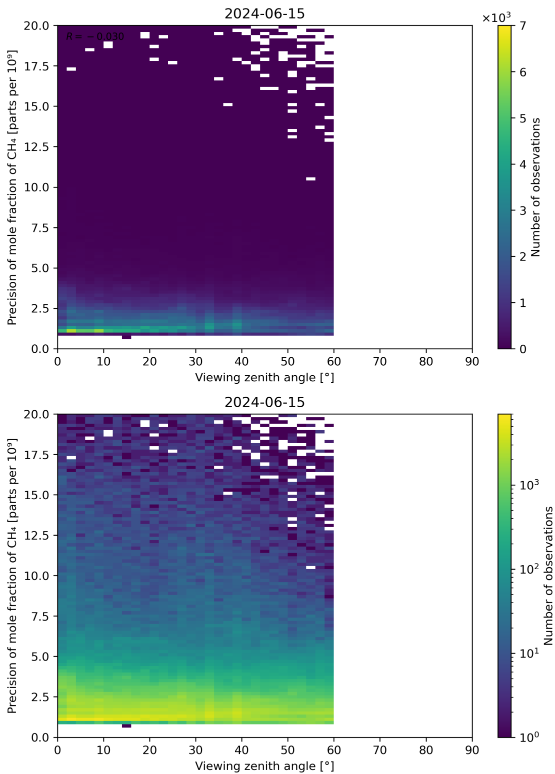
Figure 112: Scatter density plot of “Viewing zenith angle” against “Precision of mole fraction of CH 4 ” for 2024-06-14 to 2024-06-16.
