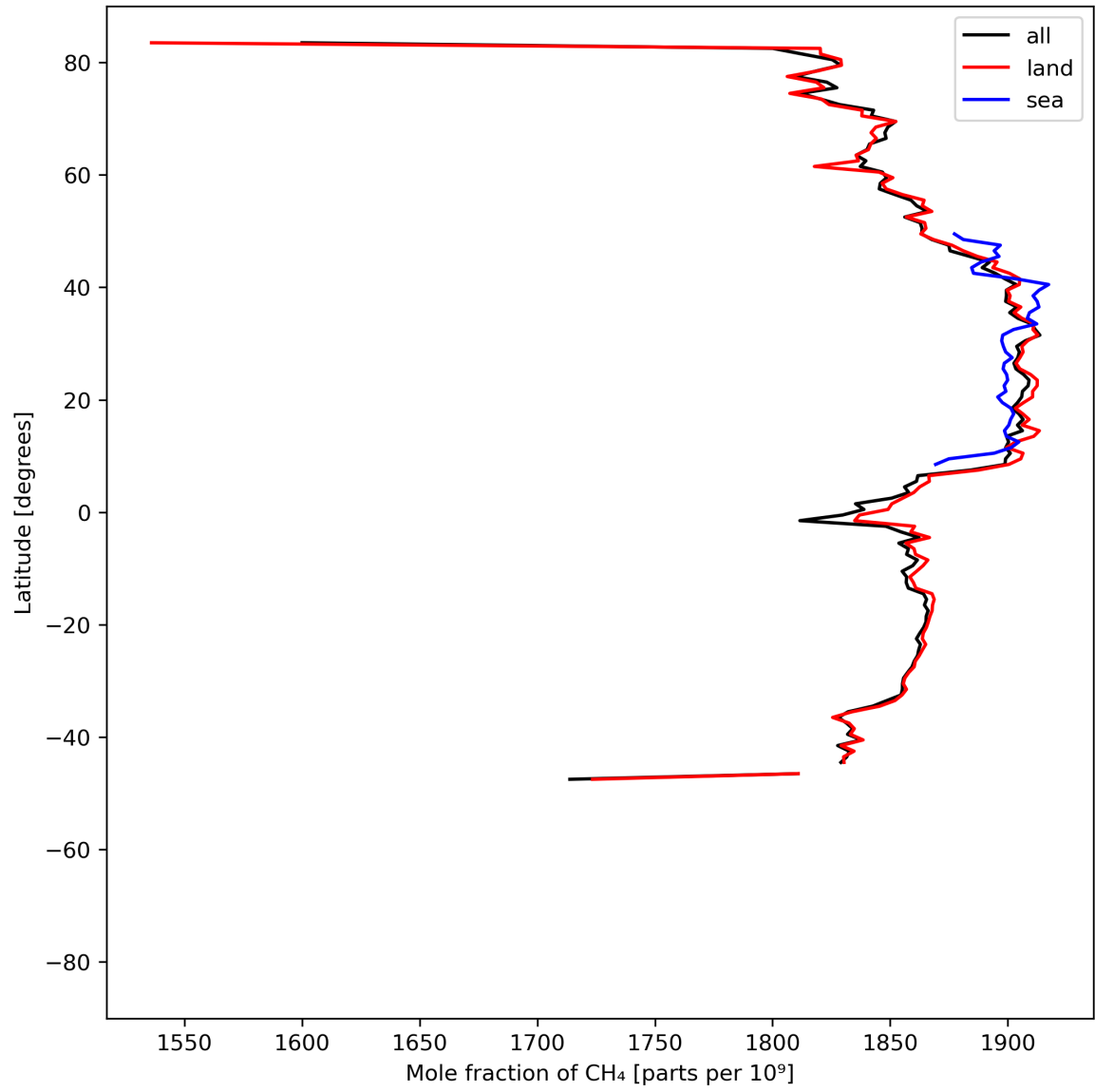
Figure 12: Zonal average of “Mole fraction of CH 4 ” for 2024-06-14 to 2024-06-16.
