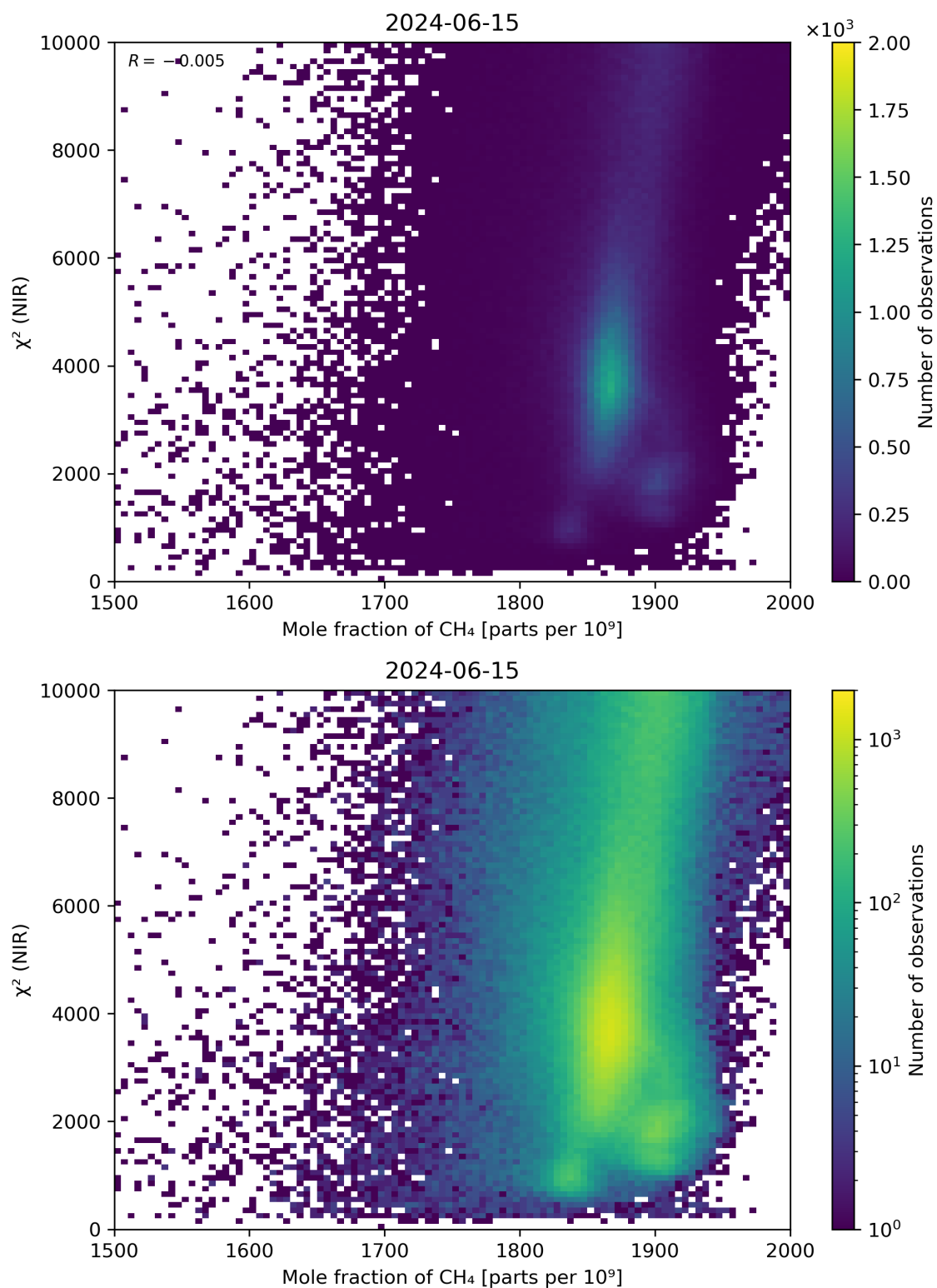
Figure 70: Scatter density plot of “Mole fraction of \text{CH}_4 ” against “ \chi^2 (NIR)” for 2024-06-14 to 2024-06-16.
