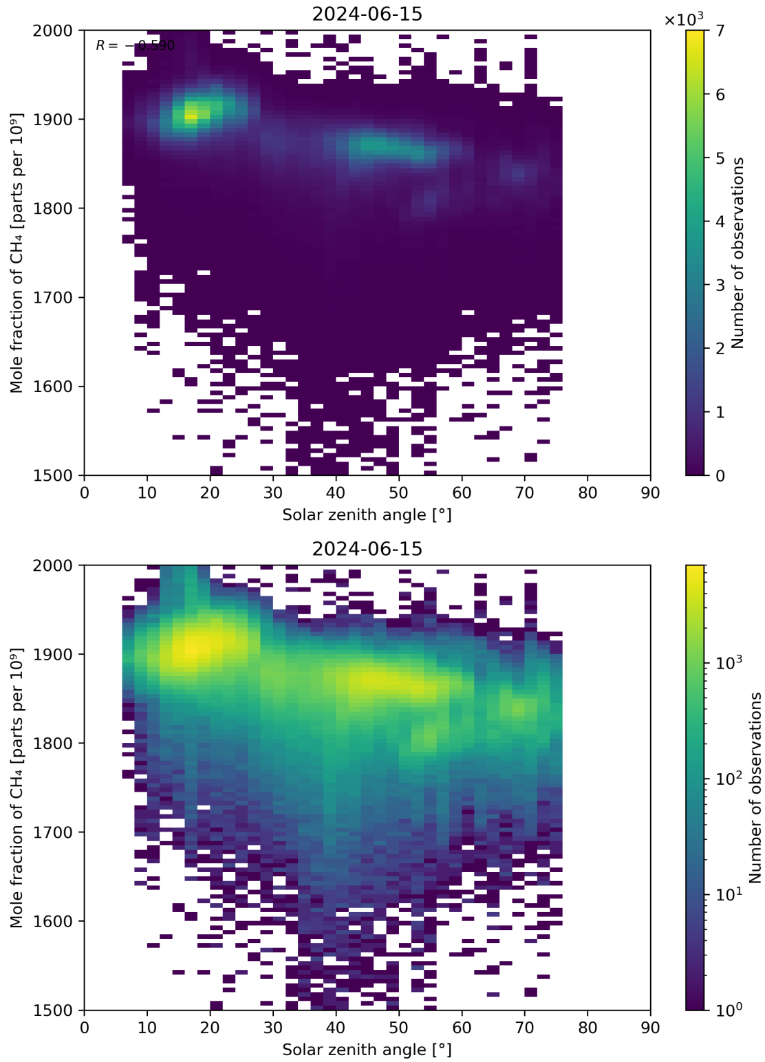
Figure 99: Scatter density plot of “Solar zenith angle” against “Mole fraction of CH 4 ” for 2024-06-14 to 2024-06-16.
