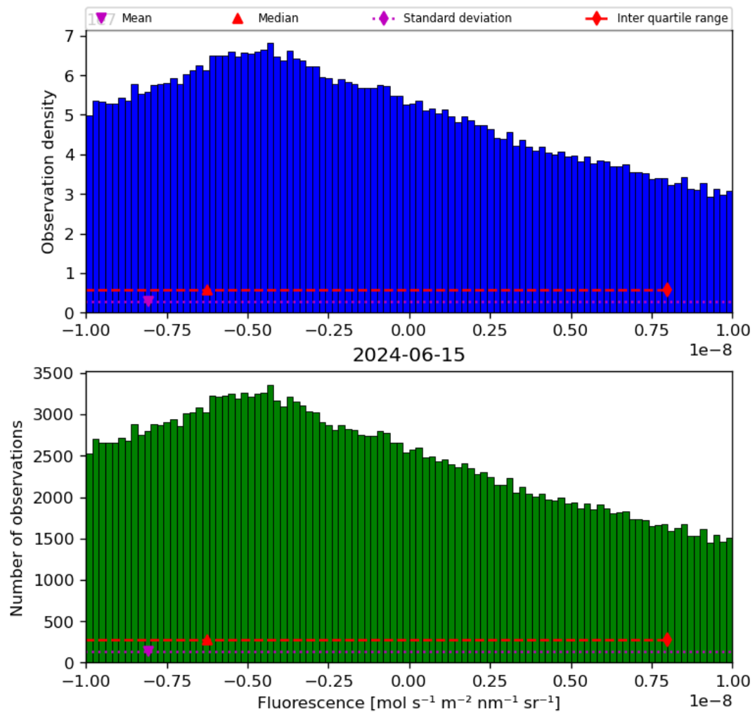
Figure 32: Histogram of “Fluorescence” for 2024-06-14 to 2024-06-16
