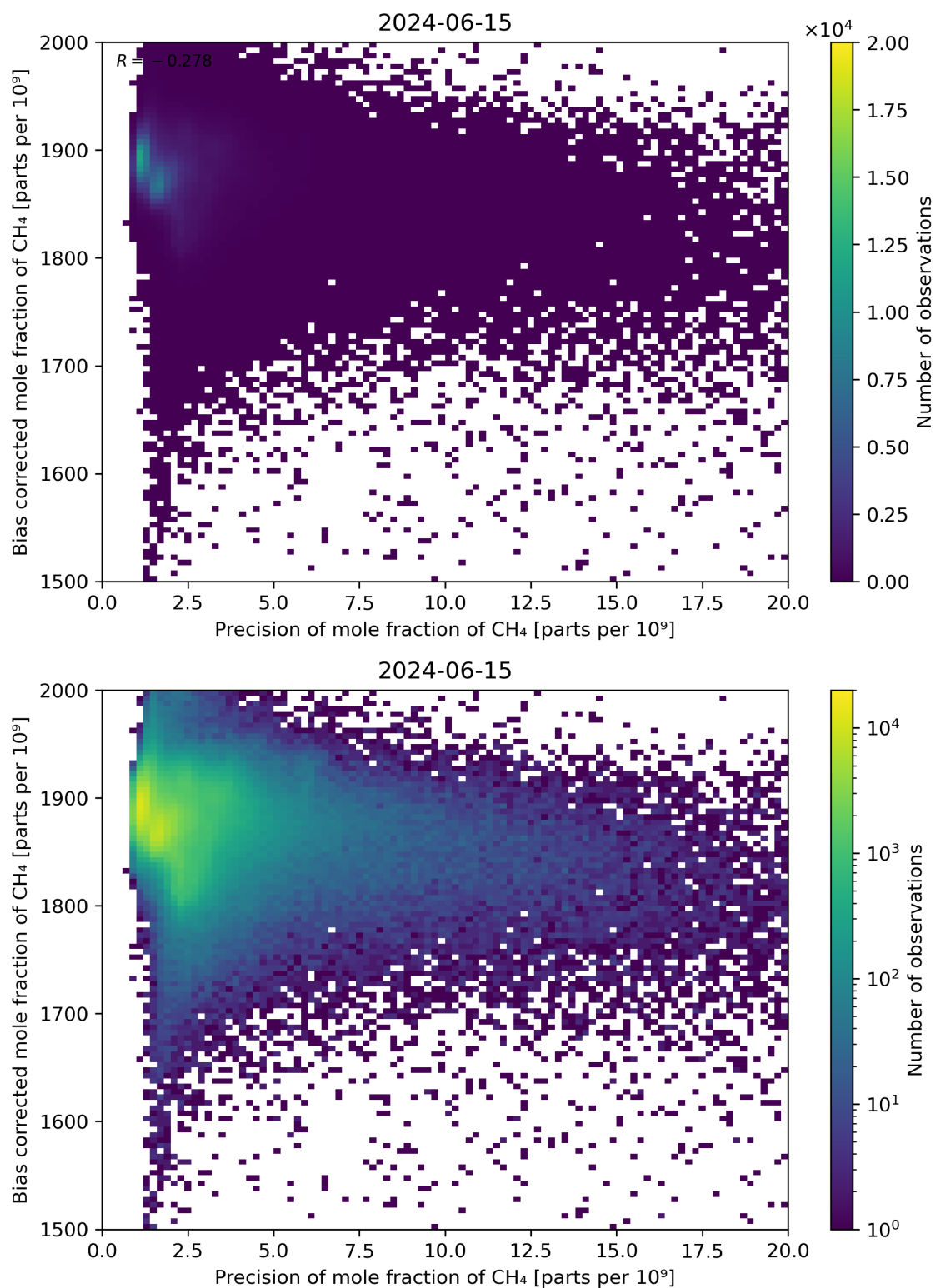
Figure 82: Scatter density plot of “Precision of mole fraction of \text{CH}_4 ” against “Bias corrected mole fraction of \text{CH}_4 ” for 2024-06-14 to 2024-06-16.
