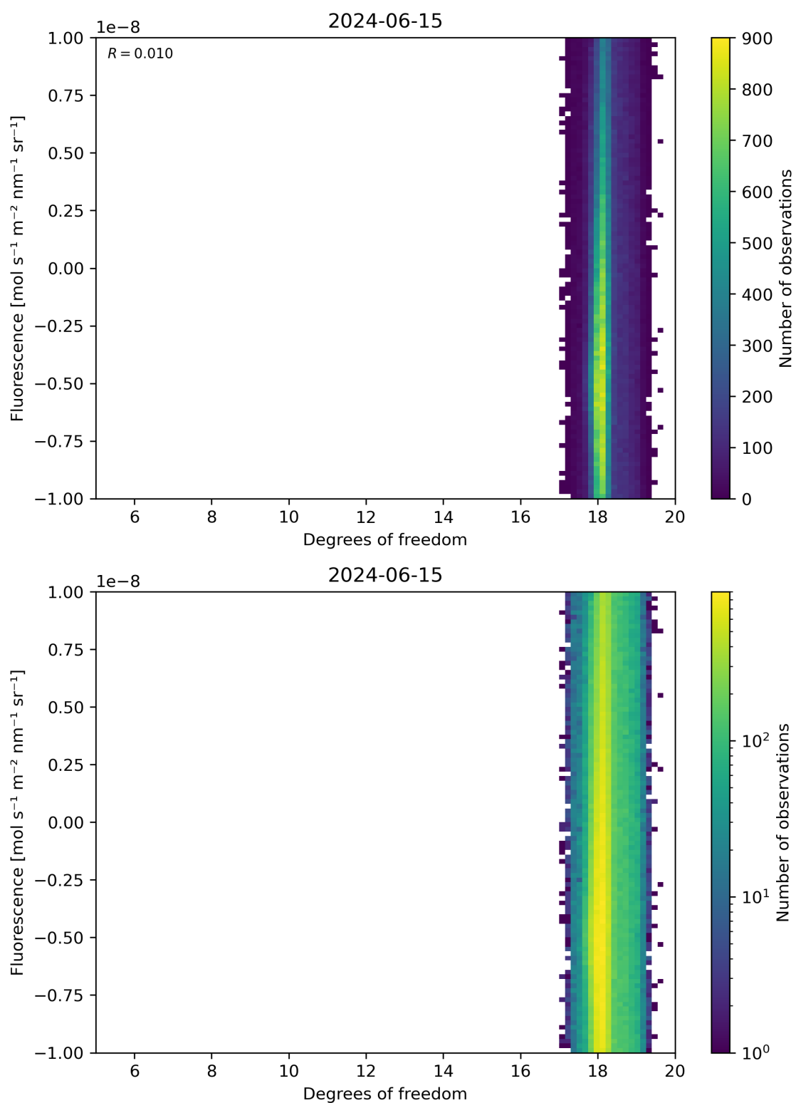
Figure 51: Scatter density plot of “Degrees of freedom” against “Fluorescence” for 2024-06-14 to 2024-06-16.
