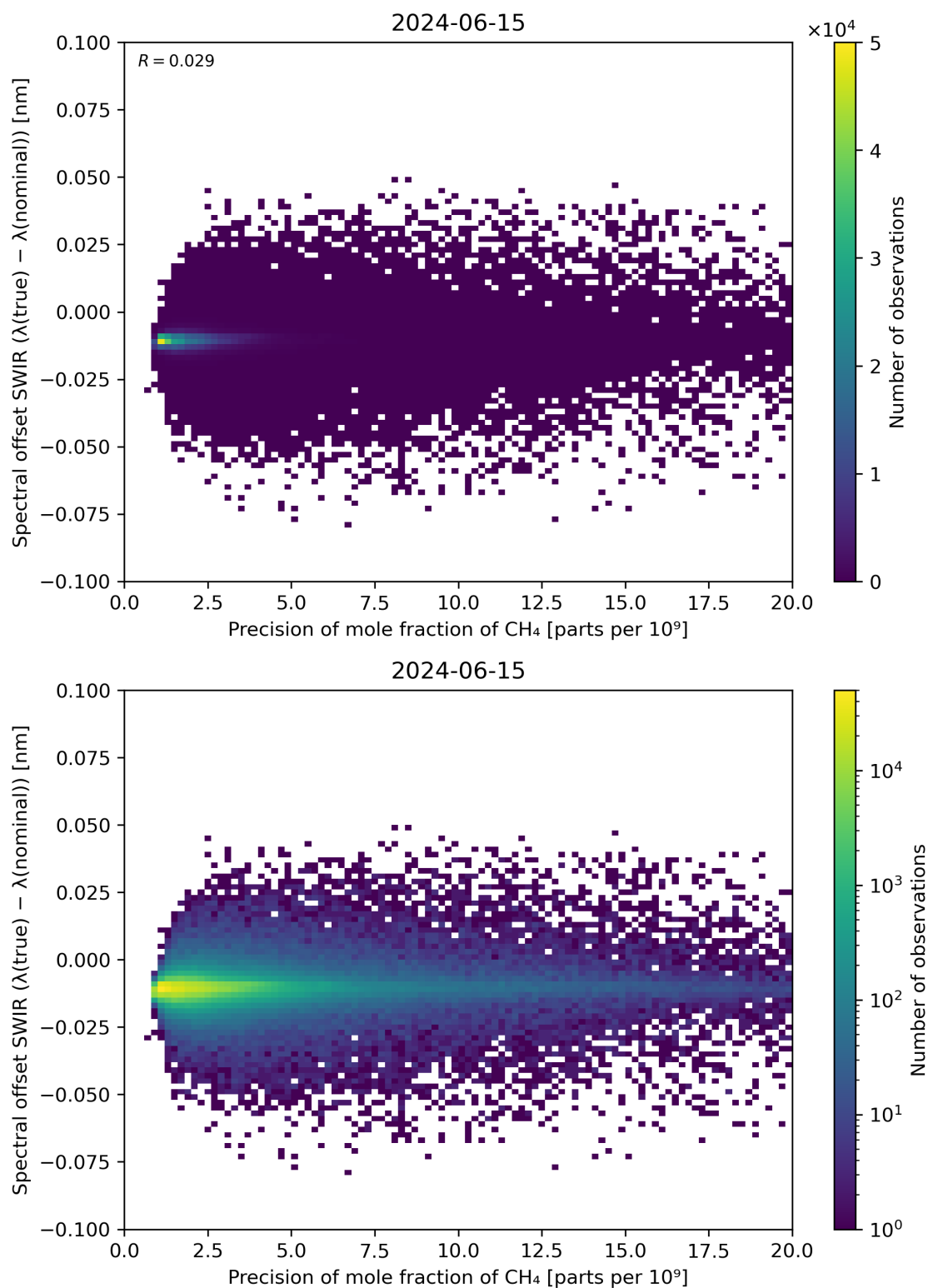
Figure 85: Scatter density plot of “Precision of mole fraction of CH 4 ” against “Spectral offset SWIR ( \lambda(\text{true}) - \lambda(\text{nominal}) )” for 2024-06-14 to 2024-06-16.
