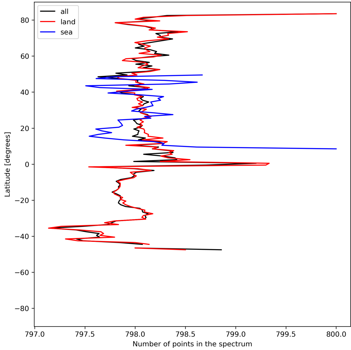
Figure 15: Zonal average of “Number of points in the spectrum” for 2024-06-14 to 2024-06-16.
