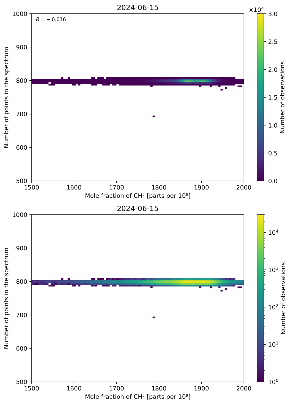
Figure 77: Scatter density plot of “Mole fraction of CH 4 ” against “Number of points in the spectrum” for 2024-06-14 to 2024-06-16.
