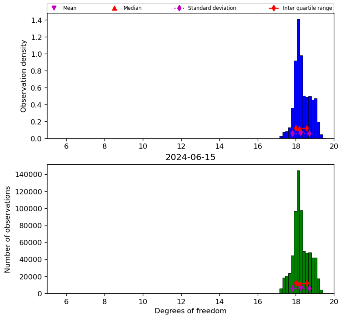
Figure 30: Histogram of “Degrees of freedom” for 2024-06-14 to 2024-06-16
