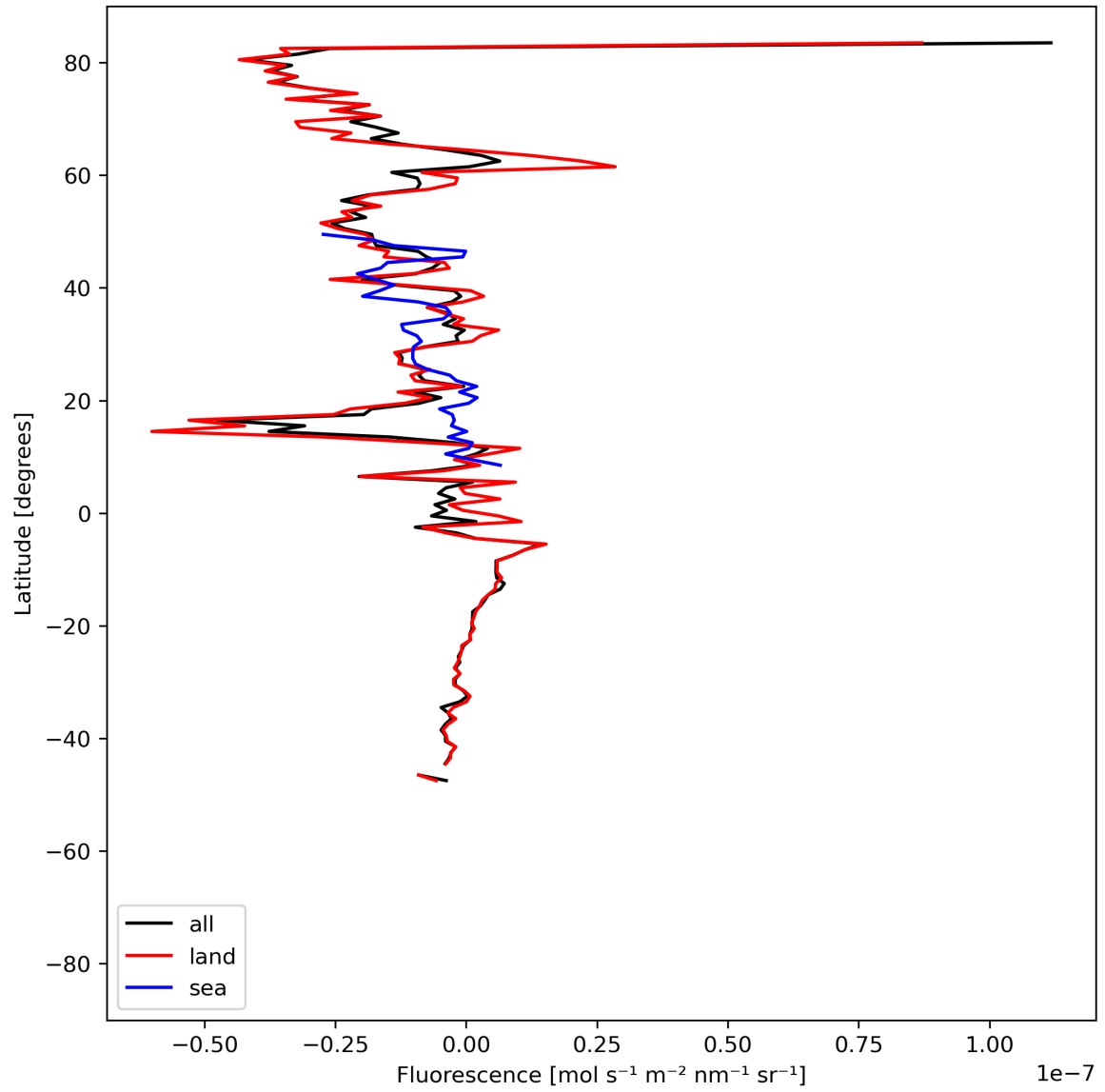
Figure 21: Zonal average of “Fluorescence” for 2024-06-14 to 2024-06-16.
