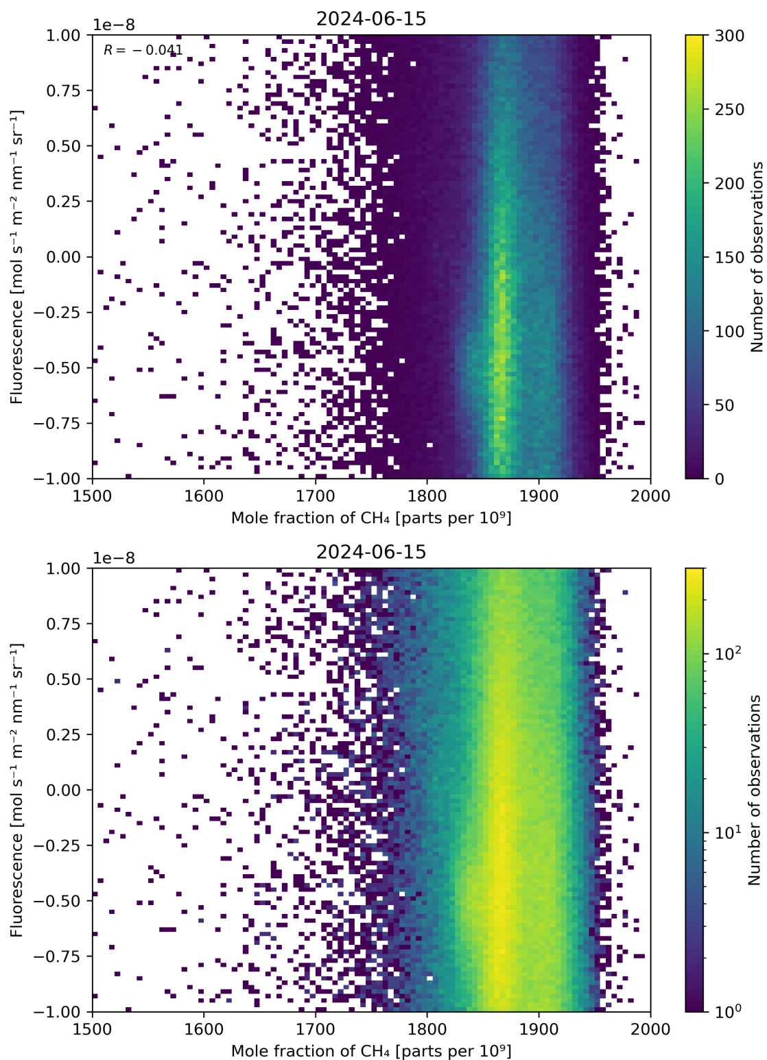
Figure 73: Scatter density plot of “Mole fraction of \text{CH}_4 ” against “Fluorescence” for 2024-06-14 to 2024-06-16.
