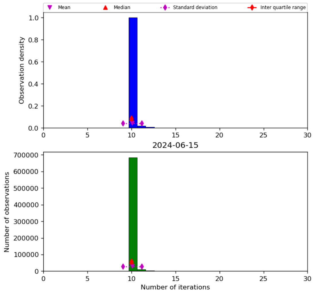
Figure 31: Histogram of “Number of iterations” for 2024-06-14 to 2024-06-16
