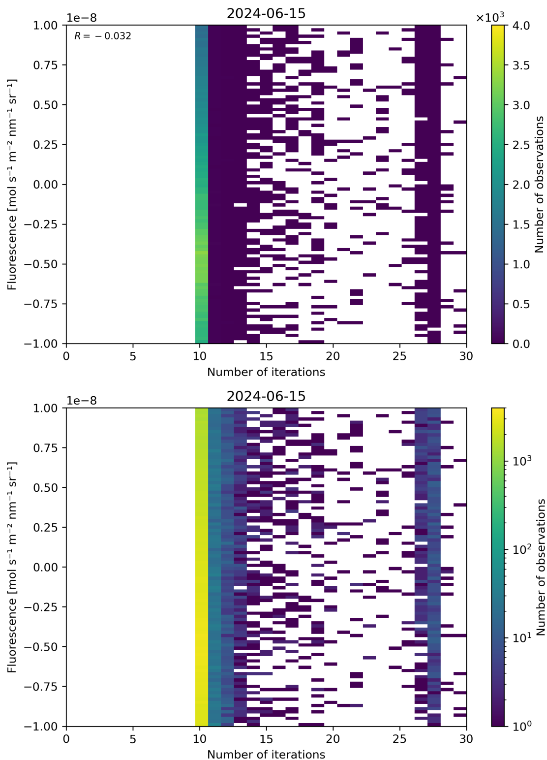
Figure 87: Scatter density plot of “Number of iterations” against “Fluorescence” for 2024-06-14 to 2024-06-16.
