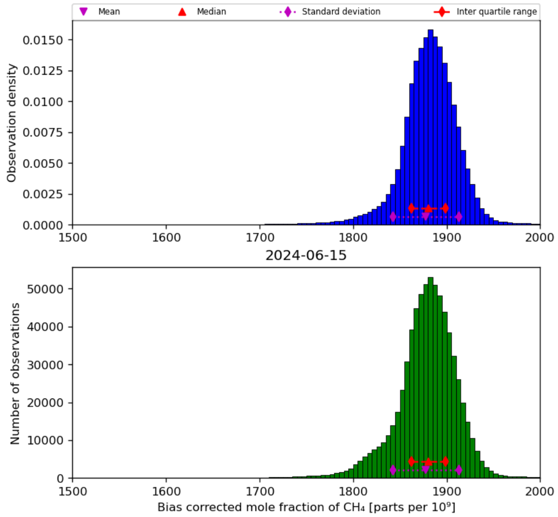
Figure 25: Histogram of “Bias corrected mole fraction of CH 4 ” for 2024-06-14 to 2024-06-16
