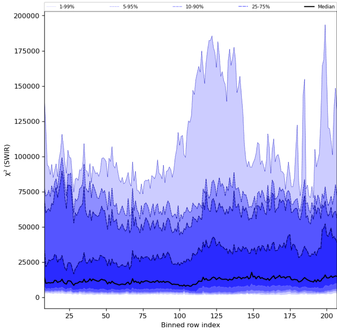
Figure 39: Along track statistics of " \chi^2 (SWIR)" for 2024-06-14 to 2024-06-16
