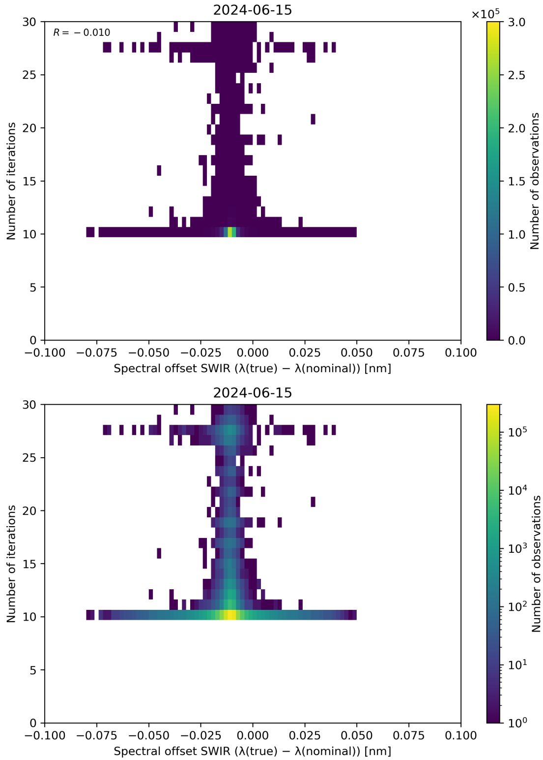
Figure 121: Scatter density plot of “Spectral offset SWIR ( \lambda(\text{true}) - \lambda(\text{nominal}) )” against “Number of iterations” for 2024-06-14 to 2024-06-16.
