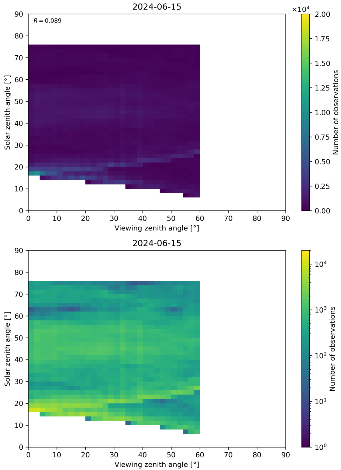
Figure 115: Scatter density plot of “Viewing zenith angle” against “Solar zenith angle” for 2024-06-14 to 2024-06-16.
