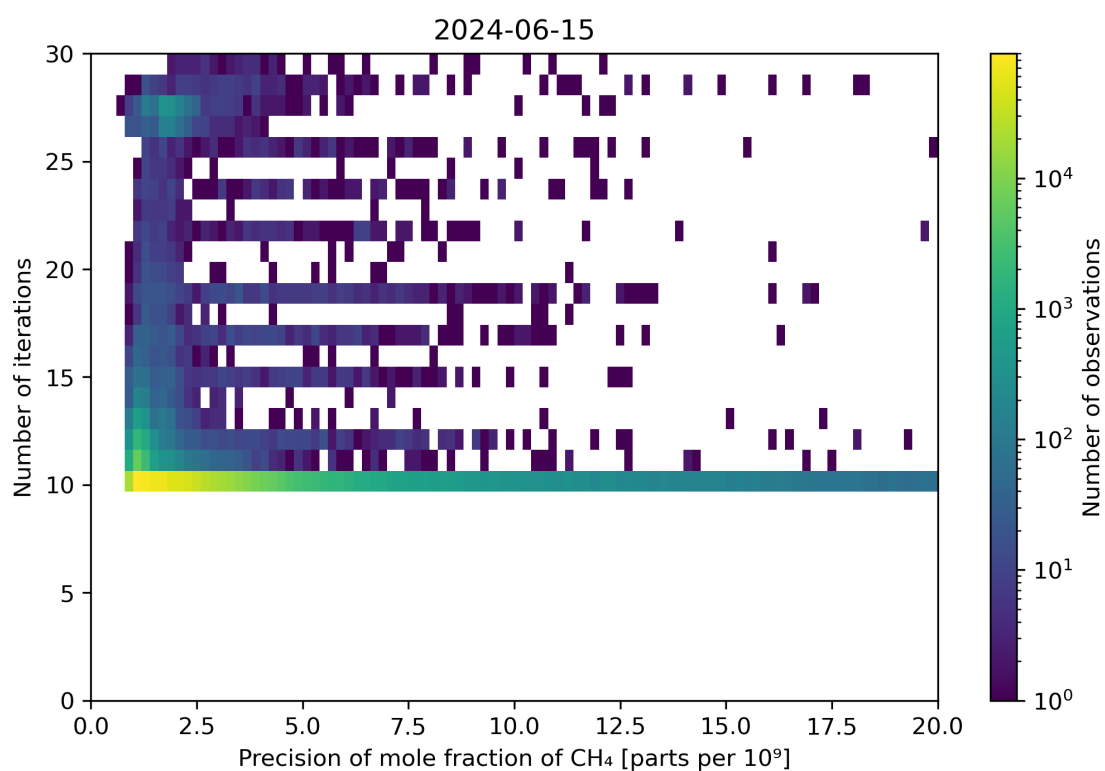
Figure 83: Scatter density plot of “Precision of mole fraction of CH 4 ” against “Number of iterations” for 2024-06-14 to 2024-06-16.
