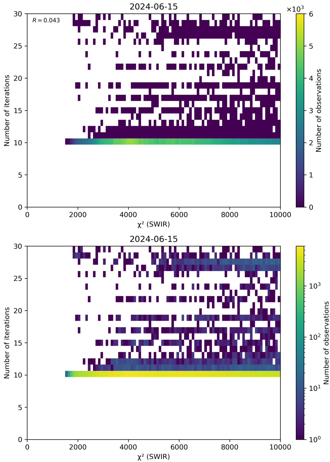
Figure 50: Scatter density plot of “ \chi^2 (SWIR)” against “Number of iterations” for 2024-06-14 to 2024-06-16.
