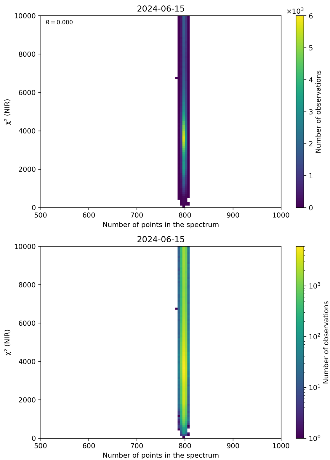
Figure 88: Scatter density plot of “Number of points in the spectrum” against “ \chi^2 (NIR)” for 2024-06-14 to 2024-06-16.
