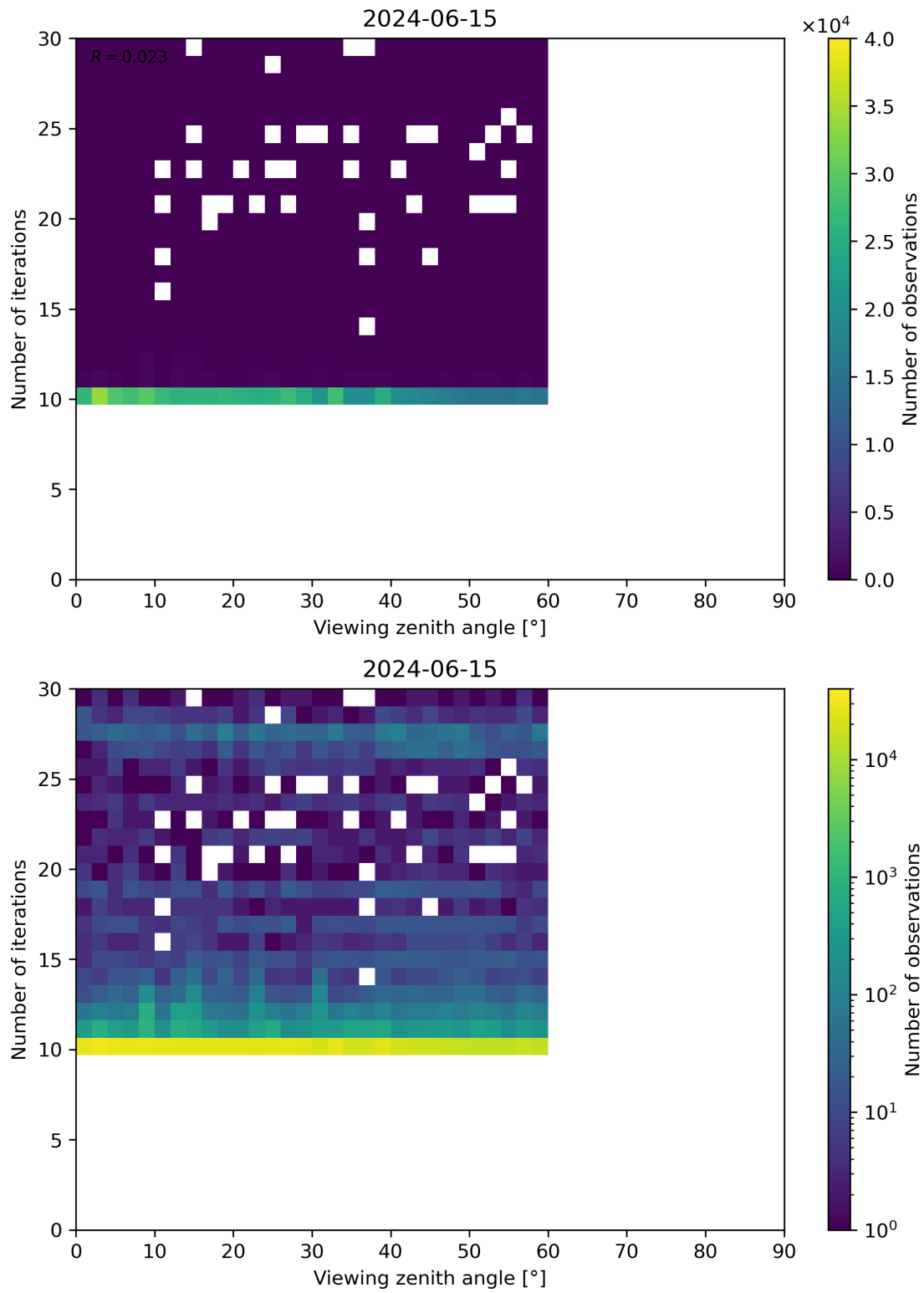
Figure 113: Scatter density plot of “Viewing zenith angle” against “Number of iterations” for 2024-06-14 to 2024-06-16.
