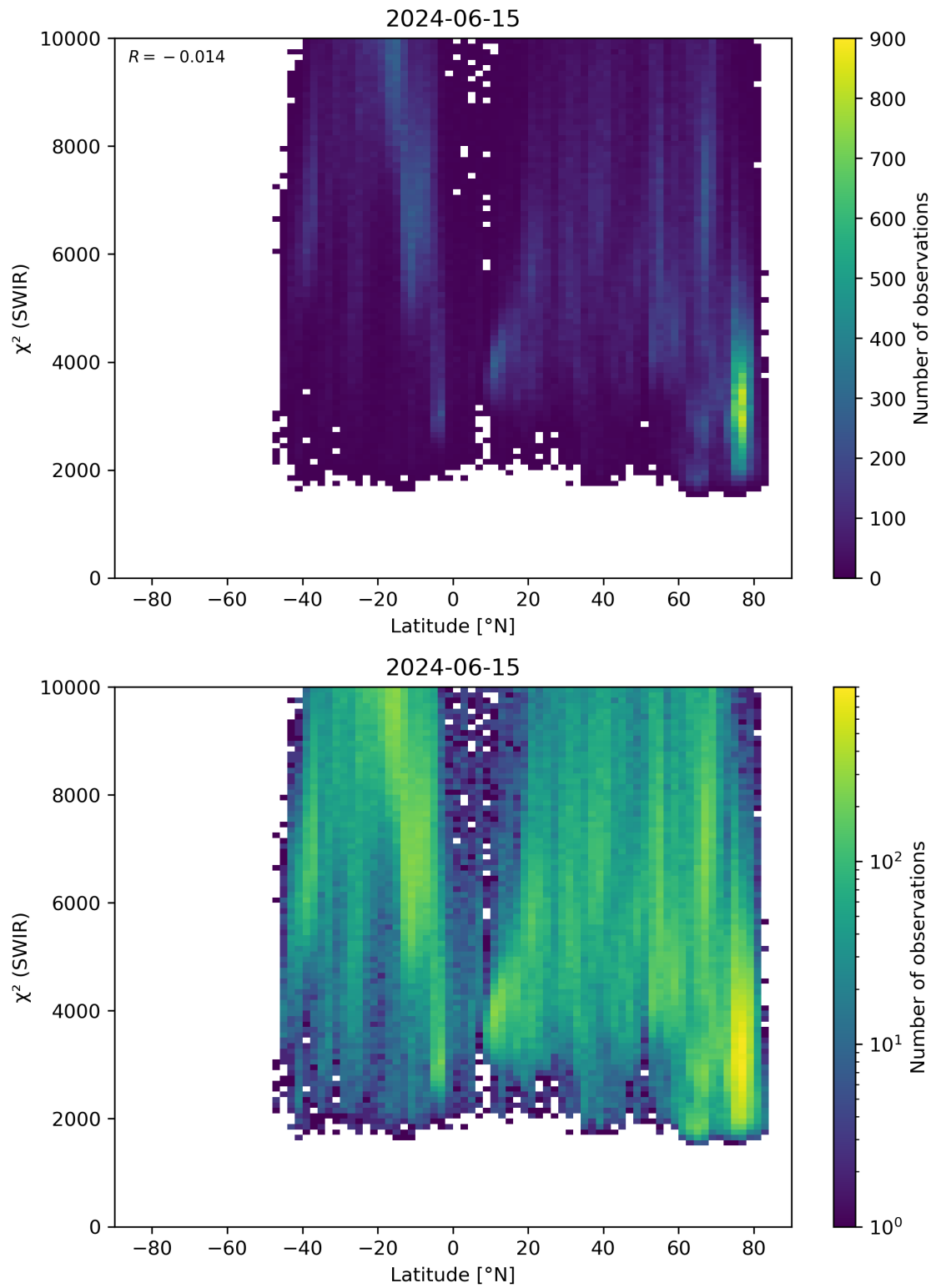
Figure 54: Scatter density plot of “Latitude” against “ \chi^2 (SWIR)” for 2024-06-14 to 2024-06-16.
