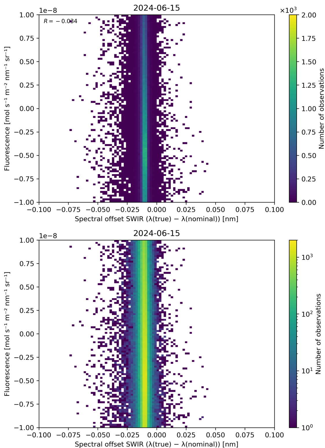
Figure 120: Scatter density plot of “Spectral offset SWIR ( \lambda(\text{true}) - \lambda(\text{nominal}) )” against “Fluorescence” for 2024-06-14 to 2024-06-16.
