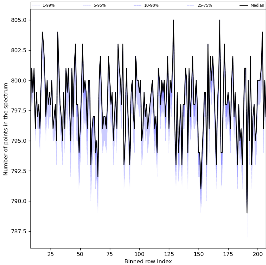
Figure 37: Along track statistics of “Number of points in the spectrum” for 2024-06-14 to 2024-06-16
