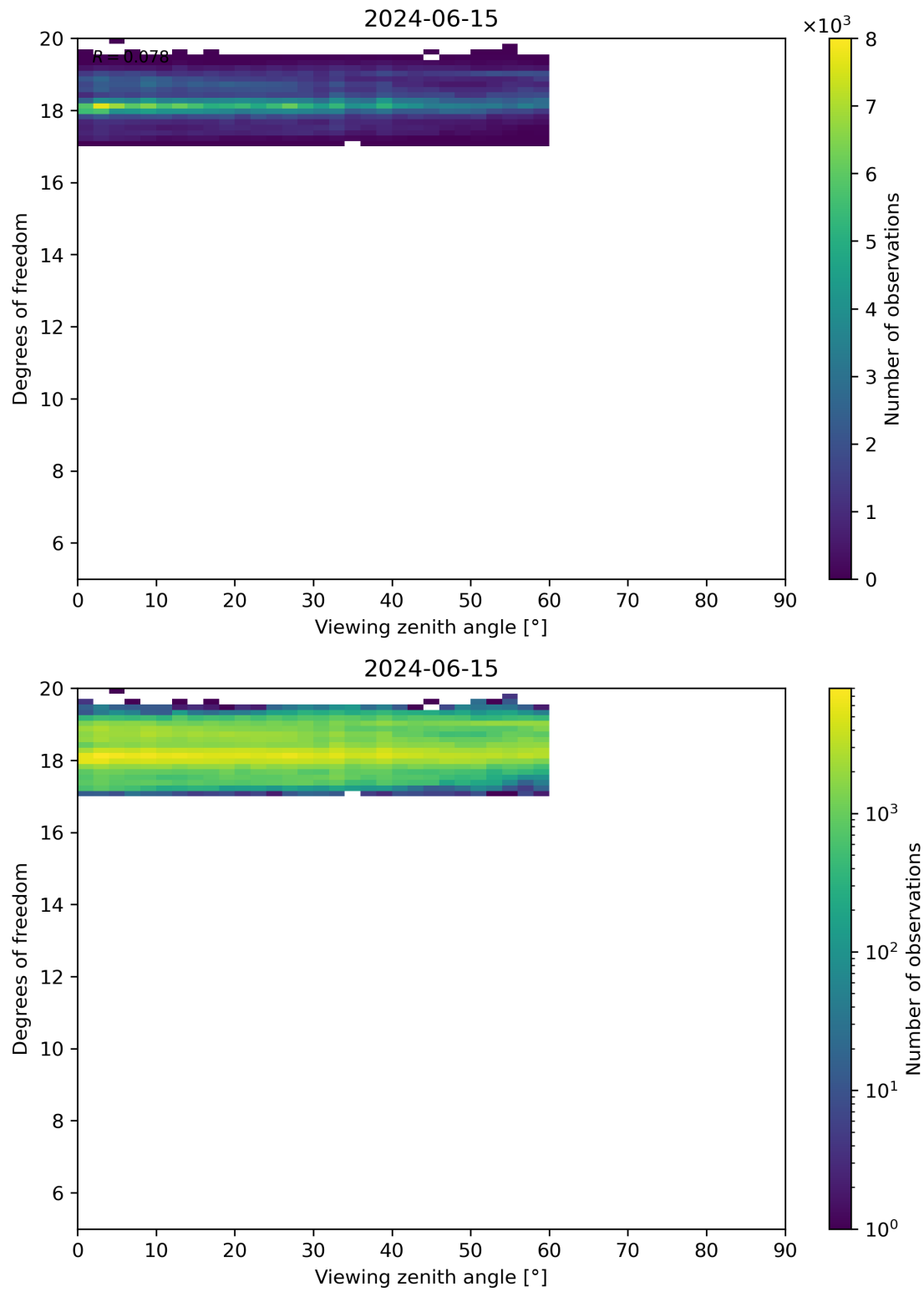
Figure 107: Scatter density plot of “Viewing zenith angle” against “Degrees of freedom” for 2024-06-14 to 2024-06-16.
