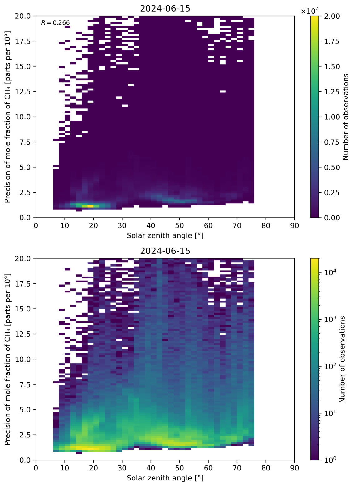
Figure 101: Scatter density plot of “Solar zenith angle” against “Precision of mole fraction of CH 4 ” for 2024-06-14 to 2024-06-16.
