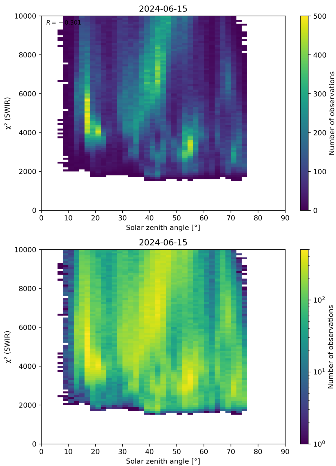
Figure 95: Scatter density plot of “Solar zenith angle” against “ \chi^2 (SWIR)” for 2024-06-14 to 2024-06-16.
