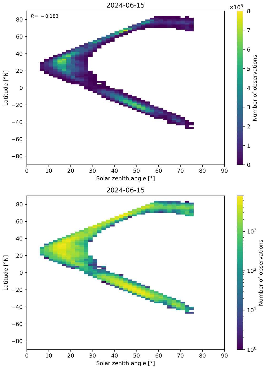
Figure 98: Scatter density plot of “Solar zenith angle” against “Latitude” for 2024-06-14 to 2024-06-16.
