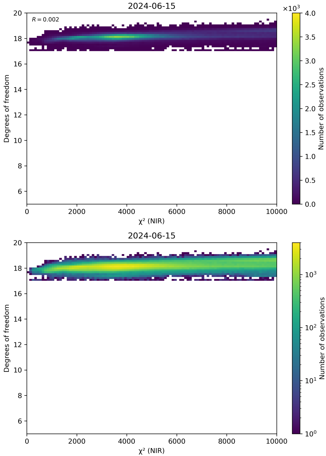
Figure 44: Scatter density plot of “ \chi^2 (NIR)” against “Degrees of freedom” for 2024-06-14 to 2024-06-16.
