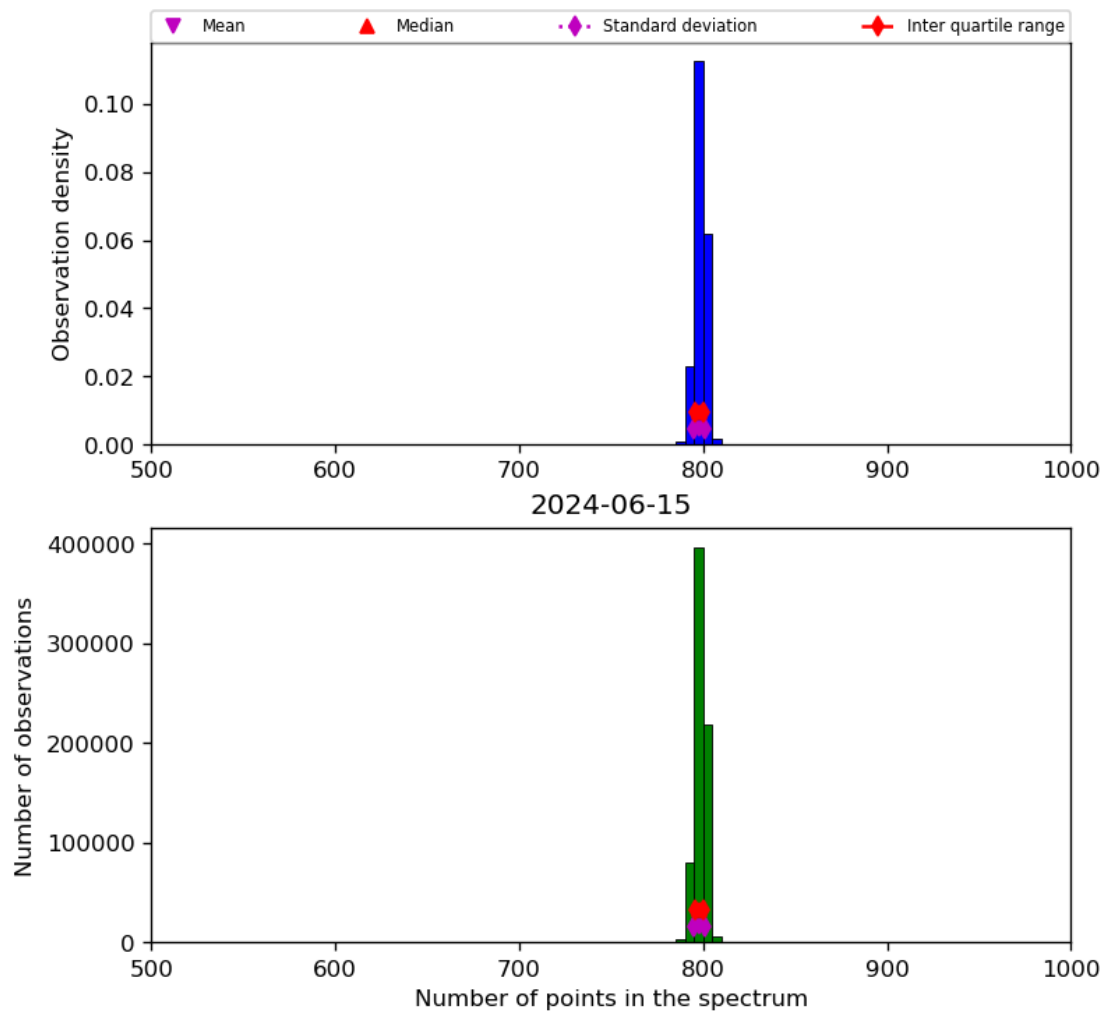
Figure 26: Histogram of “Number of points in the spectrum” for 2024-06-14 to 2024-06-16
