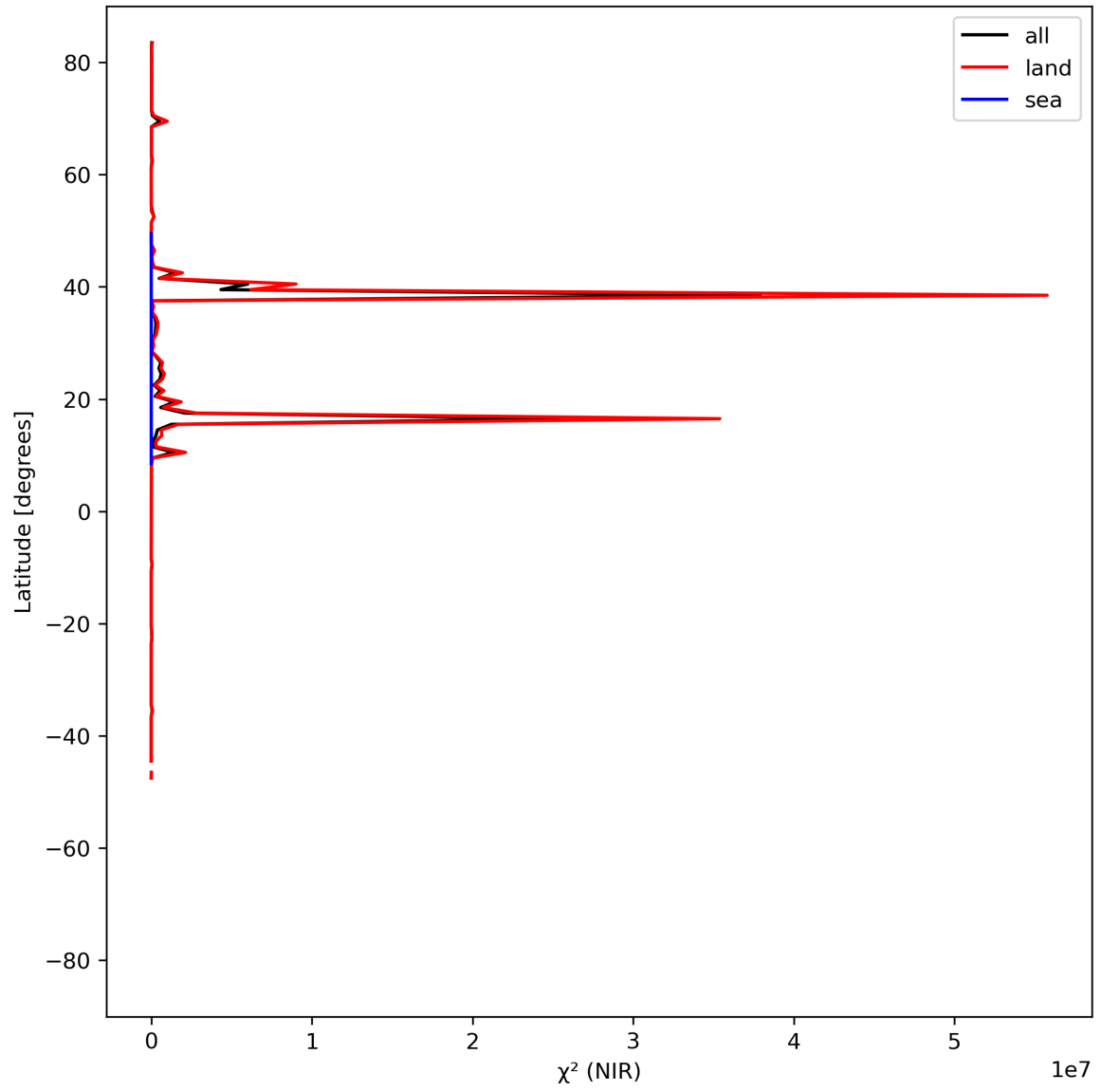
Figure 18: Zonal average of “ \chi^2 (NIR)” for 2024-06-14 to 2024-06-16.
