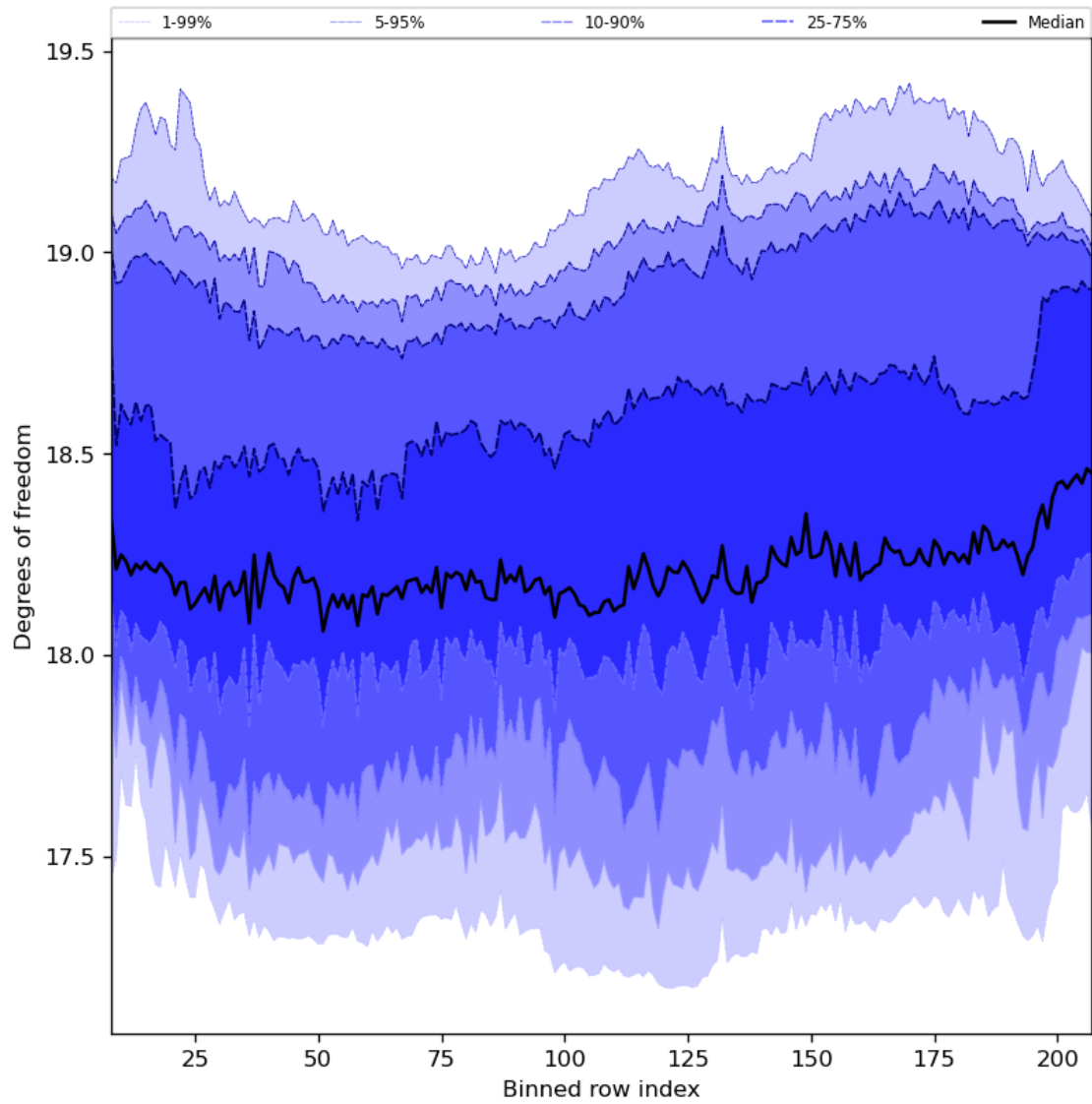
Figure 41: Along track statistics of “Degrees of freedom” for 2024-06-14 to 2024-06-16
