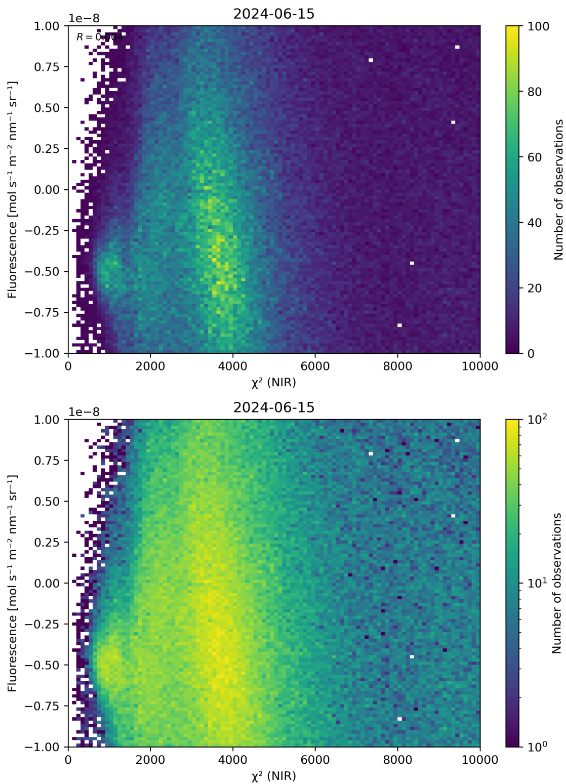
Figure 45: Scatter density plot of “ \chi^2 (NIR)” against “Fluorescence” for 2024-06-14 to 2024-06-16.
