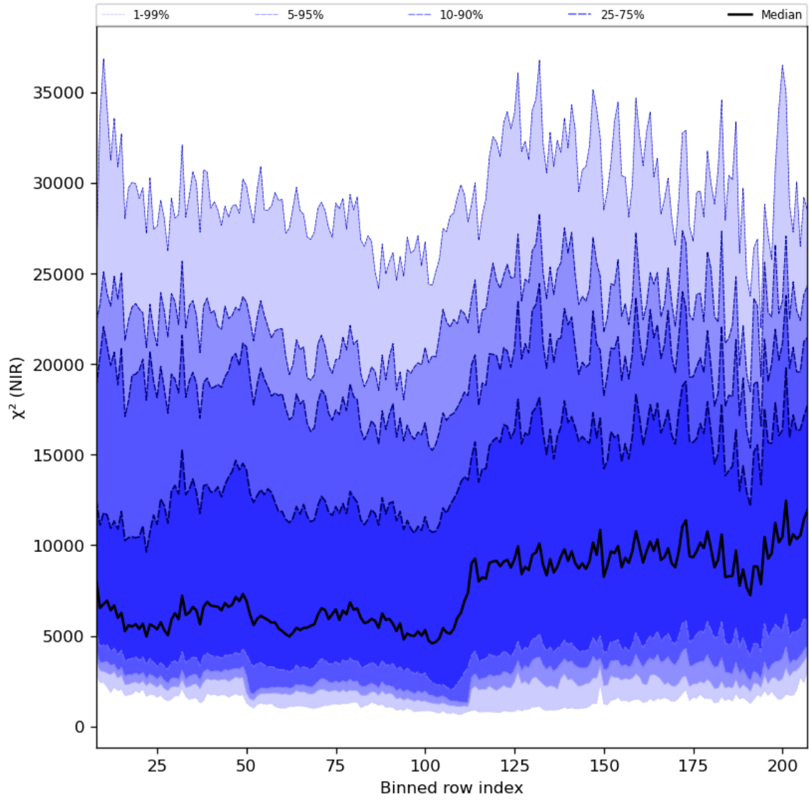
Figure 40: Along track statistics of “ \chi^2 (NIR)” for 2024-06-14 to 2024-06-16
