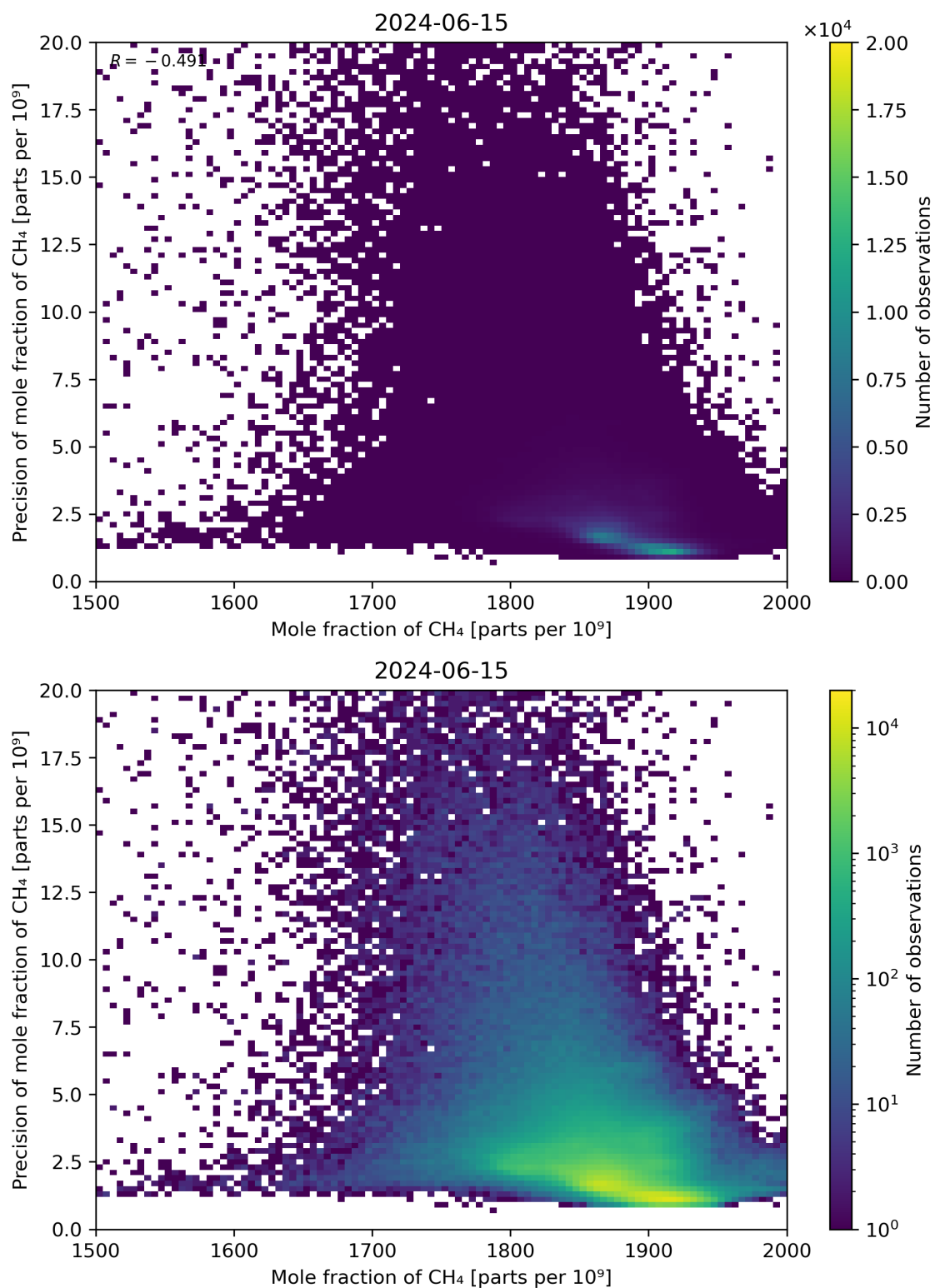
Figure 75: Scatter density plot of “Mole fraction of CH 4 ” against “Precision of mole fraction of CH 4 ” for 2024-06-14 to 2024-06-16.
