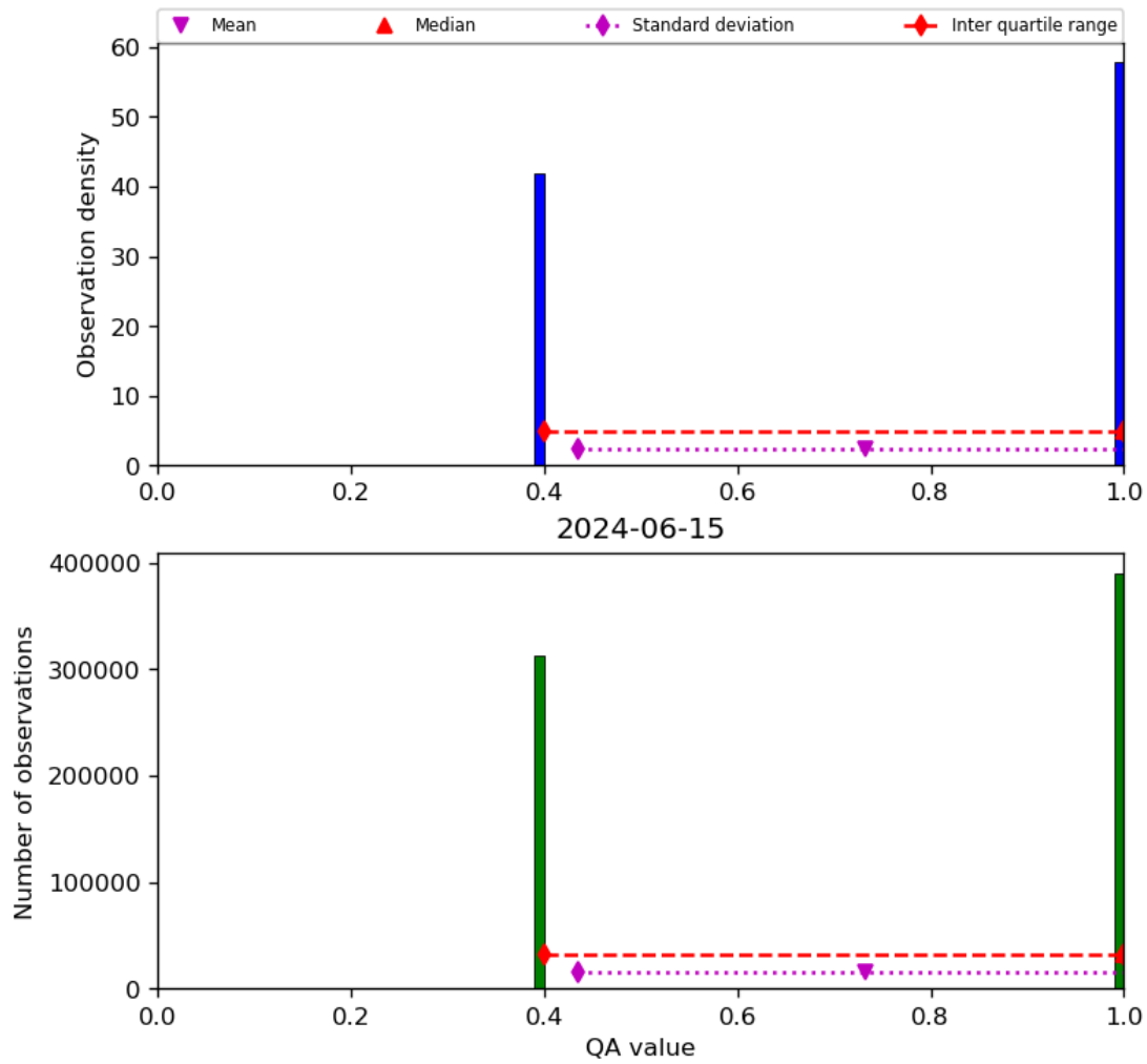
Figure 22: Histogram of “QA value” for 2024-06-14 to 2024-06-16
