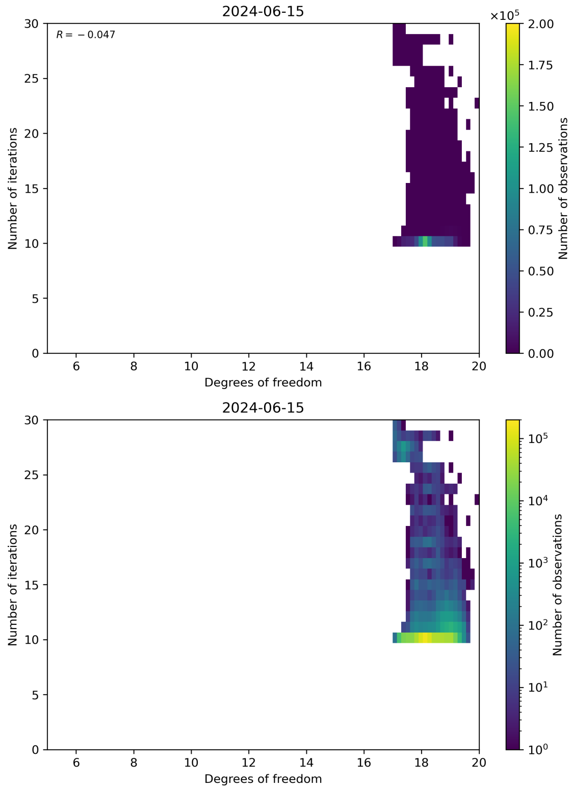
Figure 52: Scatter density plot of “Degrees of freedom” against “Number of iterations” for 2024-06-14 to 2024-06-16.
