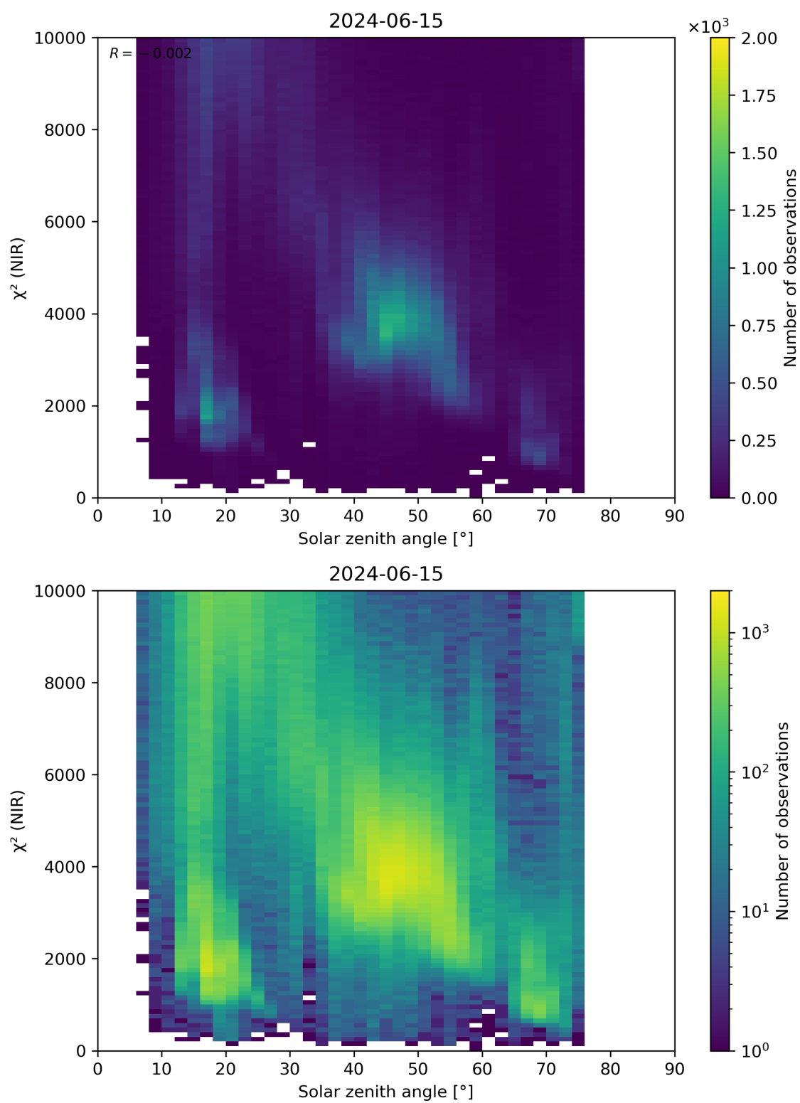
Figure 94: Scatter density plot of “Solar zenith angle” against “ \chi^2 (NIR)” for 2024-06-14 to 2024-06-16.
