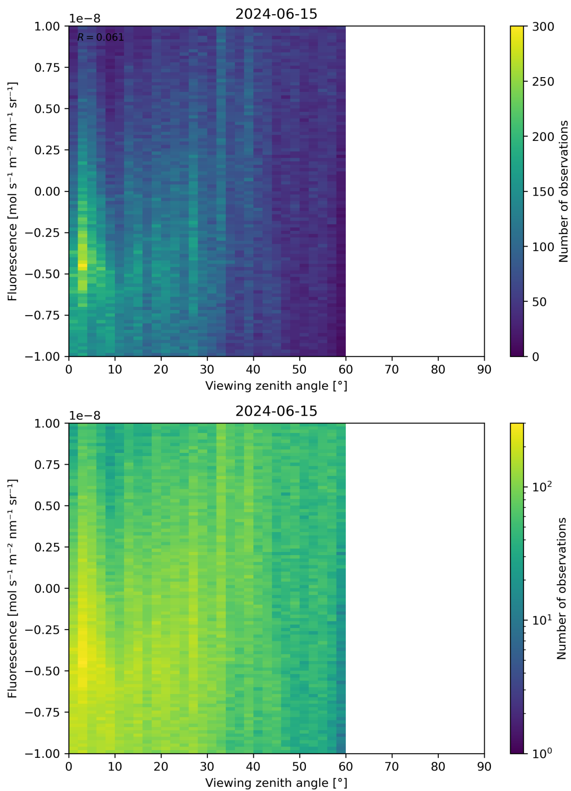
Figure 108: Scatter density plot of “Viewing zenith angle” against “Fluorescence” for 2024-06-14 to 2024-06-16.
