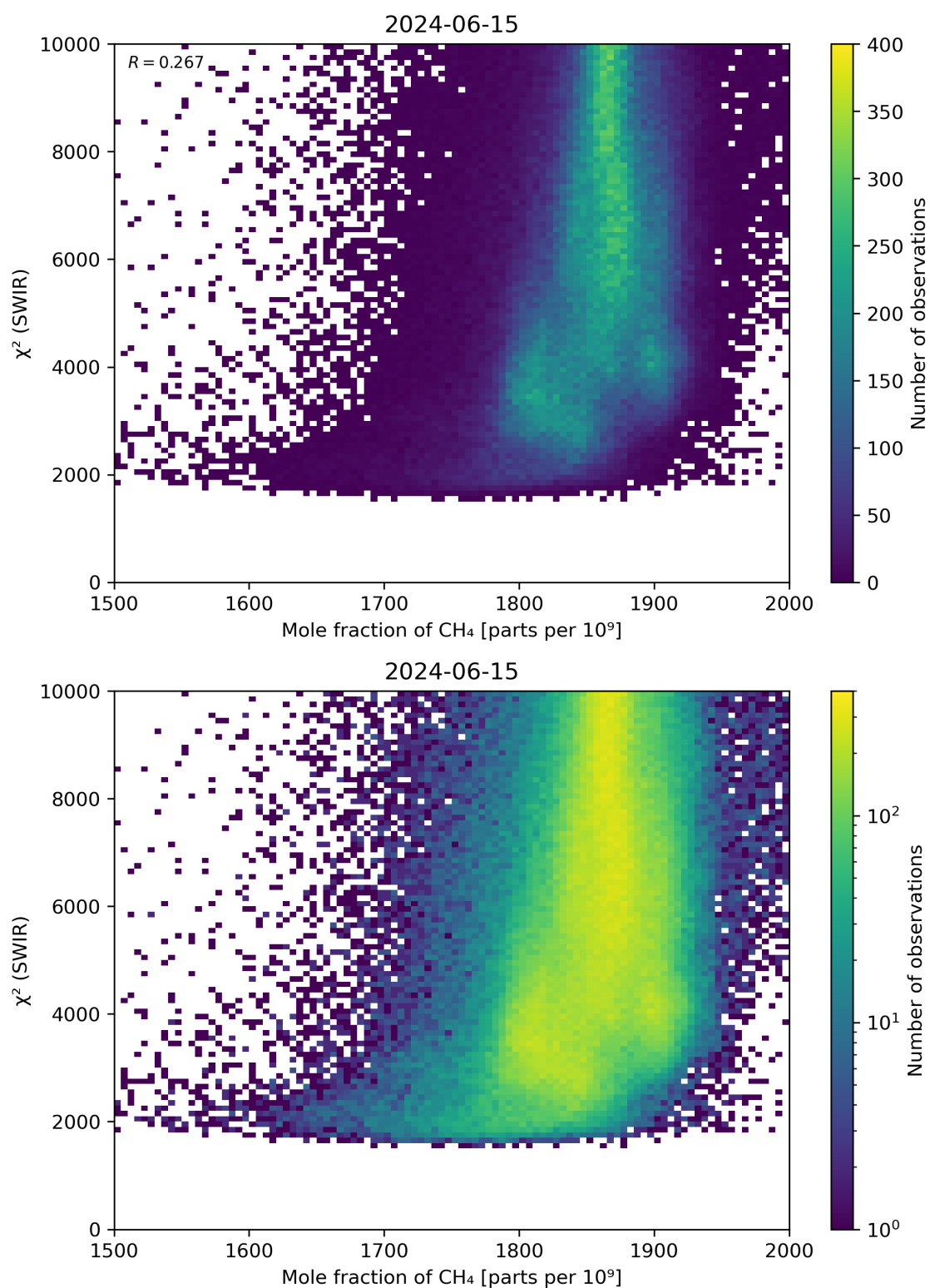
Figure 71: Scatter density plot of “Mole fraction of \text{CH}_4 ” against “ \chi^2 (SWIR)” for 2024-06-14 to 2024-06-16.
