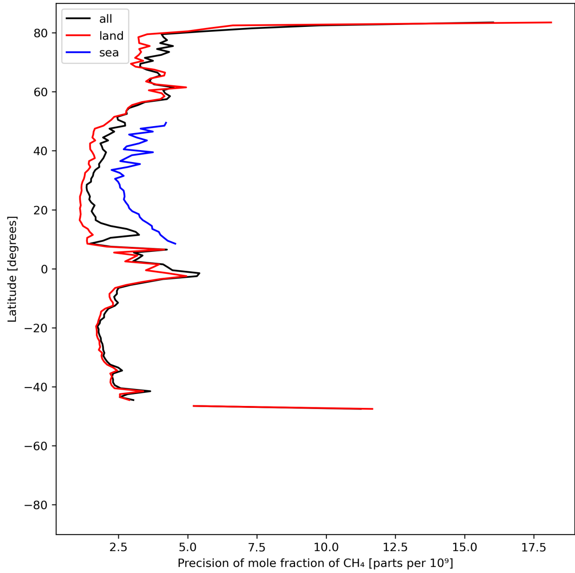
Figure 13: Zonal average of “Precision of mole fraction of CH 4 ” for 2024-06-14 to 2024-06-16.
