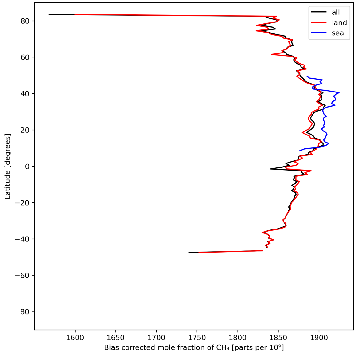
Figure 14: Zonal average of “Bias corrected mole fraction of CH 4 ” for 2024-06-14 to 2024-06-16.
