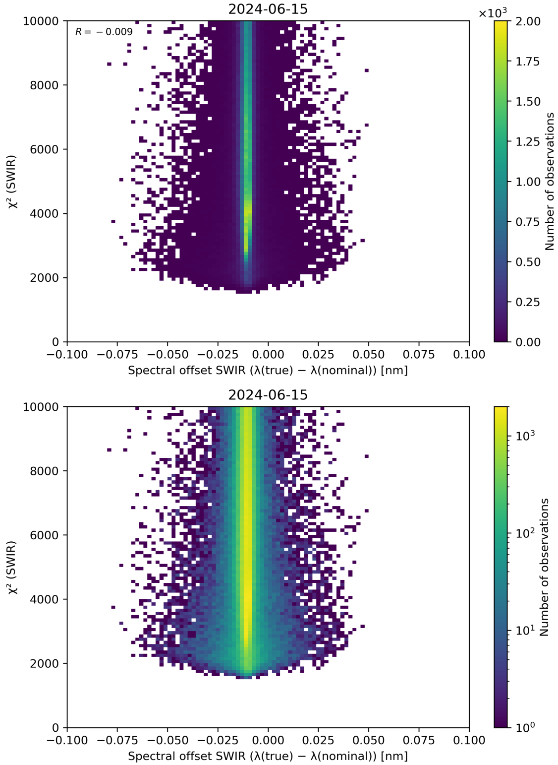
Figure 118: Scatter density plot of “Spectral offset SWIR ( \lambda(\text{true}) - \lambda(\text{nominal}) )” against “ \chi^2 (SWIR)” for 2024-06-14 to 2024-06-16.
