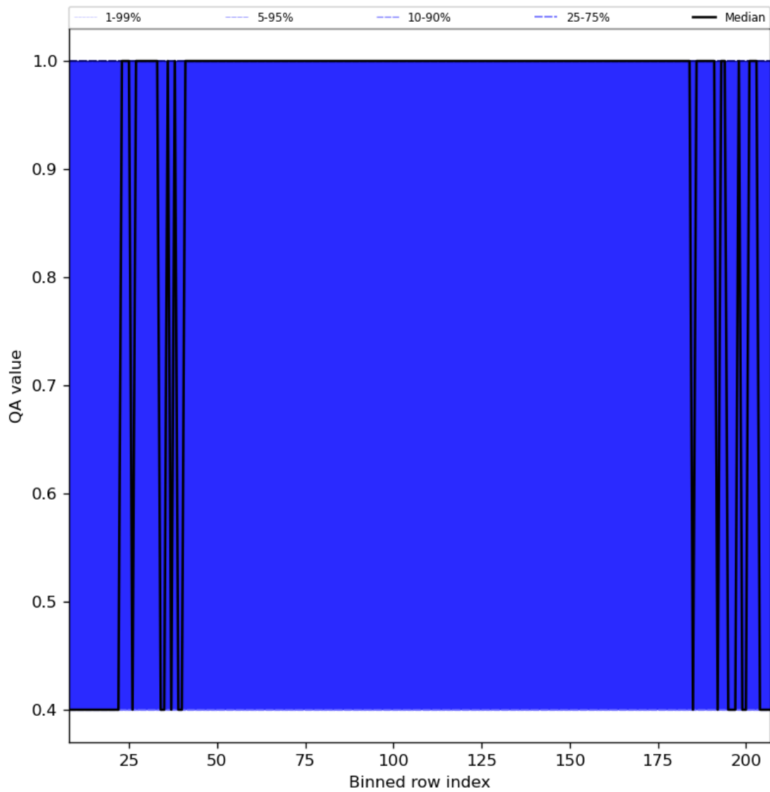
Figure 33: Along track statistics of “QA value” for 2024-06-14 to 2024-06-16
