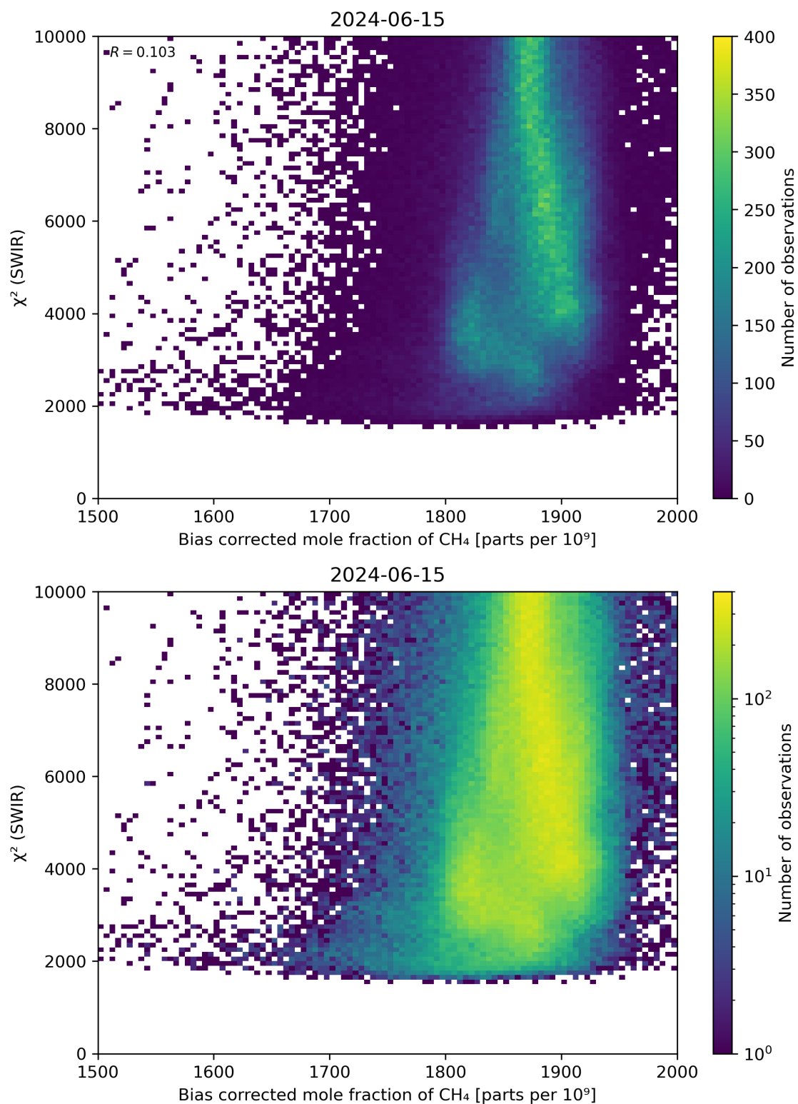
Figure 64: Scatter density plot of “Bias corrected mole fraction of CH 4 ” against “ \chi^2 (SWIR)” for 2024-06-14 to 2024-06-16.
