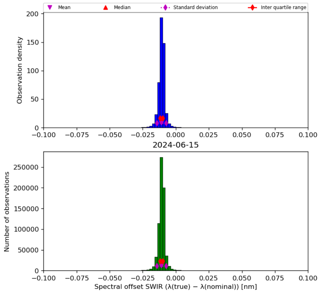
Figure 27: Histogram of “Spectral offset SWIR ( \lambda(\text{true}) - \lambda(\text{nominal}) )” for 2024-06-14 to 2024-06-16
