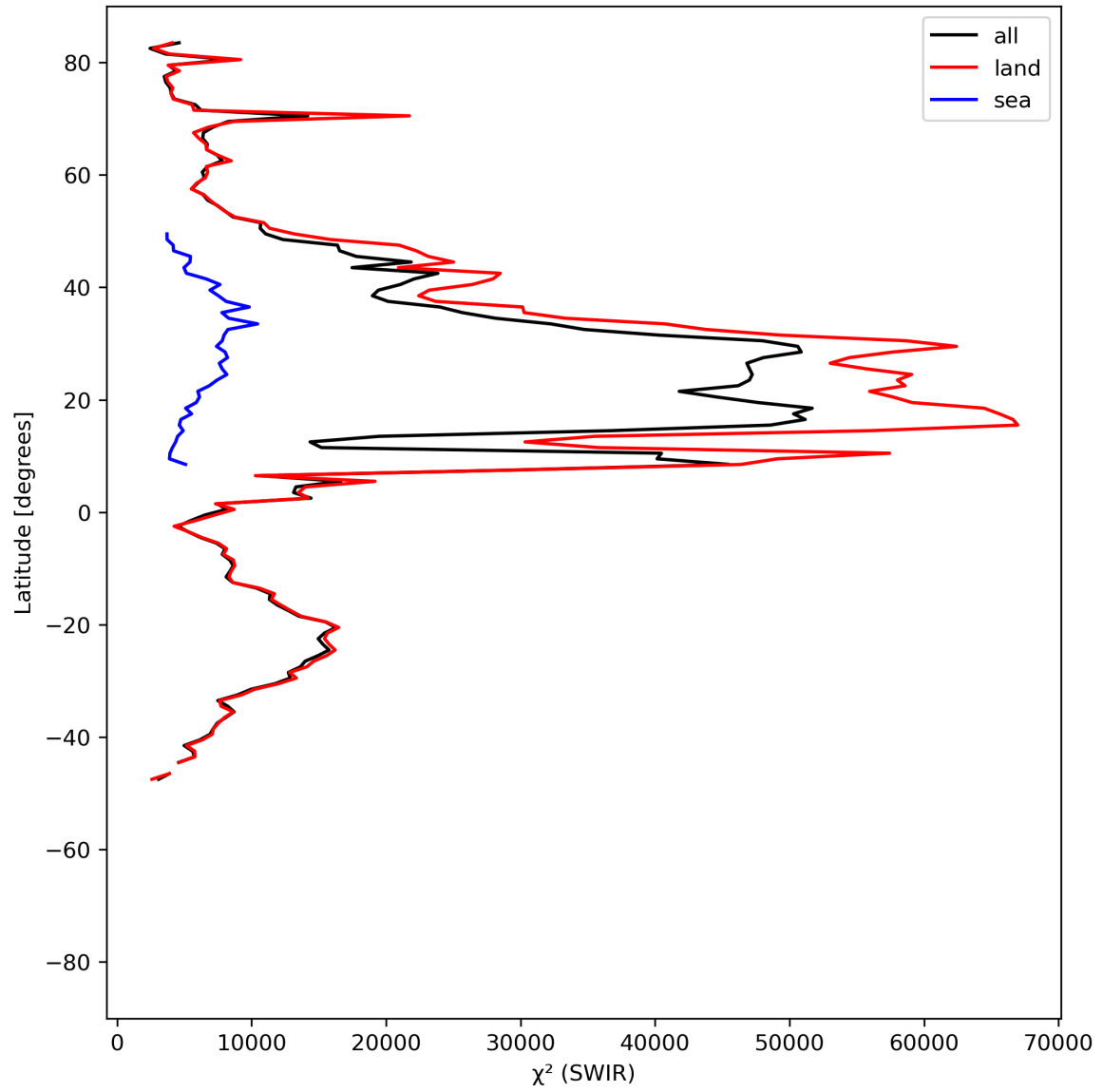
Figure 17: Zonal average of “ \chi^2 (SWIR)” for 2024-06-14 to 2024-06-16.
