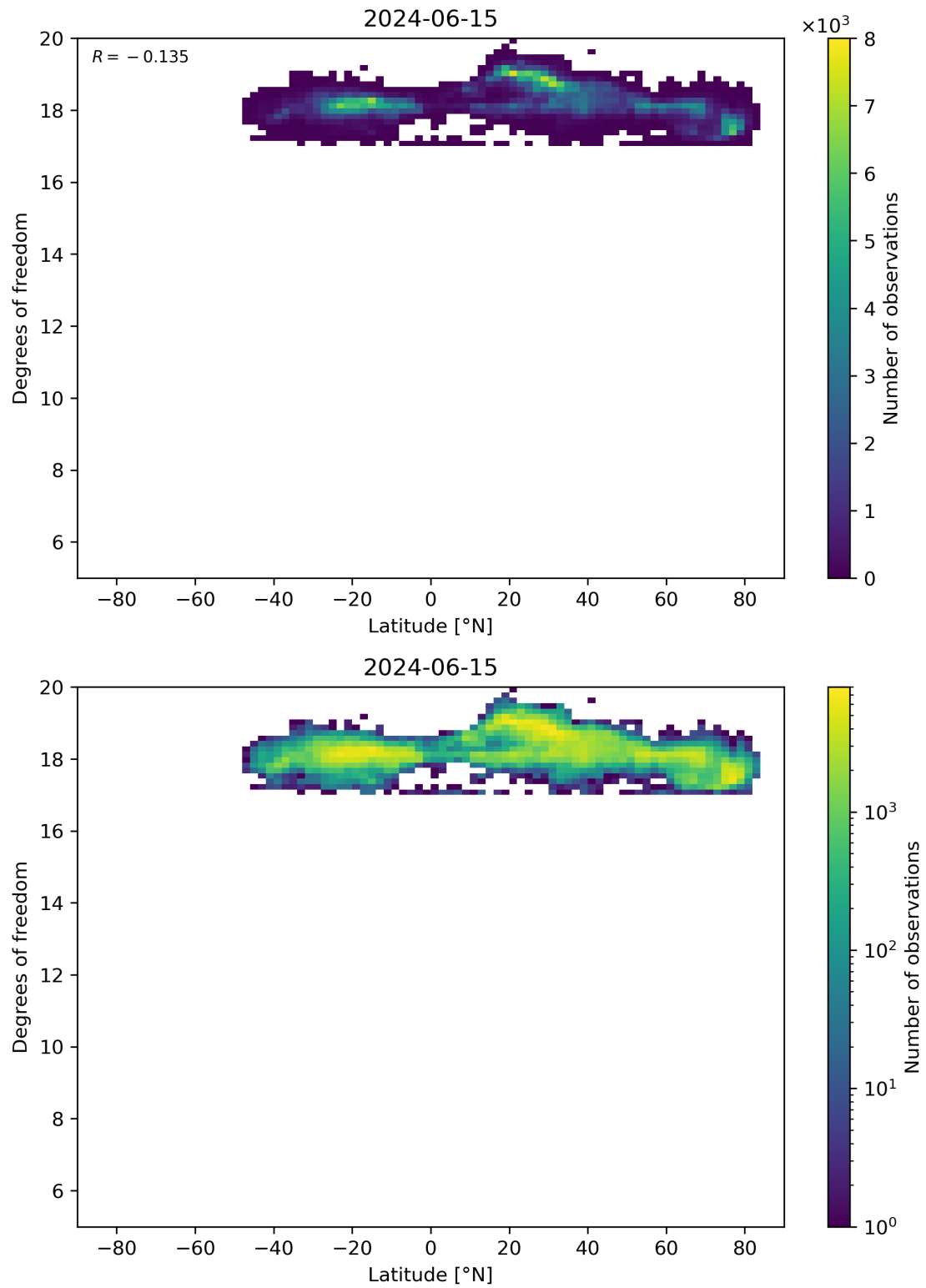
Figure 55: Scatter density plot of “Latitude” against “Degrees of freedom” for 2024-06-14 to 2024-06-16.
