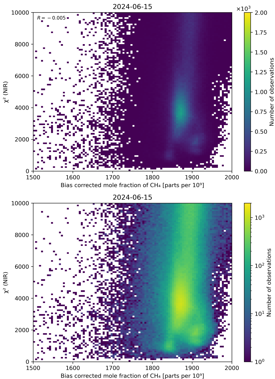
Figure 63: Scatter density plot of “Bias corrected mole fraction of CH 4 ” against “ \chi^2 (NIR)” for 2024-06-14 to 2024-06-16.
