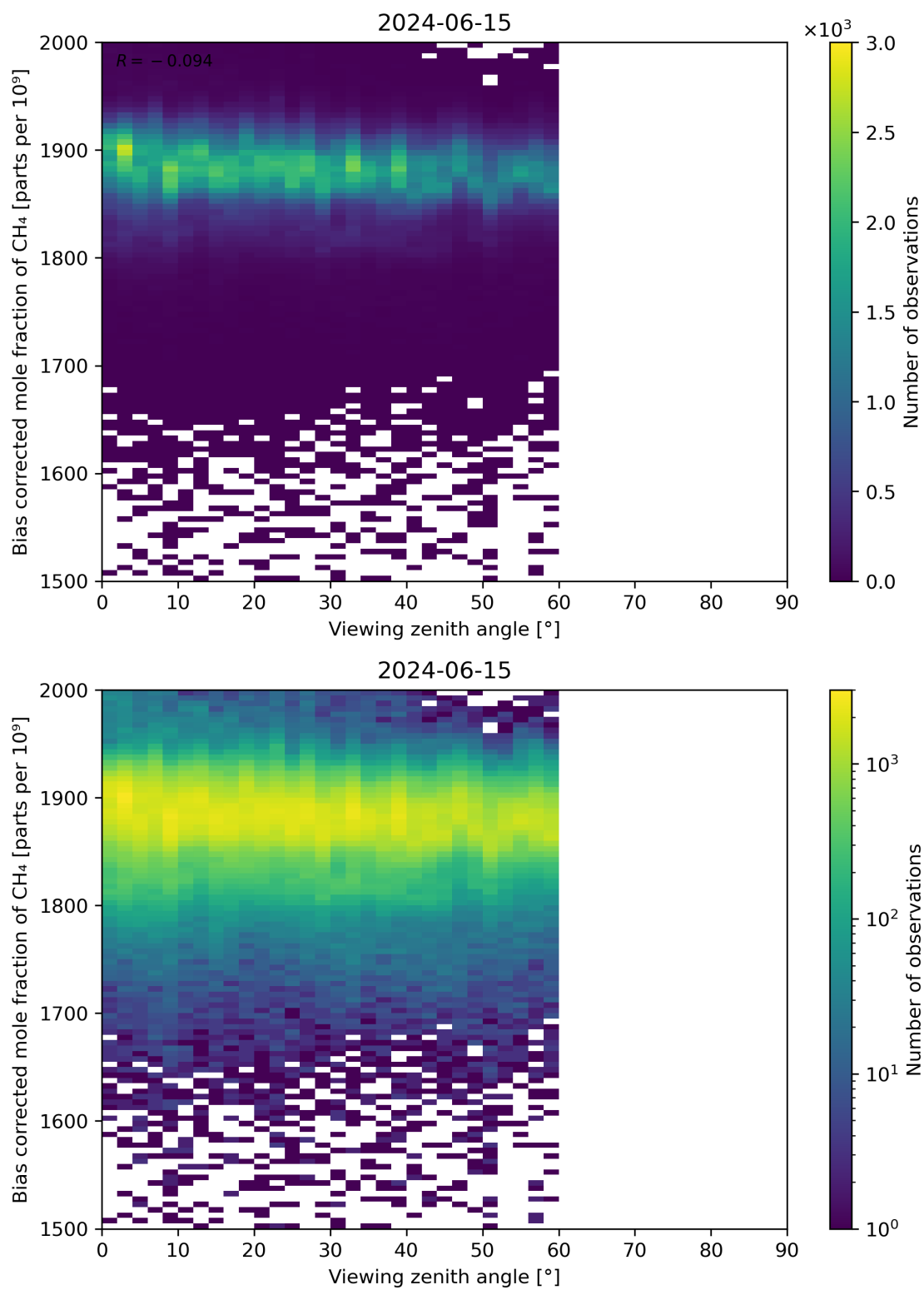
Figure 111: Scatter density plot of “Viewing zenith angle” against “Bias corrected mole fraction of CH 4 ” for 2024-06-14 to 2024-06-16.
