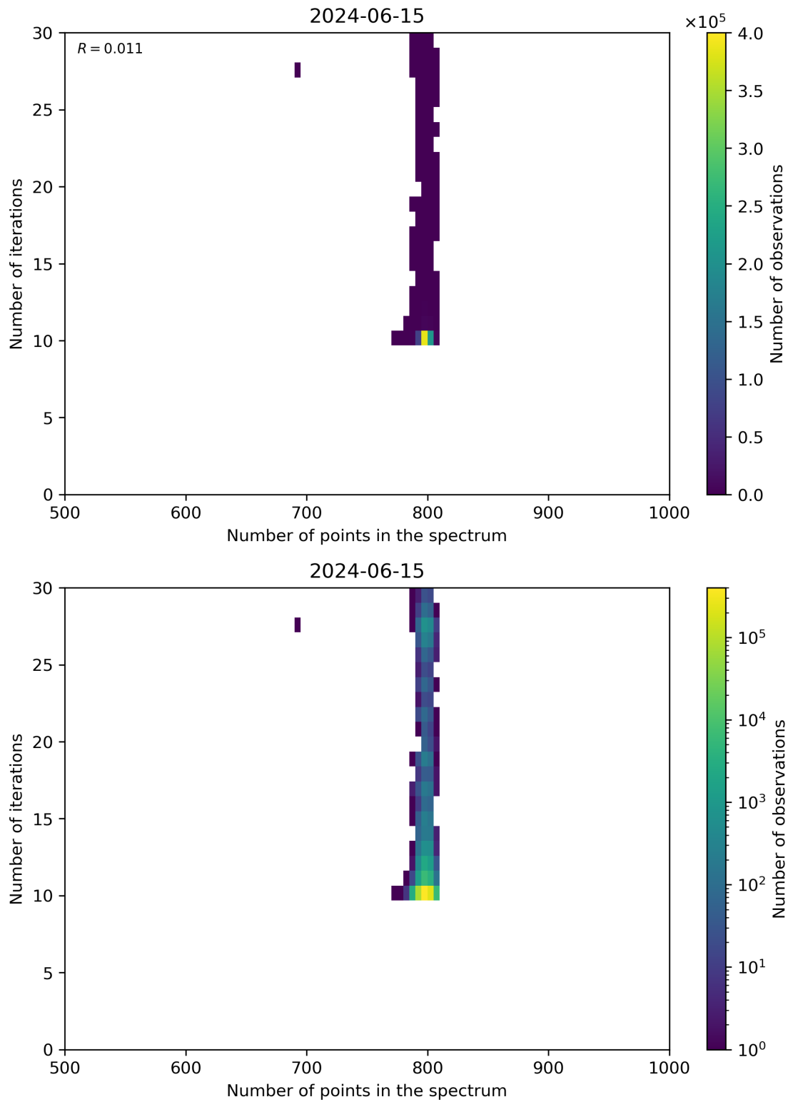
Figure 92: Scatter density plot of “Number of points in the spectrum” against “Number of iterations” for 2024-06-14 to 2024-06-16.
