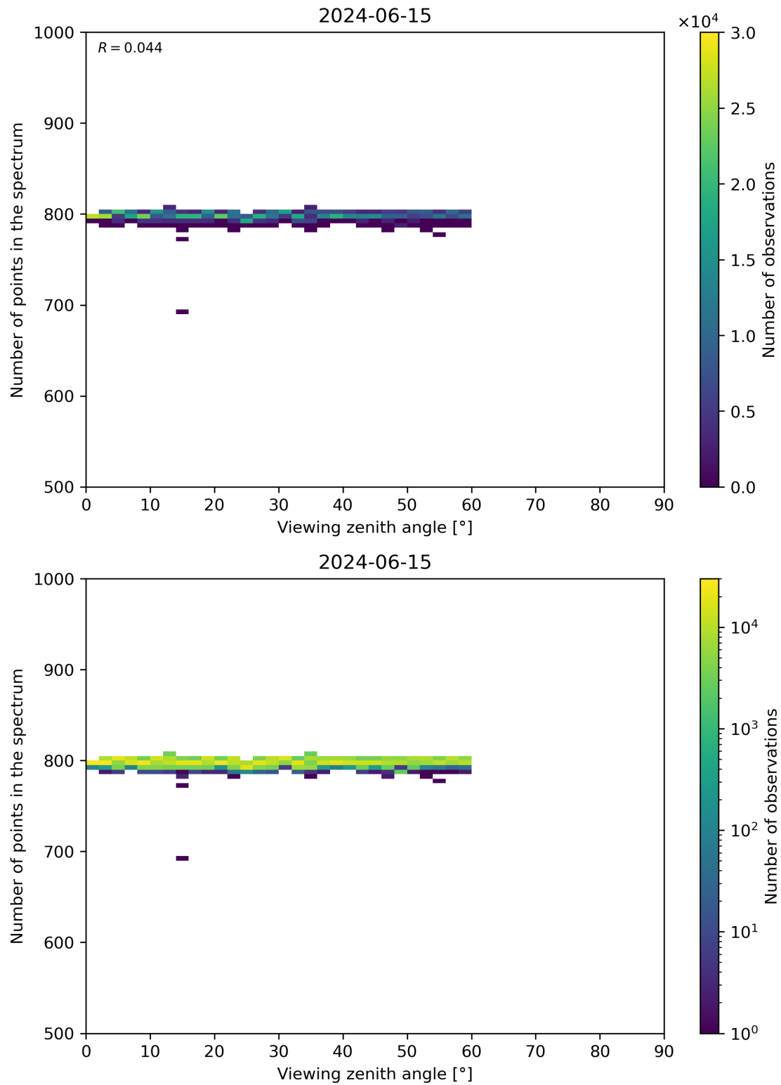
Figure 114: Scatter density plot of “Viewing zenith angle” against “Number of points in the spectrum” for 2024-06-14 to 2024-06-16.
