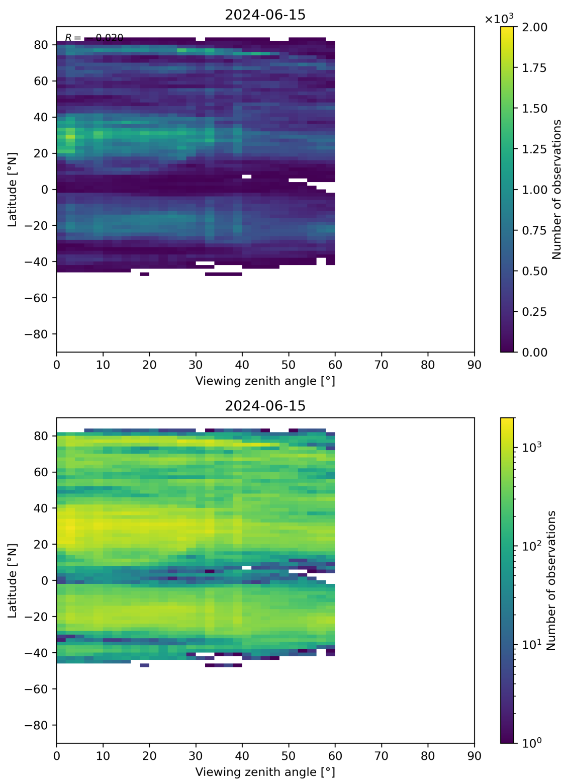
Figure 109: Scatter density plot of “Viewing zenith angle” against “Latitude” for 2024-06-14 to 2024-06-16.
