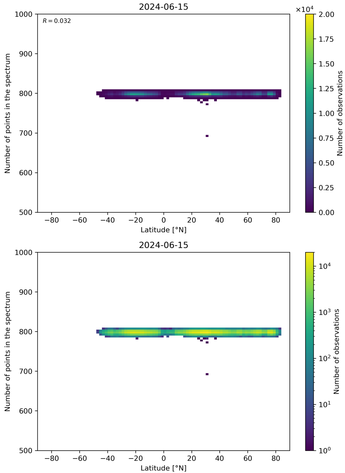
Figure 61: Scatter density plot of “Latitude” against “Number of points in the spectrum” for 2024-06-14 to 2024-06-16.
