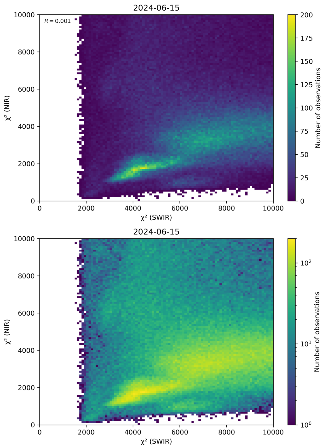
Figure 47: Scatter density plot of “ \chi^2 (SWIR)” against “ \chi^2 (NIR)” for 2024-06-14 to 2024-06-16.
