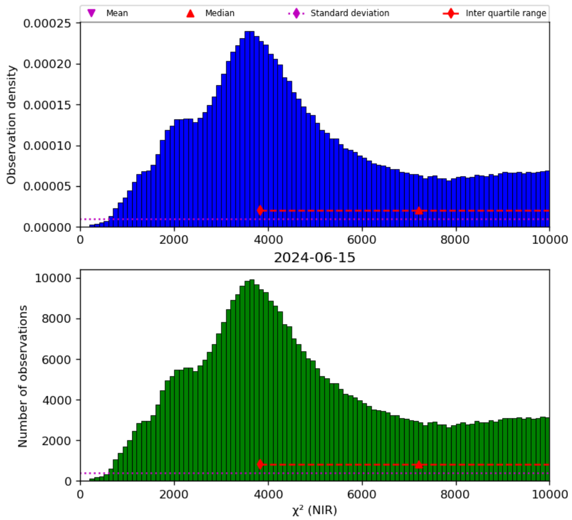
Figure 29: Histogram of “ \chi^2 (NIR)” for 2024-06-14 to 2024-06-16
