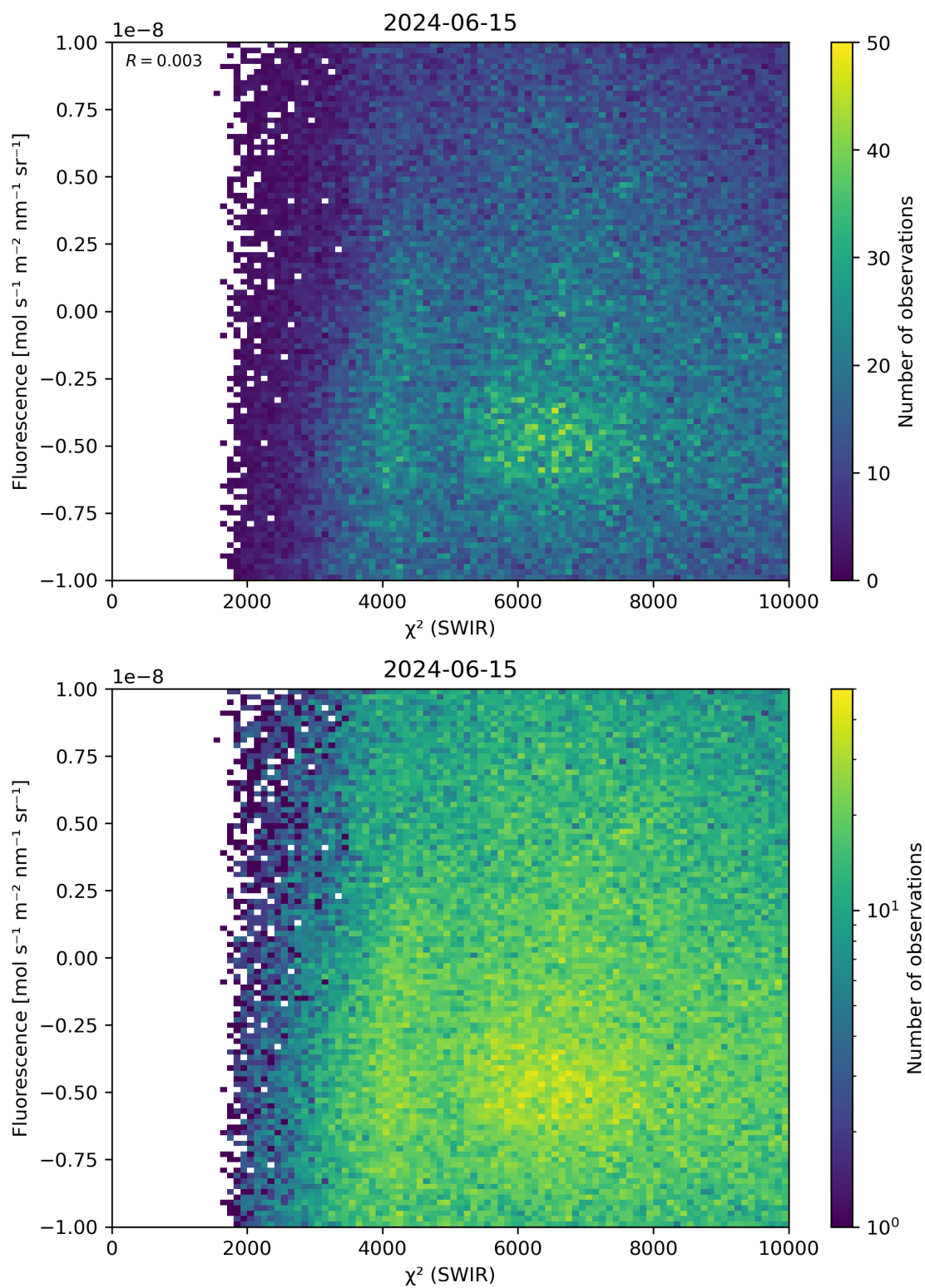
Figure 49: Scatter density plot of “ \chi^2 (SWIR)” against “Fluorescence” for 2024-06-14 to 2024-06-16.
