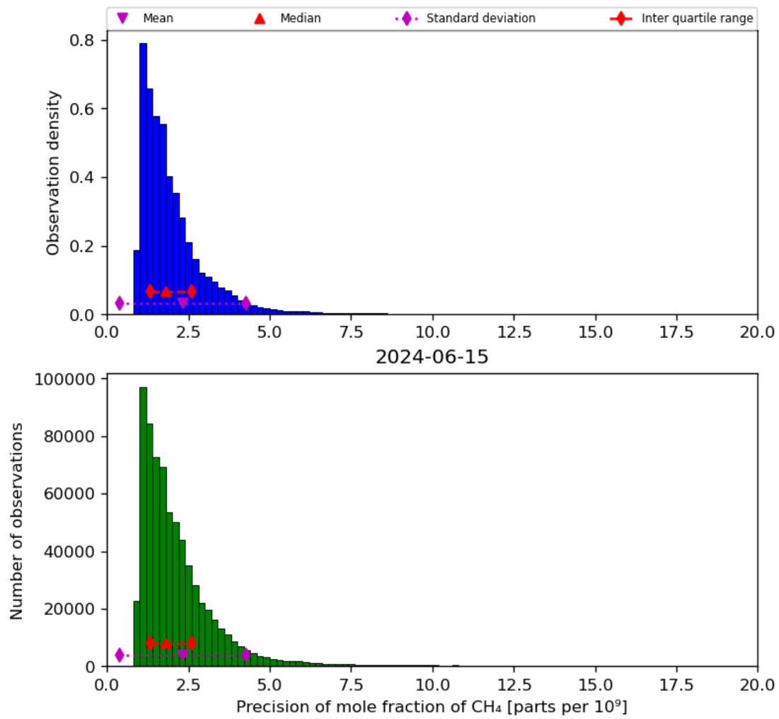
Figure 24: Histogram of “Precision of mole fraction of CH 4 ” for 2024-06-14 to 2024-06-16
