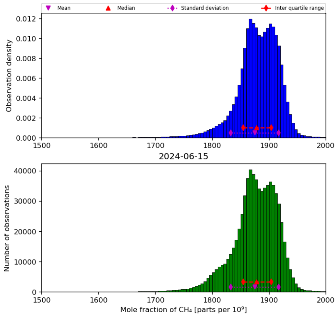
Figure 23: Histogram of “Mole fraction of CH 4 ” for 2024-06-14 to 2024-06-16
