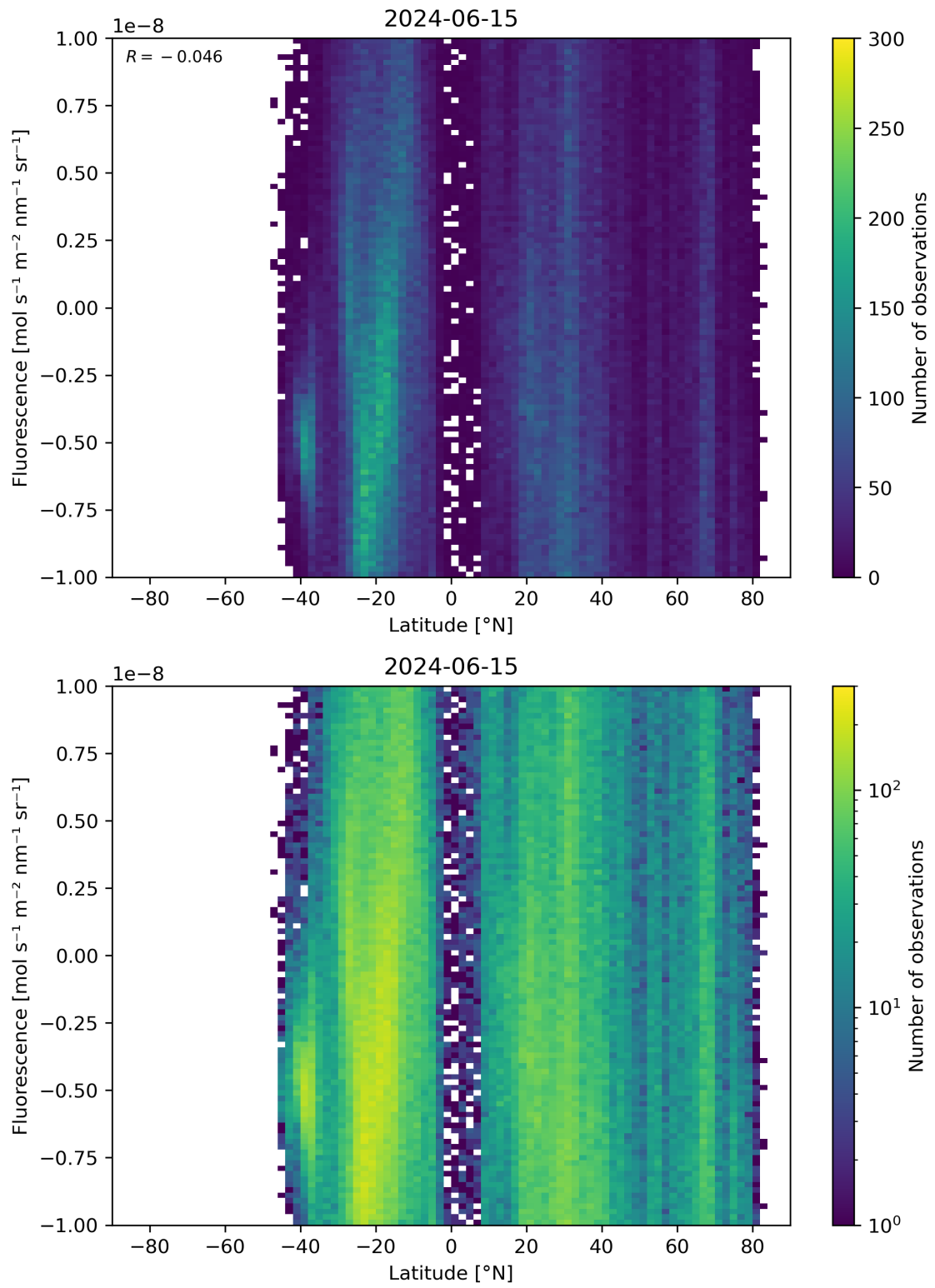
Figure 56: Scatter density plot of “Latitude” against “Fluorescence” for 2024-06-14 to 2024-06-16.
