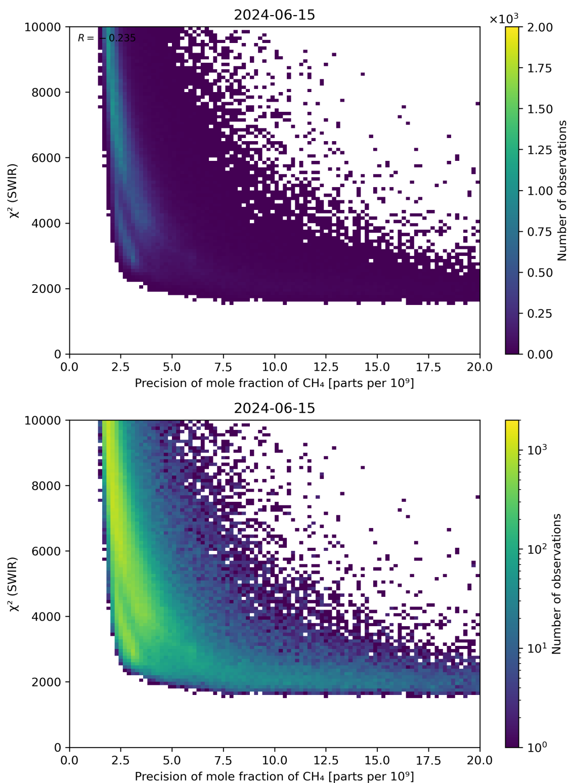
Figure 79: Scatter density plot of “Precision of mole fraction of \text{CH}_4 ” against “ \chi^2 (SWIR)” for 2024-06-14 to 2024-06-16.
