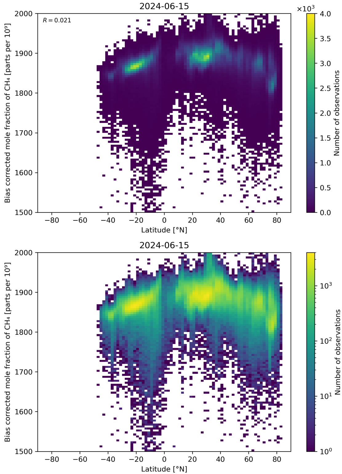
Figure 58: Scatter density plot of “Latitude” against “Bias corrected mole fraction of \text{CH}_4 ” for 2024-06-14 to 2024-06-16.
