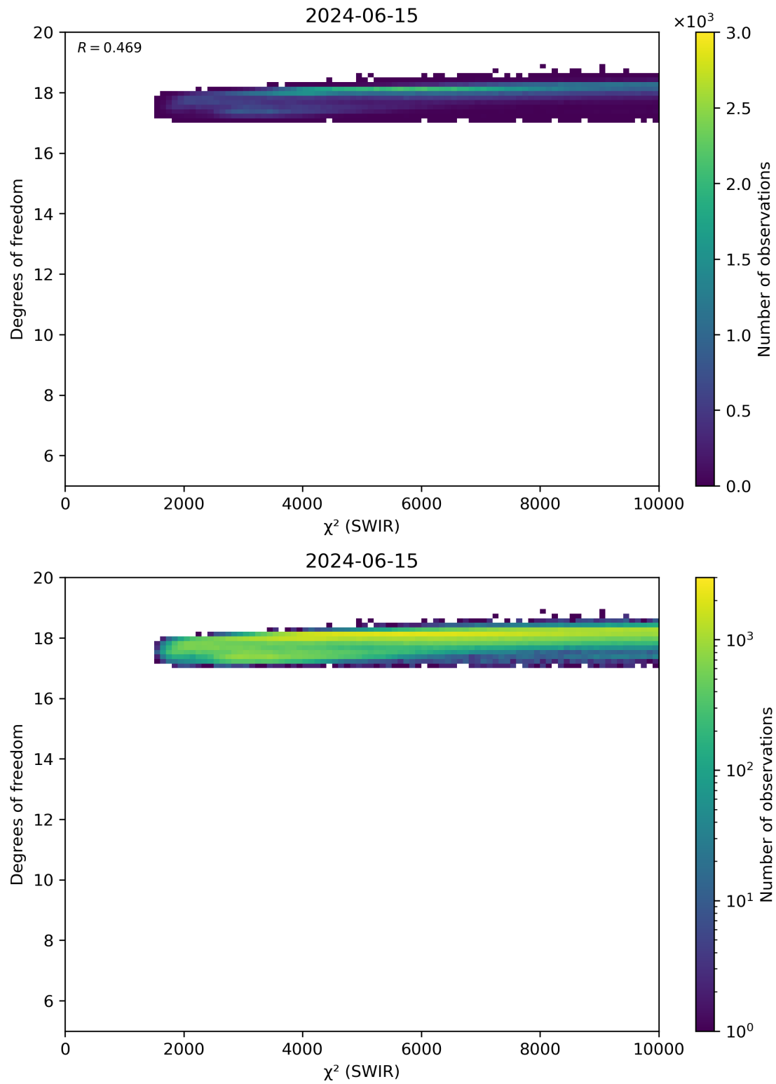
Figure 48: Scatter density plot of “ \chi^2 (SWIR)” against “Degrees of freedom” for 2024-06-14 to 2024-06-16.
