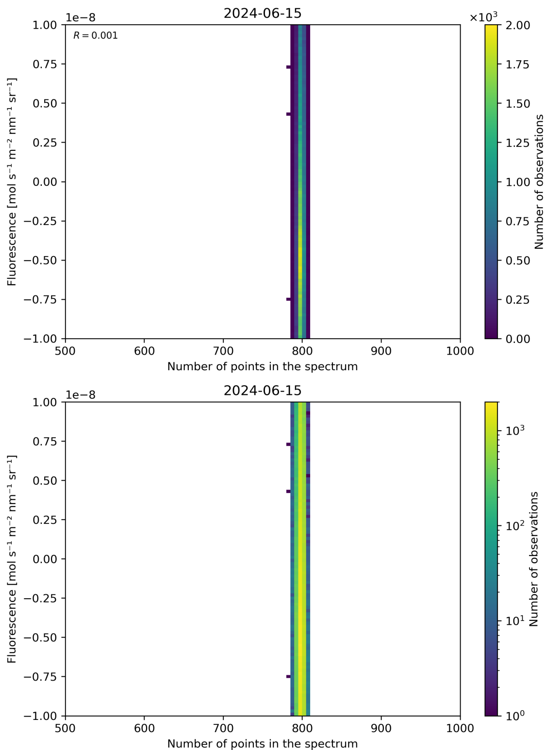
Figure 91: Scatter density plot of “Number of points in the spectrum” against “Fluorescence” for 2024-06-14 to 2024-06-16.
