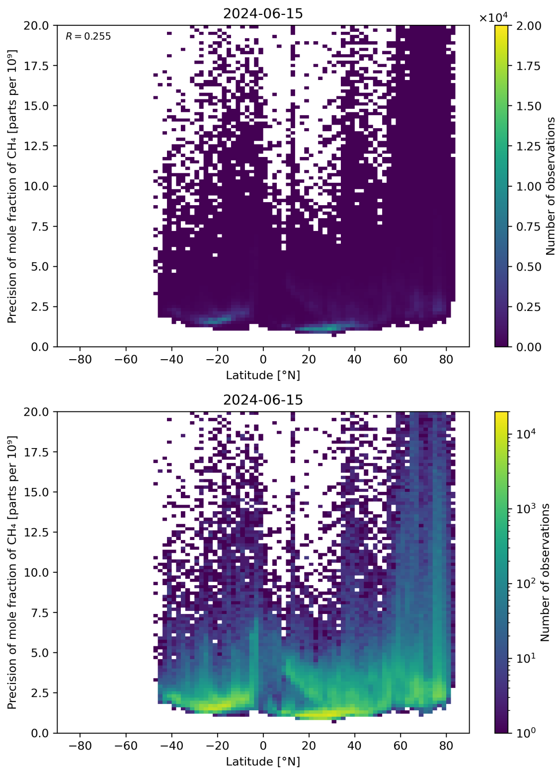
Figure 59: Scatter density plot of “Latitude” against “Precision of mole fraction of \text{CH}_4 ” for 2024-06-14 to 2024-06-16.
