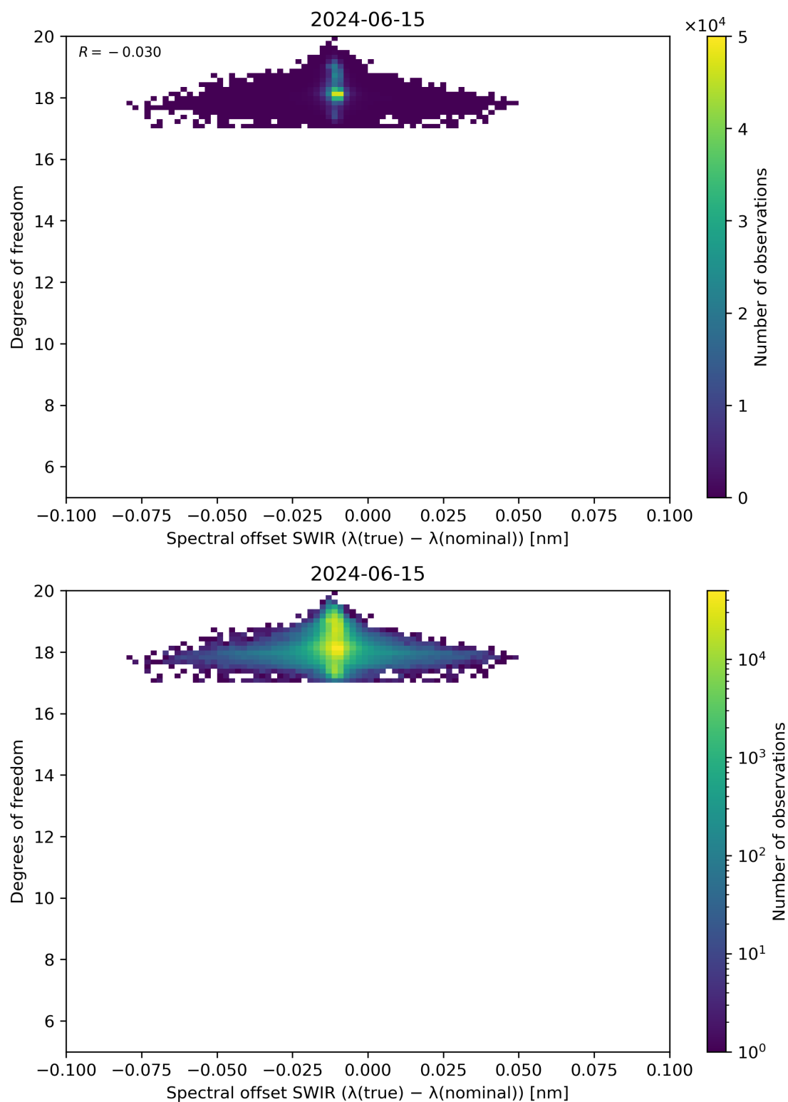
Figure 119: Scatter density plot of “Spectral offset SWIR ( \lambda(\text{true}) - \lambda(\text{nominal}) )” against “Degrees of freedom” for 2024-06-14 to 2024-06-16.
