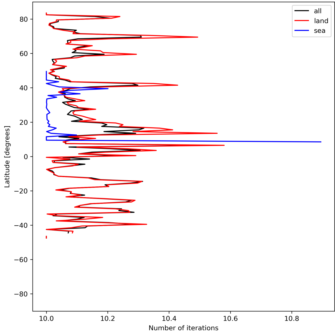
Figure 20: Zonal average of “Number of iterations” for 2024-06-14 to 2024-06-16.
