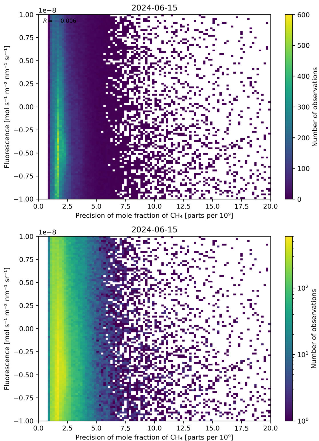
Figure 81: Scatter density plot of “Precision of mole fraction of CH 4 ” against “Fluorescence” for 2024-06-14 to 2024-06-16.
