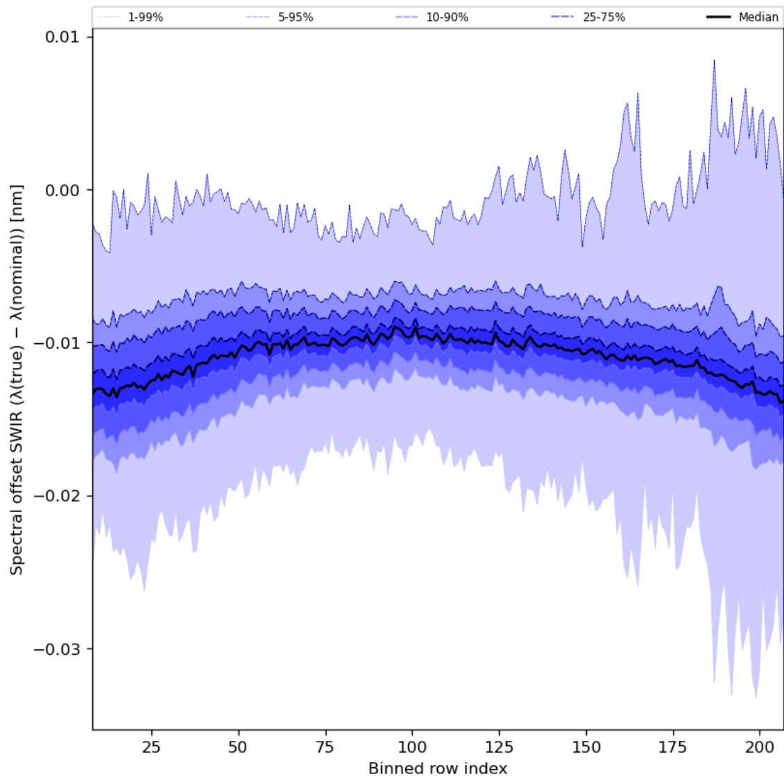
Figure 38: Along track statistics of “Spectral offset SWIR ( \lambda(\text{true}) - \lambda(\text{nominal}) )” for 2024-06-14 to 2024-06-16
