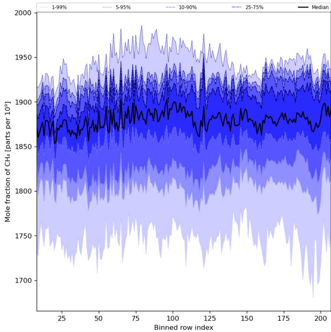
Figure 34: Along track statistics of “Mole fraction of CH 4 ” for 2024-06-14 to 2024-06-16
