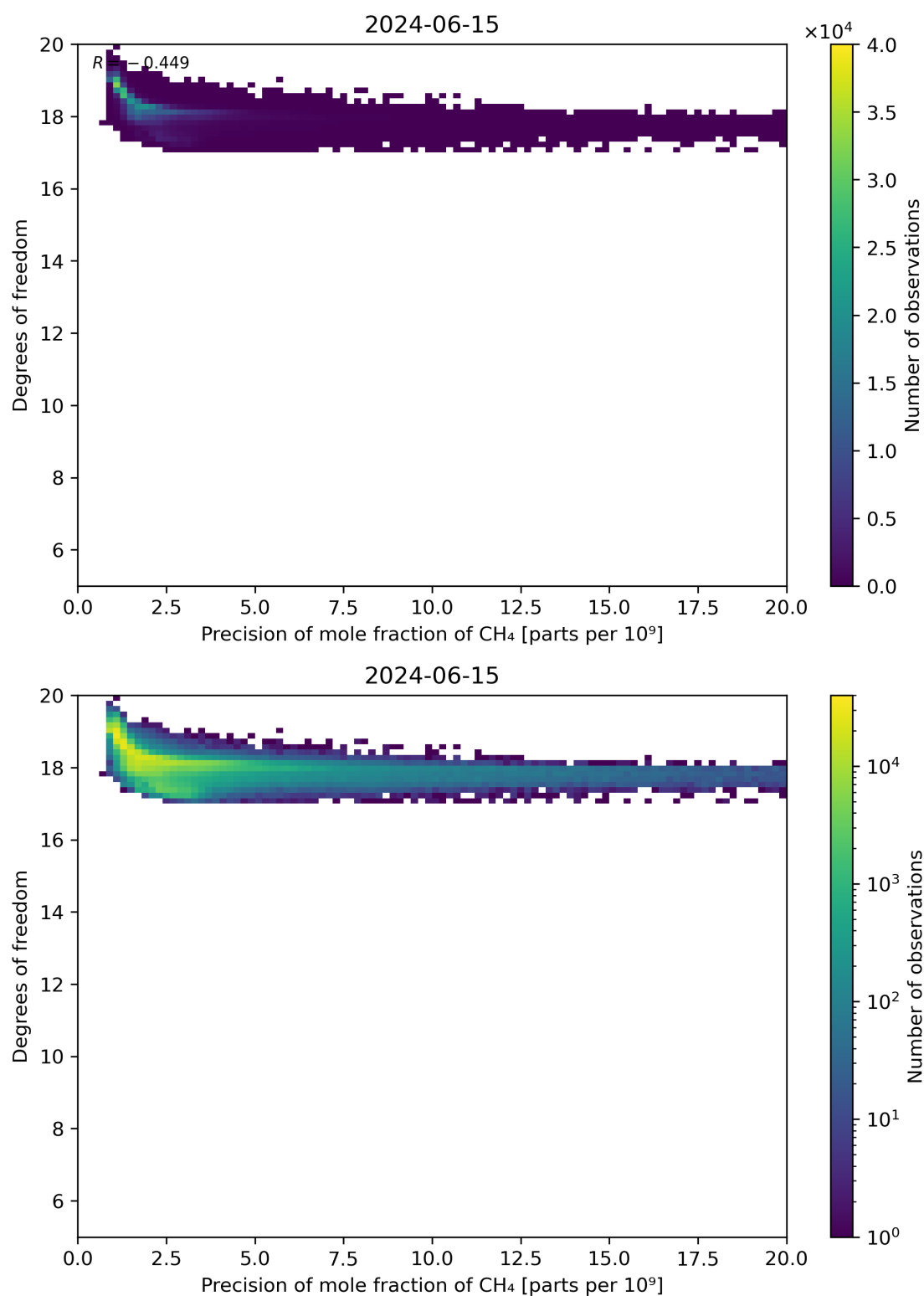
Figure 80: Scatter density plot of “Precision of mole fraction of CH 4 ” against “Degrees of freedom” for 2024-06-14 to 2024-06-16.
