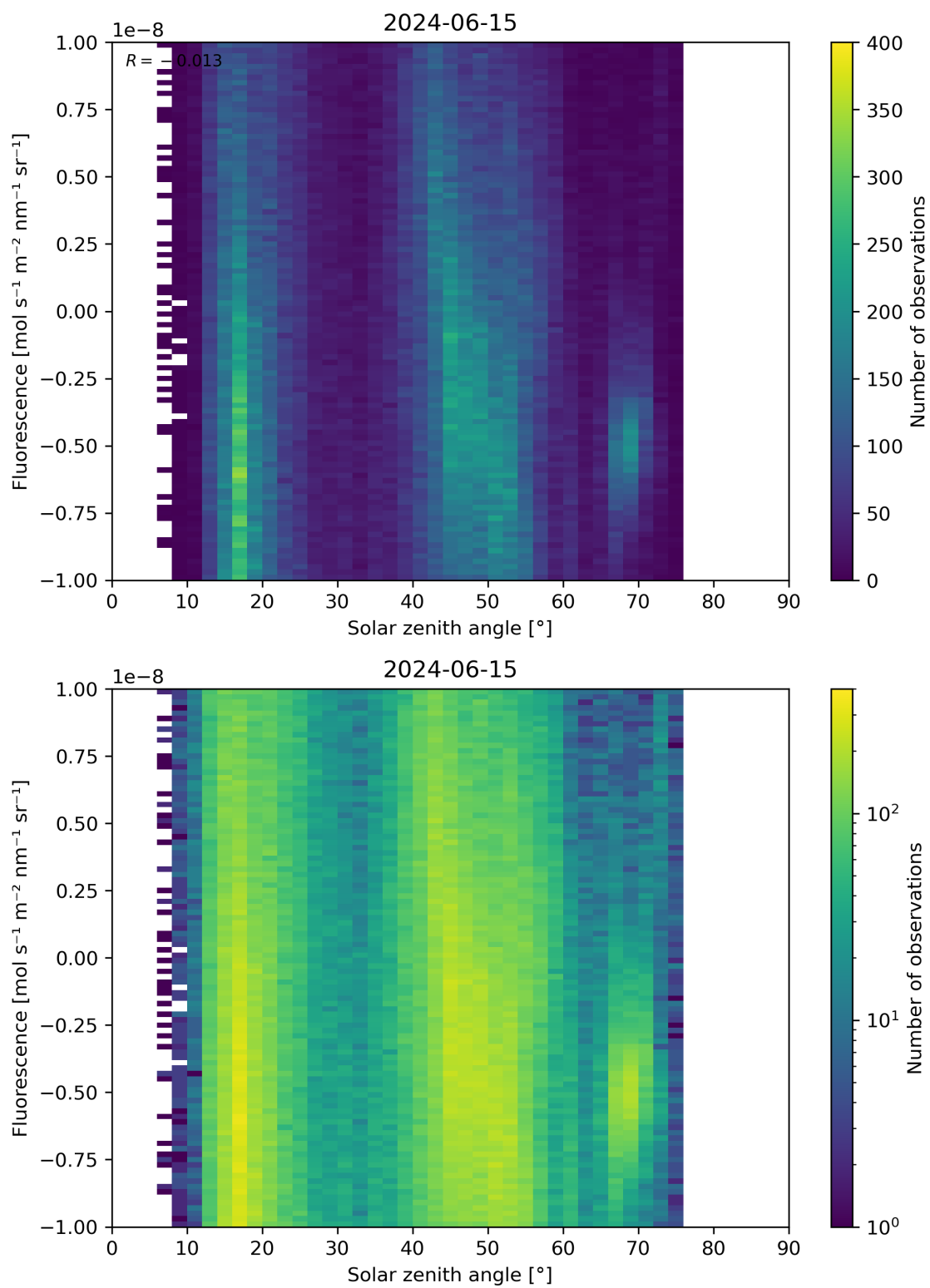
Figure 97: Scatter density plot of “Solar zenith angle” against “Fluorescence” for 2024-06-14 to 2024-06-16.
