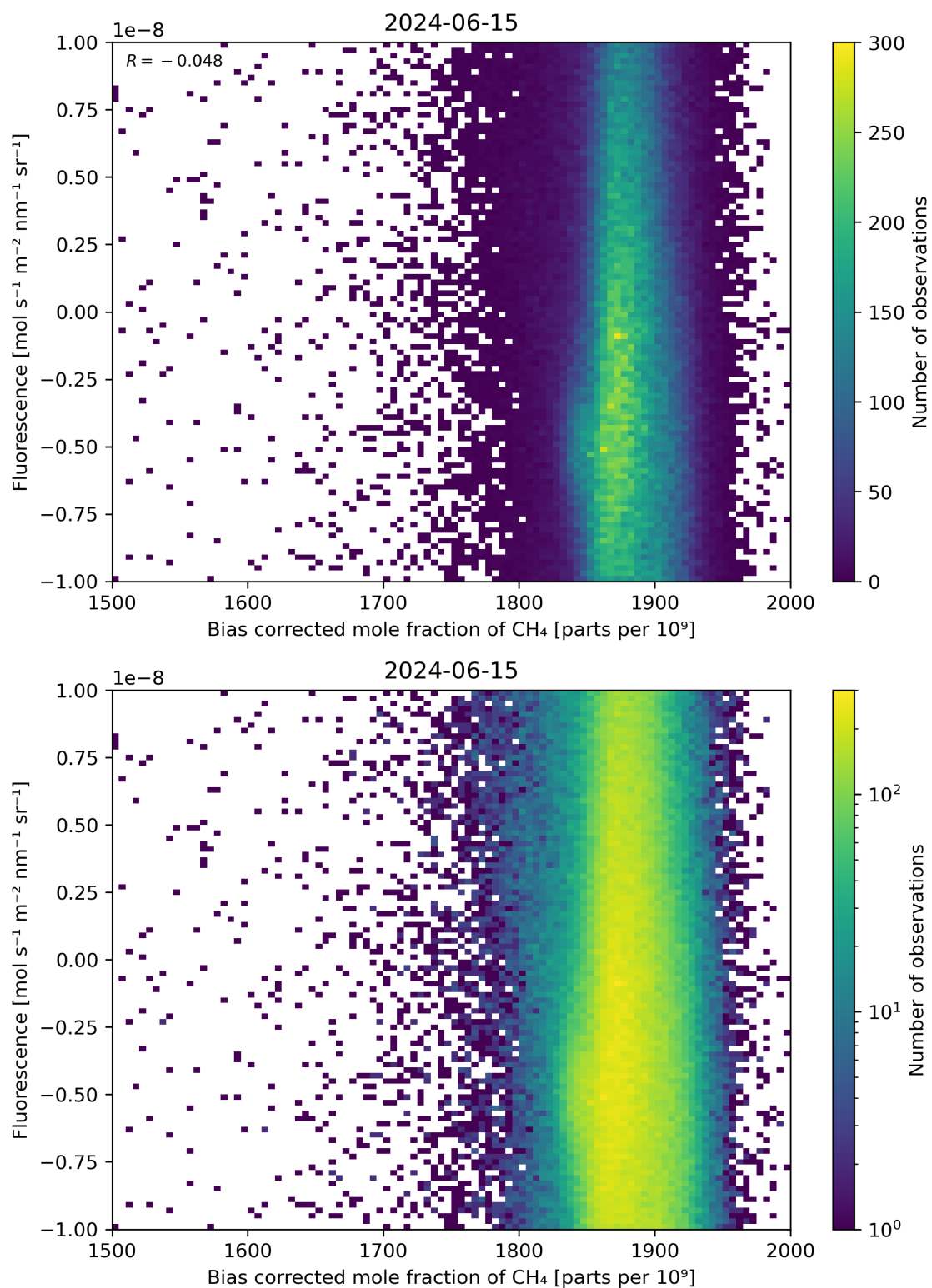
Figure 66: Scatter density plot of “Bias corrected mole fraction of \text{CH}_4 ” against “Fluorescence” for 2024-06-14 to 2024-06-16.
