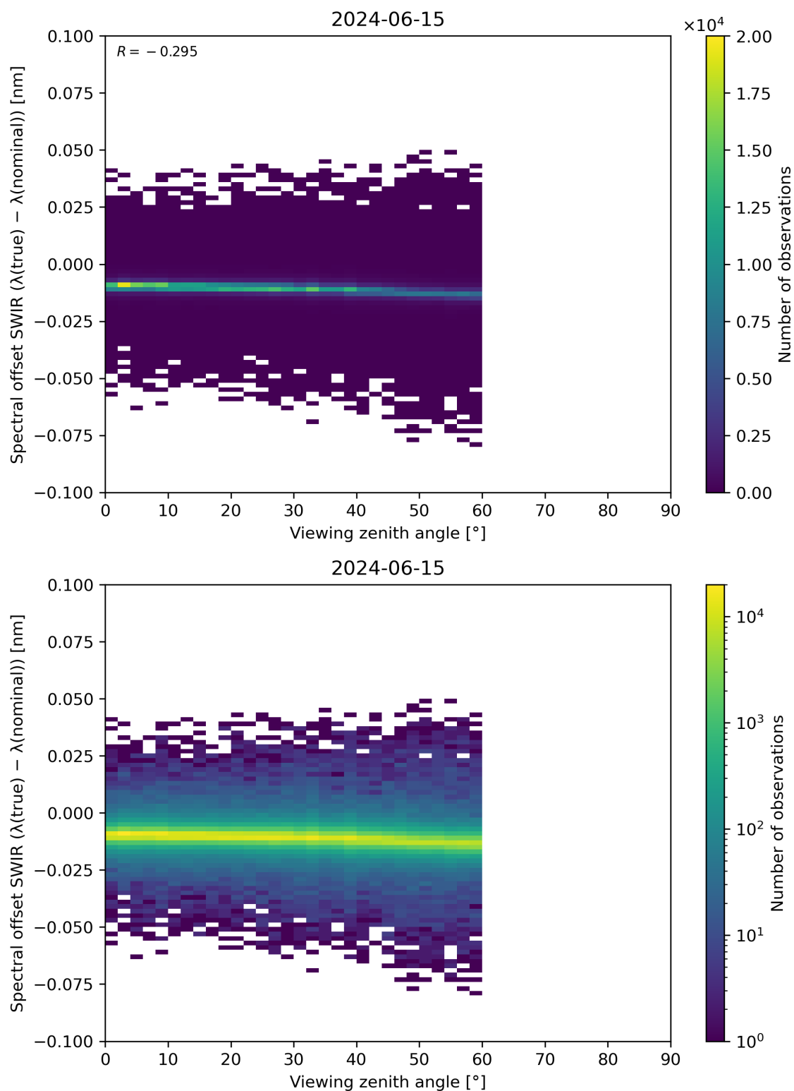
Figure 116: Scatter density plot of “Viewing zenith angle” against “Spectral offset SWIR ( \lambda(\text{true}) - \lambda(\text{nominal}) )” for 2024-06-14 to 2024-06-16.
