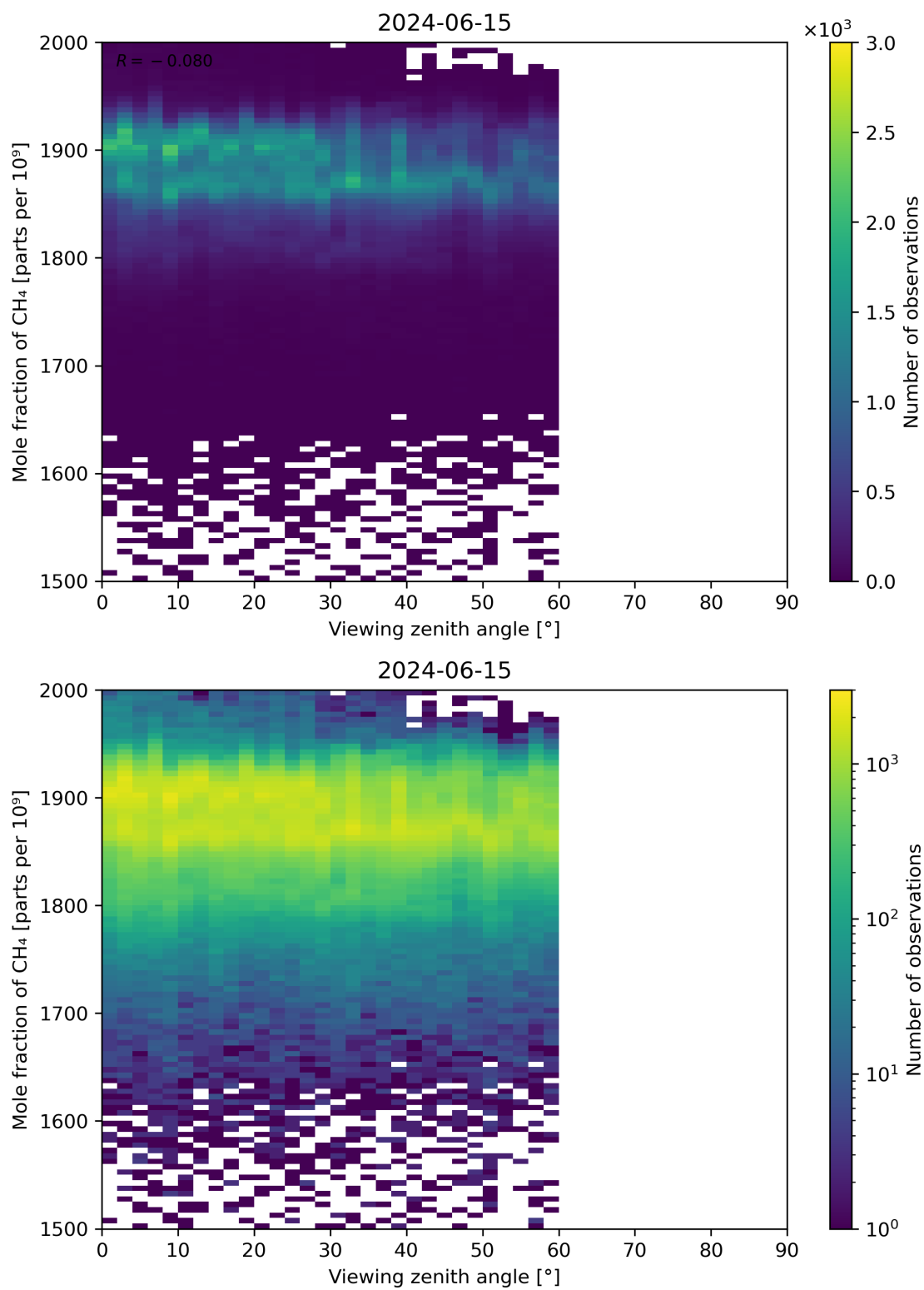
Figure 110: Scatter density plot of “Viewing zenith angle” against “Mole fraction of CH 4 ” for 2024-06-14 to 2024-06-16.
