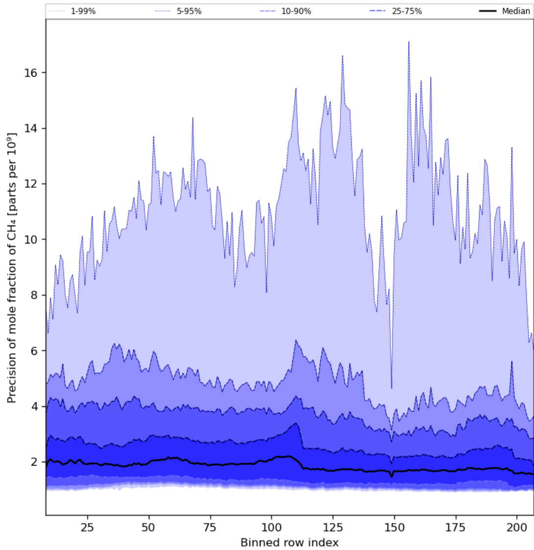
Figure 35: Along track statistics of “Precision of mole fraction of CH 4 ” for 2024-06-14 to 2024-06-16
