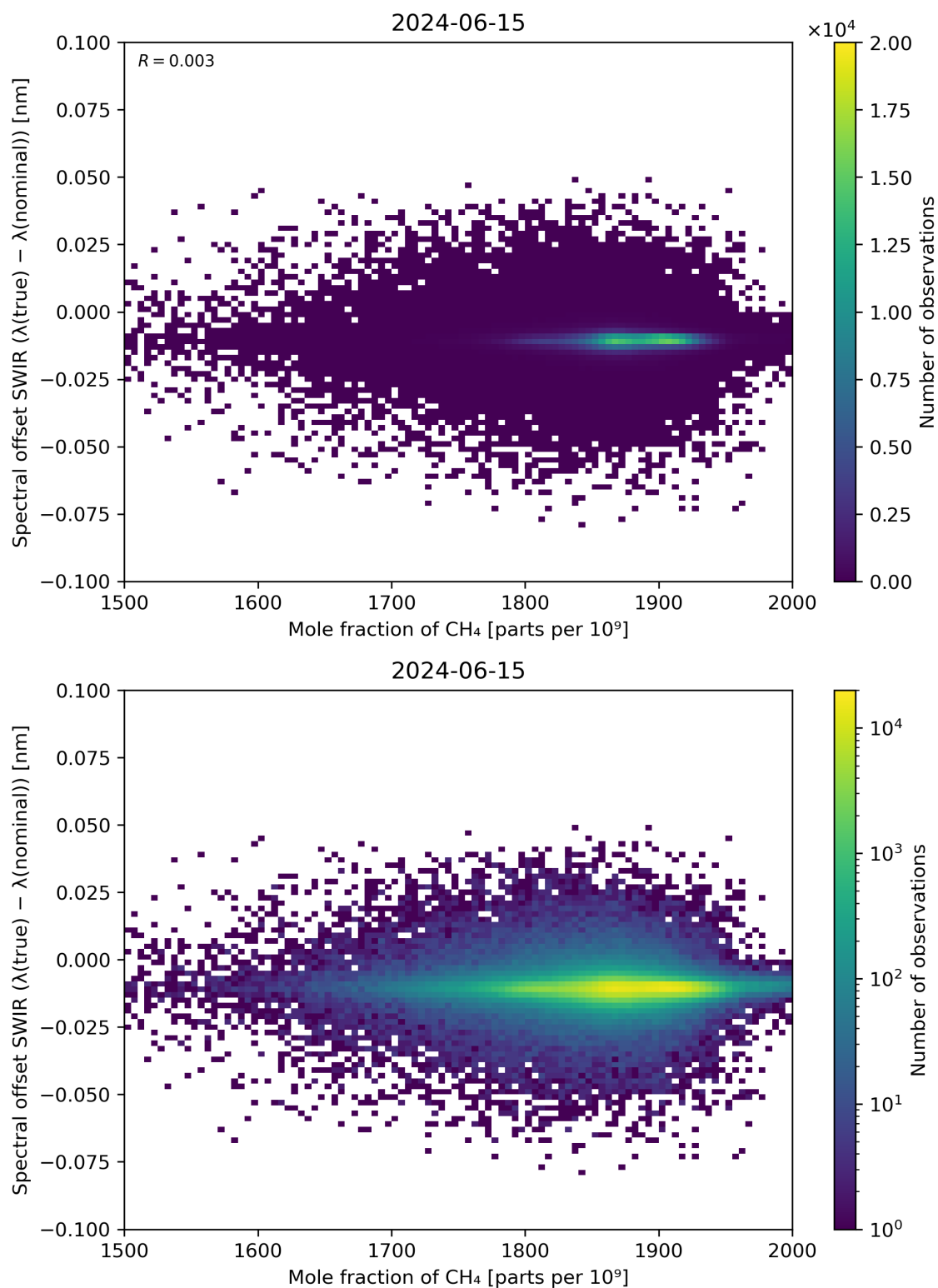
Figure 86: Scatter density plot of “Mole fraction of CH 4 ” against “Spectral offset SWIR ( \lambda(\text{true}) - \lambda(\text{nominal}) )” for 2024-06-14 to 2024-06-16.
