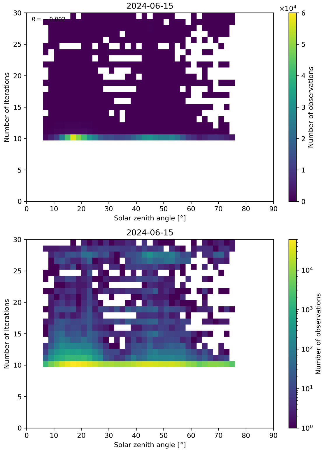
Figure 102: Scatter density plot of “Solar zenith angle” against “Number of iterations” for 2024-06-14 to 2024-06-16.
