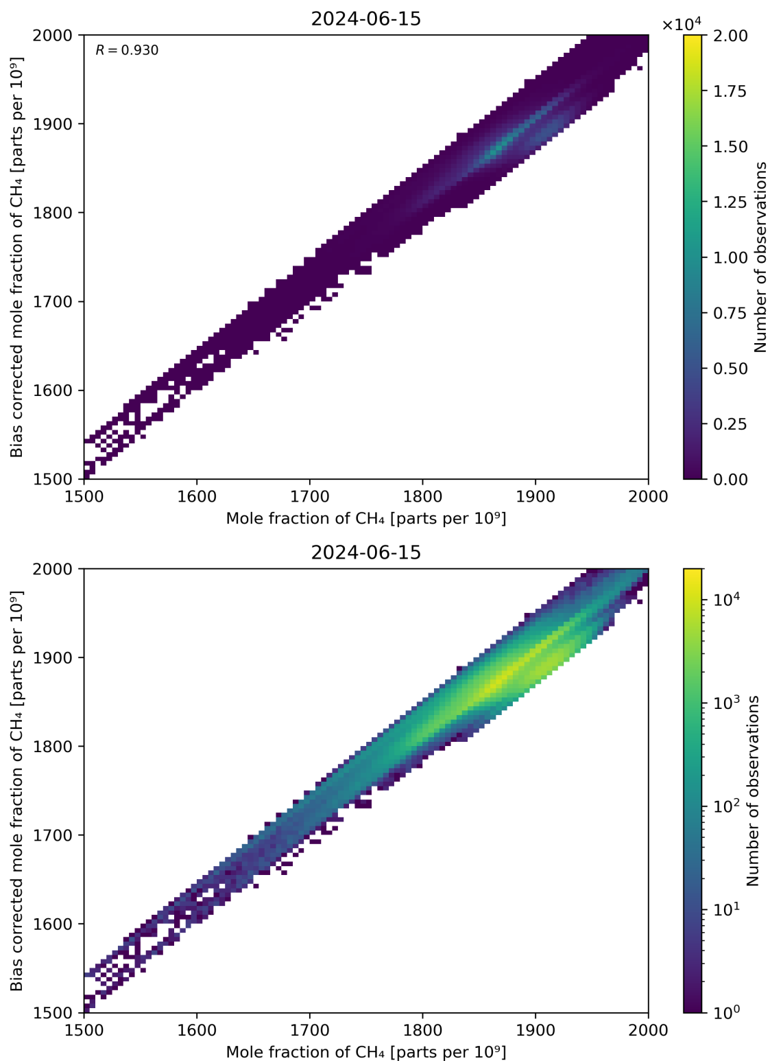
Figure 74: Scatter density plot of “Mole fraction of CH 4 ” against “Bias corrected mole fraction of CH 4 ” for 2024-06-14 to 2024-06-16.
