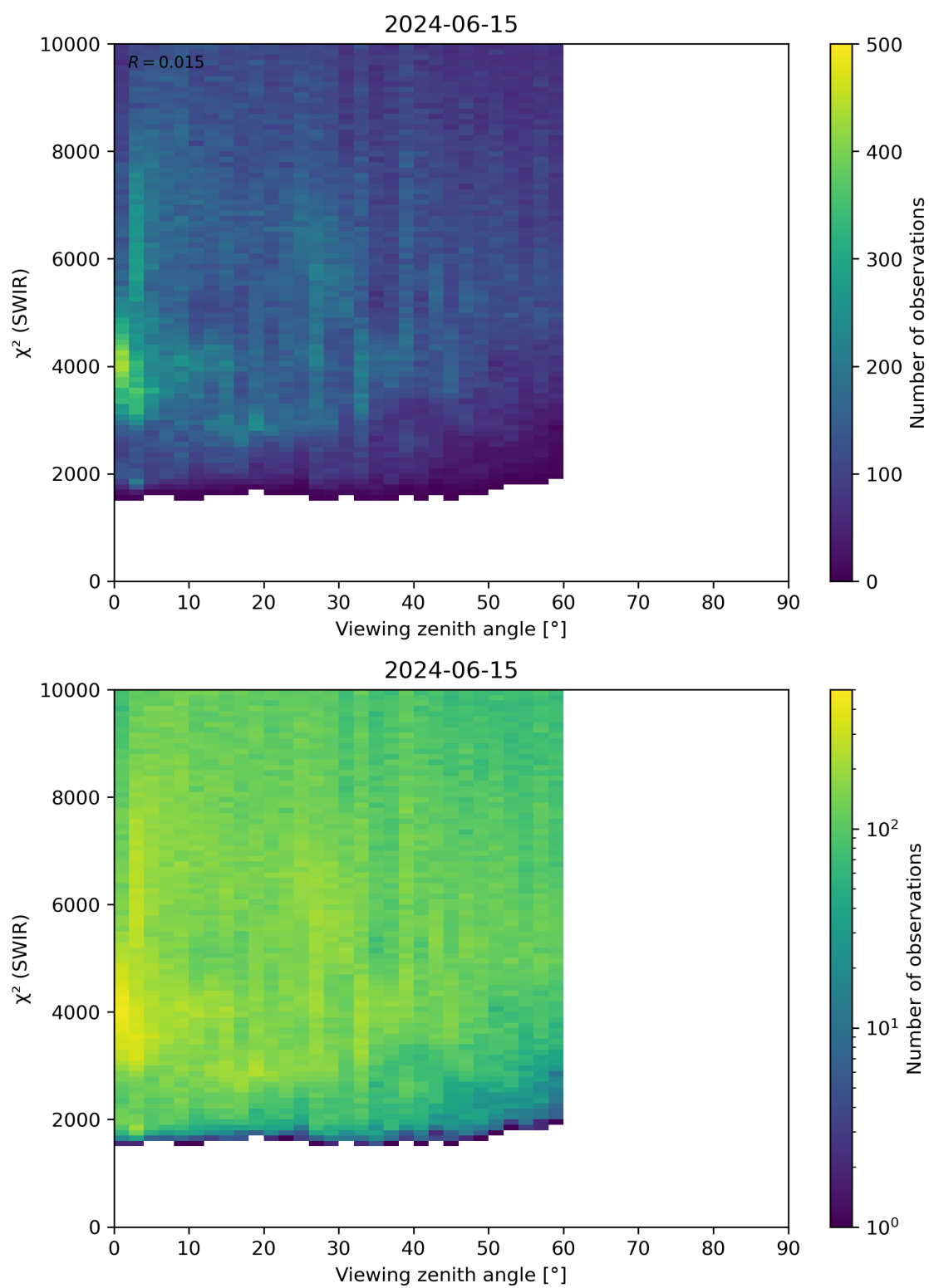
Figure 106: Scatter density plot of “Viewing zenith angle” against “ \chi^2 (SWIR)” for 2024-06-14 to 2024-06-16.
