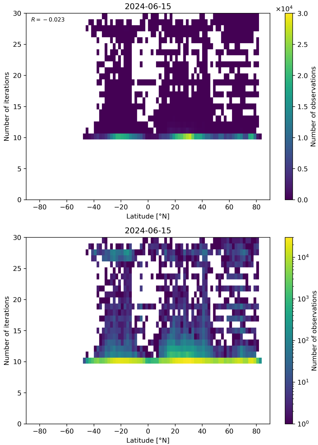
Figure 60: Scatter density plot of “Latitude” against “Number of iterations” for 2024-06-14 to 2024-06-16.
