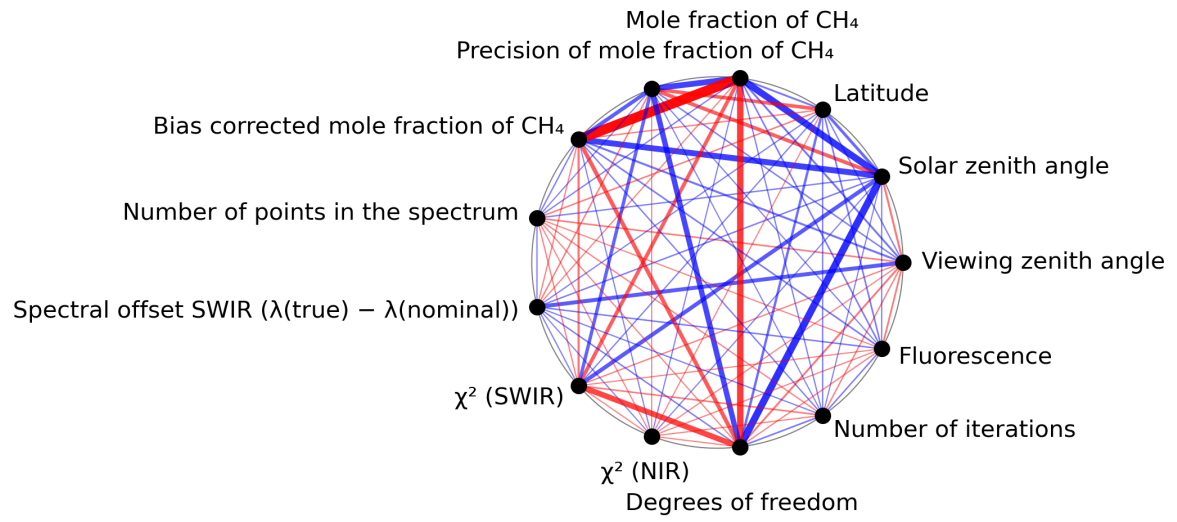
Figure 1: Map of correlation graph for 2024-06-14 to 2024-06-16.
