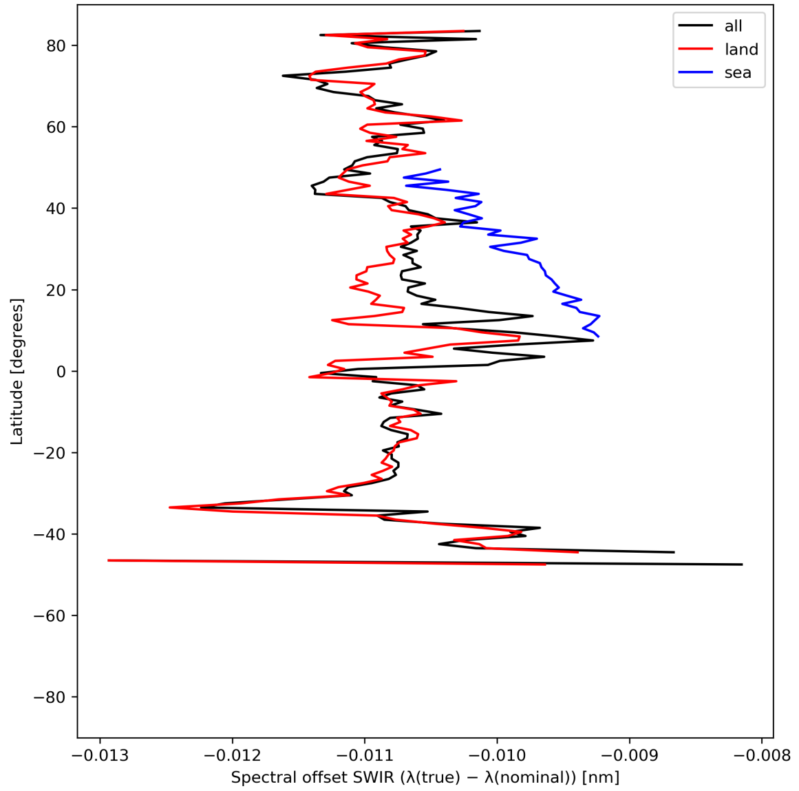
Figure 16: Zonal average of “Spectral offset SWIR ( \lambda(\text{true}) - \lambda(\text{nominal}) )” for 2024-06-14 to 2024-06-16.
