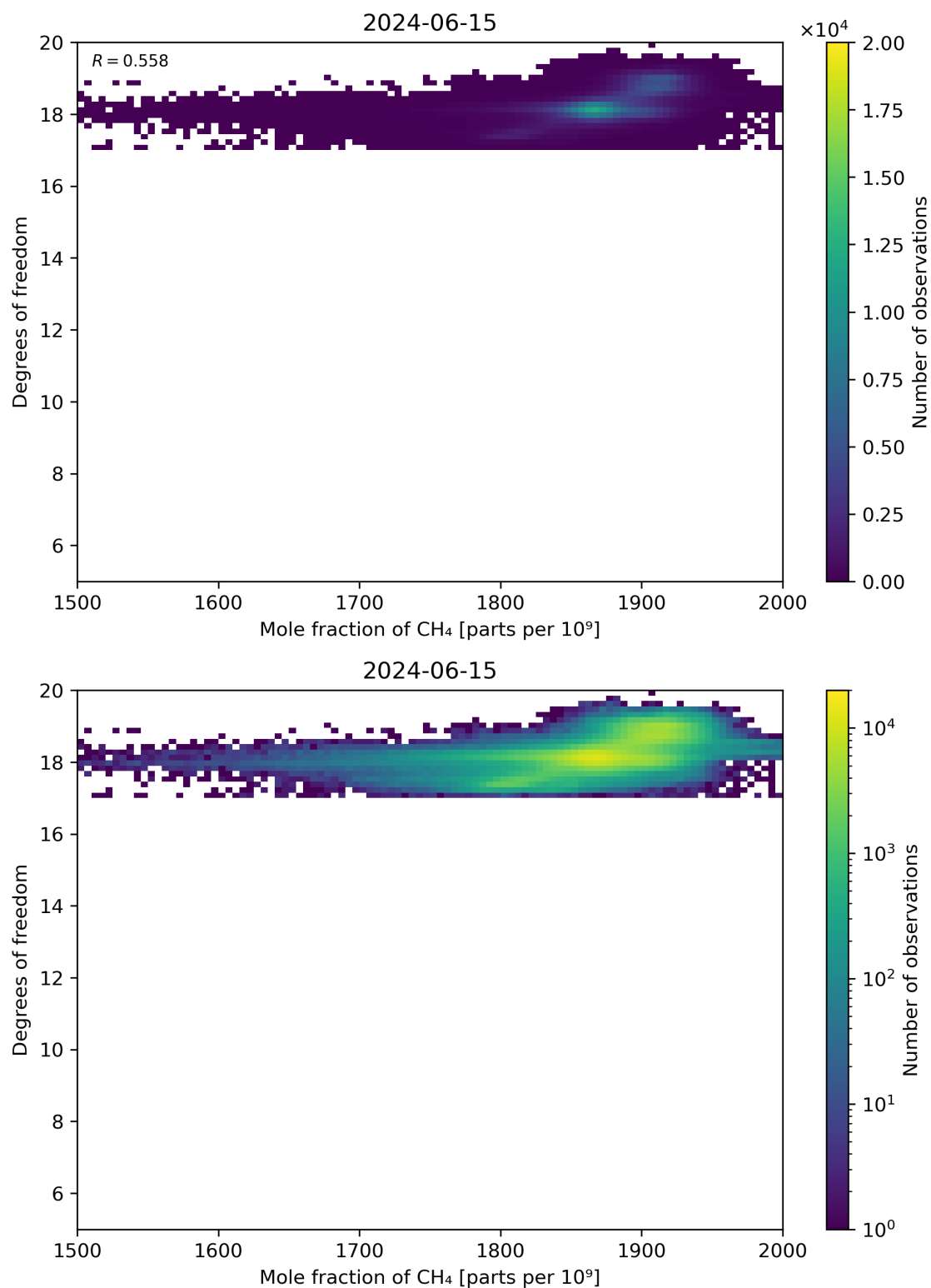
Figure 72: Scatter density plot of “Mole fraction of CH 4 ” against “Degrees of freedom” for 2024-06-14 to 2024-06-16.
