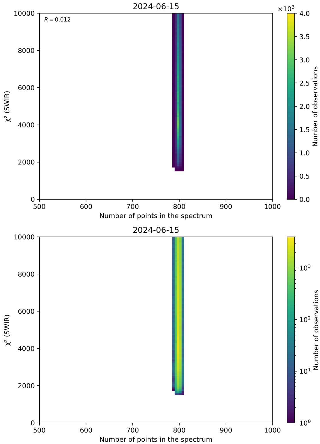
Figure 89: Scatter density plot of “Number of points in the spectrum” against “ \chi^2 (SWIR)” for 2024-06-14 to 2024-06-16.
