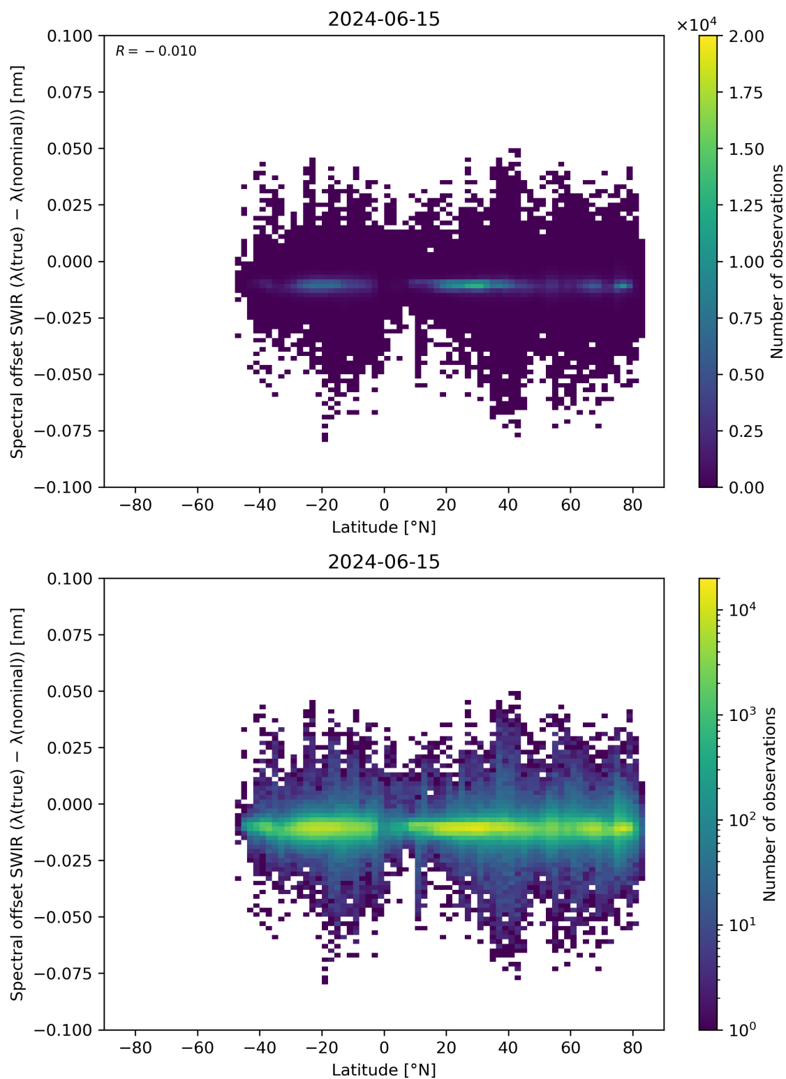
Figure 62: Scatter density plot of “Latitude” against “Spectral offset SWIR ( \lambda(\text{true}) - \lambda(\text{nominal}) )” for 2024-06-14 to 2024-06-16.
