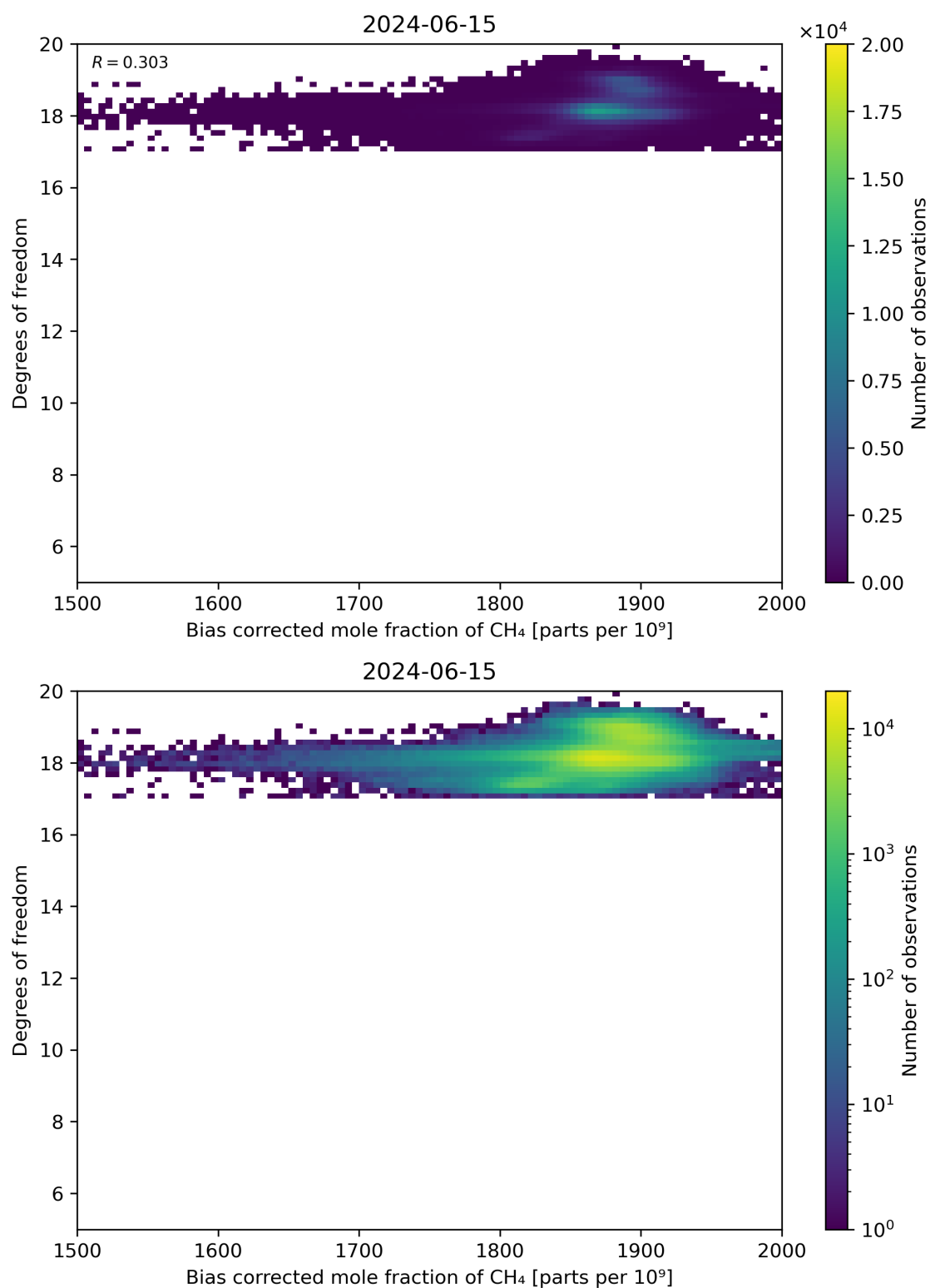
Figure 65: Scatter density plot of “Bias corrected mole fraction of CH 4 ” against “Degrees of freedom” for 2024-06-14 to 2024-06-16.
