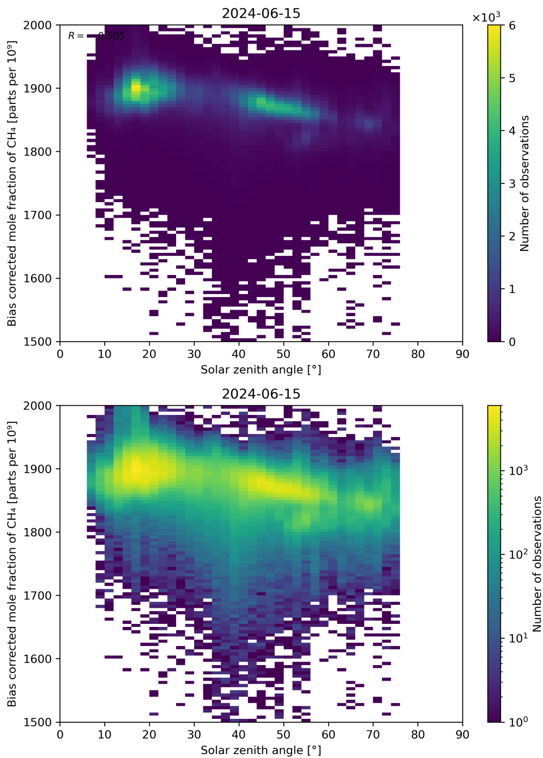
Figure 100: Scatter density plot of “Solar zenith angle” against “Bias corrected mole fraction of CH 4 ” for 2024-06-14 to 2024-06-16.
