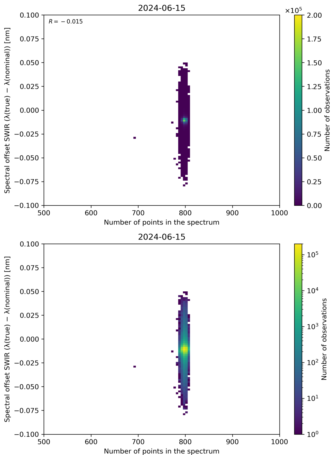
Figure 93: Scatter density plot of “Number of points in the spectrum” against “Spectral offset SWIR ( \lambda(\text{true}) - \lambda(\text{nominal}) )” for 2024-06-14 to 2024-06-16.
