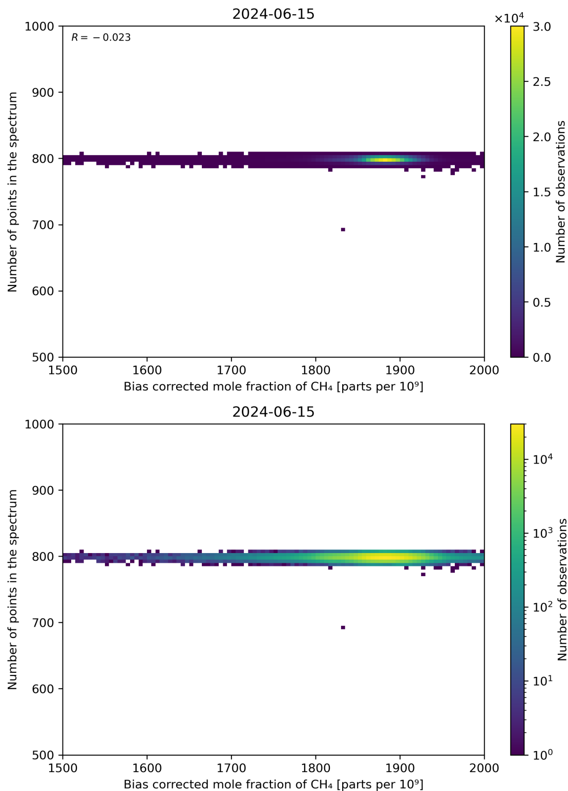
Figure 68: Scatter density plot of “Bias corrected mole fraction of CH 4 ” against “Number of points in the spectrum” for 2024-06-14 to 2024-06-16.
