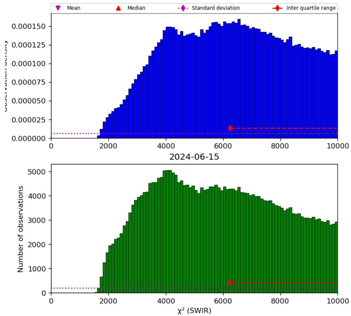
Figure 28: Histogram of “ \chi^2 (SWIR)” for 2024-06-14 to 2024-06-16
