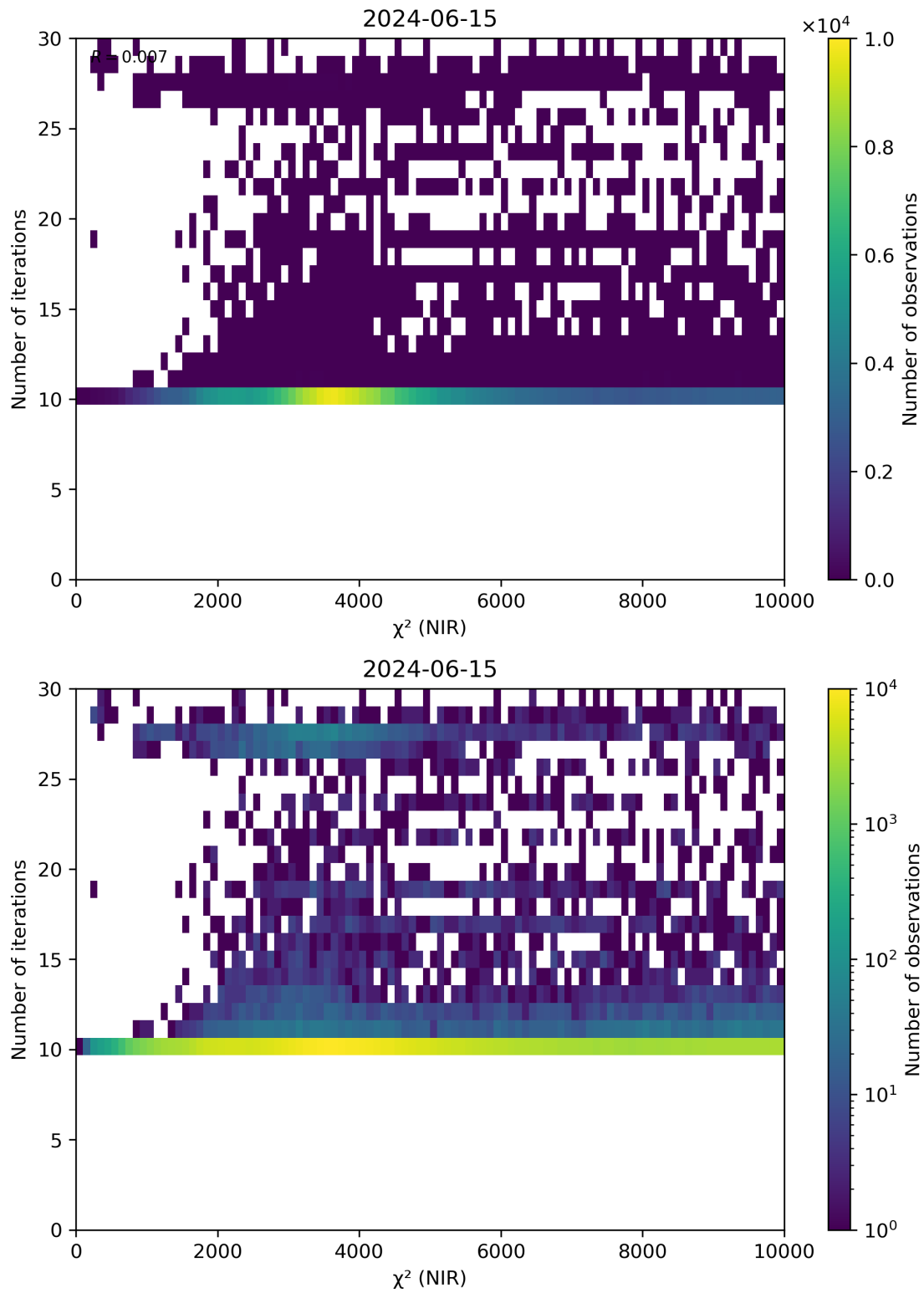
Figure 46: Scatter density plot of “ \chi^2 (NIR)” against “Number of iterations” for 2024-06-14 to 2024-06-16.
