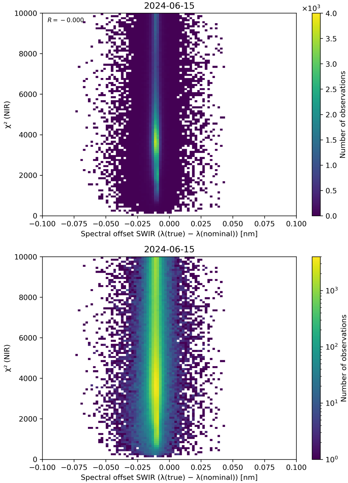
Figure 117: Scatter density plot of “Spectral offset SWIR ( \lambda(\text{true}) - \lambda(\text{nominal}) )” against “ \chi^2 (NIR)” for 2024-06-14 to 2024-06-16.
