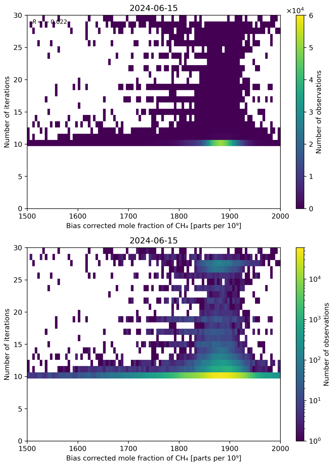
Figure 67: Scatter density plot of “Bias corrected mole fraction of CH 4 ” against “Number of iterations” for 2024-06-14 to 2024-06-16.
