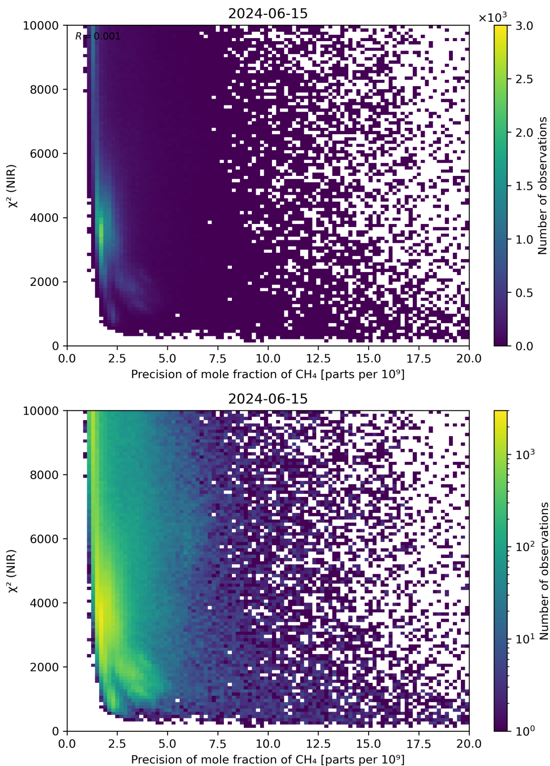
Figure 78: Scatter density plot of “Precision of mole fraction of CH 4 ” against “ \chi^2 (NIR)” for 2024-06-14 to 2024-06-16.
