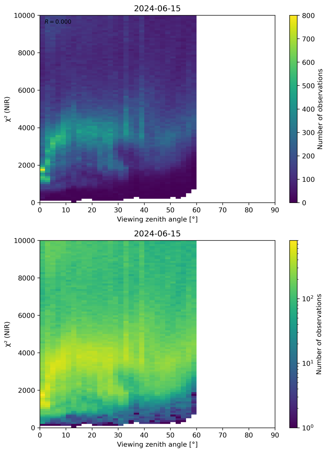
Figure 105: Scatter density plot of “Viewing zenith angle” against “ \chi^2 (NIR)” for 2024-06-14 to 2024-06-16.
