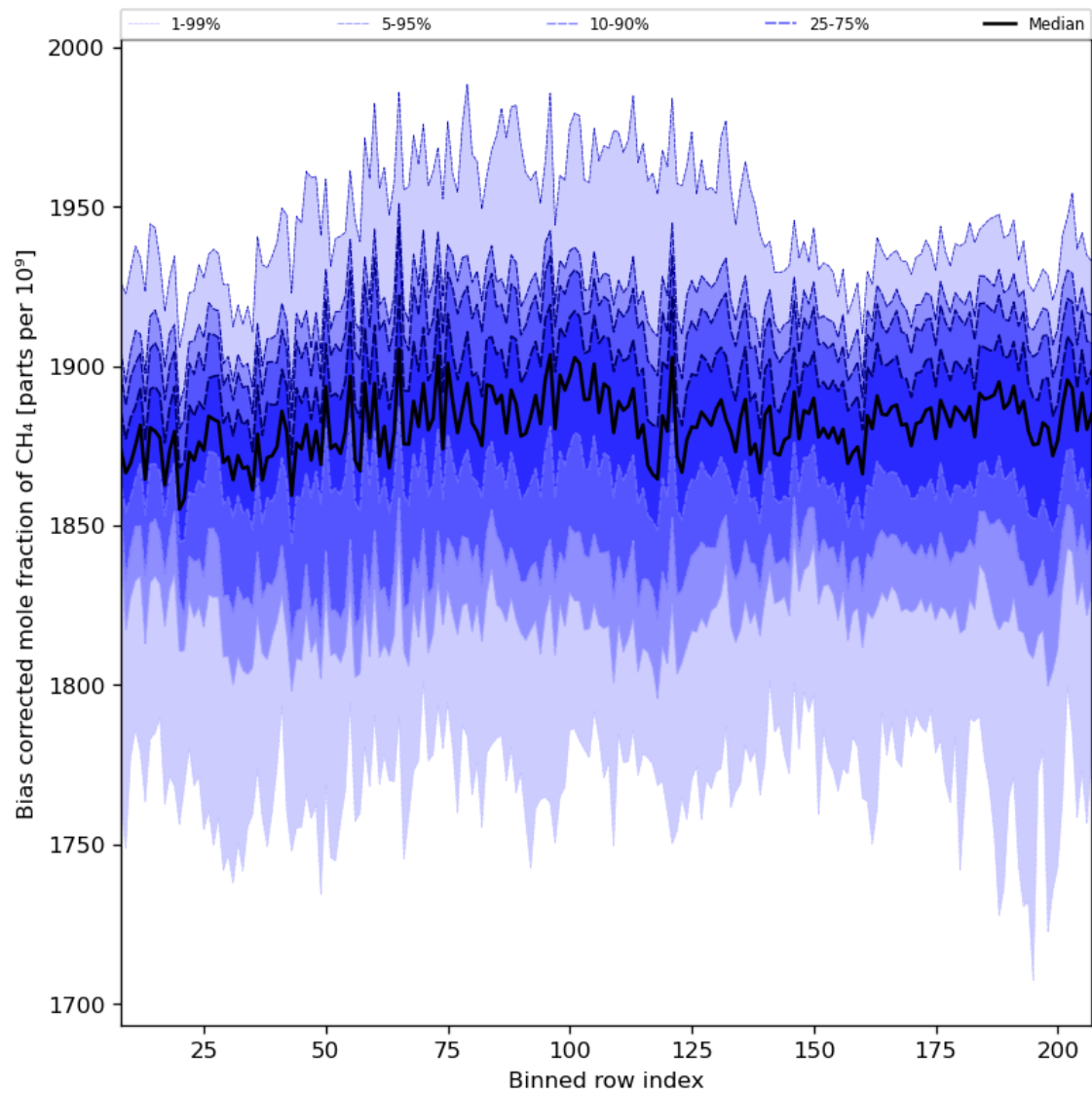
Figure 36: Along track statistics of “Bias corrected mole fraction of CH 4 ” for 2024-06-14 to 2024-06-16
