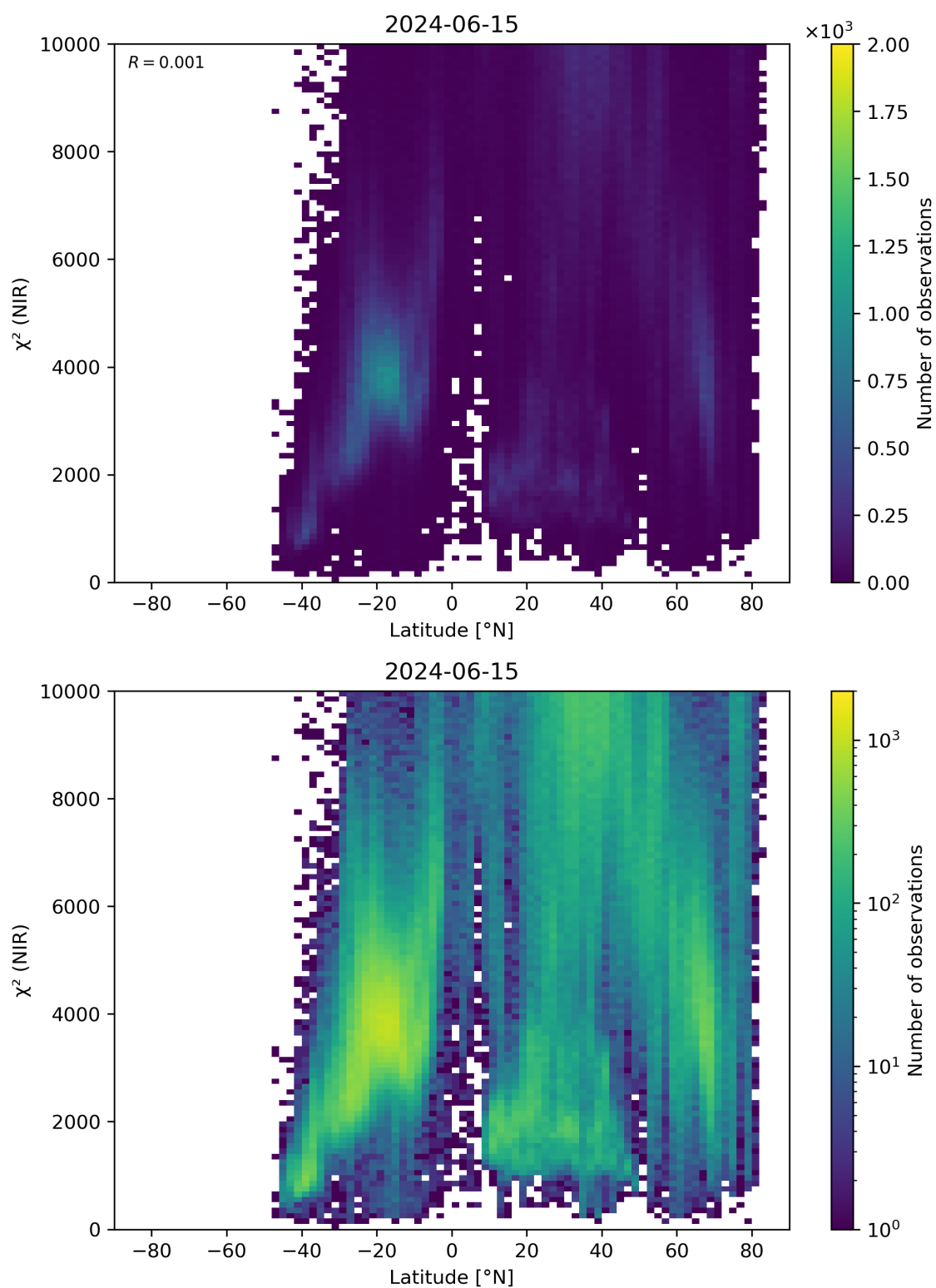
Figure 53: Scatter density plot of “Latitude” against “ \chi^2 (NIR)” for 2024-06-14 to 2024-06-16.
