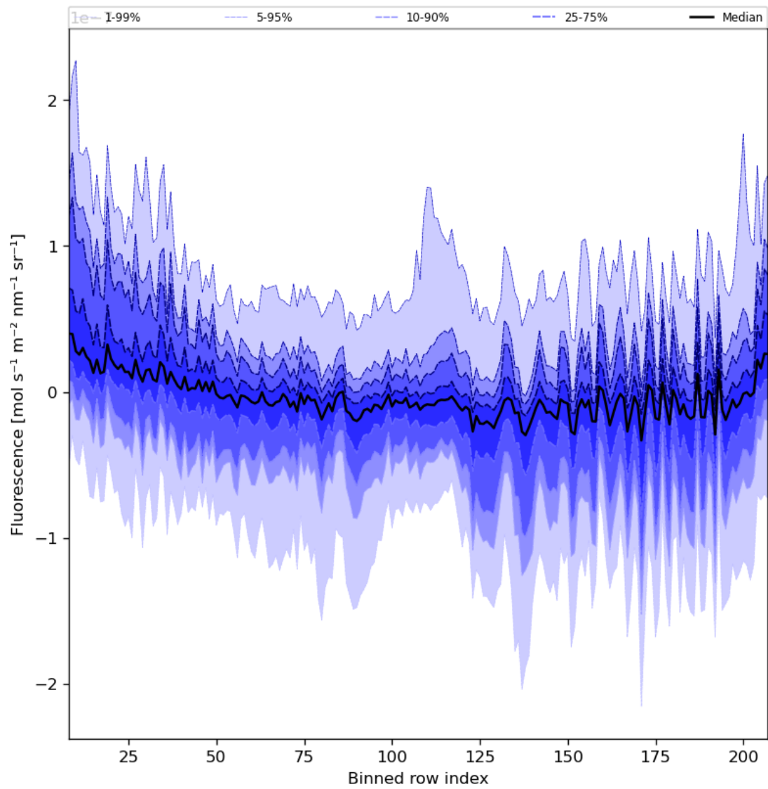
Figure 43: Along track statistics of “Fluorescence” for 2024-06-14 to 2024-06-16
