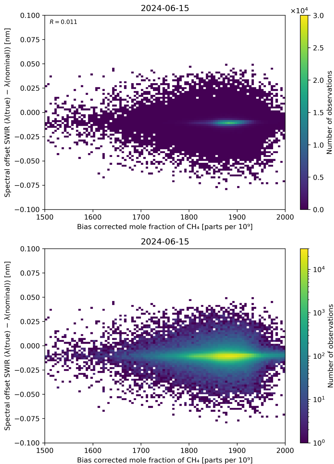
Figure 69: Scatter density plot of “Bias corrected mole fraction of \text{CH}_4 ” against “Spectral offset SWIR ( \lambda(\text{true}) - \lambda(\text{nominal}) )” for 2024-06-14 to 2024-06-16.
