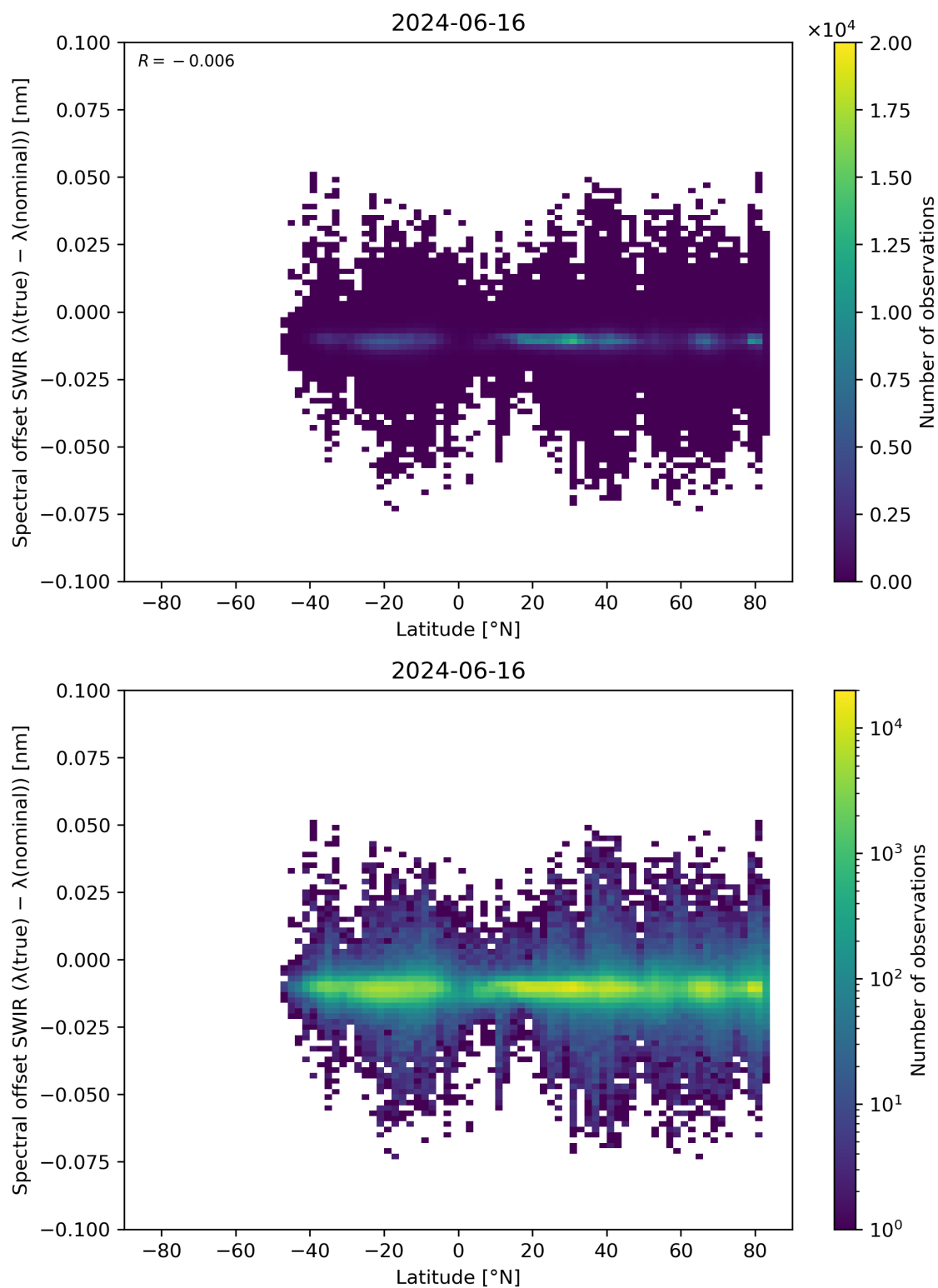
Figure 62: Scatter density plot of “Latitude” against “Spectral offset SWIR ( \lambda(\text{true}) - \lambda(\text{nominal}) )” for 2024-06-15 to 2024-06-17.
