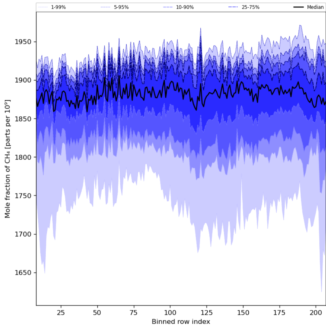
Figure 34: Along track statistics of “Mole fraction of CH 4 ” for 2024-06-15 to 2024-06-17
