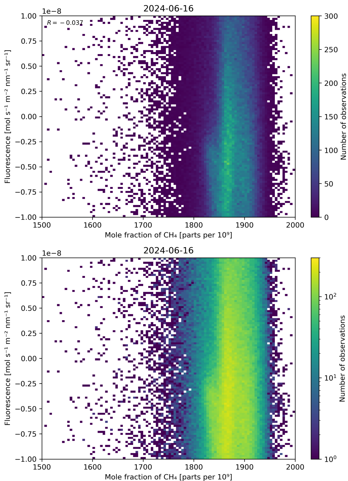
Figure 73: Scatter density plot of “Mole fraction of \text{CH}_4 ” against “Fluorescence” for 2024-06-15 to 2024-06-17.
