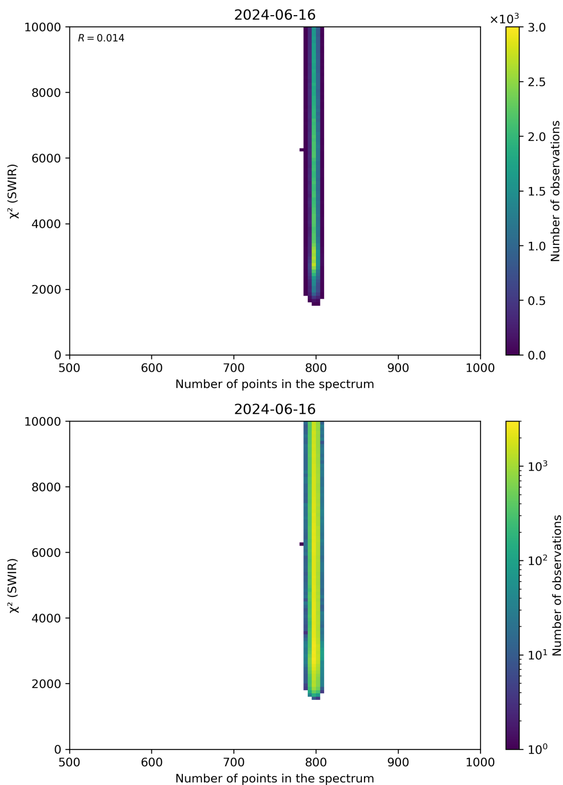
Figure 89: Scatter density plot of “Number of points in the spectrum” against “ \chi^2 (SWIR)” for 2024-06-15 to 2024-06-17.
