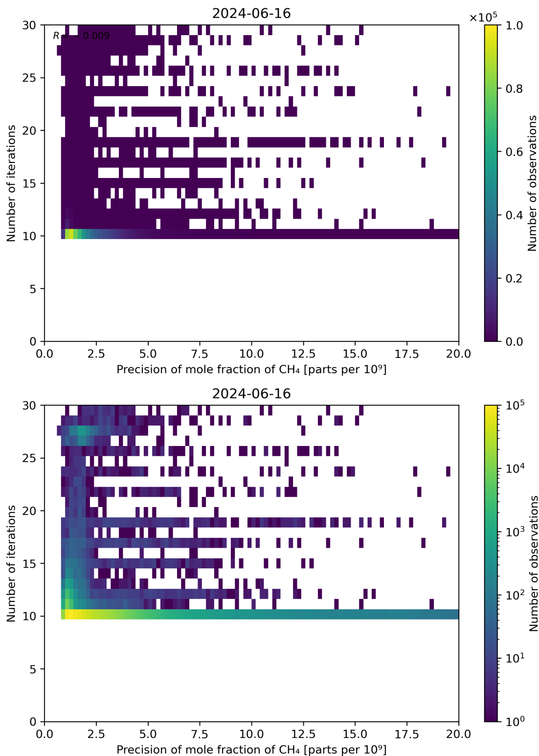
Figure 83: Scatter density plot of “Precision of mole fraction of CH 4 ” against “Number of iterations” for 2024-06-15 to 2024-06-17.
