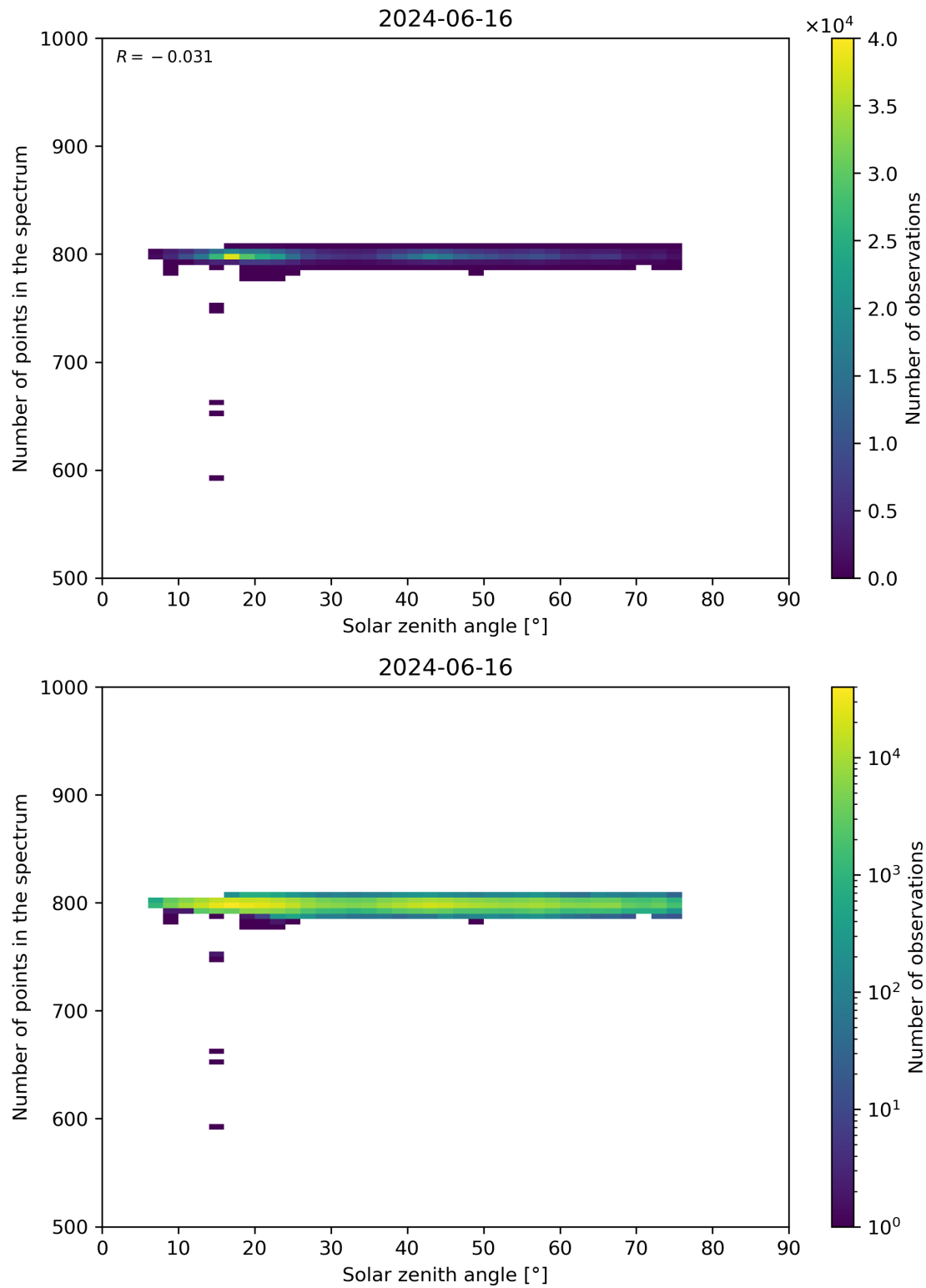
Figure 103: Scatter density plot of “Solar zenith angle” against “Number of points in the spectrum” for 2024-06-15 to 2024-06-17.
