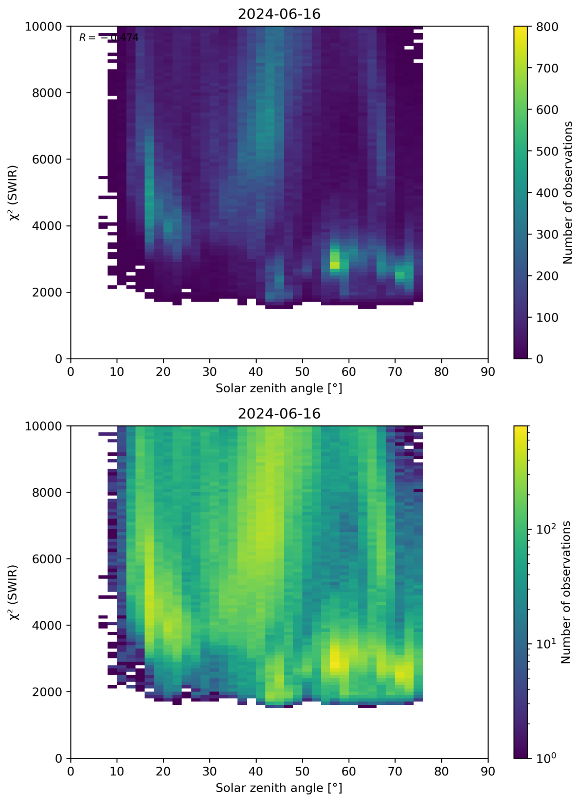
Figure 95: Scatter density plot of “Solar zenith angle” against “ \chi^2 (SWIR)” for 2024-06-15 to 2024-06-17.
