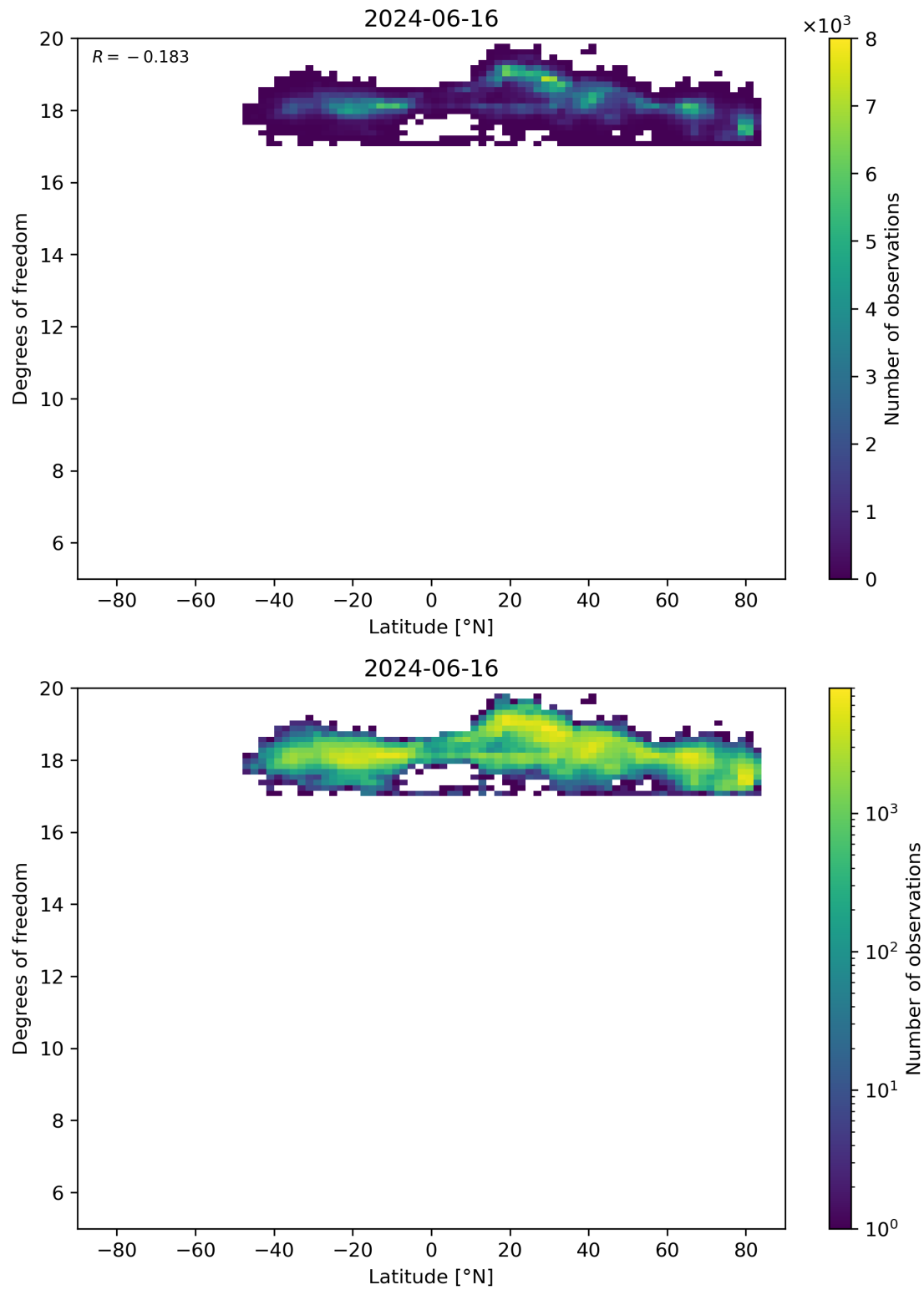
Figure 55: Scatter density plot of “Latitude” against “Degrees of freedom” for 2024-06-15 to 2024-06-17.
