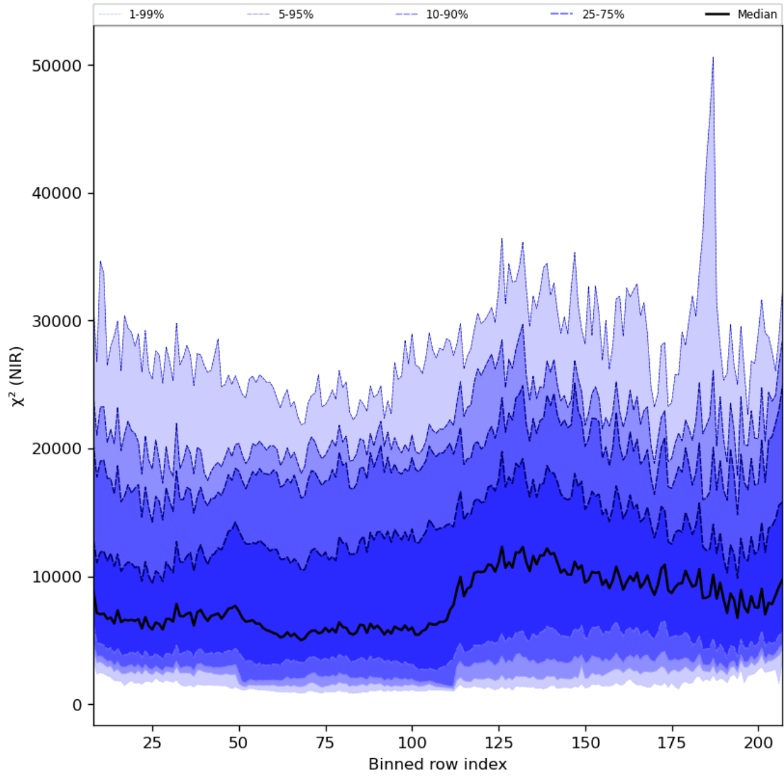
Figure 40: Along track statistics of “ \chi^2 (NIR)” for 2024-06-15 to 2024-06-17
