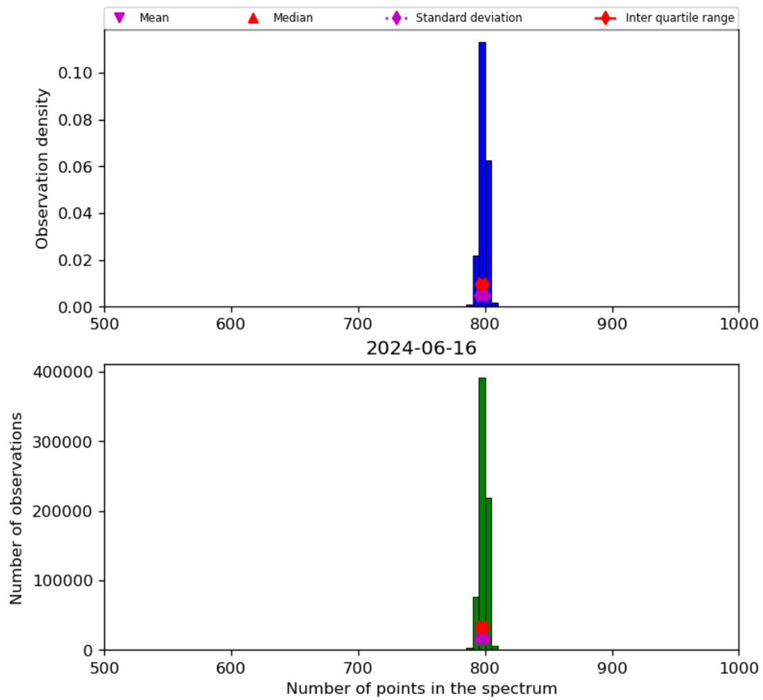
Figure 26: Histogram of “Number of points in the spectrum” for 2024-06-15 to 2024-06-17
