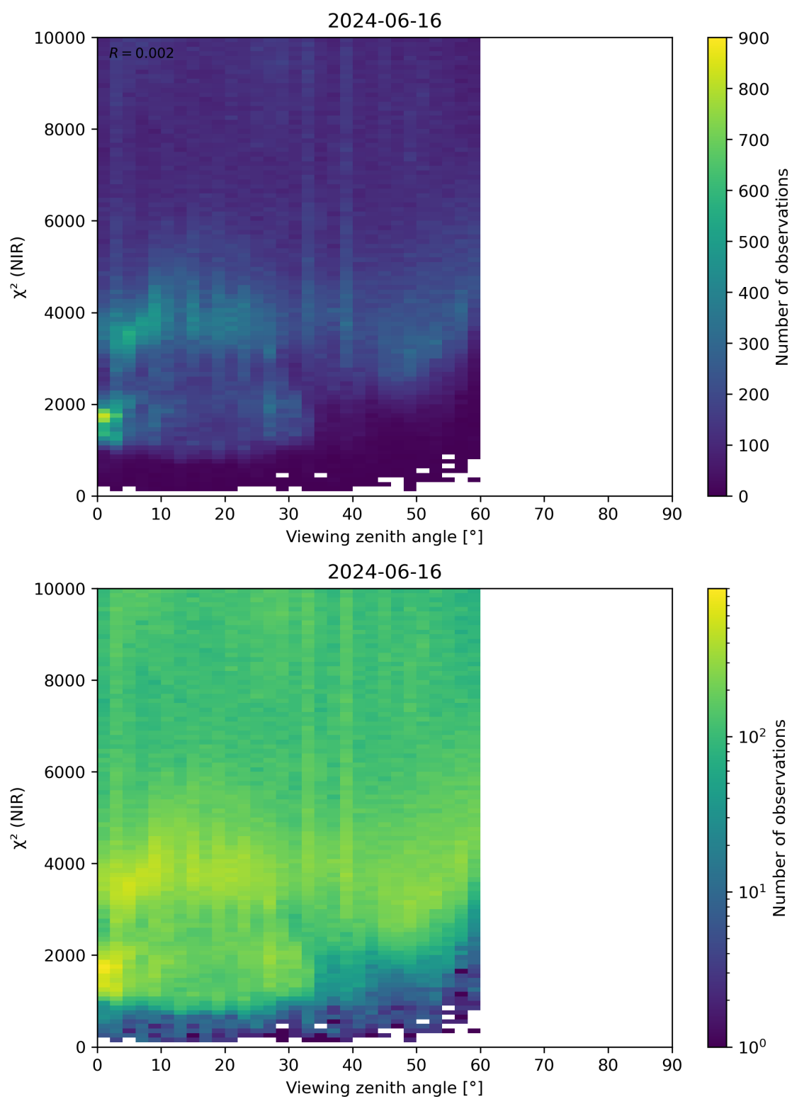
Figure 105: Scatter density plot of “Viewing zenith angle” against “ \chi^2 (NIR)” for 2024-06-15 to 2024-06-17.
