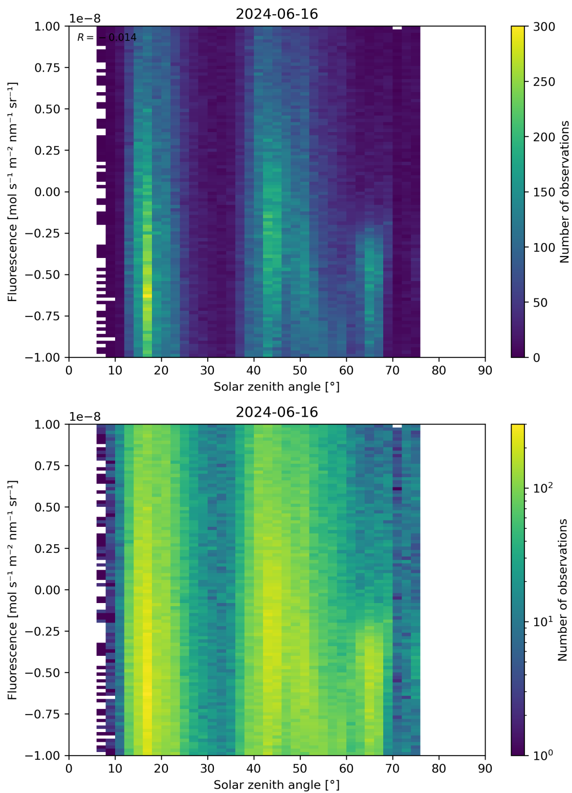
Figure 97: Scatter density plot of “Solar zenith angle” against “Fluorescence” for 2024-06-15 to 2024-06-17.
