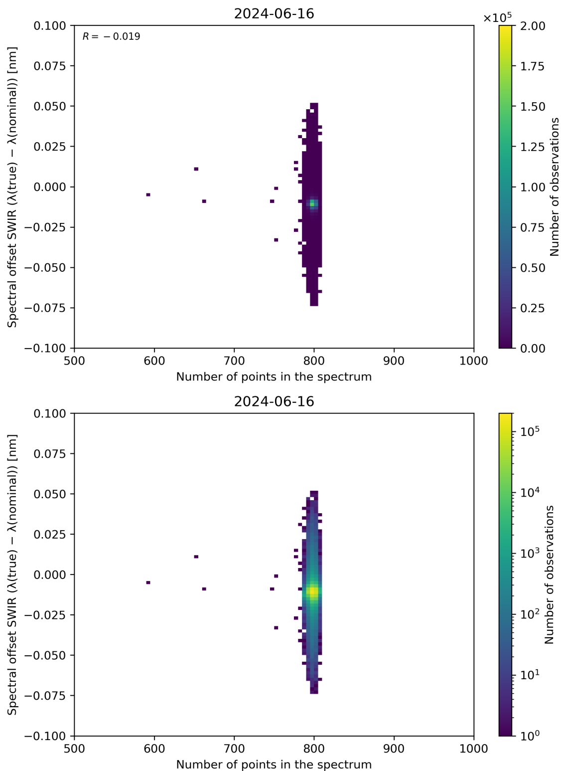
Figure 93: Scatter density plot of “Number of points in the spectrum” against “Spectral offset SWIR ( \lambda(\text{true}) - \lambda(\text{nominal}) )” for 2024-06-15 to 2024-06-17.
