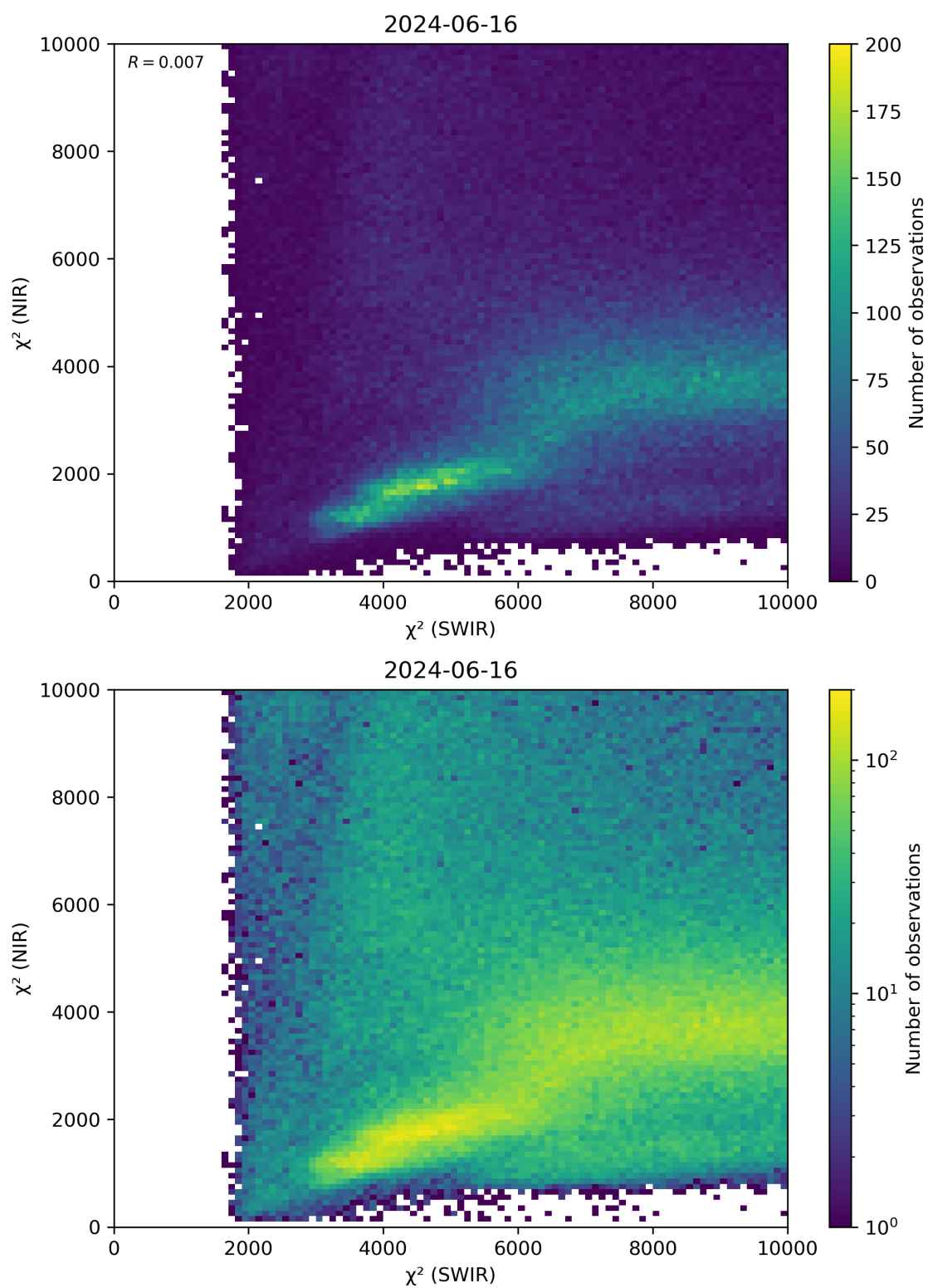
Figure 47: Scatter density plot of “ \chi^2 (SWIR)” against “ \chi^2 (NIR)” for 2024-06-15 to 2024-06-17.
