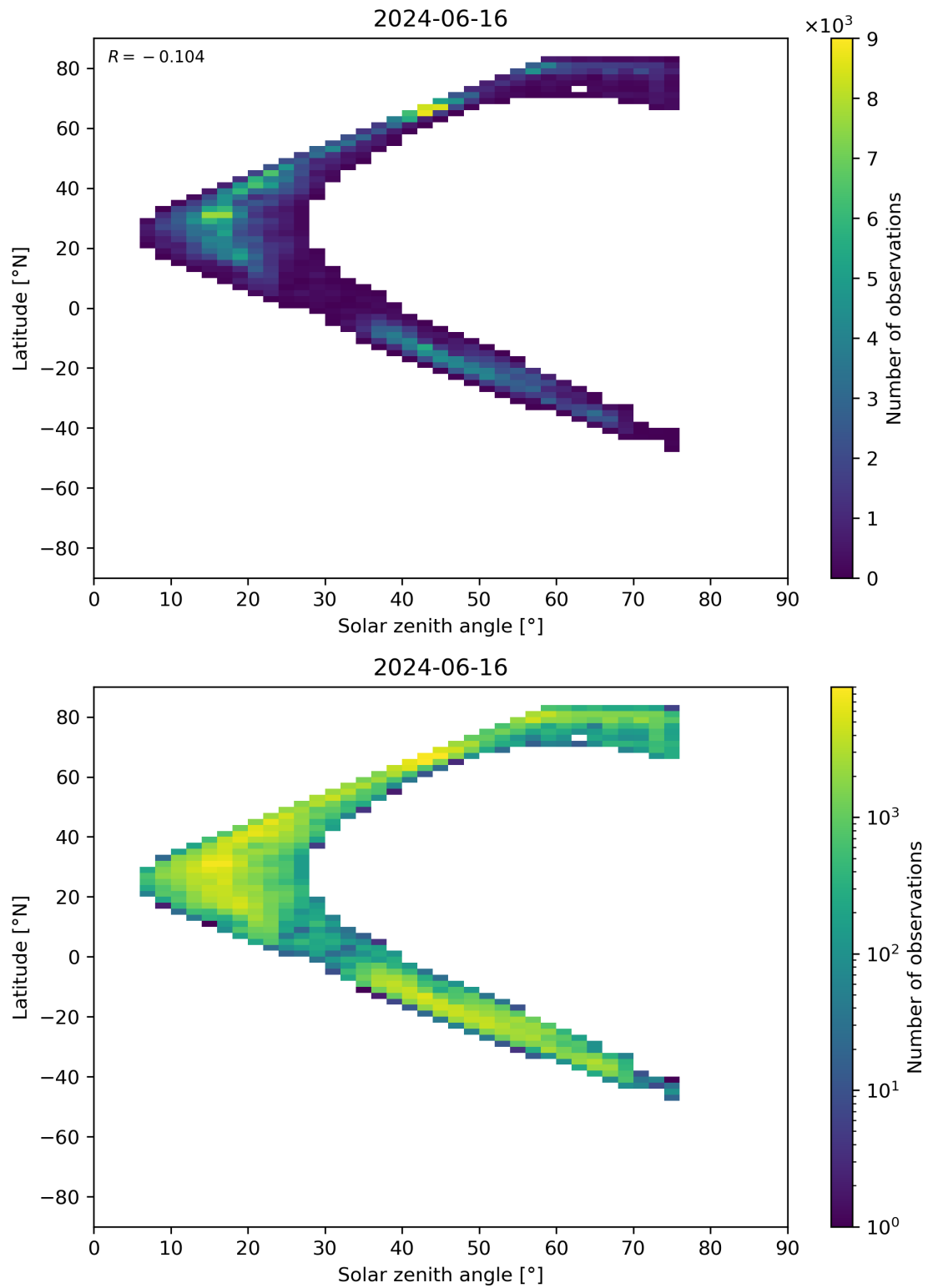
Figure 98: Scatter density plot of “Solar zenith angle” against “Latitude” for 2024-06-15 to 2024-06-17.
