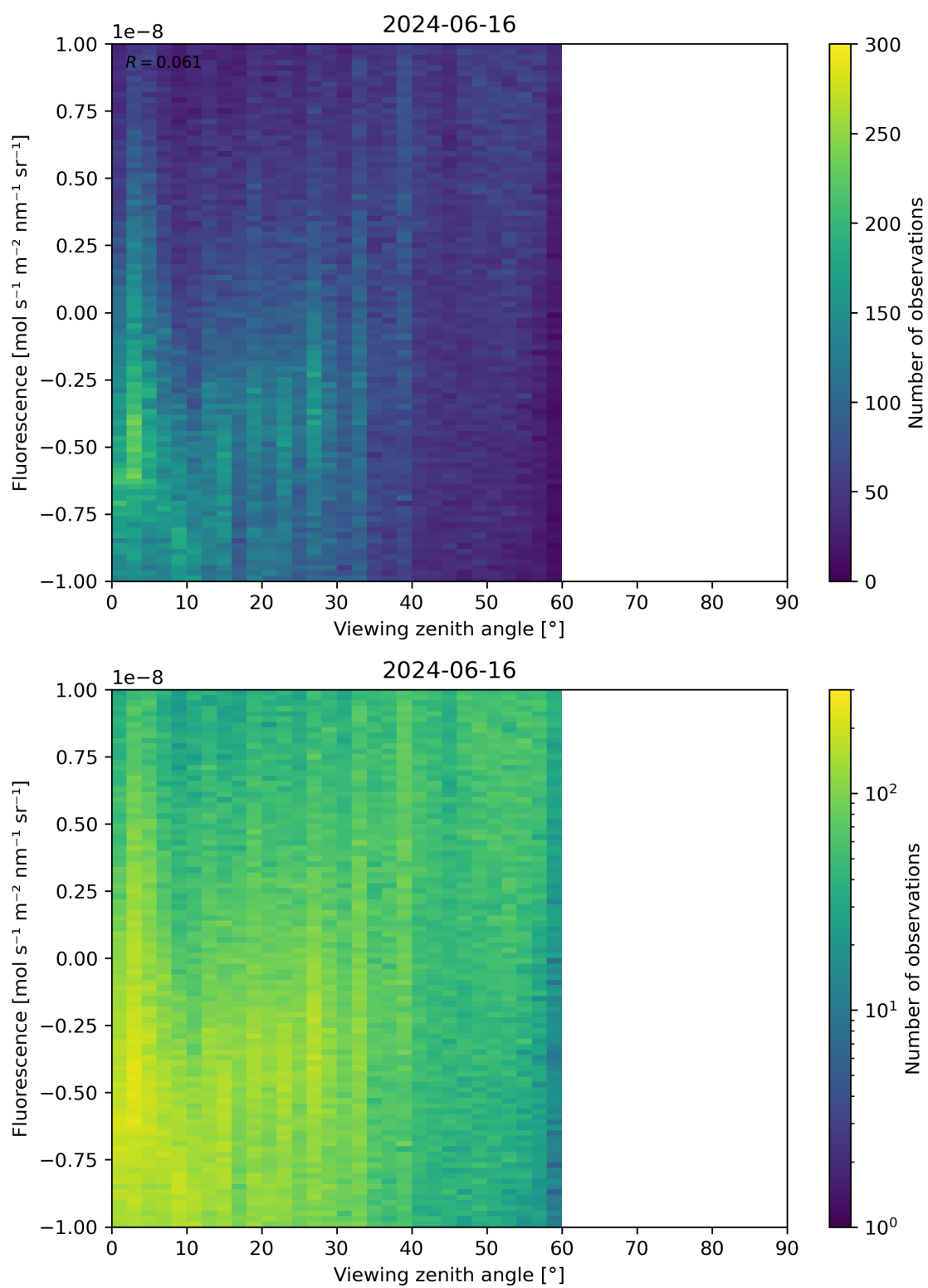
Figure 108: Scatter density plot of “Viewing zenith angle” against “Fluorescence” for 2024-06-15 to 2024-06-17.
