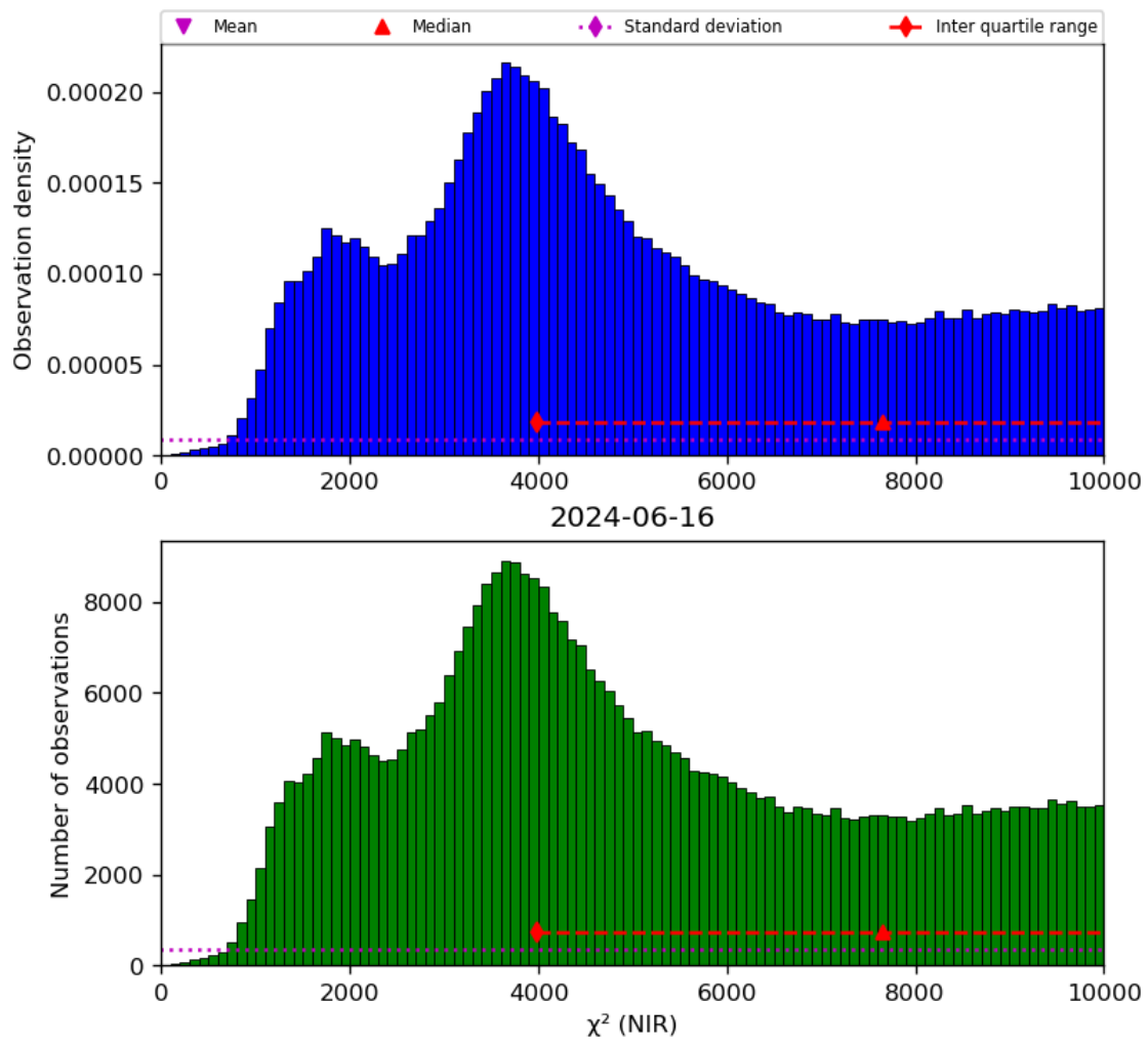
Figure 29: Histogram of “ \chi^2 (NIR)” for 2024-06-15 to 2024-06-17
