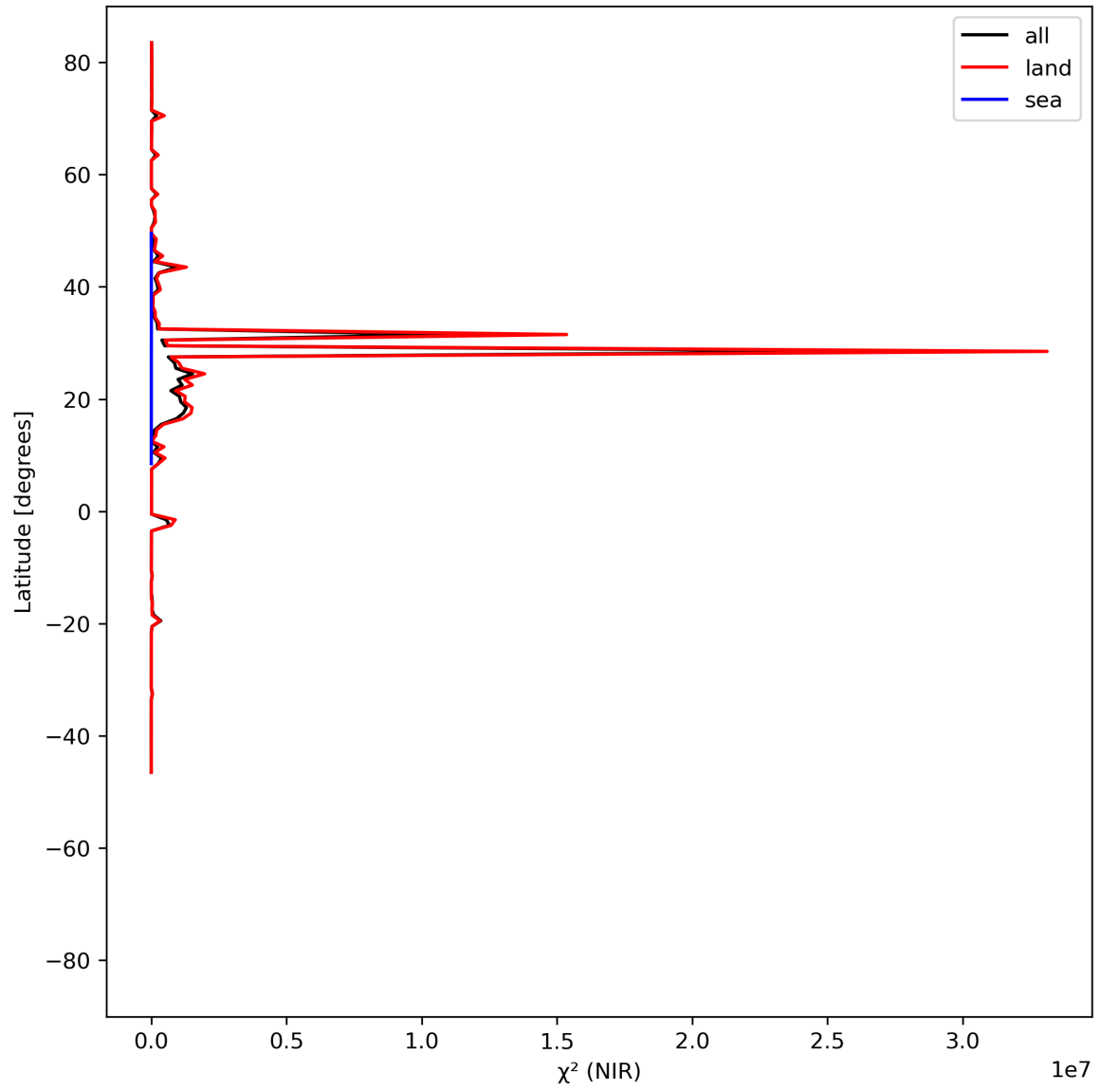
Figure 18: Zonal average of “ \chi^2 (NIR)” for 2024-06-15 to 2024-06-17.
