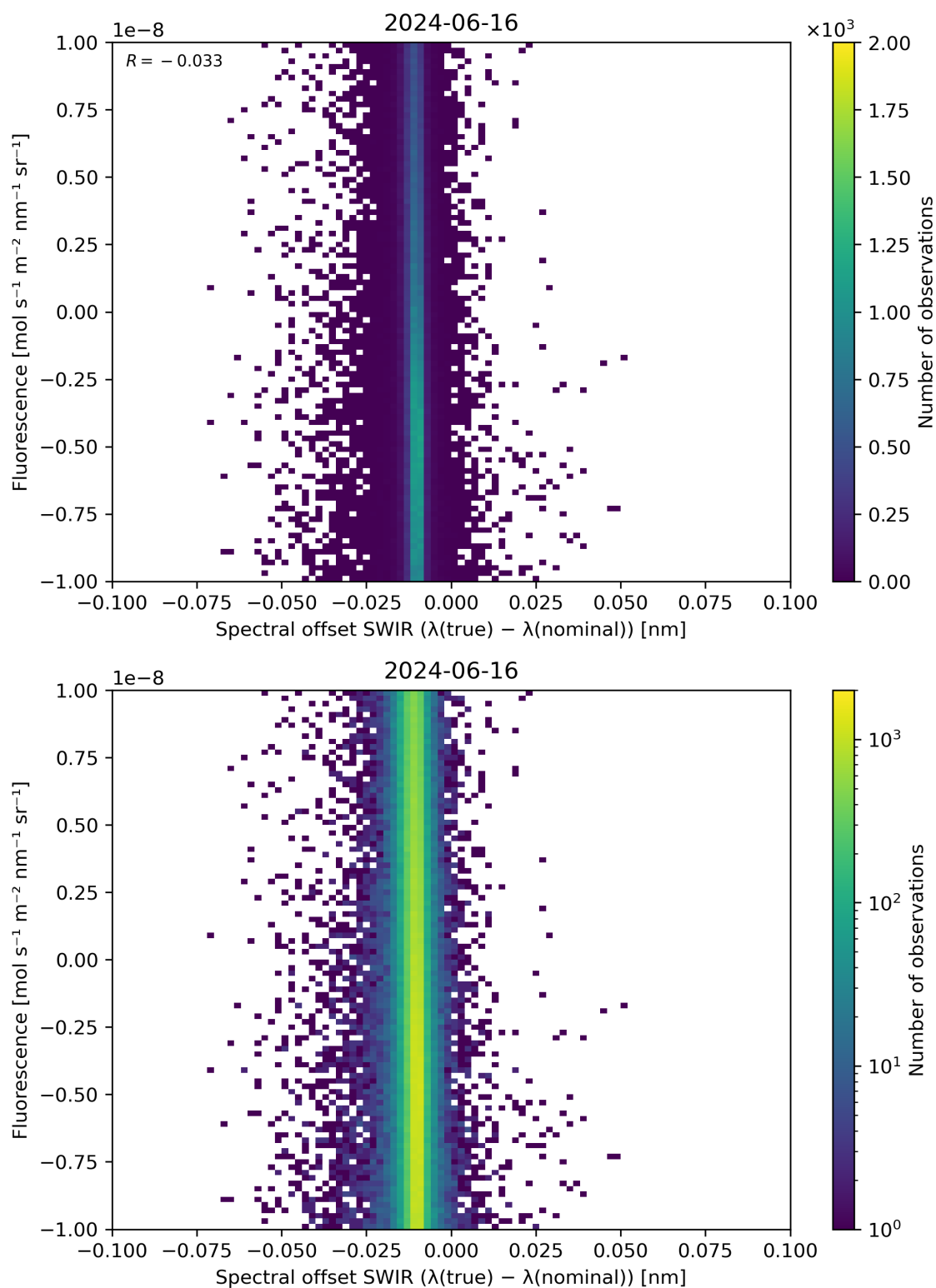
Figure 120: Scatter density plot of “Spectral offset SWIR ( \lambda(\text{true}) - \lambda(\text{nominal}) )” against “Fluorescence” for 2024-06-15 to 2024-06-17.
