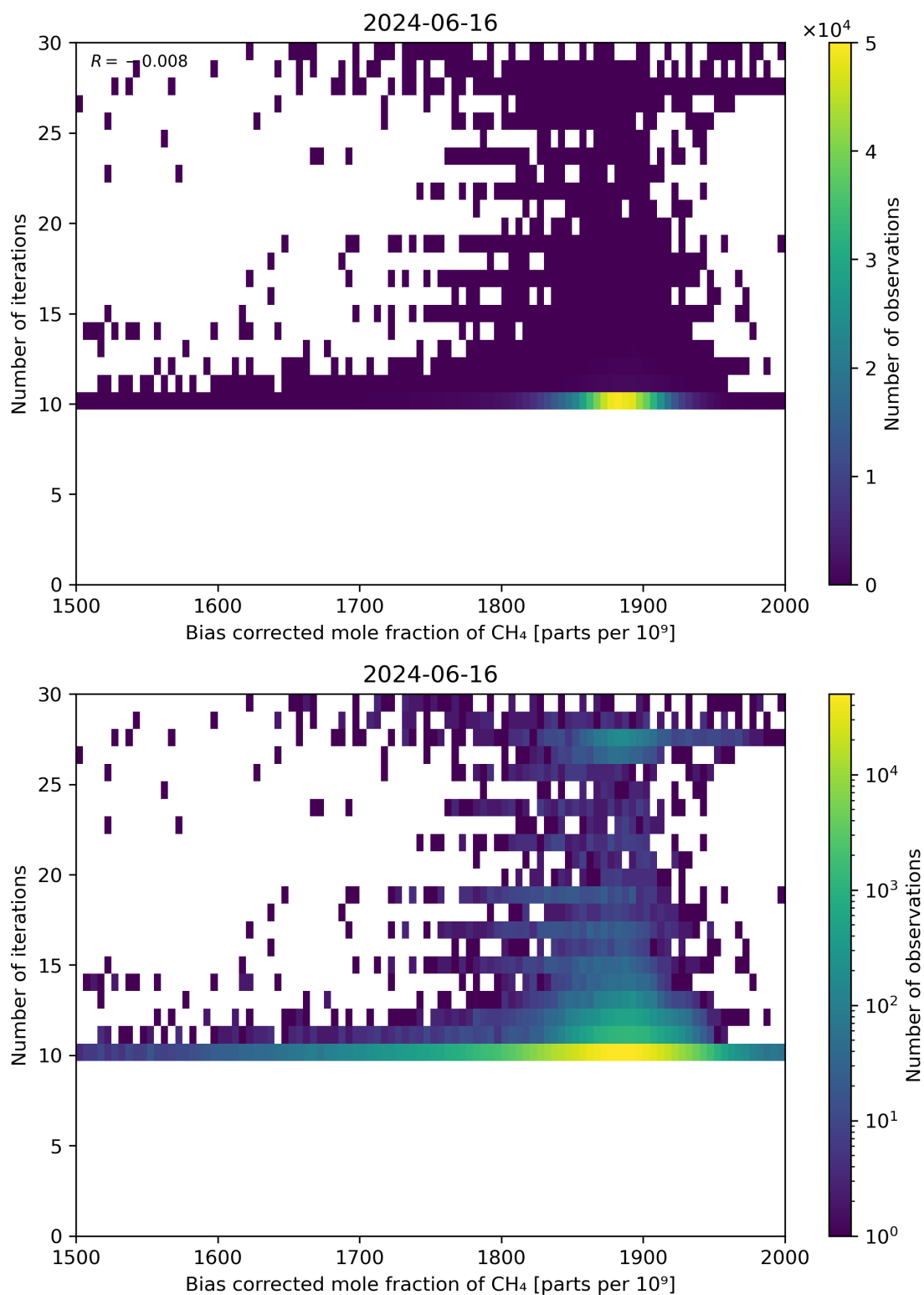
Figure 67: Scatter density plot of “Bias corrected mole fraction of CH 4 ” against “Number of iterations” for 2024-06-15 to 2024-06-17.
