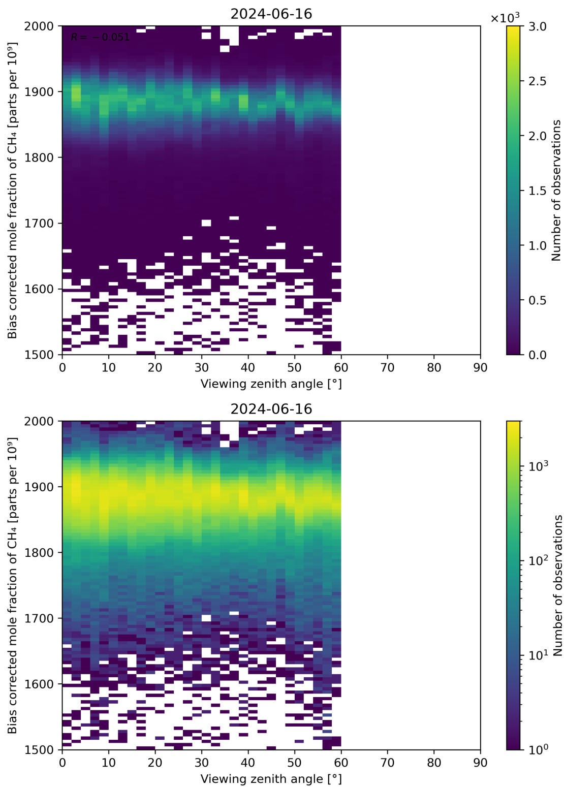
Figure 111: Scatter density plot of “Viewing zenith angle” against “Bias corrected mole fraction of CH 4 ” for 2024-06-15 to 2024-06-17.
