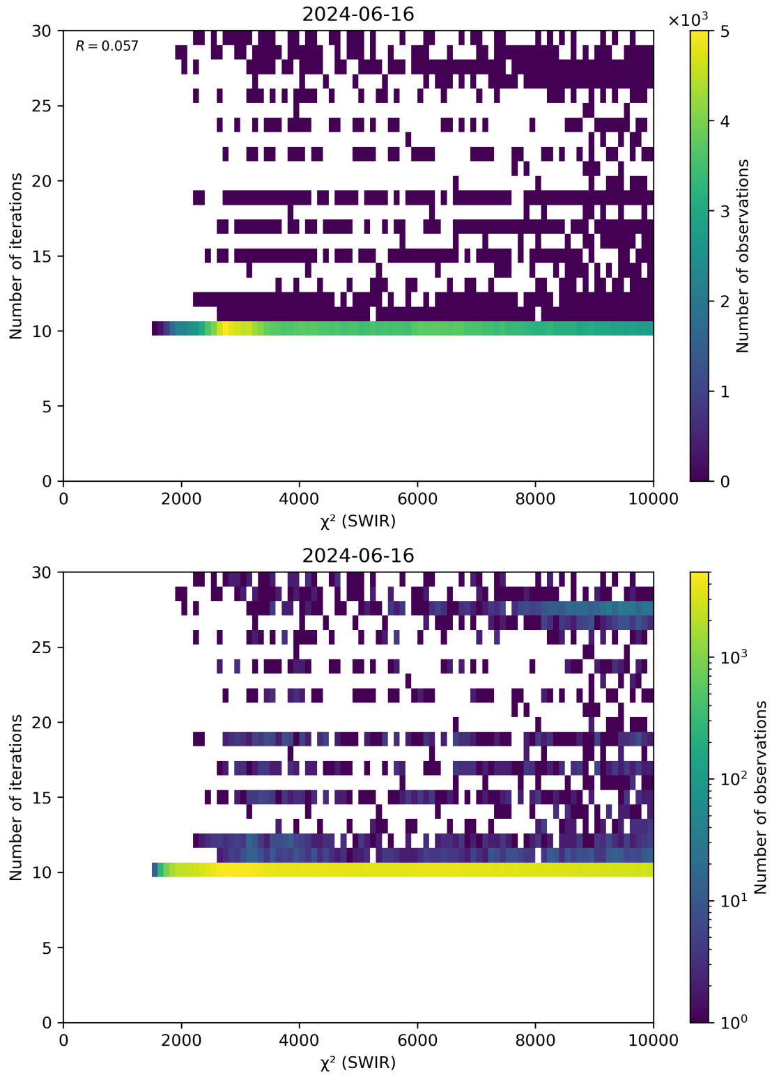
Figure 50: Scatter density plot of “ \chi^2 (SWIR)” against “Number of iterations” for 2024-06-15 to 2024-06-17.
