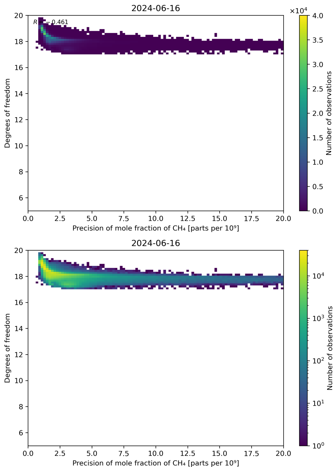
Figure 80: Scatter density plot of “Precision of mole fraction of CH 4 ” against “Degrees of freedom” for 2024-06-15 to 2024-06-17.
