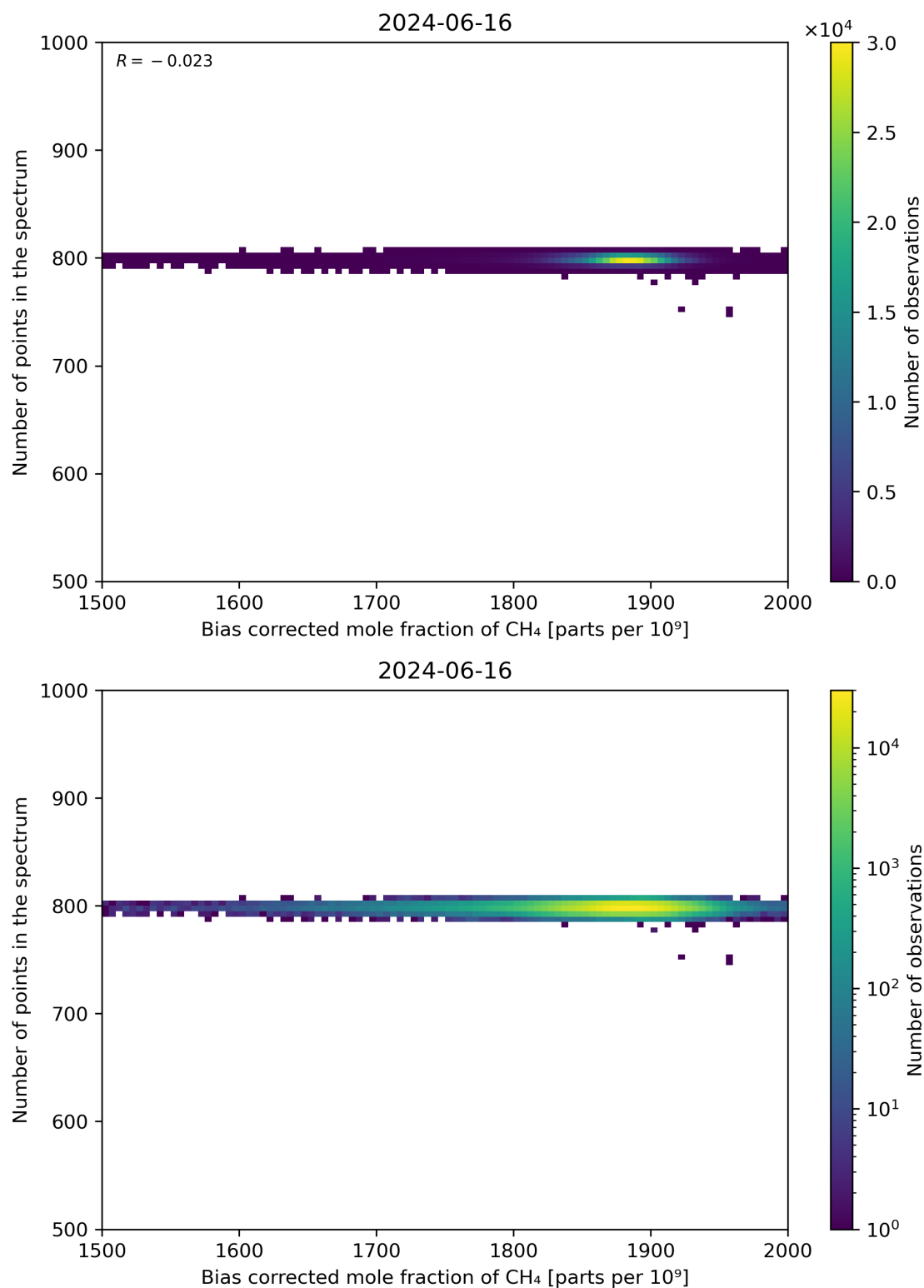
Figure 68: Scatter density plot of “Bias corrected mole fraction of CH 4 ” against “Number of points in the spectrum” for 2024-06-15 to 2024-06-17.
