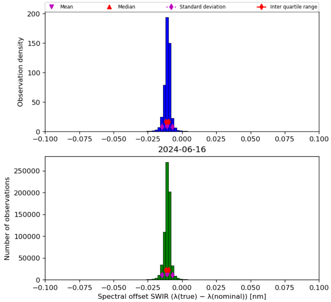
Figure 27: Histogram of “Spectral offset SWIR ( \lambda(\text{true}) - \lambda(\text{nominal}) )” for 2024-06-15 to 2024-06-17
