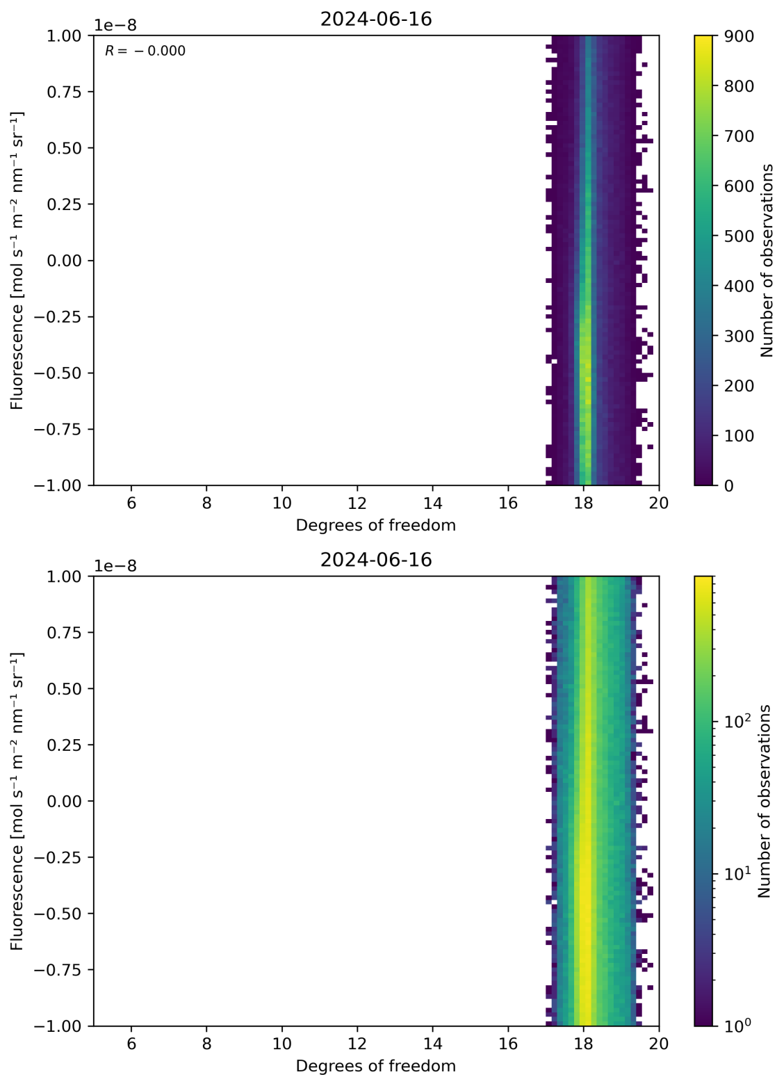
Figure 51: Scatter density plot of “Degrees of freedom” against “Fluorescence” for 2024-06-15 to 2024-06-17.
