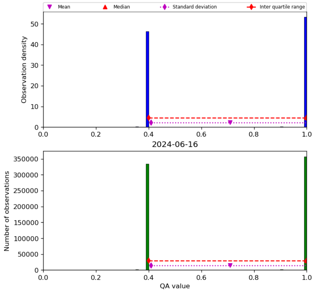
Figure 22: Histogram of “QA value” for 2024-06-15 to 2024-06-17
