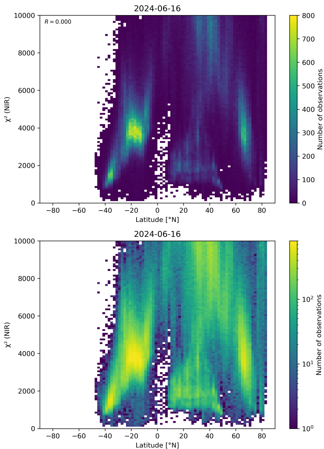
Figure 53: Scatter density plot of “Latitude” against “ \chi^2 (NIR)” for 2024-06-15 to 2024-06-17.
