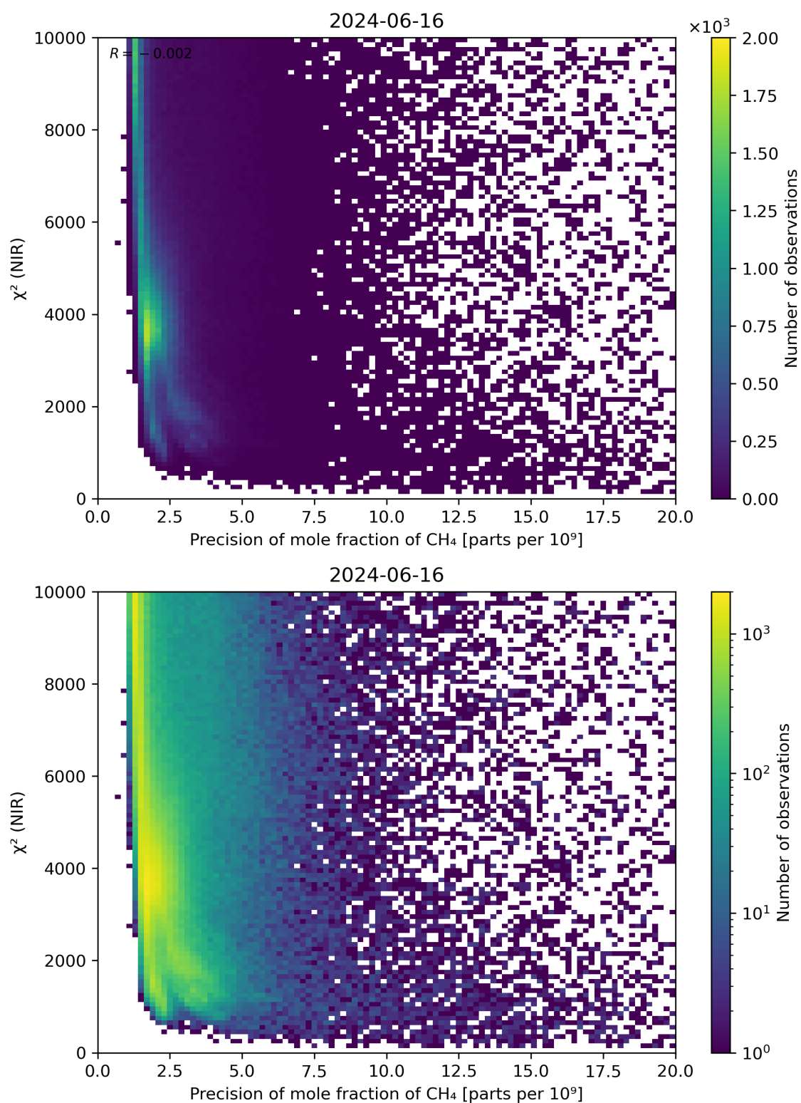
Figure 78: Scatter density plot of “Precision of mole fraction of CH 4 ” against “ \chi^2 (NIR)” for 2024-06-15 to 2024-06-17.
