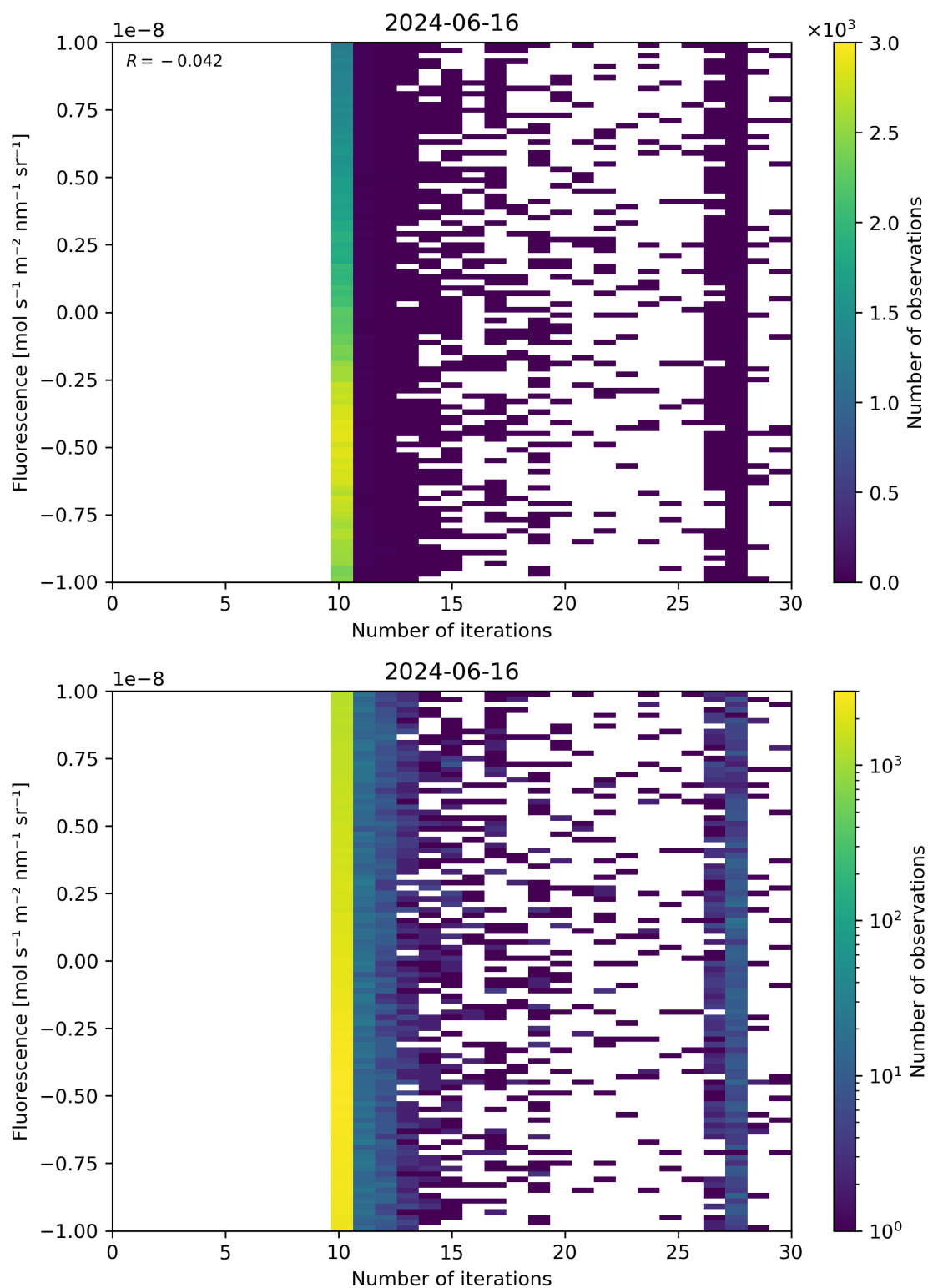
Figure 87: Scatter density plot of “Number of iterations” against “Fluorescence” for 2024-06-15 to 2024-06-17.
