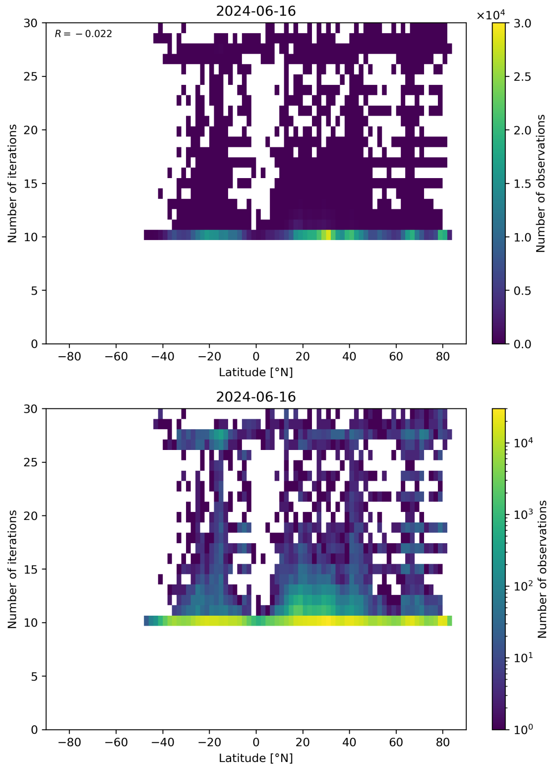
Figure 60: Scatter density plot of “Latitude” against “Number of iterations” for 2024-06-15 to 2024-06-17.
