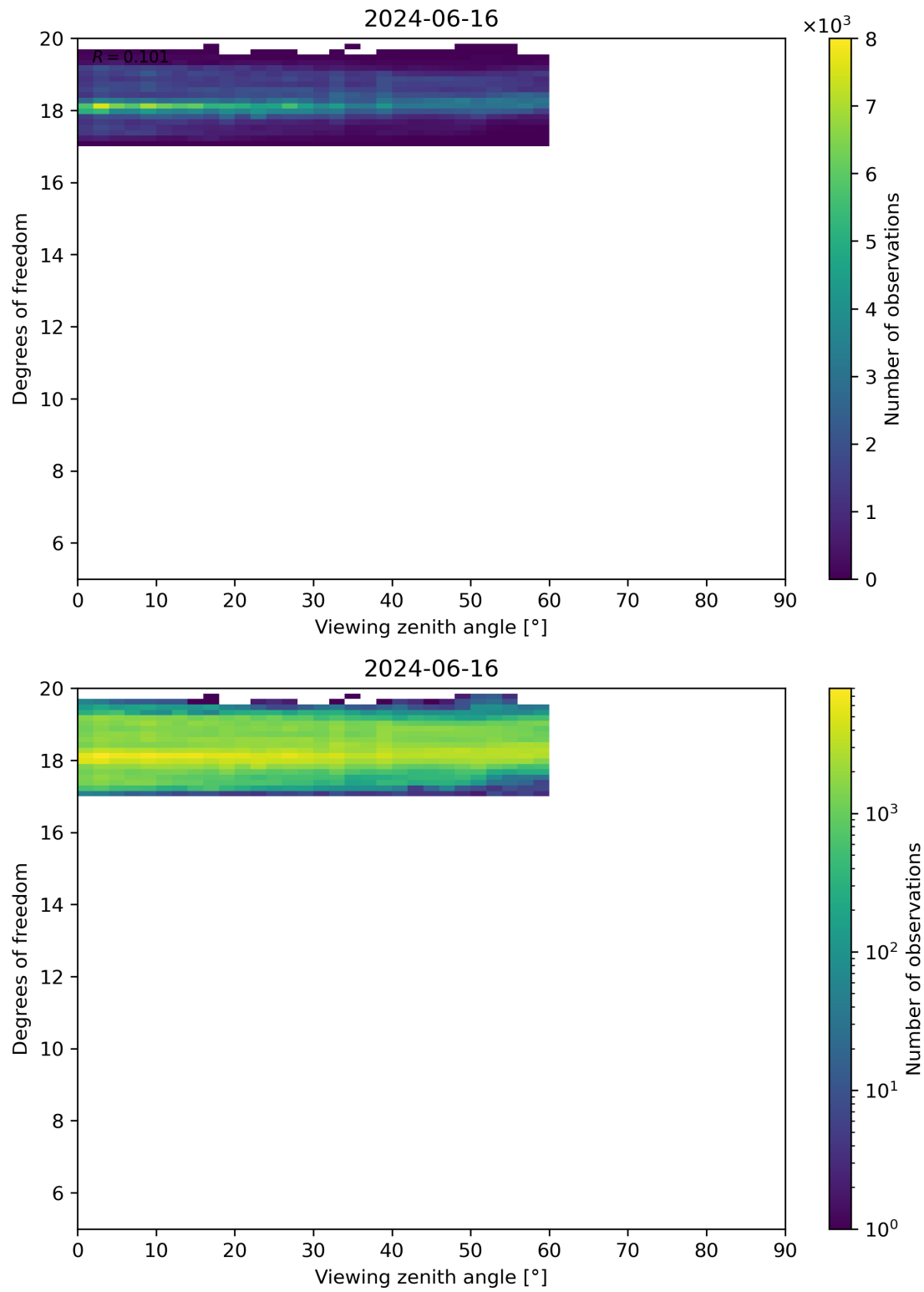
Figure 107: Scatter density plot of “Viewing zenith angle” against “Degrees of freedom” for 2024-06-15 to 2024-06-17.
