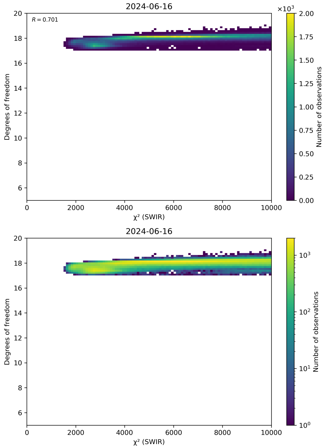
Figure 48: Scatter density plot of “ \chi^2 (SWIR)” against “Degrees of freedom” for 2024-06-15 to 2024-06-17.
