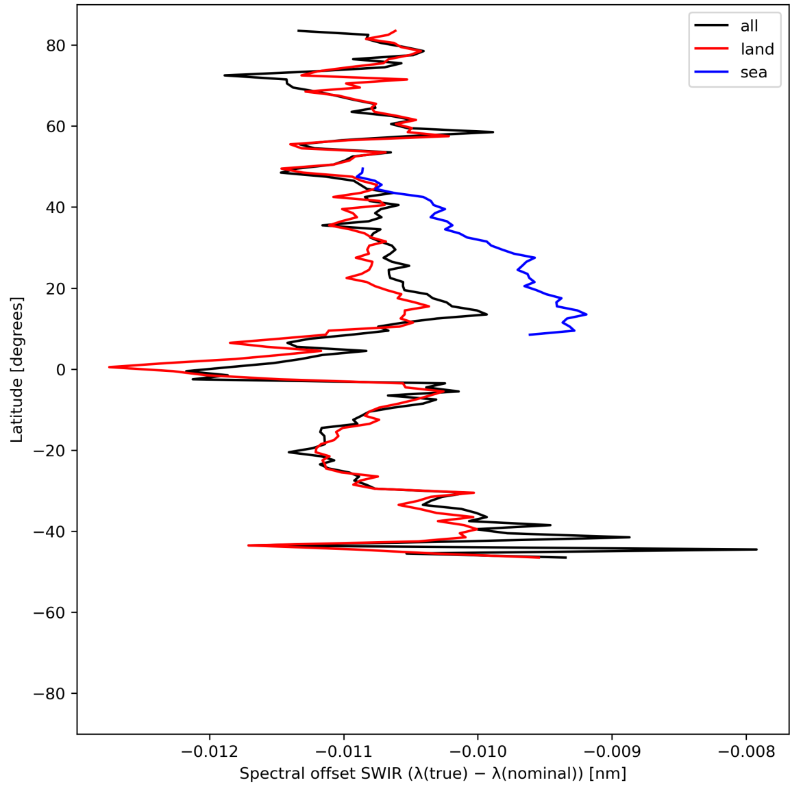
Figure 16: Zonal average of “Spectral offset SWIR ( \lambda(\text{true}) - \lambda(\text{nominal}) )” for 2024-06-15 to 2024-06-17.
