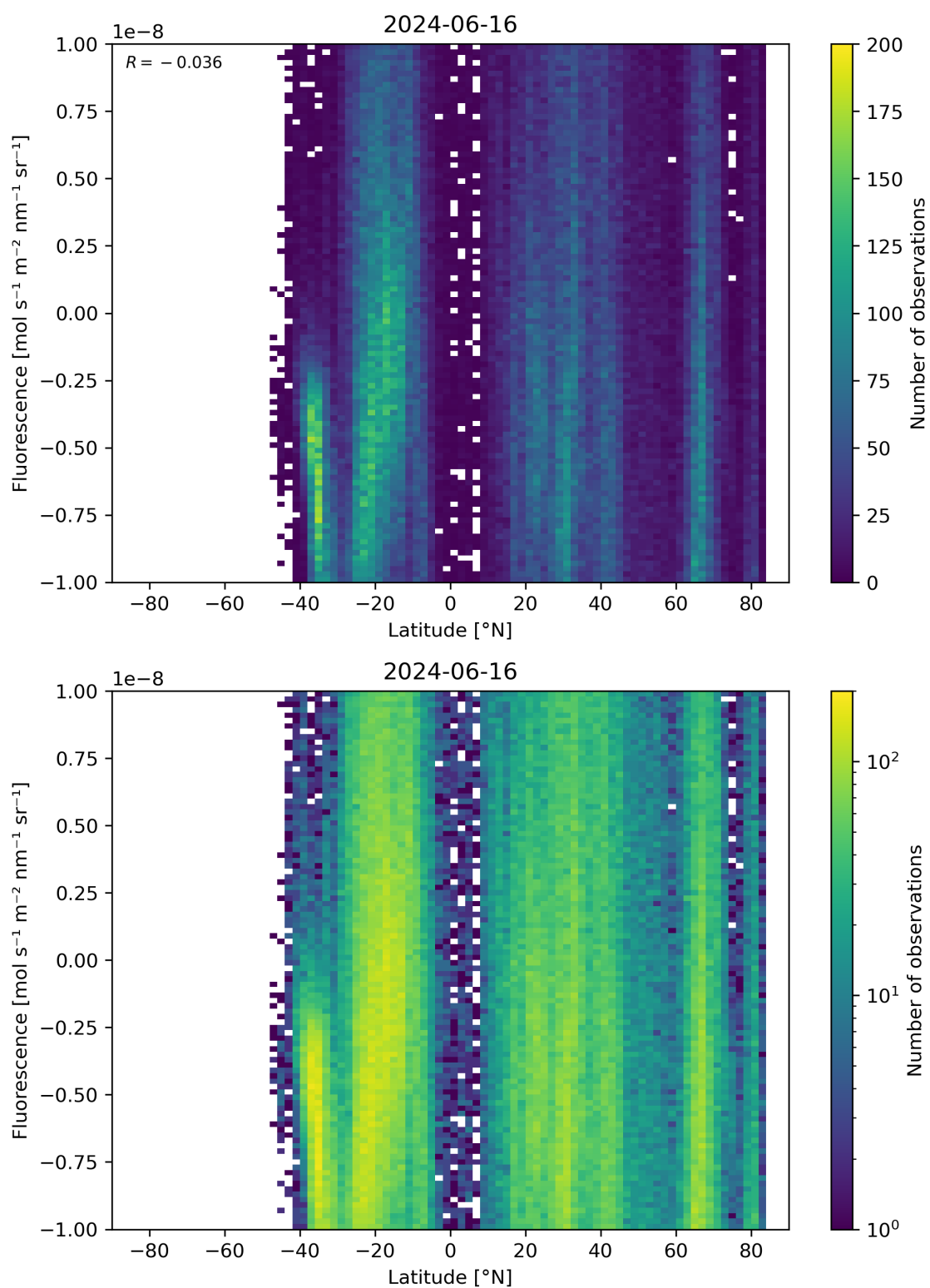
Figure 56: Scatter density plot of “Latitude” against “Fluorescence” for 2024-06-15 to 2024-06-17.
