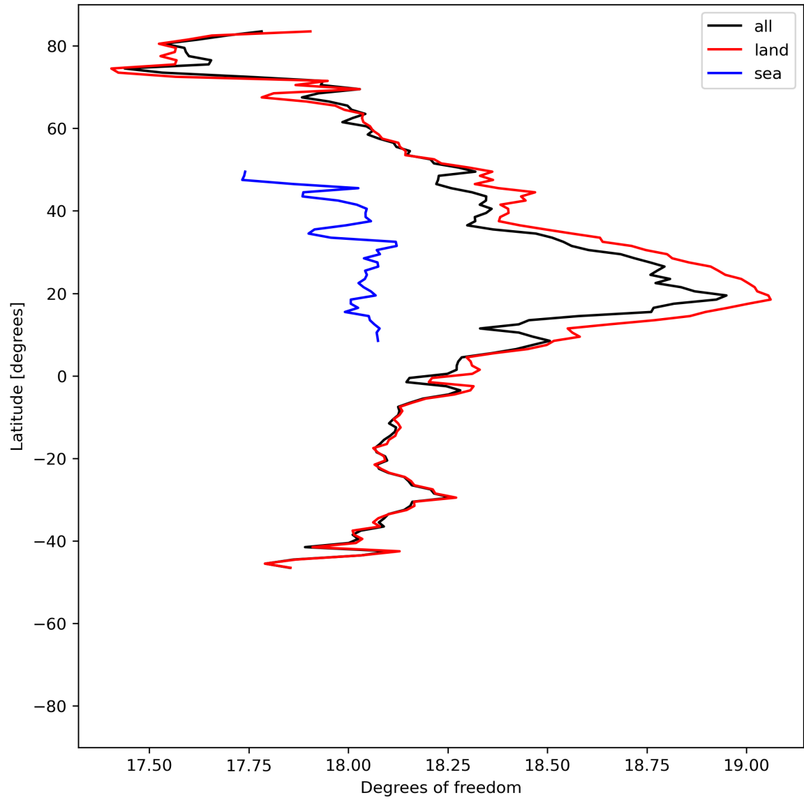
Figure 19: Zonal average of “Degrees of freedom” for 2024-06-15 to 2024-06-17.
