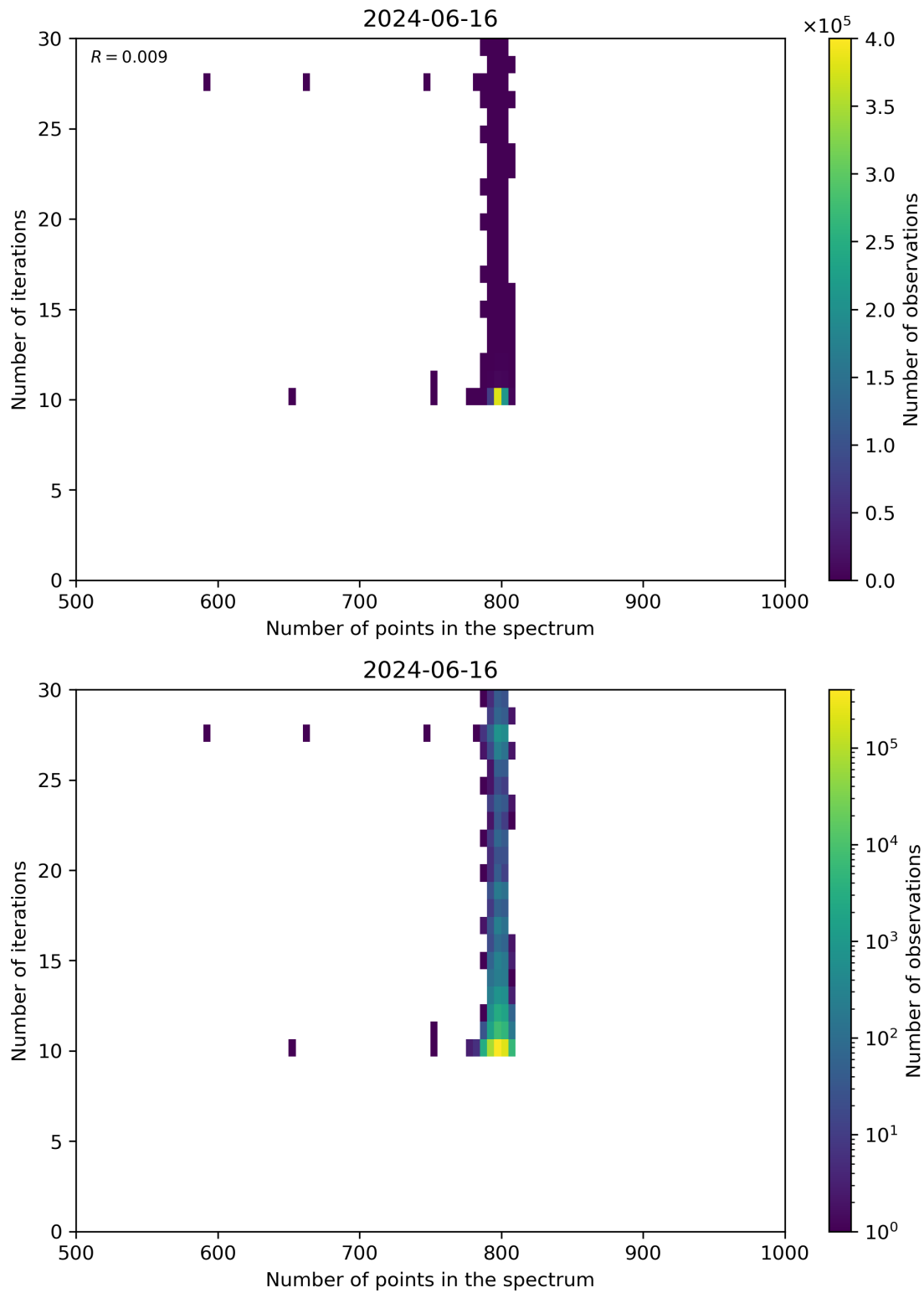
Figure 92: Scatter density plot of “Number of points in the spectrum” against “Number of iterations” for 2024-06-15 to 2024-06-17.
