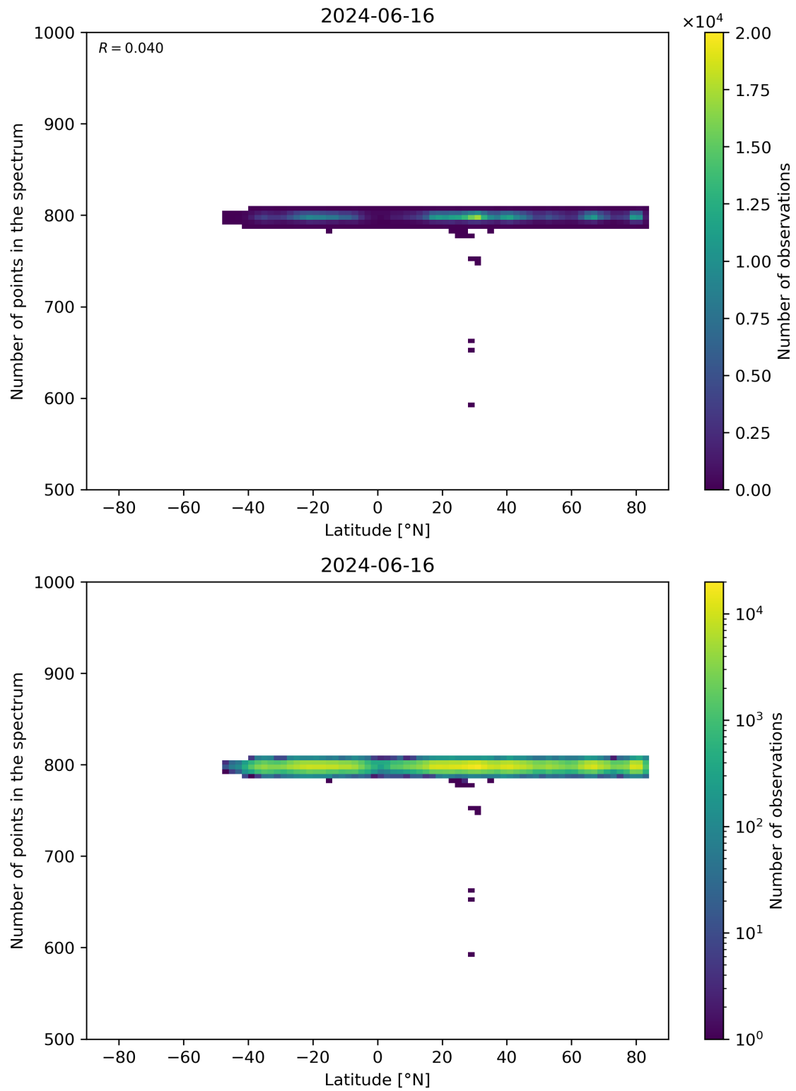
Figure 61: Scatter density plot of “Latitude” against “Number of points in the spectrum” for 2024-06-15 to 2024-06-17.
