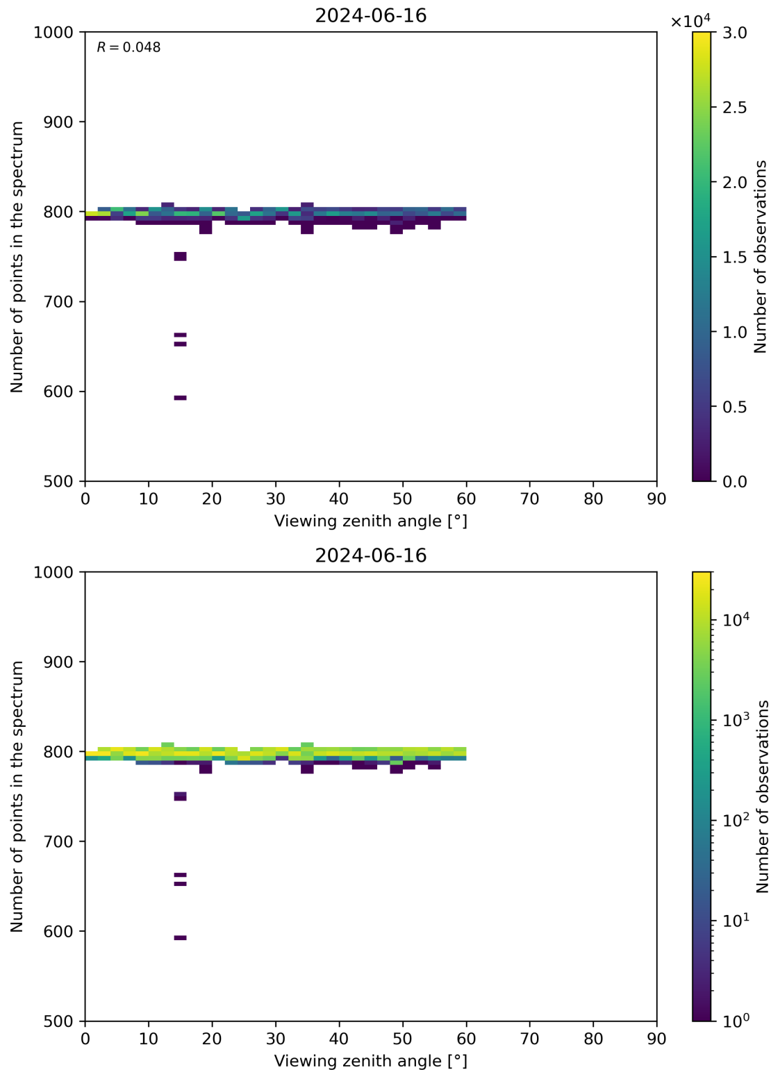
Figure 114: Scatter density plot of “Viewing zenith angle” against “Number of points in the spectrum” for 2024-06-15 to 2024-06-17.
