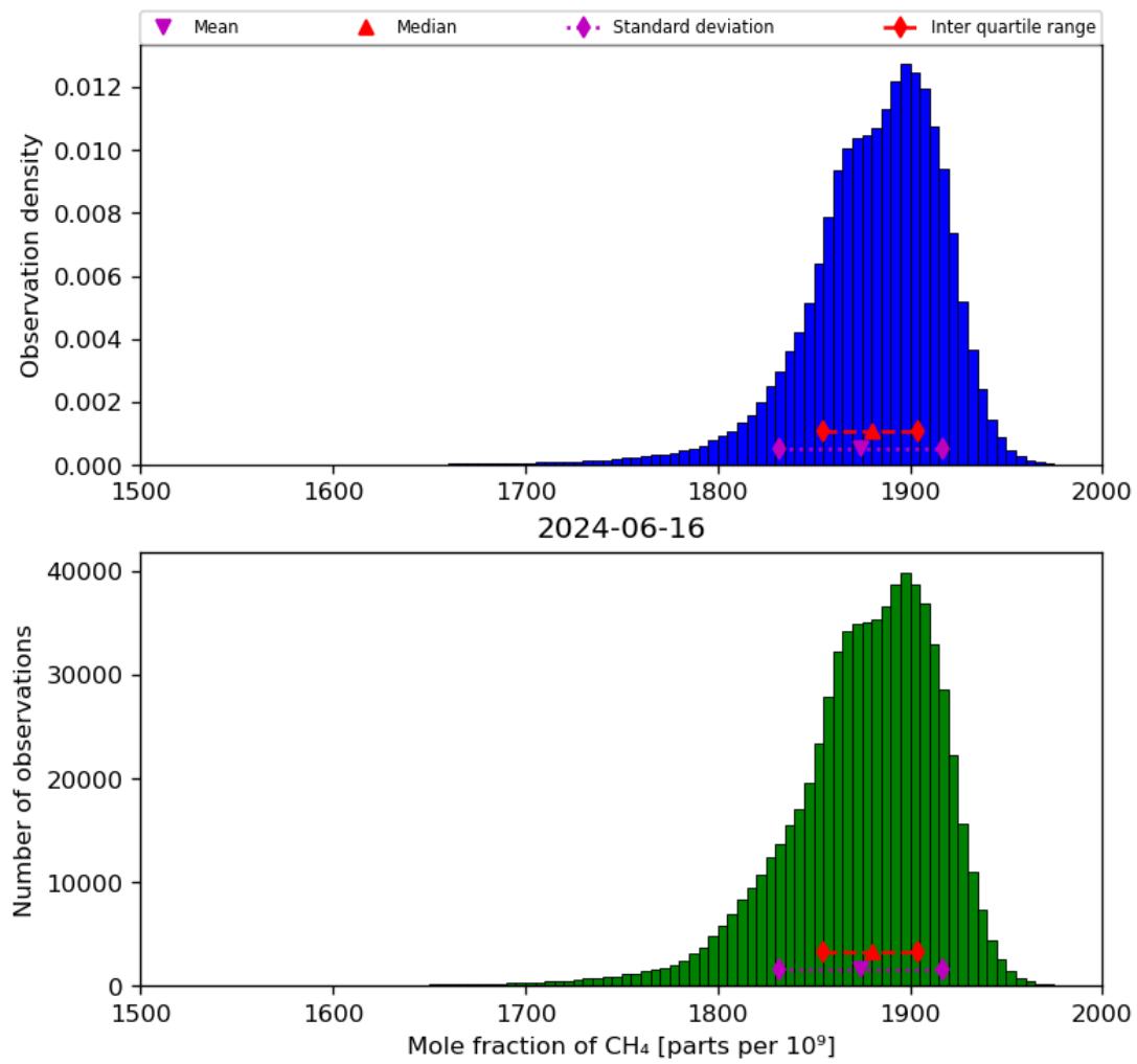
Figure 23: Histogram of “Mole fraction of CH 4 ” for 2024-06-15 to 2024-06-17
