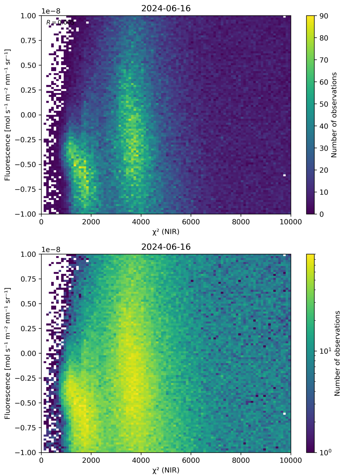
Figure 45: Scatter density plot of “ \chi^2 (NIR)” against “Fluorescence” for 2024-06-15 to 2024-06-17.
