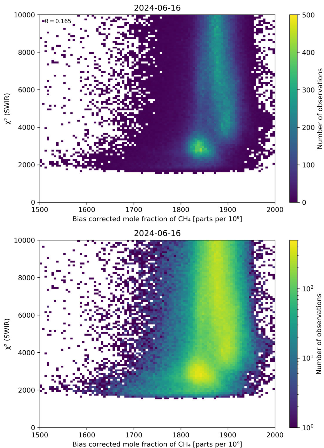
Figure 64: Scatter density plot of “Bias corrected mole fraction of CH 4 ” against “ \chi^2 (SWIR)” for 2024-06-15 to 2024-06-17.
