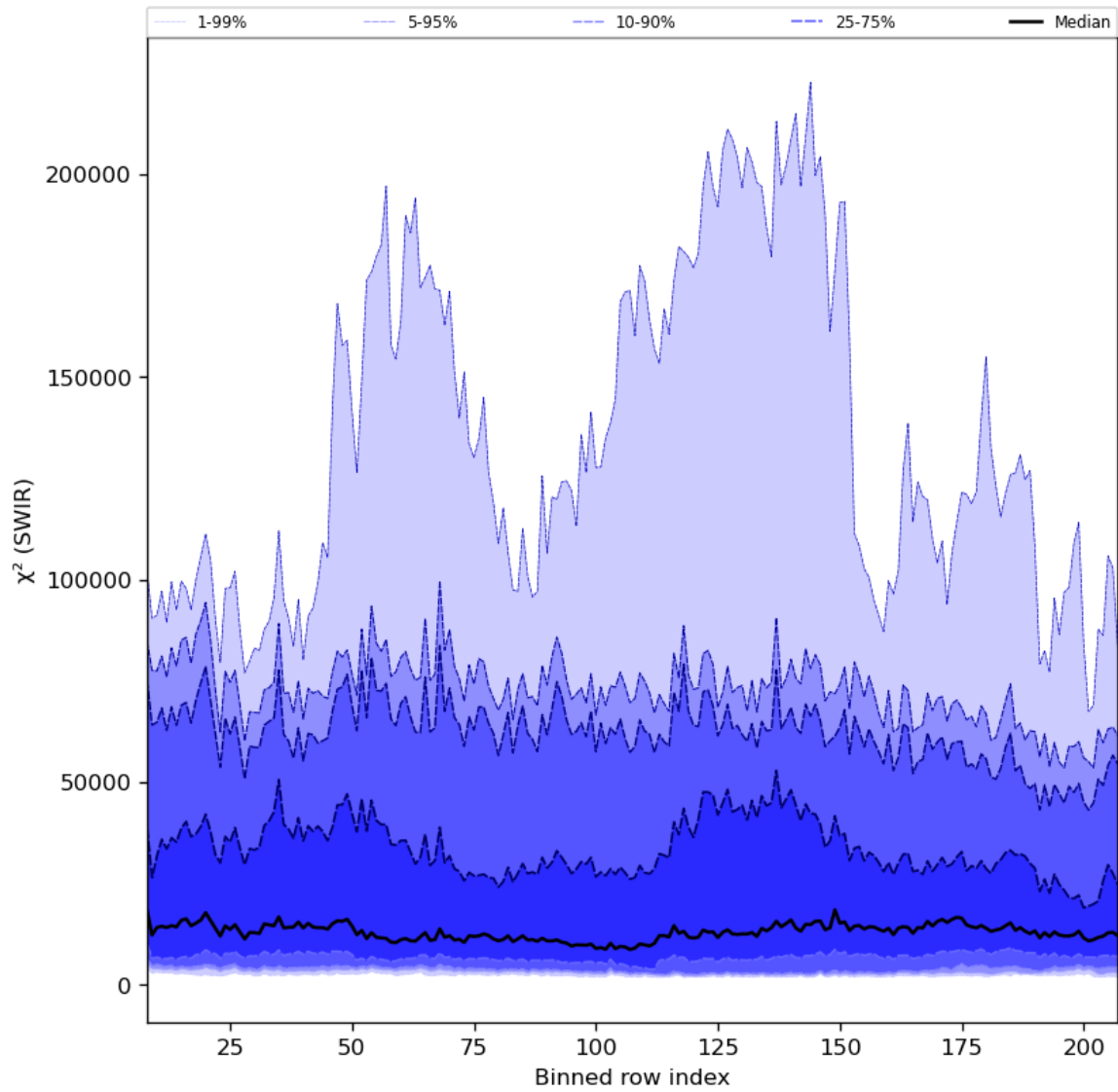
Figure 39: Along track statistics of “ \chi^2 (SWIR)” for 2024-06-15 to 2024-06-17
