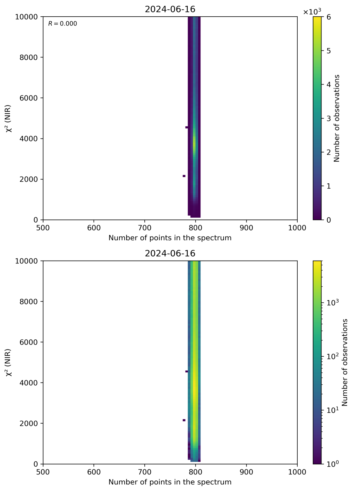
Figure 88: Scatter density plot of “Number of points in the spectrum” against “ \chi^2 (NIR)” for 2024-06-15 to 2024-06-17.
