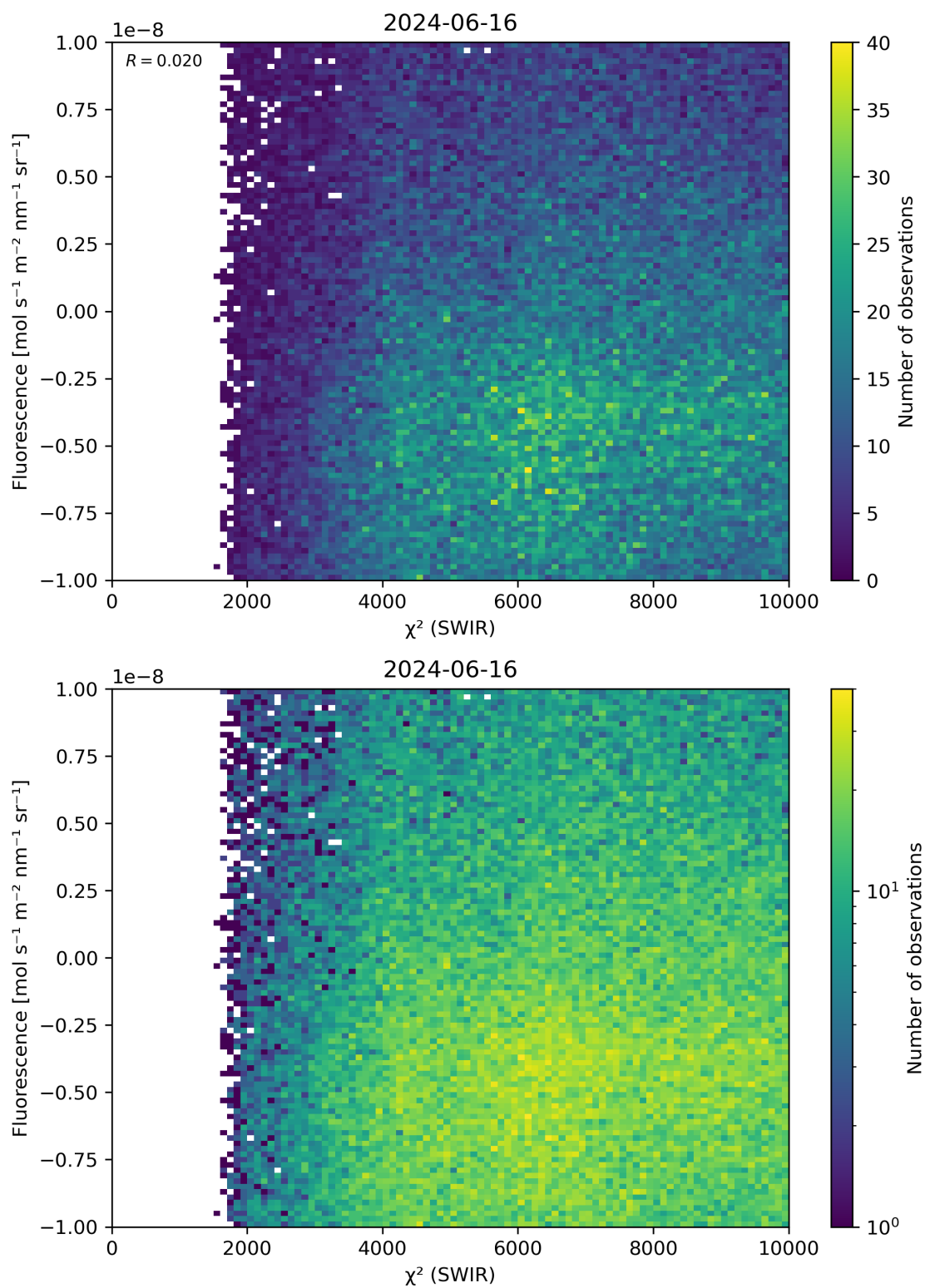
Figure 49: Scatter density plot of “ \chi^2 (SWIR)” against “Fluorescence” for 2024-06-15 to 2024-06-17.
