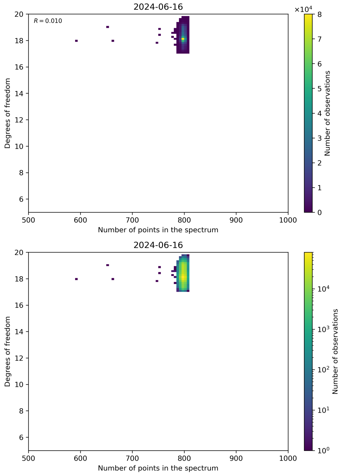
Figure 90: Scatter density plot of “Number of points in the spectrum” against “Degrees of freedom” for 2024-06-15 to 2024-06-17.
