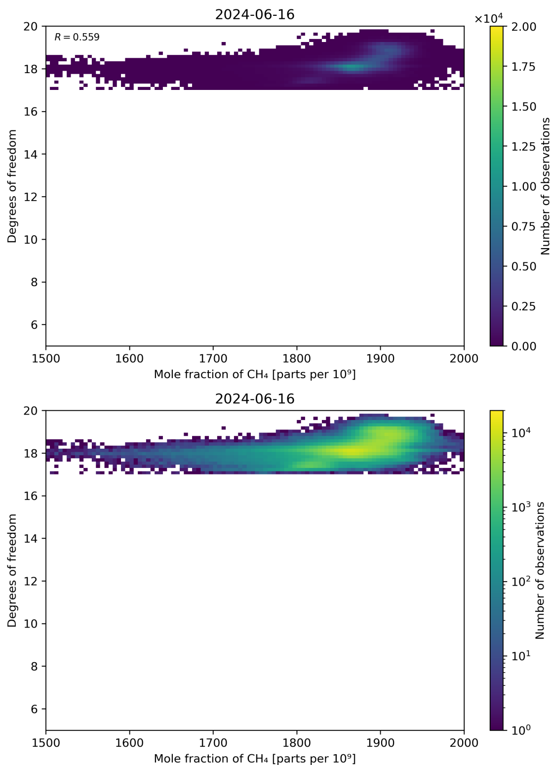
Figure 72: Scatter density plot of “Mole fraction of CH 4 ” against “Degrees of freedom” for 2024-06-15 to 2024-06-17.
