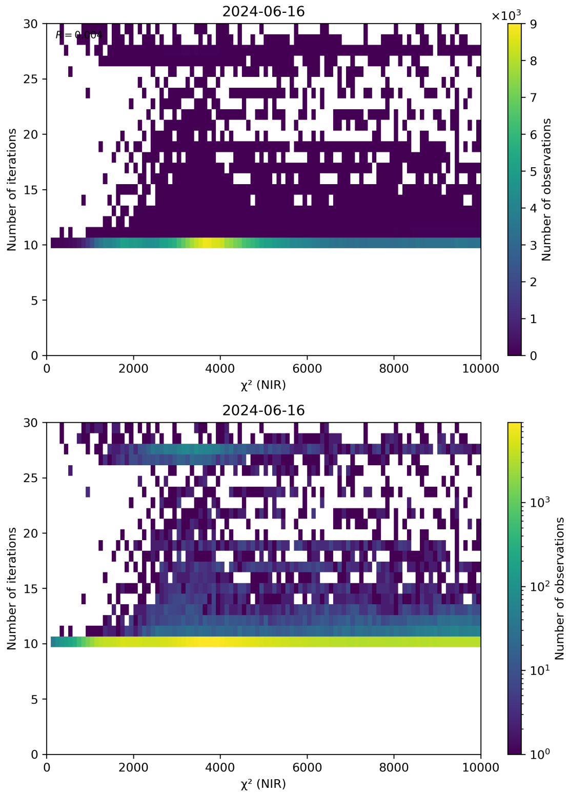
Figure 46: Scatter density plot of “ \chi^2 (NIR)” against “Number of iterations” for 2024-06-15 to 2024-06-17.
