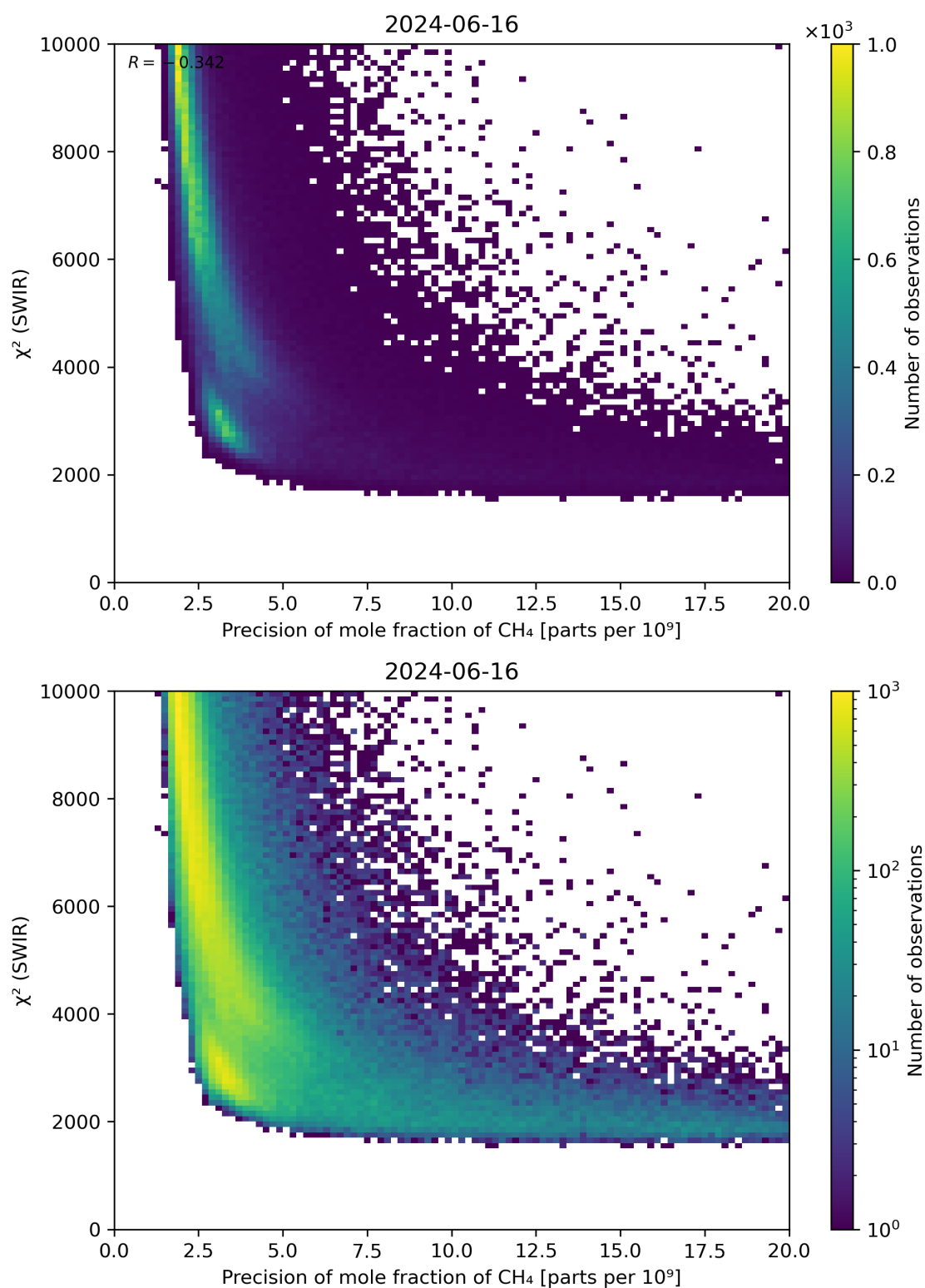
Figure 79: Scatter density plot of “Precision of mole fraction of \text{CH}_4 ” against “ \chi^2 (SWIR)” for 2024-06-15 to 2024-06-17.
