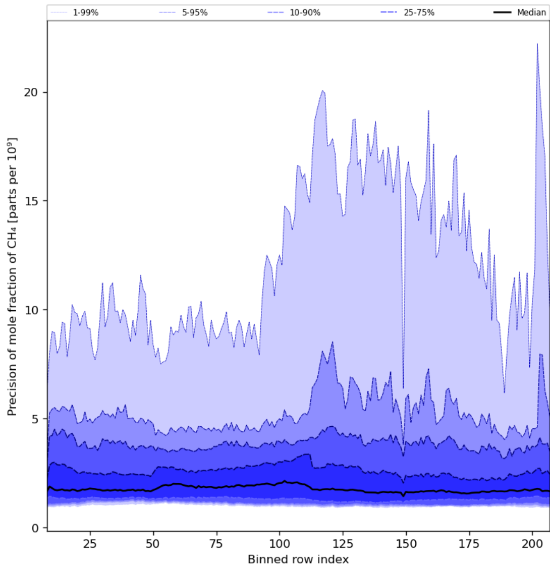
Figure 35: Along track statistics of “Precision of mole fraction of CH 4 ” for 2024-06-15 to 2024-06-17
