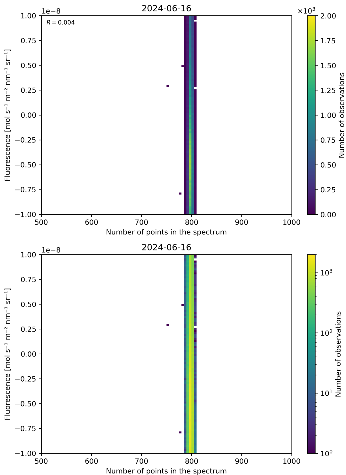
Figure 91: Scatter density plot of “Number of points in the spectrum” against “Fluorescence” for 2024-06-15 to 2024-06-17.
