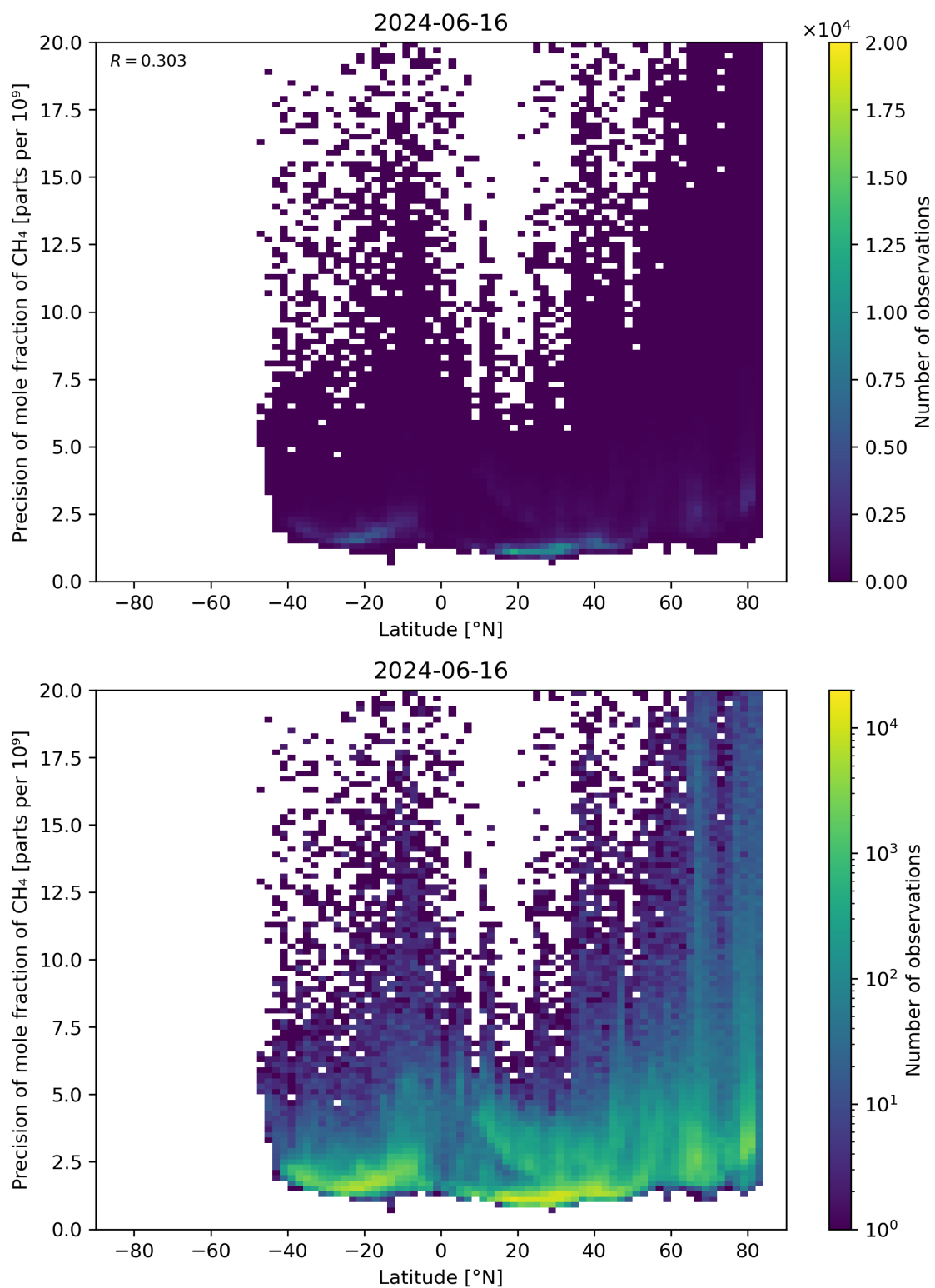
Figure 59: Scatter density plot of “Latitude” against “Precision of mole fraction of \text{CH}_4 ” for 2024-06-15 to 2024-06-17.
