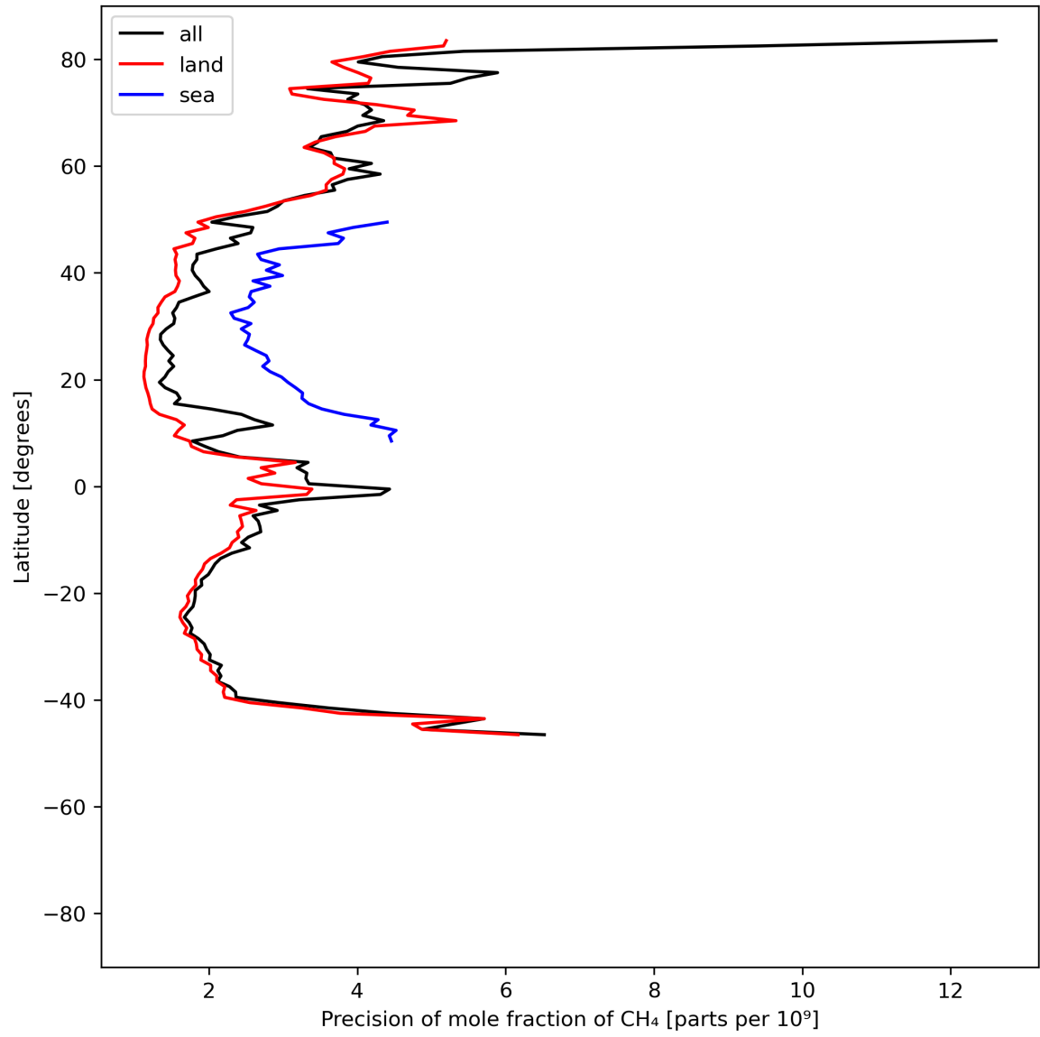
Figure 13: Zonal average of “Precision of mole fraction of CH 4 ” for 2024-06-15 to 2024-06-17.
