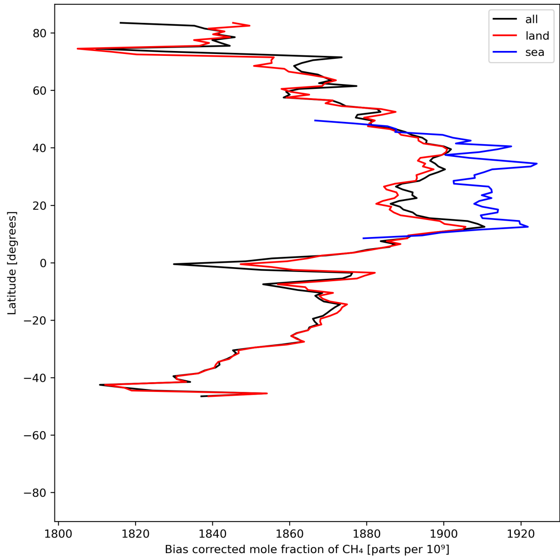
Figure 14: Zonal average of “Bias corrected mole fraction of CH 4 ” for 2024-06-15 to 2024-06-17.
