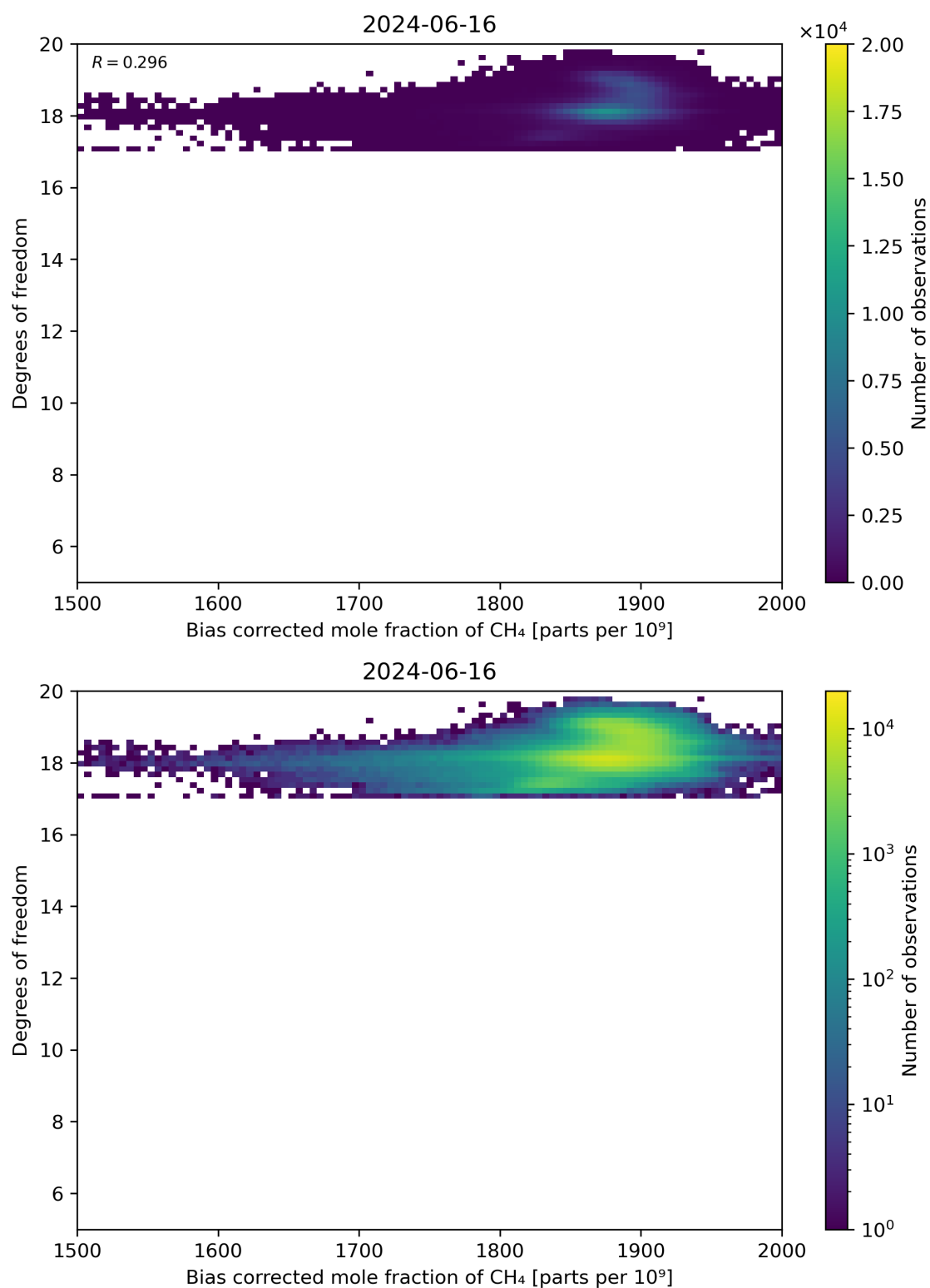
Figure 65: Scatter density plot of “Bias corrected mole fraction of CH 4 ” against “Degrees of freedom” for 2024-06-15 to 2024-06-17.
