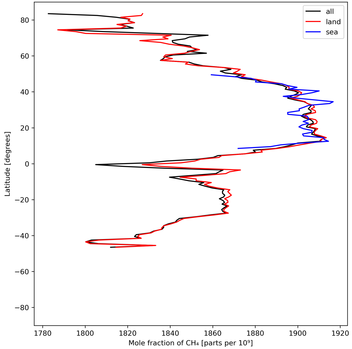
Figure 12: Zonal average of “Mole fraction of \text{CH}_4 ” for 2024-06-15 to 2024-06-17.
