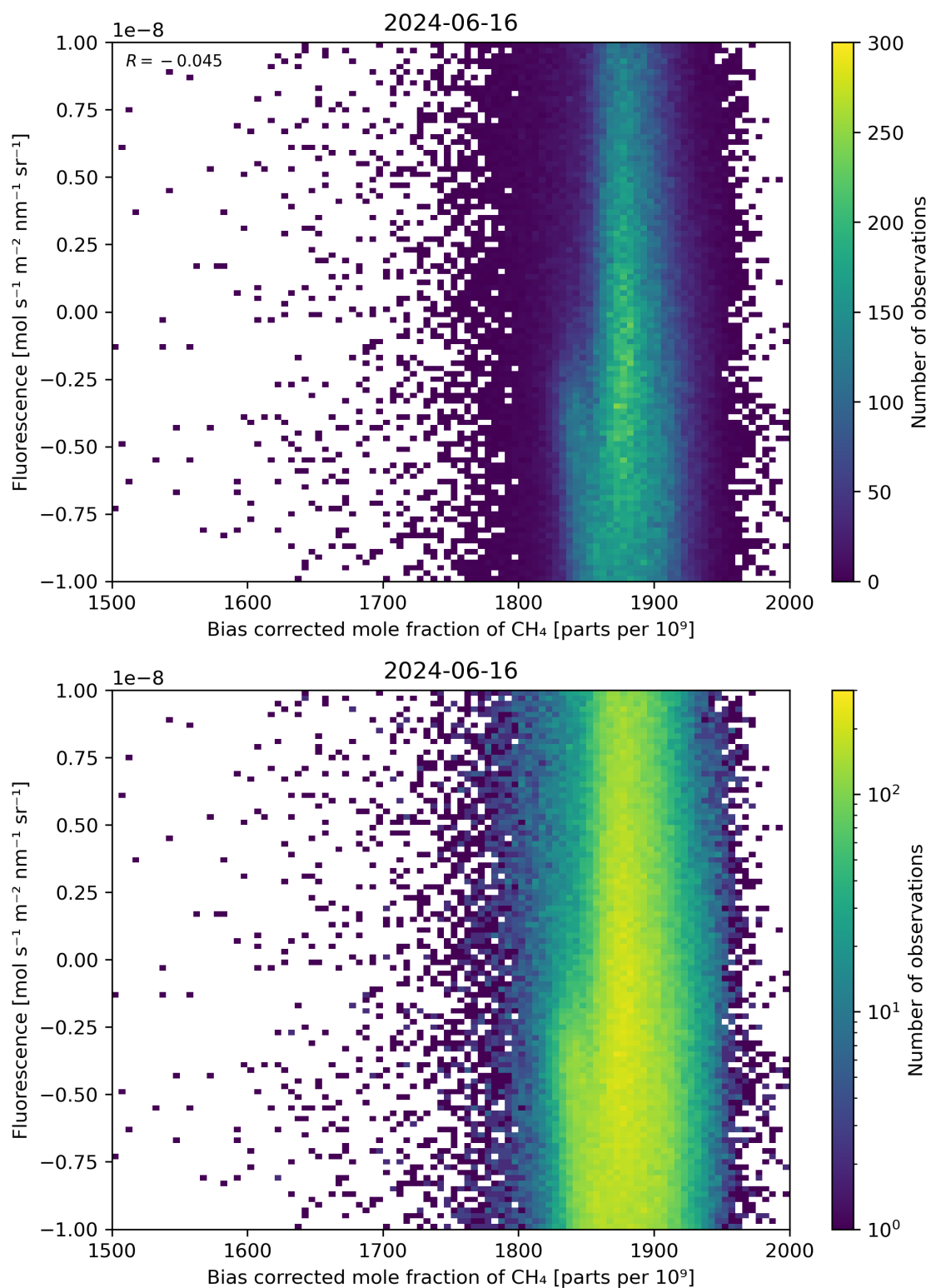
Figure 66: Scatter density plot of “Bias corrected mole fraction of \text{CH}_4 ” against “Fluorescence” for 2024-06-15 to 2024-06-17.
