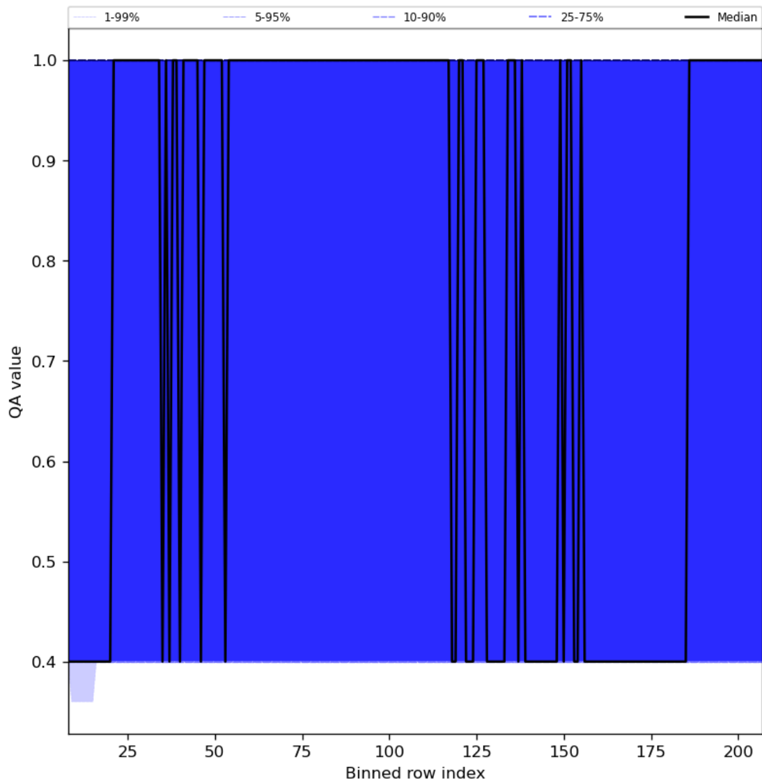
Figure 33: Along track statistics of “QA value” for 2024-06-15 to 2024-06-17
