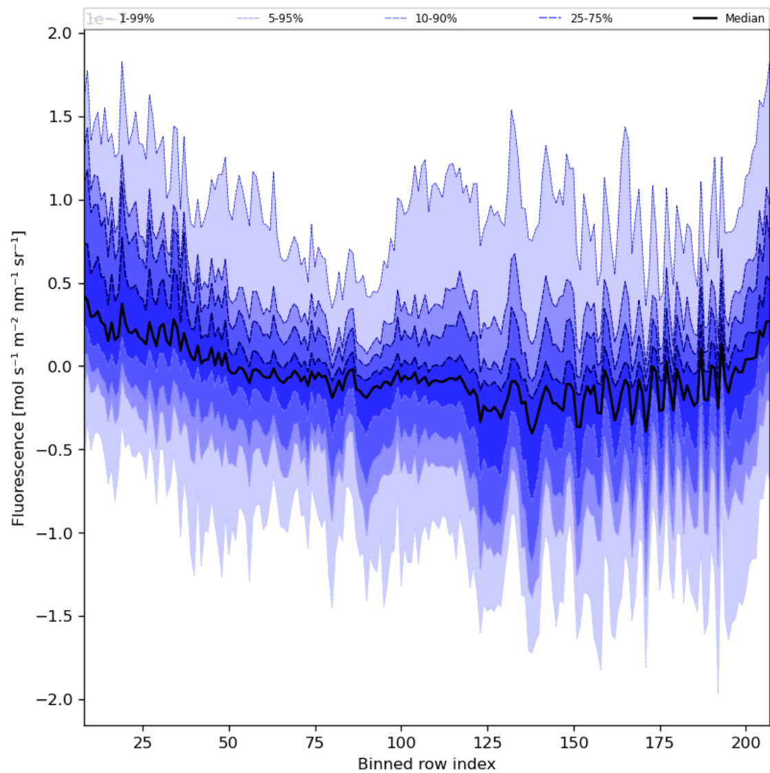
Figure 43: Along track statistics of “Fluorescence” for 2024-06-15 to 2024-06-17
