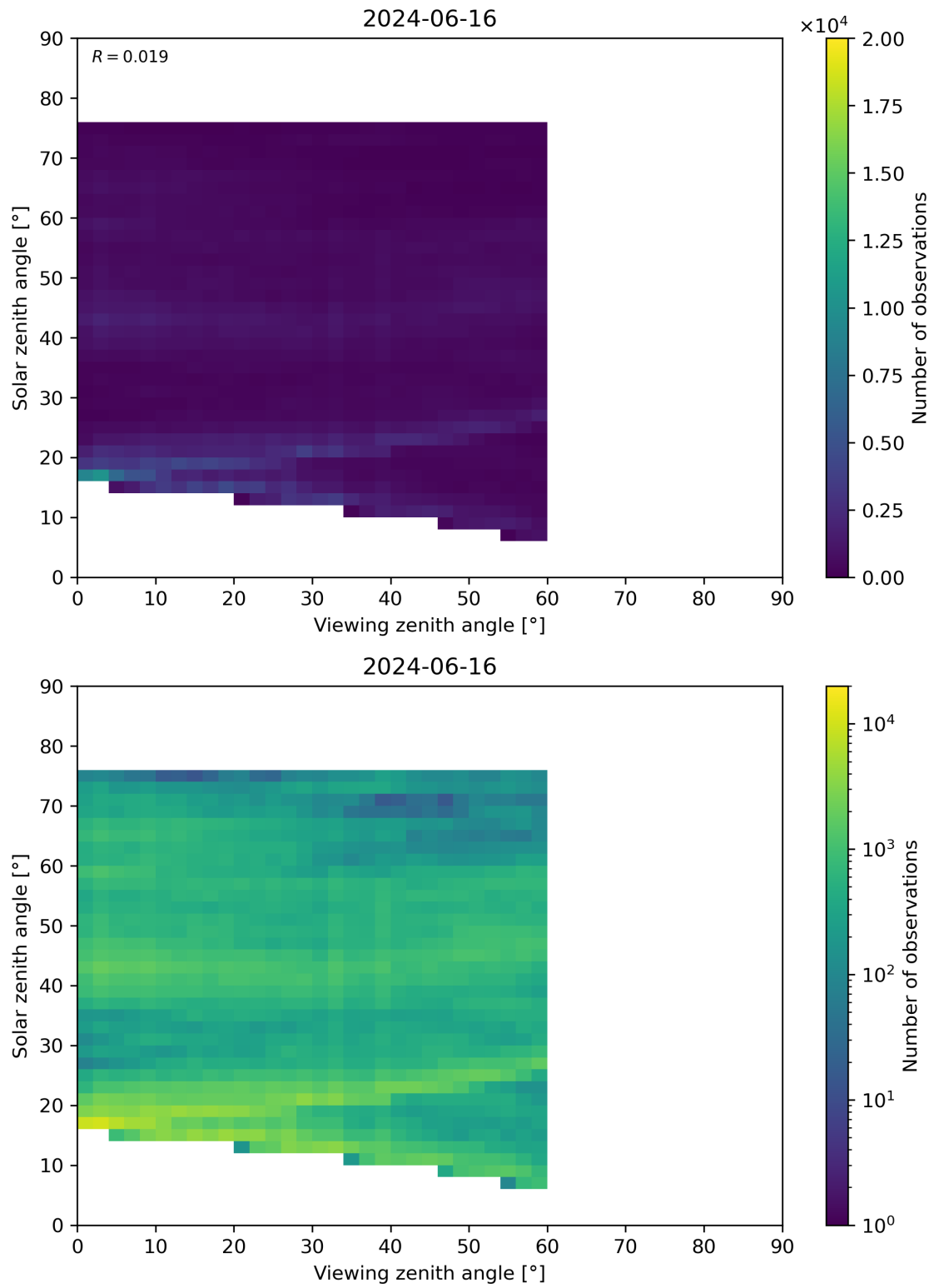
Figure 115: Scatter density plot of “Viewing zenith angle” against “Solar zenith angle” for 2024-06-15 to 2024-06-17.
