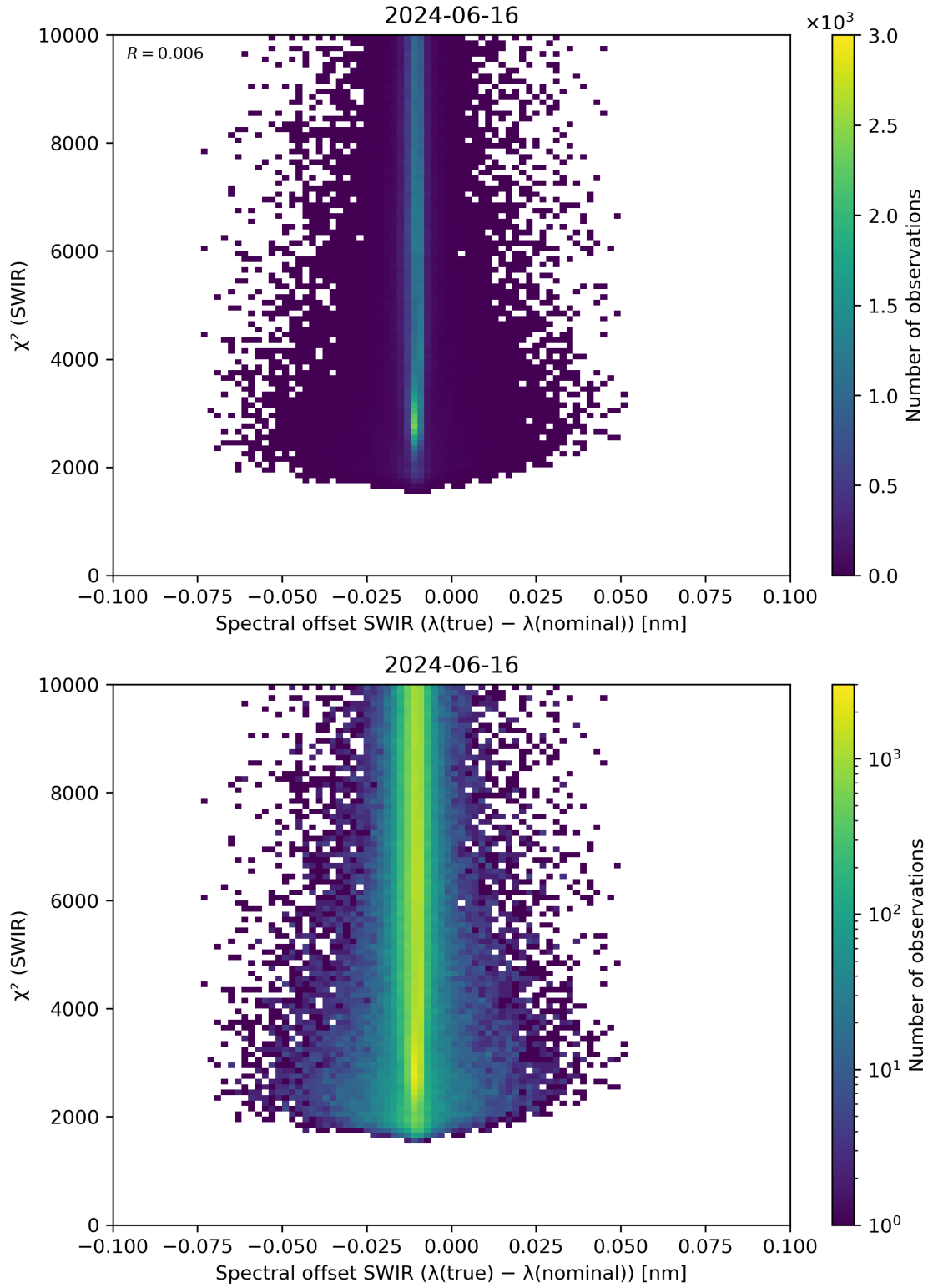
Figure 118: Scatter density plot of “Spectral offset SWIR ( \lambda(\text{true}) - \lambda(\text{nominal}) )” against “ \chi^2 (SWIR)” for 2024-06-15 to 2024-06-17.
