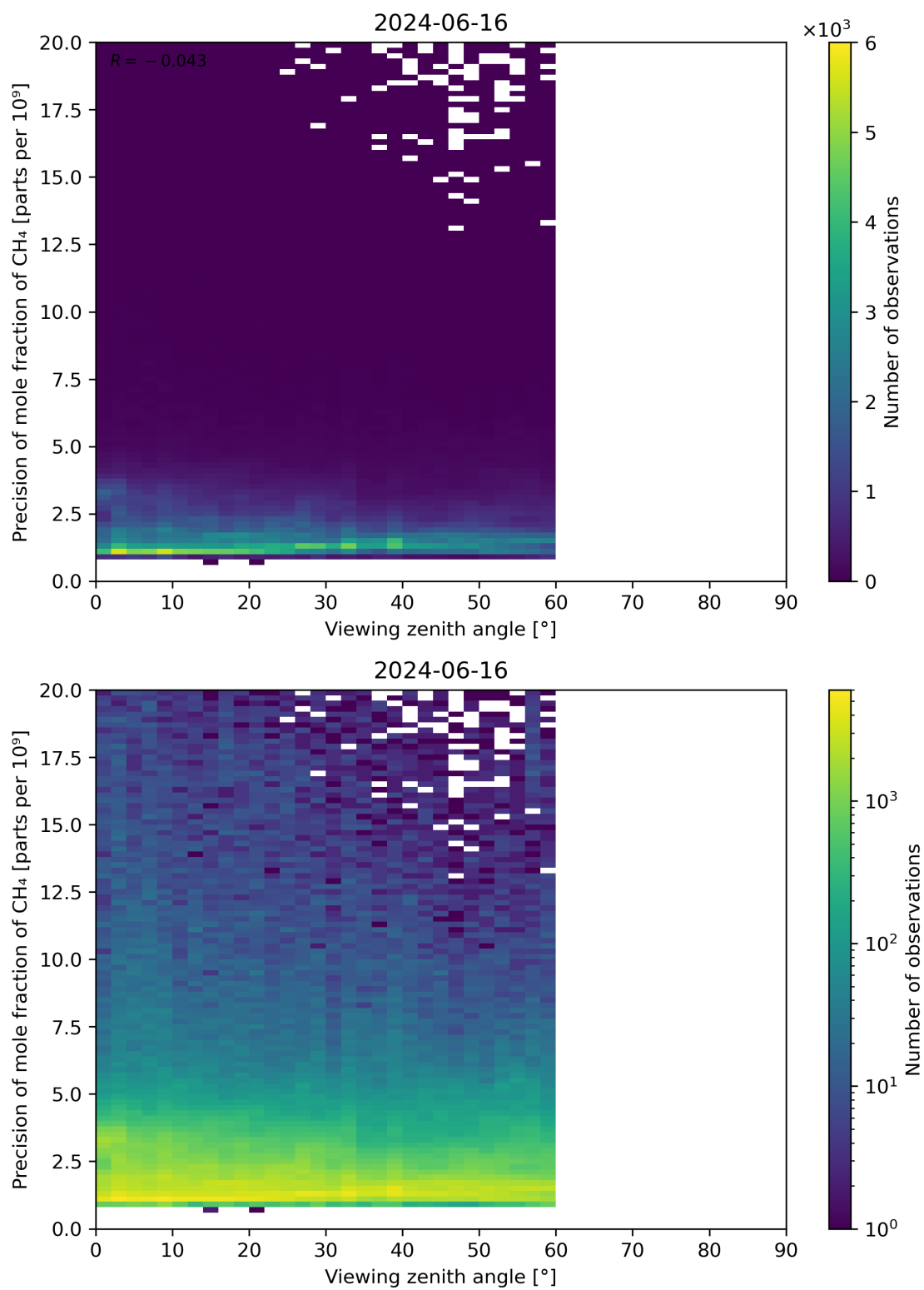
Figure 112: Scatter density plot of “Viewing zenith angle” against “Precision of mole fraction of CH 4 ” for 2024-06-15 to 2024-06-17.
