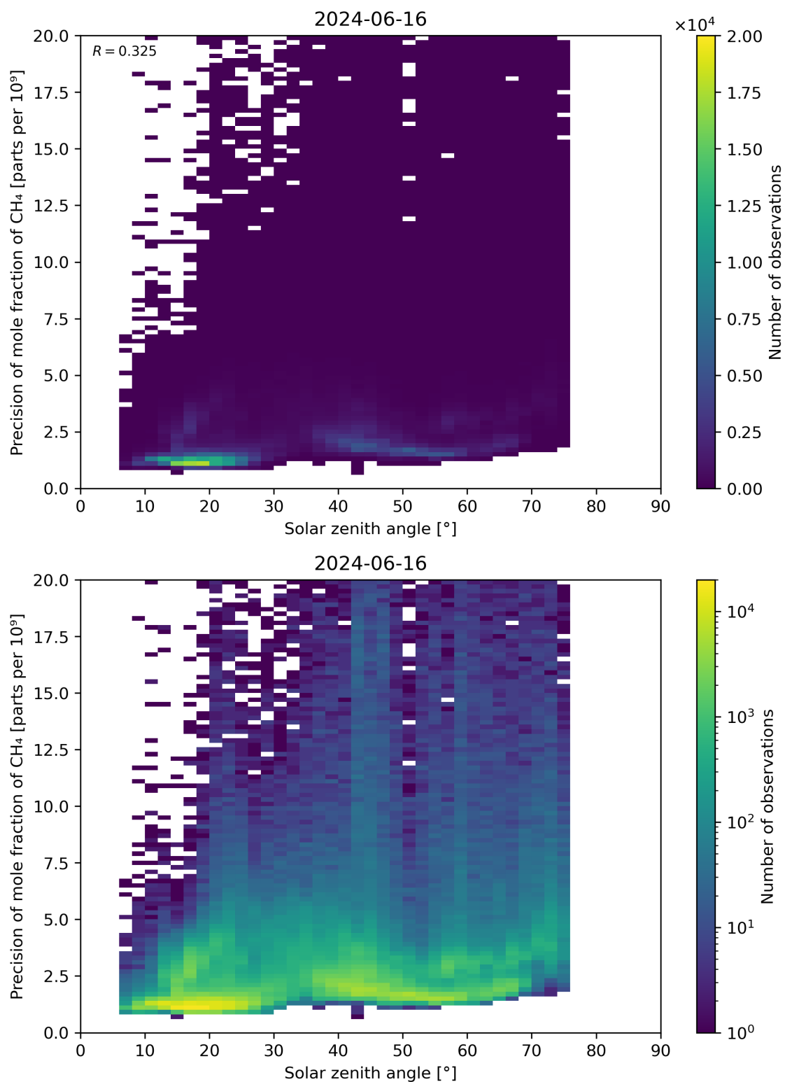
Figure 101: Scatter density plot of “Solar zenith angle” against “Precision of mole fraction of CH 4 ” for 2024-06-15 to 2024-06-17.
