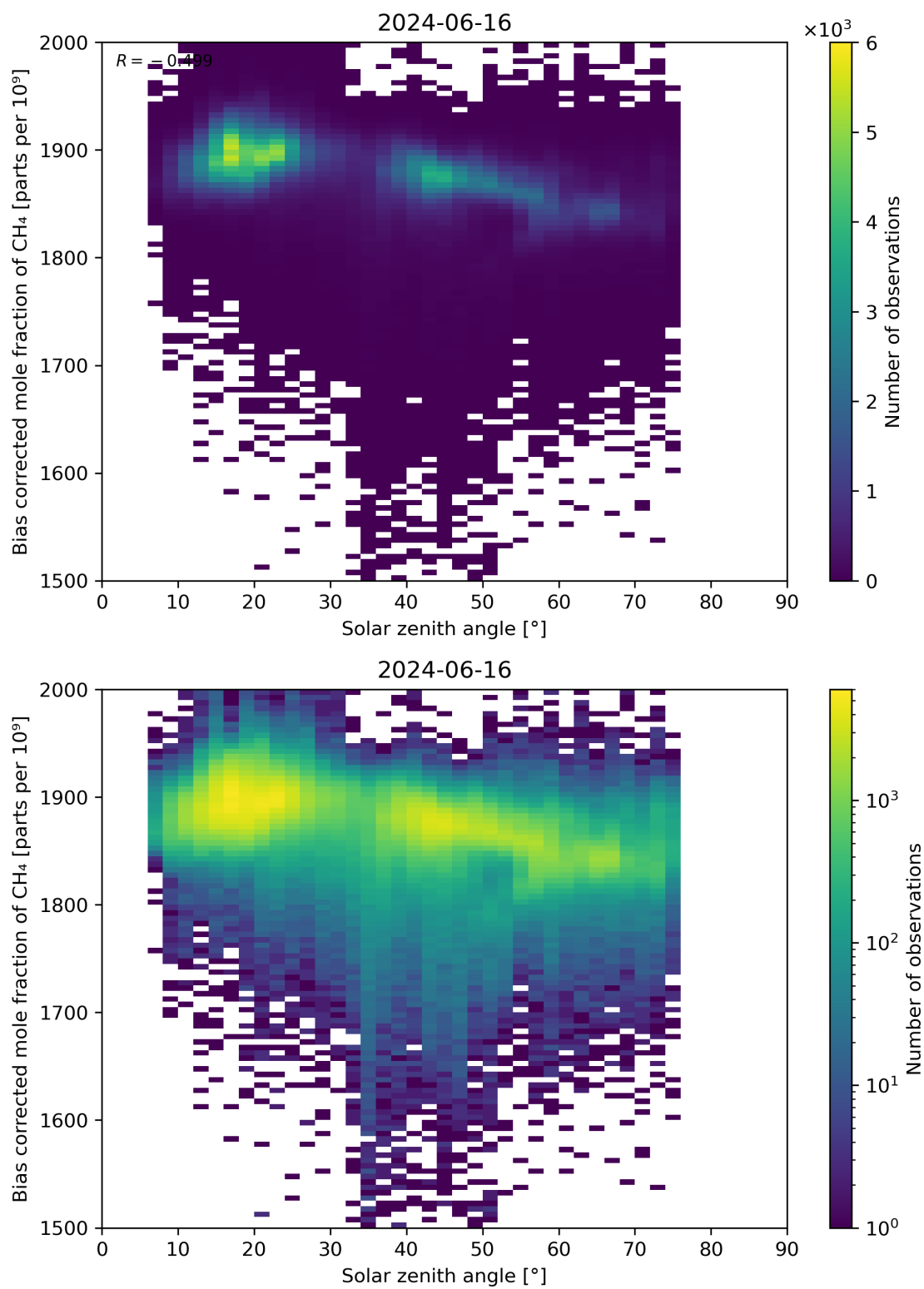
Figure 100: Scatter density plot of “Solar zenith angle” against “Bias corrected mole fraction of CH 4 ” for 2024-06-15 to 2024-06-17.
