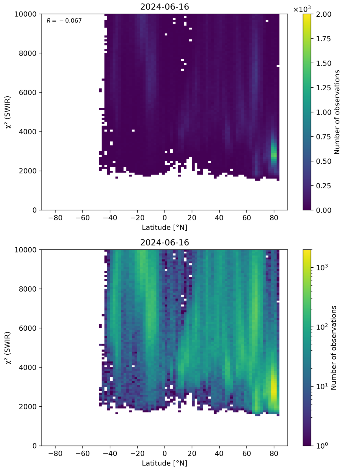
Figure 54: Scatter density plot of “Latitude” against “ \chi^2 (SWIR)” for 2024-06-15 to 2024-06-17.
