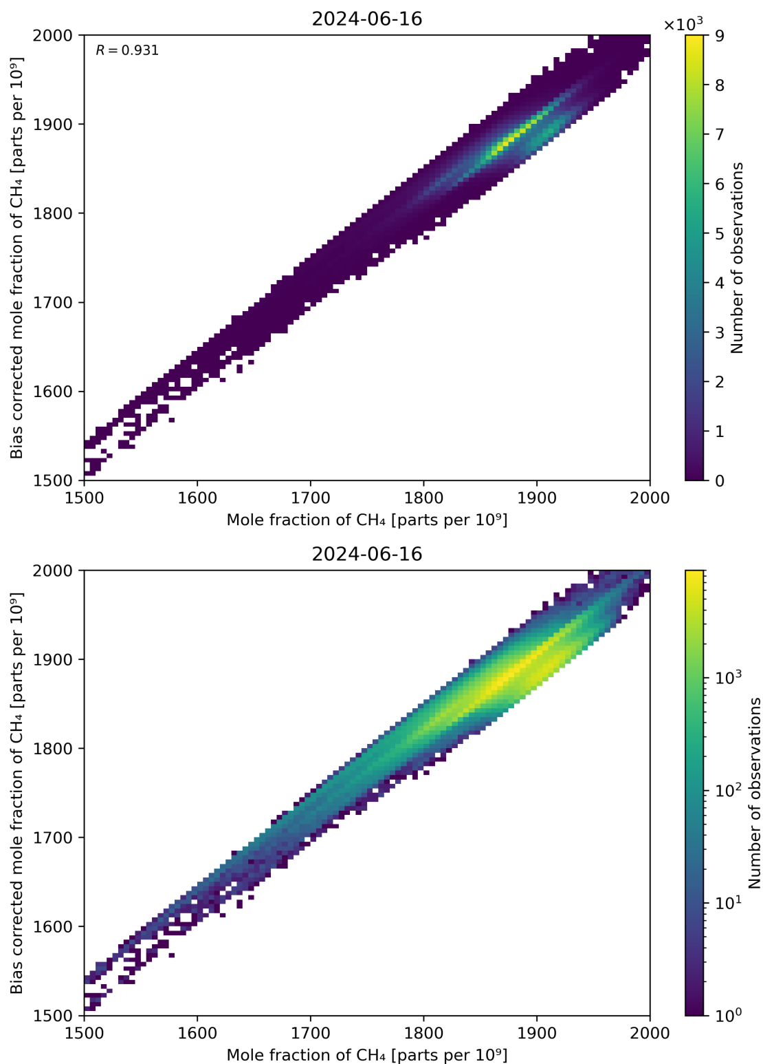
Figure 74: Scatter density plot of “Mole fraction of CH 4 ” against “Bias corrected mole fraction of CH 4 ” for 2024-06-15 to 2024-06-17.
