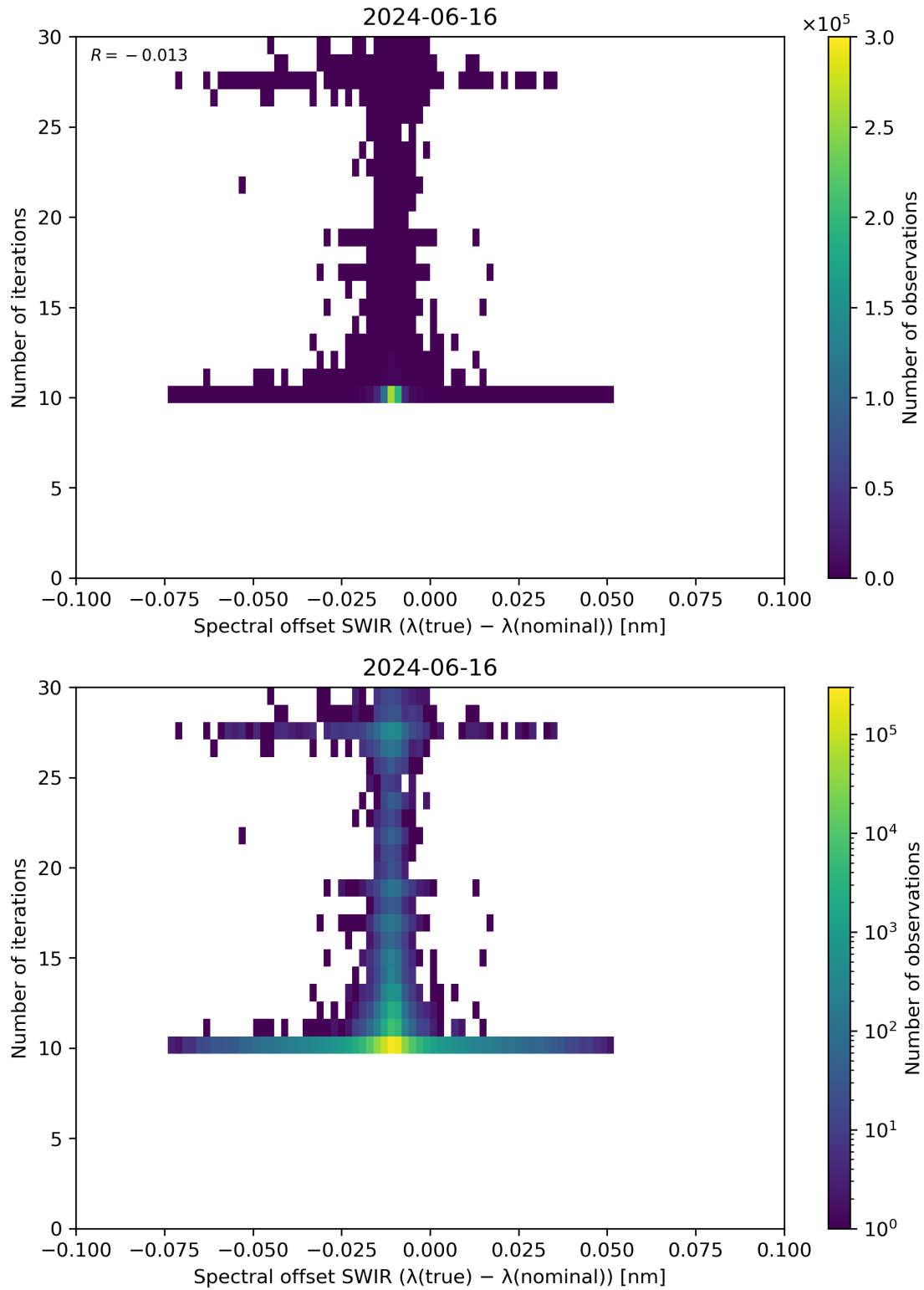
Figure 121: Scatter density plot of “Spectral offset SWIR ( \lambda(\text{true}) - \lambda(\text{nominal}) )” against “Number of iterations” for 2024-06-15 to 2024-06-17.
