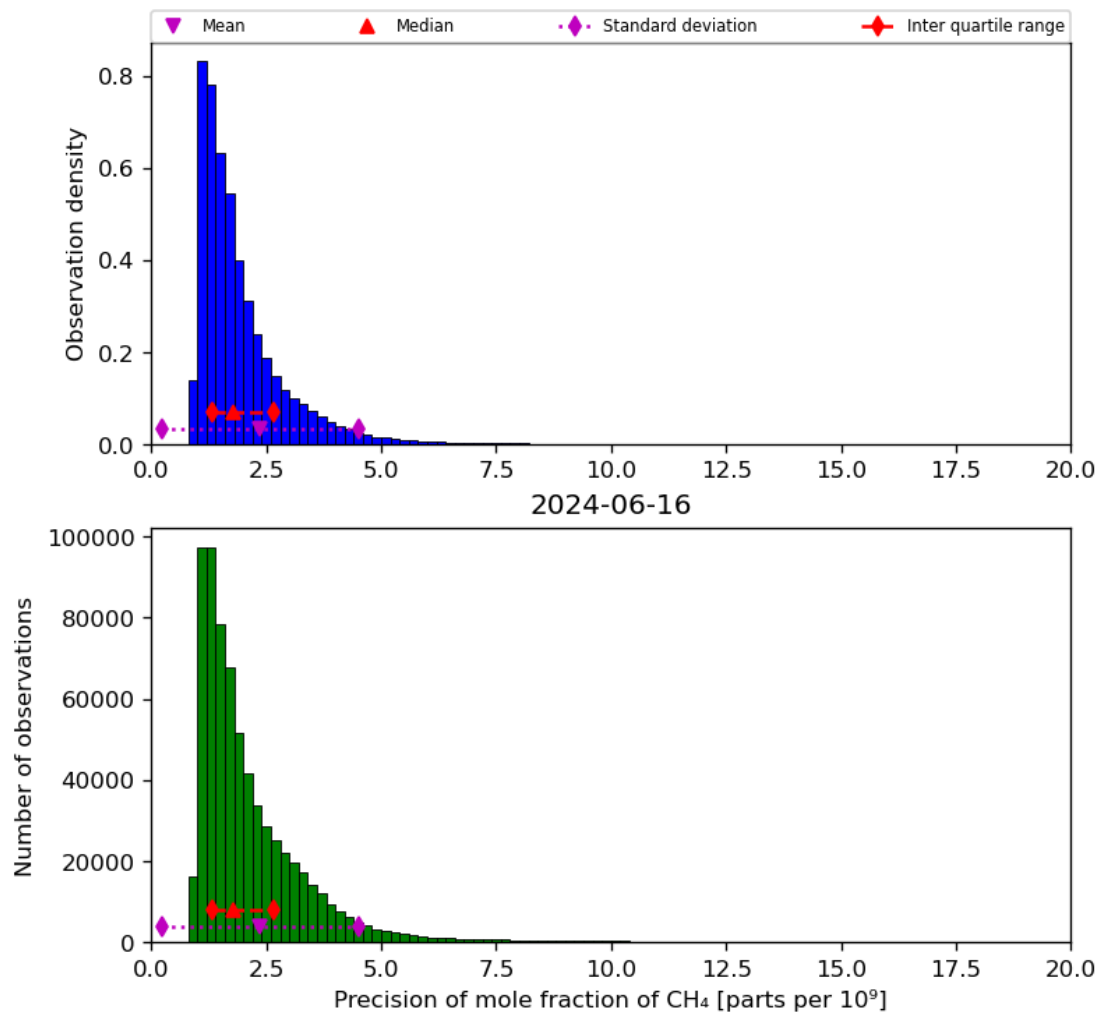
Figure 24: Histogram of “Precision of mole fraction of CH 4 ” for 2024-06-15 to 2024-06-17
