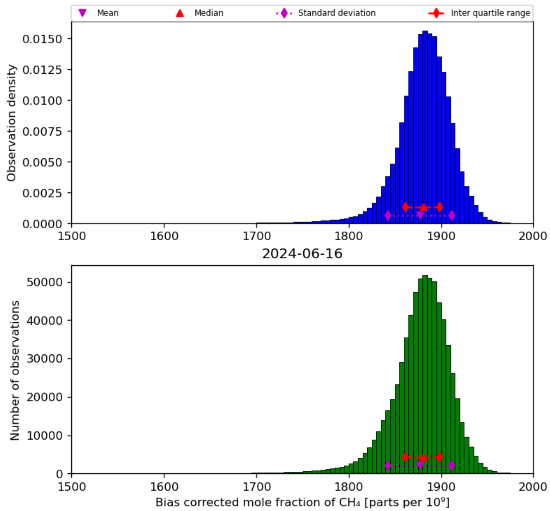
Figure 25: Histogram of “Bias corrected mole fraction of CH 4 ” for 2024-06-15 to 2024-06-17
