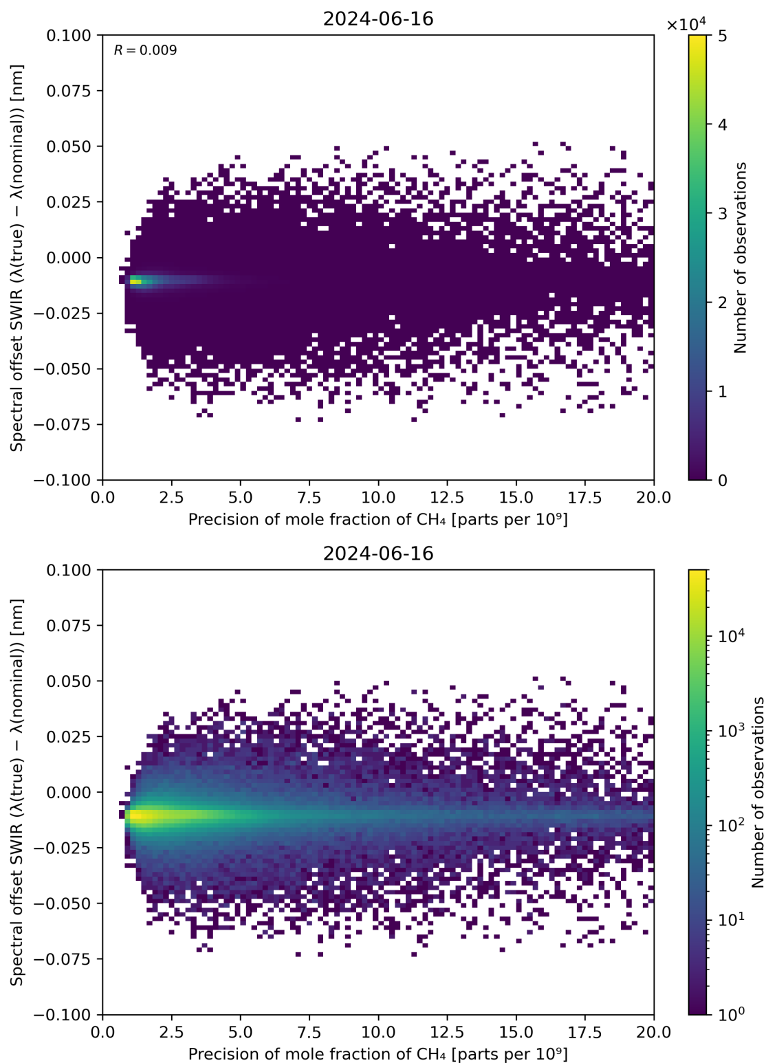
Figure 85: Scatter density plot of “Precision of mole fraction of CH 4 ” against “Spectral offset SWIR ( \lambda(\text{true}) - \lambda(\text{nominal}) )” for 2024-06-15 to 2024-06-17.
