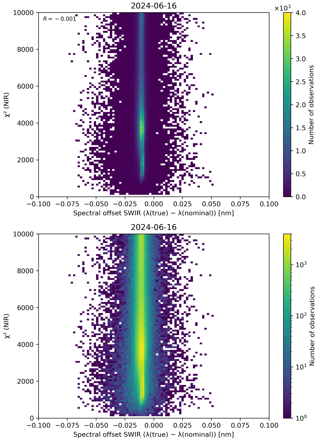
Figure 117: Scatter density plot of “Spectral offset SWIR ( \lambda(\text{true}) - \lambda(\text{nominal}) )” against “ \chi^2 (NIR)” for 2024-06-15 to 2024-06-17.
