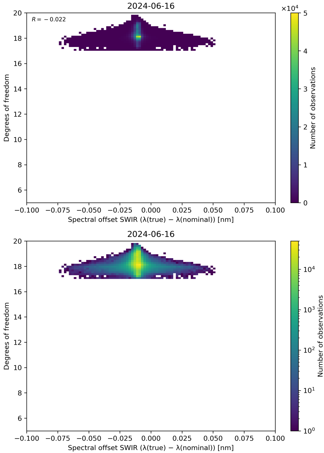
Figure 119: Scatter density plot of “Spectral offset SWIR ( \lambda(\text{true}) - \lambda(\text{nominal}) )” against “Degrees of freedom” for 2024-06-15 to 2024-06-17.
