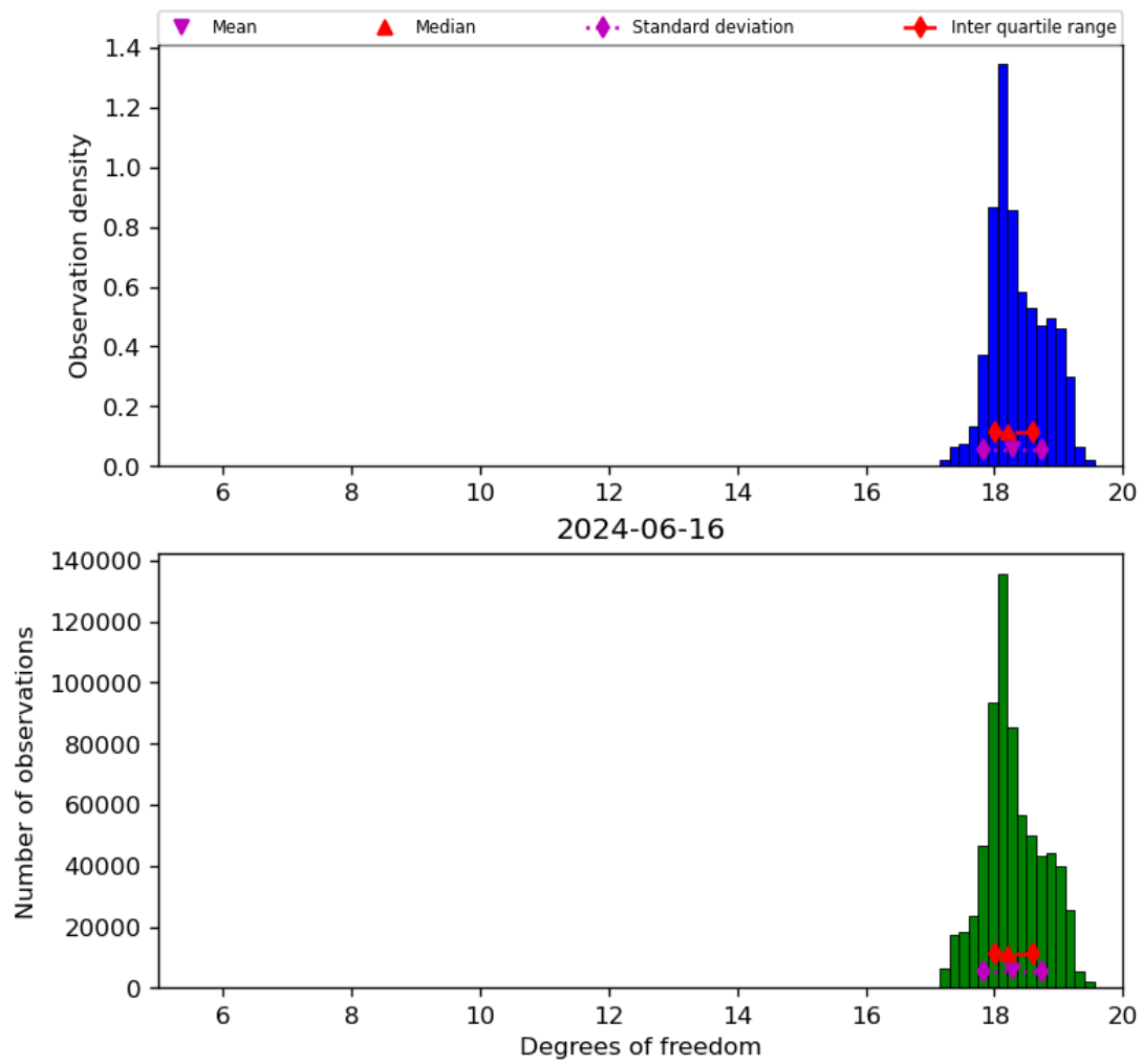
Figure 30: Histogram of “Degrees of freedom” for 2024-06-15 to 2024-06-17
