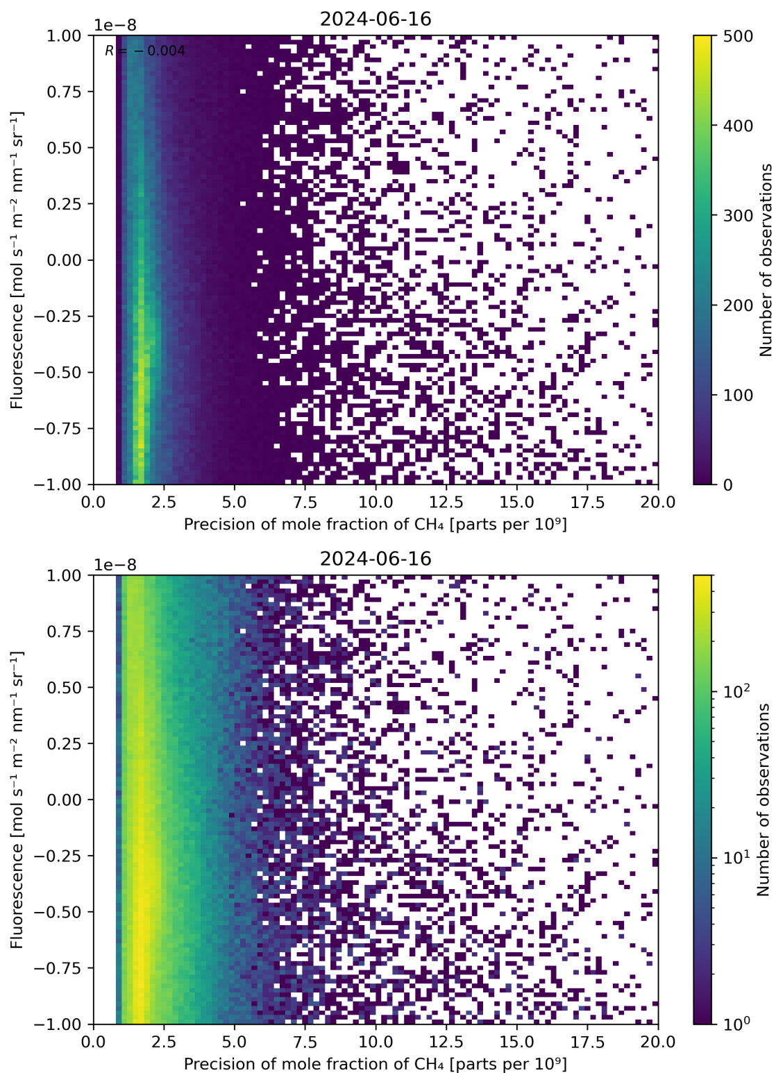
Figure 81: Scatter density plot of “Precision of mole fraction of \text{CH}_4 ” against “Fluorescence” for 2024-06-15 to 2024-06-17.
