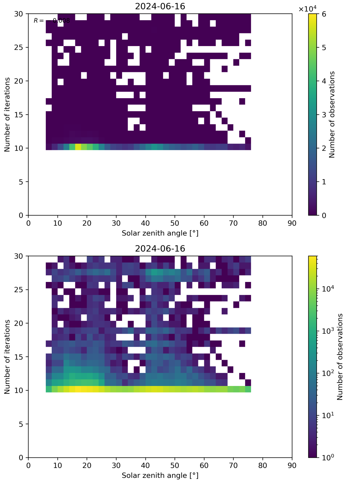
Figure 102: Scatter density plot of “Solar zenith angle” against “Number of iterations” for 2024-06-15 to 2024-06-17.
