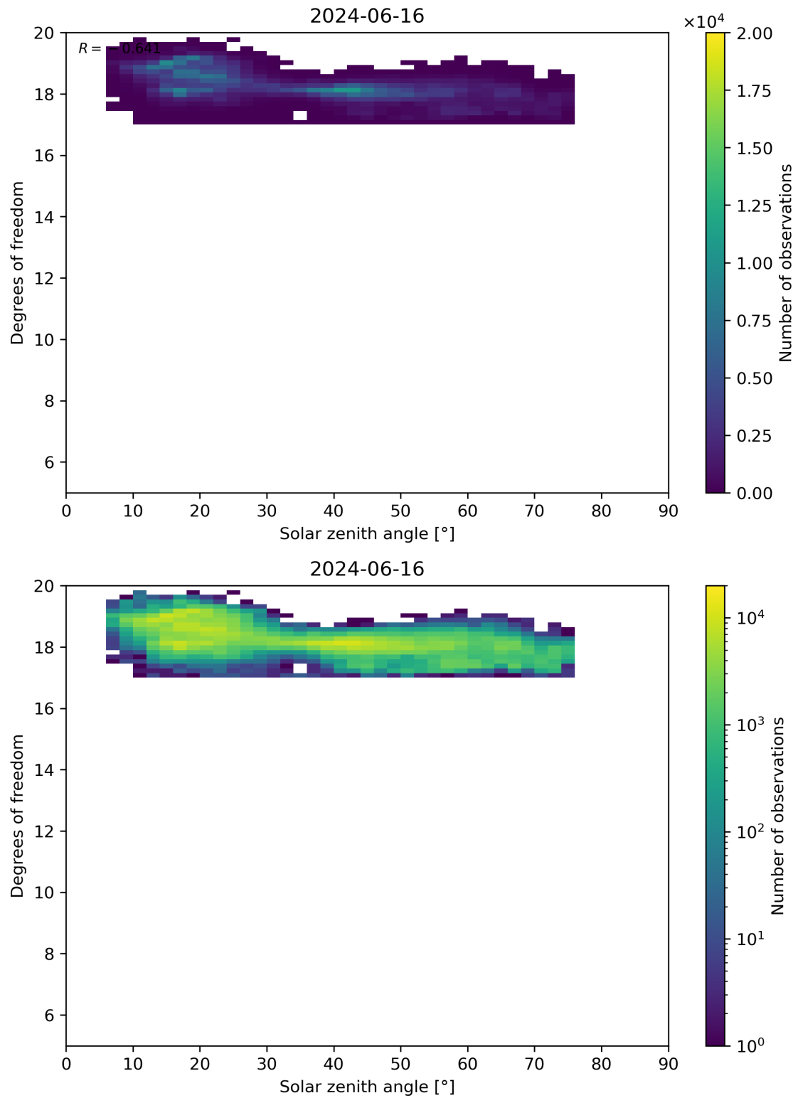
Figure 96: Scatter density plot of “Solar zenith angle” against “Degrees of freedom” for 2024-06-15 to 2024-06-17.
