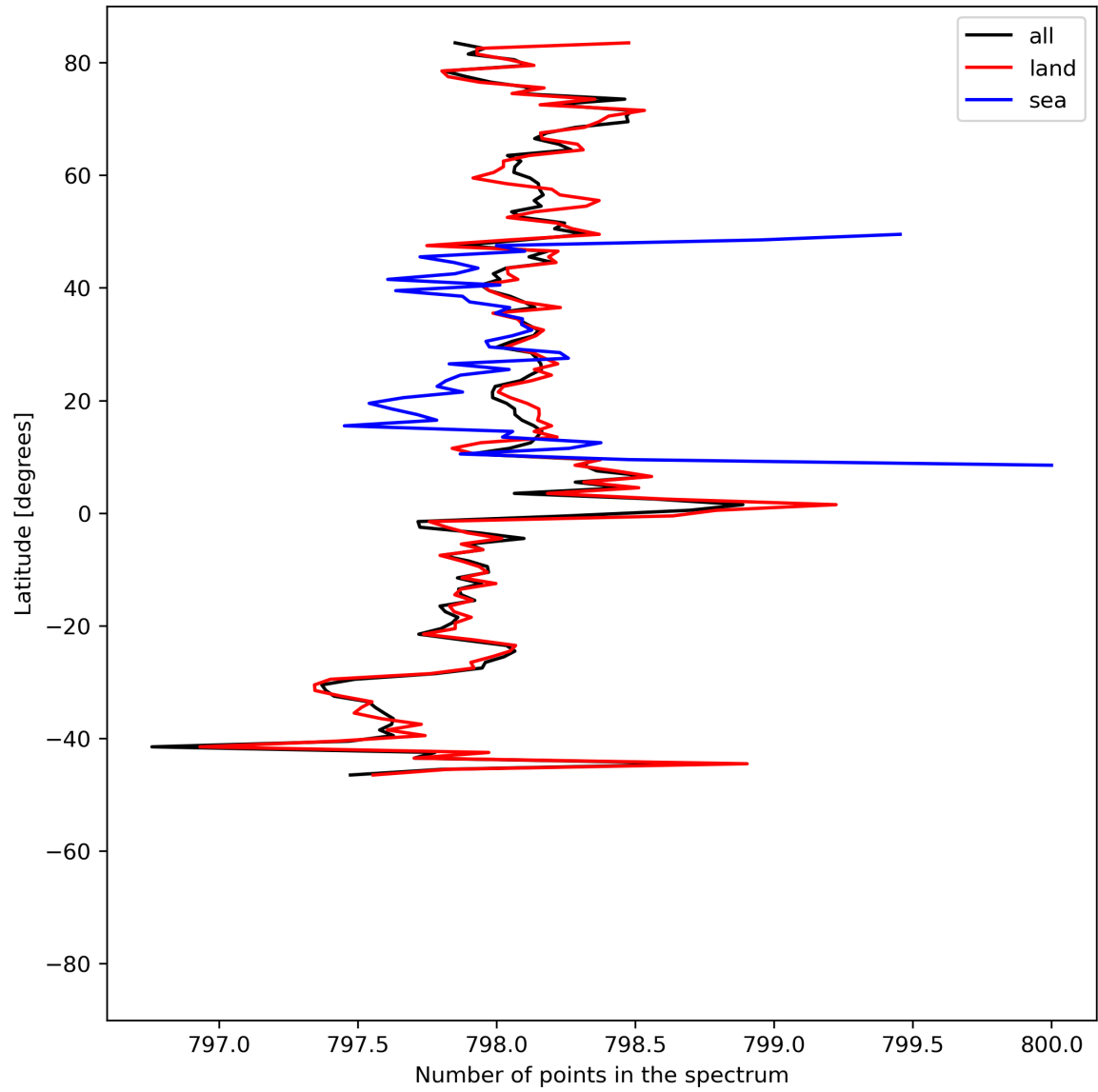
Figure 15: Zonal average of “Number of points in the spectrum” for 2024-06-15 to 2024-06-17.
