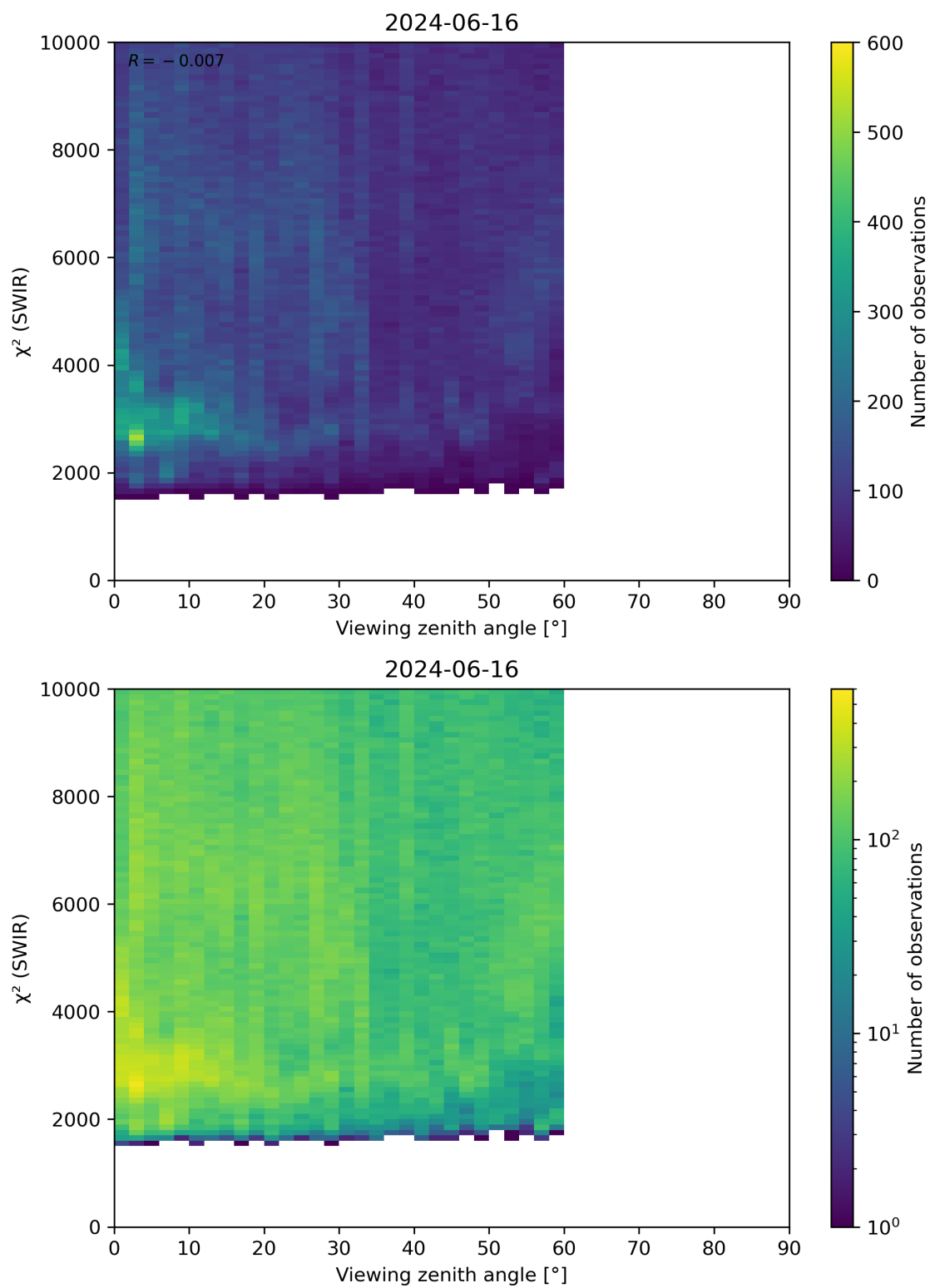
Figure 106: Scatter density plot of “Viewing zenith angle” against “ \chi^2 (SWIR)” for 2024-06-15 to 2024-06-17.
