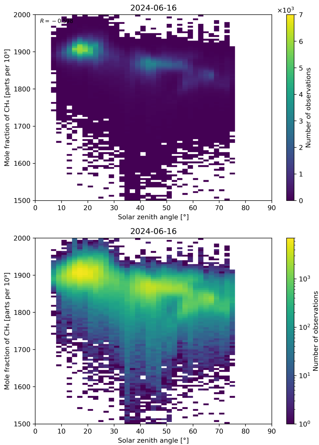
Figure 99: Scatter density plot of “Solar zenith angle” against “Mole fraction of \text{CH}_4 ” for 2024-06-15 to 2024-06-17.
