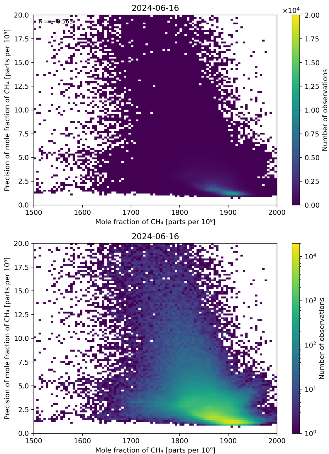
Figure 75: Scatter density plot of “Mole fraction of CH 4 ” against “Precision of mole fraction of CH 4 ” for 2024-06-15 to 2024-06-17.
