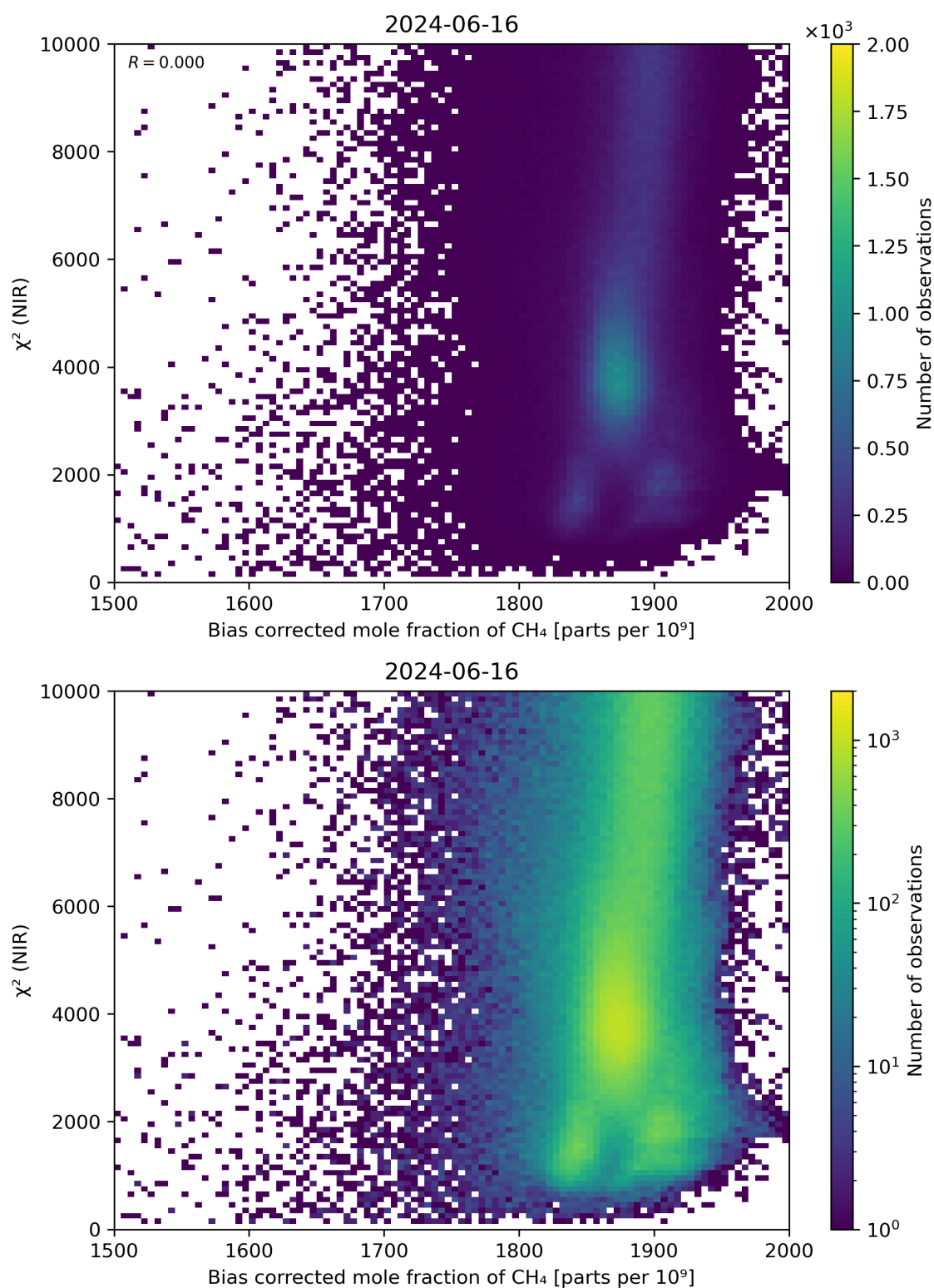
Figure 63: Scatter density plot of “Bias corrected mole fraction of \text{CH}_4 ” against “ \chi^2 (NIR)” for 2024-06-15 to 2024-06-17.
