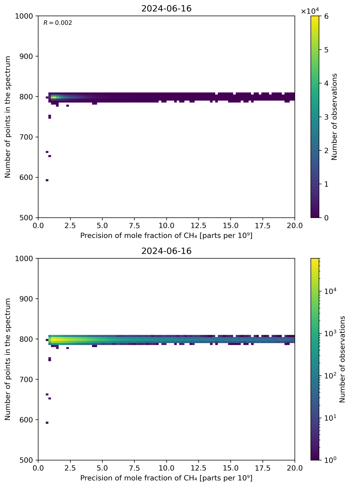
Figure 84: Scatter density plot of “Precision of mole fraction of CH 4 ” against “Number of points in the spectrum” for 2024-06-15 to 2024-06-17.
