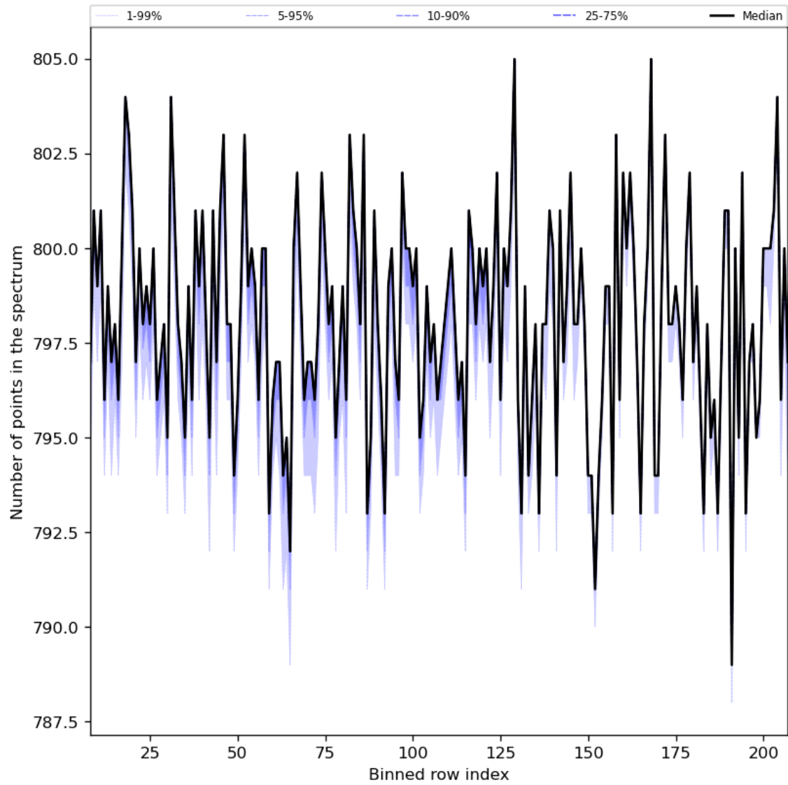
Figure 37: Along track statistics of “Number of points in the spectrum” for 2024-06-15 to 2024-06-17
