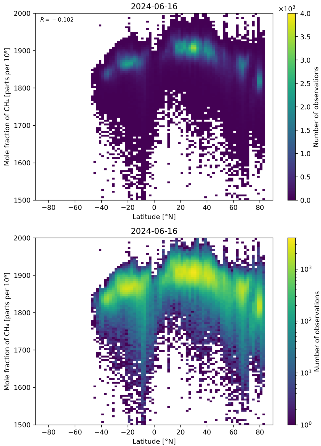
Figure 57: Scatter density plot of “Latitude” against “Mole fraction of CH 4 ” for 2024-06-15 to 2024-06-17.
