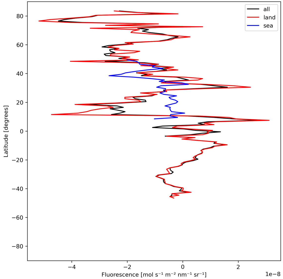
Figure 21: Zonal average of “Fluorescence” for 2024-06-15 to 2024-06-17.
