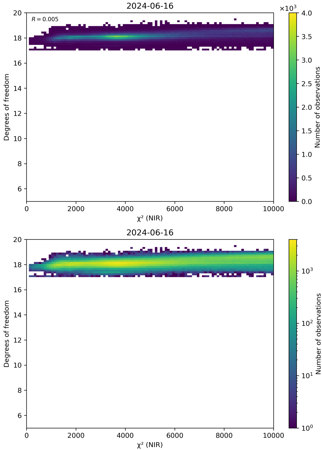
Figure 44: Scatter density plot of “ \chi^2 (NIR)” against “Degrees of freedom” for 2024-06-15 to 2024-06-17.
