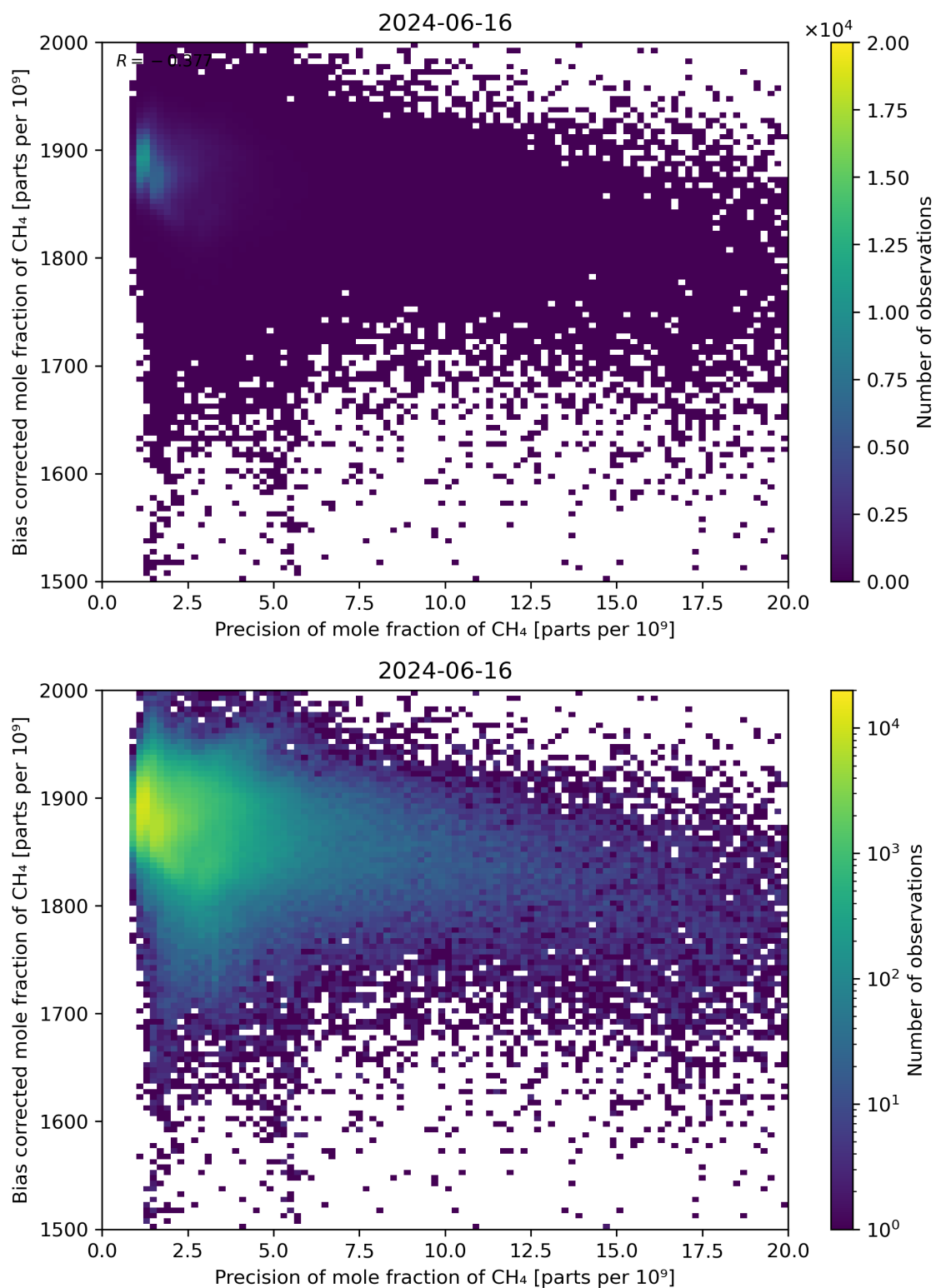
Figure 82: Scatter density plot of “Precision of mole fraction of CH 4 ” against “Bias corrected mole fraction of CH 4 ” for 2024-06-15 to 2024-06-17.
