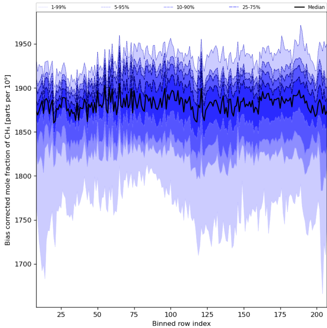
Figure 36: Along track statistics of “Bias corrected mole fraction of CH 4 ” for 2024-06-15 to 2024-06-17
