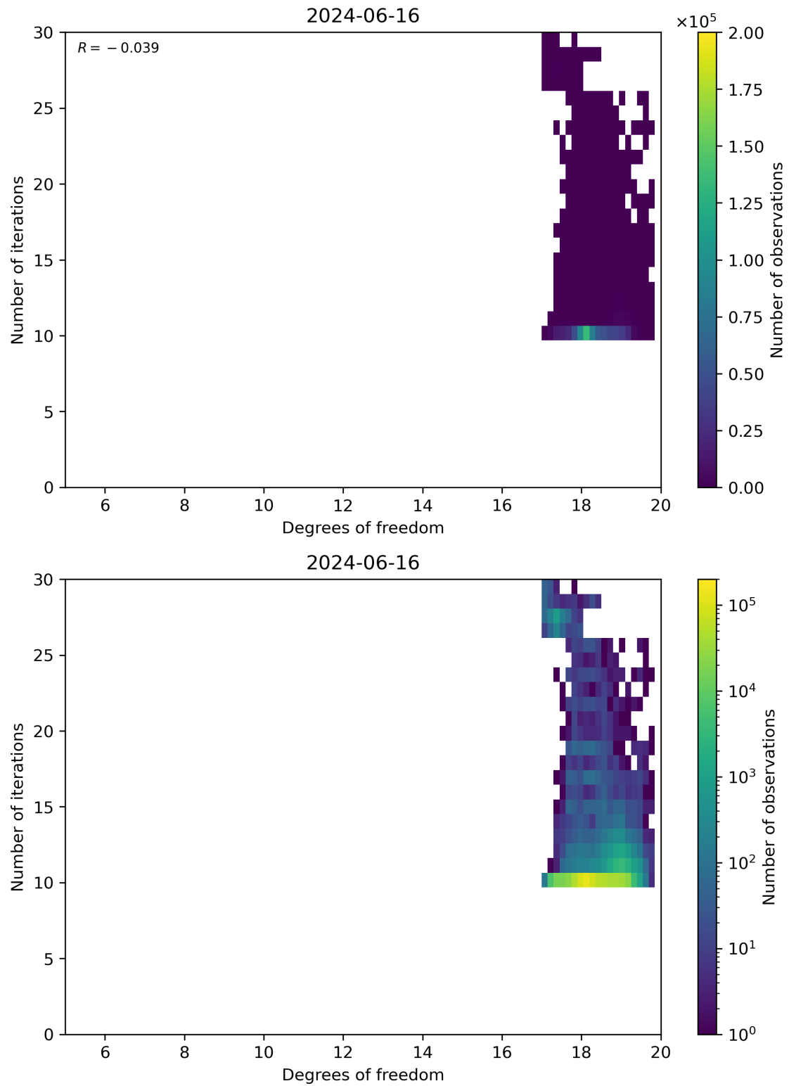
Figure 52: Scatter density plot of “Degrees of freedom” against “Number of iterations” for 2024-06-15 to 2024-06-17.
