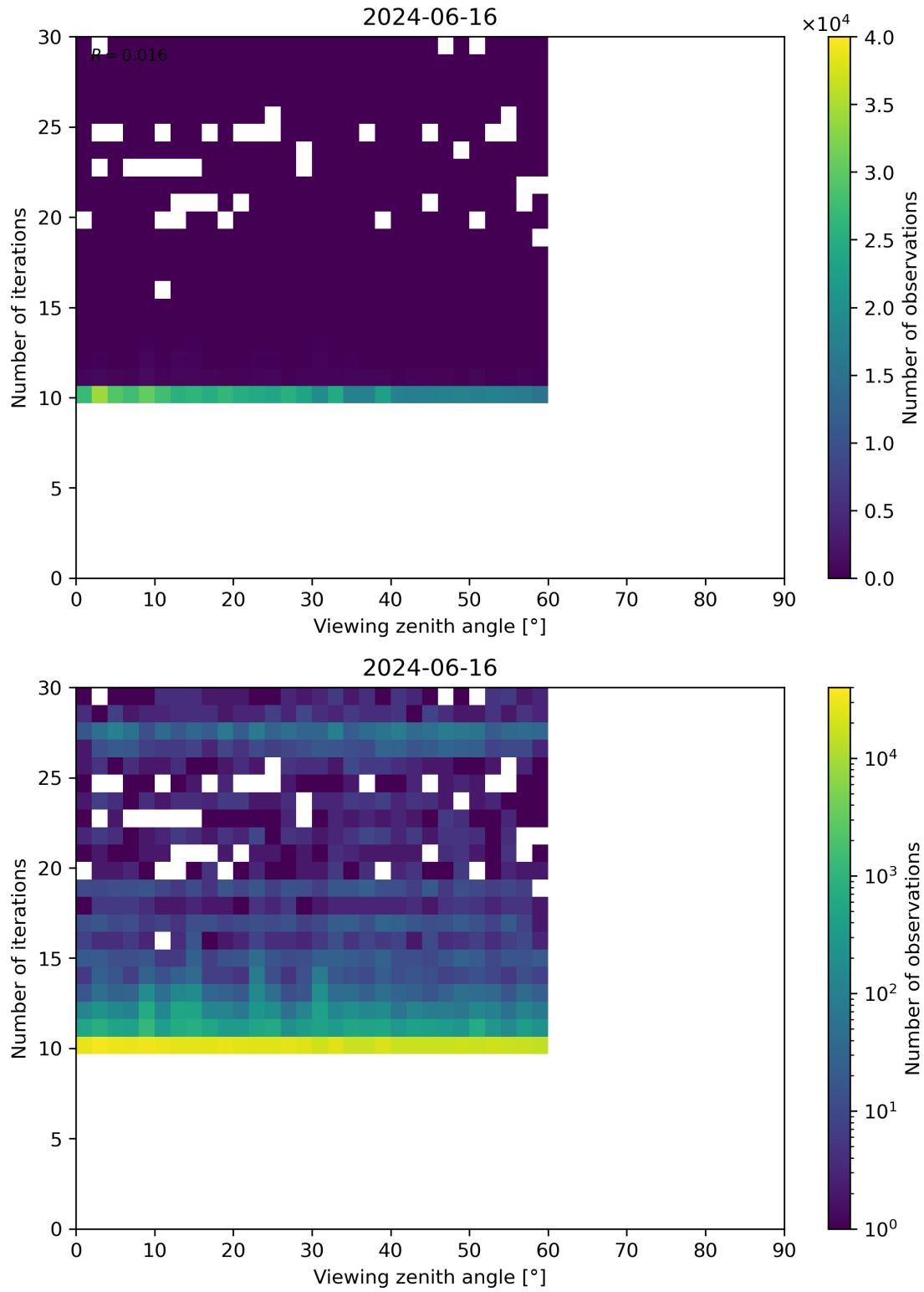
Figure 113: Scatter density plot of “Viewing zenith angle” against “Number of iterations” for 2024-06-15 to 2024-06-17.
