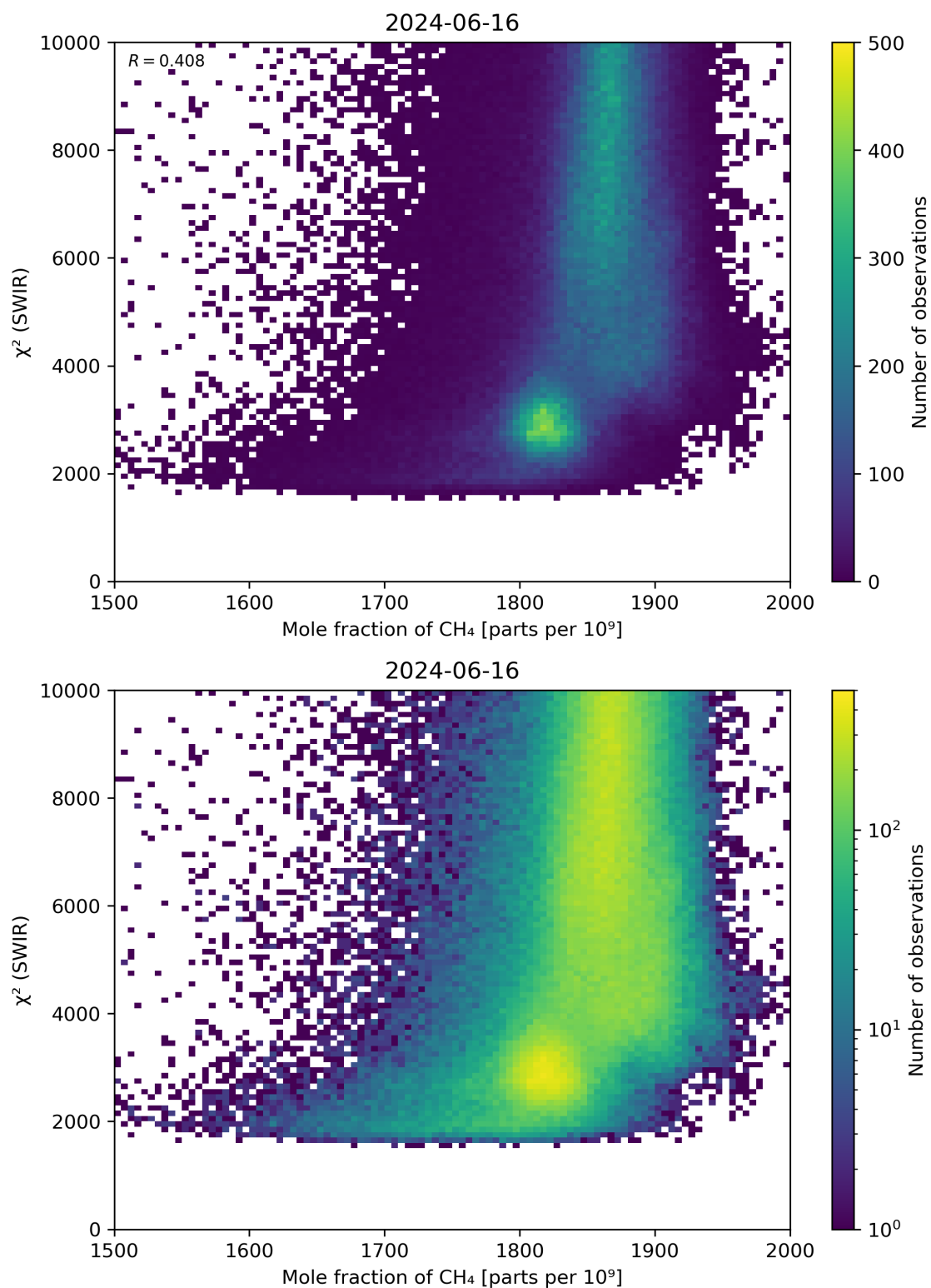
Figure 71: Scatter density plot of “Mole fraction of \text{CH}_4 ” against “ \chi^2 (SWIR)” for 2024-06-15 to 2024-06-17.
