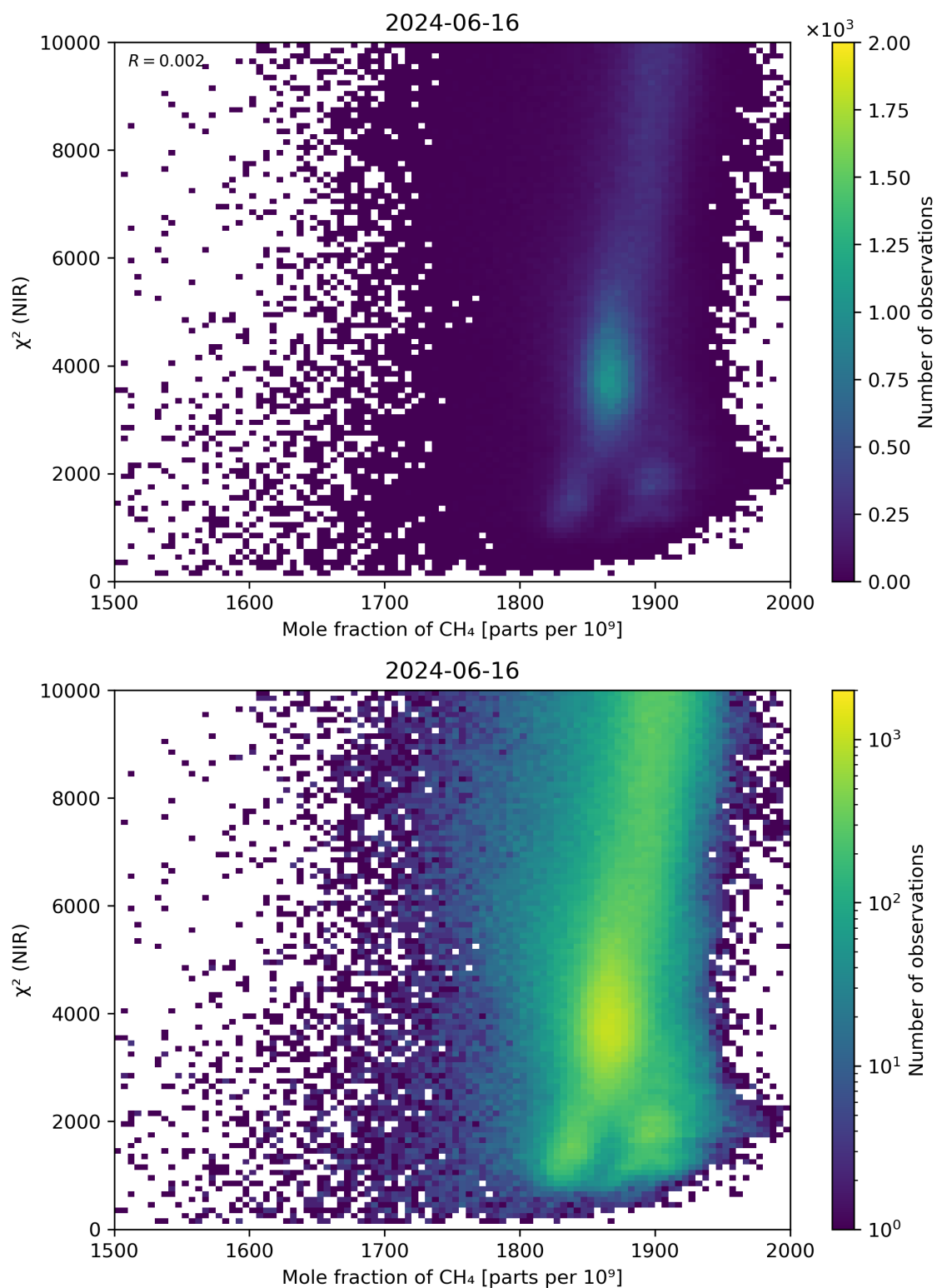
Figure 70: Scatter density plot of “Mole fraction of \text{CH}_4 ” against “ \chi^2 (NIR)” for 2024-06-15 to 2024-06-17.
