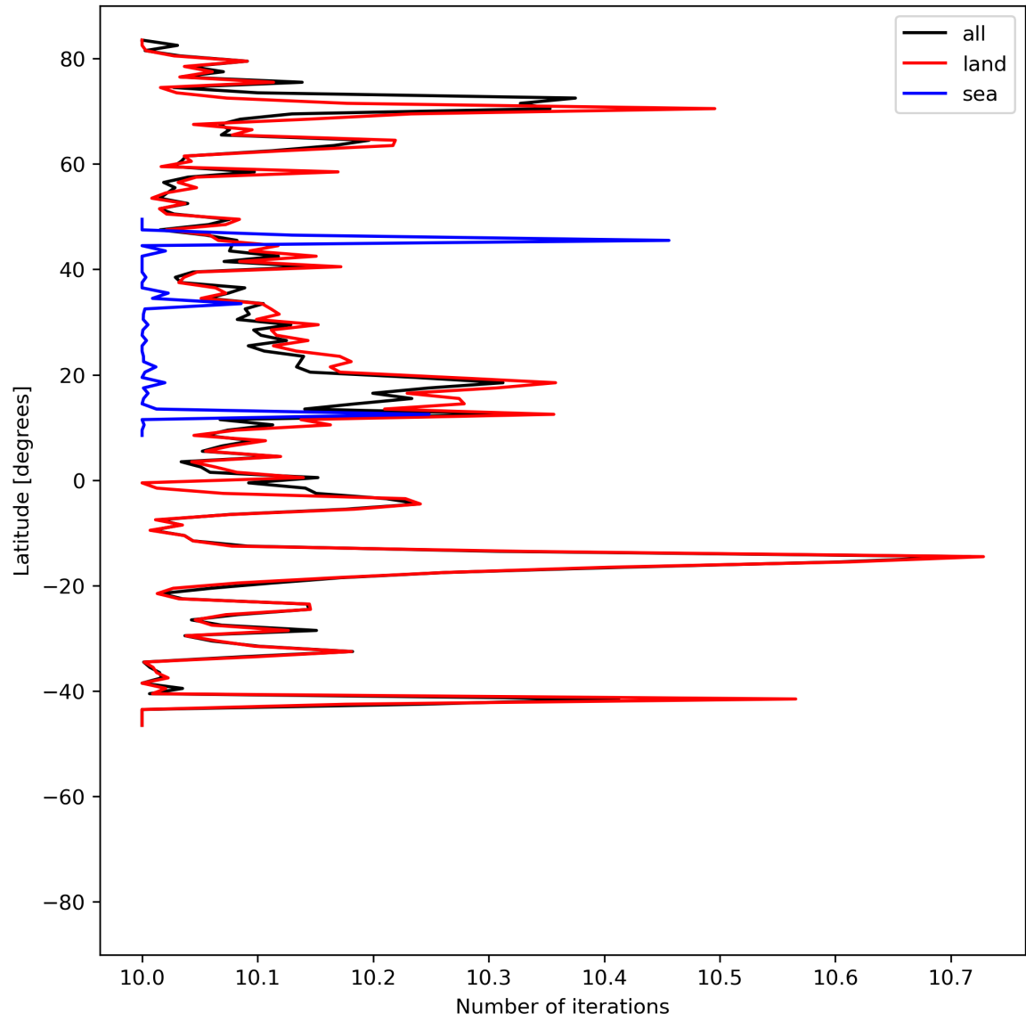
Figure 20: Zonal average of “Number of iterations” for 2024-06-15 to 2024-06-17.
