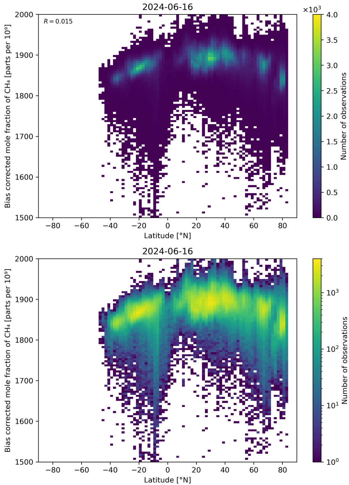
Figure 58: Scatter density plot of “Latitude” against “Bias corrected mole fraction of CH 4 ” for 2024-06-15 to 2024-06-17.
