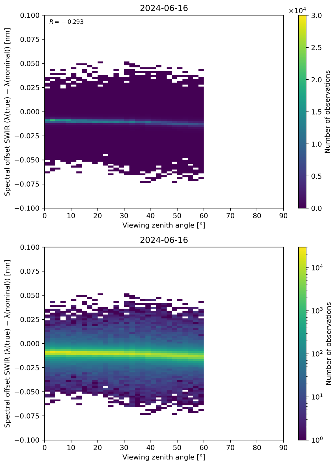
Figure 116: Scatter density plot of “Viewing zenith angle” against “Spectral offset SWIR ( \lambda(\text{true}) - \lambda(\text{nominal}) )” for 2024-06-15 to 2024-06-17.
