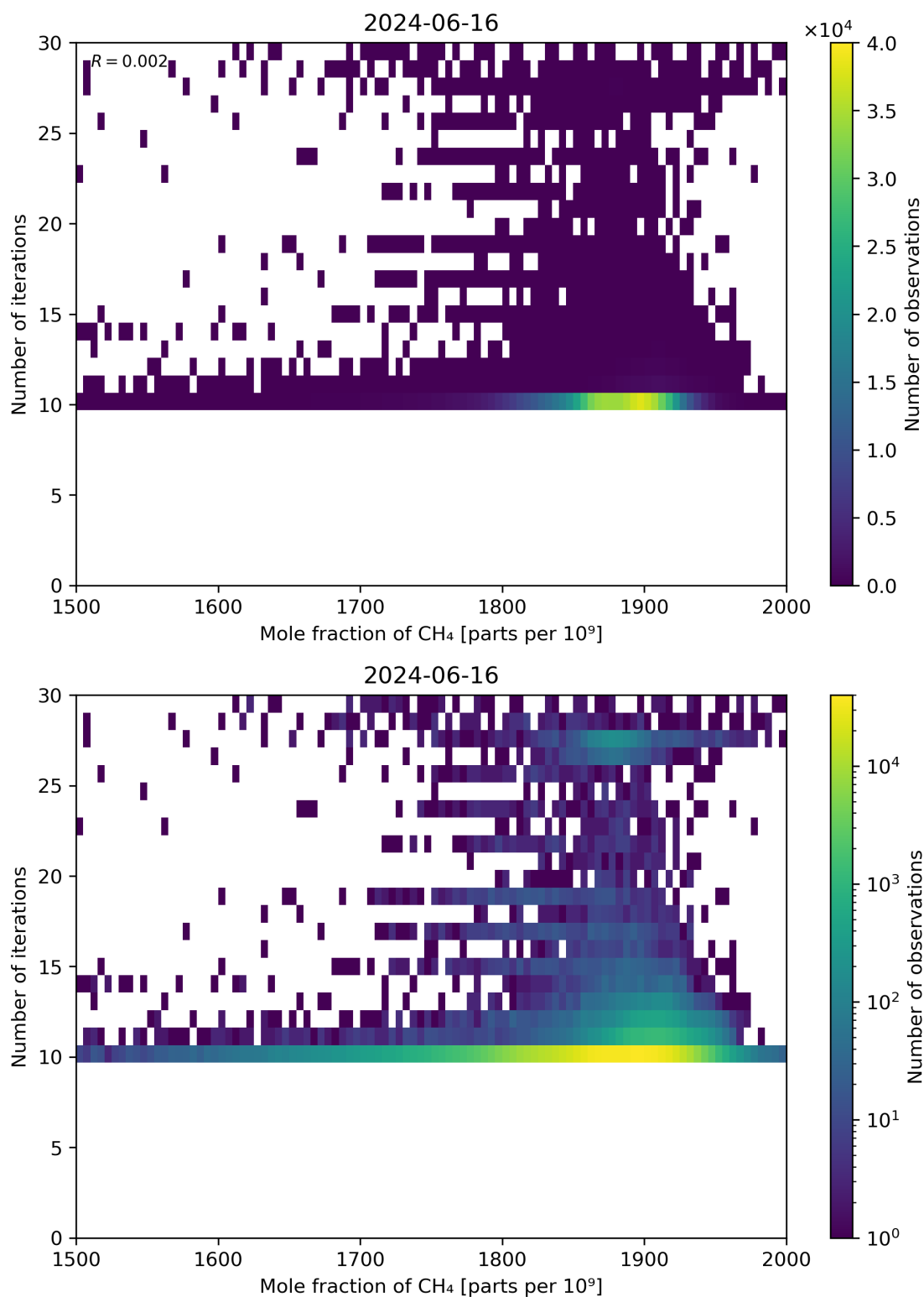
Figure 76: Scatter density plot of “Mole fraction of CH 4 ” against “Number of iterations” for 2024-06-15 to 2024-06-17.
