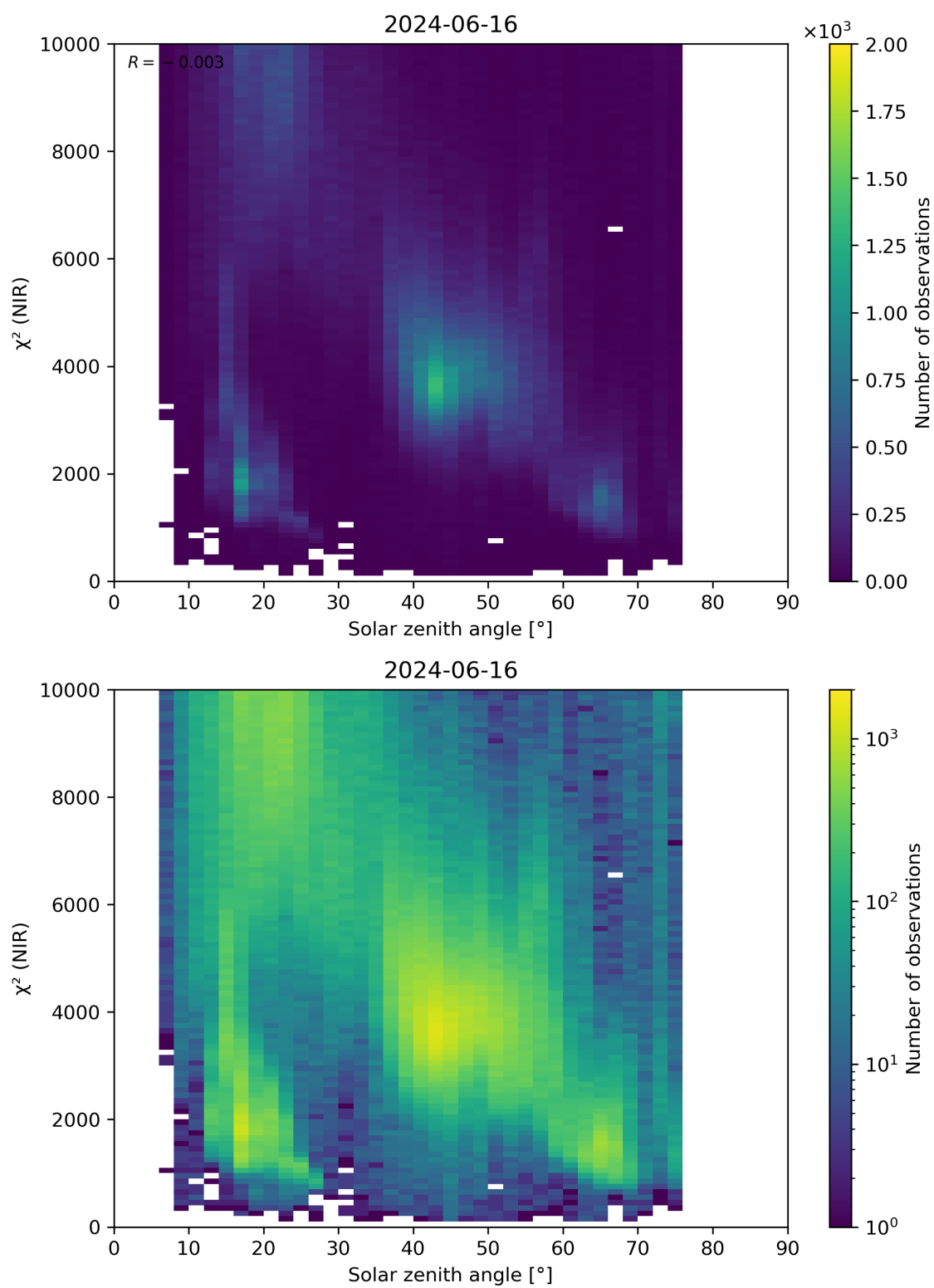
Figure 94: Scatter density plot of “Solar zenith angle” against “ \chi^2 (NIR)” for 2024-06-15 to 2024-06-17.
