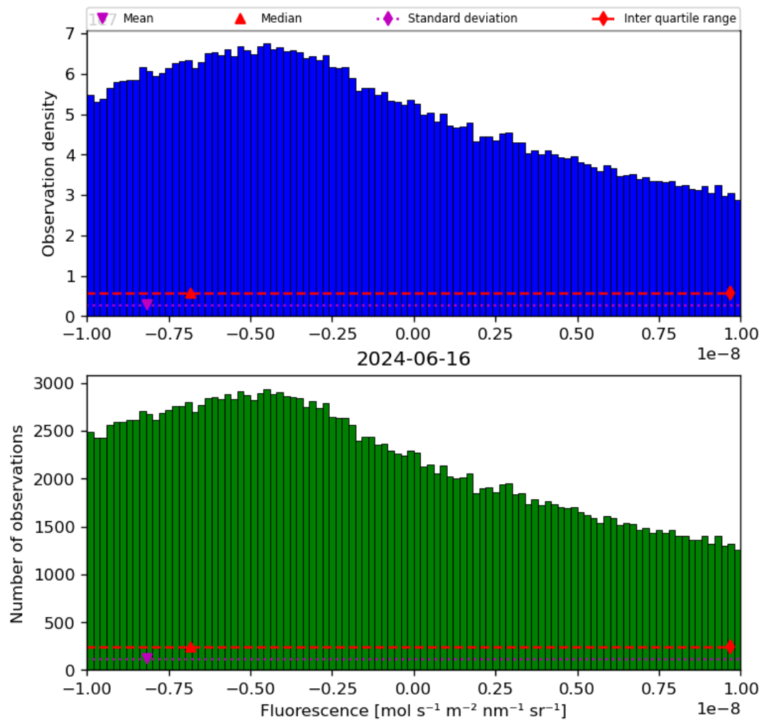
Figure 32: Histogram of “Fluorescence” for 2024-06-15 to 2024-06-17
