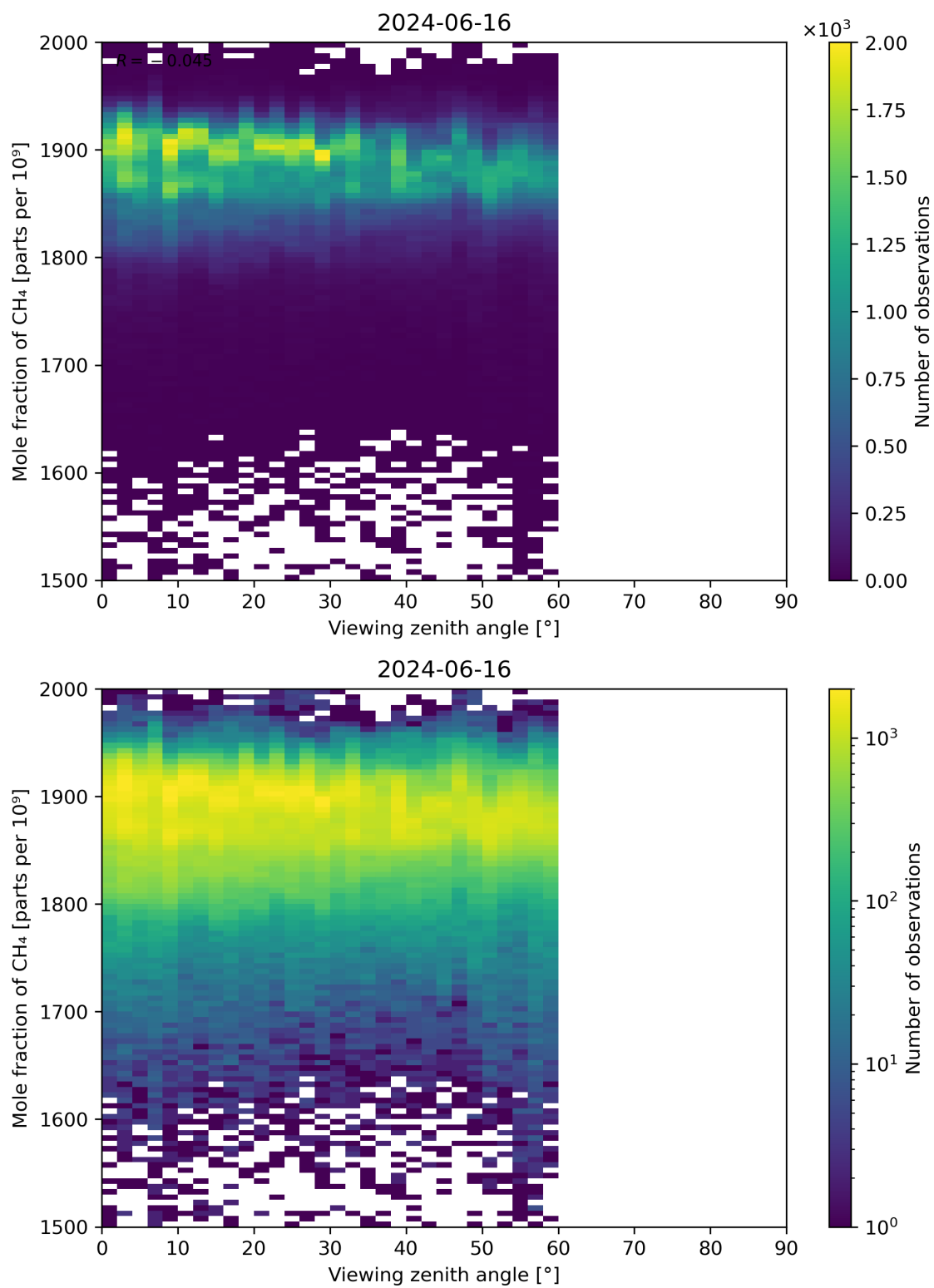
Figure 110: Scatter density plot of “Viewing zenith angle” against “Mole fraction of CH 4 ” for 2024-06-15 to 2024-06-17.
