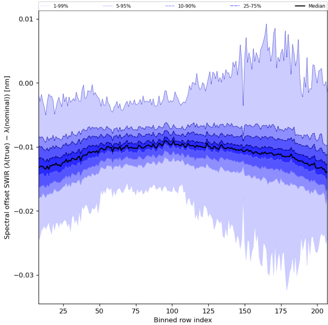
Figure 38: Along track statistics of “Spectral offset SWIR ( \lambda(\text{true}) - \lambda(\text{nominal}) )” for 2024-06-15 to 2024-06-17
