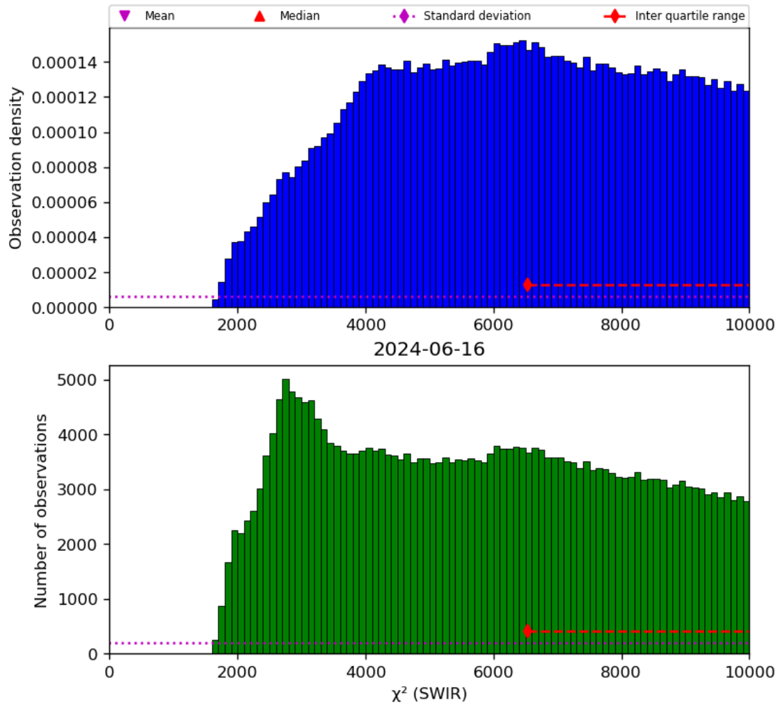
Figure 28: Histogram of “ \chi^2 (SWIR)” for 2024-06-15 to 2024-06-17
