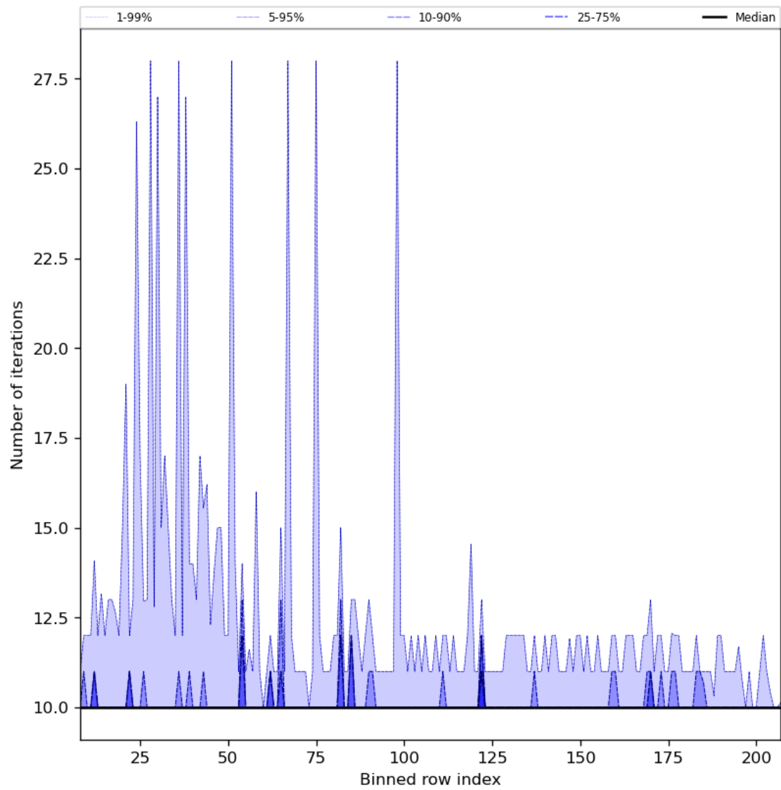
Figure 42: Along track statistics of “Number of iterations” for 2024-06-15 to 2024-06-17
