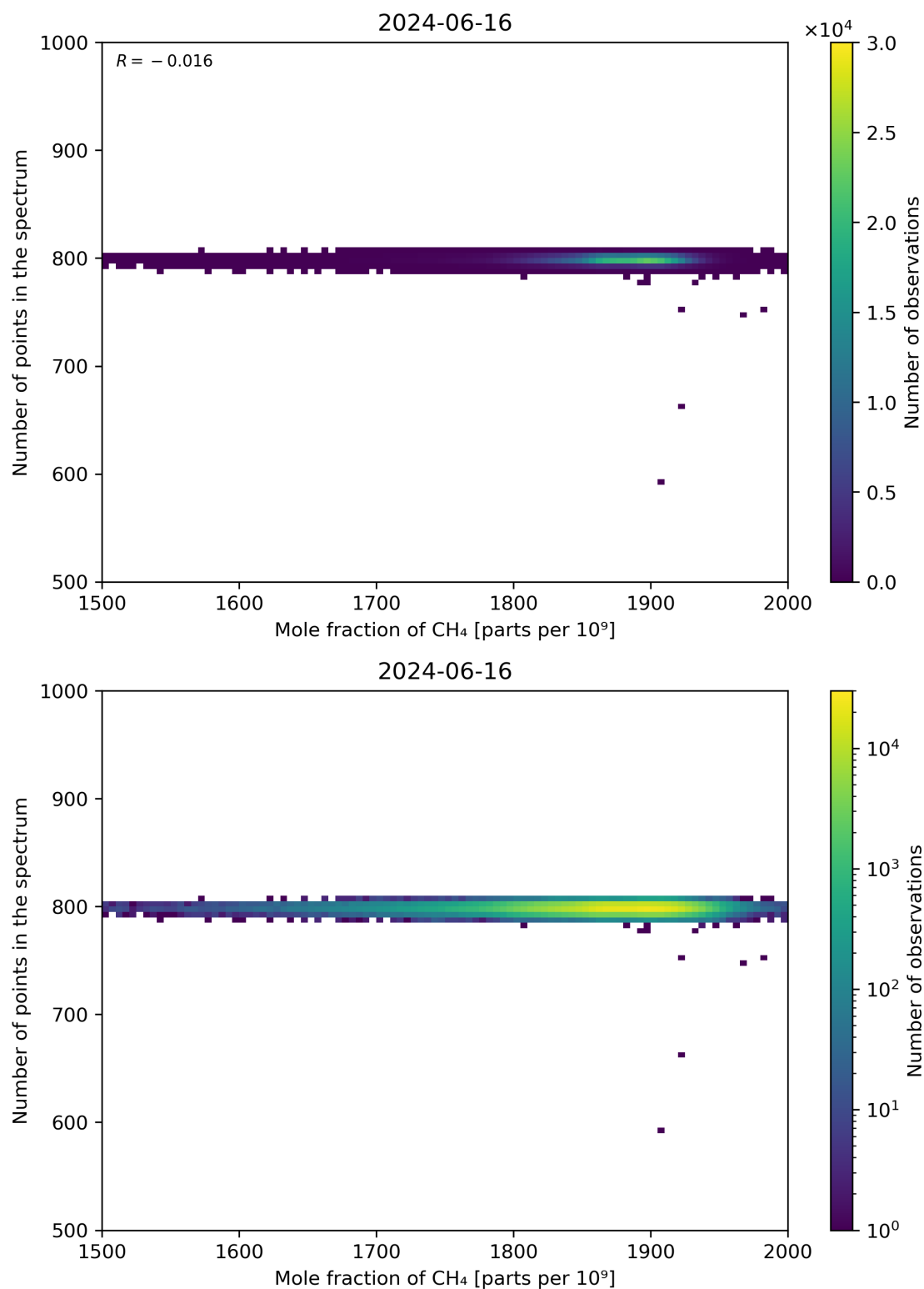
Figure 77: Scatter density plot of “Mole fraction of CH 4 ” against “Number of points in the spectrum” for 2024-06-15 to 2024-06-17.
