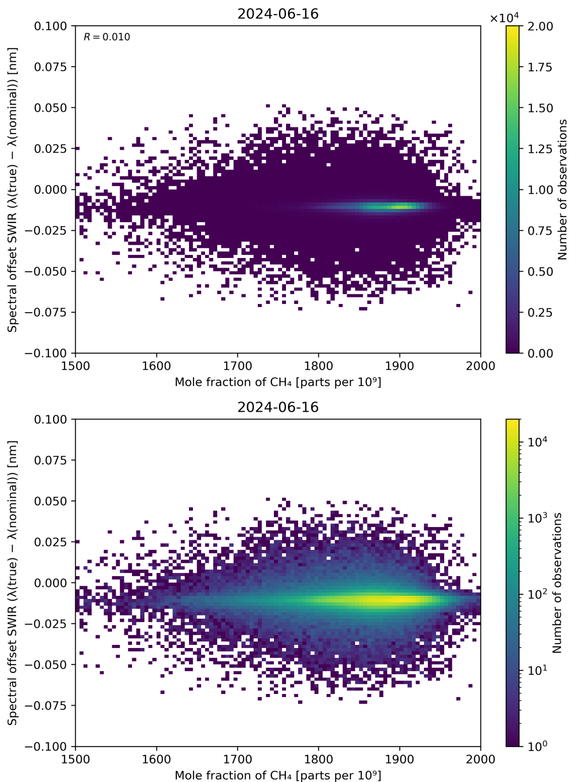
Figure 86: Scatter density plot of “Mole fraction of CH 4 ” against “Spectral offset SWIR ( \lambda(\text{true}) - \lambda(\text{nominal}) )” for 2024-06-15 to 2024-06-17.
