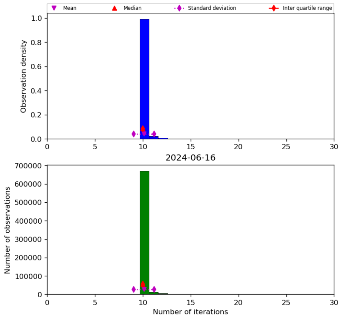
Figure 31: Histogram of “Number of iterations” for 2024-06-15 to 2024-06-17
