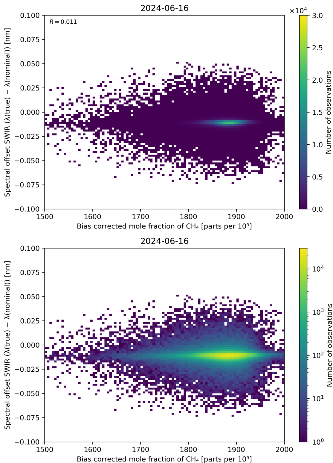
Figure 69: Scatter density plot of “Bias corrected mole fraction of \text{CH}_4 ” against “Spectral offset SWIR ( \lambda(\text{true}) - \lambda(\text{nominal}) )” for 2024-06-15 to 2024-06-17.
