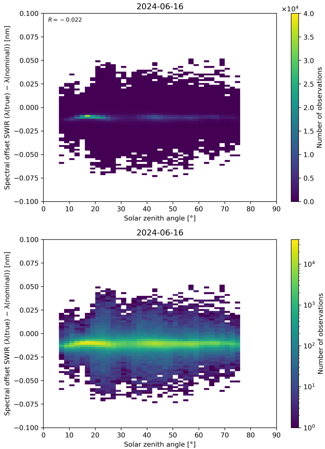
Figure 104: Scatter density plot of “Solar zenith angle” against “Spectral offset SWIR ( \lambda(\text{true}) - \lambda(\text{nominal}) )” for 2024-06-15 to 2024-06-17.
