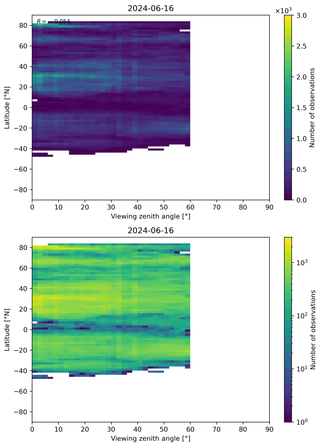
Figure 109: Scatter density plot of “Viewing zenith angle” against “Latitude” for 2024-06-15 to 2024-06-17.
