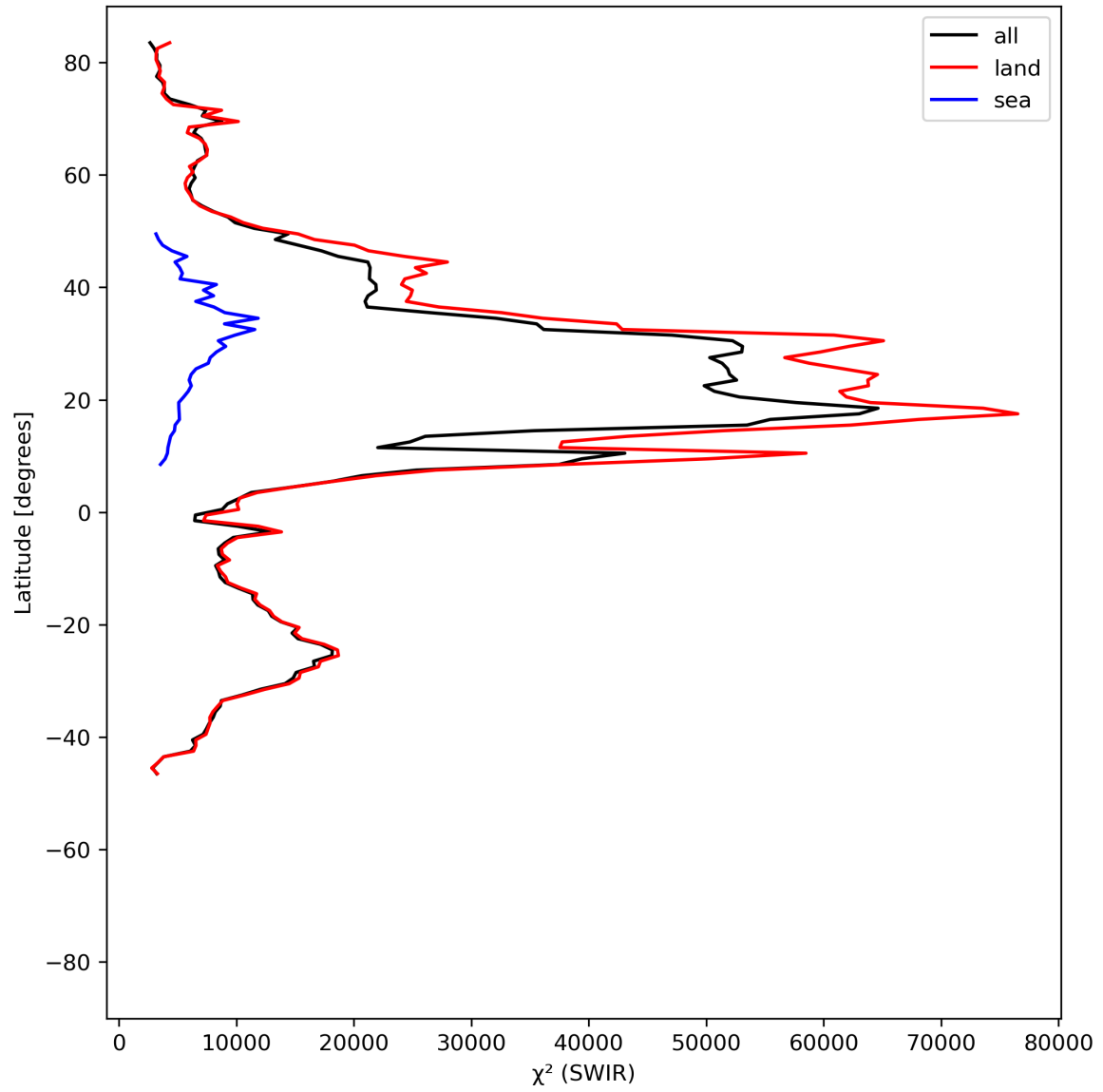
Figure 17: Zonal average of “ \chi^2 (SWIR)” for 2024-06-15 to 2024-06-17.
