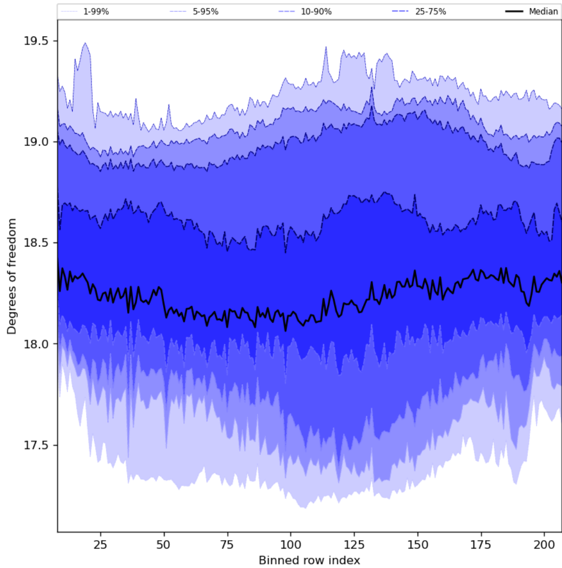
Figure 41: Along track statistics of “Degrees of freedom” for 2024-06-15 to 2024-06-17
