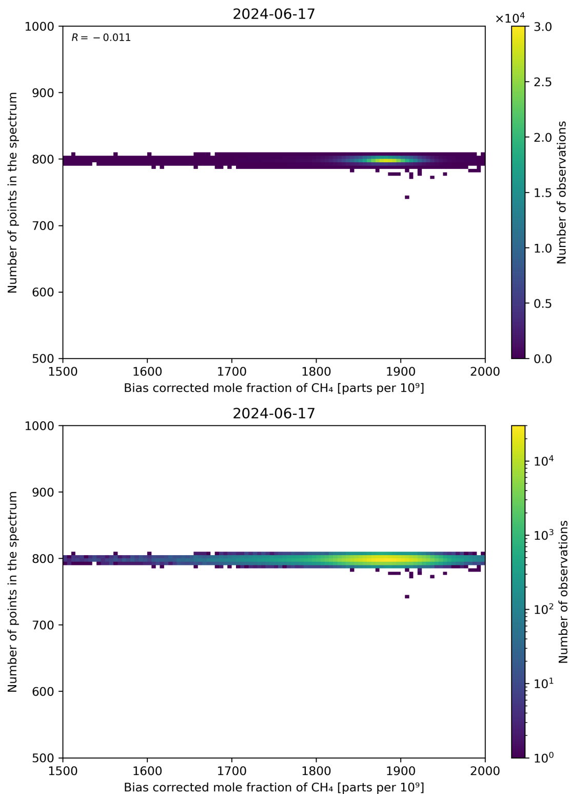
Figure 68: Scatter density plot of “Bias corrected mole fraction of CH 4 ” against “Number of points in the spectrum” for 2024-06-16 to 2024-06-18.
