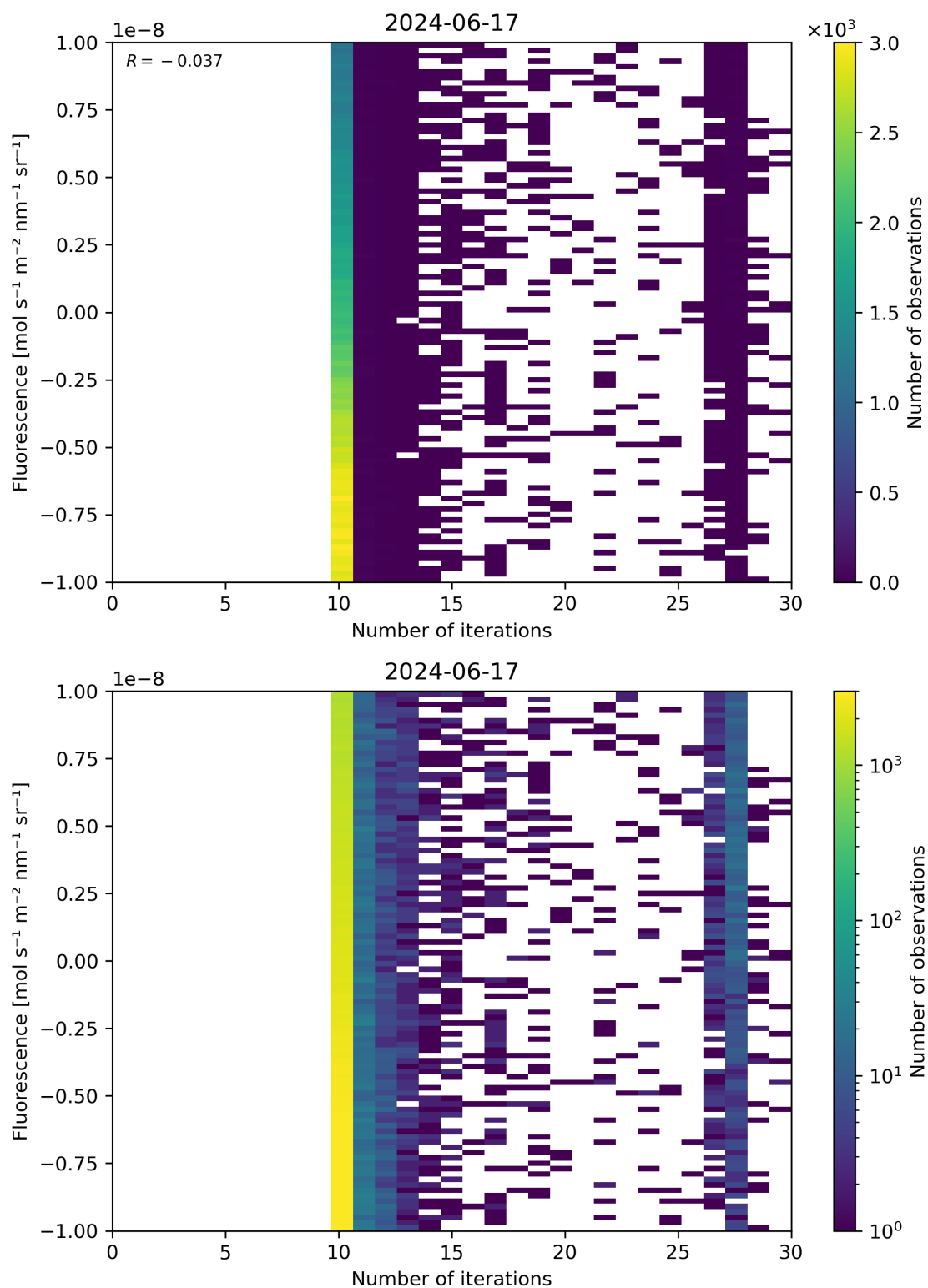
Figure 87: Scatter density plot of “Number of iterations” against “Fluorescence” for 2024-06-16 to 2024-06-18.
