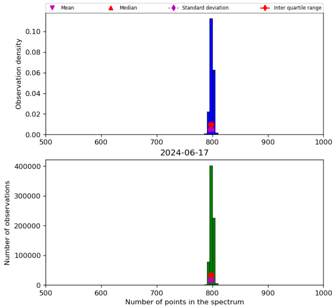
Figure 26: Histogram of “Number of points in the spectrum” for 2024-06-16 to 2024-06-18
