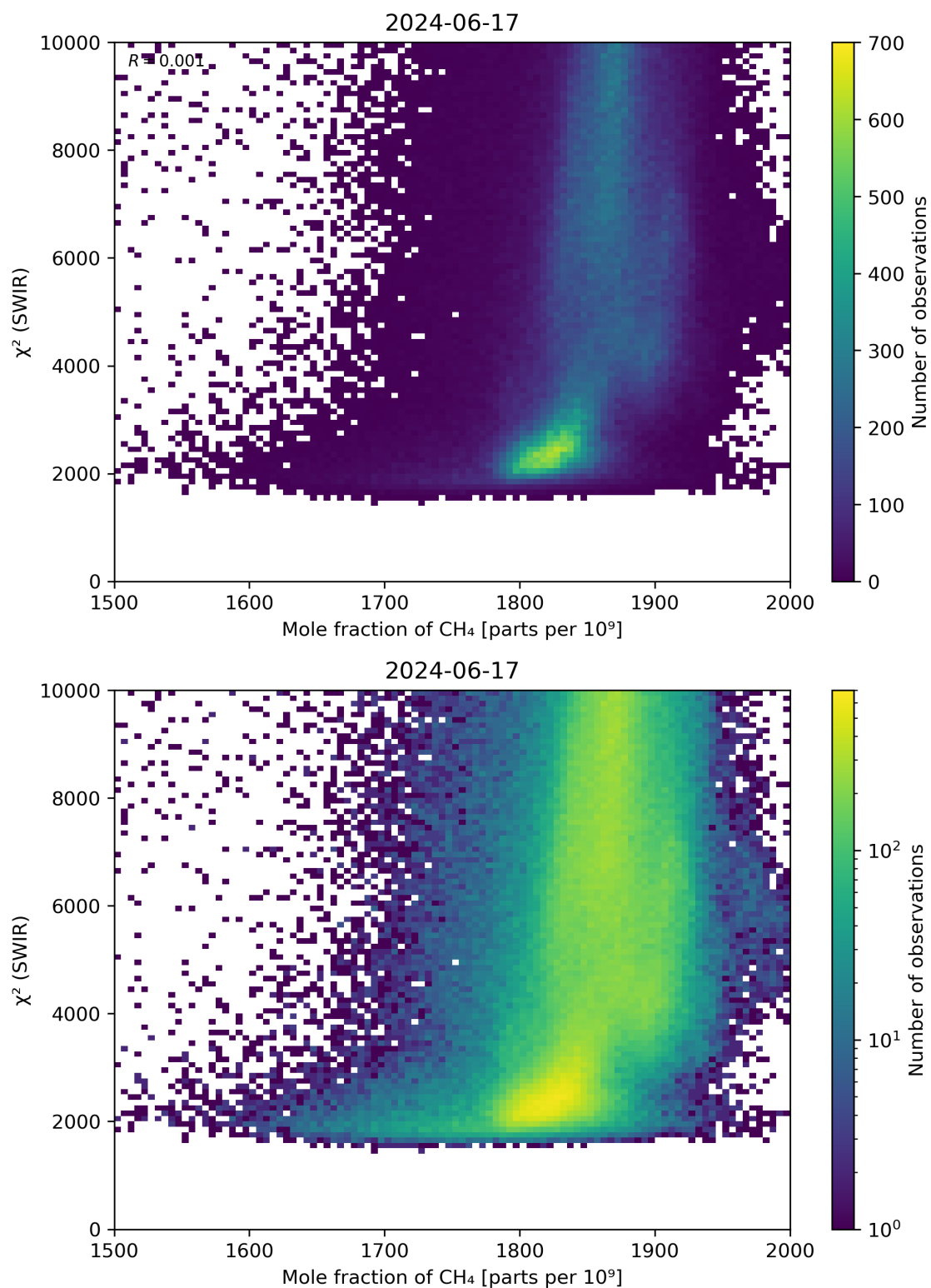
Figure 71: Scatter density plot of “Mole fraction of \text{CH}_4 ” against “ \chi^2 (SWIR)” for 2024-06-16 to 2024-06-18.
