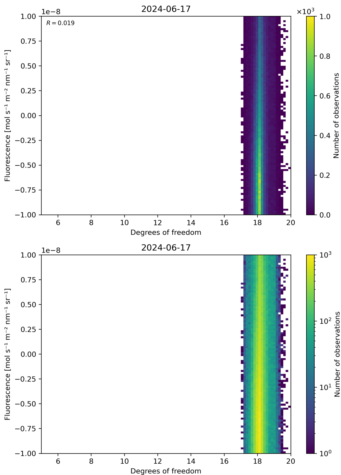
Figure 51: Scatter density plot of “Degrees of freedom” against “Fluorescence” for 2024-06-16 to 2024-06-18.
