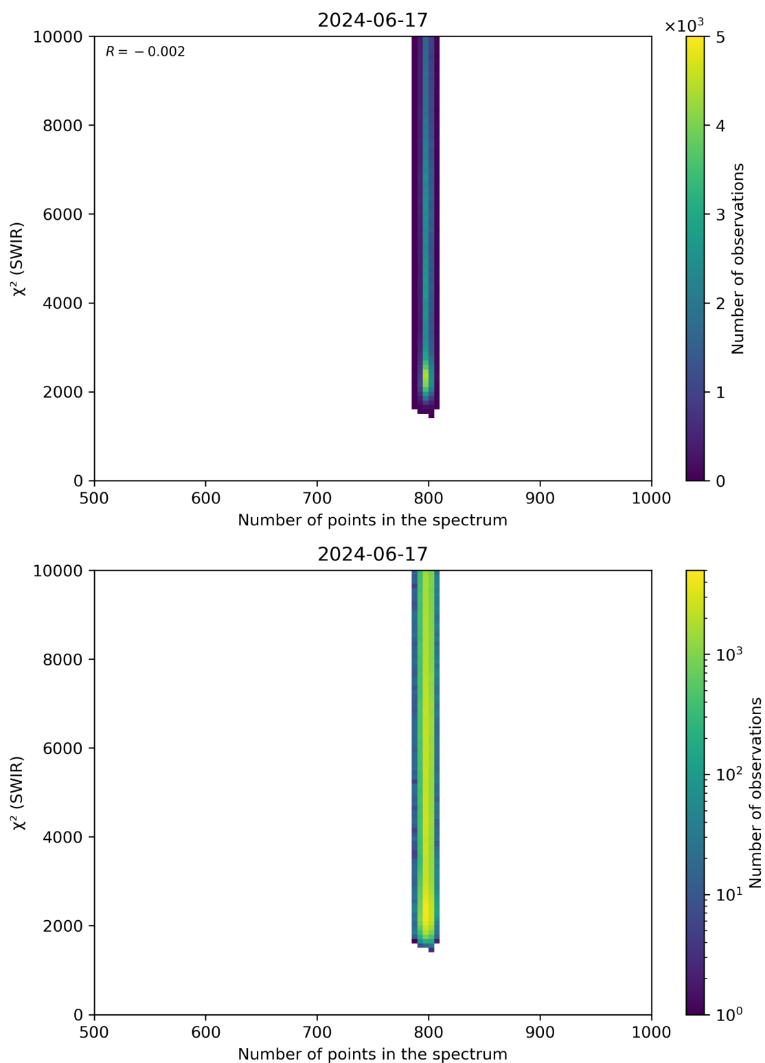
Figure 89: Scatter density plot of “Number of points in the spectrum” against “ \chi^2 (SWIR)” for 2024-06-16 to 2024-06-18.
