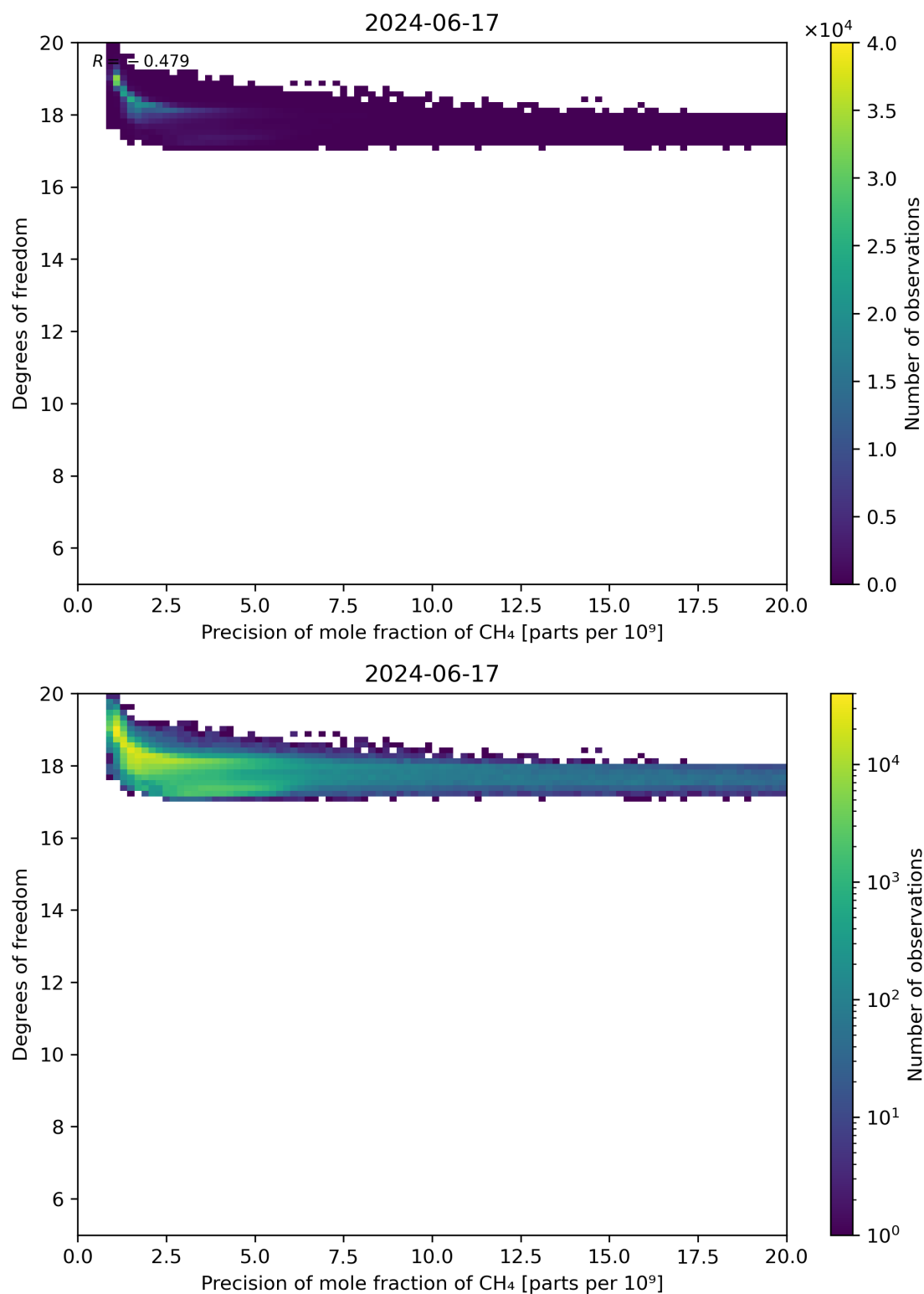
Figure 80: Scatter density plot of “Precision of mole fraction of CH 4 ” against “Degrees of freedom” for 2024-06-16 to 2024-06-18.
