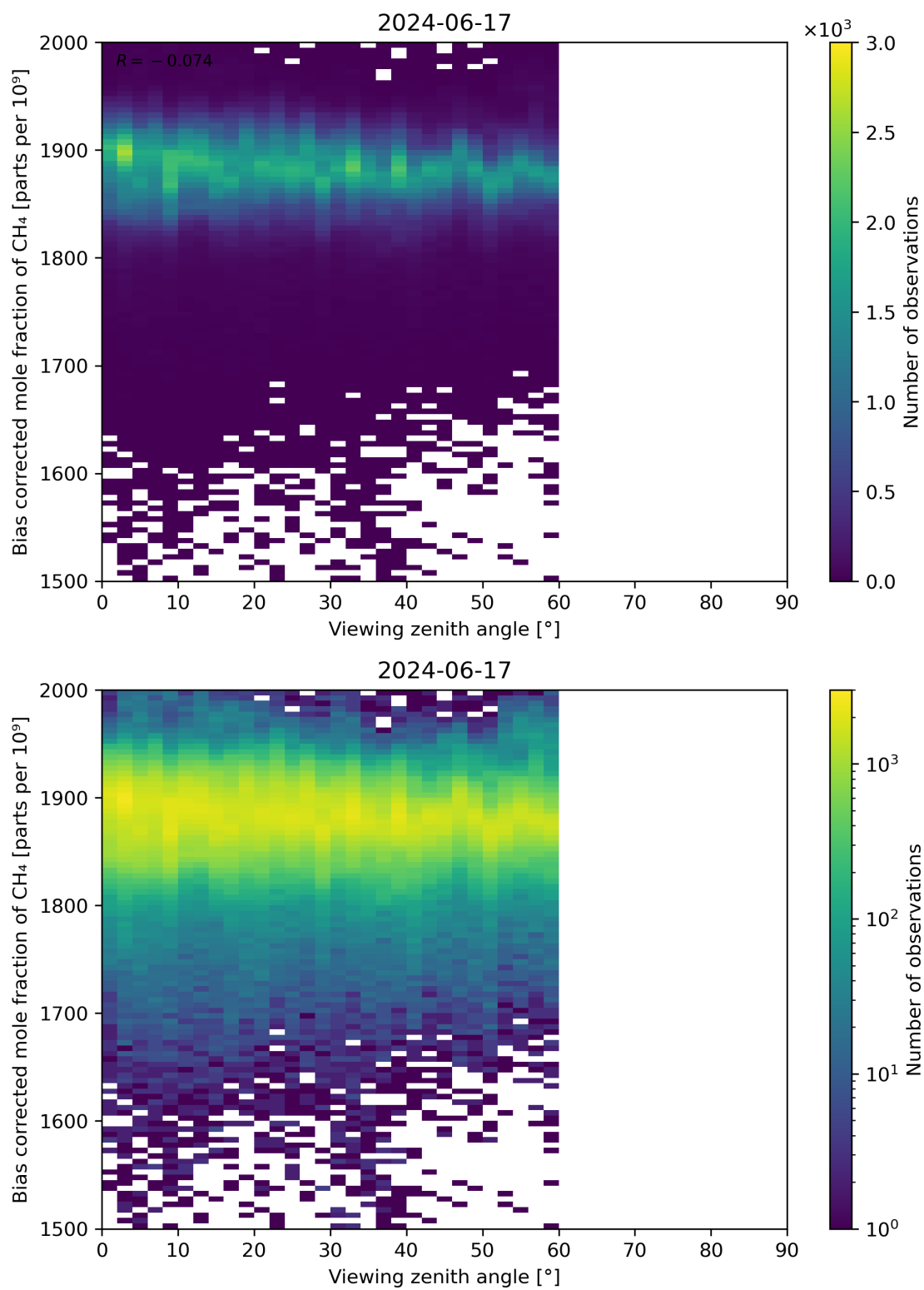
Figure 111: Scatter density plot of “Viewing zenith angle” against “Bias corrected mole fraction of CH 4 ” for 2024-06-16 to 2024-06-18.
