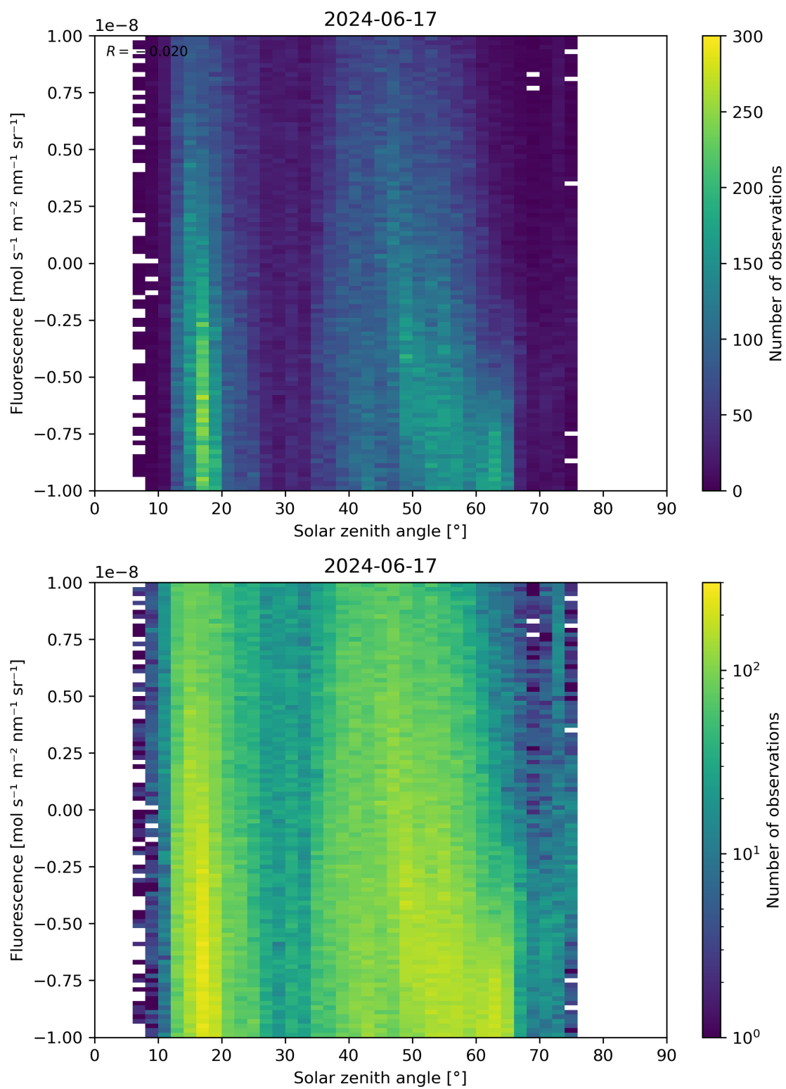
Figure 97: Scatter density plot of “Solar zenith angle” against “Fluorescence” for 2024-06-16 to 2024-06-18.
