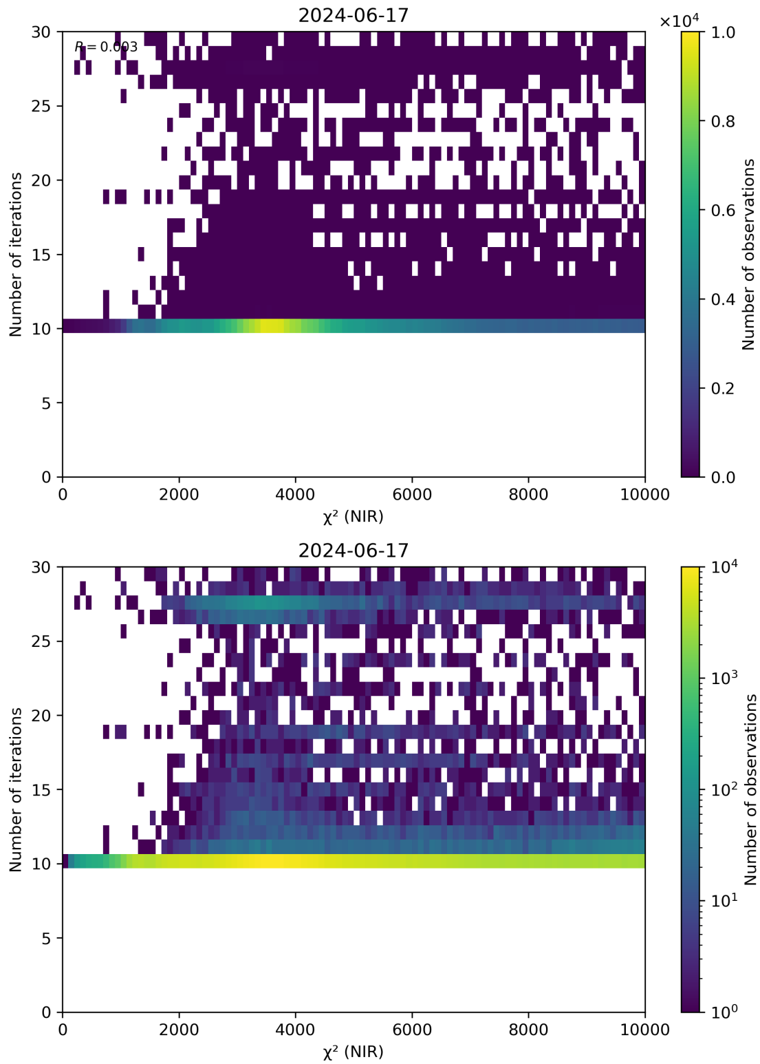
Figure 46: Scatter density plot of “ \chi^2 (NIR)” against “Number of iterations” for 2024-06-16 to 2024-06-18.
