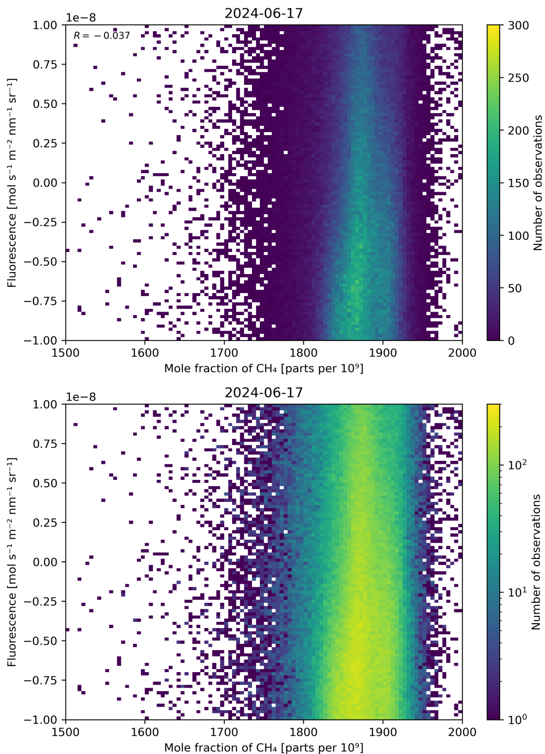
Figure 73: Scatter density plot of “Mole fraction of \text{CH}_4 ” against “Fluorescence” for 2024-06-16 to 2024-06-18.
