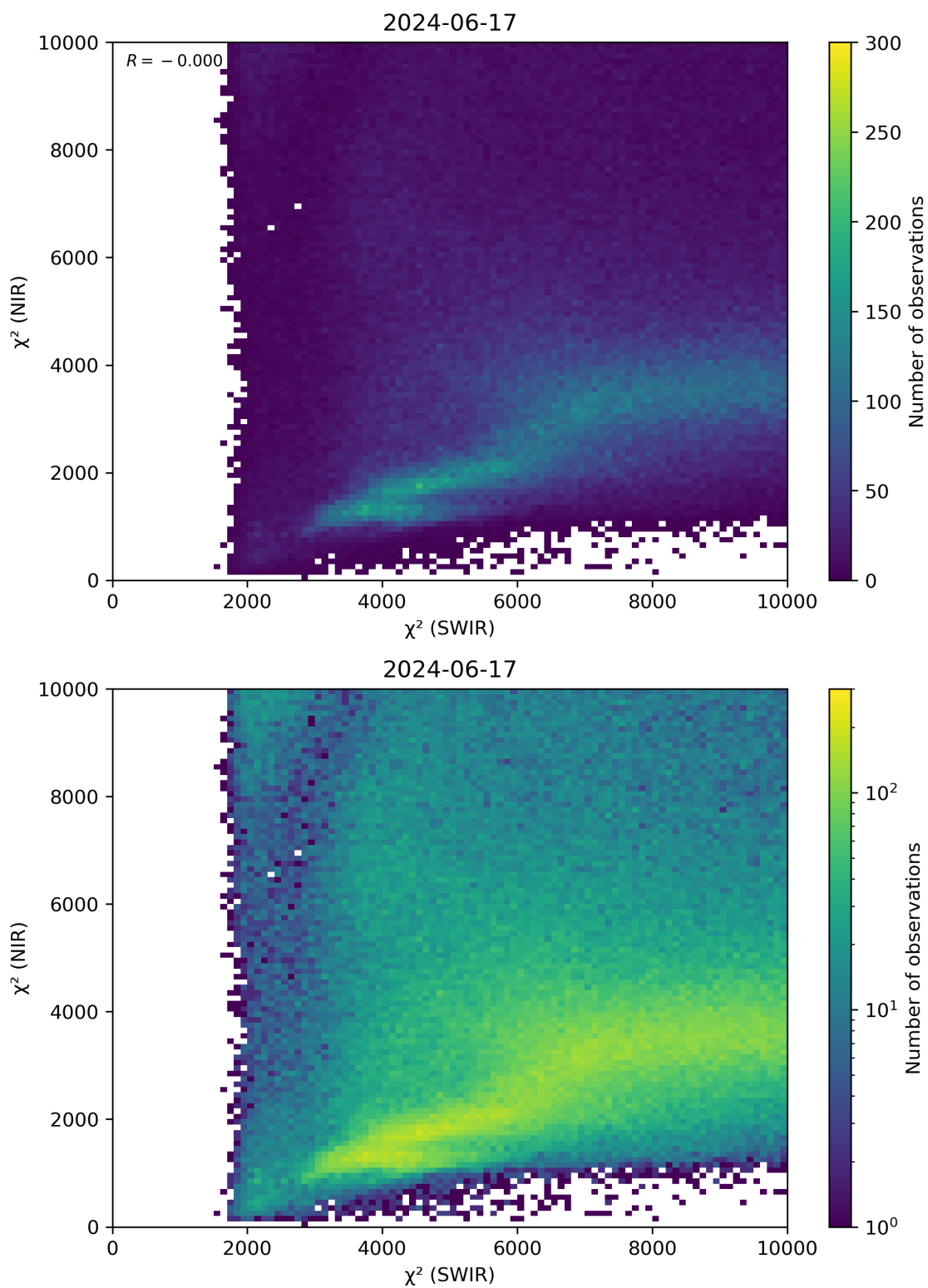
Figure 47: Scatter density plot of “ \chi^2 (SWIR)” against “ \chi^2 (NIR)” for 2024-06-16 to 2024-06-18.
