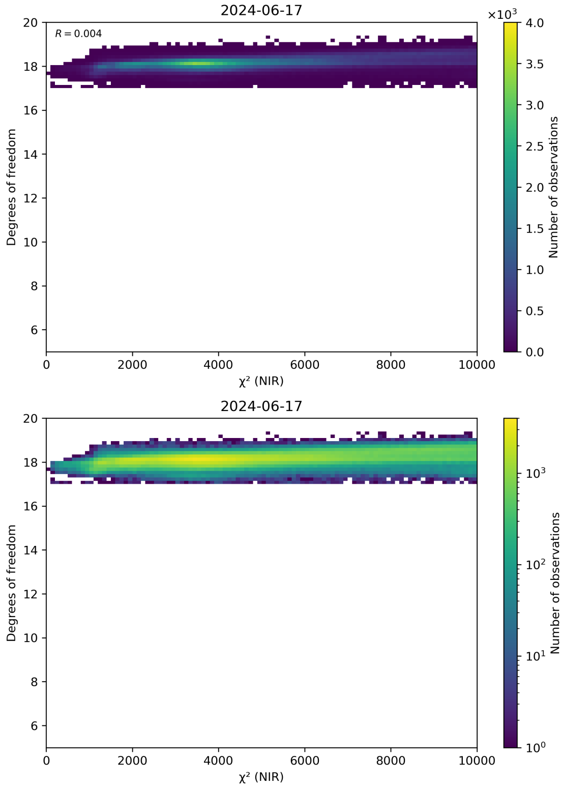
Figure 44: Scatter density plot of “ \chi^2 (NIR)” against “Degrees of freedom” for 2024-06-16 to 2024-06-18.
