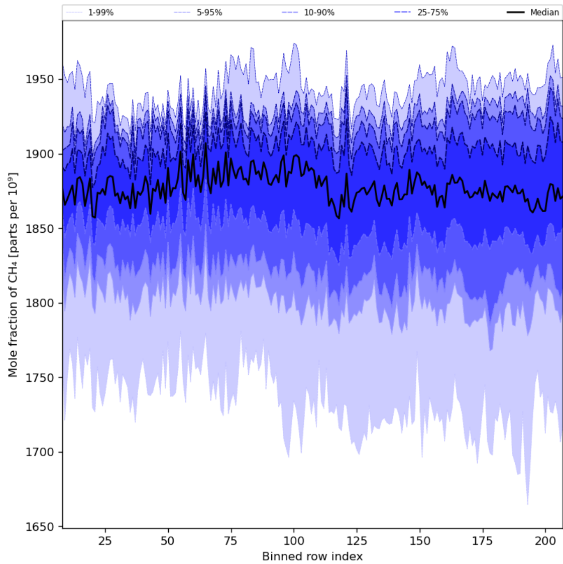
Figure 34: Along track statistics of “Mole fraction of CH 4 ” for 2024-06-16 to 2024-06-18
