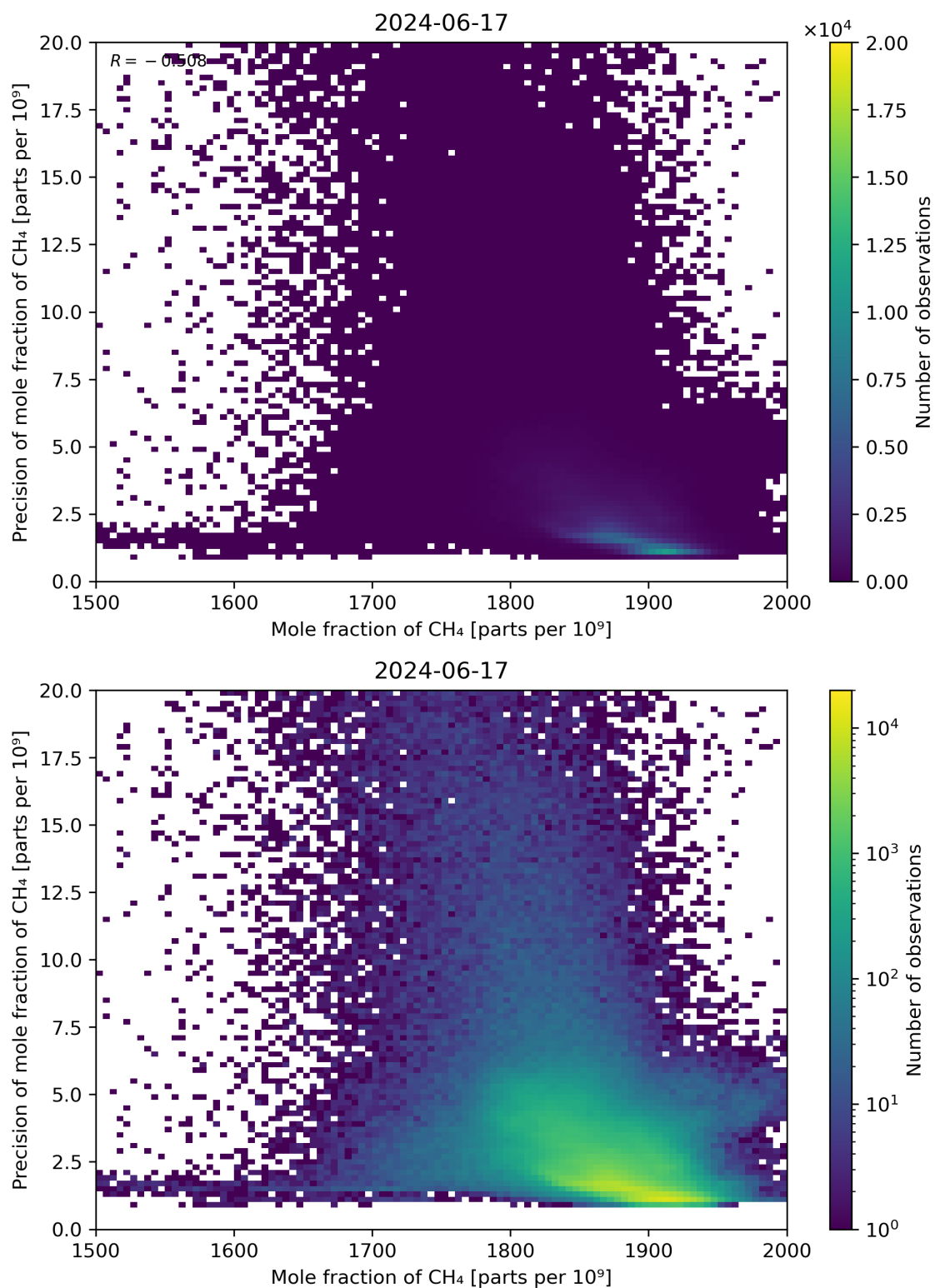
Figure 75: Scatter density plot of “Mole fraction of CH 4 ” against “Precision of mole fraction of CH 4 ” for 2024-06-16 to 2024-06-18.
