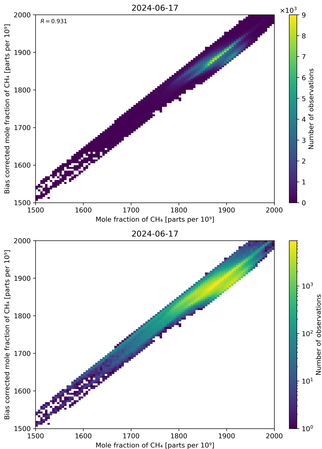
Figure 74: Scatter density plot of “Mole fraction of CH 4 ” against “Bias corrected mole fraction of CH 4 ” for 2024-06-16 to 2024-06-18.
