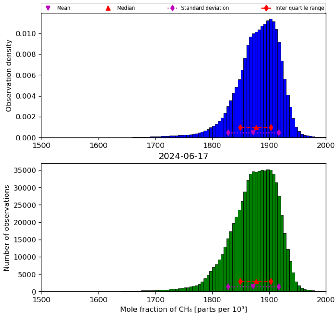
Figure 23: Histogram of “Mole fraction of CH 4 ” for 2024-06-16 to 2024-06-18
