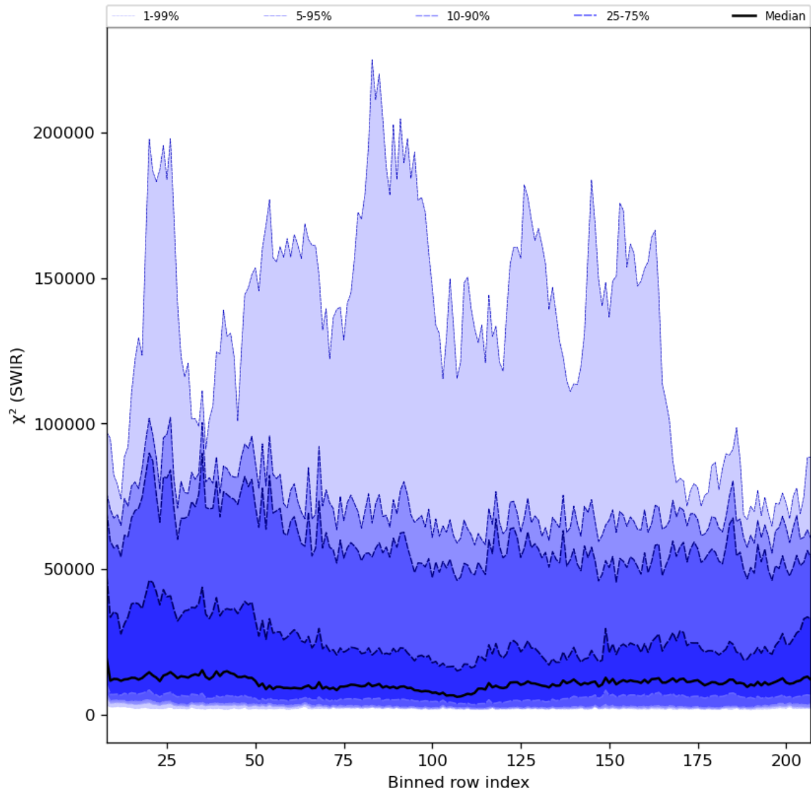
Figure 39: Along track statistics of “ \chi^2 (SWIR)” for 2024-06-16 to 2024-06-18
