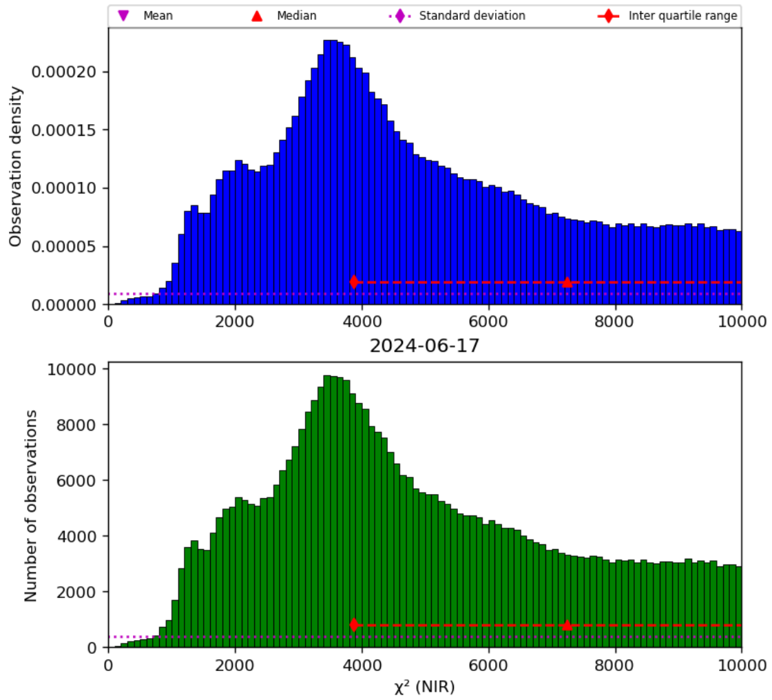
Figure 29: Histogram of “ \chi^2 (NIR)” for 2024-06-16 to 2024-06-18
