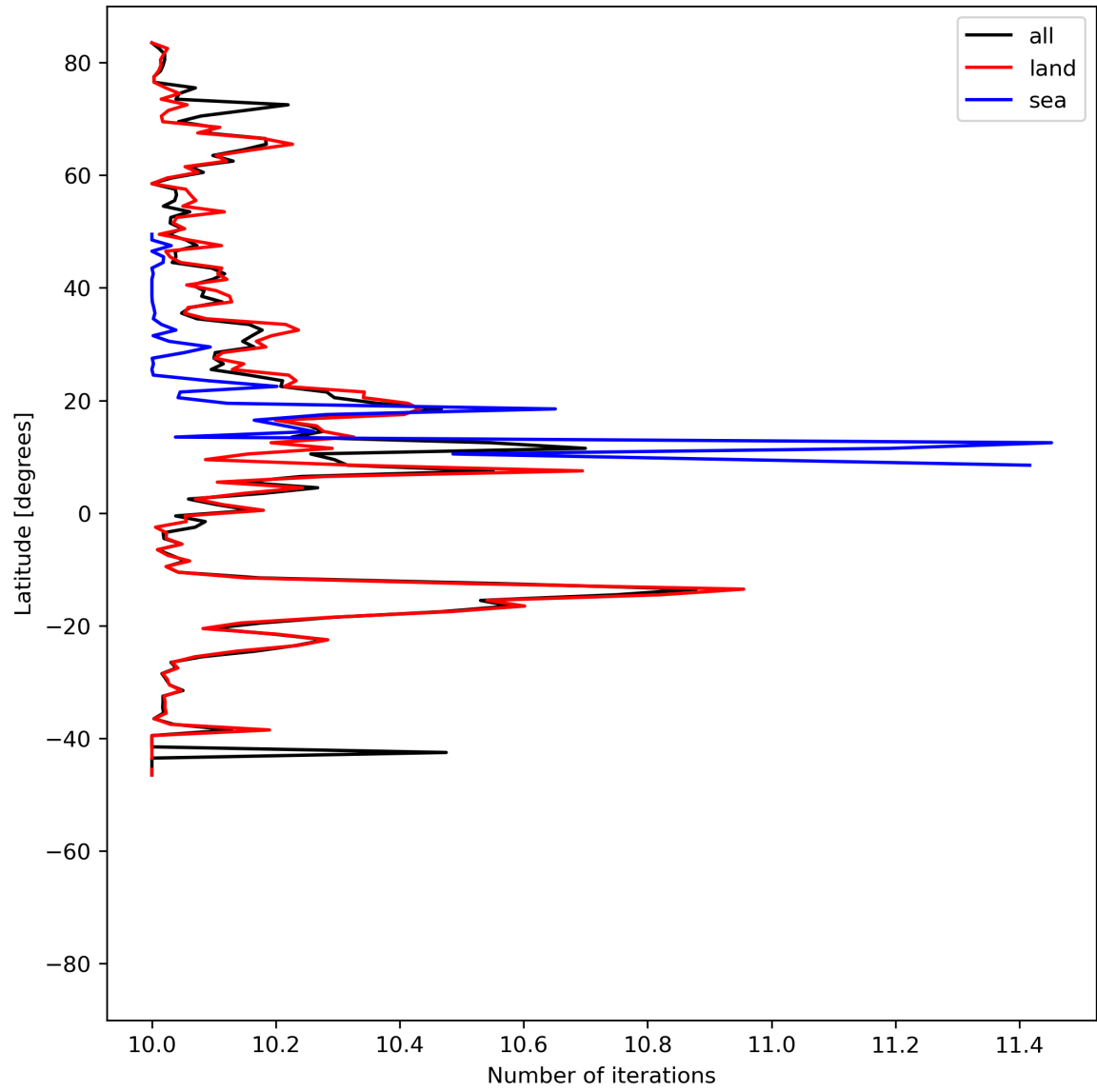
Figure 20: Zonal average of “Number of iterations” for 2024-06-16 to 2024-06-18.
