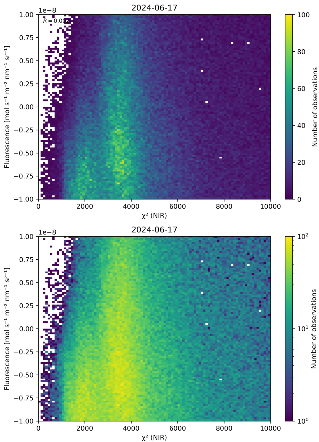
Figure 45: Scatter density plot of “ \chi^2 (NIR)” against “Fluorescence” for 2024-06-16 to 2024-06-18.
