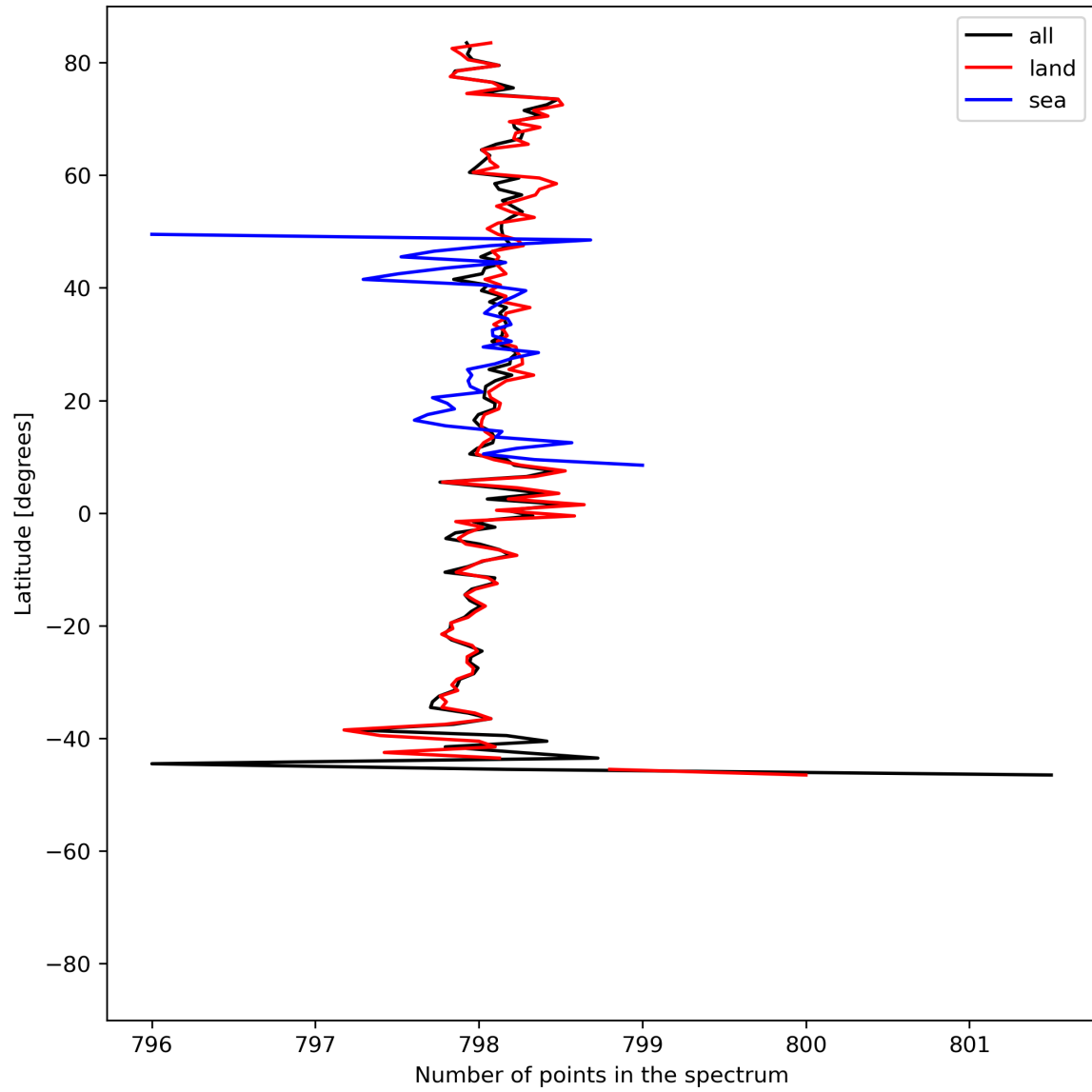
Figure 15: Zonal average of “Number of points in the spectrum” for 2024-06-16 to 2024-06-18.
