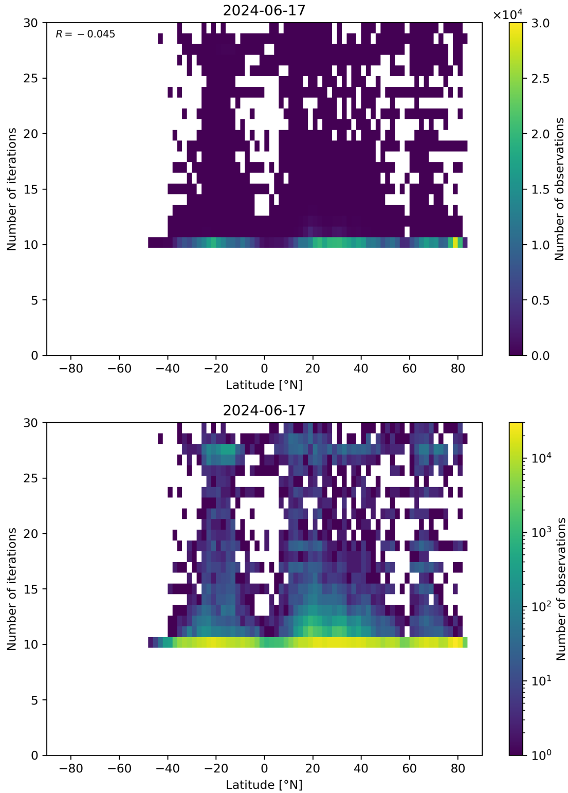
Figure 60: Scatter density plot of “Latitude” against “Number of iterations” for 2024-06-16 to 2024-06-18.
