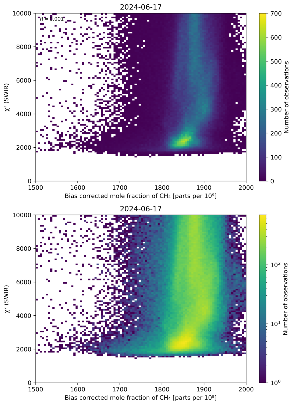
Figure 64: Scatter density plot of “Bias corrected mole fraction of CH 4 ” against “ \chi^2 (SWIR)” for 2024-06-16 to 2024-06-18.
