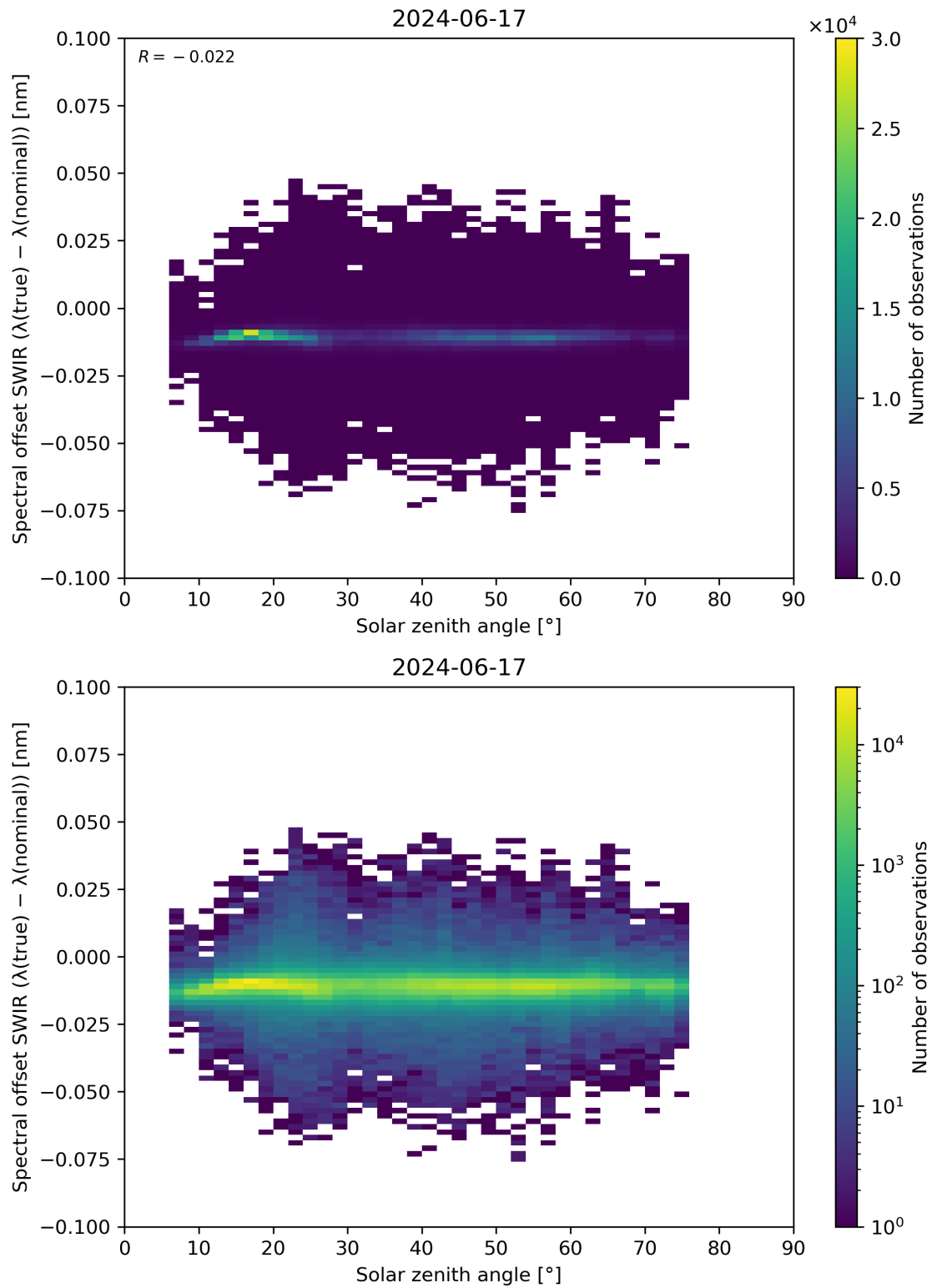
Figure 104: Scatter density plot of “Solar zenith angle” against “Spectral offset SWIR ( \lambda(\text{true}) - \lambda(\text{nominal}) )” for 2024-06-16 to 2024-06-18.
