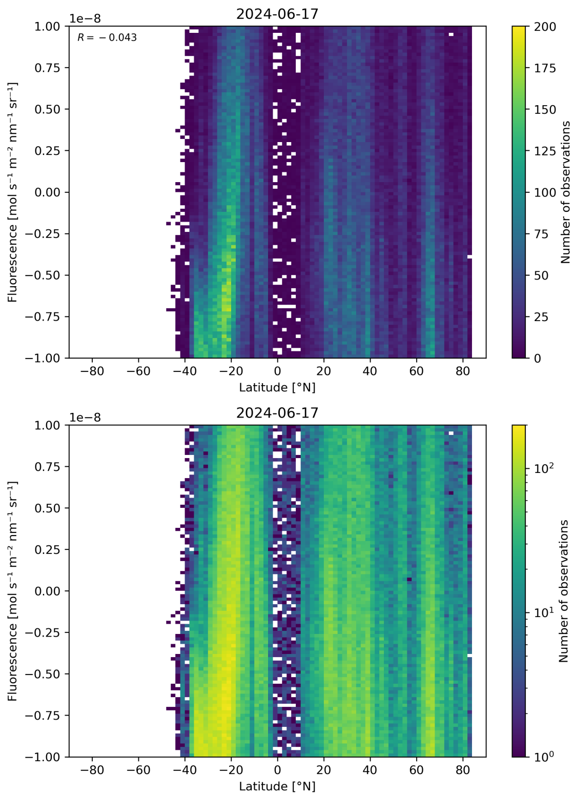
Figure 56: Scatter density plot of “Latitude” against “Fluorescence” for 2024-06-16 to 2024-06-18.
