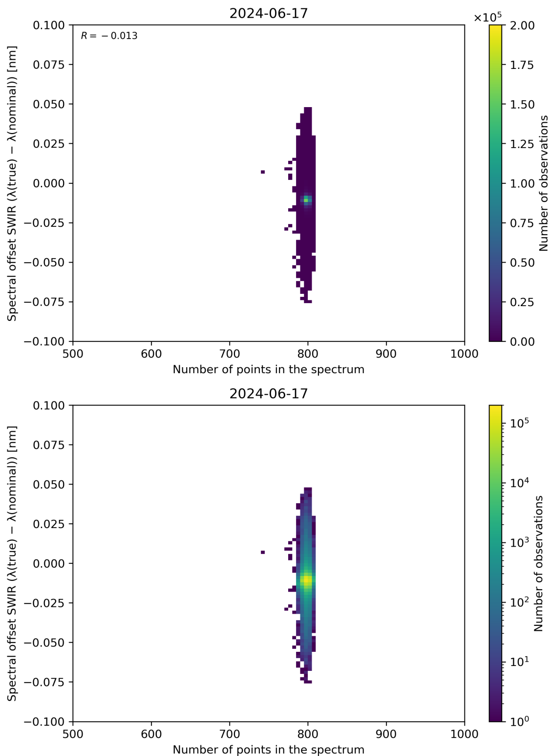
Figure 93: Scatter density plot of “Number of points in the spectrum” against “Spectral offset SWIR ( \lambda(\text{true}) - \lambda(\text{nominal}) )” for 2024-06-16 to 2024-06-18.
