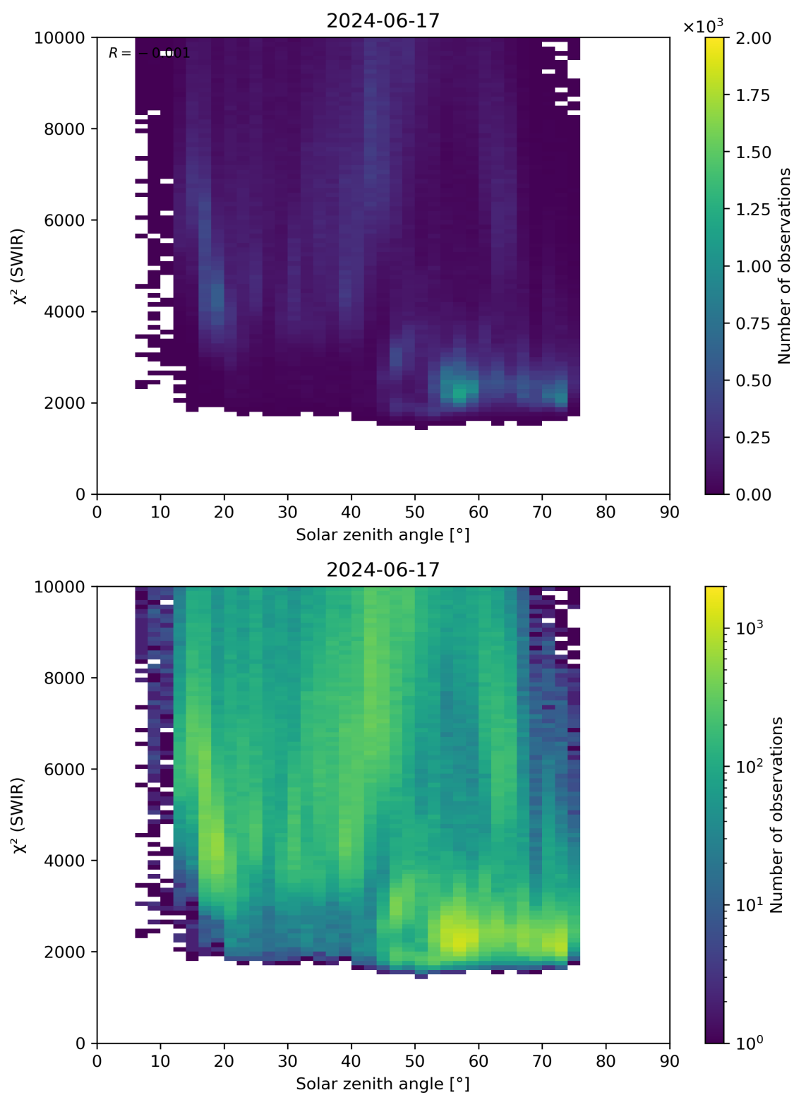
Figure 95: Scatter density plot of “Solar zenith angle” against “ \chi^2 (SWIR)” for 2024-06-16 to 2024-06-18.
