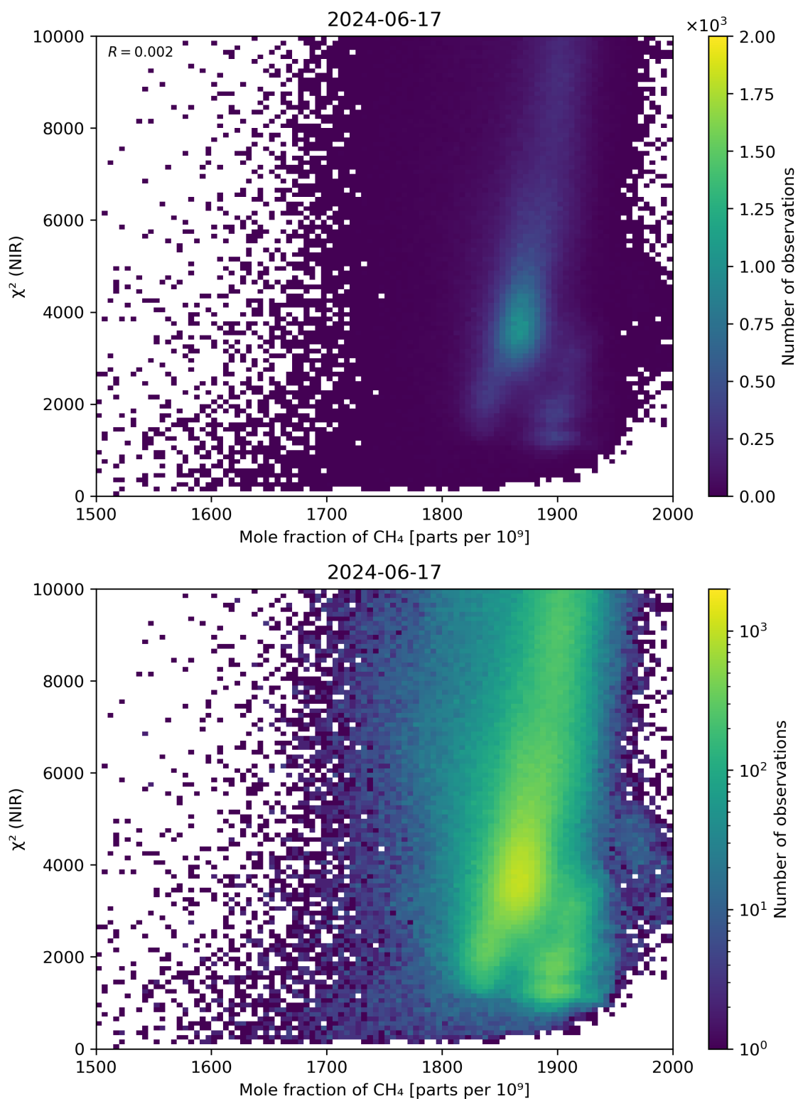
Figure 70: Scatter density plot of “Mole fraction of \text{CH}_4 ” against “ \chi^2 (NIR)” for 2024-06-16 to 2024-06-18.
