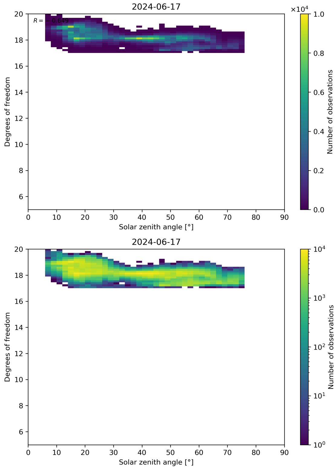
Figure 96: Scatter density plot of “Solar zenith angle” against “Degrees of freedom” for 2024-06-16 to 2024-06-18.
