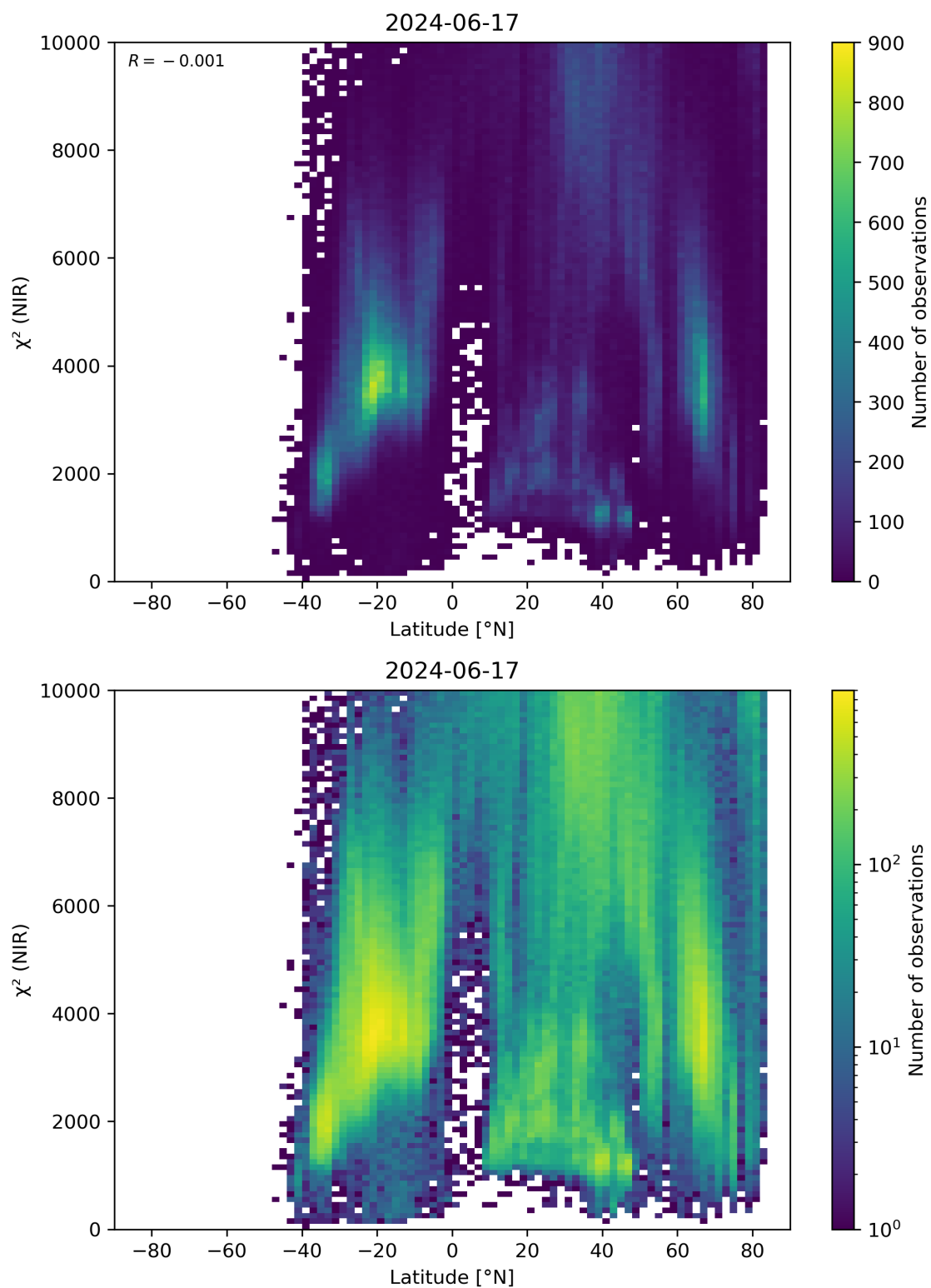
Figure 53: Scatter density plot of “Latitude” against “ \chi^2 (NIR)” for 2024-06-16 to 2024-06-18.
