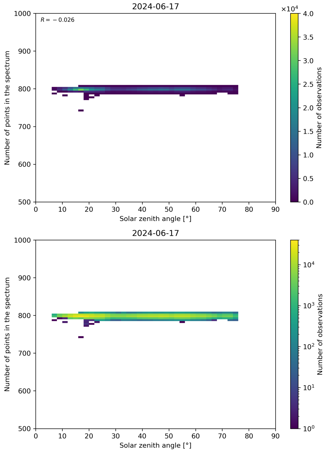
Figure 103: Scatter density plot of “Solar zenith angle” against “Number of points in the spectrum” for 2024-06-16 to 2024-06-18.
