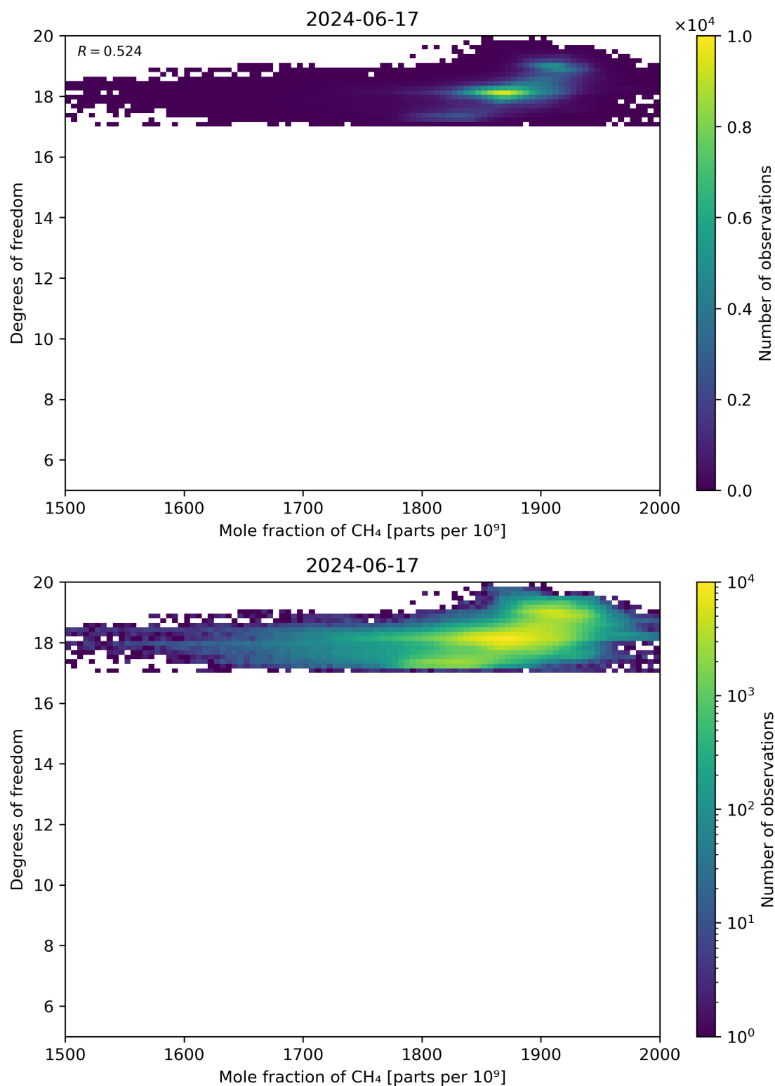
Figure 72: Scatter density plot of “Mole fraction of CH 4 ” against “Degrees of freedom” for 2024-06-16 to 2024-06-18.
