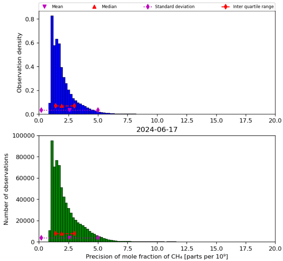
Figure 24: Histogram of “Precision of mole fraction of CH 4 ” for 2024-06-16 to 2024-06-18
