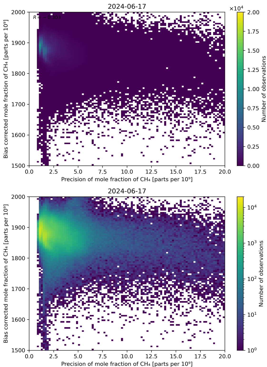
Figure 82: Scatter density plot of “Precision of mole fraction of CH 4 ” against “Bias corrected mole fraction of CH 4 ” for 2024-06-16 to 2024-06-18.
