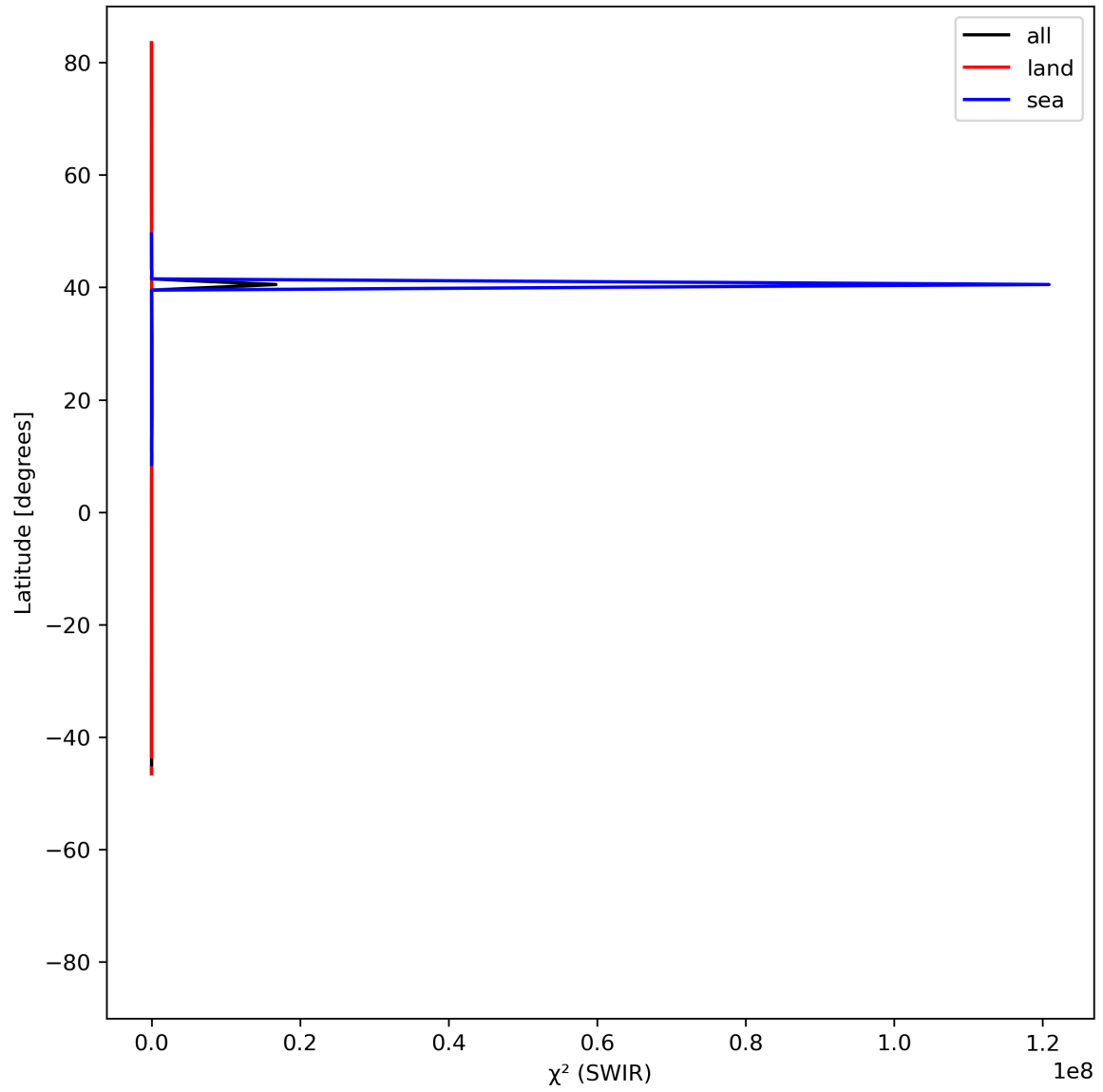
Figure 17: Zonal average of “ \chi^2 (SWIR)” for 2024-06-16 to 2024-06-18.
