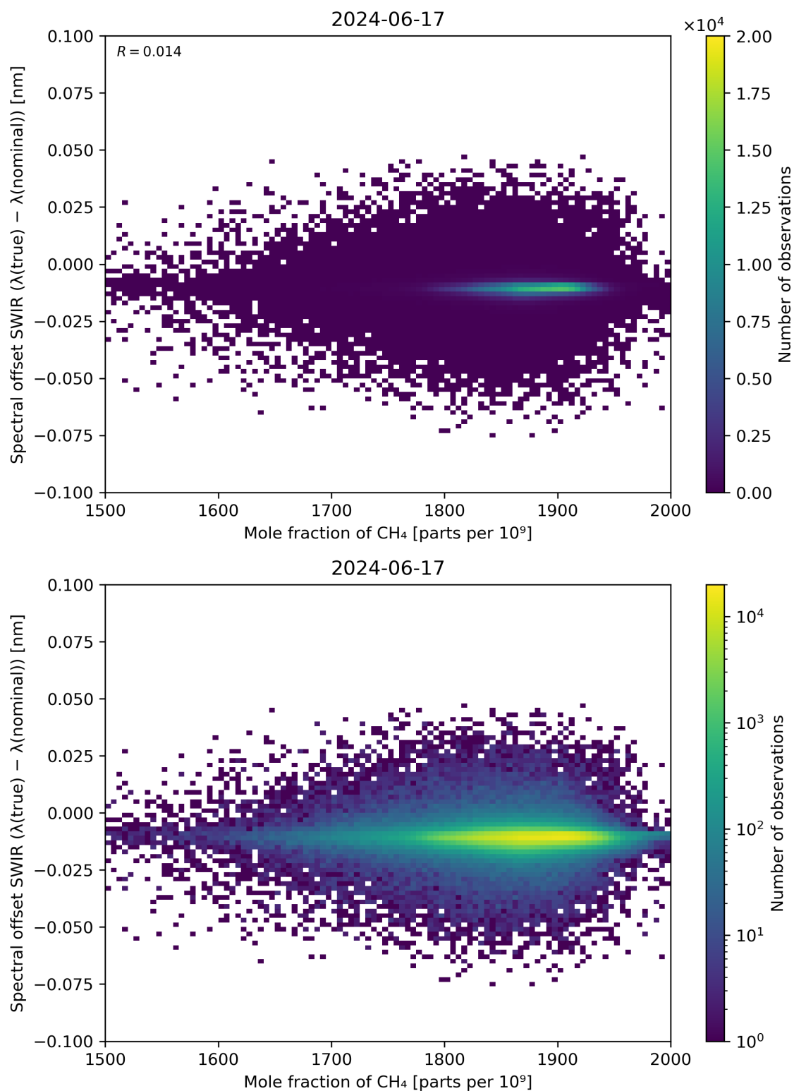
Figure 86: Scatter density plot of “Mole fraction of CH 4 ” against “Spectral offset SWIR ( \lambda(\text{true}) - \lambda(\text{nominal}) )” for 2024-06-16 to 2024-06-18.
