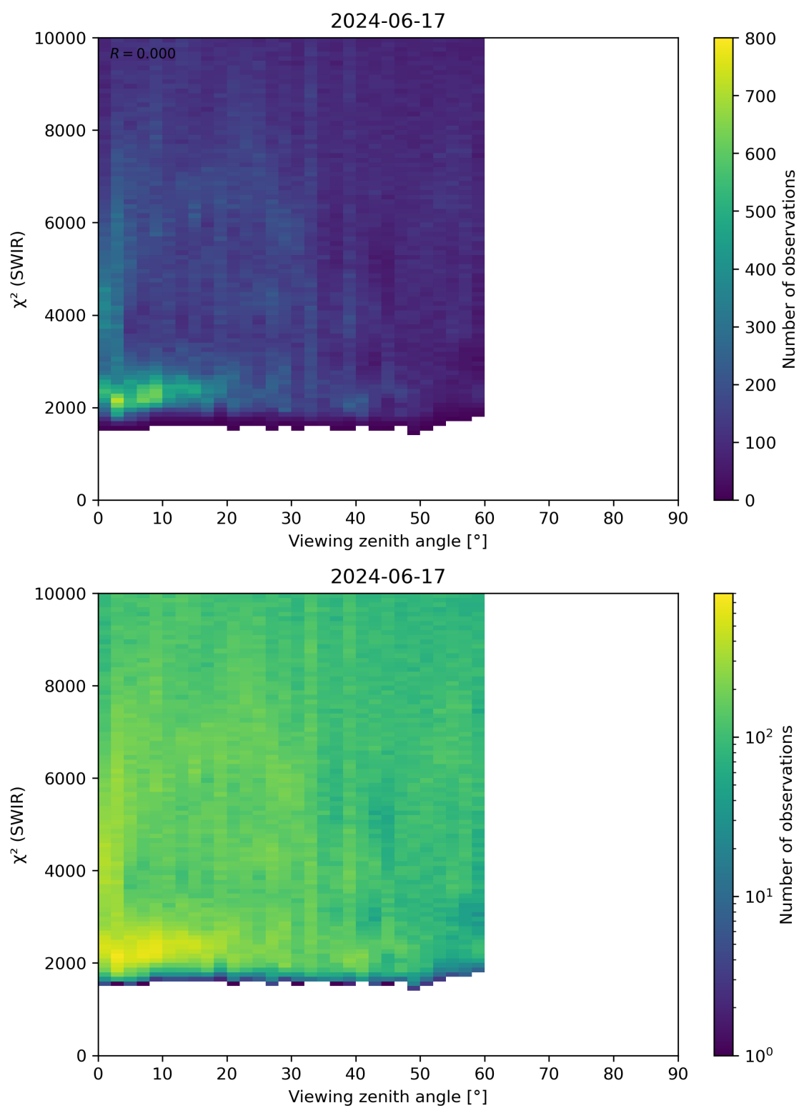
Figure 106: Scatter density plot of “Viewing zenith angle” against “ \chi^2 (SWIR)” for 2024-06-16 to 2024-06-18.
