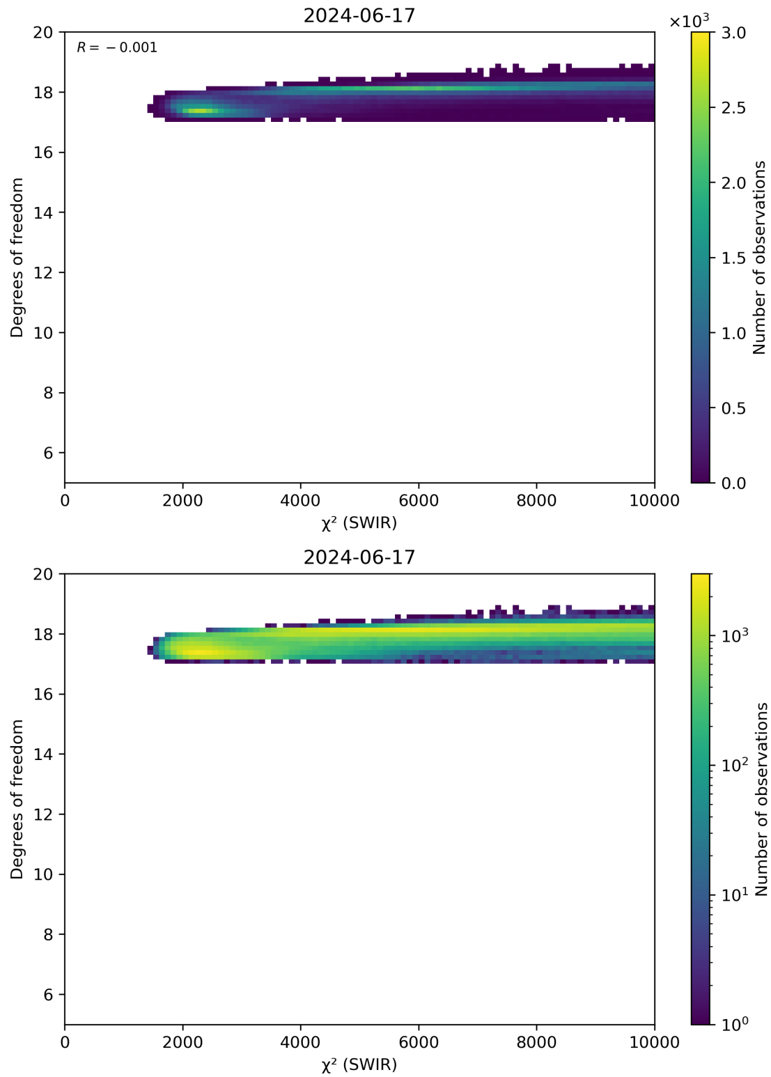
Figure 48: Scatter density plot of “ \chi^2 (SWIR)” against “Degrees of freedom” for 2024-06-16 to 2024-06-18.
