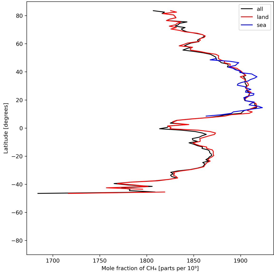
Figure 12: Zonal average of “Mole fraction of \text{CH}_4 ” for 2024-06-16 to 2024-06-18.
