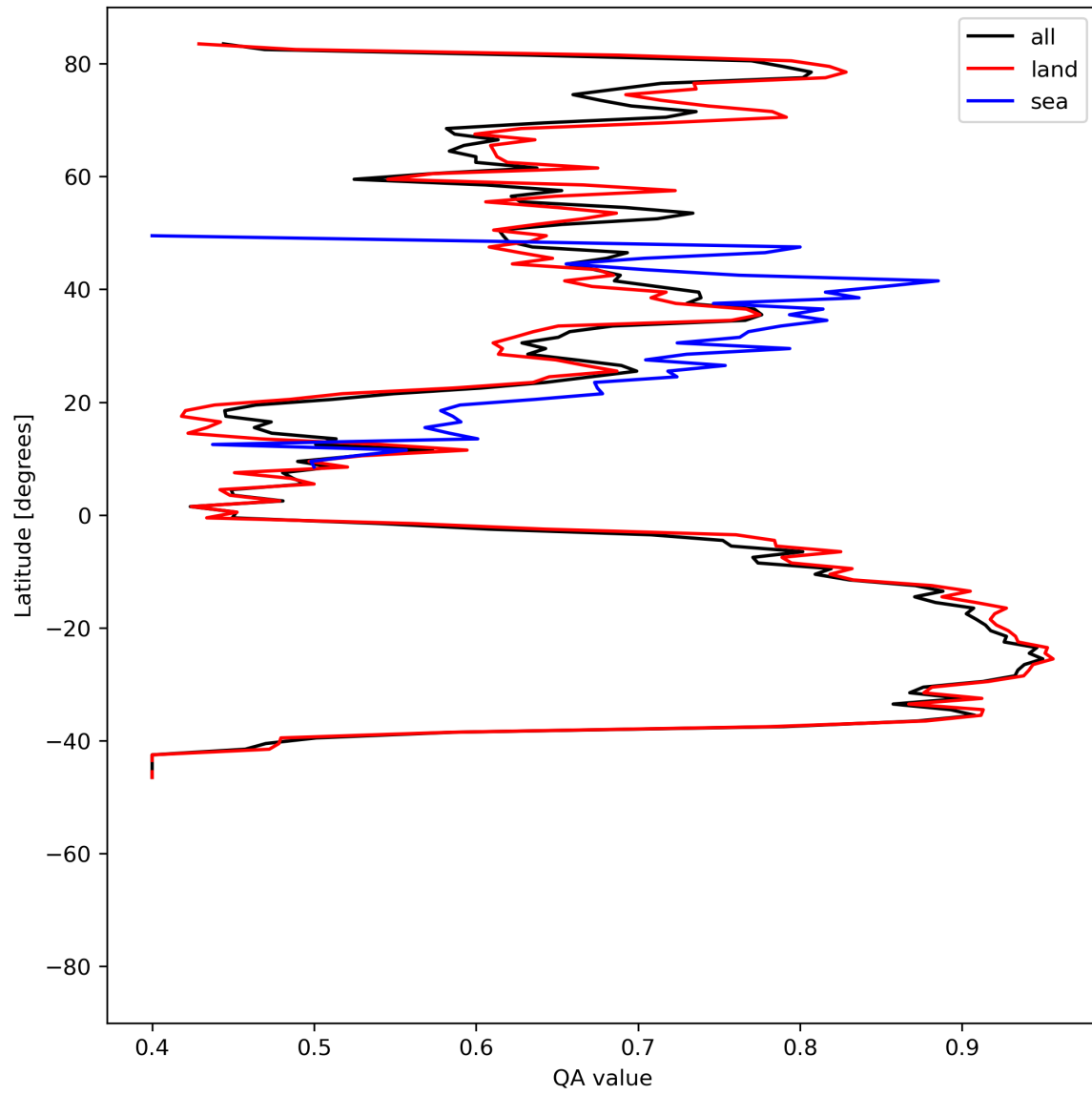
Figure 11: Zonal average of “QA value” for 2024-06-16 to 2024-06-18.
