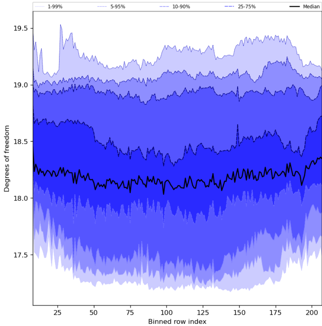
Figure 41: Along track statistics of “Degrees of freedom” for 2024-06-16 to 2024-06-18
