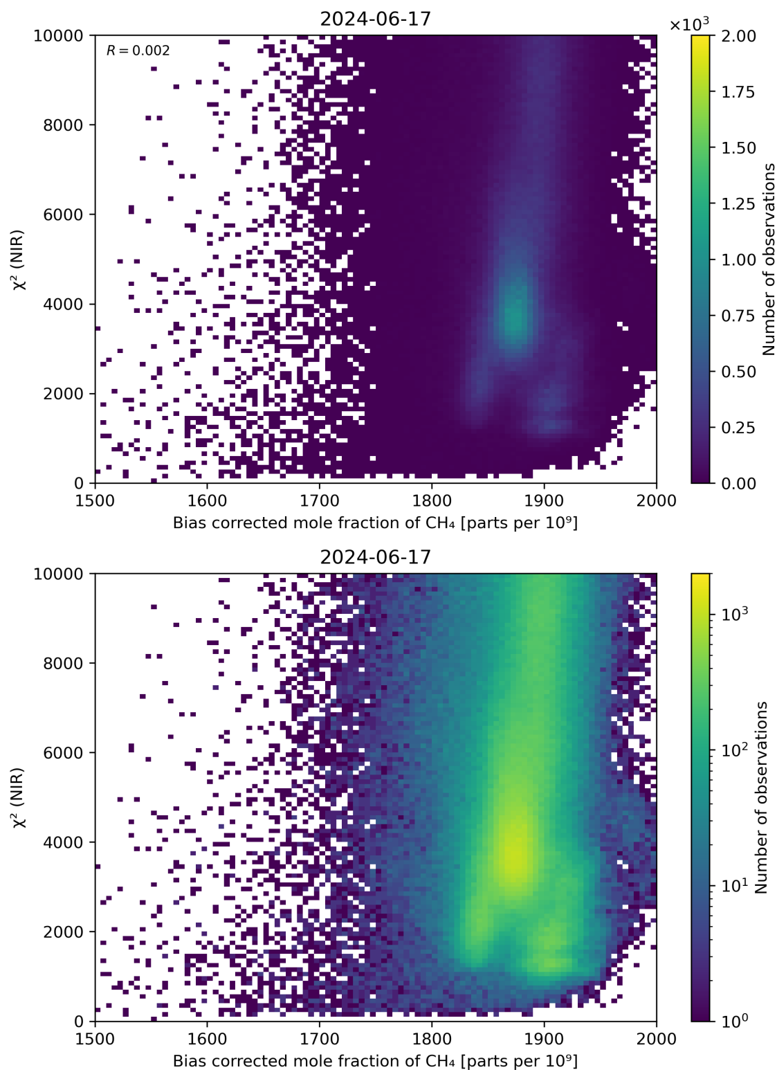
Figure 63: Scatter density plot of “Bias corrected mole fraction of \text{CH}_4 ” against “ \chi^2 (NIR)” for 2024-06-16 to 2024-06-18.
