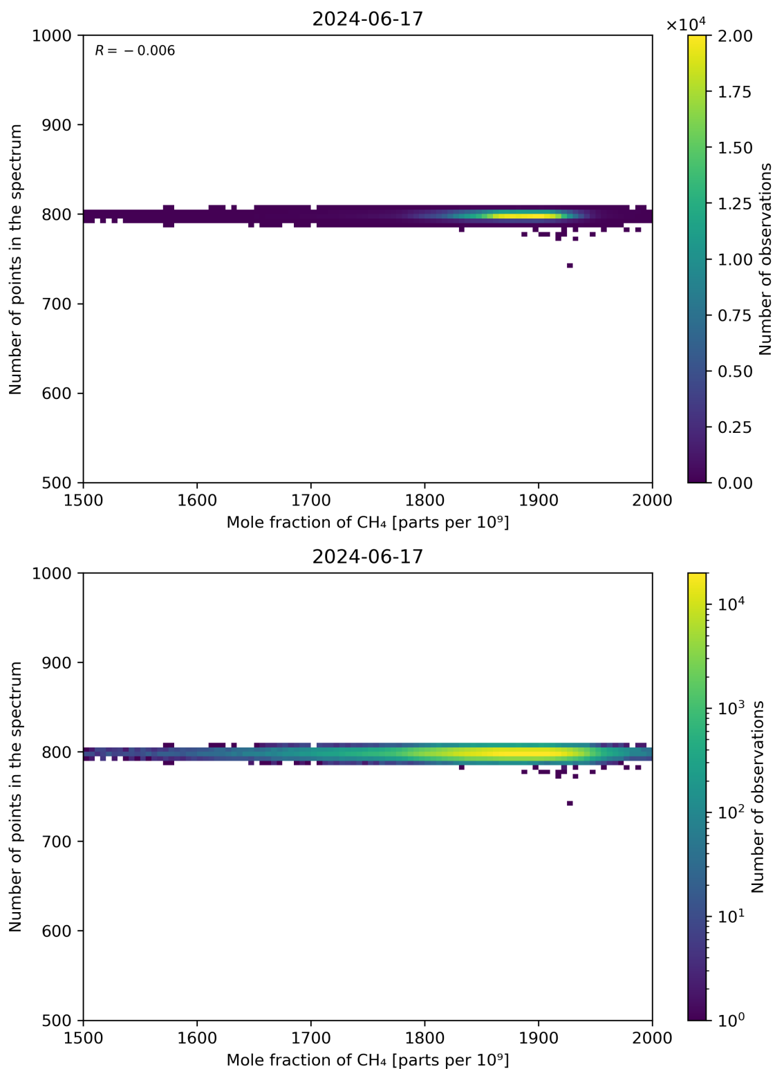
Figure 77: Scatter density plot of “Mole fraction of CH 4 ” against “Number of points in the spectrum” for 2024-06-16 to 2024-06-18.
