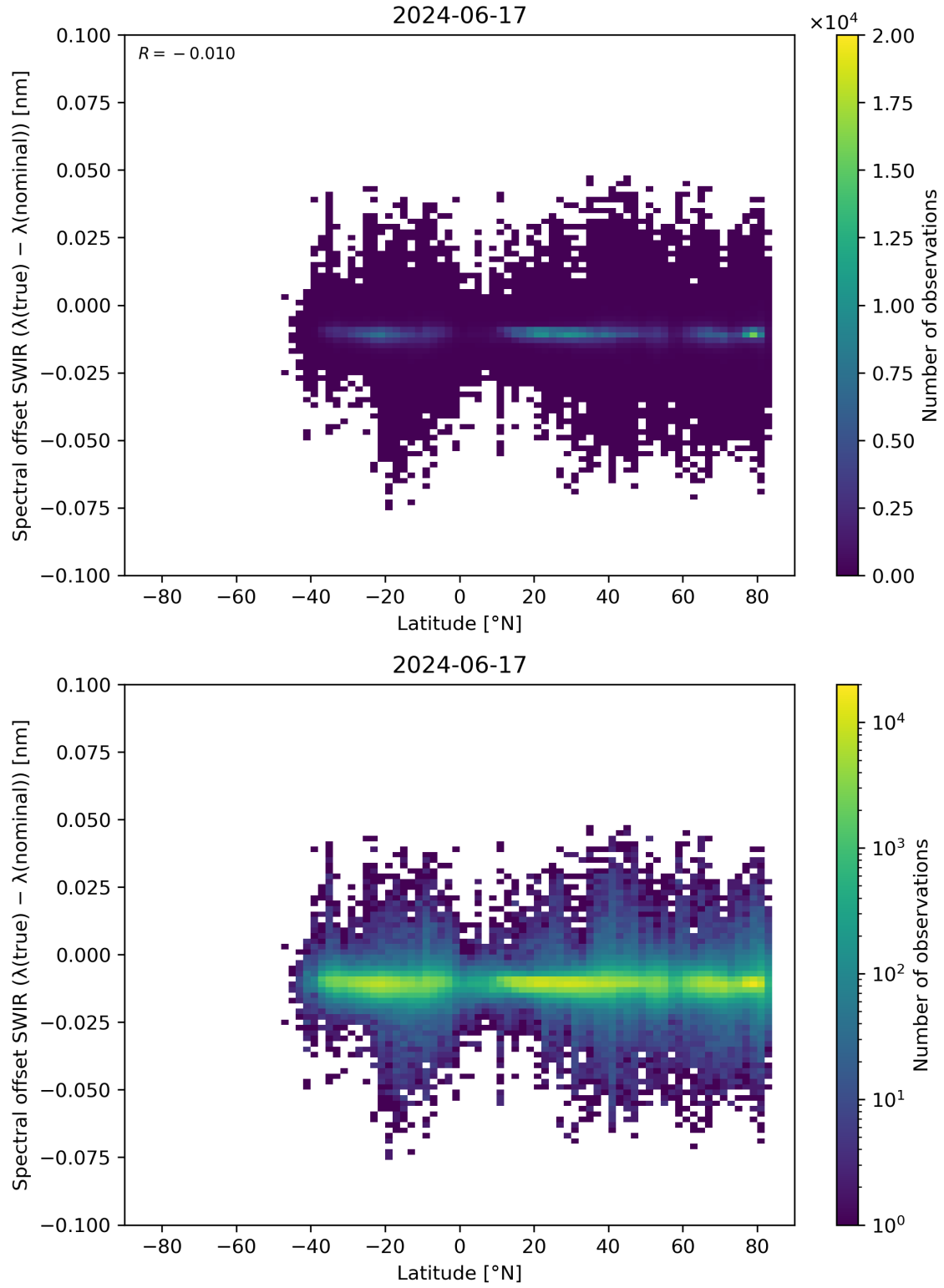
Figure 62: Scatter density plot of “Latitude” against “Spectral offset SWIR ( \lambda(\text{true}) - \lambda(\text{nominal}) )” for 2024-06-16 to 2024-06-18.
