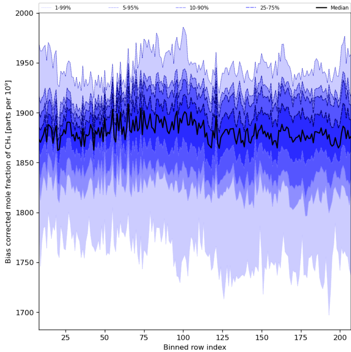
Figure 36: Along track statistics of “Bias corrected mole fraction of CH 4 ” for 2024-06-16 to 2024-06-18
