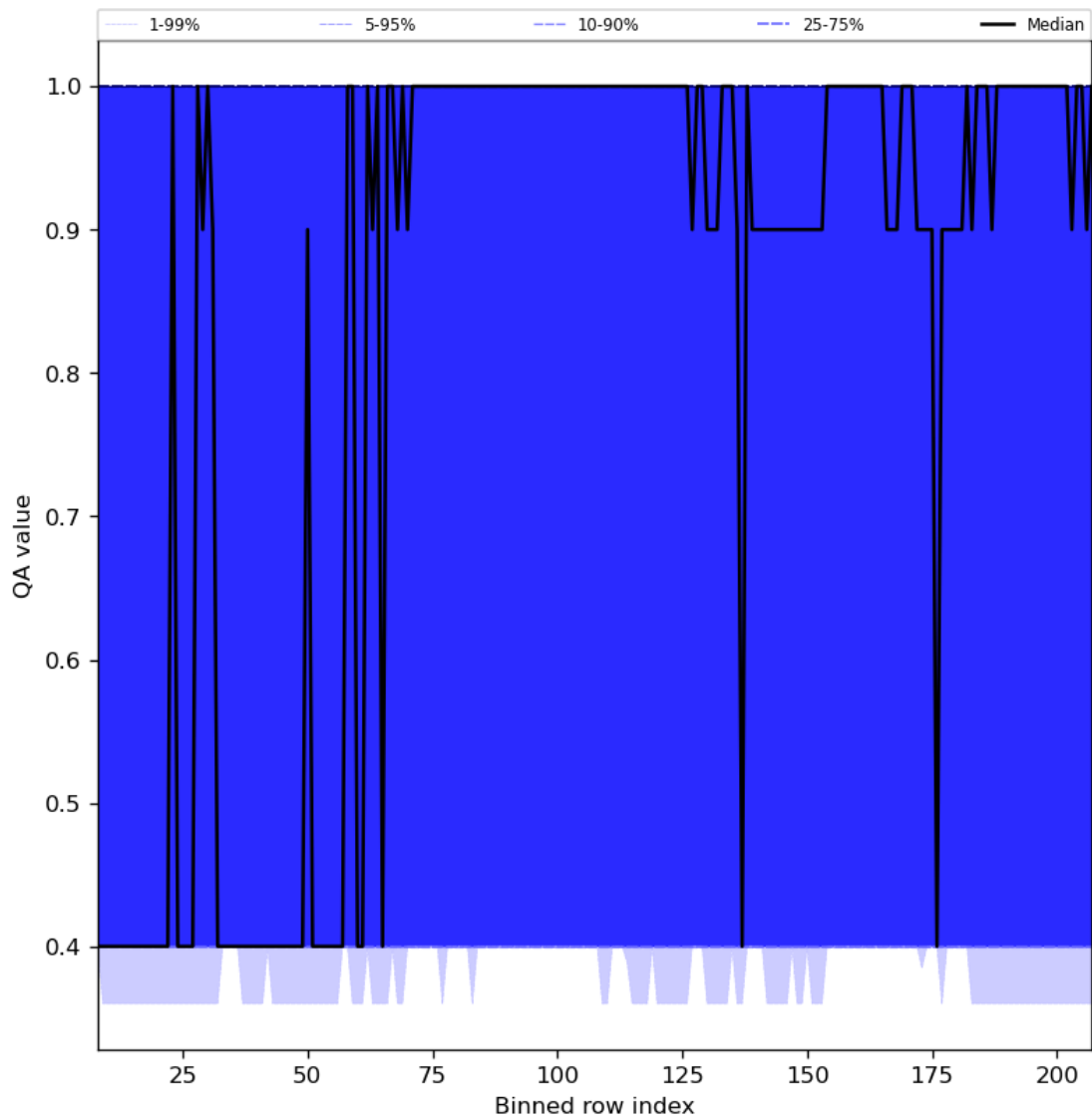
Figure 33: Along track statistics of “QA value” for 2024-06-16 to 2024-06-18
