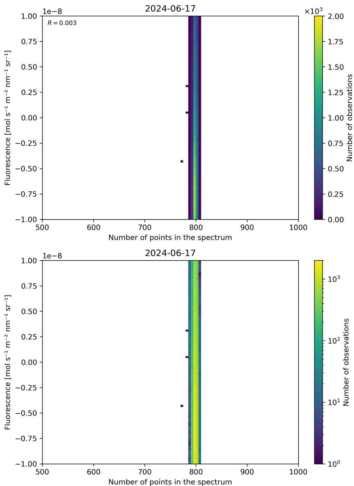
Figure 91: Scatter density plot of “Number of points in the spectrum” against “Fluorescence” for 2024-06-16 to 2024-06-18.
