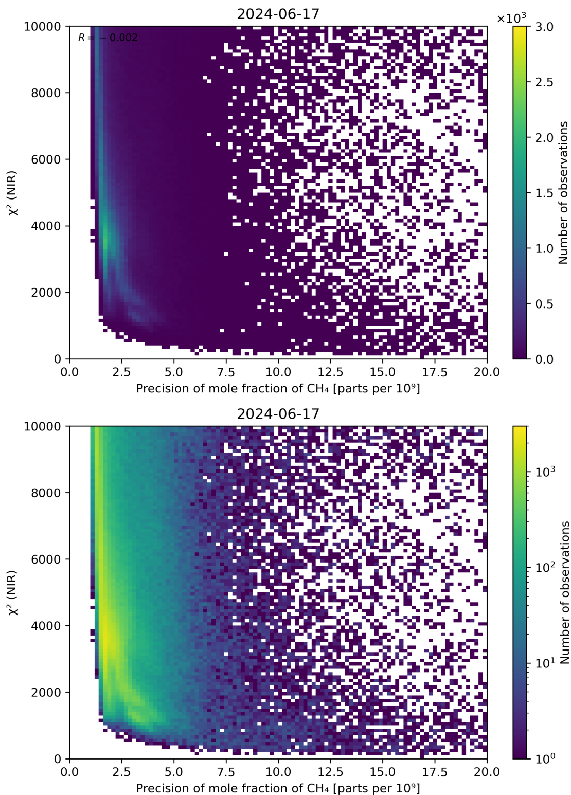
Figure 78: Scatter density plot of “Precision of mole fraction of CH 4 ” against “ \chi^2 (NIR)” for 2024-06-16 to 2024-06-18.
