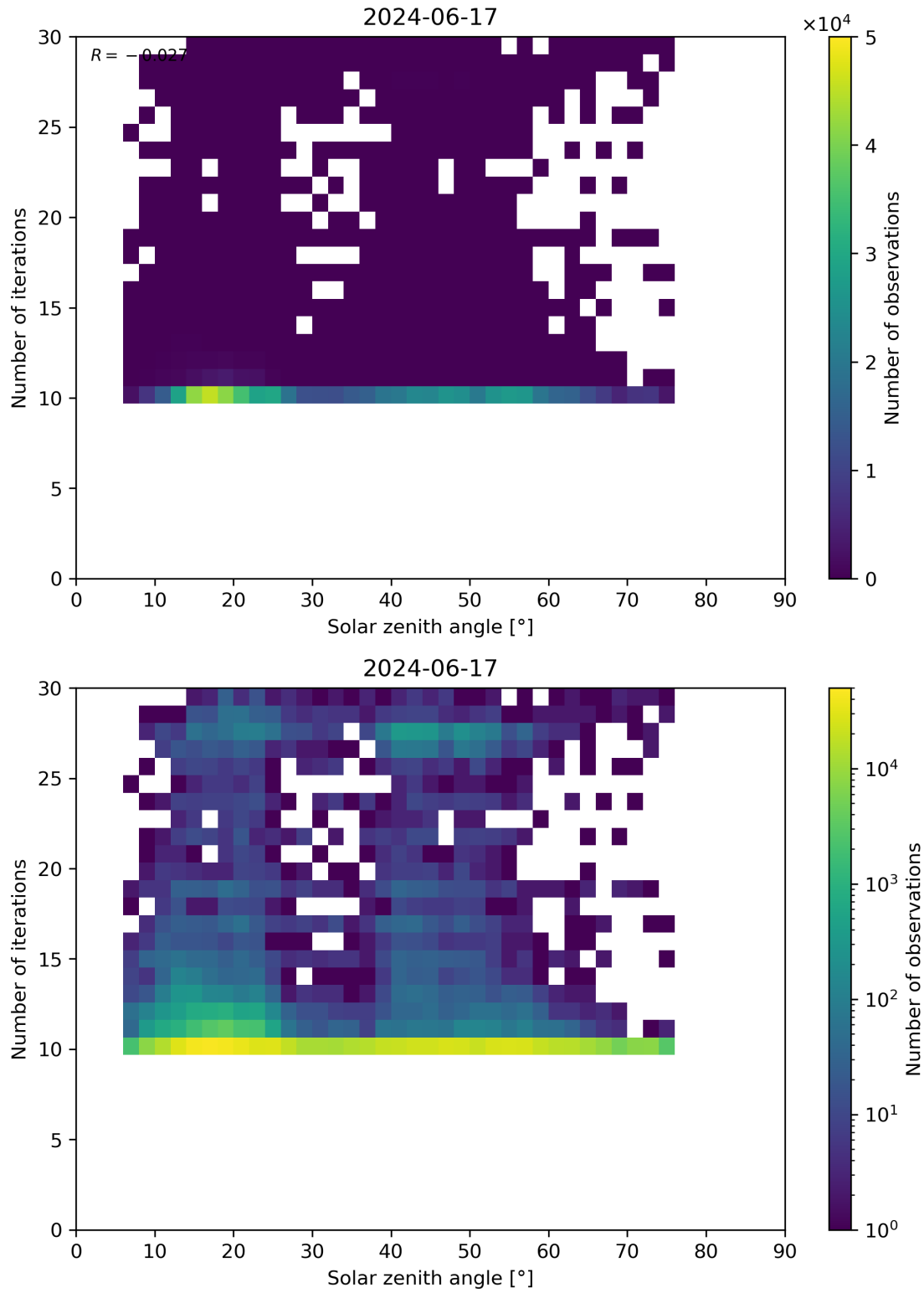
Figure 102: Scatter density plot of “Solar zenith angle” against “Number of iterations” for 2024-06-16 to 2024-06-18.
