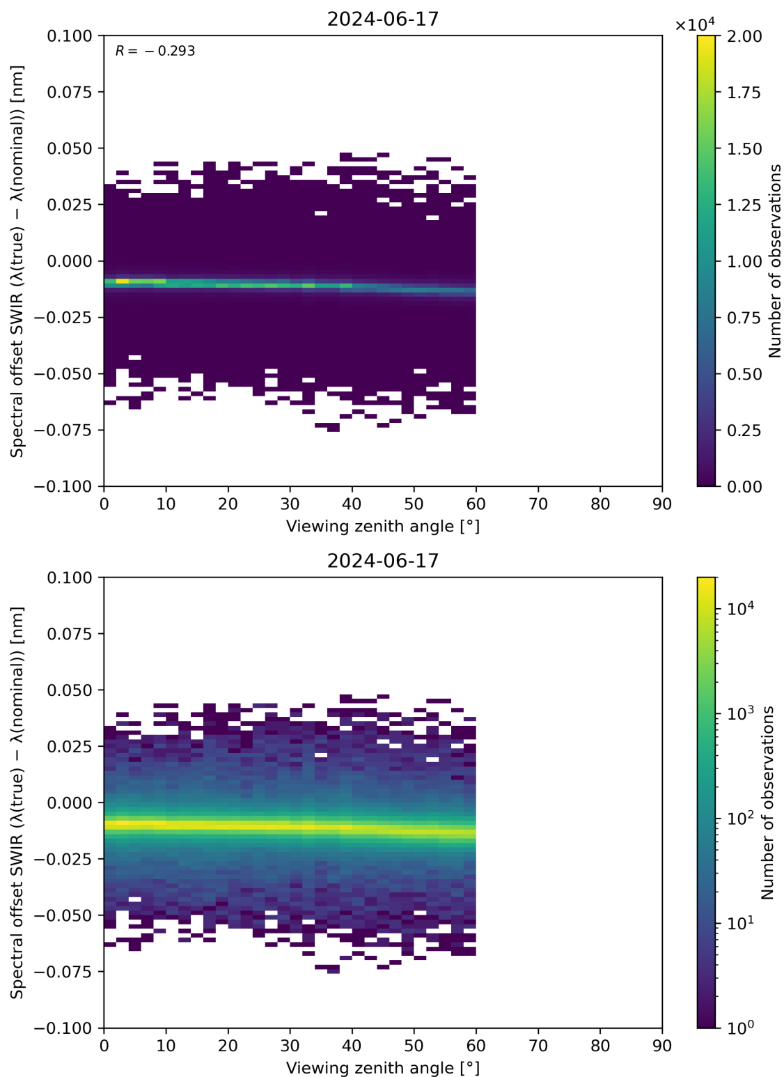
Figure 116: Scatter density plot of “Viewing zenith angle” against “Spectral offset SWIR ( \lambda(\text{true}) - \lambda(\text{nominal}) )” for 2024-06-16 to 2024-06-18.
