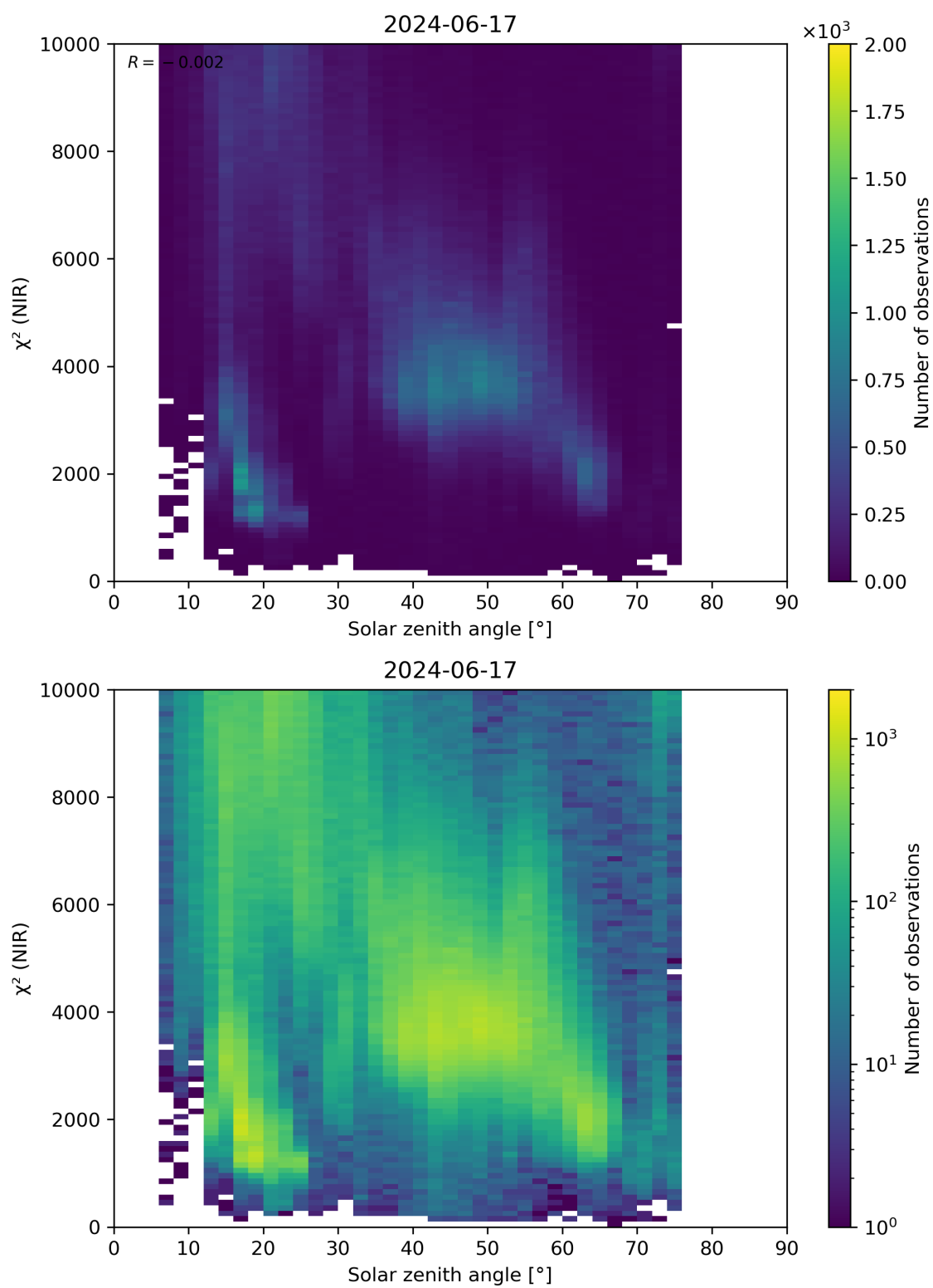
Figure 94: Scatter density plot of “Solar zenith angle” against “ \chi^2 (NIR)” for 2024-06-16 to 2024-06-18.
