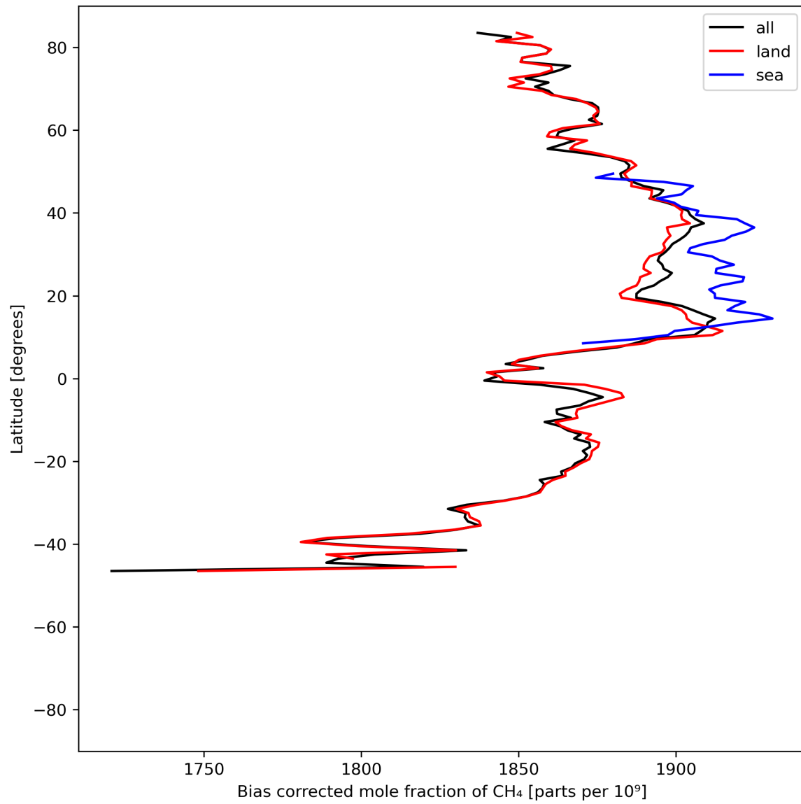
Figure 14: Zonal average of “Bias corrected mole fraction of CH 4 ” for 2024-06-16 to 2024-06-18.
