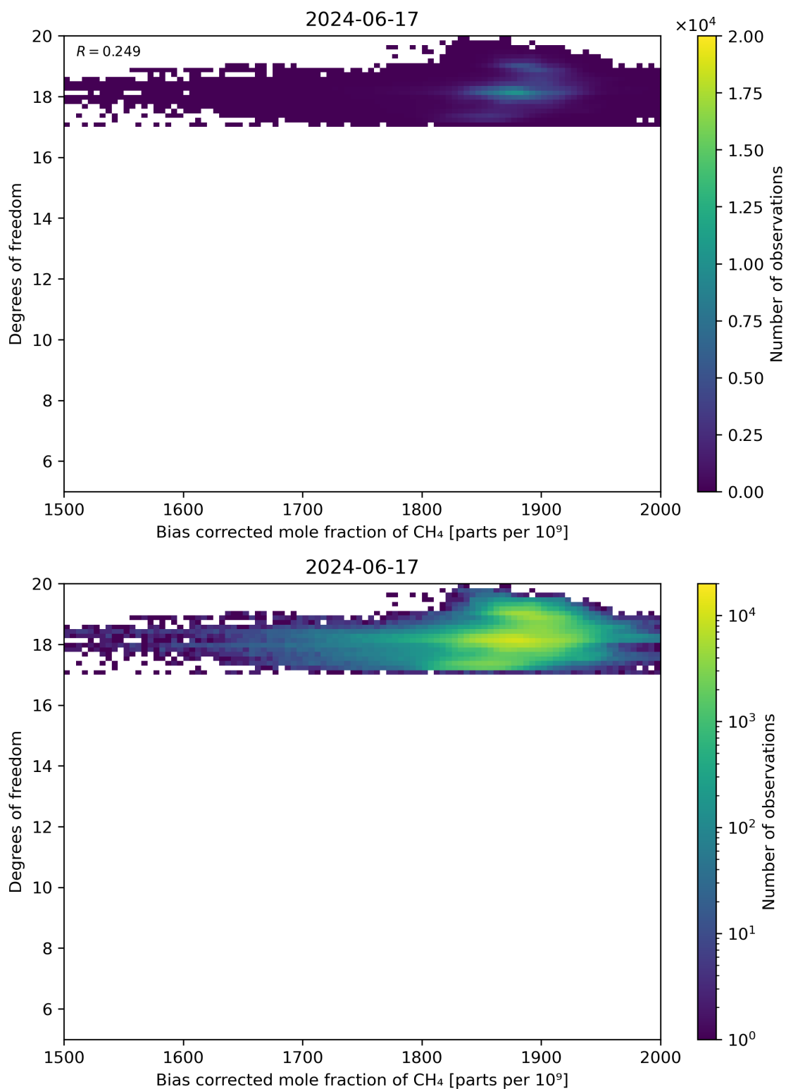
Figure 65: Scatter density plot of “Bias corrected mole fraction of CH 4 ” against “Degrees of freedom” for 2024-06-16 to 2024-06-18.
