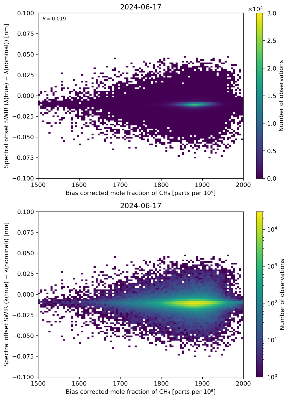
Figure 69: Scatter density plot of “Bias corrected mole fraction of \text{CH}_4 ” against “Spectral offset SWIR ( \lambda(\text{true}) - \lambda(\text{nominal}) )” for 2024-06-16 to 2024-06-18.
