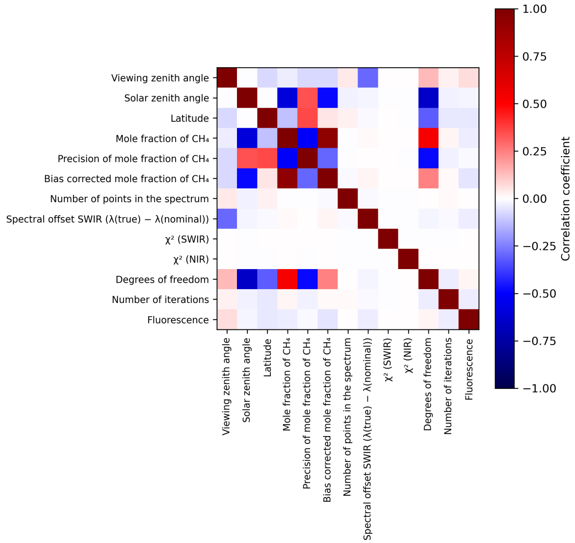
Figure 2: Map of correlation matrix for 2024-06-16 to 2024-06-18.
