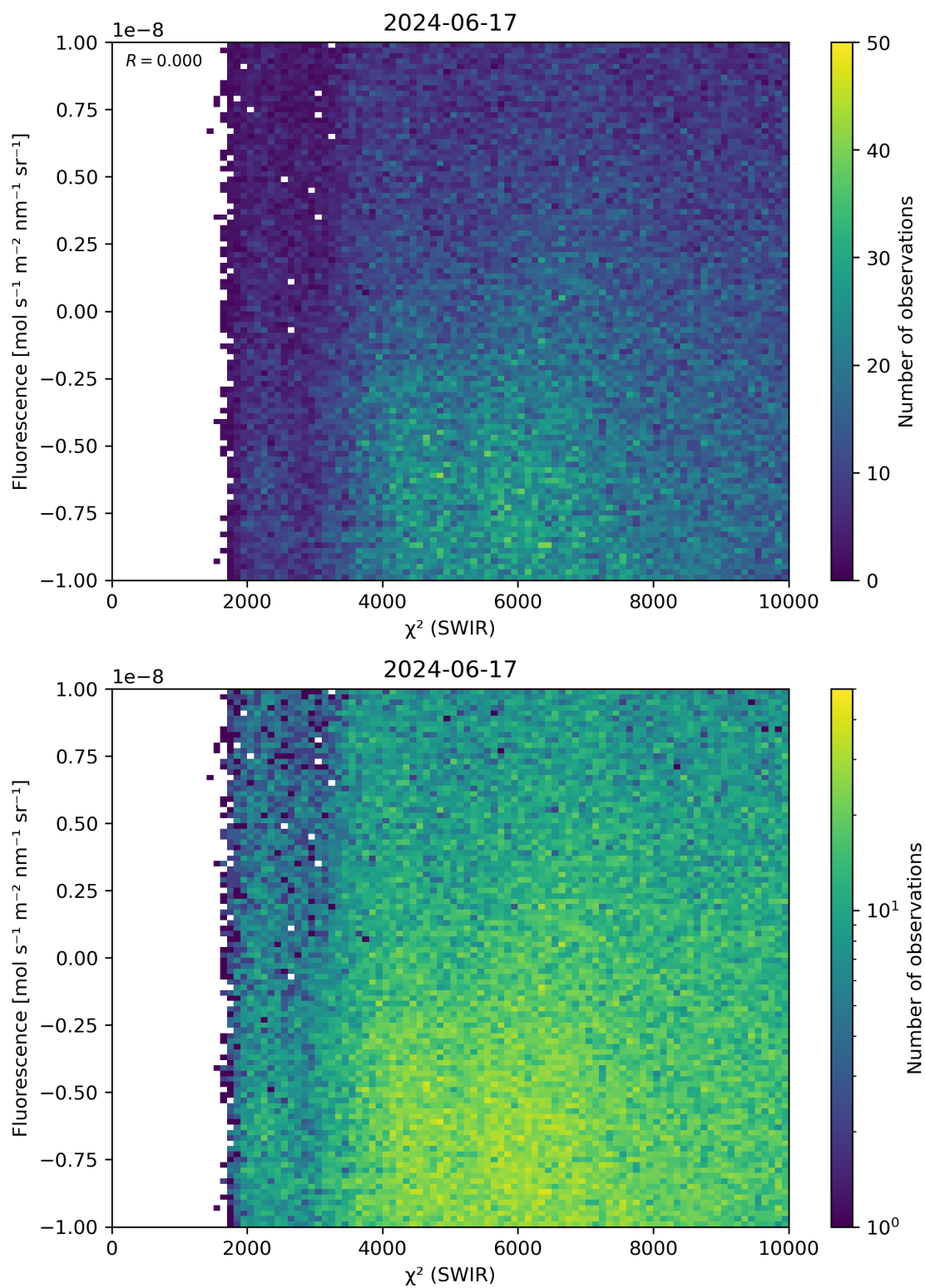
Figure 49: Scatter density plot of “ \chi^2 (SWIR)” against “Fluorescence” for 2024-06-16 to 2024-06-18.
