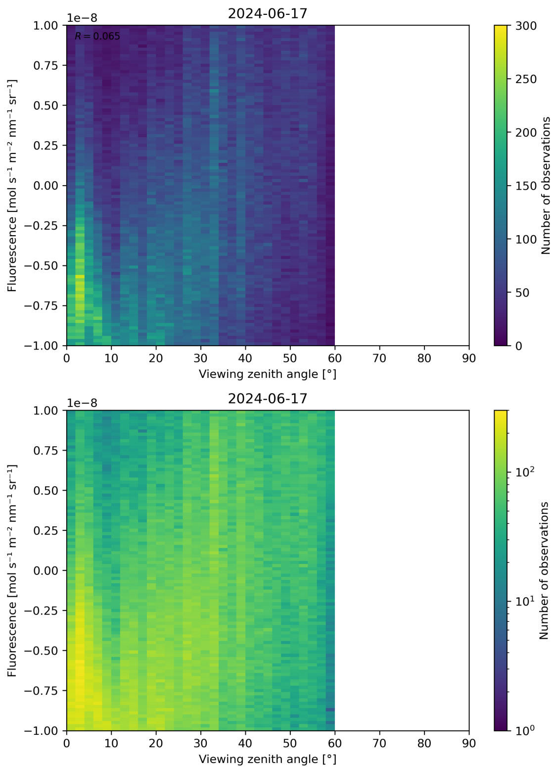
Figure 108: Scatter density plot of “Viewing zenith angle” against “Fluorescence” for 2024-06-16 to 2024-06-18.
