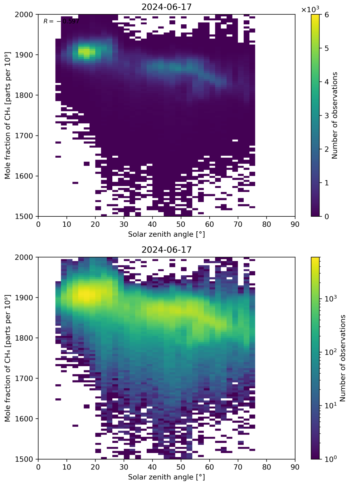
Figure 99: Scatter density plot of “Solar zenith angle” against “Mole fraction of \text{CH}_4 ” for 2024-06-16 to 2024-06-18.
