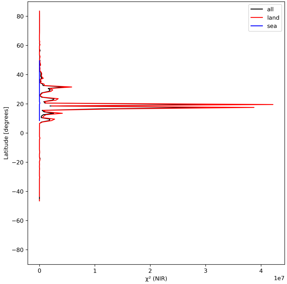
Figure 18: Zonal average of “ \chi^2 (NIR)” for 2024-06-16 to 2024-06-18.
