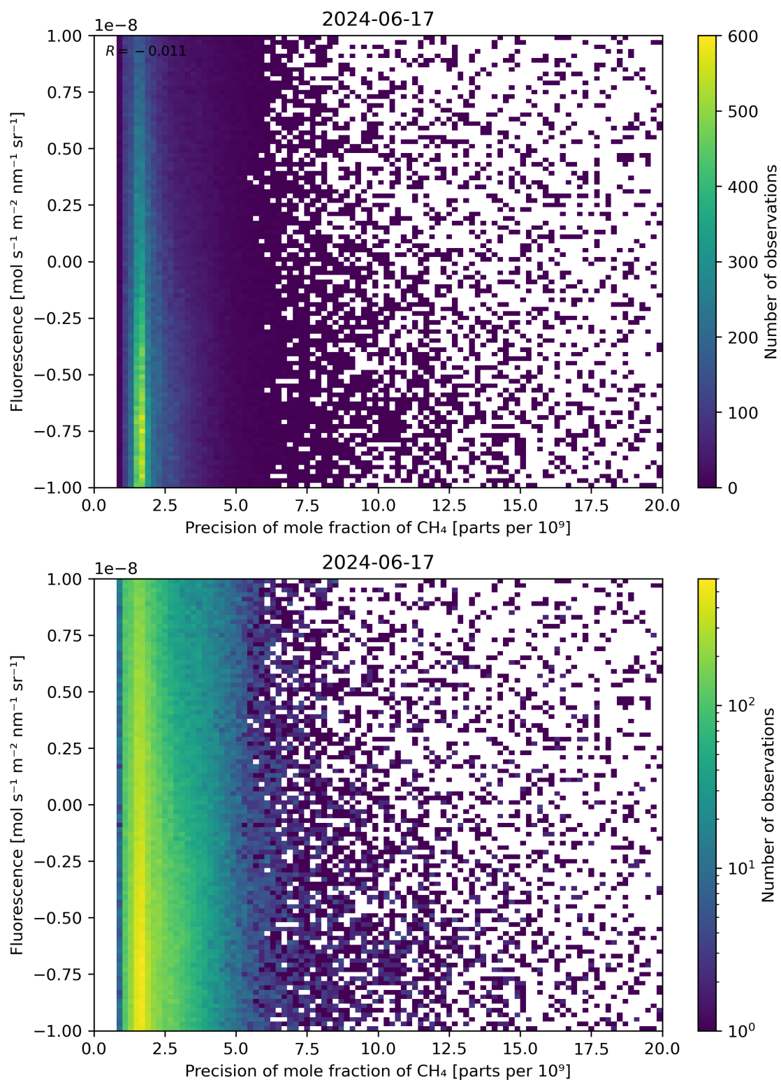
Figure 81: Scatter density plot of “Precision of mole fraction of CH 4 ” against “Fluorescence” for 2024-06-16 to 2024-06-18.
