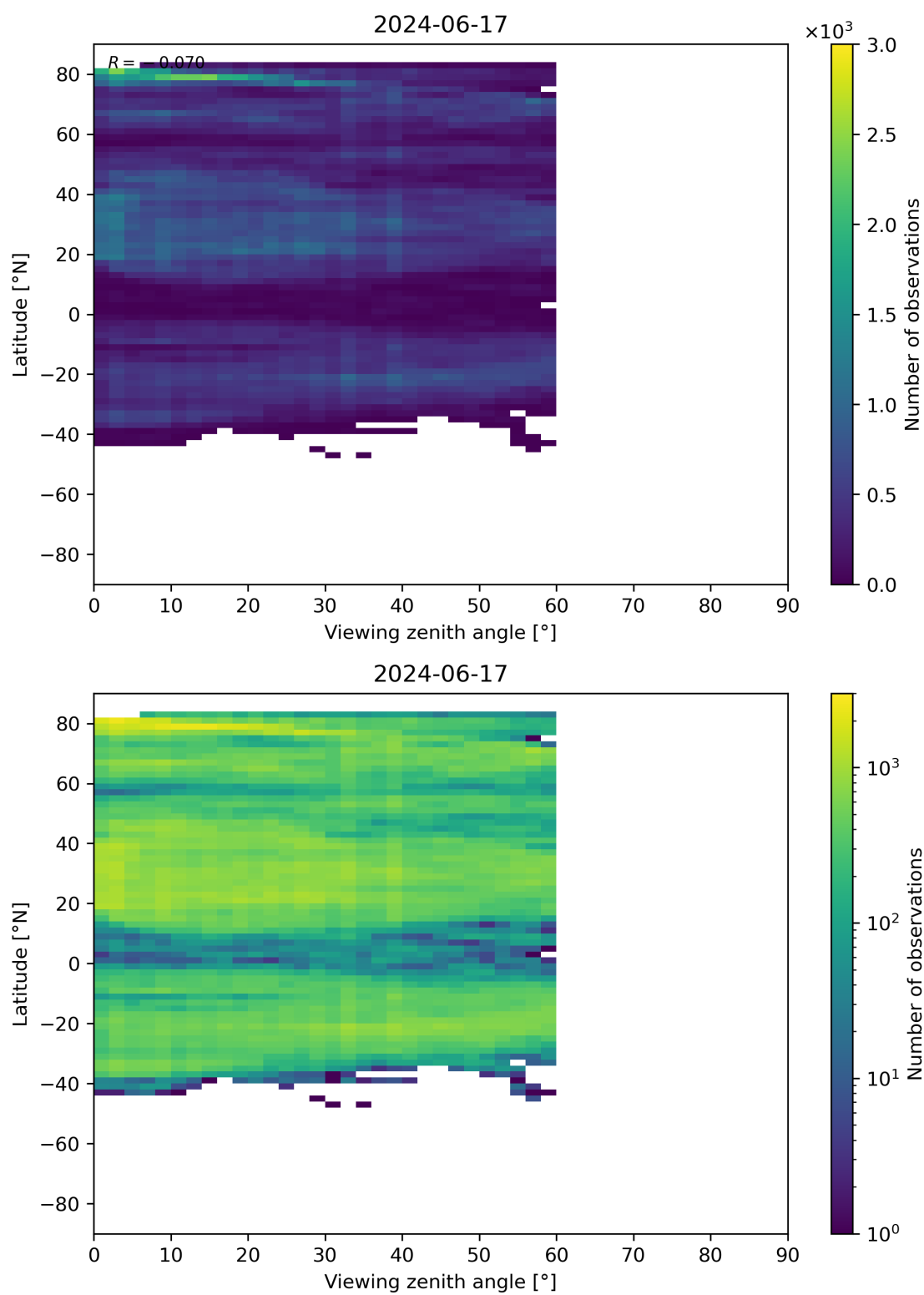
Figure 109: Scatter density plot of “Viewing zenith angle” against “Latitude” for 2024-06-16 to 2024-06-18.
