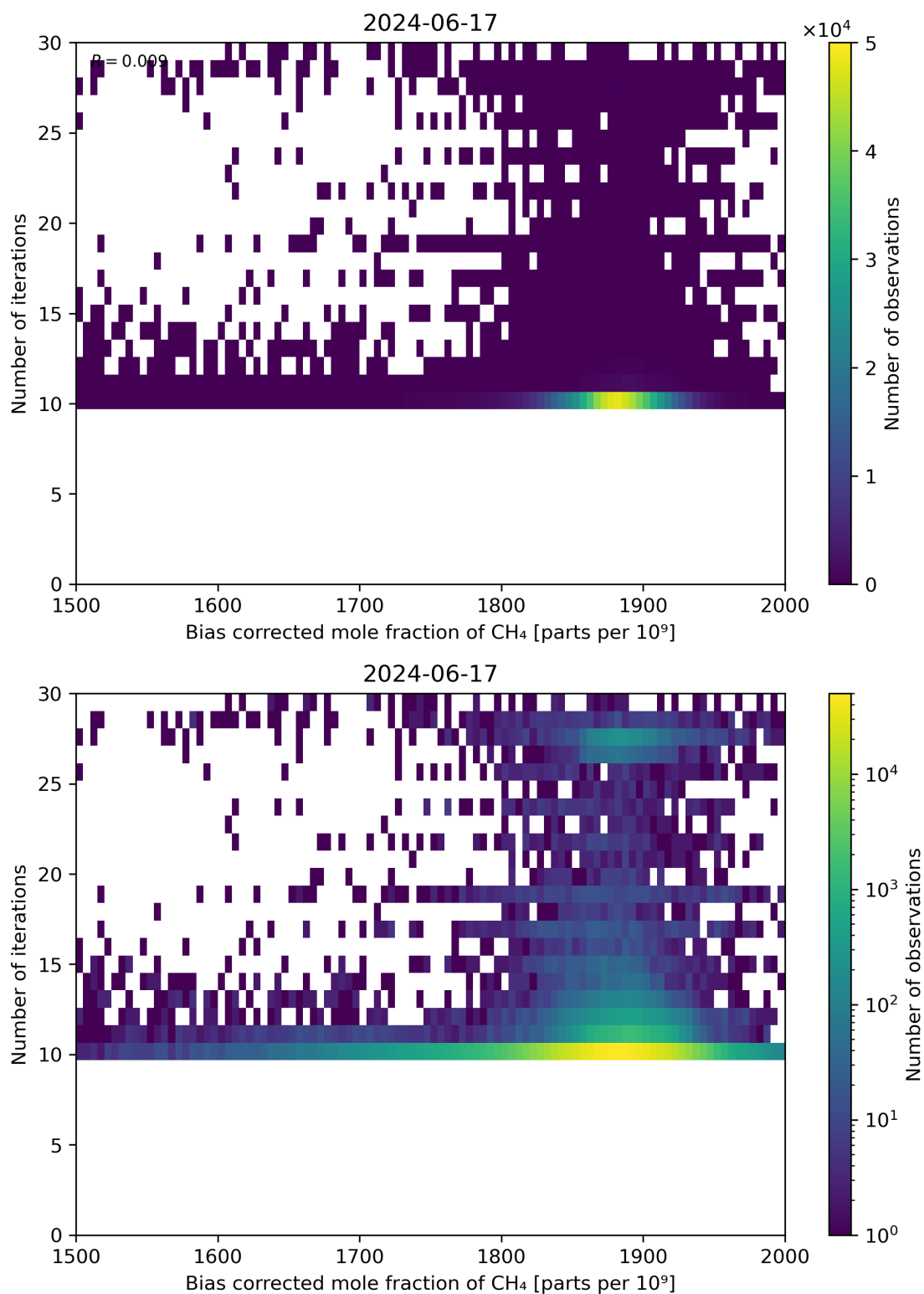
Figure 67: Scatter density plot of “Bias corrected mole fraction of CH 4 ” against “Number of iterations” for 2024-06-16 to 2024-06-18.
