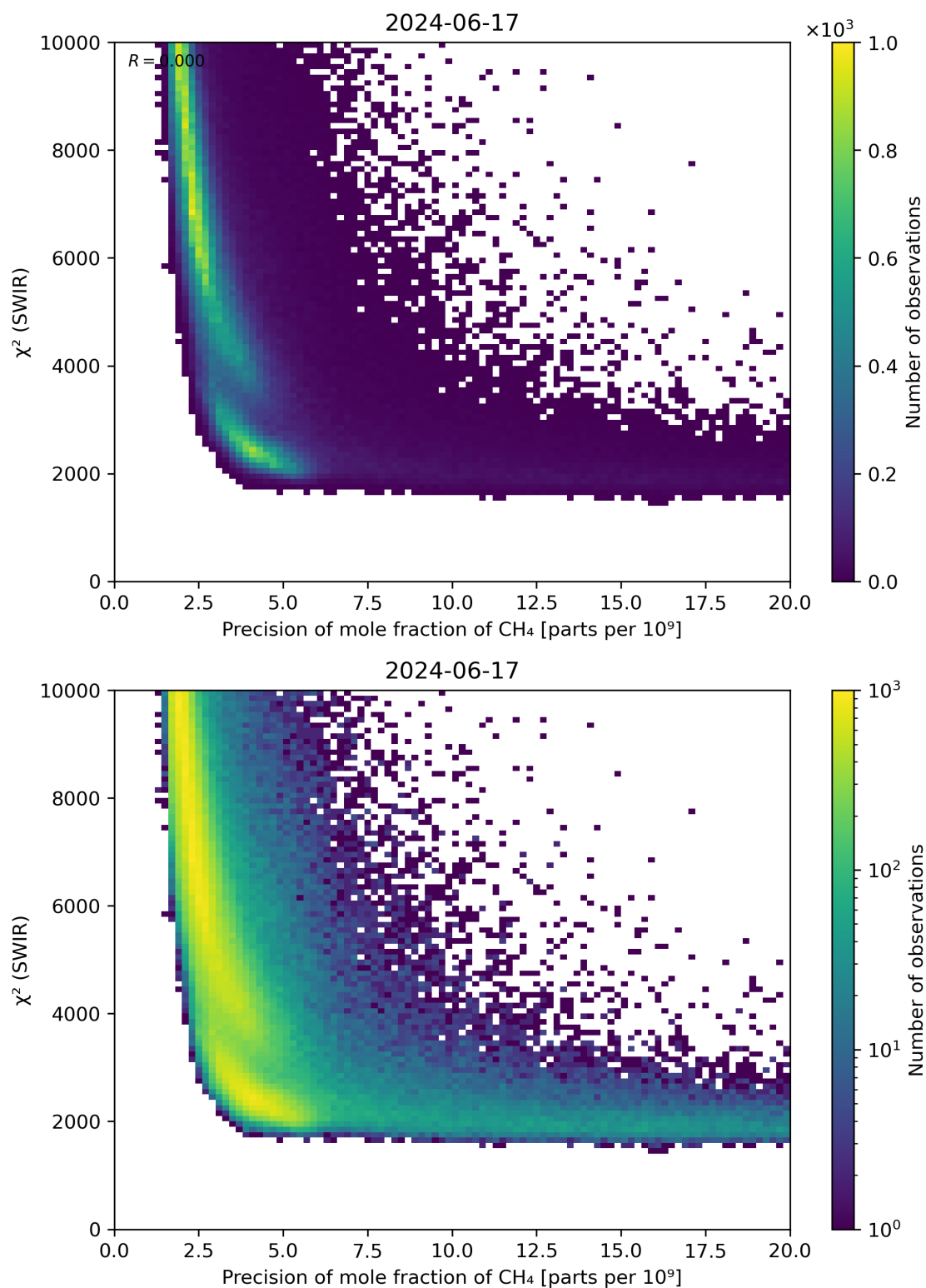
Figure 79: Scatter density plot of “Precision of mole fraction of CH 4 ” against “ \chi^2 (SWIR)” for 2024-06-16 to 2024-06-18.
