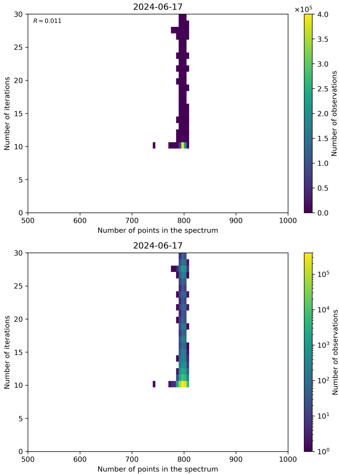
Figure 92: Scatter density plot of “Number of points in the spectrum” against “Number of iterations” for 2024-06-16 to 2024-06-18.
