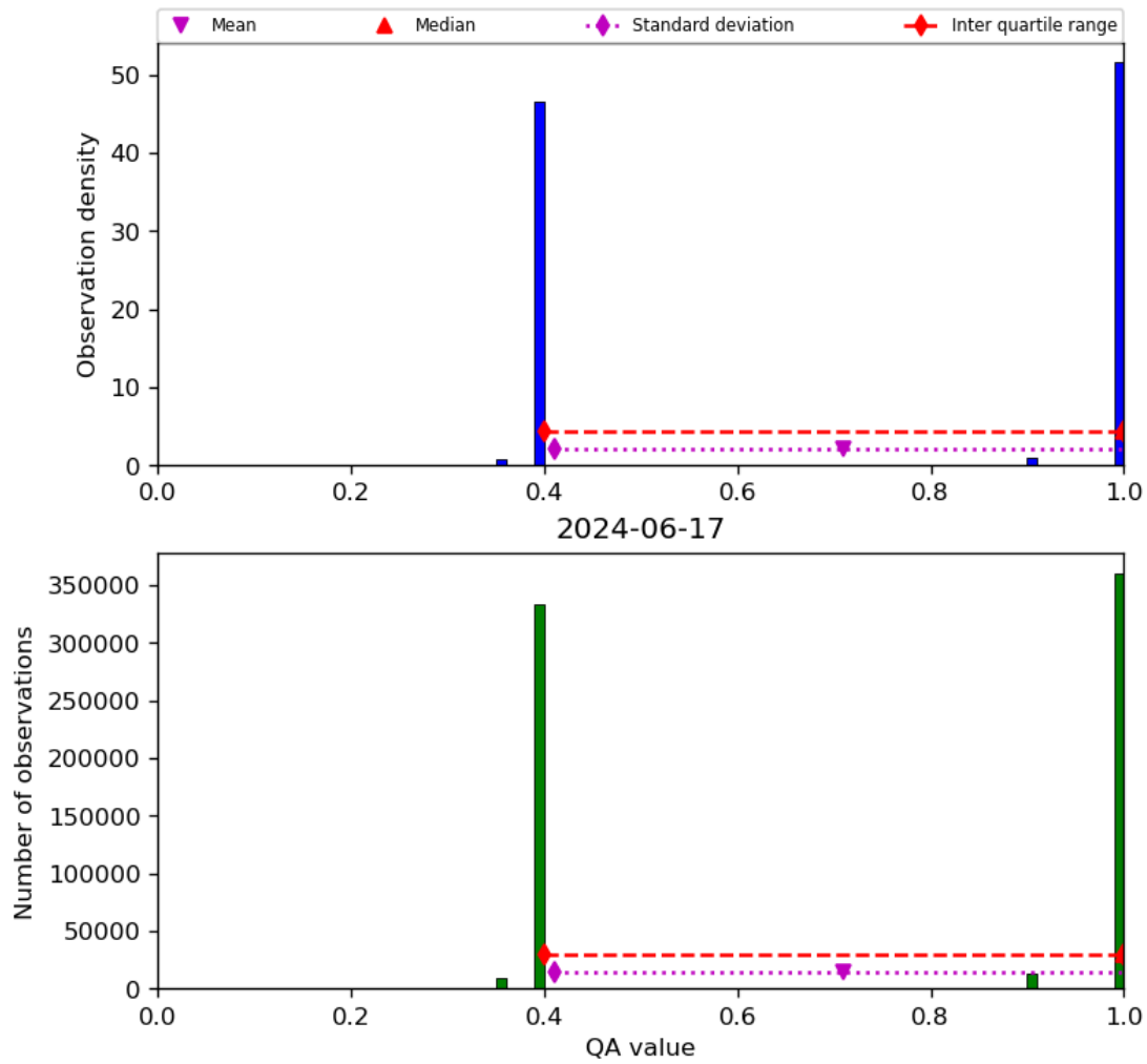
Figure 22: Histogram of “QA value” for 2024-06-16 to 2024-06-18
