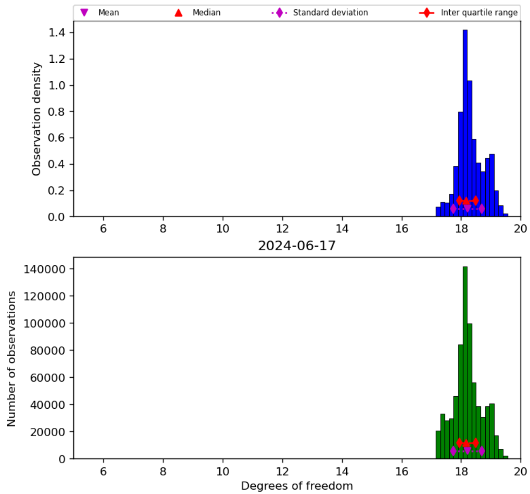
Figure 30: Histogram of “Degrees of freedom” for 2024-06-16 to 2024-06-18
