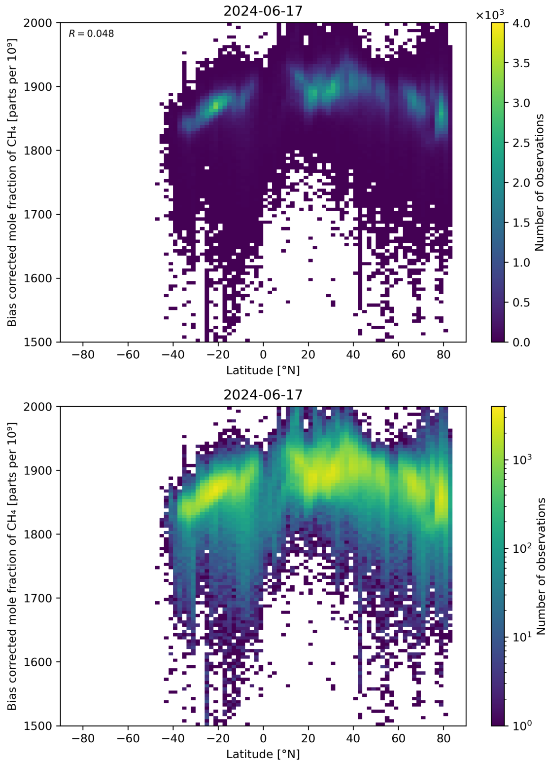
Figure 58: Scatter density plot of “Latitude” against “Bias corrected mole fraction of CH 4 ” for 2024-06-16 to 2024-06-18.
