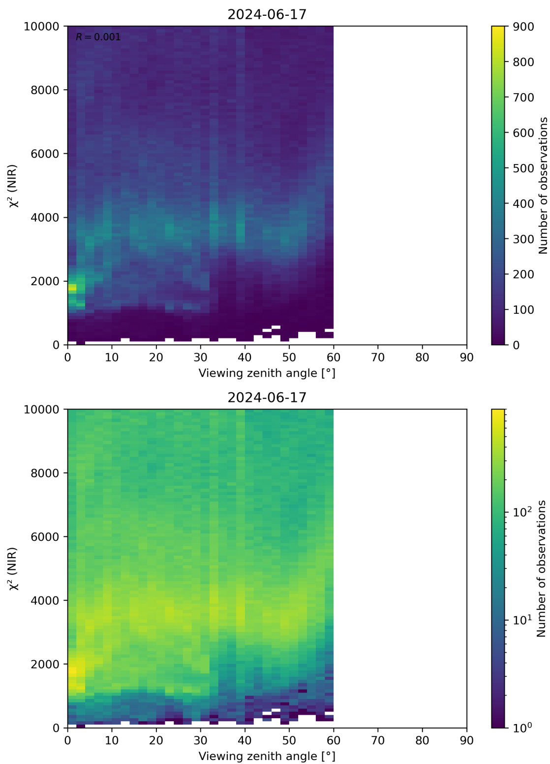
Figure 105: Scatter density plot of “Viewing zenith angle” against “ \chi^2 (NIR)” for 2024-06-16 to 2024-06-18.
