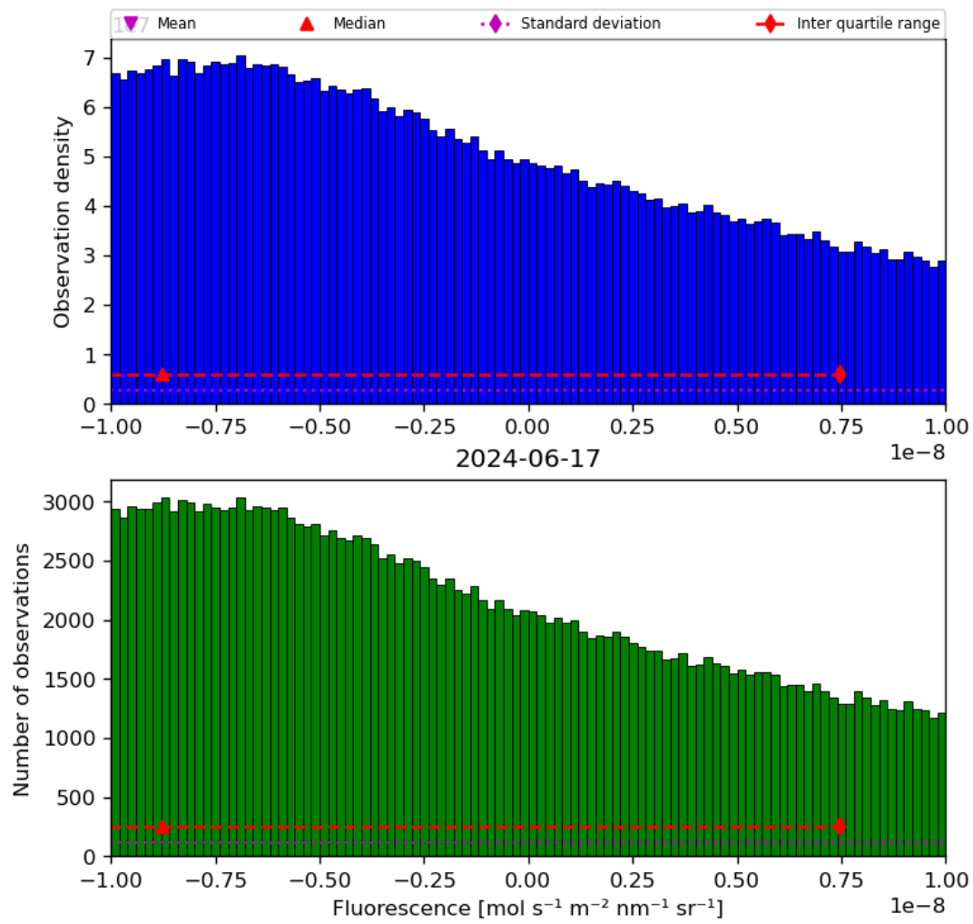
Figure 32: Histogram of “Fluorescence” for 2024-06-16 to 2024-06-18
