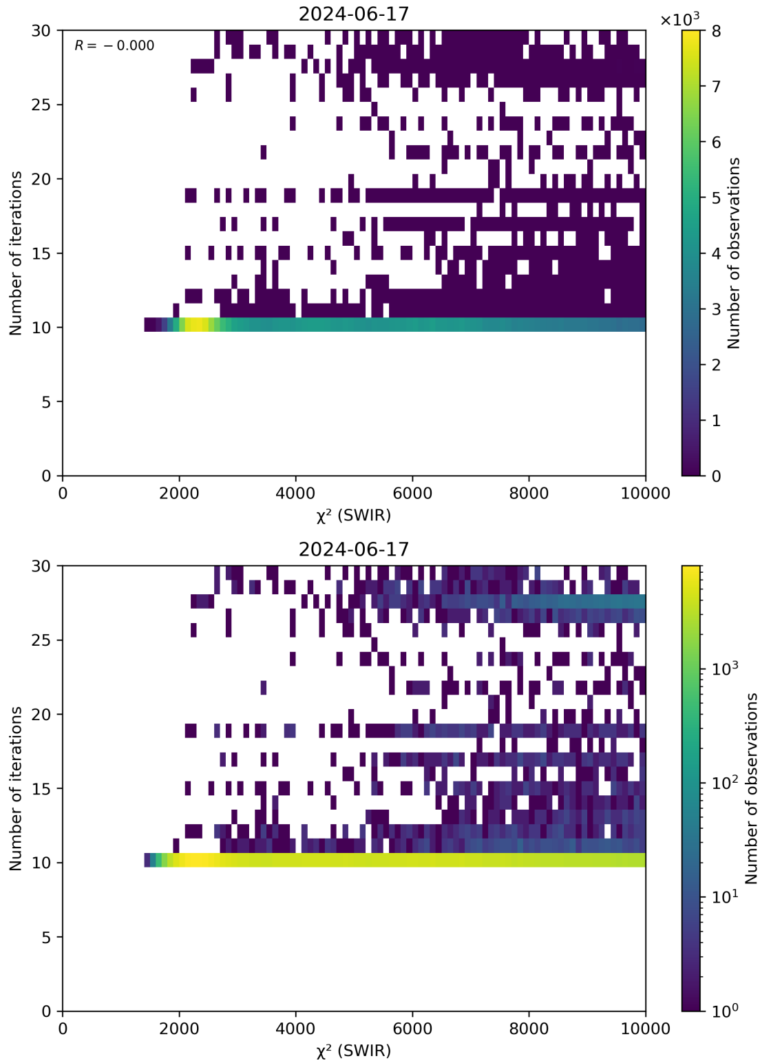
Figure 50: Scatter density plot of “ \chi^2 (SWIR)” against “Number of iterations” for 2024-06-16 to 2024-06-18.
