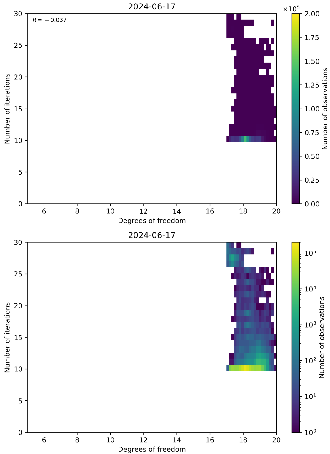
Figure 52: Scatter density plot of “Degrees of freedom” against “Number of iterations” for 2024-06-16 to 2024-06-18.
