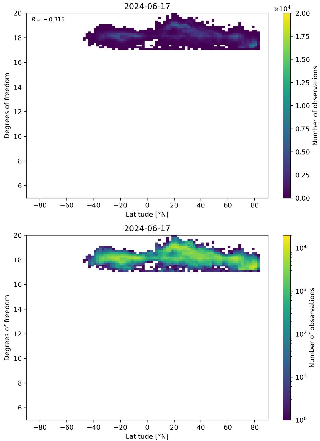
Figure 55: Scatter density plot of “Latitude” against “Degrees of freedom” for 2024-06-16 to 2024-06-18.
