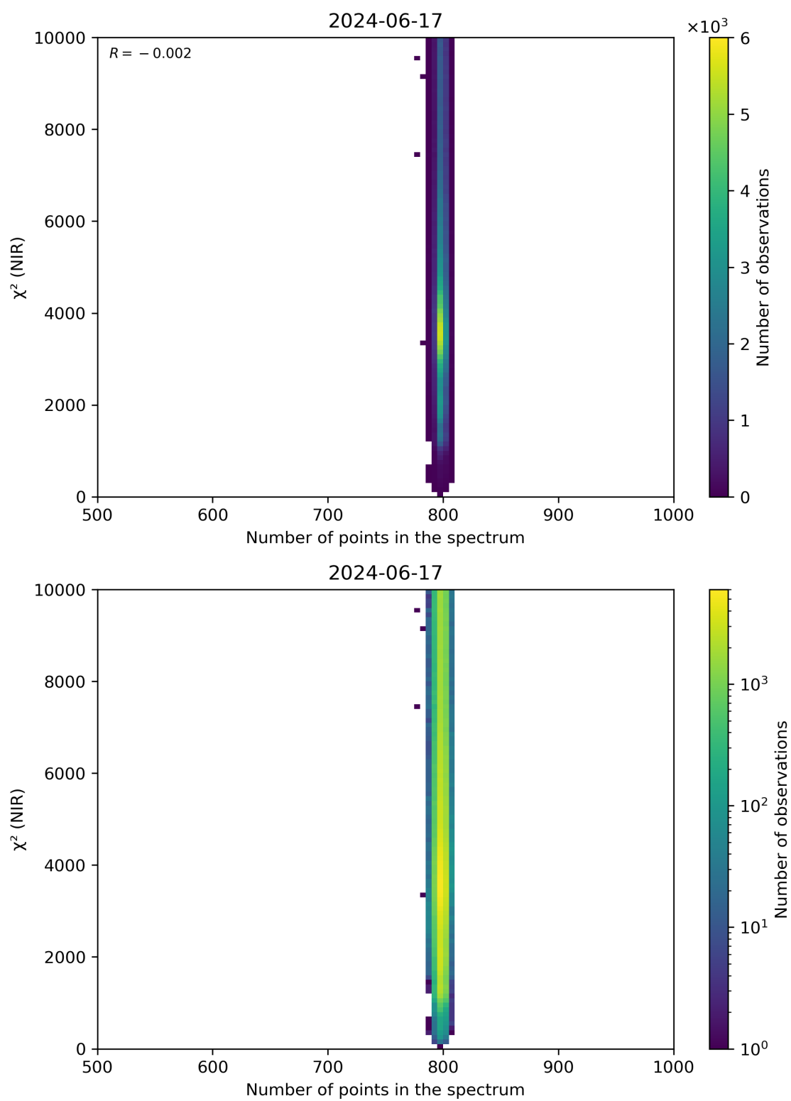
Figure 88: Scatter density plot of “Number of points in the spectrum” against “ \chi^2 (NIR)” for 2024-06-16 to 2024-06-18.
