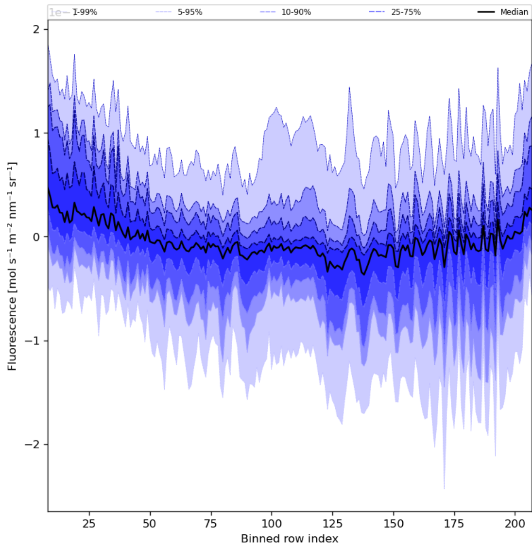
Figure 43: Along track statistics of “Fluorescence” for 2024-06-16 to 2024-06-18
