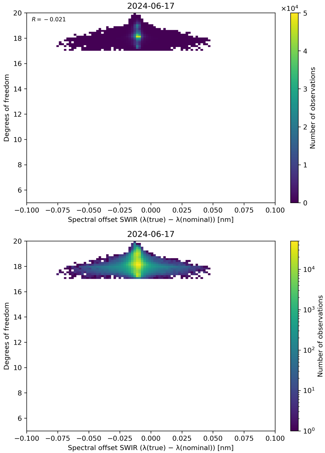
Figure 119: Scatter density plot of “Spectral offset SWIR ( \lambda(\text{true}) - \lambda(\text{nominal}) )” against “Degrees of freedom” for 2024-06-16 to 2024-06-18.
