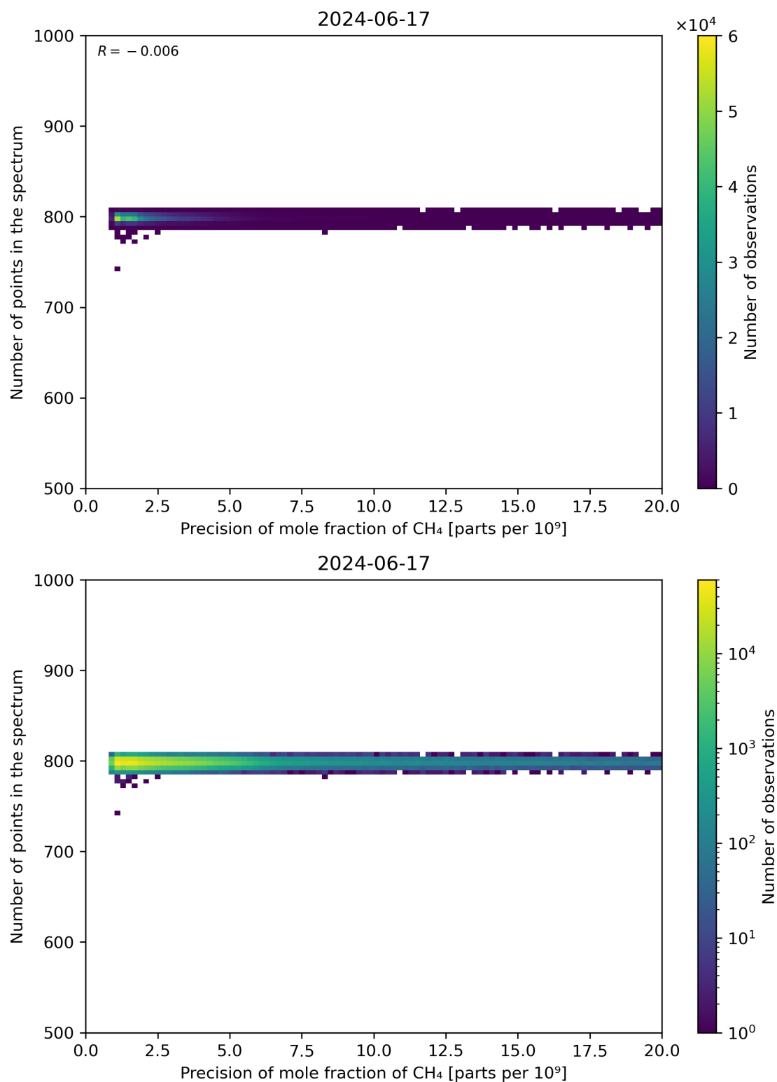
Figure 84: Scatter density plot of “Precision of mole fraction of CH 4 ” against “Number of points in the spectrum” for 2024-06-16 to 2024-06-18.
