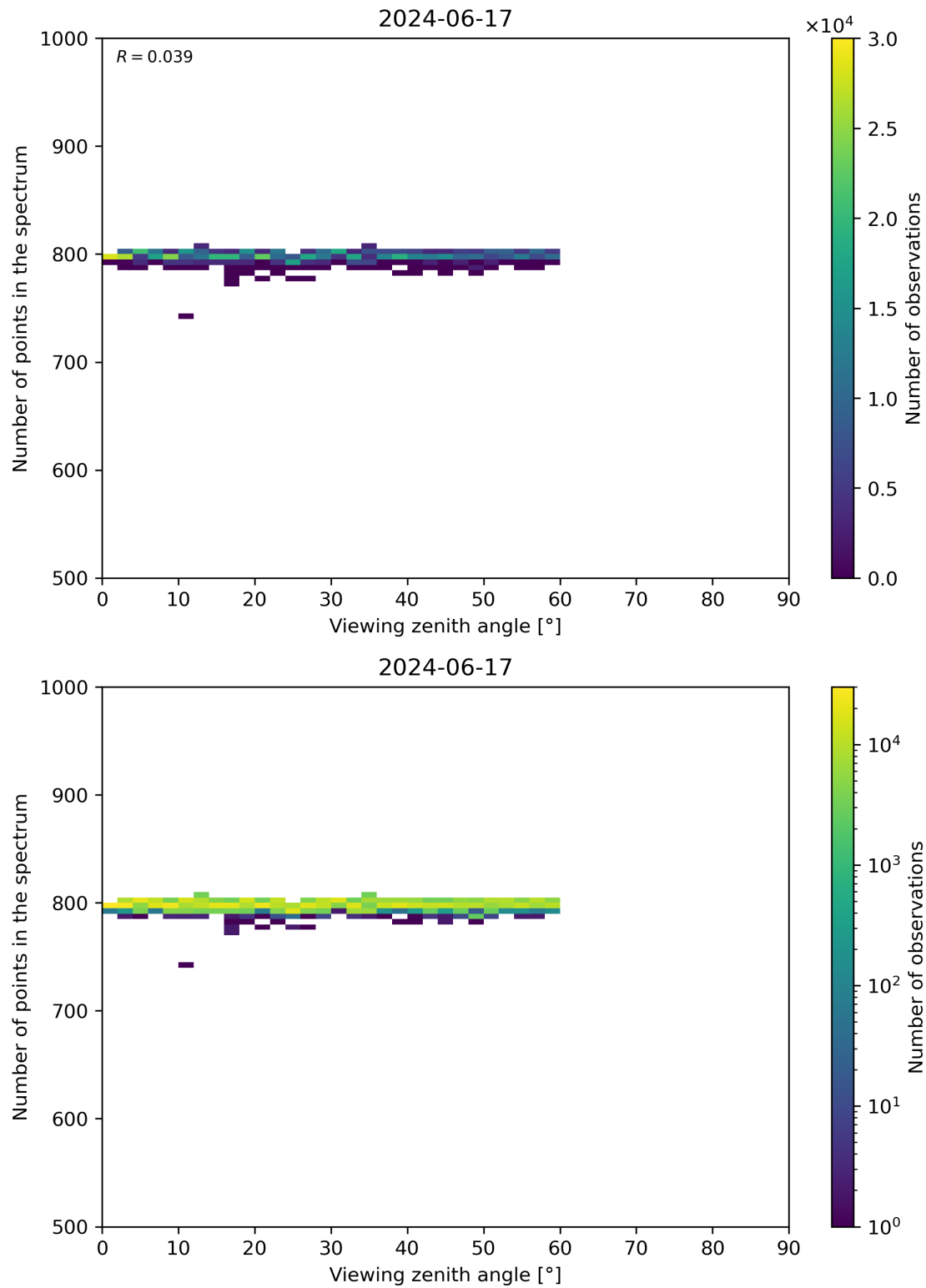
Figure 114: Scatter density plot of “Viewing zenith angle” against “Number of points in the spectrum” for 2024-06-16 to 2024-06-18.
