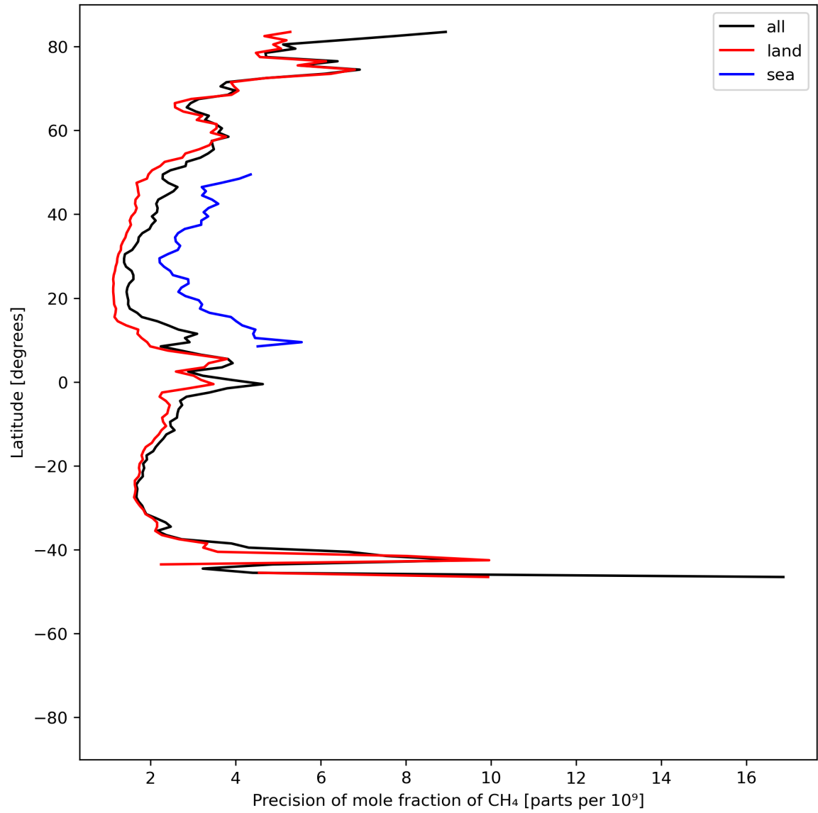
Figure 13: Zonal average of “Precision of mole fraction of CH 4 ” for 2024-06-16 to 2024-06-18.
