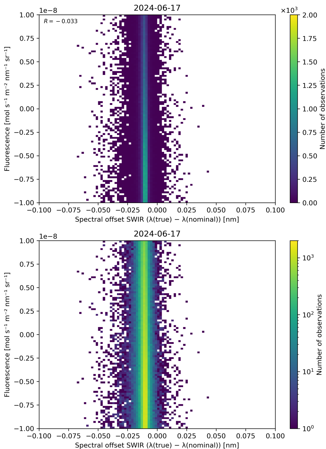
Figure 120: Scatter density plot of “Spectral offset SWIR ( \lambda(\text{true}) - \lambda(\text{nominal}) )” against “Fluorescence” for 2024-06-16 to 2024-06-18.
