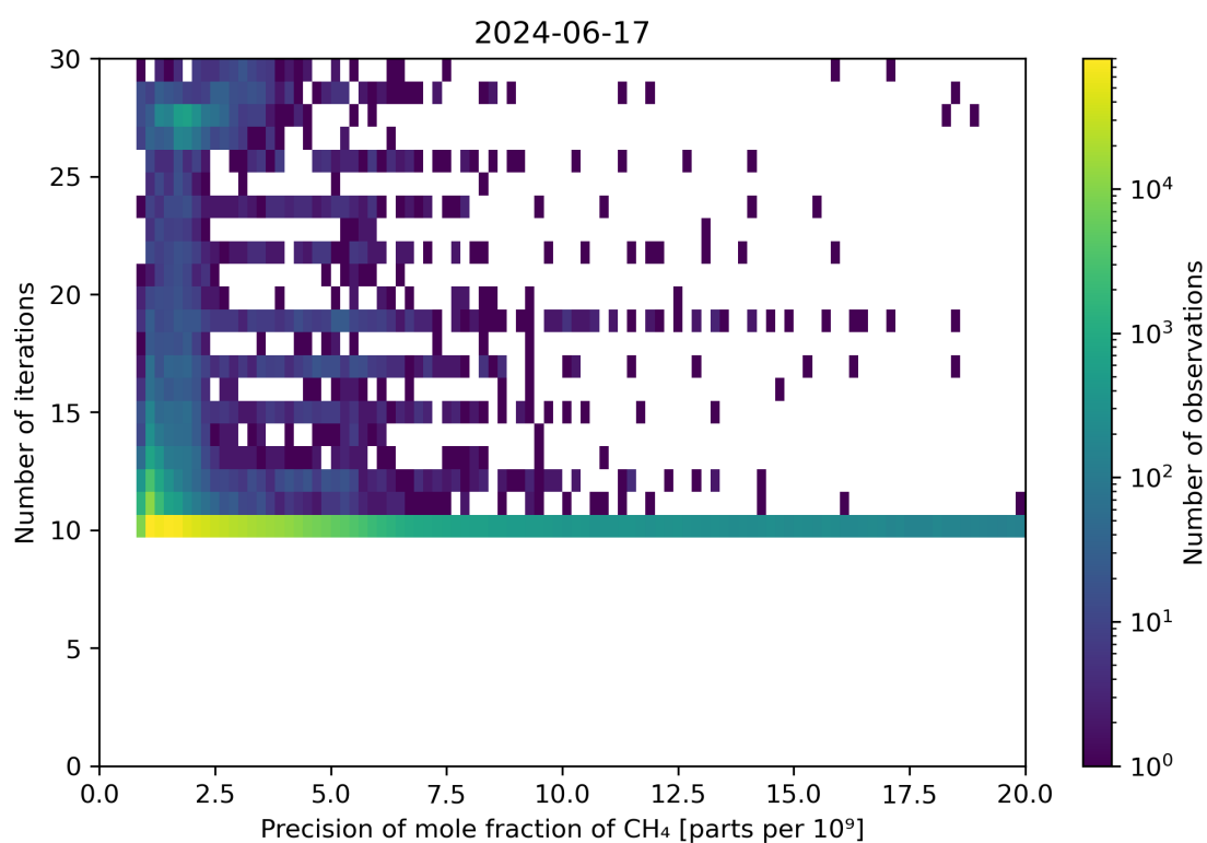
Figure 83: Scatter density plot of “Precision of mole fraction of CH 4 ” against “Number of iterations” for 2024-06-16 to 2024-06-18.
