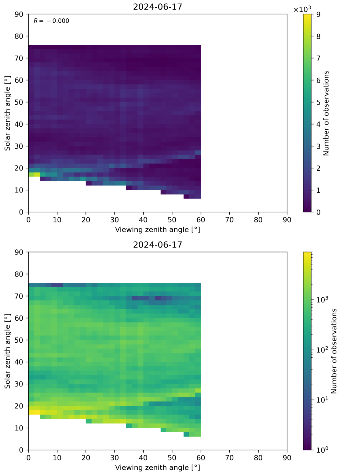
Figure 115: Scatter density plot of “Viewing zenith angle” against “Solar zenith angle” for 2024-06-16 to 2024-06-18.
