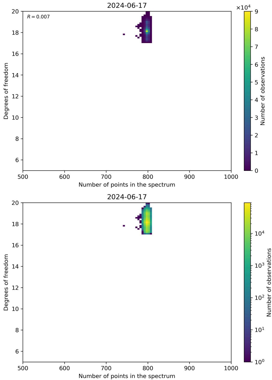
Figure 90: Scatter density plot of “Number of points in the spectrum” against “Degrees of freedom” for 2024-06-16 to 2024-06-18.
