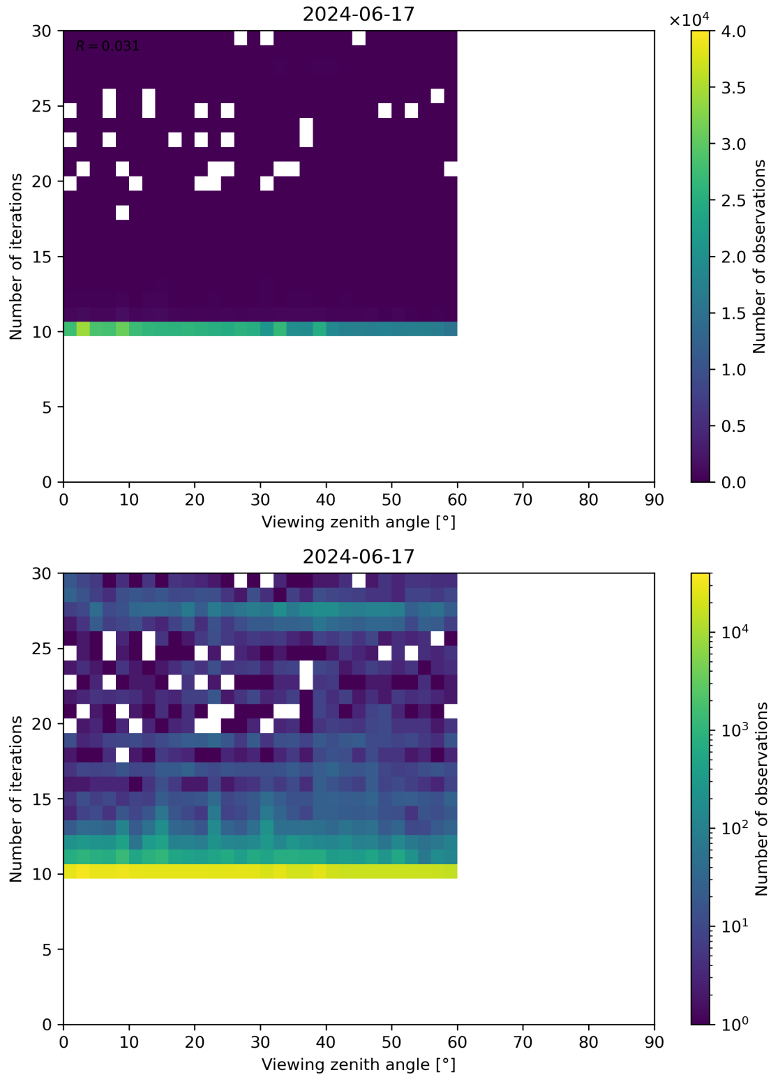
Figure 113: Scatter density plot of “Viewing zenith angle” against “Number of iterations” for 2024-06-16 to 2024-06-18.
