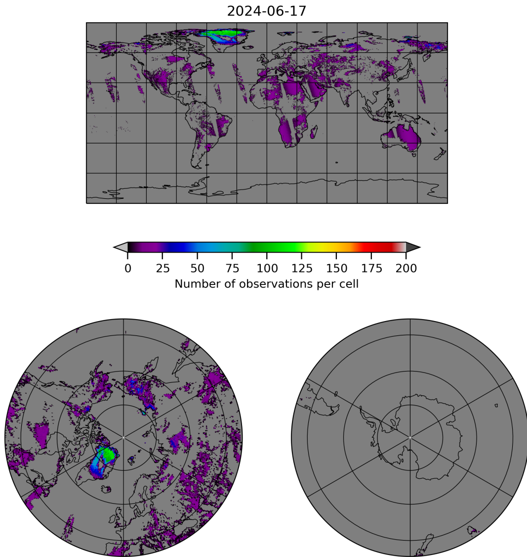
Figure 10: Map of the number of observations for 2024-06-16 to 2024-06-18
