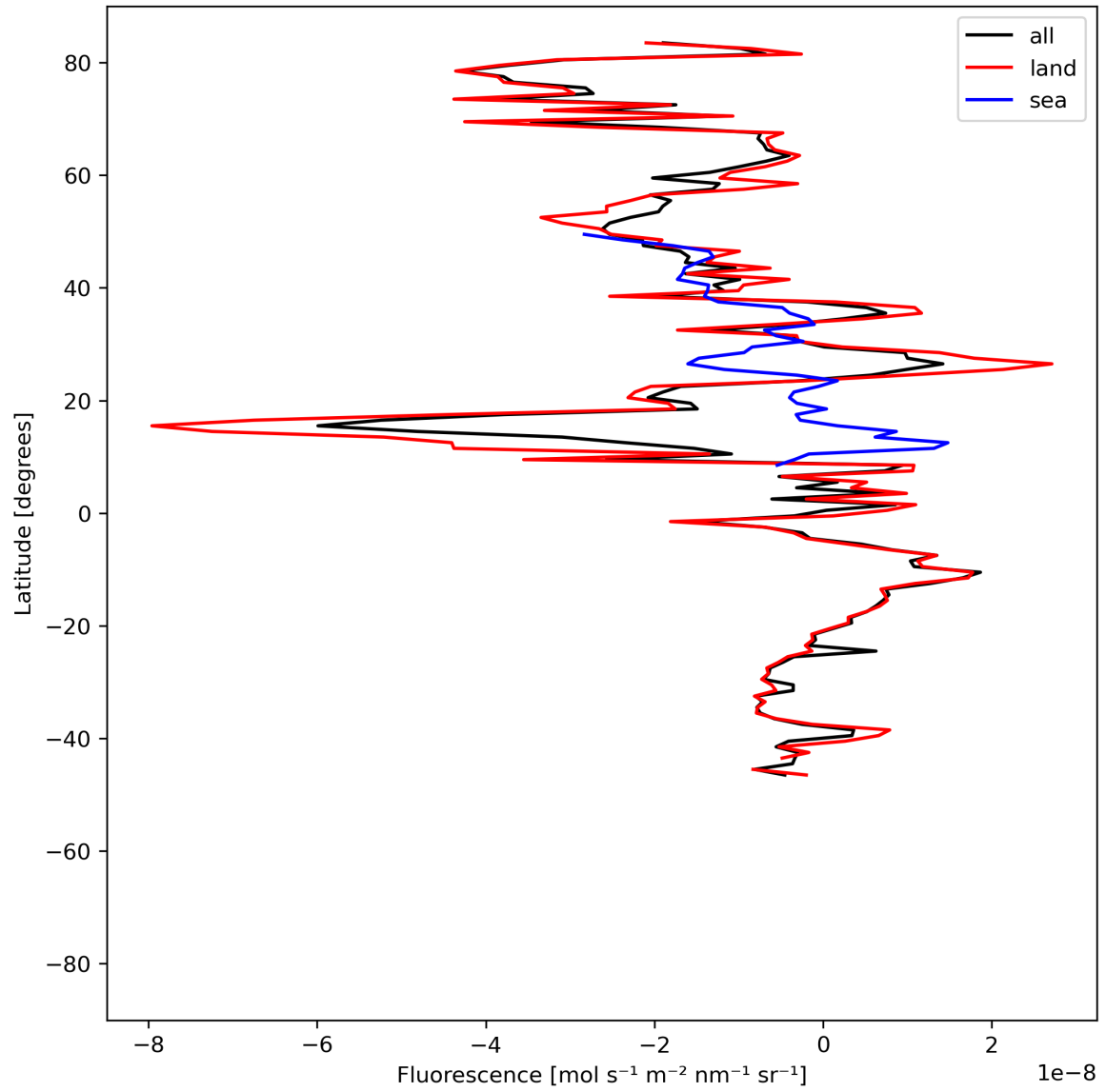
Figure 21: Zonal average of “Fluorescence” for 2024-06-16 to 2024-06-18.
