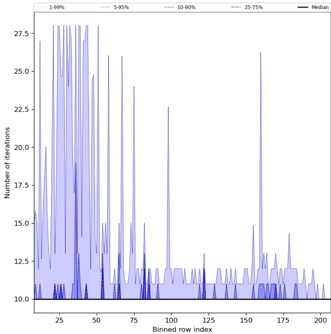
Figure 42: Along track statistics of “Number of iterations” for 2024-06-16 to 2024-06-18
