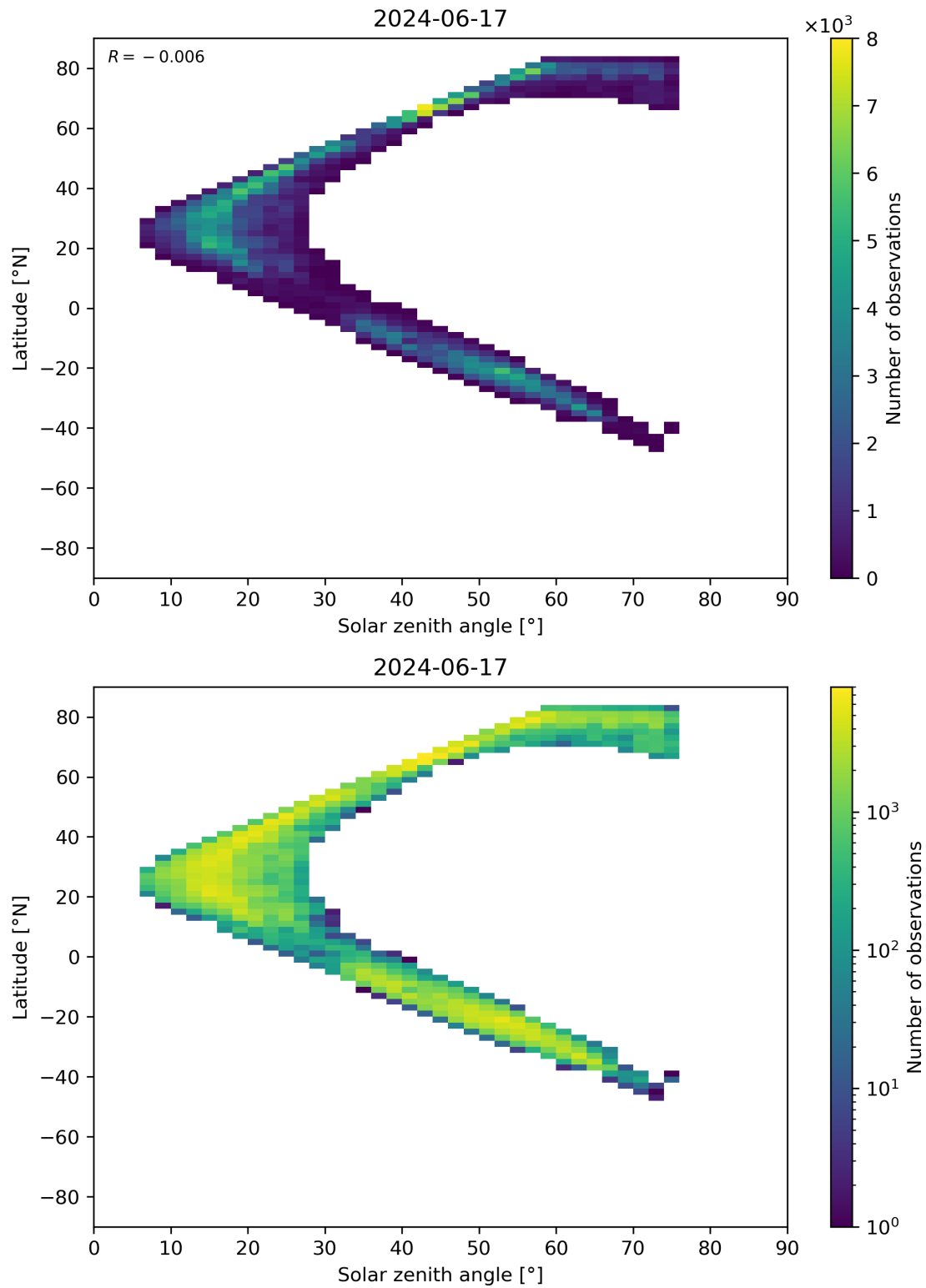
Figure 98: Scatter density plot of “Solar zenith angle” against “Latitude” for 2024-06-16 to 2024-06-18.
