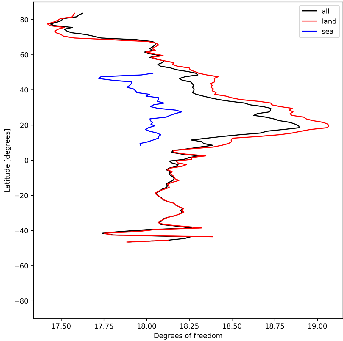
Figure 19: Zonal average of “Degrees of freedom” for 2024-06-16 to 2024-06-18.
