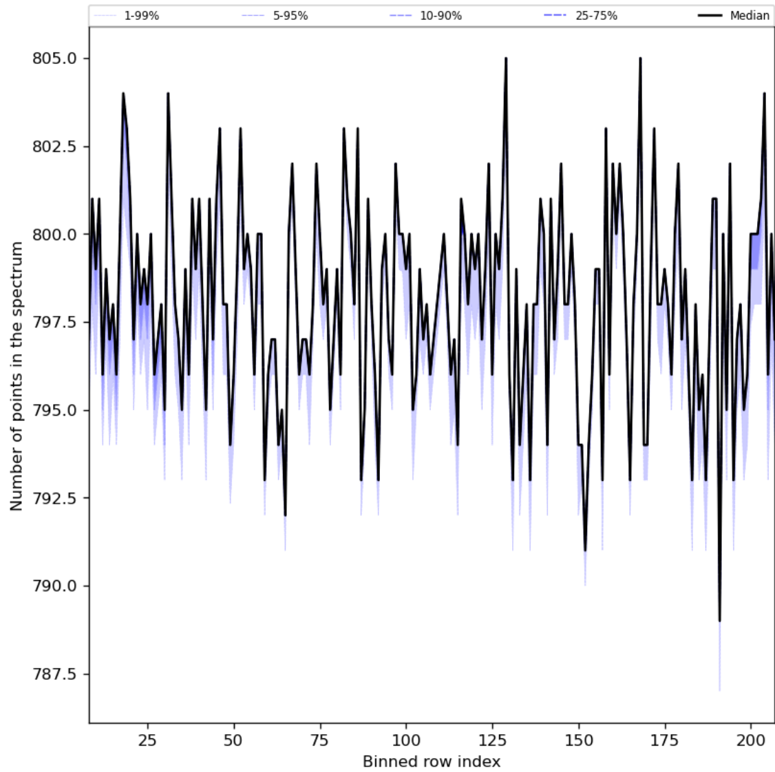
Figure 37: Along track statistics of “Number of points in the spectrum” for 2024-06-16 to 2024-06-18
