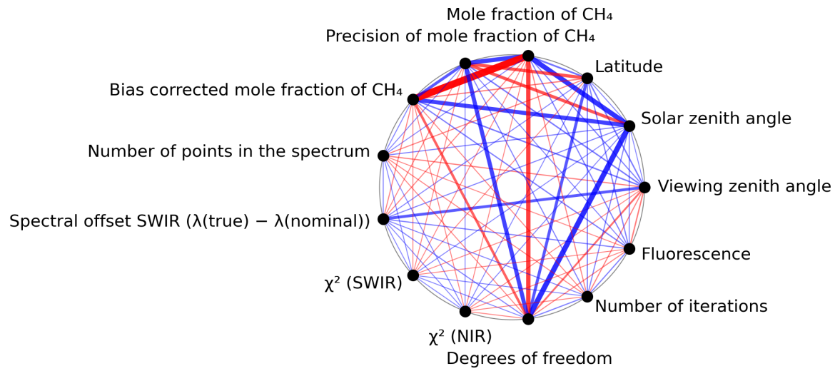
Figure 1: Map of correlation graph for 2024-06-16 to 2024-06-18.
