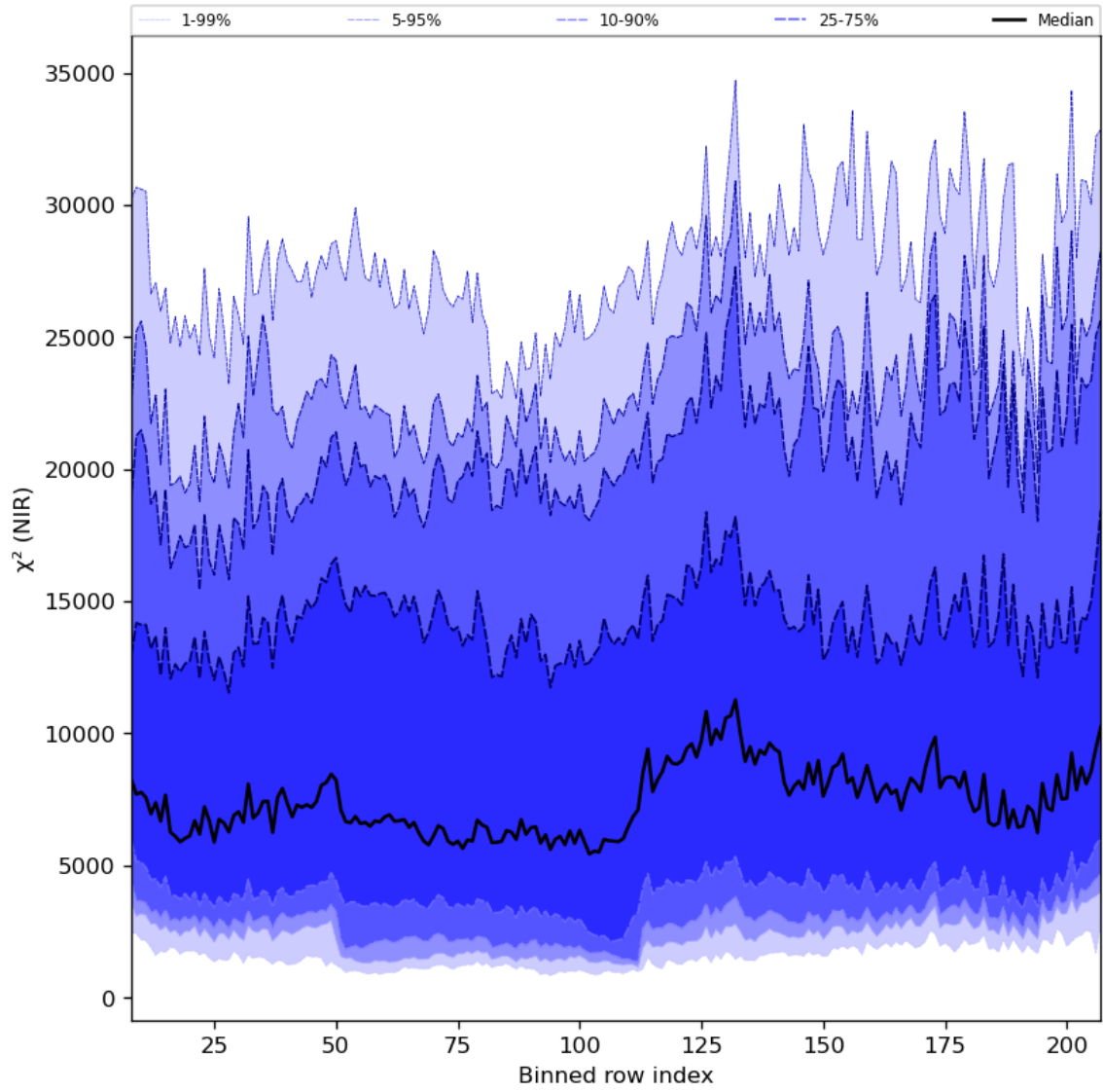
Figure 40: Along track statistics of “ \chi^2 (NIR)” for 2024-06-16 to 2024-06-18
