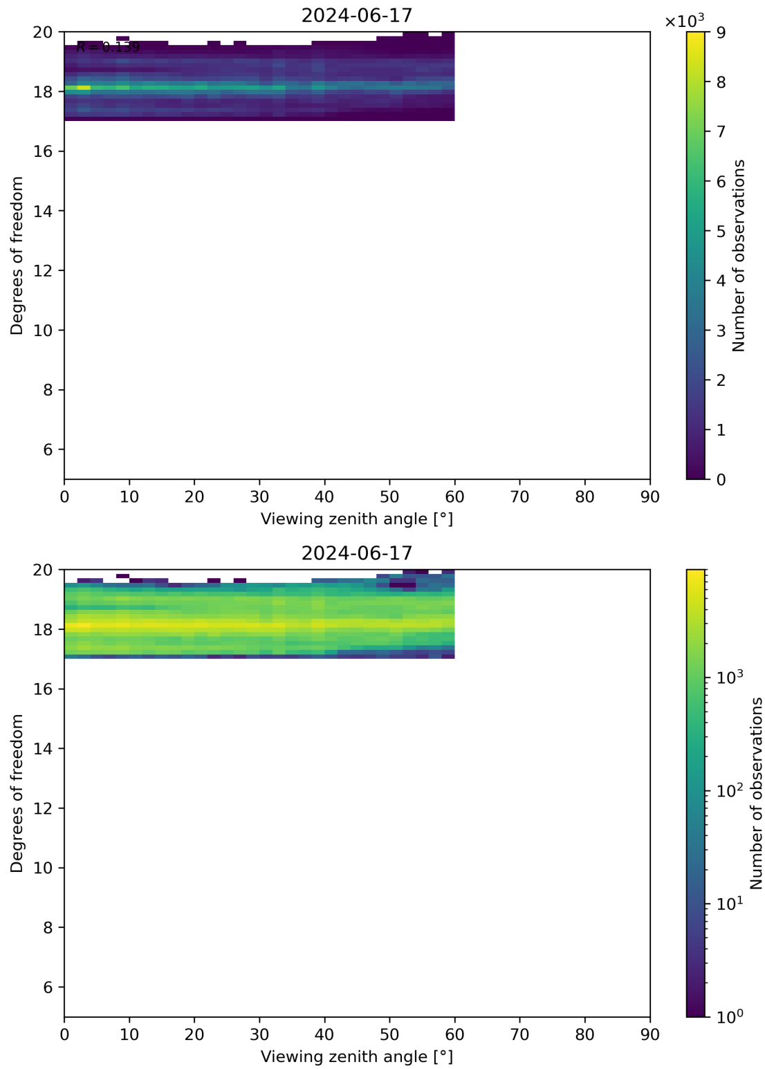
Figure 107: Scatter density plot of “Viewing zenith angle” against “Degrees of freedom” for 2024-06-16 to 2024-06-18.
