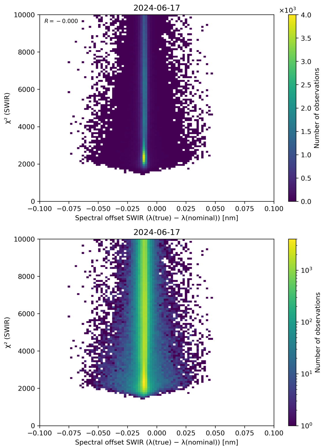
Figure 118: Scatter density plot of “Spectral offset SWIR ( \lambda(\text{true}) - \lambda(\text{nominal}) )” against “ \chi^2 (SWIR)” for 2024-06-16 to 2024-06-18.
