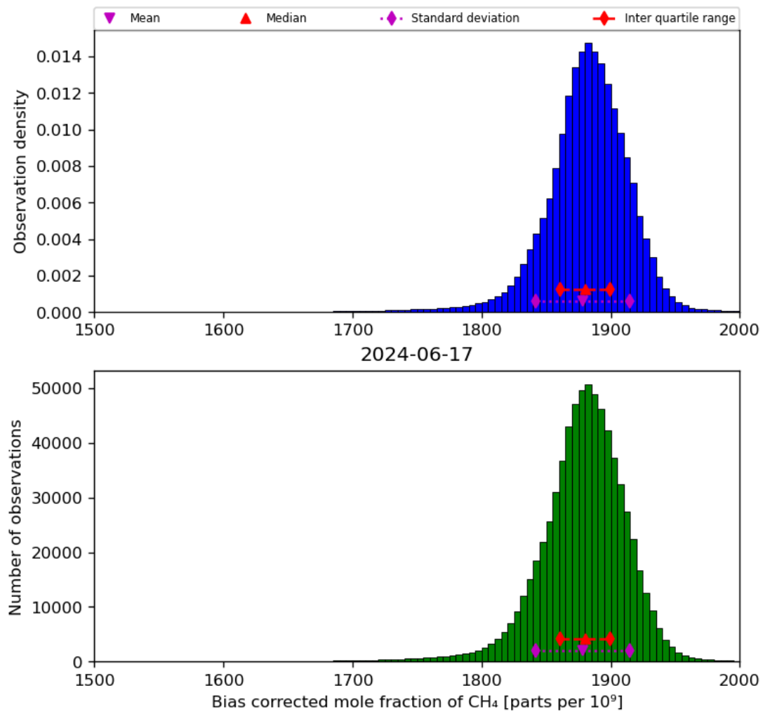
Figure 25: Histogram of “Bias corrected mole fraction of CH 4 ” for 2024-06-16 to 2024-06-18
