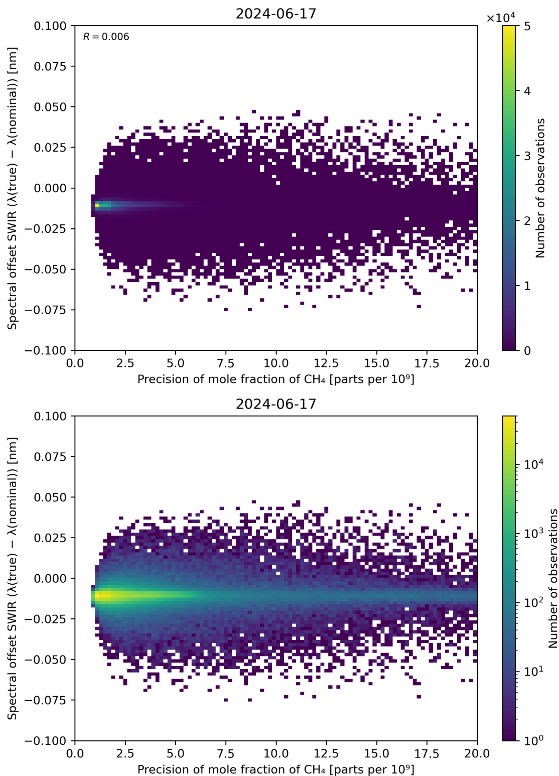
Figure 85: Scatter density plot of “Precision of mole fraction of CH 4 ” against “Spectral offset SWIR ( \lambda(\text{true}) - \lambda(\text{nominal}) )” for 2024-06-16 to 2024-06-18.
