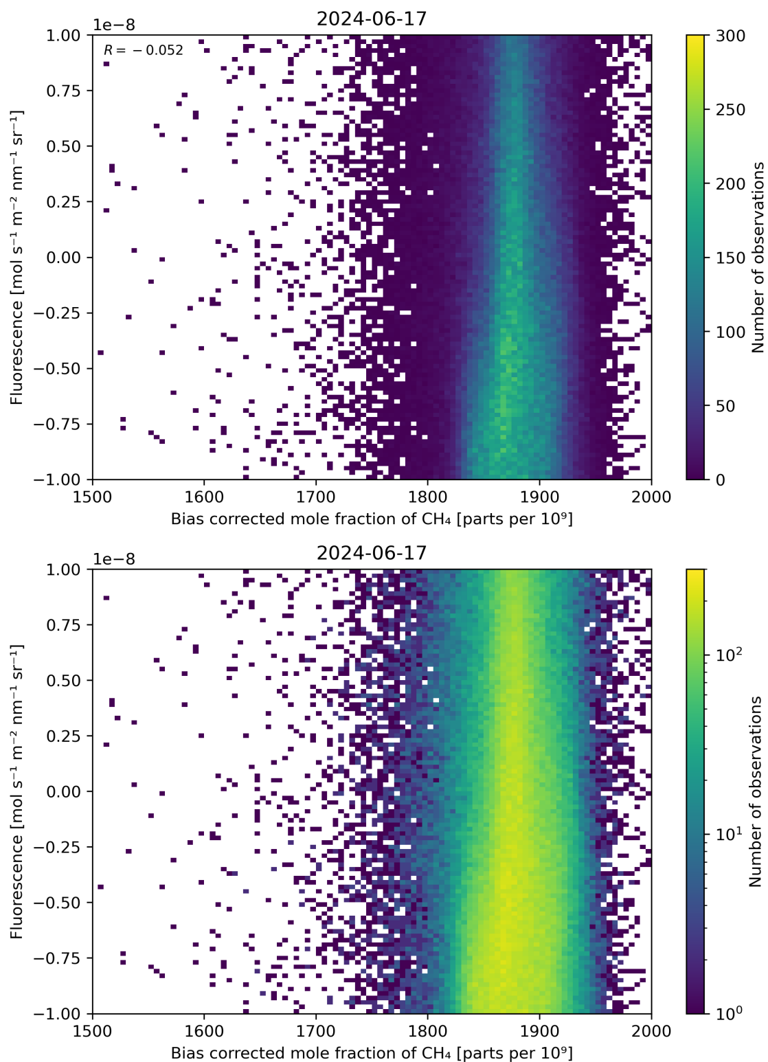
Figure 66: Scatter density plot of “Bias corrected mole fraction of \text{CH}_4 ” against “Fluorescence” for 2024-06-16 to 2024-06-18.
