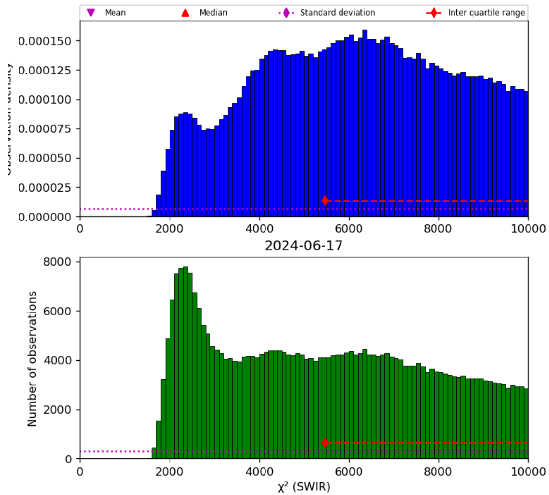
Figure 28: Histogram of “ \chi^2 (SWIR)” for 2024-06-16 to 2024-06-18
