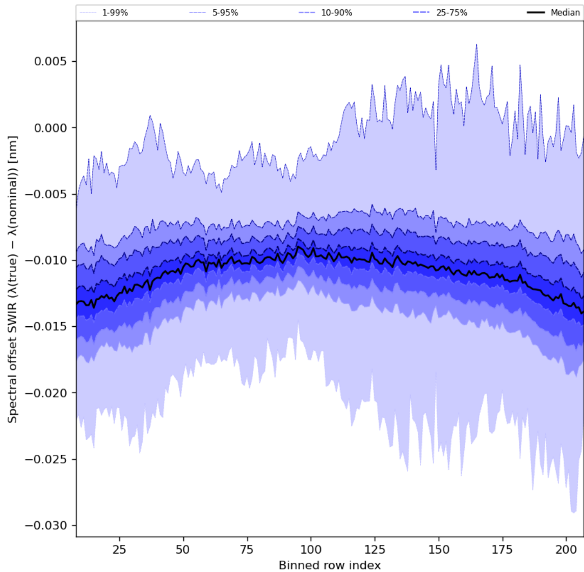
Figure 38: Along track statistics of “Spectral offset SWIR ( \lambda(\text{true}) - \lambda(\text{nominal}) )” for 2024-06-16 to 2024-06-18
