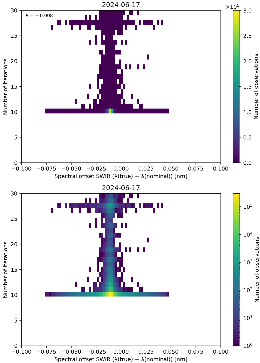
Figure 121: Scatter density plot of “Spectral offset SWIR ( \lambda(\text{true}) - \lambda(\text{nominal}) )” against “Number of iterations” for 2024-06-16 to 2024-06-18.
