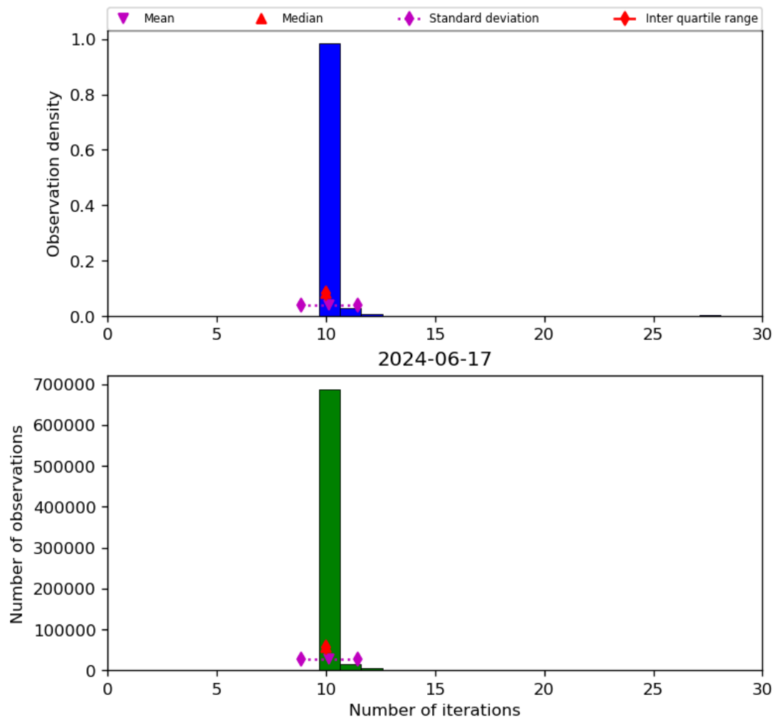
Figure 31: Histogram of “Number of iterations” for 2024-06-16 to 2024-06-18
