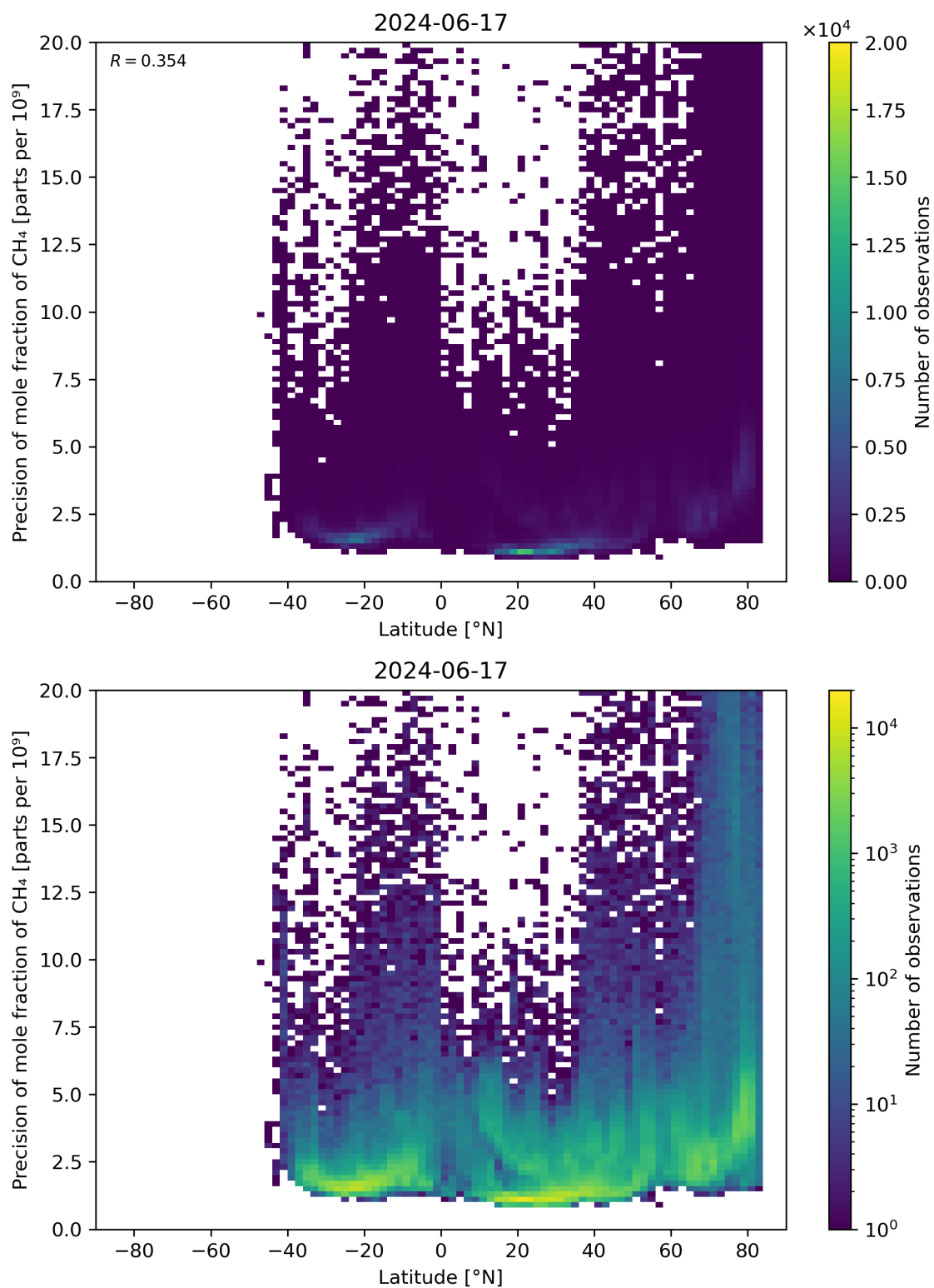
Figure 59: Scatter density plot of “Latitude” against “Precision of mole fraction of \text{CH}_4 ” for 2024-06-16 to 2024-06-18.
