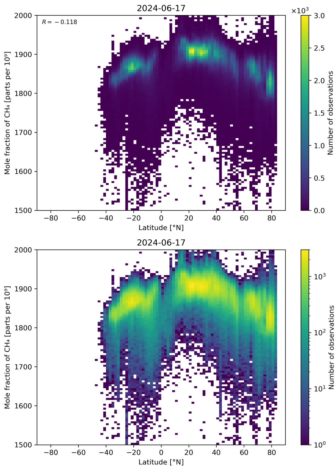
Figure 57: Scatter density plot of “Latitude” against “Mole fraction of \text{CH}_4 ” for 2024-06-16 to 2024-06-18.
