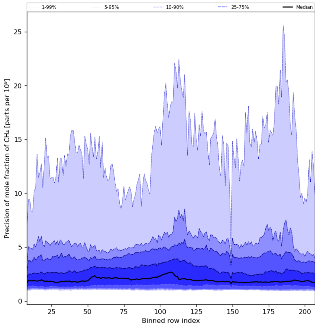
Figure 35: Along track statistics of “Precision of mole fraction of CH 4 ” for 2024-06-16 to 2024-06-18
