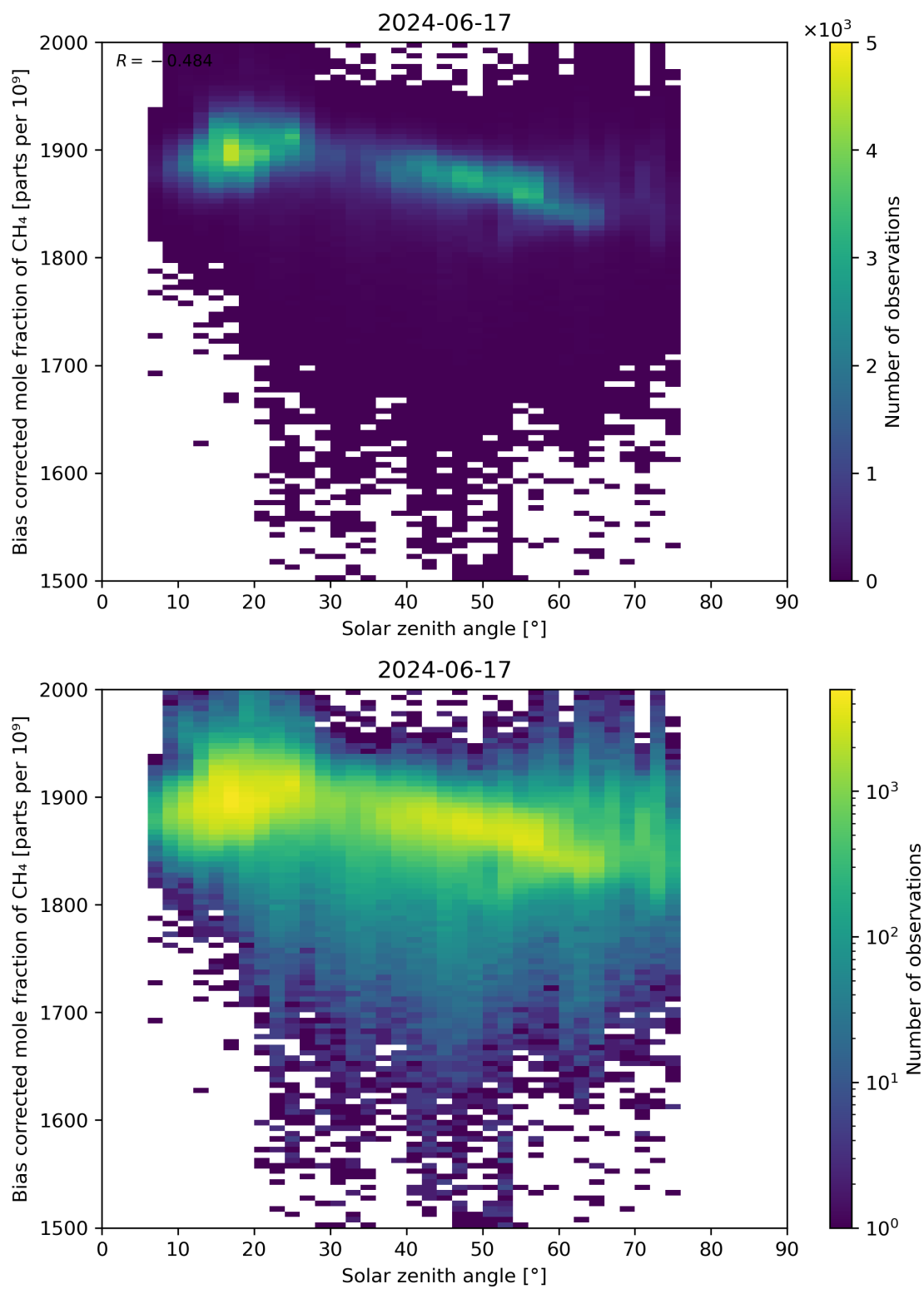
Figure 100: Scatter density plot of “Solar zenith angle” against “Bias corrected mole fraction of \text{CH}_4 ” for 2024-06-16 to 2024-06-18.
