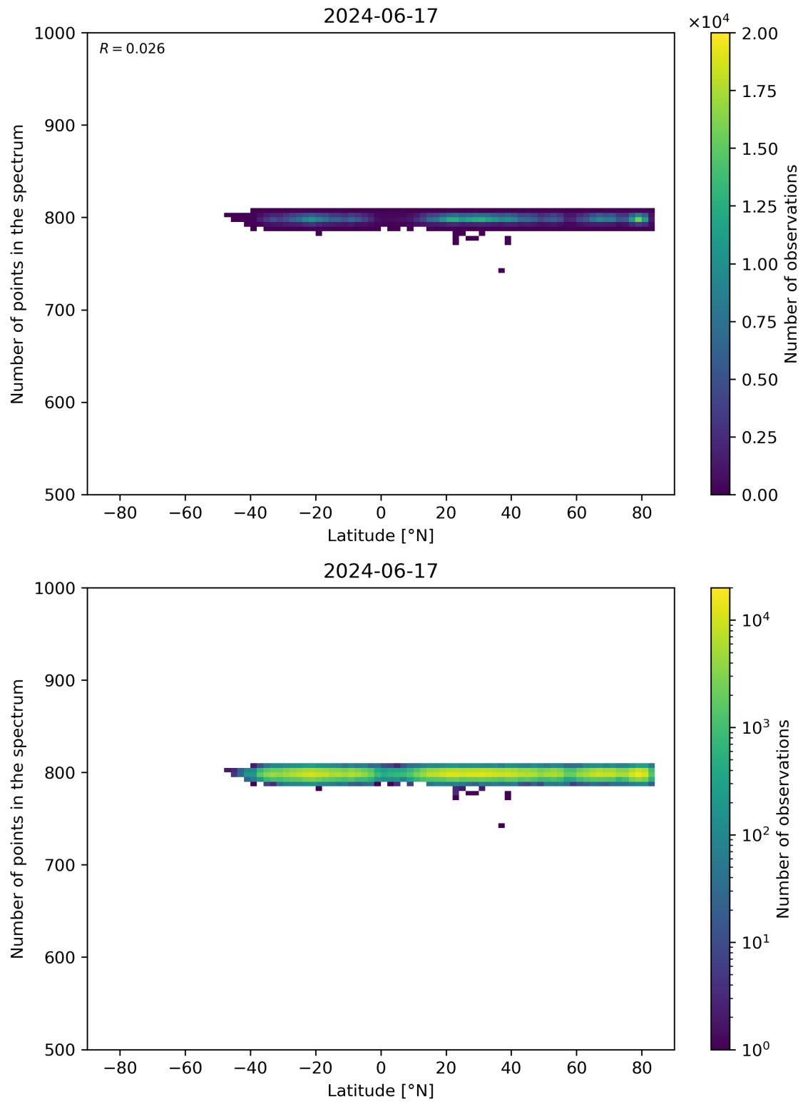
Figure 61: Scatter density plot of “Latitude” against “Number of points in the spectrum” for 2024-06-16 to 2024-06-18.
