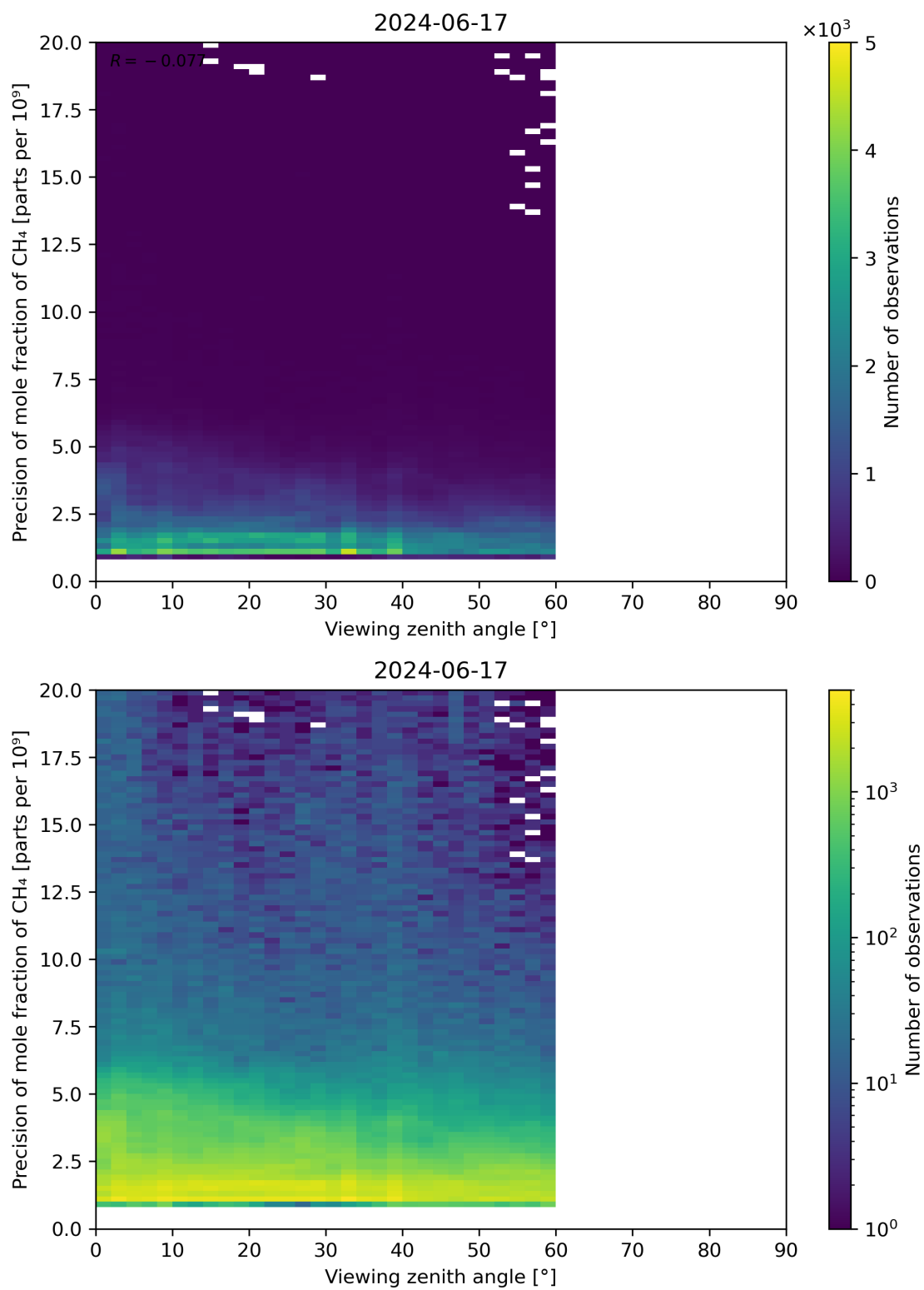
Figure 112: Scatter density plot of “Viewing zenith angle” against “Precision of mole fraction of CH 4 ” for 2024-06-16 to 2024-06-18.
