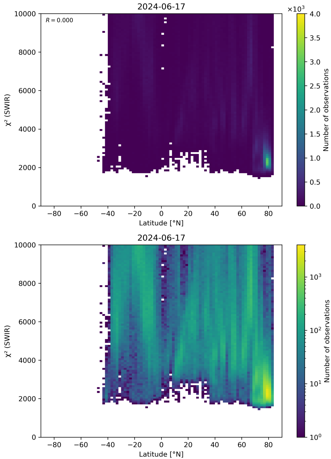
Figure 54: Scatter density plot of “Latitude” against “ \chi^2 (SWIR)” for 2024-06-16 to 2024-06-18.
