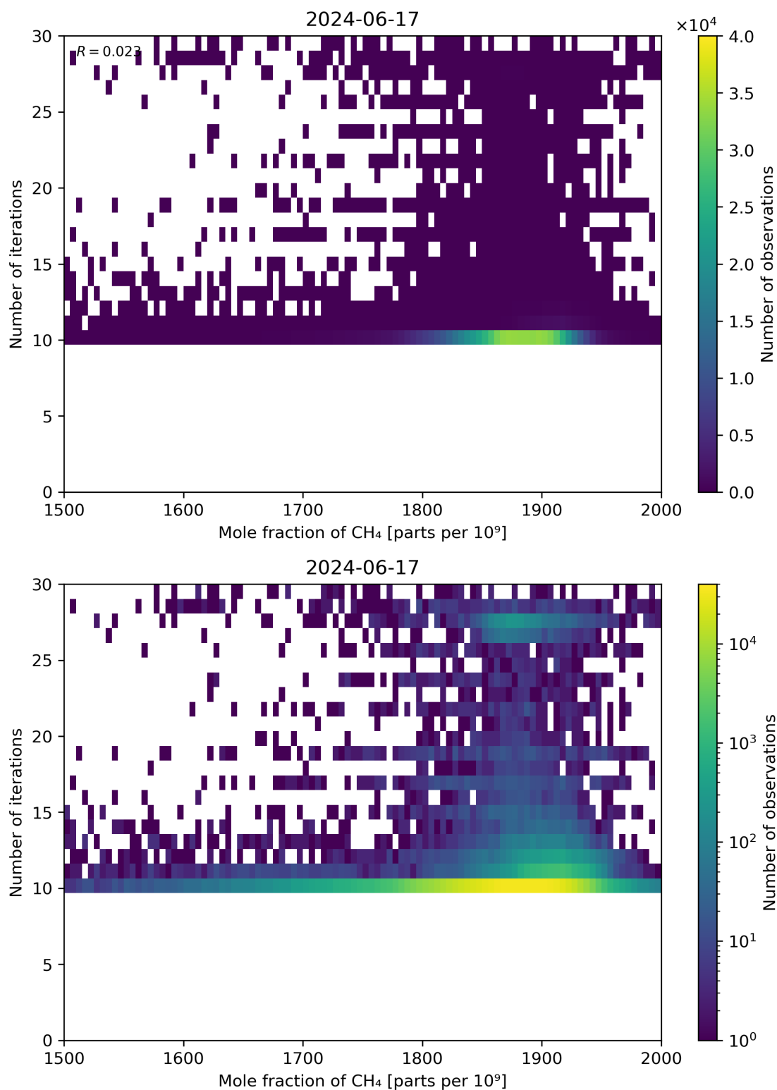
Figure 76: Scatter density plot of “Mole fraction of CH 4 ” against “Number of iterations” for 2024-06-16 to 2024-06-18.
