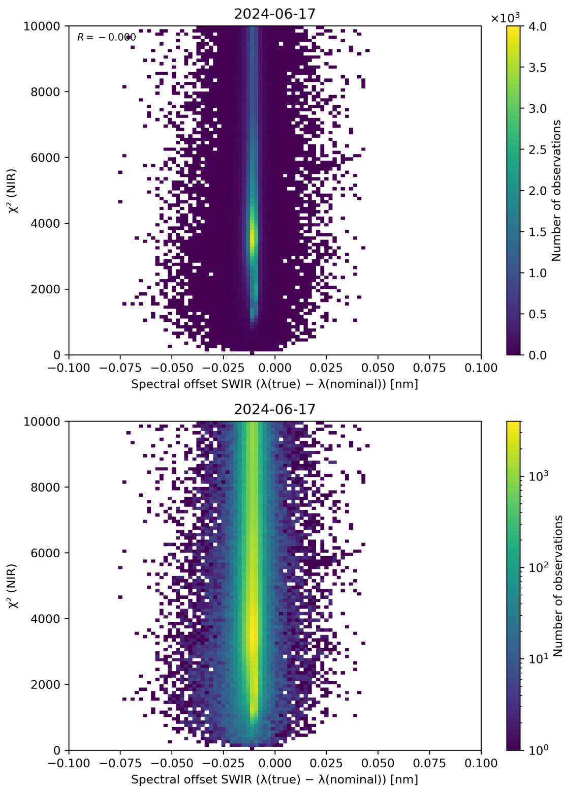
Figure 117: Scatter density plot of “Spectral offset SWIR ( \lambda(\text{true}) - \lambda(\text{nominal}) )” against “ \chi^2 (NIR)” for 2024-06-16 to 2024-06-18.
