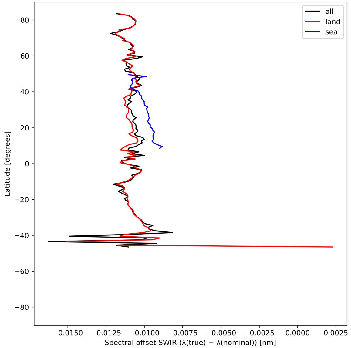
Figure 16: Zonal average of “Spectral offset SWIR ( \lambda(\text{true}) - \lambda(\text{nominal}) )” for 2024-06-16 to 2024-06-18.
