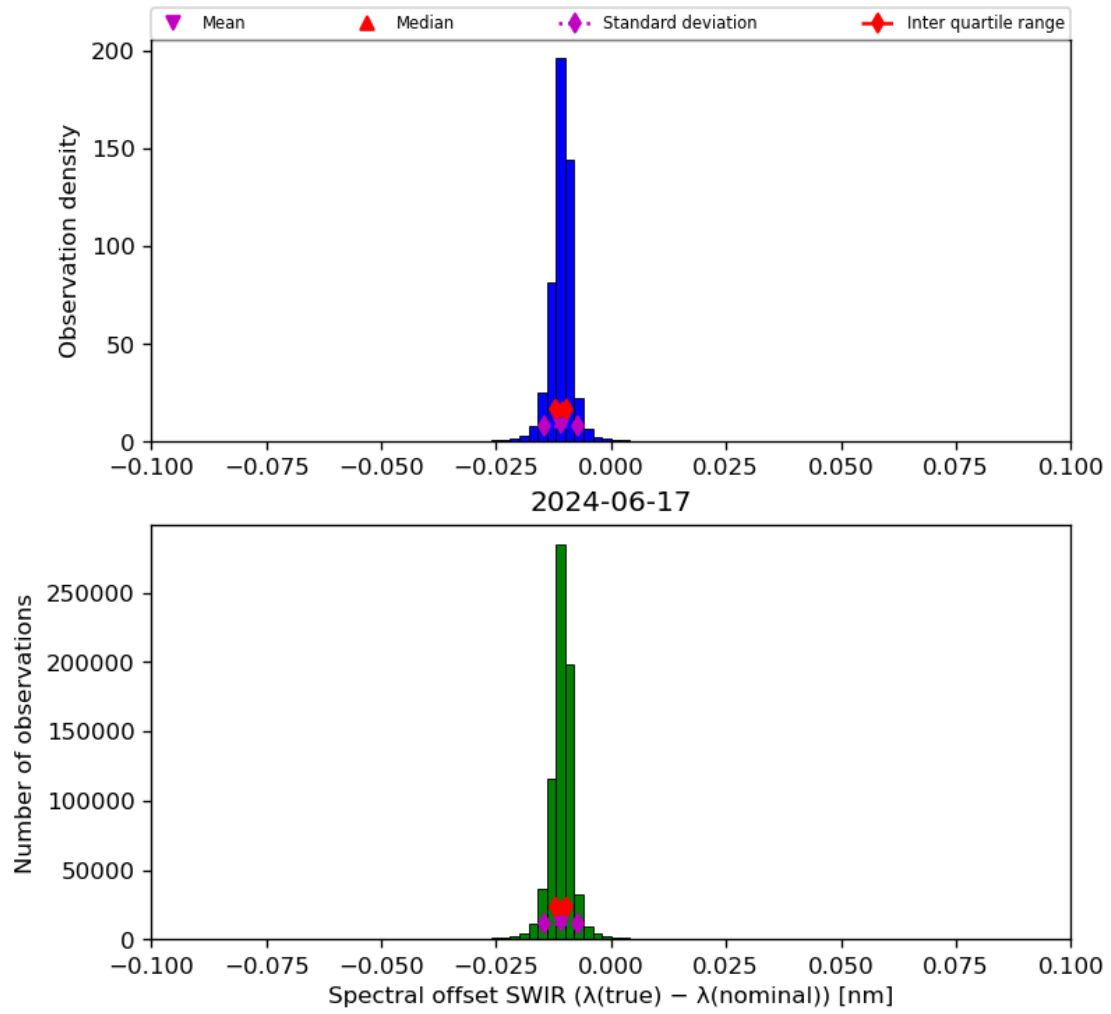
Figure 27: Histogram of “Spectral offset SWIR ( \lambda(\text{true}) - \lambda(\text{nominal}) )” for 2024-06-16 to 2024-06-18
