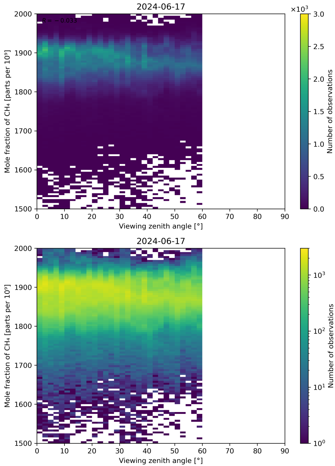
Figure 110: Scatter density plot of “Viewing zenith angle” against “Mole fraction of CH 4 ” for 2024-06-16 to 2024-06-18.
