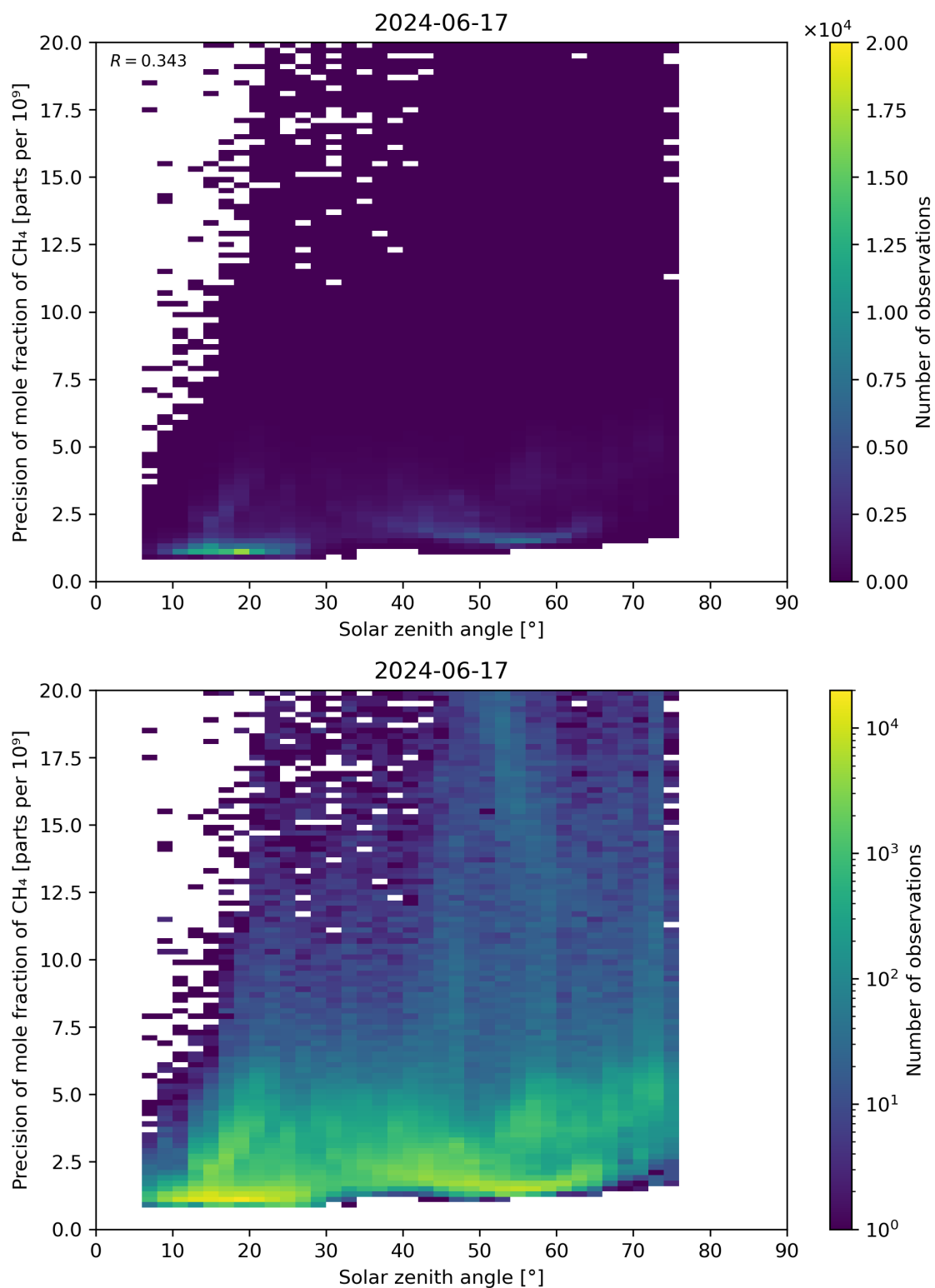
Figure 101: Scatter density plot of “Solar zenith angle” against “Precision of mole fraction of CH 4 ” for 2024-06-16 to 2024-06-18.
