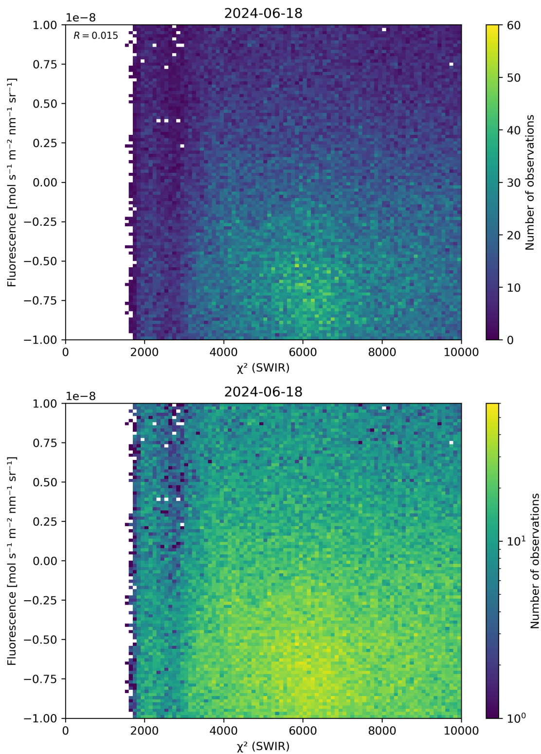
Figure 49: Scatter density plot of “ \chi^2 (SWIR)” against “Fluorescence” for 2024-06-17 to 2024-06-19.
