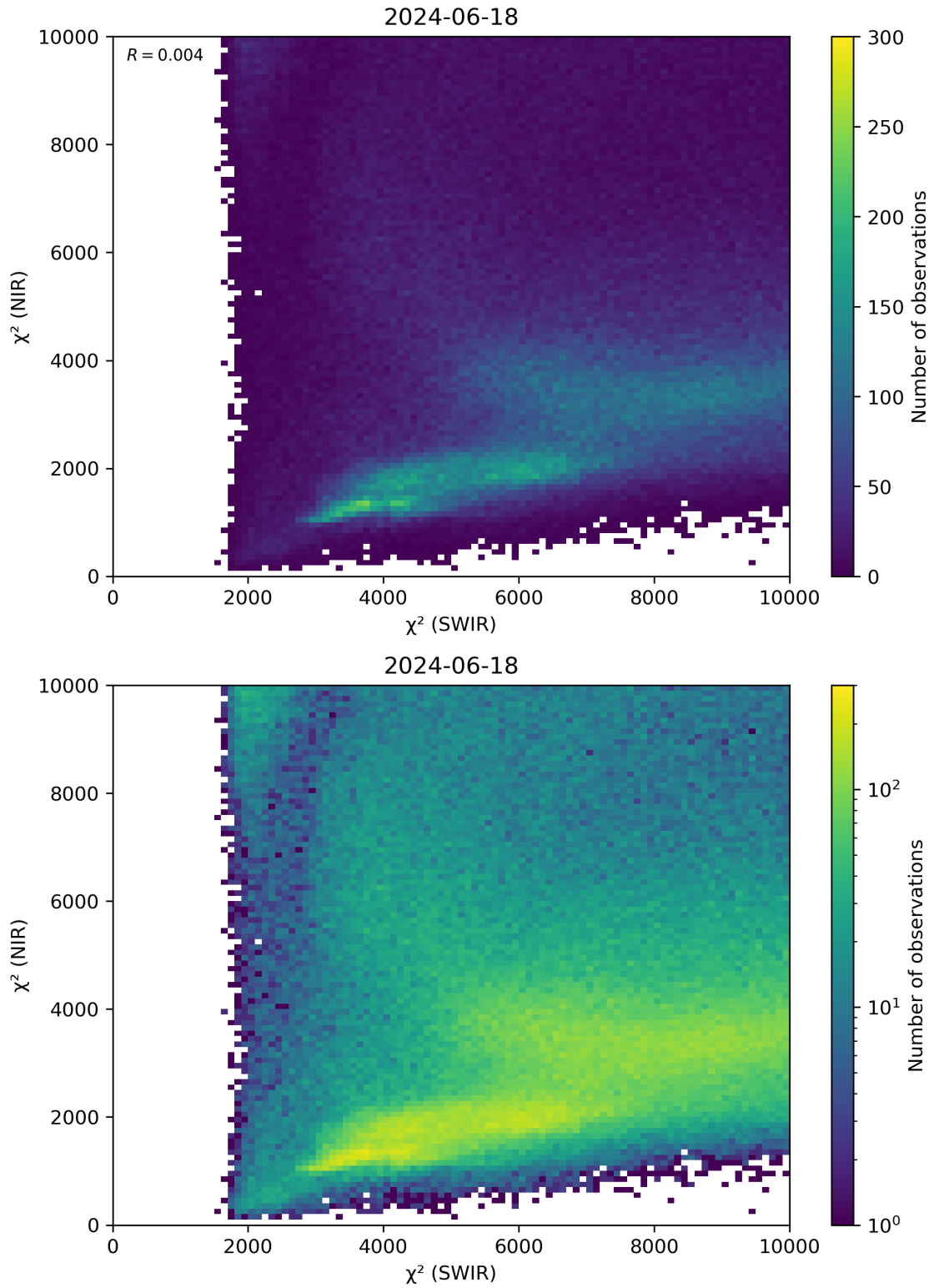
Figure 47: Scatter density plot of “ \chi^2 (SWIR)” against “ \chi^2 (NIR)” for 2024-06-17 to 2024-06-19.
