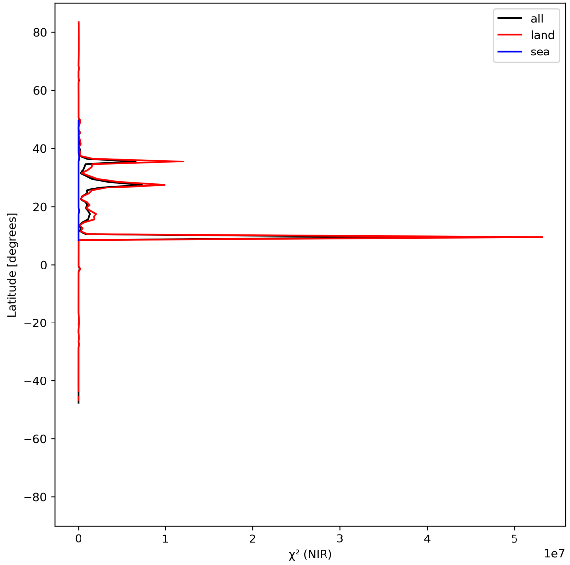
Figure 18: Zonal average of “ \chi^2 (NIR)” for 2024-06-17 to 2024-06-19.
