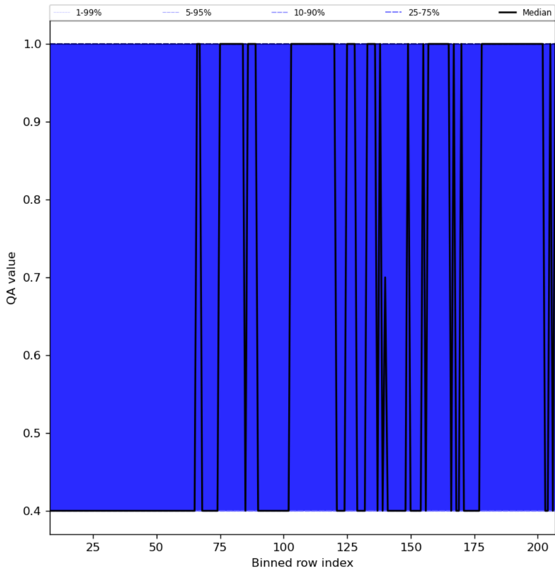
Figure 33: Along track statistics of “QA value” for 2024-06-17 to 2024-06-19
