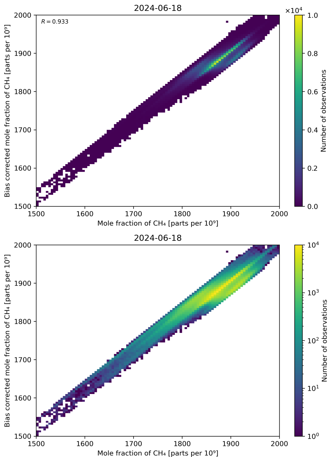
Figure 74: Scatter density plot of “Mole fraction of CH 4 ” against “Bias corrected mole fraction of CH 4 ” for 2024-06-17 to 2024-06-19.
