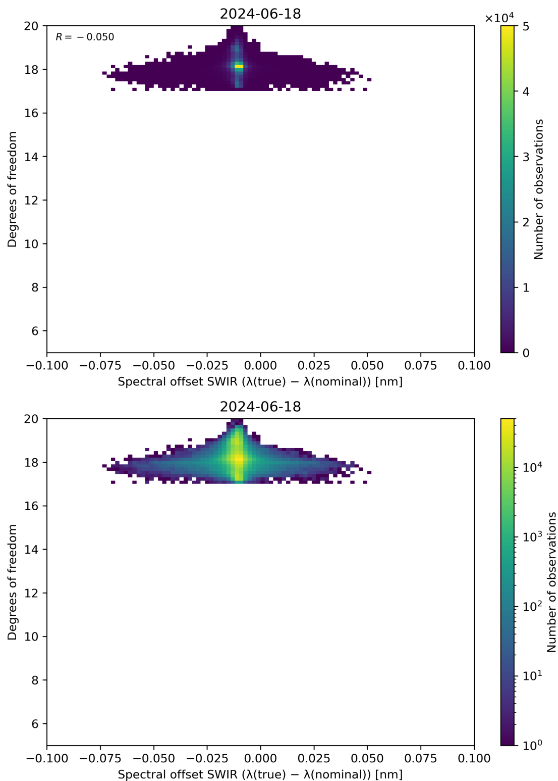
Figure 119: Scatter density plot of “Spectral offset SWIR ( \lambda(\text{true}) - \lambda(\text{nominal}) )” against “Degrees of freedom” for 2024-06-17 to 2024-06-19.
