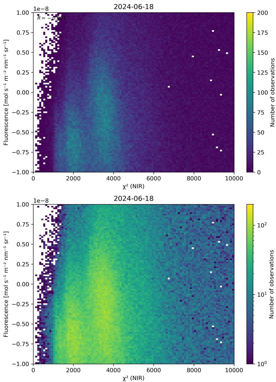
Figure 45: Scatter density plot of “ \chi^2 (NIR)” against “Fluorescence” for 2024-06-17 to 2024-06-19.
