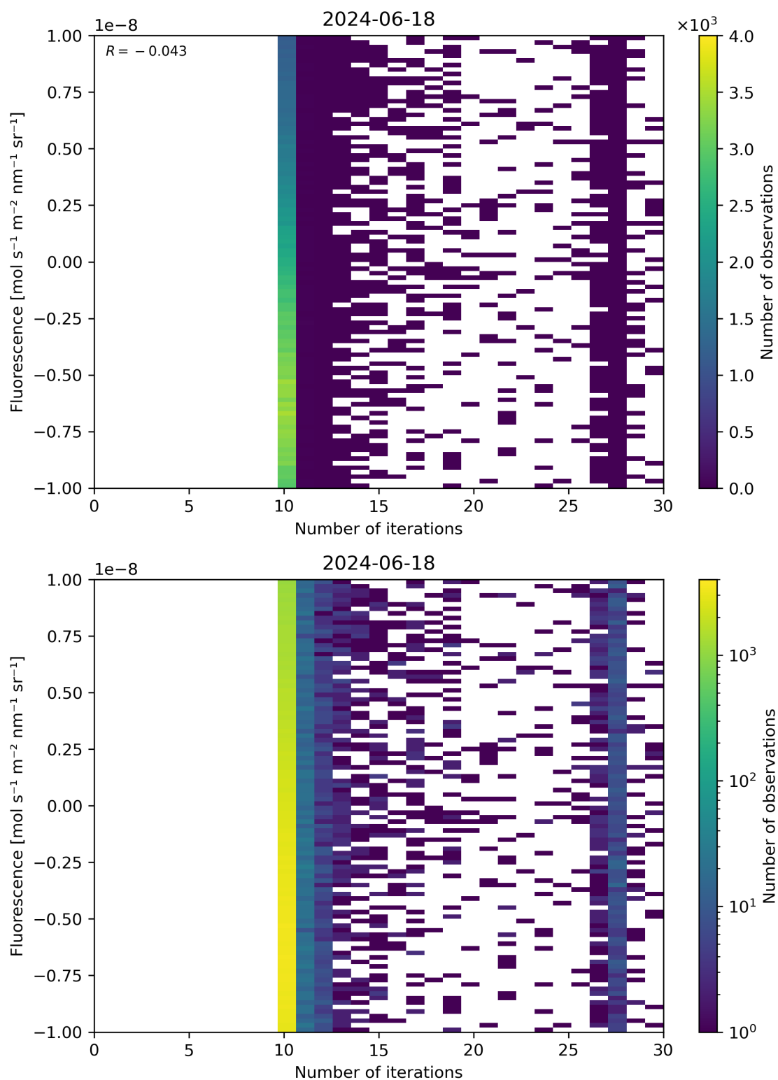
Figure 87: Scatter density plot of “Number of iterations” against “Fluorescence” for 2024-06-17 to 2024-06-19.
