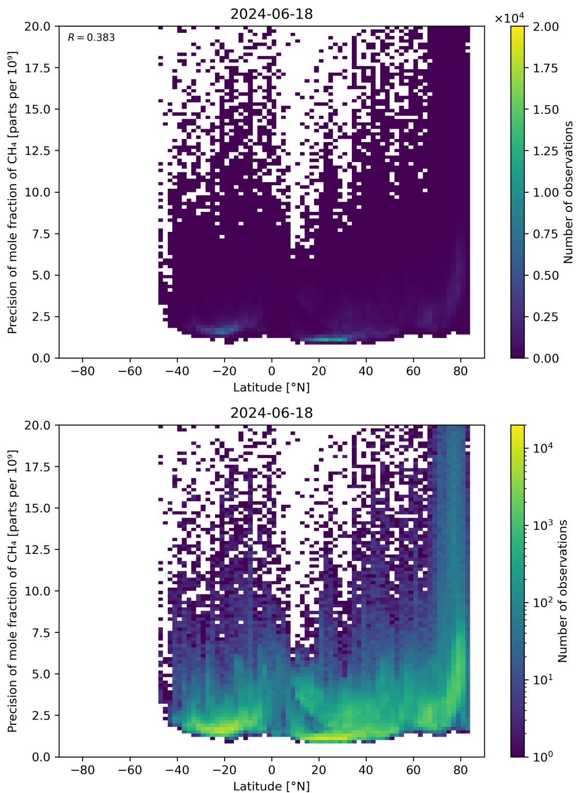
Figure 59: Scatter density plot of “Latitude” against “Precision of mole fraction of \text{CH}_4 ” for 2024-06-17 to 2024-06-19.
