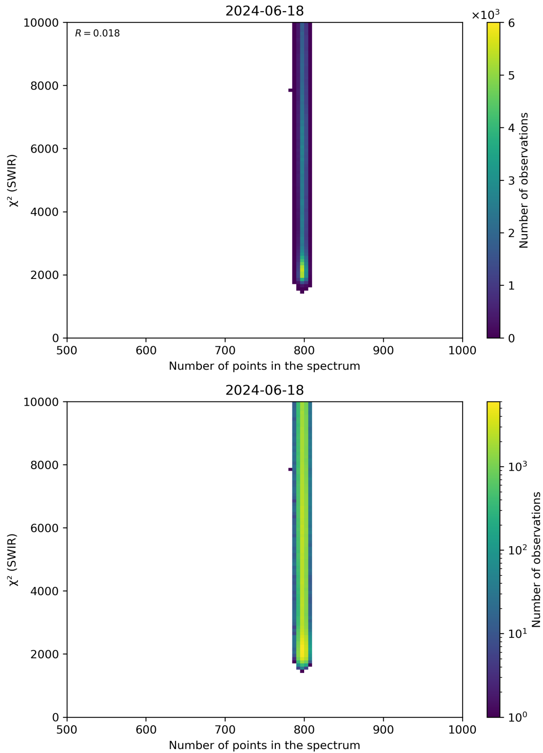
Figure 89: Scatter density plot of “Number of points in the spectrum” against “ \chi^2 (SWIR)” for 2024-06-17 to 2024-06-19.
