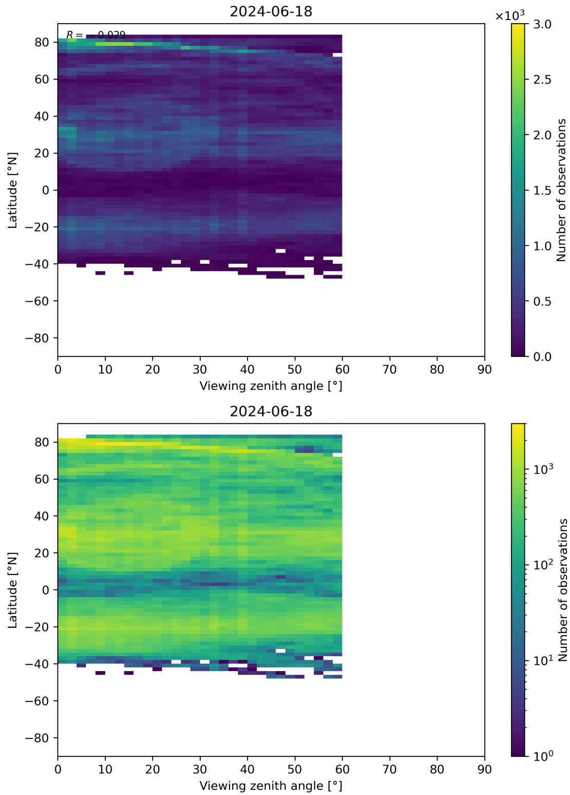
Figure 109: Scatter density plot of “Viewing zenith angle” against “Latitude” for 2024-06-17 to 2024-06-19.
