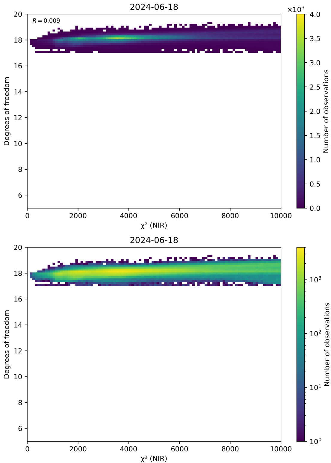
Figure 44: Scatter density plot of “ \chi^2 (NIR)” against “Degrees of freedom” for 2024-06-17 to 2024-06-19.
