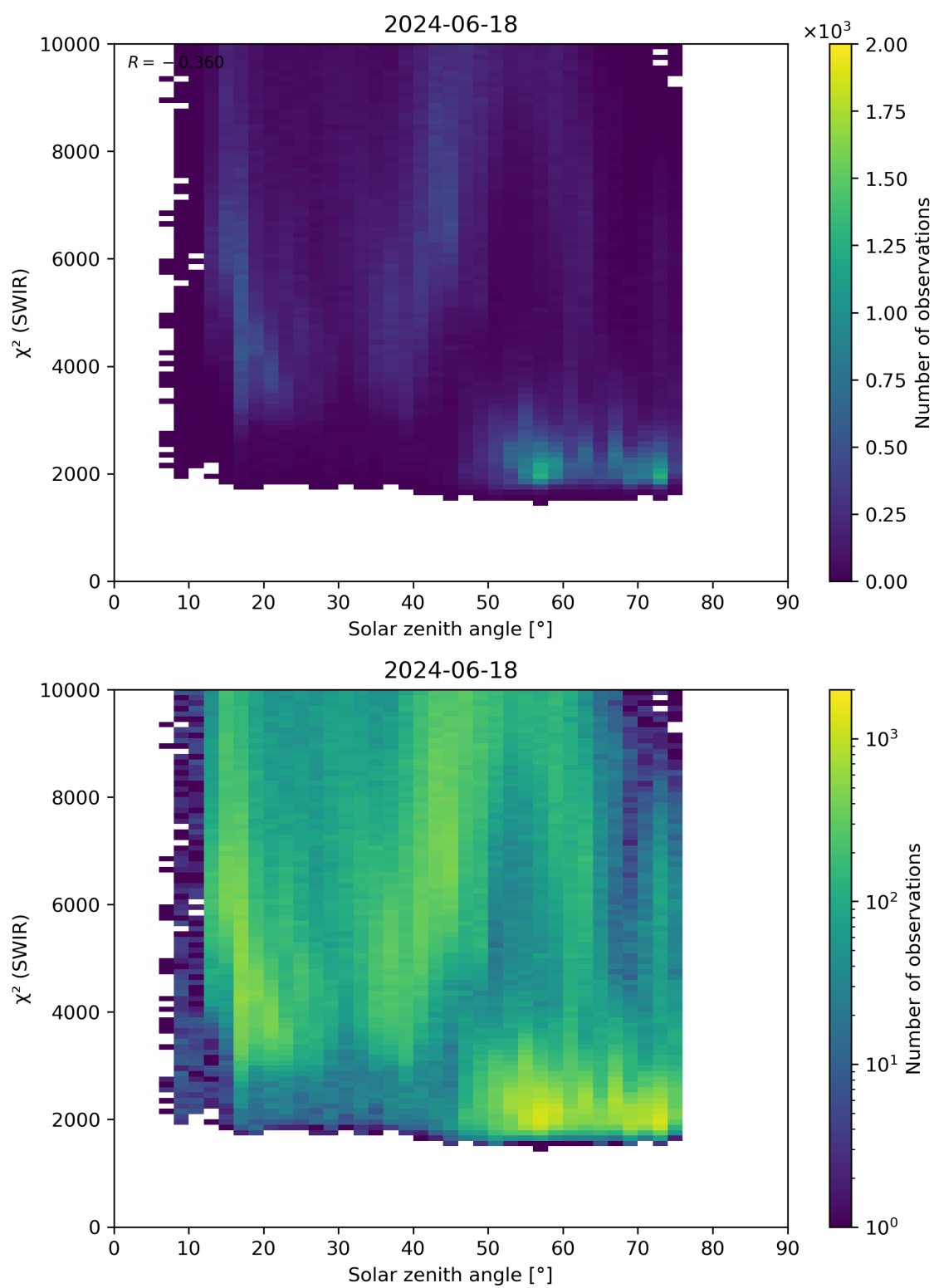
Figure 95: Scatter density plot of “Solar zenith angle” against “ \chi^2 (SWIR)” for 2024-06-17 to 2024-06-19.
