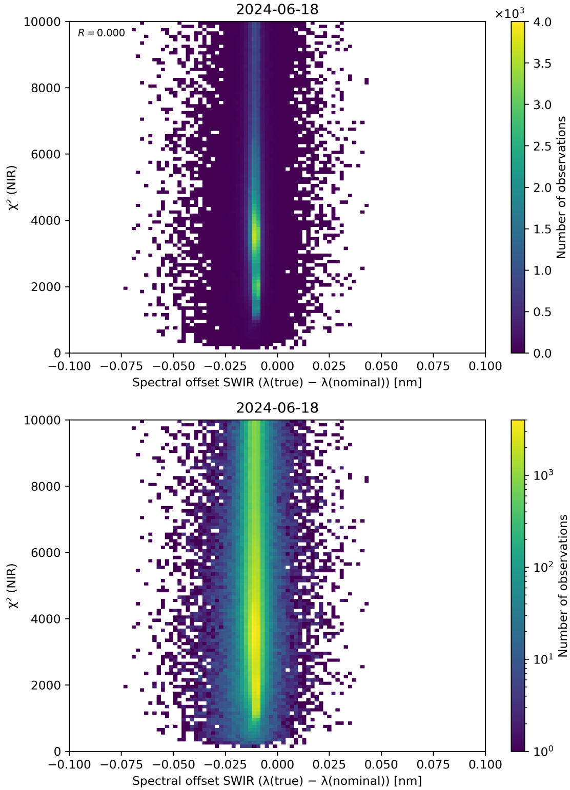
Figure 117: Scatter density plot of “Spectral offset SWIR ( \lambda(\text{true}) - \lambda(\text{nominal}) )” against “ \chi^2 (NIR)” for 2024-06-17 to 2024-06-19.
