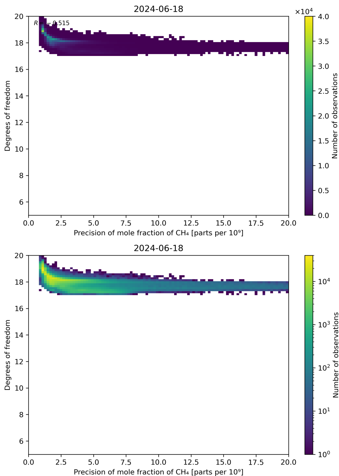
Figure 80: Scatter density plot of “Precision of mole fraction of CH 4 ” against “Degrees of freedom” for 2024-06-17 to 2024-06-19.
