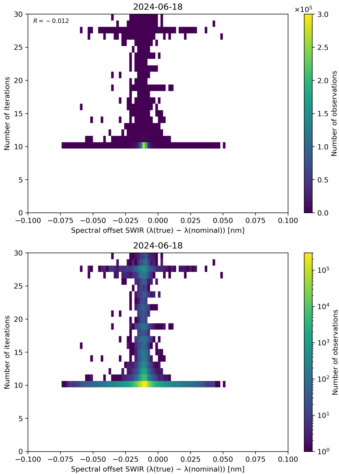
Figure 121: Scatter density plot of “Spectral offset SWIR ( \lambda(\text{true}) - \lambda(\text{nominal}) )” against “Number of iterations” for 2024-06-17 to 2024-06-19.
