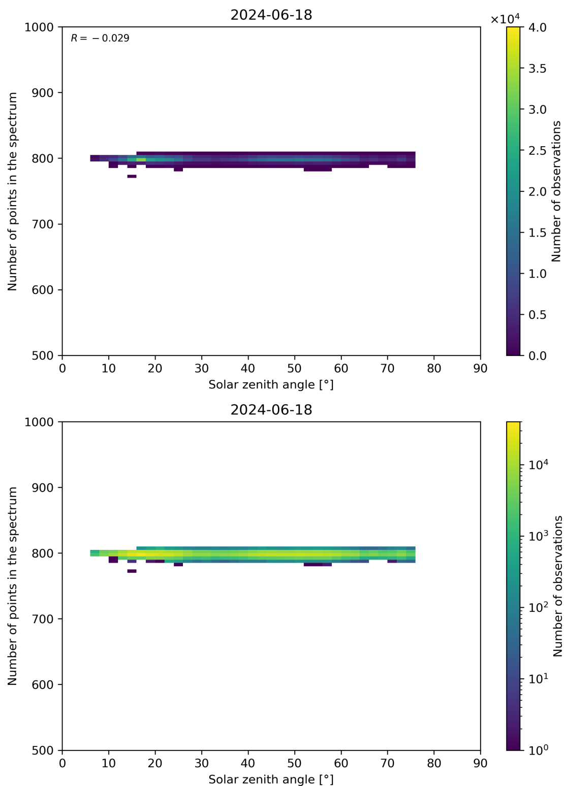
Figure 103: Scatter density plot of “Solar zenith angle” against “Number of points in the spectrum” for 2024-06-17 to 2024-06-19.
