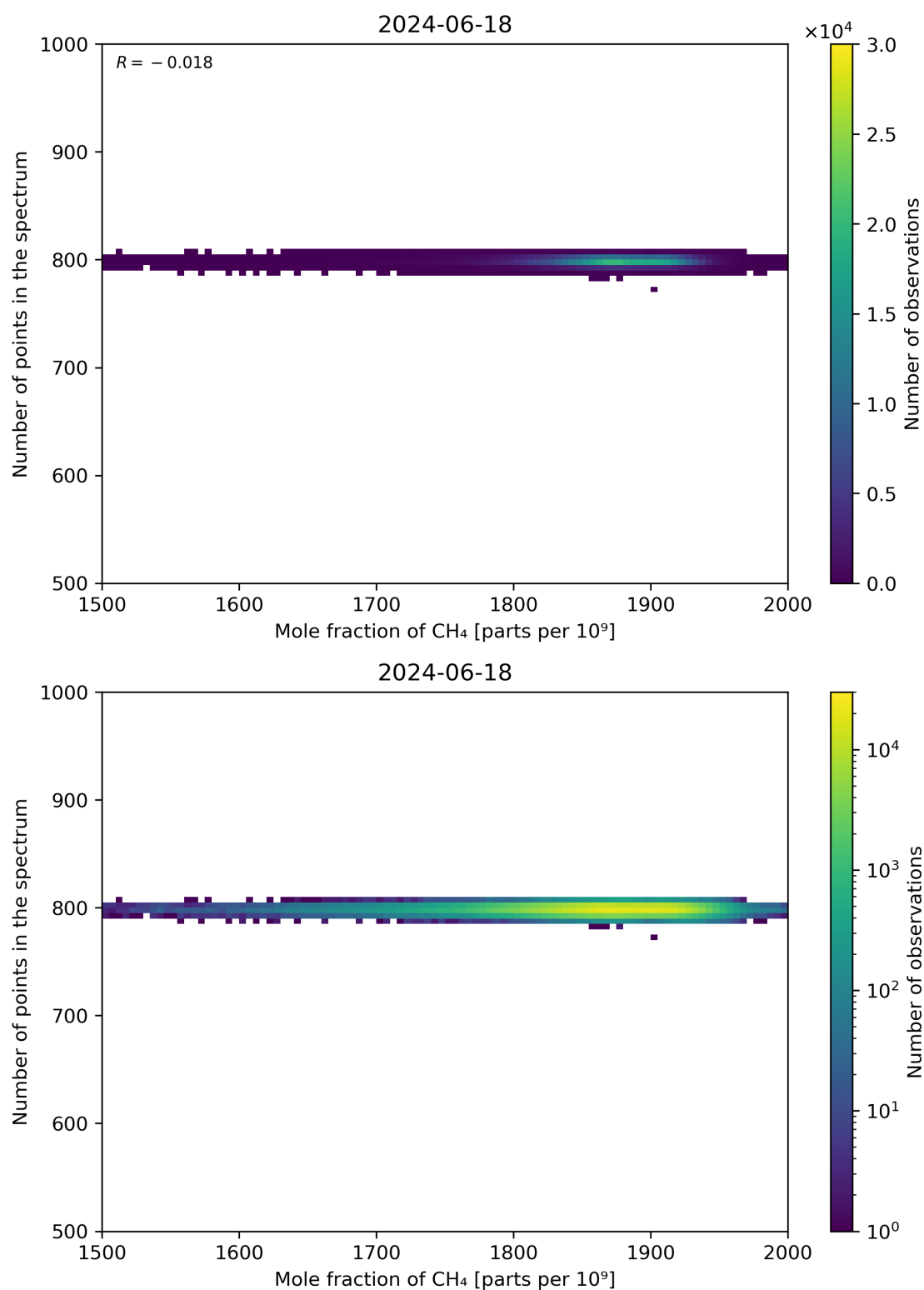
Figure 77: Scatter density plot of “Mole fraction of CH 4 ” against “Number of points in the spectrum” for 2024-06-17 to 2024-06-19.
