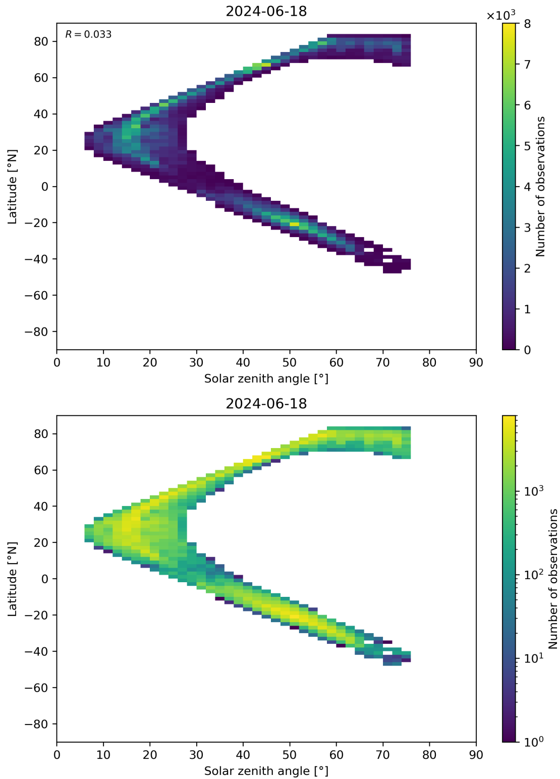
Figure 98: Scatter density plot of “Solar zenith angle” against “Latitude” for 2024-06-17 to 2024-06-19.
