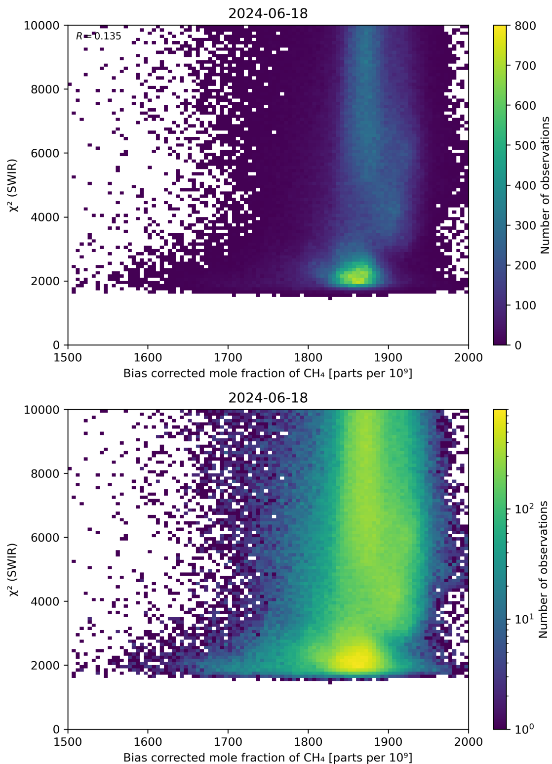
Figure 64: Scatter density plot of “Bias corrected mole fraction of CH 4 ” against “ \chi^2 (SWIR)” for 2024-06-17 to 2024-06-19.
