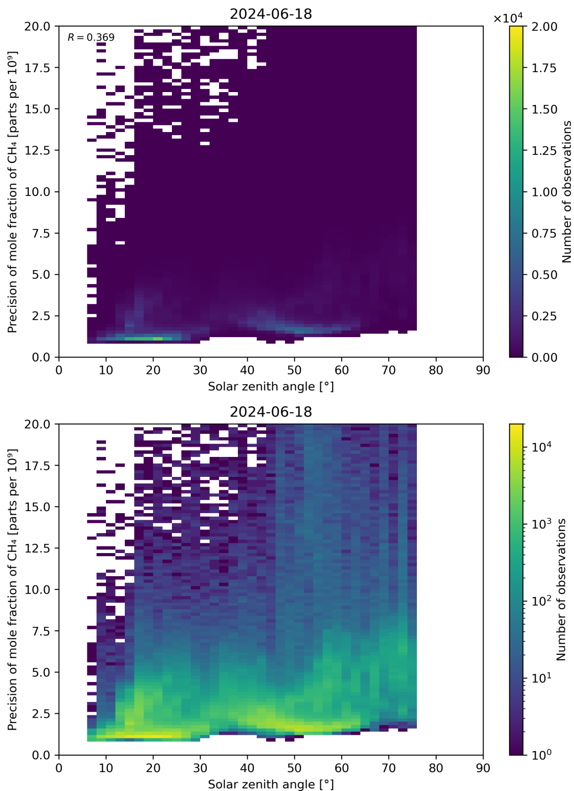
Figure 101: Scatter density plot of “Solar zenith angle” against “Precision of mole fraction of CH 4 ” for 2024-06-17 to 2024-06-19.
