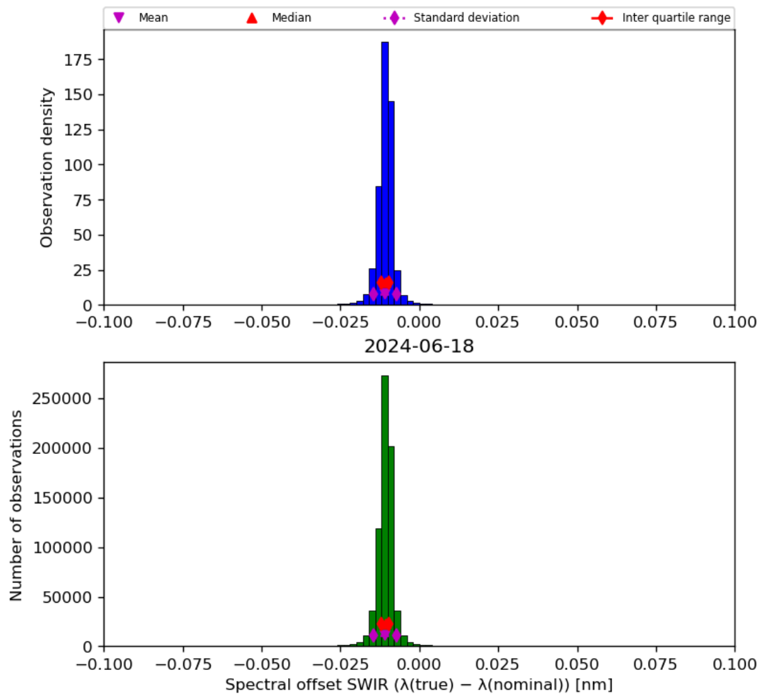
Figure 27: Histogram of “Spectral offset SWIR ( \lambda(\text{true}) - \lambda(\text{nominal}) )” for 2024-06-17 to 2024-06-19
