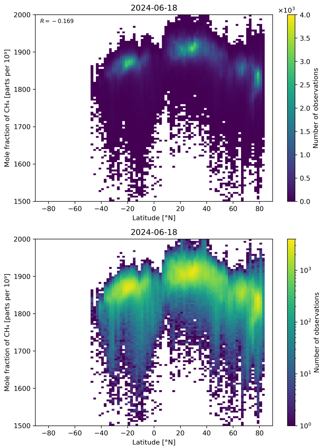
Figure 57: Scatter density plot of “Latitude” against “Mole fraction of CH 4 ” for 2024-06-17 to 2024-06-19.
