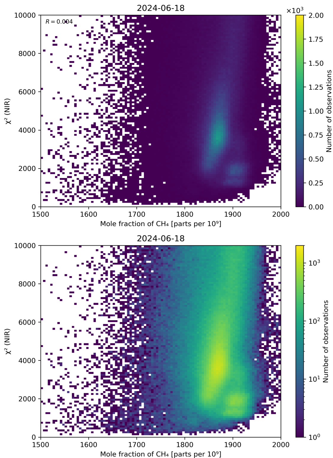
Figure 70: Scatter density plot of “Mole fraction of \text{CH}_4 ” against “ \chi^2 (NIR)” for 2024-06-17 to 2024-06-19.
