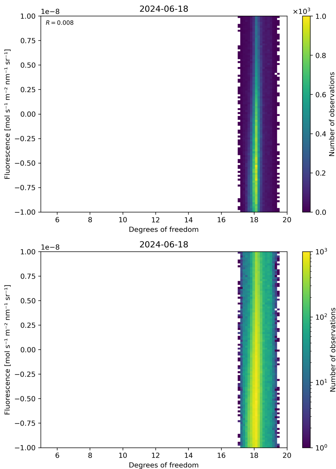
Figure 51: Scatter density plot of “Degrees of freedom” against “Fluorescence” for 2024-06-17 to 2024-06-19.
