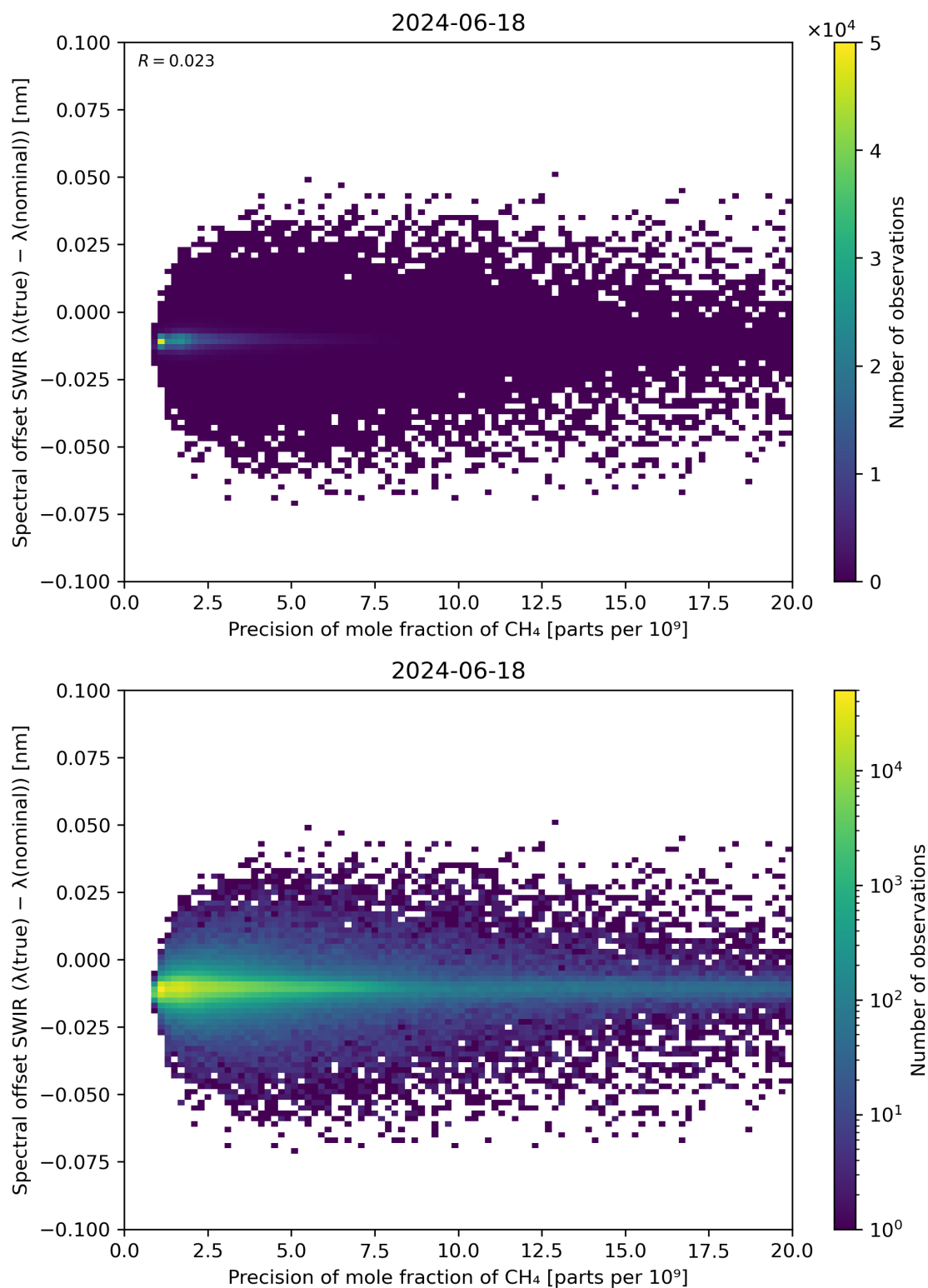
Figure 85: Scatter density plot of “Precision of mole fraction of CH 4 ” against “Spectral offset SWIR ( \lambda(\text{true}) - \lambda(\text{nominal}) )” for 2024-06-17 to 2024-06-19.
