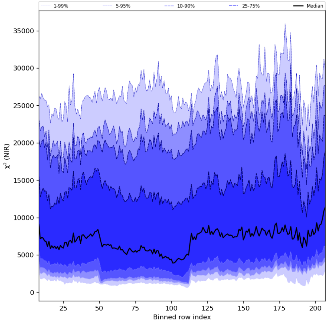
Figure 40: Along track statistics of “ \chi^2 (NIR)” for 2024-06-17 to 2024-06-19
