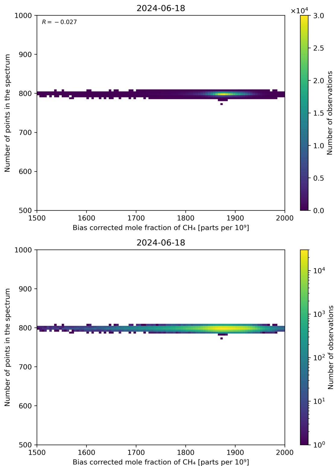
Figure 68: Scatter density plot of “Bias corrected mole fraction of CH 4 ” against “Number of points in the spectrum” for 2024-06-17 to 2024-06-19.
