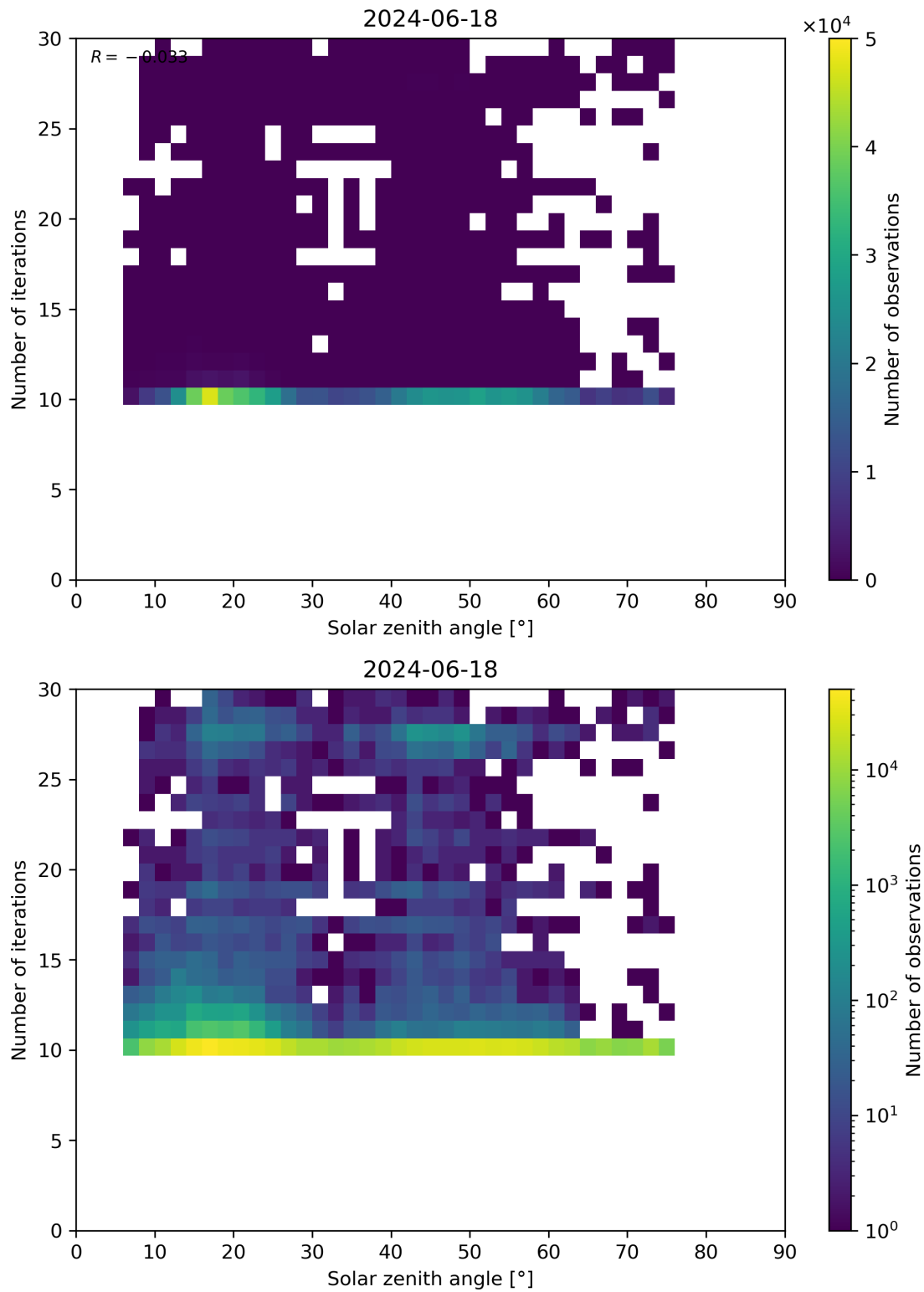
Figure 102: Scatter density plot of “Solar zenith angle” against “Number of iterations” for 2024-06-17 to 2024-06-19.
