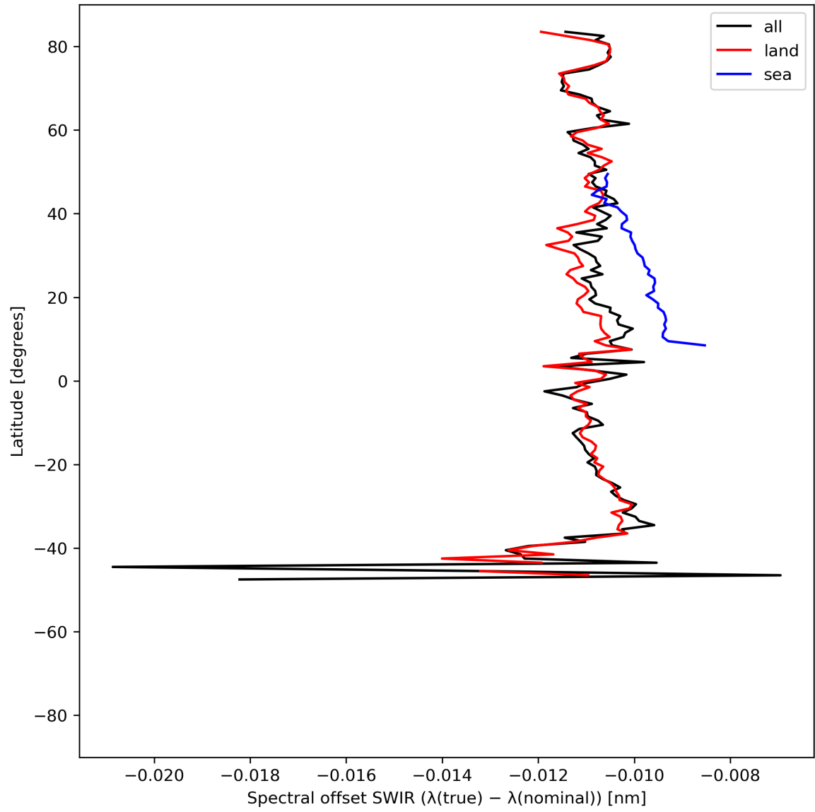
Figure 16: Zonal average of “Spectral offset SWIR ( \lambda(\text{true}) - \lambda(\text{nominal}) )” for 2024-06-17 to 2024-06-19.
