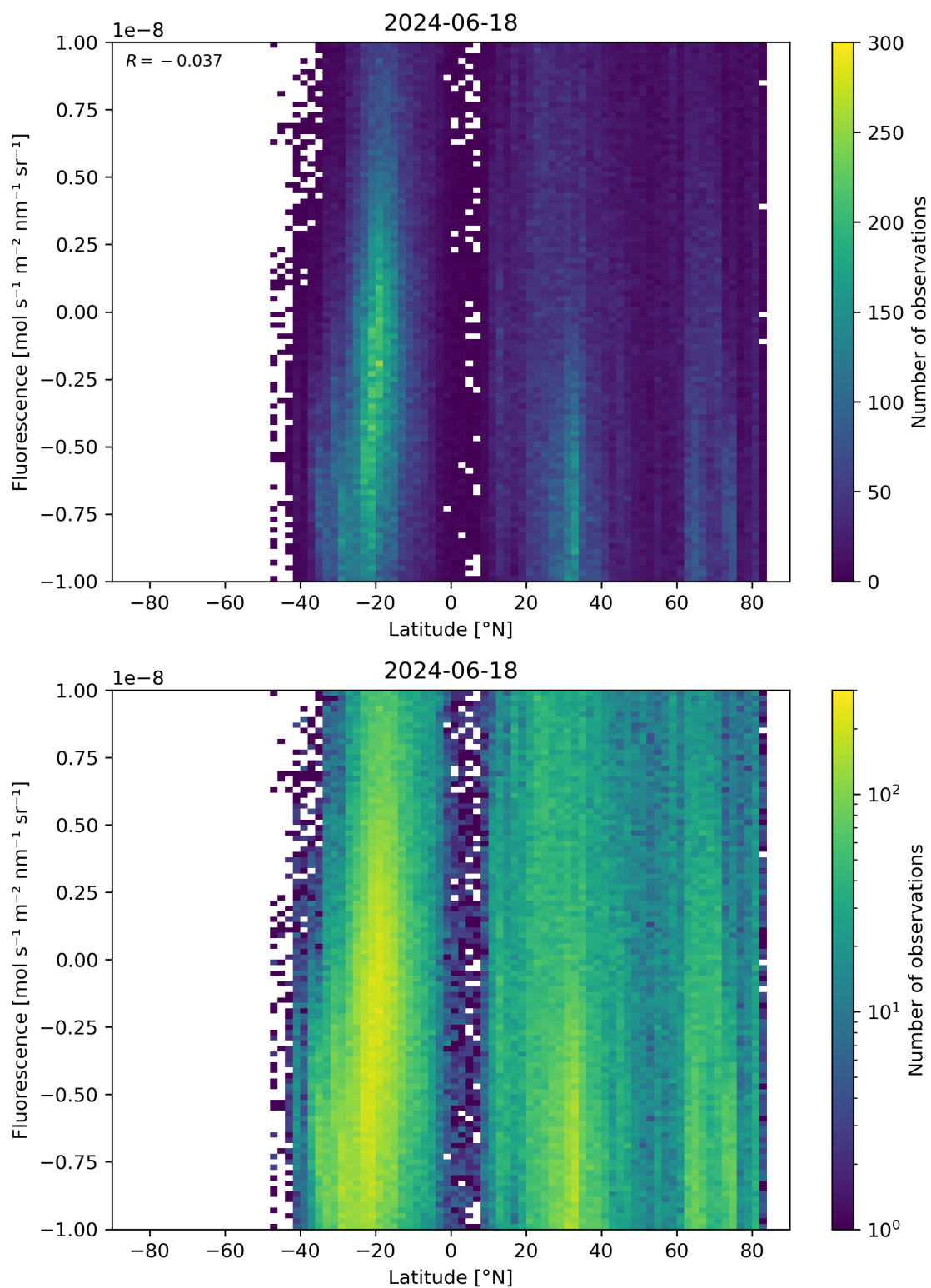
Figure 56: Scatter density plot of “Latitude” against “Fluorescence” for 2024-06-17 to 2024-06-19.
