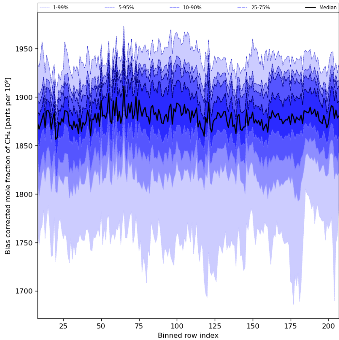
Figure 36: Along track statistics of “Bias corrected mole fraction of CH 4 ” for 2024-06-17 to 2024-06-19
