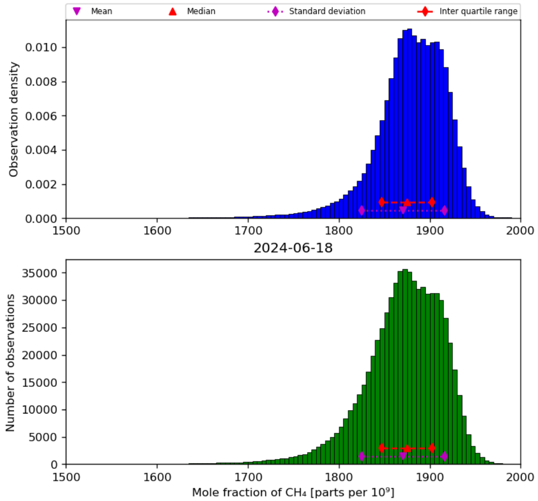
Figure 23: Histogram of "Mole fraction of CH 4 " for 2024-06-17 to 2024-06-19
