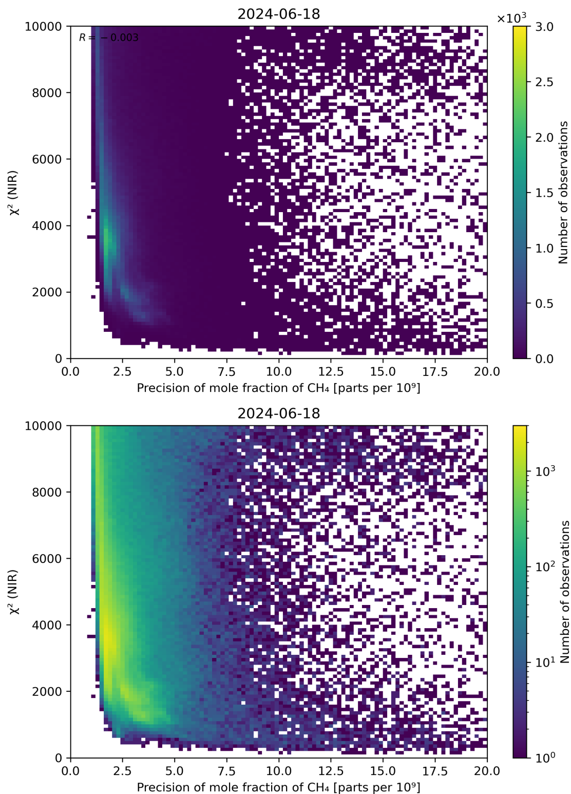
Figure 78: Scatter density plot of “Precision of mole fraction of CH 4 ” against “ \chi^2 (NIR)” for 2024-06-17 to 2024-06-19.
