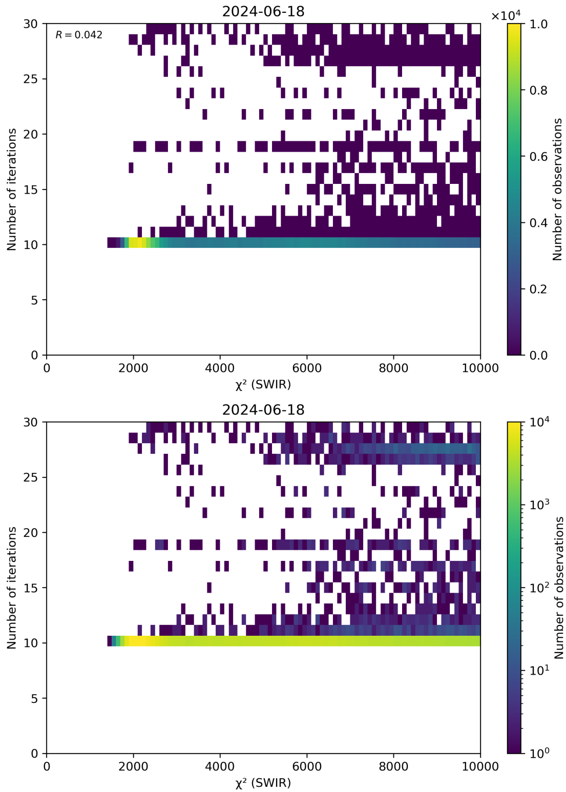
Figure 50: Scatter density plot of “ \chi^2 (SWIR)” against “Number of iterations” for 2024-06-17 to 2024-06-19.
