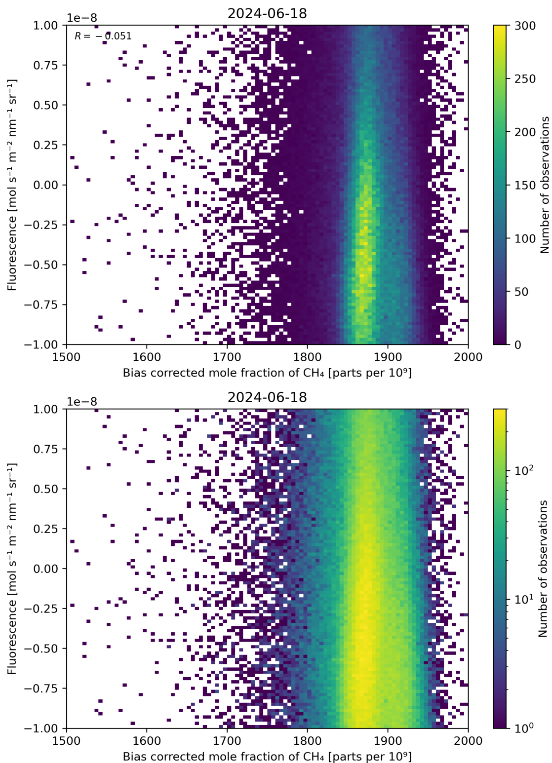
Figure 66: Scatter density plot of “Bias corrected mole fraction of \text{CH}_4 ” against “Fluorescence” for 2024-06-17 to 2024-06-19.
