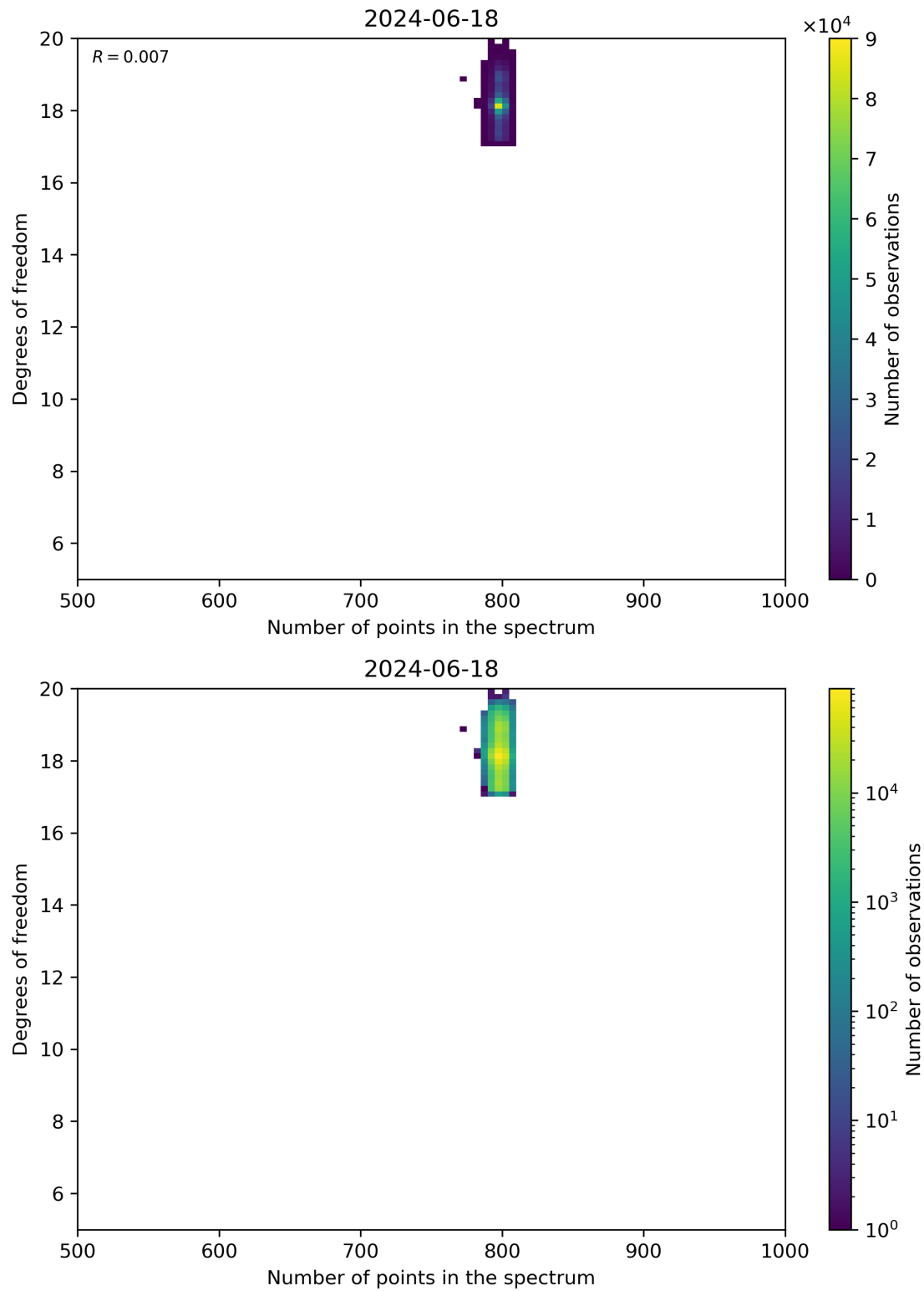
Figure 90: Scatter density plot of “Number of points in the spectrum” against “Degrees of freedom” for 2024-06-17 to 2024-06-19.
