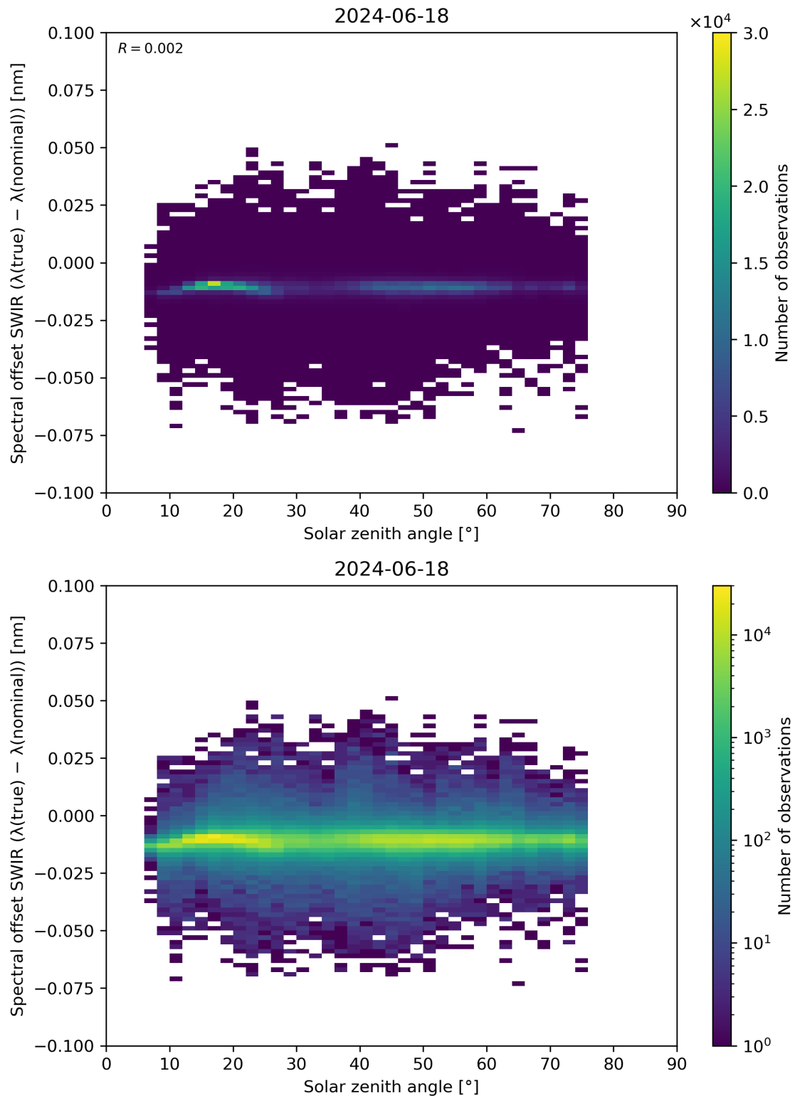
Figure 104: Scatter density plot of “Solar zenith angle” against “Spectral offset SWIR ( \lambda(\text{true}) - \lambda(\text{nominal}) )” for 2024-06-17 to 2024-06-19.
