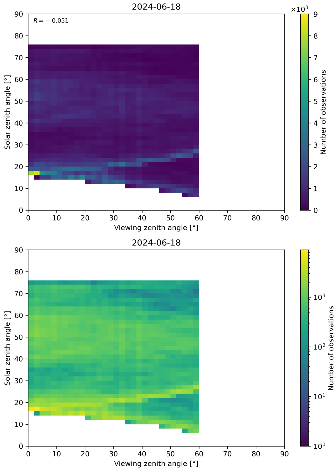
Figure 115: Scatter density plot of “Viewing zenith angle” against “Solar zenith angle” for 2024-06-17 to 2024-06-19.
