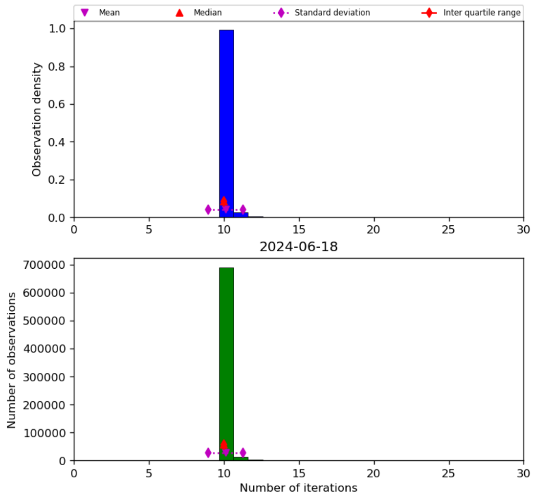
Figure 31: Histogram of “Number of iterations” for 2024-06-17 to 2024-06-19
