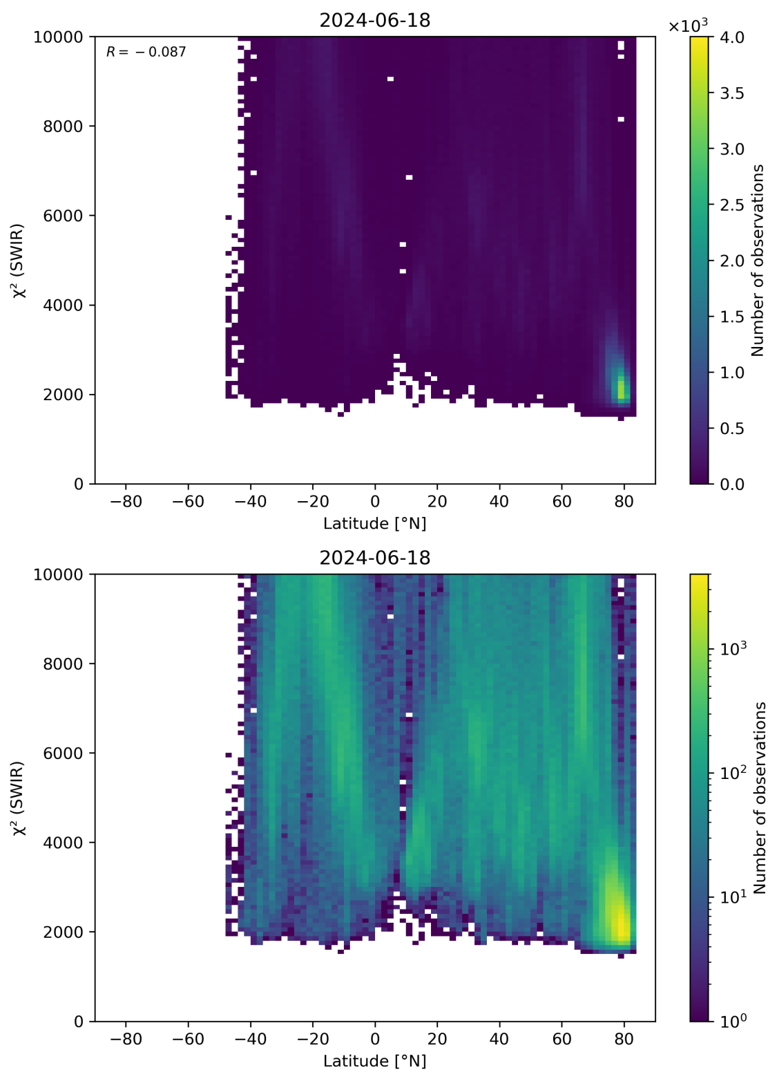
Figure 54: Scatter density plot of “Latitude” against “ \chi^2 (SWIR)” for 2024-06-17 to 2024-06-19.
