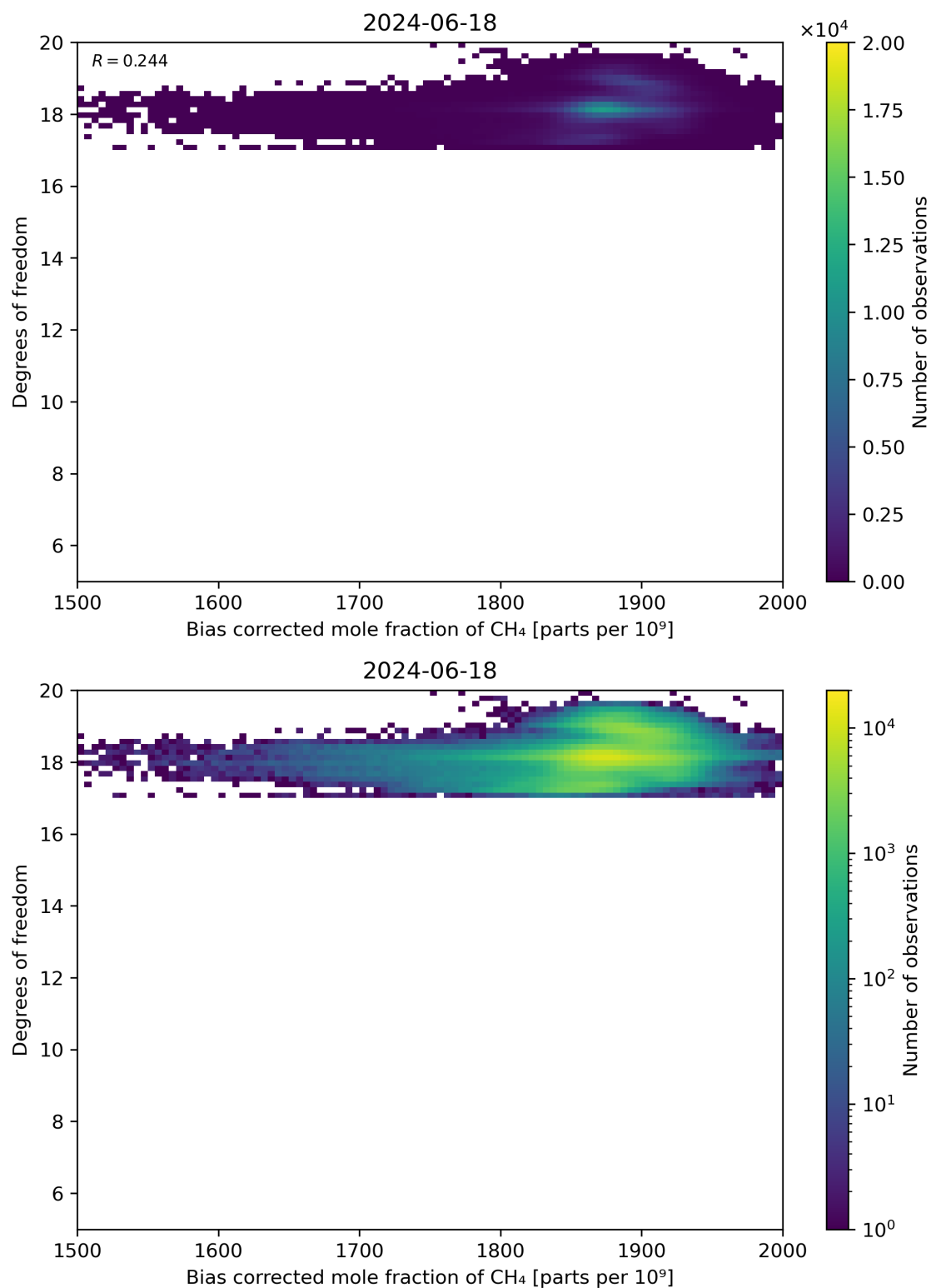
Figure 65: Scatter density plot of “Bias corrected mole fraction of CH 4 ” against “Degrees of freedom” for 2024-06-17 to 2024-06-19.
