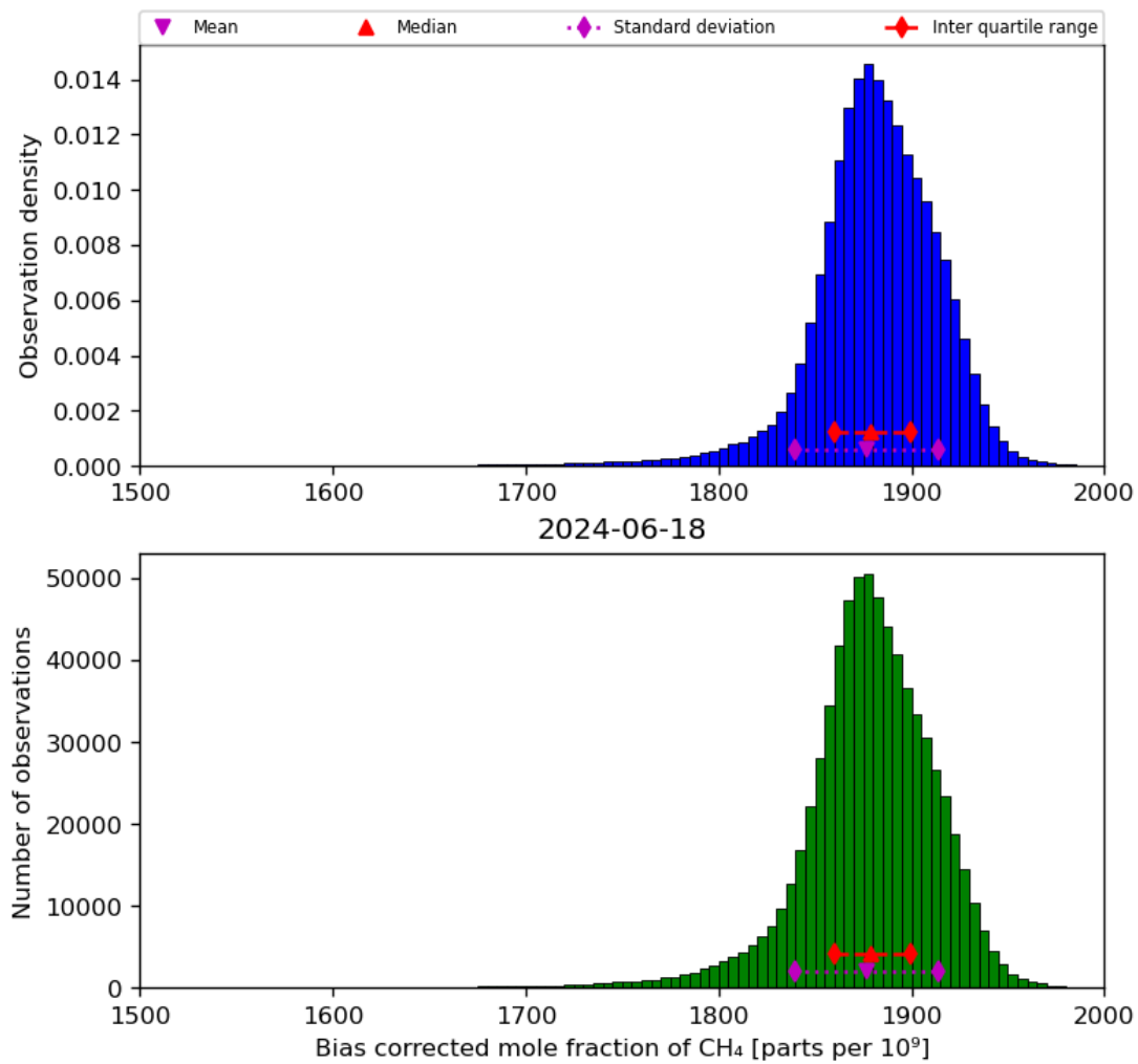
Figure 25: Histogram of “Bias corrected mole fraction of CH 4 ” for 2024-06-17 to 2024-06-19
