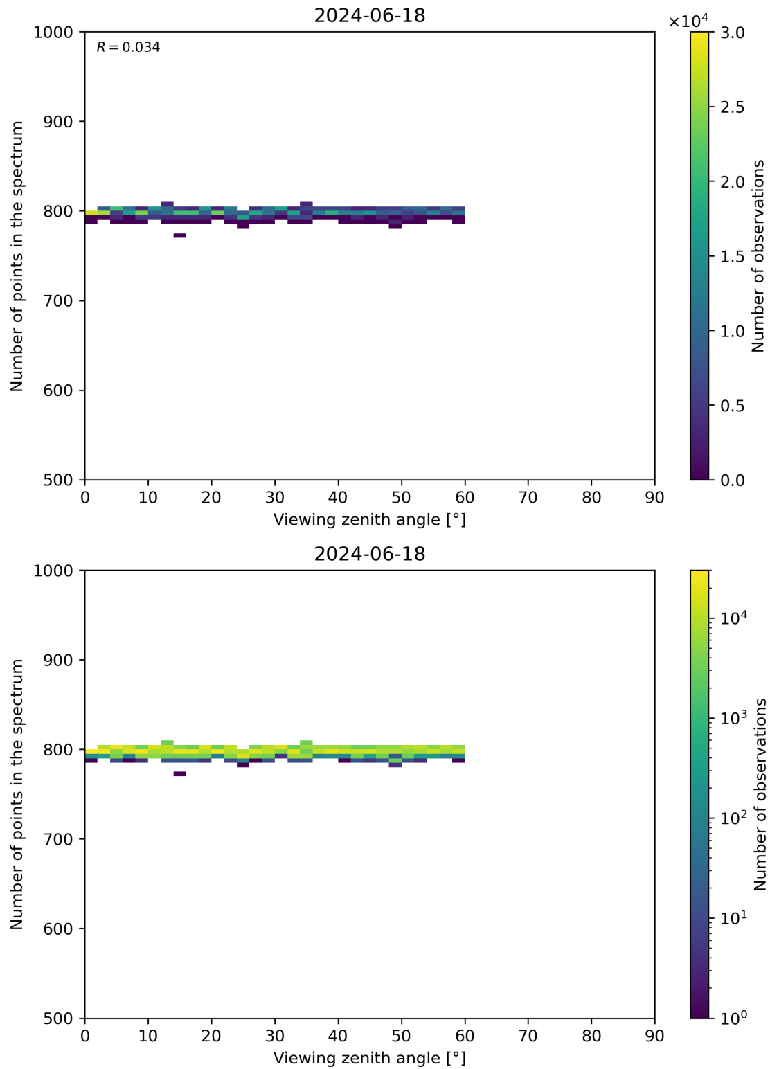
Figure 114: Scatter density plot of “Viewing zenith angle” against “Number of points in the spectrum” for 2024-06-17 to 2024-06-19.
