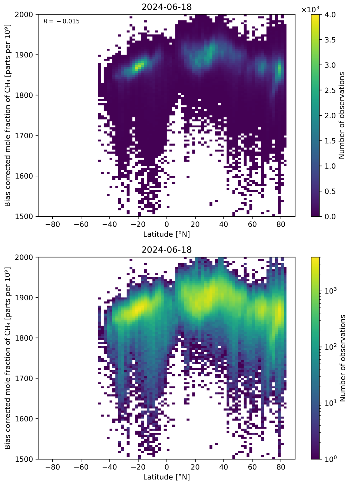
Figure 58: Scatter density plot of “Latitude” against “Bias corrected mole fraction of \text{CH}_4 ” for 2024-06-17 to 2024-06-19.
