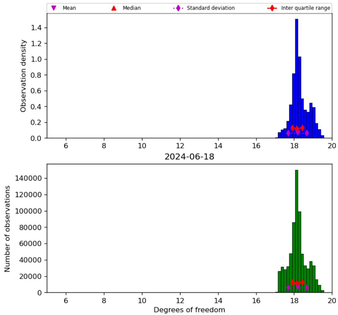
Figure 30: Histogram of “Degrees of freedom” for 2024-06-17 to 2024-06-19
