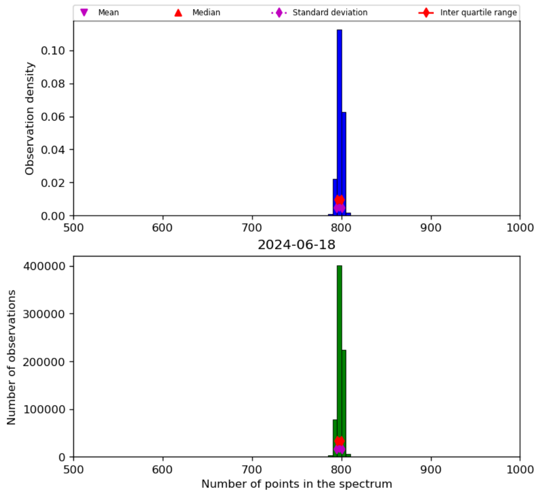
Figure 26: Histogram of “Number of points in the spectrum” for 2024-06-17 to 2024-06-19
