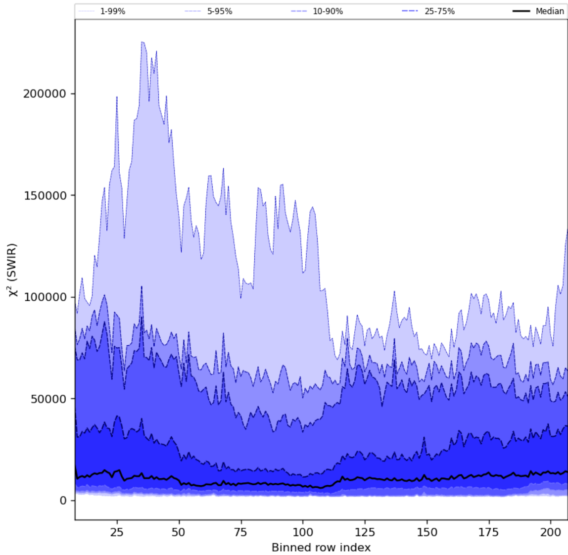
Figure 39: Along track statistics of “ \chi^2 (SWIR)” for 2024-06-17 to 2024-06-19
