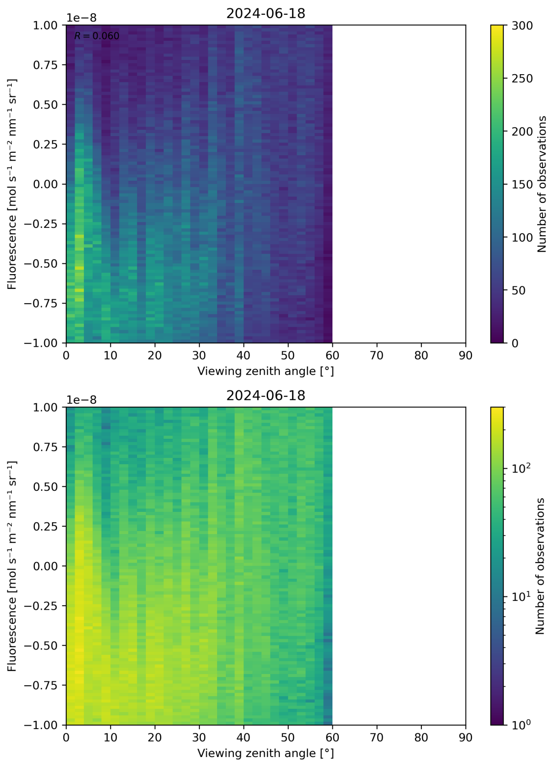
Figure 108: Scatter density plot of “Viewing zenith angle” against “Fluorescence” for 2024-06-17 to 2024-06-19.
