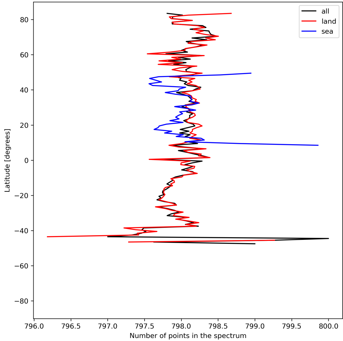
Figure 15: Zonal average of “Number of points in the spectrum” for 2024-06-17 to 2024-06-19.
