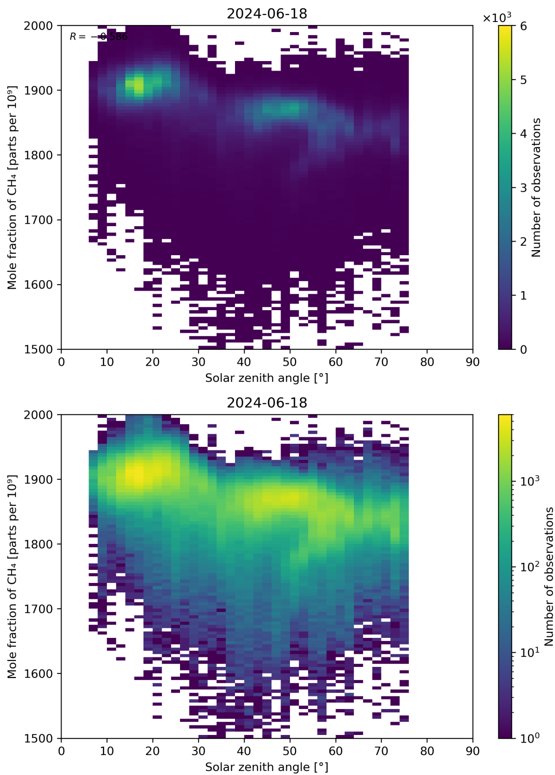
Figure 99: Scatter density plot of “Solar zenith angle” against “Mole fraction of CH 4 ” for 2024-06-17 to 2024-06-19.
