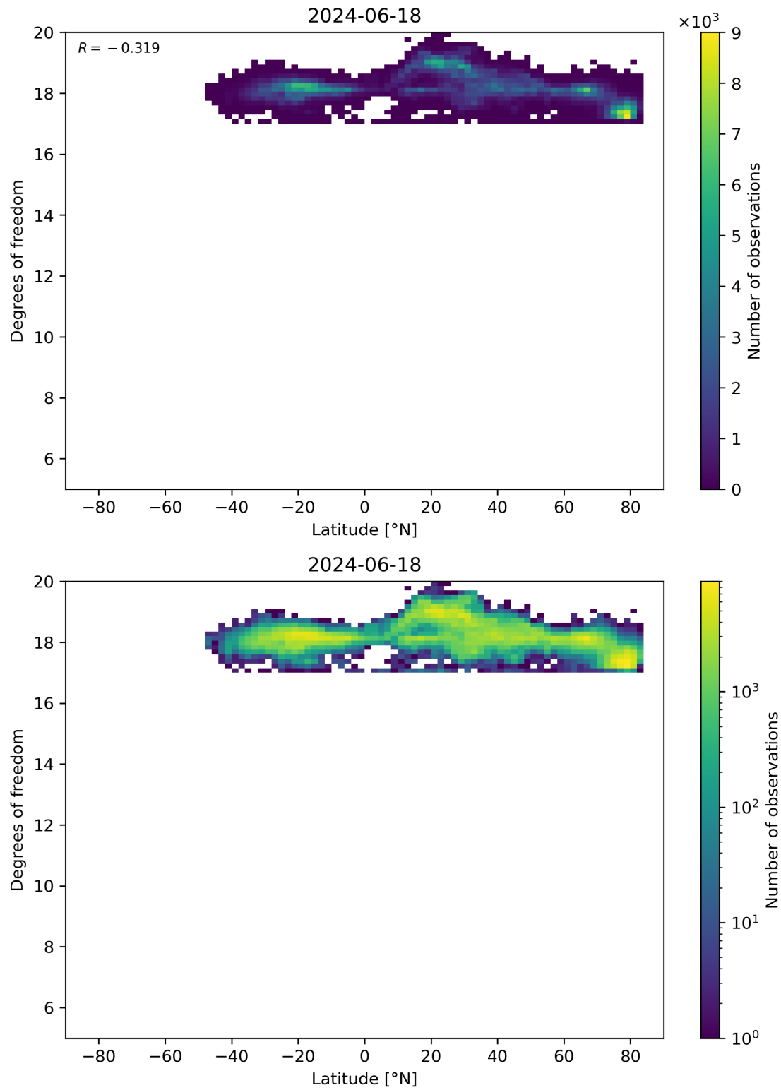
Figure 55: Scatter density plot of “Latitude” against “Degrees of freedom” for 2024-06-17 to 2024-06-19.
