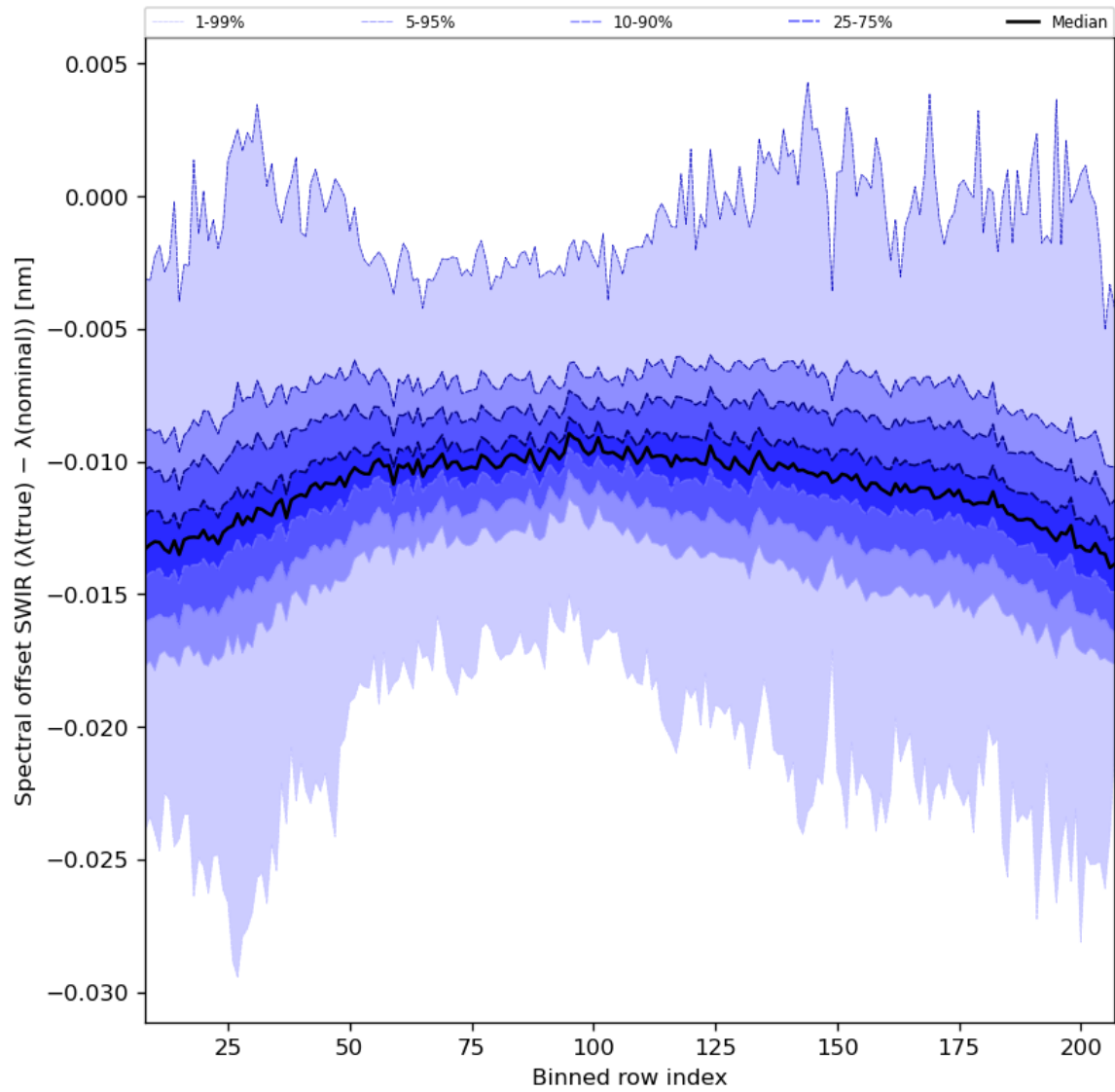
Figure 38: Along track statistics of "Spectral offset SWIR ( \lambda(\text{true}) - \lambda(\text{nominal}) )" for 2024-06-17 to 2024-06-19
