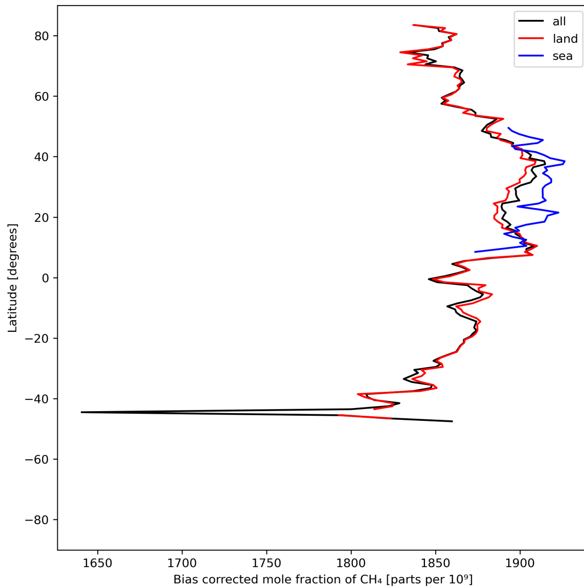
Figure 14: Zonal average of “Bias corrected mole fraction of CH 4 ” for 2024-06-17 to 2024-06-19.
