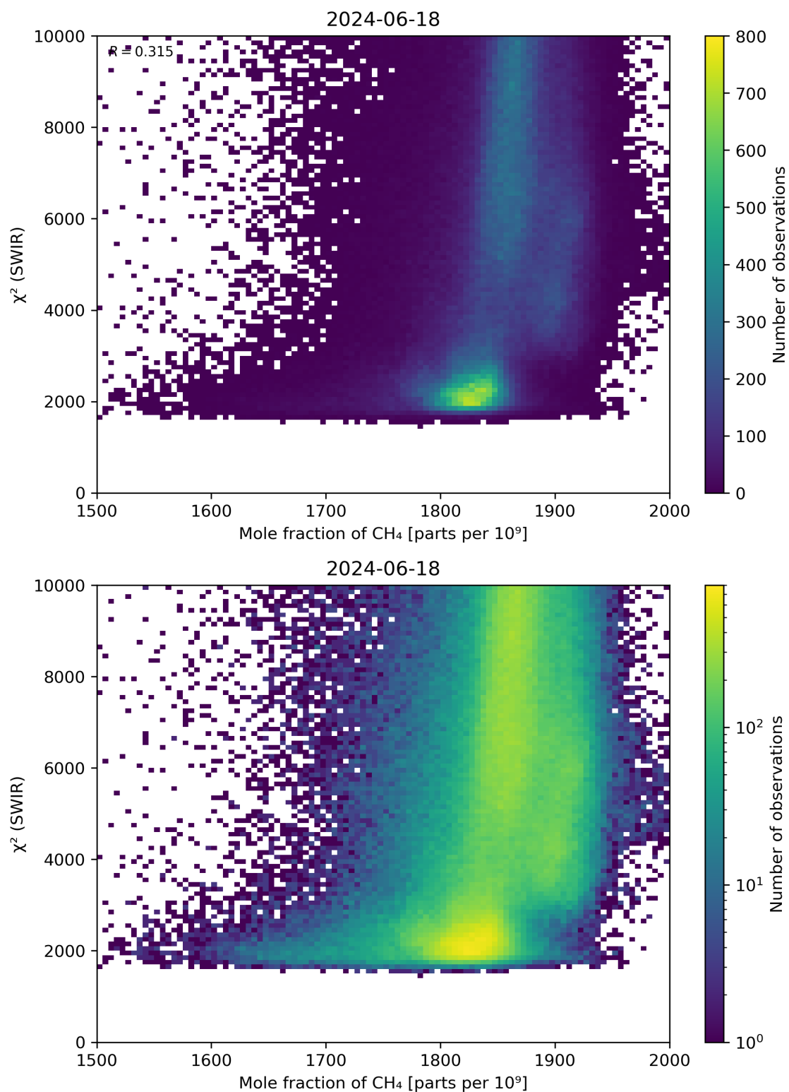
Figure 71: Scatter density plot of “Mole fraction of CH 4 ” against “ \chi^2 (SWIR)” for 2024-06-17 to 2024-06-19.
