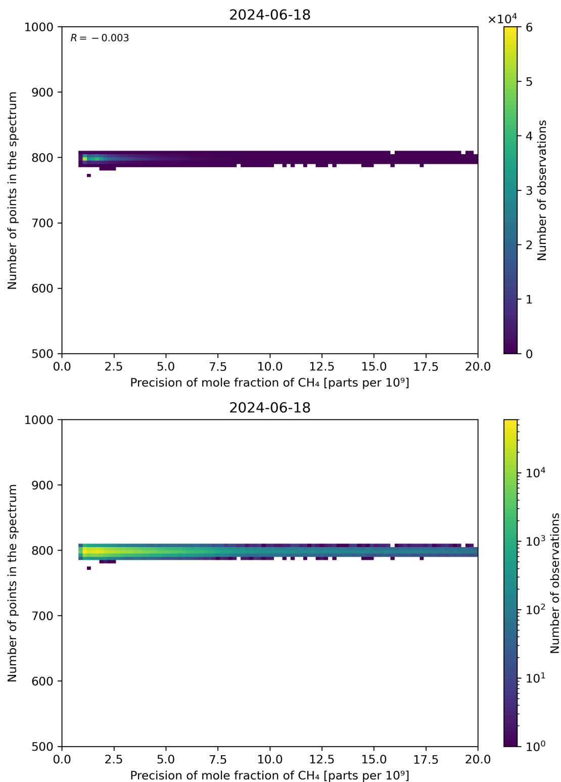
Figure 84: Scatter density plot of “Precision of mole fraction of CH 4 ” against “Number of points in the spectrum” for 2024-06-17 to 2024-06-19.
