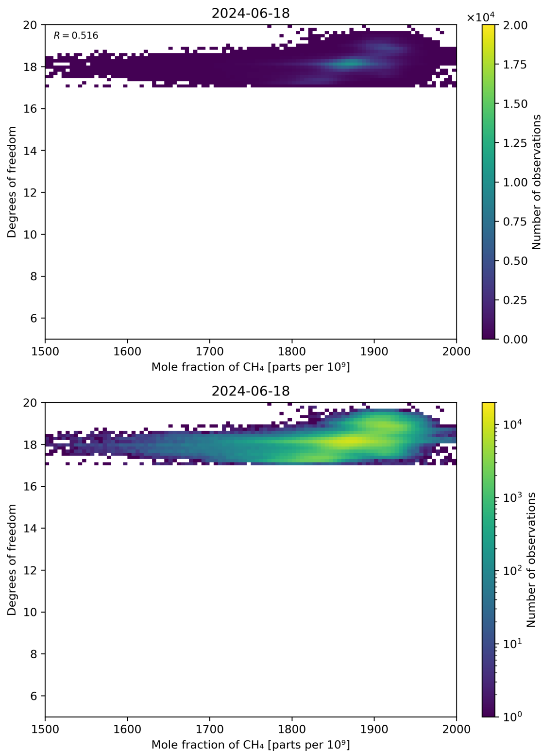
Figure 72: Scatter density plot of “Mole fraction of CH 4 ” against “Degrees of freedom” for 2024-06-17 to 2024-06-19.
