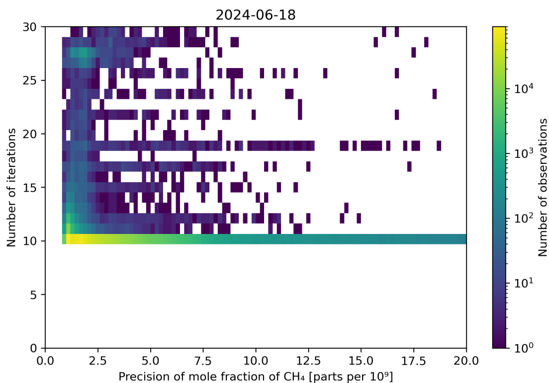
Figure 83: Scatter density plot of “Precision of mole fraction of CH 4 ” against “Number of iterations” for 2024-06-17 to 2024-06-19.
