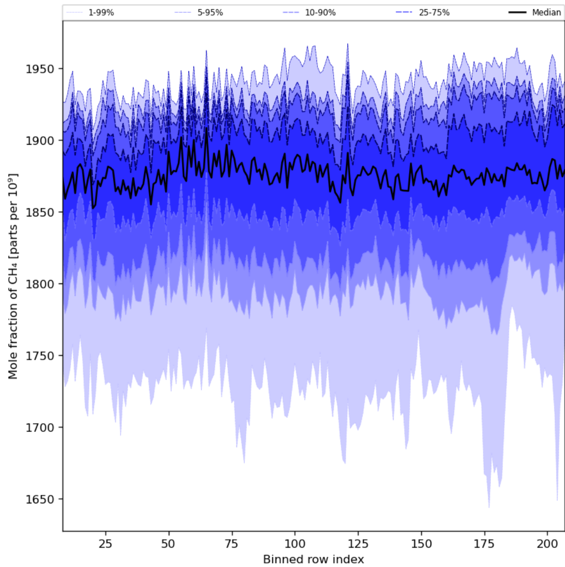
Figure 34: Along track statistics of “Mole fraction of CH 4 ” for 2024-06-17 to 2024-06-19
