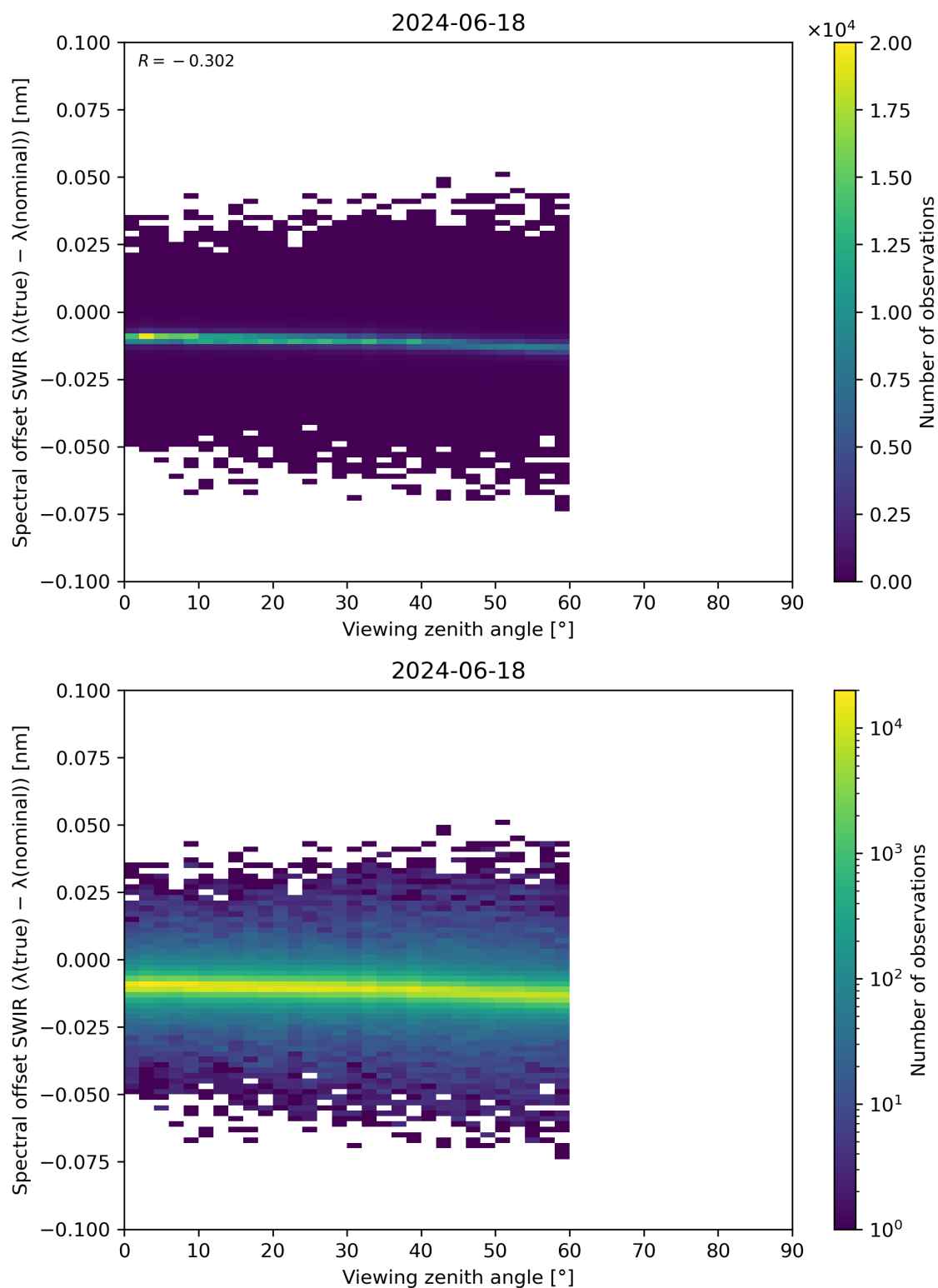
Figure 116: Scatter density plot of “Viewing zenith angle” against “Spectral offset SWIR ( \lambda(\text{true}) - \lambda(\text{nominal}) )” for 2024-06-17 to 2024-06-19.
