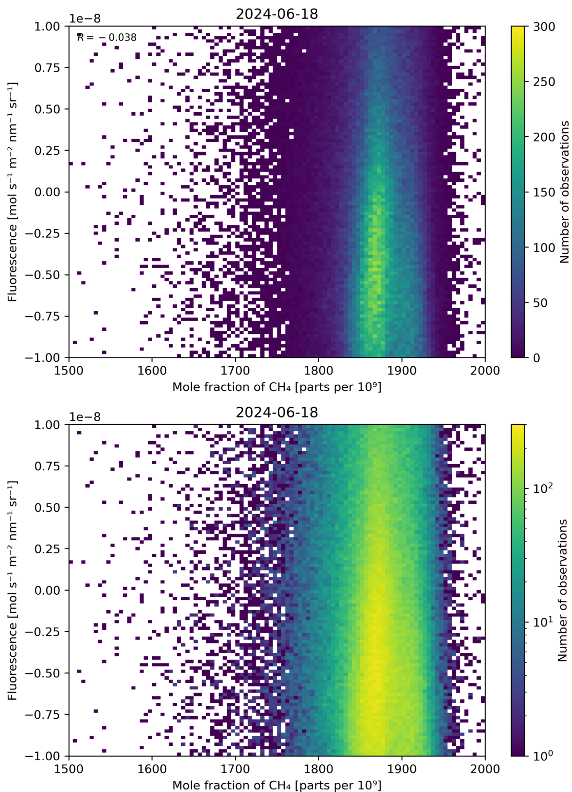
Figure 73: Scatter density plot of “Mole fraction of \text{CH}_4 ” against “Fluorescence” for 2024-06-17 to 2024-06-19.
