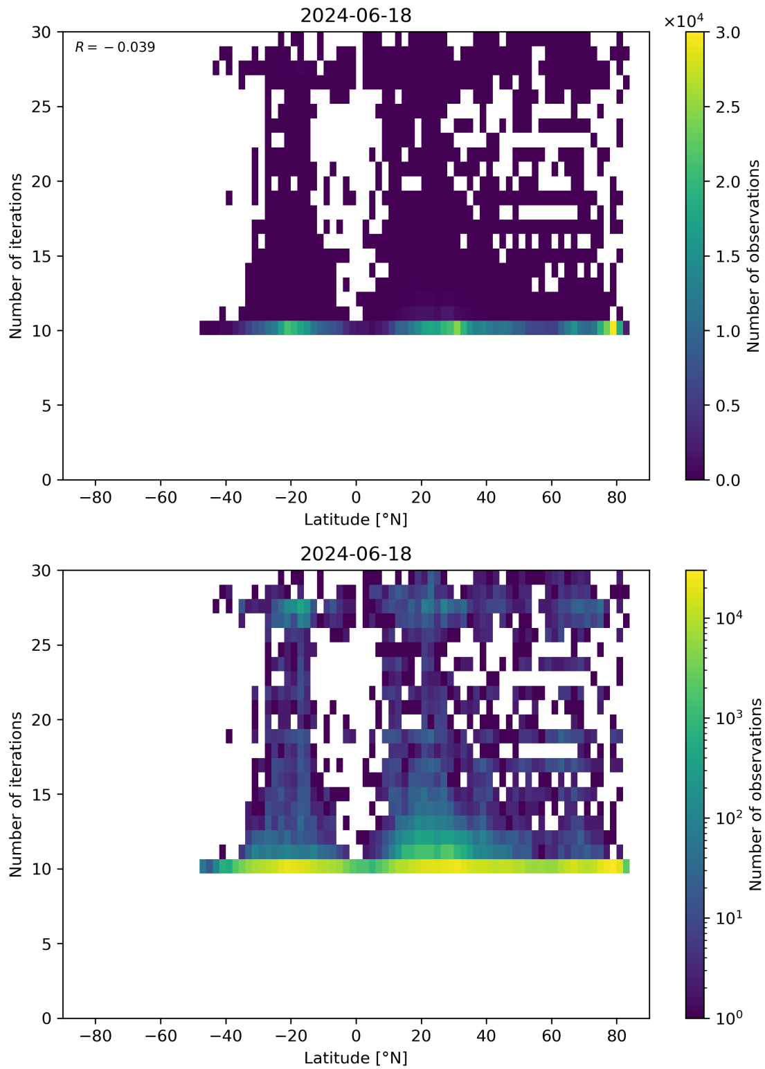
Figure 60: Scatter density plot of “Latitude” against “Number of iterations” for 2024-06-17 to 2024-06-19.
