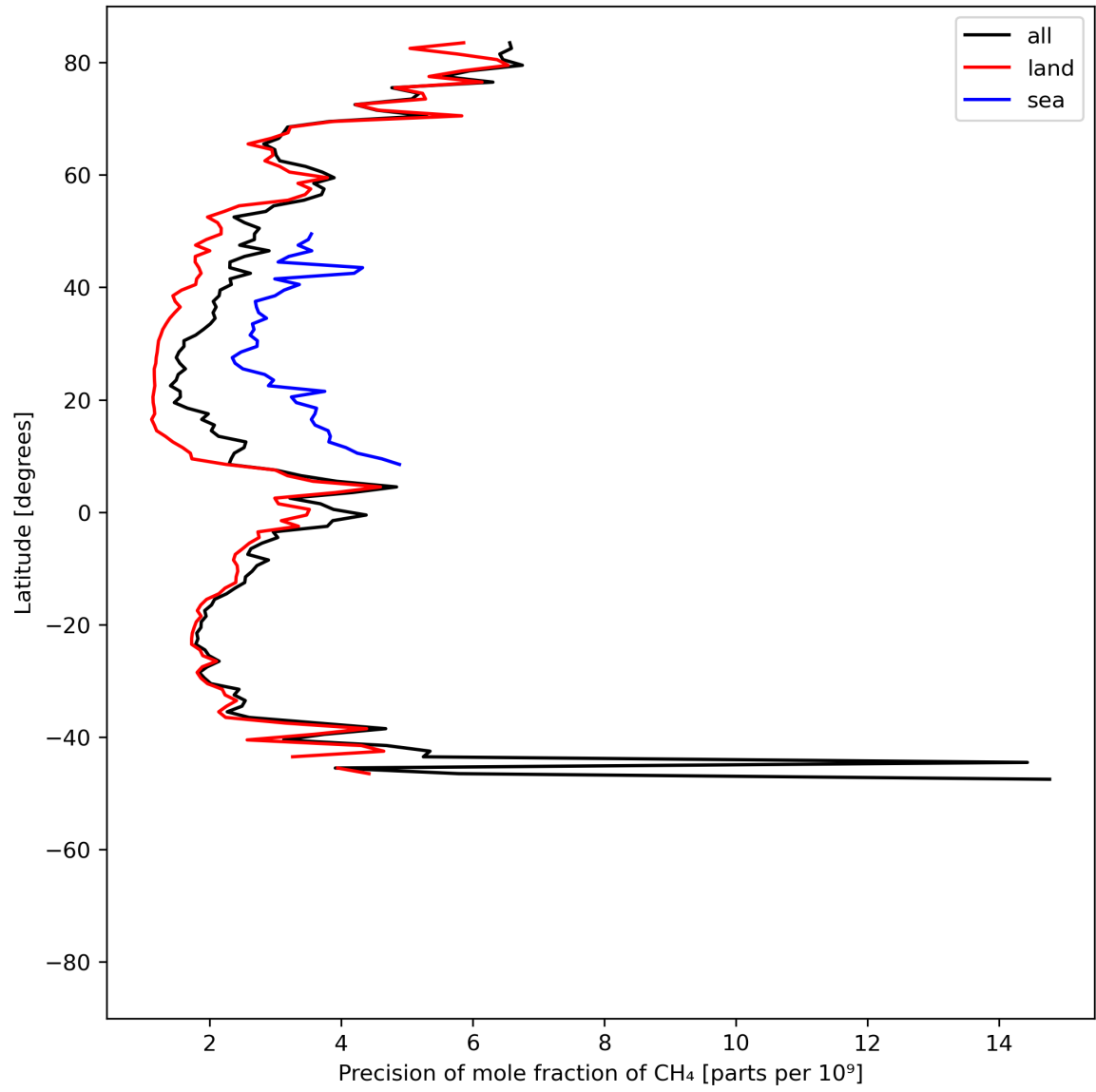
Figure 13: Zonal average of “Precision of mole fraction of \text{CH}_4 ” for 2024-06-17 to 2024-06-19.
