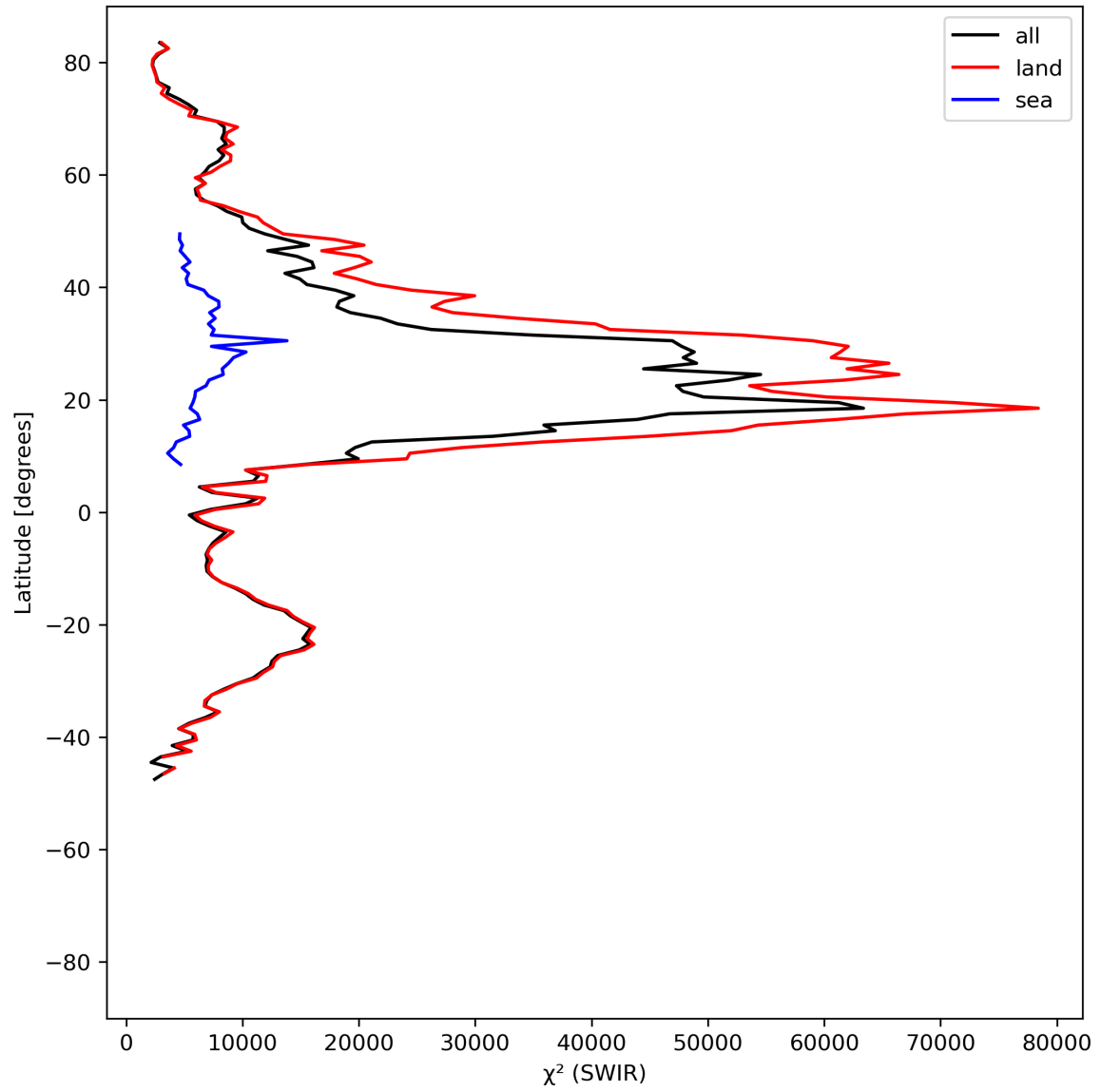
Figure 17: Zonal average of “ \chi^2 (SWIR)” for 2024-06-17 to 2024-06-19.
