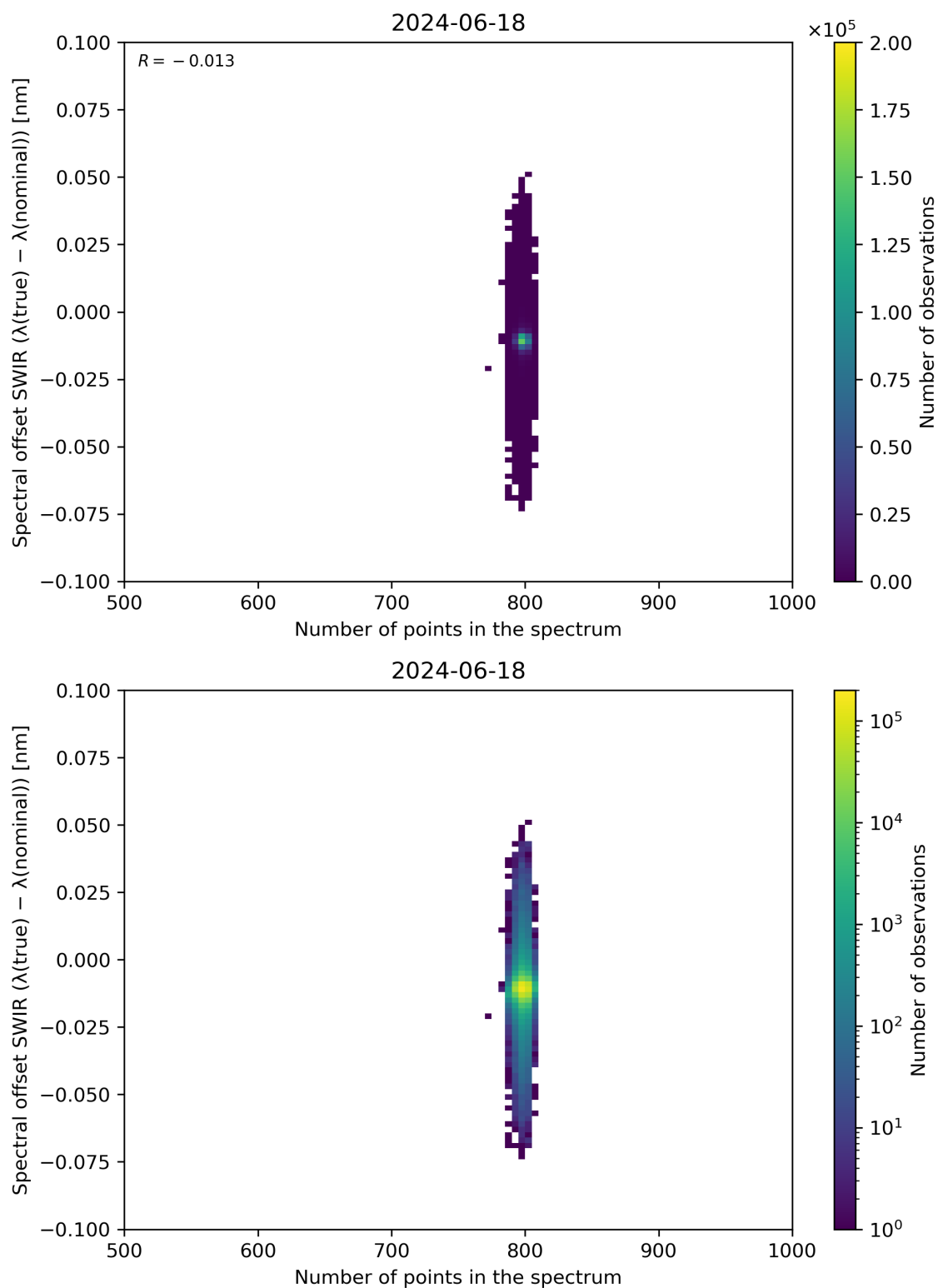
Figure 93: Scatter density plot of “Number of points in the spectrum” against “Spectral offset SWIR ( \lambda(\text{true}) - \lambda(\text{nominal}) )” for 2024-06-17 to 2024-06-19.
