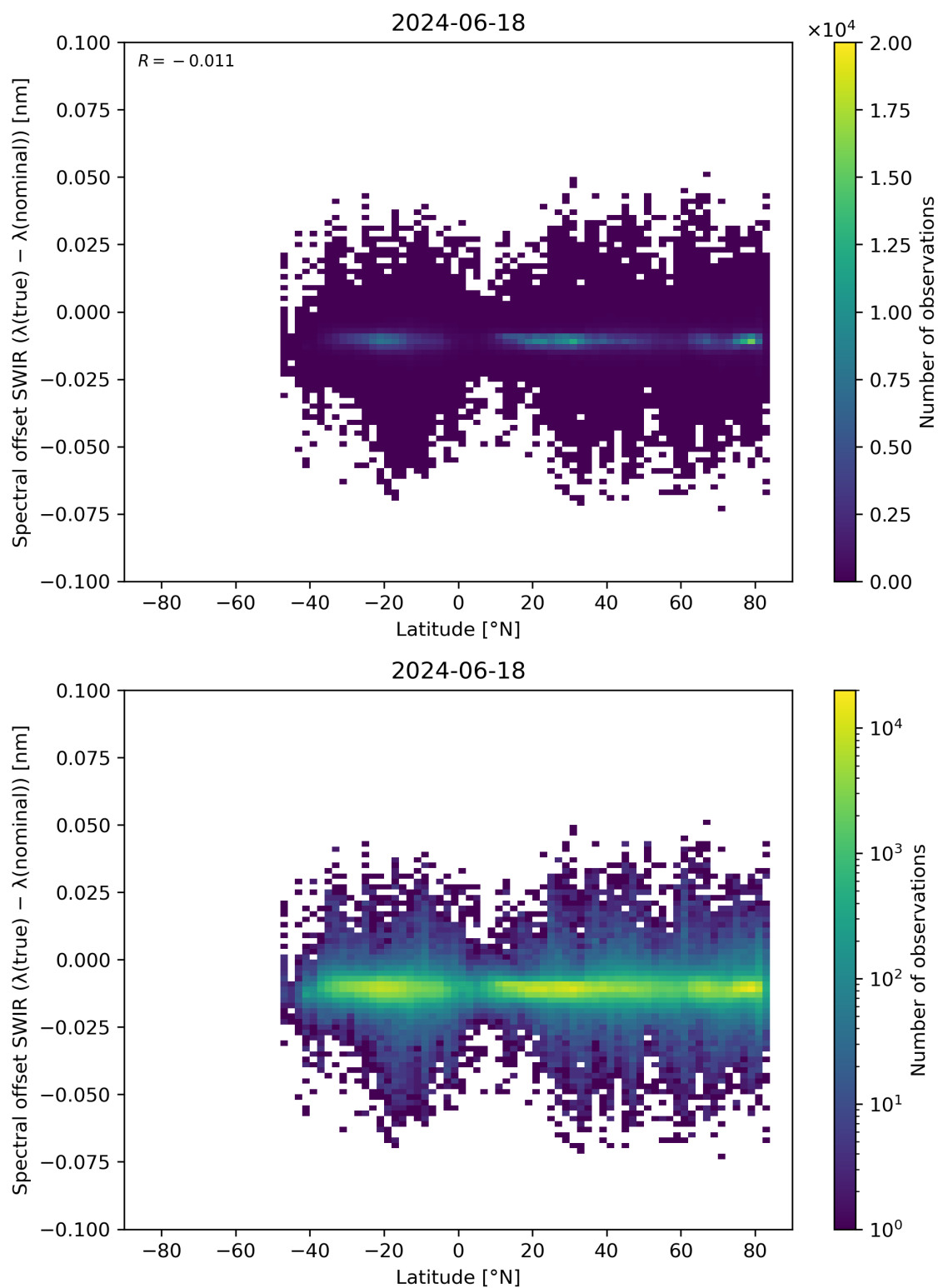
Figure 62: Scatter density plot of “Latitude” against “Spectral offset SWIR ( \lambda(\text{true}) - \lambda(\text{nominal}) )” for 2024-06-17 to 2024-06-19.
