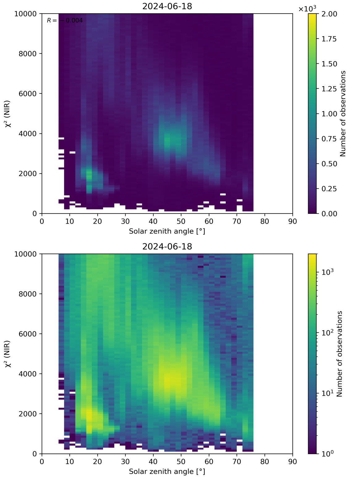
Figure 94: Scatter density plot of “Solar zenith angle” against “ \chi^2 (NIR)” for 2024-06-17 to 2024-06-19.
