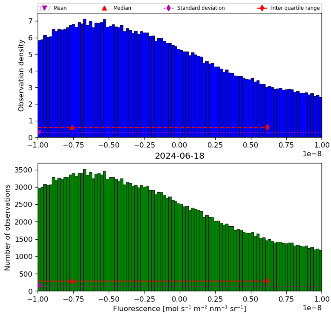
Figure 32: Histogram of “Fluorescence” for 2024-06-17 to 2024-06-19
