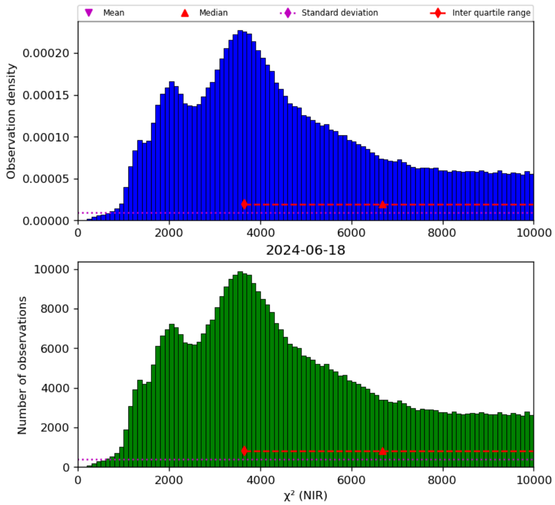
Figure 29: Histogram of “ \chi^2 (NIR)” for 2024-06-17 to 2024-06-19
