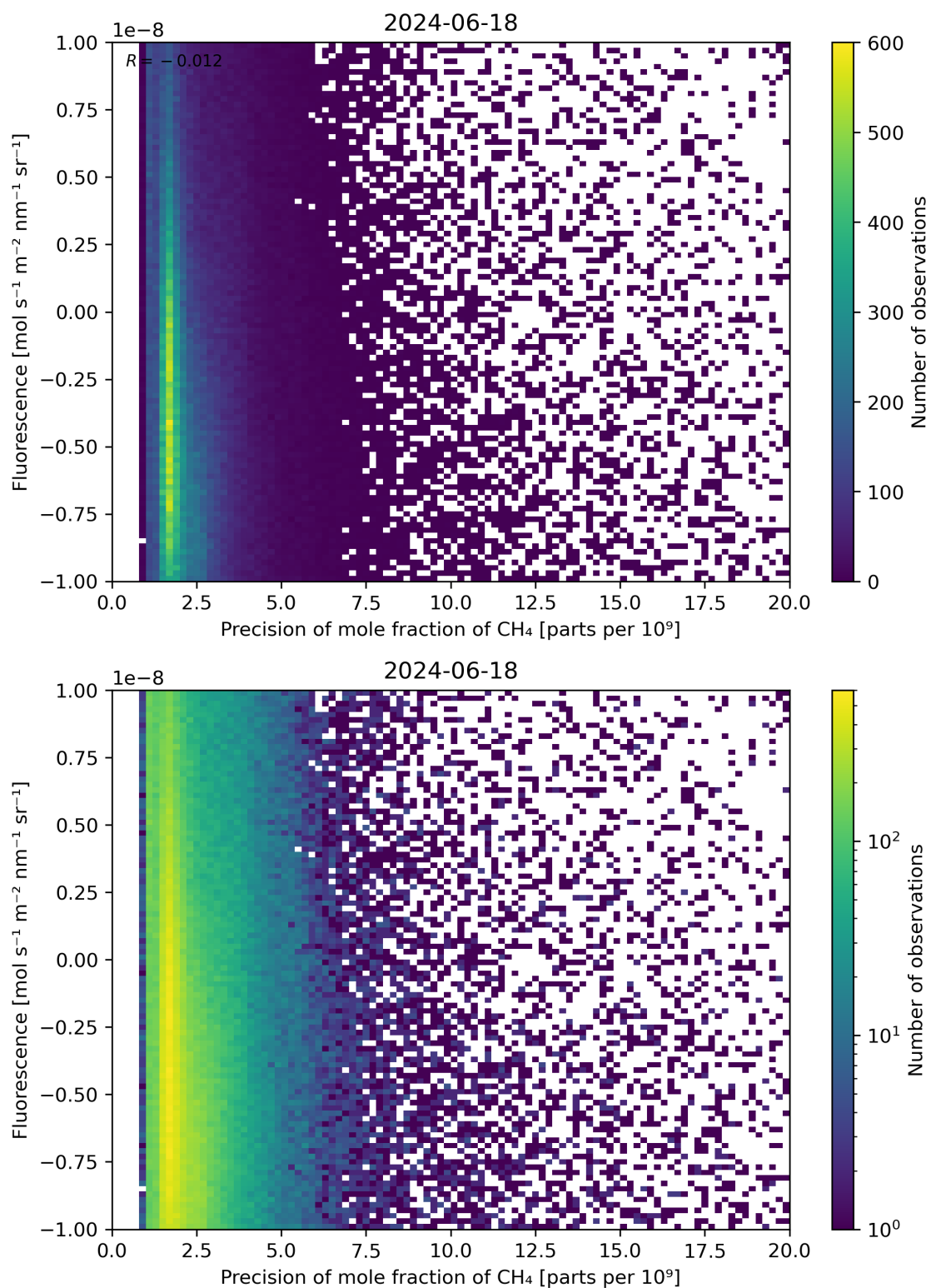
Figure 81: Scatter density plot of “Precision of mole fraction of \text{CH}_4 ” against “Fluorescence” for 2024-06-17 to 2024-06-19.
