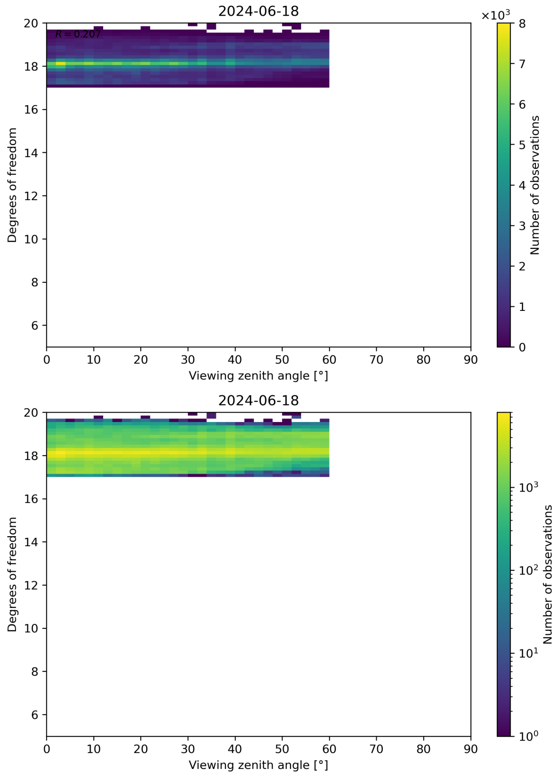
Figure 107: Scatter density plot of “Viewing zenith angle” against “Degrees of freedom” for 2024-06-17 to 2024-06-19.
