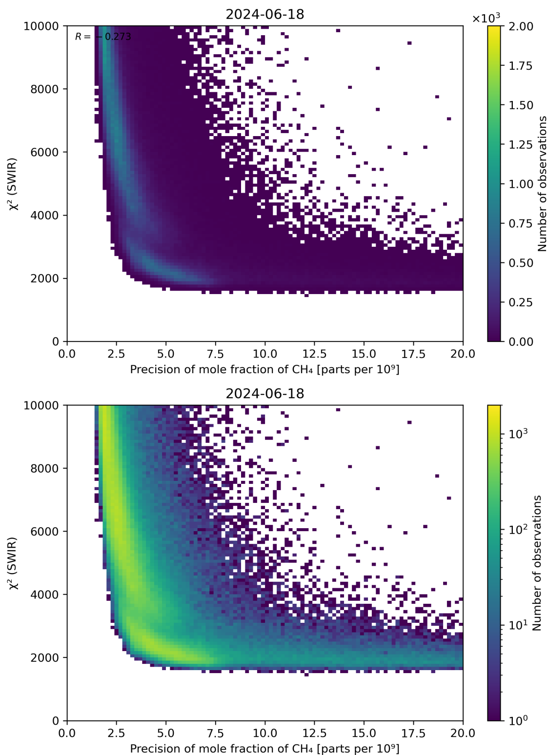
Figure 79: Scatter density plot of “Precision of mole fraction of \text{CH}_4 ” against “ \chi^2 (SWIR)” for 2024-06-17 to 2024-06-19.
