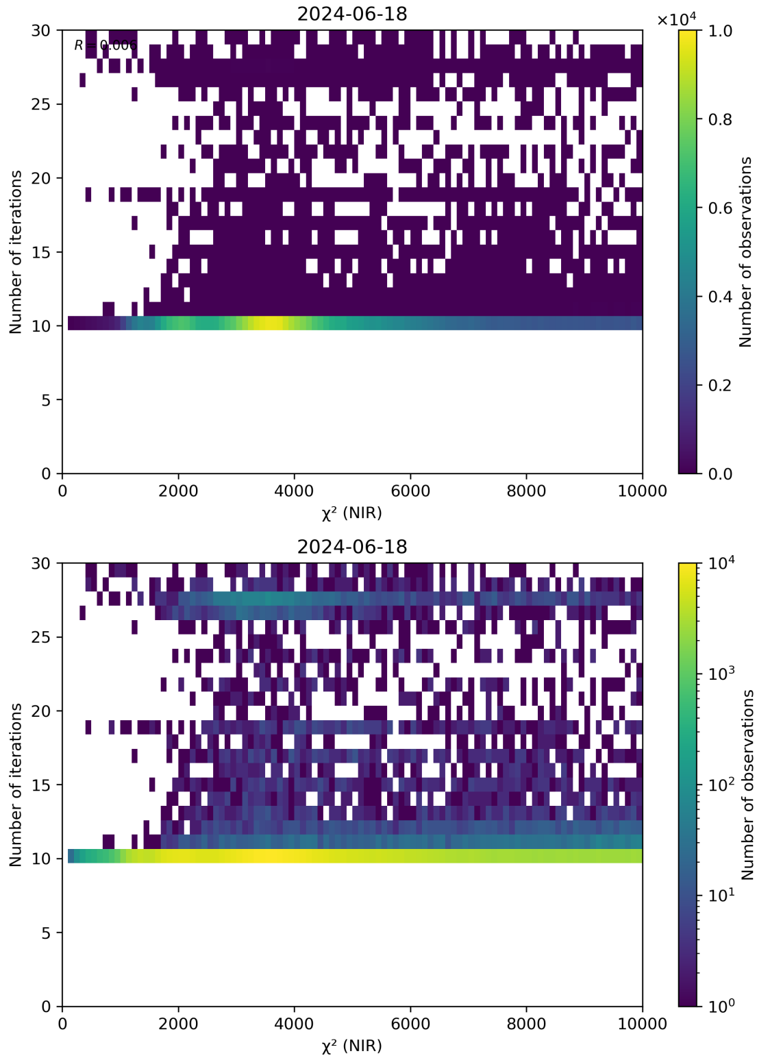
Figure 46: Scatter density plot of “ \chi^2 (NIR)” against “Number of iterations” for 2024-06-17 to 2024-06-19.
