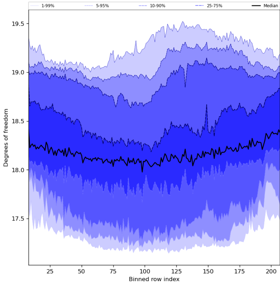
Figure 41: Along track statistics of “Degrees of freedom” for 2024-06-17 to 2024-06-19
