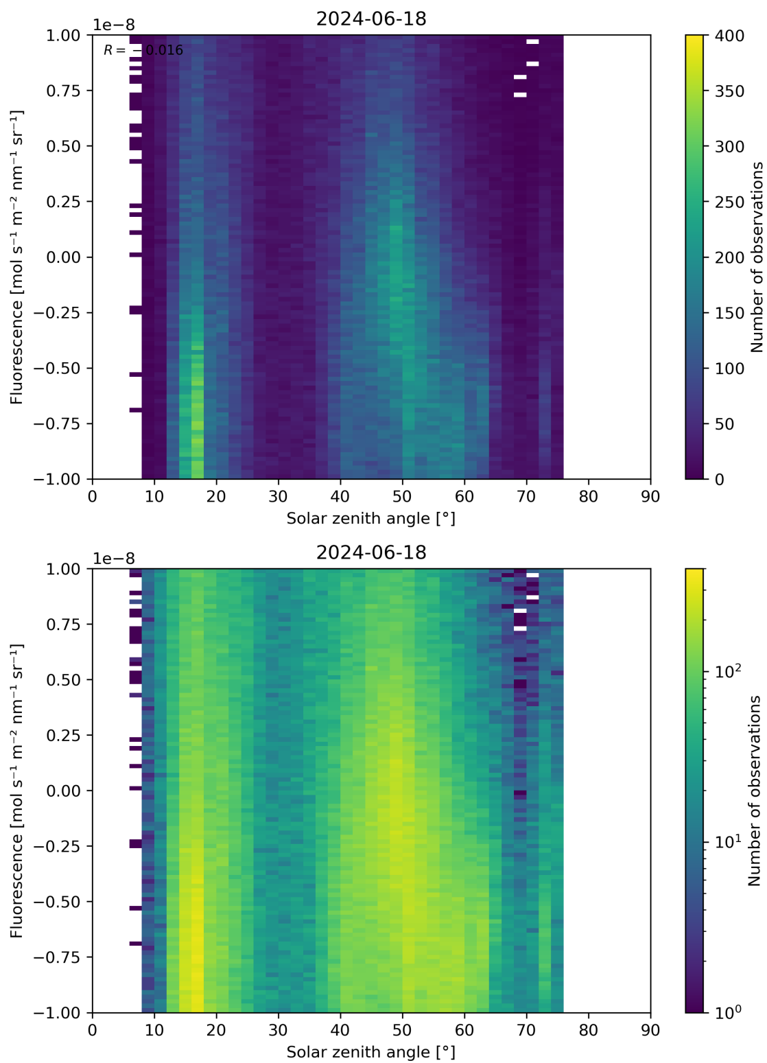
Figure 97: Scatter density plot of “Solar zenith angle” against “Fluorescence” for 2024-06-17 to 2024-06-19.
