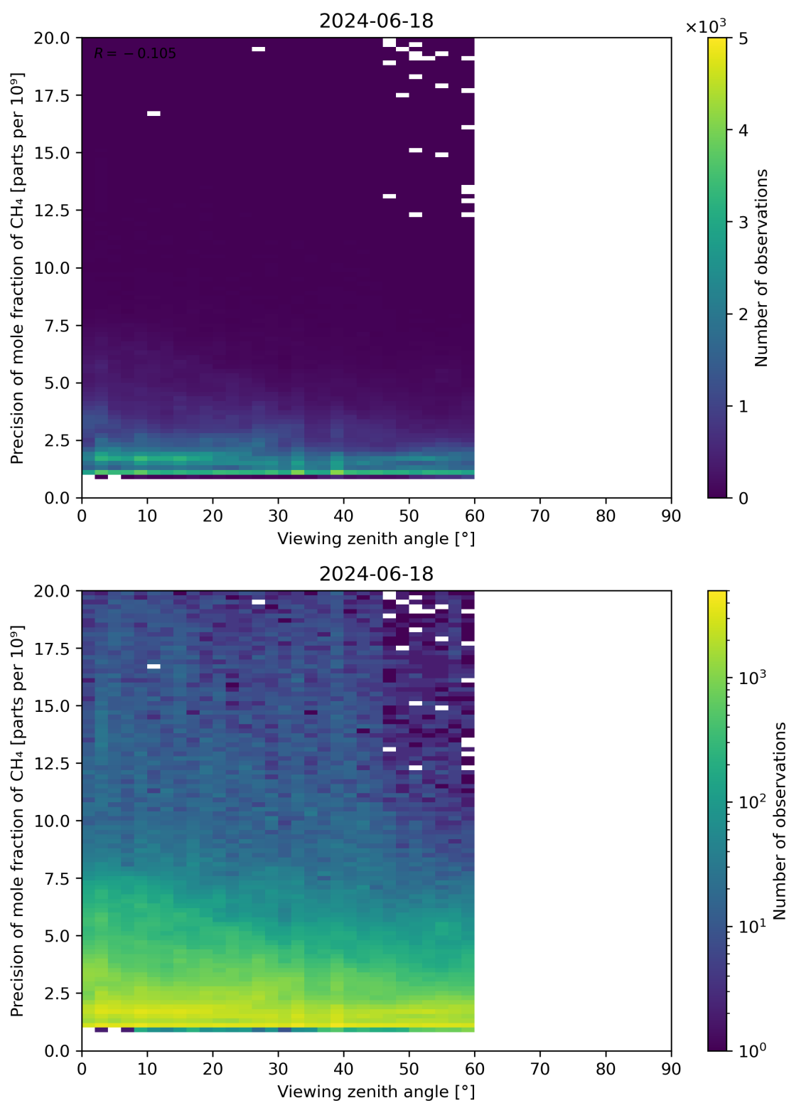
Figure 112: Scatter density plot of “Viewing zenith angle” against “Precision of mole fraction of CH 4 ” for 2024-06-17 to 2024-06-19.
