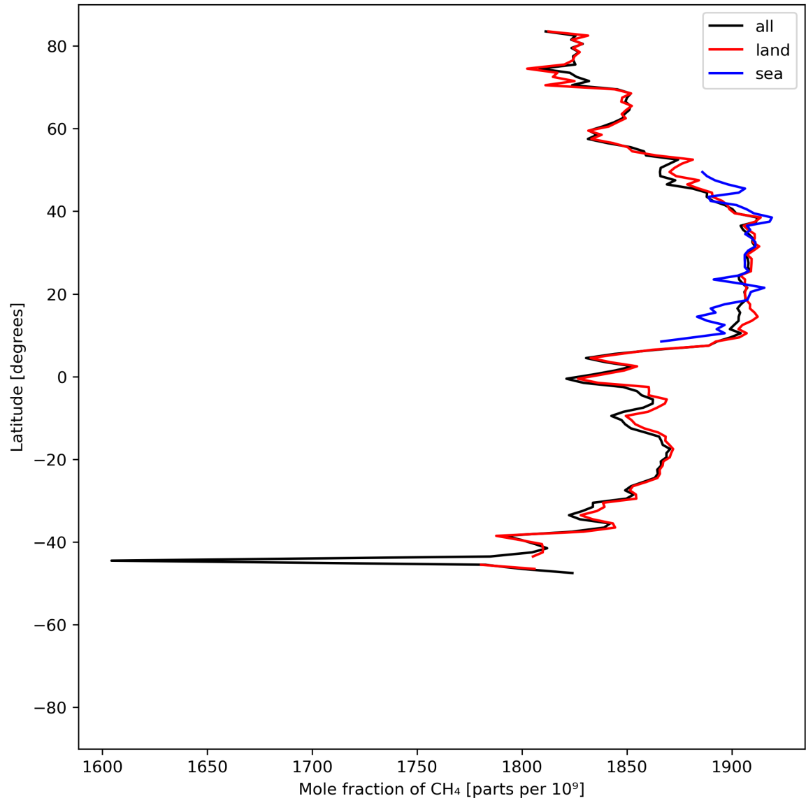
Figure 12: Zonal average of “Mole fraction of \text{CH}_4 ” for 2024-06-17 to 2024-06-19.
