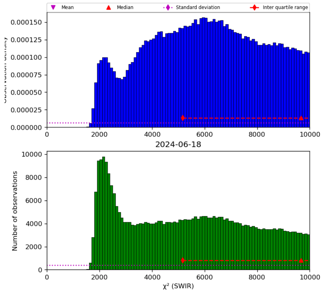
Figure 28: Histogram of “ \chi^2 (SWIR)” for 2024-06-17 to 2024-06-19
