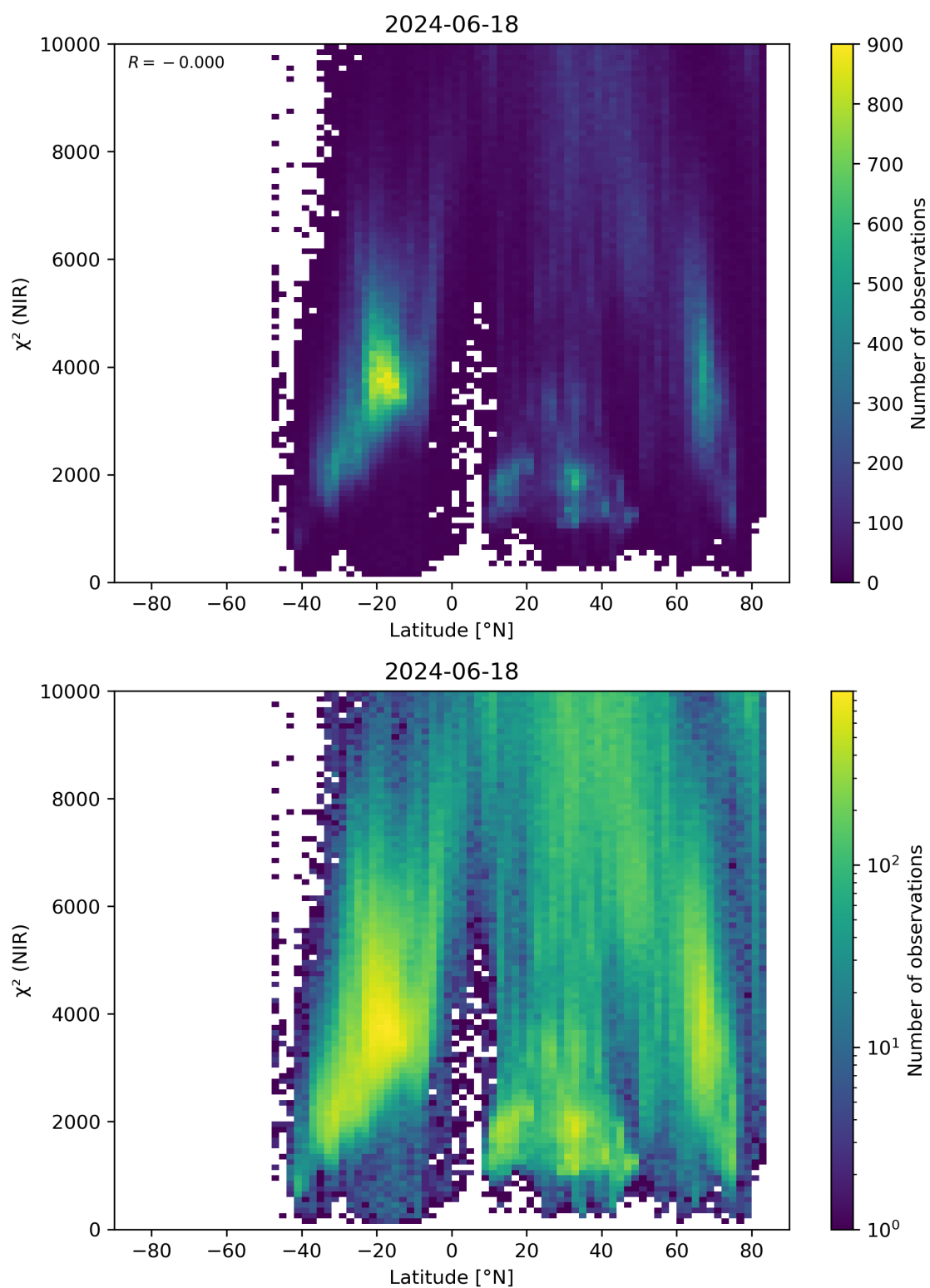
Figure 53: Scatter density plot of “Latitude” against “ \chi^2 (NIR)” for 2024-06-17 to 2024-06-19.
