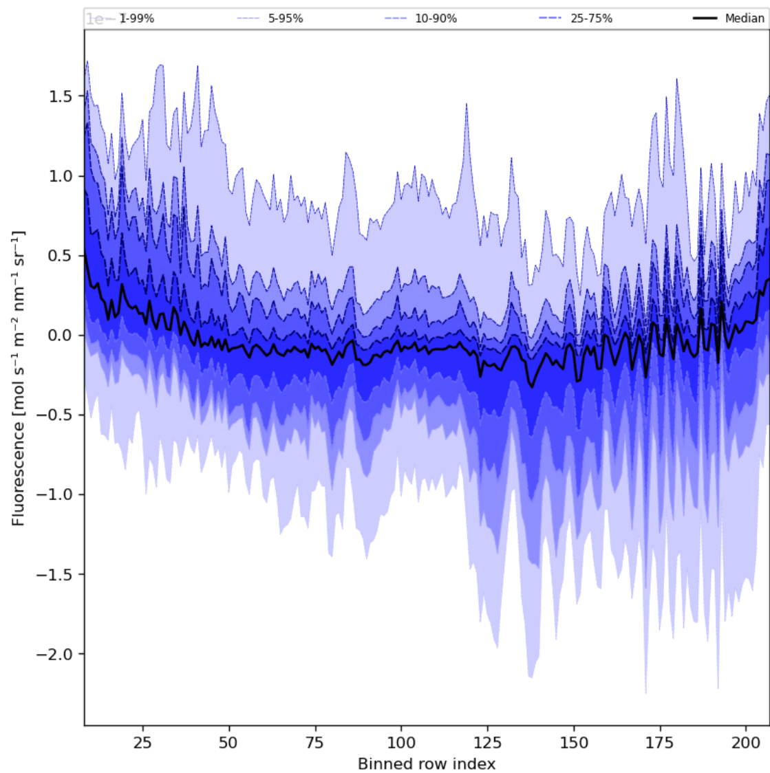
Figure 43: Along track statistics of “Fluorescence” for 2024-06-17 to 2024-06-19
