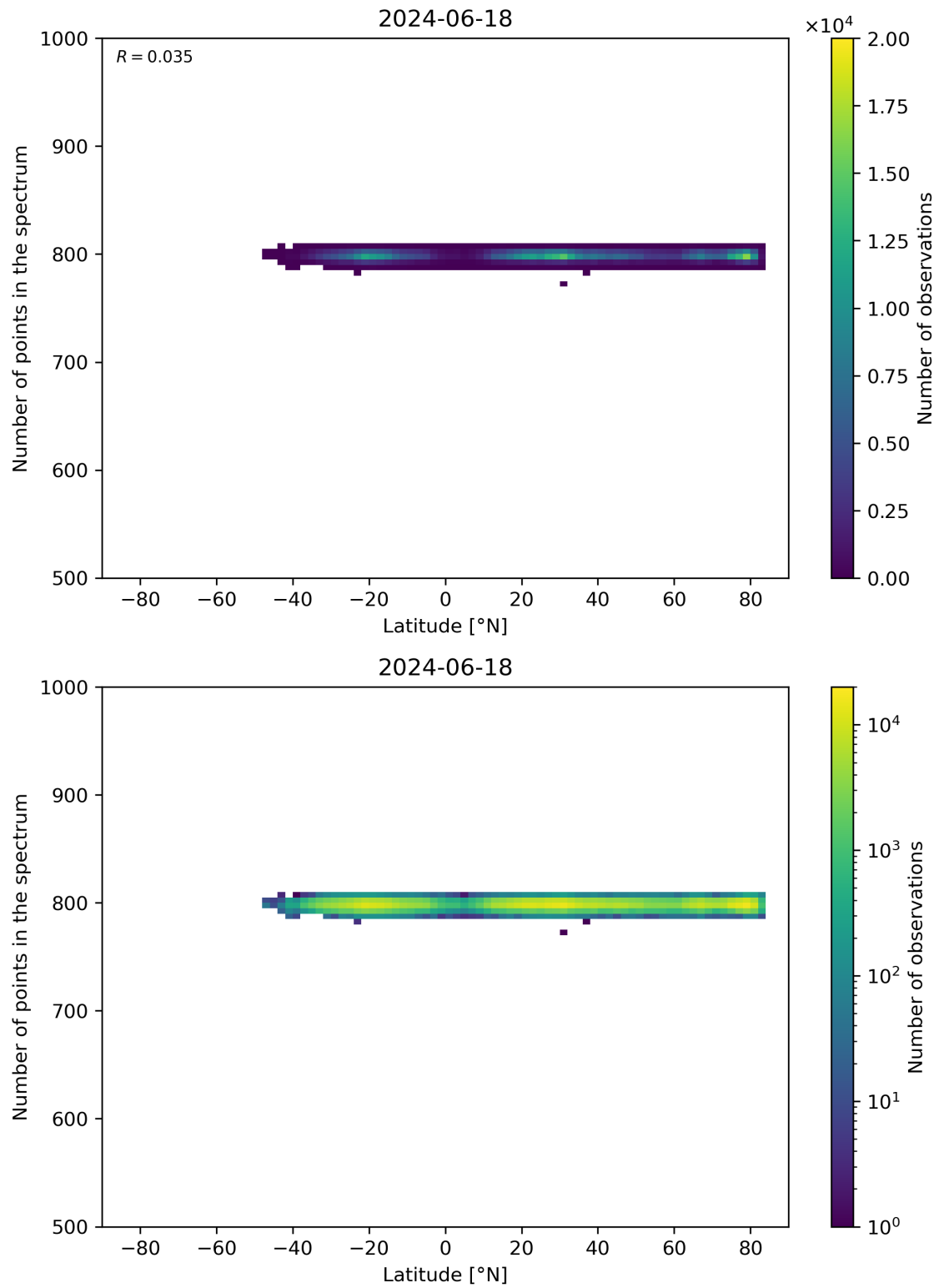
Figure 61: Scatter density plot of “Latitude” against “Number of points in the spectrum” for 2024-06-17 to 2024-06-19.
