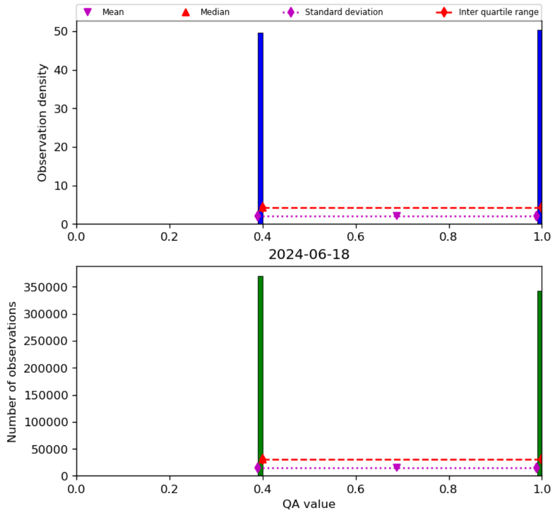
Figure 22: Histogram of “QA value” for 2024-06-17 to 2024-06-19
