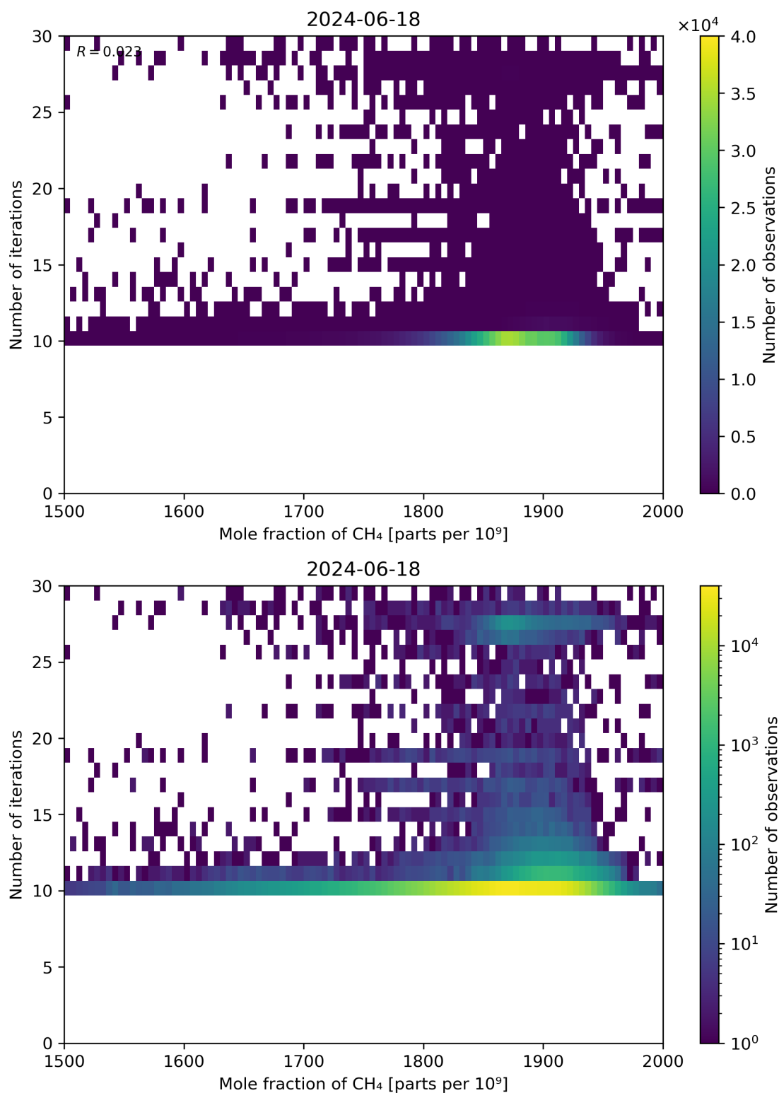
Figure 76: Scatter density plot of “Mole fraction of CH 4 ” against “Number of iterations” for 2024-06-17 to 2024-06-19.
