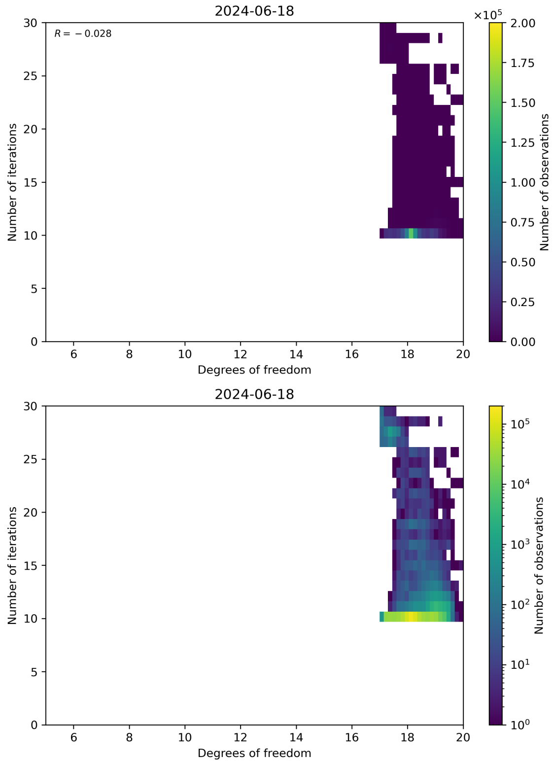
Figure 52: Scatter density plot of “Degrees of freedom” against “Number of iterations” for 2024-06-17 to 2024-06-19.
