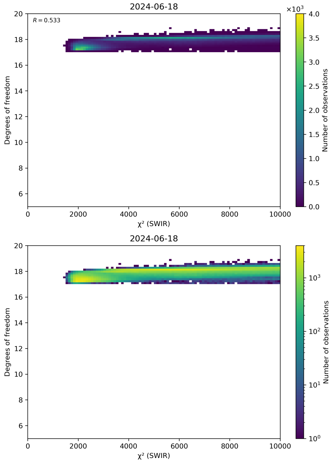
Figure 48: Scatter density plot of “ \chi^2 (SWIR)” against “Degrees of freedom” for 2024-06-17 to 2024-06-19.
