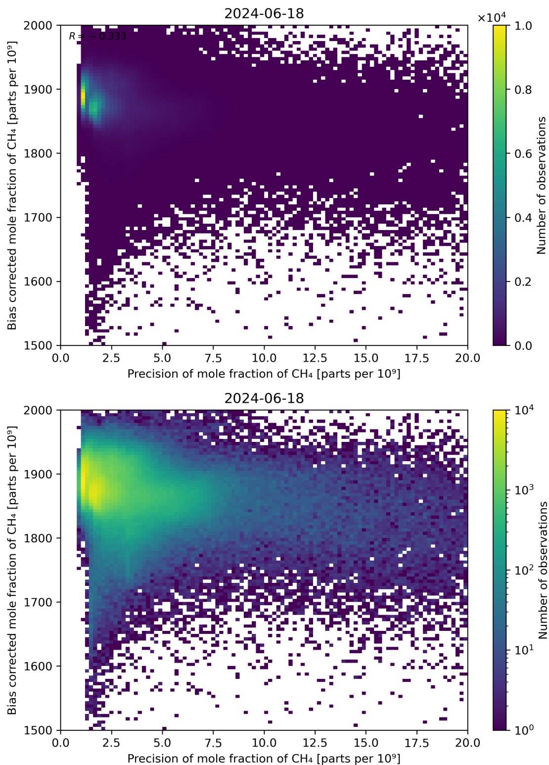
Figure 82: Scatter density plot of “Precision of mole fraction of CH 4 ” against “Bias corrected mole fraction of CH 4 ” for 2024-06-17 to 2024-06-19.
