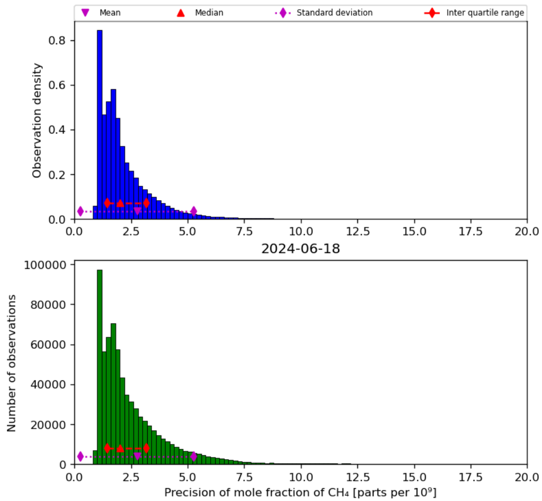
Figure 24: Histogram of “Precision of mole fraction of CH 4 ” for 2024-06-17 to 2024-06-19
