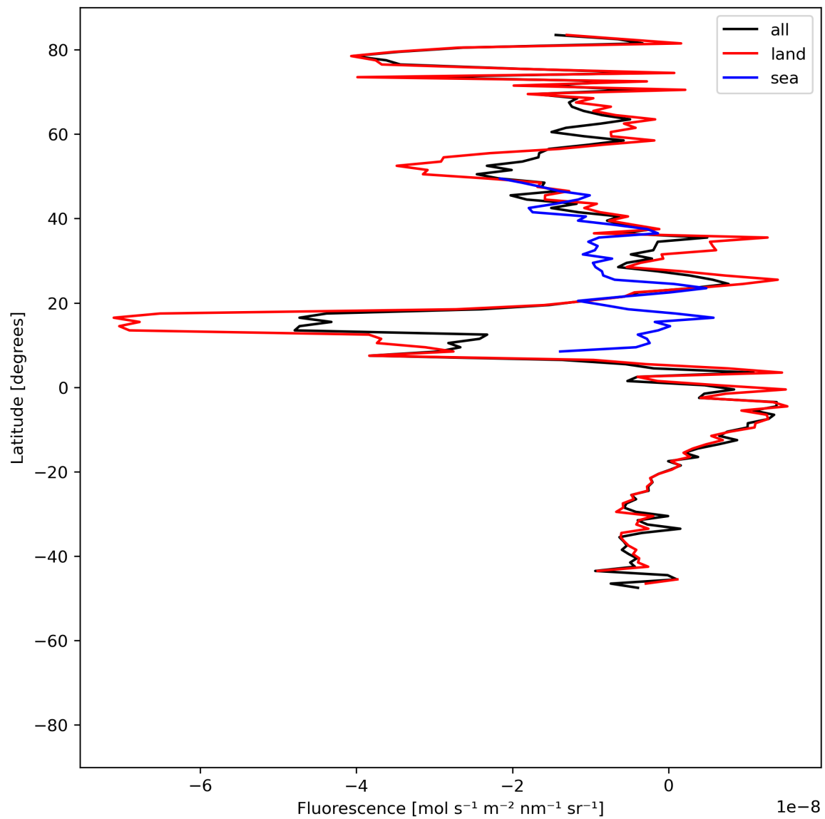
Figure 21: Zonal average of “Fluorescence” for 2024-06-17 to 2024-06-19.
