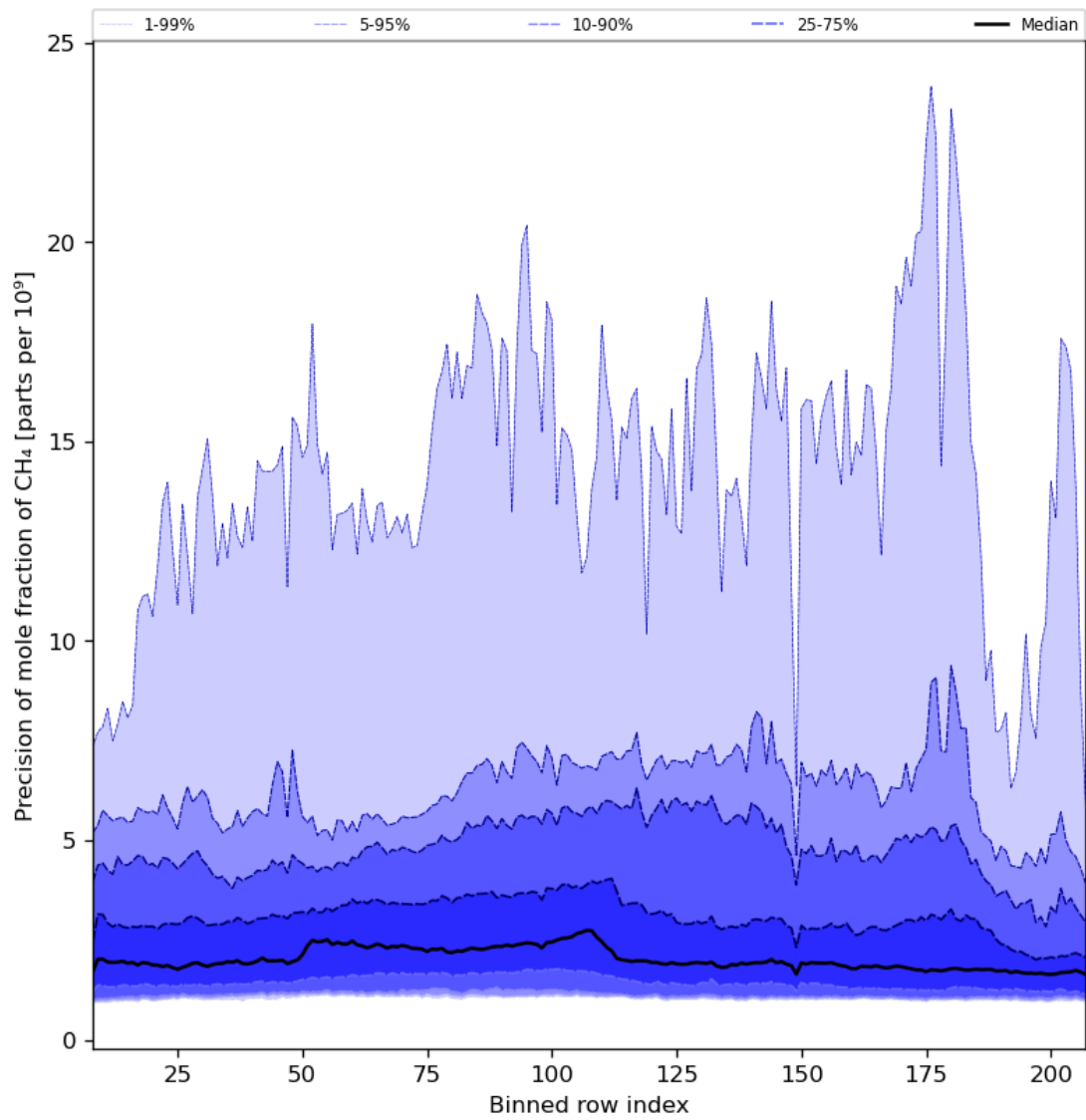
Figure 35: Along track statistics of “Precision of mole fraction of CH 4 ” for 2024-06-17 to 2024-06-19
