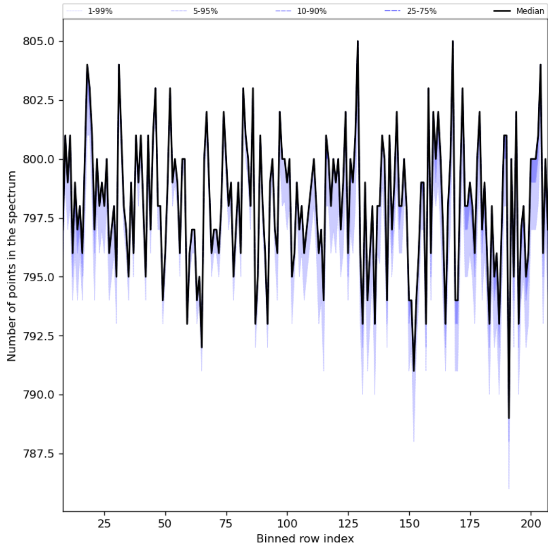
Figure 37: Along track statistics of “Number of points in the spectrum” for 2024-06-17 to 2024-06-19
