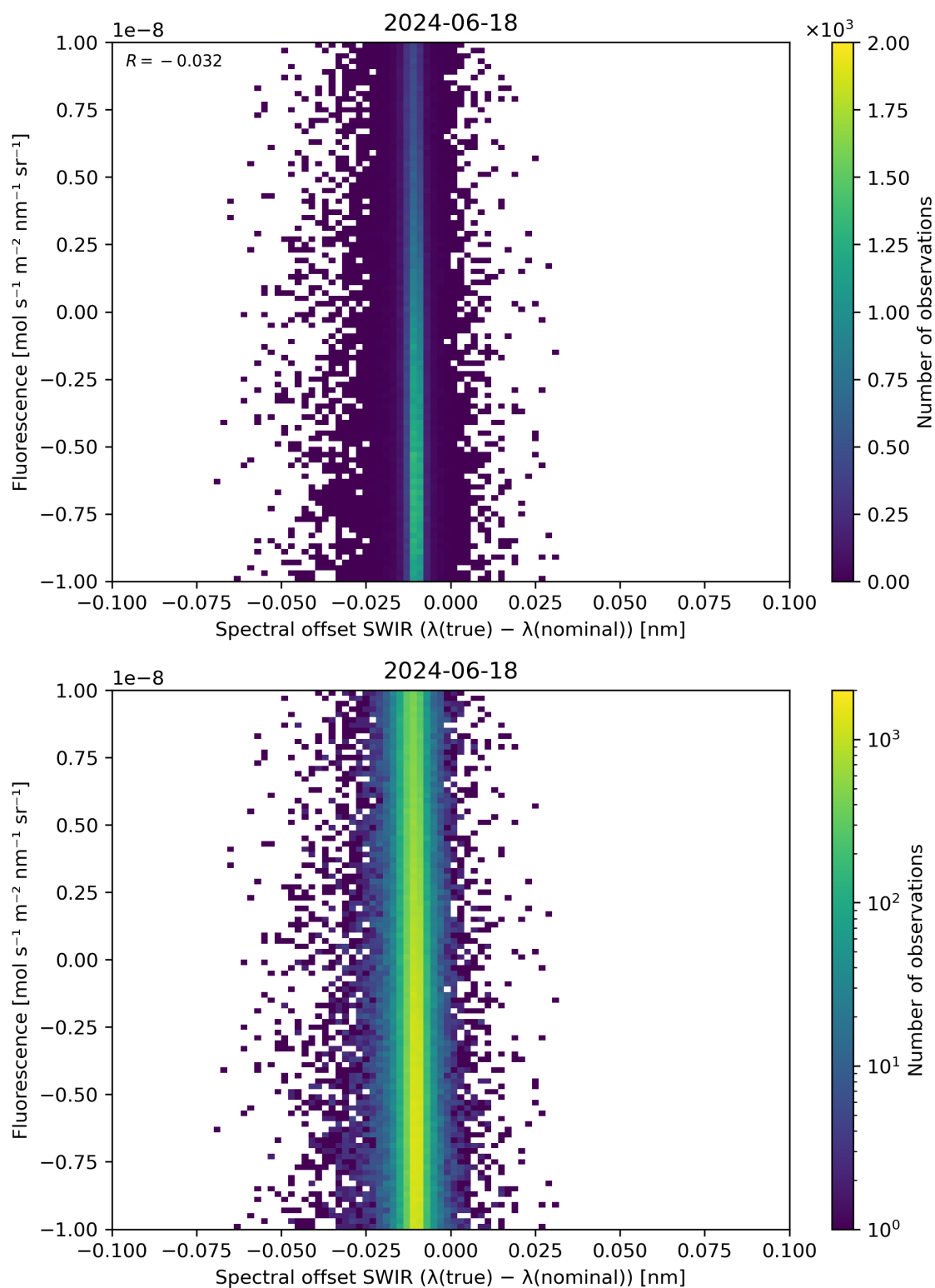
Figure 120: Scatter density plot of “Spectral offset SWIR ( \lambda(\text{true}) - \lambda(\text{nominal}) )” against “Fluorescence” for 2024-06-17 to 2024-06-19.
