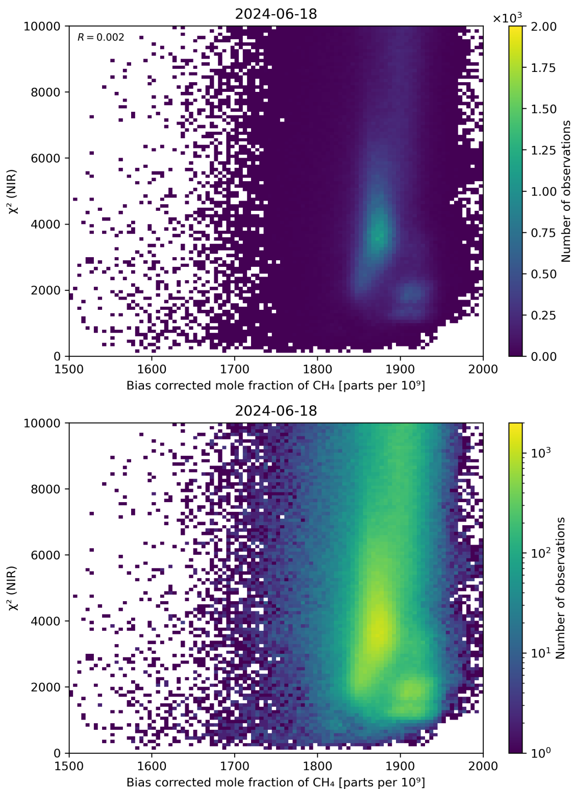
Figure 63: Scatter density plot of “Bias corrected mole fraction of \text{CH}_4 ” against “ \chi^2 (NIR)” for 2024-06-17 to 2024-06-19.
