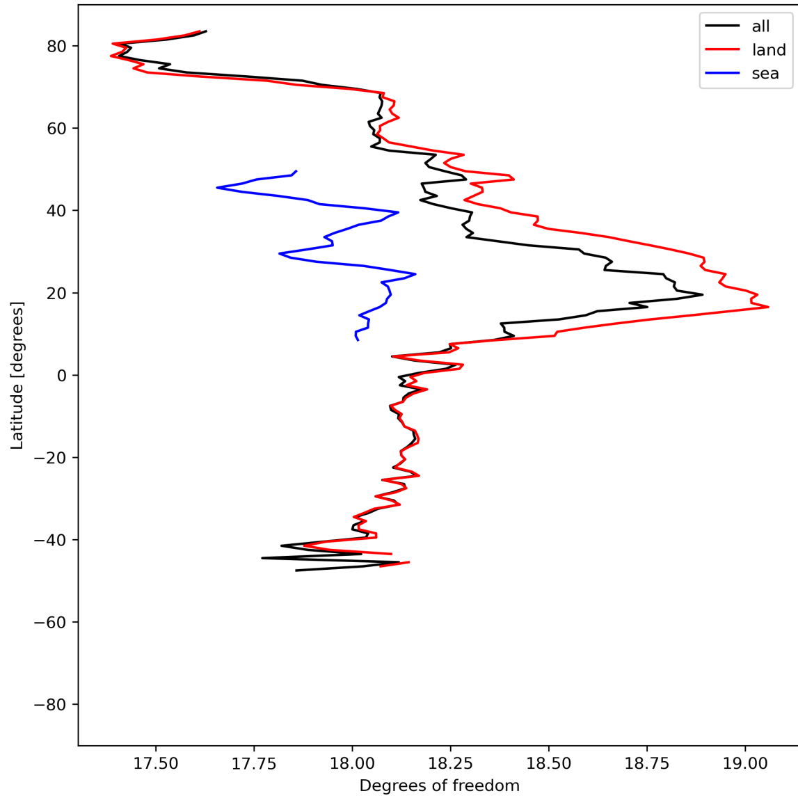
Figure 19: Zonal average of “Degrees of freedom” for 2024-06-17 to 2024-06-19.
