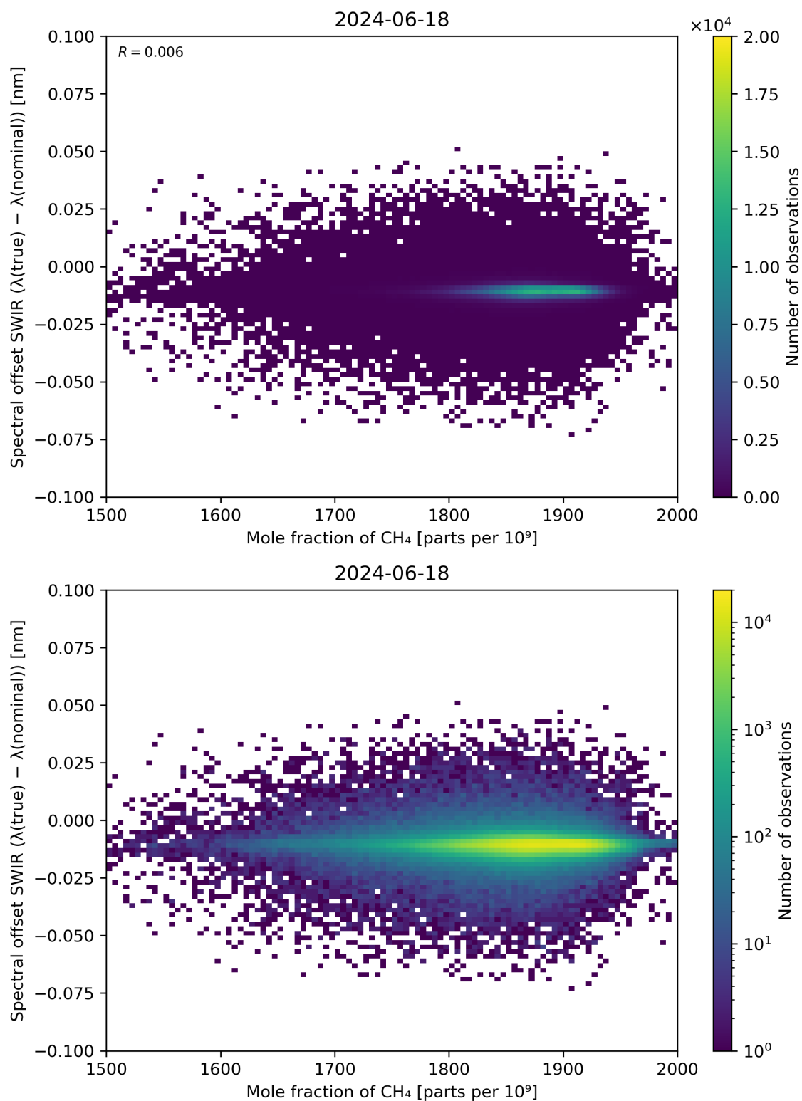
Figure 86: Scatter density plot of “Mole fraction of CH 4 ” against “Spectral offset SWIR ( \lambda(\text{true}) - \lambda(\text{nominal}) )” for 2024-06-17 to 2024-06-19.
