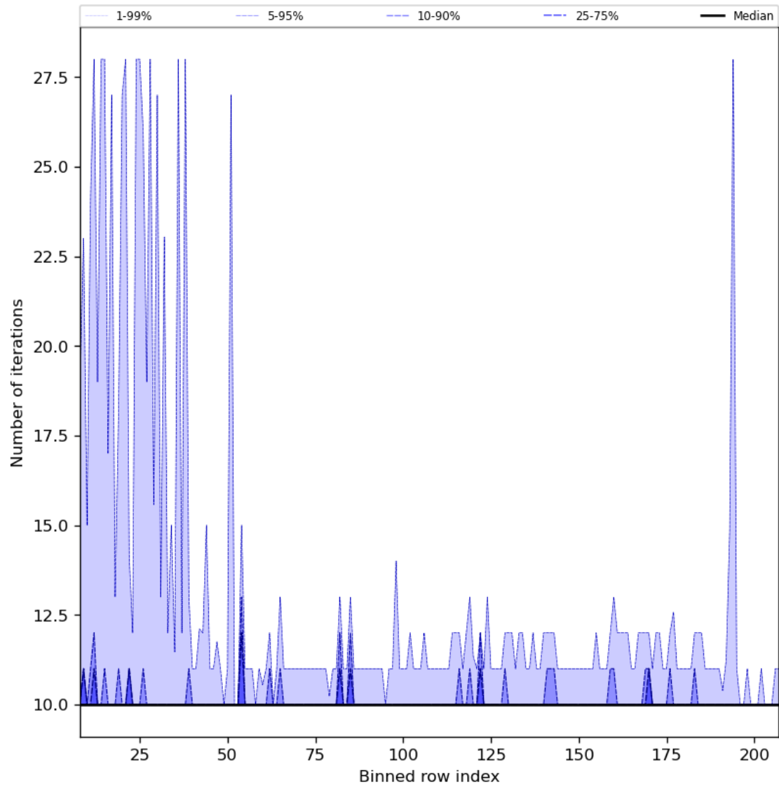
Figure 42: Along track statistics of “Number of iterations” for 2024-06-17 to 2024-06-19
