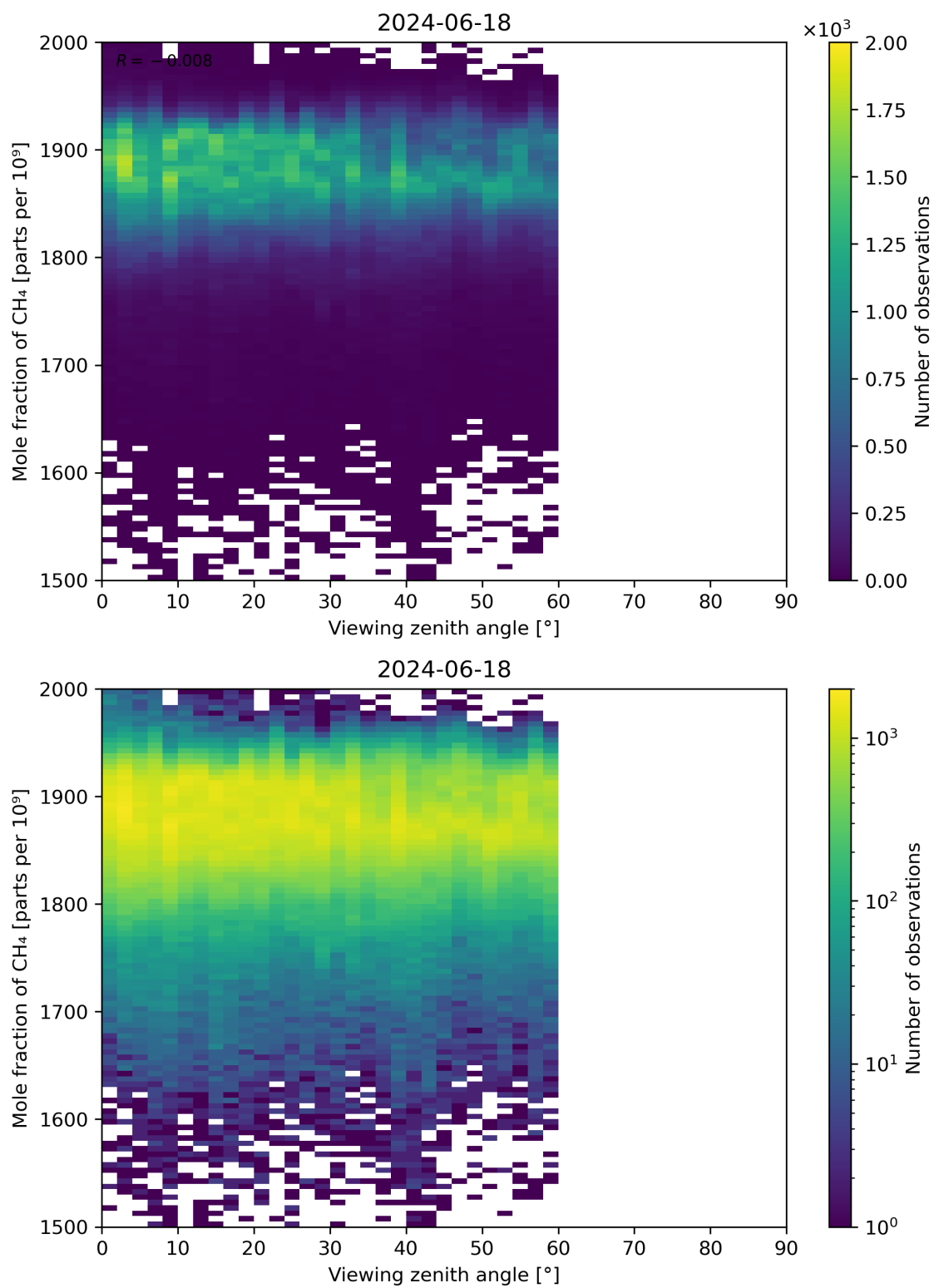
Figure 110: Scatter density plot of “Viewing zenith angle” against “Mole fraction of CH 4 ” for 2024-06-17 to 2024-06-19.
