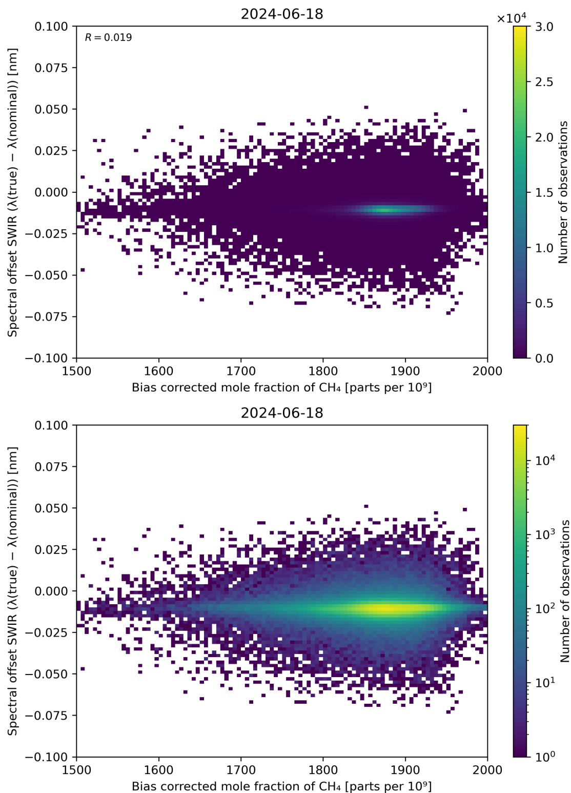
Figure 69: Scatter density plot of “Bias corrected mole fraction of \text{CH}_4 ” against “Spectral offset SWIR ( \lambda(\text{true}) - \lambda(\text{nominal}) )” for 2024-06-17 to 2024-06-19.
