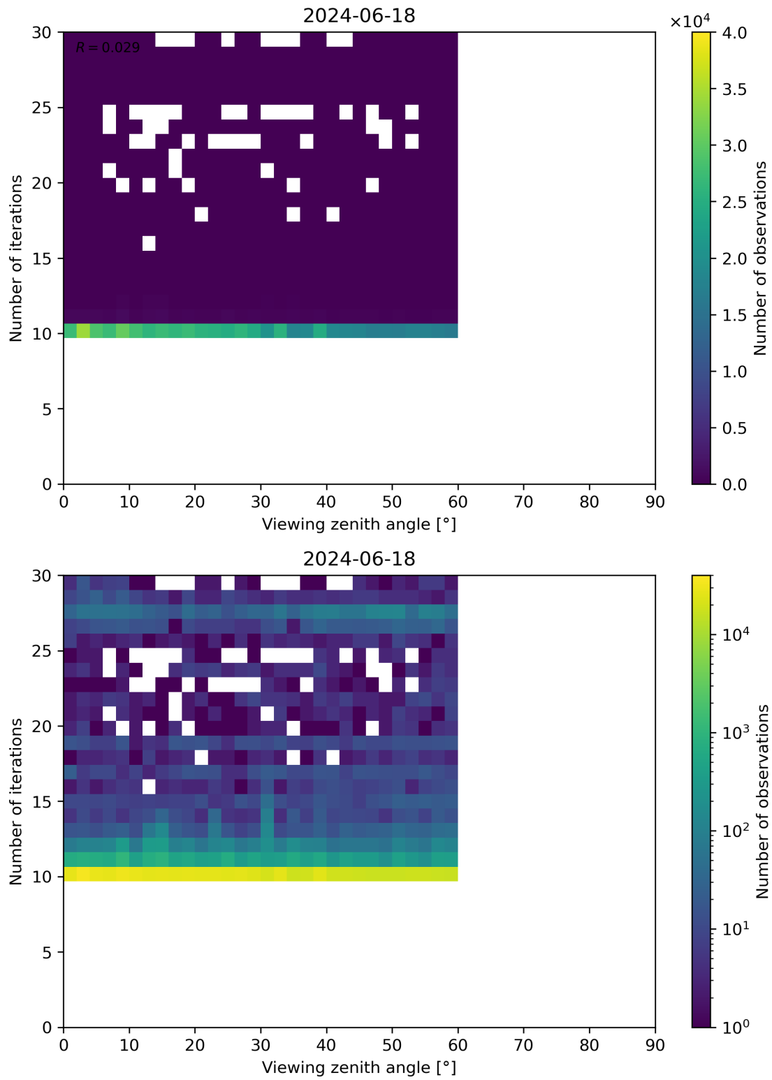
Figure 113: Scatter density plot of “Viewing zenith angle” against “Number of iterations” for 2024-06-17 to 2024-06-19.
