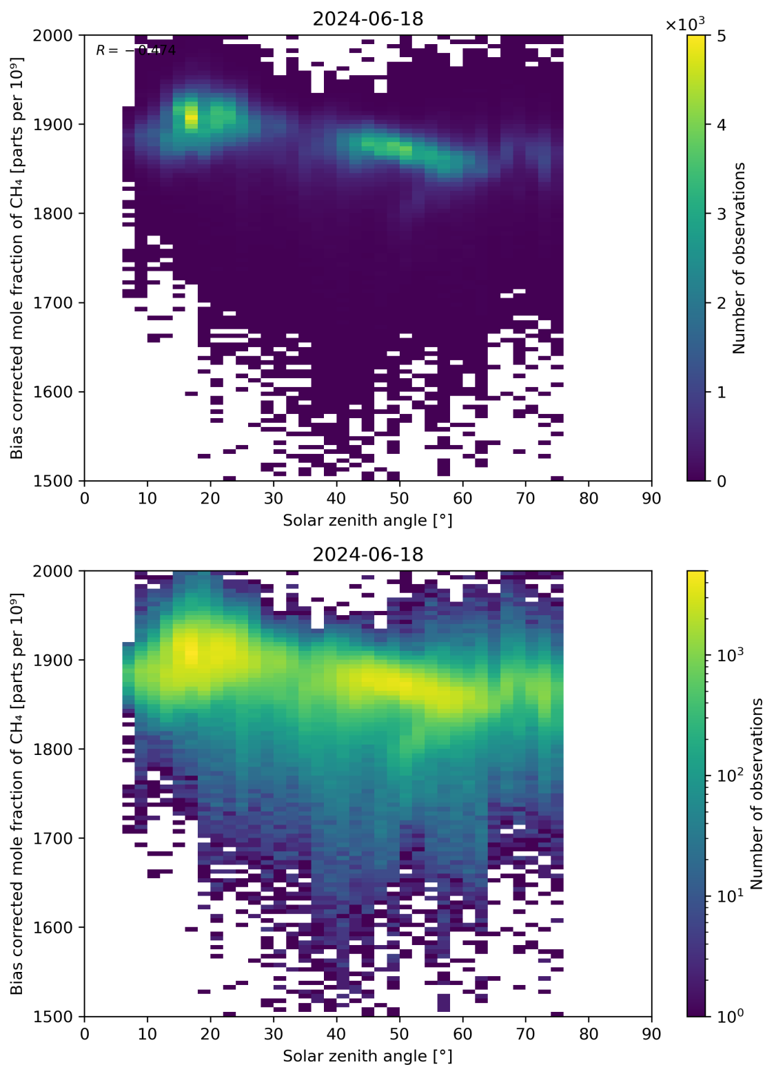
Figure 100: Scatter density plot of “Solar zenith angle” against “Bias corrected mole fraction of CH 4 ” for 2024-06-17 to 2024-06-19.
