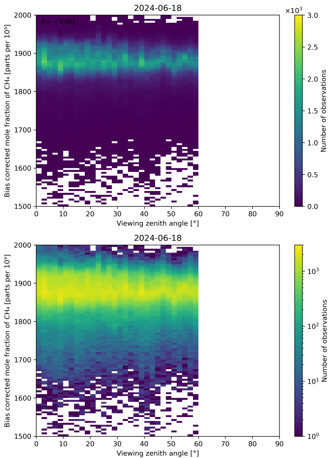
Figure 111: Scatter density plot of “Viewing zenith angle” against “Bias corrected mole fraction of CH 4 ” for 2024-06-17 to 2024-06-19.
