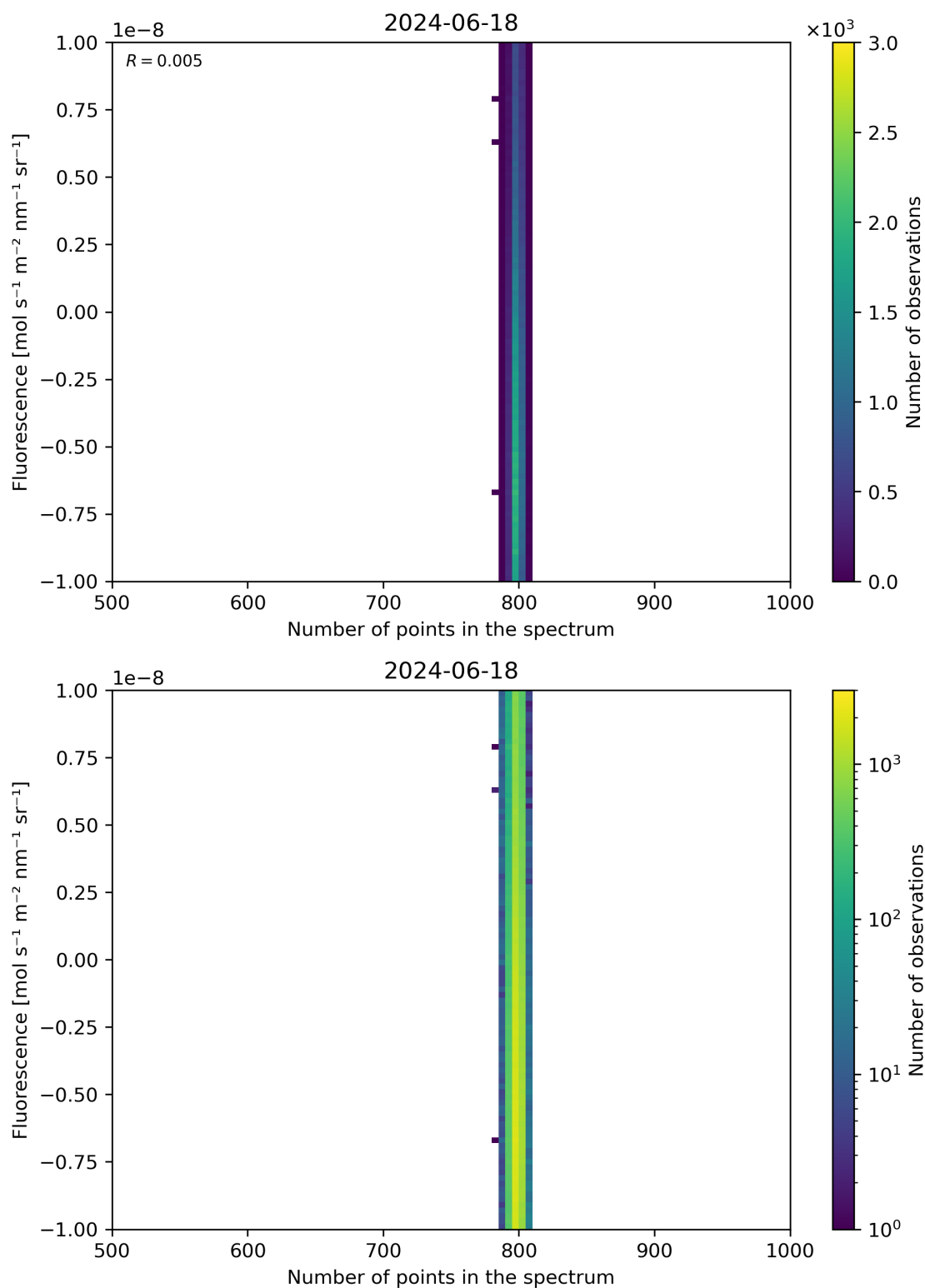
Figure 91: Scatter density plot of “Number of points in the spectrum” against “Fluorescence” for 2024-06-17 to 2024-06-19.
