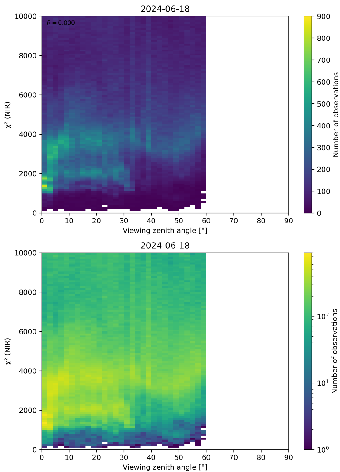
Figure 105: Scatter density plot of “Viewing zenith angle” against “ \chi^2 (NIR)” for 2024-06-17 to 2024-06-19.
