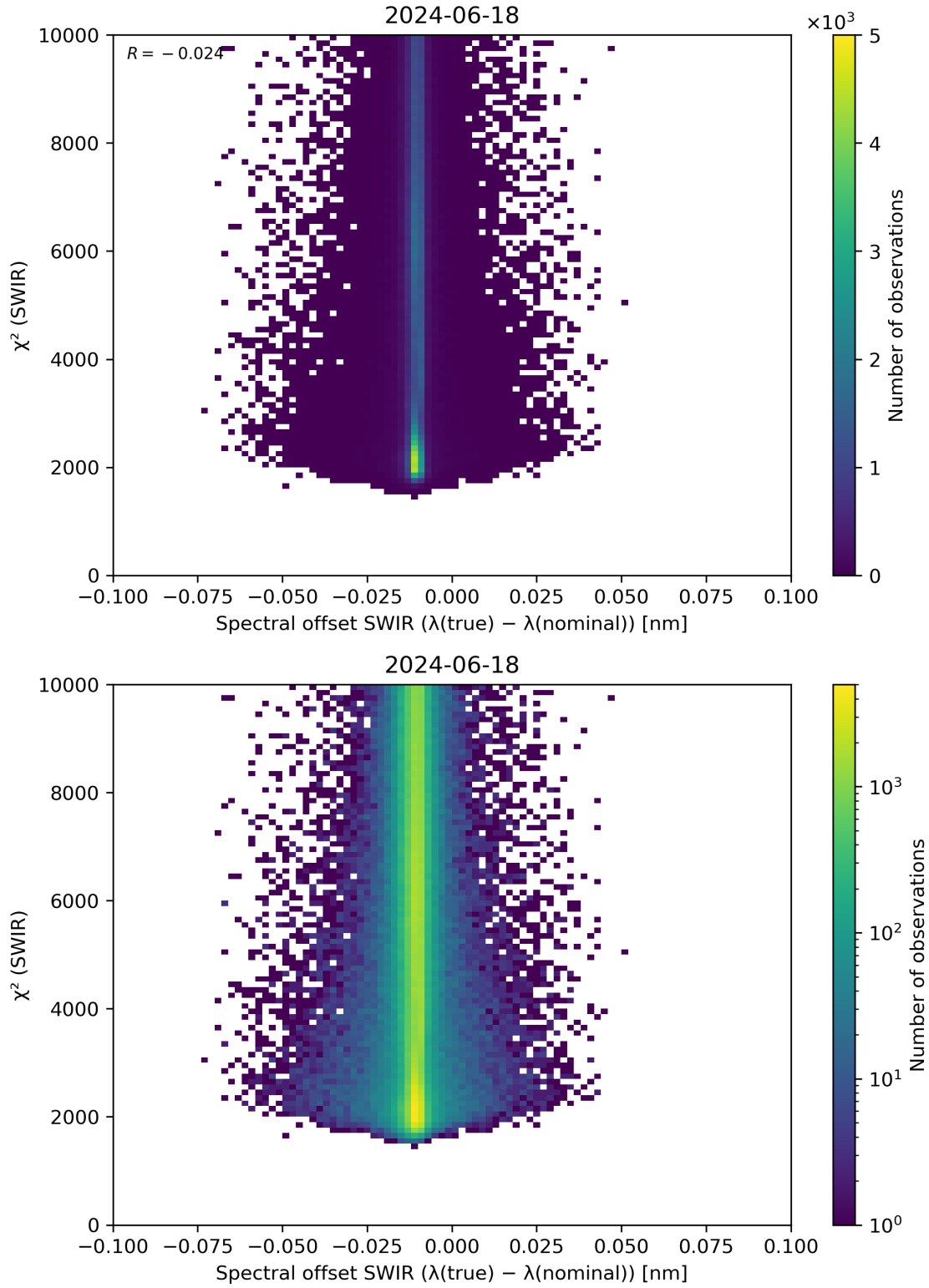
Figure 118: Scatter density plot of “Spectral offset SWIR ( \lambda(\text{true}) - \lambda(\text{nominal}) )” against “ \chi^2 (SWIR)” for 2024-06-17 to 2024-06-19.
