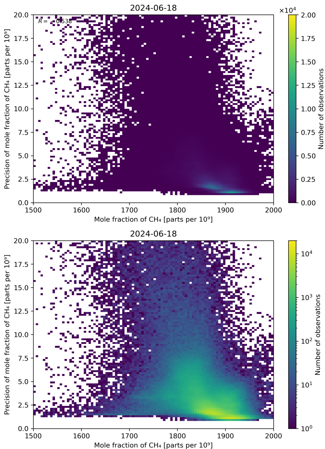
Figure 75: Scatter density plot of “Mole fraction of CH 4 ” against “Precision of mole fraction of CH 4 ” for 2024-06-17 to 2024-06-19.
