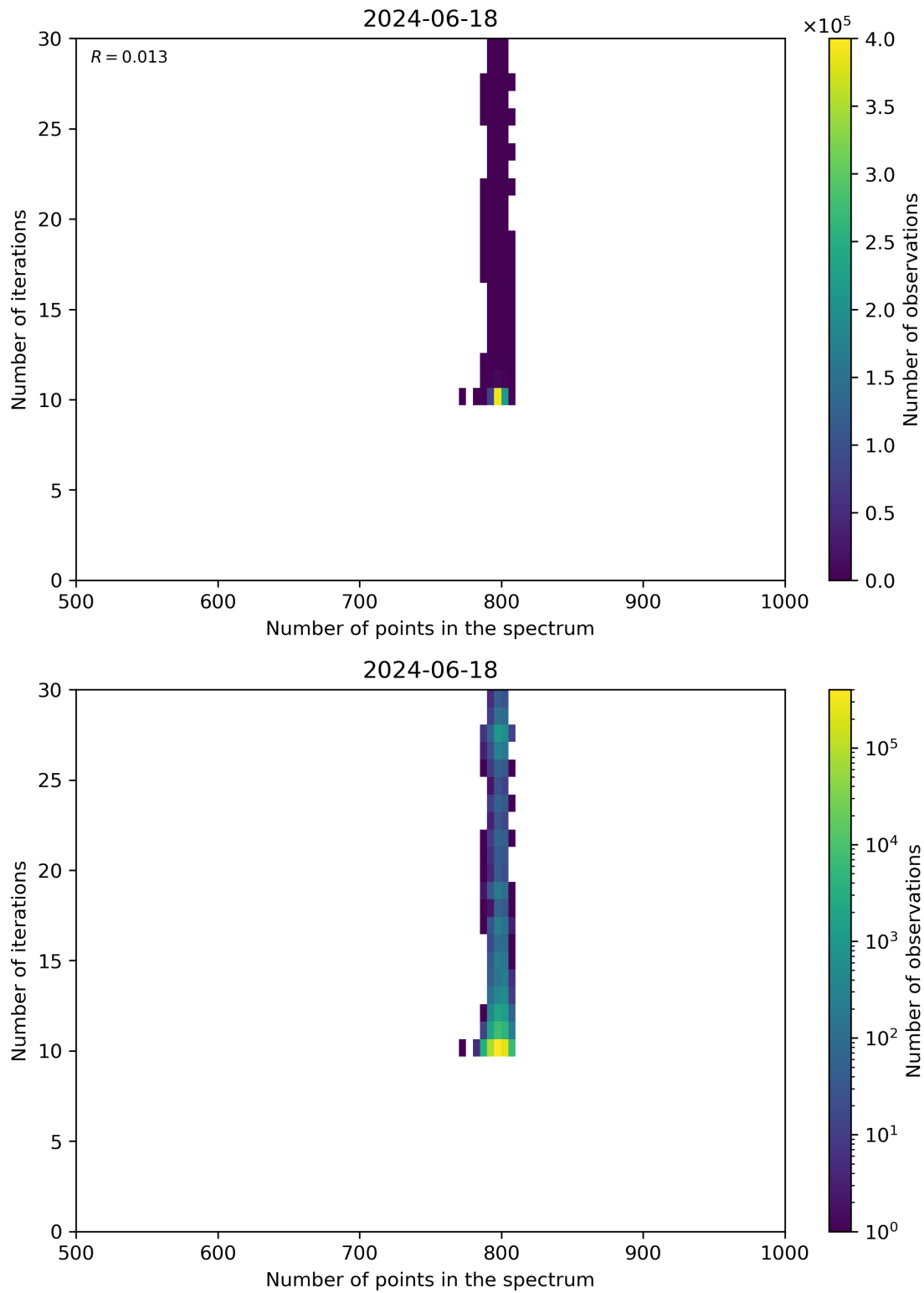
Figure 92: Scatter density plot of “Number of points in the spectrum” against “Number of iterations” for 2024-06-17 to 2024-06-19.
