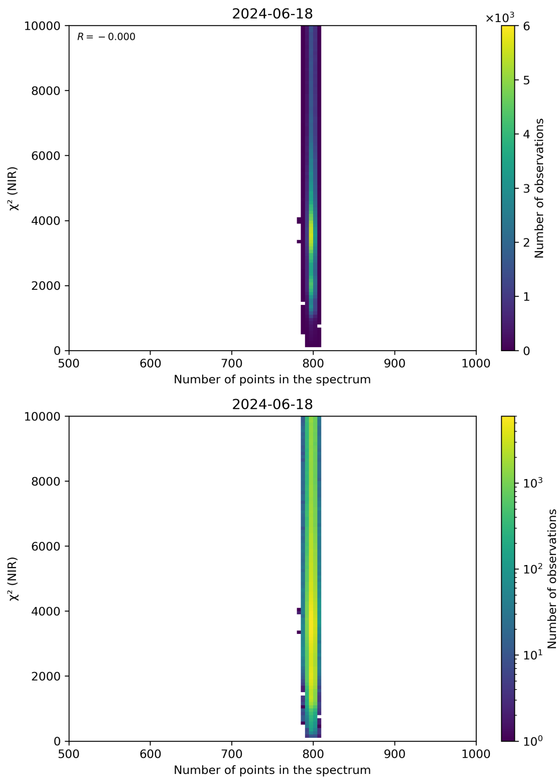
Figure 88: Scatter density plot of “Number of points in the spectrum” against “ \chi^2 (NIR)” for 2024-06-17 to 2024-06-19.
