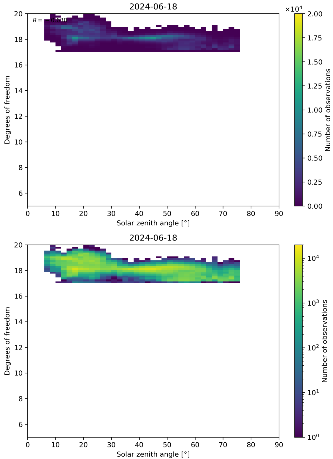
Figure 96: Scatter density plot of “Solar zenith angle” against “Degrees of freedom” for 2024-06-17 to 2024-06-19.
