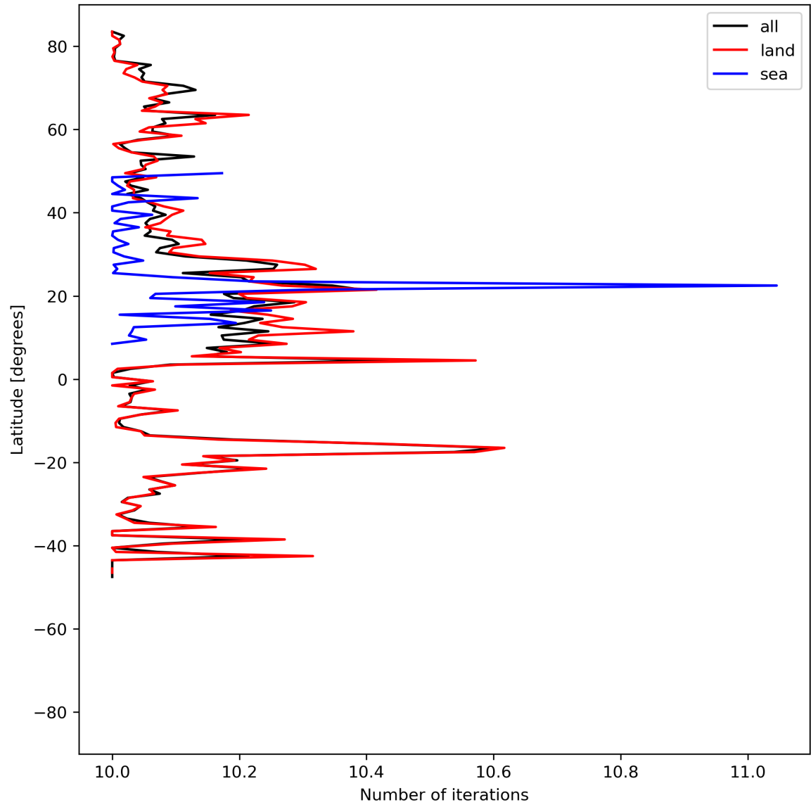
Figure 20: Zonal average of “Number of iterations” for 2024-06-17 to 2024-06-19.
