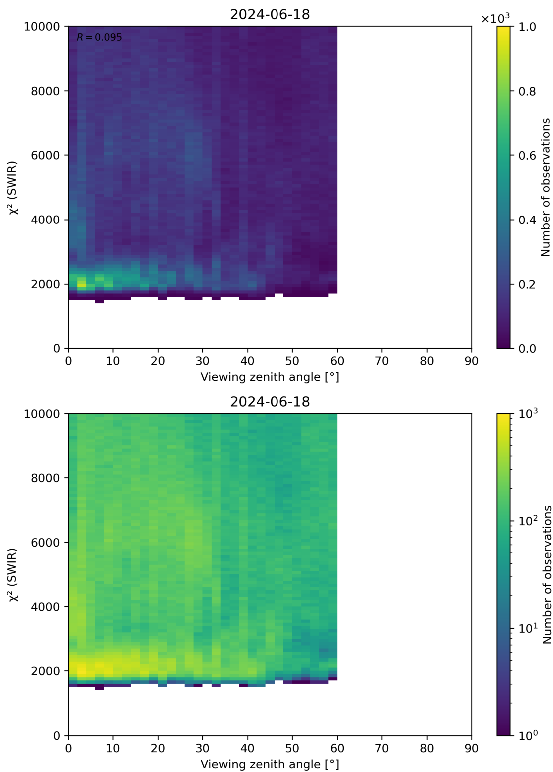
Figure 106: Scatter density plot of “Viewing zenith angle” against “ \chi^2 (SWIR)” for 2024-06-17 to 2024-06-19.
