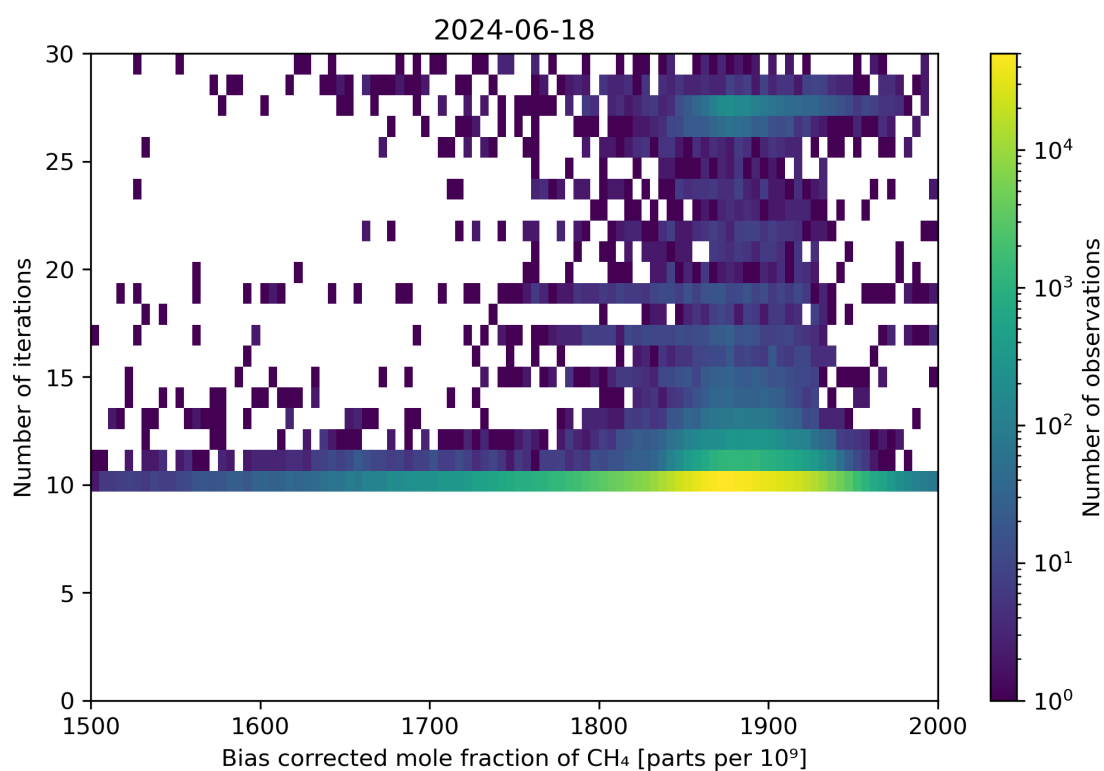
Figure 67: Scatter density plot of “Bias corrected mole fraction of CH 4 ” against “Number of iterations” for 2024-06-17 to 2024-06-19.
