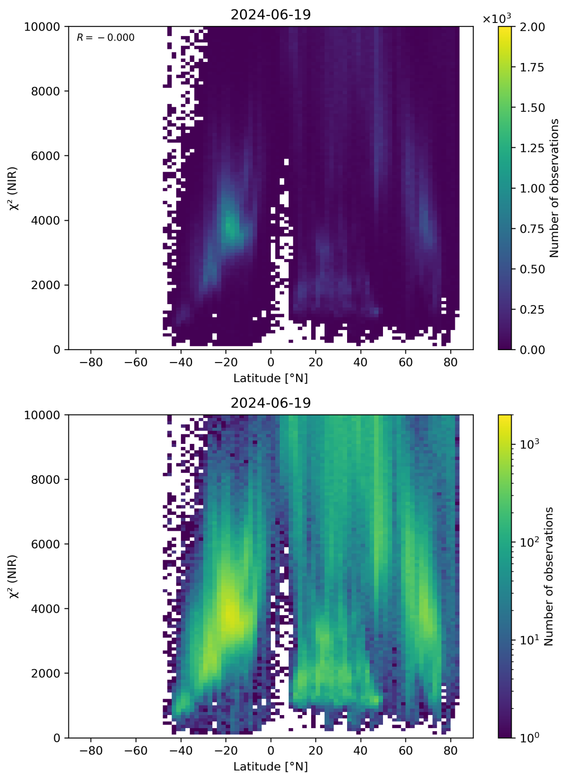
Figure 53: Scatter density plot of “Latitude” against “ \chi^2 (NIR)” for 2024-06-19 to 2024-06-20.
