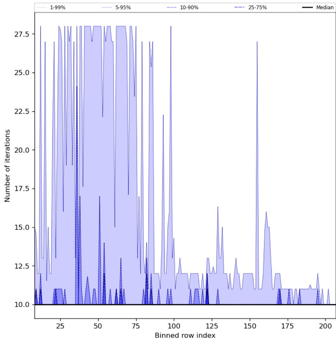
Figure 42: Along track statistics of “Number of iterations” for 2024-06-19 to 2024-06-20
