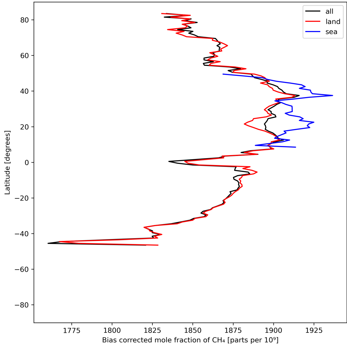
Figure 14: Zonal average of “Bias corrected mole fraction of CH 4 ” for 2024-06-19 to 2024-06-20.
