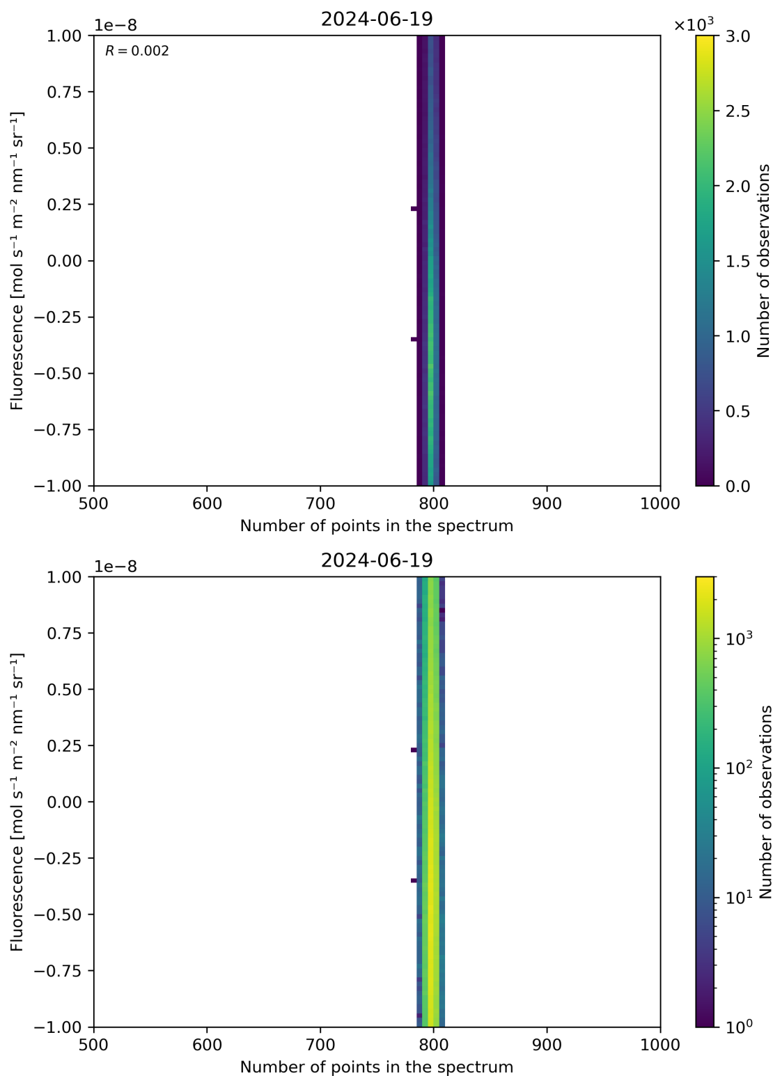
Figure 91: Scatter density plot of “Number of points in the spectrum” against “Fluorescence” for 2024-06-19 to 2024-06-20.
