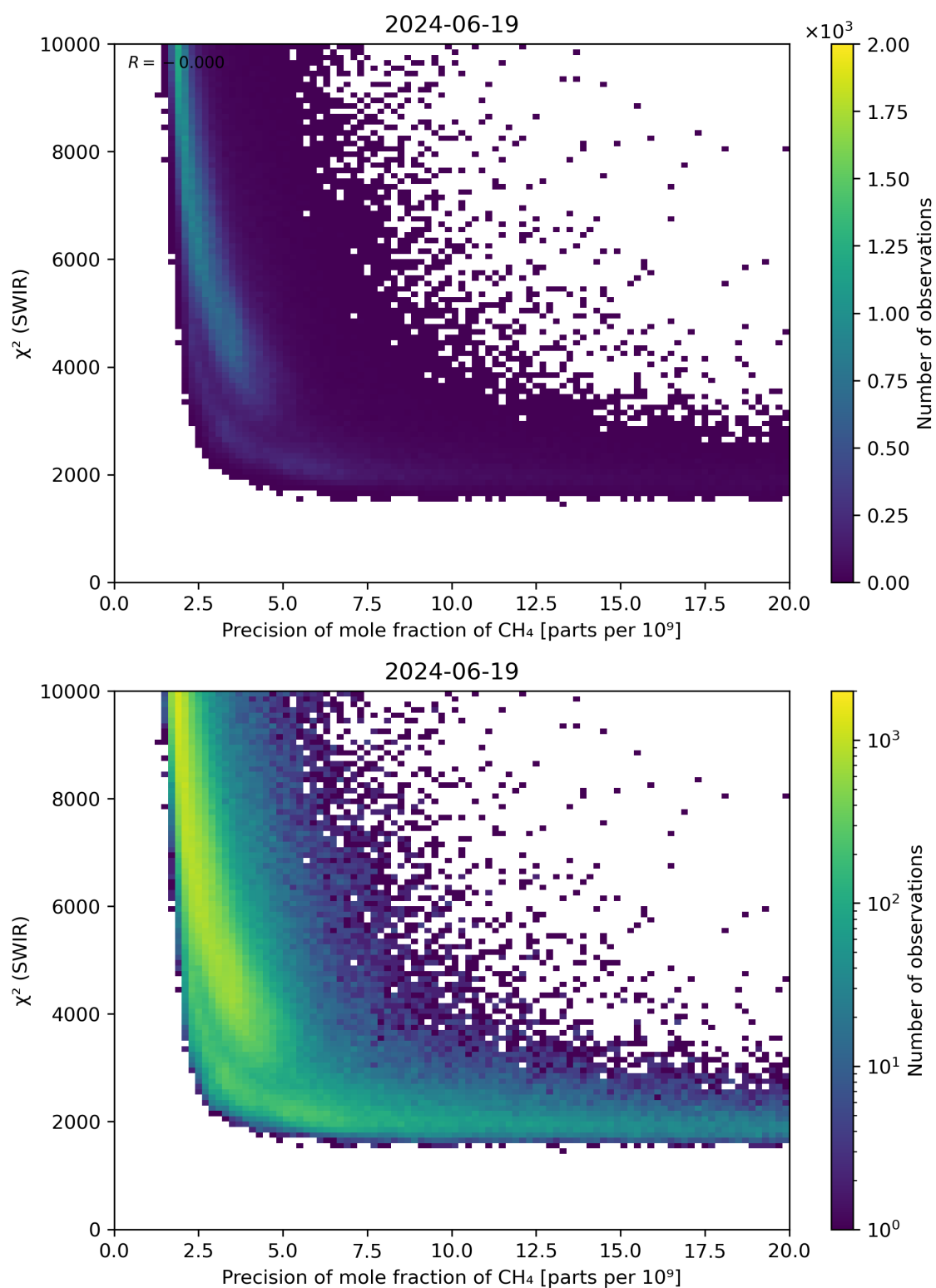
Figure 79: Scatter density plot of “Precision of mole fraction of CH 4 ” against “ \chi^2 (SWIR)” for 2024-06-19 to 2024-06-20.
