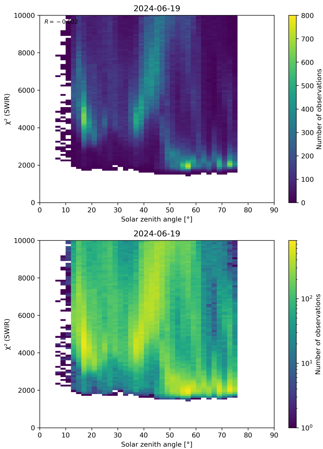
Figure 95: Scatter density plot of “Solar zenith angle” against “ \chi^2 (SWIR)” for 2024-06-19 to 2024-06-20.
