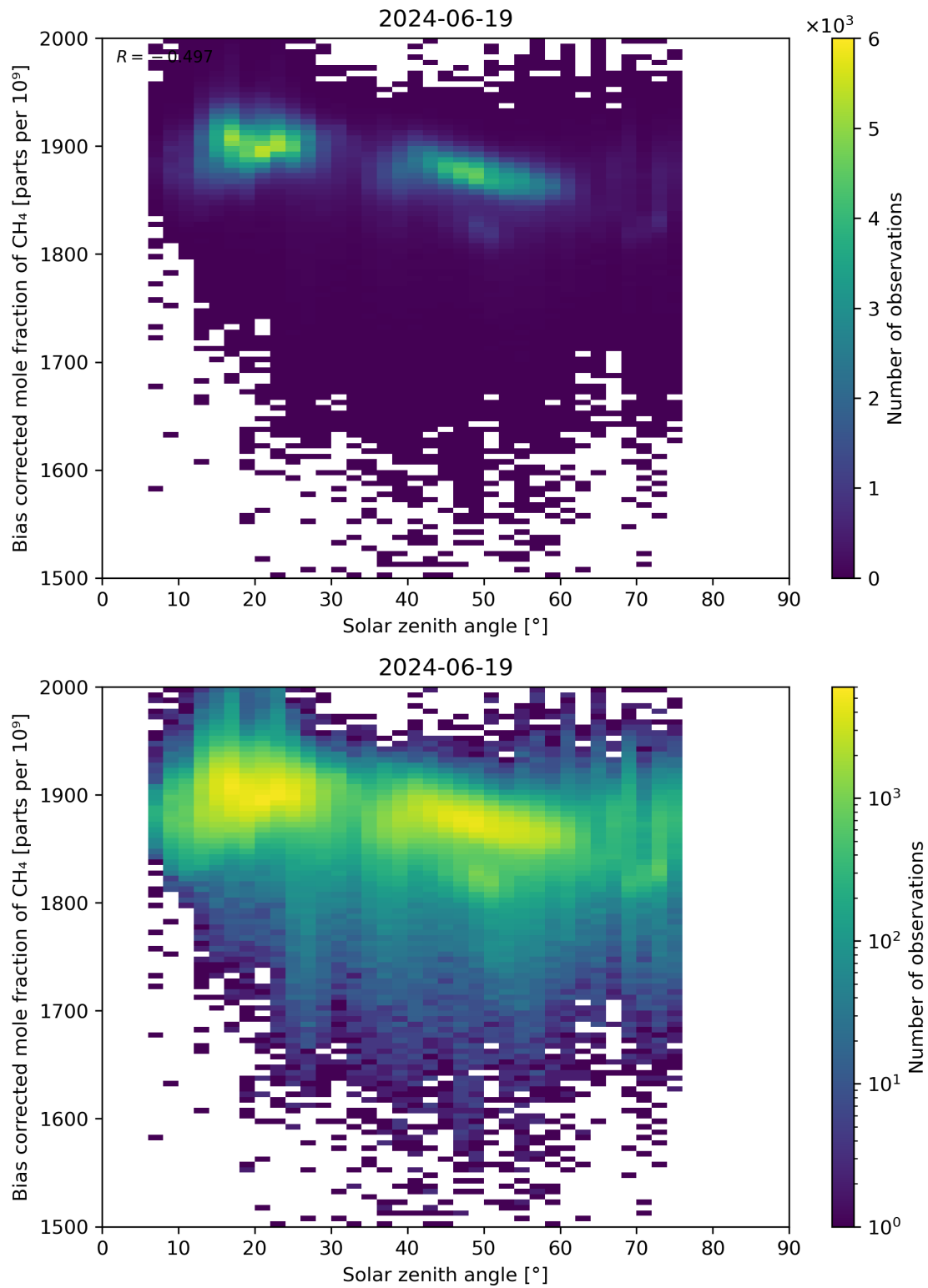
Figure 100: Scatter density plot of “Solar zenith angle” against “Bias corrected mole fraction of CH 4 ” for 2024-06-19 to 2024-06-20.
