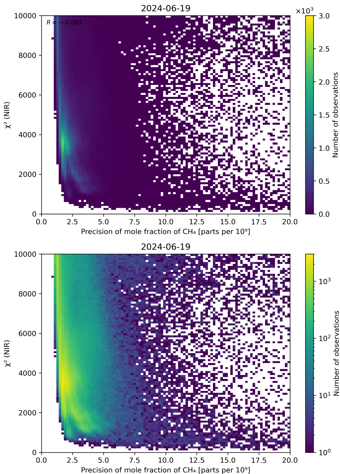
Figure 78: Scatter density plot of “Precision of mole fraction of CH 4 ” against “ \chi^2 (NIR)” for 2024-06-19 to 2024-06-20.
