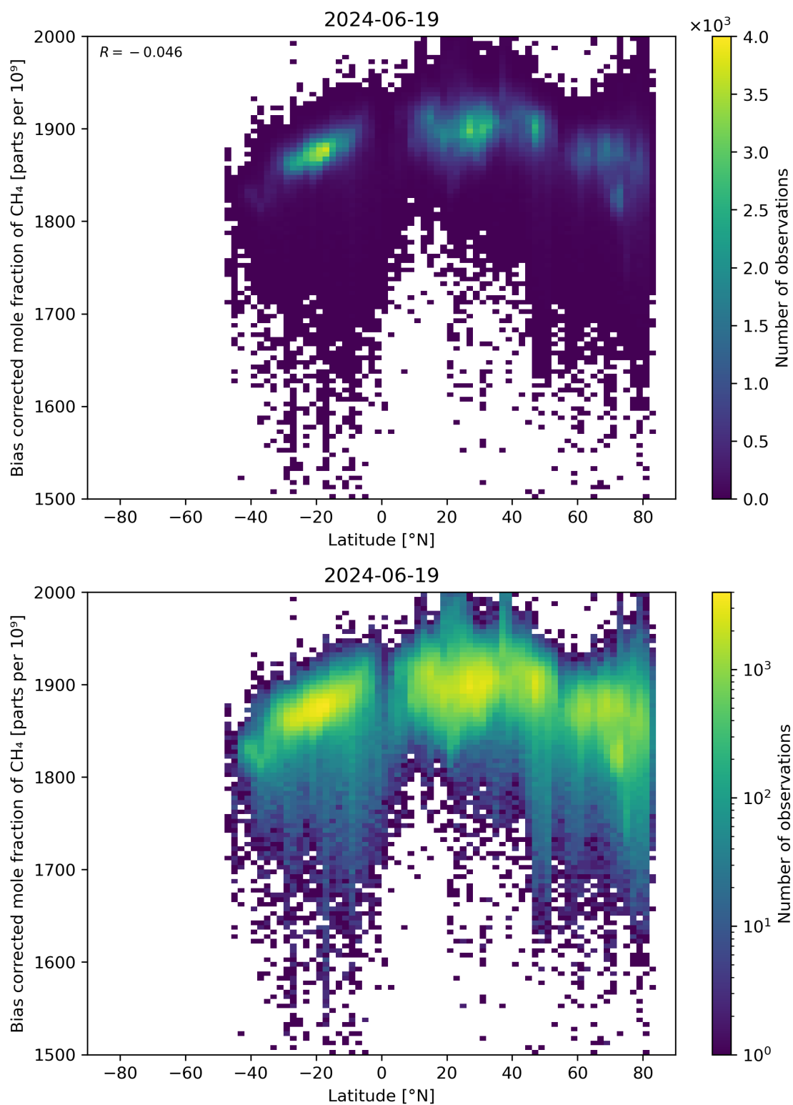
Figure 58: Scatter density plot of “Latitude” against “Bias corrected mole fraction of CH 4 ” for 2024-06-19 to 2024-06-20.
