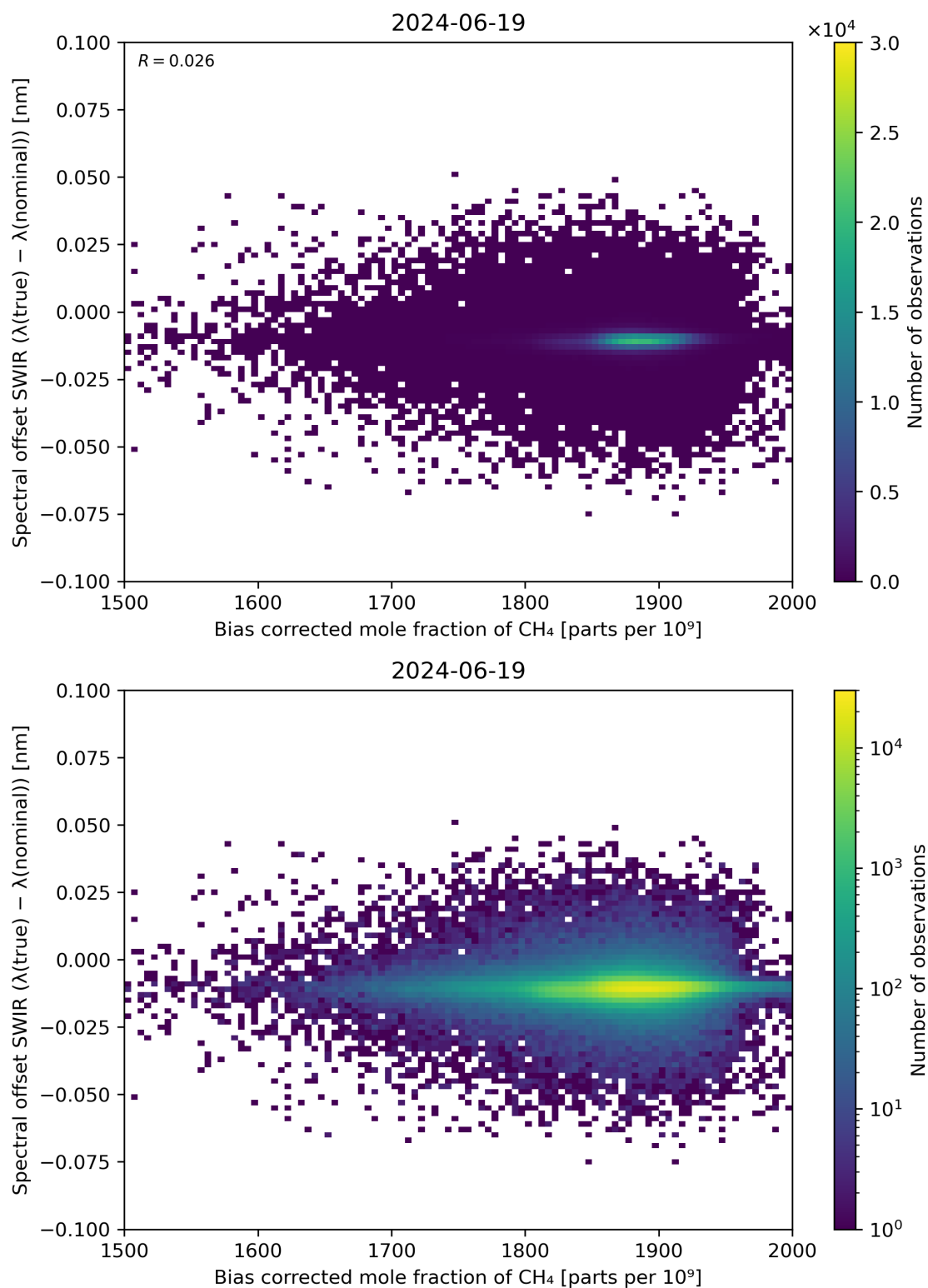
Figure 69: Scatter density plot of “Bias corrected mole fraction of \text{CH}_4 ” against “Spectral offset SWIR ( \lambda(\text{true}) - \lambda(\text{nominal}) )” for 2024-06-19 to 2024-06-20.
