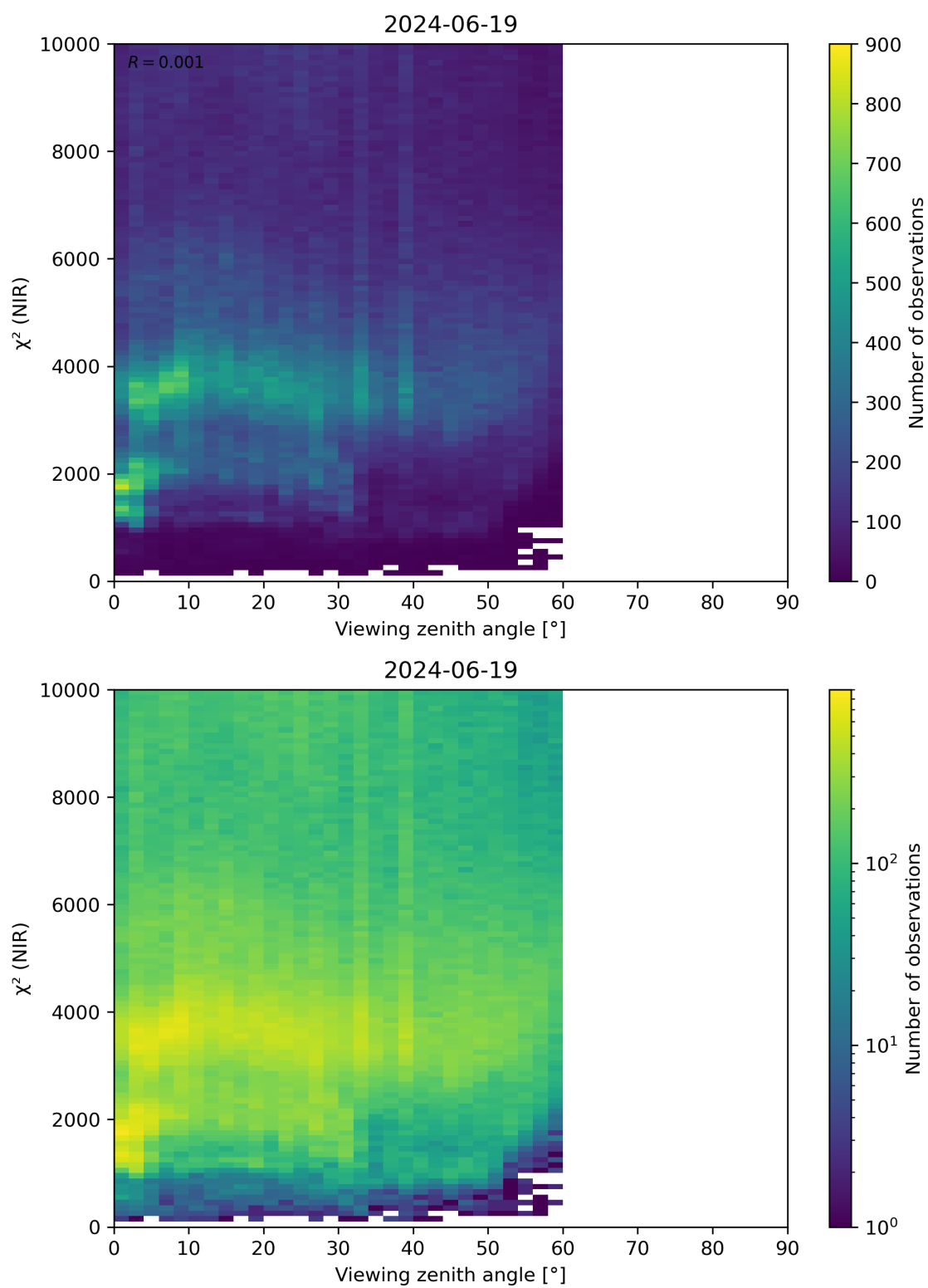
Figure 105: Scatter density plot of “Viewing zenith angle” against “ \chi^2 (NIR)” for 2024-06-19 to 2024-06-20.
