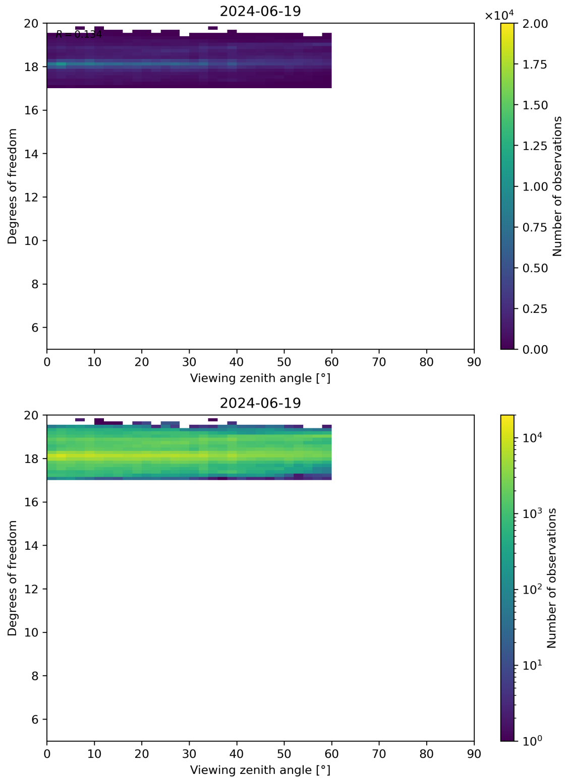
Figure 107: Scatter density plot of “Viewing zenith angle” against “Degrees of freedom” for 2024-06-19 to 2024-06-20.
