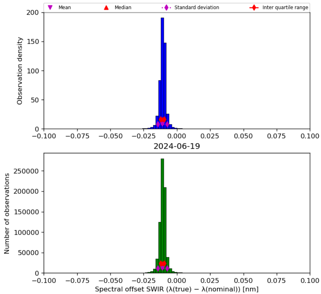
Figure 27: Histogram of “Spectral offset SWIR ( \lambda(\text{true}) - \lambda(\text{nominal}) )” for 2024-06-19 to 2024-06-20
