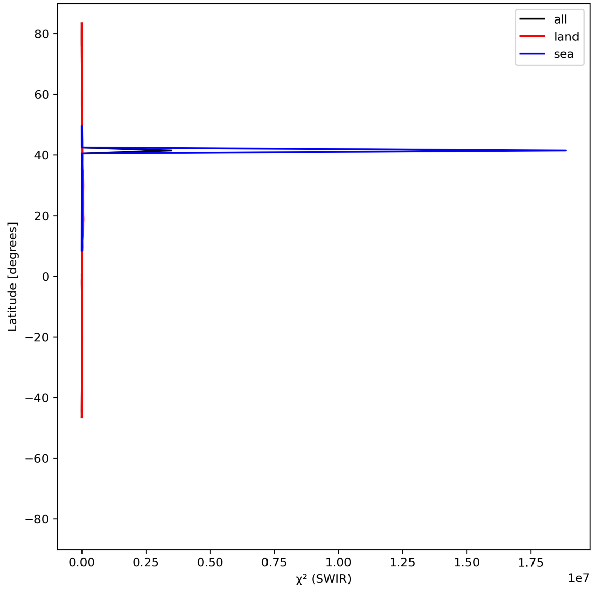
Figure 17: Zonal average of “ \chi^2 (SWIR)” for 2024-06-19 to 2024-06-20.
