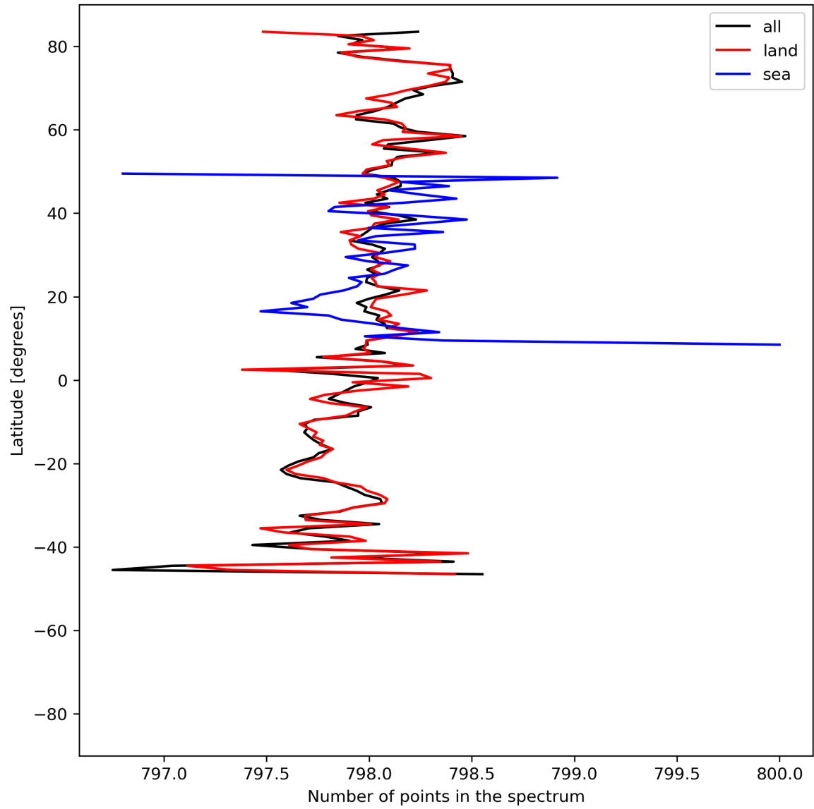
Figure 15: Zonal average of “Number of points in the spectrum” for 2024-06-19 to 2024-06-20.
