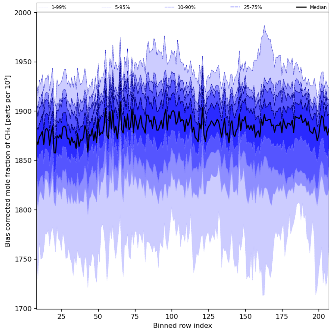
Figure 36: Along track statistics of “Bias corrected mole fraction of CH 4 ” for 2024-06-19 to 2024-06-20
