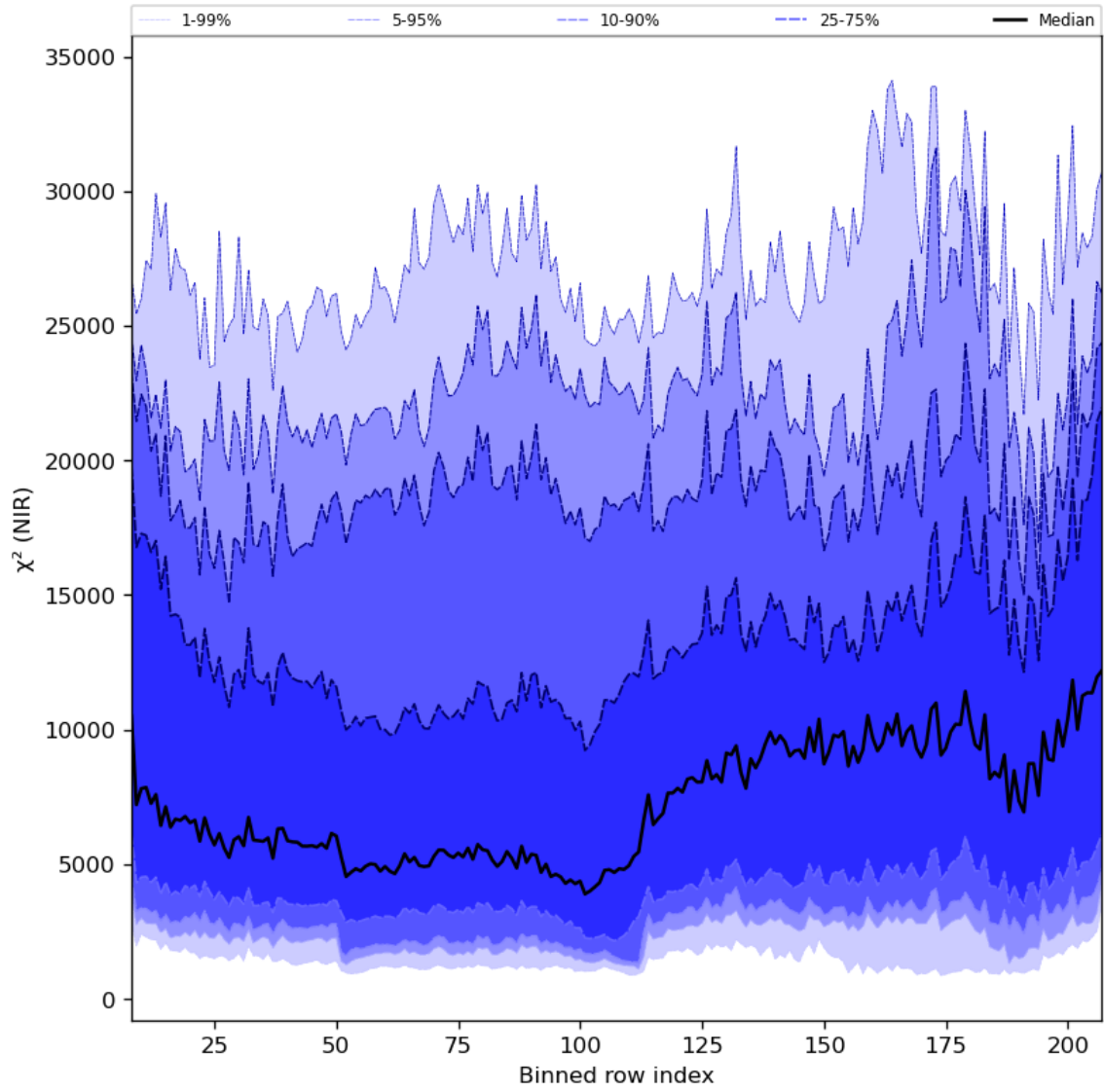
Figure 40: Along track statistics of “ \chi^2 (NIR)” for 2024-06-19 to 2024-06-20
