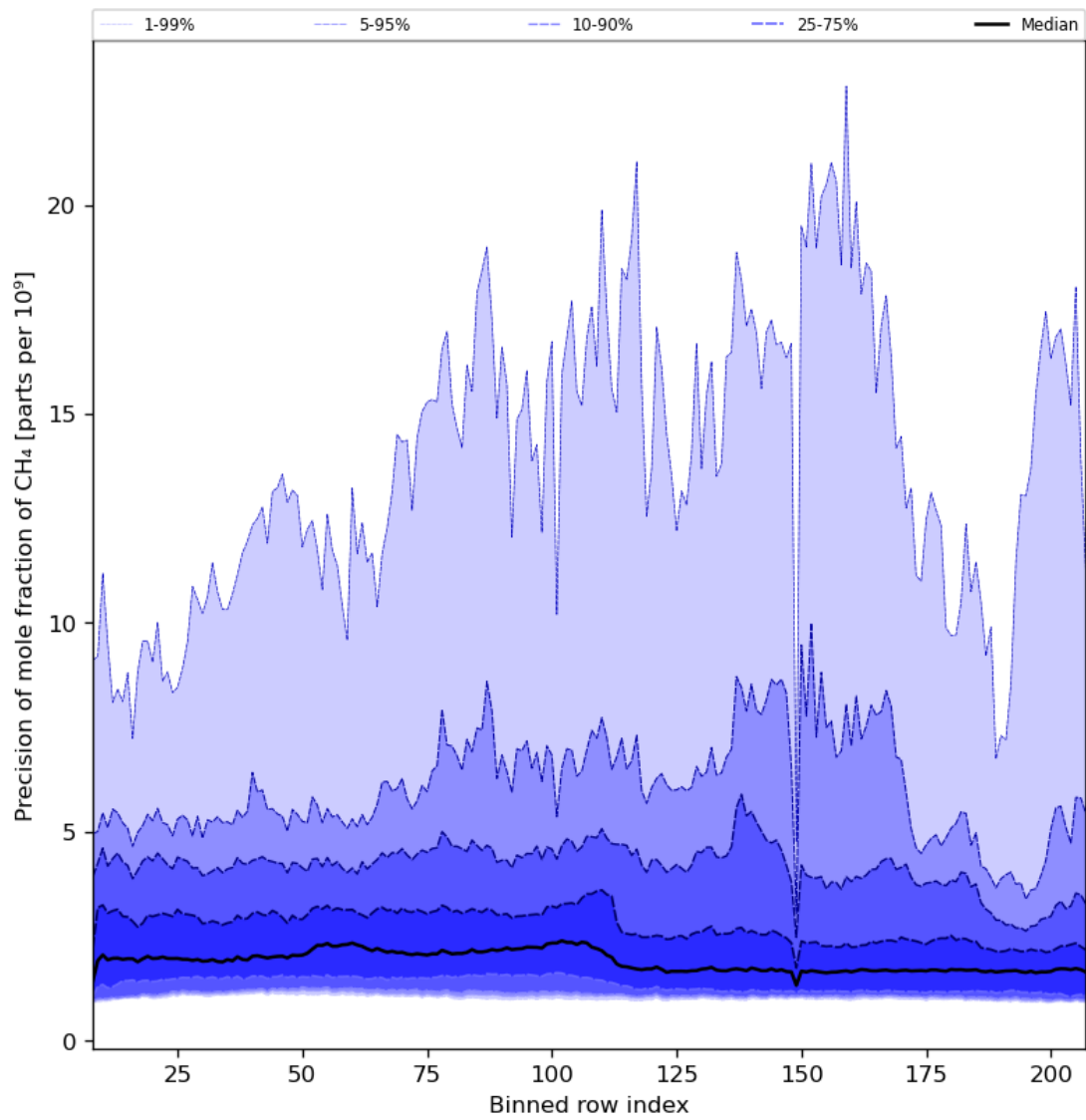
Figure 35: Along track statistics of “Precision of mole fraction of CH 4 ” for 2024-06-19 to 2024-06-20
