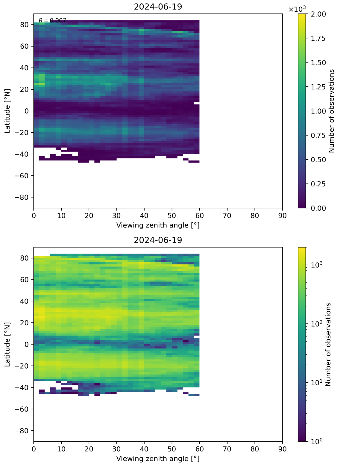
Figure 109: Scatter density plot of “Viewing zenith angle” against “Latitude” for 2024-06-19 to 2024-06-20.
