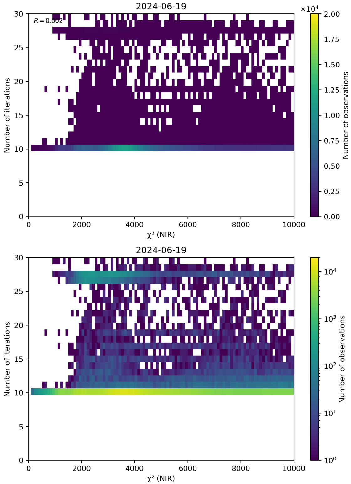
Figure 46: Scatter density plot of “ \chi^2 (NIR)” against “Number of iterations” for 2024-06-19 to 2024-06-20.
