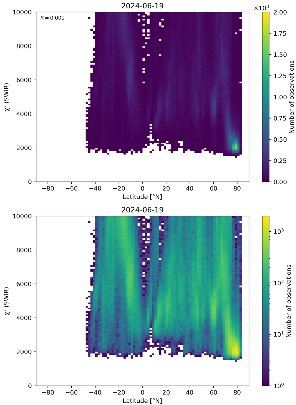
Figure 54: Scatter density plot of “Latitude” against “ \chi^2 (SWIR)” for 2024-06-19 to 2024-06-20.
