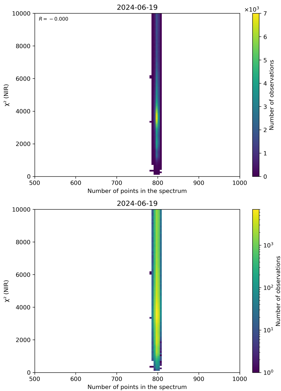
Figure 88: Scatter density plot of “Number of points in the spectrum” against “ \chi^2 (NIR)” for 2024-06-19 to 2024-06-20.
