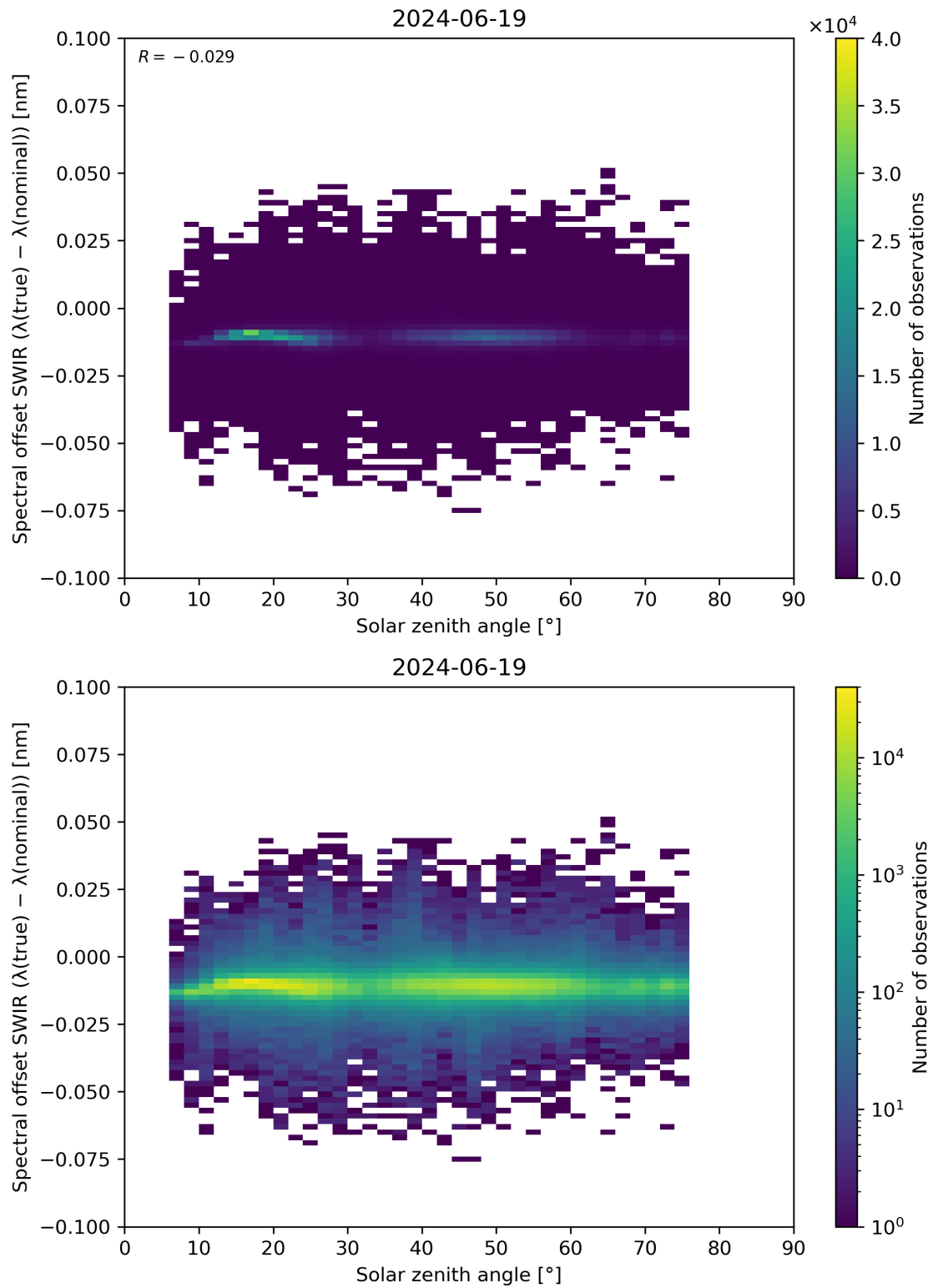
Figure 104: Scatter density plot of “Solar zenith angle” against “Spectral offset SWIR ( \lambda(\text{true}) - \lambda(\text{nominal}) )” for 2024-06-19 to 2024-06-20.
