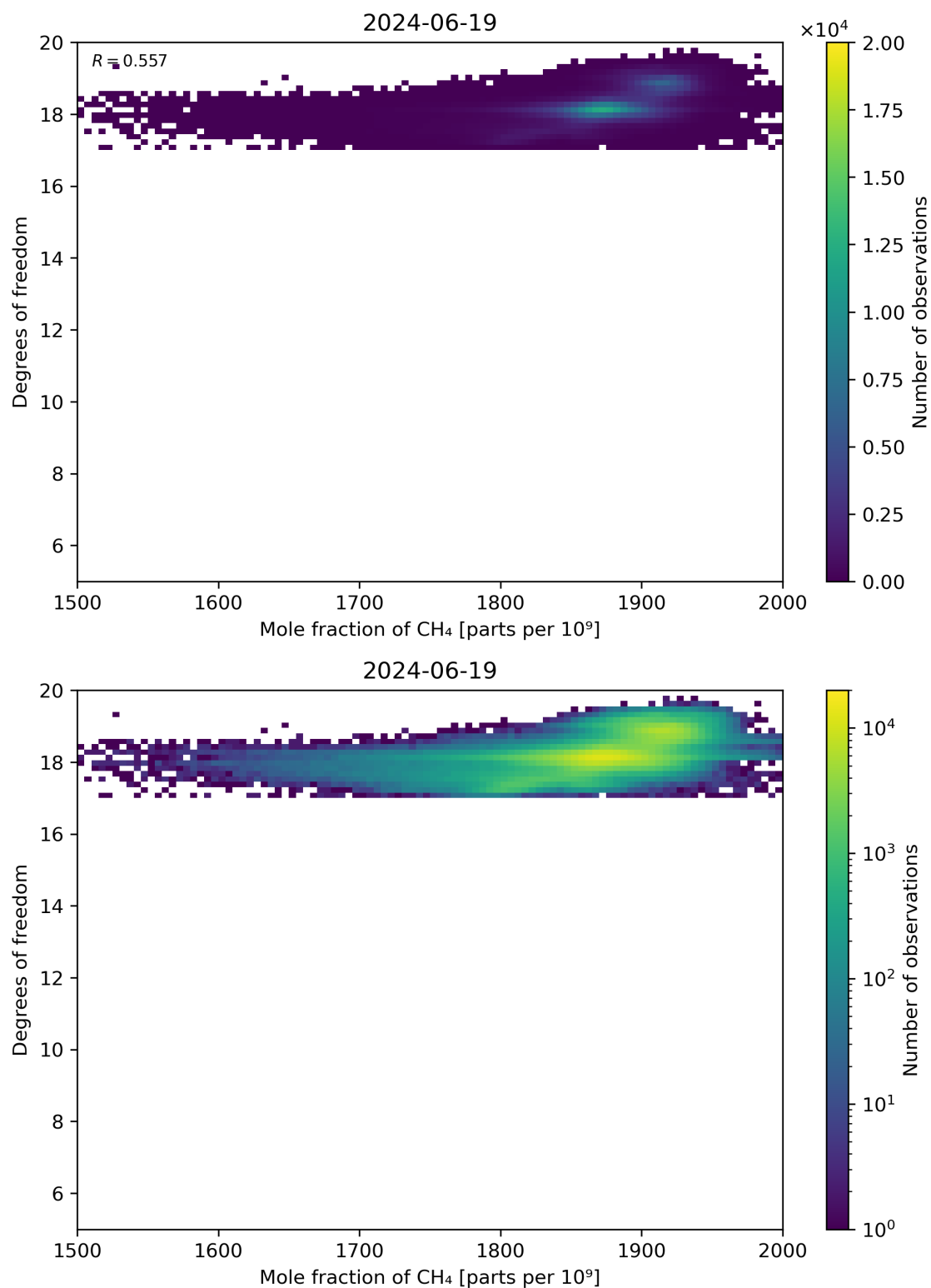
Figure 72: Scatter density plot of “Mole fraction of CH 4 ” against “Degrees of freedom” for 2024-06-19 to 2024-06-20.
