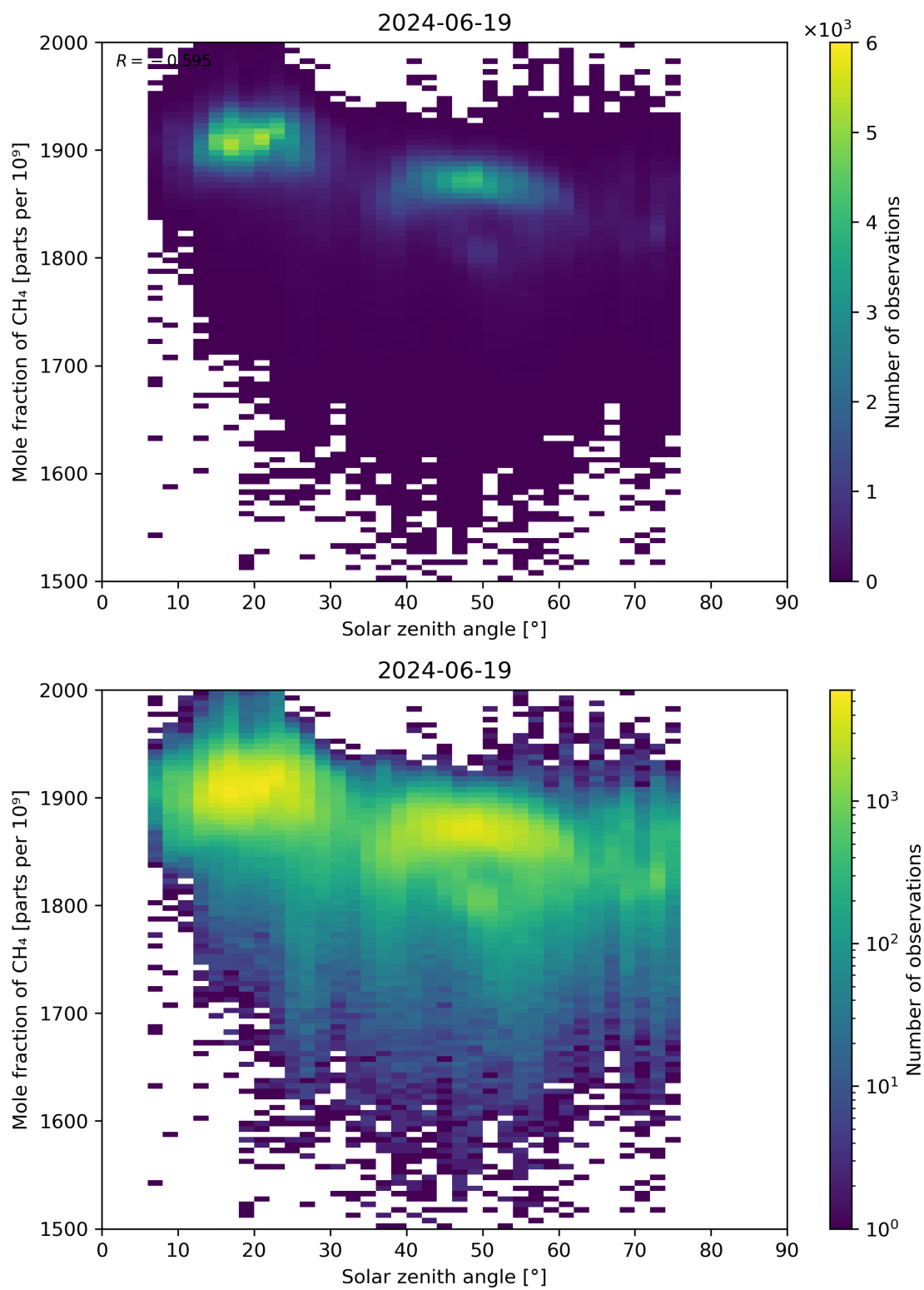
Figure 99: Scatter density plot of “Solar zenith angle” against “Mole fraction of \text{CH}_4 ” for 2024-06-19 to 2024-06-20.
