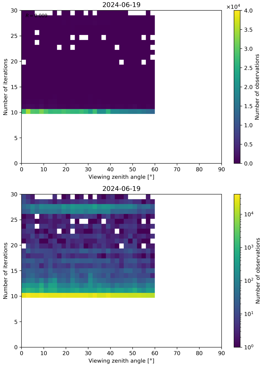
Figure 113: Scatter density plot of “Viewing zenith angle” against “Number of iterations” for 2024-06-19 to 2024-06-20.
