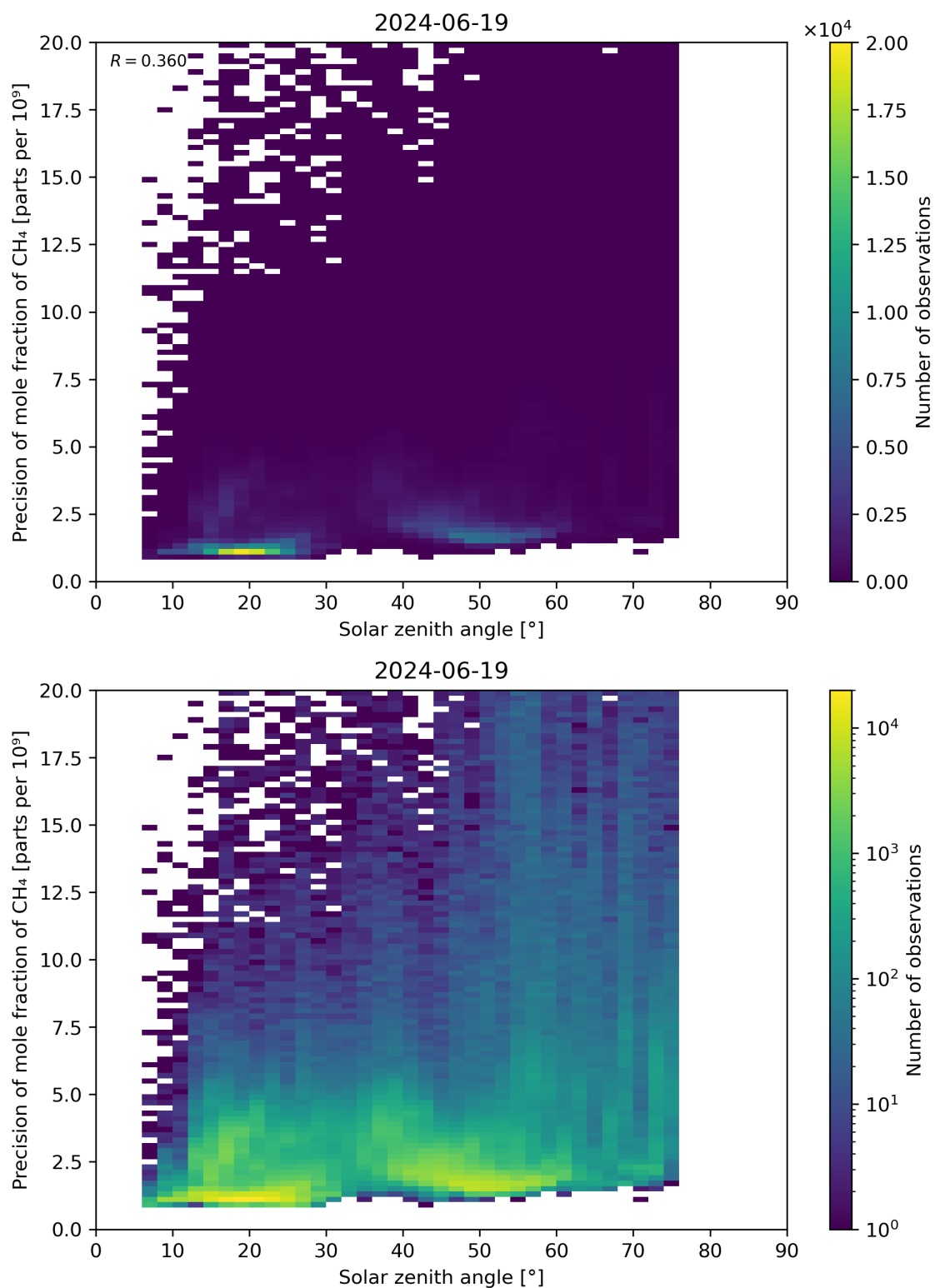
Figure 101: Scatter density plot of “Solar zenith angle” against “Precision of mole fraction of CH 4 ” for 2024-06-19 to 2024-06-20.
