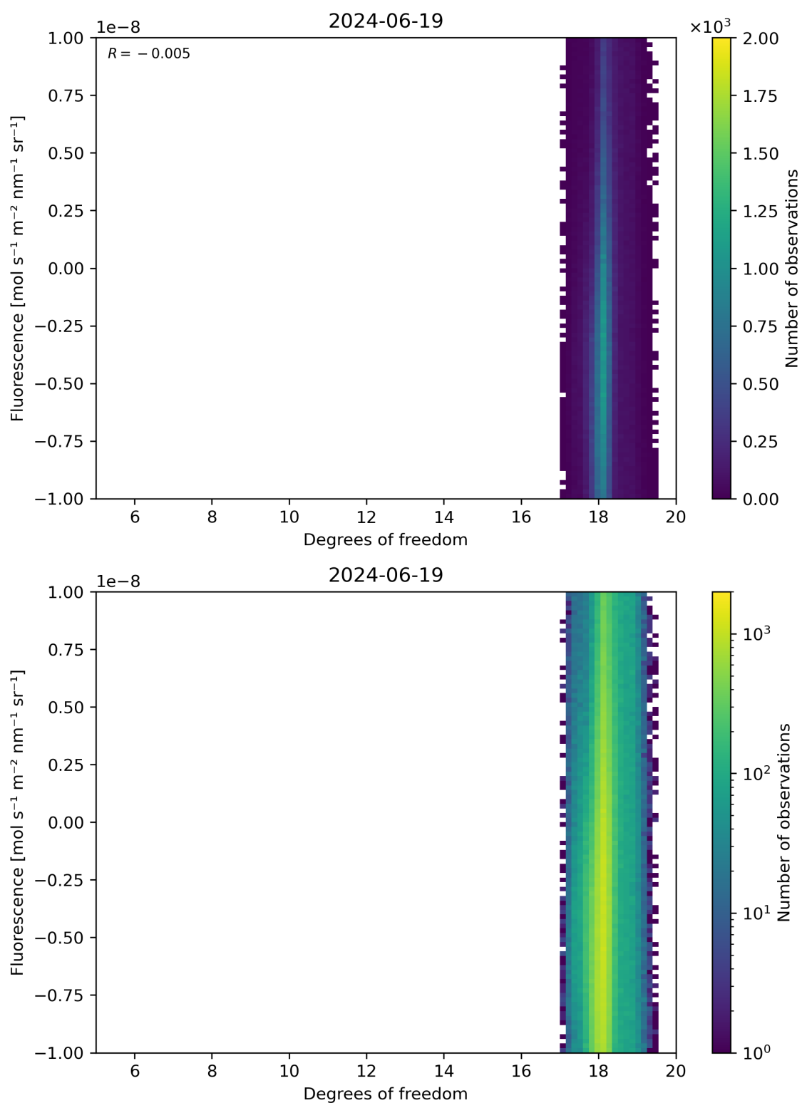
Figure 51: Scatter density plot of “Degrees of freedom” against “Fluorescence” for 2024-06-19 to 2024-06-20.
