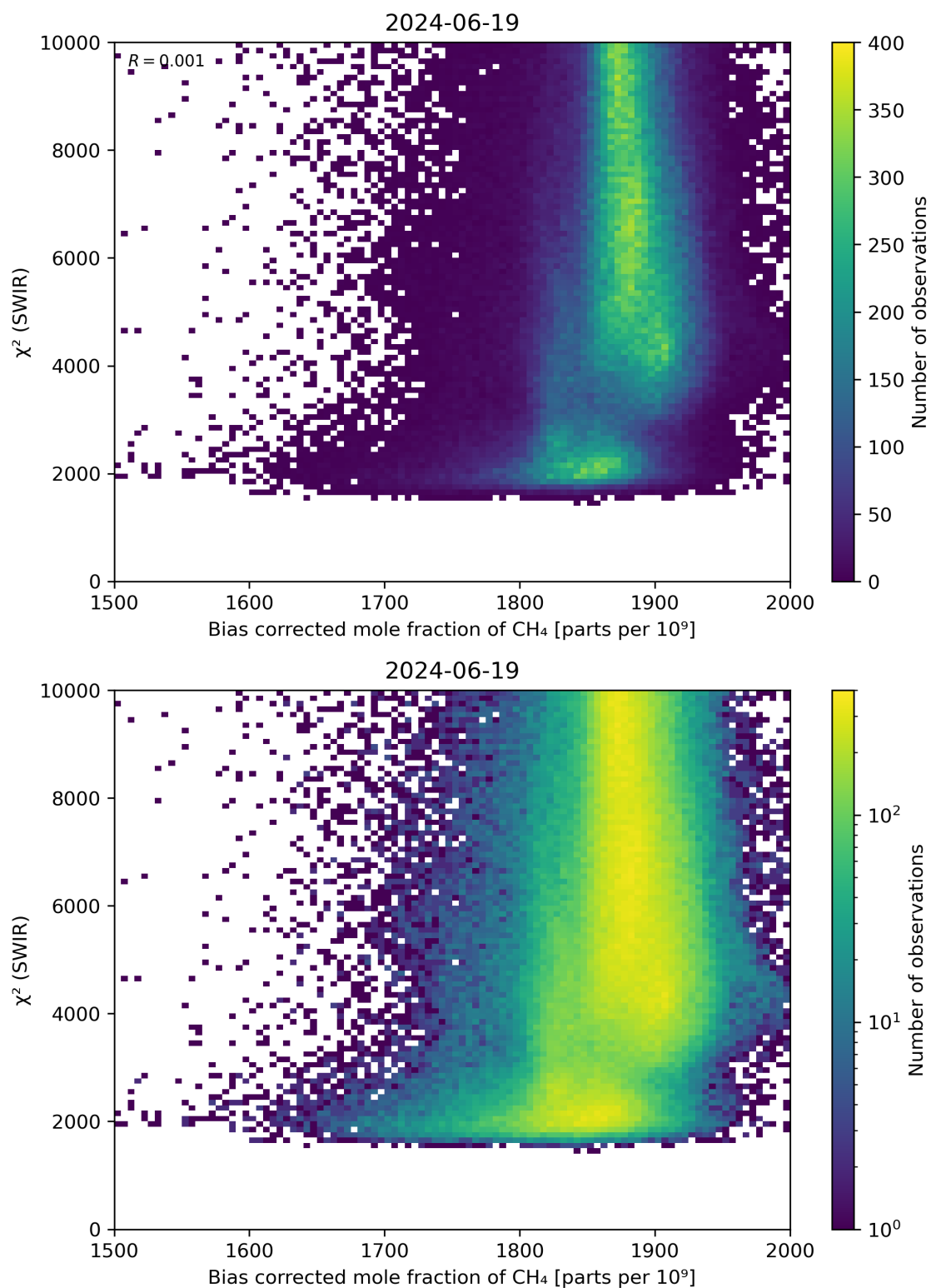
Figure 64: Scatter density plot of “Bias corrected mole fraction of CH 4 ” against “ \chi^2 (SWIR)” for 2024-06-19 to 2024-06-20.
