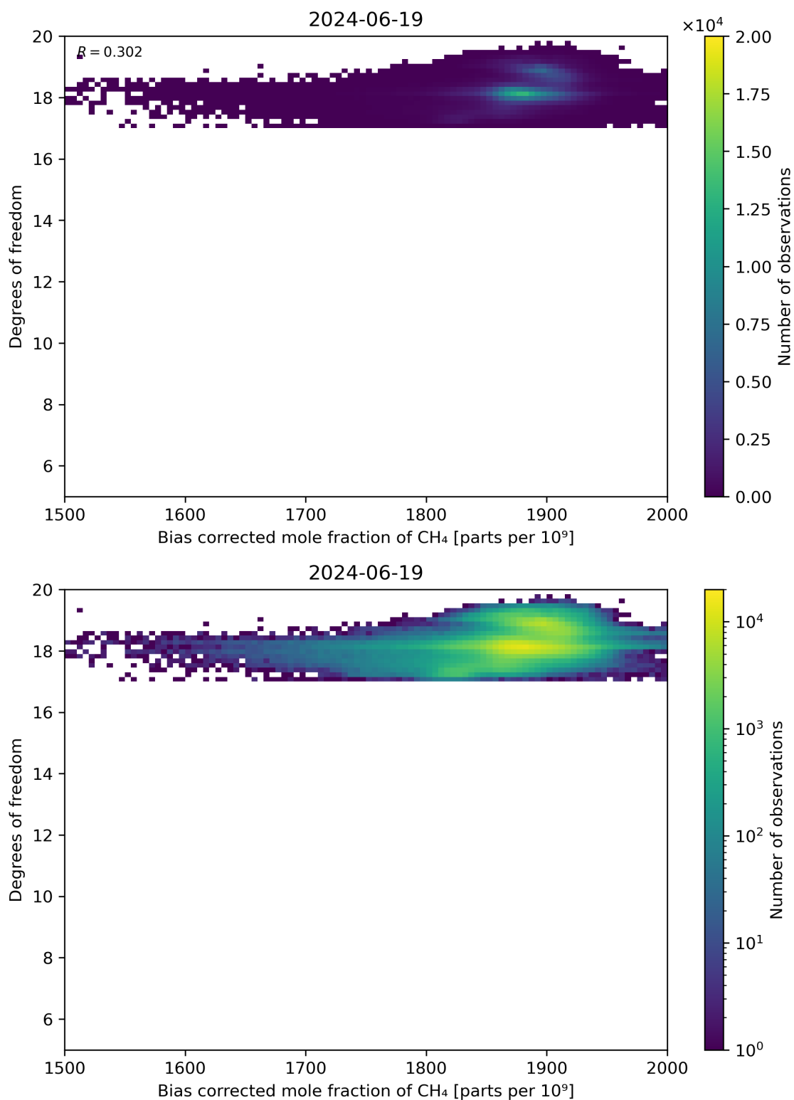
Figure 65: Scatter density plot of “Bias corrected mole fraction of CH 4 ” against “Degrees of freedom” for 2024-06-19 to 2024-06-20.
