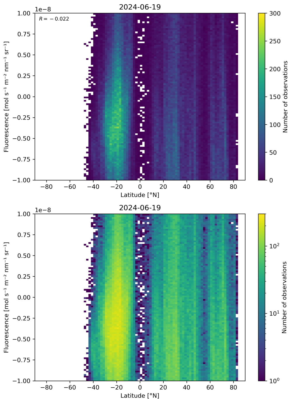
Figure 56: Scatter density plot of “Latitude” against “Fluorescence” for 2024-06-19 to 2024-06-20.
