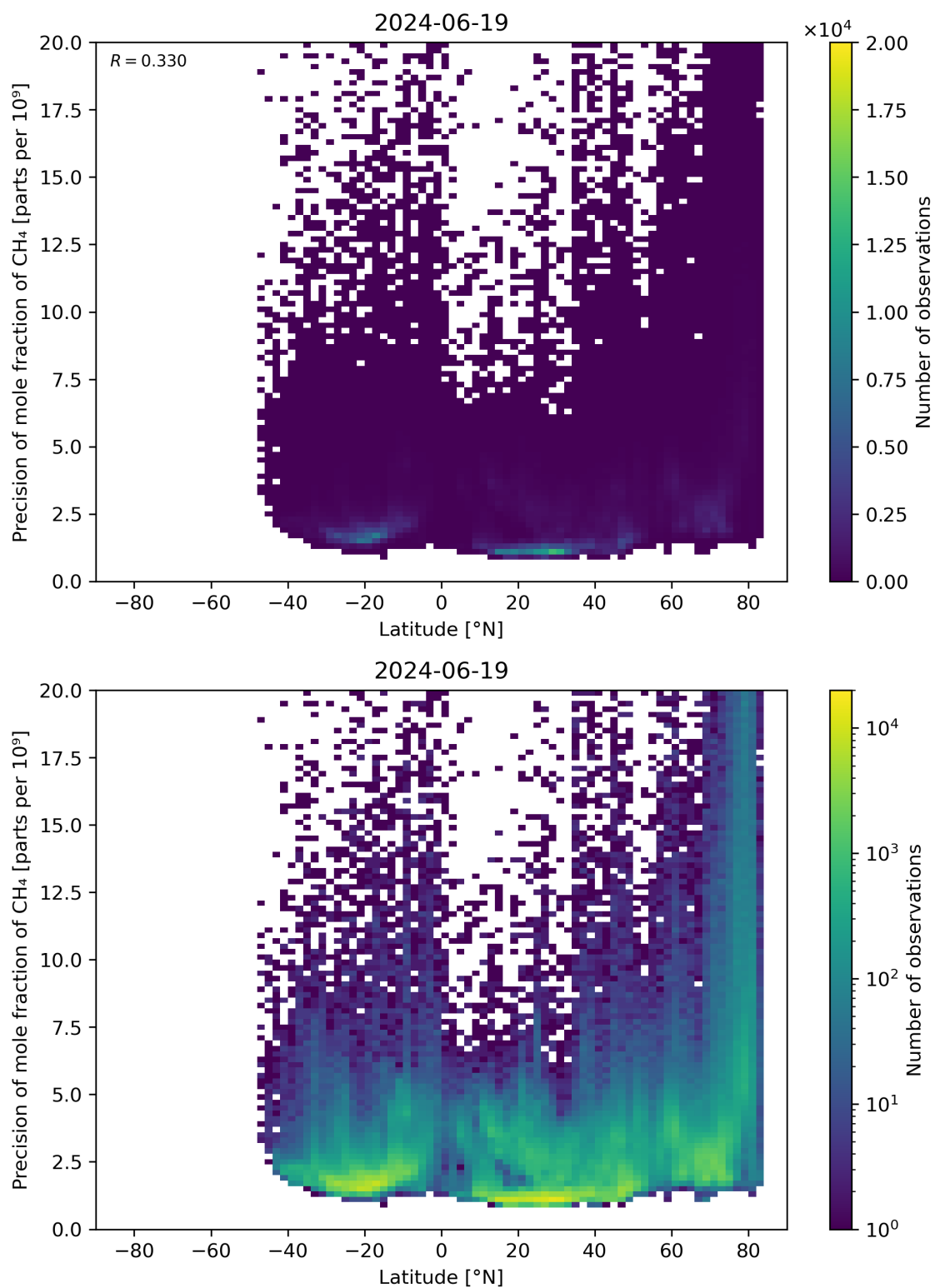
Figure 59: Scatter density plot of “Latitude” against “Precision of mole fraction of \text{CH}_4 ” for 2024-06-19 to 2024-06-20.
