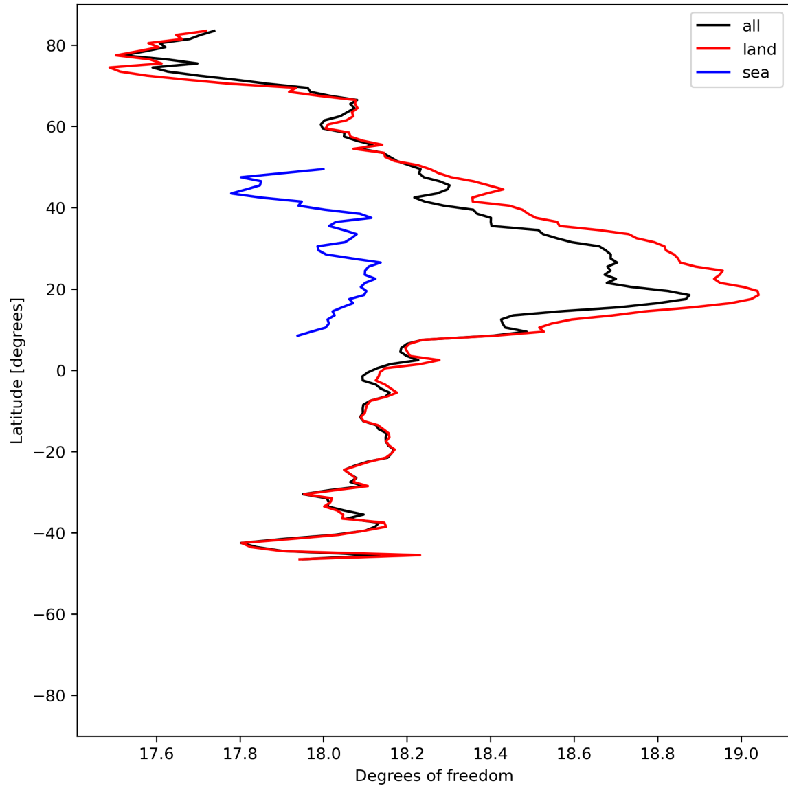
Figure 19: Zonal average of “Degrees of freedom” for 2024-06-19 to 2024-06-20.
