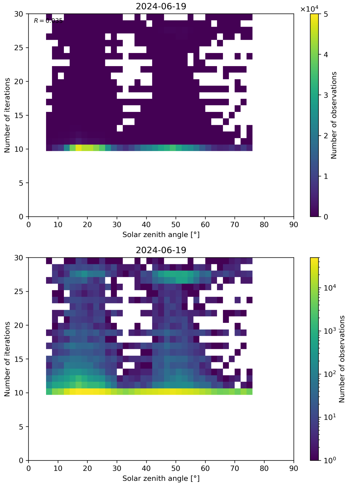
Figure 102: Scatter density plot of “Solar zenith angle” against “Number of iterations” for 2024-06-19 to 2024-06-20.
