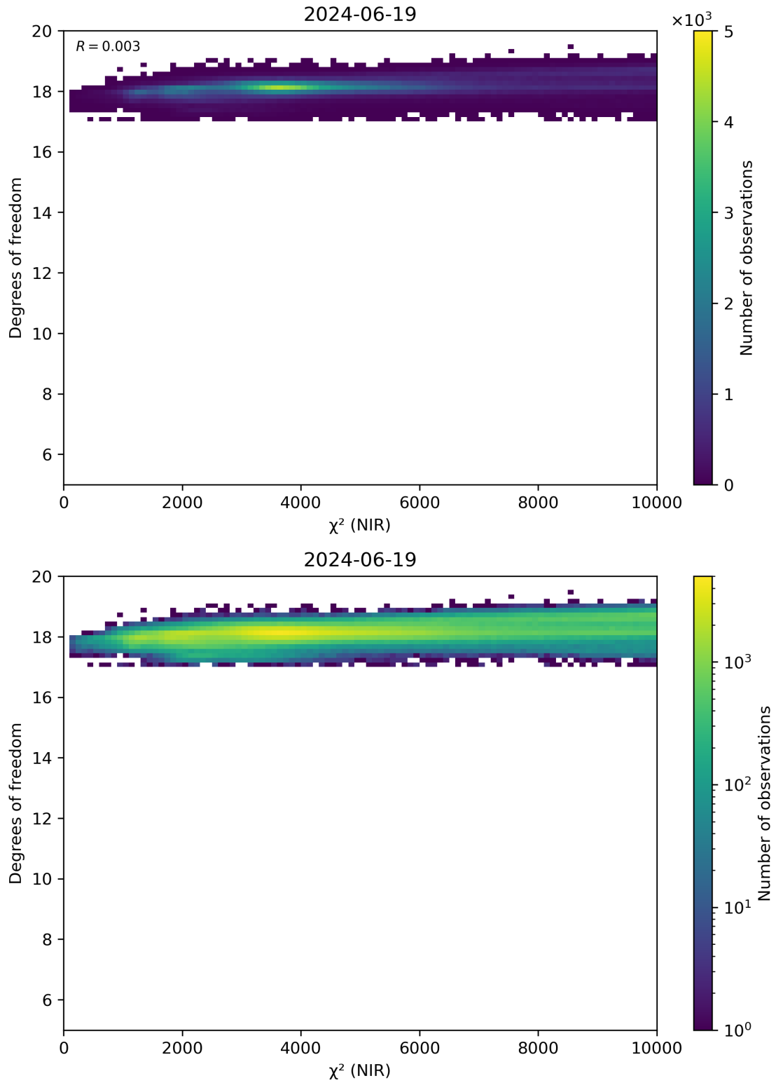
Figure 44: Scatter density plot of “ \chi^2 (NIR)” against “Degrees of freedom” for 2024-06-19 to 2024-06-20.
