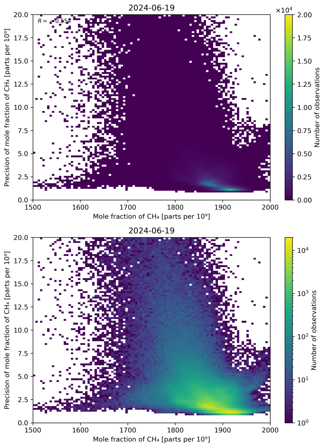
Figure 75: Scatter density plot of “Mole fraction of CH 4 ” against “Precision of mole fraction of CH 4 ” for 2024-06-19 to 2024-06-20.
