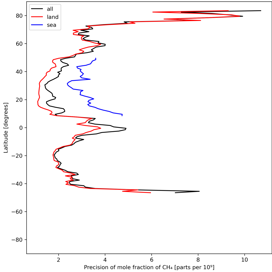
Figure 13: Zonal average of “Precision of mole fraction of CH 4 ” for 2024-06-19 to 2024-06-20.
