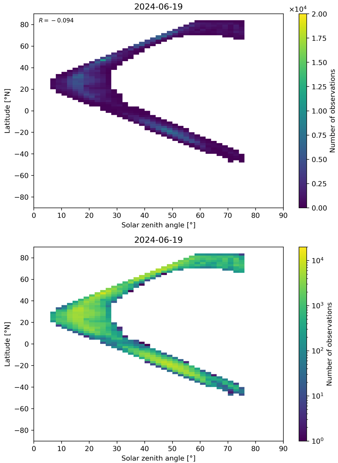
Figure 98: Scatter density plot of “Solar zenith angle” against “Latitude” for 2024-06-19 to 2024-06-20.
