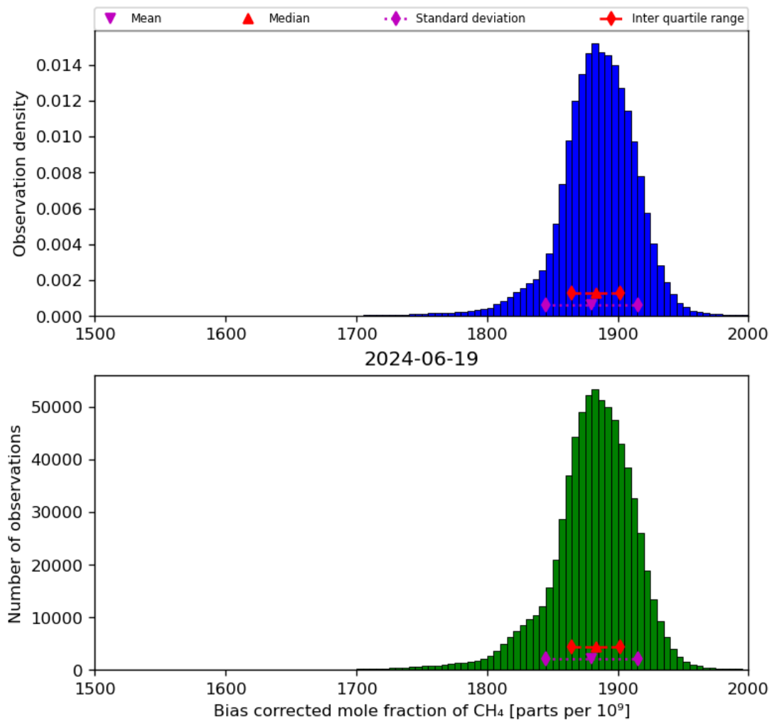
Figure 25: Histogram of “Bias corrected mole fraction of CH 4 ” for 2024-06-19 to 2024-06-20
