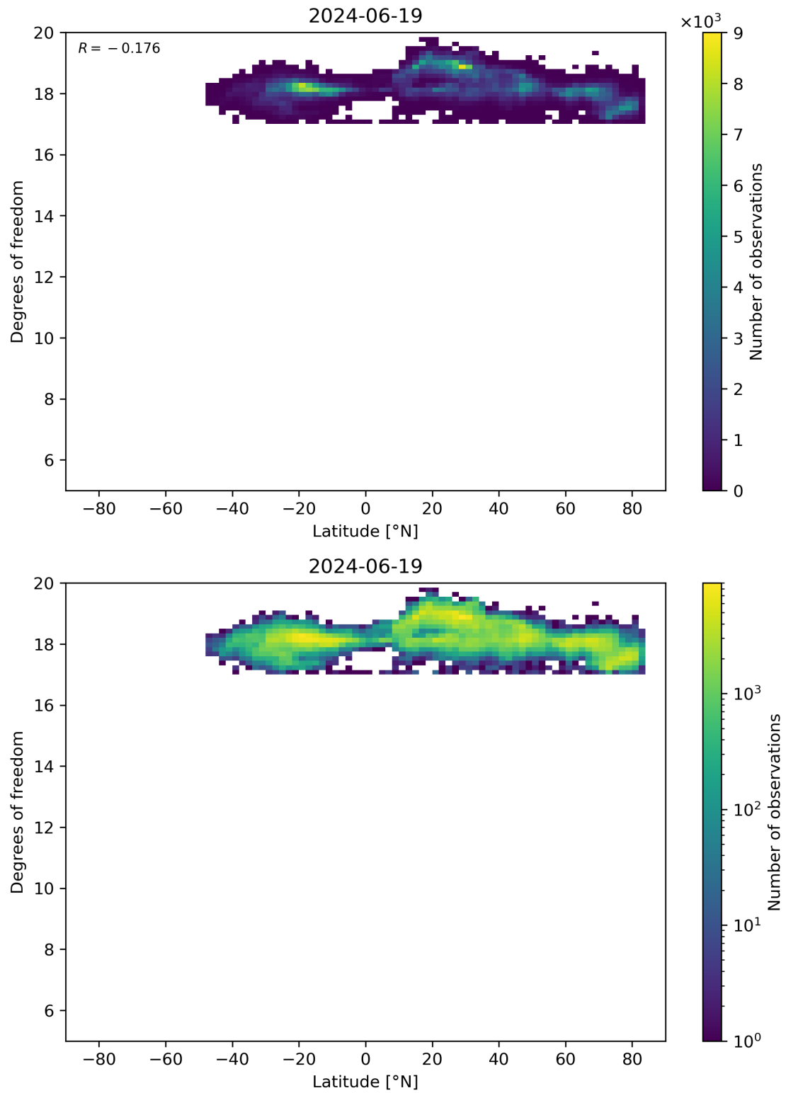
Figure 55: Scatter density plot of “Latitude” against “Degrees of freedom” for 2024-06-19 to 2024-06-20.
