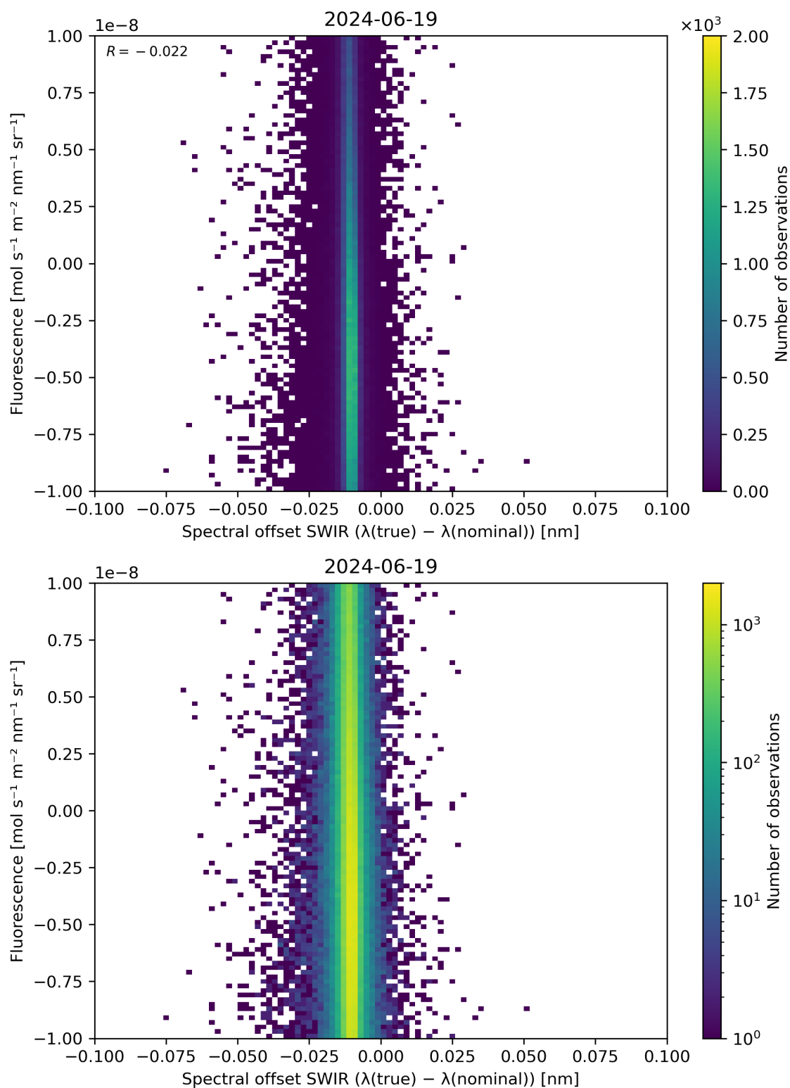
Figure 120: Scatter density plot of “Spectral offset SWIR ( \lambda(\text{true}) - \lambda(\text{nominal}) )” against “Fluorescence” for 2024-06-19 to 2024-06-20.
