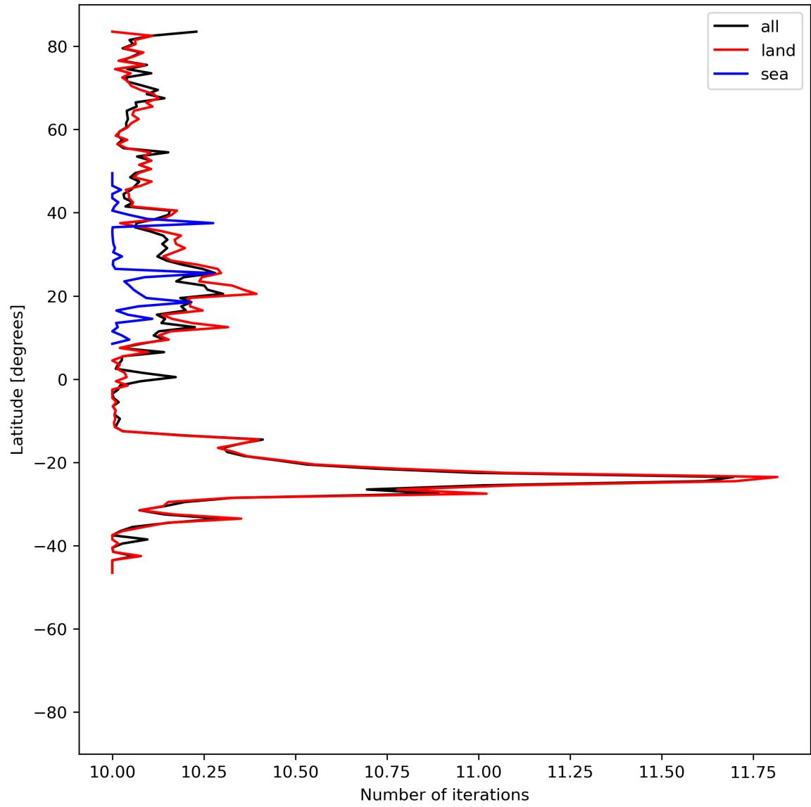
Figure 20: Zonal average of “Number of iterations” for 2024-06-19 to 2024-06-20.
