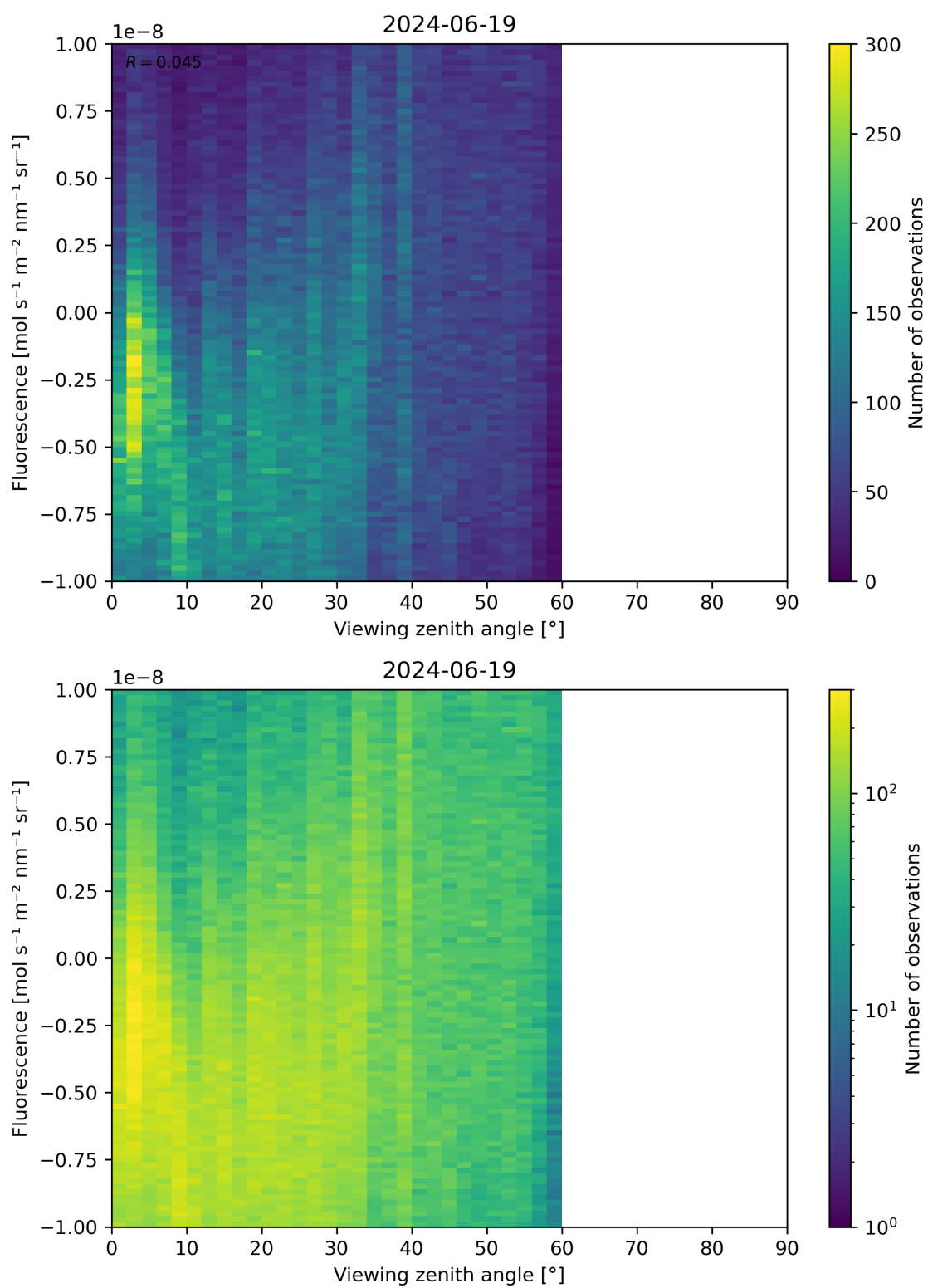
Figure 108: Scatter density plot of “Viewing zenith angle” against “Fluorescence” for 2024-06-19 to 2024-06-20.
