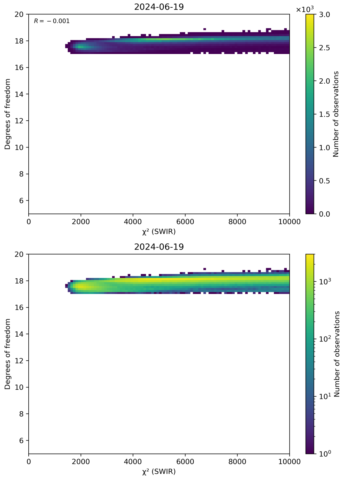
Figure 48: Scatter density plot of “ \chi^2 (SWIR)” against “Degrees of freedom” for 2024-06-19 to 2024-06-20.
