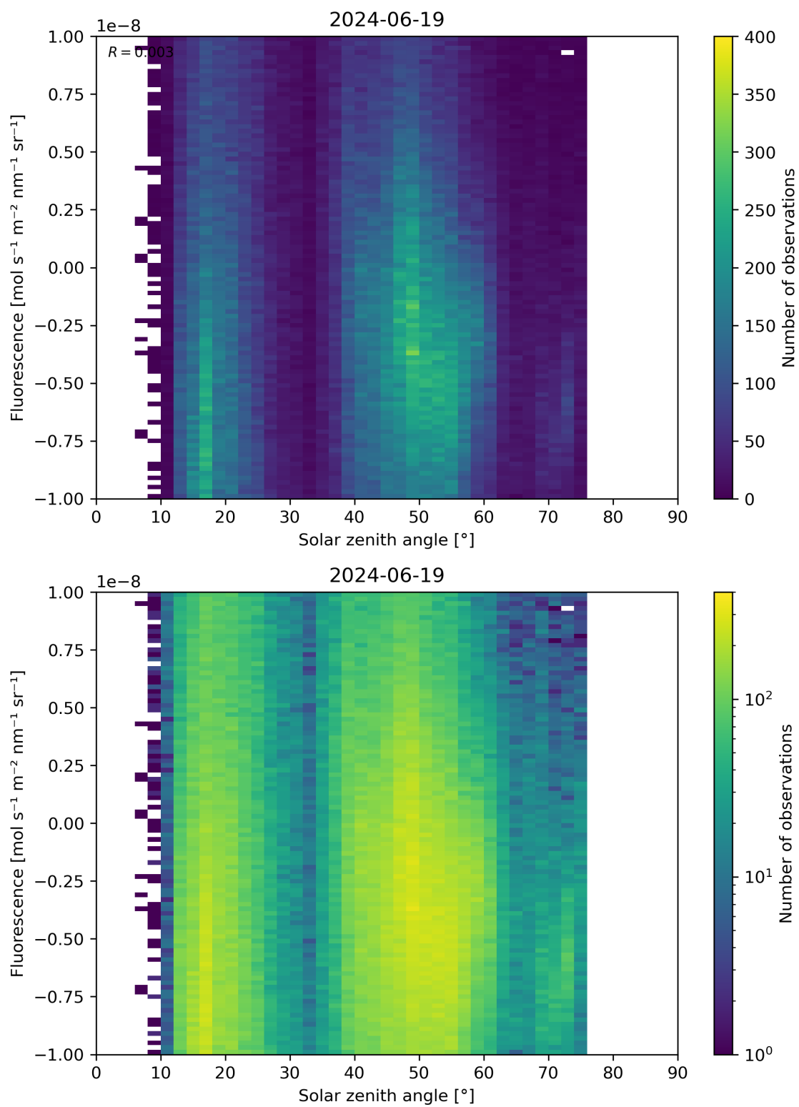
Figure 97: Scatter density plot of “Solar zenith angle” against “Fluorescence” for 2024-06-19 to 2024-06-20.
