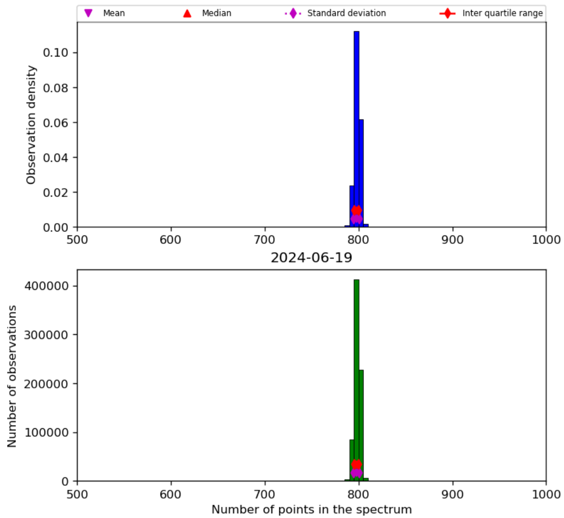
Figure 26: Histogram of “Number of points in the spectrum” for 2024-06-19 to 2024-06-20
