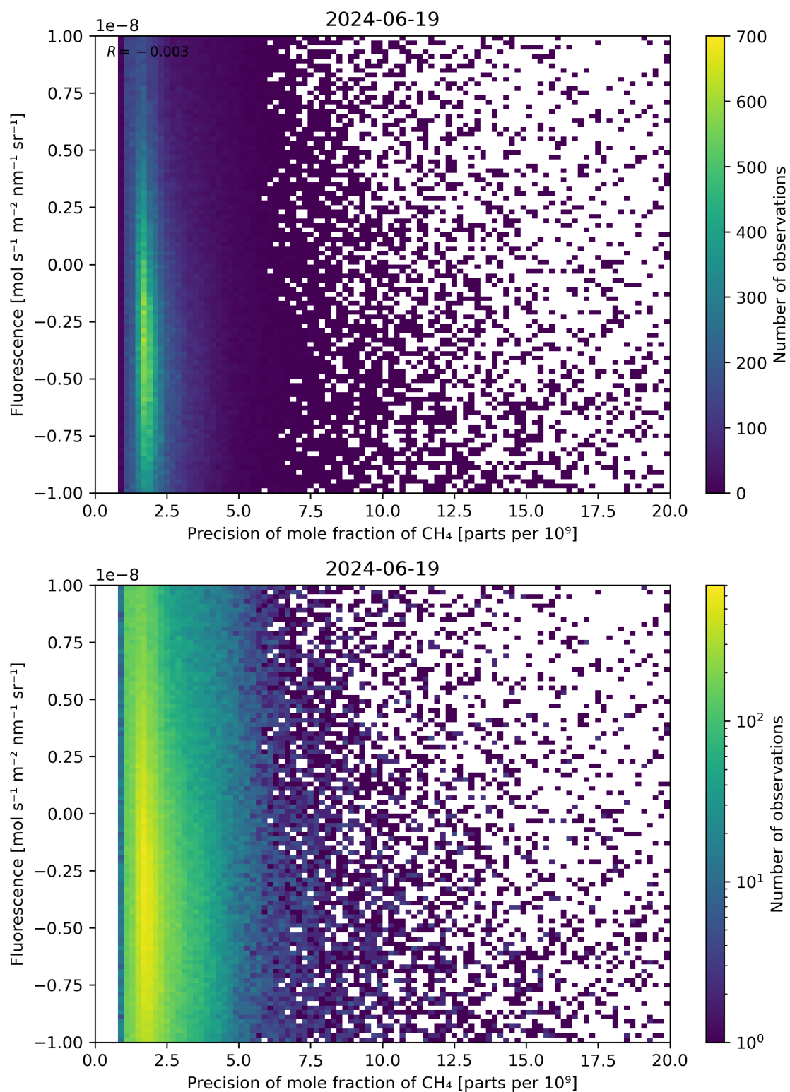
Figure 81: Scatter density plot of “Precision of mole fraction of \text{CH}_4 ” against “Fluorescence” for 2024-06-19 to 2024-06-20.
