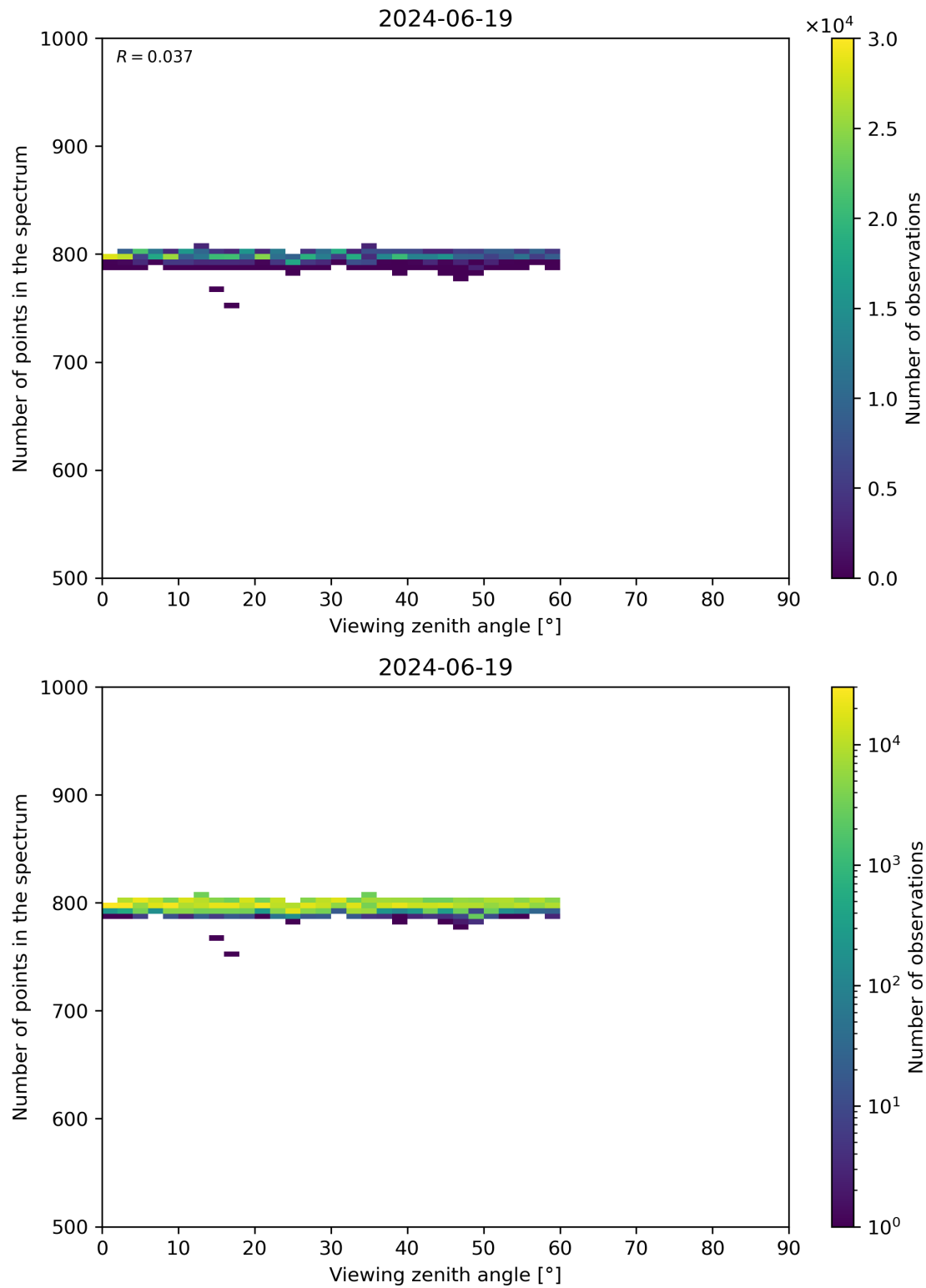
Figure 114: Scatter density plot of “Viewing zenith angle” against “Number of points in the spectrum” for 2024-06-19 to 2024-06-20.
