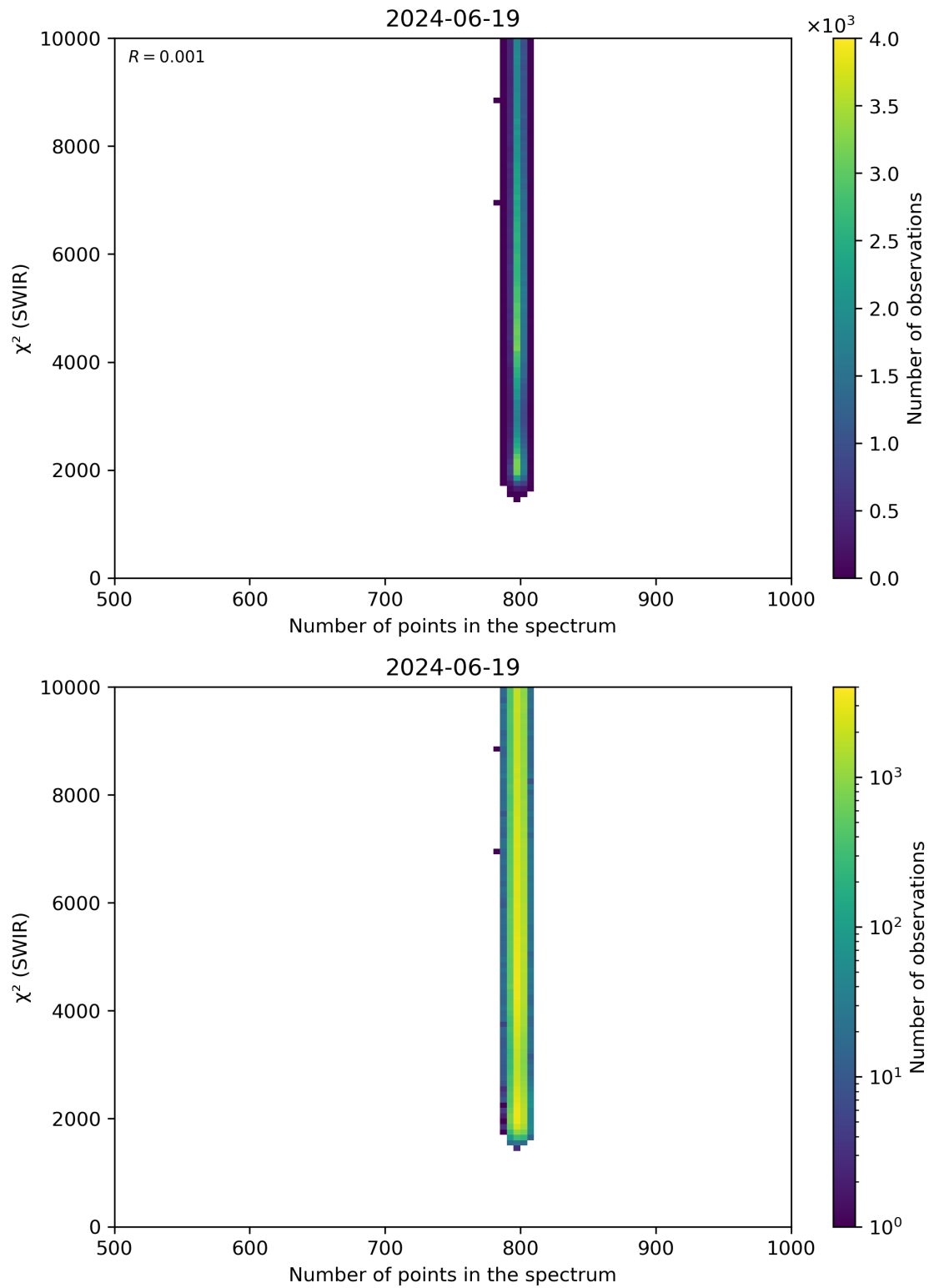
Figure 89: Scatter density plot of “Number of points in the spectrum” against “ \chi^2 (SWIR)” for 2024-06-19 to 2024-06-20.
