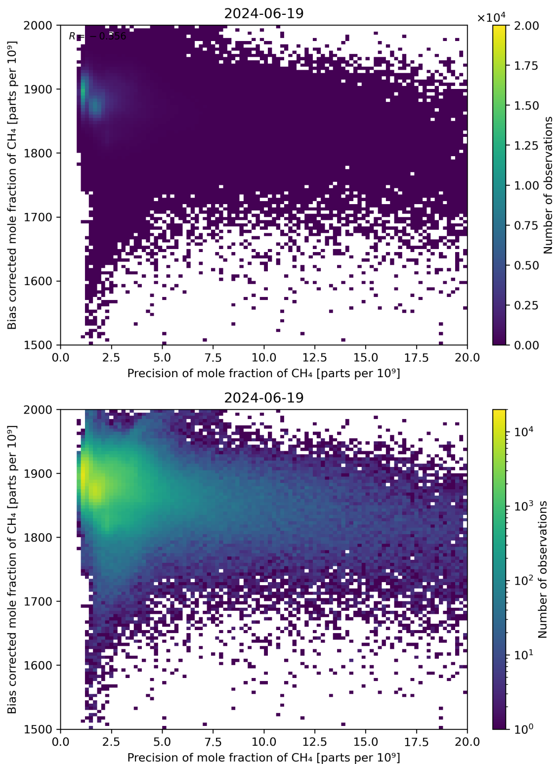
Figure 82: Scatter density plot of “Precision of mole fraction of CH 4 ” against “Bias corrected mole fraction of CH 4 ” for 2024-06-19 to 2024-06-20.
