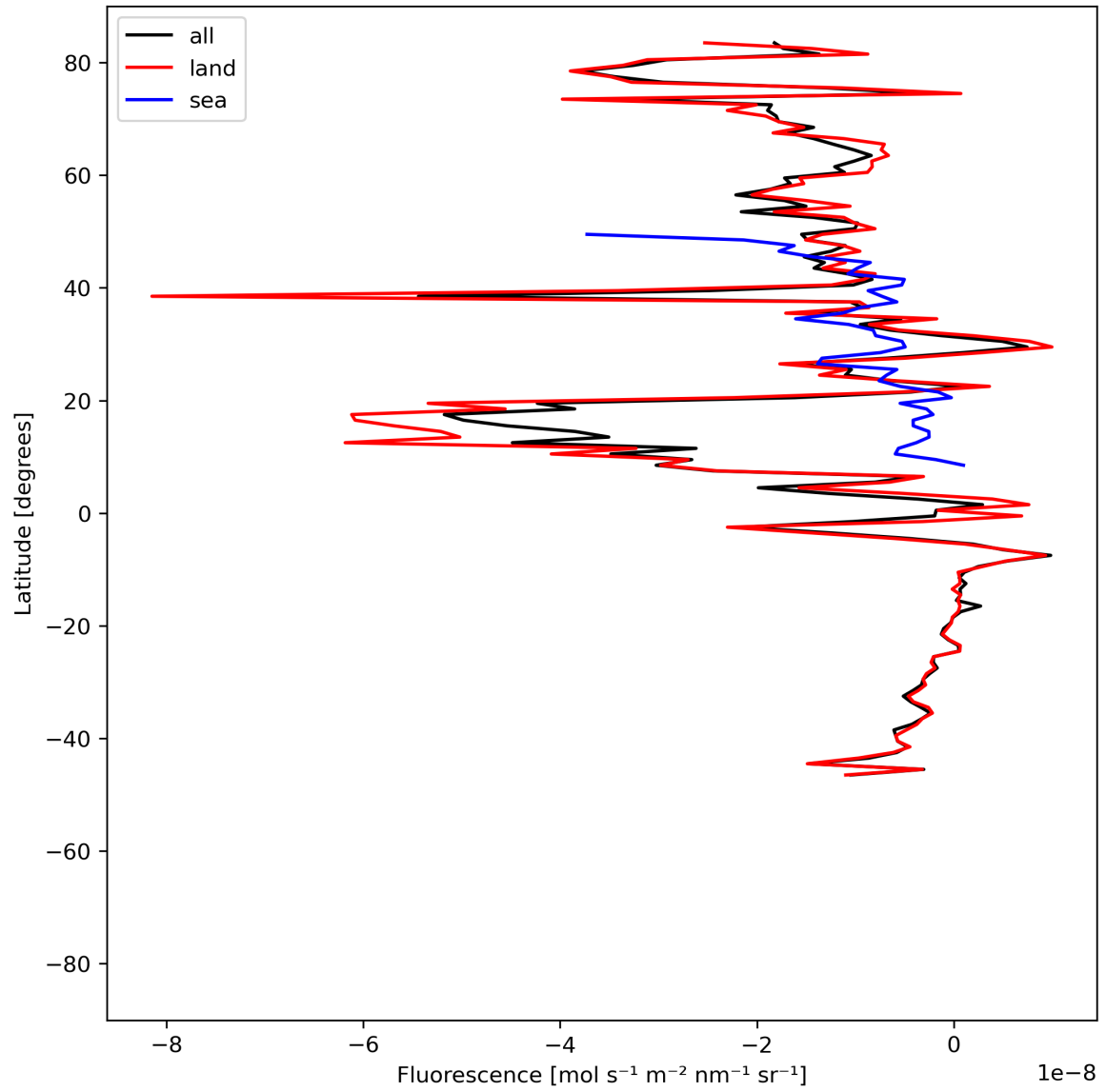
Figure 21: Zonal average of “Fluorescence” for 2024-06-19 to 2024-06-20.
