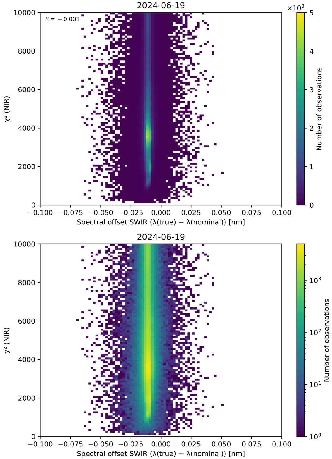
Figure 117: Scatter density plot of “Spectral offset SWIR ( \lambda(\text{true}) - \lambda(\text{nominal}) )” against “ \chi^2 (NIR)” for 2024-06-19 to 2024-06-20.
