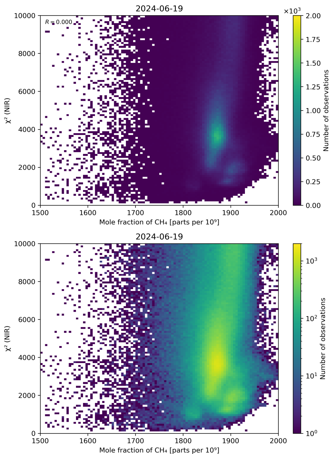
Figure 70: Scatter density plot of “Mole fraction of \text{CH}_4 ” against “ \chi^2 (NIR)” for 2024-06-19 to 2024-06-20.
