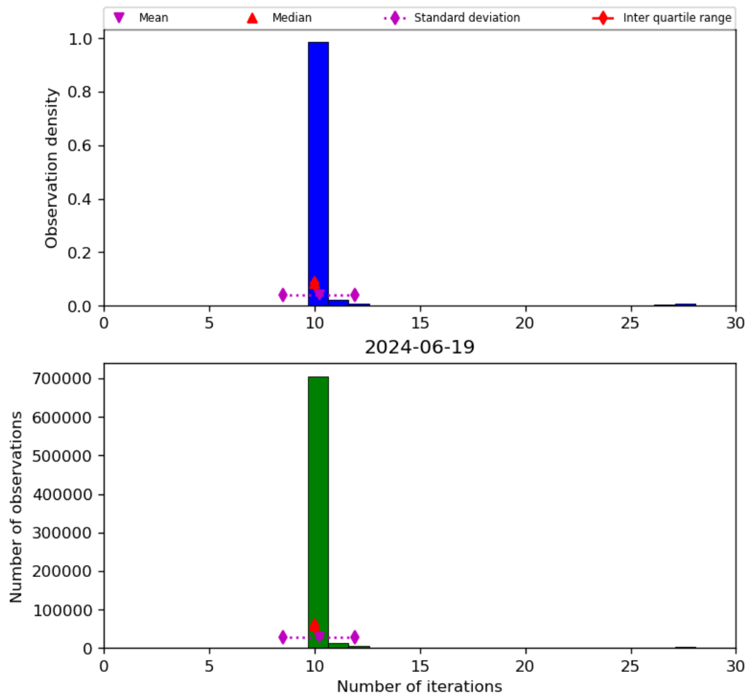
Figure 31: Histogram of “Number of iterations” for 2024-06-19 to 2024-06-20
