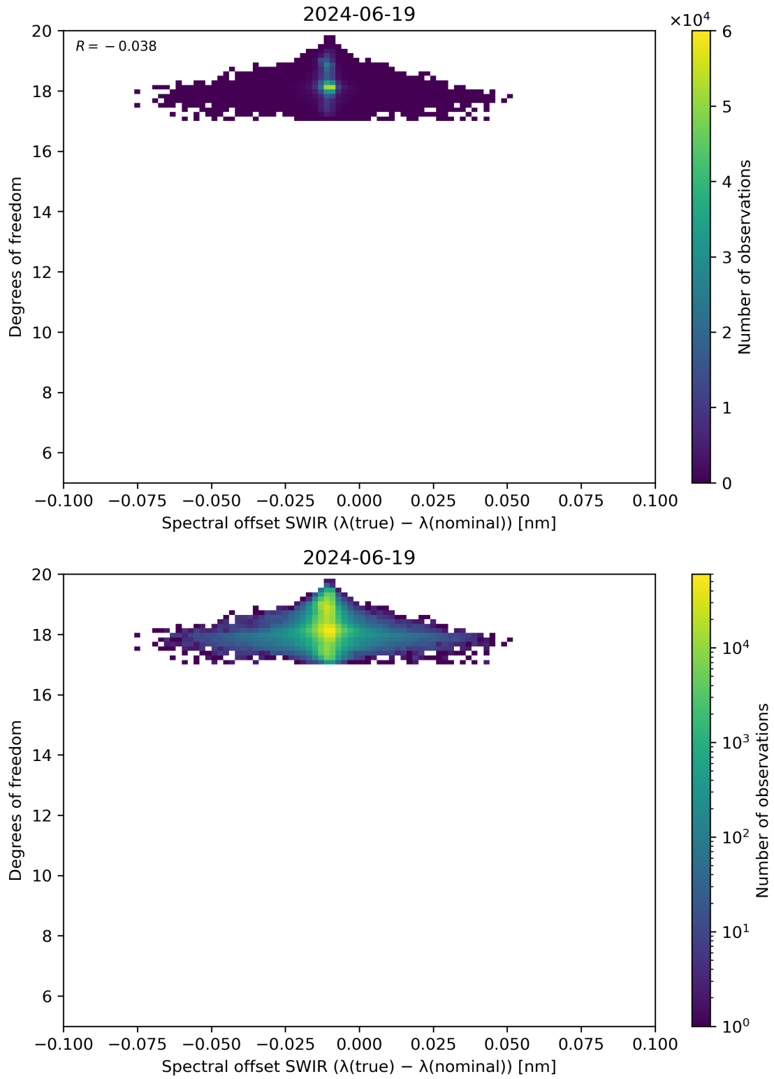
Figure 119: Scatter density plot of “Spectral offset SWIR ( \lambda(\text{true}) - \lambda(\text{nominal}) )” against “Degrees of freedom” for 2024-06-19 to 2024-06-20.
