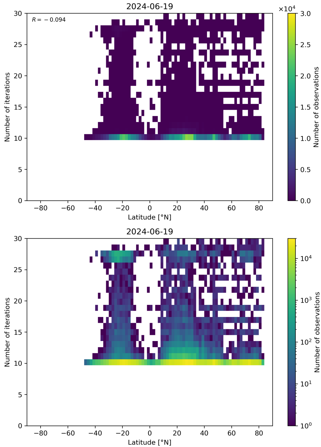
Figure 60: Scatter density plot of “Latitude” against “Number of iterations” for 2024-06-19 to 2024-06-20.
