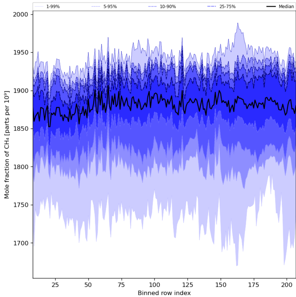
Figure 34: Along track statistics of “Mole fraction of CH 4 ” for 2024-06-19 to 2024-06-20
