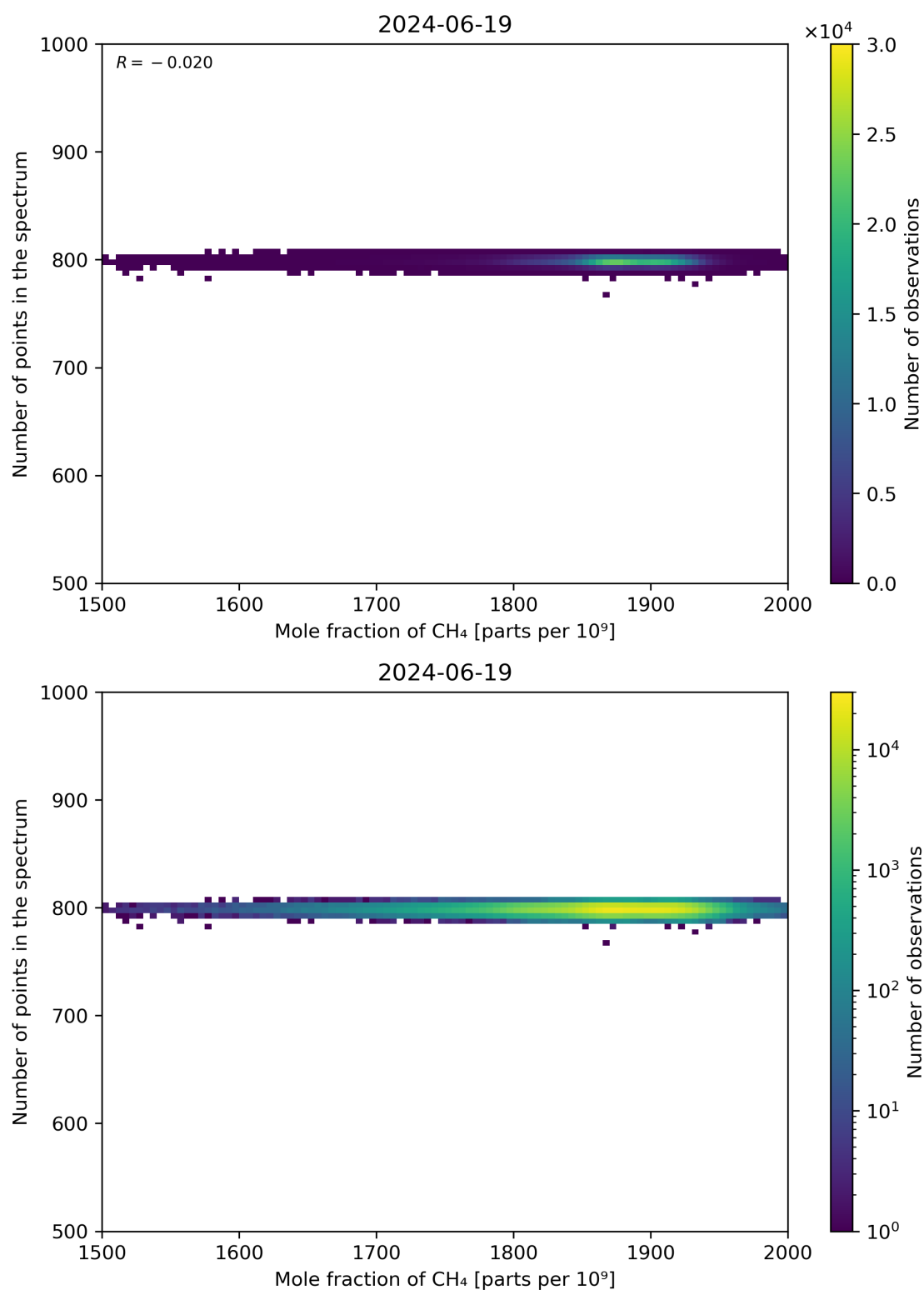
Figure 77: Scatter density plot of “Mole fraction of CH 4 ” against “Number of points in the spectrum” for 2024-06-19 to 2024-06-20.
