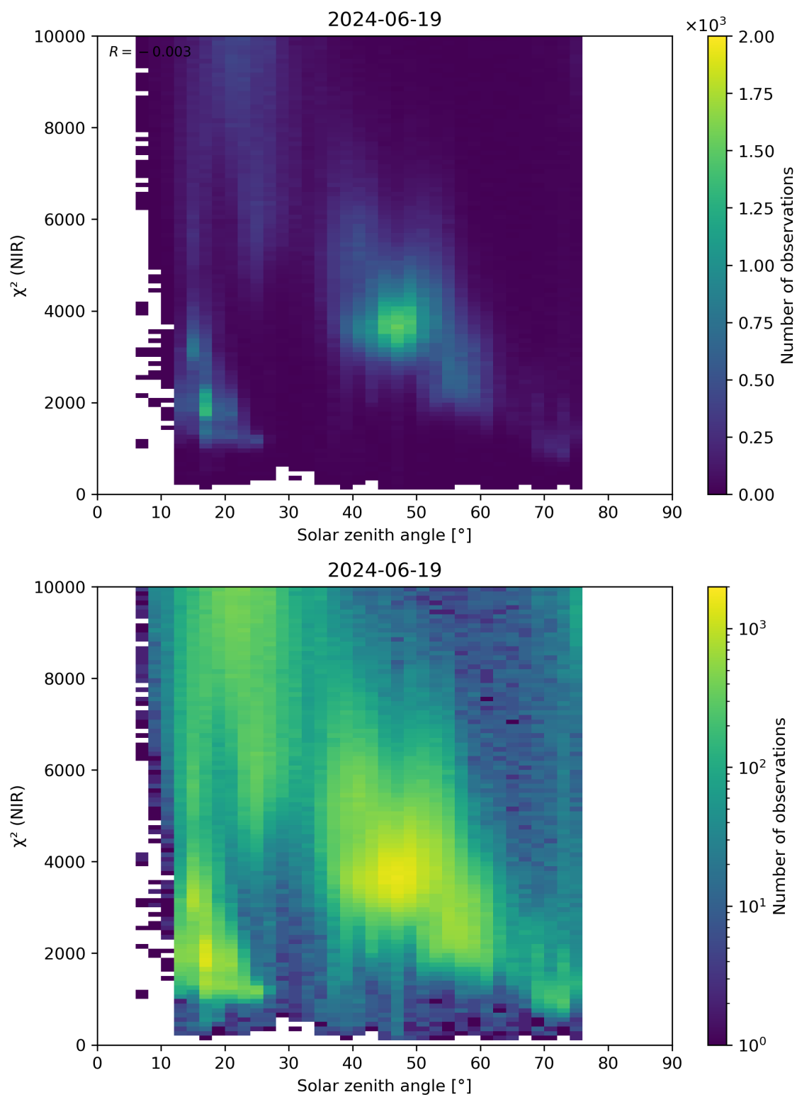
Figure 94: Scatter density plot of “Solar zenith angle” against “ \chi^2 (NIR)” for 2024-06-19 to 2024-06-20.
