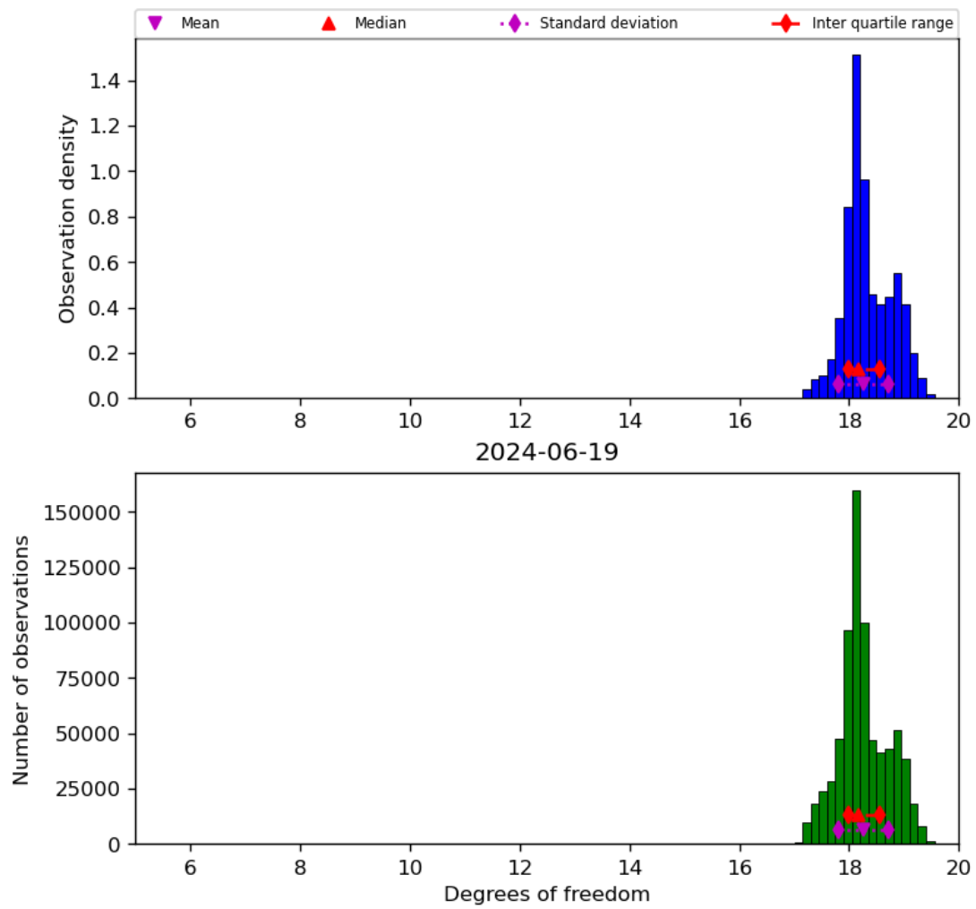
Figure 30: Histogram of “Degrees of freedom” for 2024-06-19 to 2024-06-20
