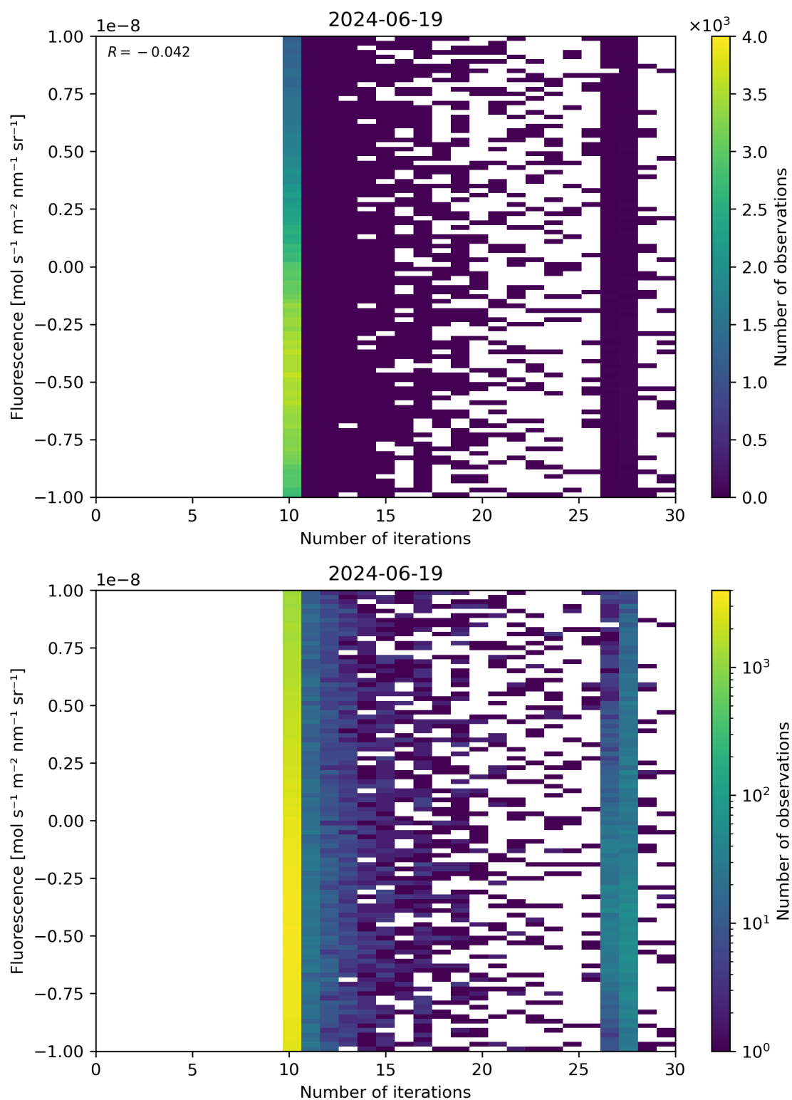
Figure 87: Scatter density plot of “Number of iterations” against “Fluorescence” for 2024-06-19 to 2024-06-20.
