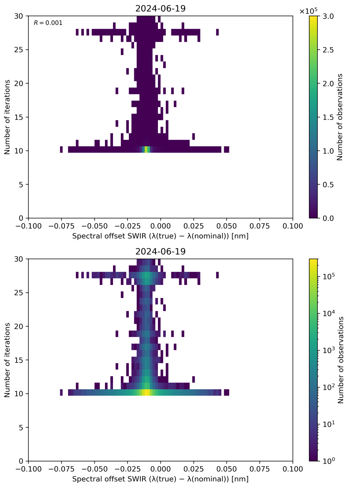
Figure 121: Scatter density plot of “Spectral offset SWIR ( \lambda(\text{true}) - \lambda(\text{nominal}) )” against “Number of iterations” for 2024-06-19 to 2024-06-20.
