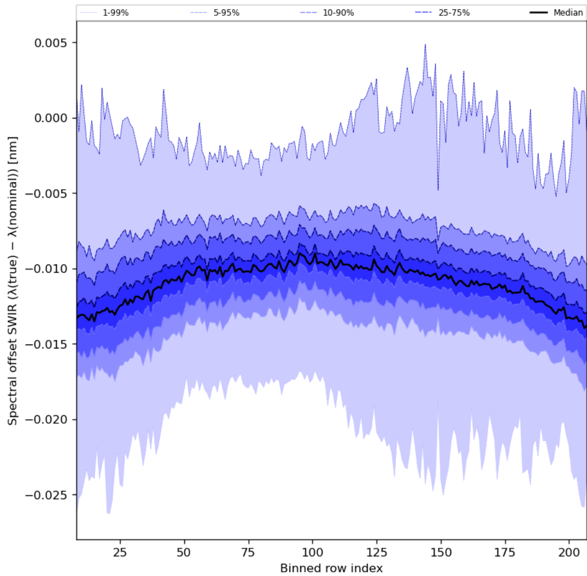
Figure 38: Along track statistics of “Spectral offset SWIR ( \lambda(\text{true}) - \lambda(\text{nominal}) )” for 2024-06-19 to 2024-06-20
