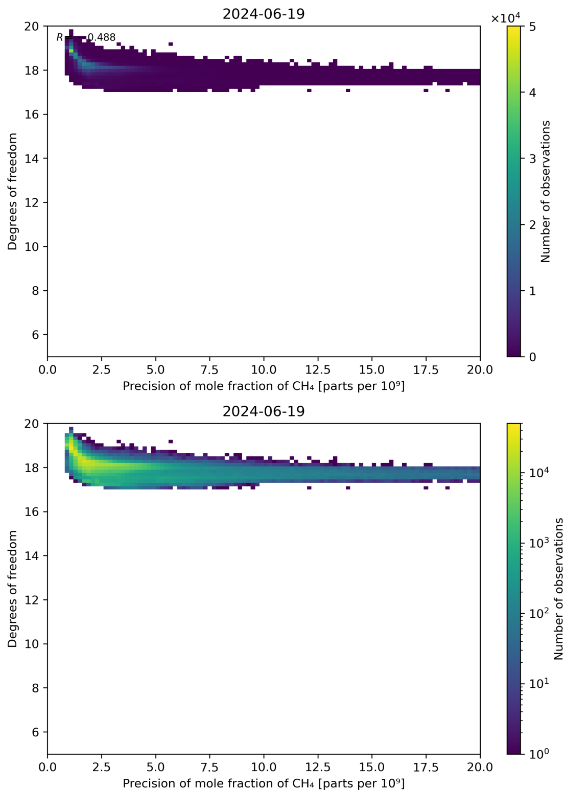
Figure 80: Scatter density plot of “Precision of mole fraction of CH 4 ” against “Degrees of freedom” for 2024-06-19 to 2024-06-20.
