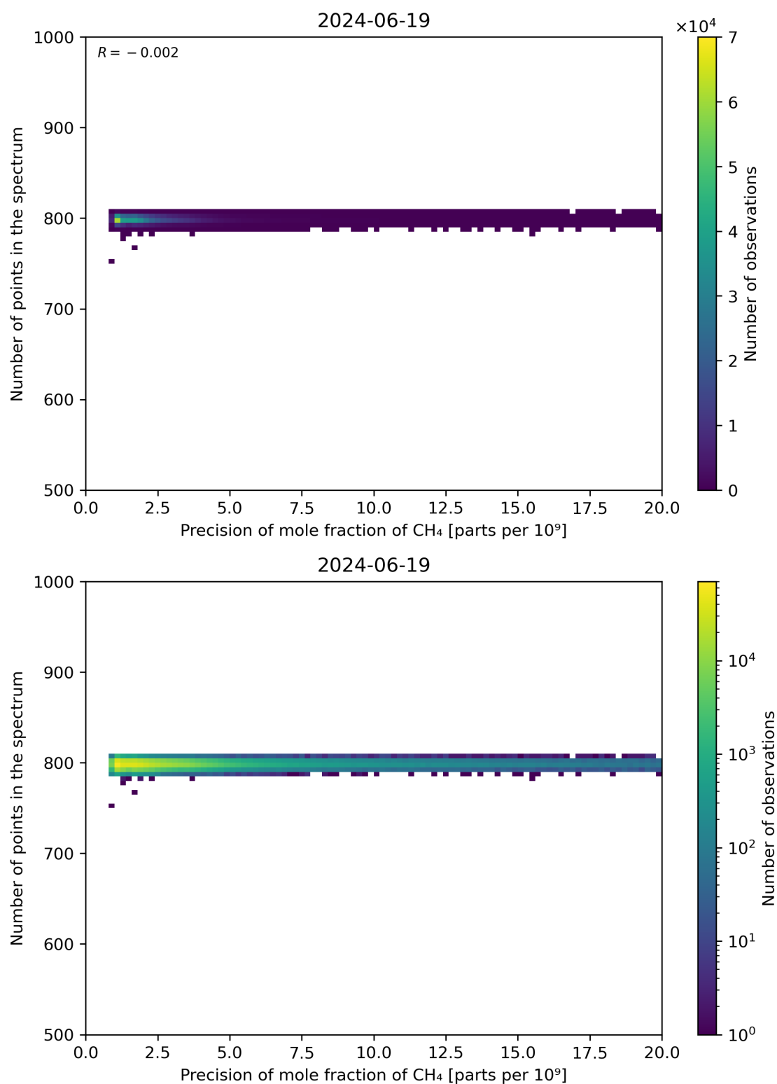
Figure 84: Scatter density plot of “Precision of mole fraction of CH 4 ” against “Number of points in the spectrum” for 2024-06-19 to 2024-06-20.
