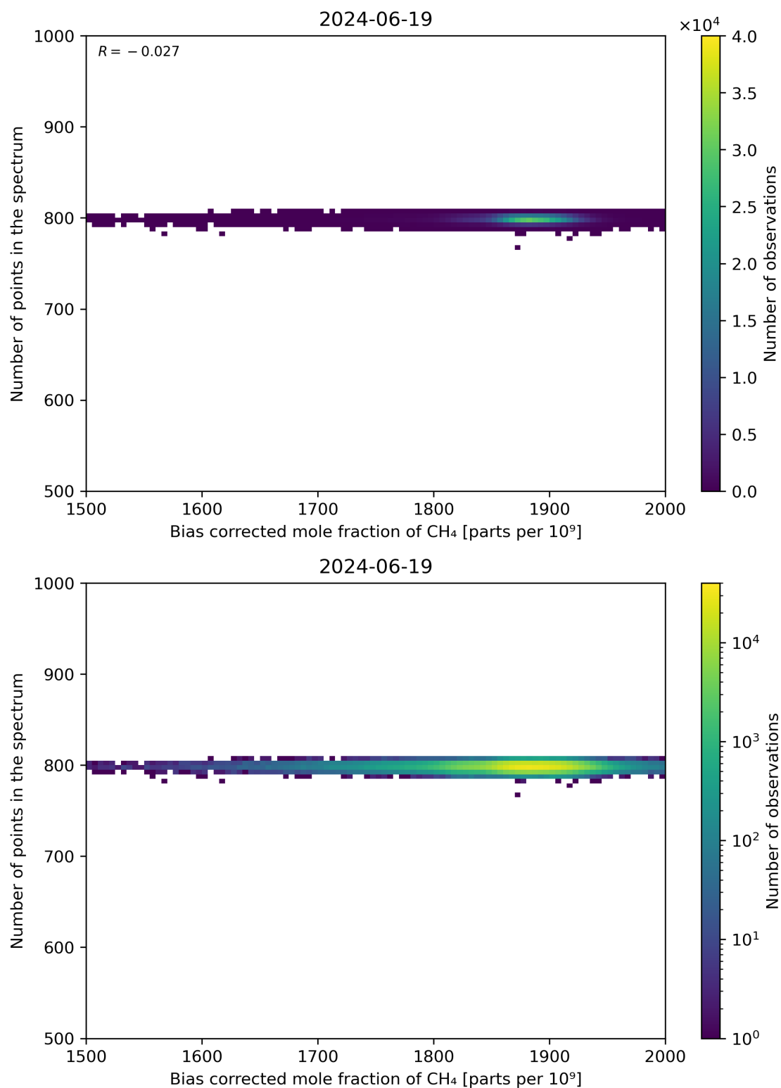
Figure 68: Scatter density plot of “Bias corrected mole fraction of CH 4 ” against “Number of points in the spectrum” for 2024-06-19 to 2024-06-20.
