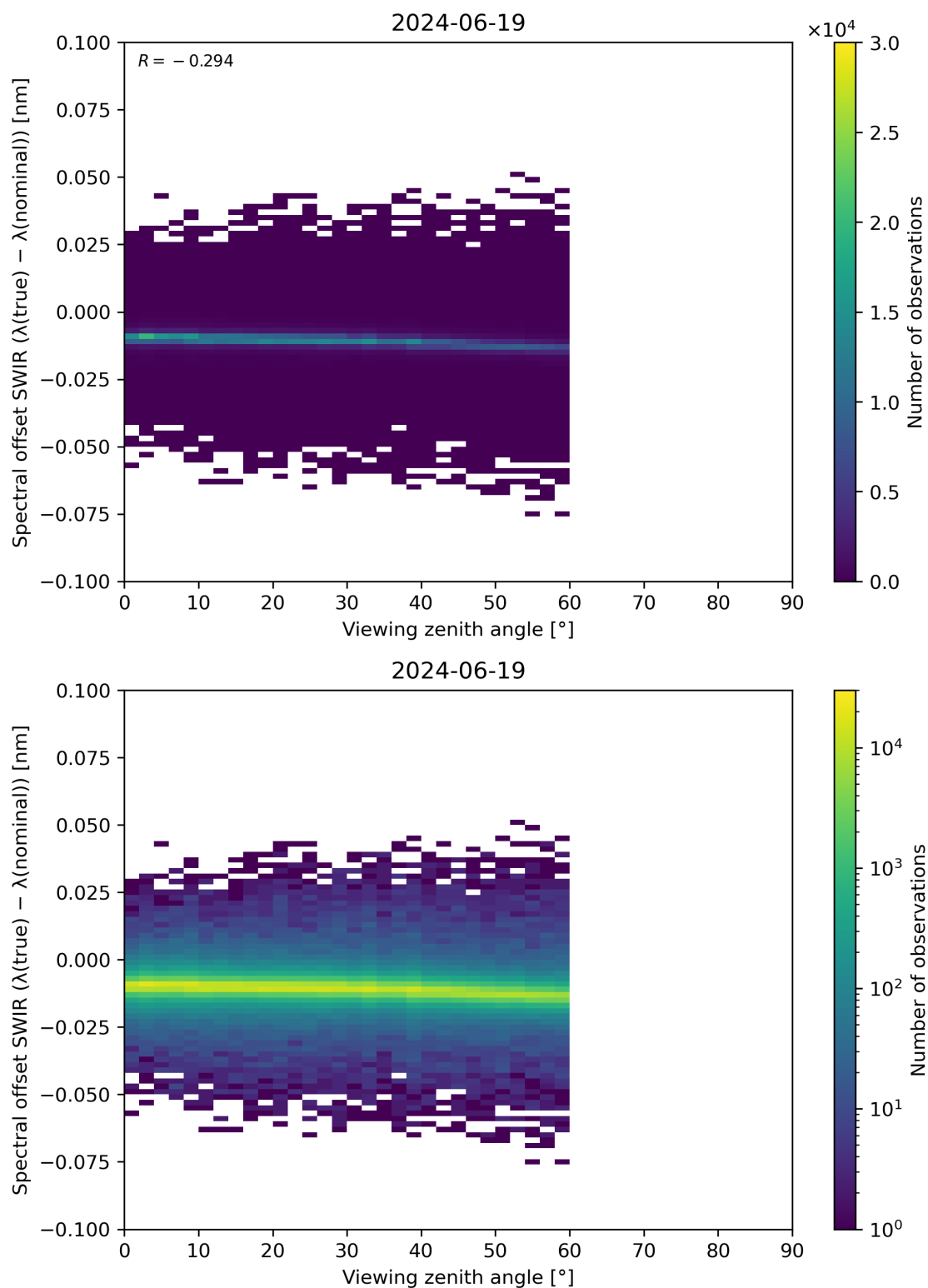
Figure 116: Scatter density plot of “Viewing zenith angle” against “Spectral offset SWIR ( \lambda(\text{true}) - \lambda(\text{nominal}) )” for 2024-06-19 to 2024-06-20.
