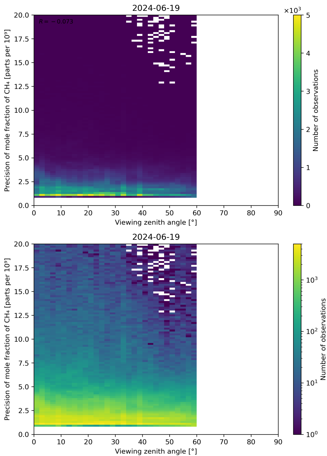
Figure 112: Scatter density plot of “Viewing zenith angle” against “Precision of mole fraction of CH 4 ” for 2024-06-19 to 2024-06-20.
