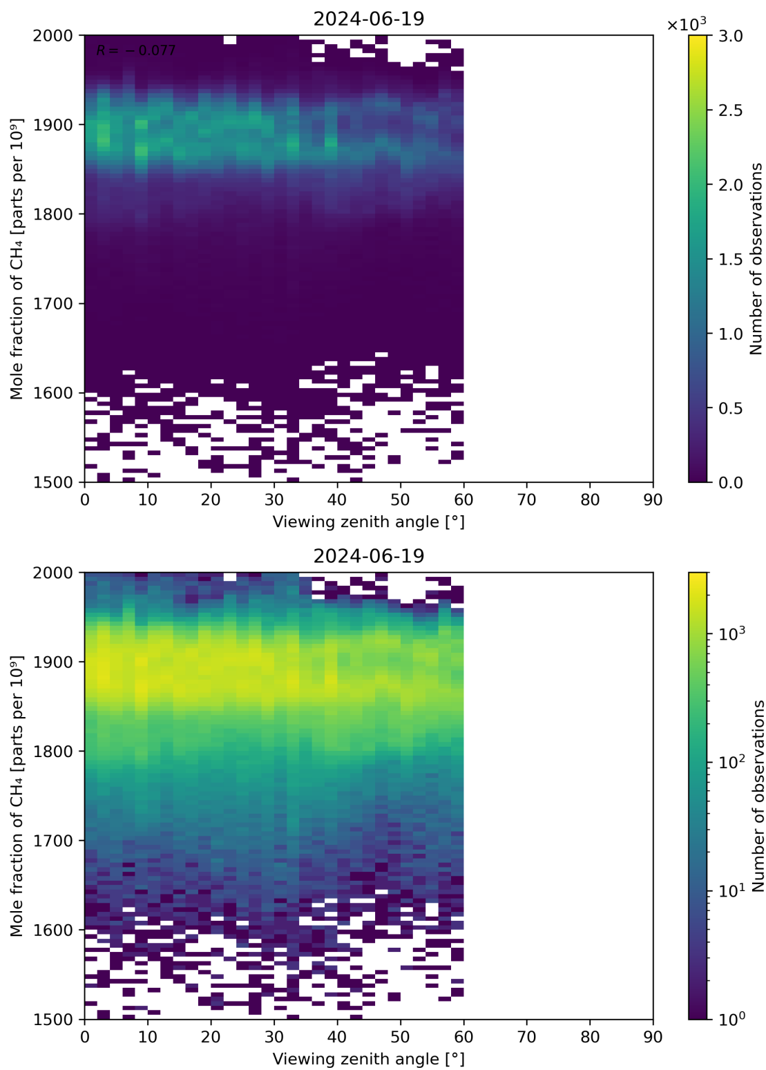
Figure 110: Scatter density plot of “Viewing zenith angle” against “Mole fraction of CH 4 ” for 2024-06-19 to 2024-06-20.
