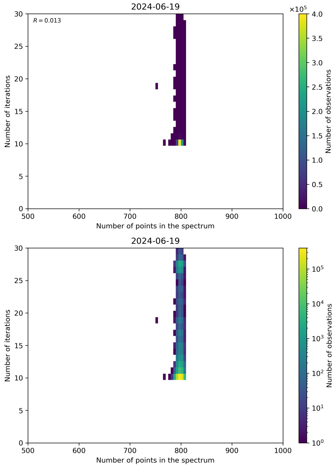
Figure 92: Scatter density plot of “Number of points in the spectrum” against “Number of iterations” for 2024-06-19 to 2024-06-20.
