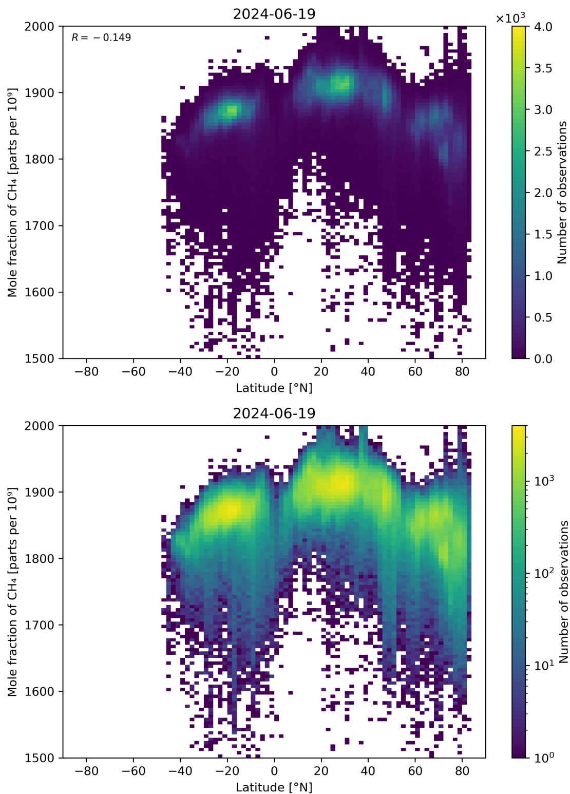
Figure 57: Scatter density plot of “Latitude” against “Mole fraction of CH 4 ” for 2024-06-19 to 2024-06-20.
