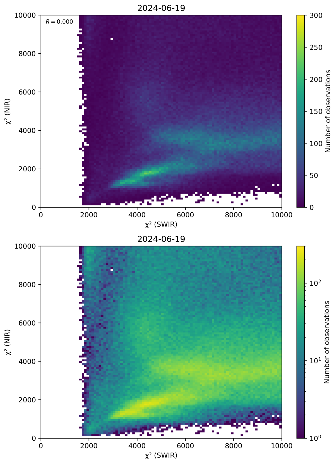
Figure 47: Scatter density plot of “ \chi^2 (SWIR)” against “ \chi^2 (NIR)” for 2024-06-19 to 2024-06-20.
