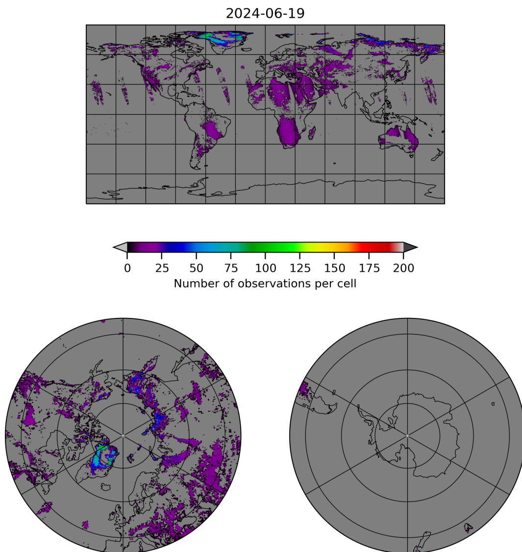
Figure 10: Map of the number of observations for 2024-06-19 to 2024-06-20
