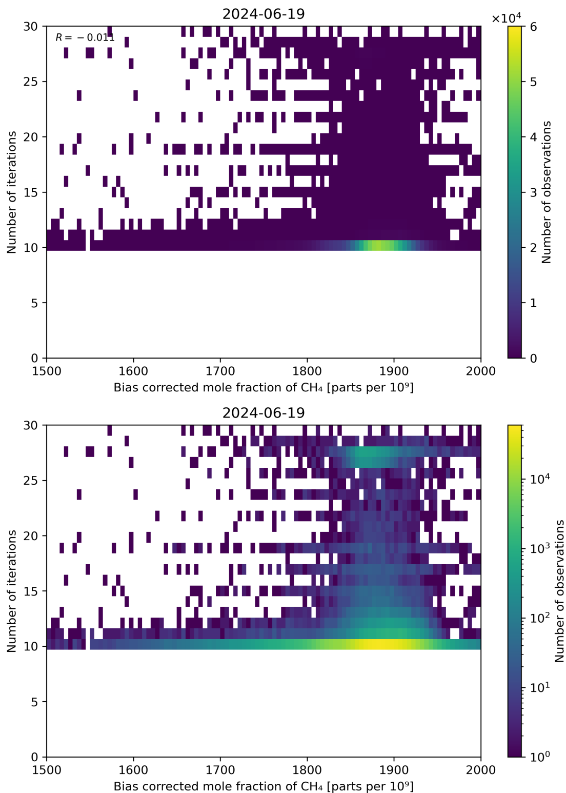
Figure 67: Scatter density plot of “Bias corrected mole fraction of CH 4 ” against “Number of iterations” for 2024-06-19 to 2024-06-20.
