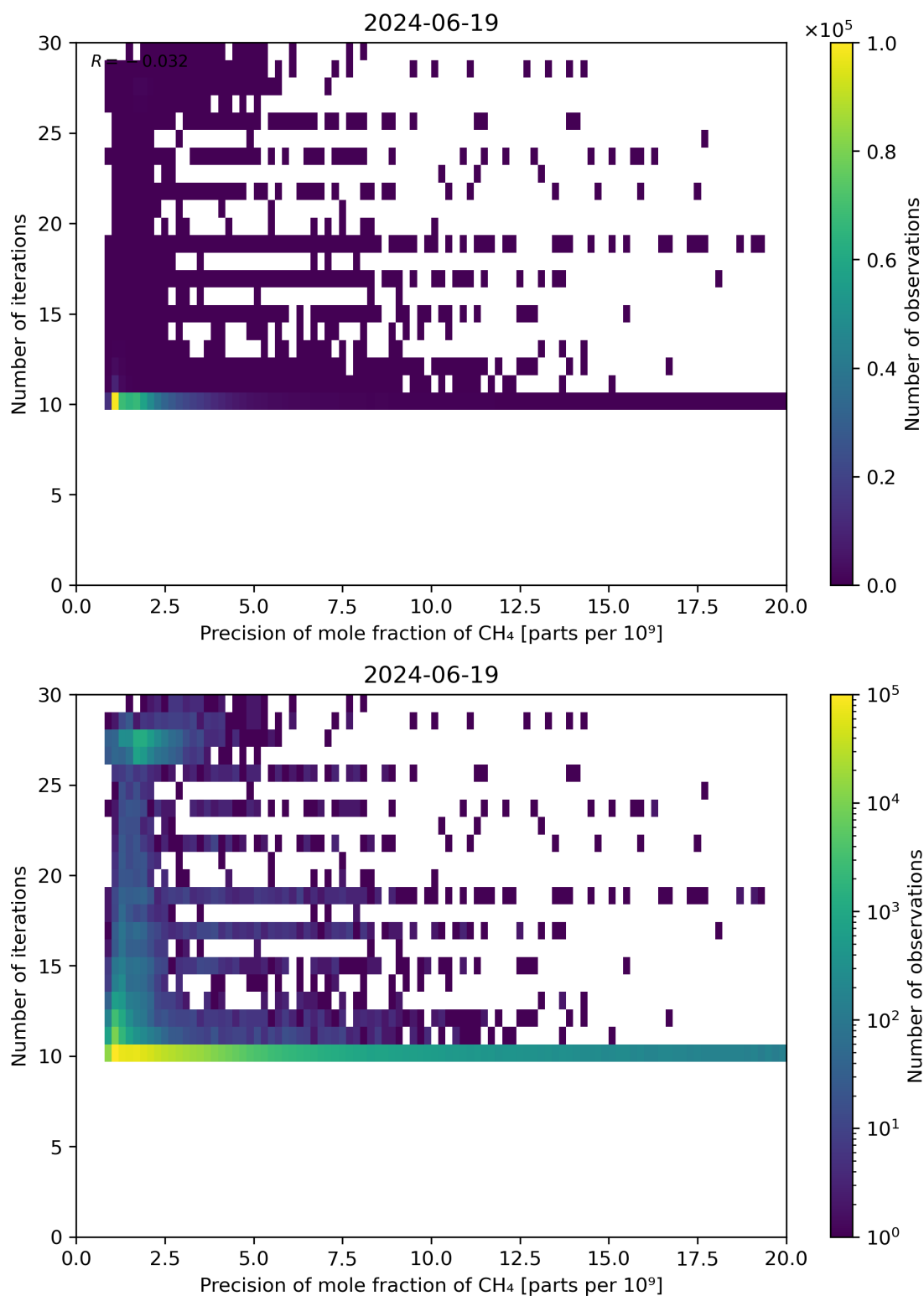
Figure 83: Scatter density plot of “Precision of mole fraction of CH 4 ” against “Number of iterations” for 2024-06-19 to 2024-06-20.
