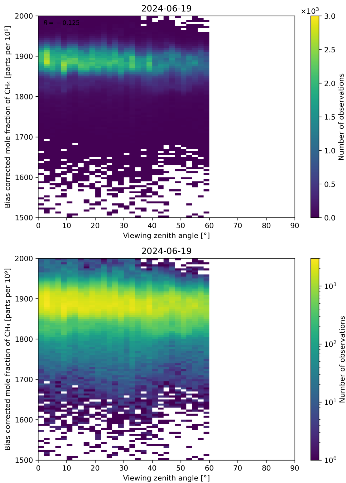
Figure 111: Scatter density plot of “Viewing zenith angle” against “Bias corrected mole fraction of CH 4 ” for 2024-06-19 to 2024-06-20.
