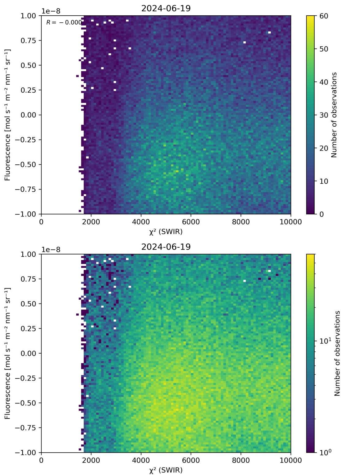
Figure 49: Scatter density plot of “ \chi^2 (SWIR)” against “Fluorescence” for 2024-06-19 to 2024-06-20.
