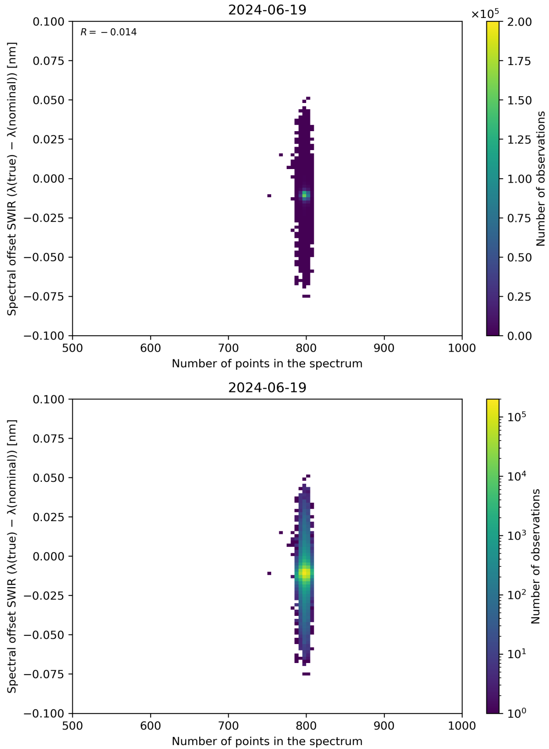
Figure 93: Scatter density plot of “Number of points in the spectrum” against “Spectral offset SWIR ( \lambda(\text{true}) - \lambda(\text{nominal}) )” for 2024-06-19 to 2024-06-20.
