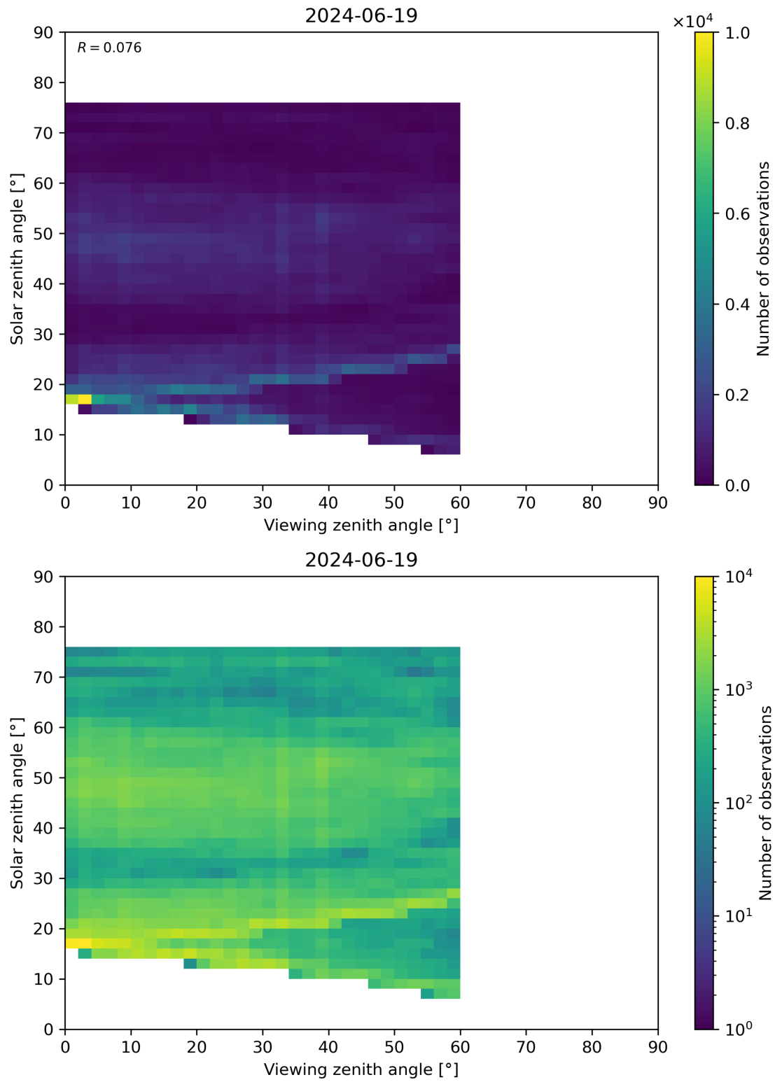
Figure 115: Scatter density plot of “Viewing zenith angle” against “Solar zenith angle” for 2024-06-19 to 2024-06-20.
