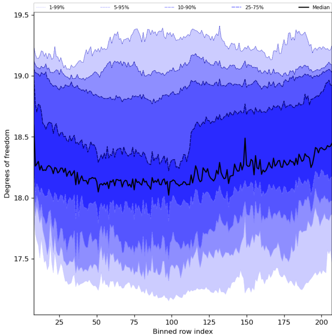
Figure 41: Along track statistics of “Degrees of freedom” for 2024-06-19 to 2024-06-20
