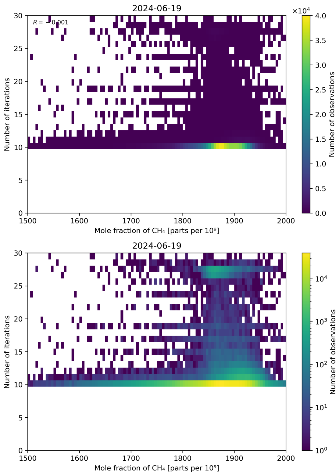
Figure 76: Scatter density plot of “Mole fraction of CH 4 ” against “Number of iterations” for 2024-06-19 to 2024-06-20.
