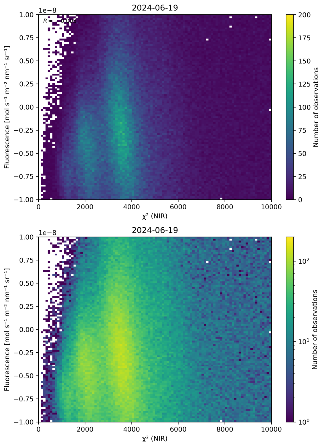
Figure 45: Scatter density plot of “ \chi^2 (NIR)” against “Fluorescence” for 2024-06-19 to 2024-06-20.
