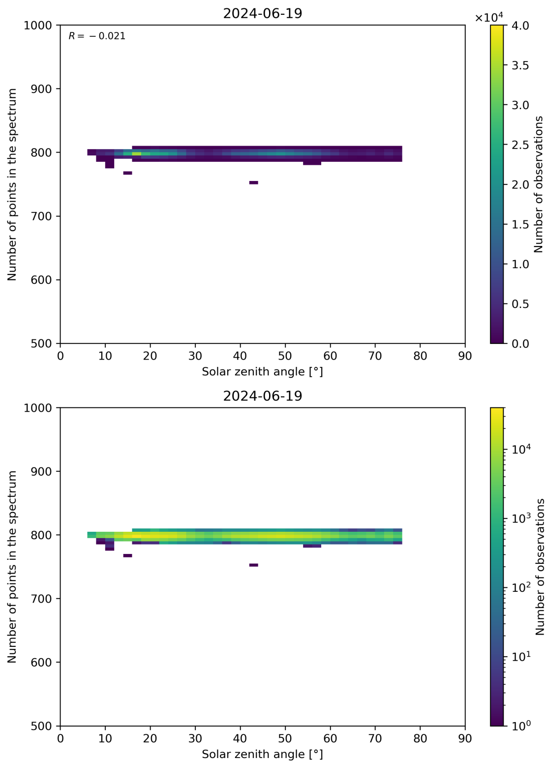
Figure 103: Scatter density plot of “Solar zenith angle” against “Number of points in the spectrum” for 2024-06-19 to 2024-06-20.
