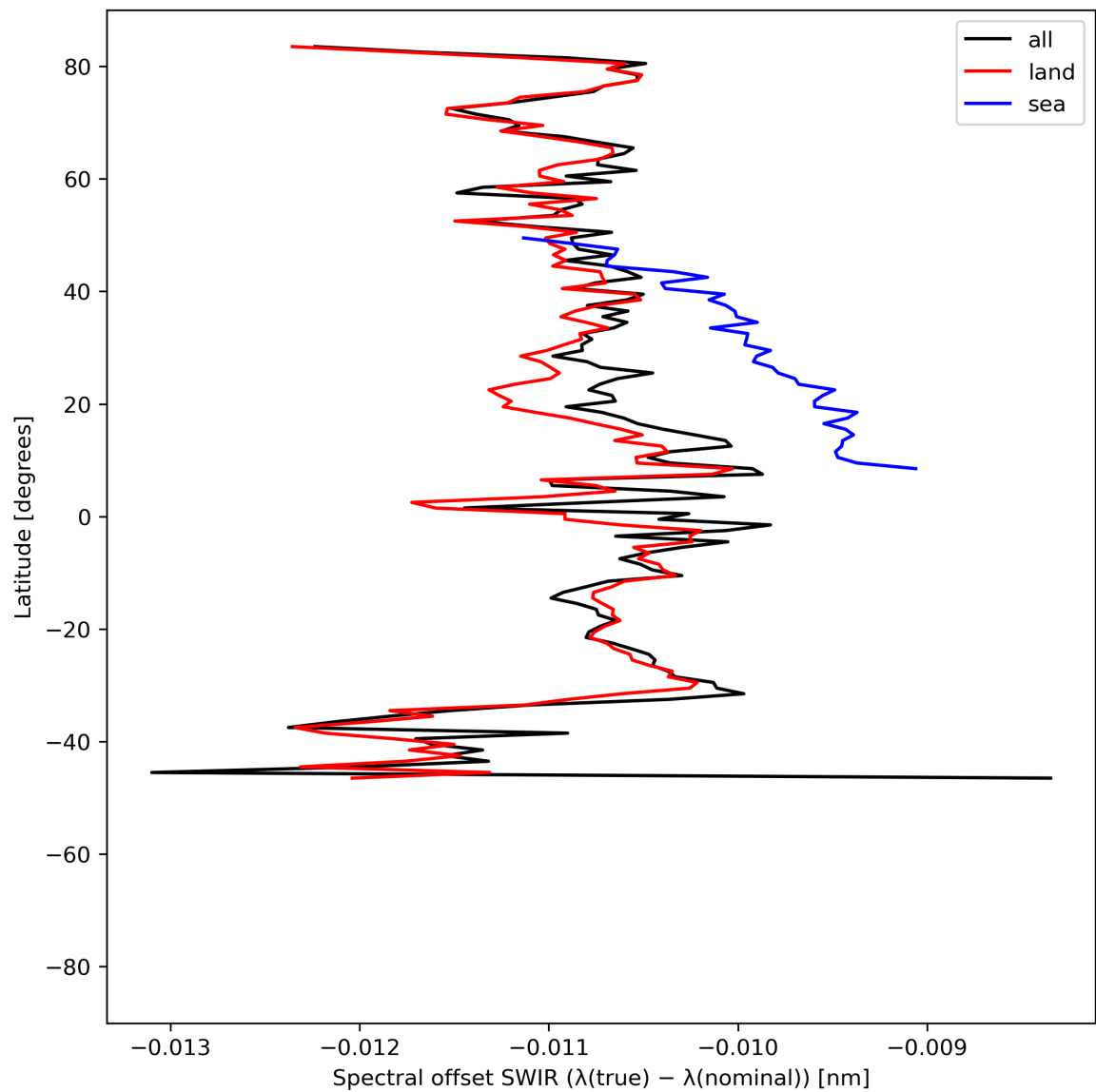
Figure 16: Zonal average of “Spectral offset SWIR ( \lambda(\text{true}) - \lambda(\text{nominal}) )” for 2024-06-19 to 2024-06-20.
