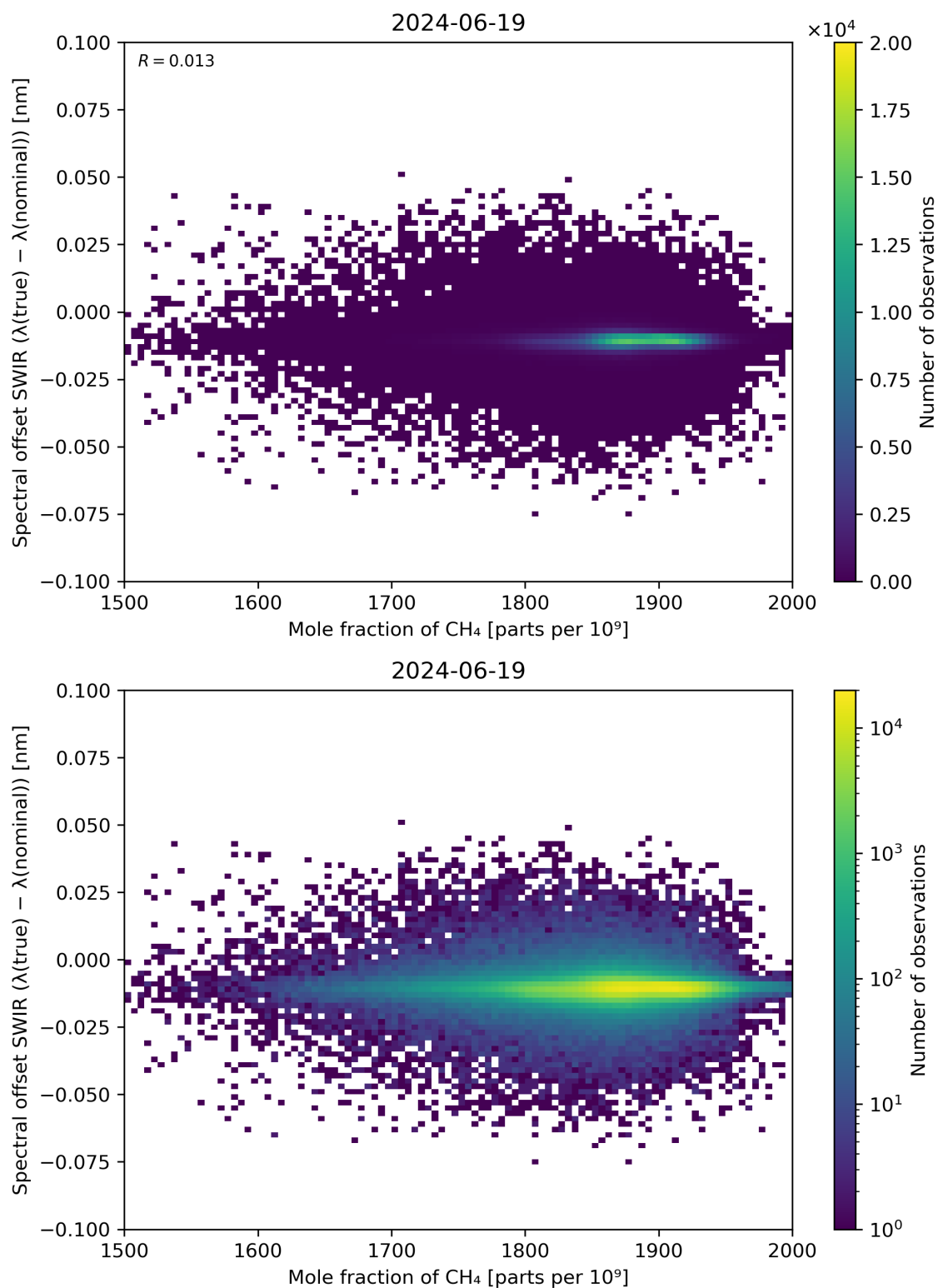
Figure 86: Scatter density plot of “Mole fraction of CH 4 ” against “Spectral offset SWIR ( \lambda(\text{true}) - \lambda(\text{nominal}) )” for 2024-06-19 to 2024-06-20.
