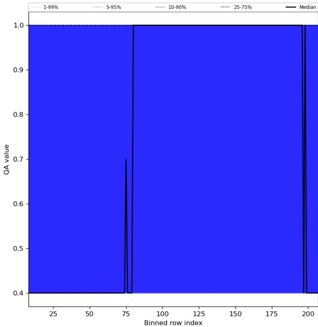
Figure 33: Along track statistics of “QA value” for 2024-06-19 to 2024-06-20
