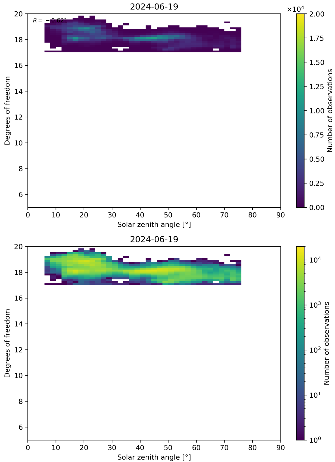
Figure 96: Scatter density plot of “Solar zenith angle” against “Degrees of freedom” for 2024-06-19 to 2024-06-20.
