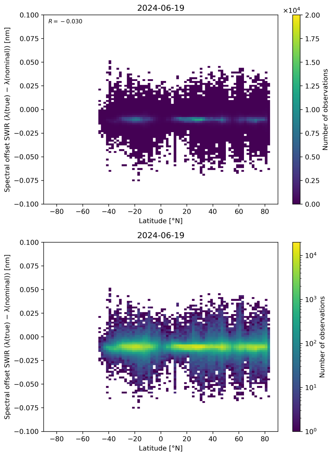
Figure 62: Scatter density plot of “Latitude” against “Spectral offset SWIR ( \lambda(\text{true}) - \lambda(\text{nominal}) )” for 2024-06-19 to 2024-06-20.
