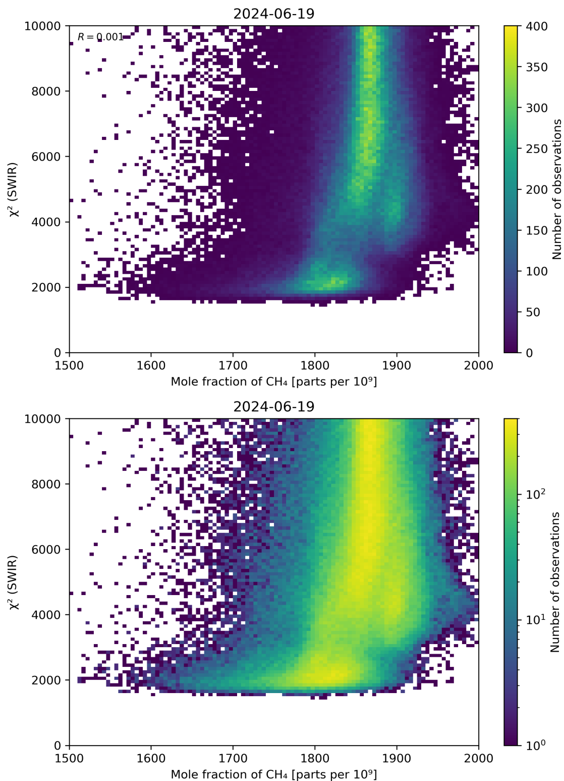
Figure 71: Scatter density plot of “Mole fraction of \text{CH}_4 ” against “ \chi^2 (SWIR)” for 2024-06-19 to 2024-06-20.
