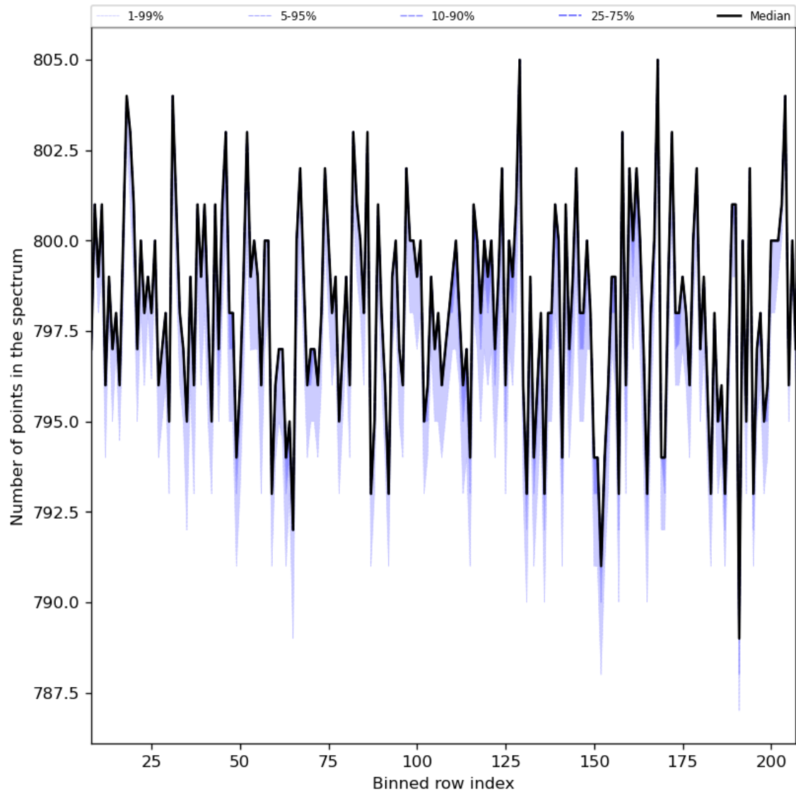
Figure 37: Along track statistics of “Number of points in the spectrum” for 2024-06-19 to 2024-06-20
