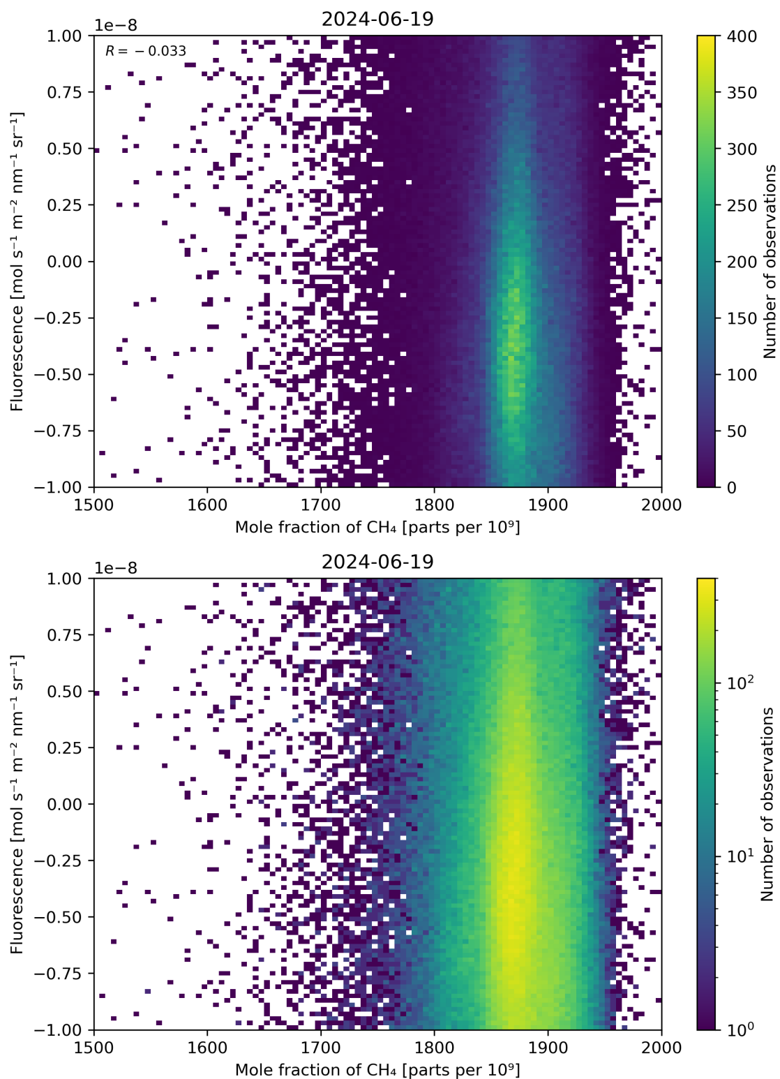
Figure 73: Scatter density plot of “Mole fraction of \text{CH}_4 ” against “Fluorescence” for 2024-06-19 to 2024-06-20.
