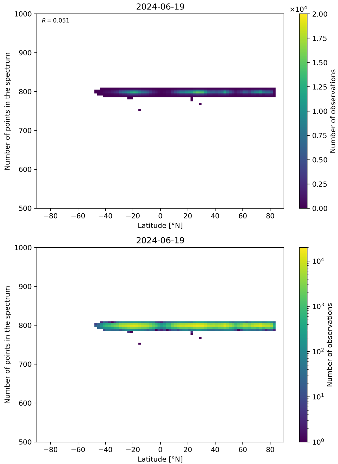
Figure 61: Scatter density plot of “Latitude” against “Number of points in the spectrum” for 2024-06-19 to 2024-06-20.
