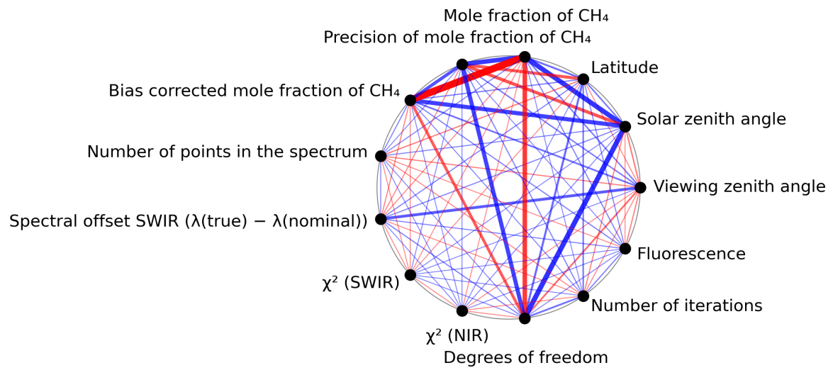
Figure 1: Map of correlation graph for 2024-06-19 to 2024-06-20.
