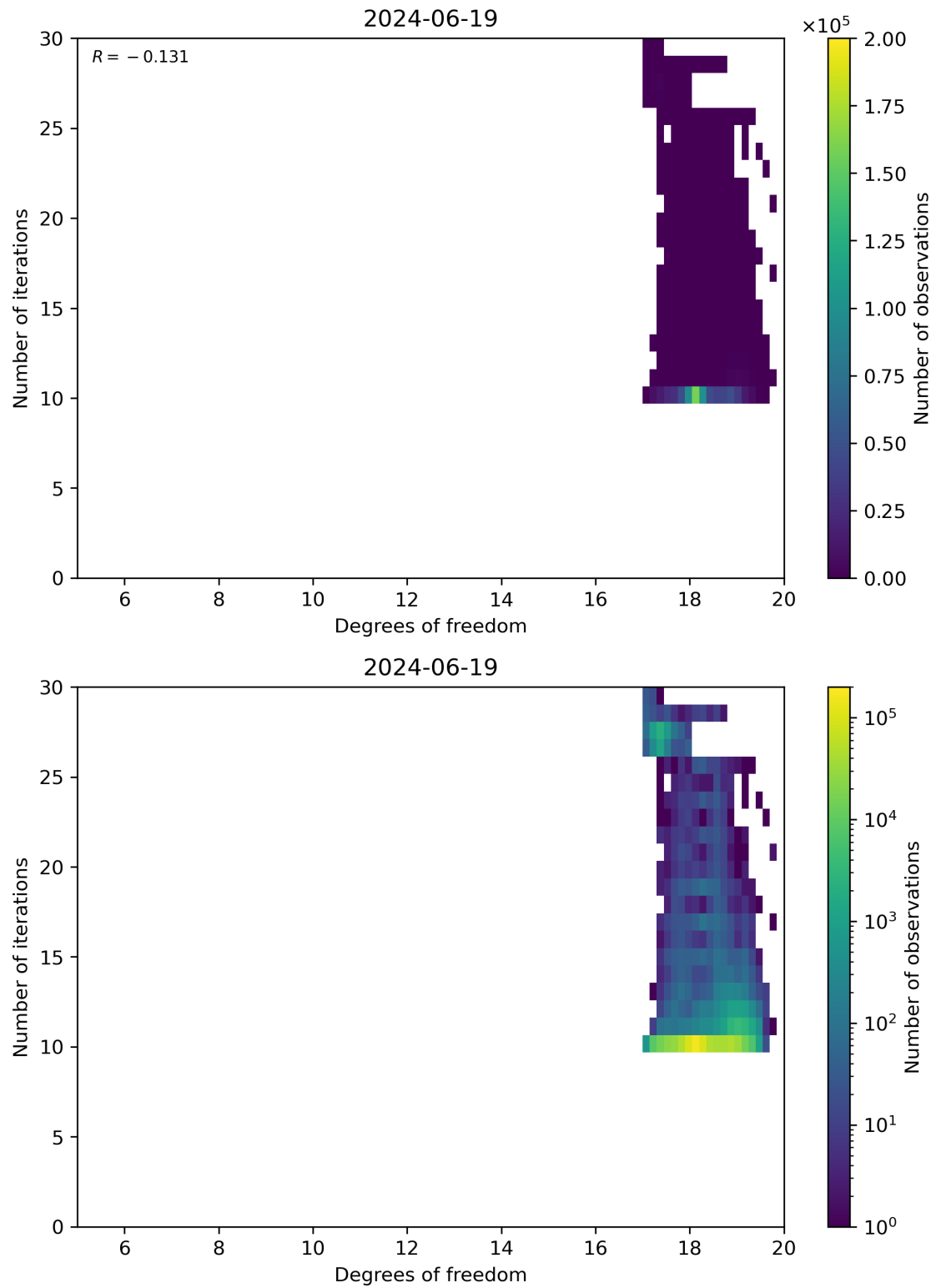
Figure 52: Scatter density plot of “Degrees of freedom” against “Number of iterations” for 2024-06-19 to 2024-06-20.
