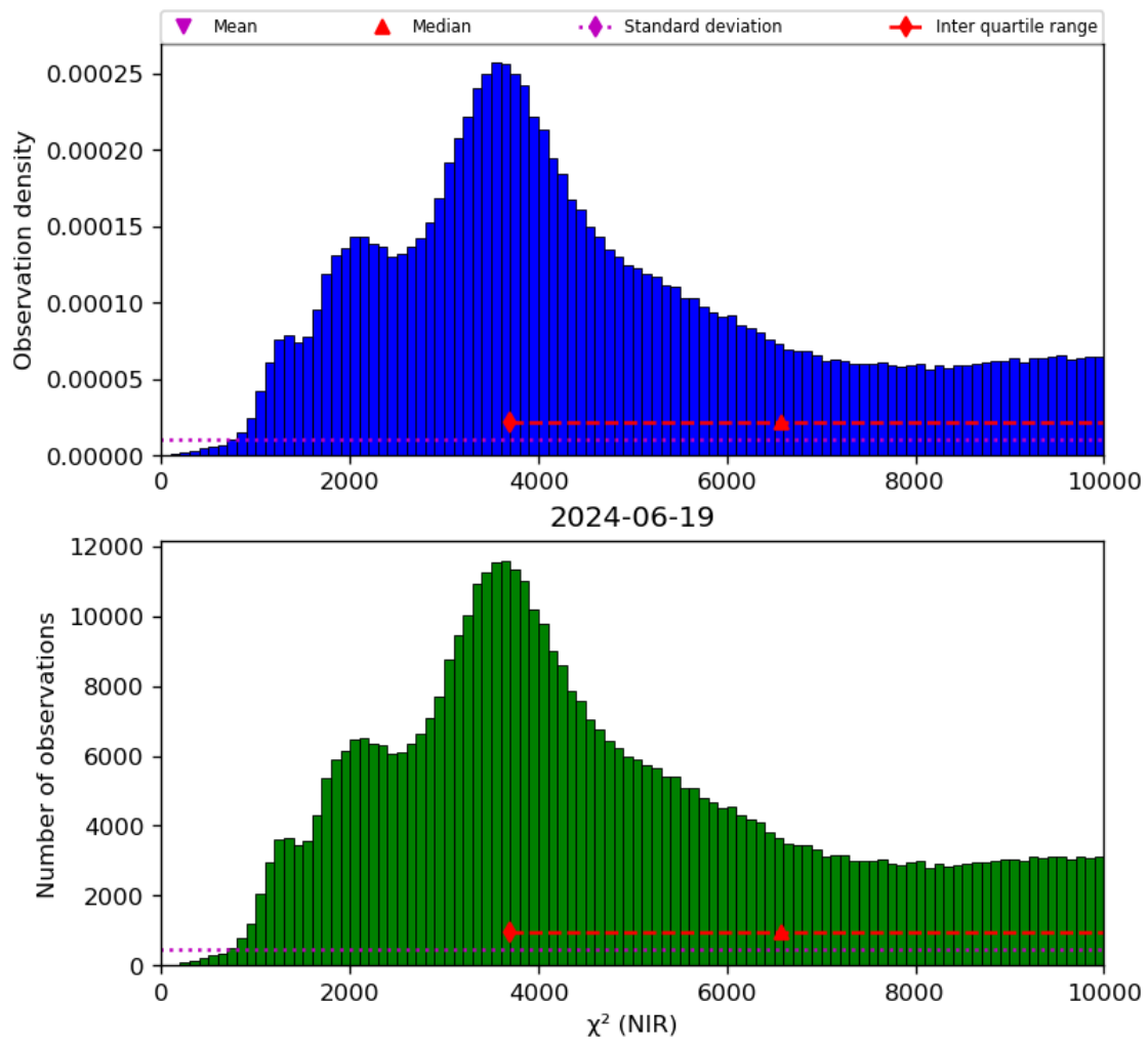
Figure 29: Histogram of “ \chi^2 (NIR)” for 2024-06-19 to 2024-06-20
