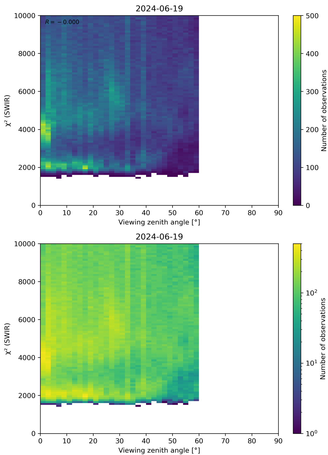
Figure 106: Scatter density plot of “Viewing zenith angle” against “ \chi^2 (SWIR)” for 2024-06-19 to 2024-06-20.
