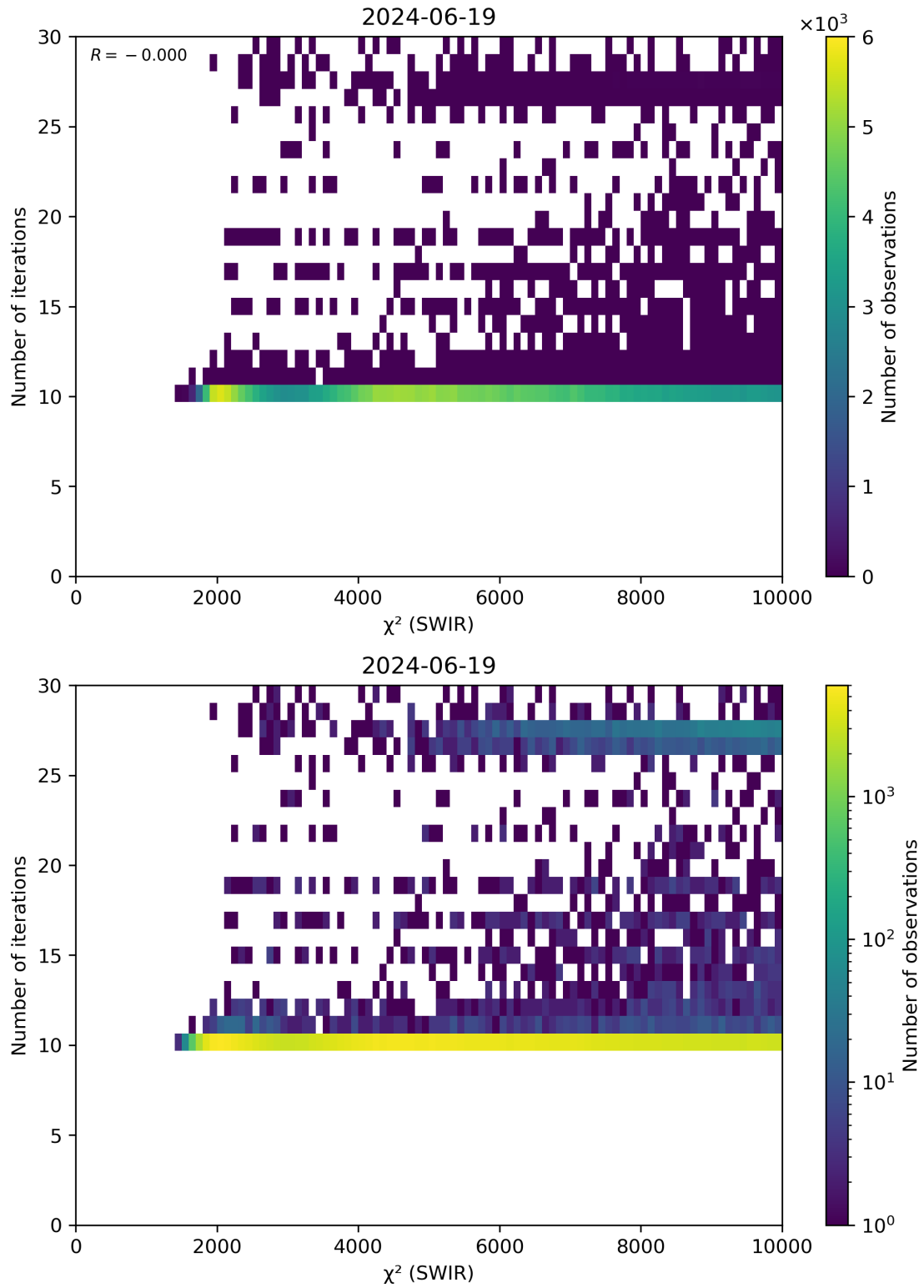
Figure 50: Scatter density plot of “ \chi^2 (SWIR)” against “Number of iterations” for 2024-06-19 to 2024-06-20.
