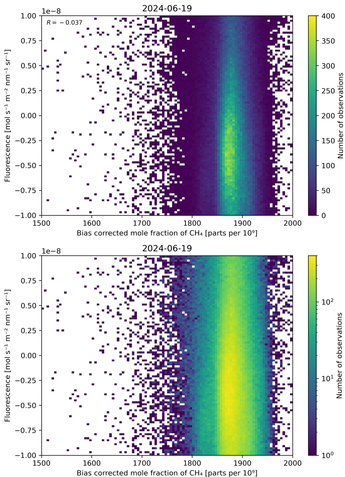
Figure 66: Scatter density plot of “Bias corrected mole fraction of \text{CH}_4 ” against “Fluorescence” for 2024-06-19 to 2024-06-20.
