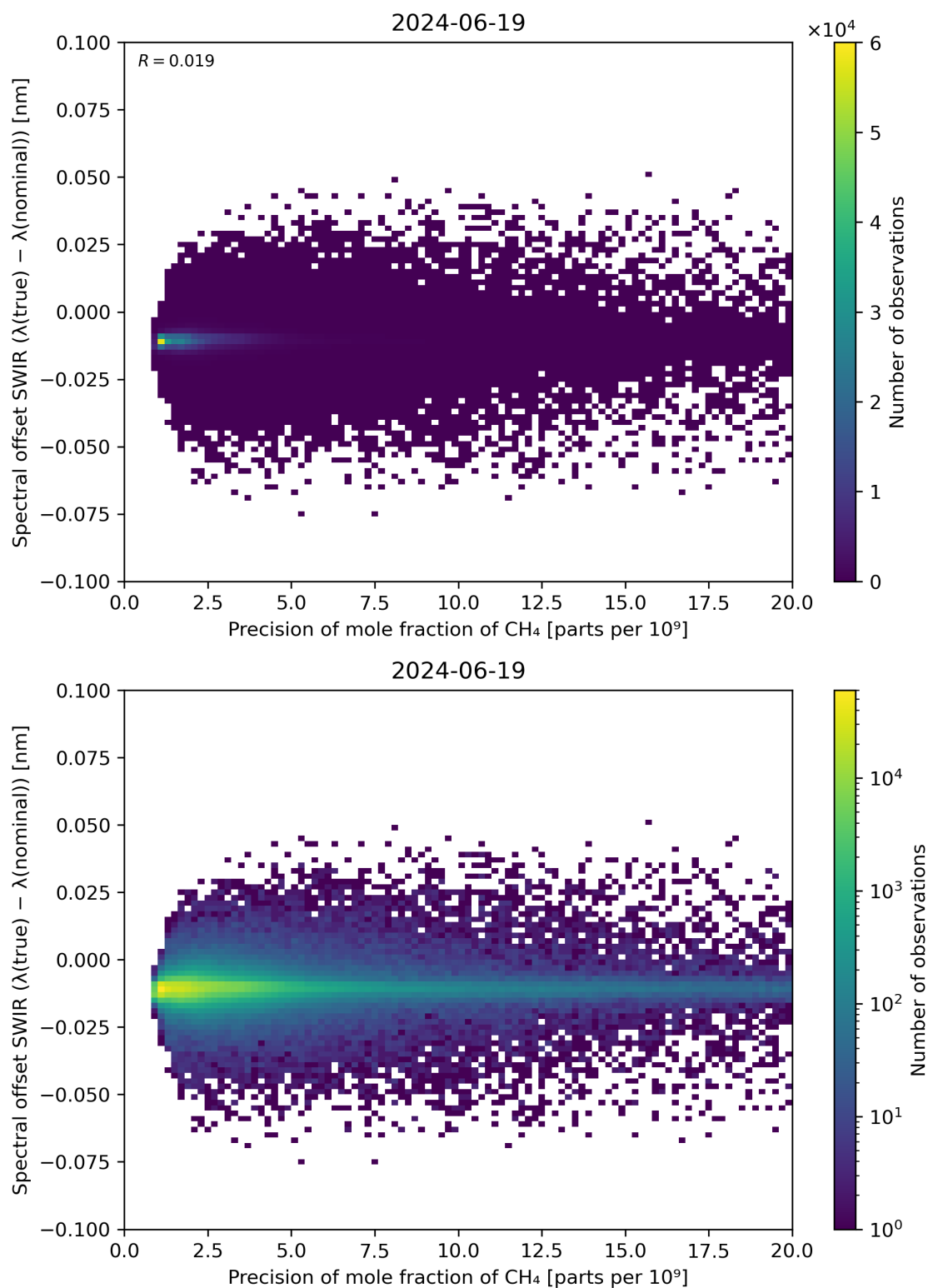
Figure 85: Scatter density plot of “Precision of mole fraction of CH 4 ” against “Spectral offset SWIR ( \lambda(\text{true}) - \lambda(\text{nominal}) )” for 2024-06-19 to 2024-06-20.
