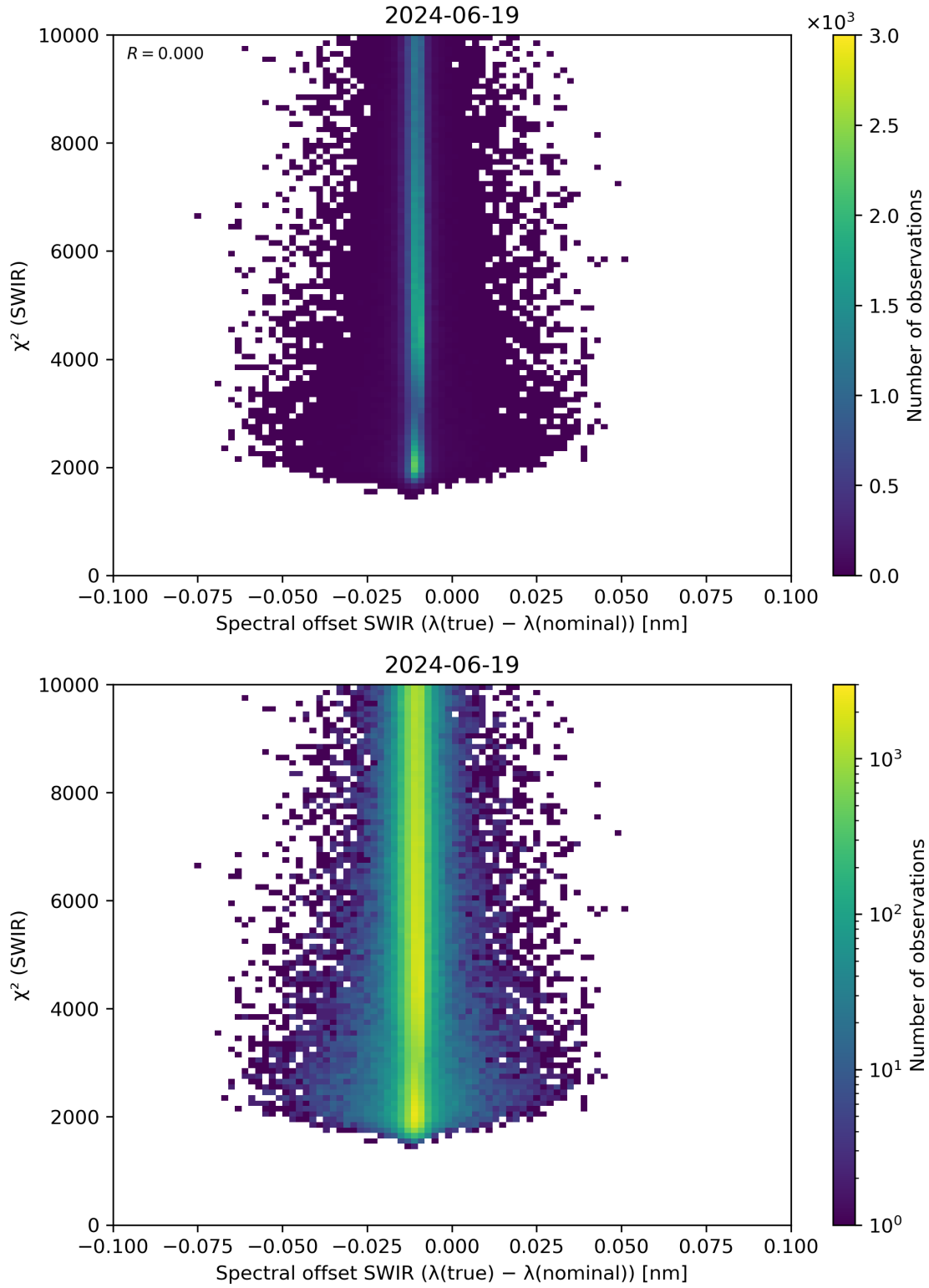
Figure 118: Scatter density plot of “Spectral offset SWIR ( \lambda(\text{true}) - \lambda(\text{nominal}) )” against “ \chi^2 (SWIR)” for 2024-06-19 to 2024-06-20.
