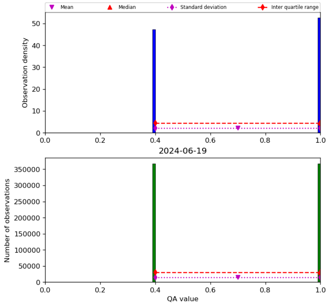
Figure 22: Histogram of “QA value” for 2024-06-19 to 2024-06-20
