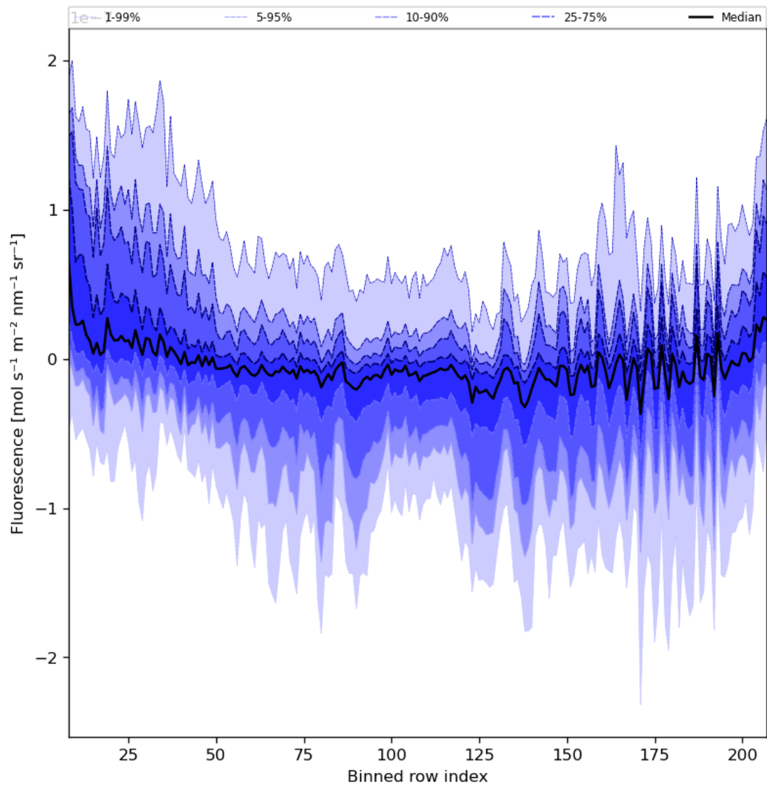
Figure 43: Along track statistics of “Fluorescence” for 2024-06-19 to 2024-06-20
