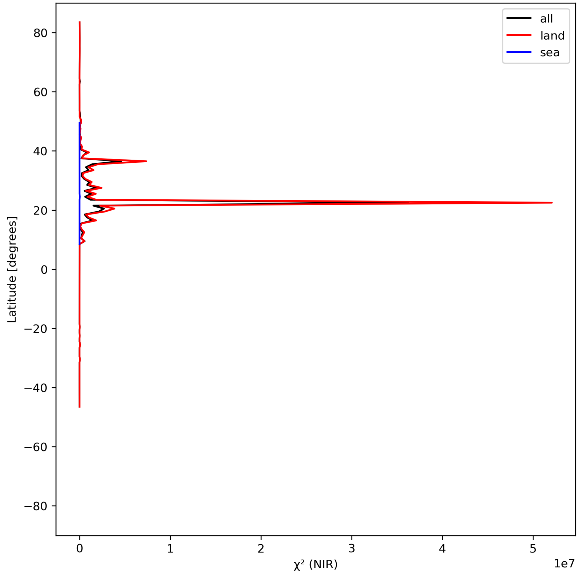
Figure 18: Zonal average of “ \chi^2 (NIR)” for 2024-06-19 to 2024-06-20.
