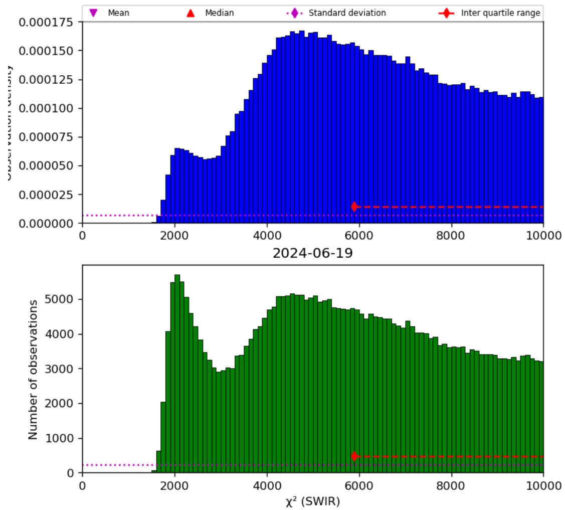
Figure 28: Histogram of “ \chi^2 (SWIR)” for 2024-06-19 to 2024-06-20
