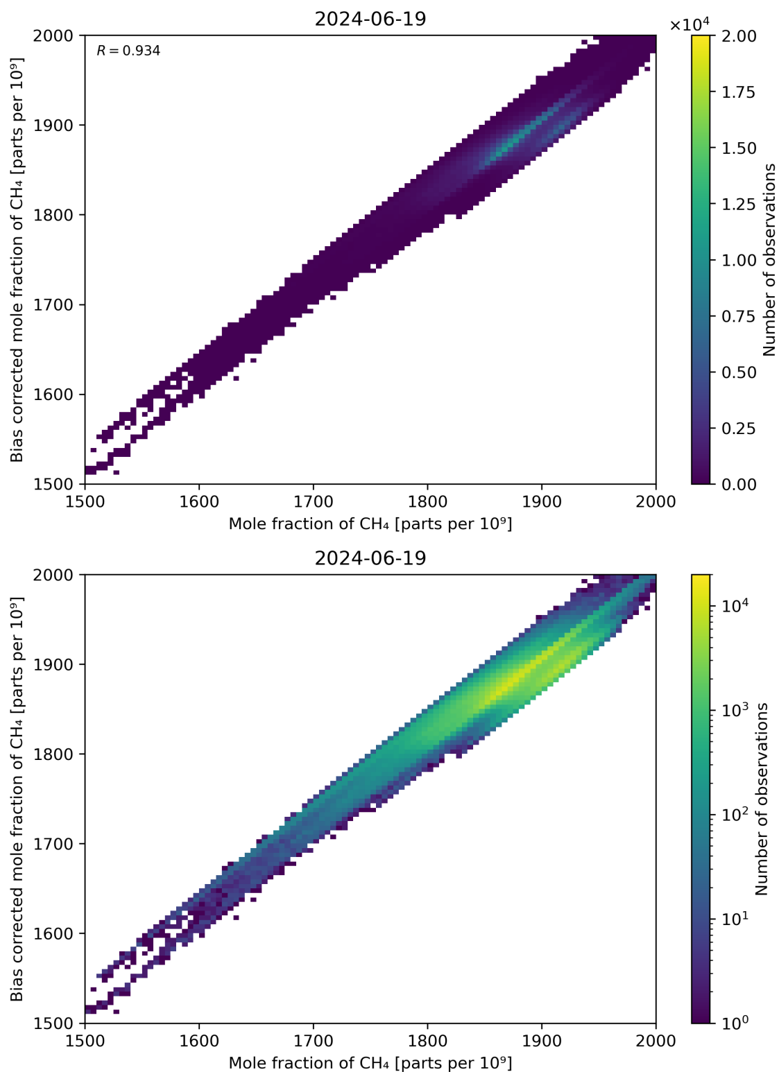
Figure 74: Scatter density plot of “Mole fraction of CH 4 ” against “Bias corrected mole fraction of CH 4 ” for 2024-06-19 to 2024-06-20.
