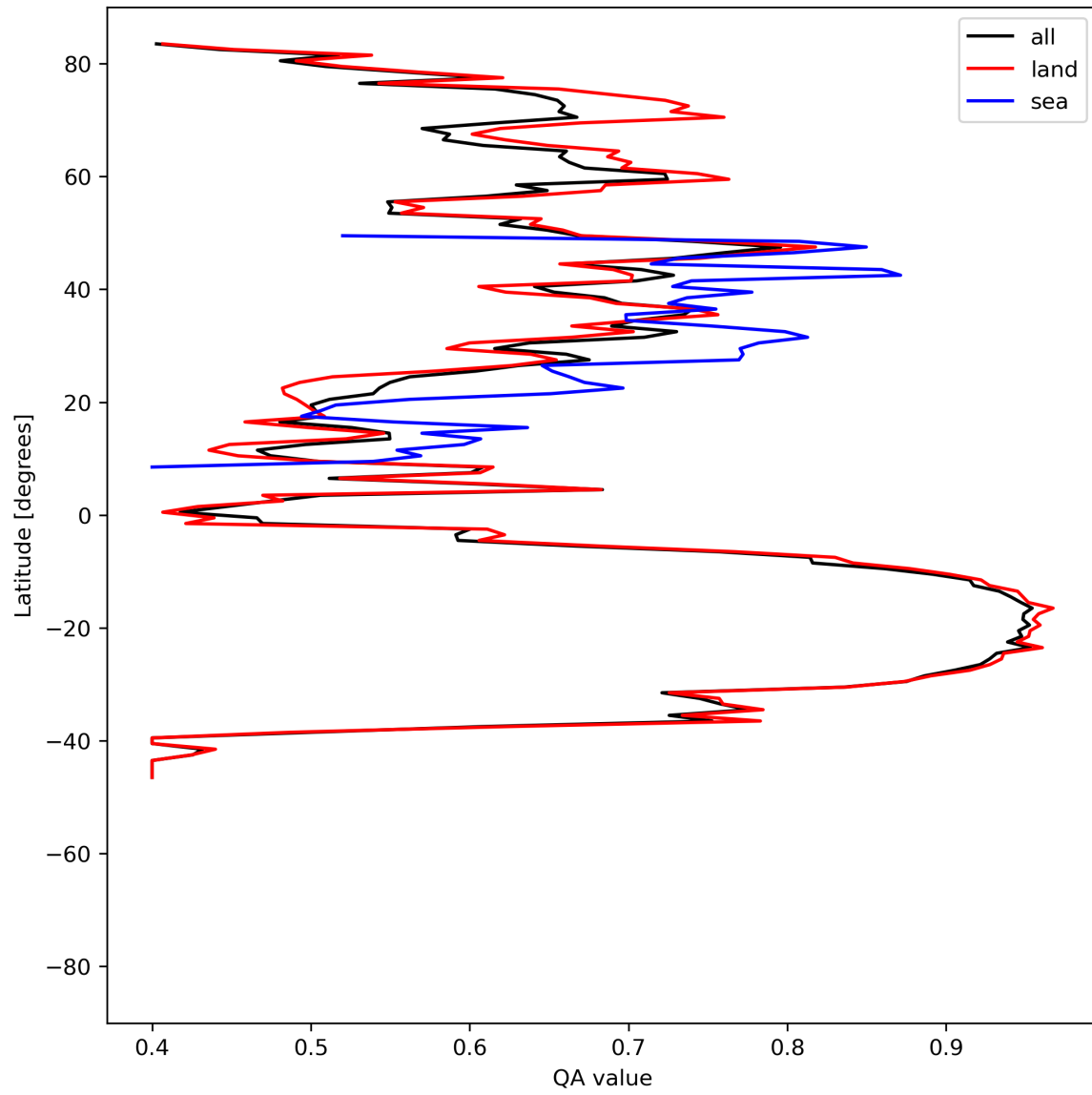
Figure 11: Zonal average of “QA value” for 2024-06-19 to 2024-06-20.
