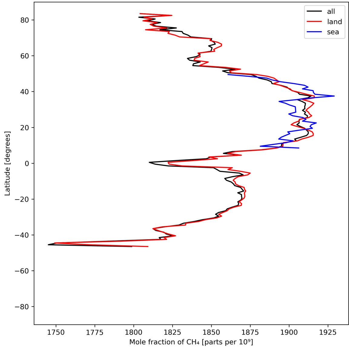
Figure 12: Zonal average of “Mole fraction of \text{CH}_4 ” for 2024-06-19 to 2024-06-20.
