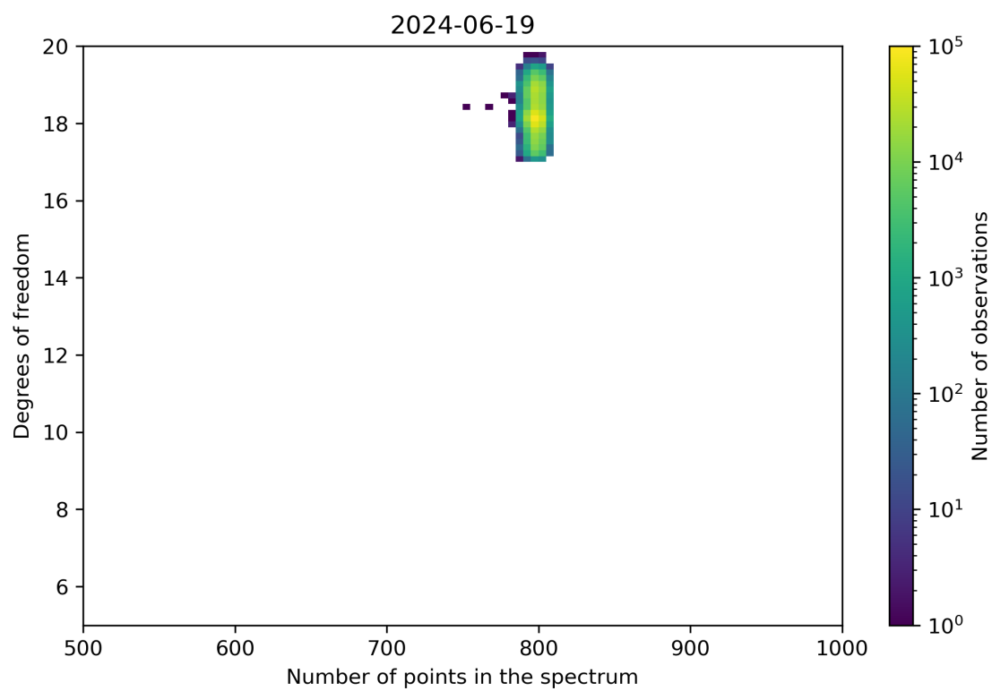
Figure 90: Scatter density plot of “Number of points in the spectrum” against “Degrees of freedom” for 2024-06-19 to 2024-06-20.
