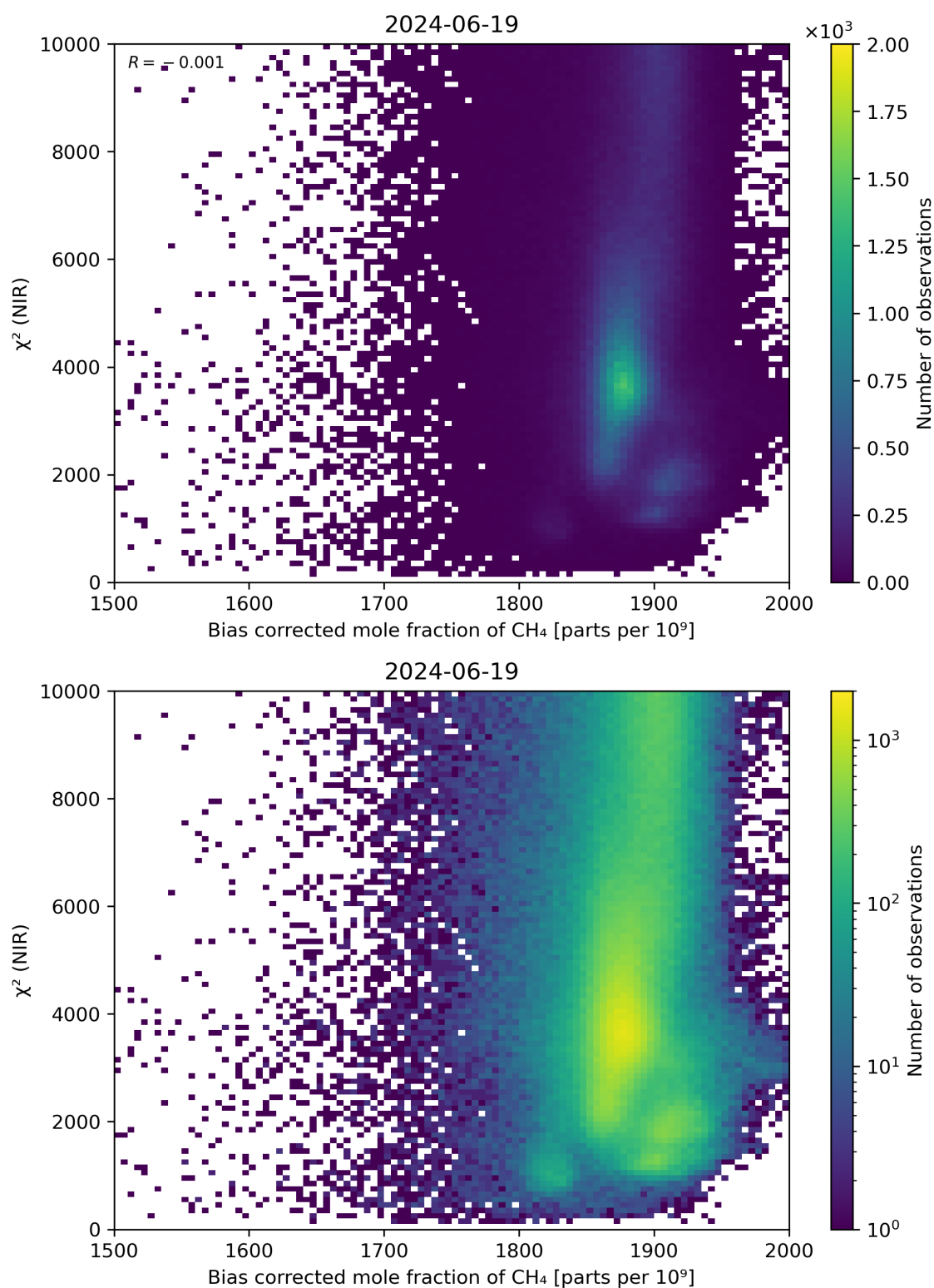
Figure 63: Scatter density plot of “Bias corrected mole fraction of \text{CH}_4 ” against “ \chi^2 (NIR)” for 2024-06-19 to 2024-06-20.
