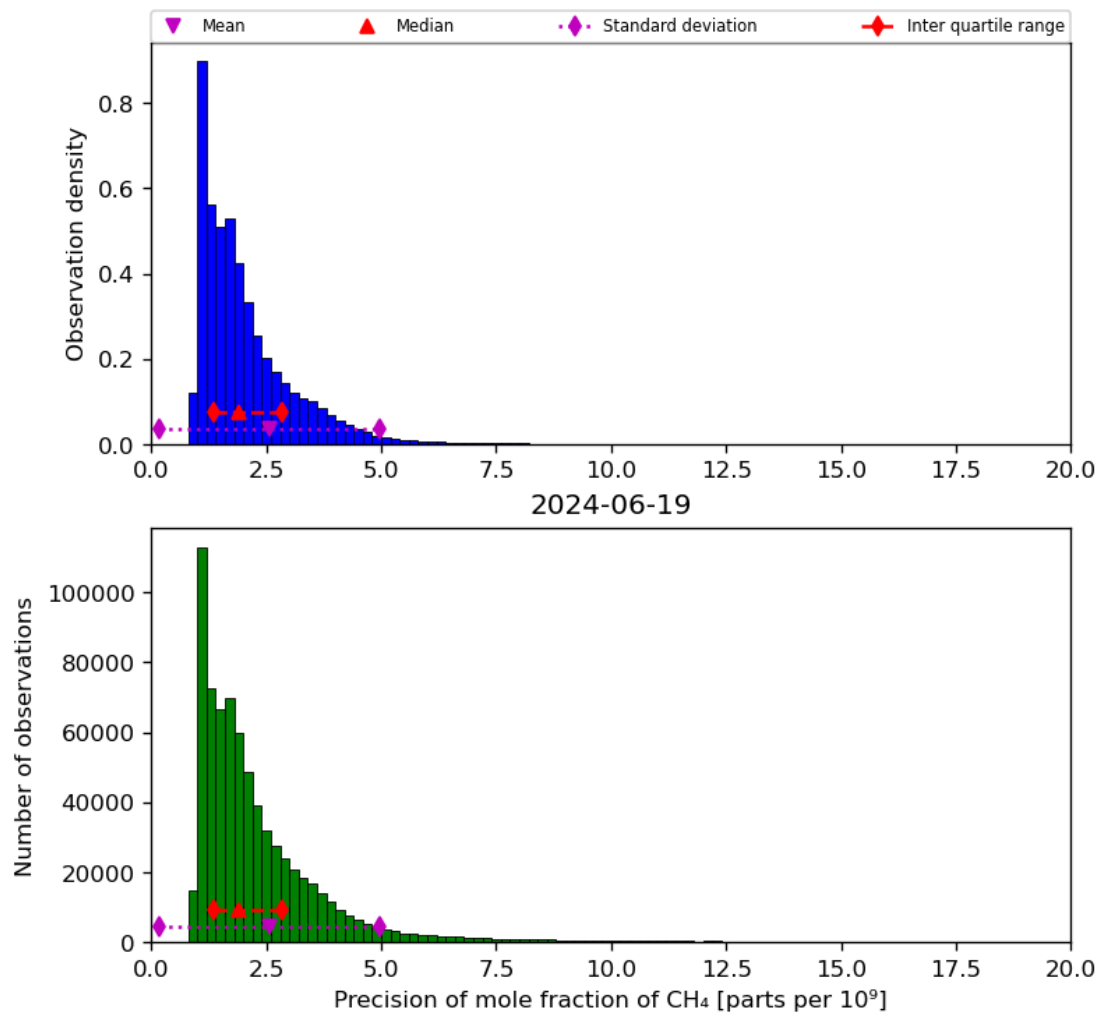
Figure 24: Histogram of “Precision of mole fraction of CH 4 ” for 2024-06-19 to 2024-06-20
