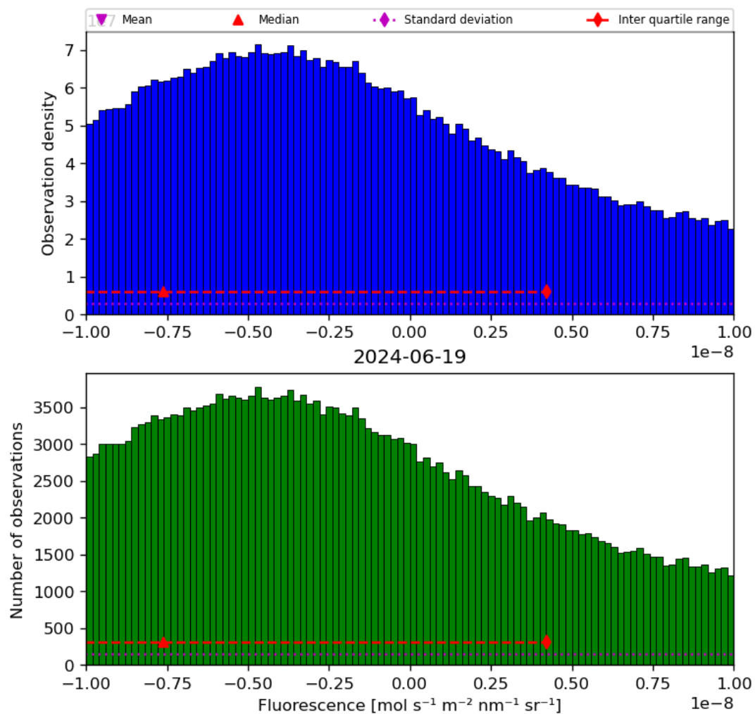
Figure 32: Histogram of “Fluorescence” for 2024-06-19 to 2024-06-20
