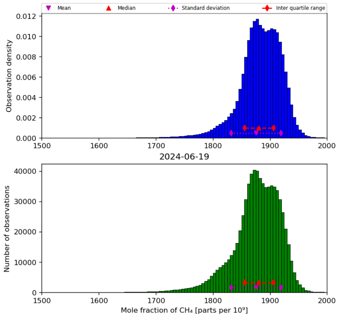
Figure 23: Histogram of “Mole fraction of CH 4 ” for 2024-06-19 to 2024-06-20
