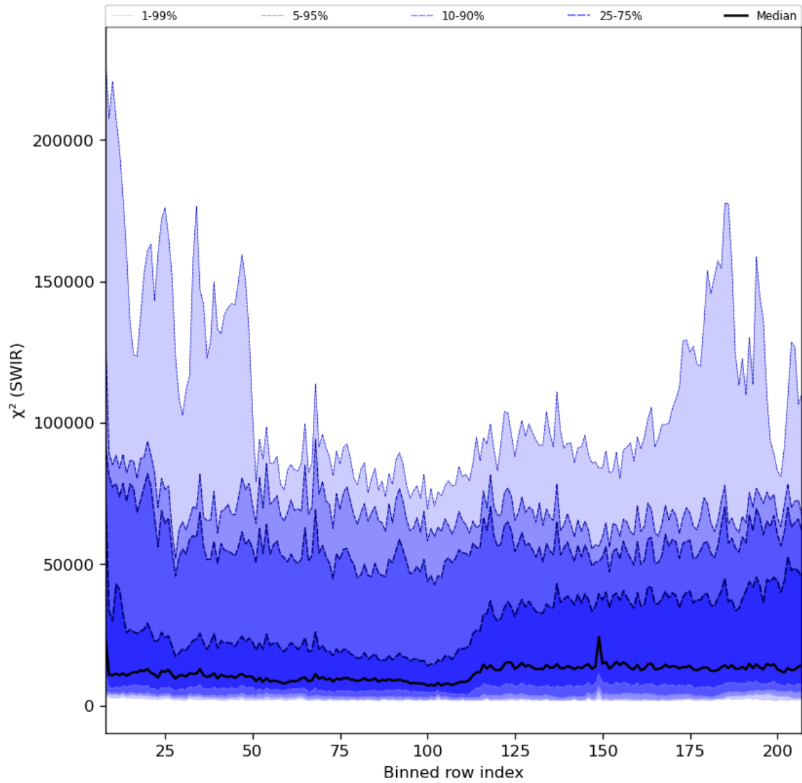
Figure 39: Along track statistics of “ \chi^2 (SWIR)” for 2024-06-19 to 2024-06-20
