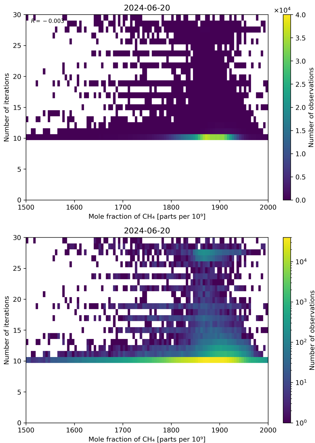
Figure 76: Scatter density plot of “Mole fraction of CH 4 ” against “Number of iterations” for 2024-06-19 to 2024-06-21.
