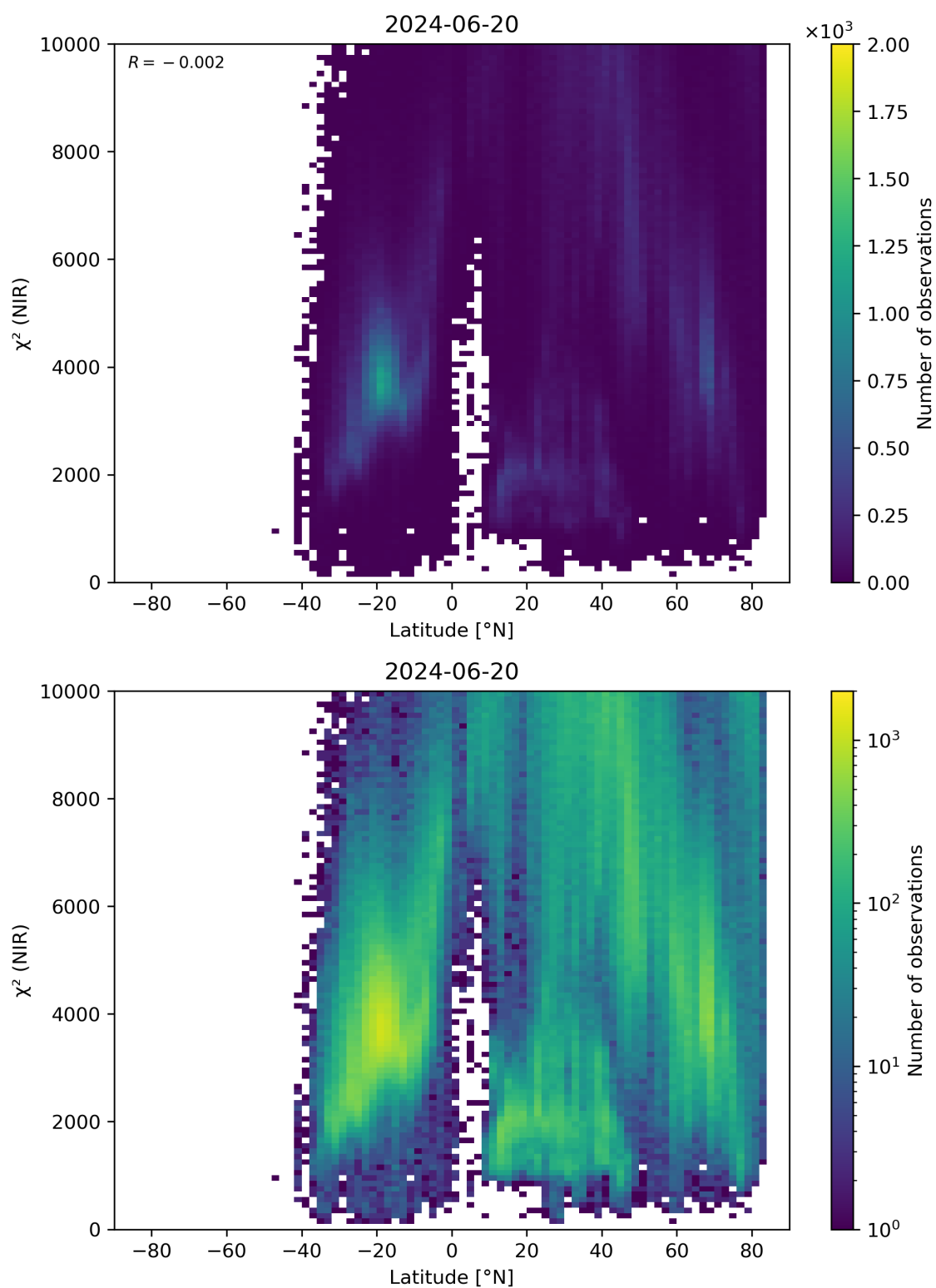
Figure 53: Scatter density plot of “Latitude” against “ \chi^2 (NIR)” for 2024-06-19 to 2024-06-21.
