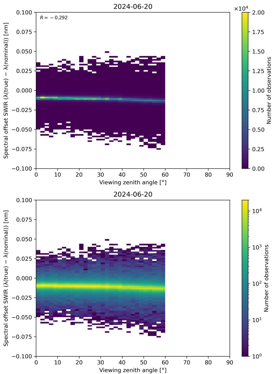
Figure 116: Scatter density plot of “Viewing zenith angle” against “Spectral offset SWIR ( \lambda(\text{true}) - \lambda(\text{nominal}) )” for 2024-06-19 to 2024-06-21.
