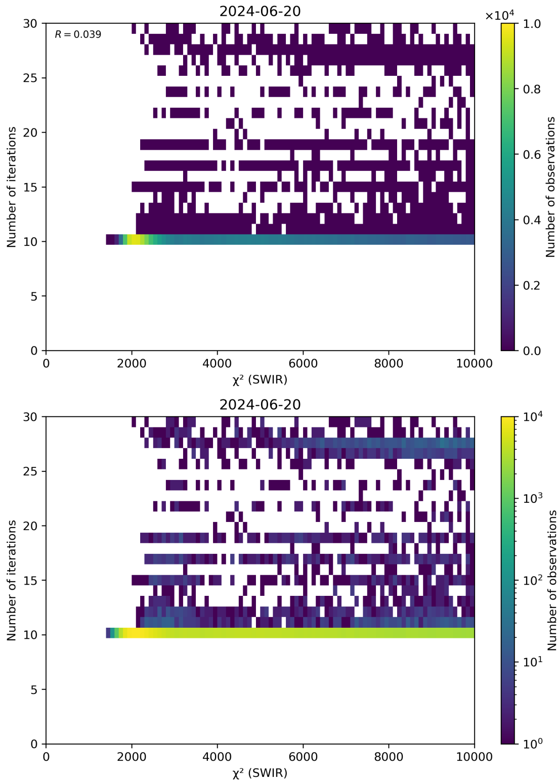
Figure 50: Scatter density plot of “ \chi^2 (SWIR)” against “Number of iterations” for 2024-06-19 to 2024-06-21.
