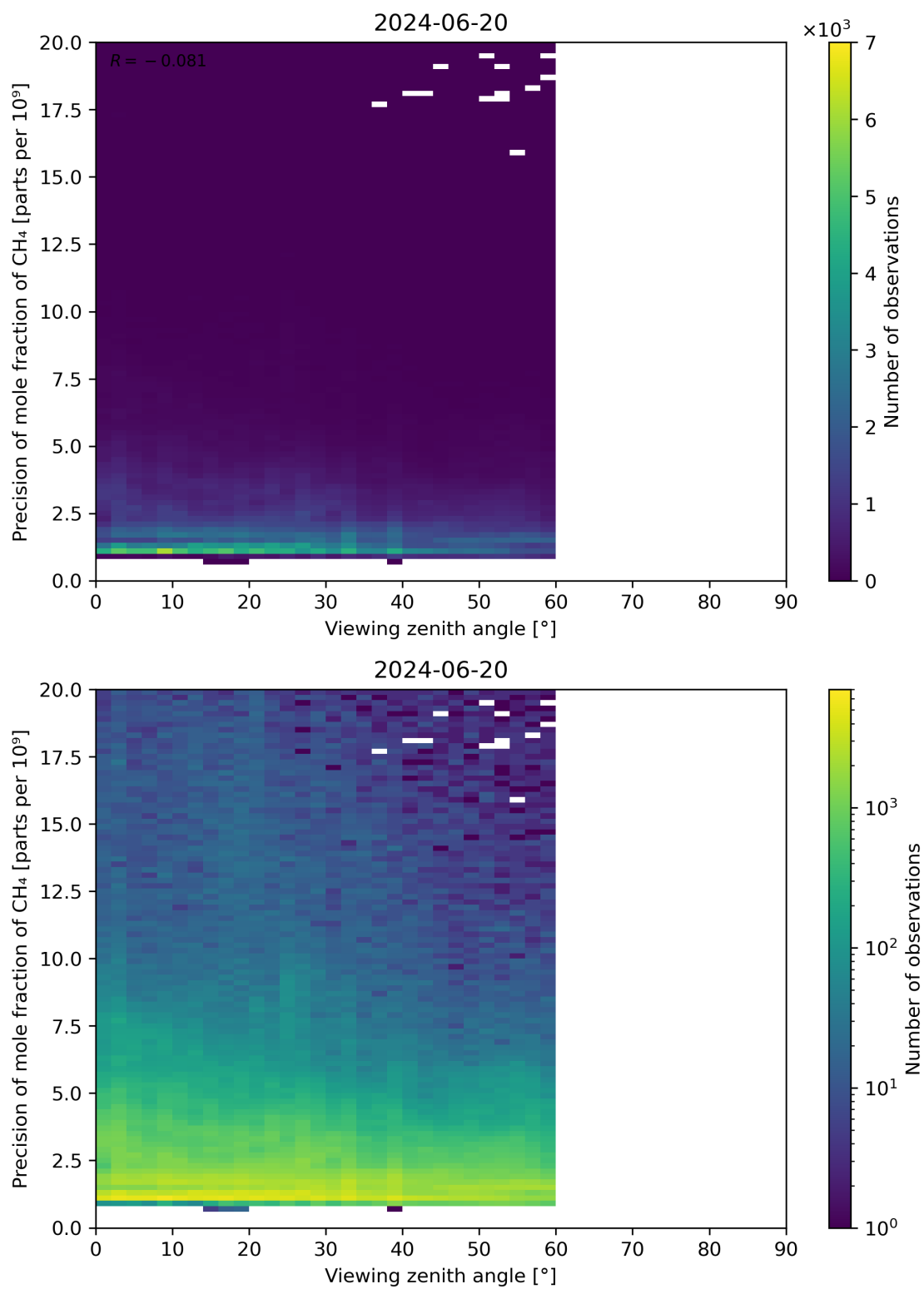
Figure 112: Scatter density plot of “Viewing zenith angle” against “Precision of mole fraction of \text{CH}_4 ” for 2024-06-19 to 2024-06-21.
