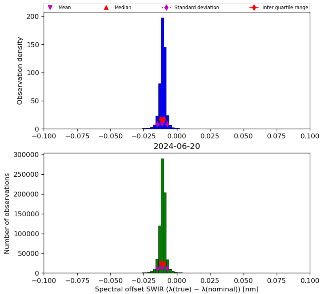
Figure 27: Histogram of “Spectral offset SWIR ( \lambda(\text{true}) - \lambda(\text{nominal}) )” for 2024-06-19 to 2024-06-21
