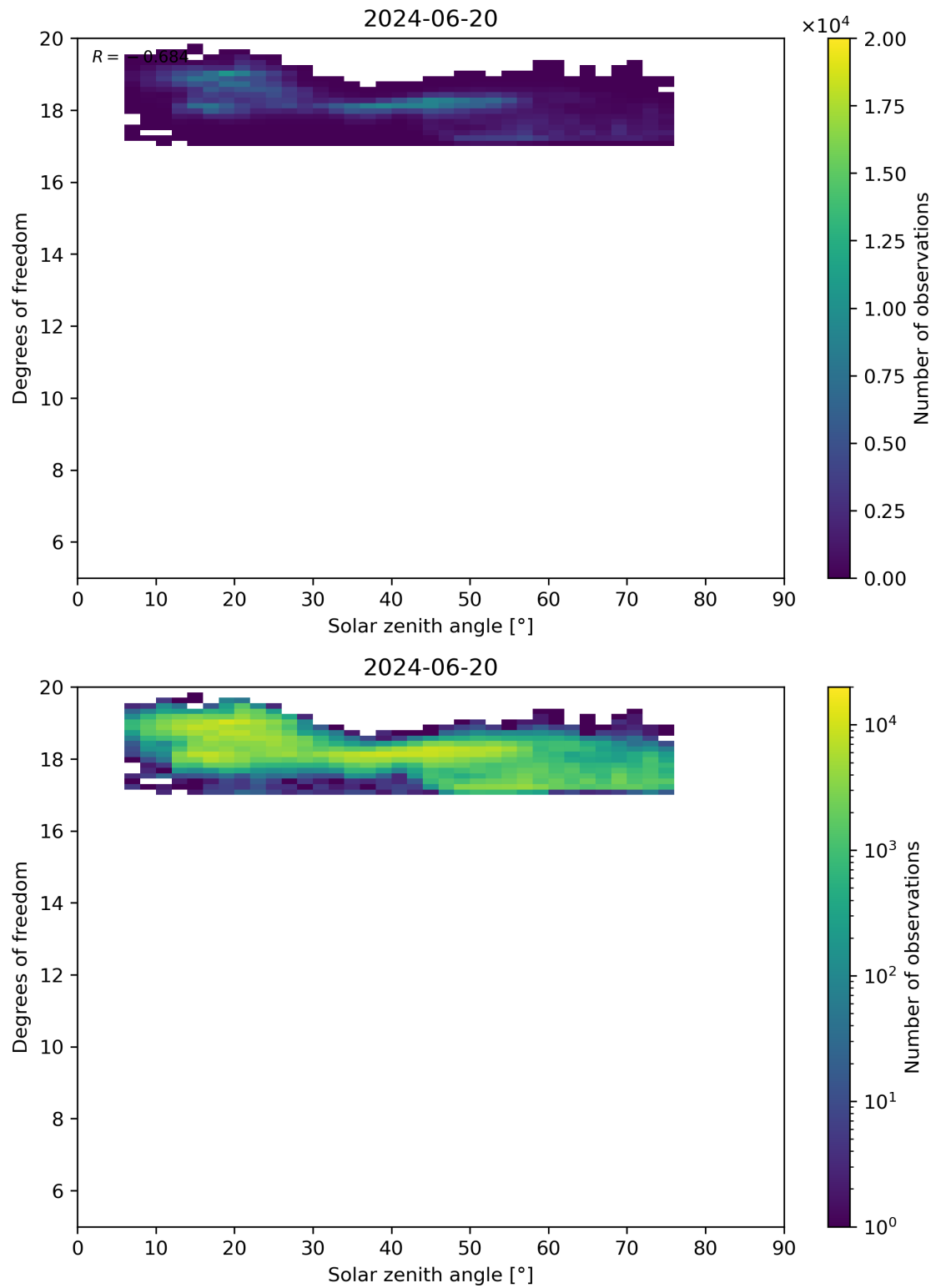
Figure 96: Scatter density plot of “Solar zenith angle” against “Degrees of freedom” for 2024-06-19 to 2024-06-21.
