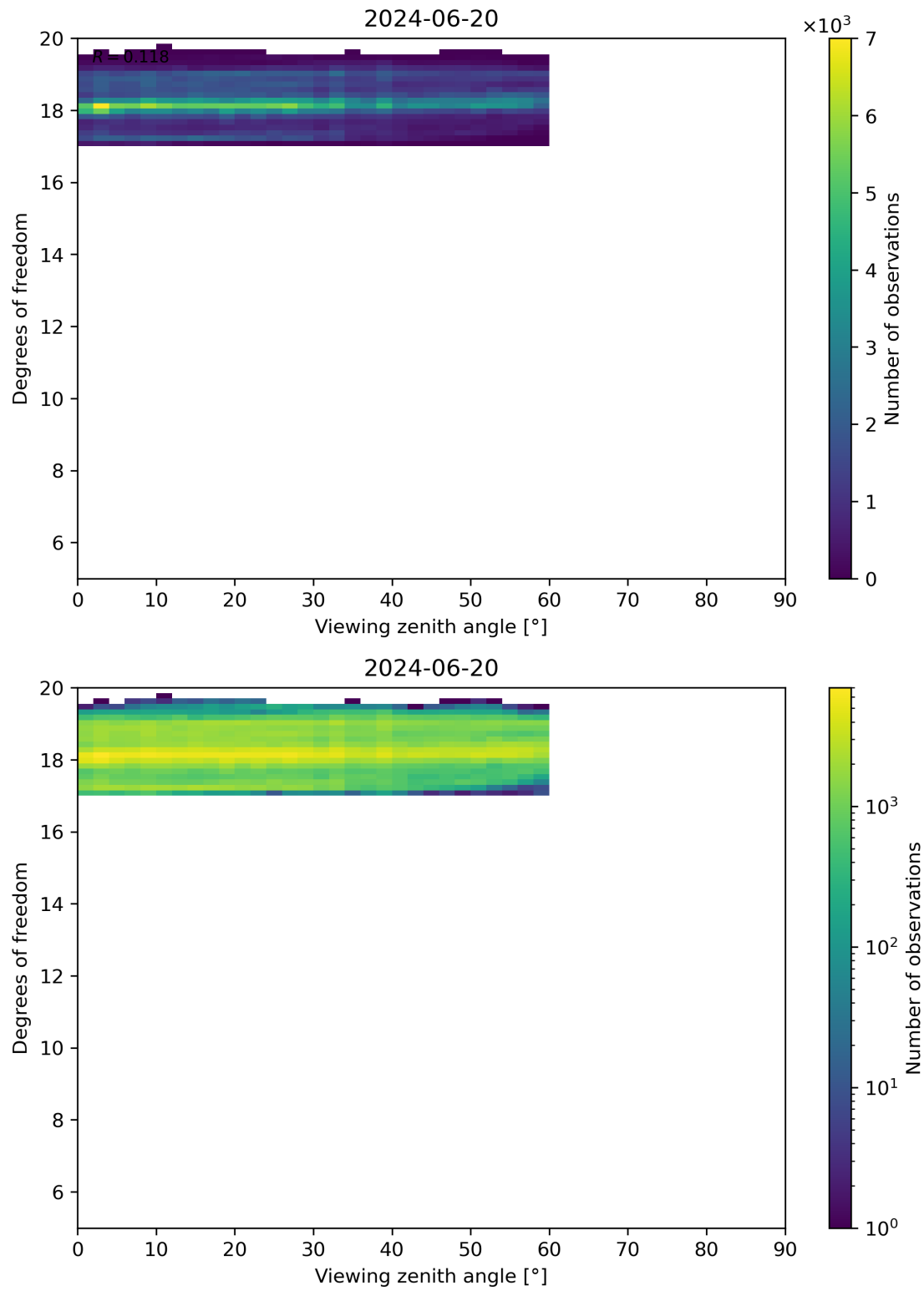
Figure 107: Scatter density plot of “Viewing zenith angle” against “Degrees of freedom” for 2024-06-19 to 2024-06-21.
