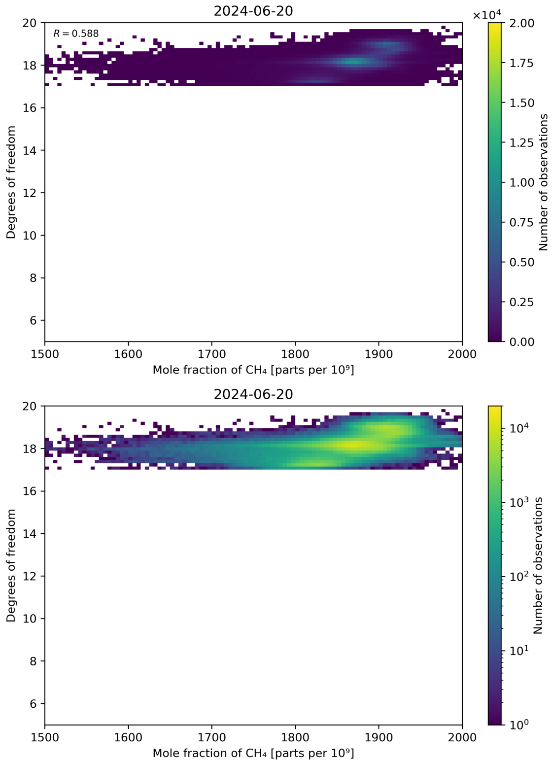
Figure 72: Scatter density plot of “Mole fraction of CH 4 ” against “Degrees of freedom” for 2024-06-19 to 2024-06-21.
