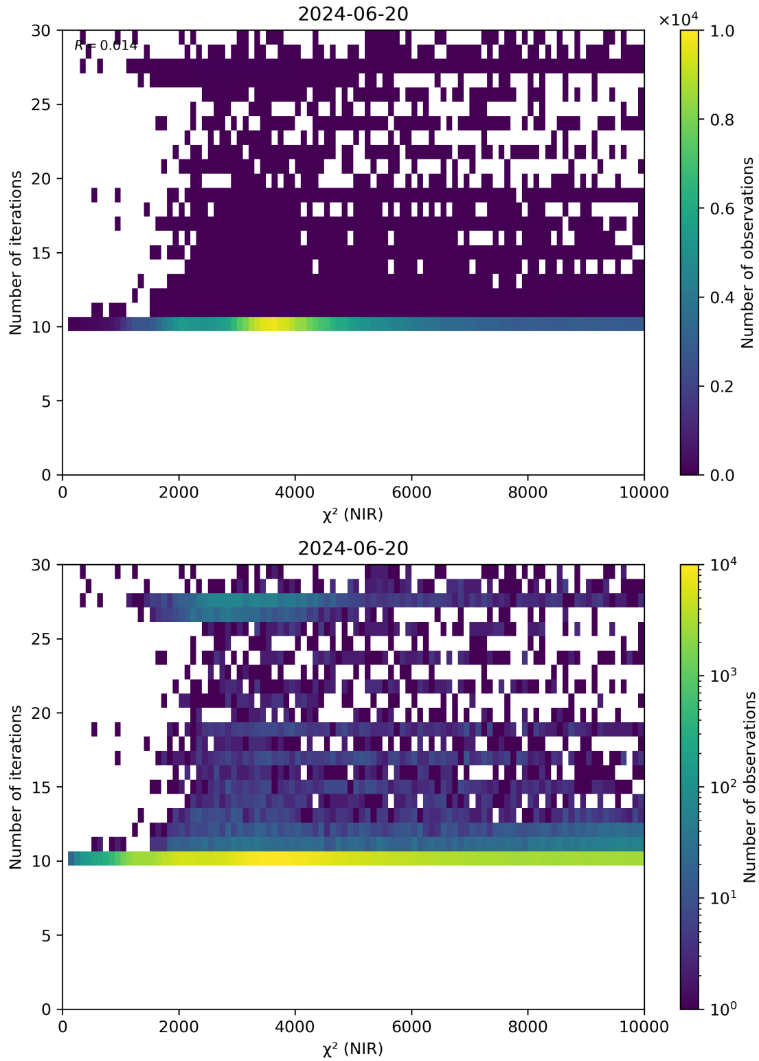
Figure 46: Scatter density plot of “ \chi^2 (NIR)” against “Number of iterations” for 2024-06-19 to 2024-06-21.
