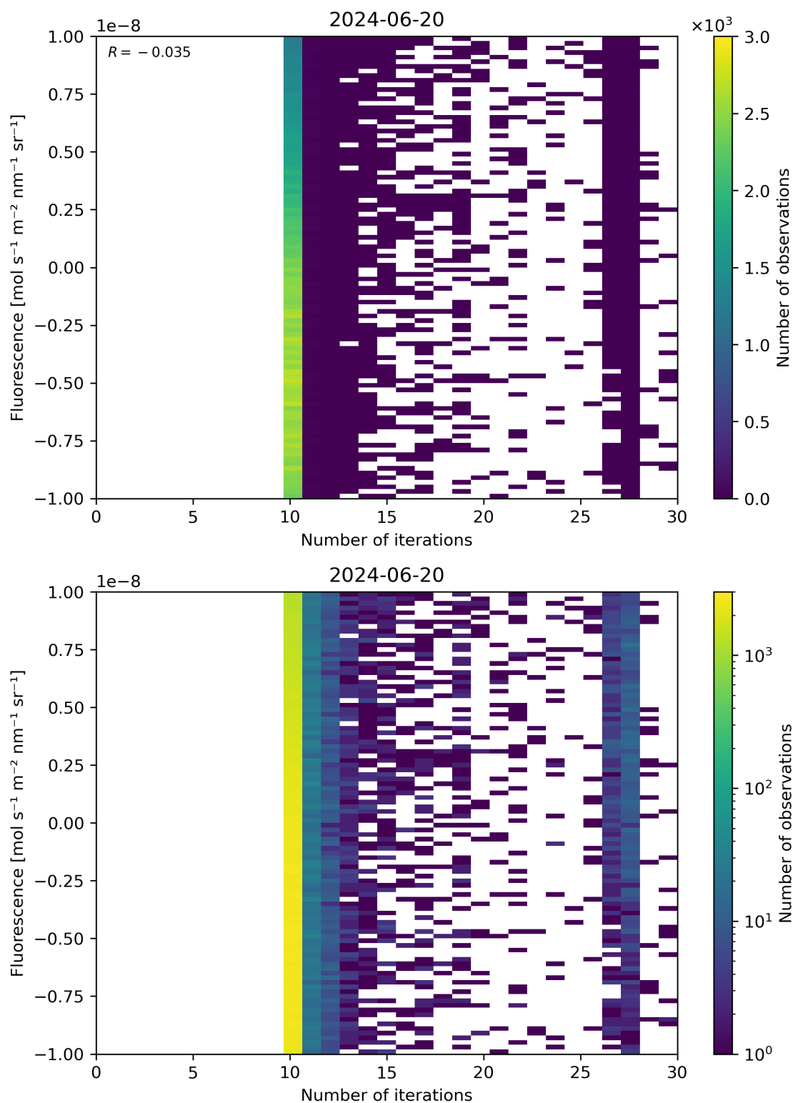
Figure 87: Scatter density plot of “Number of iterations” against “Fluorescence” for 2024-06-19 to 2024-06-21.
