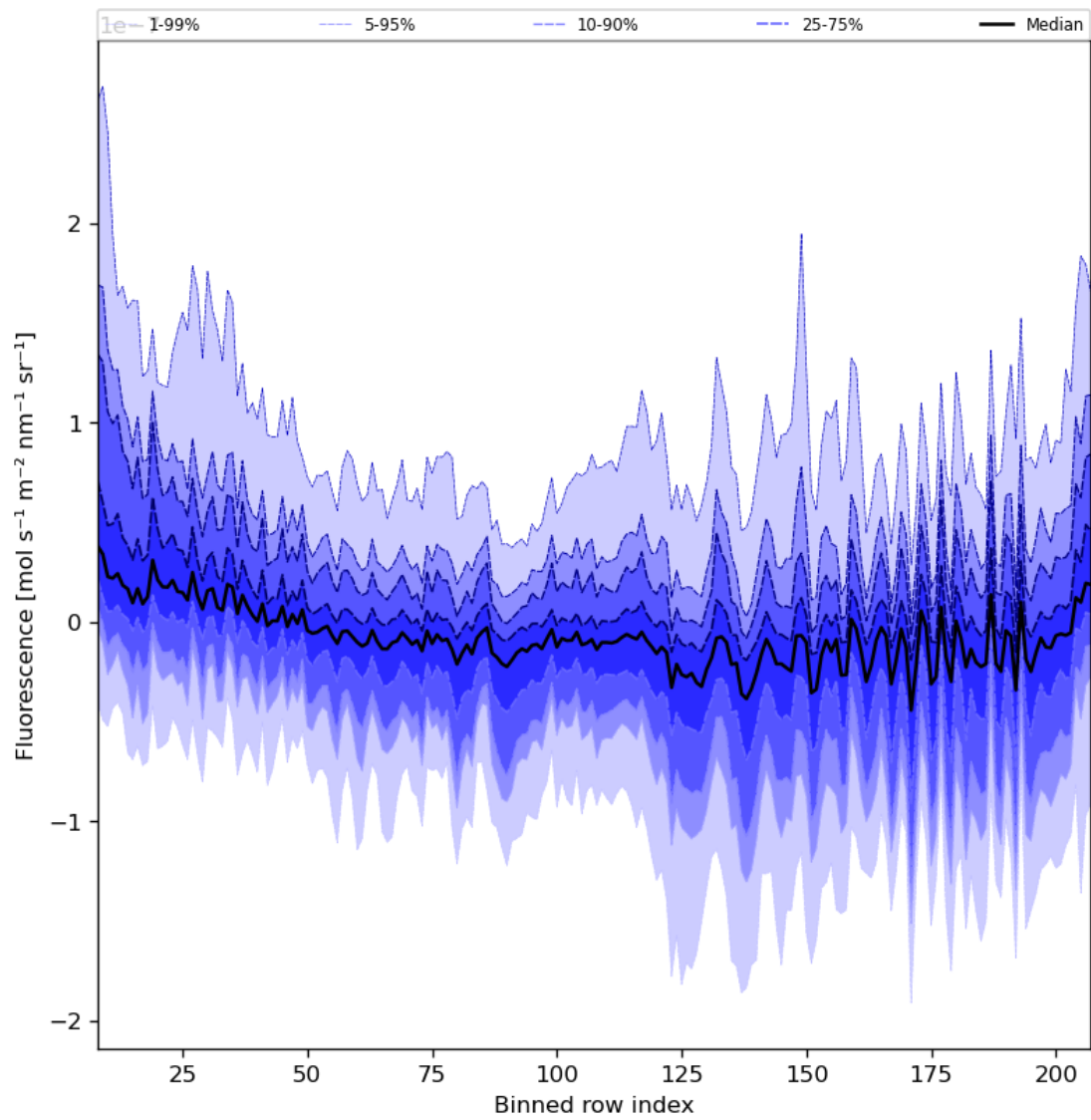
Figure 43: Along track statistics of “Fluorescence” for 2024-06-19 to 2024-06-21
