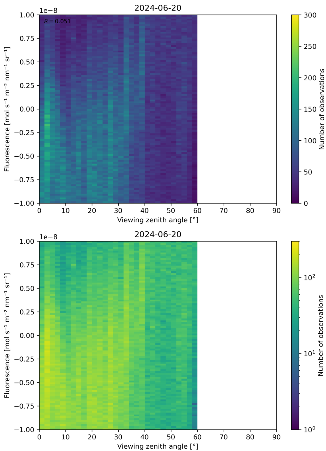
Figure 108: Scatter density plot of “Viewing zenith angle” against “Fluorescence” for 2024-06-19 to 2024-06-21.
