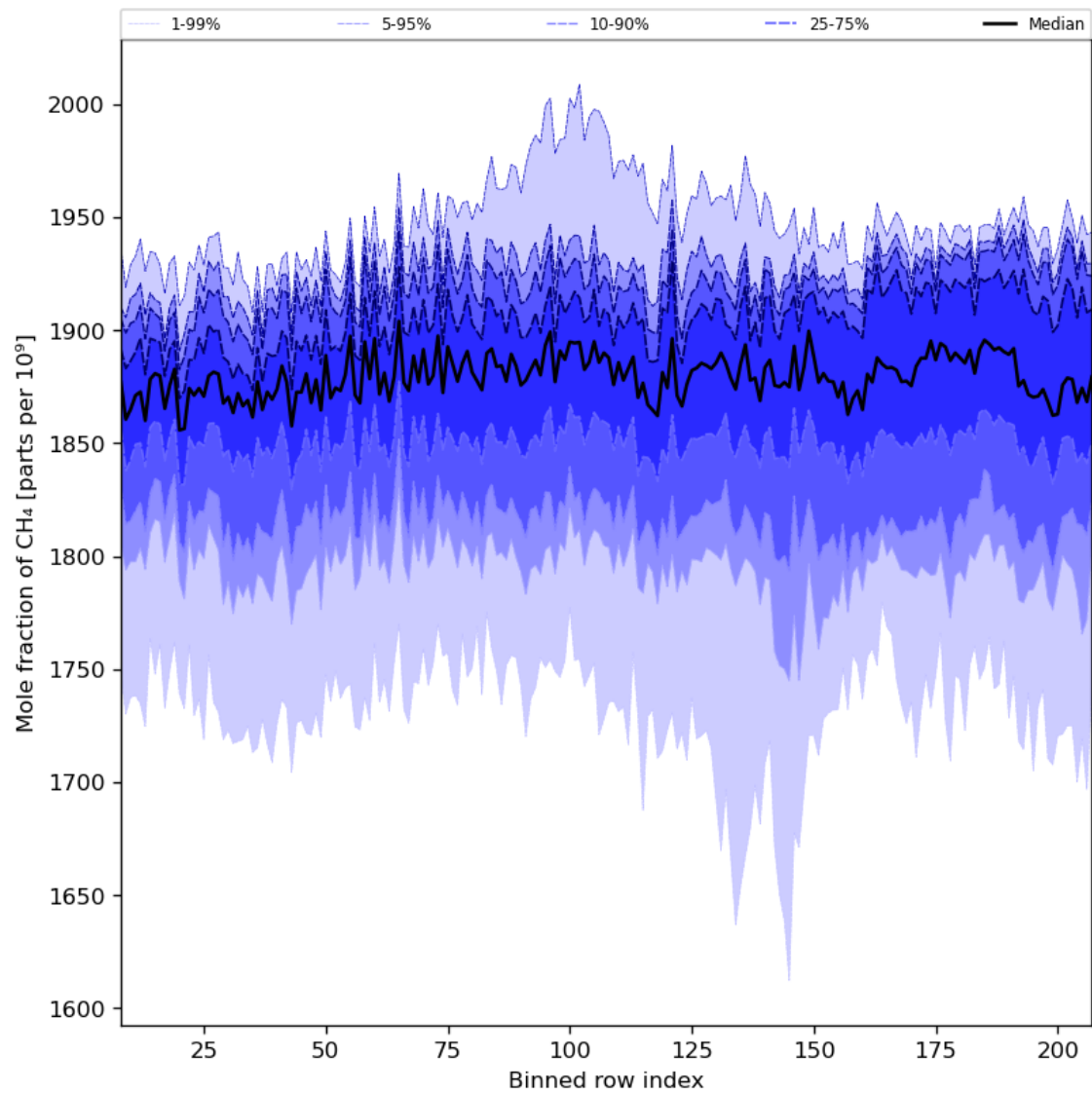
Figure 34: Along track statistics of “Mole fraction of CH 4 ” for 2024-06-19 to 2024-06-21
