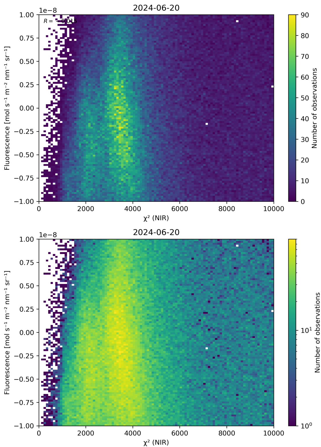
Figure 45: Scatter density plot of “ \chi^2 (NIR)” against “Fluorescence” for 2024-06-19 to 2024-06-21.
