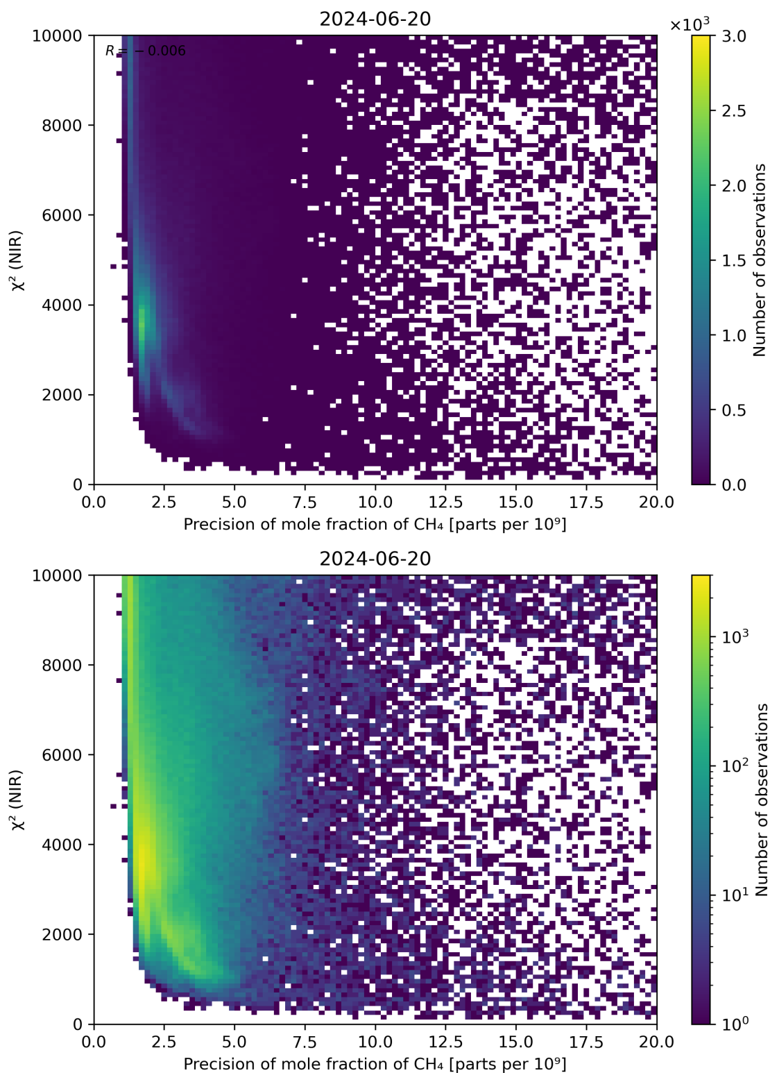
Figure 78: Scatter density plot of “Precision of mole fraction of CH 4 ” against “ \chi^2 (NIR)” for 2024-06-19 to 2024-06-21.
