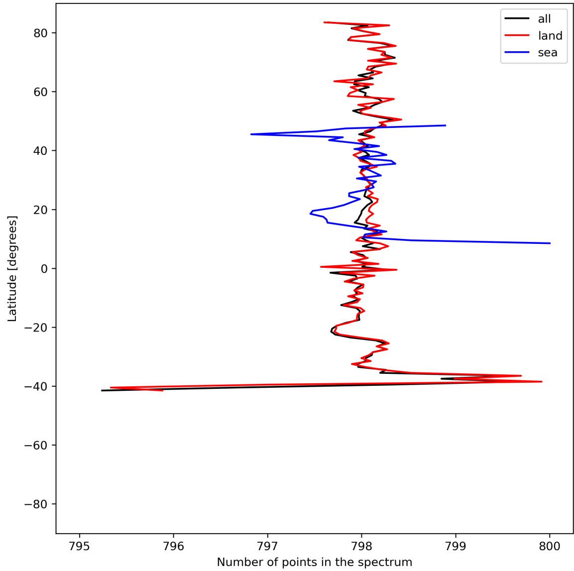
Figure 15: Zonal average of “Number of points in the spectrum” for 2024-06-19 to 2024-06-21.
