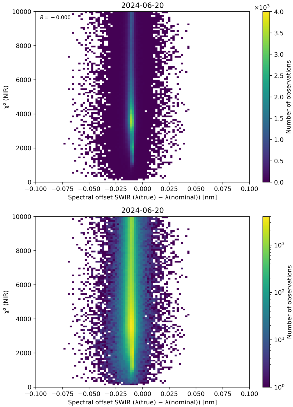
Figure 117: Scatter density plot of “Spectral offset SWIR ( \lambda(\text{true}) - \lambda(\text{nominal}) )” against “ \chi^2 (NIR)” for 2024-06-19 to 2024-06-21.
