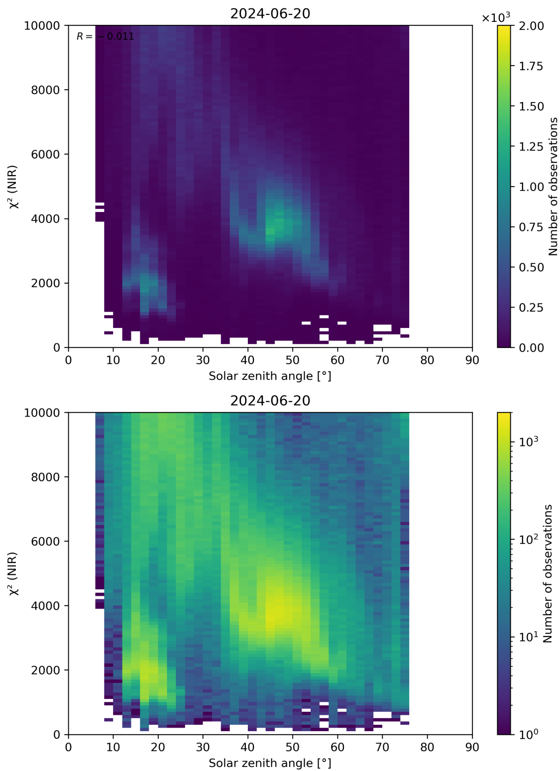
Figure 94: Scatter density plot of “Solar zenith angle” against “ \chi^2 (NIR)” for 2024-06-19 to 2024-06-21.
