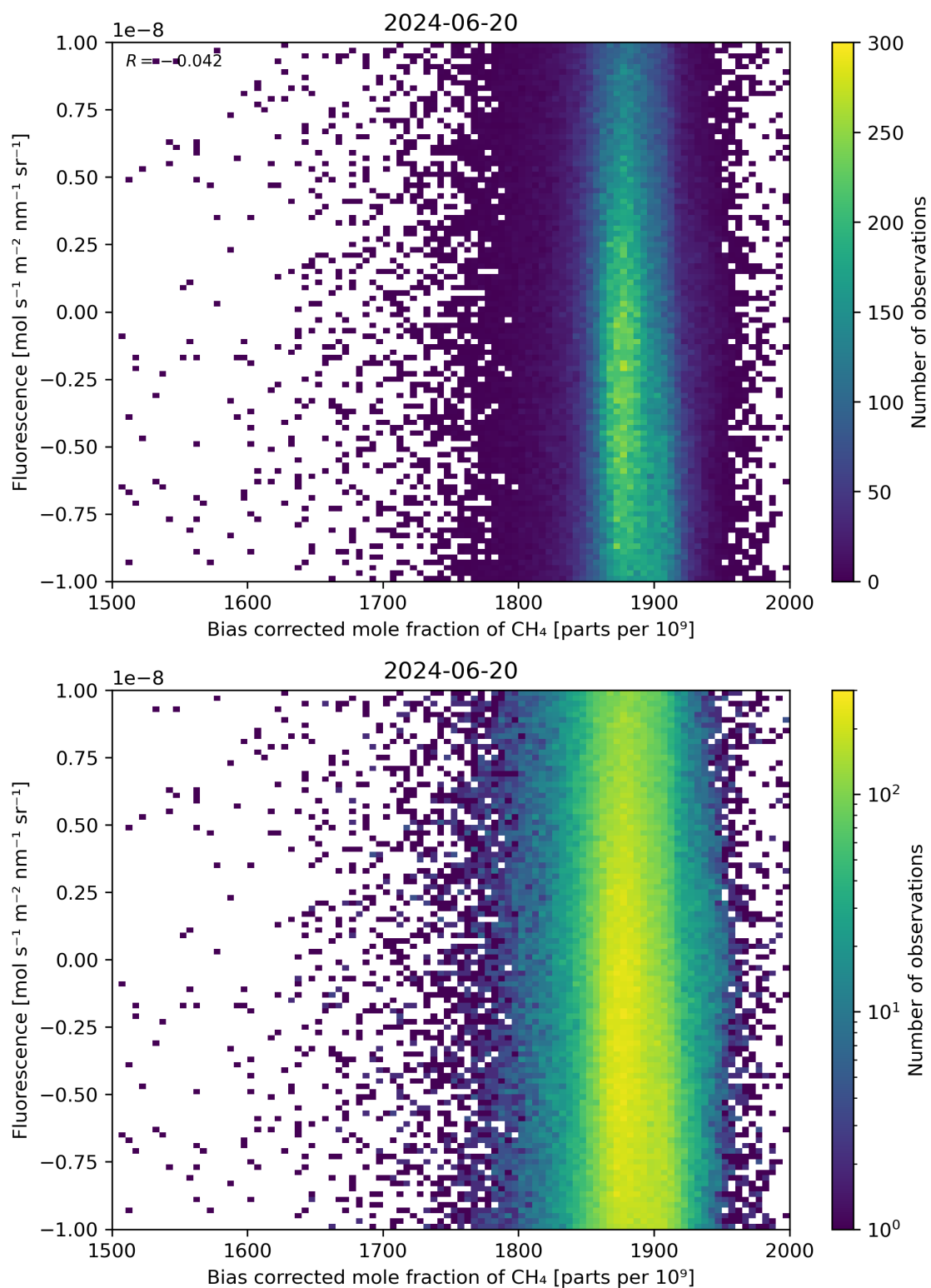
Figure 66: Scatter density plot of “Bias corrected mole fraction of CH 4 ” against “Fluorescence” for 2024-06-19 to 2024-06-21.
