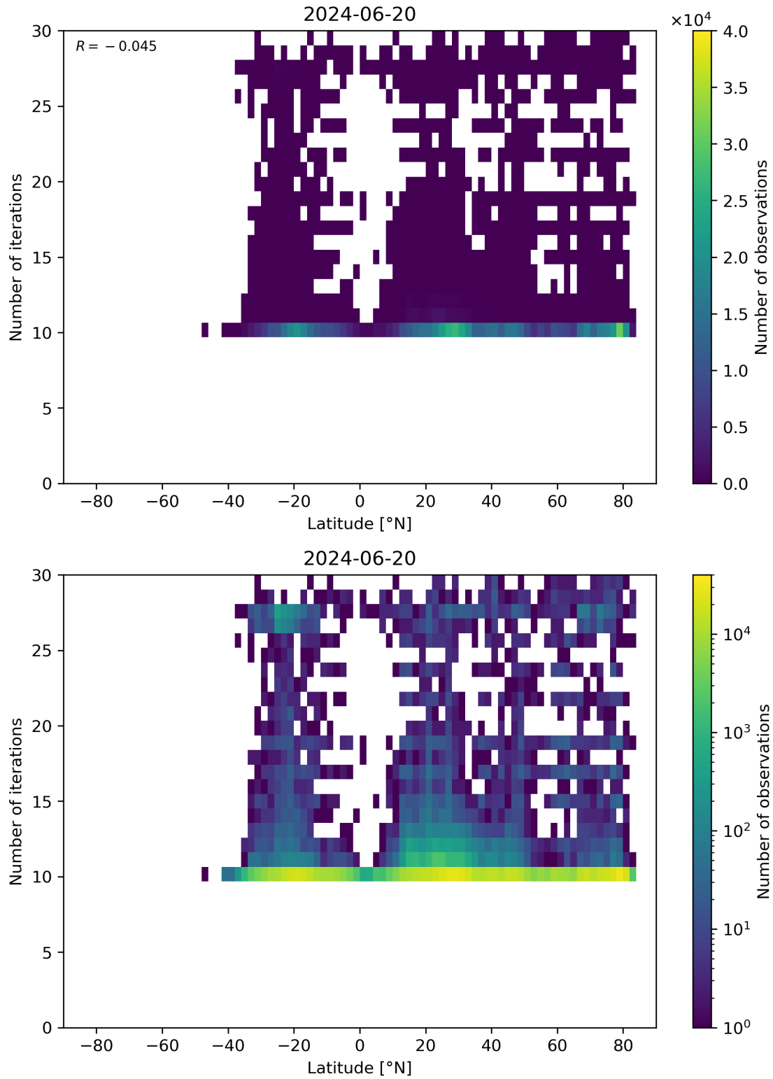
Figure 60: Scatter density plot of “Latitude” against “Number of iterations” for 2024-06-19 to 2024-06-21.
