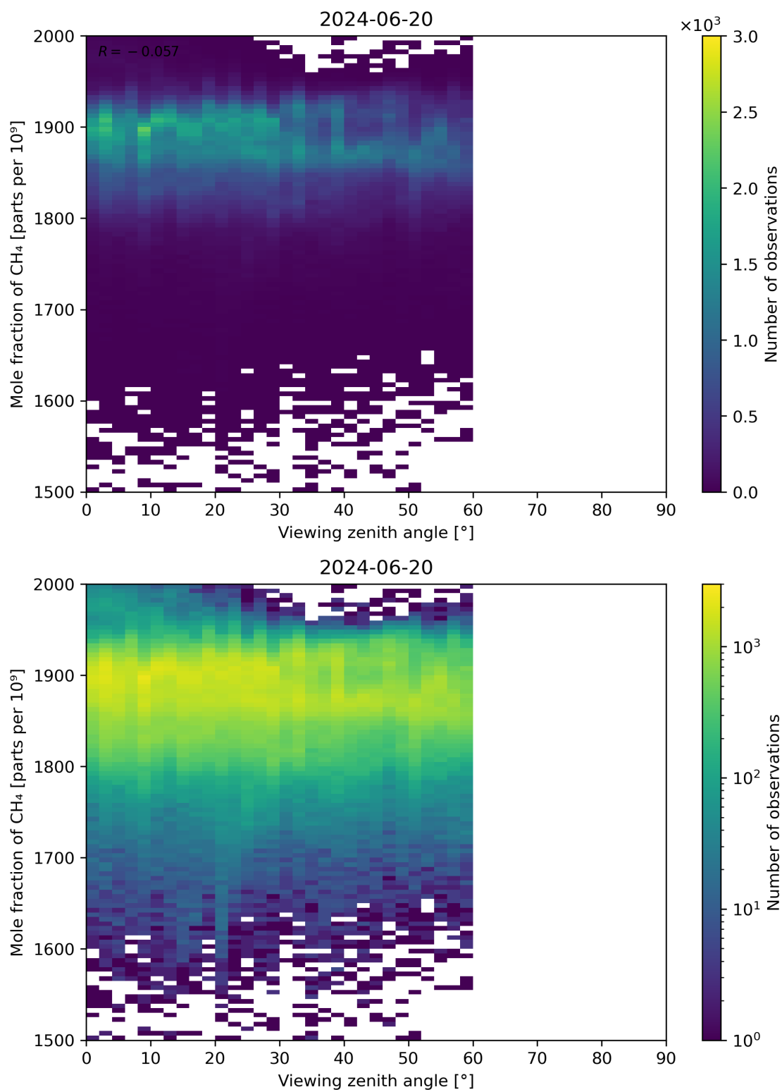
Figure 110: Scatter density plot of “Viewing zenith angle” against “Mole fraction of CH 4 ” for 2024-06-19 to 2024-06-21.
