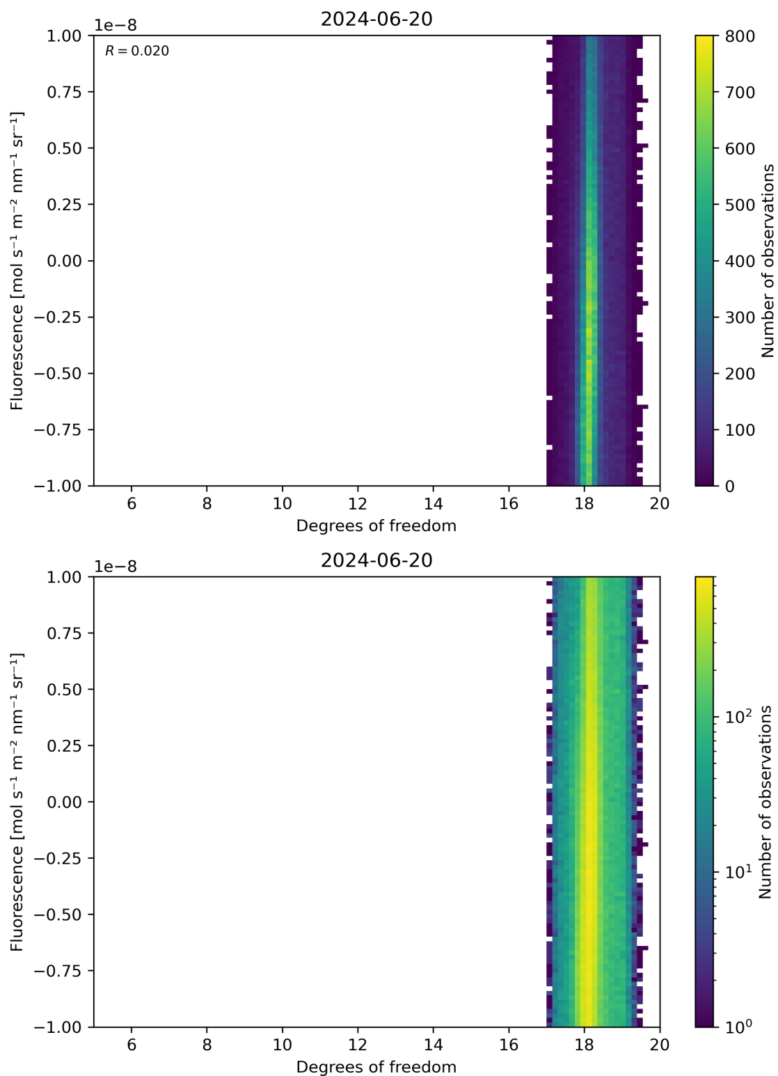
Figure 51: Scatter density plot of “Degrees of freedom” against “Fluorescence” for 2024-06-19 to 2024-06-21.
