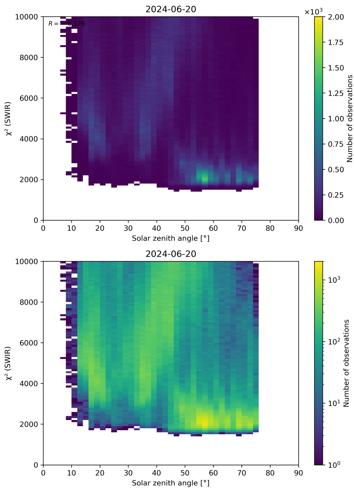
Figure 95: Scatter density plot of “Solar zenith angle” against “ \chi^2 (SWIR)” for 2024-06-19 to 2024-06-21.
