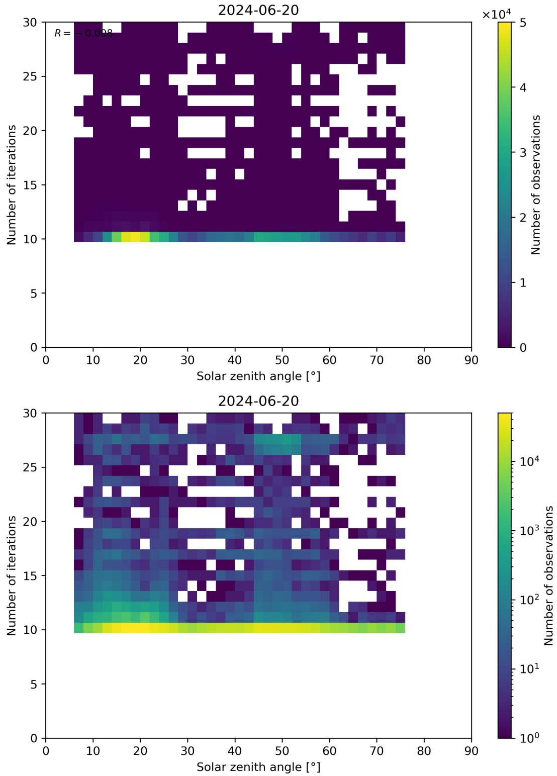
Figure 102: Scatter density plot of “Solar zenith angle” against “Number of iterations” for 2024-06-19 to 2024-06-21.
