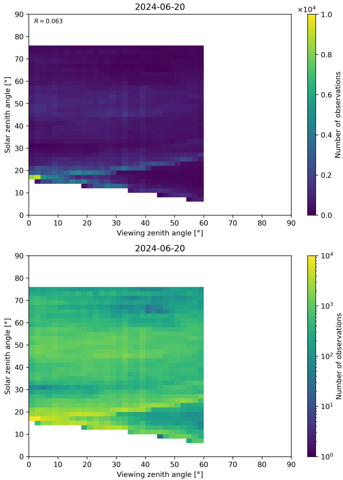
Figure 115: Scatter density plot of “Viewing zenith angle” against “Solar zenith angle” for 2024-06-19 to 2024-06-21.
