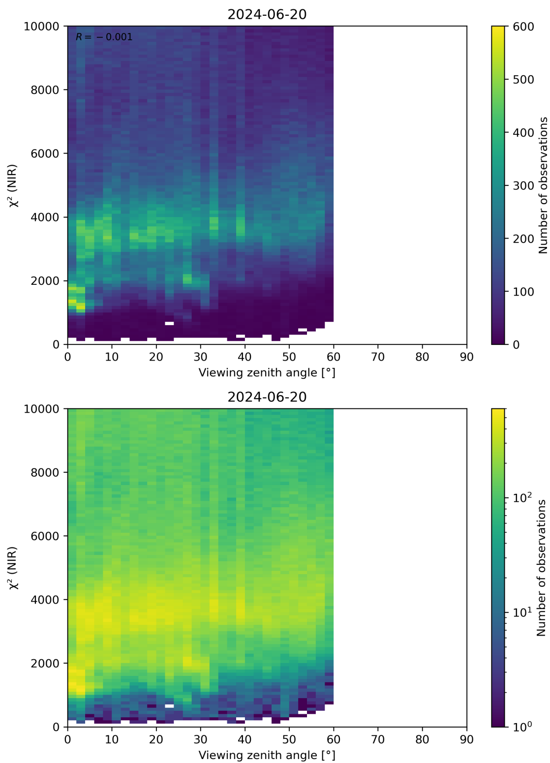
Figure 105: Scatter density plot of “Viewing zenith angle” against “ \chi^2 (NIR)” for 2024-06-19 to 2024-06-21.
