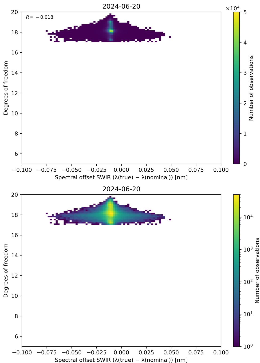
Figure 119: Scatter density plot of “Spectral offset SWIR ( \lambda(\text{true}) - \lambda(\text{nominal}) )” against “Degrees of freedom” for 2024-06-19 to 2024-06-21.
