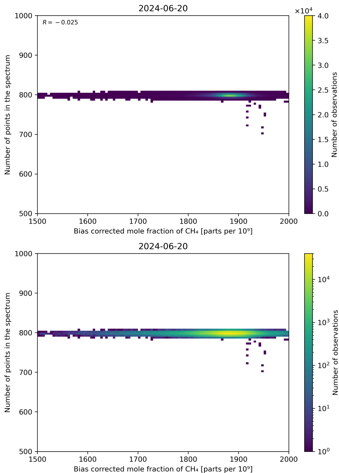
Figure 68: Scatter density plot of “Bias corrected mole fraction of CH 4 ” against “Number of points in the spectrum” for 2024-06-19 to 2024-06-21.
