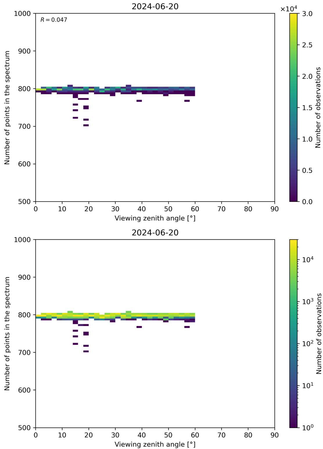
Figure 114: Scatter density plot of “Viewing zenith angle” against “Number of points in the spectrum” for 2024-06-19 to 2024-06-21.
