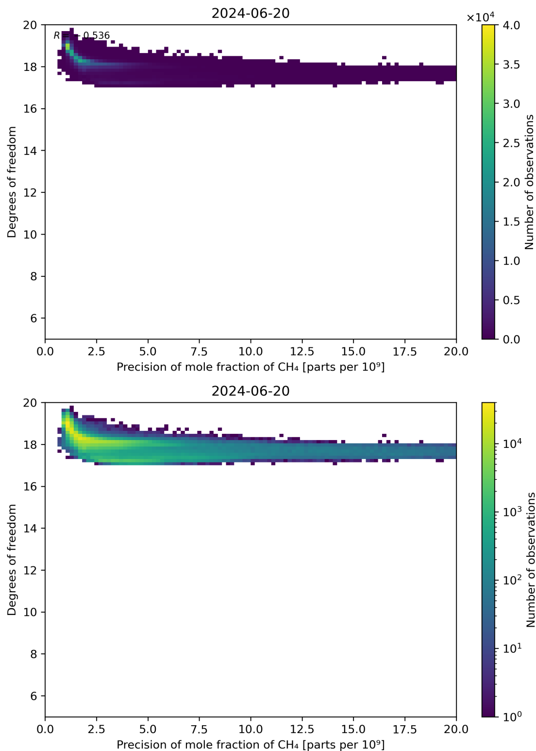
Figure 80: Scatter density plot of “Precision of mole fraction of CH 4 ” against “Degrees of freedom” for 2024-06-19 to 2024-06-21.
