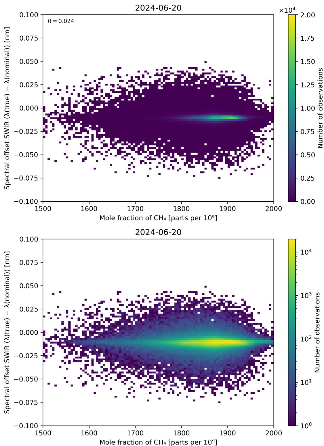
Figure 86: Scatter density plot of “Mole fraction of CH 4 ” against “Spectral offset SWIR ( \lambda(\text{true}) - \lambda(\text{nominal}) )” for 2024-06-19 to 2024-06-21.
