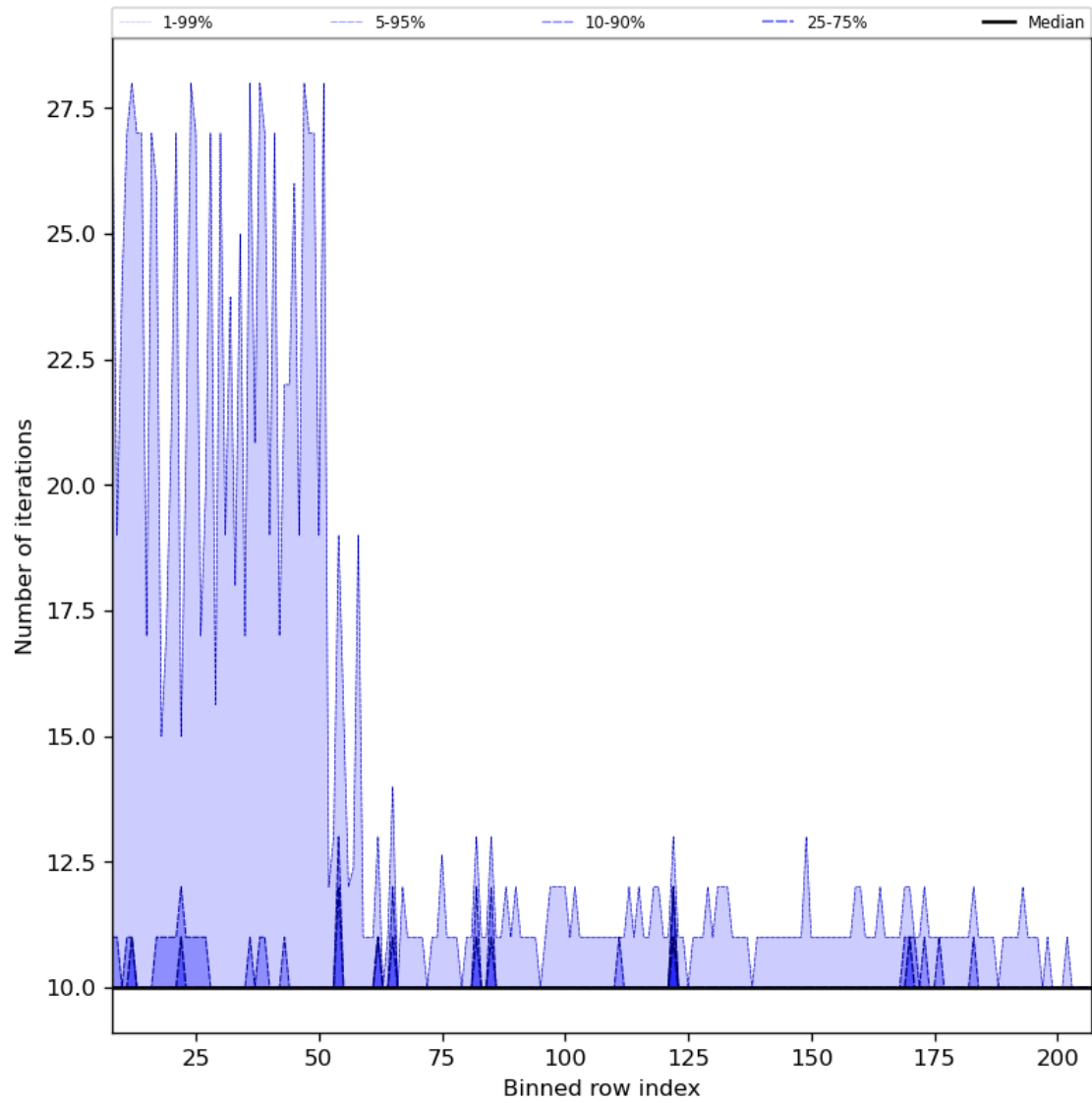
Figure 42: Along track statistics of “Number of iterations” for 2024-06-19 to 2024-06-21
