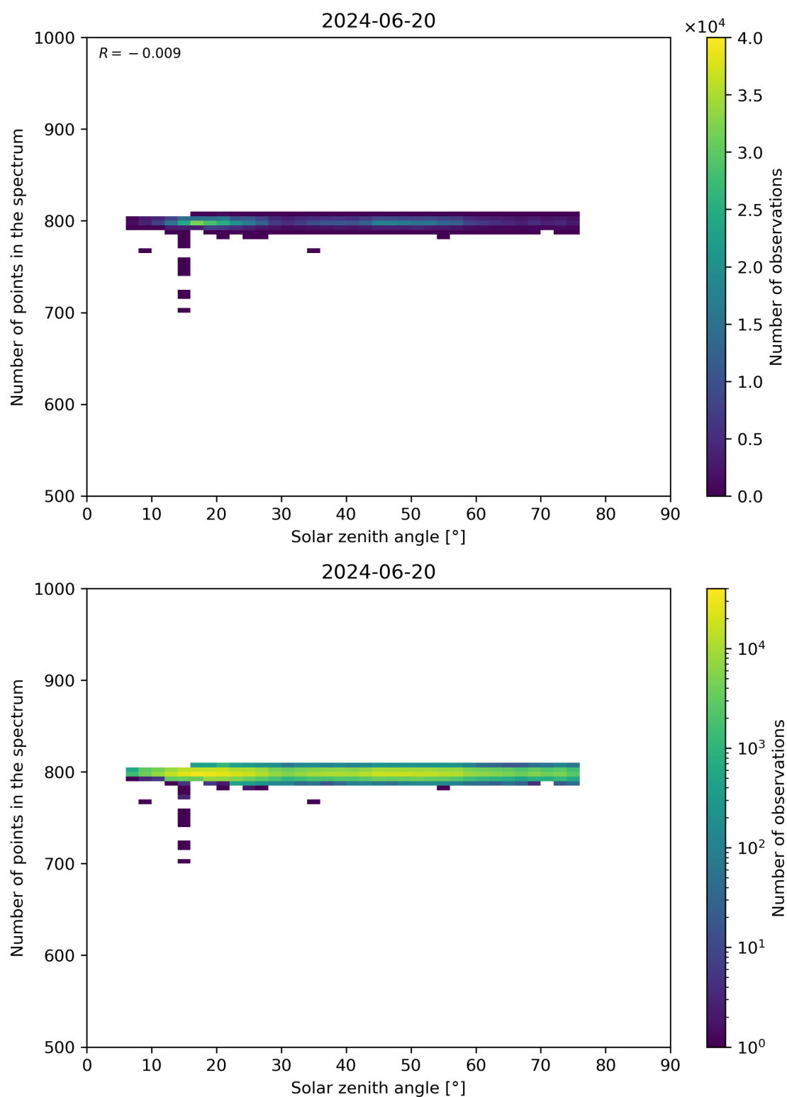
Figure 103: Scatter density plot of “Solar zenith angle” against “Number of points in the spectrum” for 2024-06-19 to 2024-06-21.
