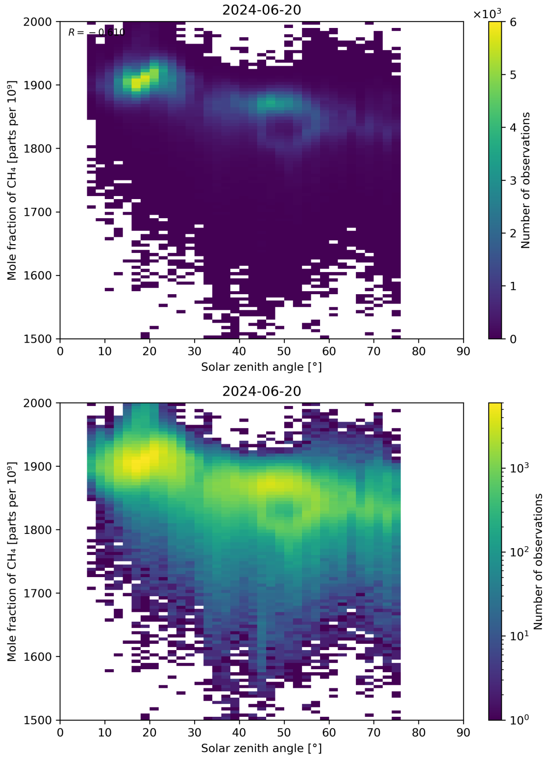
Figure 99: Scatter density plot of “Solar zenith angle” against “Mole fraction of \text{CH}_4 ” for 2024-06-19 to 2024-06-21.
