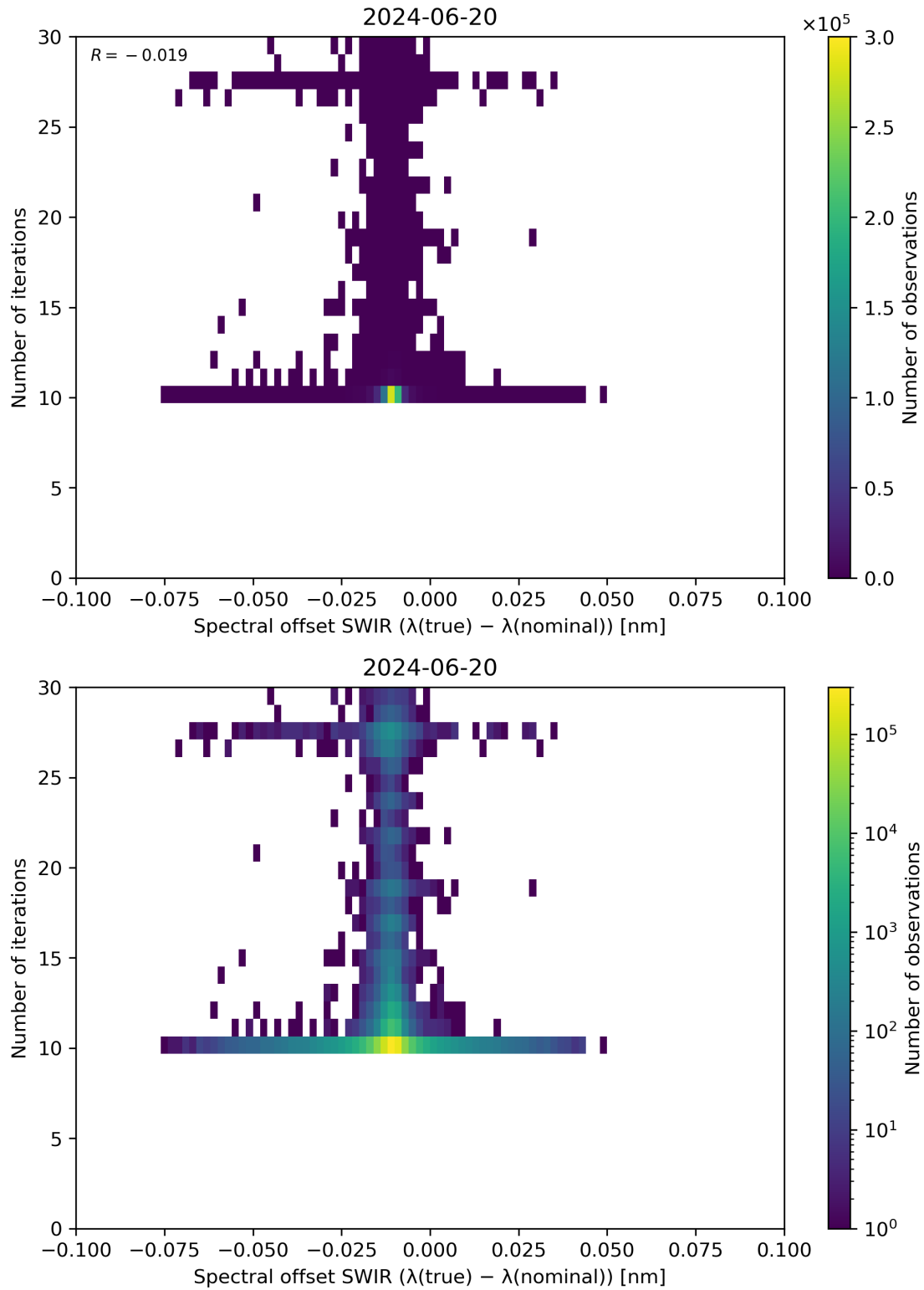
Figure 121: Scatter density plot of “Spectral offset SWIR ( \lambda(\text{true}) - \lambda(\text{nominal}) )” against “Number of iterations” for 2024-06-19 to 2024-06-21.
