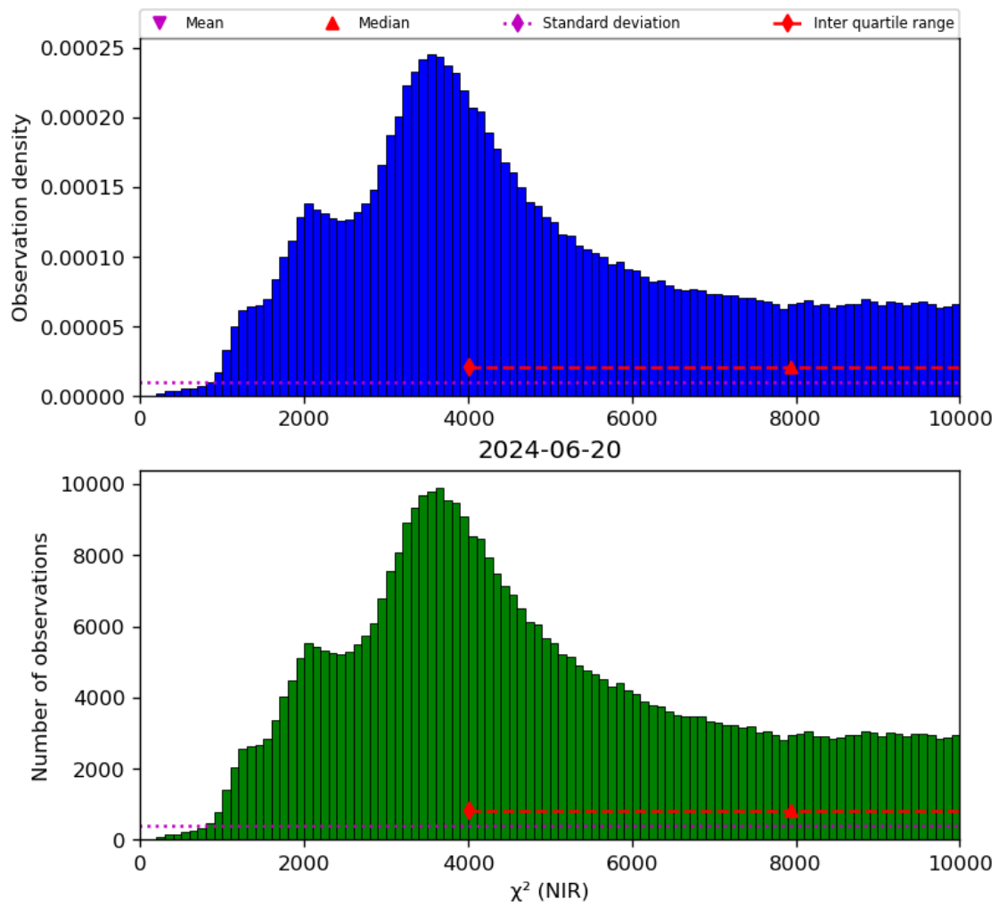
Figure 29: Histogram of “ \chi^2 (NIR)” for 2024-06-19 to 2024-06-21
