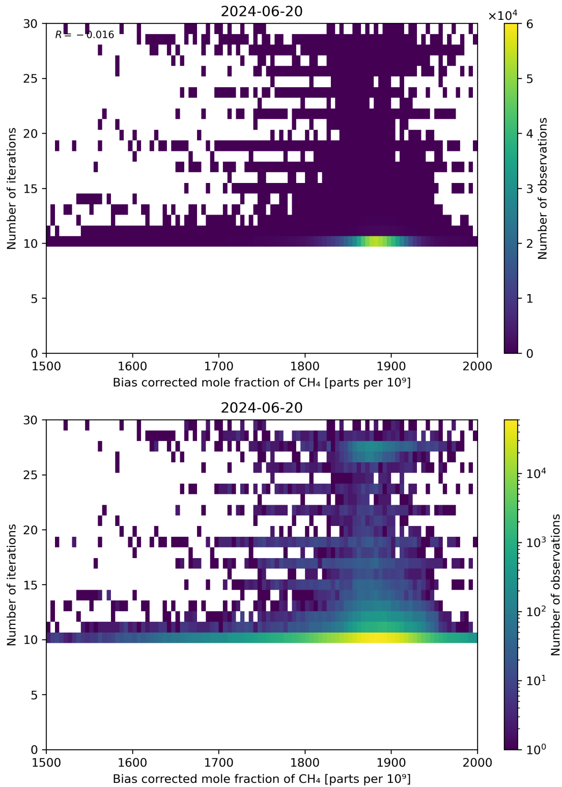
Figure 67: Scatter density plot of “Bias corrected mole fraction of CH 4 ” against “Number of iterations” for 2024-06-19 to 2024-06-21.
