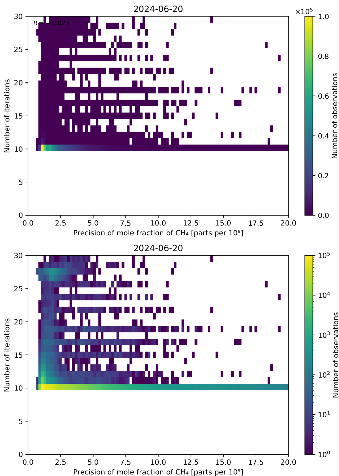
Figure 83: Scatter density plot of “Precision of mole fraction of CH 4 ” against “Number of iterations” for 2024-06-19 to 2024-06-21.
