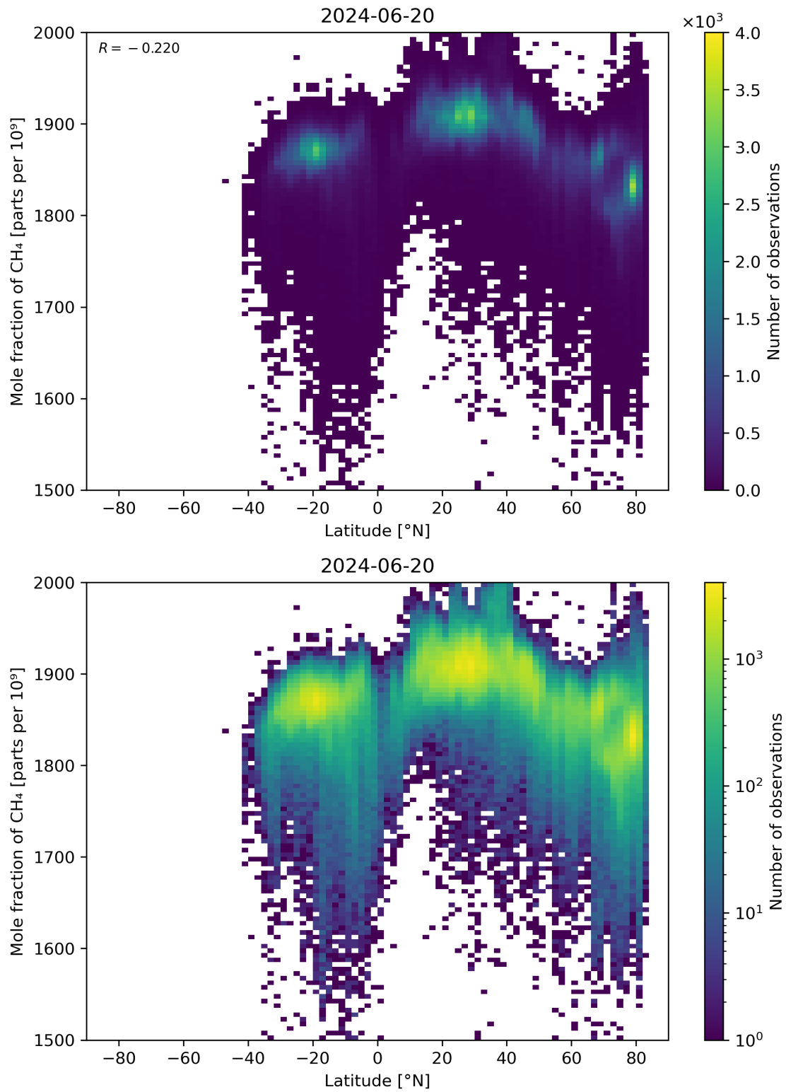
Figure 57: Scatter density plot of “Latitude” against “Mole fraction of CH 4 ” for 2024-06-19 to 2024-06-21.
