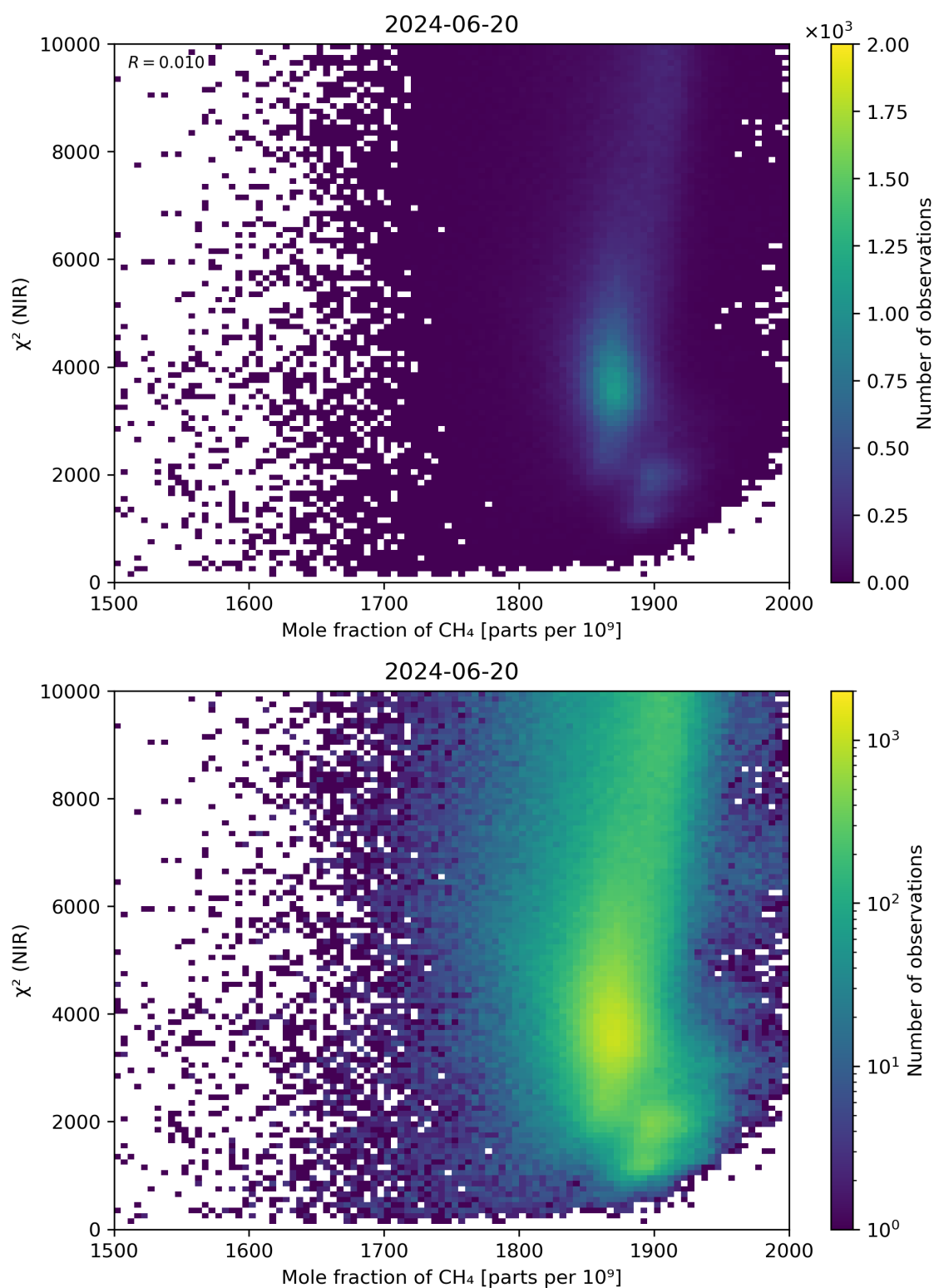
Figure 70: Scatter density plot of “Mole fraction of \text{CH}_4 ” against “ \chi^2 (NIR)” for 2024-06-19 to 2024-06-21.
