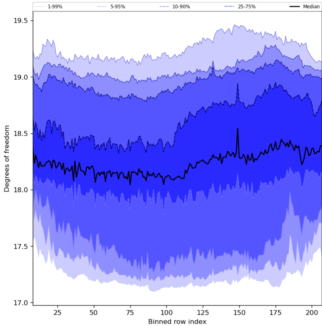
Figure 41: Along track statistics of “Degrees of freedom” for 2024-06-19 to 2024-06-21
