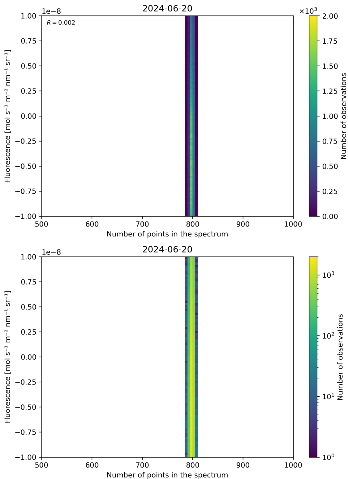
Figure 91: Scatter density plot of “Number of points in the spectrum” against “Fluorescence” for 2024-06-19 to 2024-06-21.
