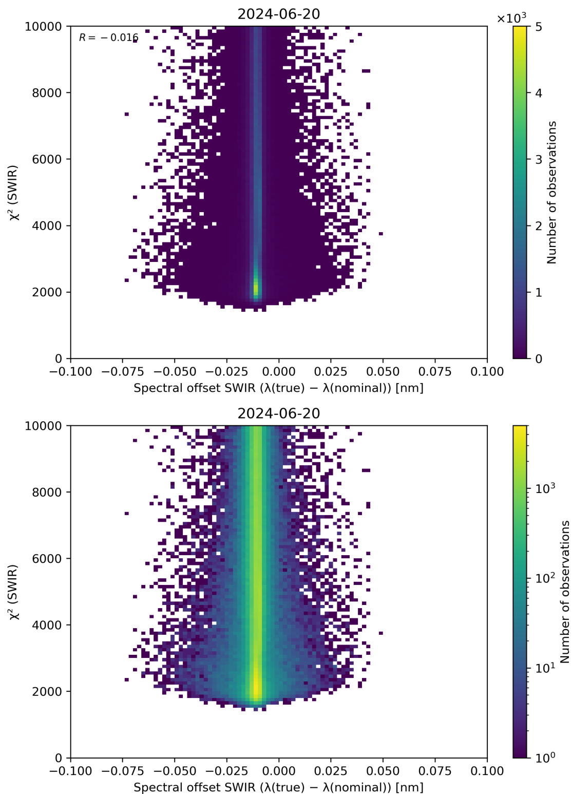
Figure 118: Scatter density plot of “Spectral offset SWIR ( \lambda(\text{true}) - \lambda(\text{nominal}) )” against “ \chi^2 (SWIR)” for 2024-06-19 to 2024-06-21.
