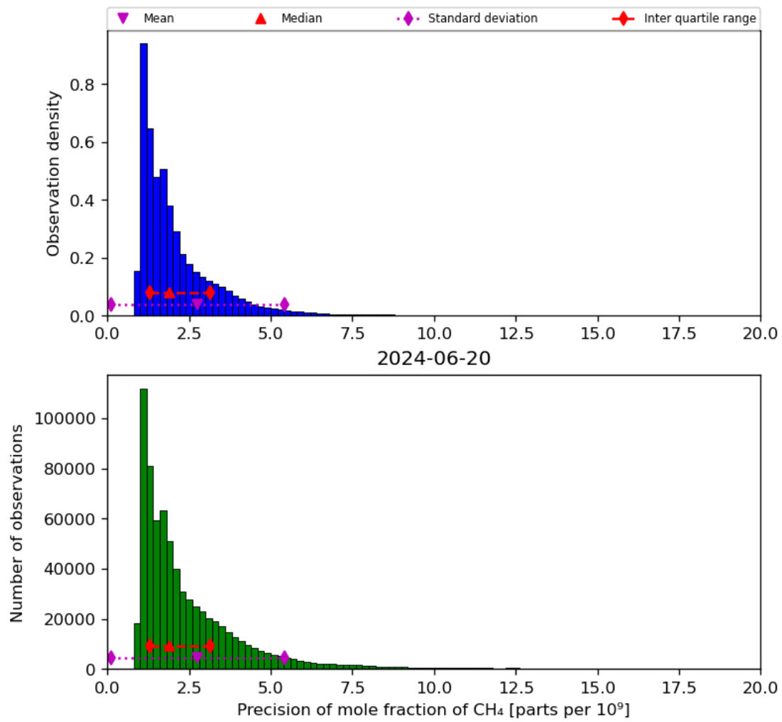
Figure 24: Histogram of “Precision of mole fraction of CH 4 ” for 2024-06-19 to 2024-06-21
