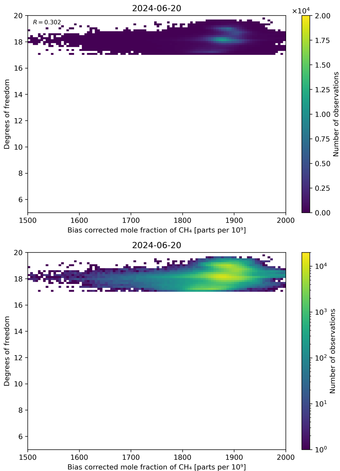
Figure 65: Scatter density plot of “Bias corrected mole fraction of CH 4 ” against “Degrees of freedom” for 2024-06-19 to 2024-06-21.
