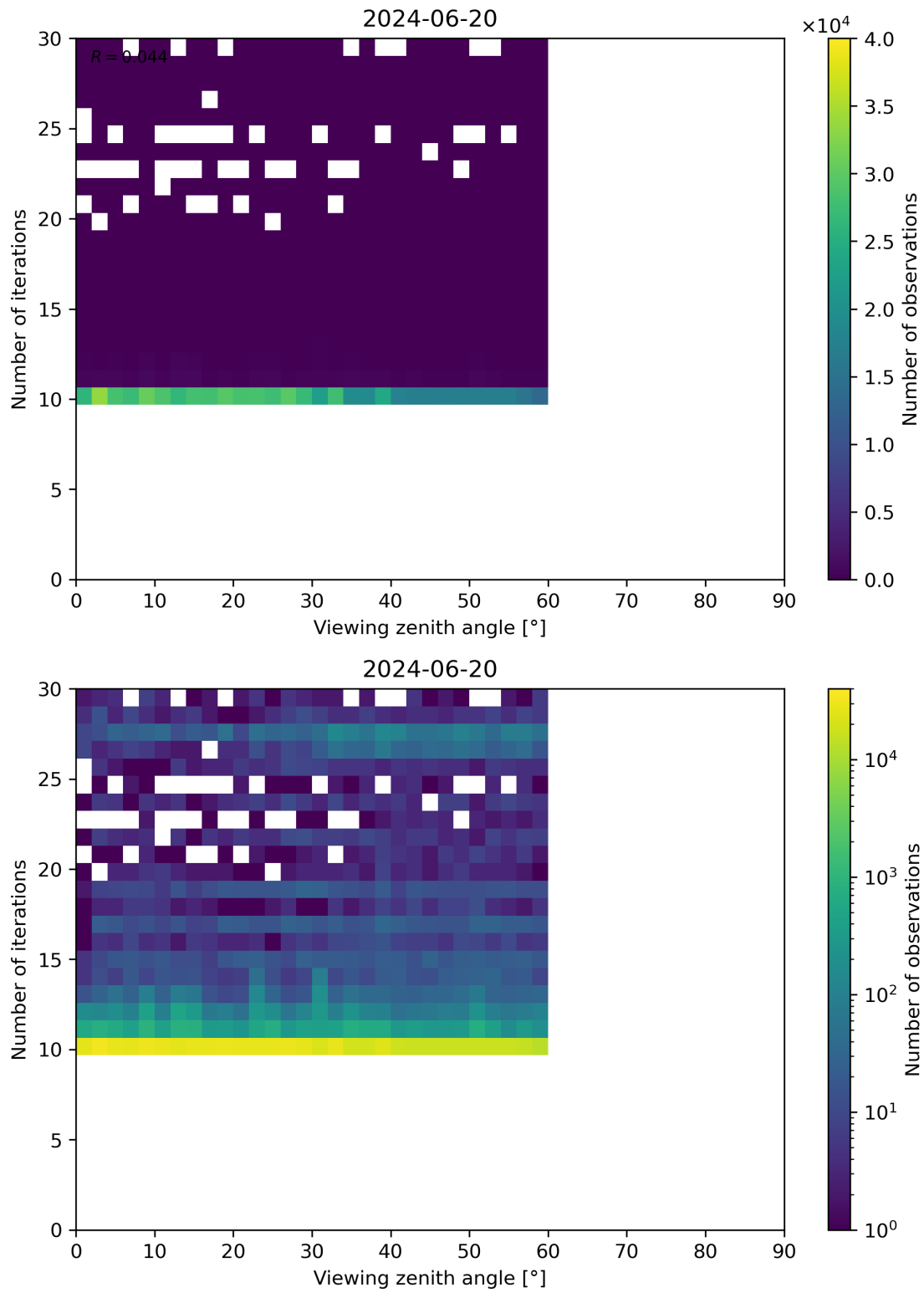
Figure 113: Scatter density plot of “Viewing zenith angle” against “Number of iterations” for 2024-06-19 to 2024-06-21.
