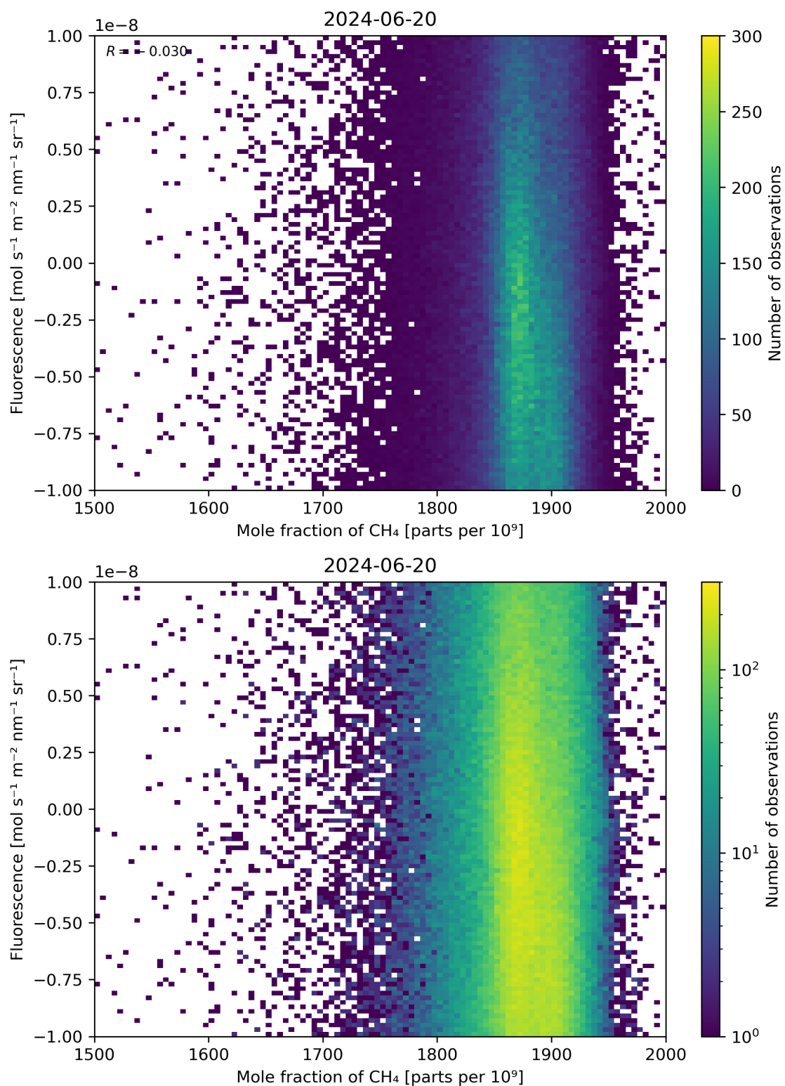
Figure 73: Scatter density plot of “Mole fraction of \text{CH}_4 ” against “Fluorescence” for 2024-06-19 to 2024-06-21.
