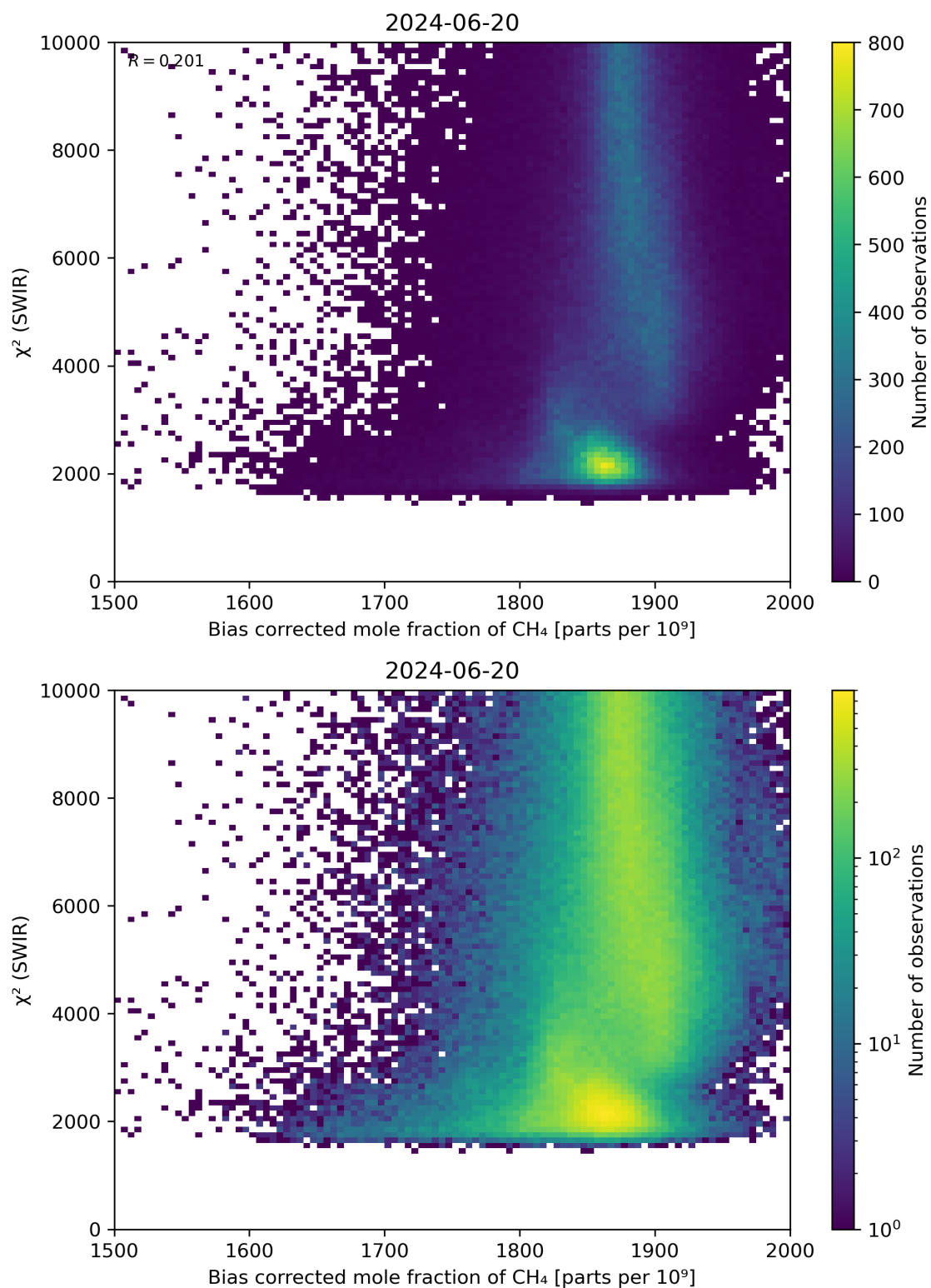
Figure 64: Scatter density plot of “Bias corrected mole fraction of \text{CH}_4 ” against “ \chi^2 (SWIR)” for 2024-06-19 to 2024-06-21.
