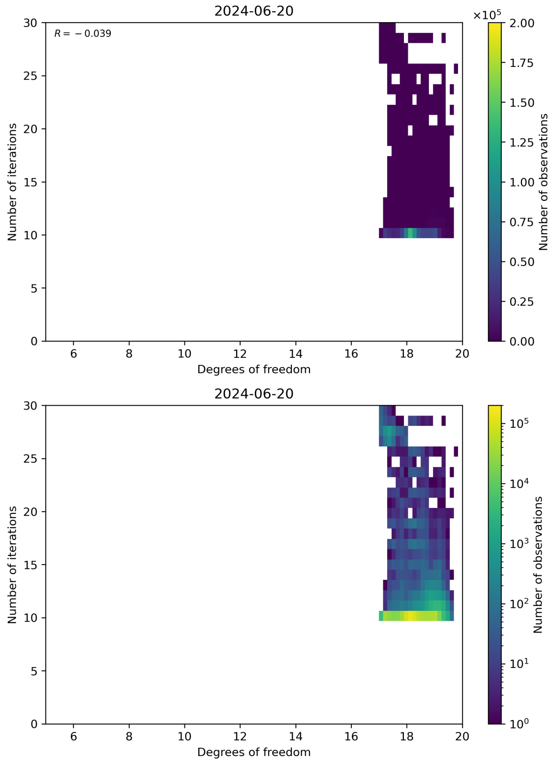
Figure 52: Scatter density plot of “Degrees of freedom” against “Number of iterations” for 2024-06-19 to 2024-06-21.
