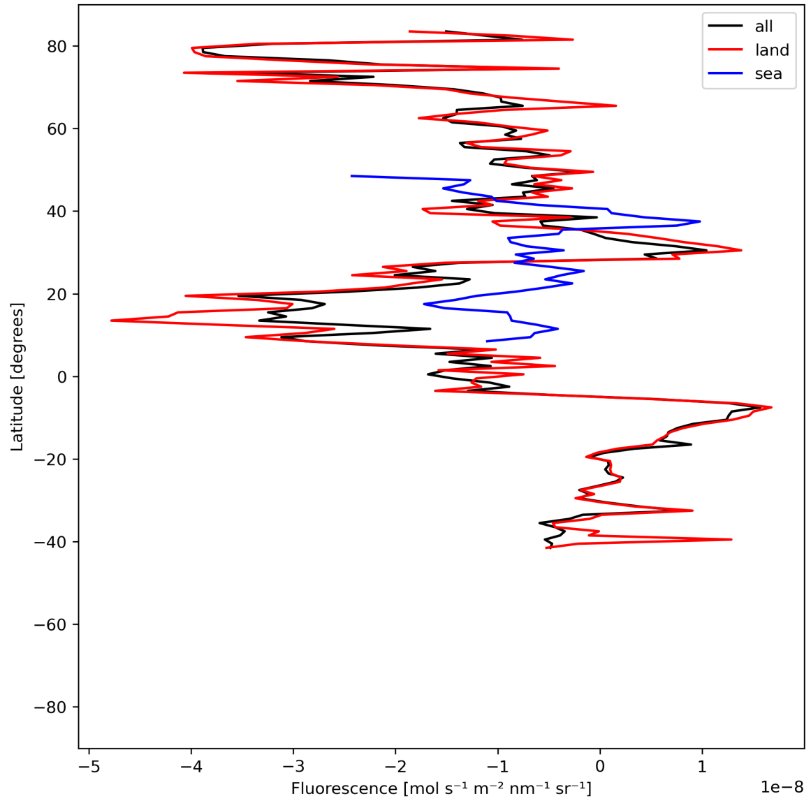
Figure 21: Zonal average of “Fluorescence” for 2024-06-19 to 2024-06-21.
