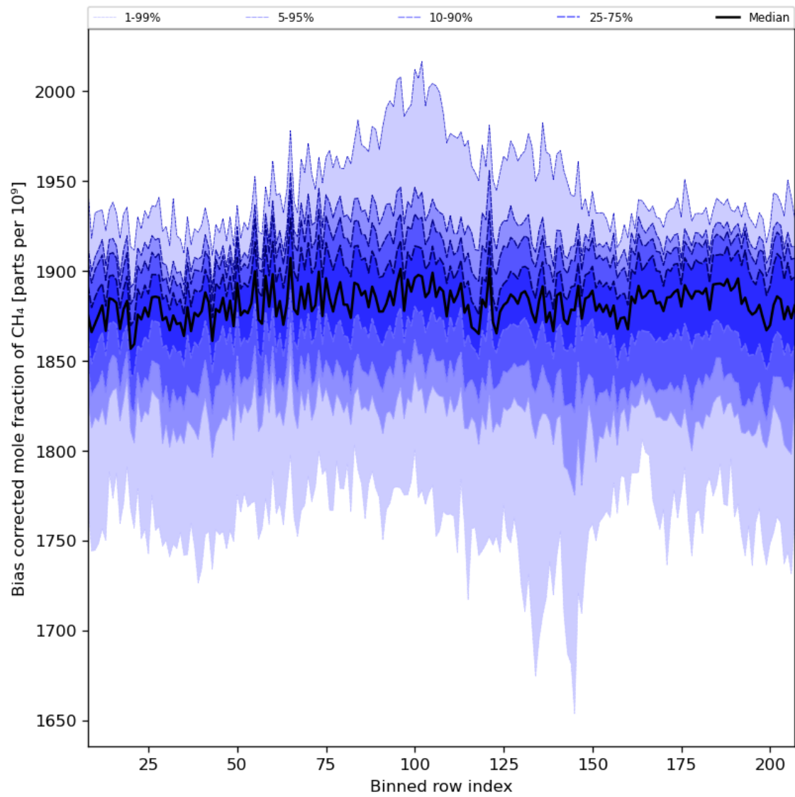
Figure 36: Along track statistics of “Bias corrected mole fraction of CH 4 ” for 2024-06-19 to 2024-06-21
