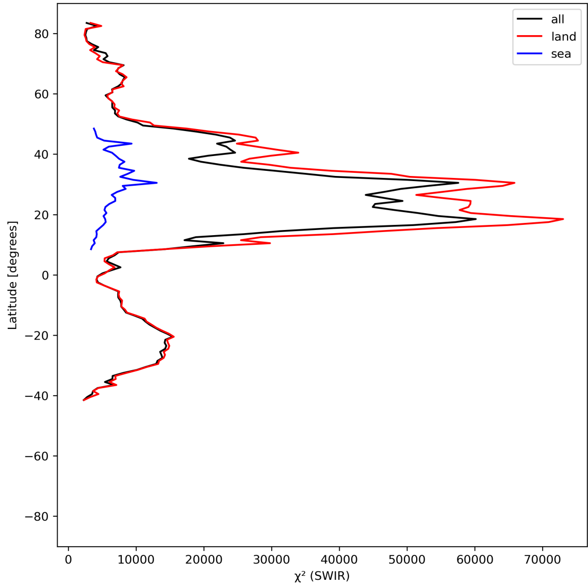
Figure 17: Zonal average of “ \chi^2 (SWIR)” for 2024-06-19 to 2024-06-21.
