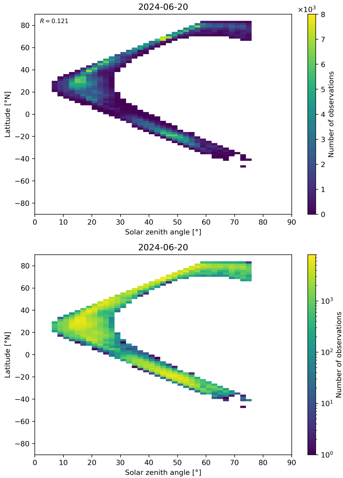
Figure 98: Scatter density plot of “Solar zenith angle” against “Latitude” for 2024-06-19 to 2024-06-21.
