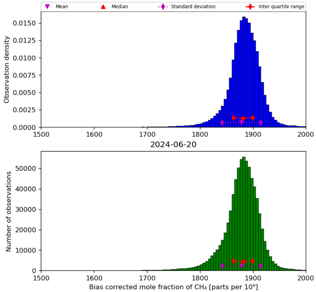
Figure 25: Histogram of “Bias corrected mole fraction of CH 4 ” for 2024-06-19 to 2024-06-21
