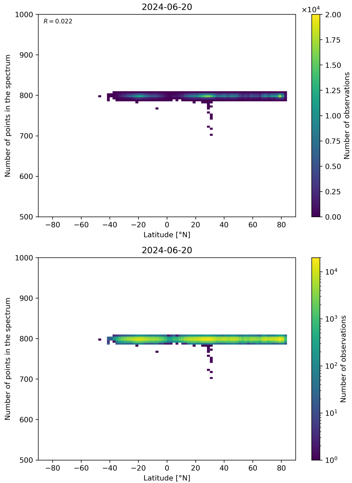
Figure 61: Scatter density plot of “Latitude” against “Number of points in the spectrum” for 2024-06-19 to 2024-06-21.
