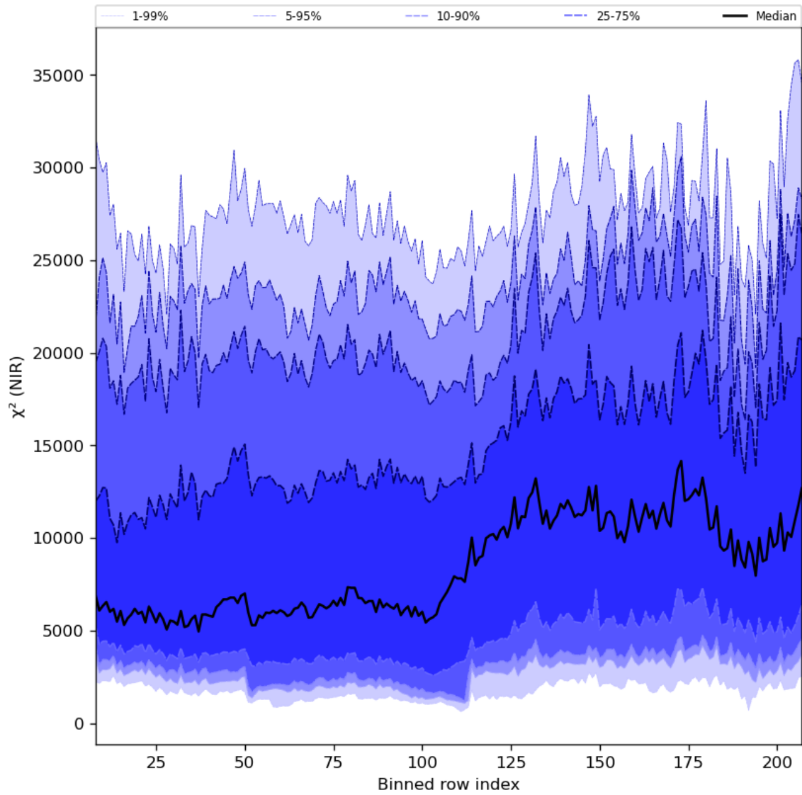
Figure 40: Along track statistics of " \chi^2 (NIR)" for 2024-06-19 to 2024-06-21
