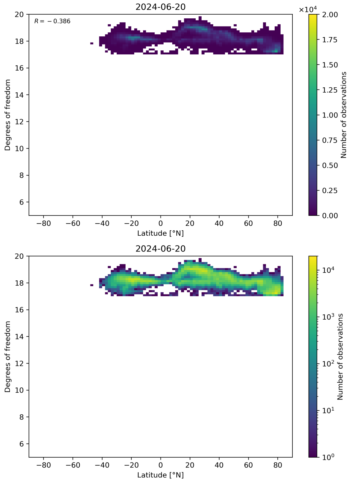
Figure 55: Scatter density plot of “Latitude” against “Degrees of freedom” for 2024-06-19 to 2024-06-21.
