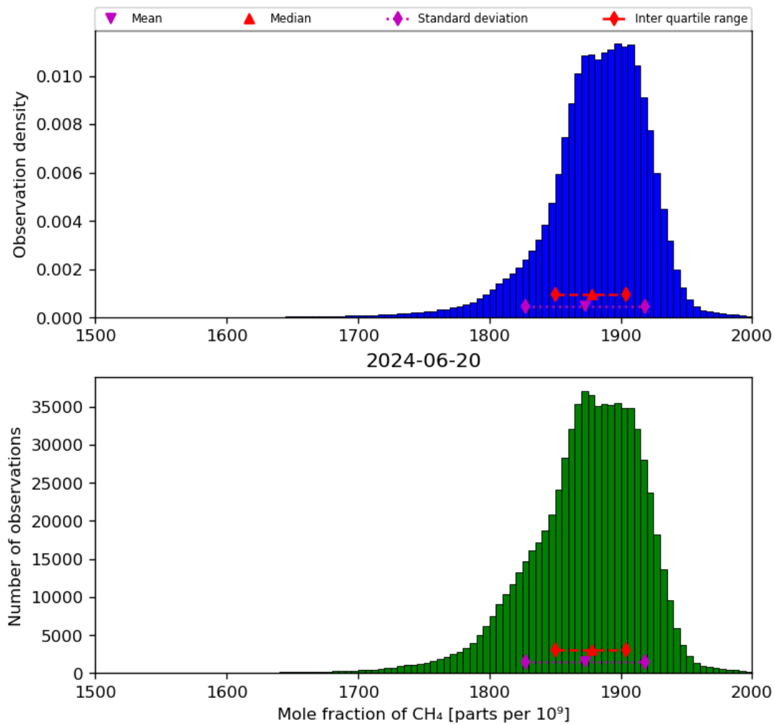
Figure 23: Histogram of “Mole fraction of CH 4 ” for 2024-06-19 to 2024-06-21
