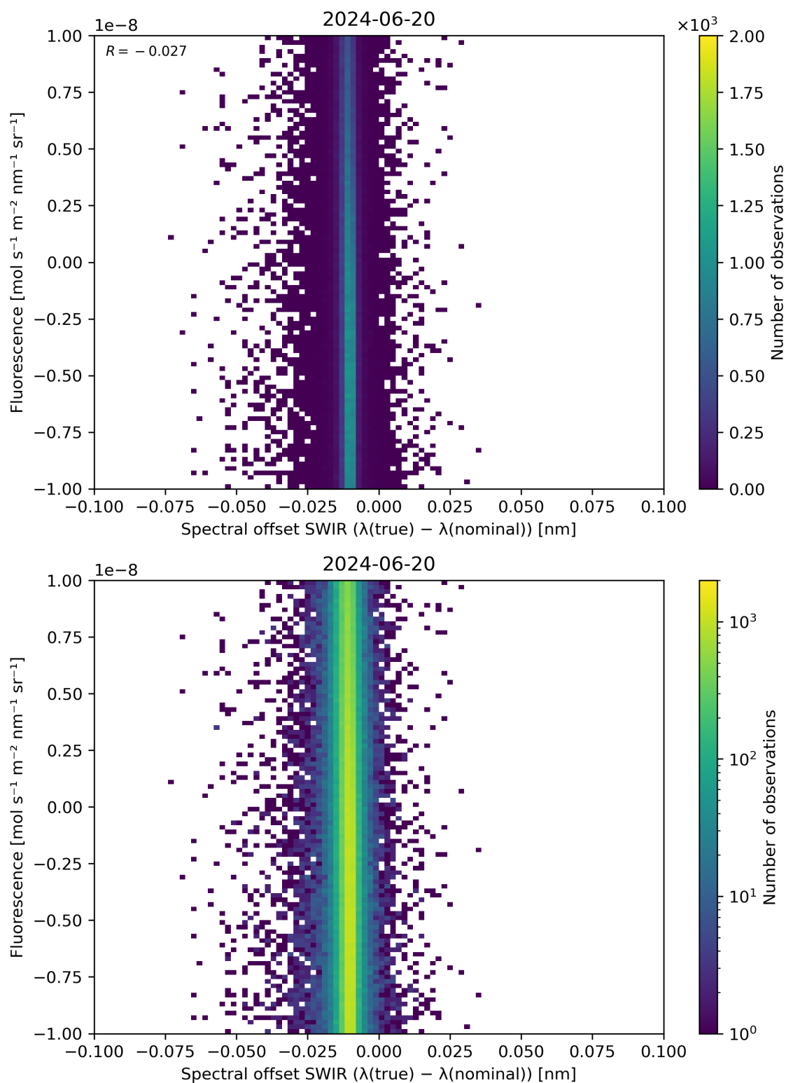
Figure 120: Scatter density plot of “Spectral offset SWIR ( \lambda(\text{true}) - \lambda(\text{nominal}) )” against “Fluorescence” for 2024-06-19 to 2024-06-21.
