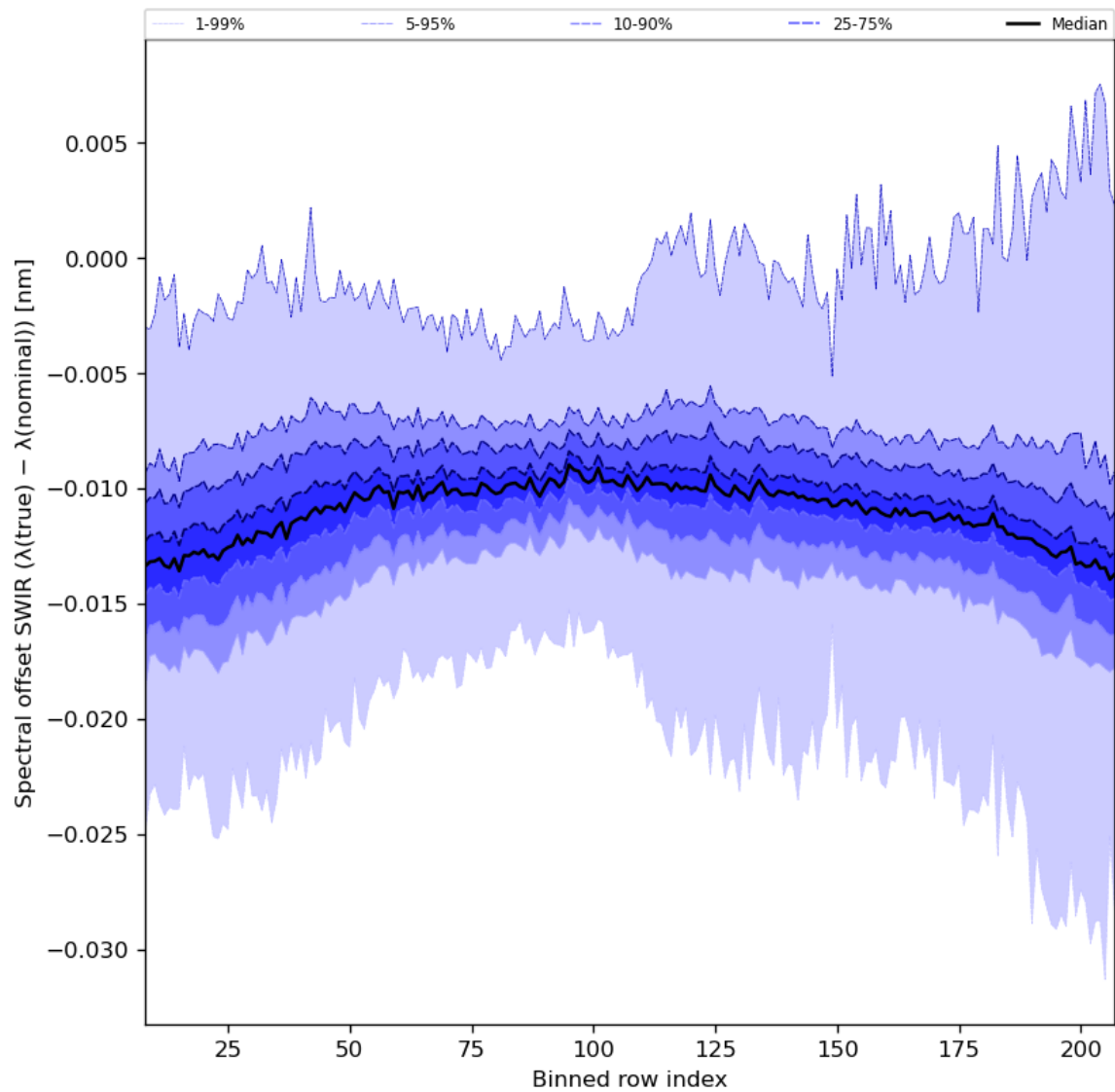
Figure 38: Along track statistics of “Spectral offset SWIR ( \lambda(\text{true}) - \lambda(\text{nominal}) )” for 2024-06-19 to 2024-06-21
