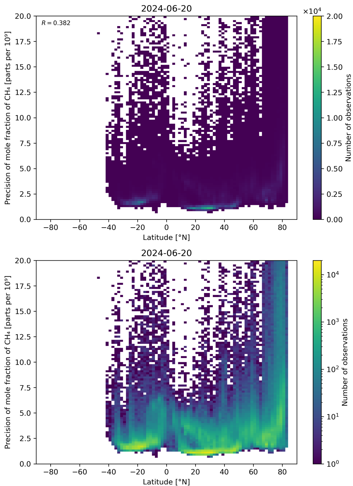
Figure 59: Scatter density plot of “Latitude” against “Precision of mole fraction of \text{CH}_4 ” for 2024-06-19 to 2024-06-21.
