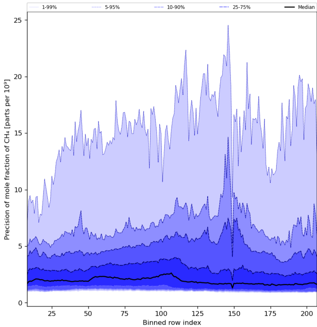
Figure 35: Along track statistics of “Precision of mole fraction of CH 4 ” for 2024-06-19 to 2024-06-21
