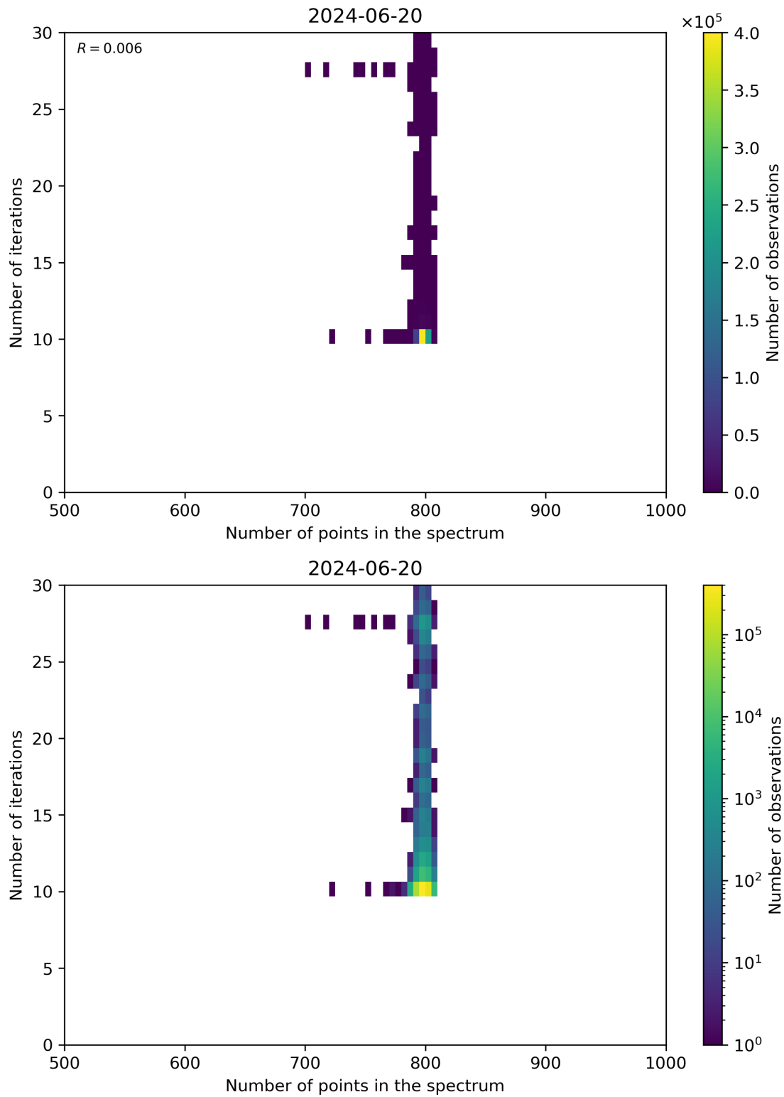
Figure 92: Scatter density plot of “Number of points in the spectrum” against “Number of iterations” for 2024-06-19 to 2024-06-21.
