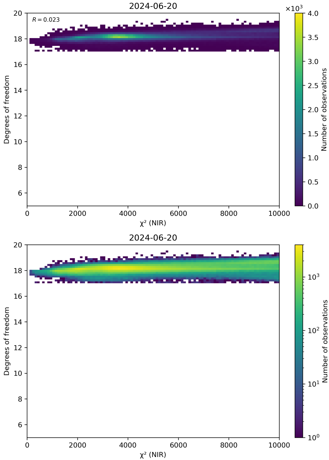
Figure 44: Scatter density plot of “ \chi^2 (NIR)” against “Degrees of freedom” for 2024-06-19 to 2024-06-21.
