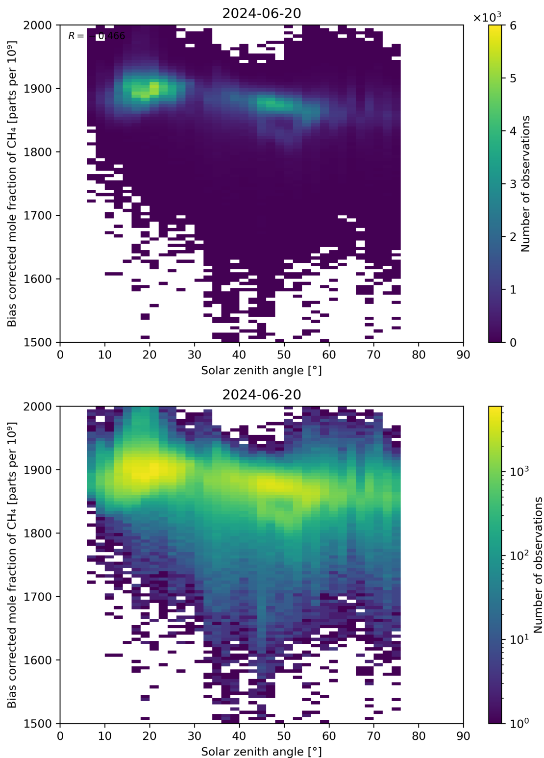
Figure 100: Scatter density plot of “Solar zenith angle” against “Bias corrected mole fraction of CH 4 ” for 2024-06-19 to 2024-06-21.
