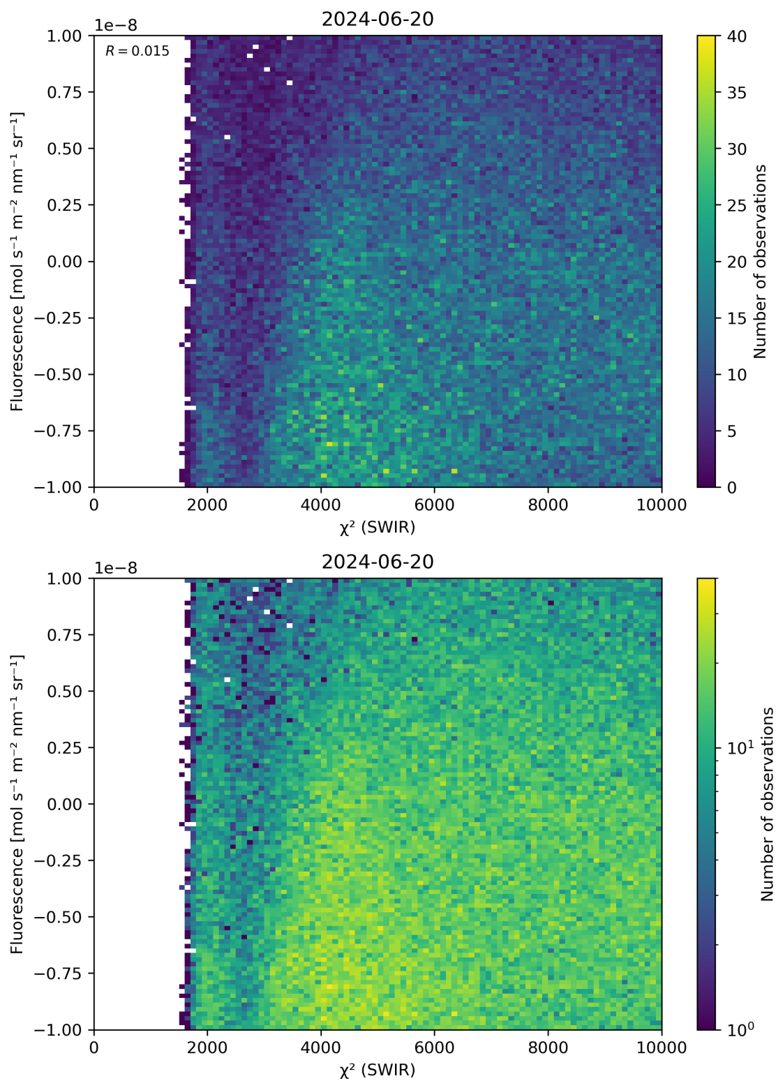
Figure 49: Scatter density plot of “ \chi^2 (SWIR)” against “Fluorescence” for 2024-06-19 to 2024-06-21.
