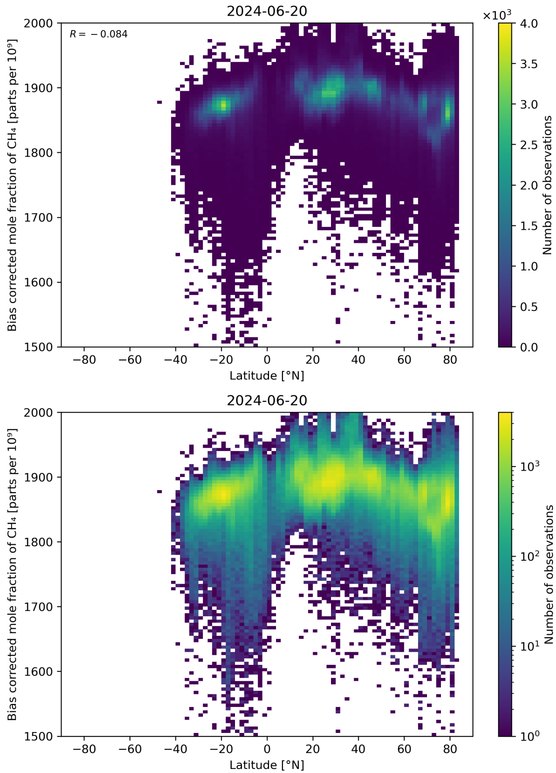
Figure 58: Scatter density plot of “Latitude” against “Bias corrected mole fraction of \text{CH}_4 ” for 2024-06-19 to 2024-06-21.
