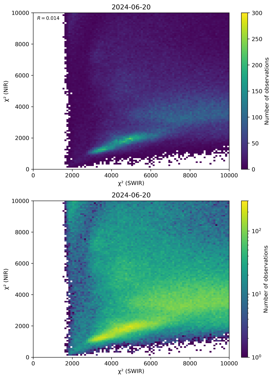
Figure 47: Scatter density plot of “ \chi^2 (SWIR)” against “ \chi^2 (NIR)” for 2024-06-19 to 2024-06-21.
