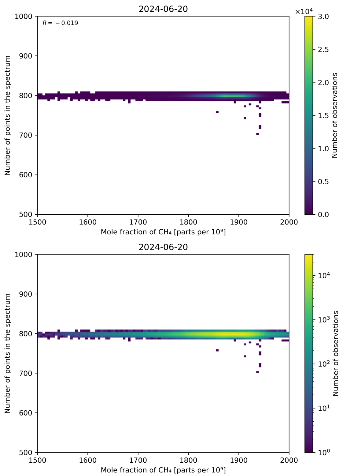
Figure 77: Scatter density plot of “Mole fraction of CH 4 ” against “Number of points in the spectrum” for 2024-06-19 to 2024-06-21.
