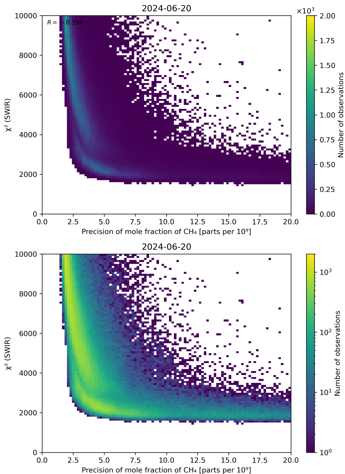
Figure 79: Scatter density plot of “Precision of mole fraction of CH 4 ” against “ \chi^2 (SWIR)” for 2024-06-19 to 2024-06-21.
