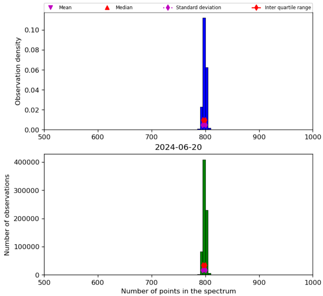
Figure 26: Histogram of “Number of points in the spectrum” for 2024-06-19 to 2024-06-21
