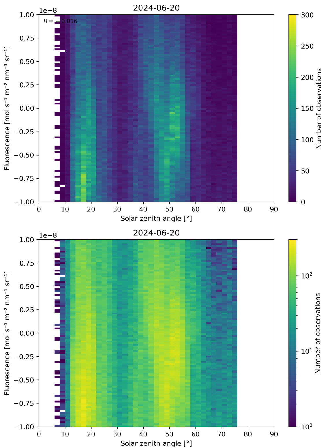
Figure 97: Scatter density plot of “Solar zenith angle” against “Fluorescence” for 2024-06-19 to 2024-06-21.
