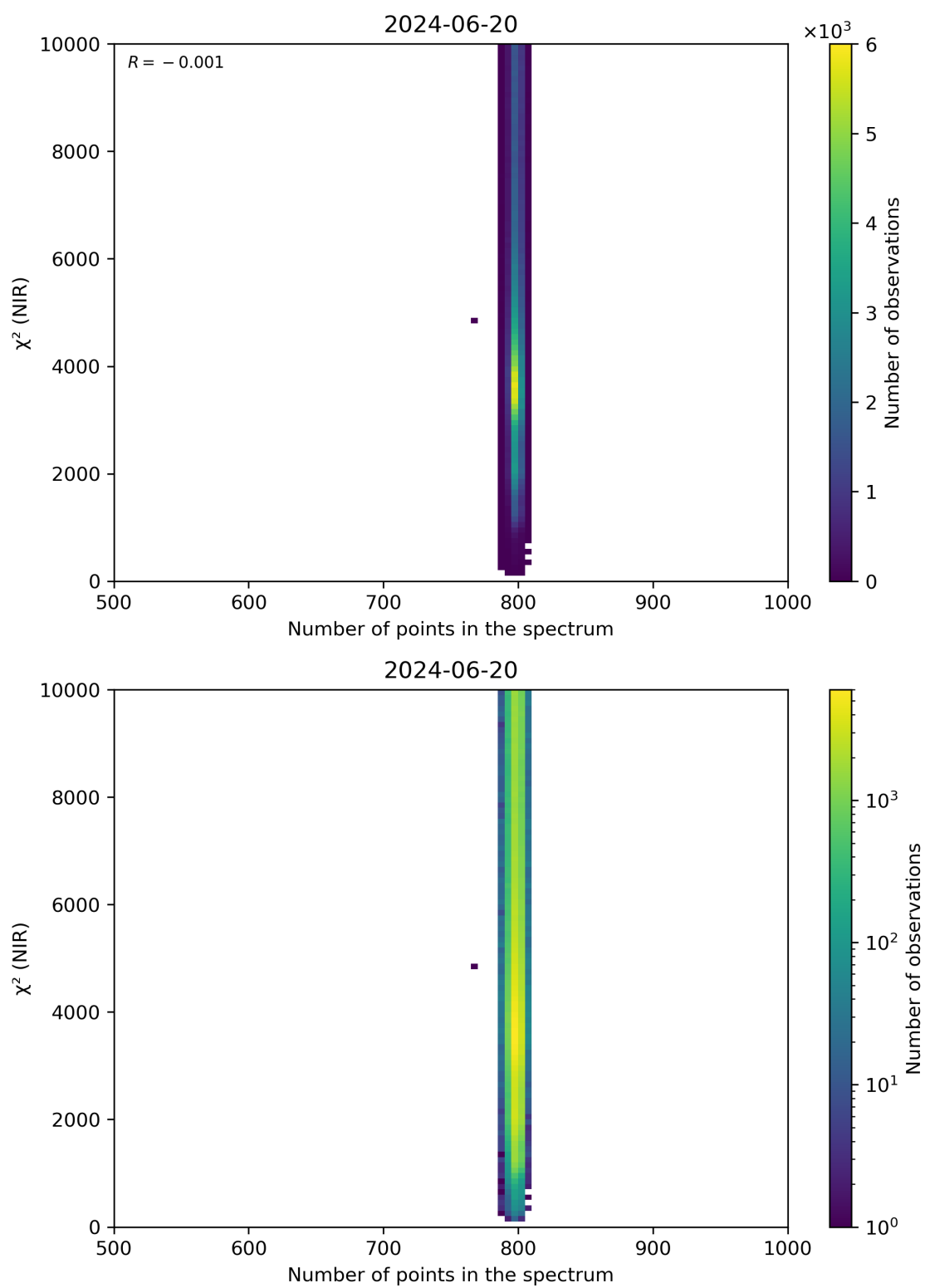
Figure 88: Scatter density plot of “Number of points in the spectrum” against “ \chi^2 (NIR)” for 2024-06-19 to 2024-06-21.
