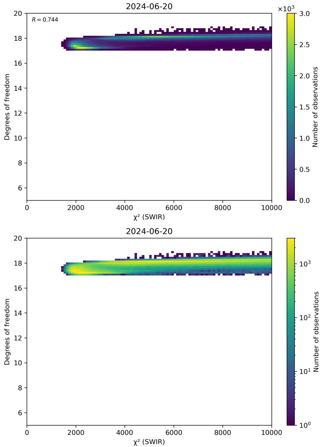
Figure 48: Scatter density plot of “ \chi^2 (SWIR)” against “Degrees of freedom” for 2024-06-19 to 2024-06-21.
