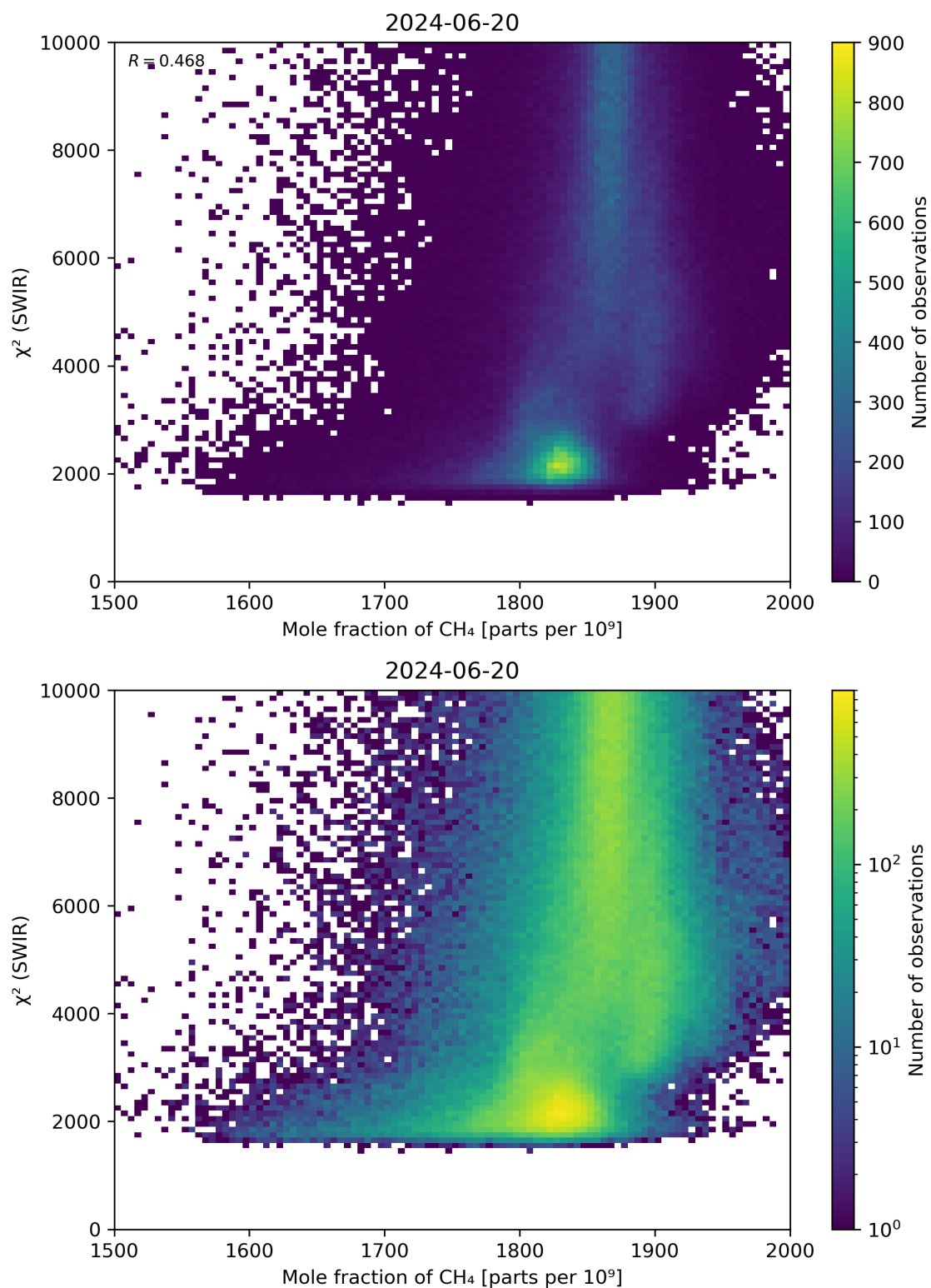
Figure 71: Scatter density plot of “Mole fraction of \text{CH}_4 ” against “ \chi^2 (SWIR)” for 2024-06-19 to 2024-06-21.
