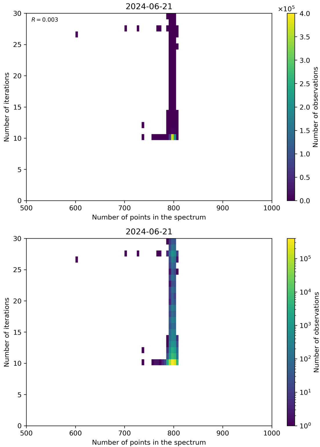
Figure 92: Scatter density plot of “Number of points in the spectrum” against “Number of iterations” for 2024-06-20 to 2024-06-22.
