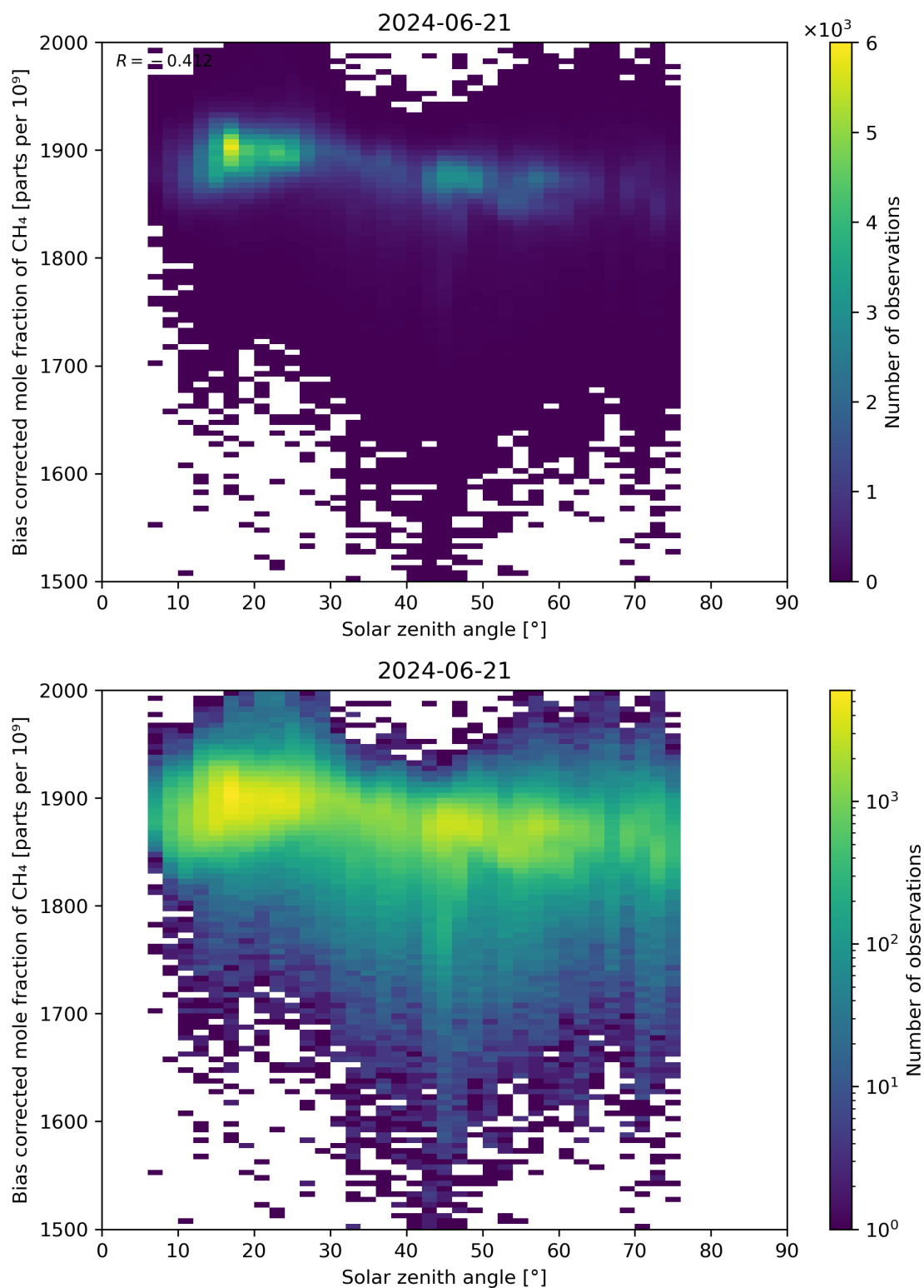
Figure 100: Scatter density plot of “Solar zenith angle” against “Bias corrected mole fraction of CH 4 ” for 2024-06-20 to 2024-06-22.
