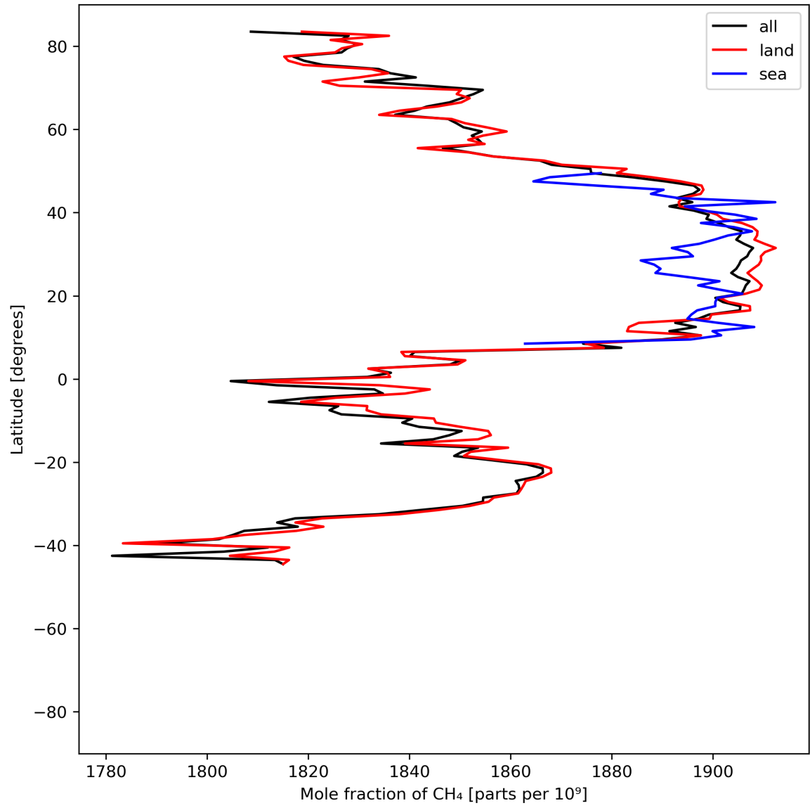
Figure 12: Zonal average of “Mole fraction of \text{CH}_4 ” for 2024-06-20 to 2024-06-22.
