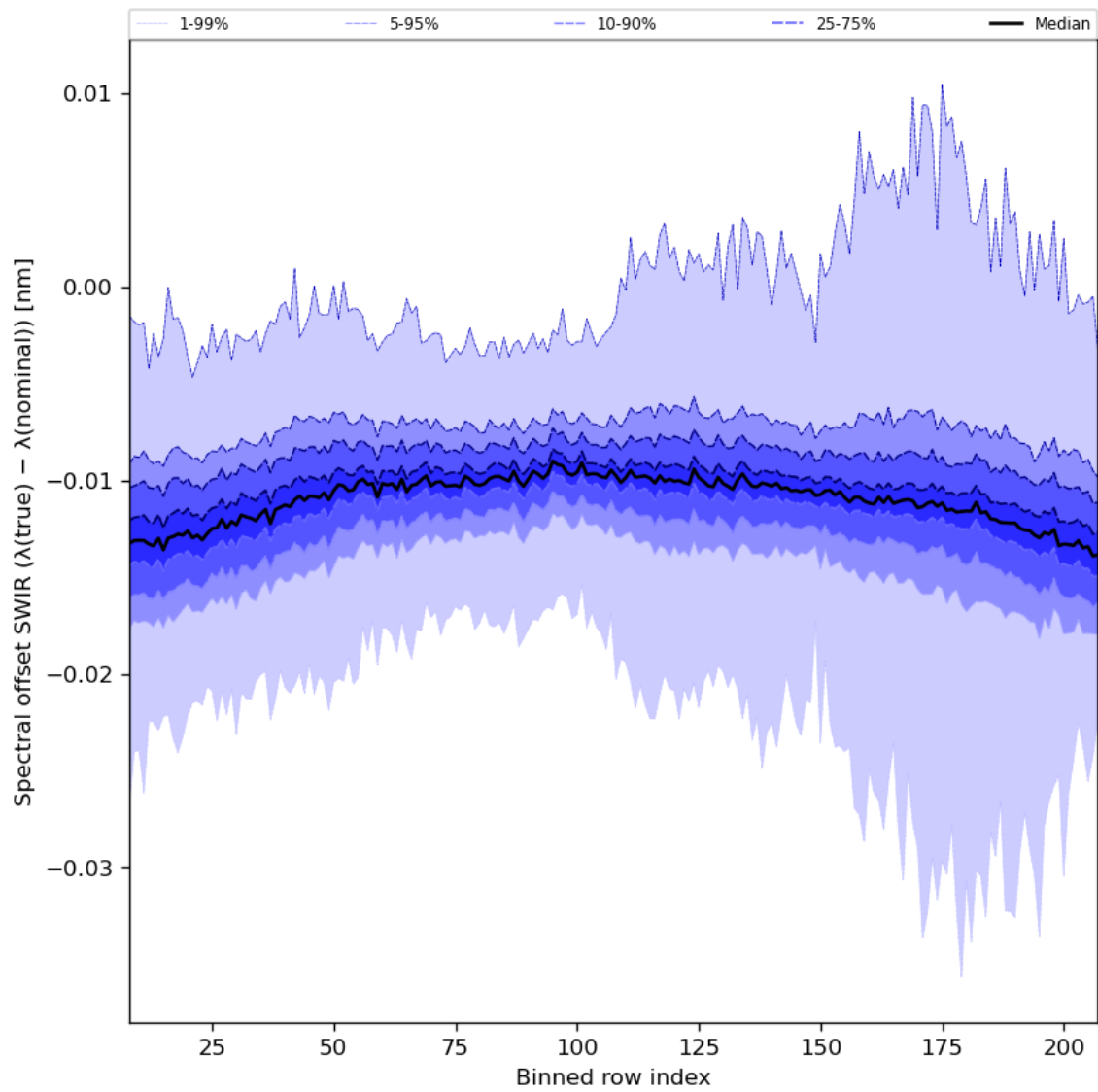
Figure 38: Along track statistics of “Spectral offset SWIR ( \lambda(\text{true}) - \lambda(\text{nominal}) )” for 2024-06-20 to 2024-06-22
