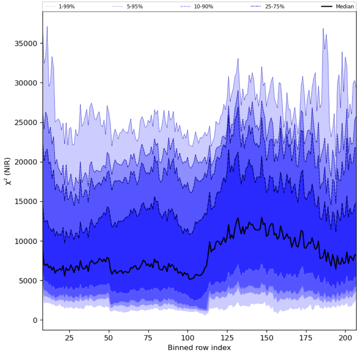
Figure 40: Along track statistics of “ \chi^2 (NIR)” for 2024-06-20 to 2024-06-22
