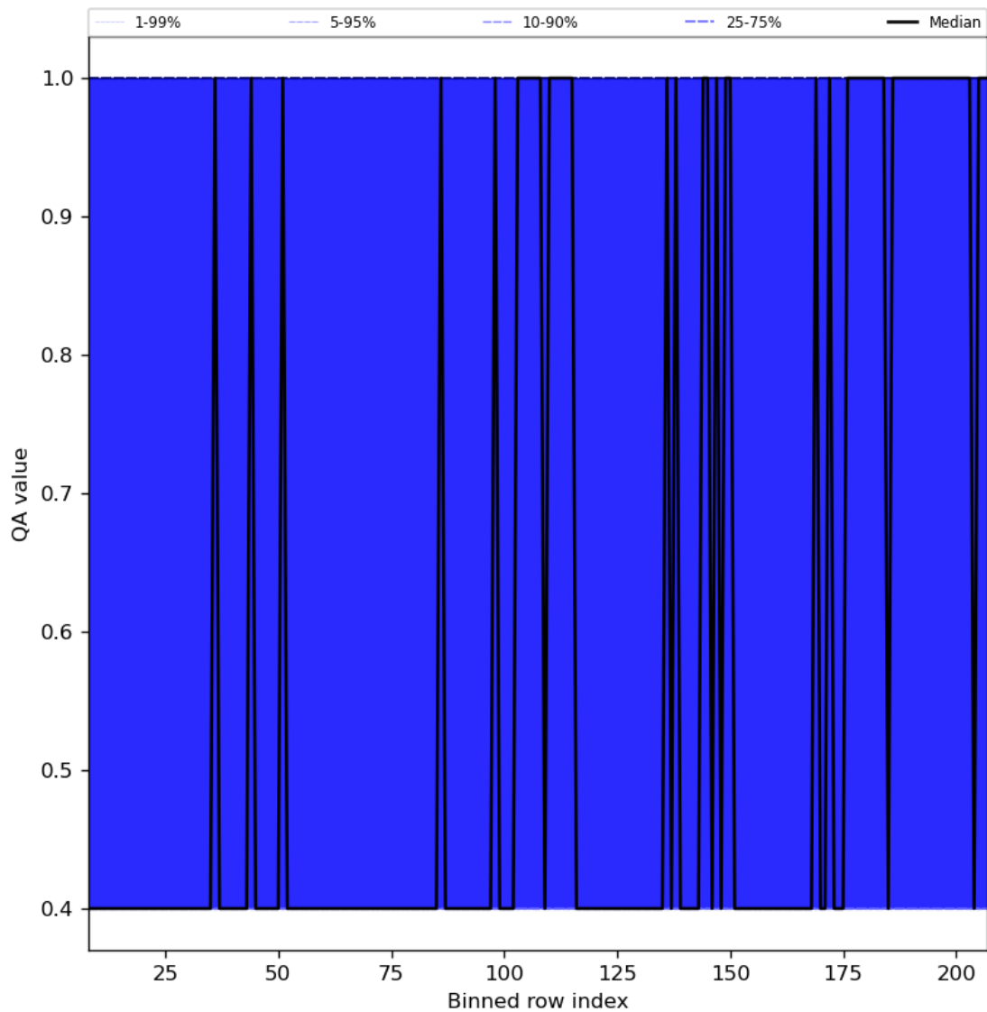
Figure 33: Along track statistics of “QA value” for 2024-06-20 to 2024-06-22
