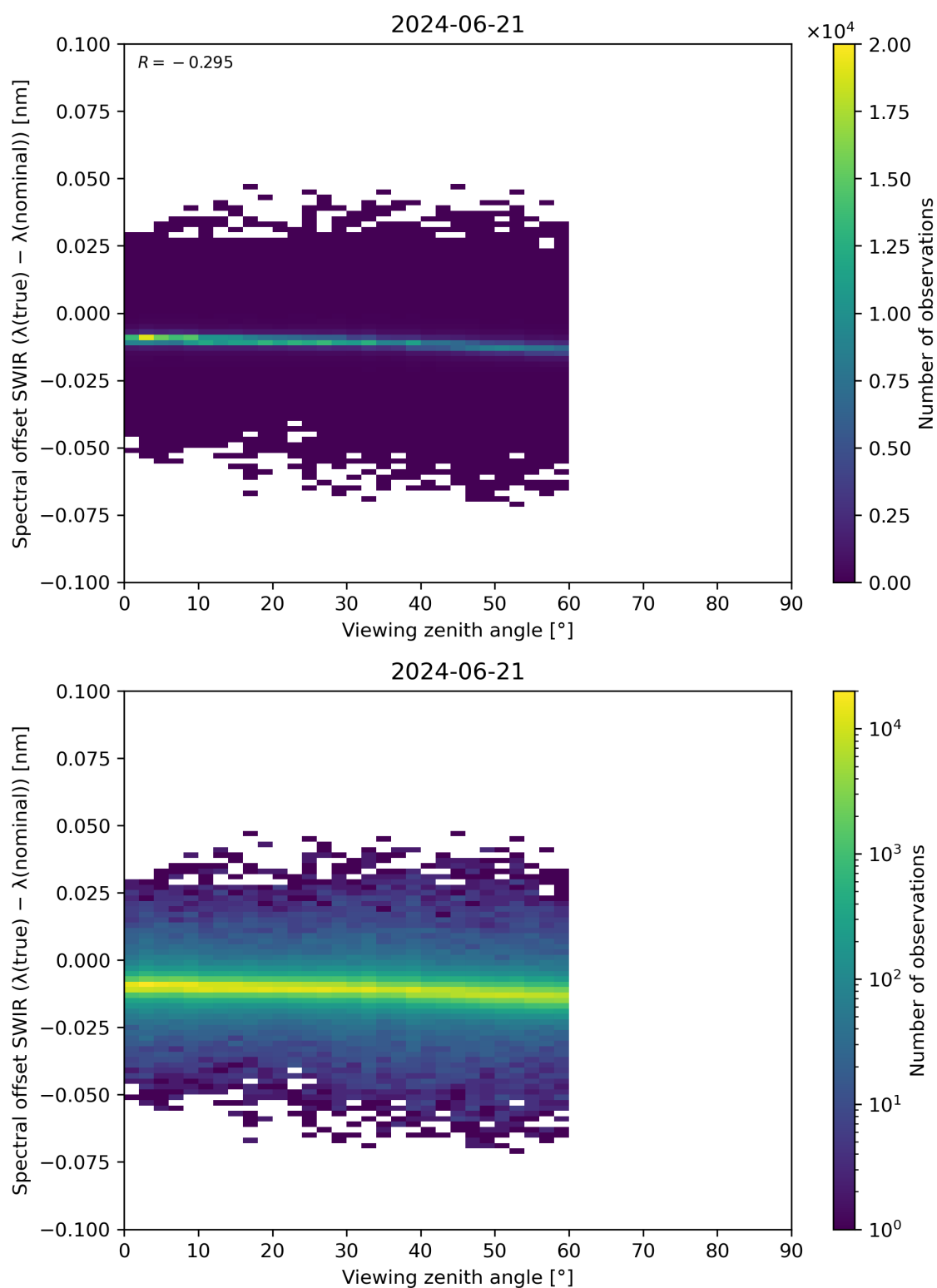
Figure 116: Scatter density plot of “Viewing zenith angle” against “Spectral offset SWIR ( \lambda(\text{true}) - \lambda(\text{nominal}) )” for 2024-06-20 to 2024-06-22.
