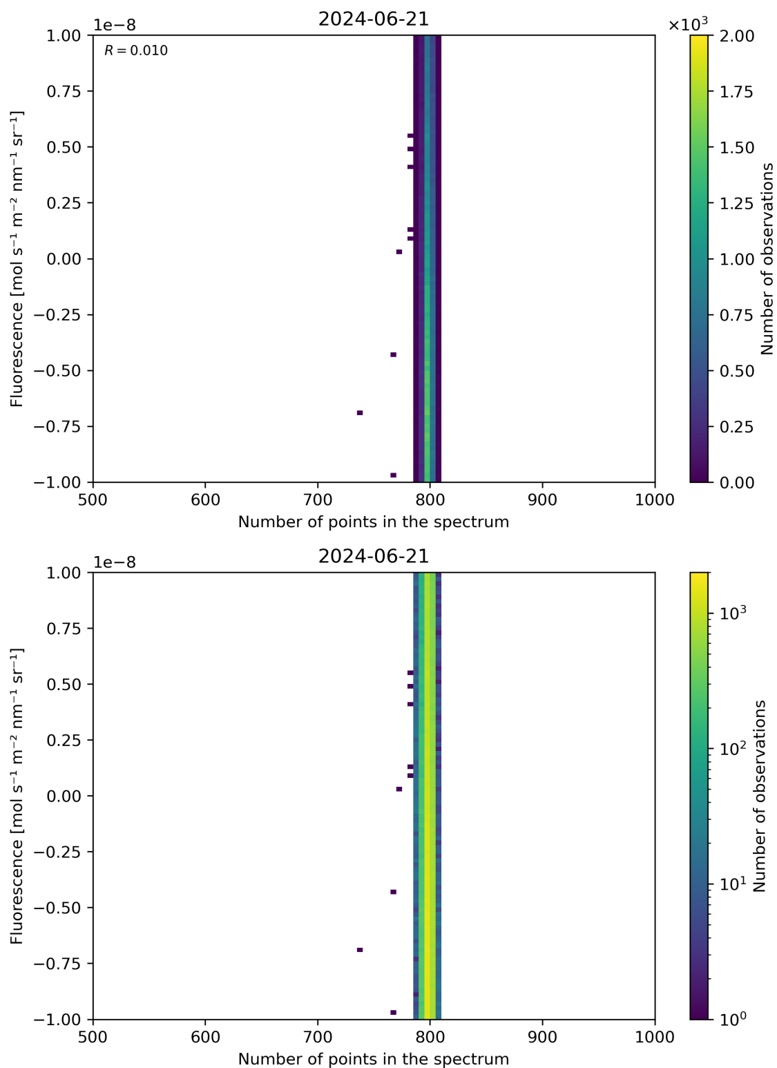
Figure 91: Scatter density plot of “Number of points in the spectrum” against “Fluorescence” for 2024-06-20 to 2024-06-22.
