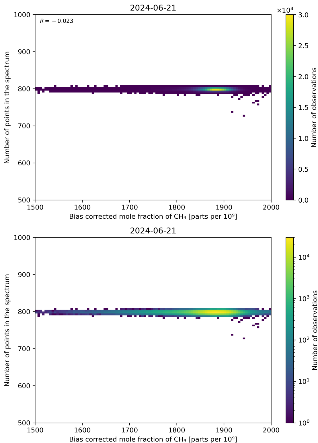
Figure 68: Scatter density plot of “Bias corrected mole fraction of CH 4 ” against “Number of points in the spectrum” for 2024-06-20 to 2024-06-22.
