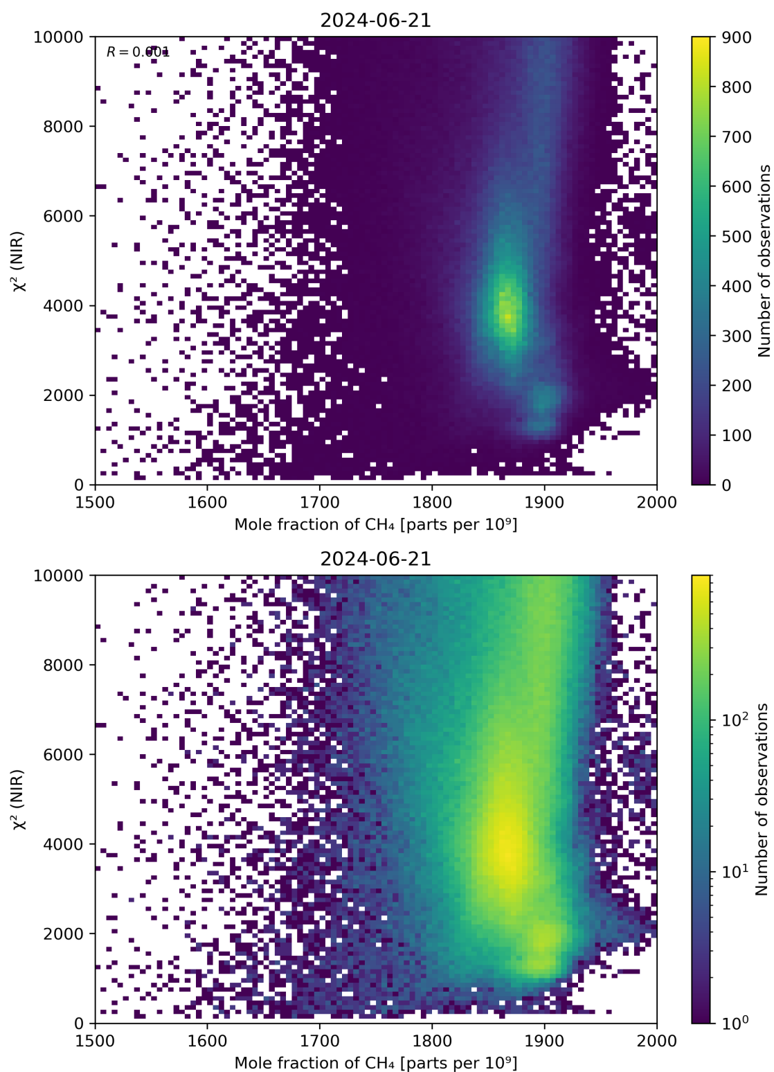
Figure 70: Scatter density plot of “Mole fraction of \text{CH}_4 ” against “ \chi^2 (NIR)” for 2024-06-20 to 2024-06-22.
