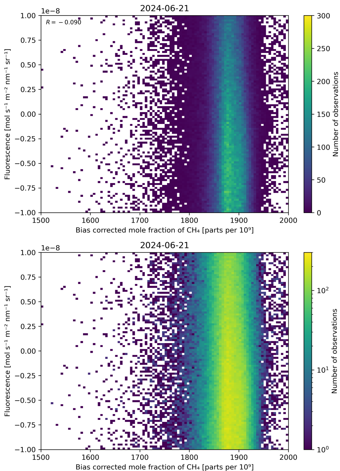
Figure 66: Scatter density plot of “Bias corrected mole fraction of \text{CH}_4 ” against “Fluorescence” for 2024-06-20 to 2024-06-22.
