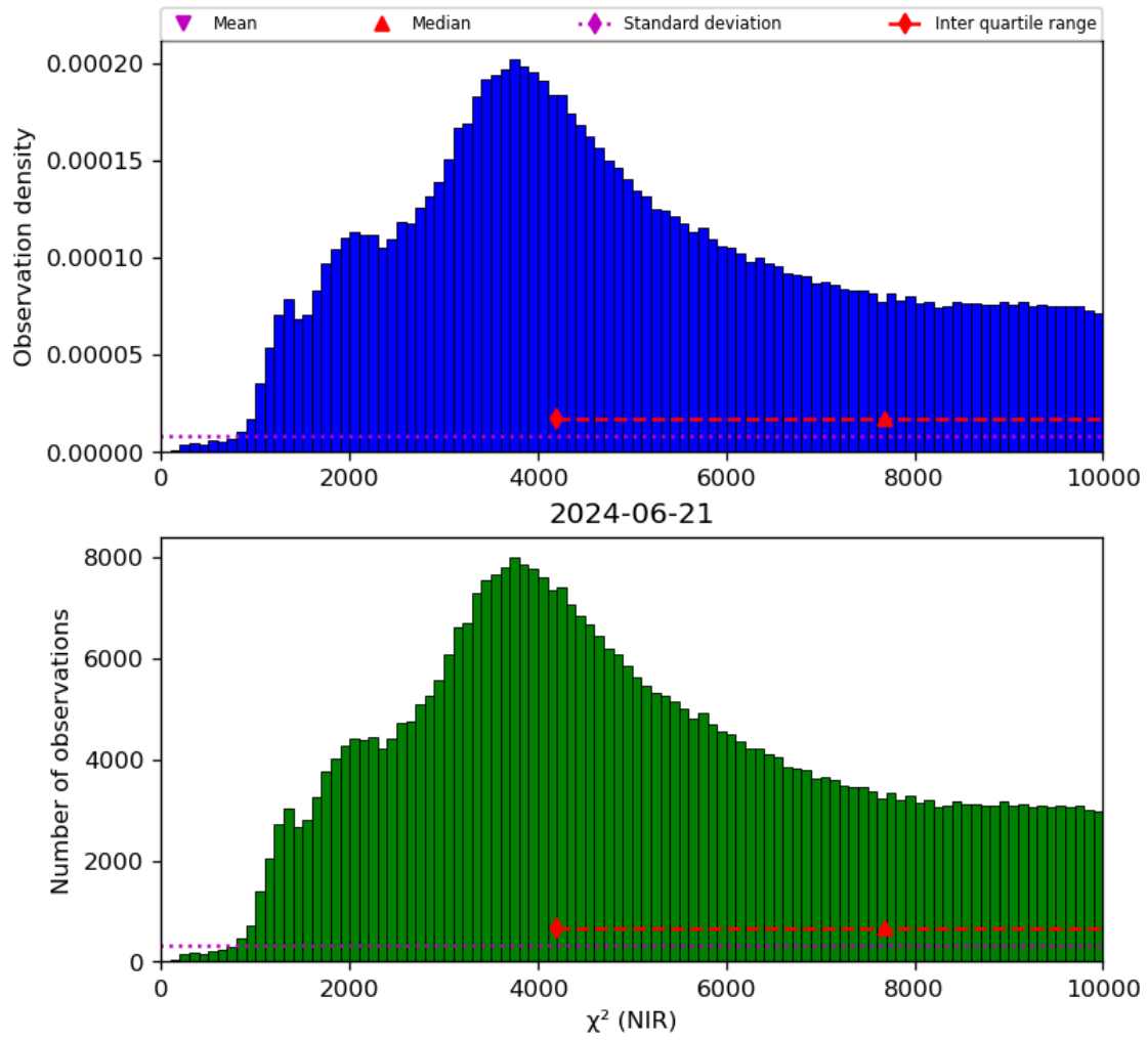
Figure 29: Histogram of “ \chi^2 (NIR)” for 2024-06-20 to 2024-06-22
