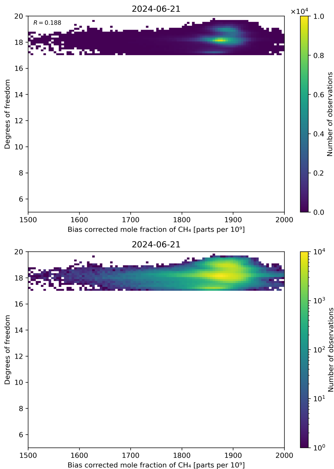
Figure 65: Scatter density plot of “Bias corrected mole fraction of CH 4 ” against “Degrees of freedom” for 2024-06-20 to 2024-06-22.
