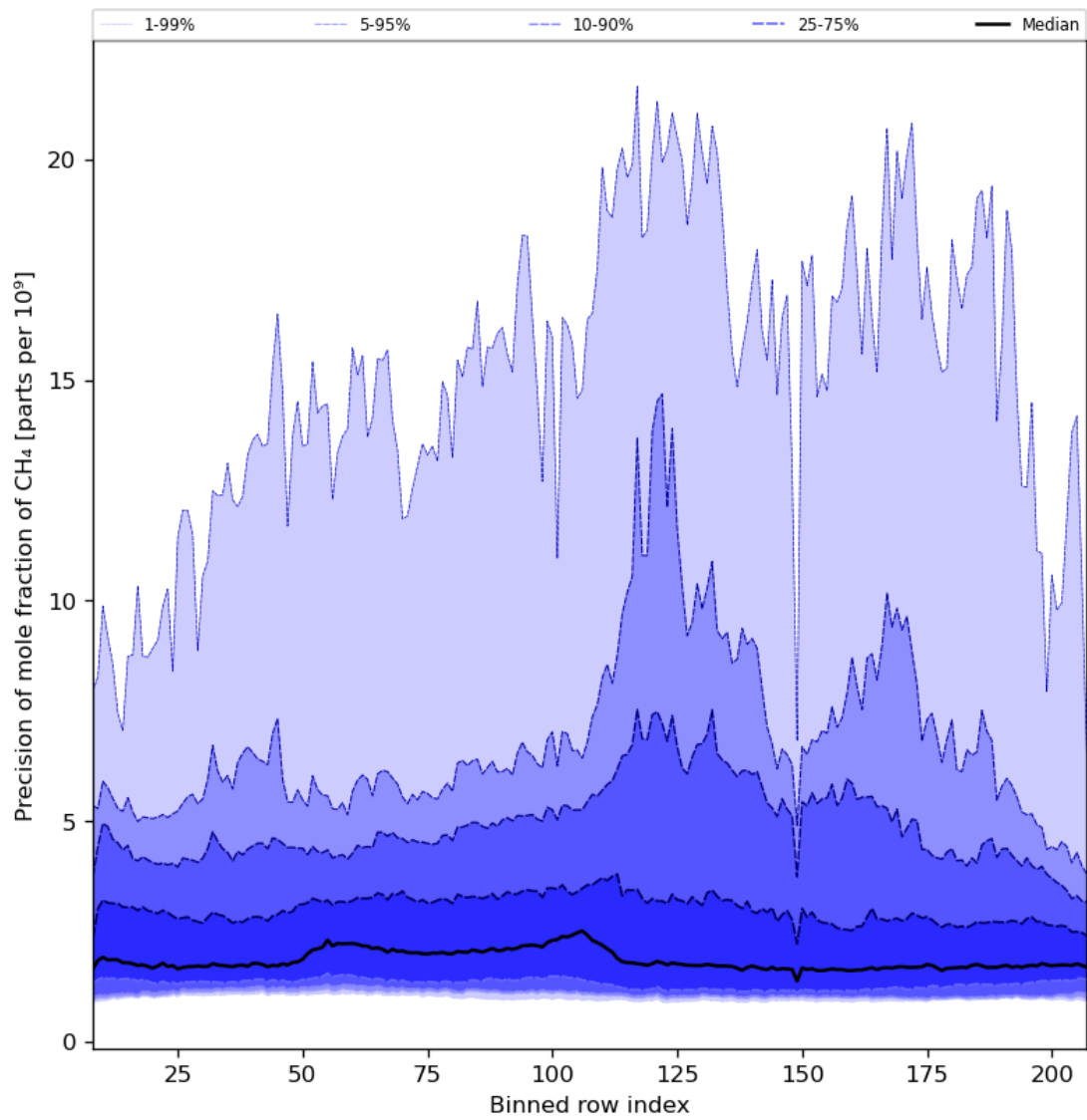
Figure 35: Along track statistics of “Precision of mole fraction of CH 4 ” for 2024-06-20 to 2024-06-22
