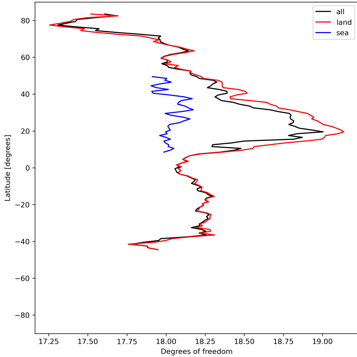
Figure 19: Zonal average of “Degrees of freedom” for 2024-06-20 to 2024-06-22.
