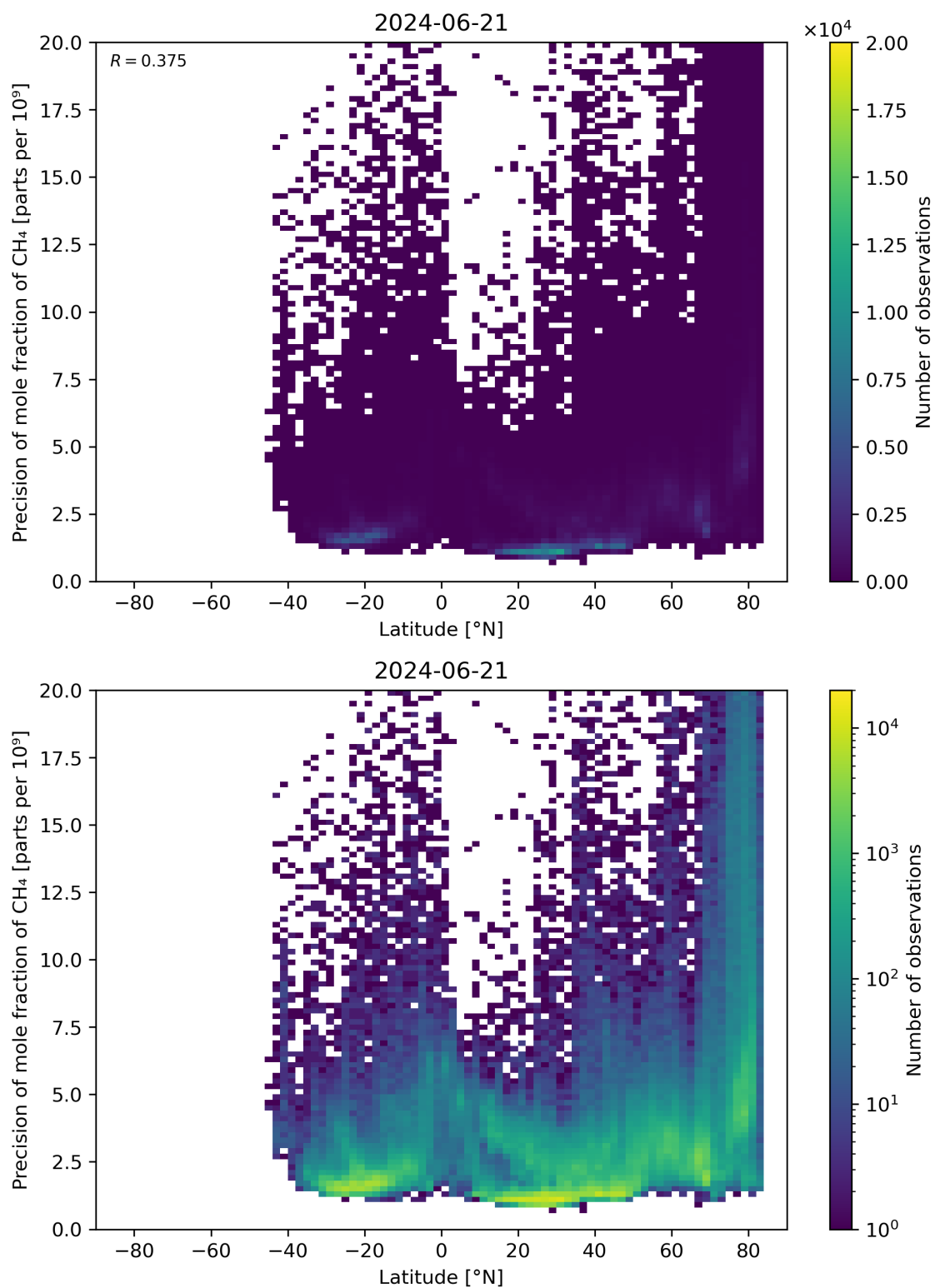
Figure 59: Scatter density plot of “Latitude” against “Precision of mole fraction of \text{CH}_4 ” for 2024-06-20 to 2024-06-22.
