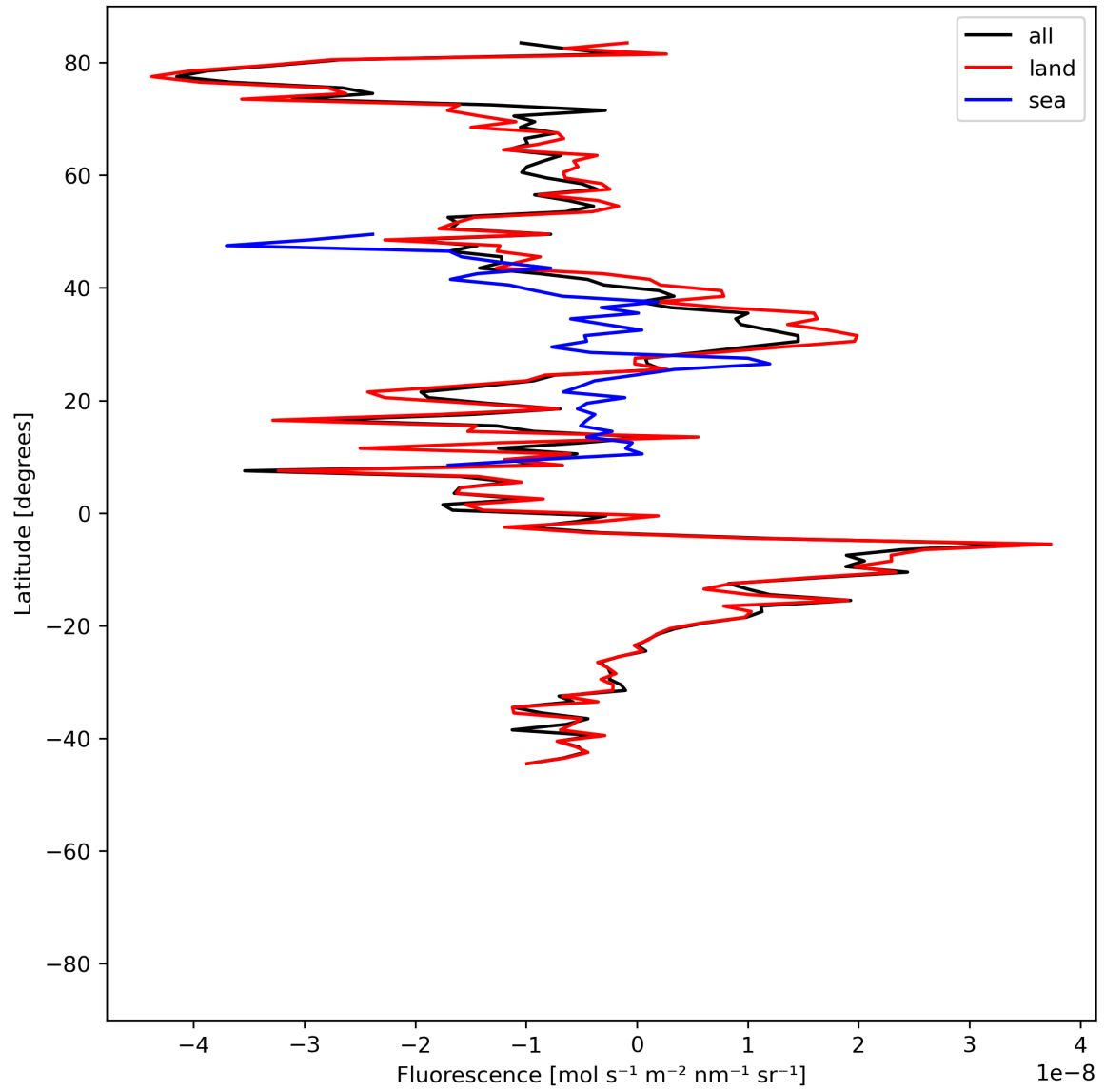
Figure 21: Zonal average of “Fluorescence” for 2024-06-20 to 2024-06-22.
