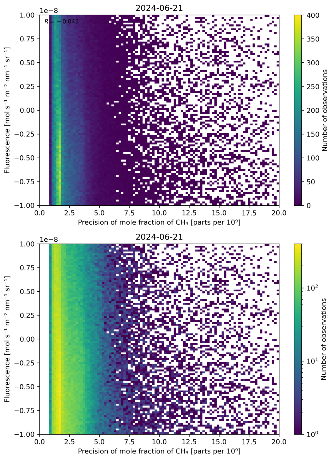
Figure 81: Scatter density plot of “Precision of mole fraction of \text{CH}_4 ” against “Fluorescence” for 2024-06-20 to 2024-06-22.
