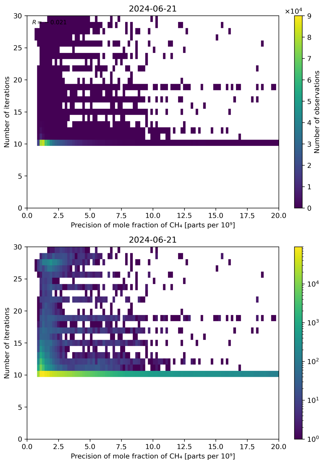
Figure 83: Scatter density plot of “Precision of mole fraction of CH 4 ” against “Number of iterations” for 2024-06-20 to 2024-06-22.
