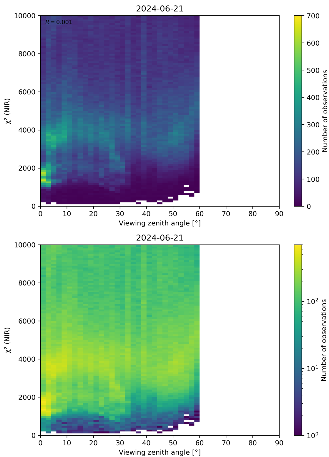
Figure 105: Scatter density plot of “Viewing zenith angle” against “ \chi^2 (NIR)” for 2024-06-20 to 2024-06-22.
