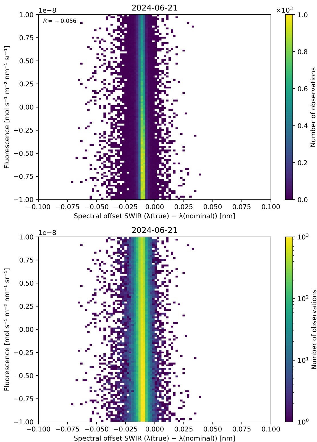
Figure 120: Scatter density plot of “Spectral offset SWIR ( \lambda(\text{true}) - \lambda(\text{nominal}) )” against “Fluorescence” for 2024-06-20 to 2024-06-22.
