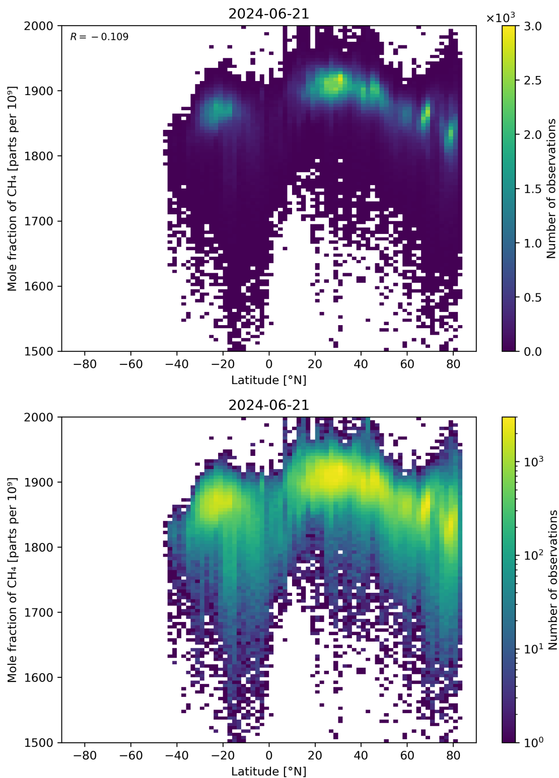
Figure 57: Scatter density plot of “Latitude” against “Mole fraction of CH 4 ” for 2024-06-20 to 2024-06-22.
