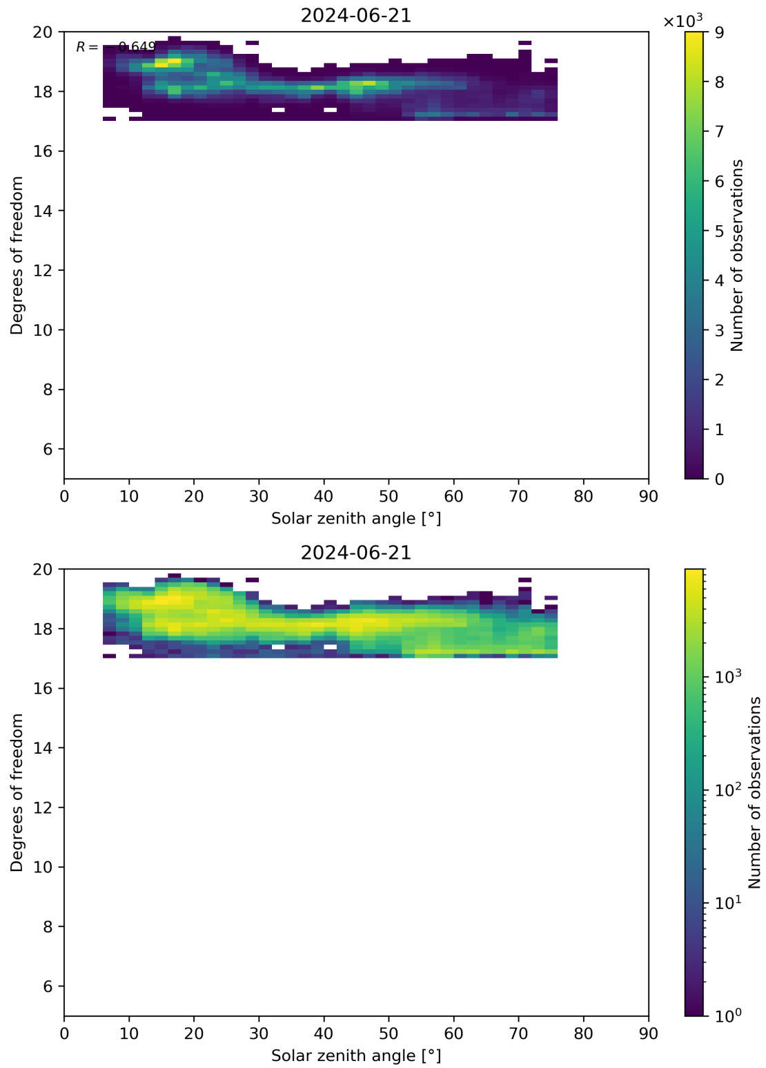
Figure 96: Scatter density plot of “Solar zenith angle” against “Degrees of freedom” for 2024-06-20 to 2024-06-22.
