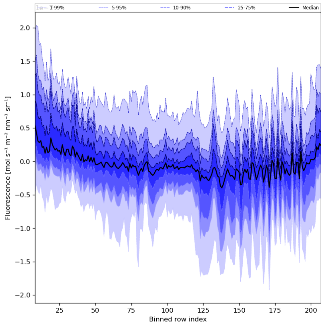
Figure 43: Along track statistics of “Fluorescence” for 2024-06-20 to 2024-06-22
