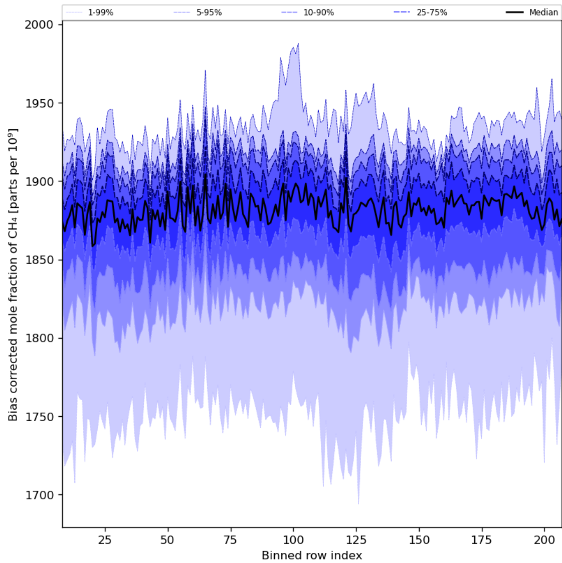
Figure 36: Along track statistics of “Bias corrected mole fraction of CH 4 ” for 2024-06-20 to 2024-06-22
