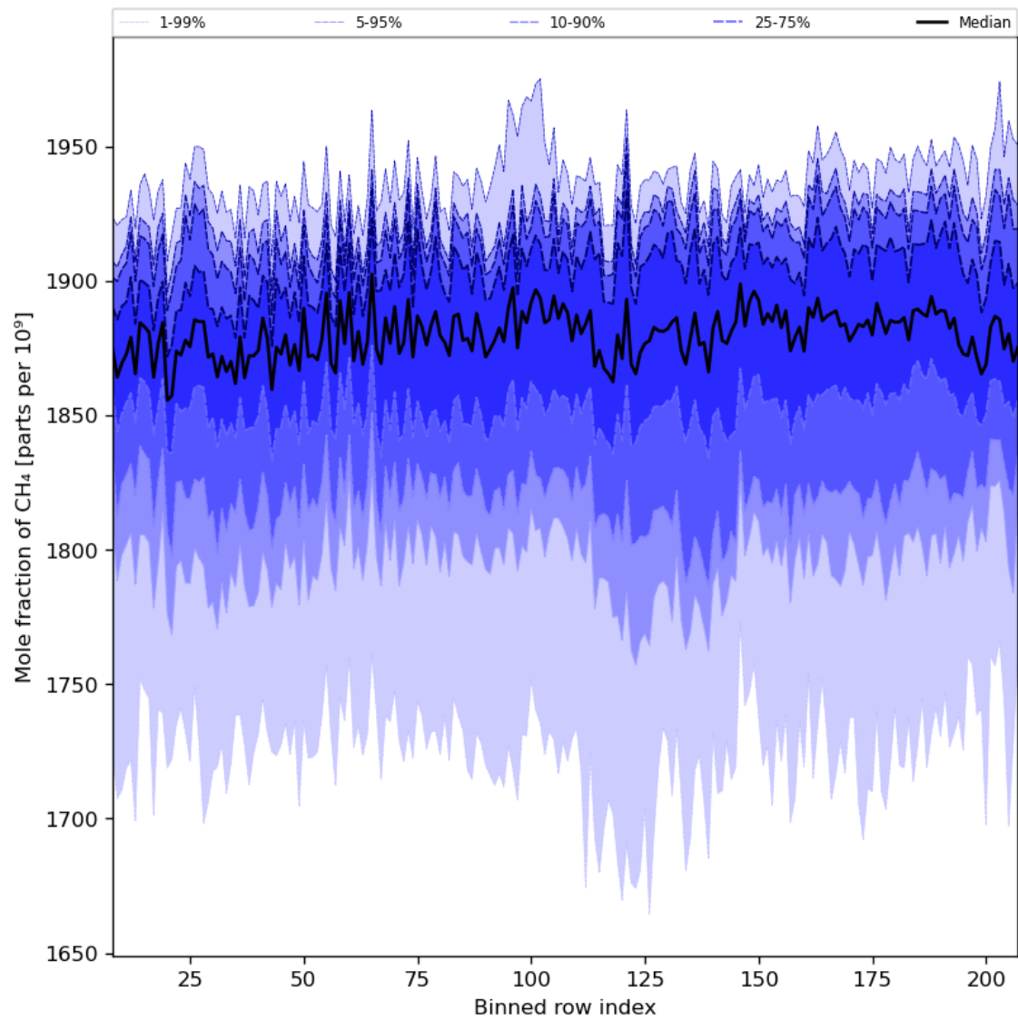
Figure 34: Along track statistics of “Mole fraction of CH 4 ” for 2024-06-20 to 2024-06-22
