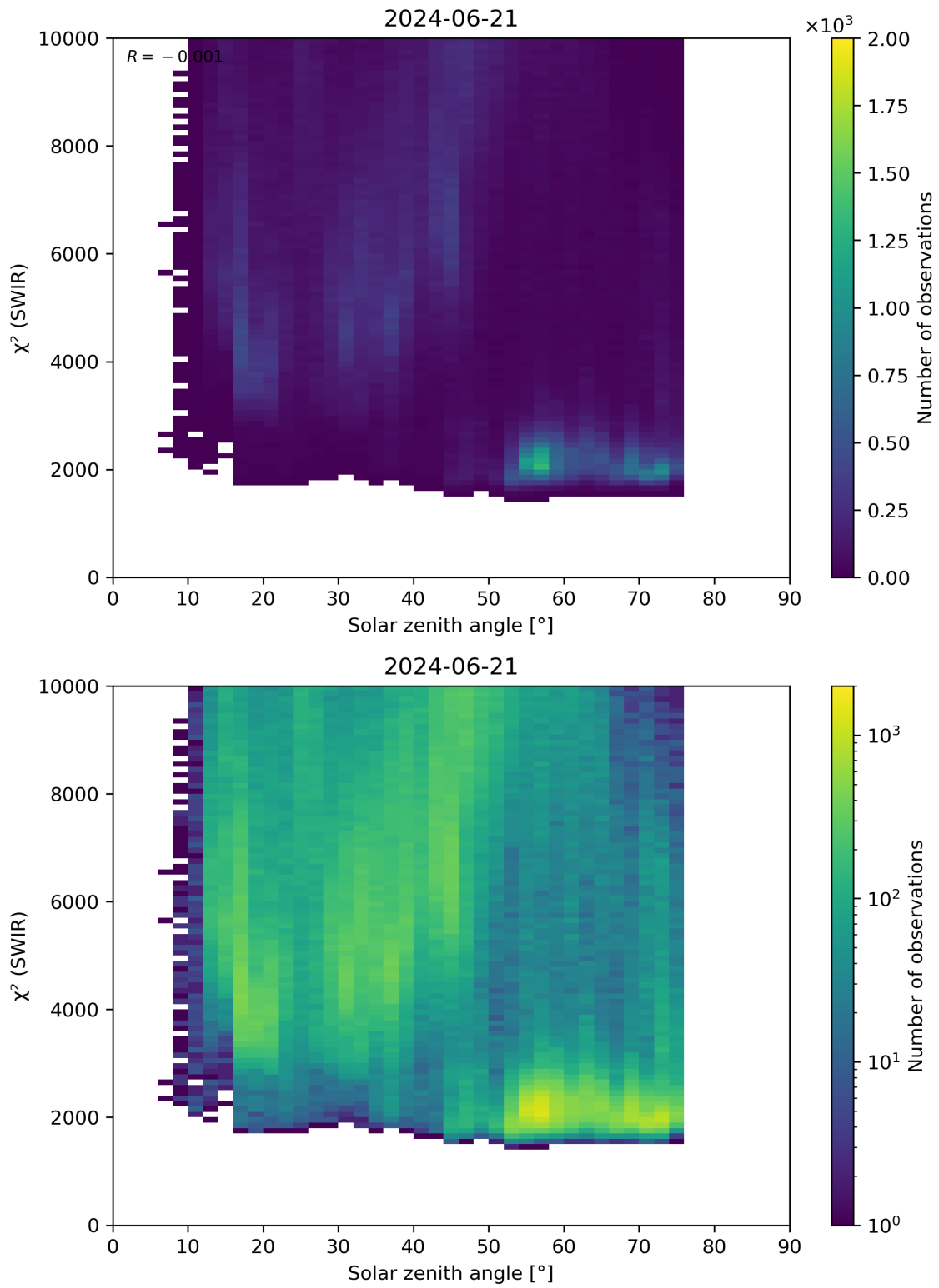
Figure 95: Scatter density plot of “Solar zenith angle” against “ \chi^2 (SWIR)” for 2024-06-20 to 2024-06-22.
