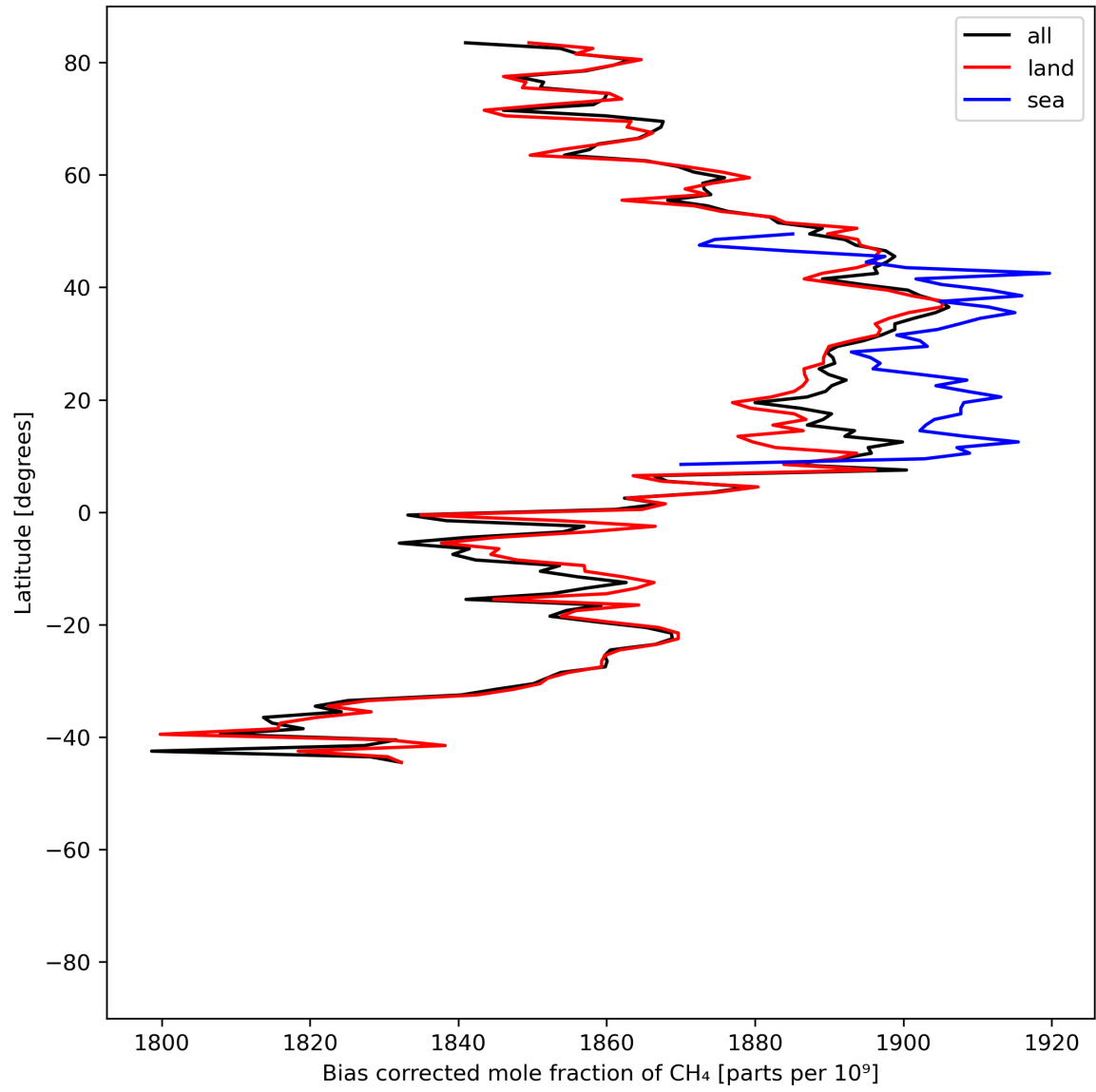
Figure 14: Zonal average of “Bias corrected mole fraction of CH 4 ” for 2024-06-20 to 2024-06-22.
