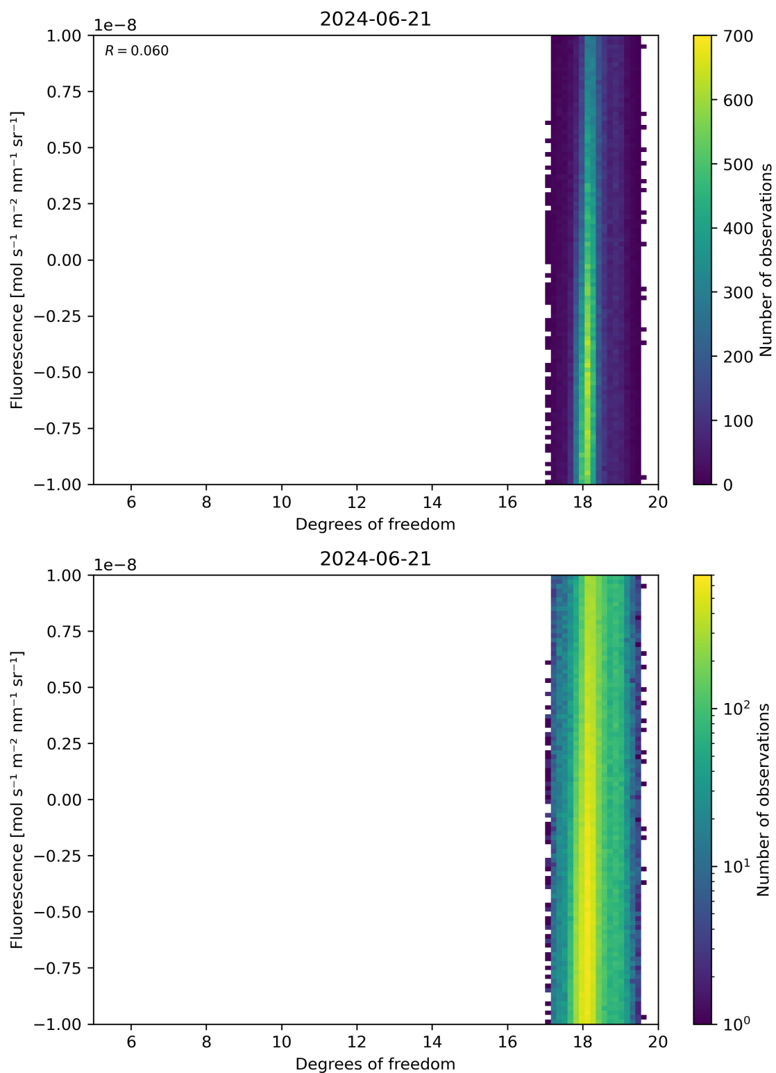
Figure 51: Scatter density plot of “Degrees of freedom” against “Fluorescence” for 2024-06-20 to 2024-06-22.
