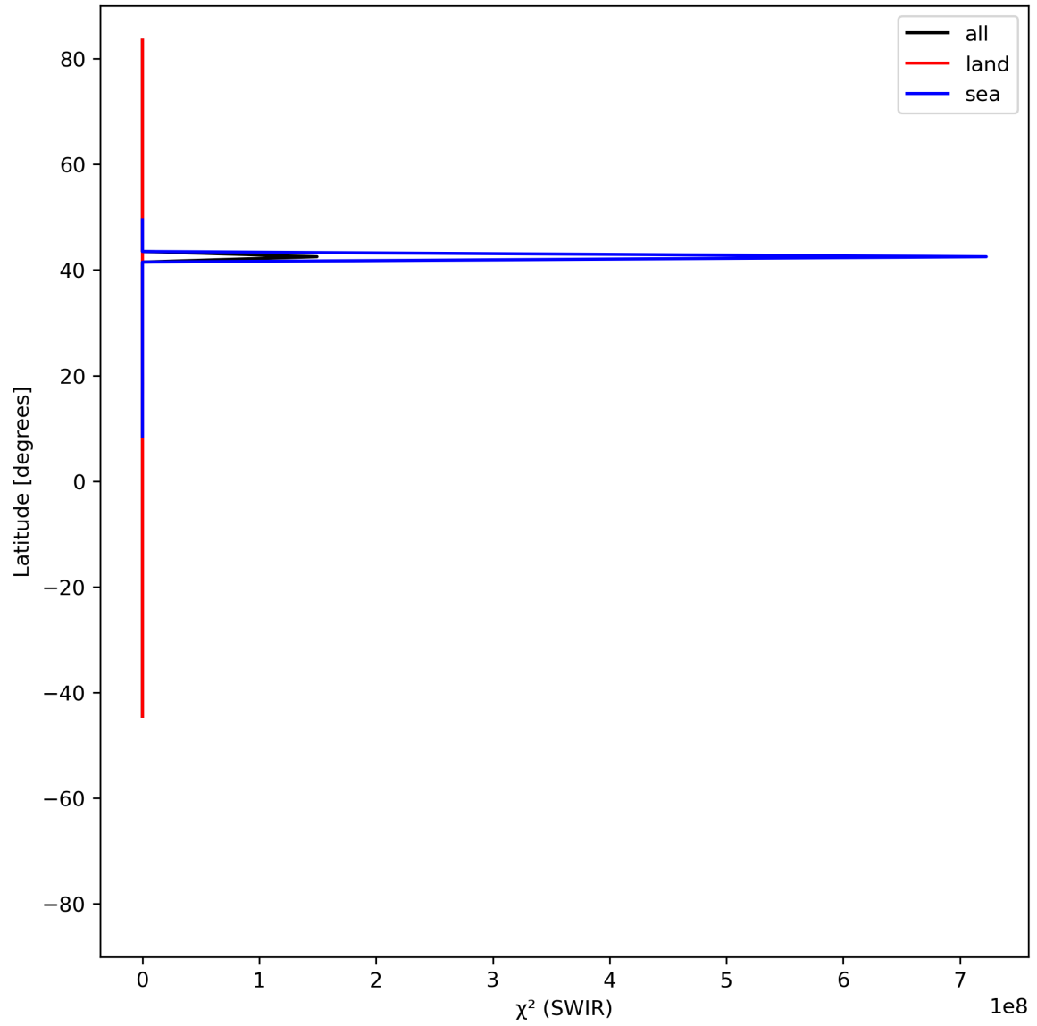
Figure 17: Zonal average of “ \chi^2 (SWIR)” for 2024-06-20 to 2024-06-22.
