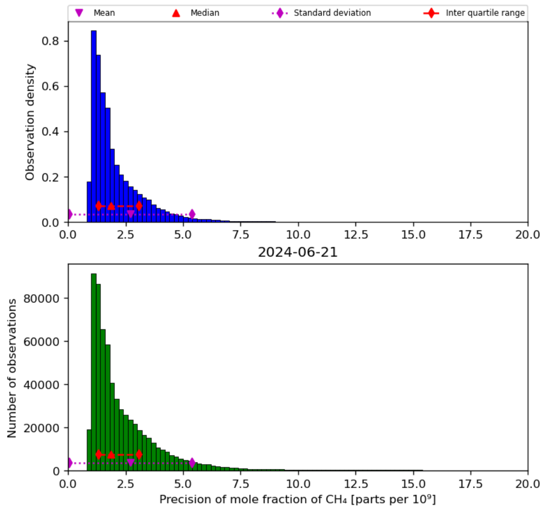
Figure 24: Histogram of “Precision of mole fraction of CH 4 ” for 2024-06-20 to 2024-06-22
