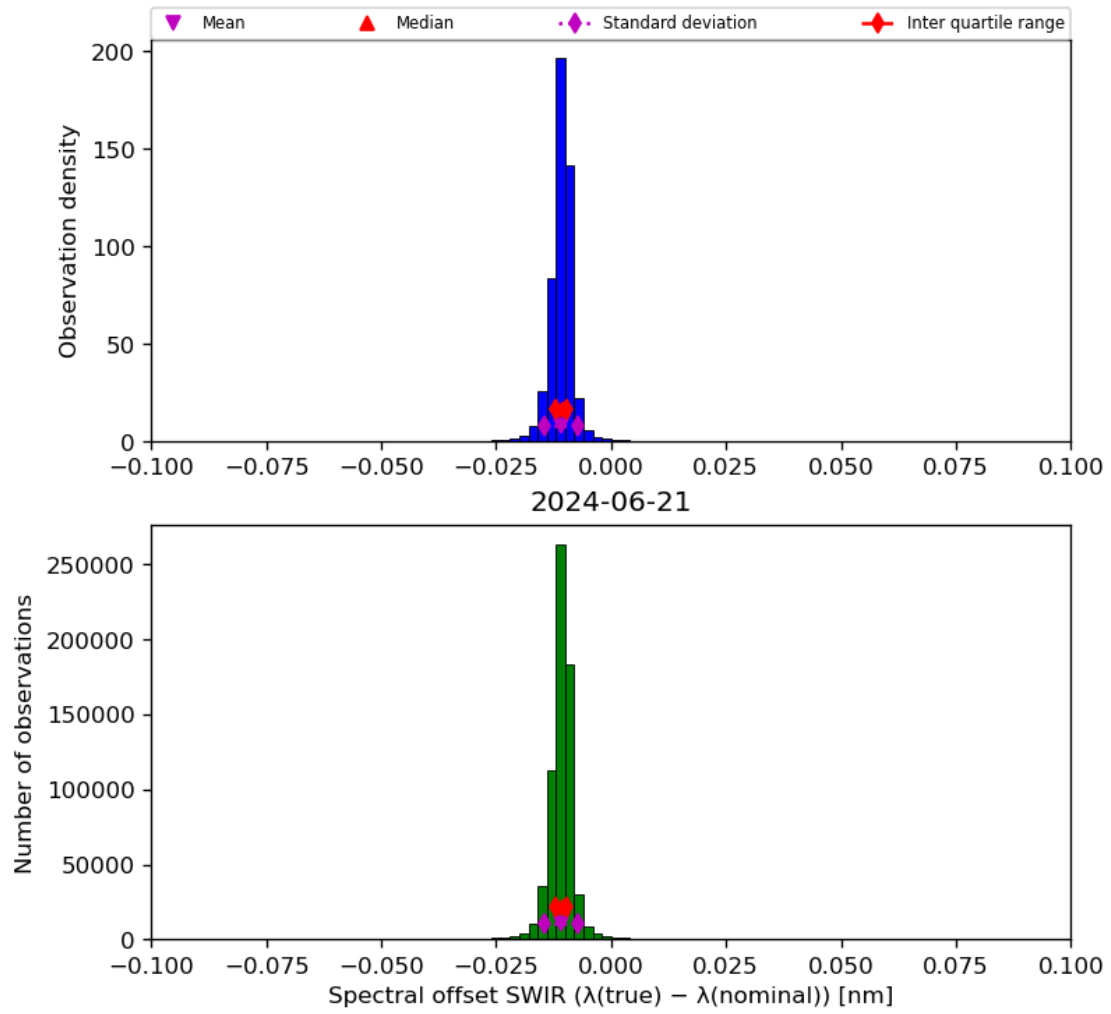
Figure 27: Histogram of “Spectral offset SWIR ( \lambda(\text{true}) - \lambda(\text{nominal}) )” for 2024-06-20 to 2024-06-22
