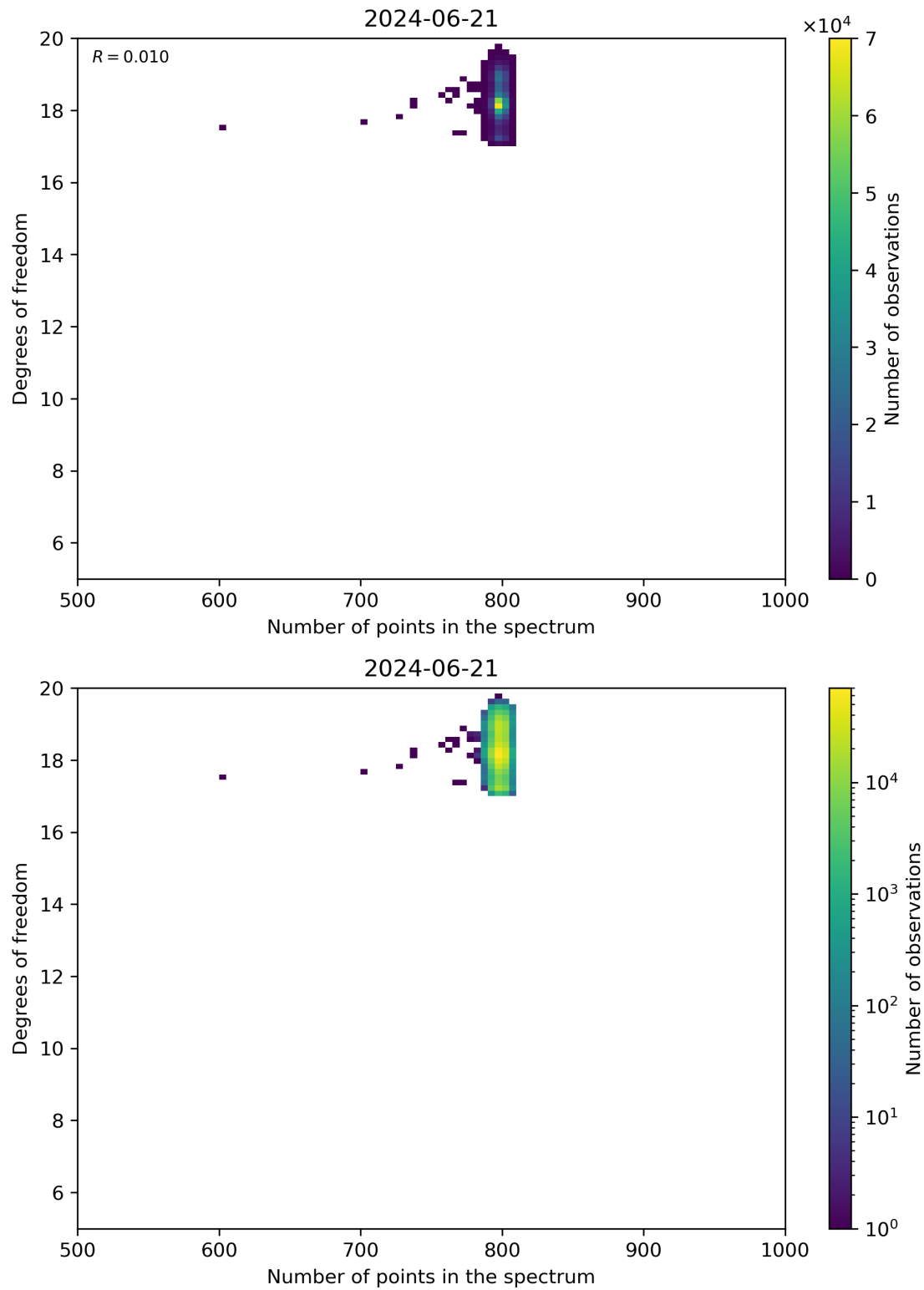
Figure 90: Scatter density plot of “Number of points in the spectrum” against “Degrees of freedom” for 2024-06-20 to 2024-06-22.
