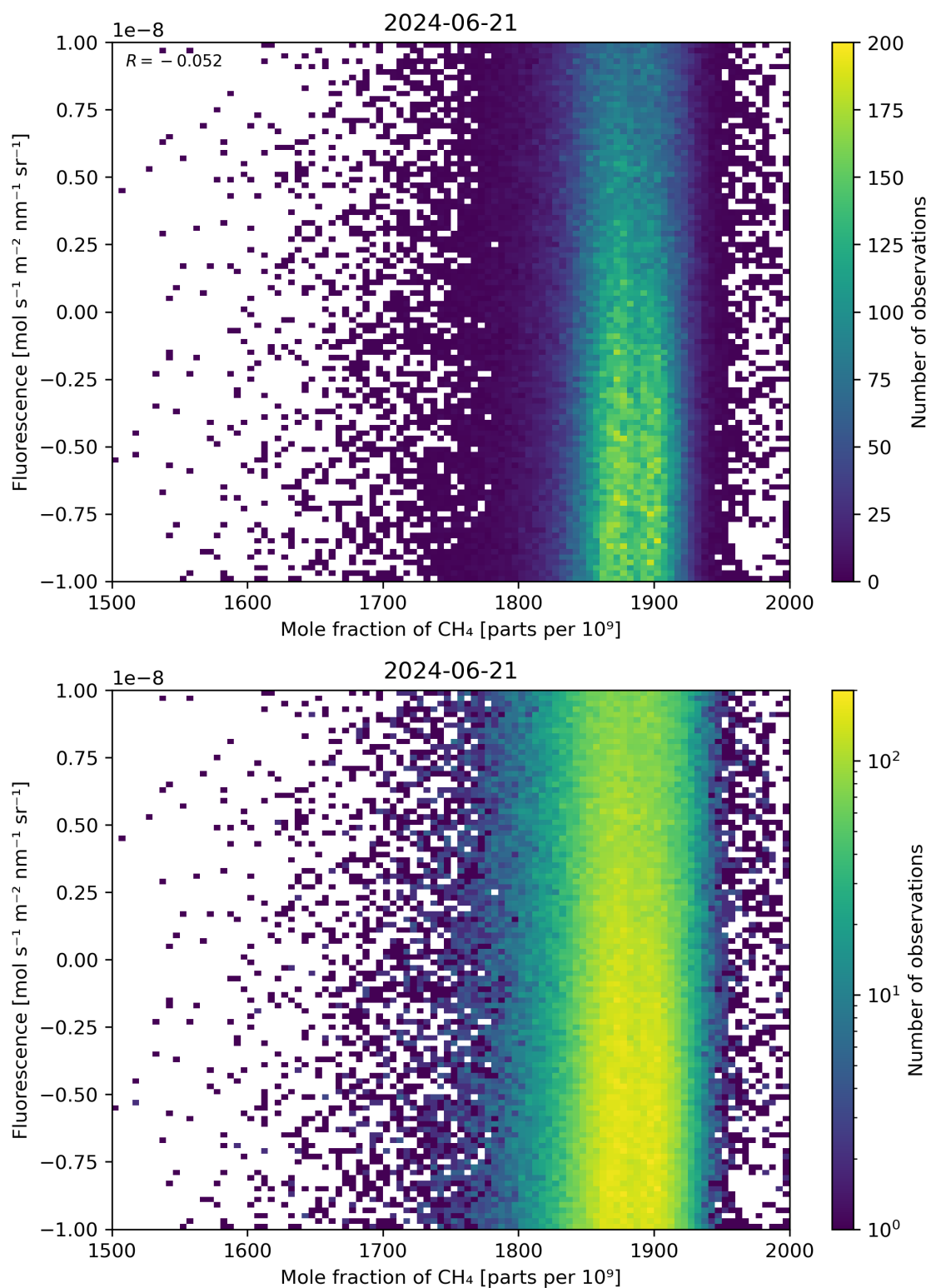
Figure 73: Scatter density plot of “Mole fraction of \text{CH}_4 ” against “Fluorescence” for 2024-06-20 to 2024-06-22.
