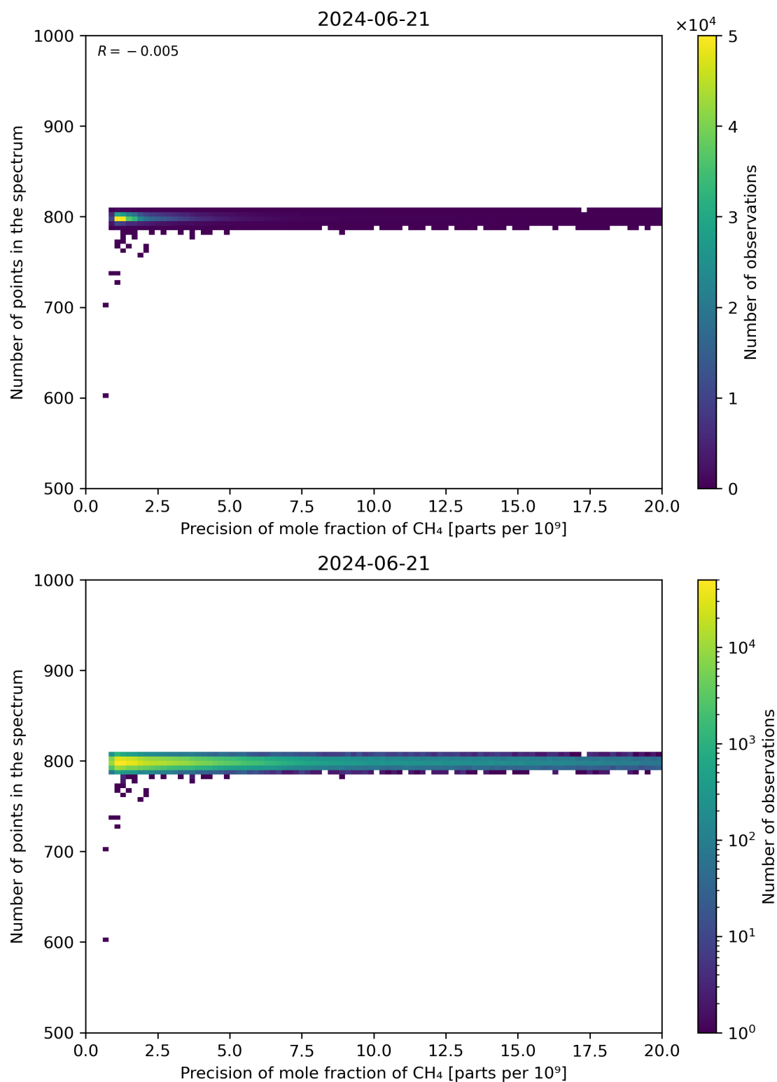
Figure 84: Scatter density plot of “Precision of mole fraction of CH 4 ” against “Number of points in the spectrum” for 2024-06-20 to 2024-06-22.
