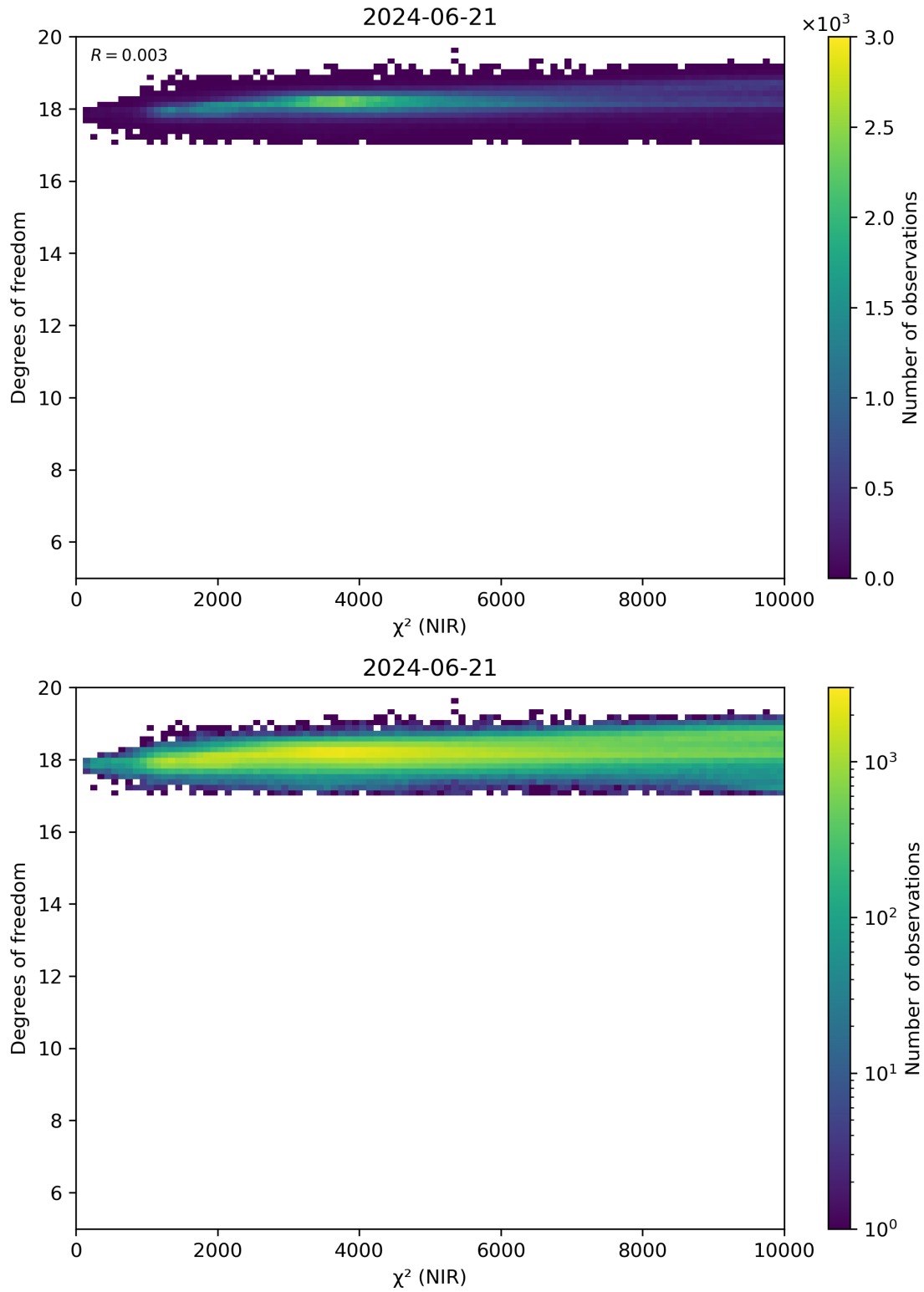
Figure 44: Scatter density plot of “ \chi^2 (NIR)” against “Degrees of freedom” for 2024-06-20 to 2024-06-22.
