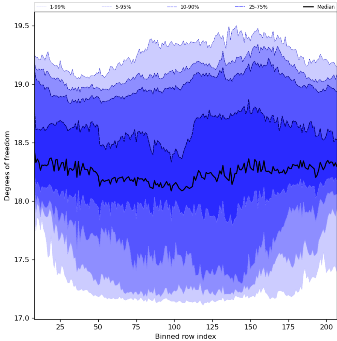
Figure 41: Along track statistics of “Degrees of freedom” for 2024-06-20 to 2024-06-22
