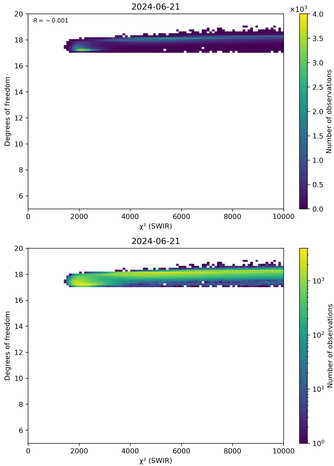
Figure 48: Scatter density plot of “ \chi^2 (SWIR)” against “Degrees of freedom” for 2024-06-20 to 2024-06-22.
