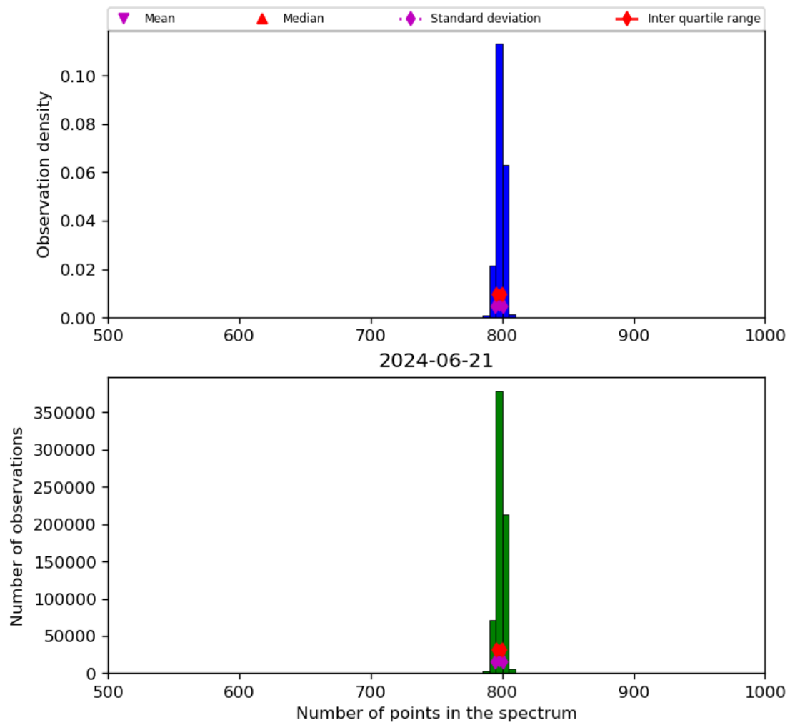
Figure 26: Histogram of “Number of points in the spectrum” for 2024-06-20 to 2024-06-22
