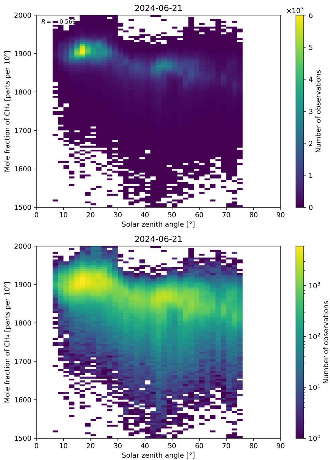
Figure 99: Scatter density plot of “Solar zenith angle” against “Mole fraction of \text{CH}_4 ” for 2024-06-20 to 2024-06-22.
