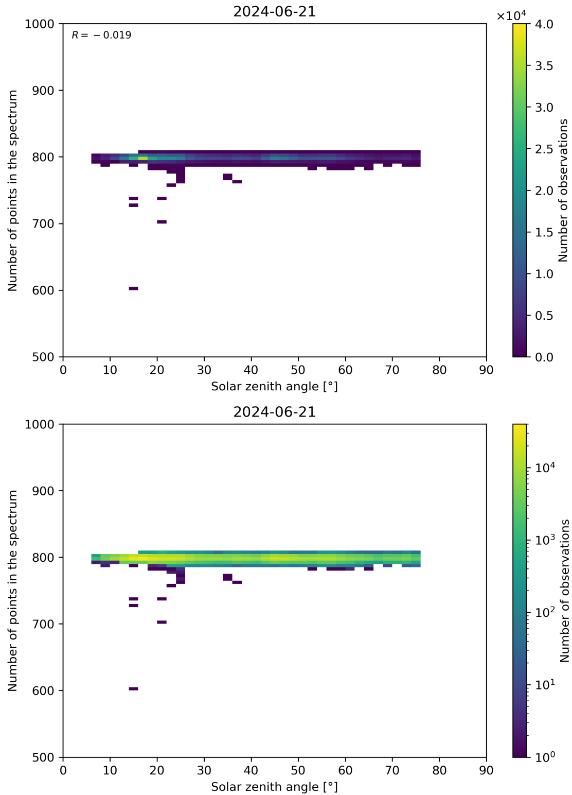
Figure 103: Scatter density plot of “Solar zenith angle” against “Number of points in the spectrum” for 2024-06-20 to 2024-06-22.
