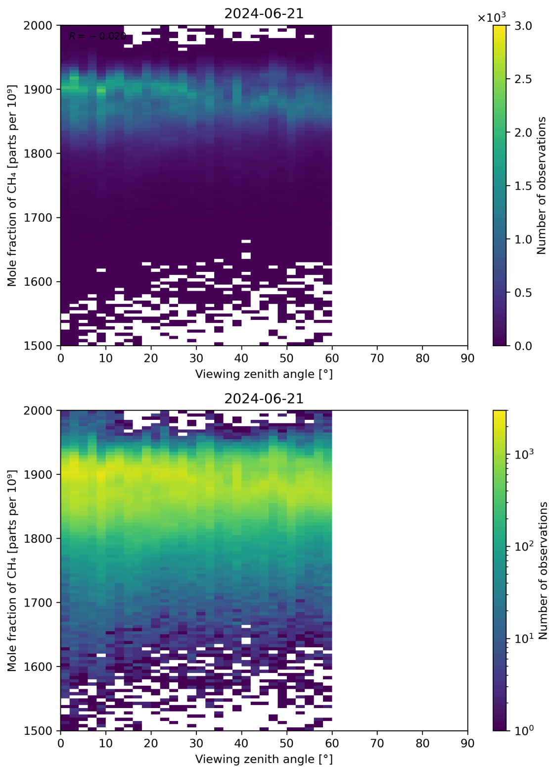
Figure 110: Scatter density plot of “Viewing zenith angle” against “Mole fraction of CH 4 ” for 2024-06-20 to 2024-06-22.
