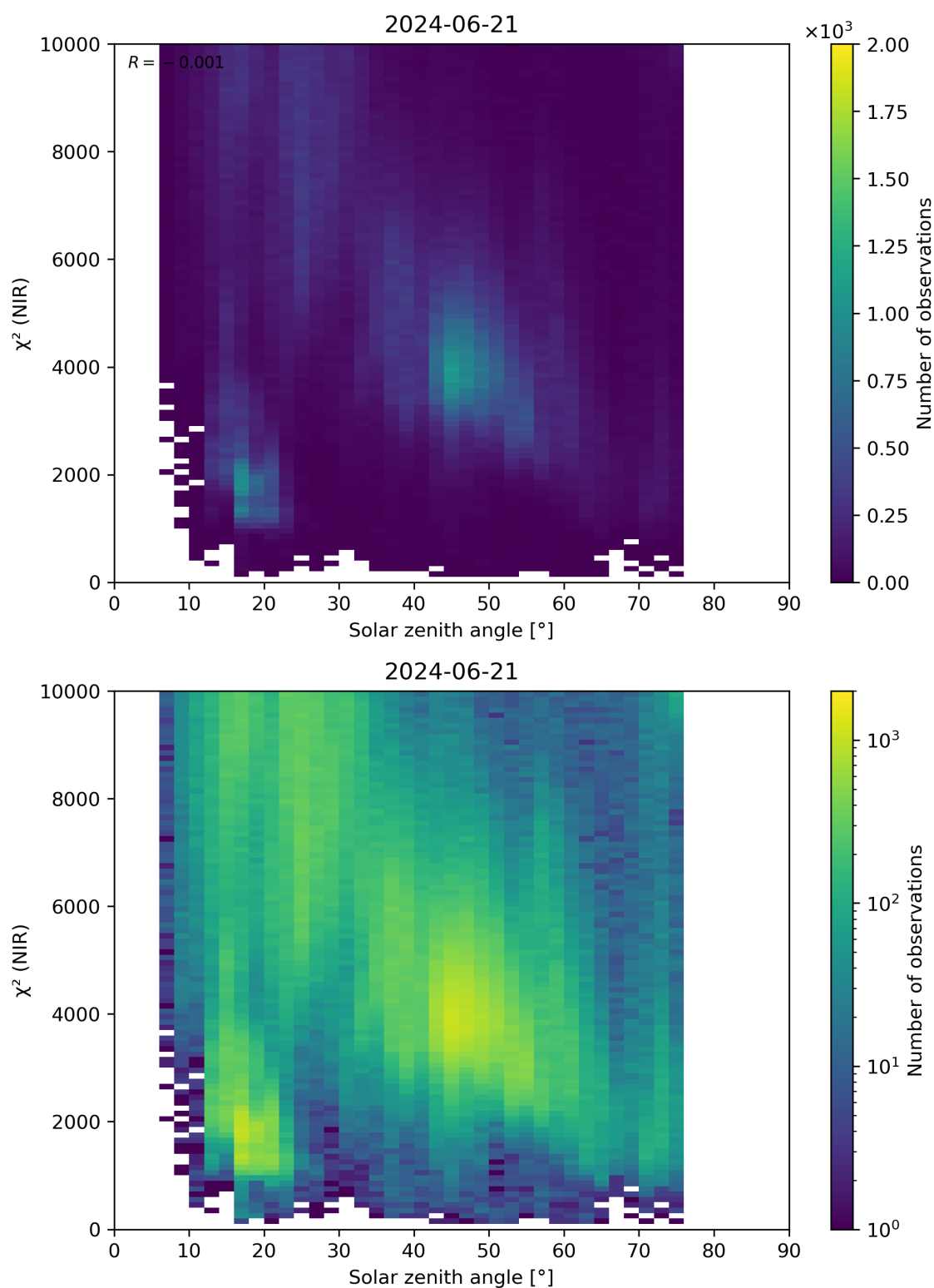
Figure 94: Scatter density plot of “Solar zenith angle” against “ \chi^2 (NIR)” for 2024-06-20 to 2024-06-22.
