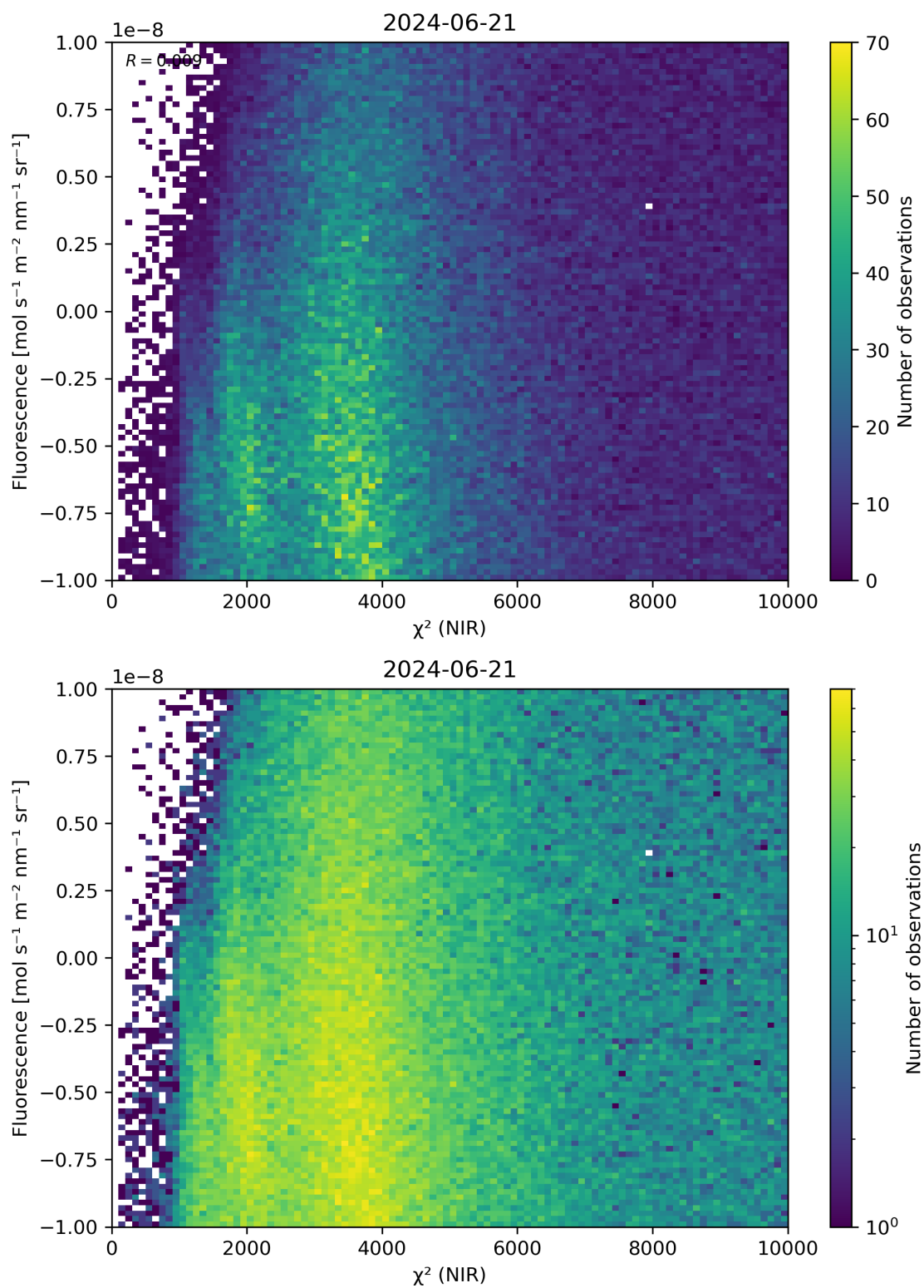
Figure 45: Scatter density plot of “ \chi^2 (NIR)” against “Fluorescence” for 2024-06-20 to 2024-06-22.
