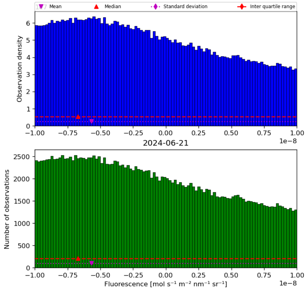
Figure 32: Histogram of “Fluorescence” for 2024-06-20 to 2024-06-22
