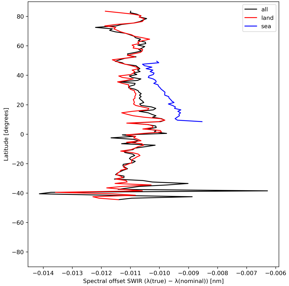
Figure 16: Zonal average of “Spectral offset SWIR ( \lambda(\text{true}) - \lambda(\text{nominal}) )” for 2024-06-20 to 2024-06-22.
