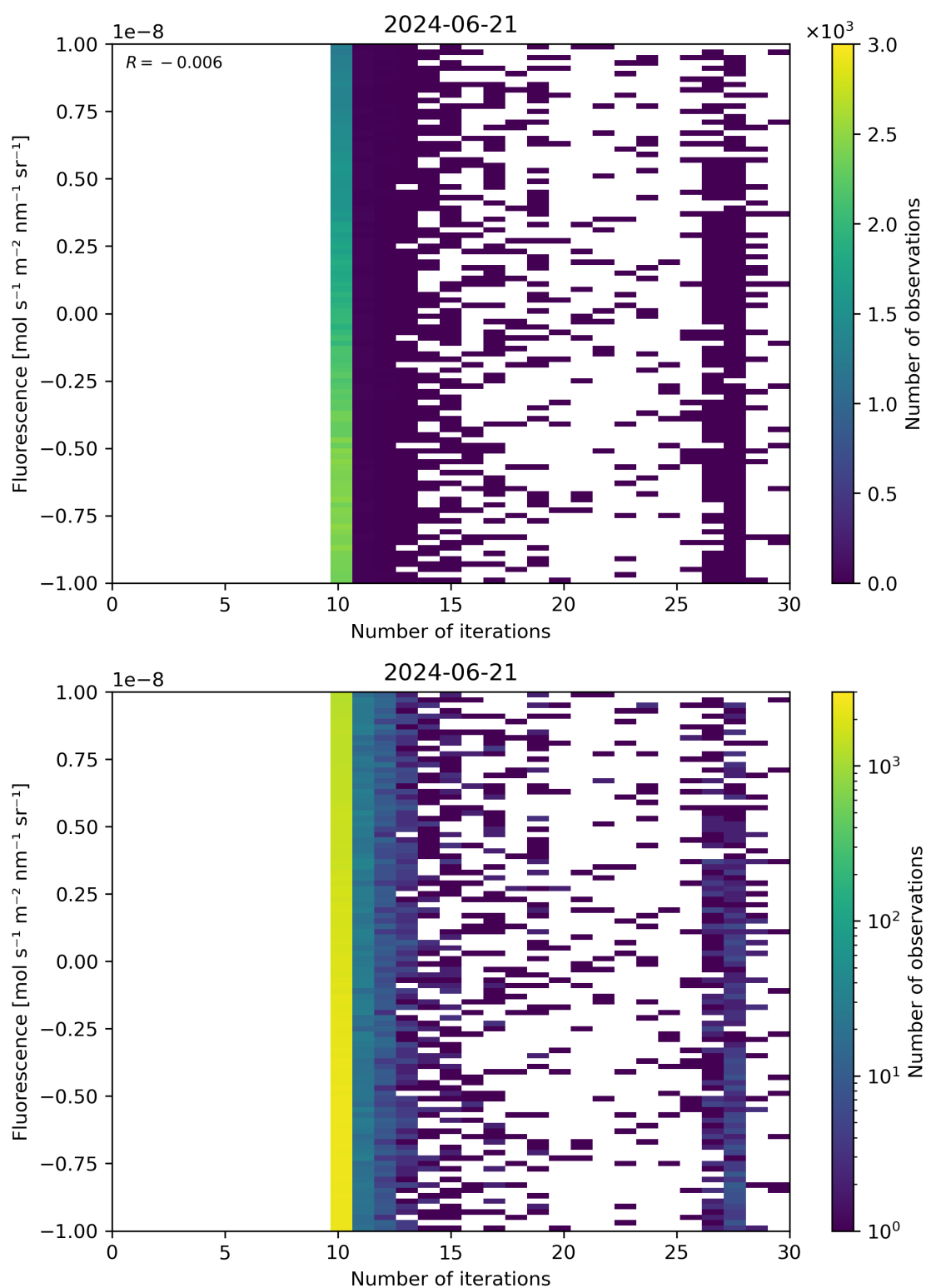
Figure 87: Scatter density plot of “Number of iterations” against “Fluorescence” for 2024-06-20 to 2024-06-22.
