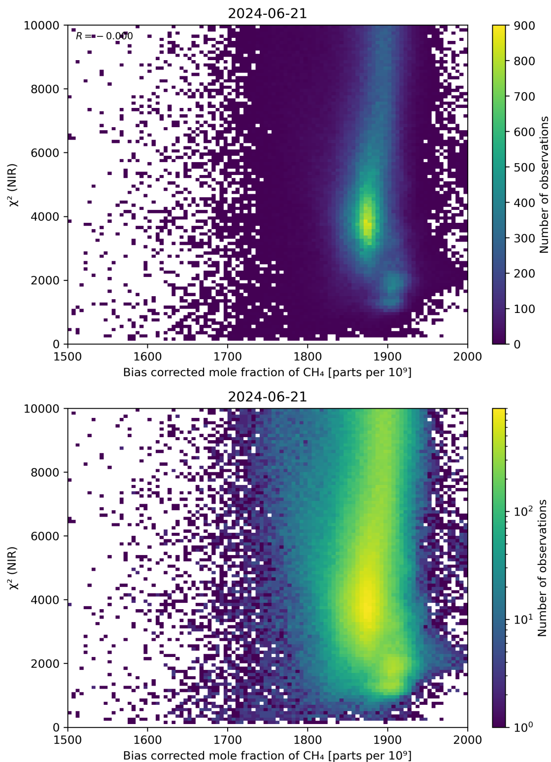
Figure 63: Scatter density plot of “Bias corrected mole fraction of CH 4 ” against “ \chi^2 (NIR)” for 2024-06-20 to 2024-06-22.
