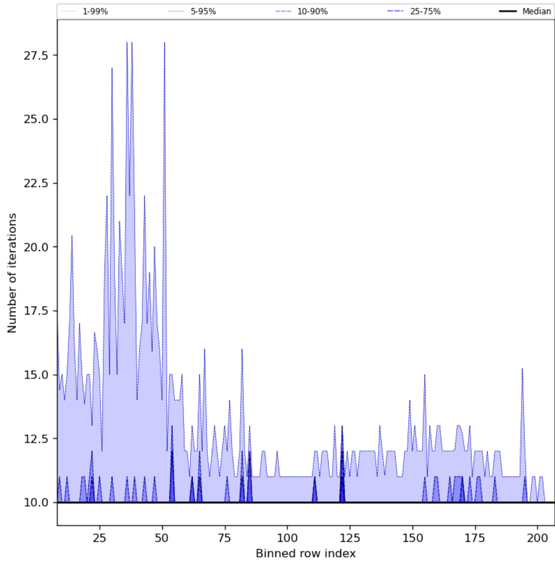
Figure 42: Along track statistics of “Number of iterations” for 2024-06-20 to 2024-06-22
