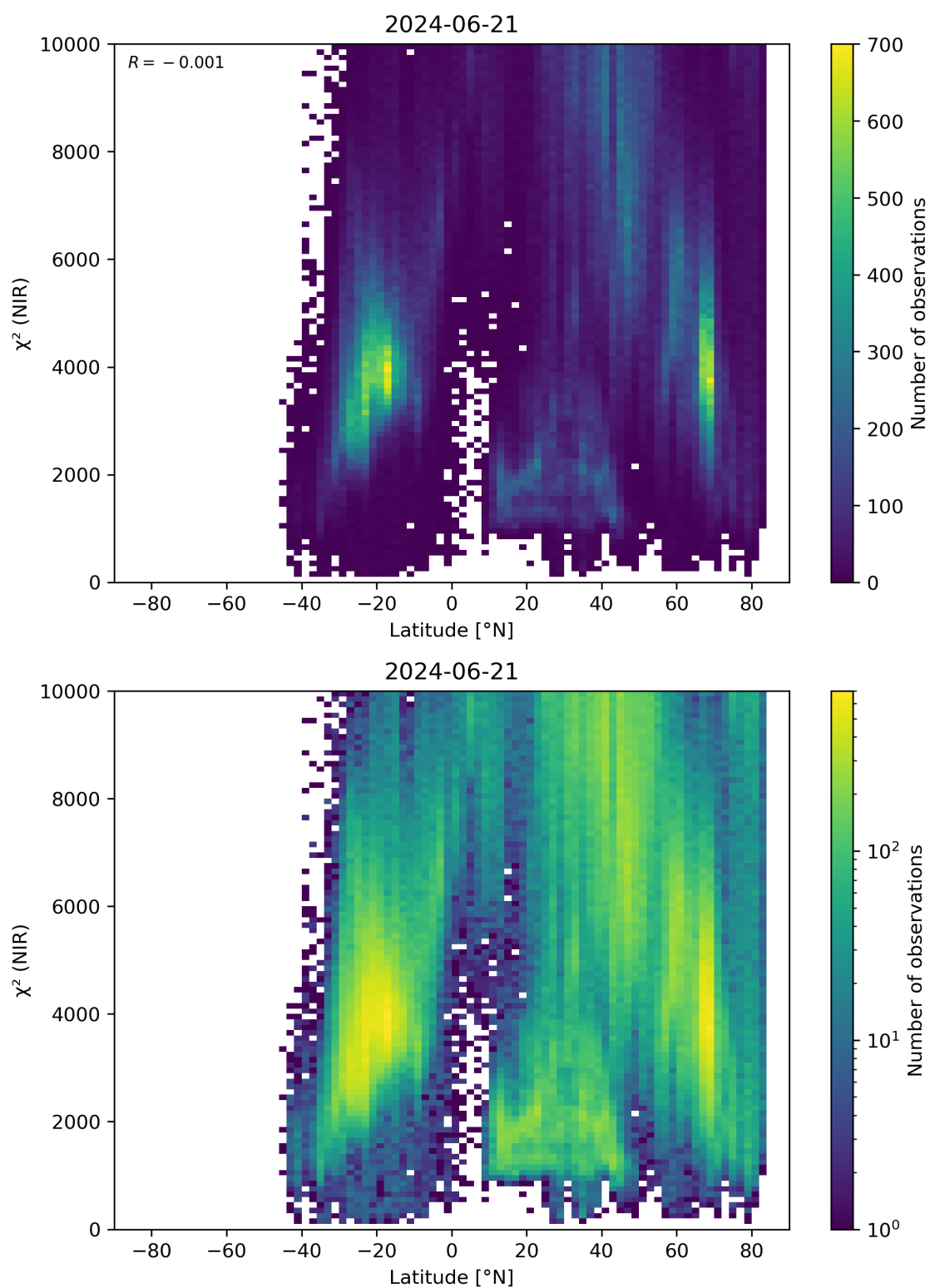
Figure 53: Scatter density plot of “Latitude” against “ \chi^2 (NIR)” for 2024-06-20 to 2024-06-22.
