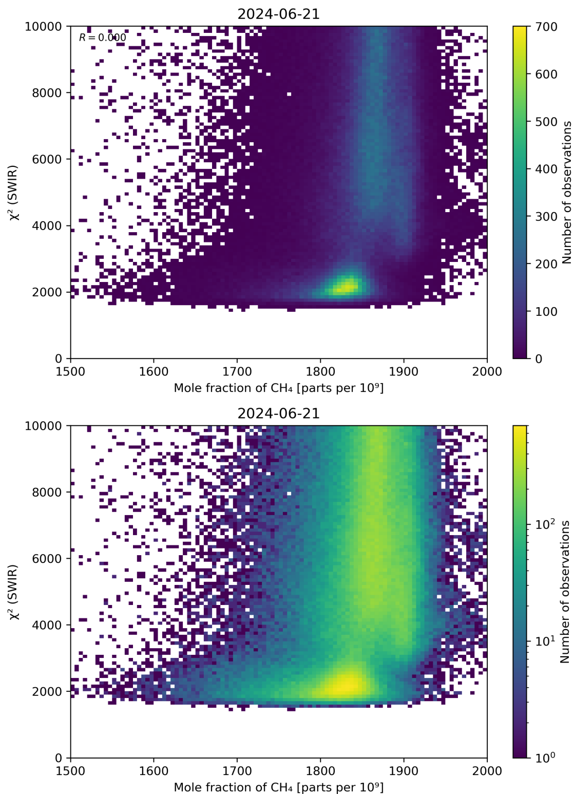
Figure 71: Scatter density plot of “Mole fraction of CH 4 ” against “ \chi^2 (SWIR)” for 2024-06-20 to 2024-06-22.
