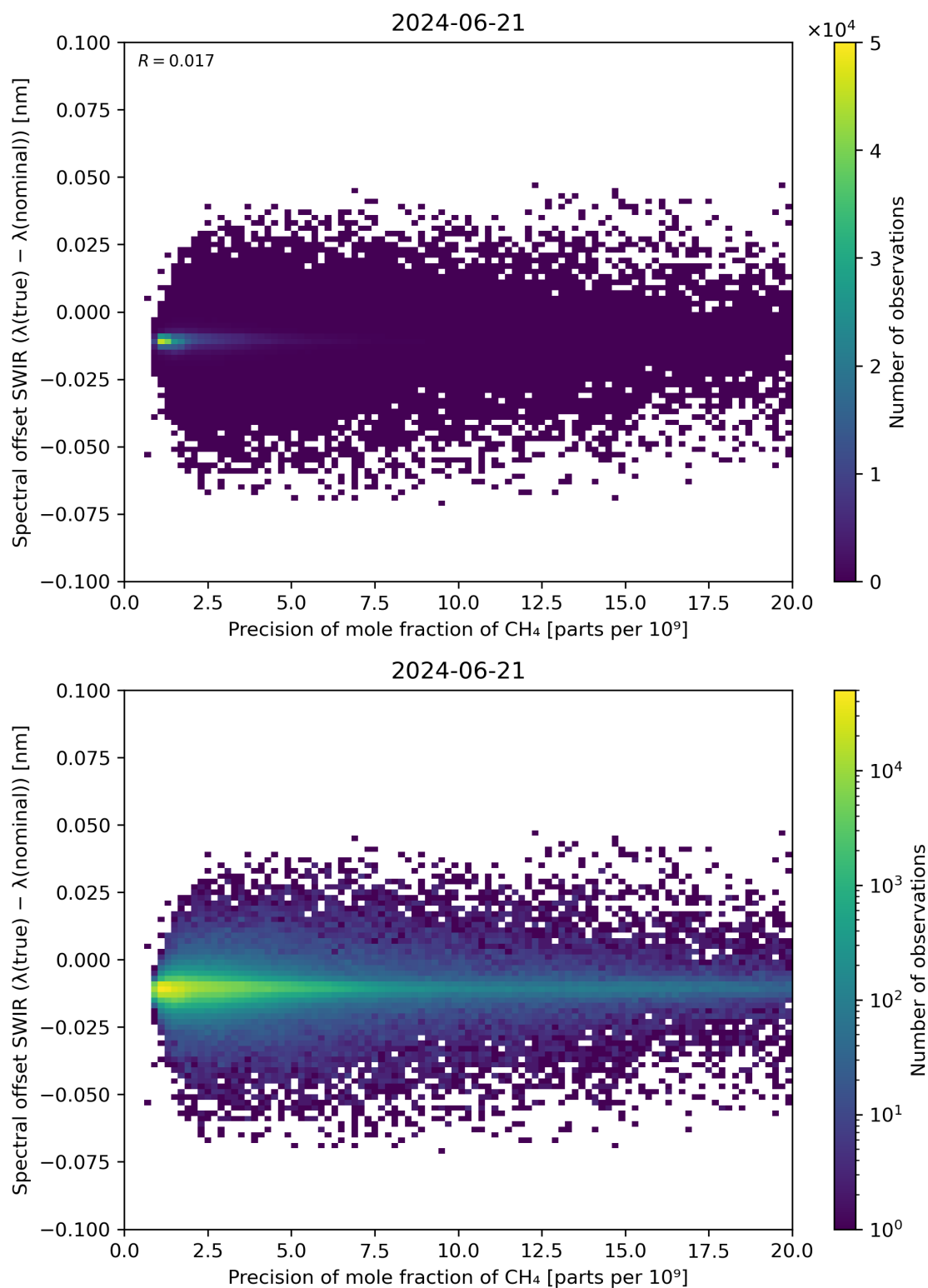
Figure 85: Scatter density plot of “Precision of mole fraction of CH 4 ” against “Spectral offset SWIR ( \lambda(\text{true}) - \lambda(\text{nominal}) )” for 2024-06-20 to 2024-06-22.
