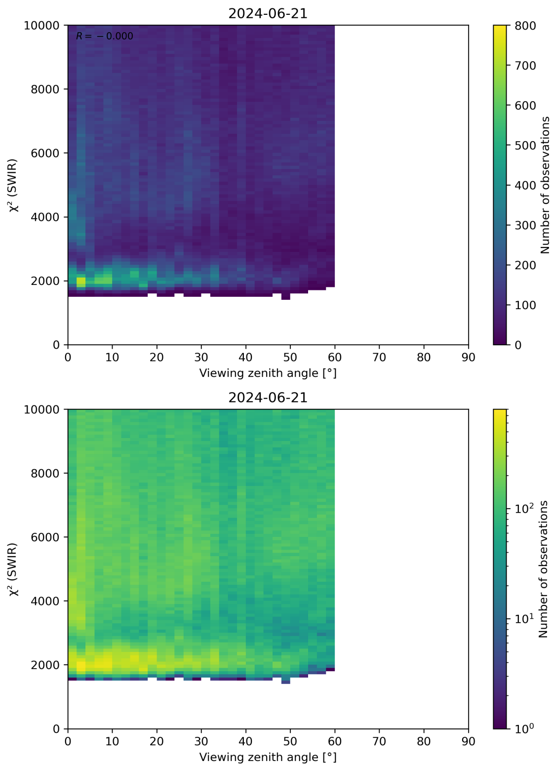
Figure 106: Scatter density plot of “Viewing zenith angle” against “ \chi^2 (SWIR)” for 2024-06-20 to 2024-06-22.
