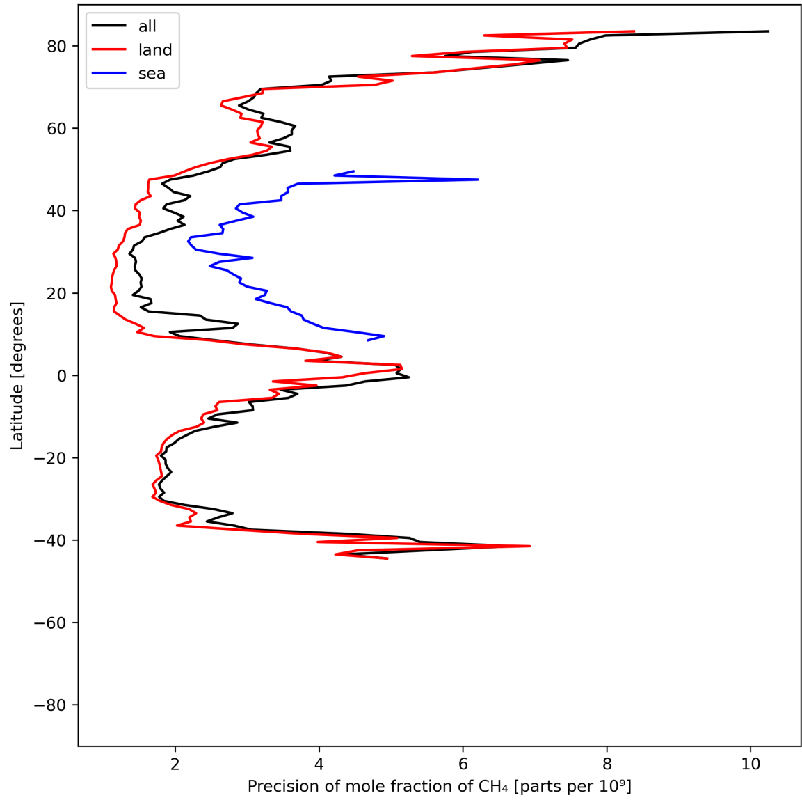
Figure 13: Zonal average of “Precision of mole fraction of CH 4 ” for 2024-06-20 to 2024-06-22.
