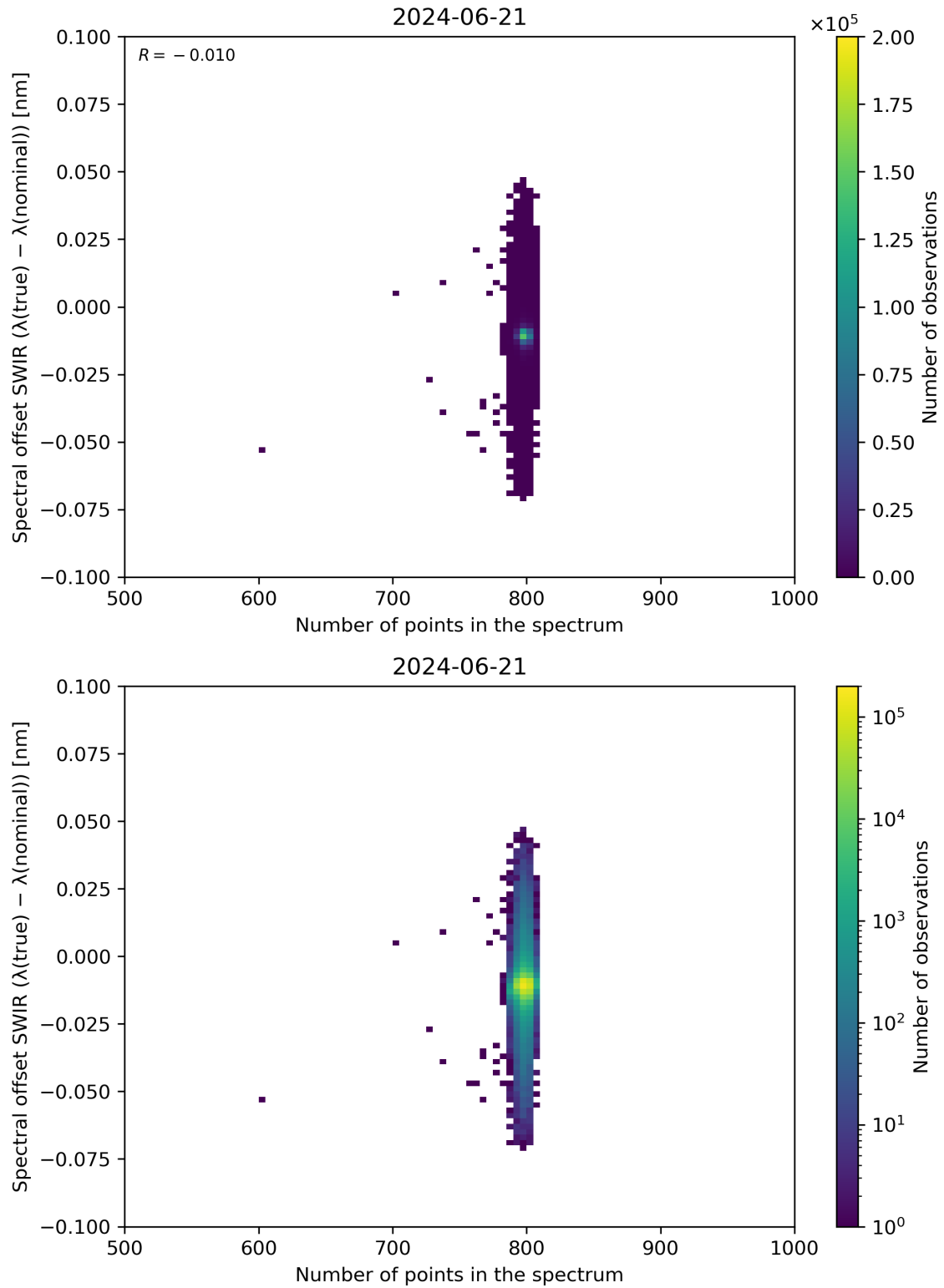
Figure 93: Scatter density plot of “Number of points in the spectrum” against “Spectral offset SWIR ( \lambda(\text{true}) - \lambda(\text{nominal}) )” for 2024-06-20 to 2024-06-22.
