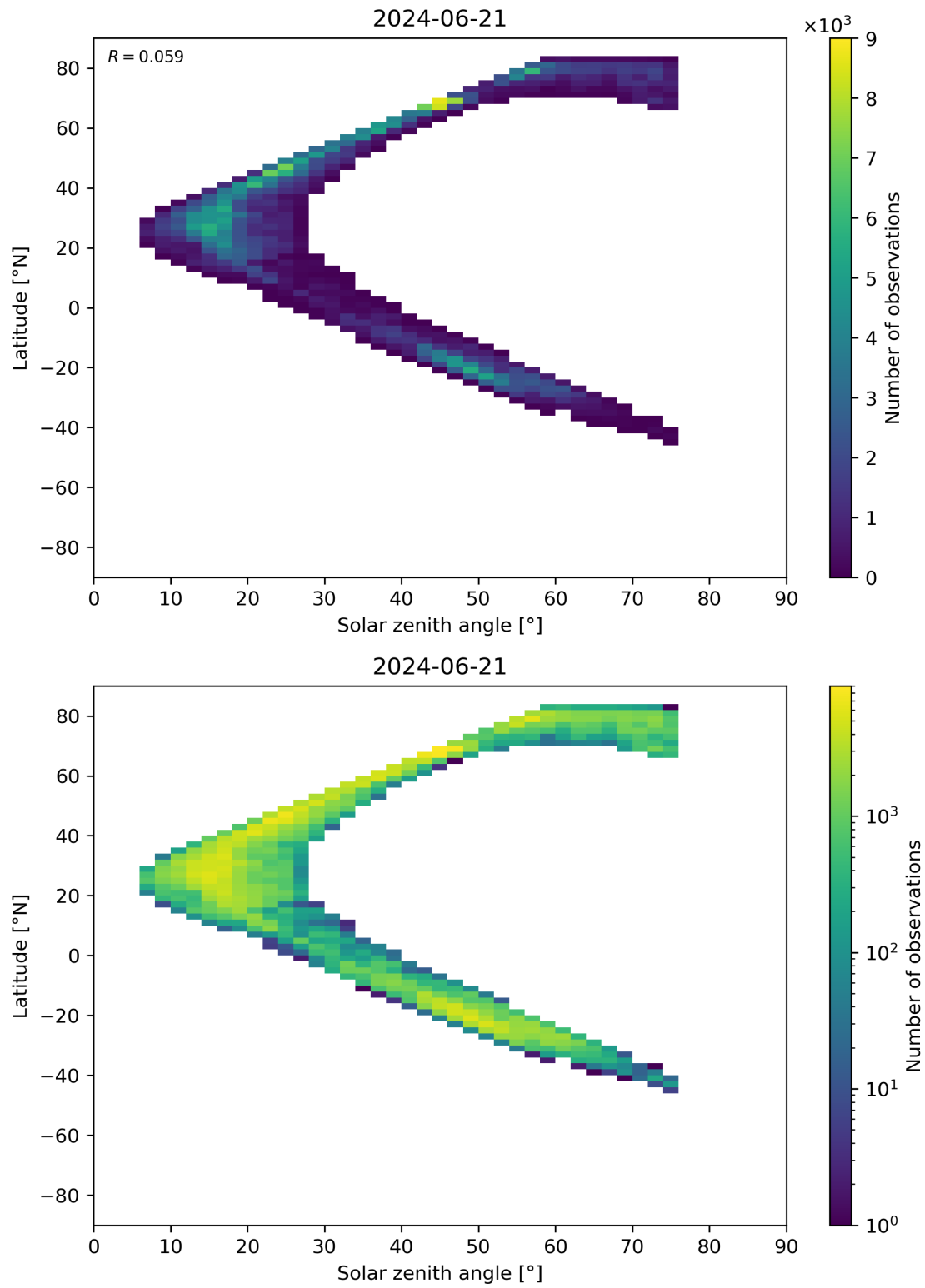
Figure 98: Scatter density plot of “Solar zenith angle” against “Latitude” for 2024-06-20 to 2024-06-22.
