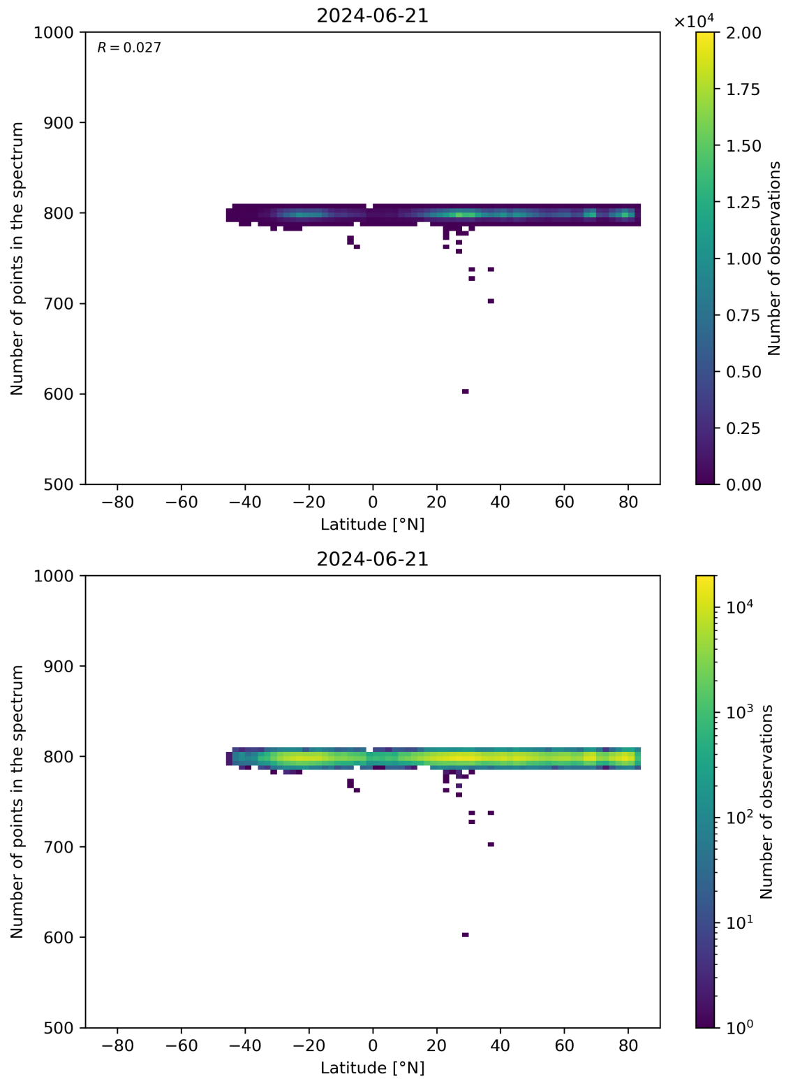
Figure 61: Scatter density plot of “Latitude” against “Number of points in the spectrum” for 2024-06-20 to 2024-06-22.
