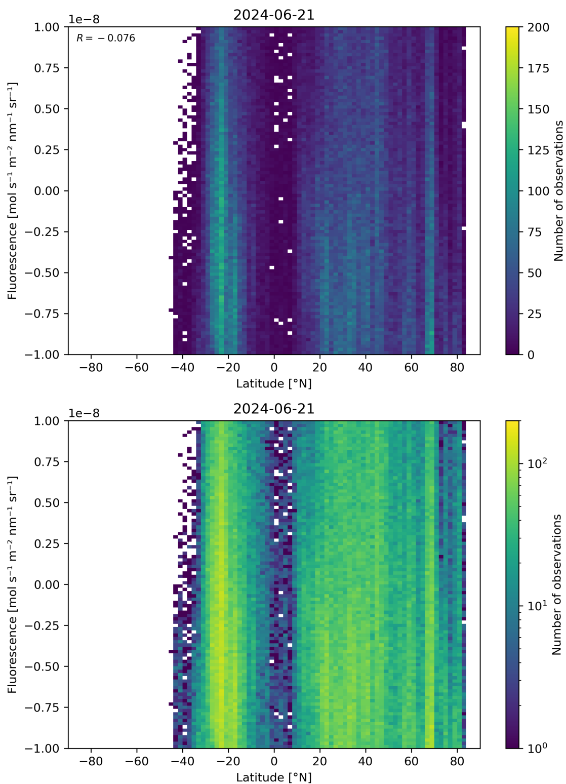
Figure 56: Scatter density plot of “Latitude” against “Fluorescence” for 2024-06-20 to 2024-06-22.
