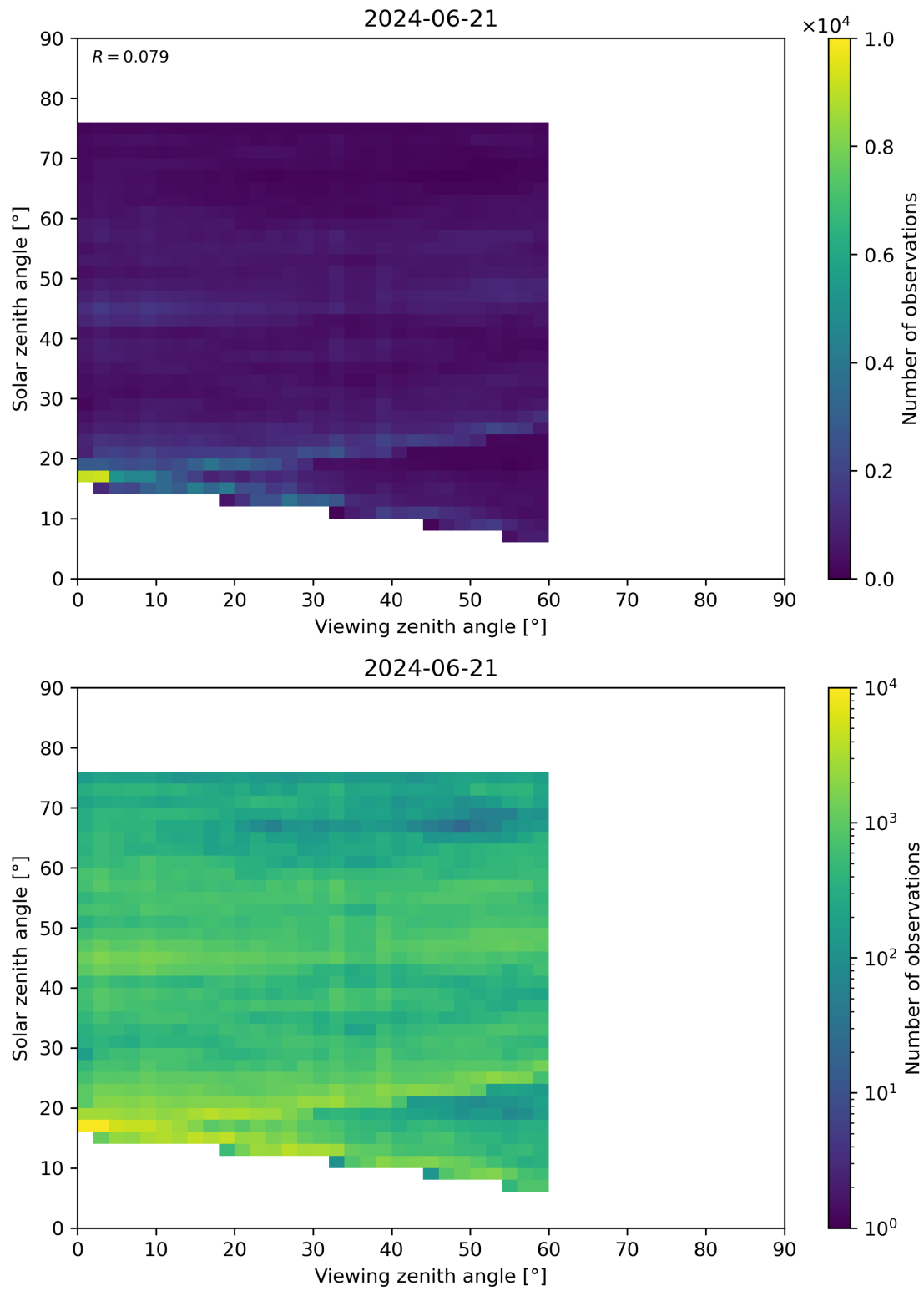
Figure 115: Scatter density plot of “Viewing zenith angle” against “Solar zenith angle” for 2024-06-20 to 2024-06-22.
