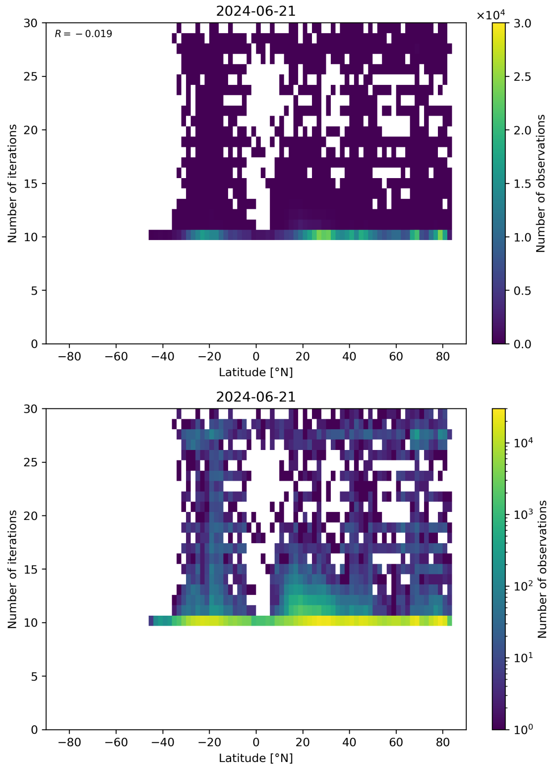
Figure 60: Scatter density plot of “Latitude” against “Number of iterations” for 2024-06-20 to 2024-06-22.
