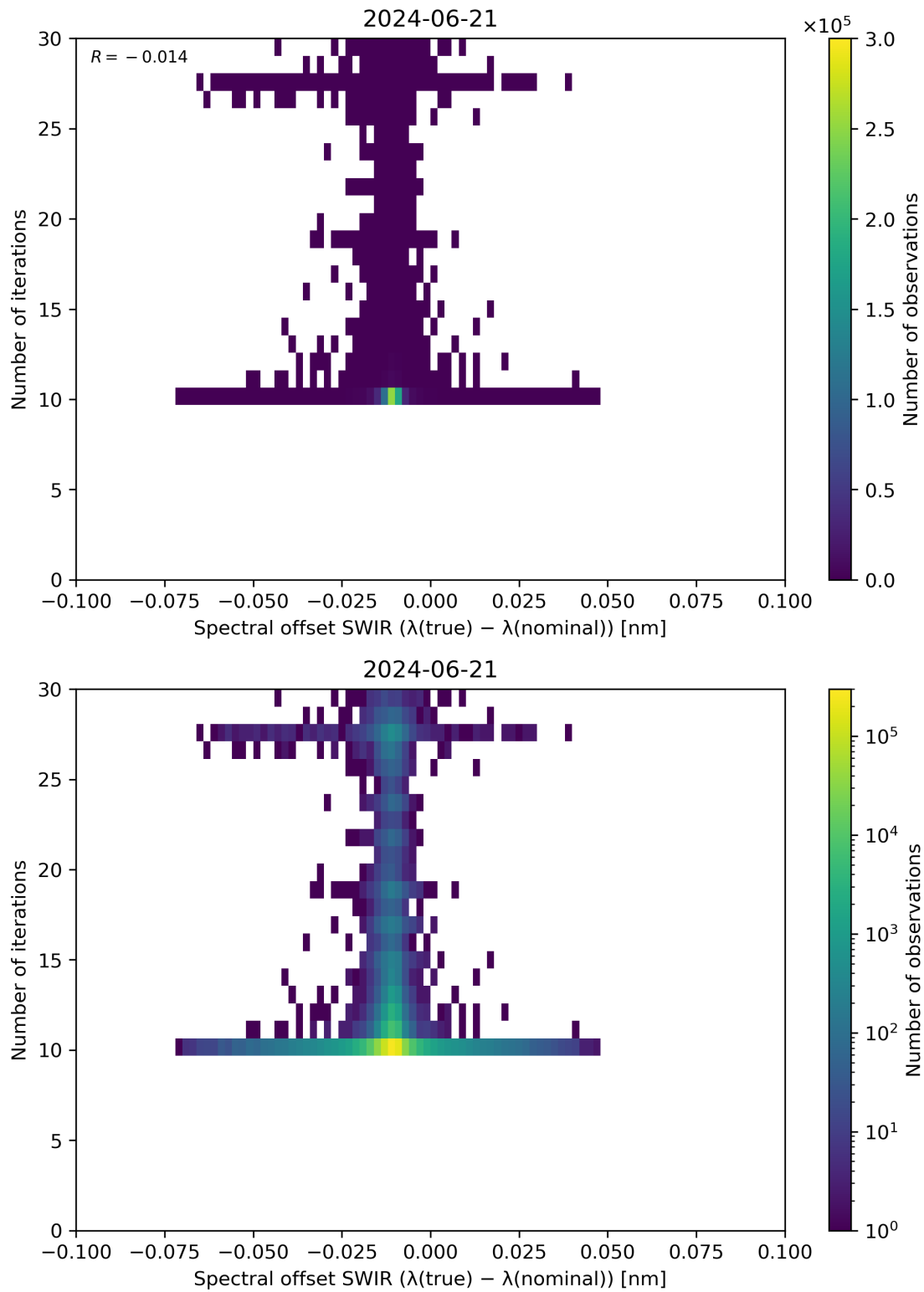
Figure 121: Scatter density plot of “Spectral offset SWIR ( \lambda(\text{true}) - \lambda(\text{nominal}) )” against “Number of iterations” for 2024-06-20 to 2024-06-22.
