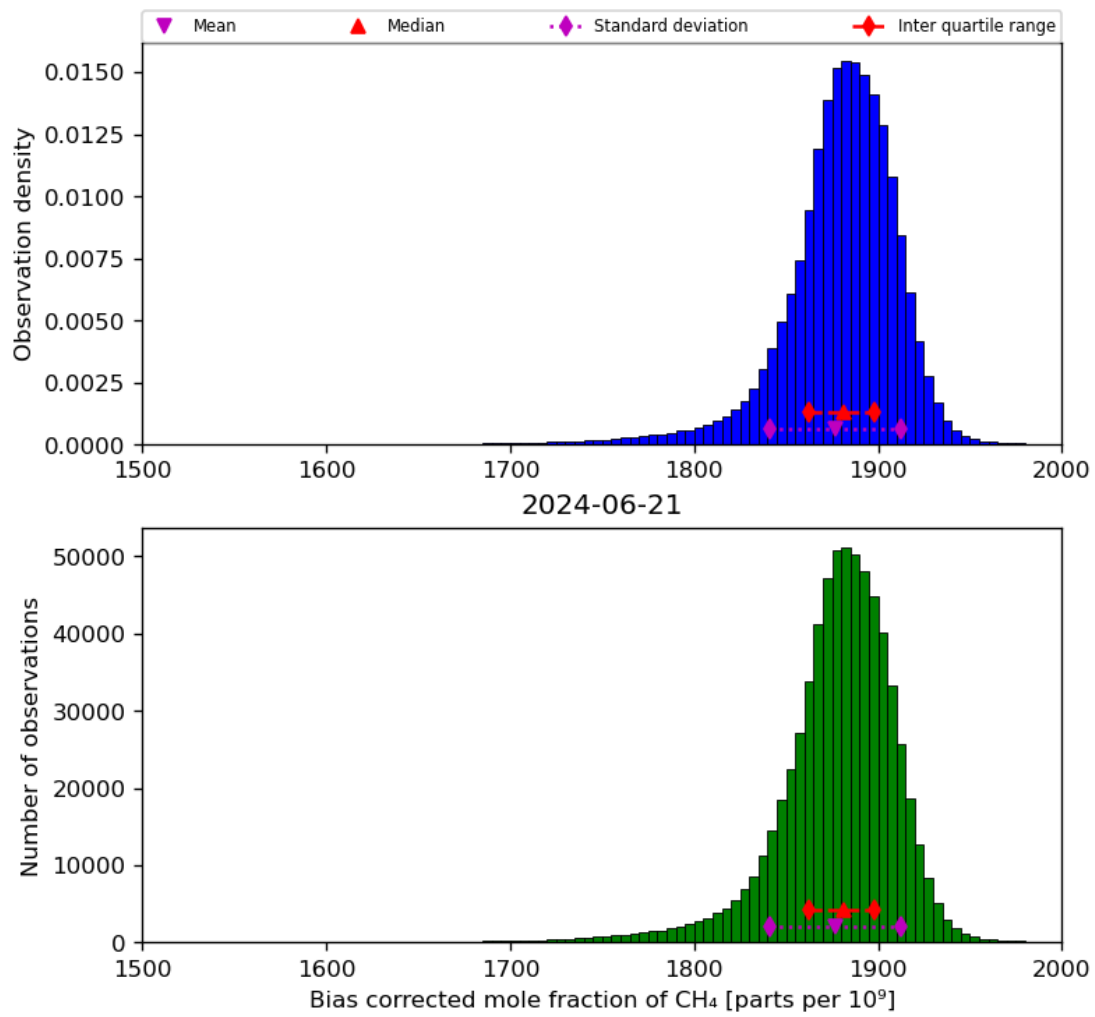
Figure 25: Histogram of “Bias corrected mole fraction of CH 4 ” for 2024-06-20 to 2024-06-22
