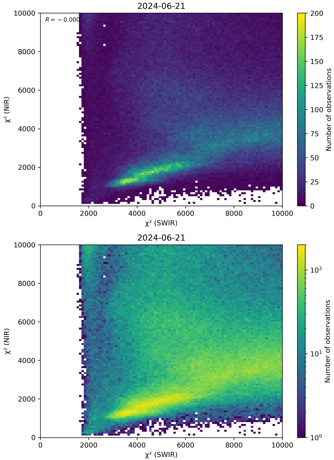
Figure 47: Scatter density plot of “ \chi^2 (SWIR)” against “ \chi^2 (NIR)” for 2024-06-20 to 2024-06-22.
