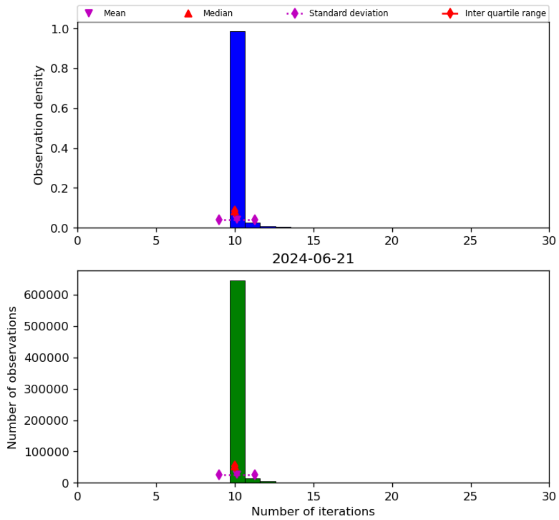
Figure 31: Histogram of "Number of iterations" for 2024-06-20 to 2024-06-22
