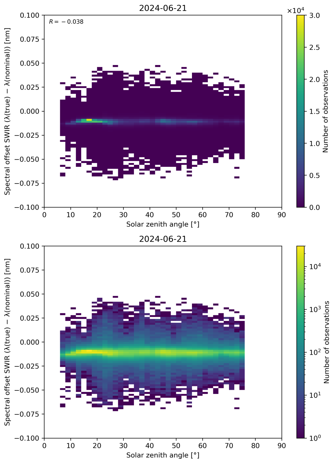
Figure 104: Scatter density plot of “Solar zenith angle” against “Spectral offset SWIR ( \lambda(\text{true}) - \lambda(\text{nominal}) )” for 2024-06-20 to 2024-06-22.
