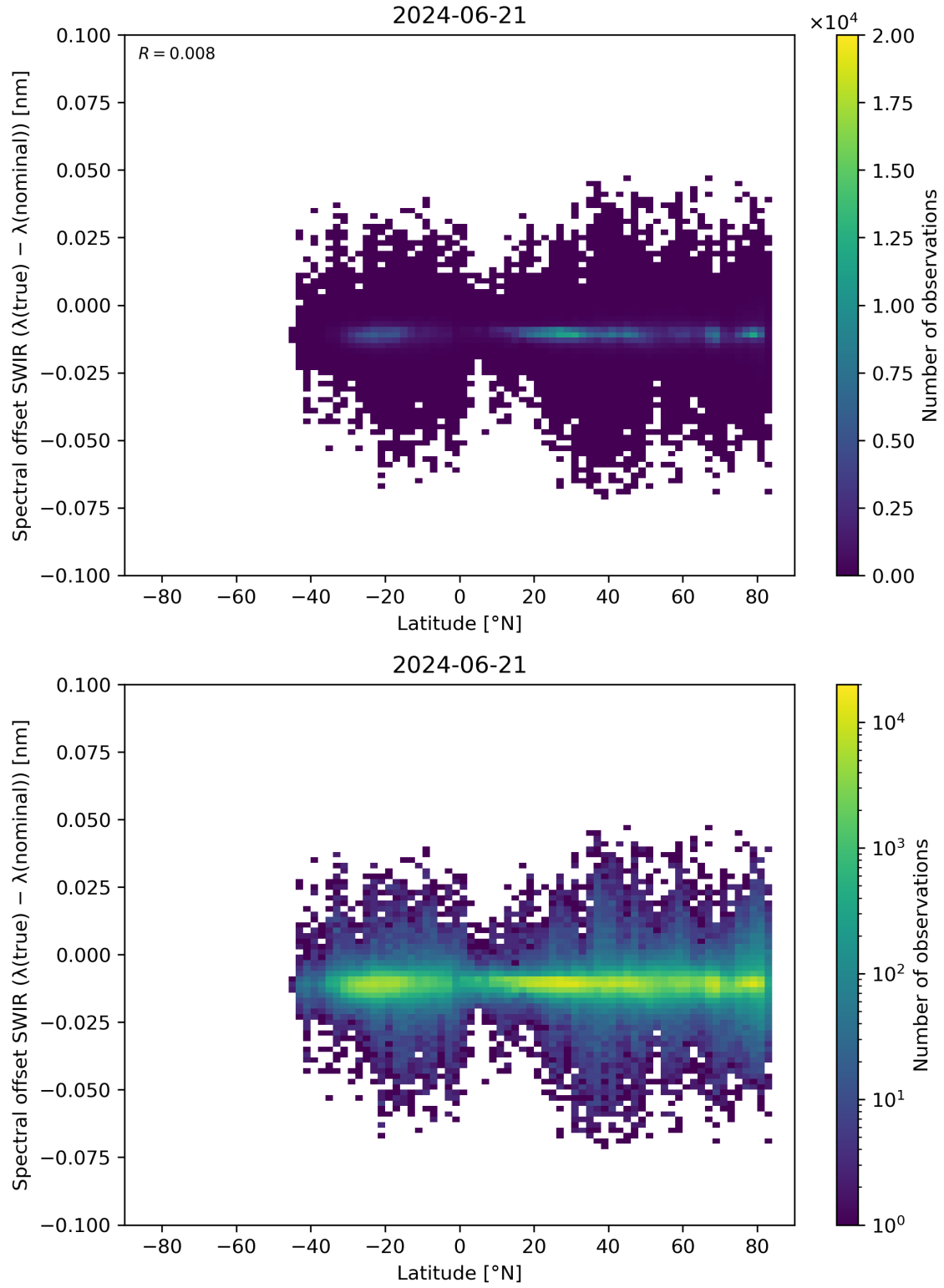
Figure 62: Scatter density plot of “Latitude” against “Spectral offset SWIR ( \lambda(\text{true}) - \lambda(\text{nominal}) )” for 2024-06-20 to 2024-06-22.
