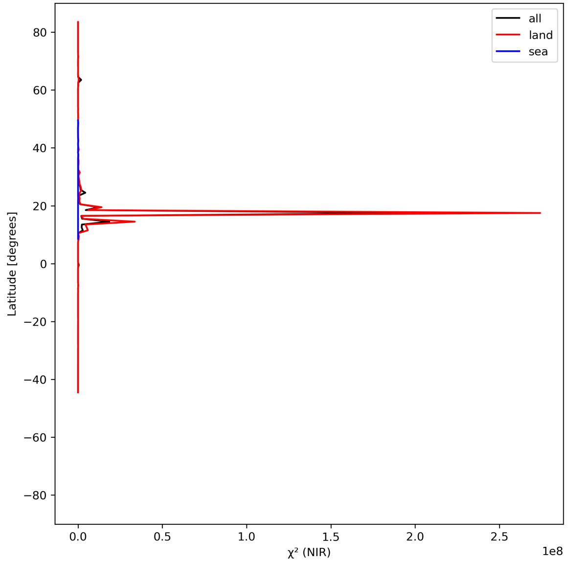
Figure 18: Zonal average of “ \chi^2 (NIR)” for 2024-06-20 to 2024-06-22.
