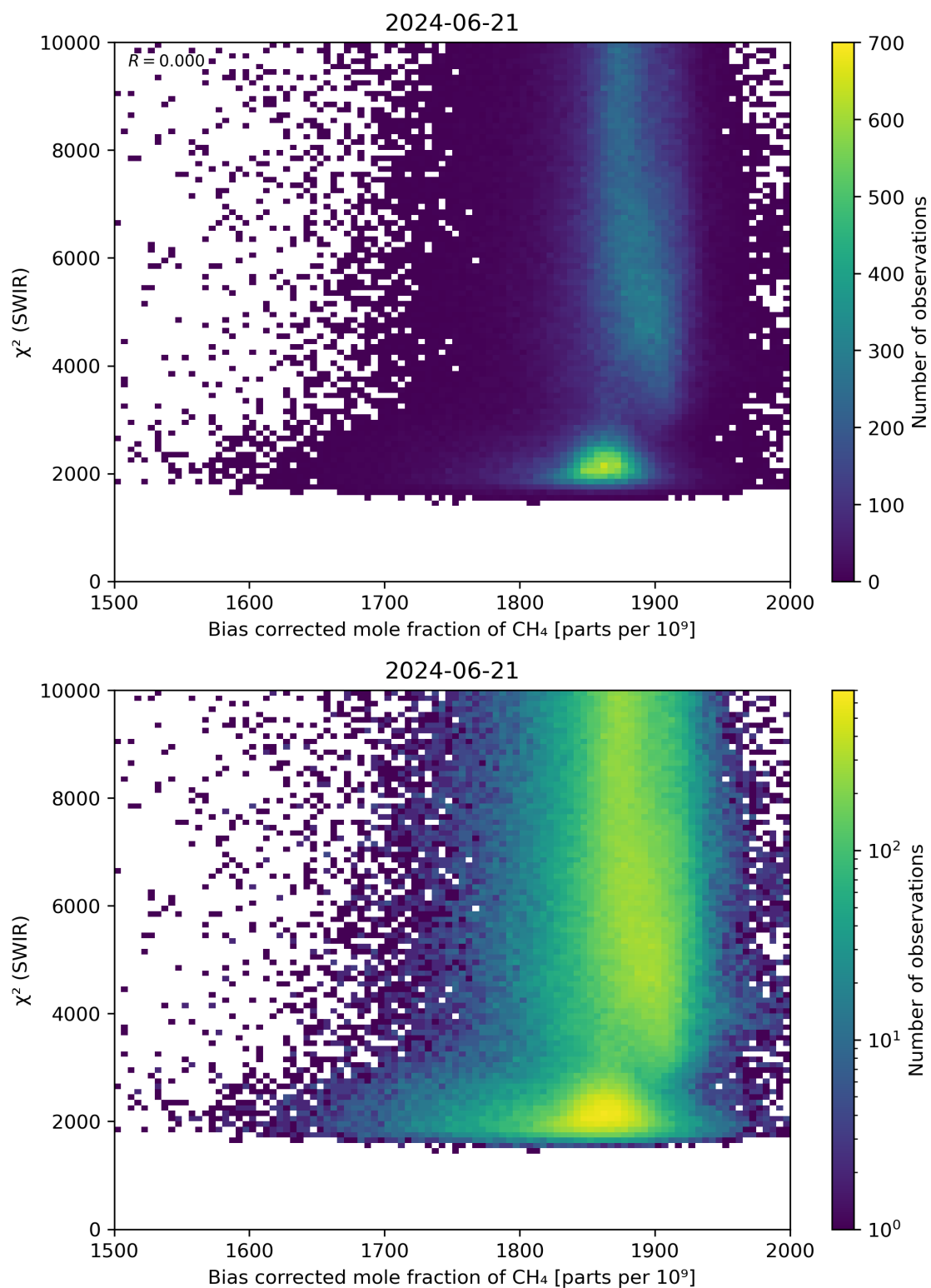
Figure 64: Scatter density plot of “Bias corrected mole fraction of CH 4 ” against “ \chi^2 (SWIR)” for 2024-06-20 to 2024-06-22.
