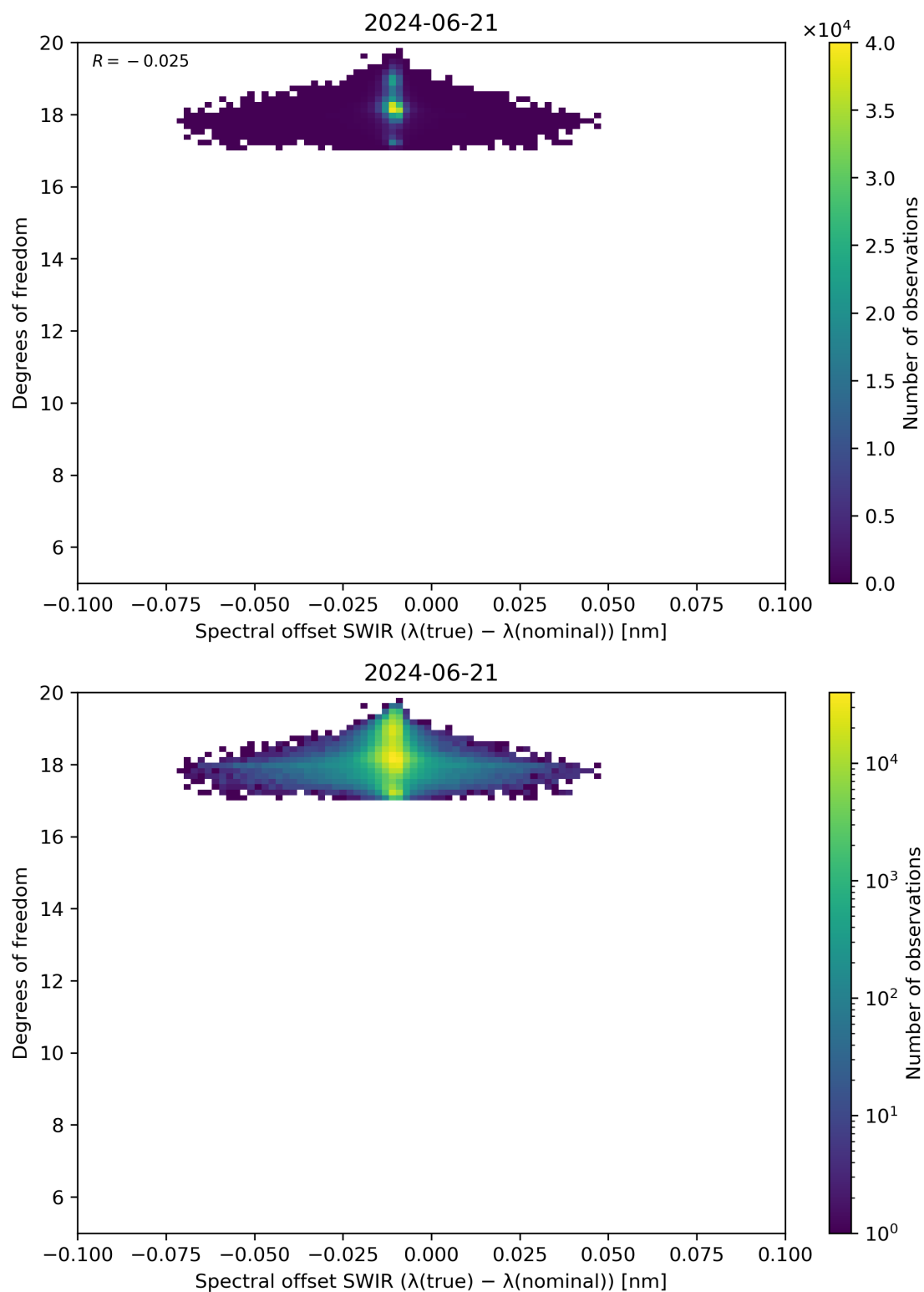
Figure 119: Scatter density plot of “Spectral offset SWIR ( \lambda(\text{true}) - \lambda(\text{nominal}) )” against “Degrees of freedom” for 2024-06-20 to 2024-06-22.
