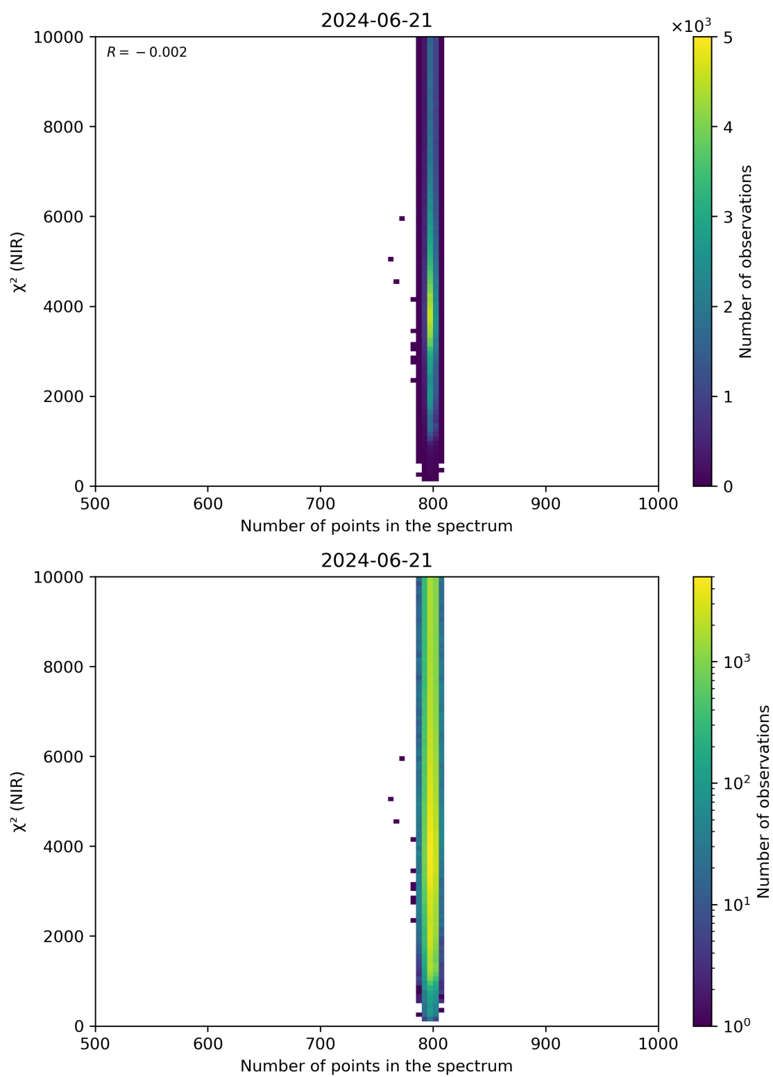
Figure 88: Scatter density plot of “Number of points in the spectrum” against “ \chi^2 (NIR)” for 2024-06-20 to 2024-06-22.
