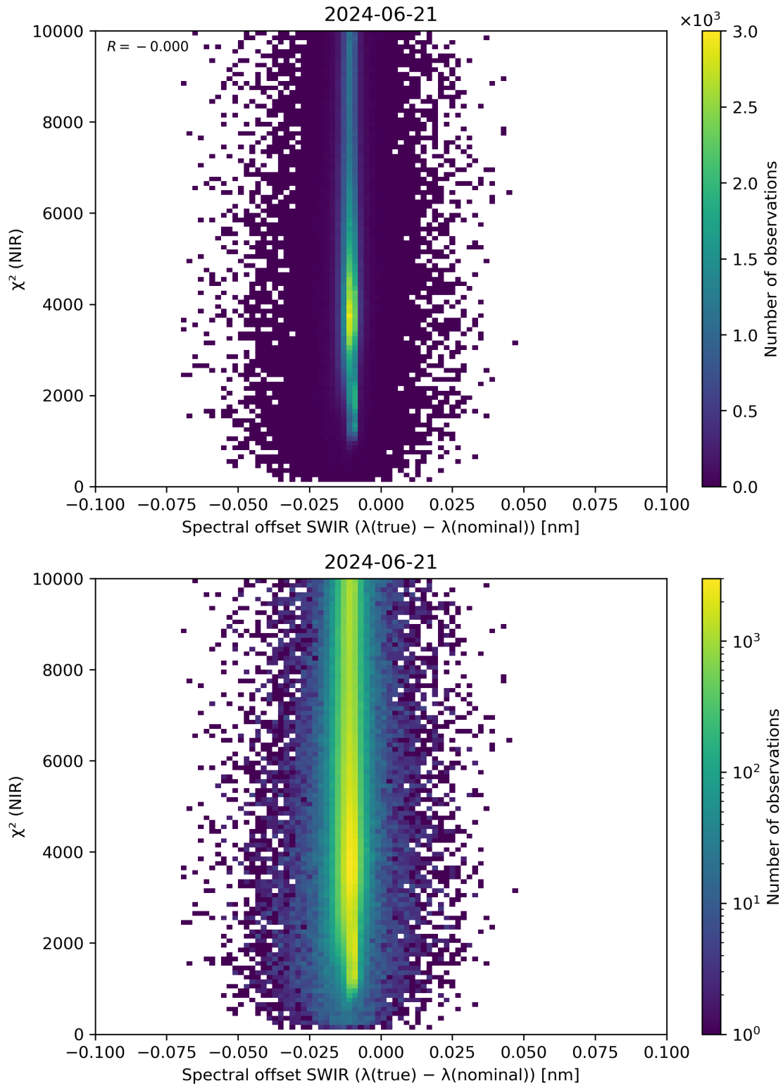
Figure 117: Scatter density plot of “Spectral offset SWIR ( \lambda(\text{true}) - \lambda(\text{nominal}) )” against “ \chi^2 (NIR)” for 2024-06-20 to 2024-06-22.
