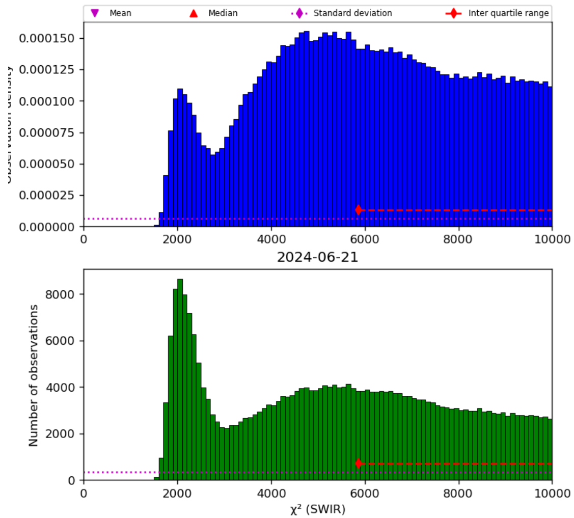
Figure 28: Histogram of “ \chi^2 (SWIR)” for 2024-06-20 to 2024-06-22
