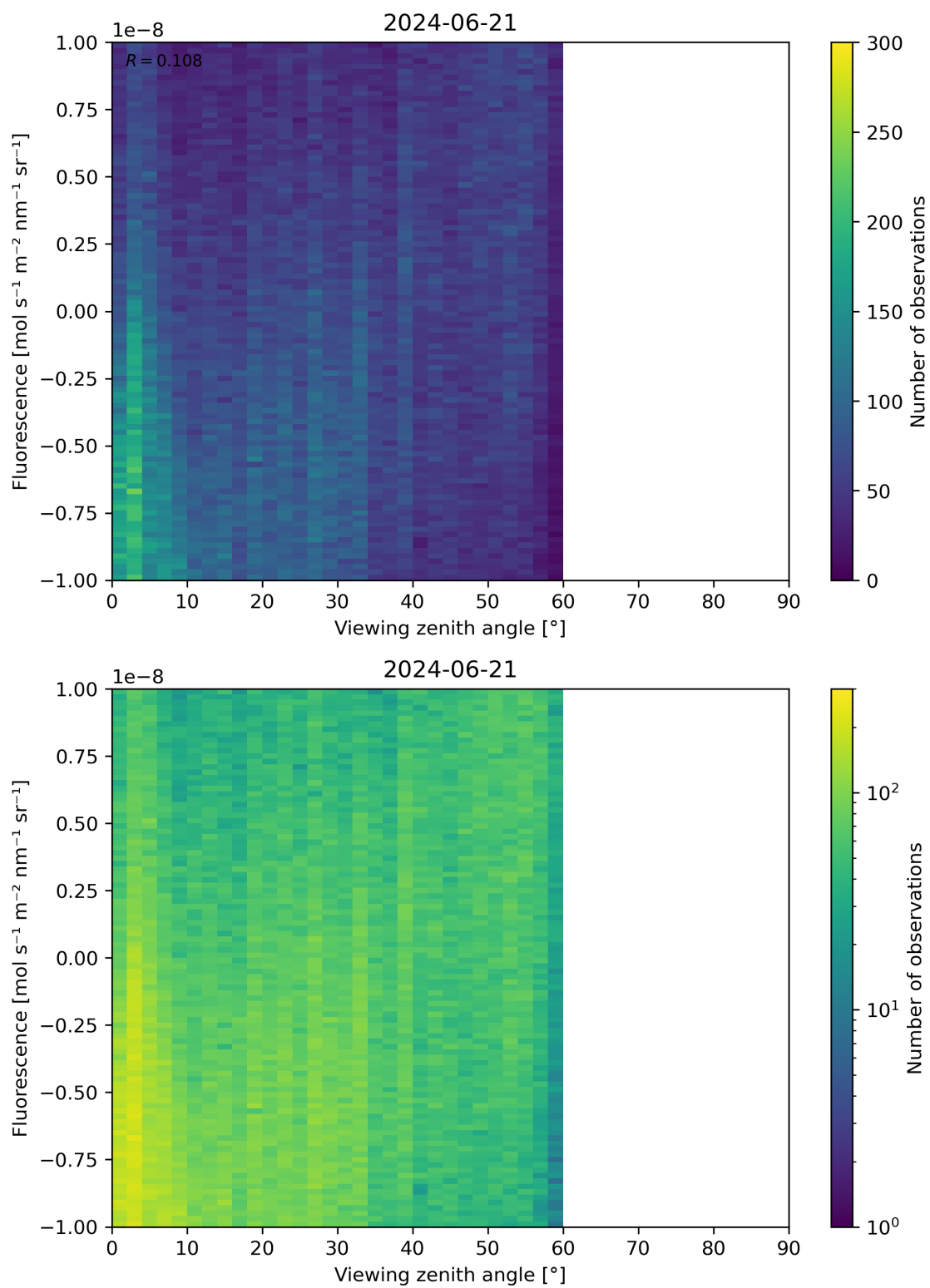
Figure 108: Scatter density plot of “Viewing zenith angle” against “Fluorescence” for 2024-06-20 to 2024-06-22.
