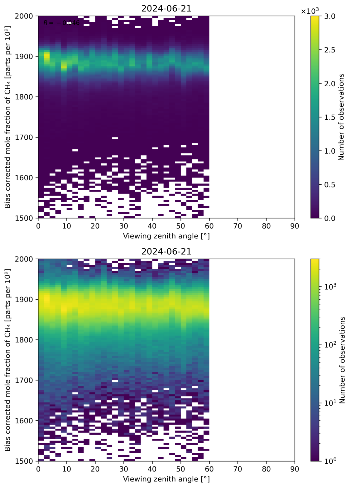
Figure 111: Scatter density plot of “Viewing zenith angle” against “Bias corrected mole fraction of CH 4 ” for 2024-06-20 to 2024-06-22.
