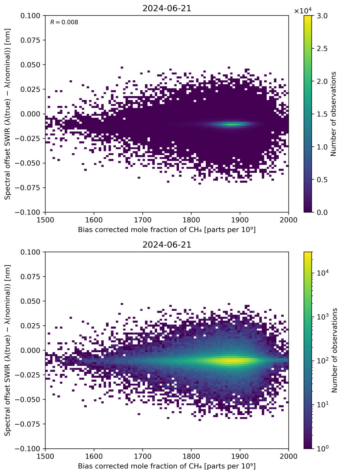
Figure 69: Scatter density plot of “Bias corrected mole fraction of \text{CH}_4 ” against “Spectral offset SWIR ( \lambda(\text{true}) - \lambda(\text{nominal}) )” for 2024-06-20 to 2024-06-22.
