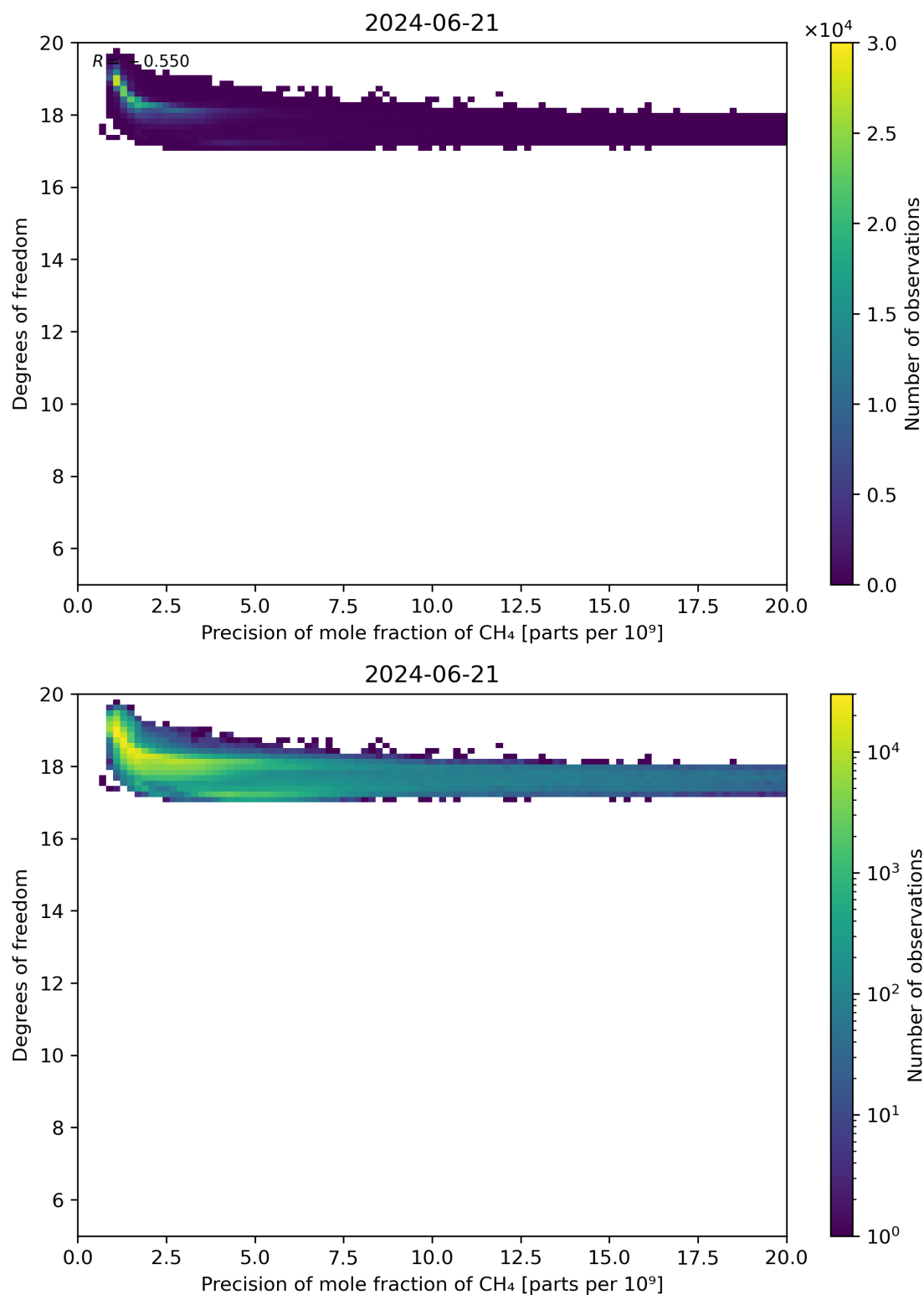
Figure 80: Scatter density plot of “Precision of mole fraction of CH 4 ” against “Degrees of freedom” for 2024-06-20 to 2024-06-22.
