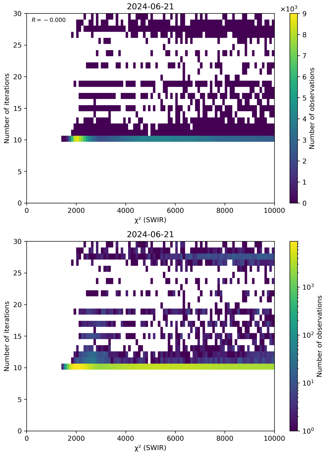
Figure 50: Scatter density plot of “ \chi^2 (SWIR)” against “Number of iterations” for 2024-06-20 to 2024-06-22.
