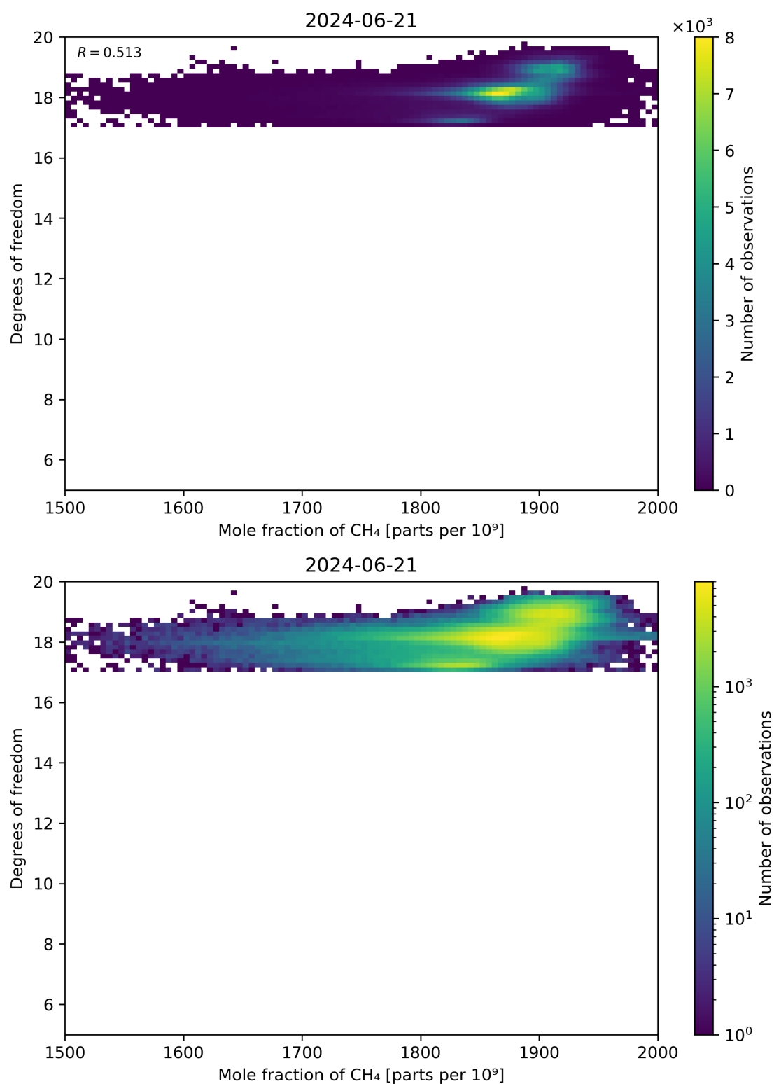
Figure 72: Scatter density plot of “Mole fraction of CH 4 ” against “Degrees of freedom” for 2024-06-20 to 2024-06-22.
