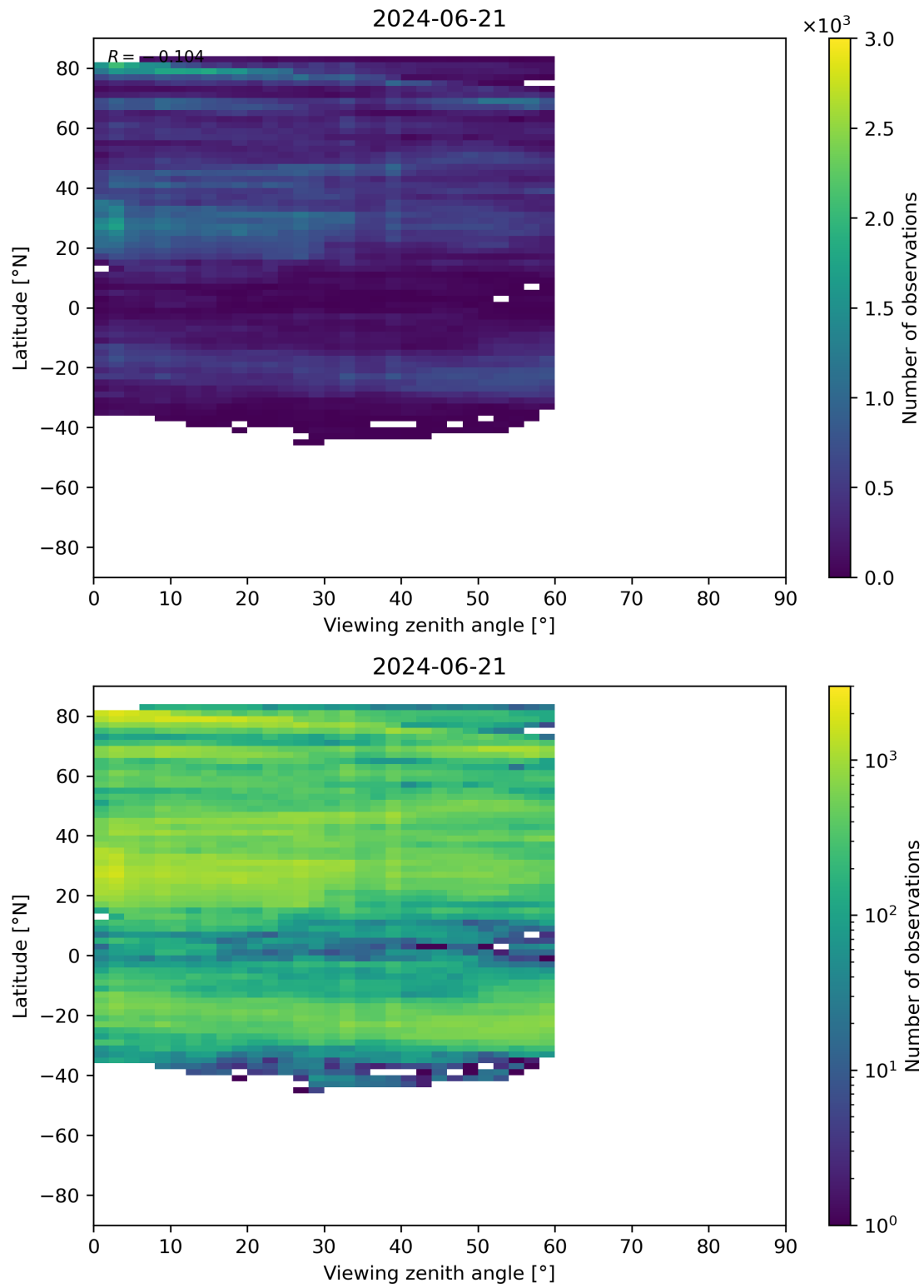
Figure 109: Scatter density plot of “Viewing zenith angle” against “Latitude” for 2024-06-20 to 2024-06-22.
