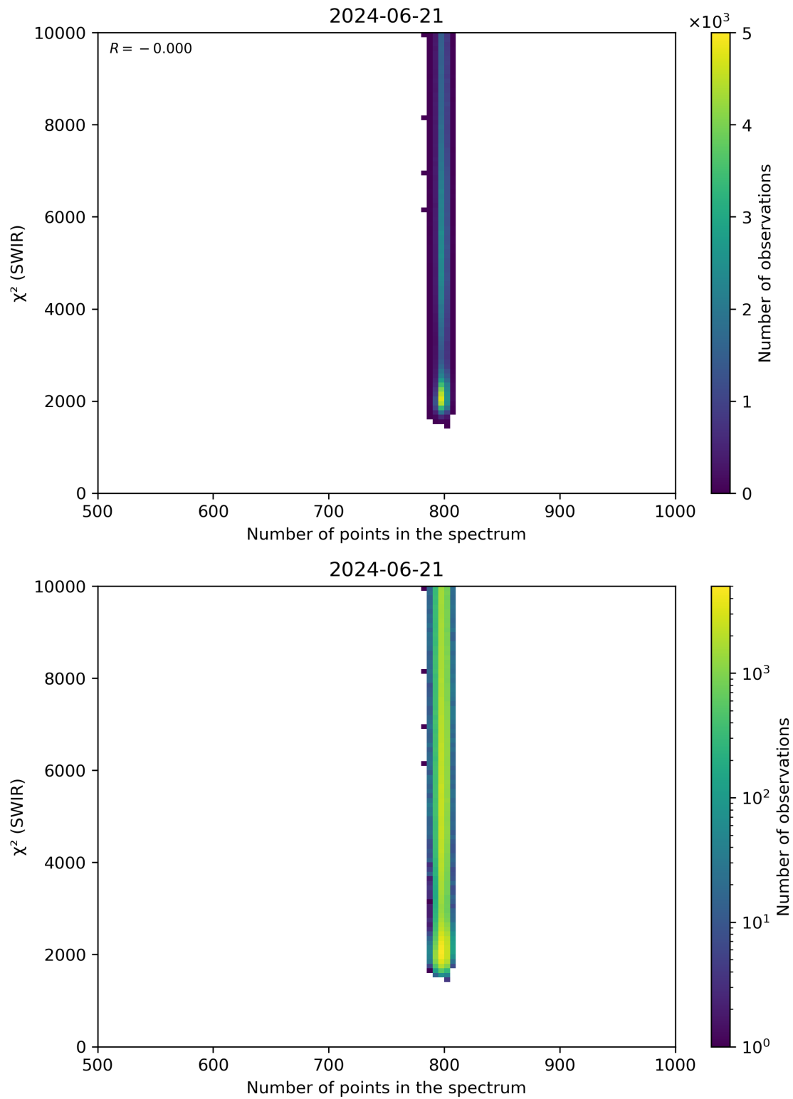
Figure 89: Scatter density plot of “Number of points in the spectrum” against “ \chi^2 (SWIR)” for 2024-06-20 to 2024-06-22.
