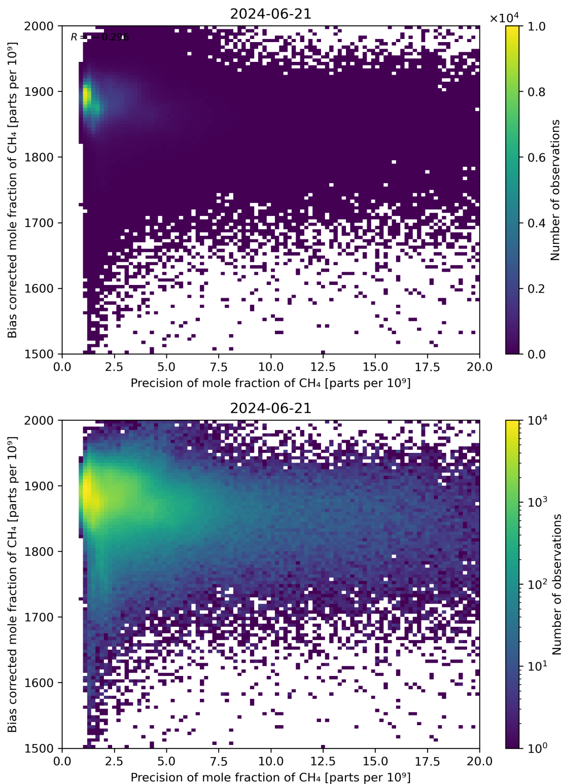
Figure 82: Scatter density plot of “Precision of mole fraction of CH 4 ” against “Bias corrected mole fraction of CH 4 ” for 2024-06-20 to 2024-06-22.
