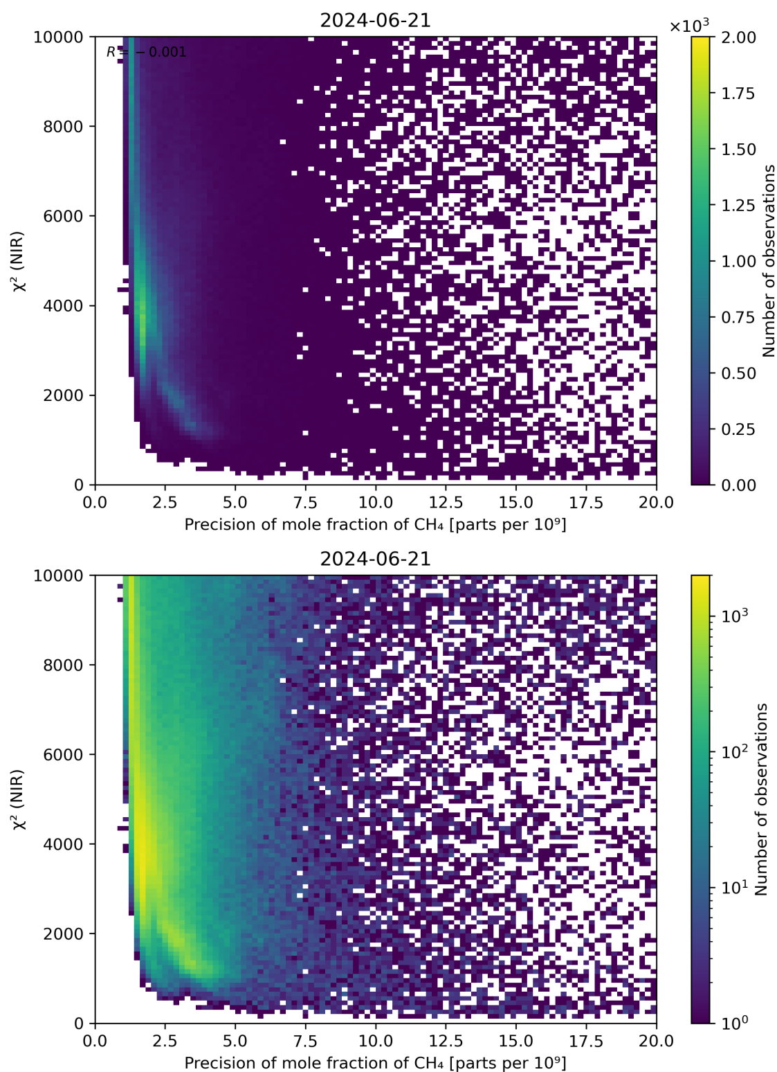
Figure 78: Scatter density plot of “Precision of mole fraction of CH 4 ” against “ \chi^2 (NIR)” for 2024-06-20 to 2024-06-22.
