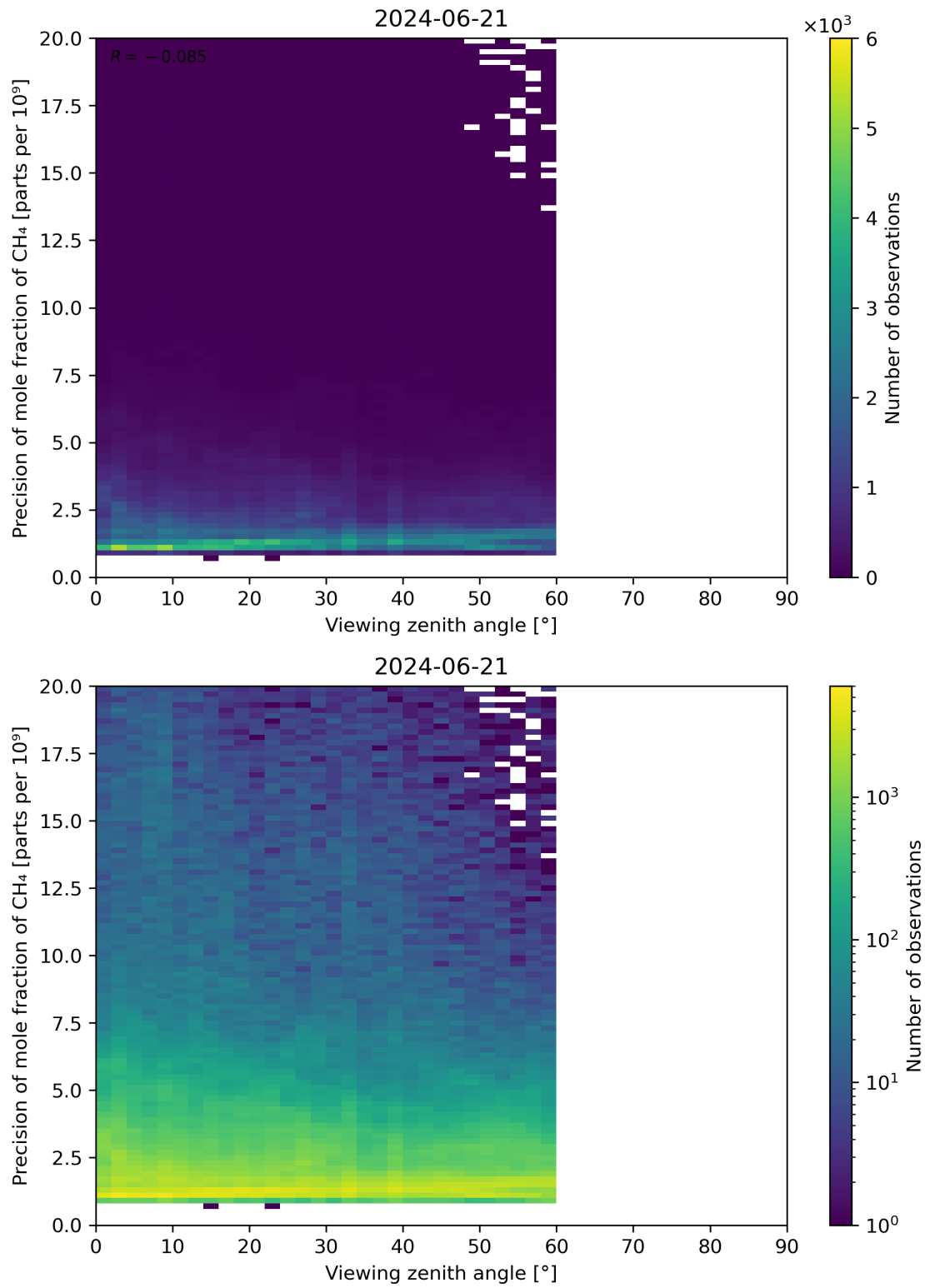
Figure 112: Scatter density plot of “Viewing zenith angle” against “Precision of mole fraction of CH 4 ” for 2024-06-20 to 2024-06-22.
