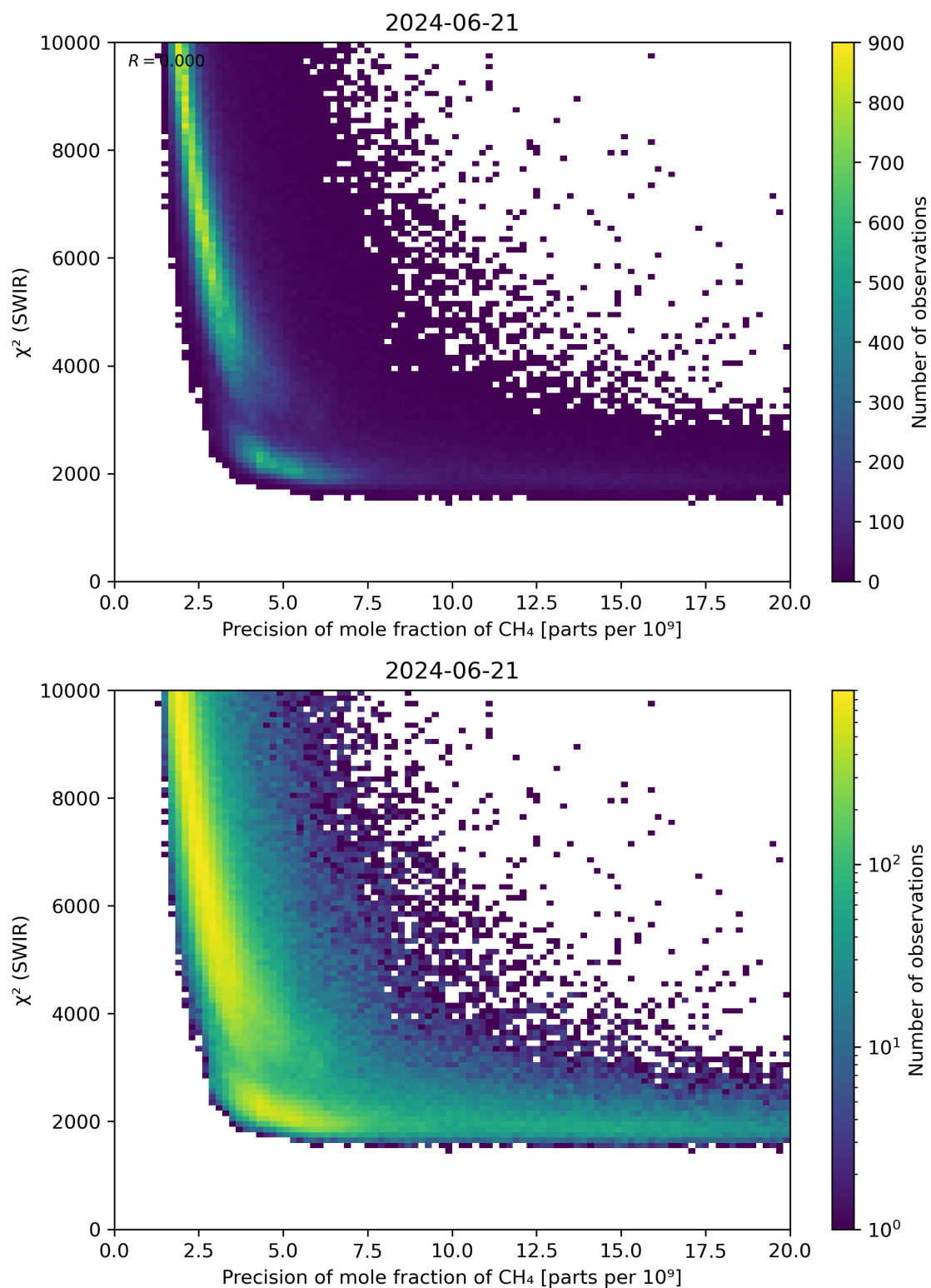
Figure 79: Scatter density plot of “Precision of mole fraction of \text{CH}_4 ” against “ \chi^2 (SWIR)” for 2024-06-20 to 2024-06-22.
