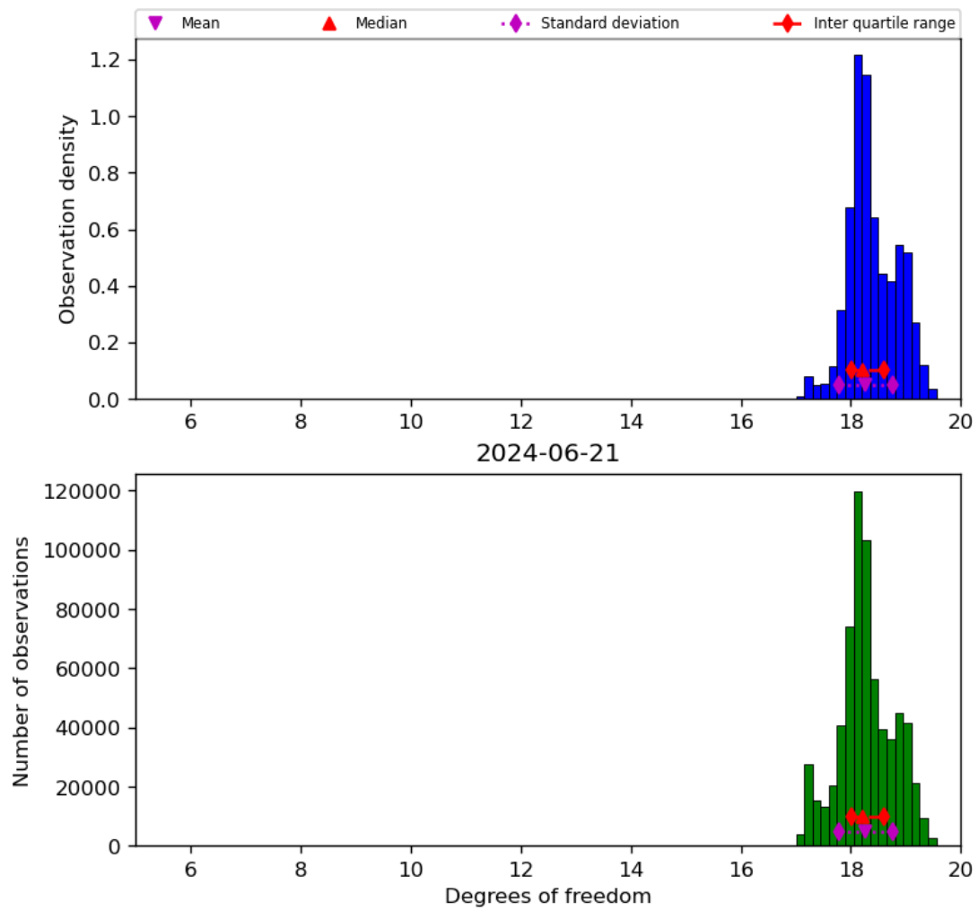
Figure 30: Histogram of “Degrees of freedom” for 2024-06-20 to 2024-06-22
