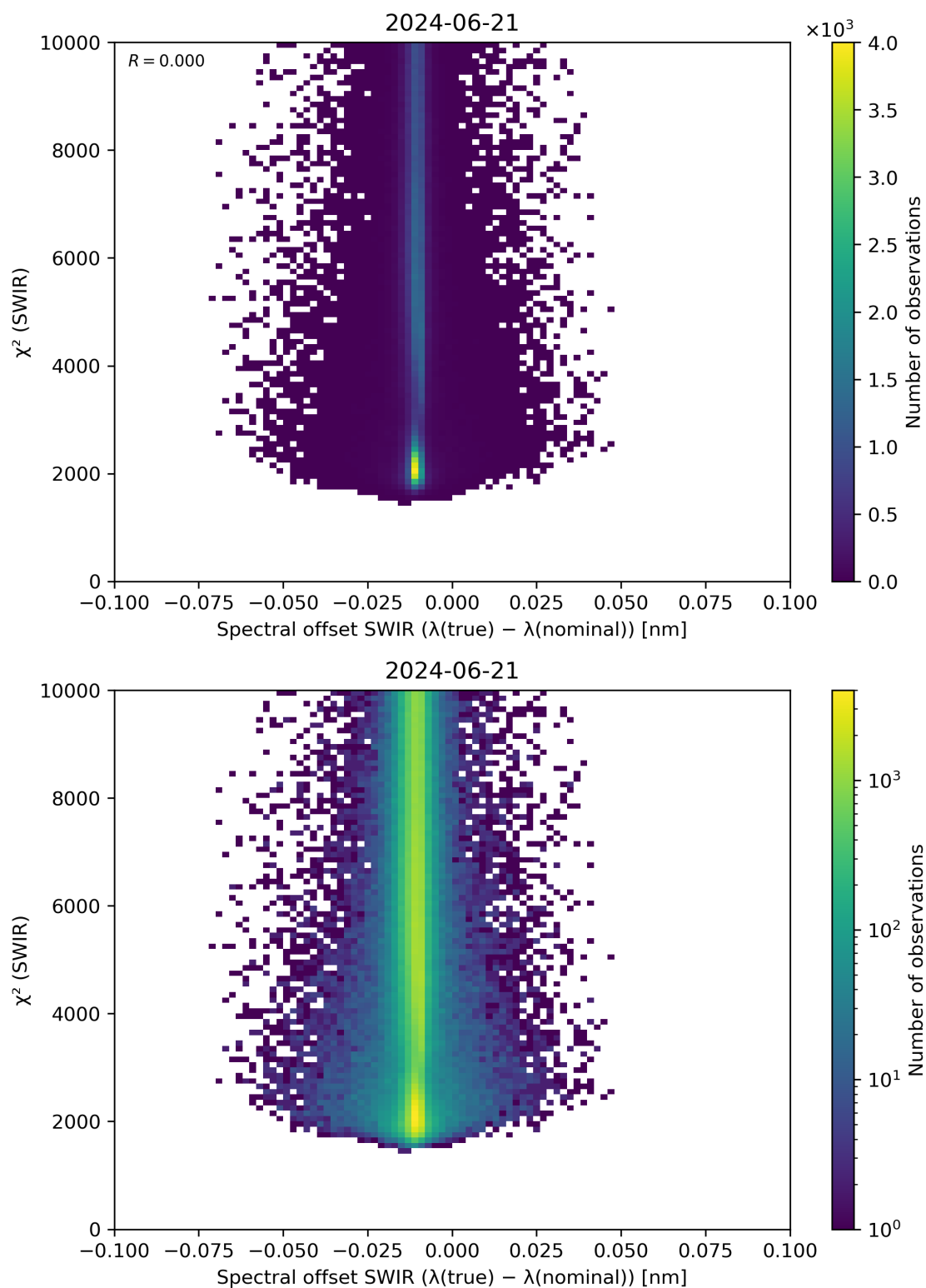
Figure 118: Scatter density plot of “Spectral offset SWIR ( \lambda(\text{true}) - \lambda(\text{nominal}) )” against “ \chi^2 (SWIR)” for 2024-06-20 to 2024-06-22.
