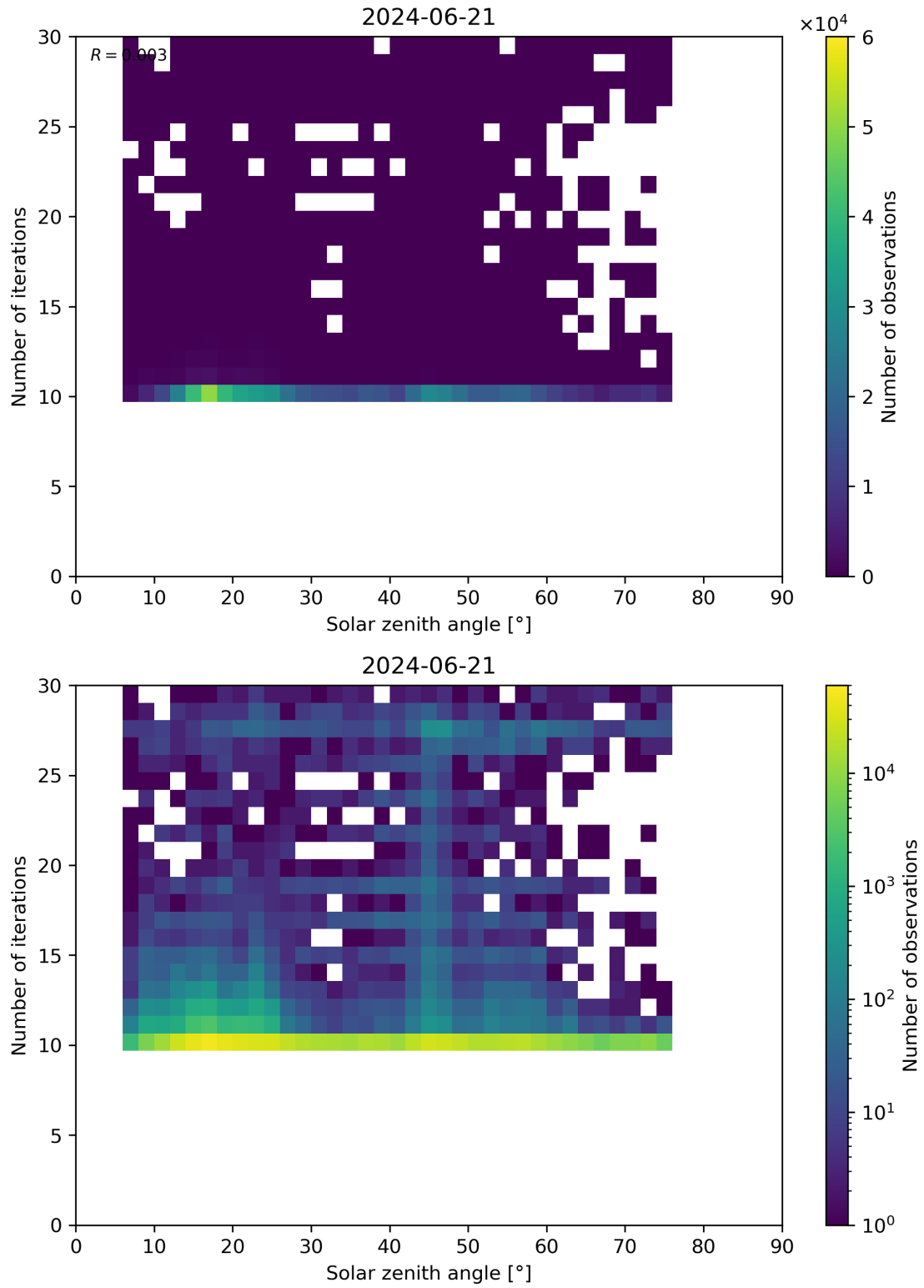
Figure 102: Scatter density plot of “Solar zenith angle” against “Number of iterations” for 2024-06-20 to 2024-06-22.
