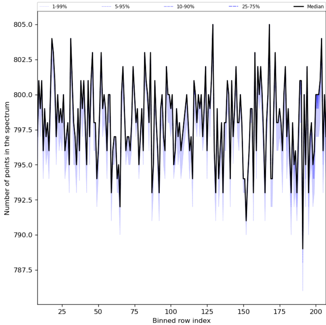
Figure 37: Along track statistics of “Number of points in the spectrum” for 2024-06-20 to 2024-06-22
