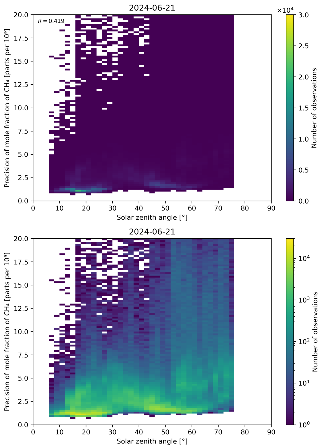
Figure 101: Scatter density plot of “Solar zenith angle” against “Precision of mole fraction of CH 4 ” for 2024-06-20 to 2024-06-22.
