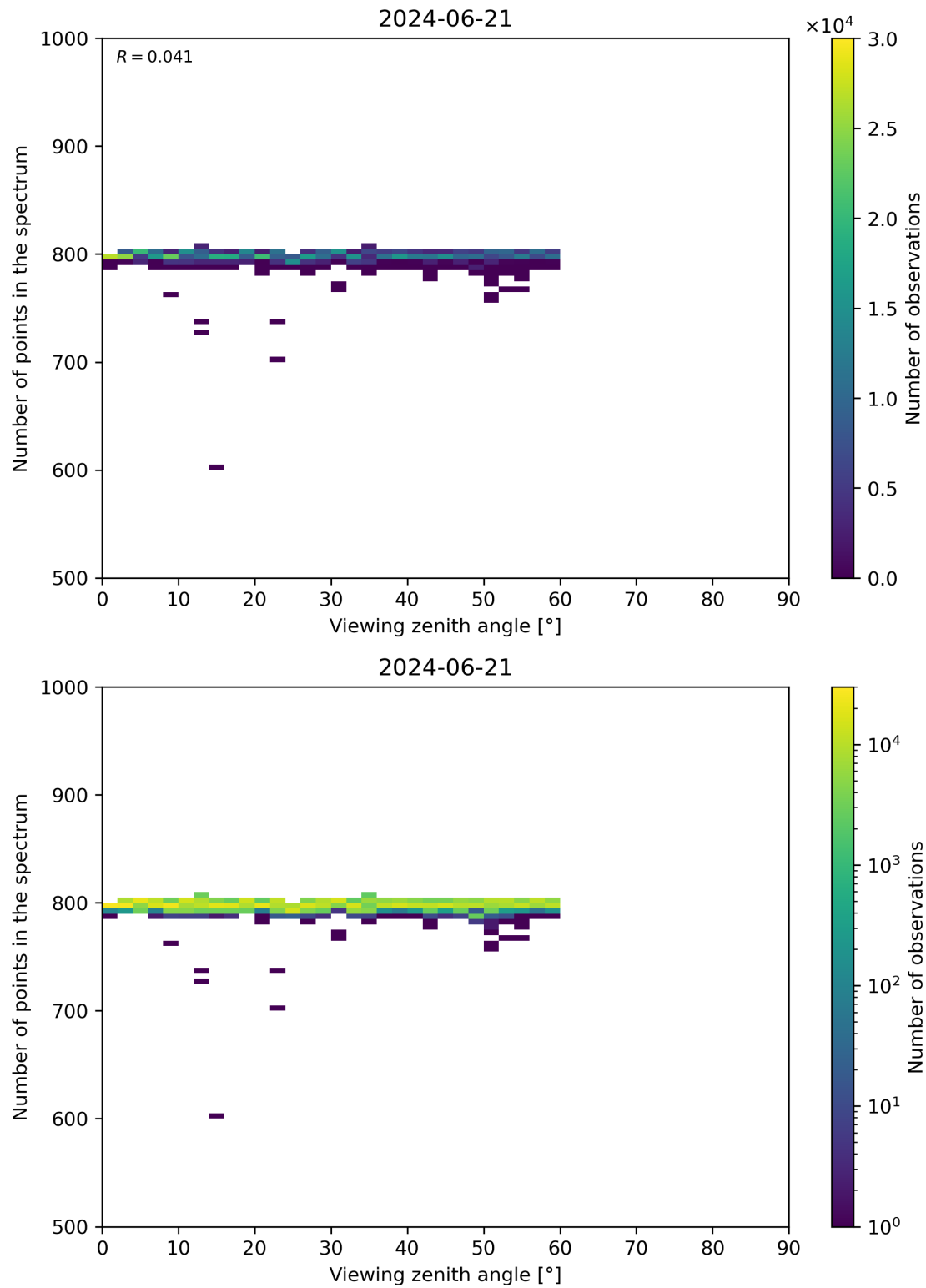
Figure 114: Scatter density plot of “Viewing zenith angle” against “Number of points in the spectrum” for 2024-06-20 to 2024-06-22.
