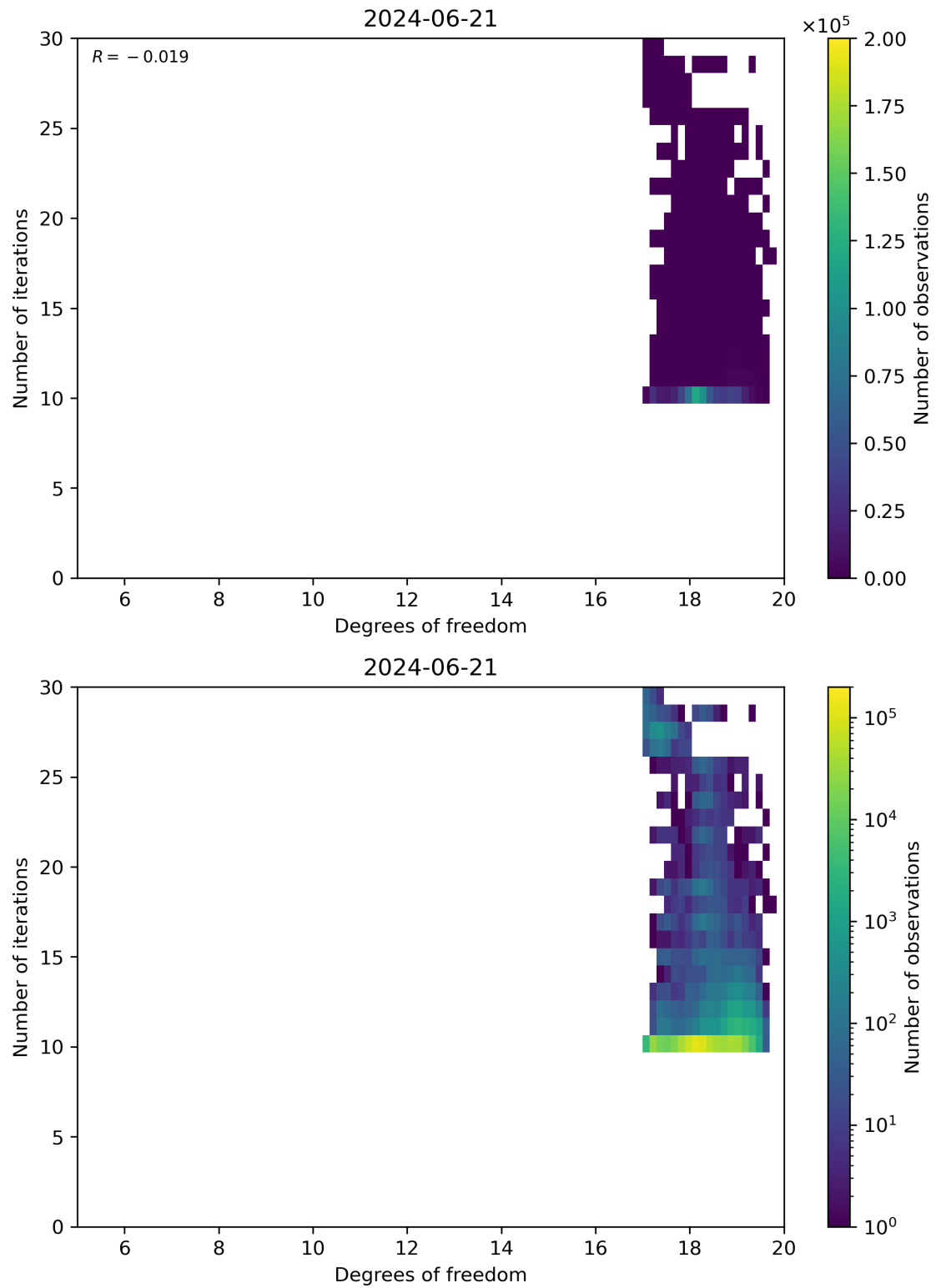
Figure 52: Scatter density plot of “Degrees of freedom” against “Number of iterations” for 2024-06-20 to 2024-06-22.
