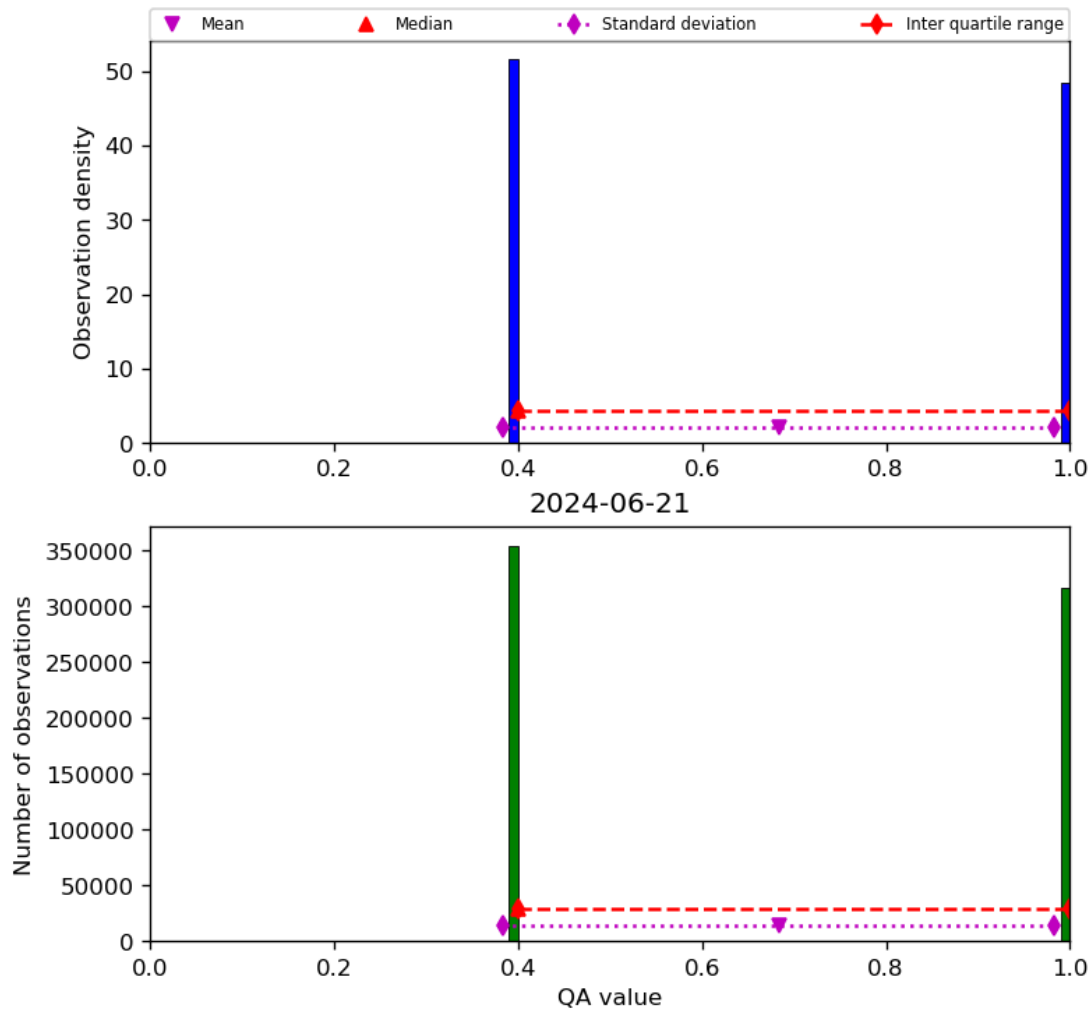
Figure 22: Histogram of “QA value” for 2024-06-20 to 2024-06-22
