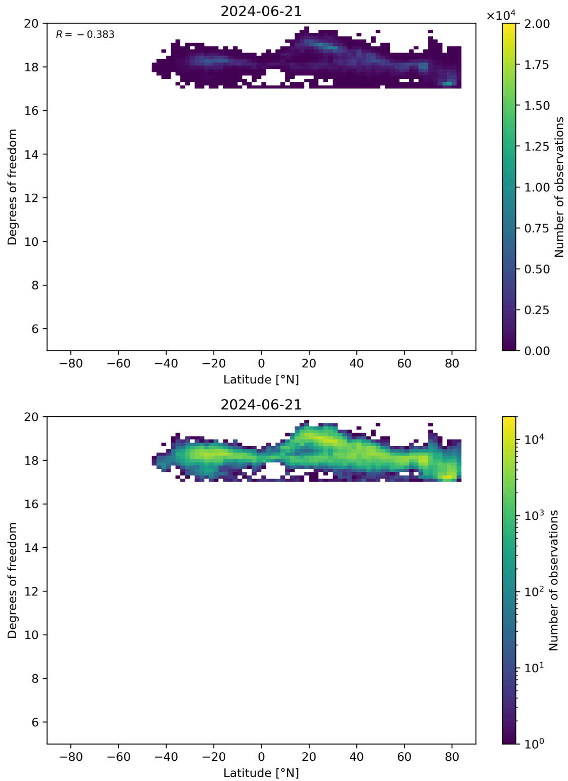
Figure 55: Scatter density plot of “Latitude” against “Degrees of freedom” for 2024-06-20 to 2024-06-22.
