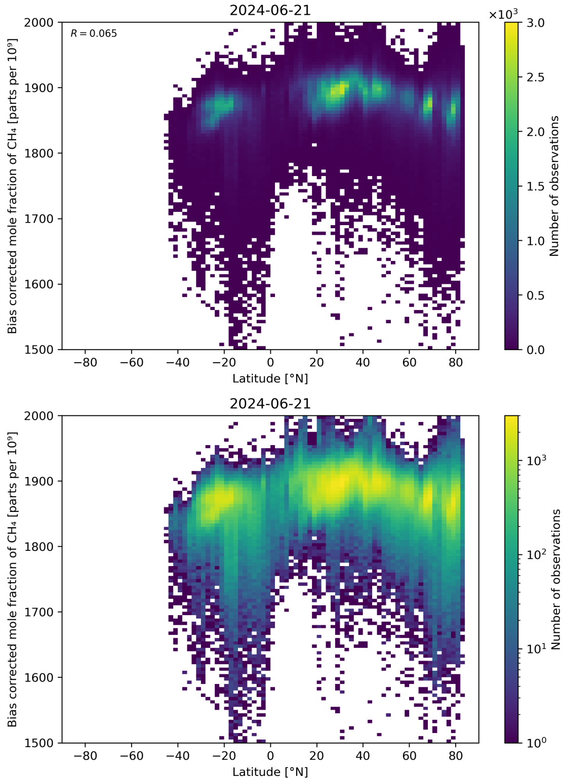
Figure 58: Scatter density plot of “Latitude” against “Bias corrected mole fraction of \text{CH}_4 ” for 2024-06-20 to 2024-06-22.
