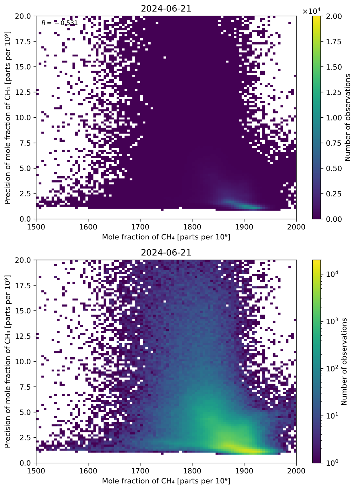
Figure 75: Scatter density plot of “Mole fraction of CH 4 ” against “Precision of mole fraction of CH 4 ” for 2024-06-20 to 2024-06-22.
