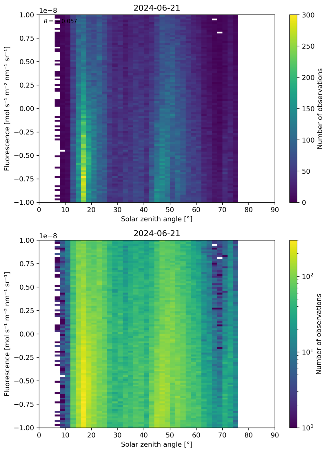
Figure 97: Scatter density plot of “Solar zenith angle” against “Fluorescence” for 2024-06-20 to 2024-06-22.
