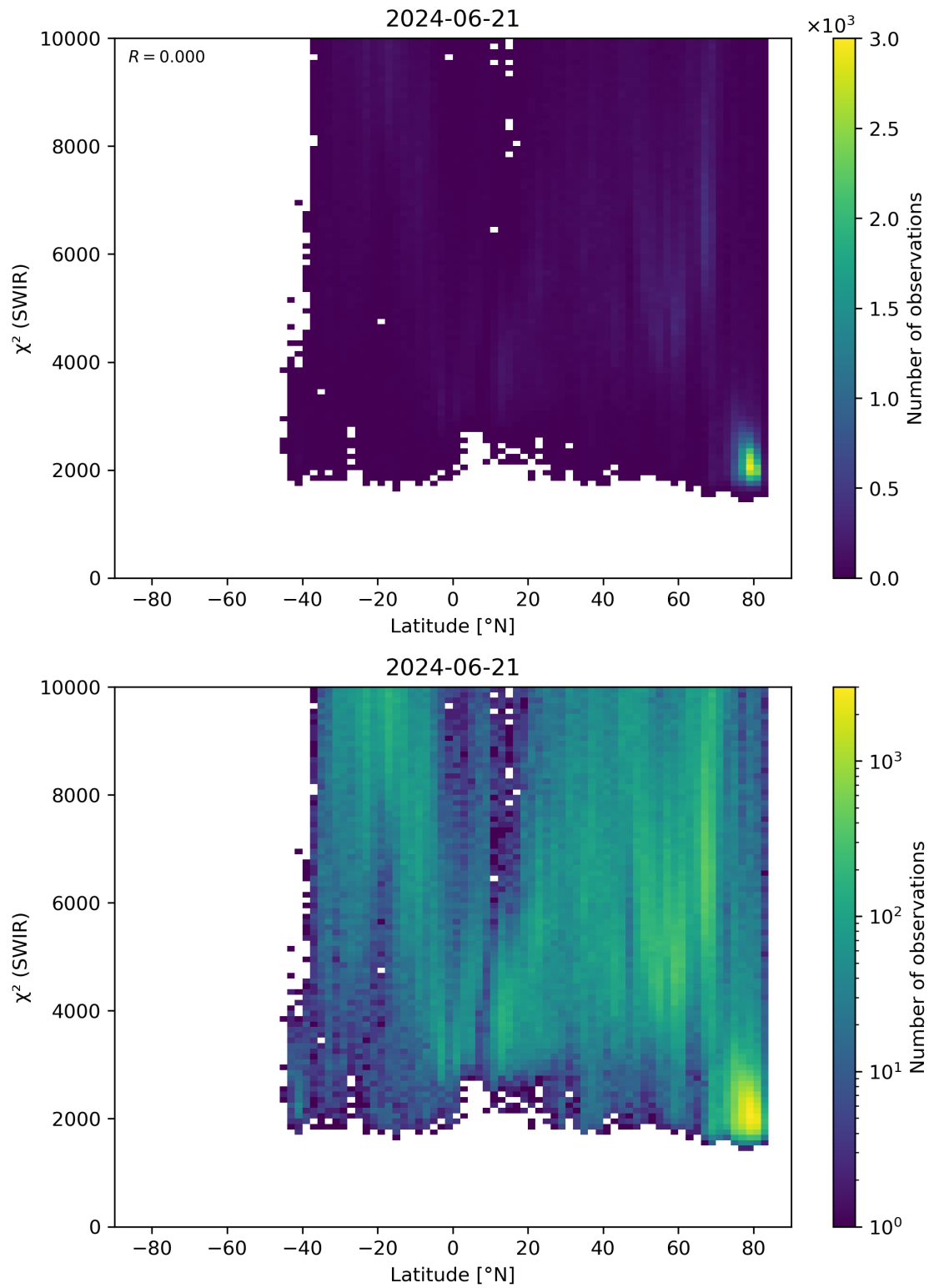
Figure 54: Scatter density plot of “Latitude” against “ \chi^2 (SWIR)” for 2024-06-20 to 2024-06-22.
