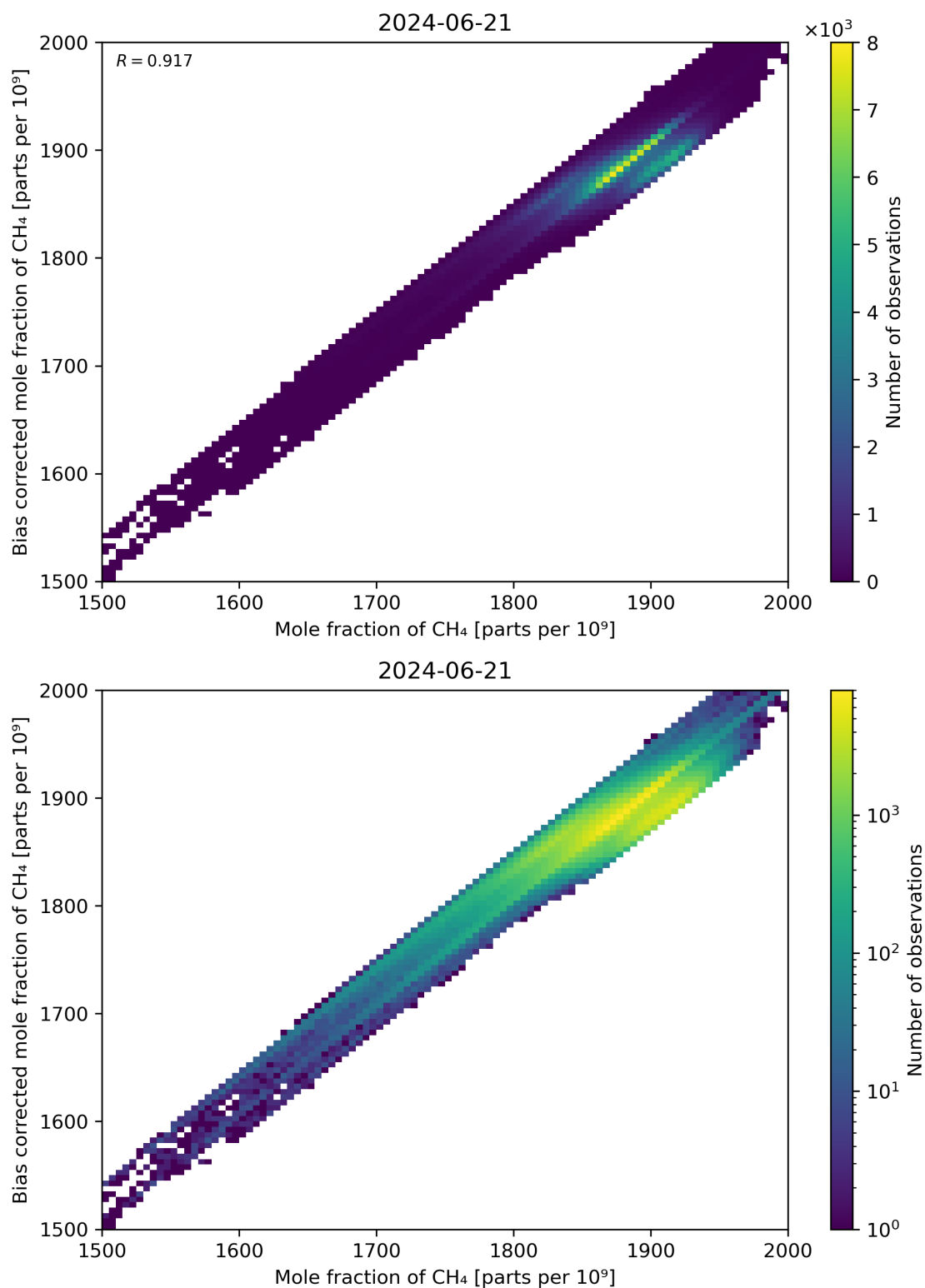
Figure 74: Scatter density plot of “Mole fraction of CH 4 ” against “Bias corrected mole fraction of CH 4 ” for 2024-06-20 to 2024-06-22.
