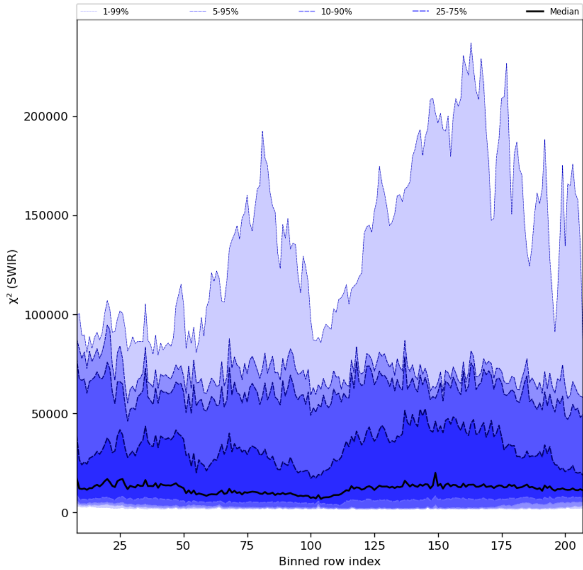
Figure 39: Along track statistics of “ \chi^2 (SWIR)” for 2024-06-20 to 2024-06-22
