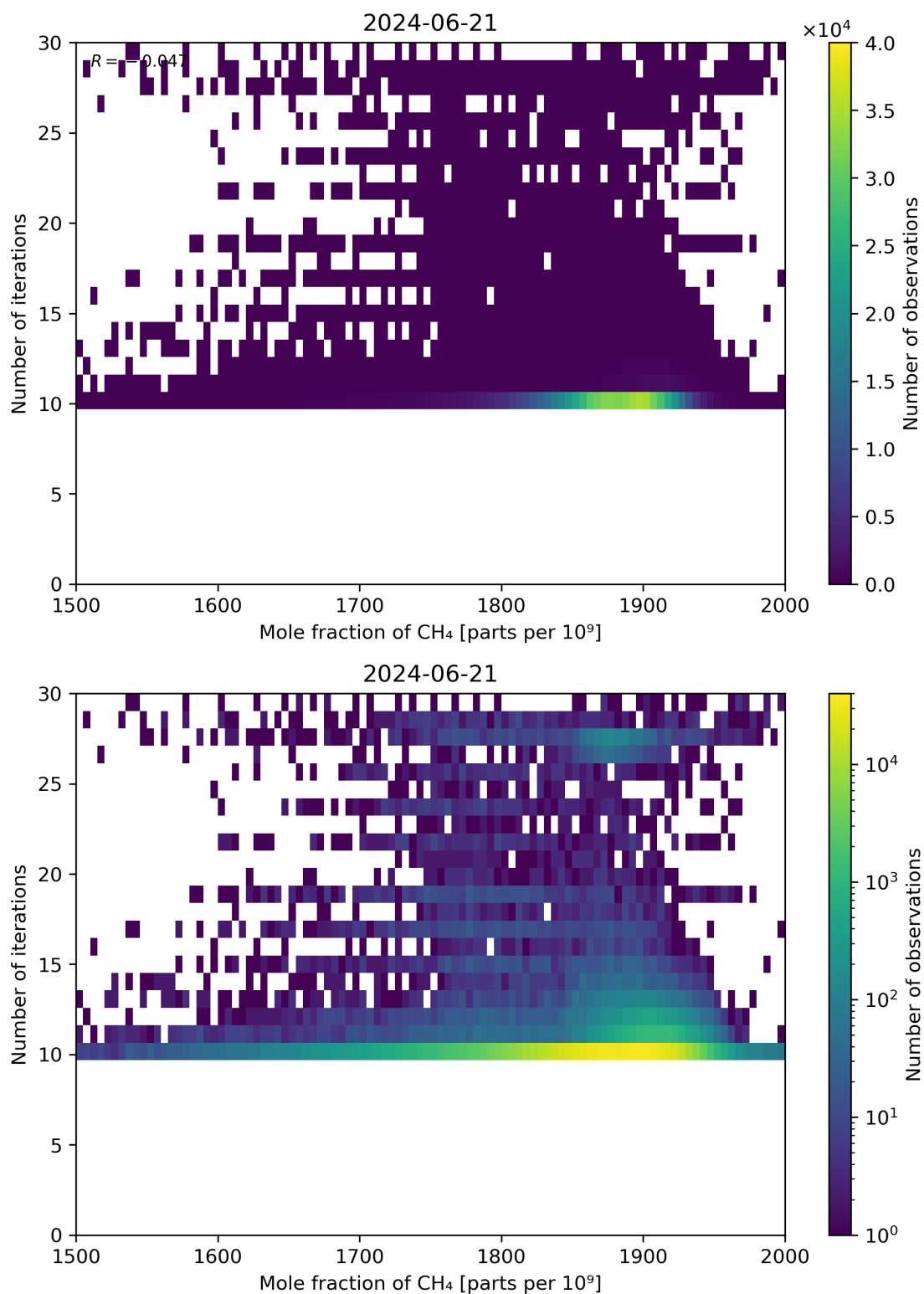
Figure 76: Scatter density plot of “Mole fraction of CH 4 ” against “Number of iterations” for 2024-06-20 to 2024-06-22.
