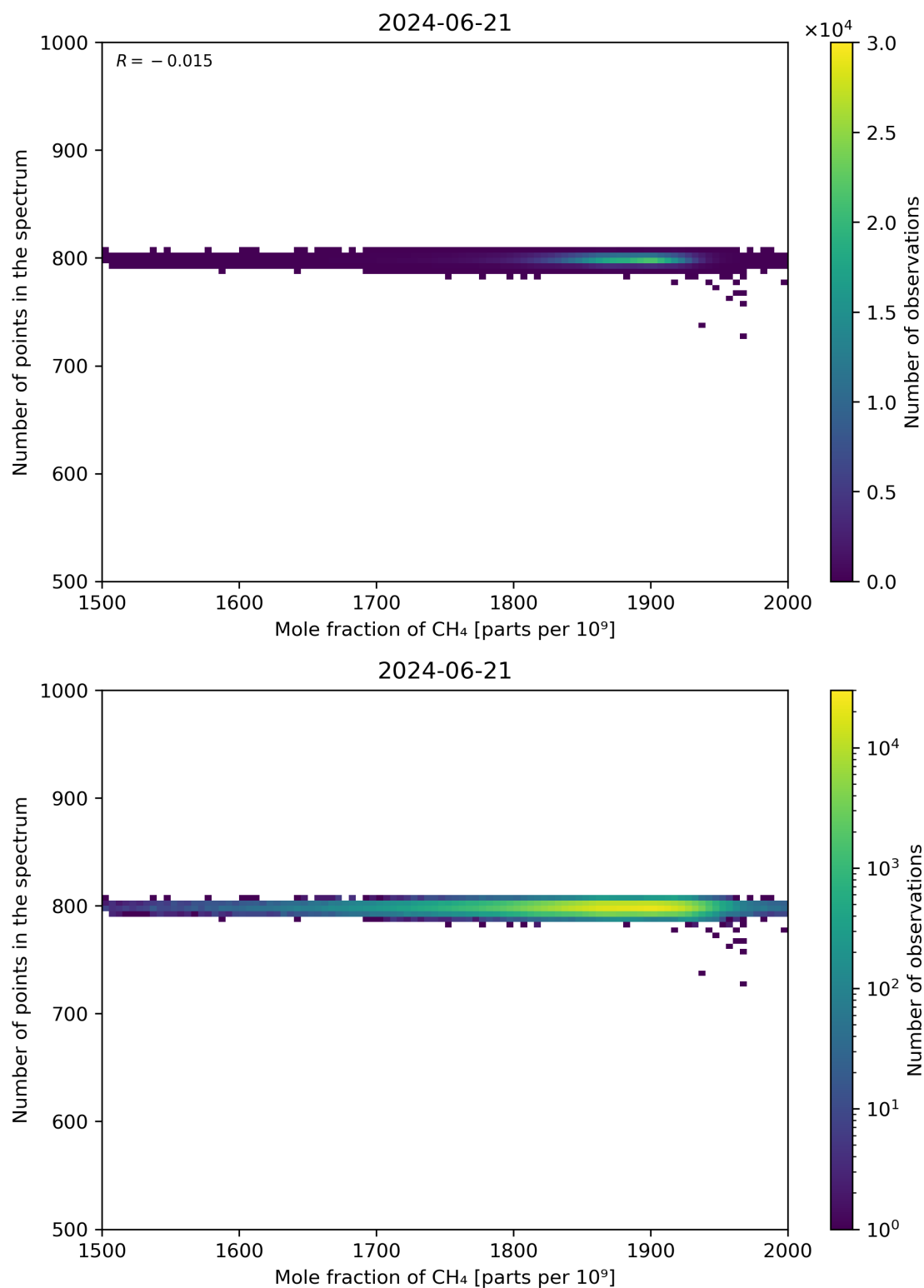
Figure 77: Scatter density plot of “Mole fraction of CH 4 ” against “Number of points in the spectrum” for 2024-06-20 to 2024-06-22.
