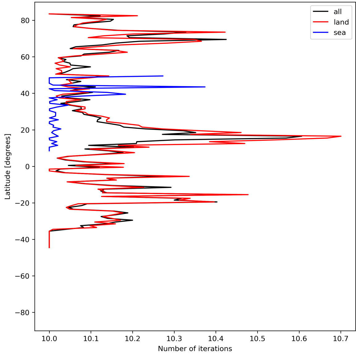
Figure 20: Zonal average of “Number of iterations” for 2024-06-20 to 2024-06-22.
