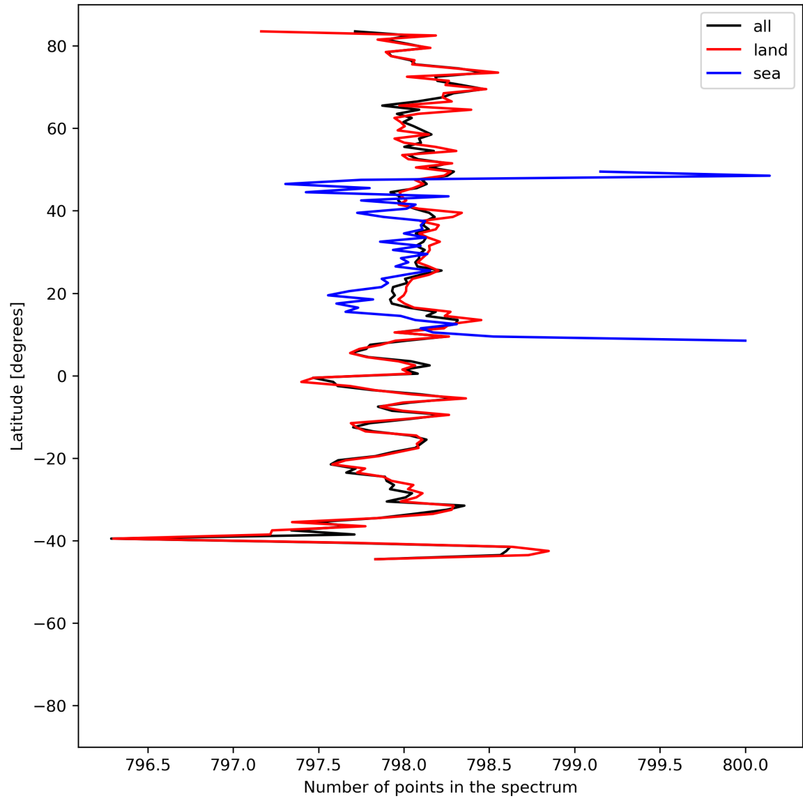
Figure 15: Zonal average of “Number of points in the spectrum” for 2024-06-20 to 2024-06-22.
