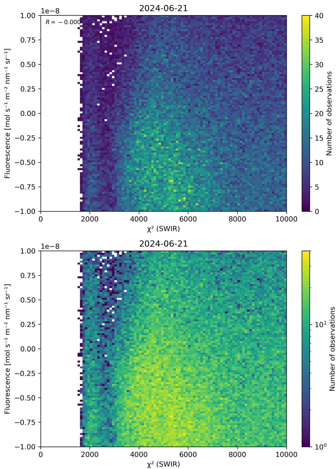
Figure 49: Scatter density plot of “ \chi^2 (SWIR)” against “Fluorescence” for 2024-06-20 to 2024-06-22.
