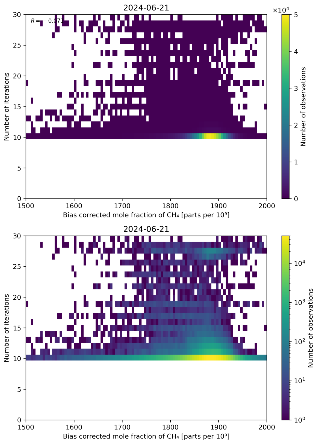
Figure 67: Scatter density plot of “Bias corrected mole fraction of CH 4 ” against “Number of iterations” for 2024-06-20 to 2024-06-22.
