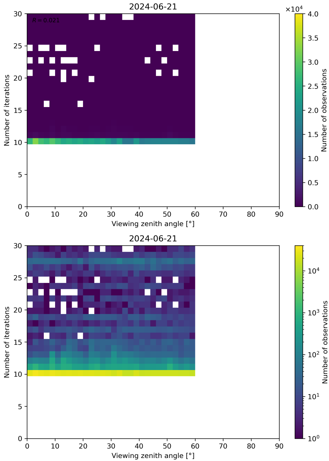
Figure 113: Scatter density plot of “Viewing zenith angle” against “Number of iterations” for 2024-06-20 to 2024-06-22.
