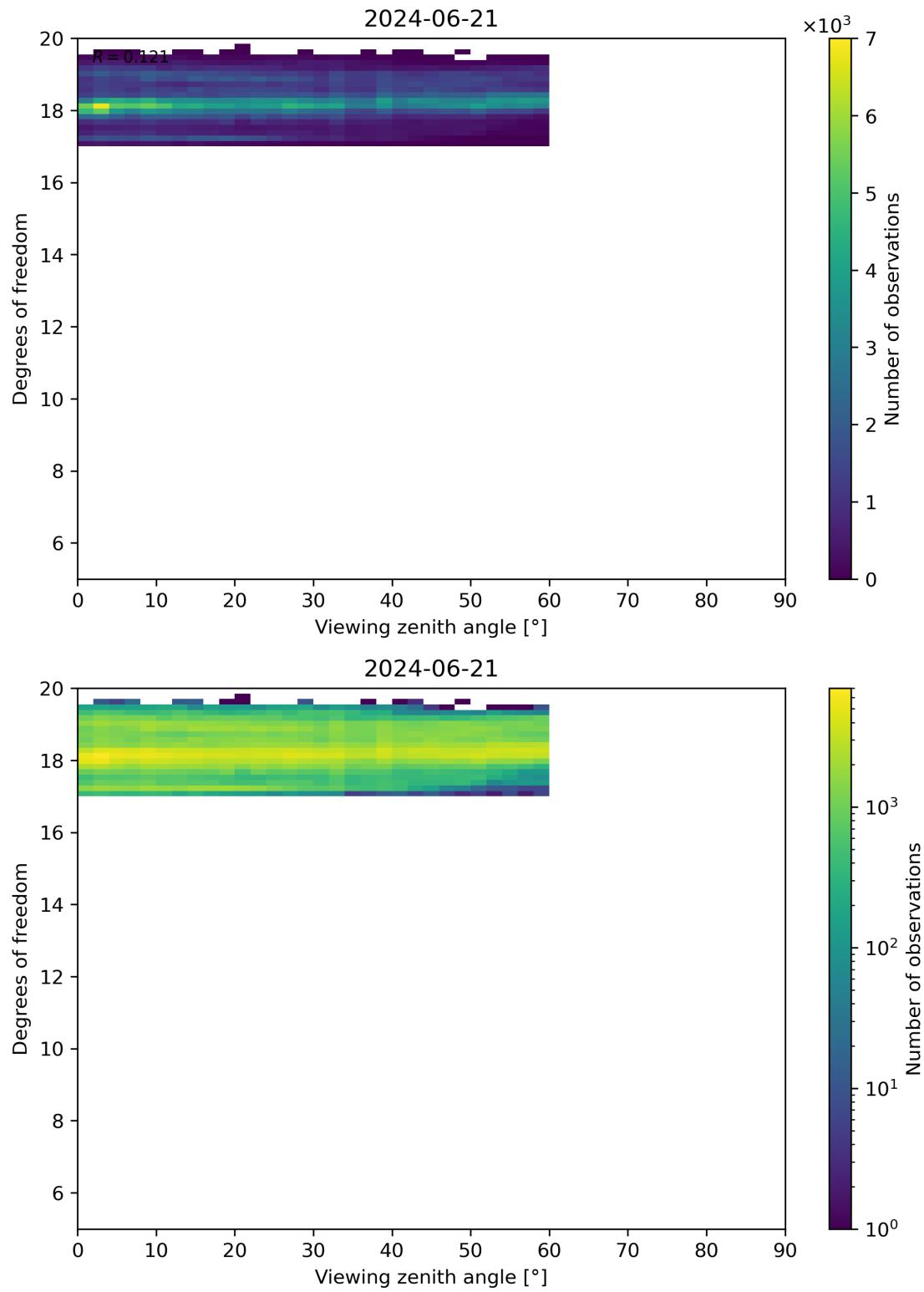
Figure 107: Scatter density plot of “Viewing zenith angle” against “Degrees of freedom” for 2024-06-20 to 2024-06-22.
