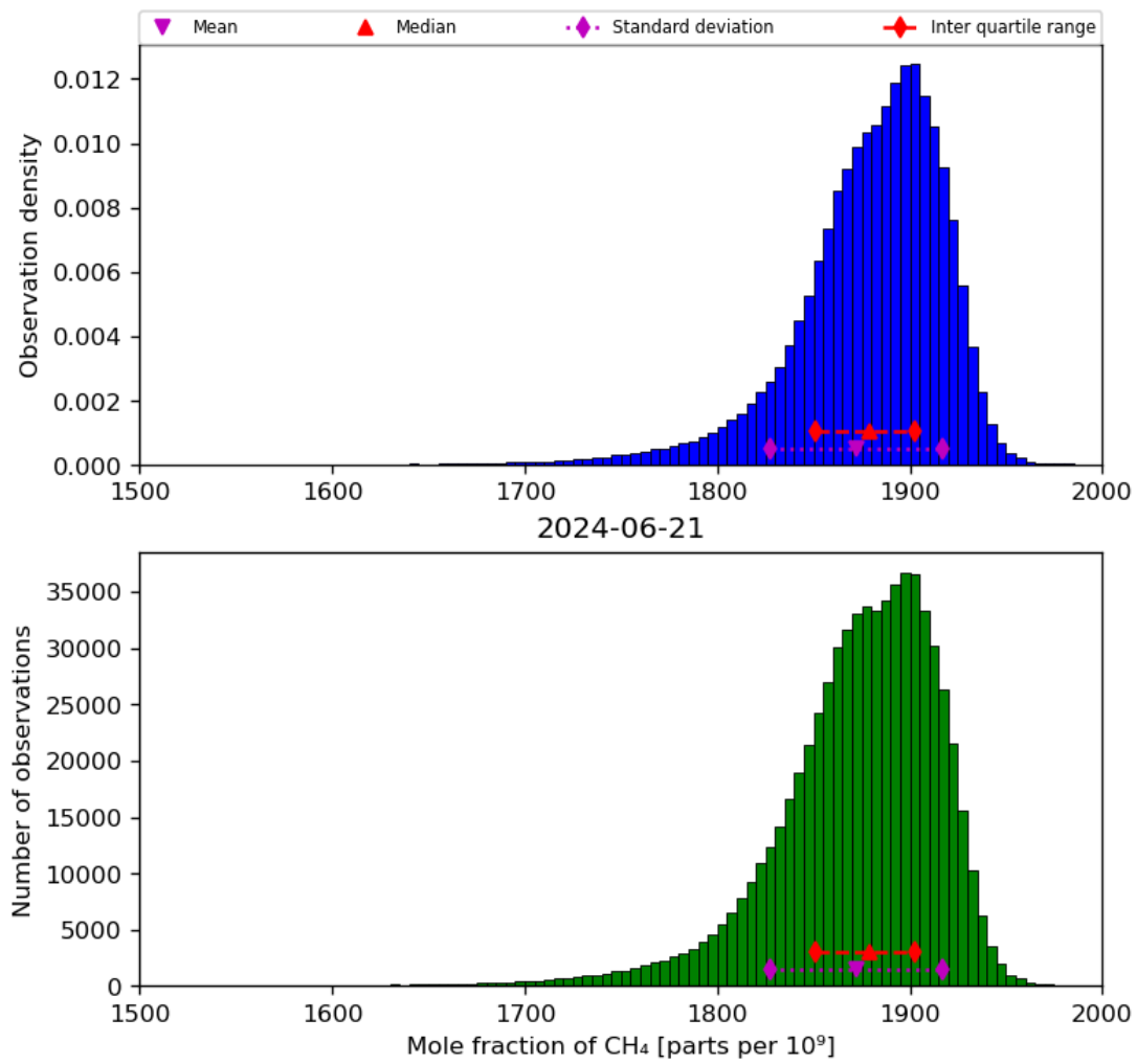
Figure 23: Histogram of “Mole fraction of CH 4 ” for 2024-06-20 to 2024-06-22
