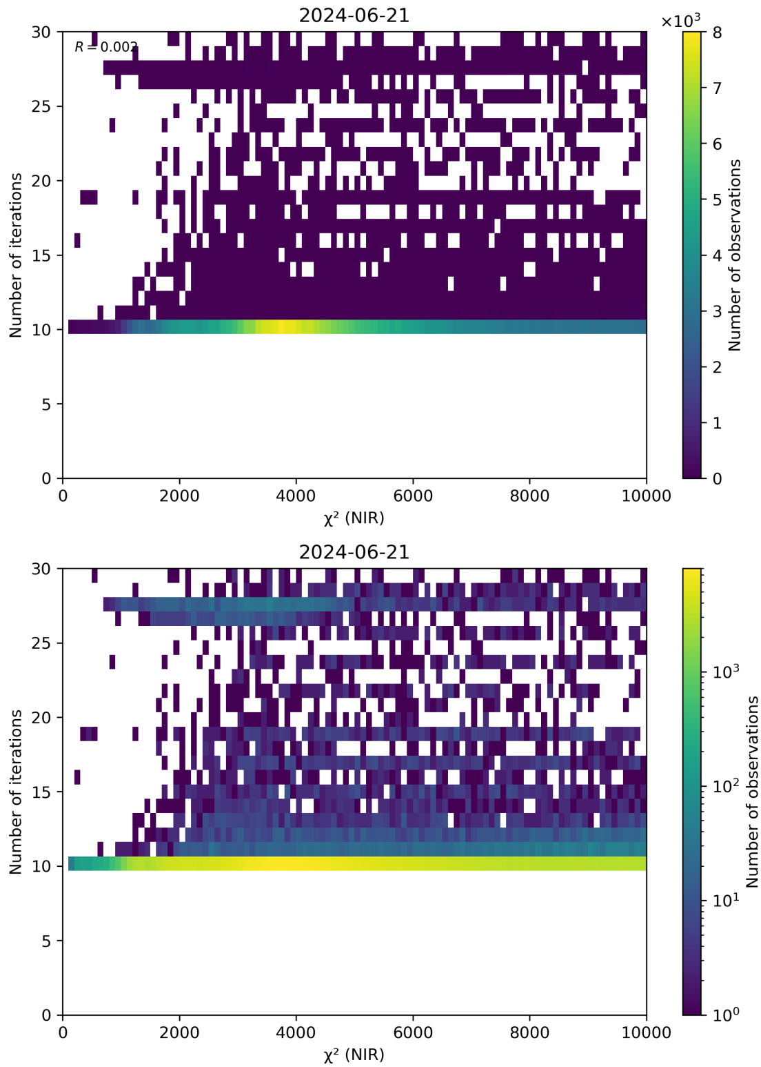
Figure 46: Scatter density plot of “ \chi^2 (NIR)” against “Number of iterations” for 2024-06-20 to 2024-06-22.
