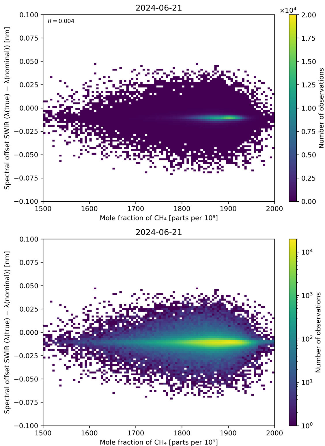
Figure 86: Scatter density plot of “Mole fraction of CH 4 ” against “Spectral offset SWIR ( \lambda(\text{true}) - \lambda(\text{nominal}) )” for 2024-06-20 to 2024-06-22.
