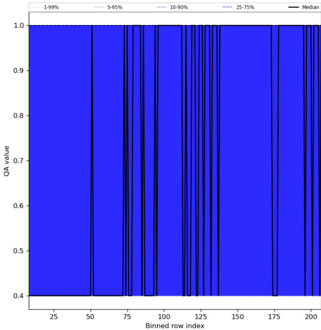
Figure 33: Along track statistics of “QA value” for 2024-06-21 to 2024-06-23
