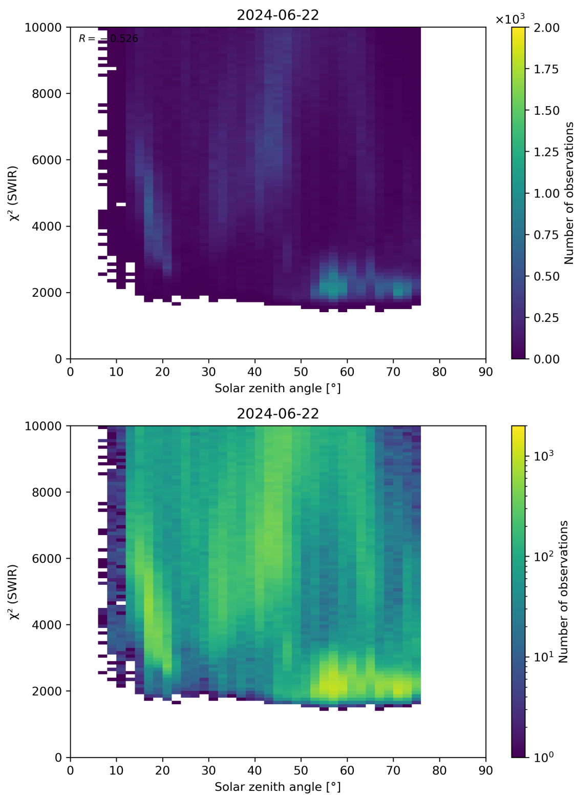
Figure 95: Scatter density plot of “Solar zenith angle” against “ \chi^2 (SWIR)” for 2024-06-21 to 2024-06-23.
