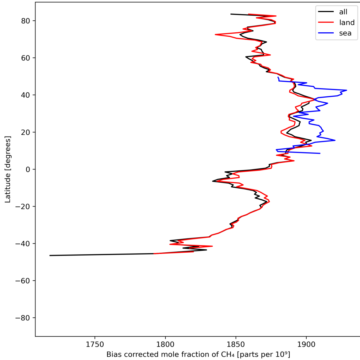
Figure 14: Zonal average of “Bias corrected mole fraction of CH 4 ” for 2024-06-21 to 2024-06-23.
