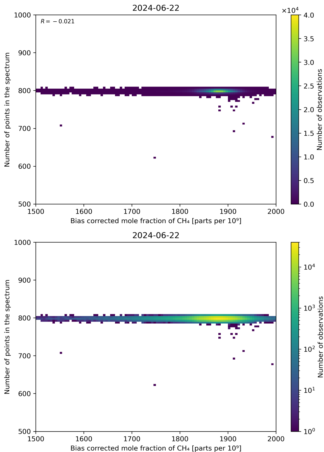
Figure 68: Scatter density plot of “Bias corrected mole fraction of CH 4 ” against “Number of points in the spectrum” for 2024-06-21 to 2024-06-23.
