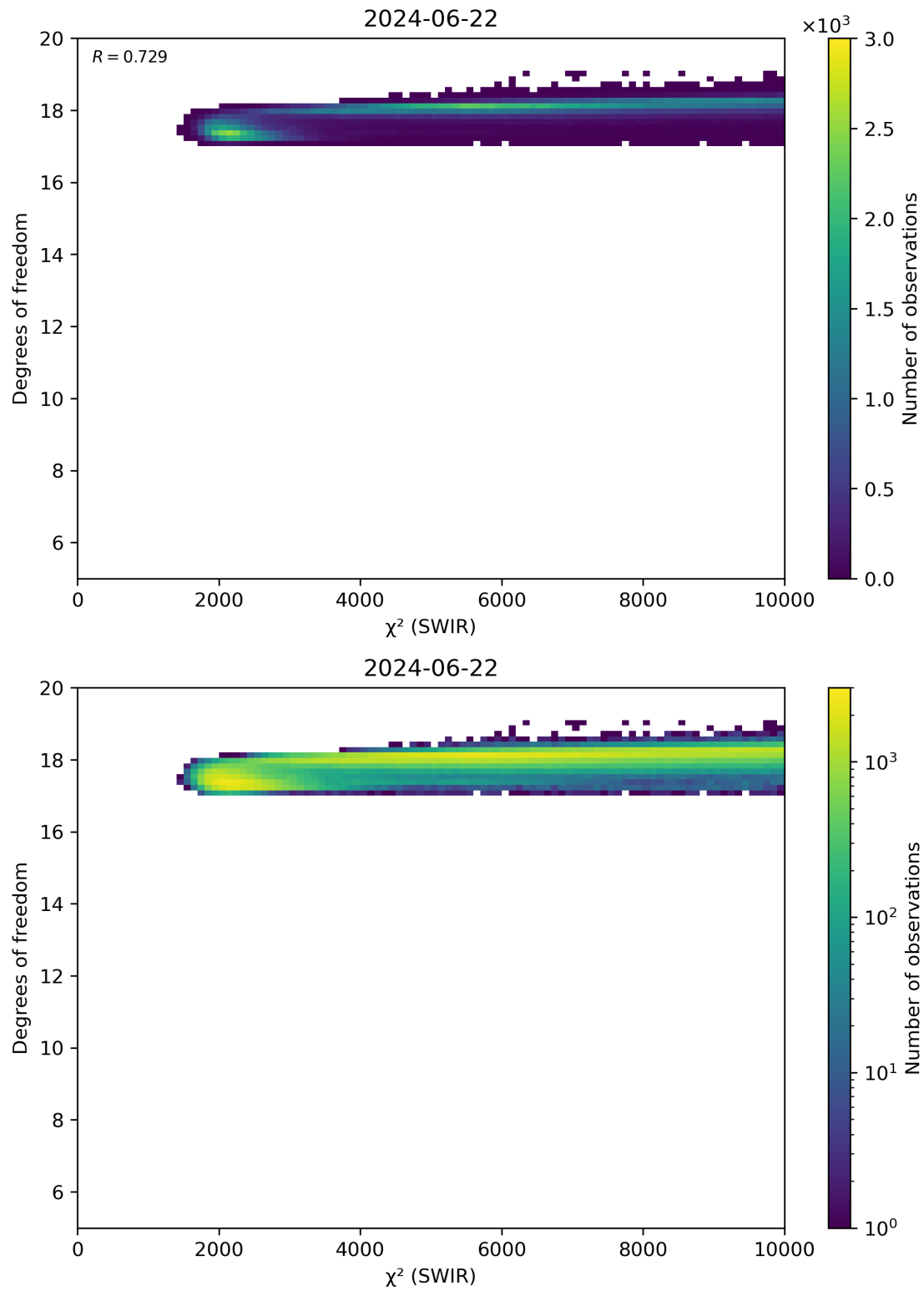
Figure 48: Scatter density plot of “ \chi^2 (SWIR)” against “Degrees of freedom” for 2024-06-21 to 2024-06-23.
