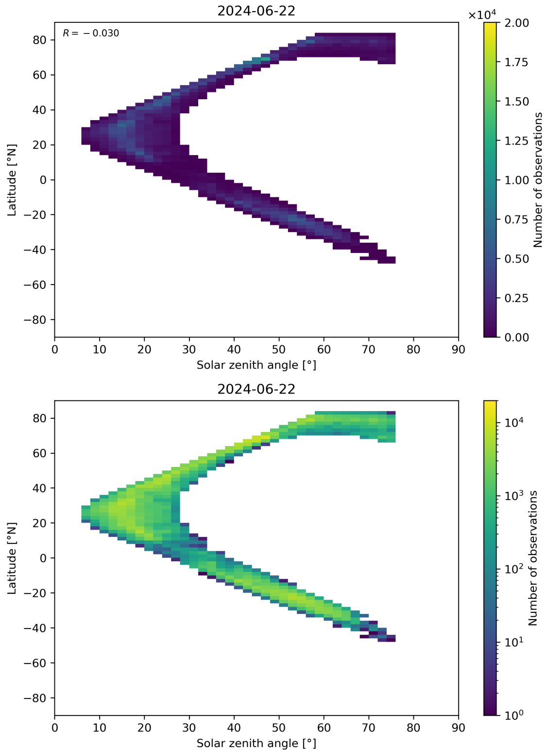
Figure 98: Scatter density plot of “Solar zenith angle” against “Latitude” for 2024-06-21 to 2024-06-23.
