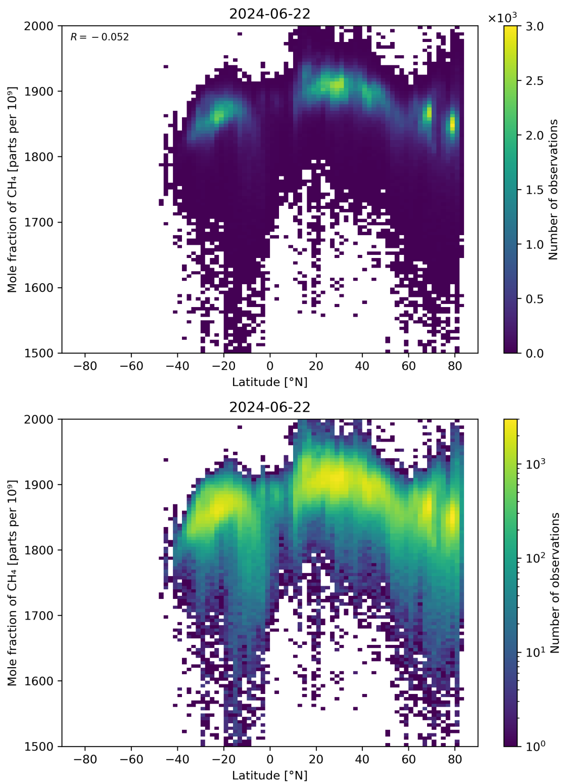
Figure 57: Scatter density plot of “Latitude” against “Mole fraction of CH 4 ” for 2024-06-21 to 2024-06-23.
