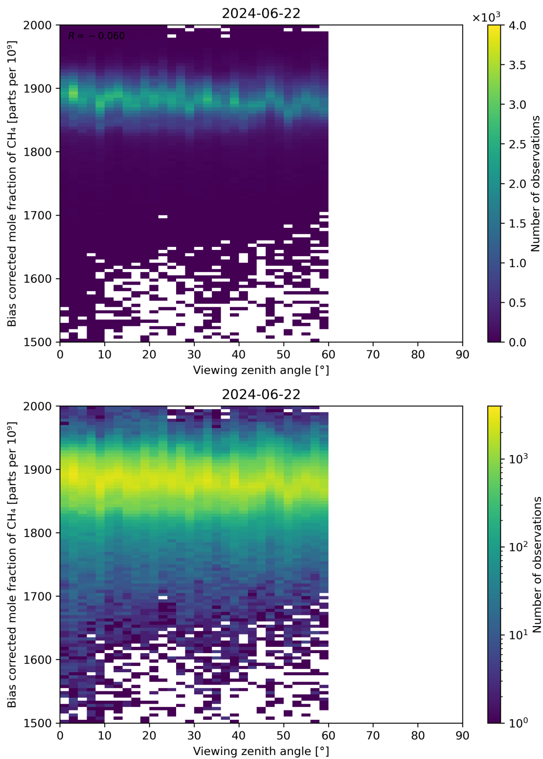
Figure 111: Scatter density plot of “Viewing zenith angle” against “Bias corrected mole fraction of CH 4 ” for 2024-06-21 to 2024-06-23.
