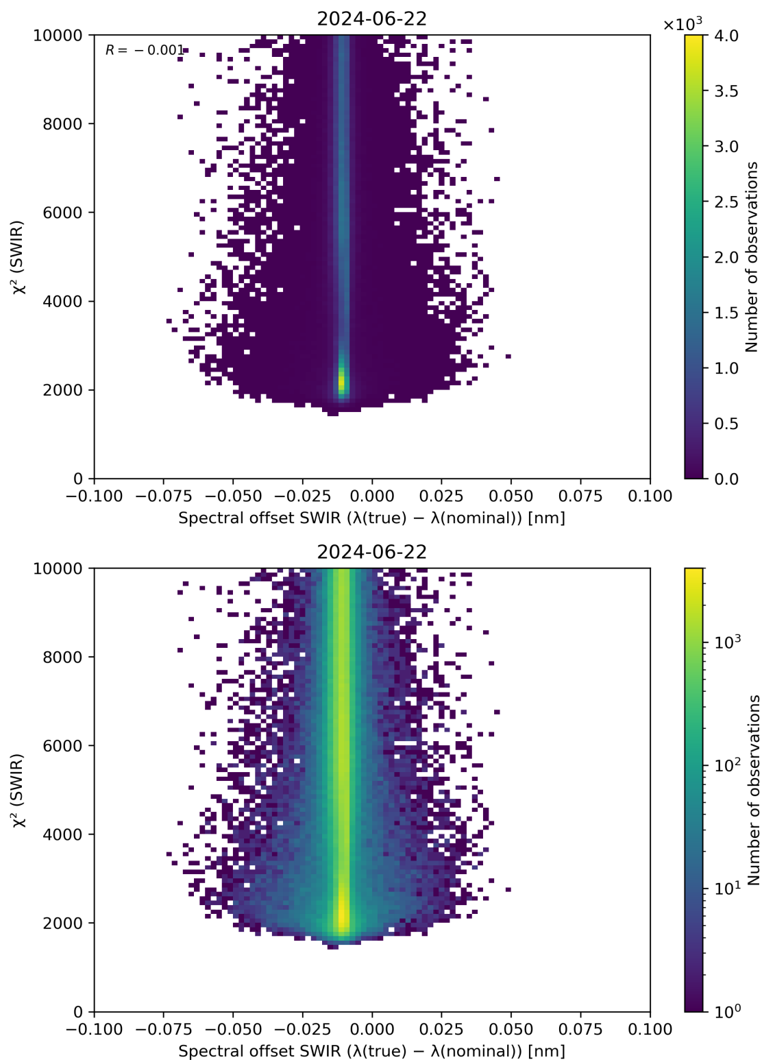
Figure 118: Scatter density plot of “Spectral offset SWIR ( \lambda(\text{true}) - \lambda(\text{nominal}) )” against “ \chi^2 (SWIR)” for 2024-06-21 to 2024-06-23.
