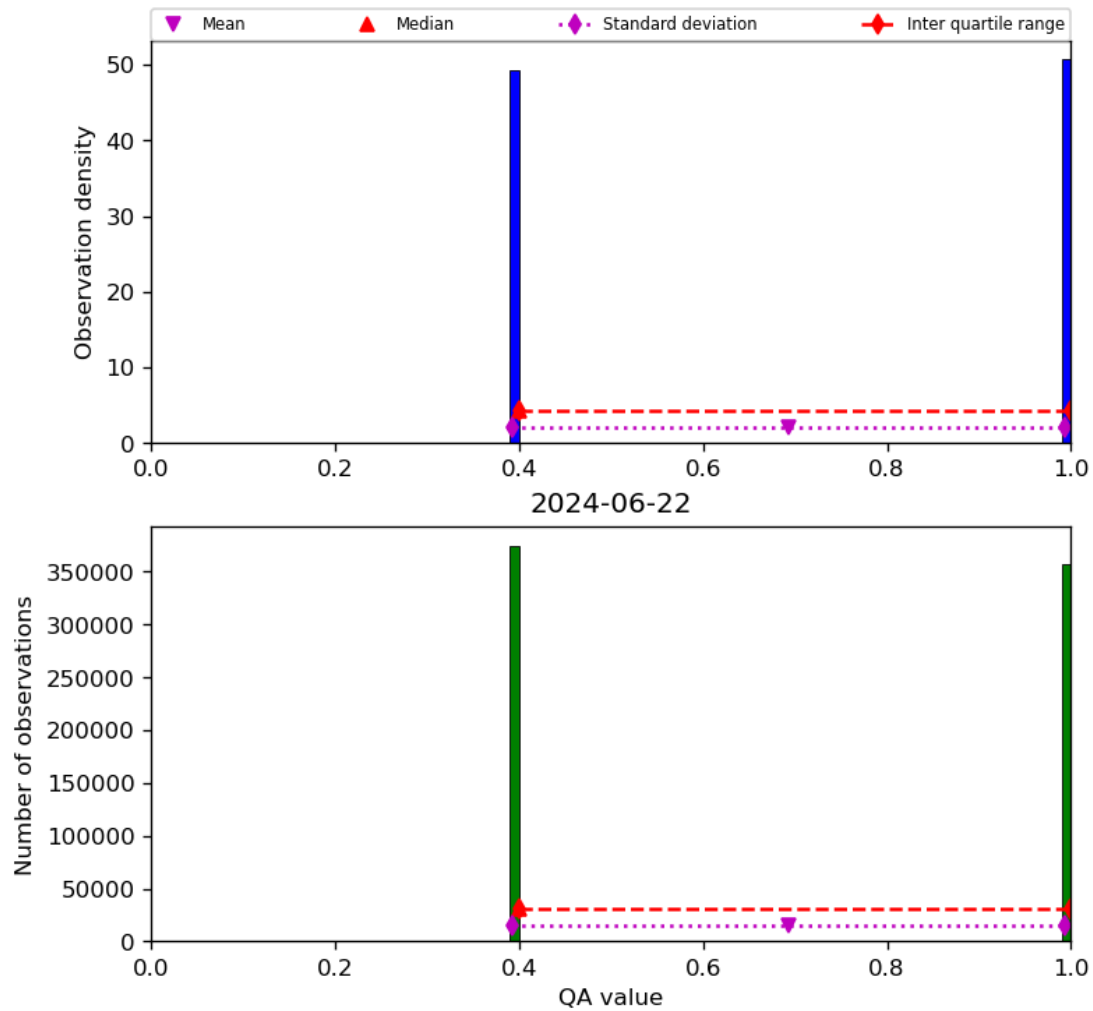
Figure 22: Histogram of “QA value” for 2024-06-21 to 2024-06-23
