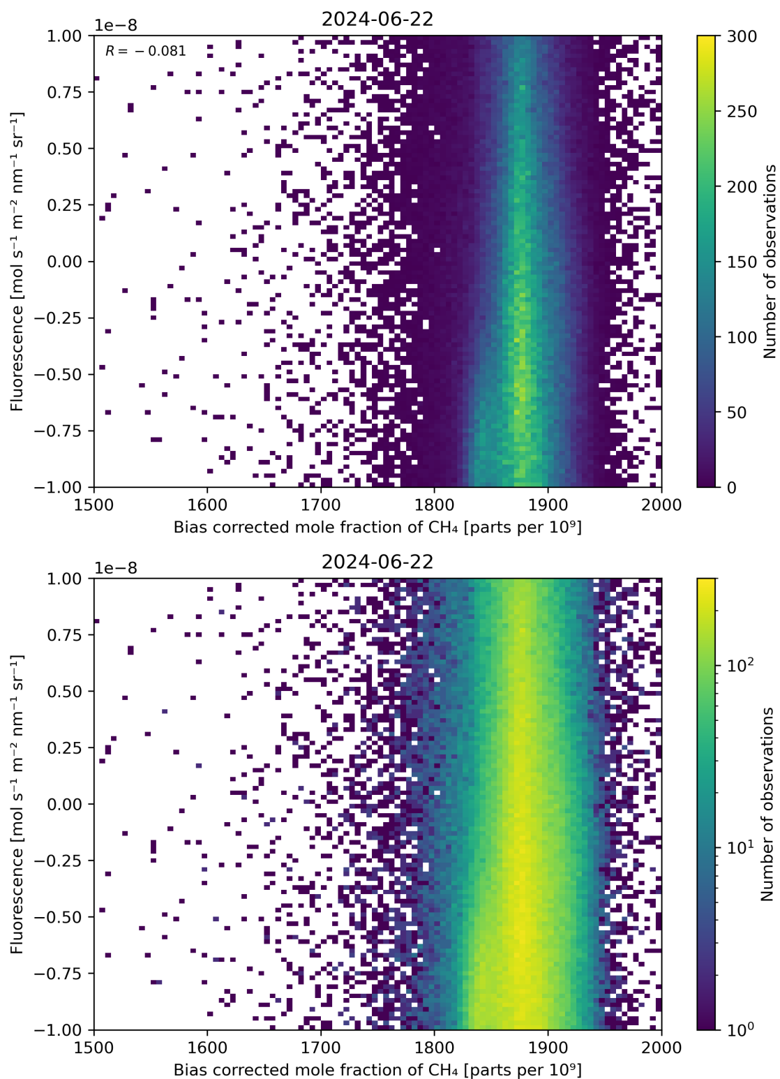
Figure 66: Scatter density plot of “Bias corrected mole fraction of \text{CH}_4 ” against “Fluorescence” for 2024-06-21 to 2024-06-23.
