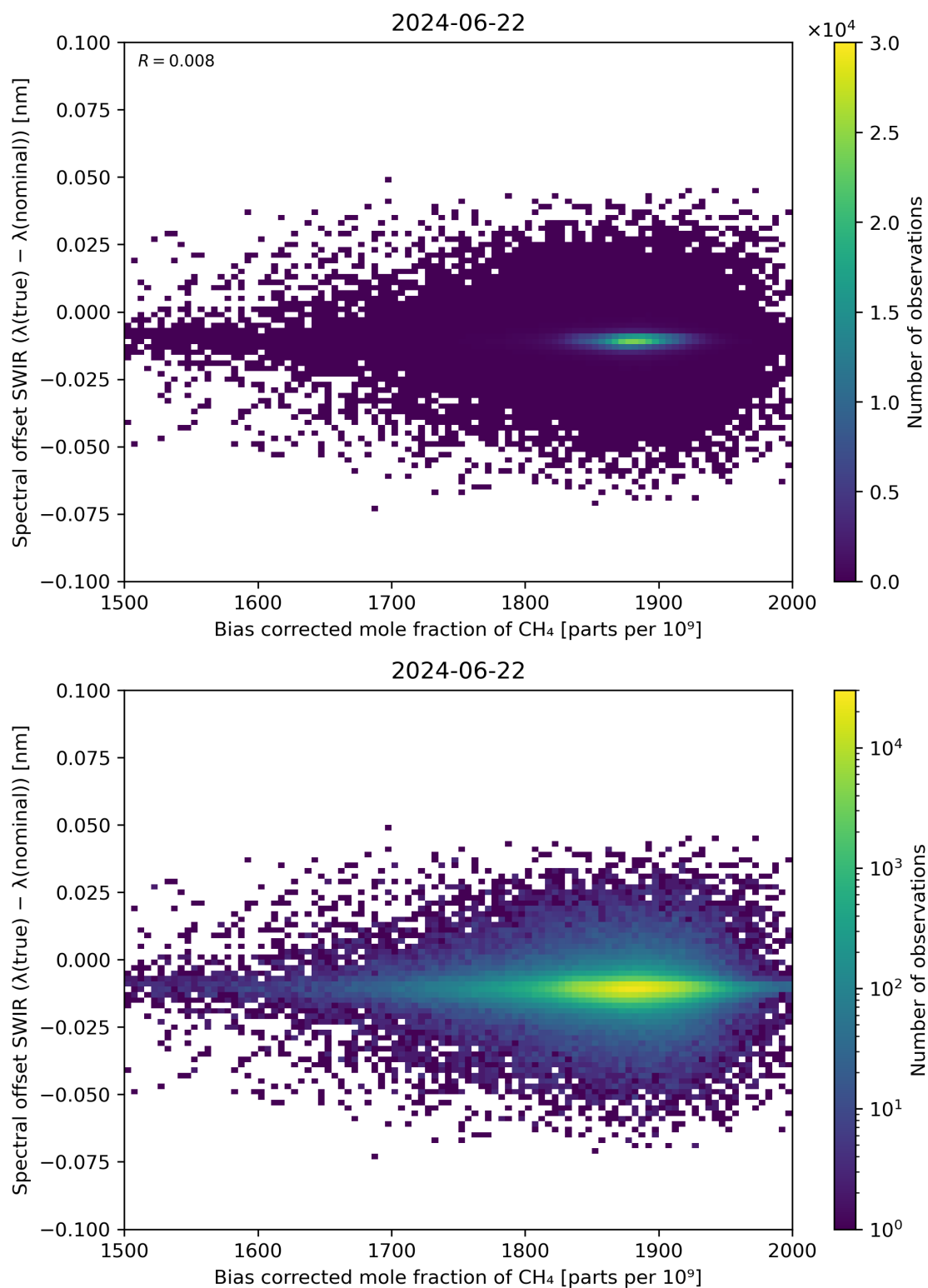
Figure 69: Scatter density plot of “Bias corrected mole fraction of \text{CH}_4 ” against “Spectral offset SWIR ( \lambda(\text{true}) - \lambda(\text{nominal}) )” for 2024-06-21 to 2024-06-23.
