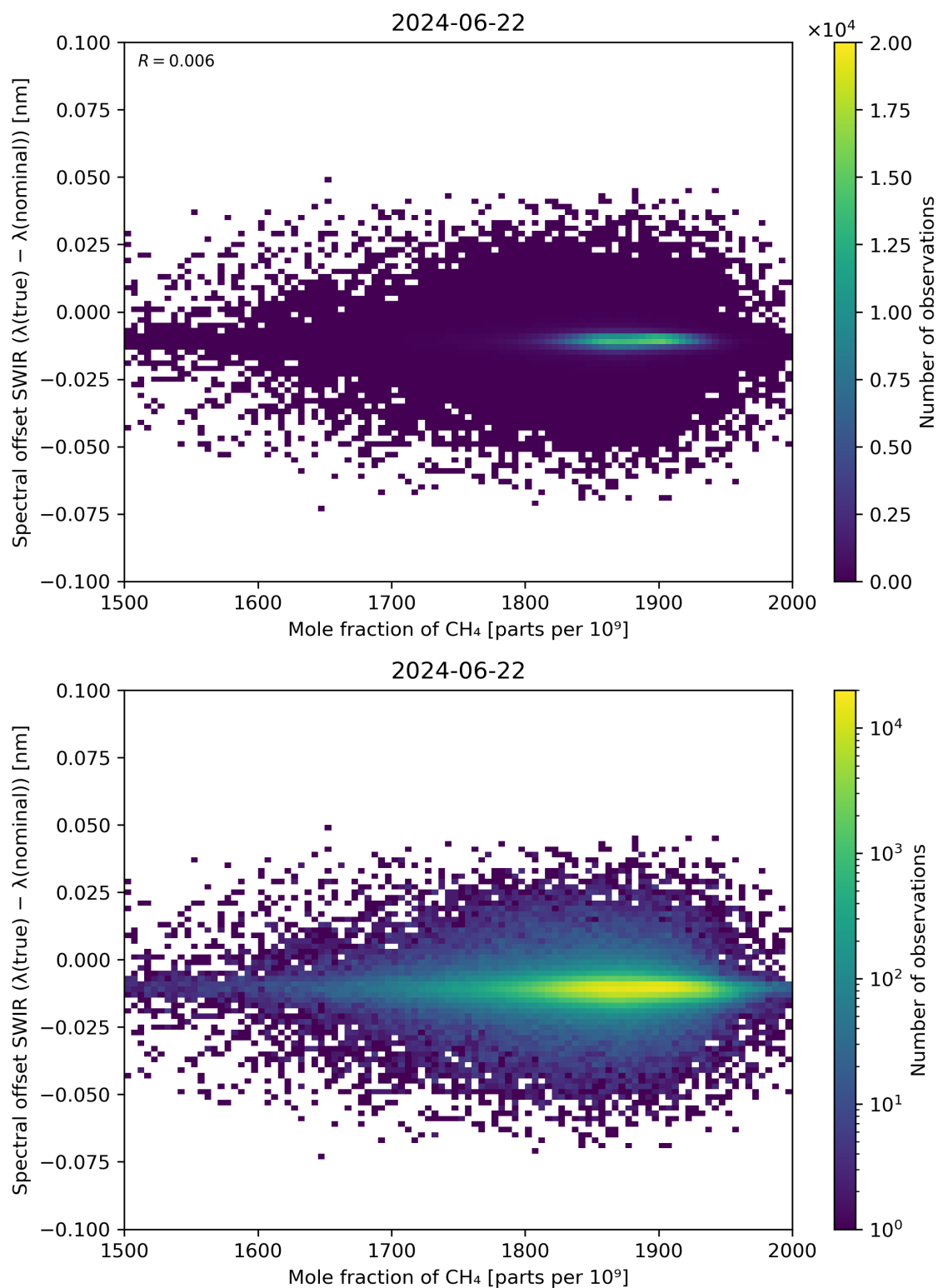
Figure 86: Scatter density plot of “Mole fraction of CH 4 ” against “Spectral offset SWIR ( \lambda(\text{true}) - \lambda(\text{nominal}) )” for 2024-06-21 to 2024-06-23.
