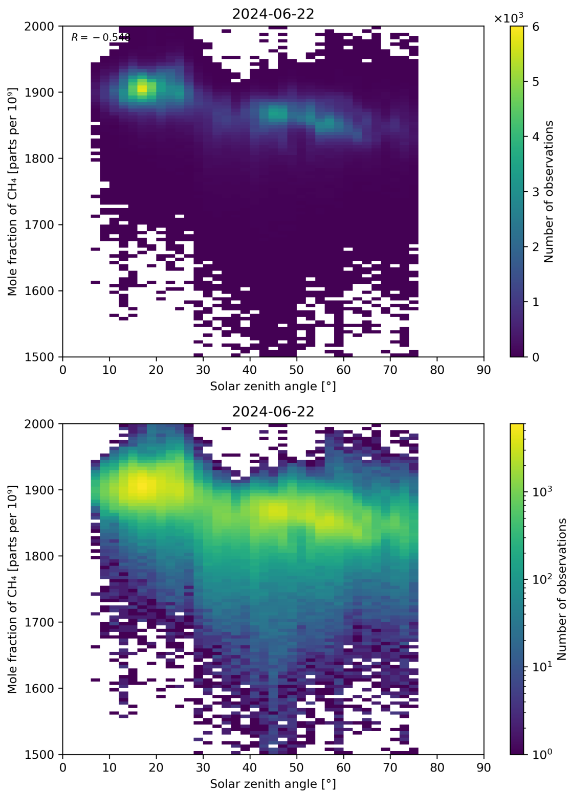
Figure 99: Scatter density plot of “Solar zenith angle” against “Mole fraction of CH 4 ” for 2024-06-21 to 2024-06-23.
