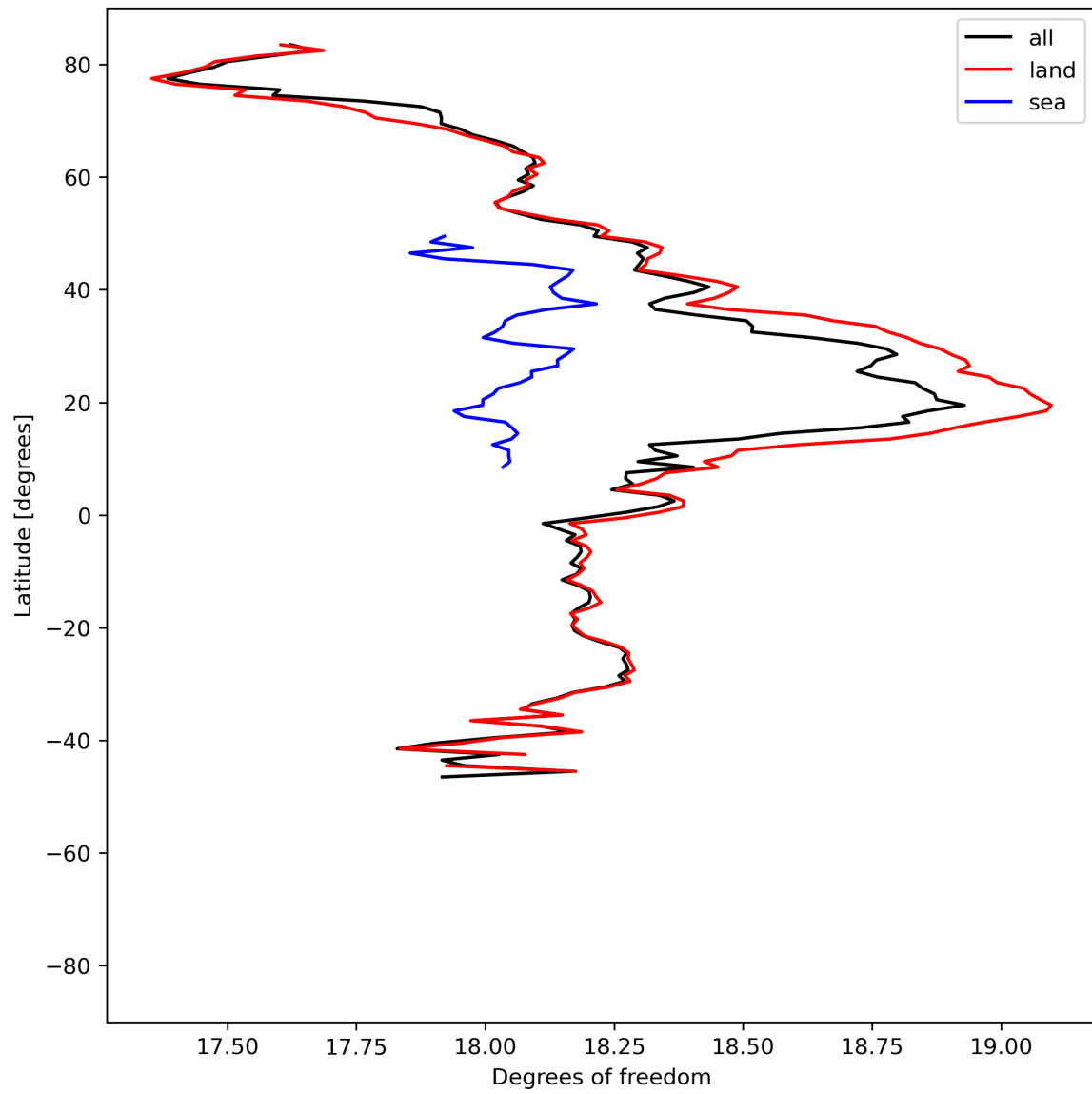
Figure 19: Zonal average of “Degrees of freedom” for 2024-06-21 to 2024-06-23.
