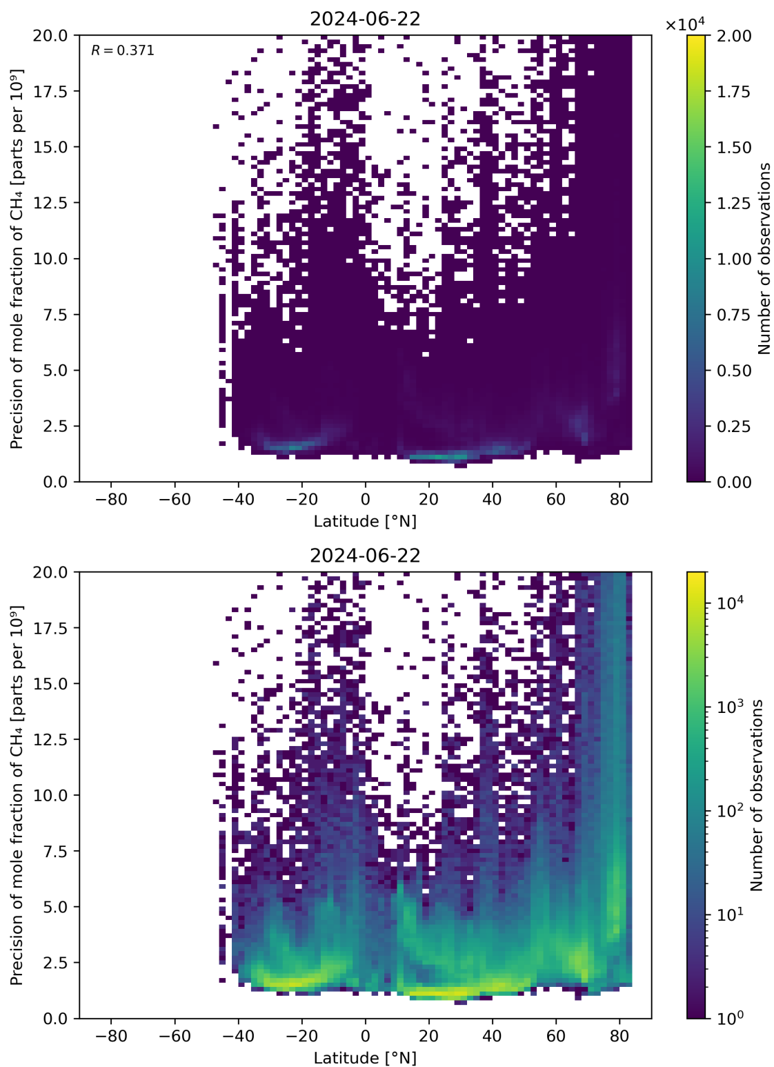
Figure 59: Scatter density plot of “Latitude” against “Precision of mole fraction of \text{CH}_4 ” for 2024-06-21 to 2024-06-23.
