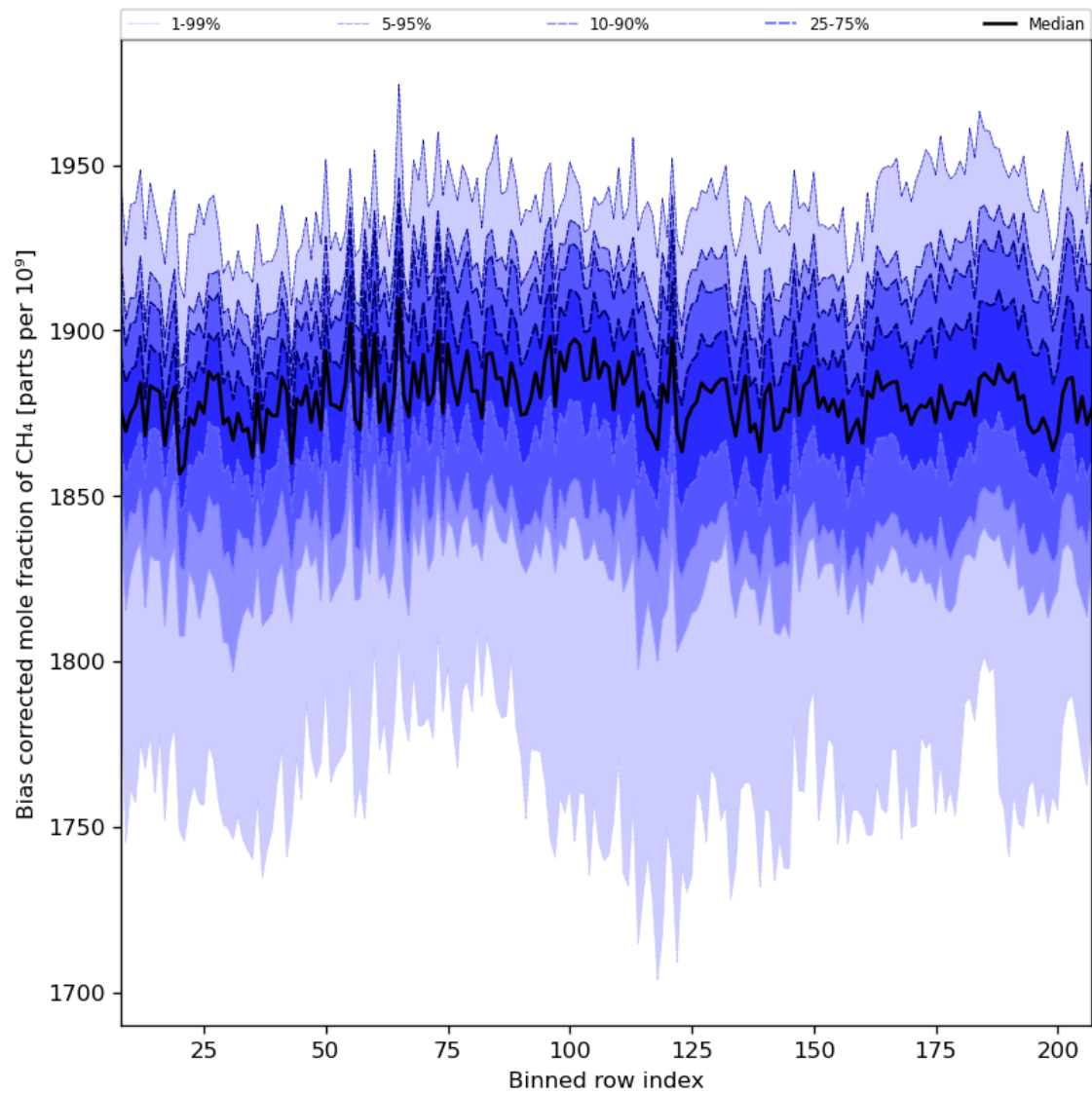
Figure 36: Along track statistics of “Bias corrected mole fraction of CH 4 ” for 2024-06-21 to 2024-06-23
