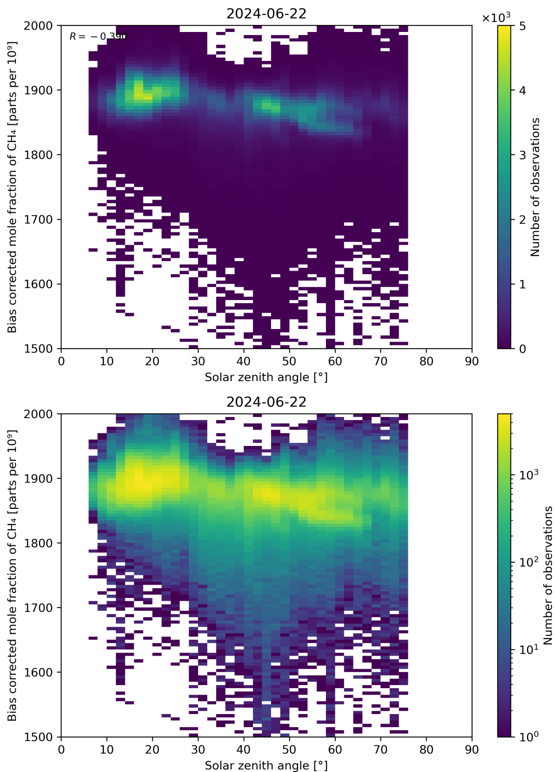
Figure 100: Scatter density plot of “Solar zenith angle” against “Bias corrected mole fraction of CH 4 ” for 2024-06-21 to 2024-06-23.
