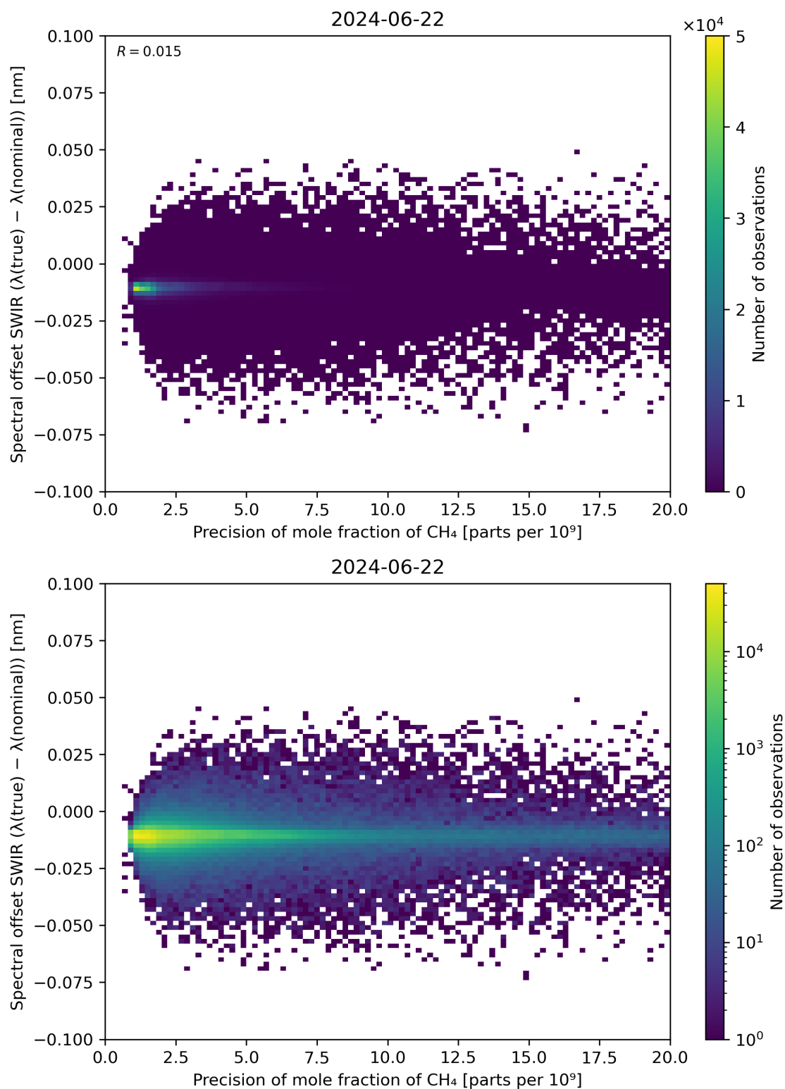
Figure 85: Scatter density plot of “Precision of mole fraction of CH 4 ” against “Spectral offset SWIR ( \lambda(\text{true}) - \lambda(\text{nominal}) )” for 2024-06-21 to 2024-06-23.
