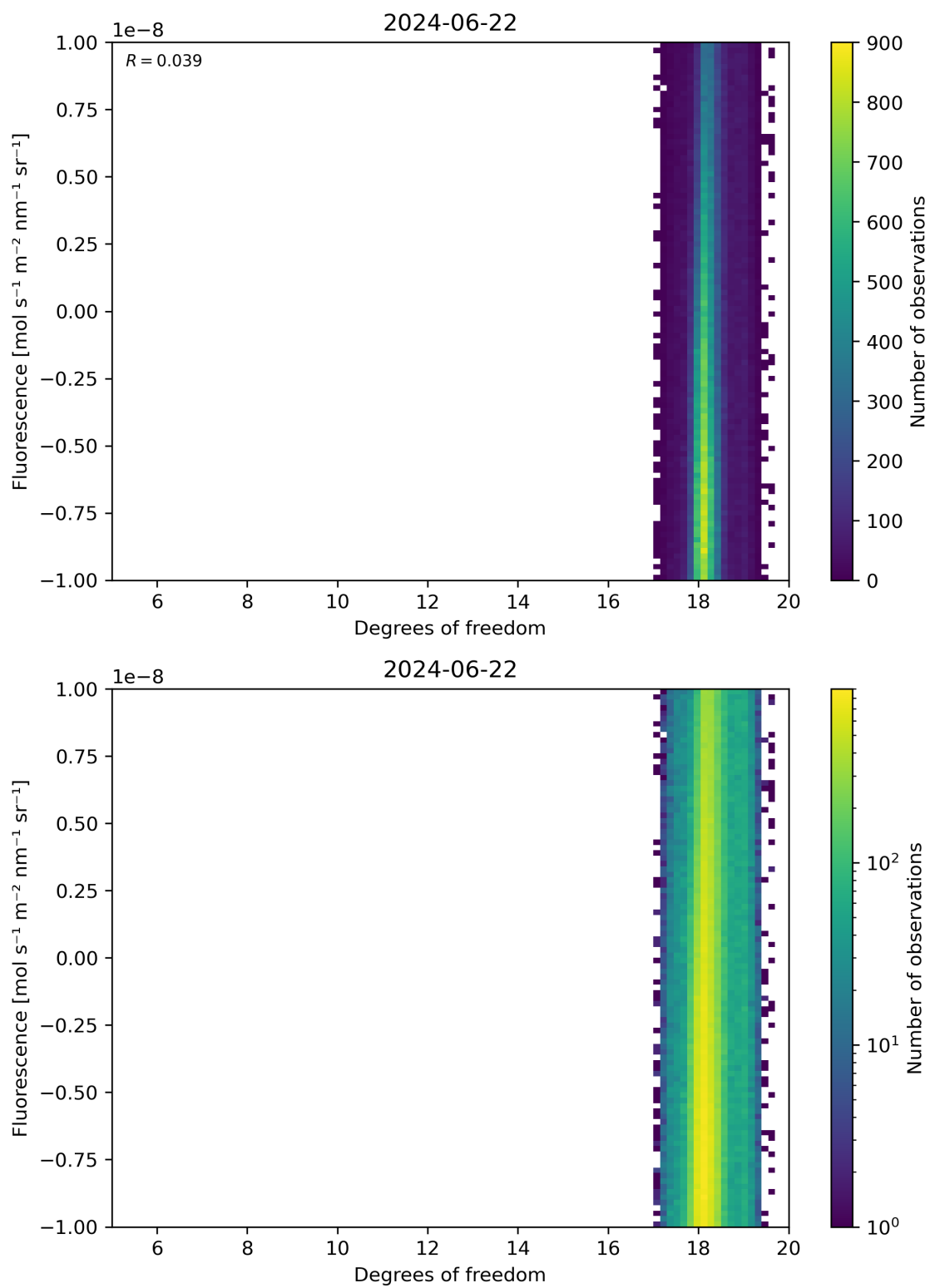
Figure 51: Scatter density plot of “Degrees of freedom” against “Fluorescence” for 2024-06-21 to 2024-06-23.
