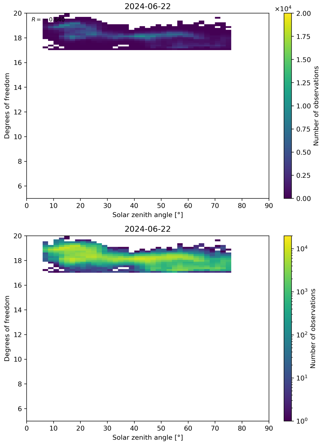
Figure 96: Scatter density plot of “Solar zenith angle” against “Degrees of freedom” for 2024-06-21 to 2024-06-23.
