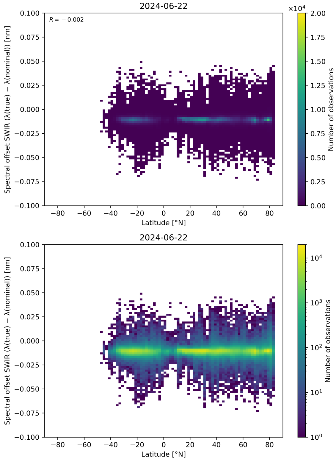
Figure 62: Scatter density plot of “Latitude” against “Spectral offset SWIR ( \lambda(\text{true}) - \lambda(\text{nominal}) )” for 2024-06-21 to 2024-06-23.
