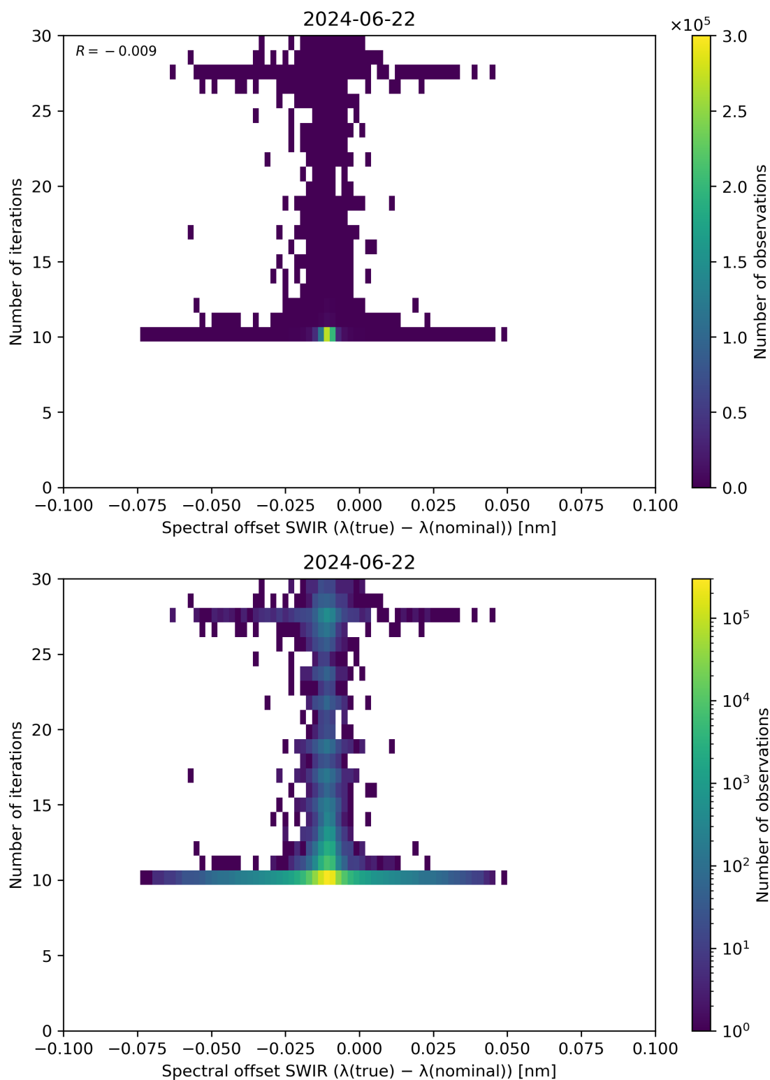
Figure 121: Scatter density plot of “Spectral offset SWIR ( \lambda(\text{true}) - \lambda(\text{nominal}) )” against “Number of iterations” for 2024-06-21 to 2024-06-23.
