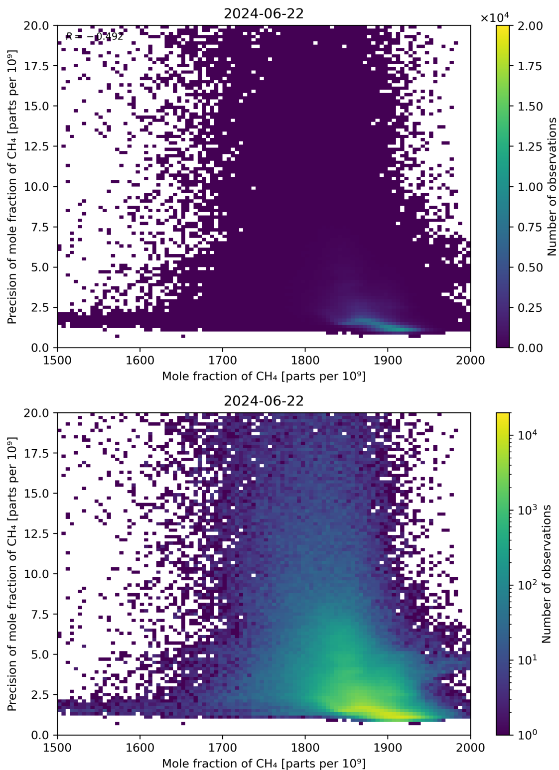
Figure 75: Scatter density plot of “Mole fraction of CH 4 ” against “Precision of mole fraction of CH 4 ” for 2024-06-21 to 2024-06-23.
