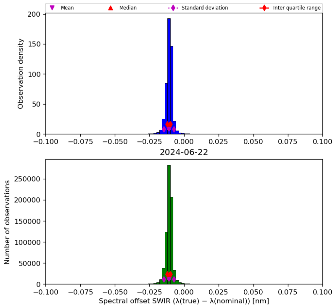
Figure 27: Histogram of “Spectral offset SWIR ( \lambda(\text{true}) - \lambda(\text{nominal}) )” for 2024-06-21 to 2024-06-23
