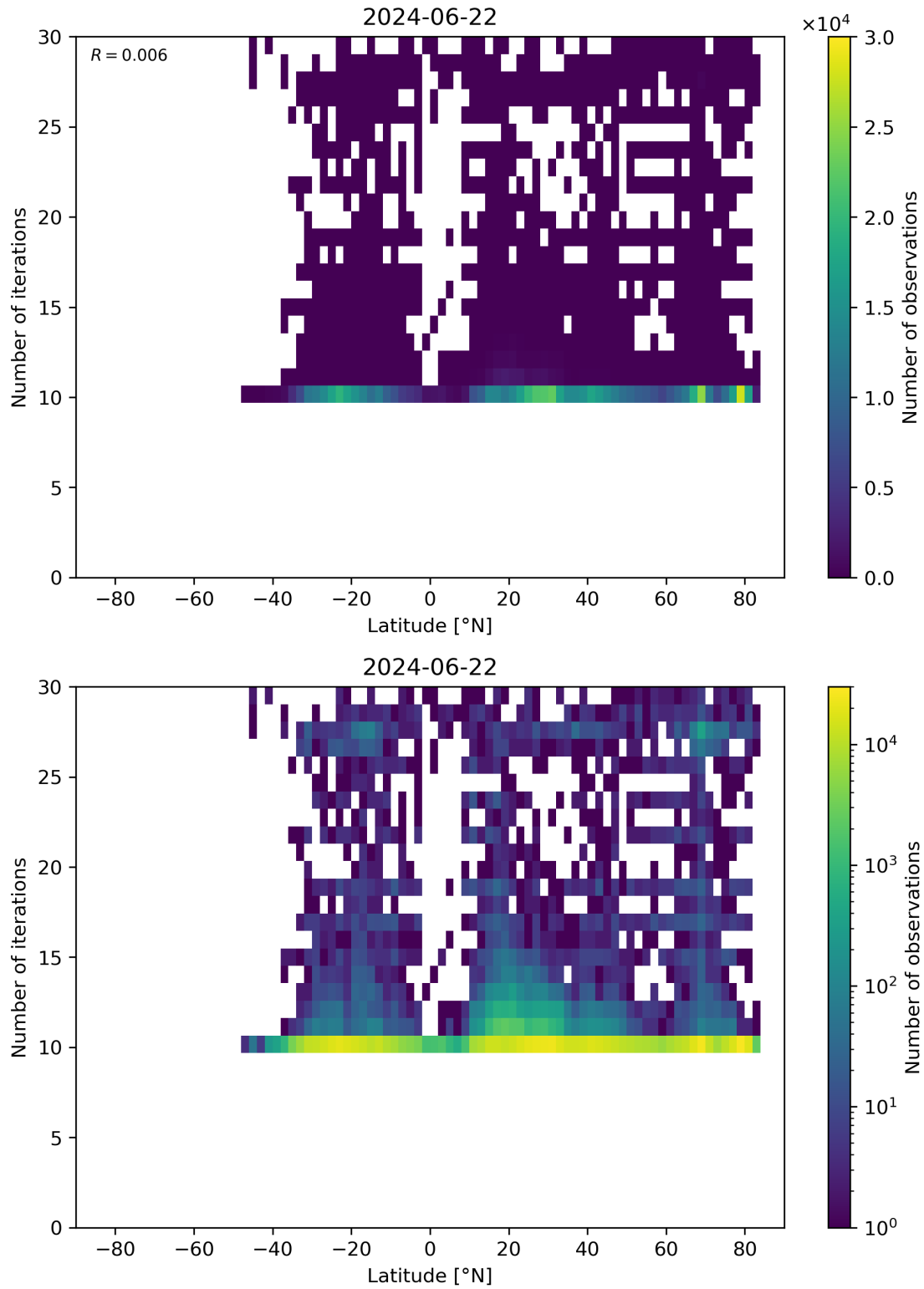
Figure 60: Scatter density plot of “Latitude” against “Number of iterations” for 2024-06-21 to 2024-06-23.
