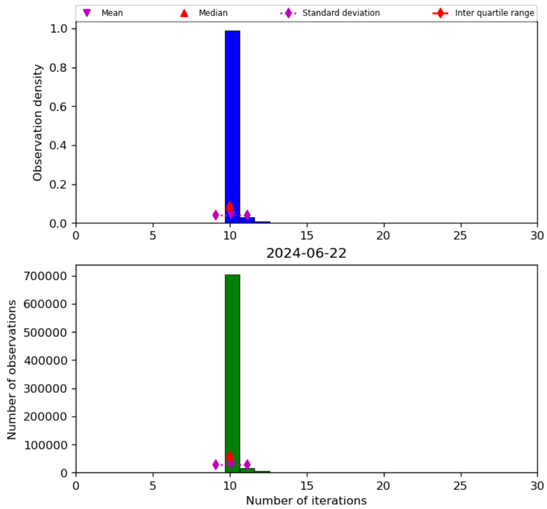
Figure 31: Histogram of “Number of iterations” for 2024-06-21 to 2024-06-23
