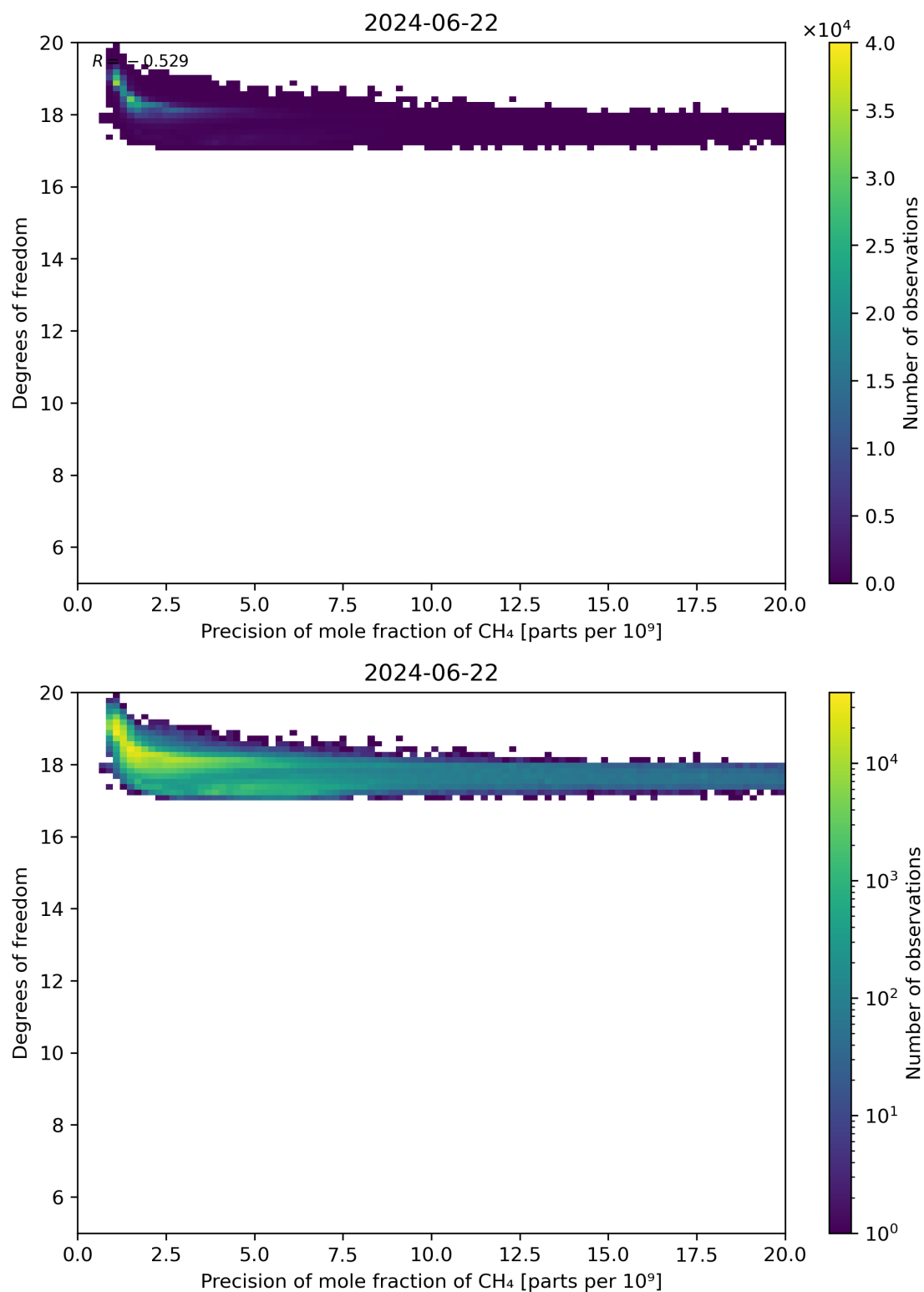
Figure 80: Scatter density plot of “Precision of mole fraction of CH 4 ” against “Degrees of freedom” for 2024-06-21 to 2024-06-23.
