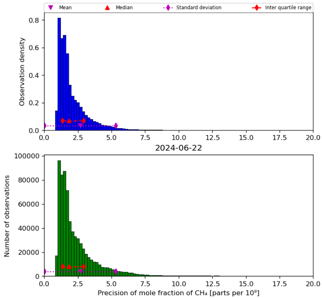
Figure 24: Histogram of “Precision of mole fraction of CH 4 ” for 2024-06-21 to 2024-06-23
