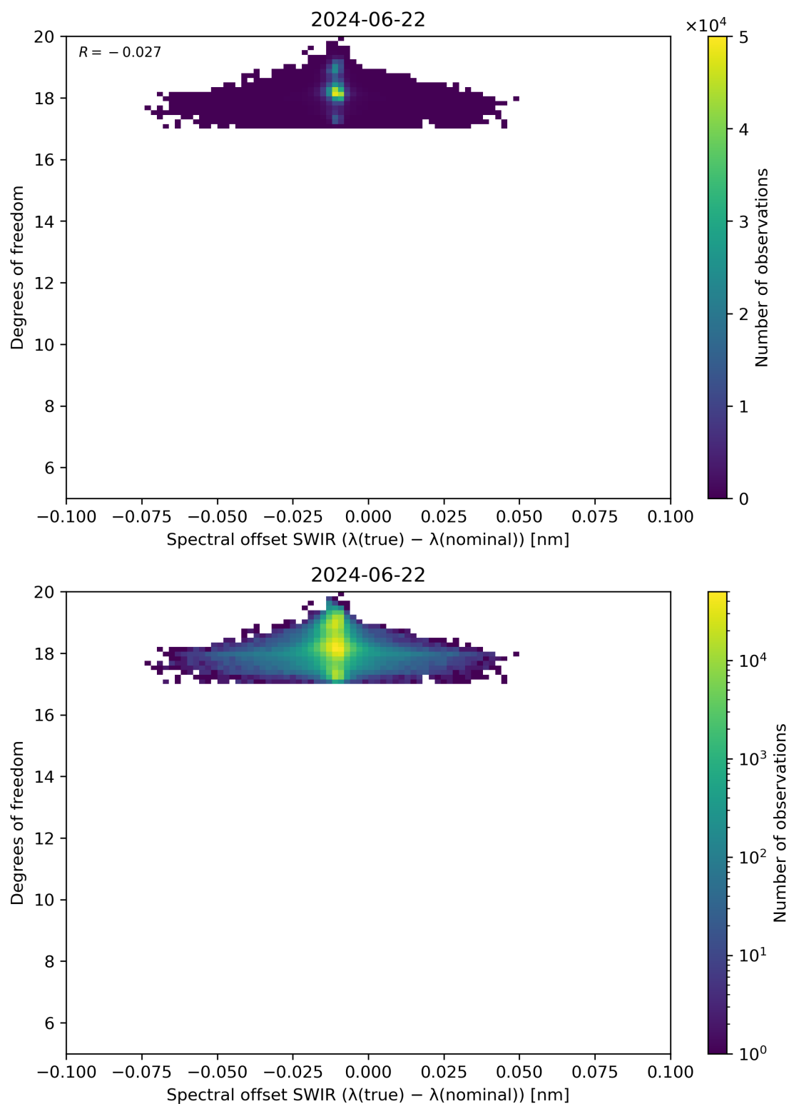
Figure 119: Scatter density plot of “Spectral offset SWIR ( \lambda(\text{true}) - \lambda(\text{nominal}) )” against “Degrees of freedom” for 2024-06-21 to 2024-06-23.
