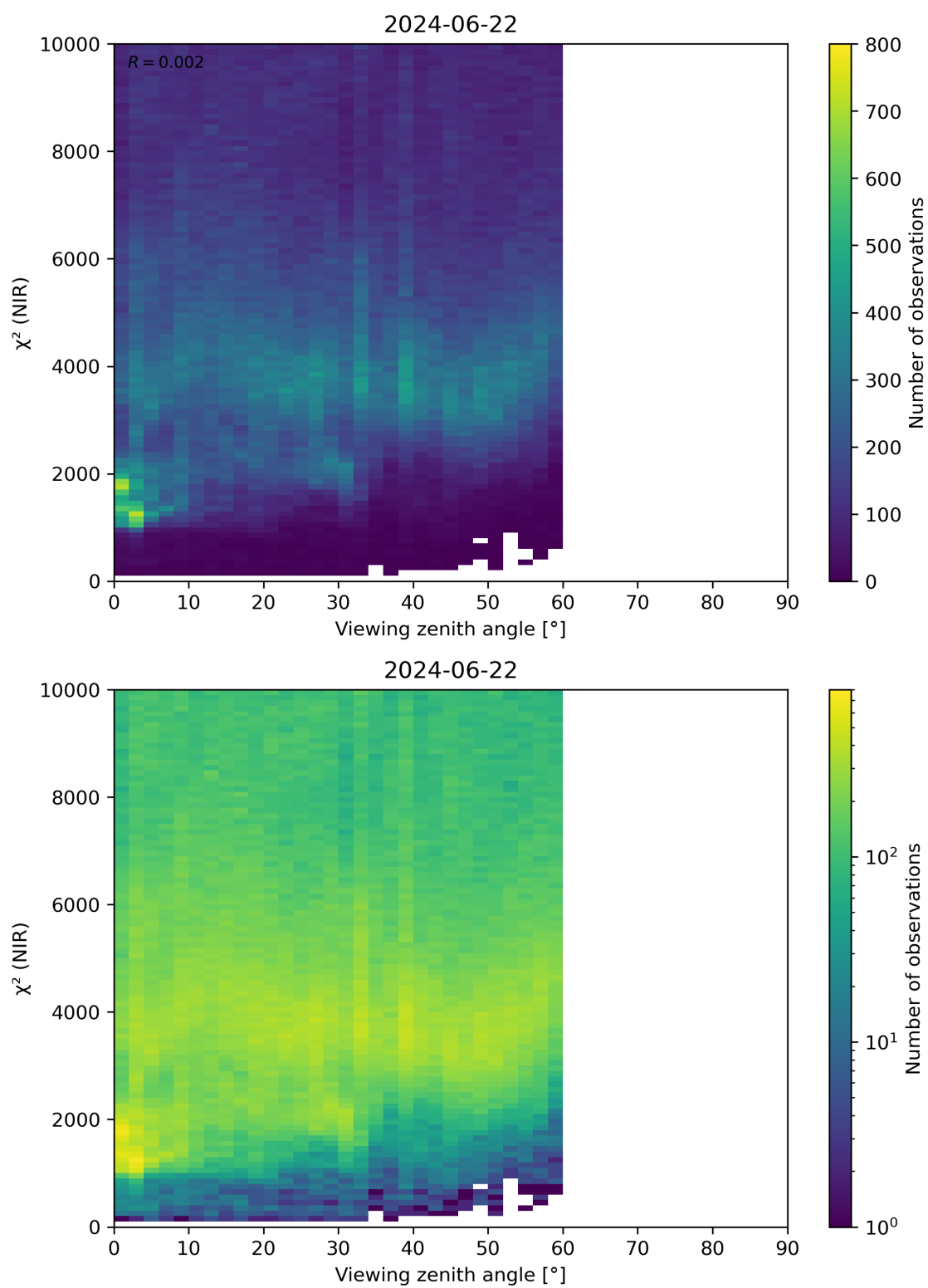
Figure 105: Scatter density plot of “Viewing zenith angle” against “ \chi^2 (NIR)” for 2024-06-21 to 2024-06-23.
