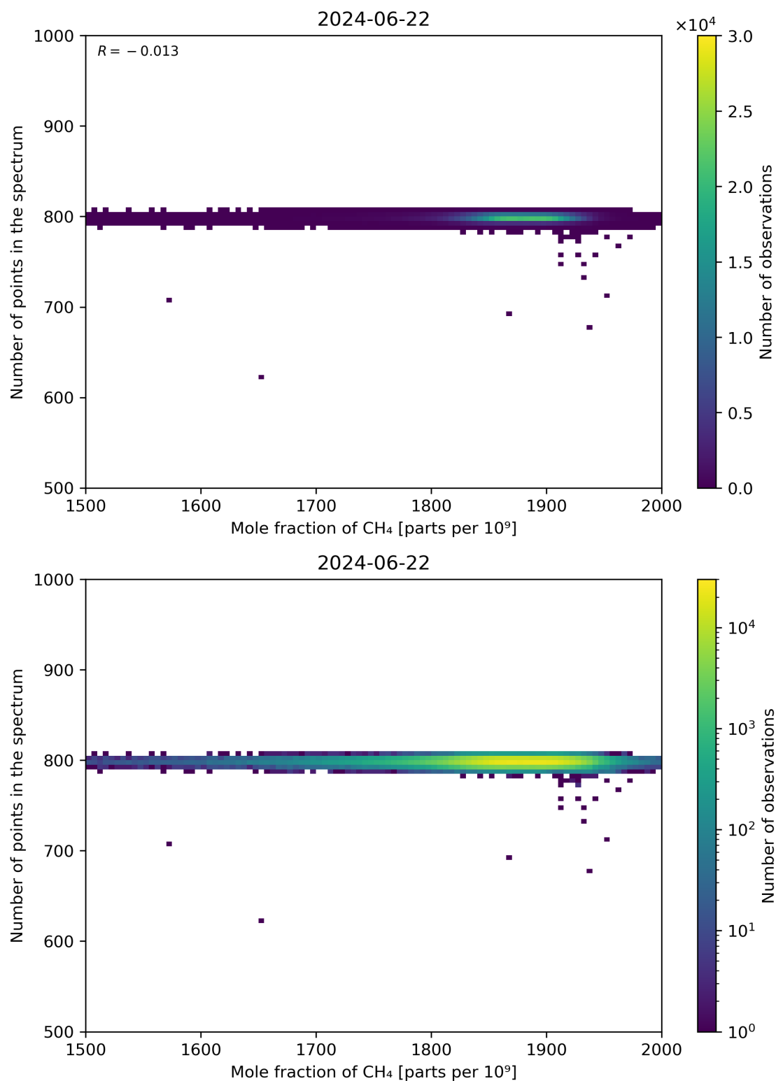
Figure 77: Scatter density plot of “Mole fraction of CH 4 ” against “Number of points in the spectrum” for 2024-06-21 to 2024-06-23.
