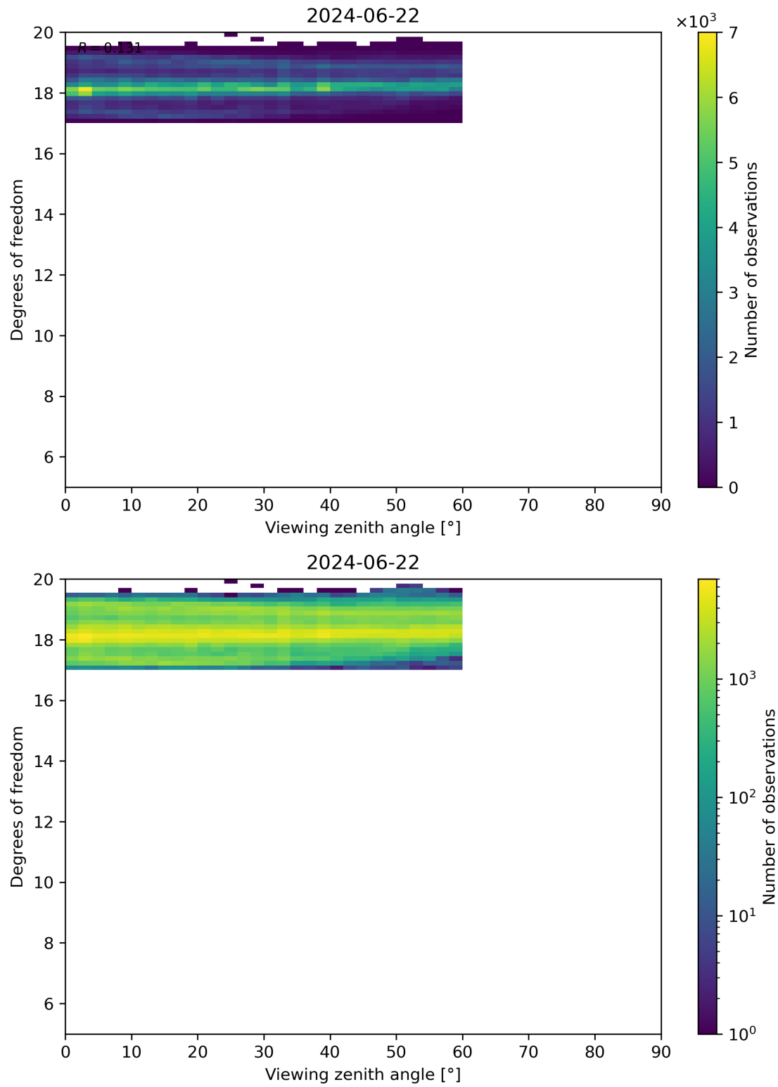
Figure 107: Scatter density plot of “Viewing zenith angle” against “Degrees of freedom” for 2024-06-21 to 2024-06-23.
