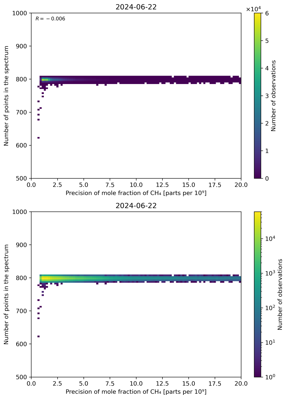
Figure 84: Scatter density plot of “Precision of mole fraction of CH 4 ” against “Number of points in the spectrum” for 2024-06-21 to 2024-06-23.
