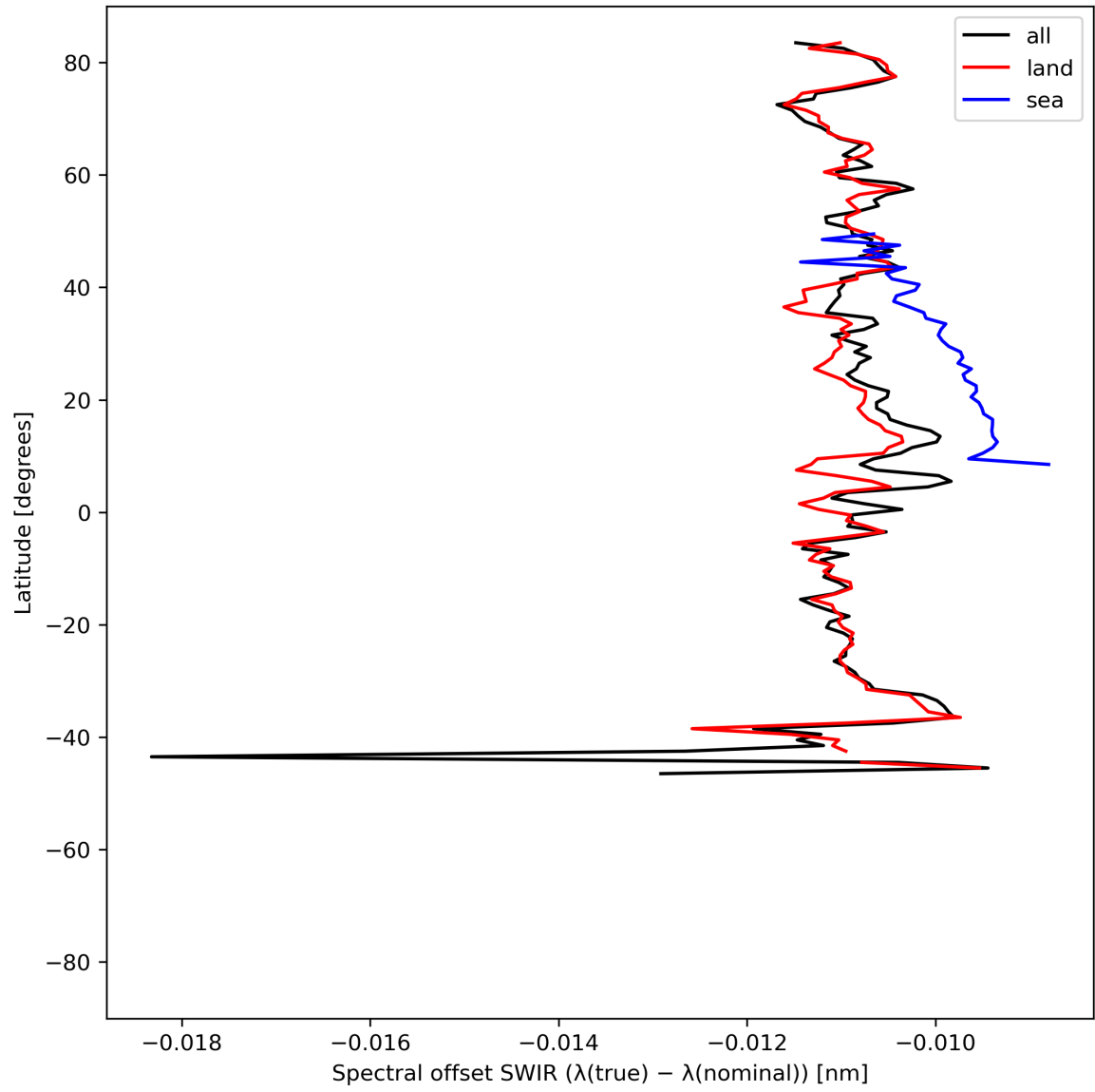
Figure 16: Zonal average of “Spectral offset SWIR ( \lambda(\text{true}) - \lambda(\text{nominal}) )” for 2024-06-21 to 2024-06-23.
