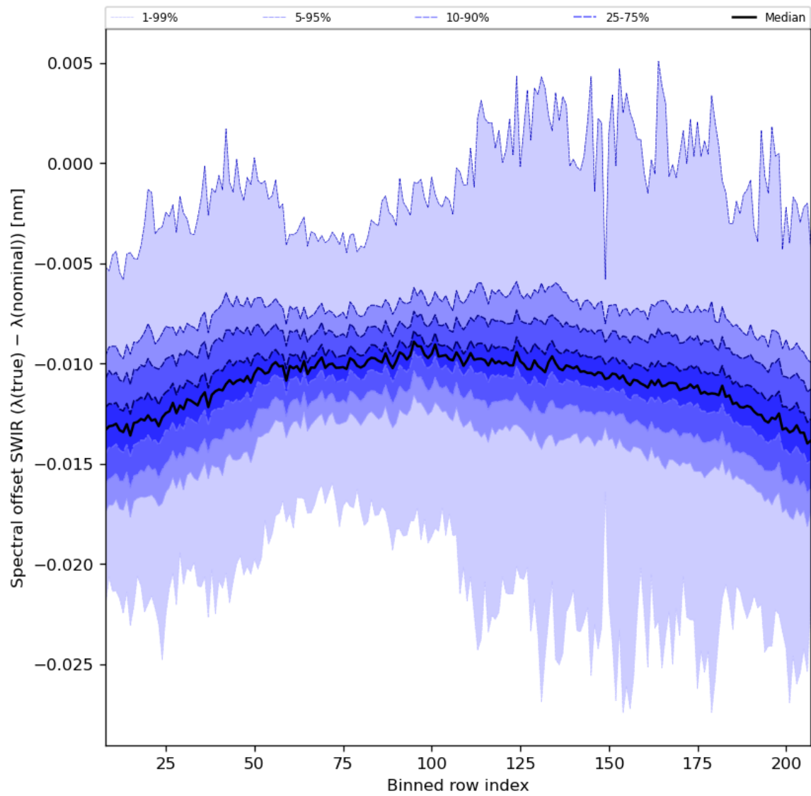
Figure 38: Along track statistics of “Spectral offset SWIR ( \lambda(\text{true}) - \lambda(\text{nominal}) )” for 2024-06-21 to 2024-06-23
