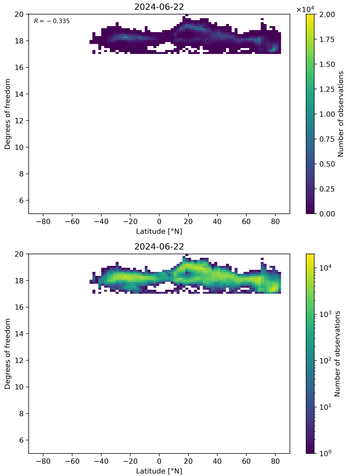
Figure 55: Scatter density plot of “Latitude” against “Degrees of freedom” for 2024-06-21 to 2024-06-23.
