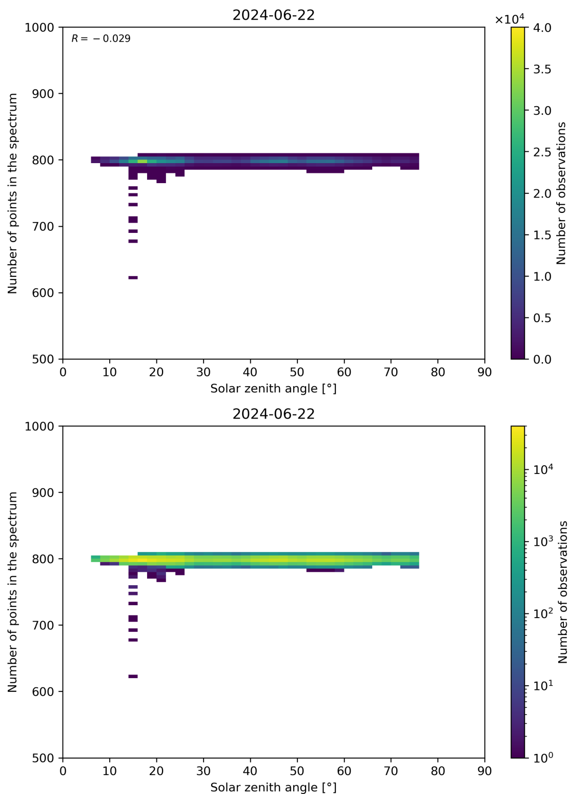
Figure 103: Scatter density plot of “Solar zenith angle” against “Number of points in the spectrum” for 2024-06-21 to 2024-06-23.
