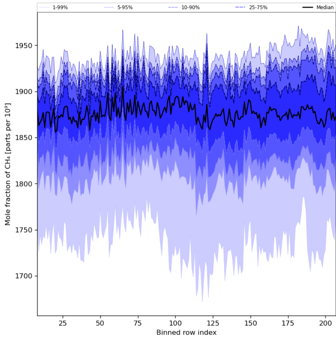
Figure 34: Along track statistics of “Mole fraction of CH 4 ” for 2024-06-21 to 2024-06-23
