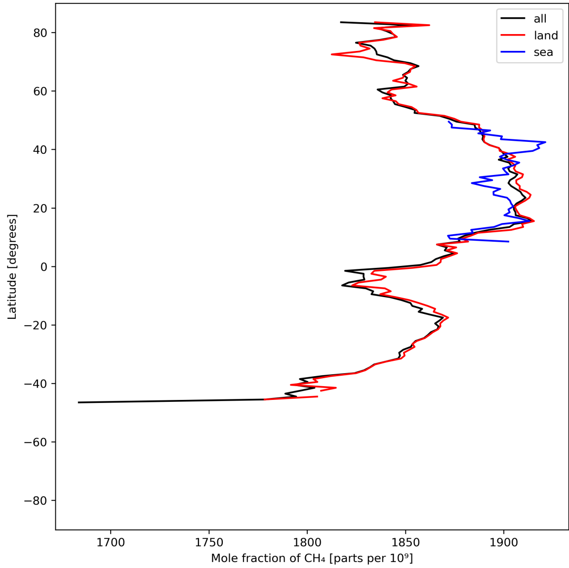
Figure 12: Zonal average of “Mole fraction of \text{CH}_4 ” for 2024-06-21 to 2024-06-23.
