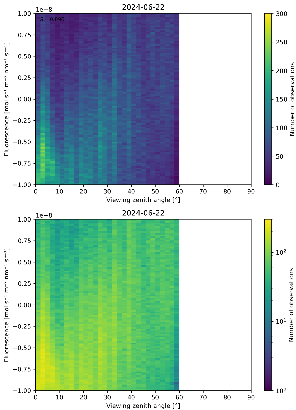
Figure 108: Scatter density plot of “Viewing zenith angle” against “Fluorescence” for 2024-06-21 to 2024-06-23.
