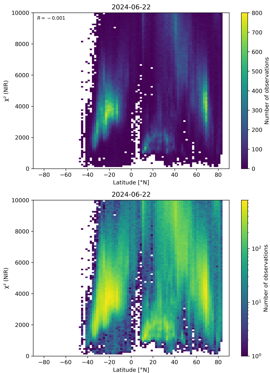
Figure 53: Scatter density plot of “Latitude” against “ \chi^2 (NIR)” for 2024-06-21 to 2024-06-23.
