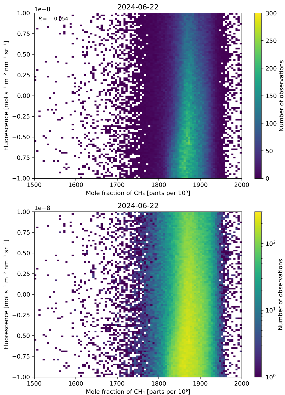
Figure 73: Scatter density plot of “Mole fraction of \text{CH}_4 ” against “Fluorescence” for 2024-06-21 to 2024-06-23.
