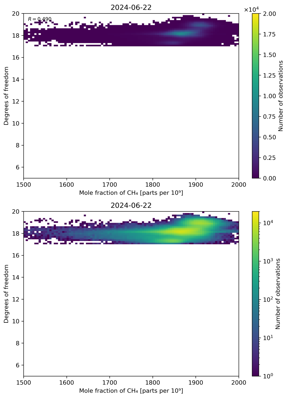
Figure 72: Scatter density plot of “Mole fraction of CH 4 ” against “Degrees of freedom” for 2024-06-21 to 2024-06-23.
