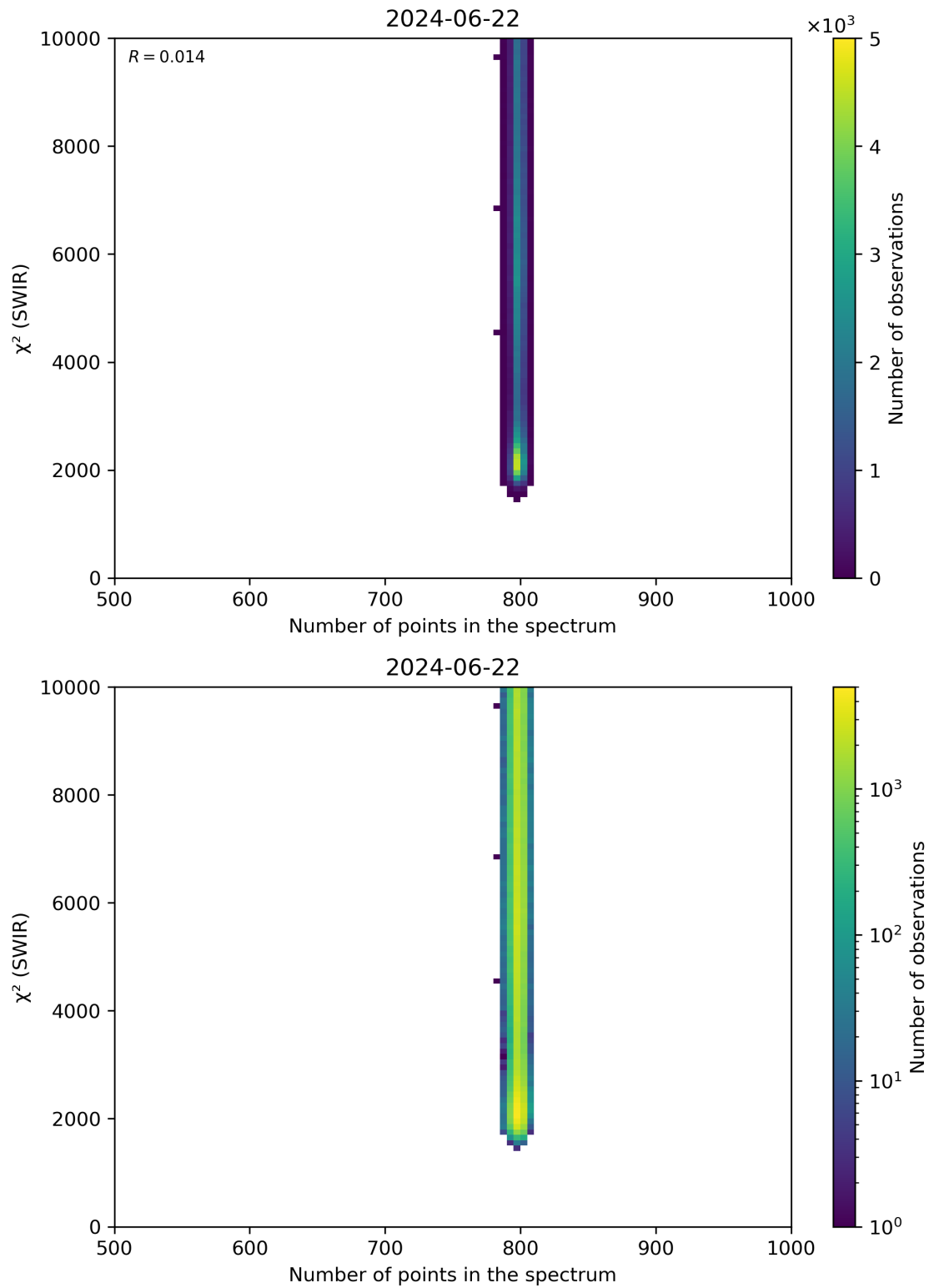
Figure 89: Scatter density plot of “Number of points in the spectrum” against “ \chi^2 (SWIR)” for 2024-06-21 to 2024-06-23.
