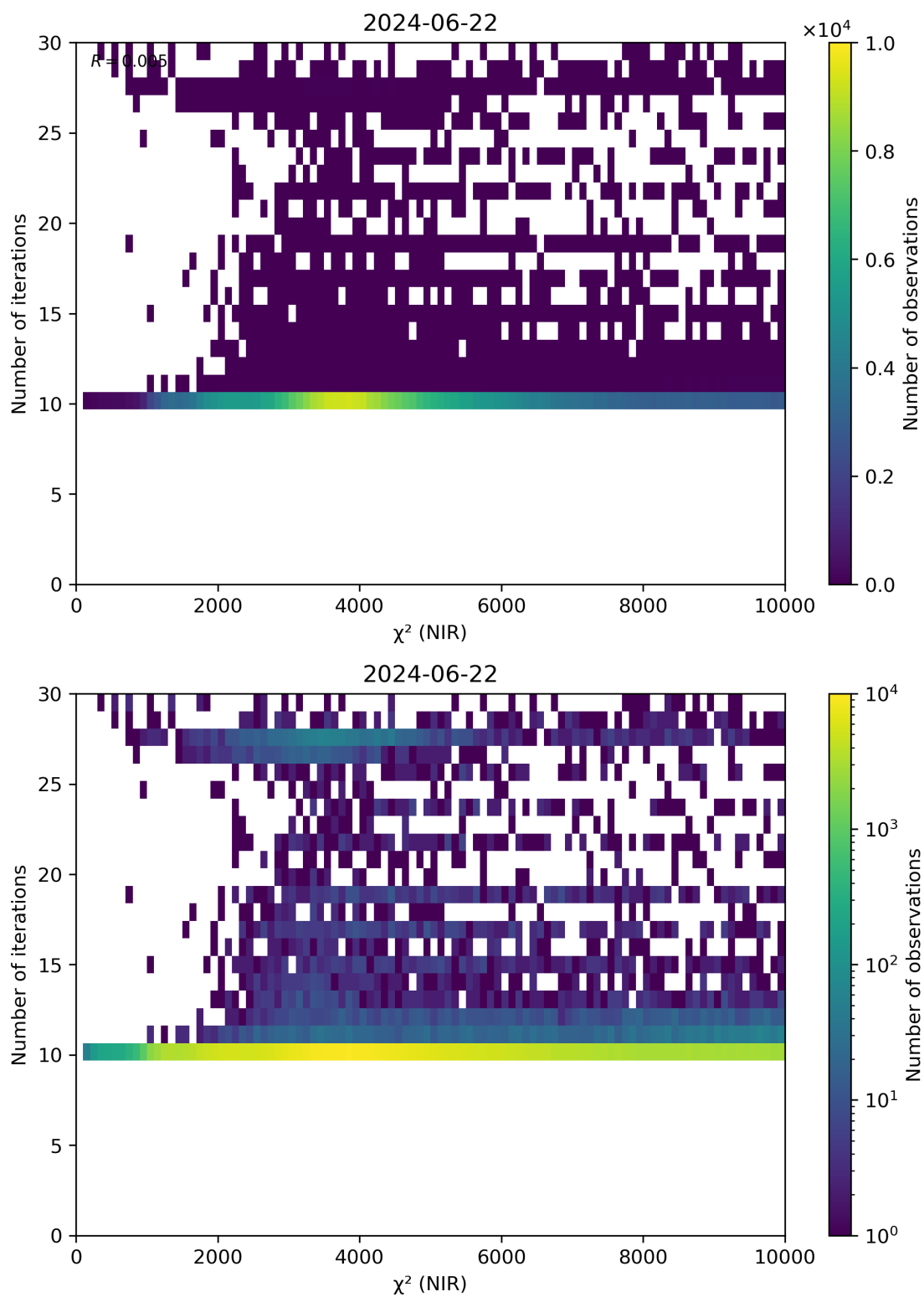
Figure 46: Scatter density plot of “ \chi^2 (NIR)” against “Number of iterations” for 2024-06-21 to 2024-06-23.
