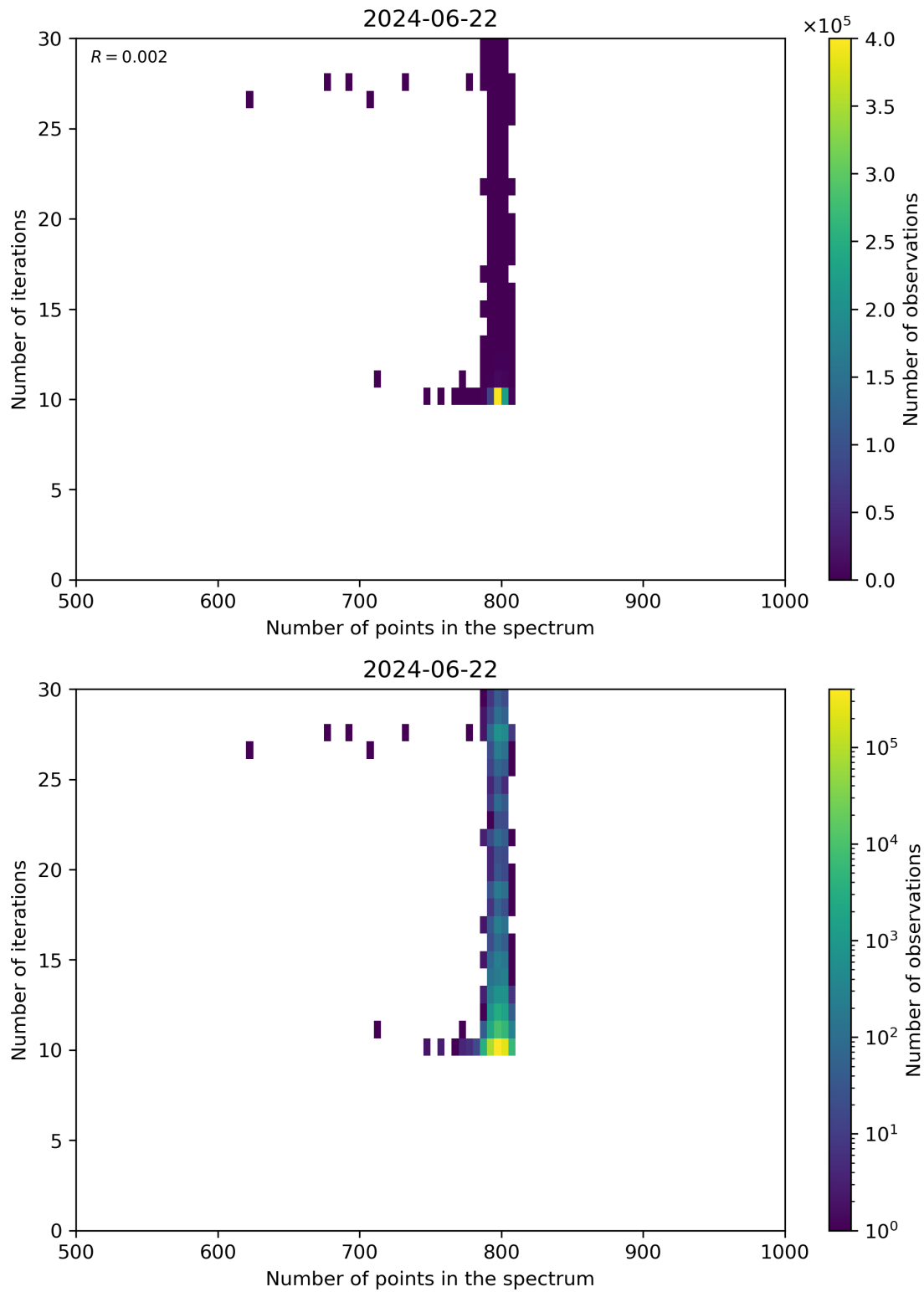
Figure 92: Scatter density plot of “Number of points in the spectrum” against “Number of iterations” for 2024-06-21 to 2024-06-23.
