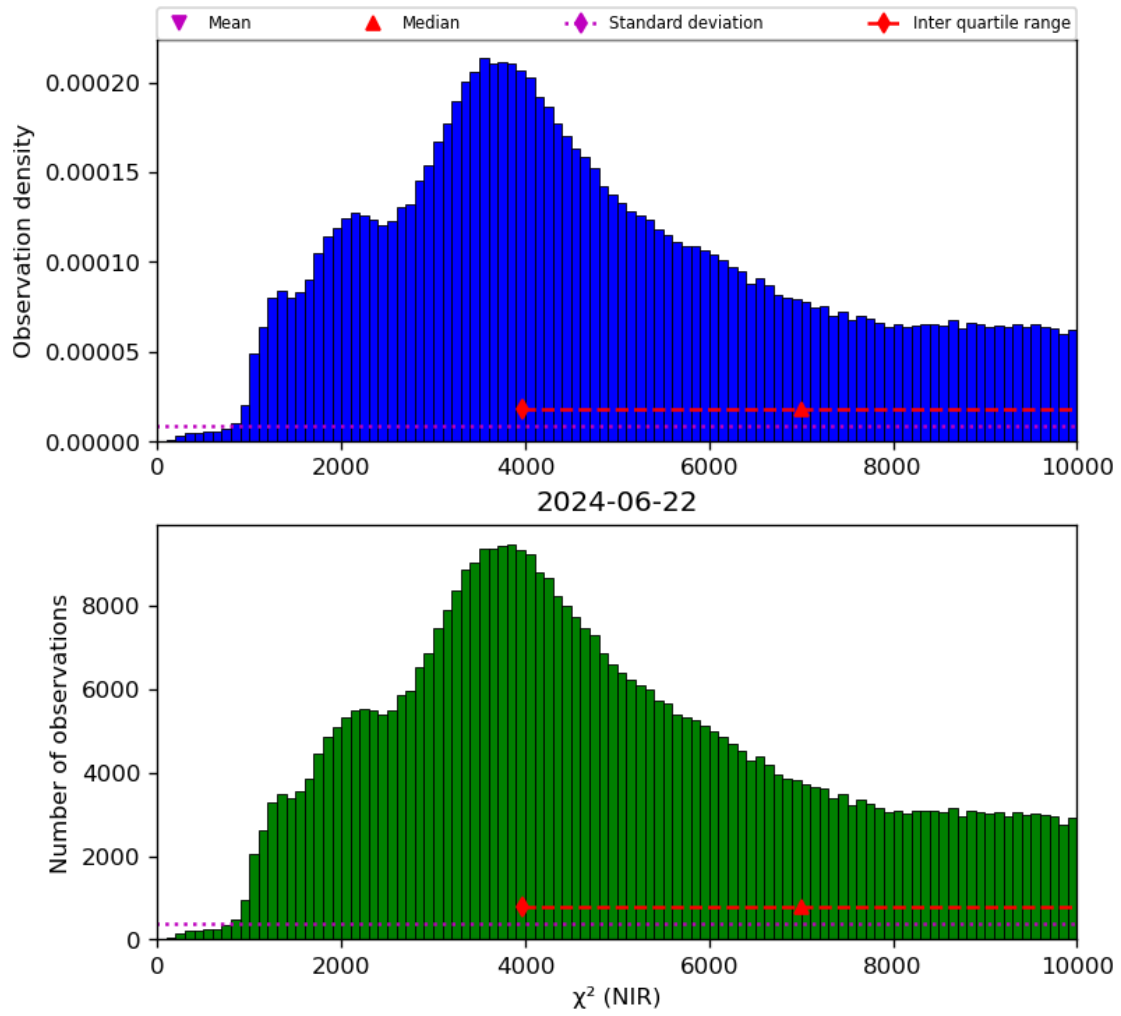
Figure 29: Histogram of “ \chi^2 (NIR)” for 2024-06-21 to 2024-06-23
