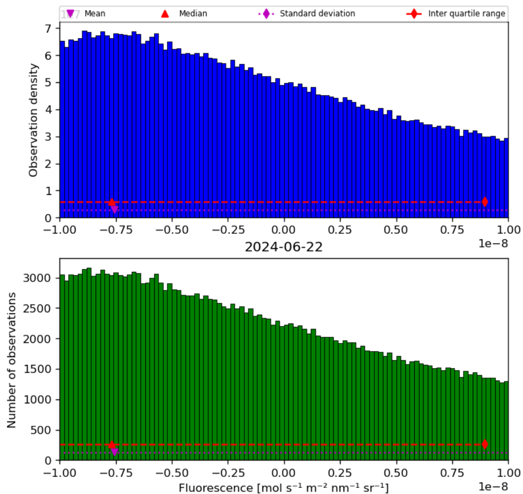
Figure 32: Histogram of “Fluorescence” for 2024-06-21 to 2024-06-23
