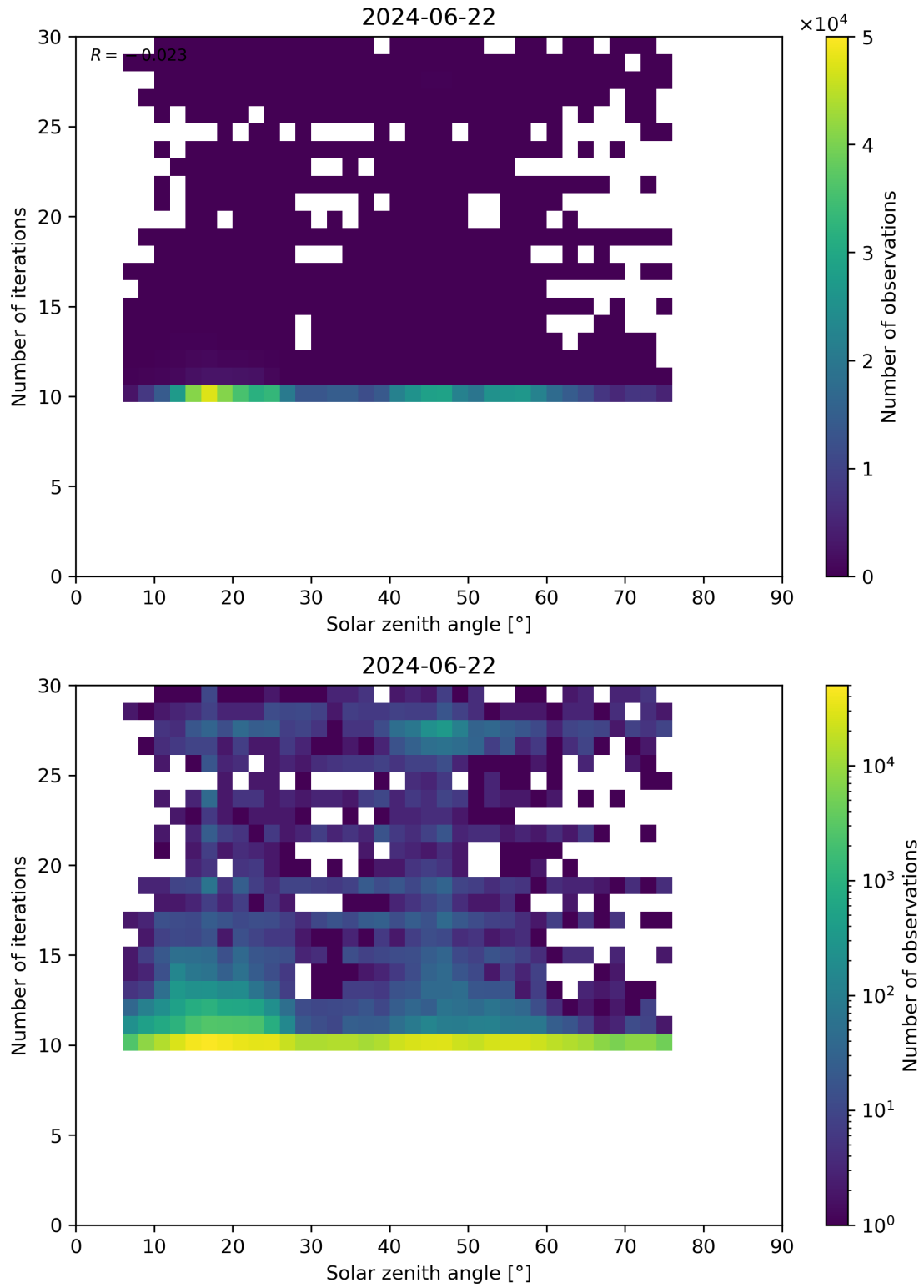
Figure 102: Scatter density plot of “Solar zenith angle” against “Number of iterations” for 2024-06-21 to 2024-06-23.
