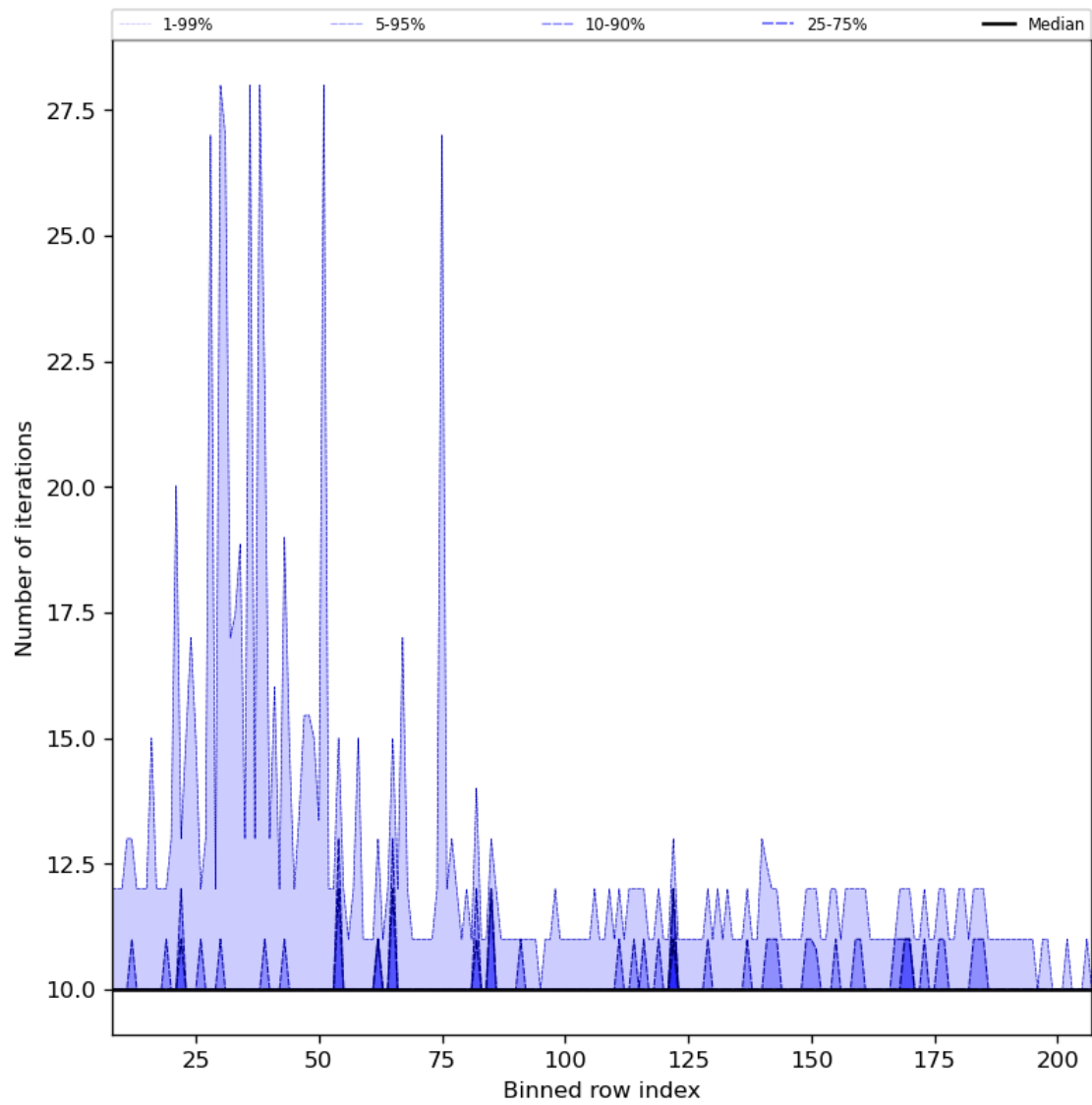
Figure 42: Along track statistics of “Number of iterations” for 2024-06-21 to 2024-06-23
