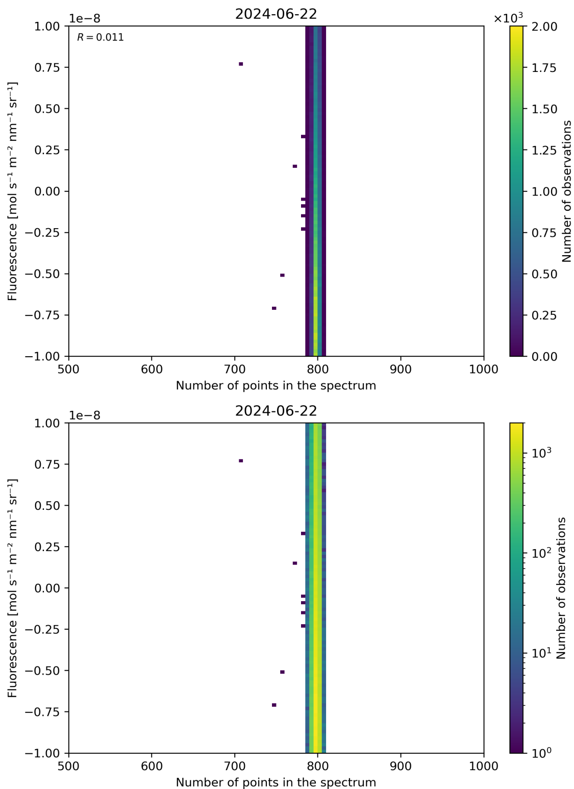
Figure 91: Scatter density plot of “Number of points in the spectrum” against “Fluorescence” for 2024-06-21 to 2024-06-23.
