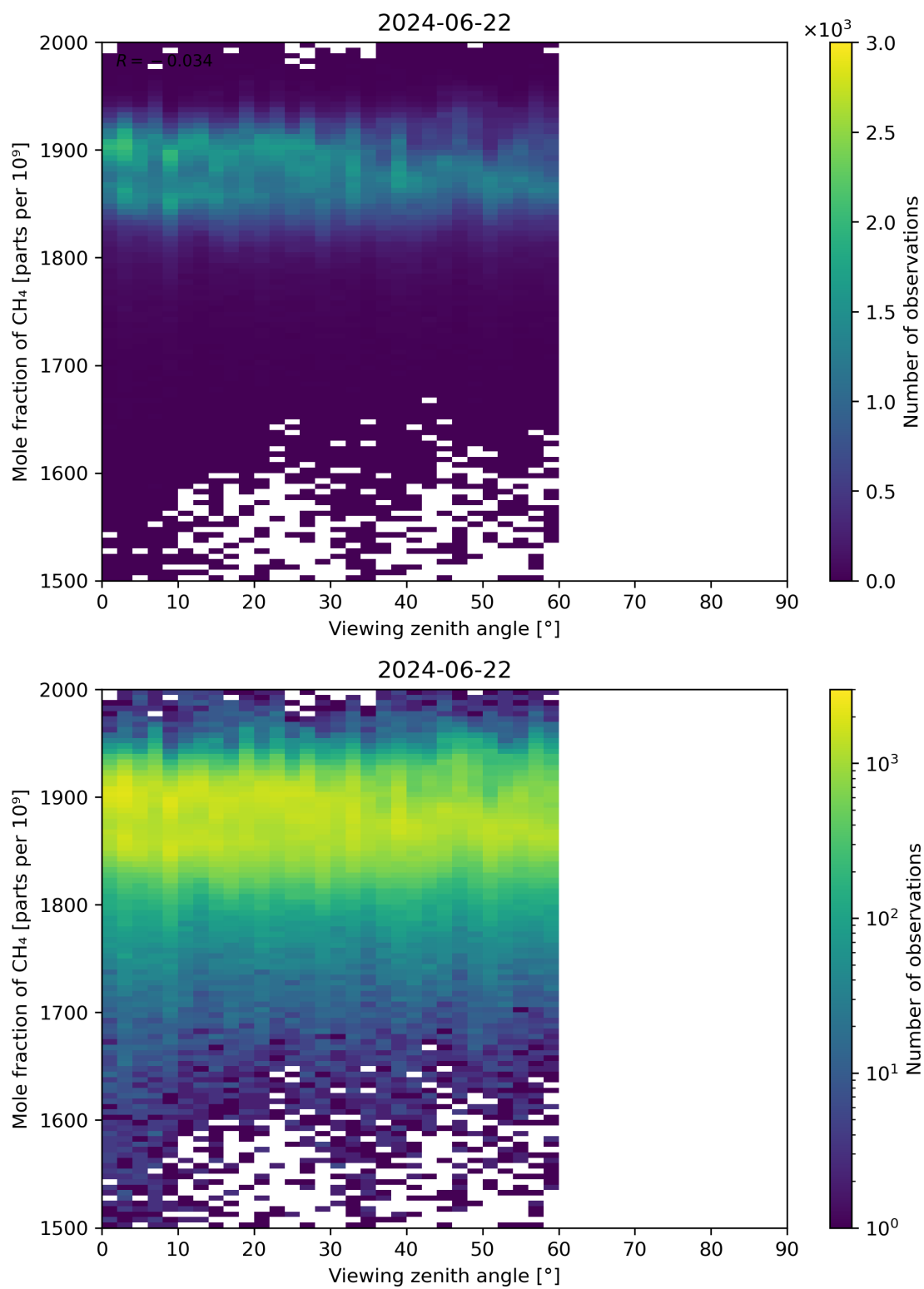
Figure 110: Scatter density plot of “Viewing zenith angle” against “Mole fraction of CH 4 ” for 2024-06-21 to 2024-06-23.
