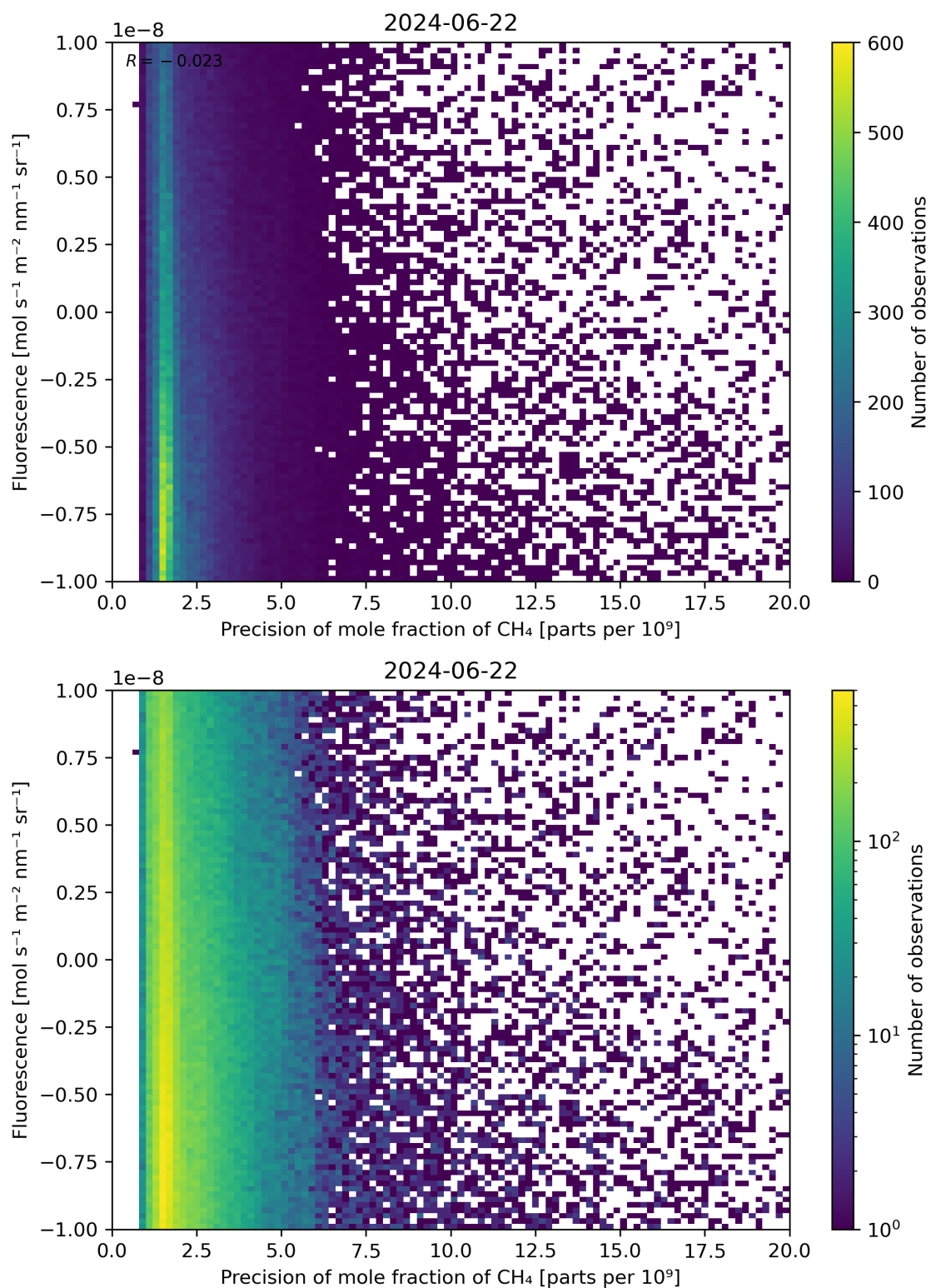
Figure 81: Scatter density plot of “Precision of mole fraction of \text{CH}_4 ” against “Fluorescence” for 2024-06-21 to 2024-06-23.
