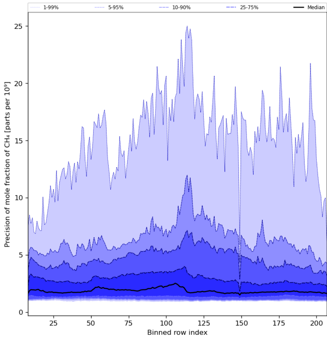
Figure 35: Along track statistics of “Precision of mole fraction of CH 4 ” for 2024-06-21 to 2024-06-23
