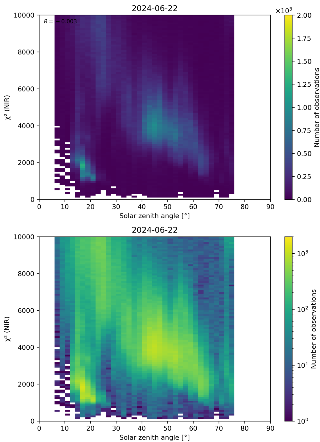
Figure 94: Scatter density plot of “Solar zenith angle” against “ \chi^2 (NIR)” for 2024-06-21 to 2024-06-23.
