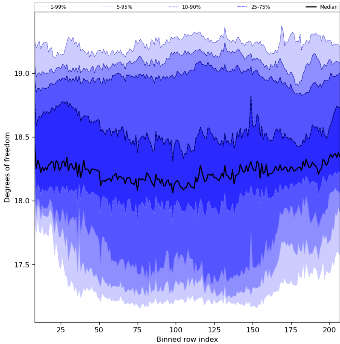
Figure 41: Along track statistics of “Degrees of freedom” for 2024-06-21 to 2024-06-23
