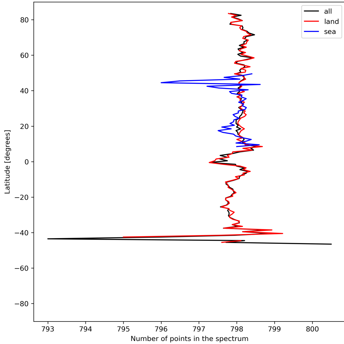
Figure 15: Zonal average of “Number of points in the spectrum” for 2024-06-21 to 2024-06-23.
