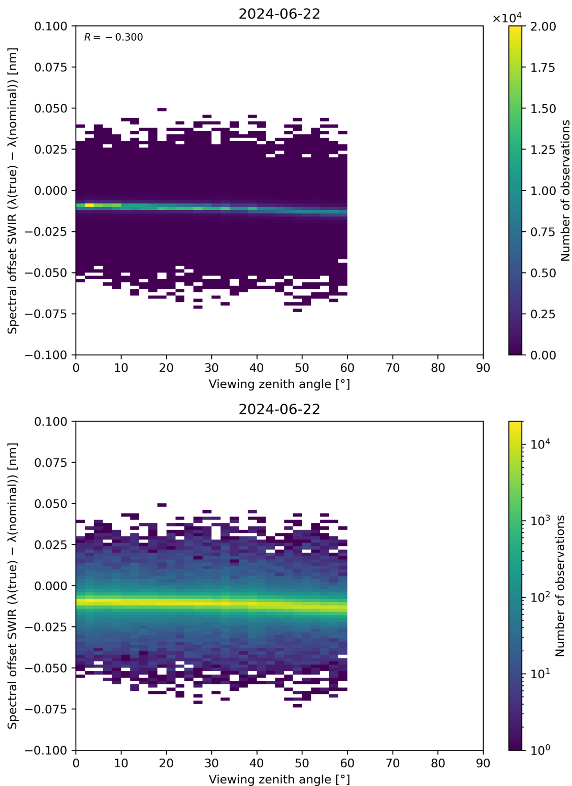
Figure 116: Scatter density plot of “Viewing zenith angle” against “Spectral offset SWIR ( \lambda(\text{true}) - \lambda(\text{nominal}) )” for 2024-06-21 to 2024-06-23.
