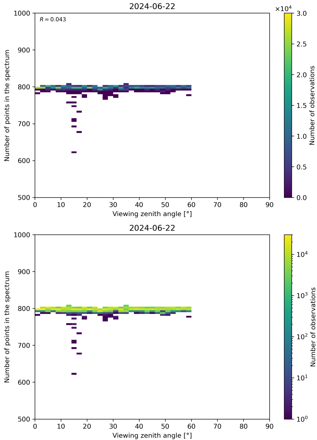
Figure 114: Scatter density plot of “Viewing zenith angle” against “Number of points in the spectrum” for 2024-06-21 to 2024-06-23.
