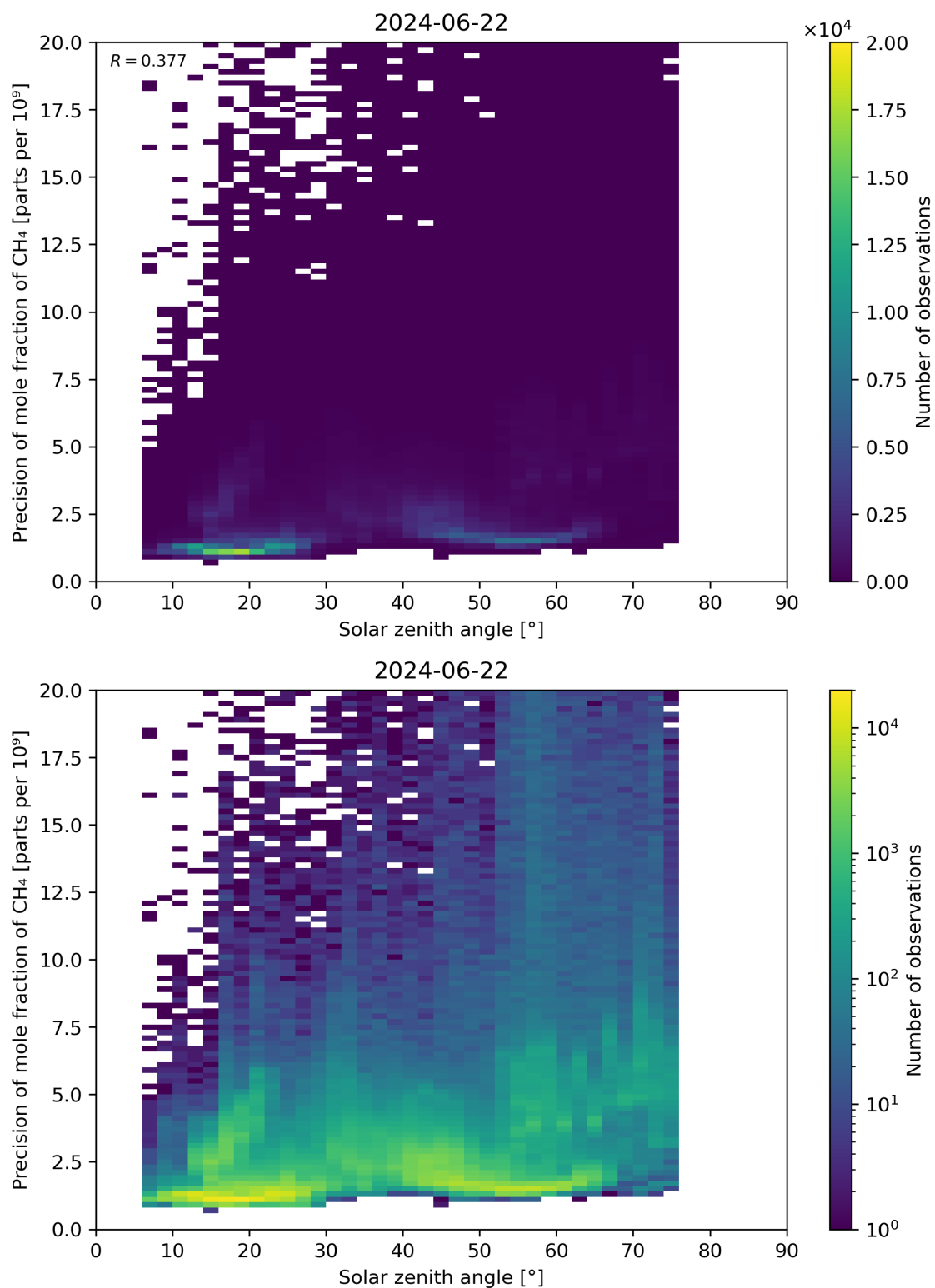
Figure 101: Scatter density plot of “Solar zenith angle” against “Precision of mole fraction of CH 4 ” for 2024-06-21 to 2024-06-23.
