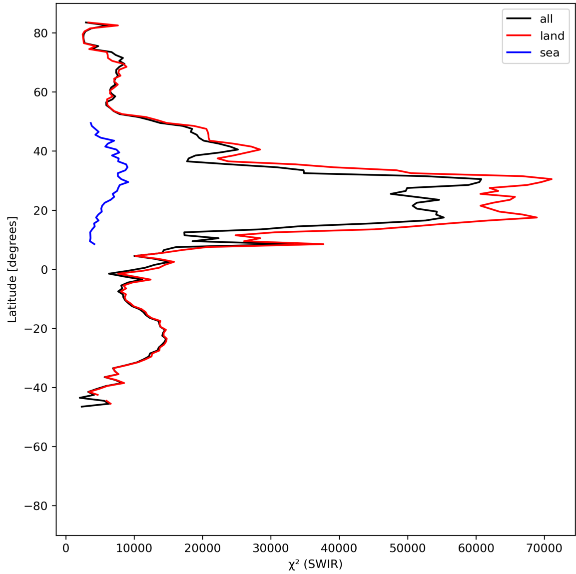
Figure 17: Zonal average of “ \chi^2 (SWIR)” for 2024-06-21 to 2024-06-23.
