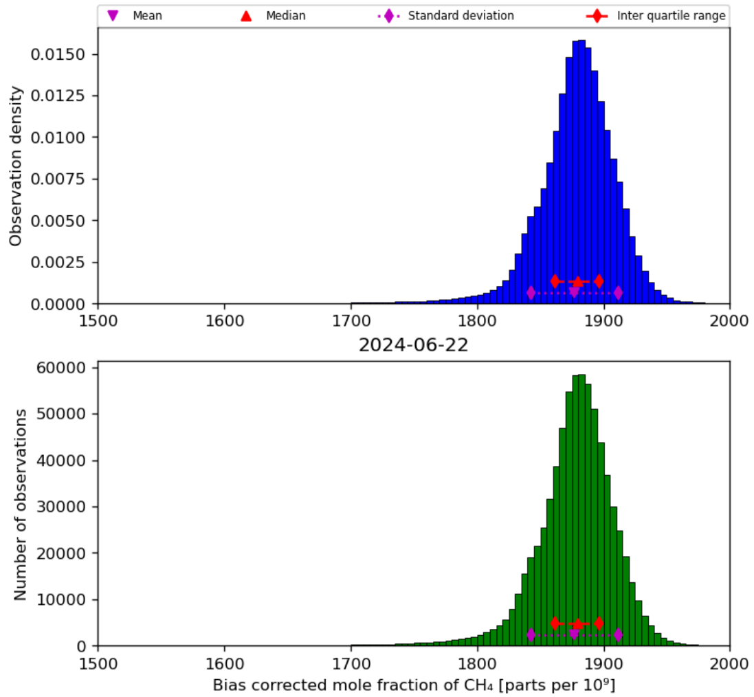
Figure 25: Histogram of “Bias corrected mole fraction of CH 4 ” for 2024-06-21 to 2024-06-23
