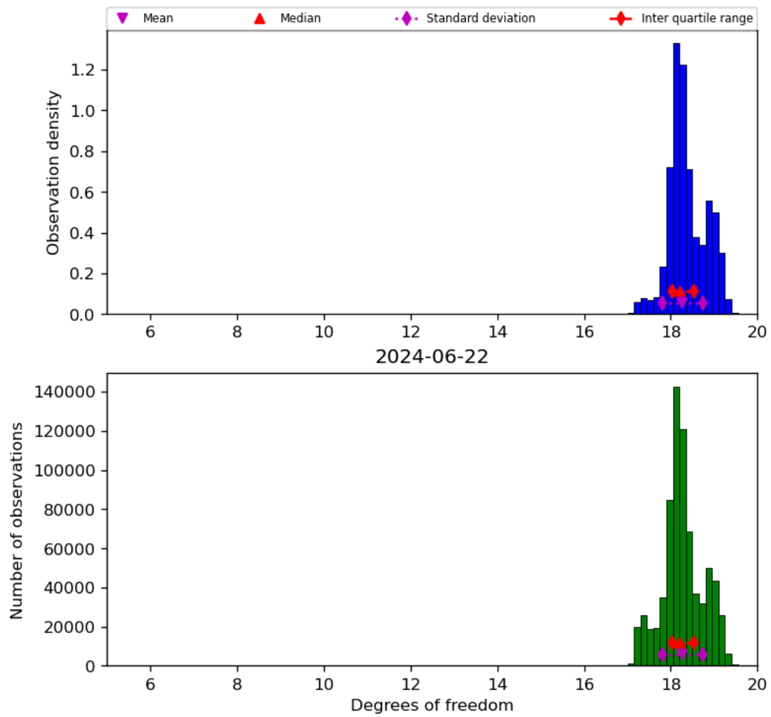
Figure 30: Histogram of “Degrees of freedom” for 2024-06-21 to 2024-06-23
