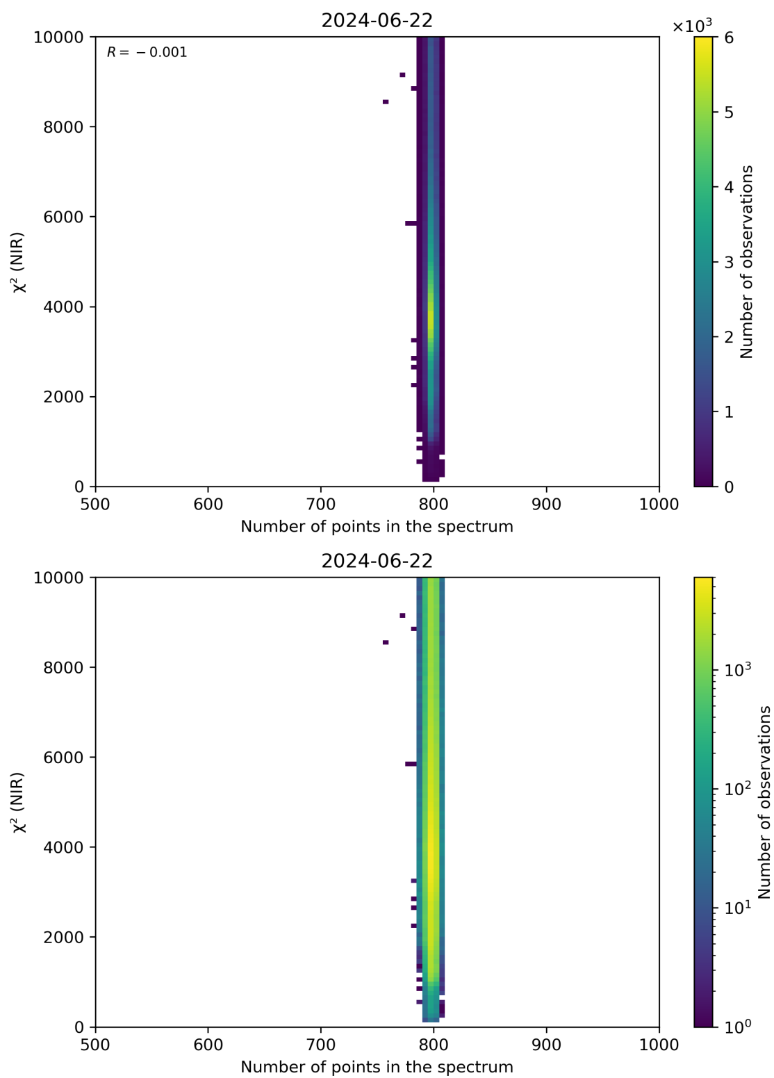
Figure 88: Scatter density plot of “Number of points in the spectrum” against “ \chi^2 (NIR)” for 2024-06-21 to 2024-06-23.
