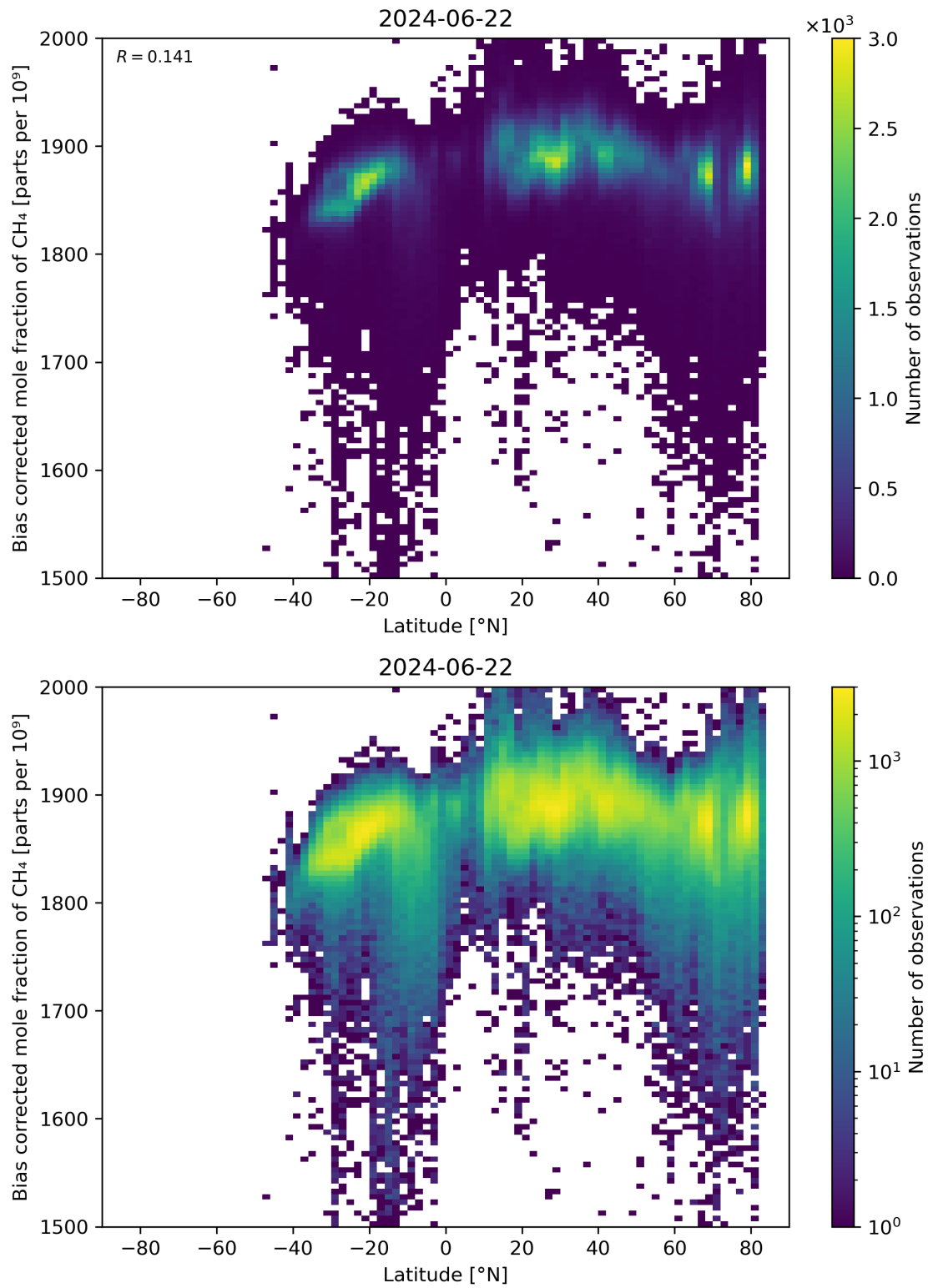
Figure 58: Scatter density plot of “Latitude” against “Bias corrected mole fraction of CH 4 ” for 2024-06-21 to 2024-06-23.
