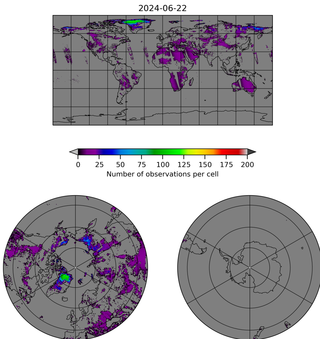
Figure 10: Map of the number of observations for 2024-06-21 to 2024-06-23
