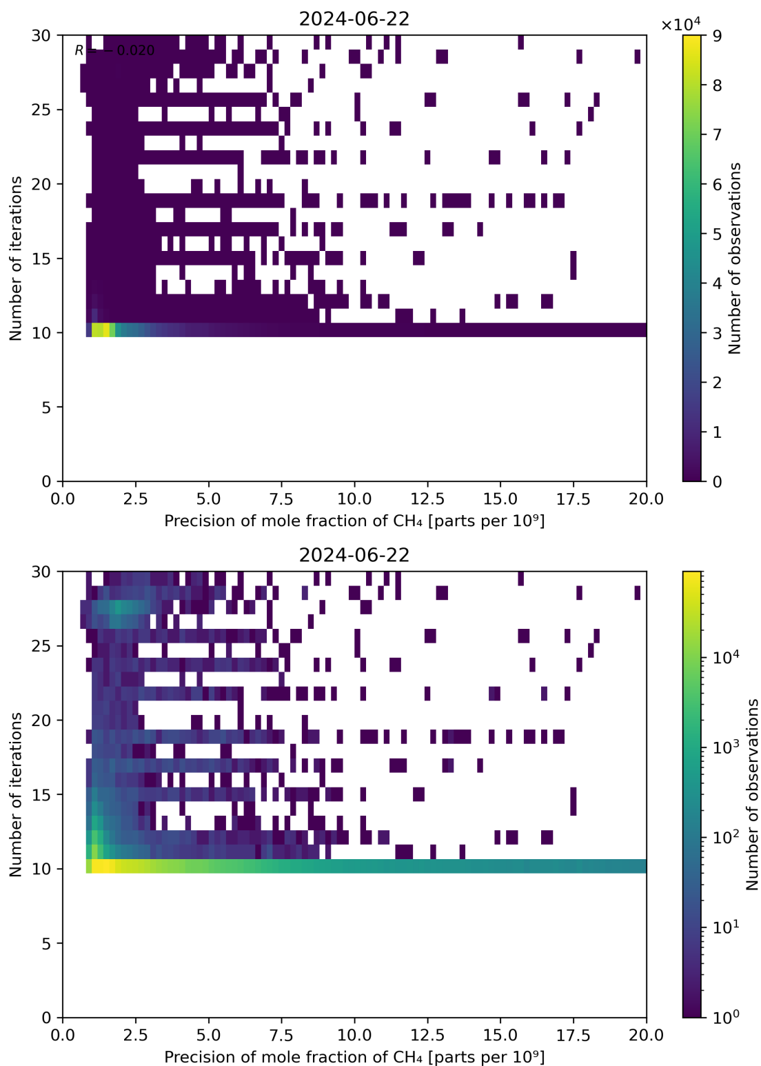
Figure 83: Scatter density plot of “Precision of mole fraction of CH 4 ” against “Number of iterations” for 2024-06-21 to 2024-06-23.
