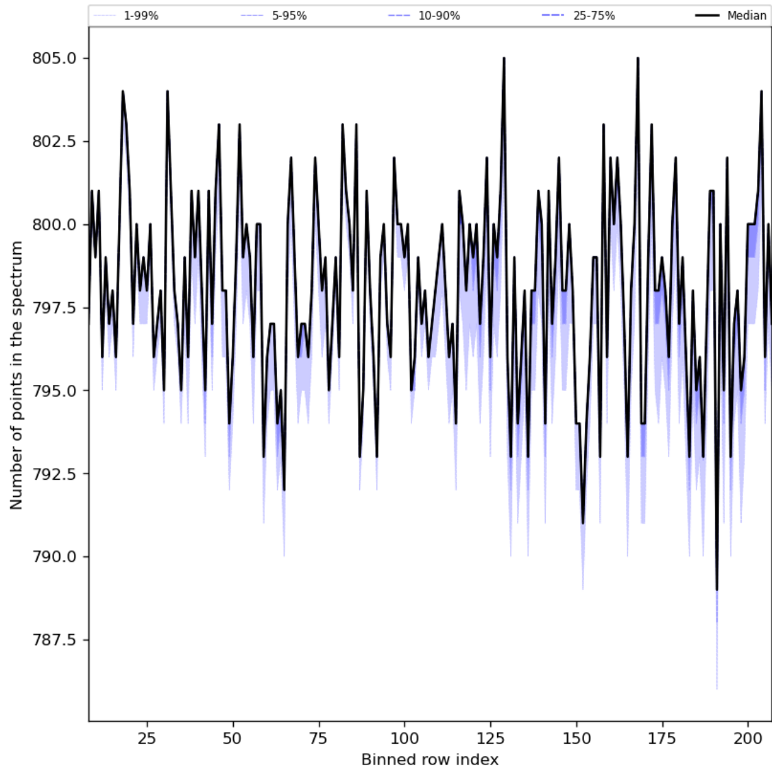
Figure 37: Along track statistics of “Number of points in the spectrum” for 2024-06-21 to 2024-06-23
