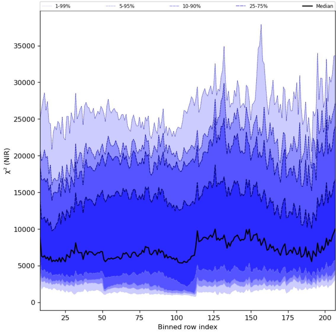
Figure 40: Along track statistics of “ \chi^2 (NIR)” for 2024-06-21 to 2024-06-23
