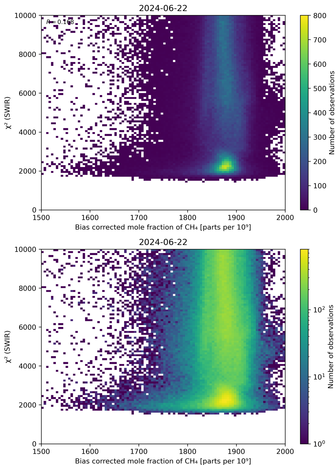
Figure 64: Scatter density plot of “Bias corrected mole fraction of \text{CH}_4 ” against “ \chi^2 (SWIR)” for 2024-06-21 to 2024-06-23.
