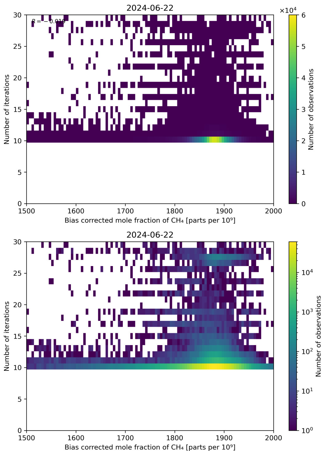
Figure 67: Scatter density plot of “Bias corrected mole fraction of CH 4 ” against “Number of iterations” for 2024-06-21 to 2024-06-23.
