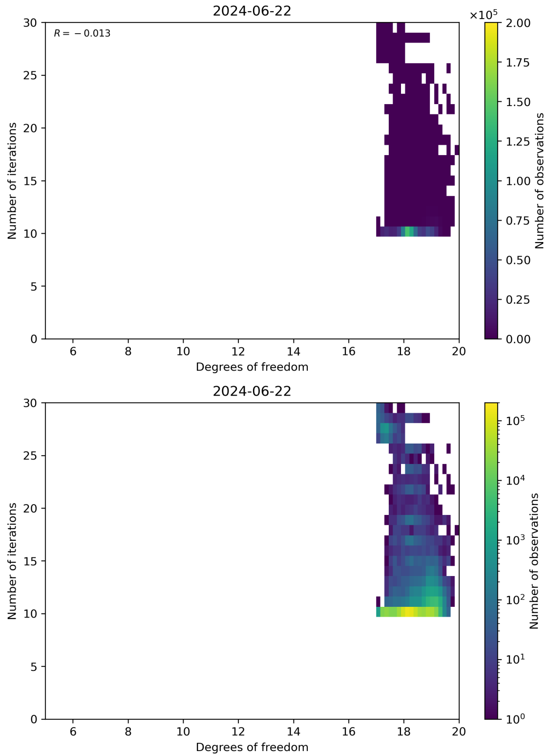
Figure 52: Scatter density plot of “Degrees of freedom” against “Number of iterations” for 2024-06-21 to 2024-06-23.
