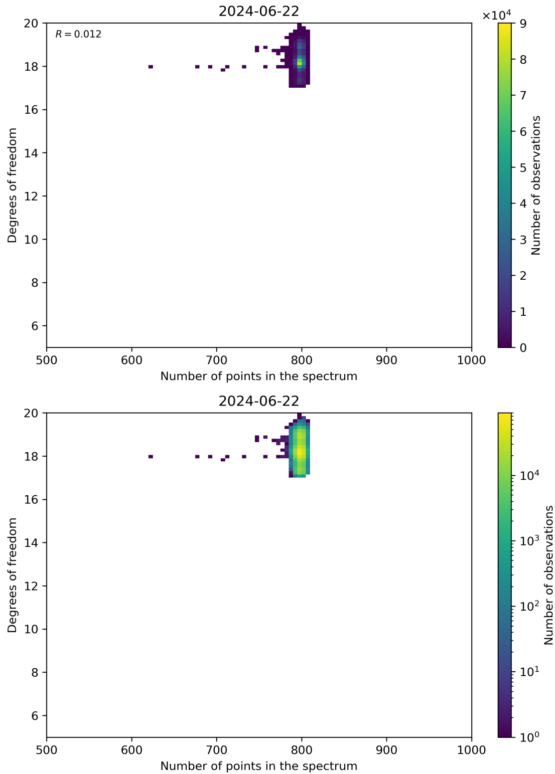
Figure 90: Scatter density plot of “Number of points in the spectrum” against “Degrees of freedom” for 2024-06-21 to 2024-06-23.
