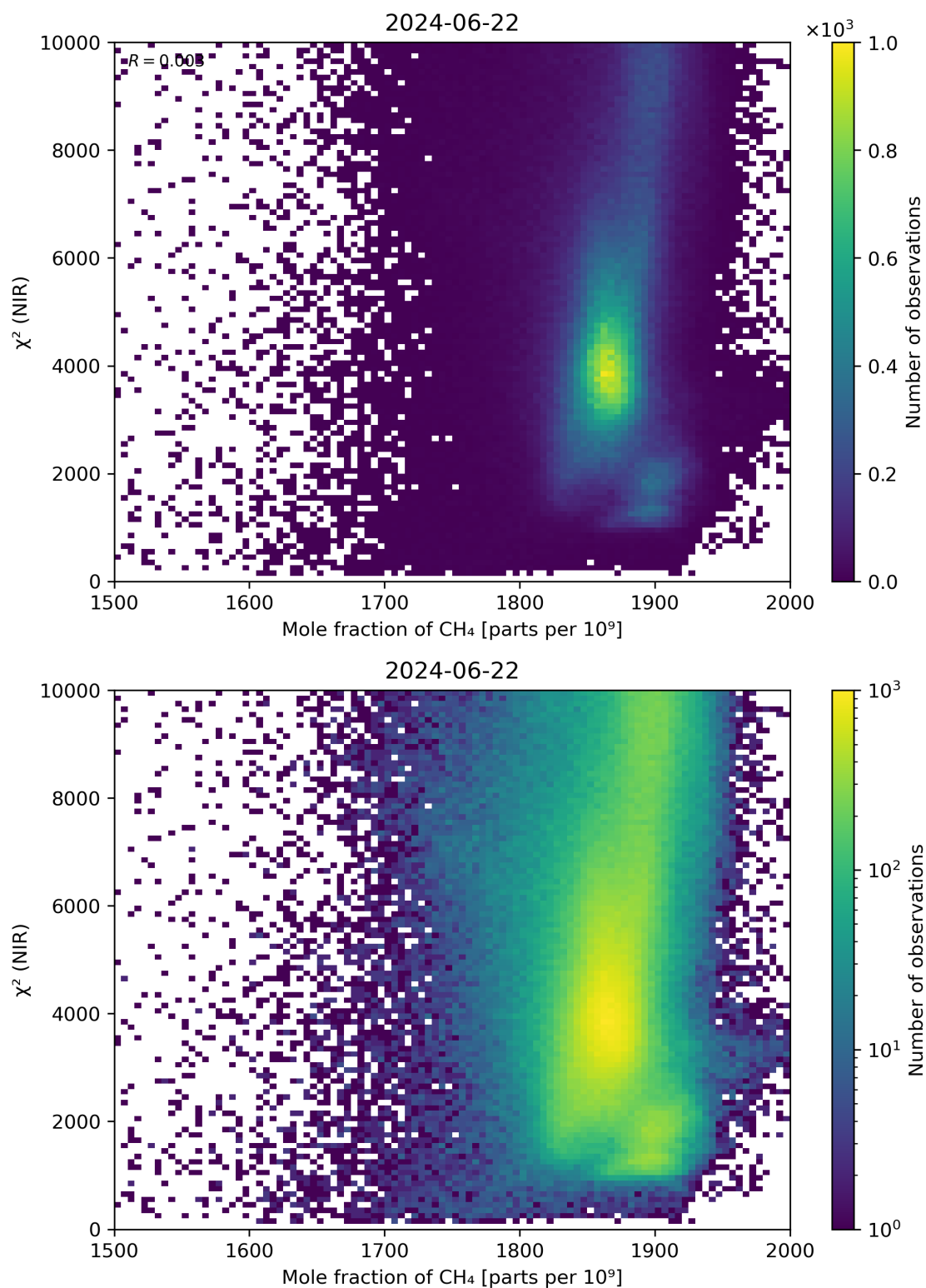
Figure 70: Scatter density plot of “Mole fraction of \text{CH}_4 ” against “ \chi^2 (NIR)” for 2024-06-21 to 2024-06-23.
