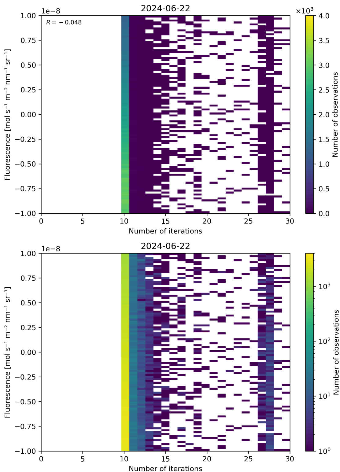
Figure 87: Scatter density plot of “Number of iterations” against “Fluorescence” for 2024-06-21 to 2024-06-23.
