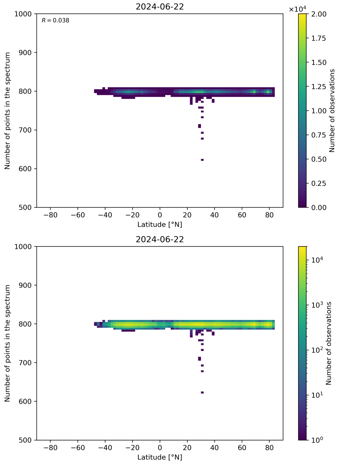
Figure 61: Scatter density plot of “Latitude” against “Number of points in the spectrum” for 2024-06-21 to 2024-06-23.
