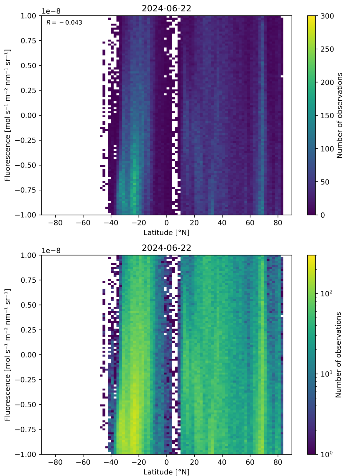
Figure 56: Scatter density plot of “Latitude” against “Fluorescence” for 2024-06-21 to 2024-06-23.
