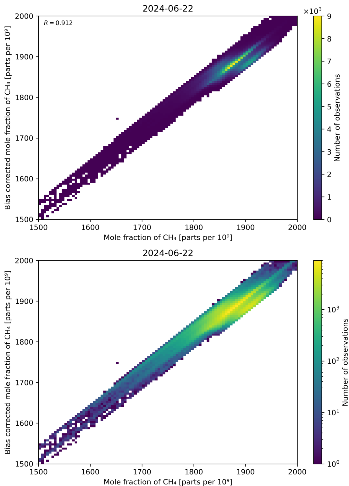
Figure 74: Scatter density plot of “Mole fraction of CH 4 ” against “Bias corrected mole fraction of CH 4 ” for 2024-06-21 to 2024-06-23.
