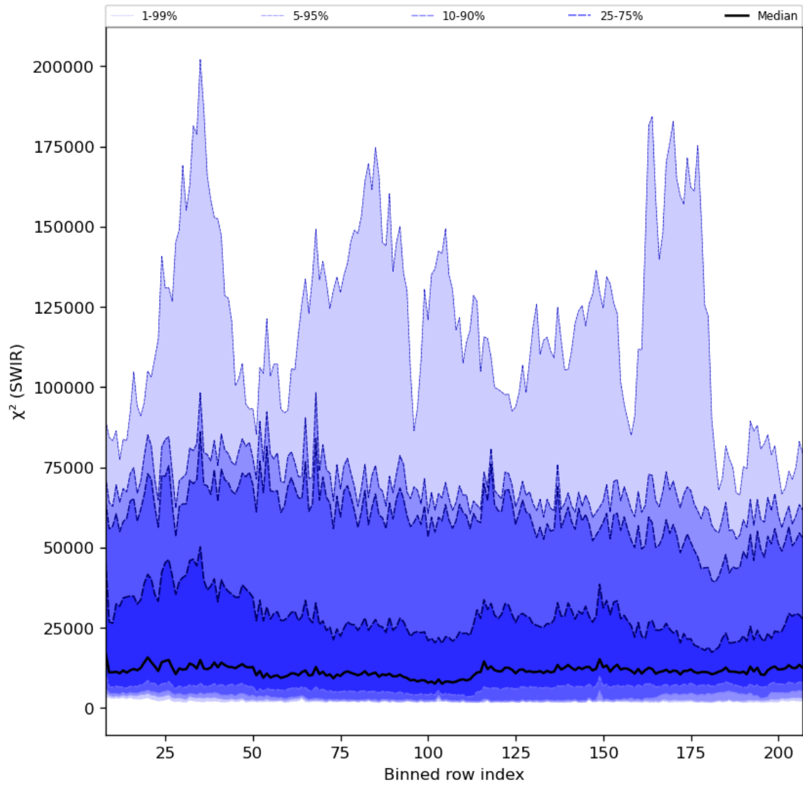
Figure 39: Along track statistics of “ \chi^2 (SWIR)” for 2024-06-21 to 2024-06-23
