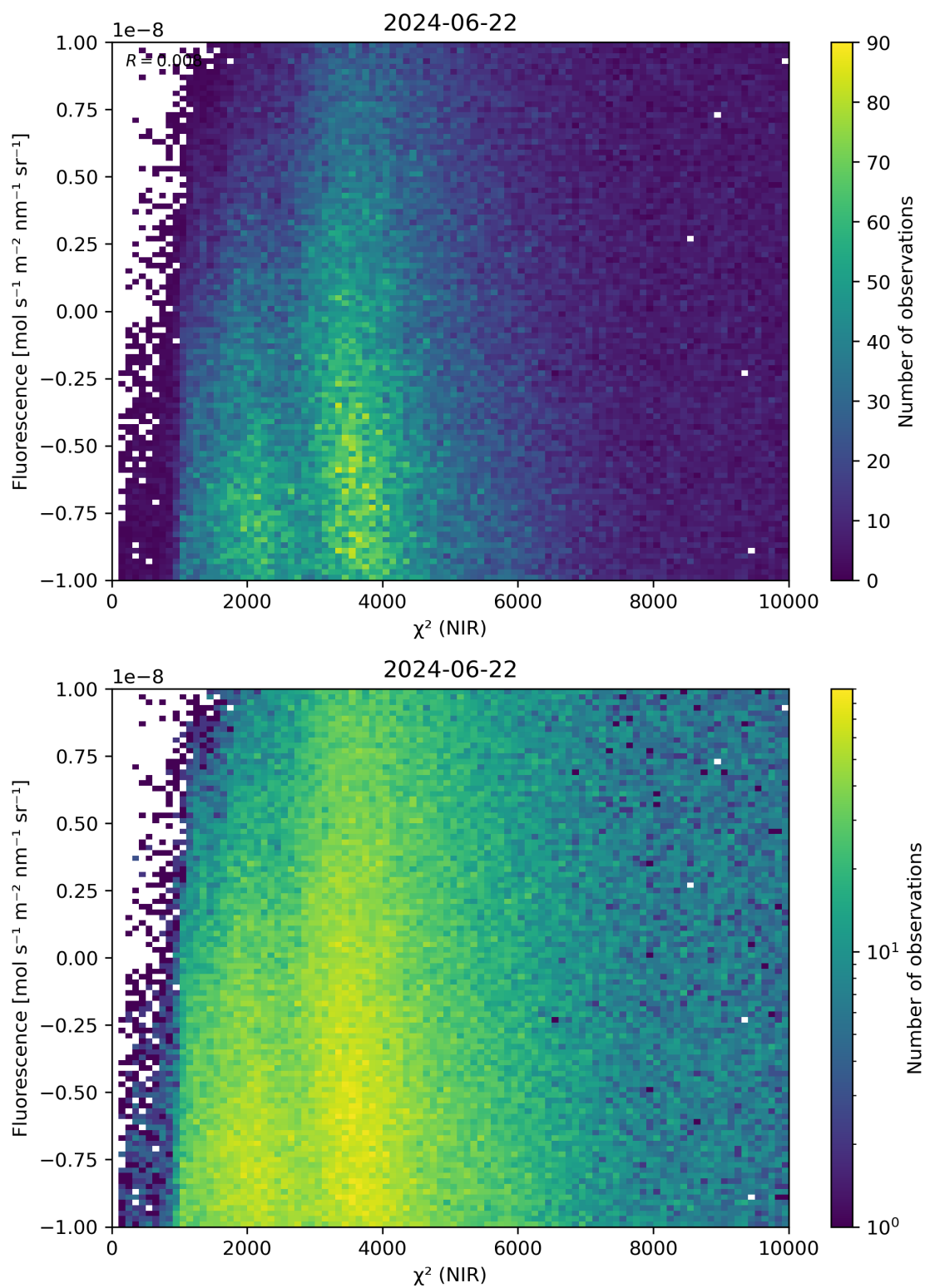
Figure 45: Scatter density plot of “ \chi^2 (NIR)” against “Fluorescence” for 2024-06-21 to 2024-06-23.
