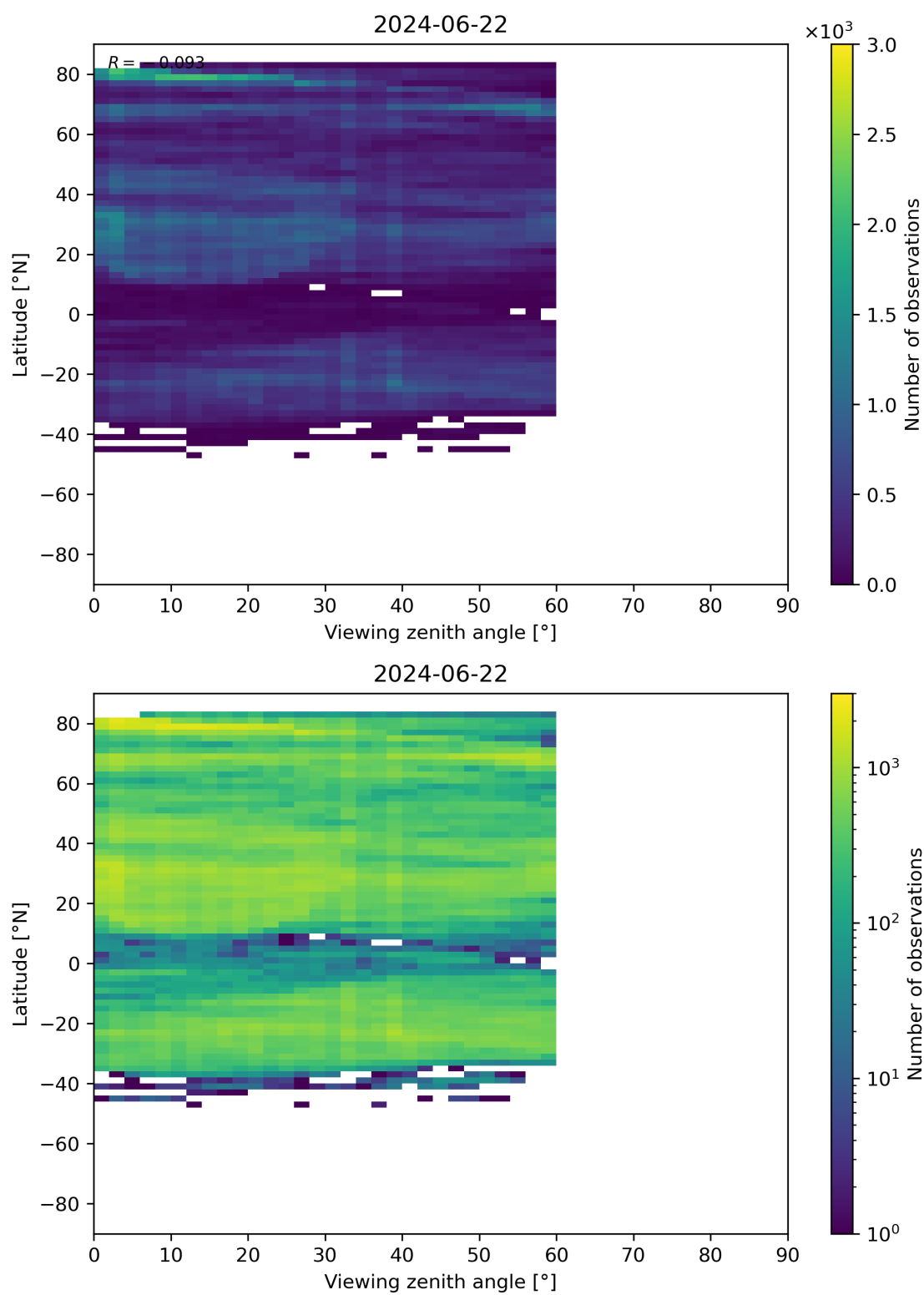
Figure 109: Scatter density plot of “Viewing zenith angle” against “Latitude” for 2024-06-21 to 2024-06-23.
