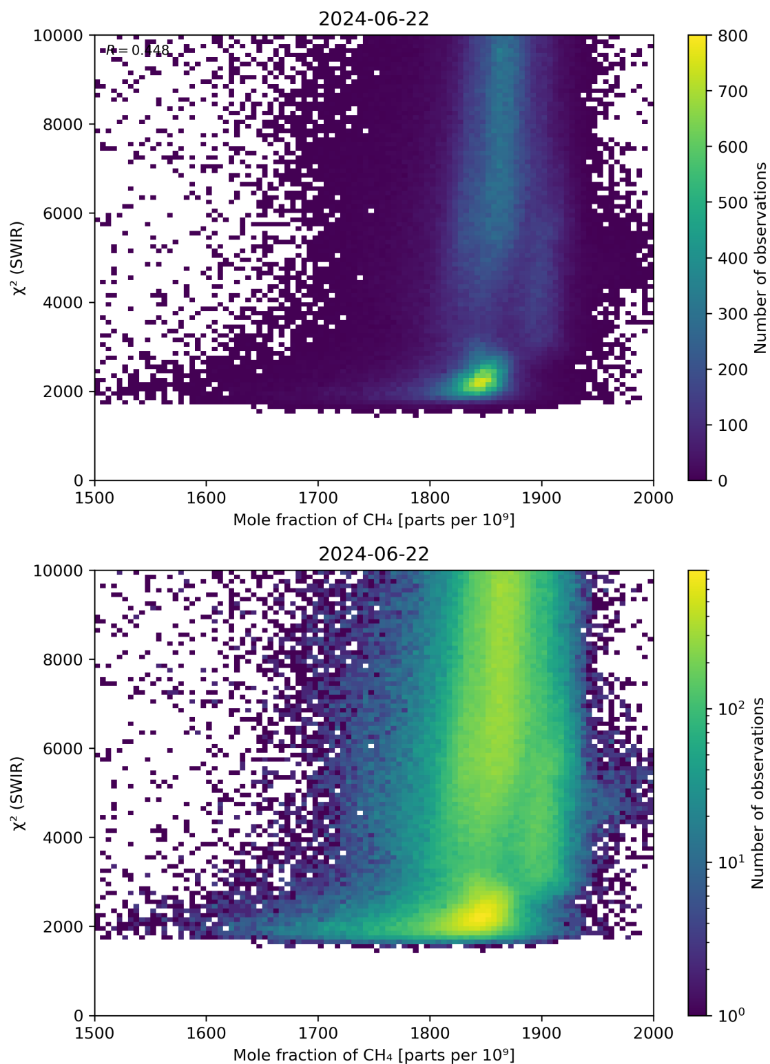
Figure 71: Scatter density plot of “Mole fraction of \text{CH}_4 ” against “ \chi^2 (SWIR)” for 2024-06-21 to 2024-06-23.
