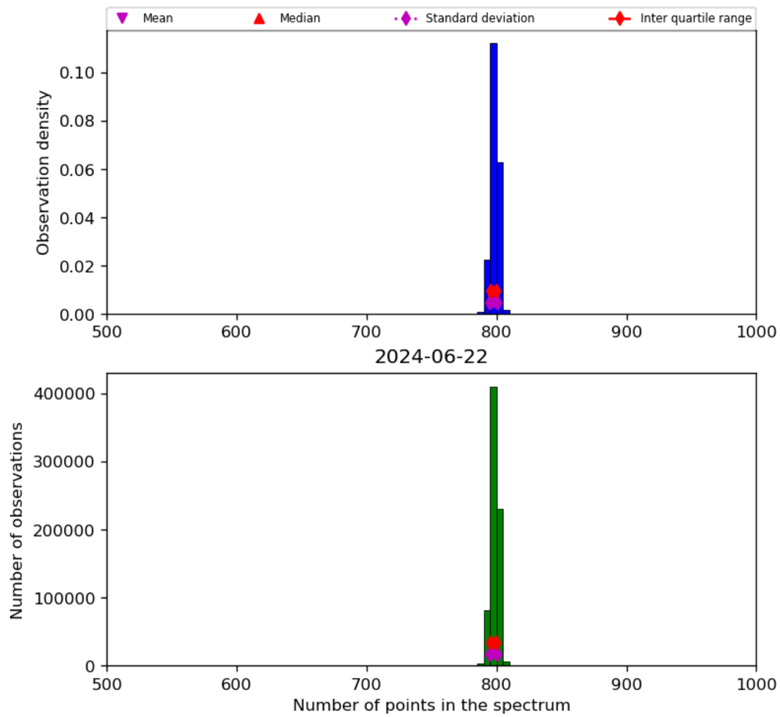
Figure 26: Histogram of “Number of points in the spectrum” for 2024-06-21 to 2024-06-23
