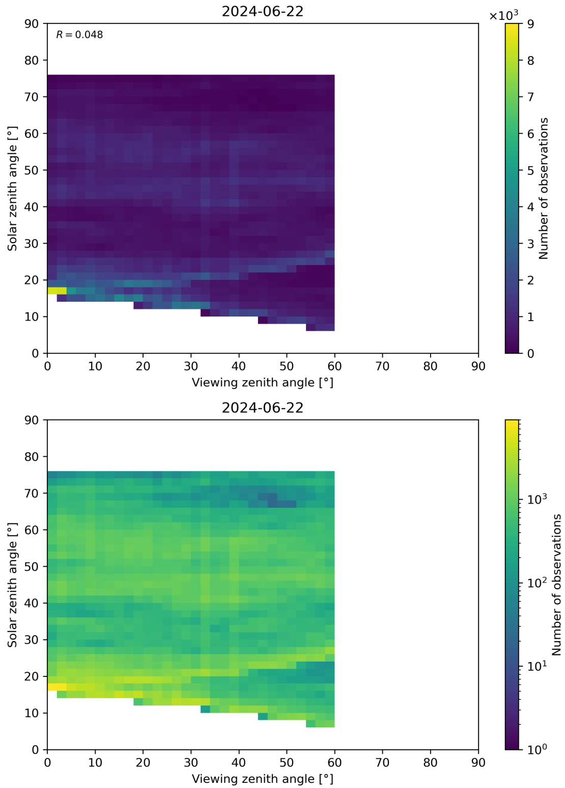
Figure 115: Scatter density plot of “Viewing zenith angle” against “Solar zenith angle” for 2024-06-21 to 2024-06-23.
