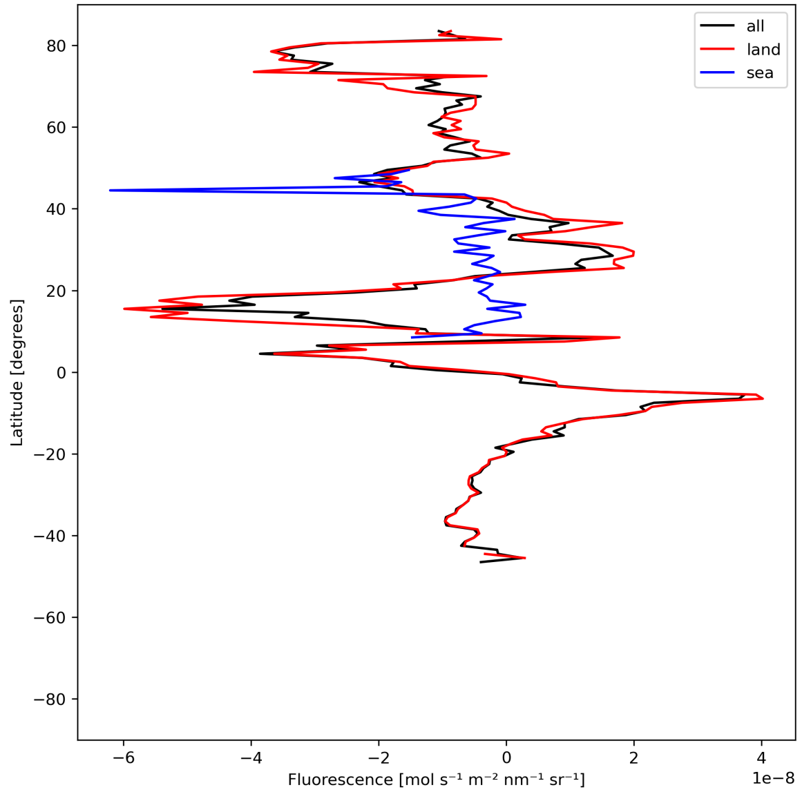
Figure 21: Zonal average of “Fluorescence” for 2024-06-21 to 2024-06-23.
