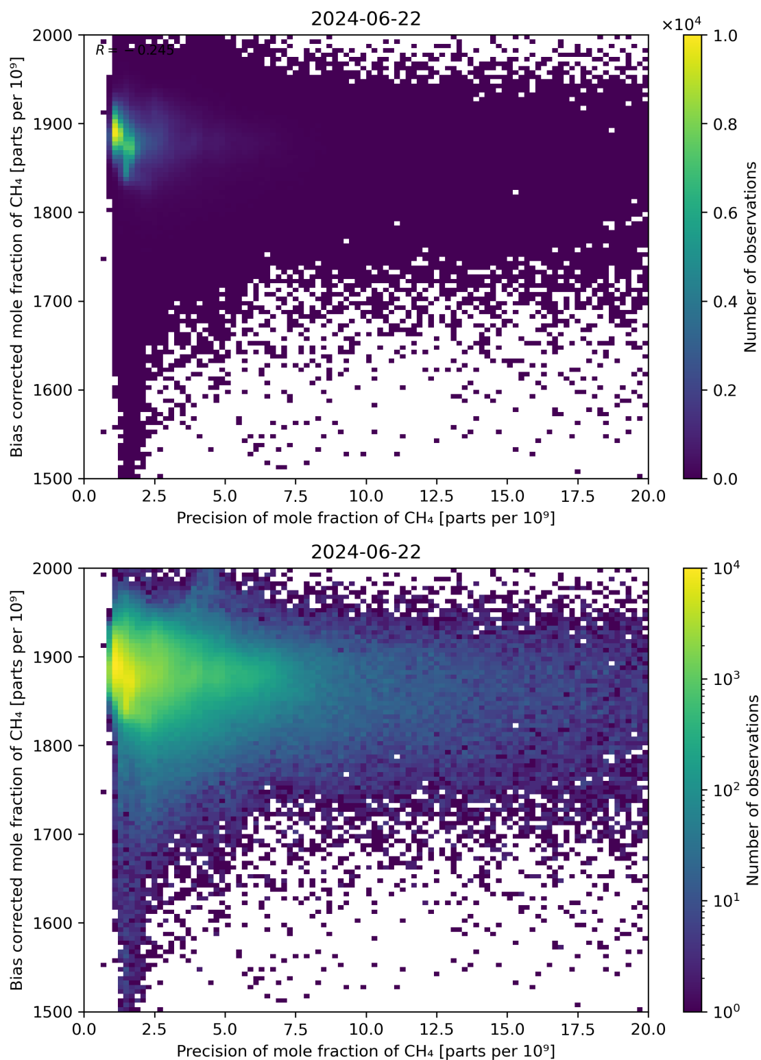
Figure 82: Scatter density plot of “Precision of mole fraction of CH 4 ” against “Bias corrected mole fraction of CH 4 ” for 2024-06-21 to 2024-06-23.
