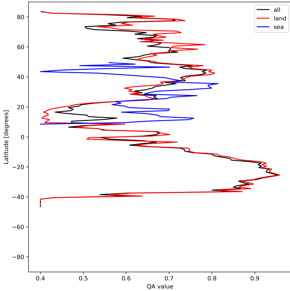
Figure 11: Zonal average of “QA value” for 2024-06-21 to 2024-06-23.
