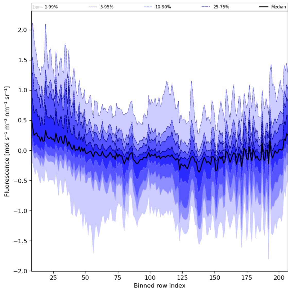
Figure 43: Along track statistics of “Fluorescence” for 2024-06-21 to 2024-06-23
