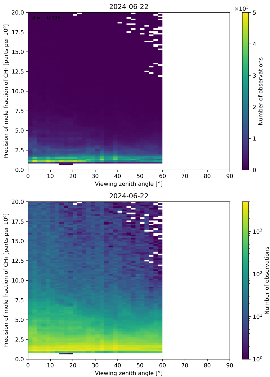
Figure 112: Scatter density plot of “Viewing zenith angle” against “Precision of mole fraction of CH 4 ” for 2024-06-21 to 2024-06-23.
