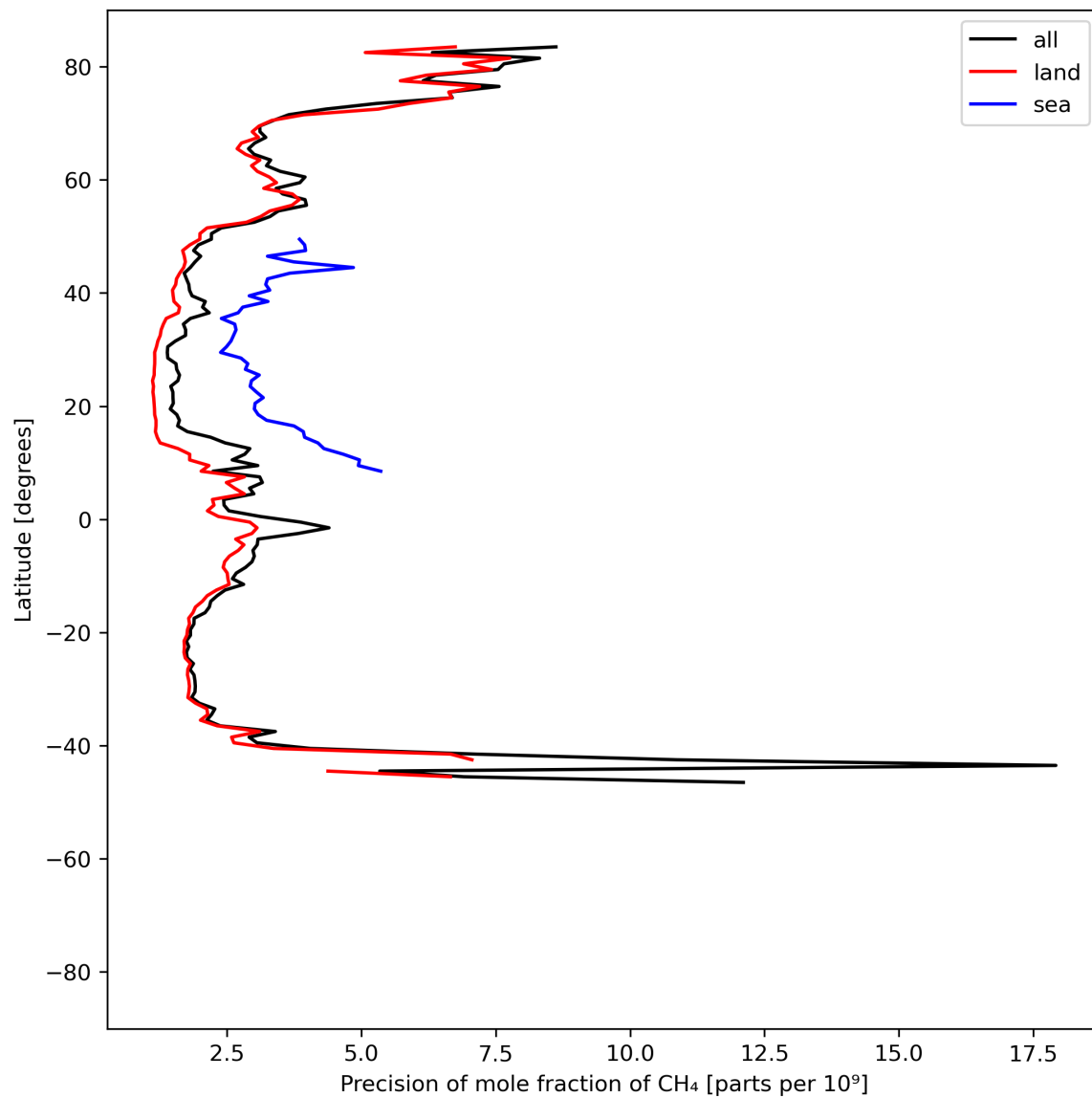
Figure 13: Zonal average of “Precision of mole fraction of CH 4 ” for 2024-06-21 to 2024-06-23.
