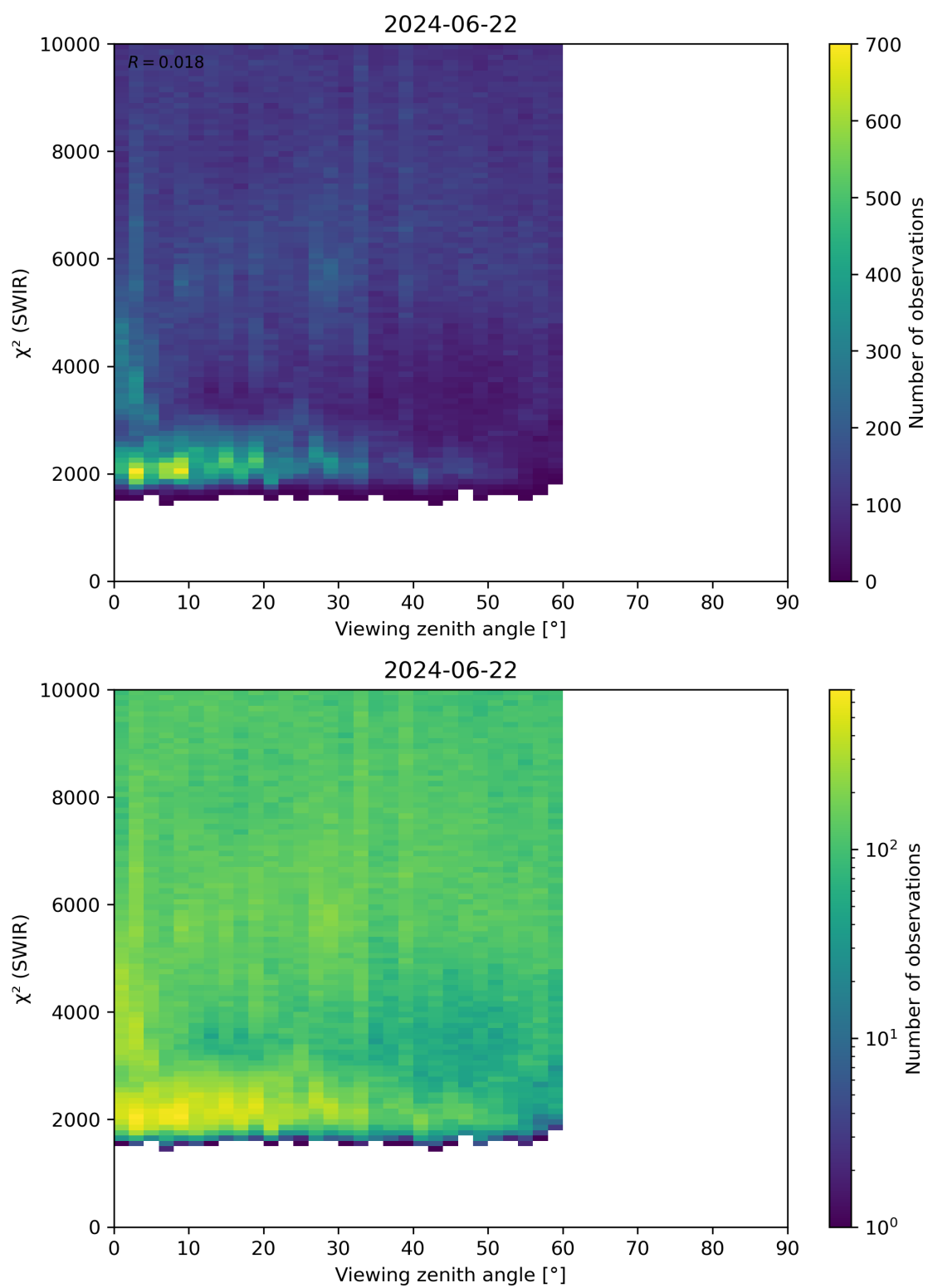
Figure 106: Scatter density plot of “Viewing zenith angle” against “ \chi^2 (SWIR)” for 2024-06-21 to 2024-06-23.
