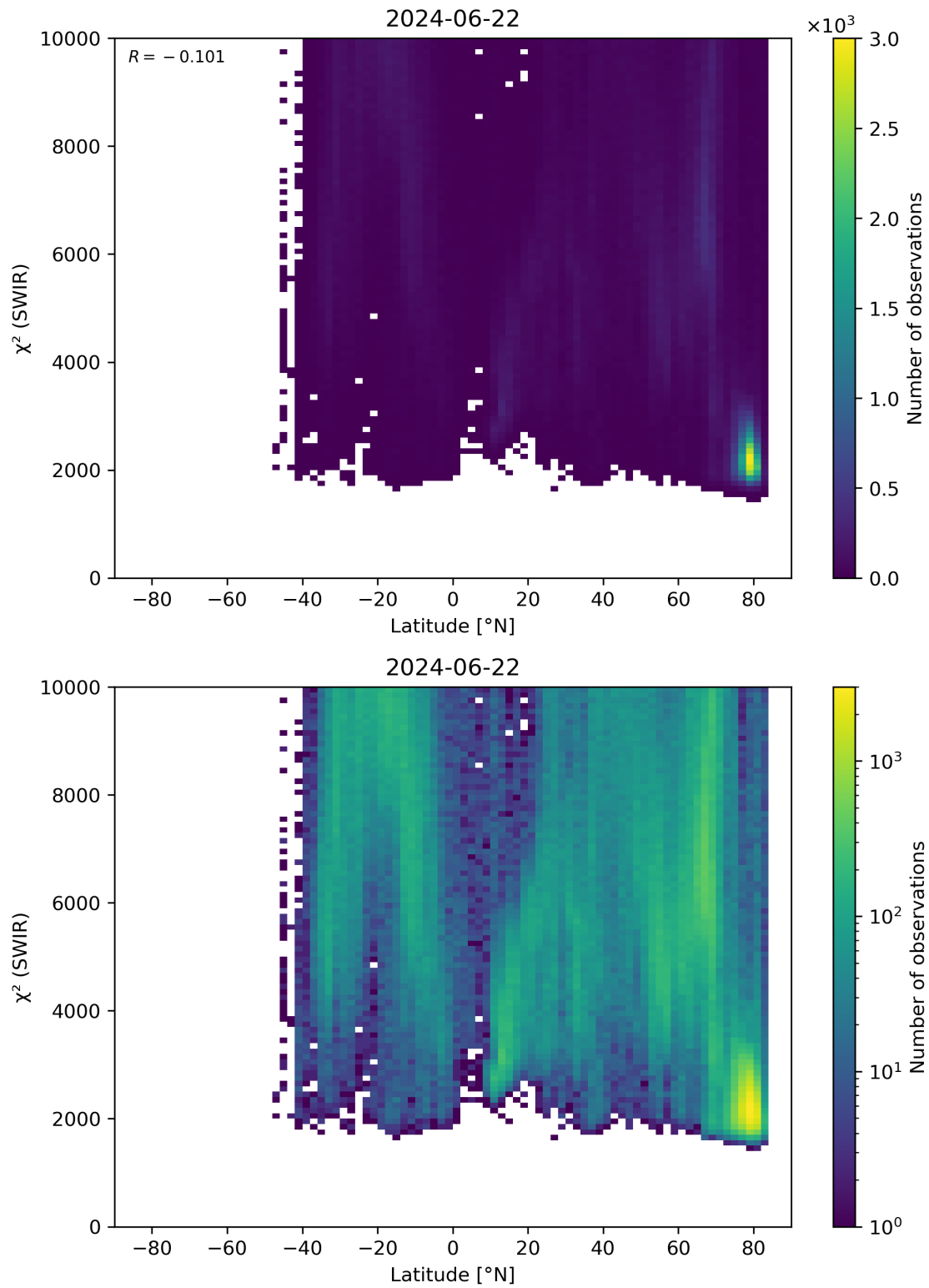
Figure 54: Scatter density plot of “Latitude” against “ \chi^2 (SWIR)” for 2024-06-21 to 2024-06-23.
