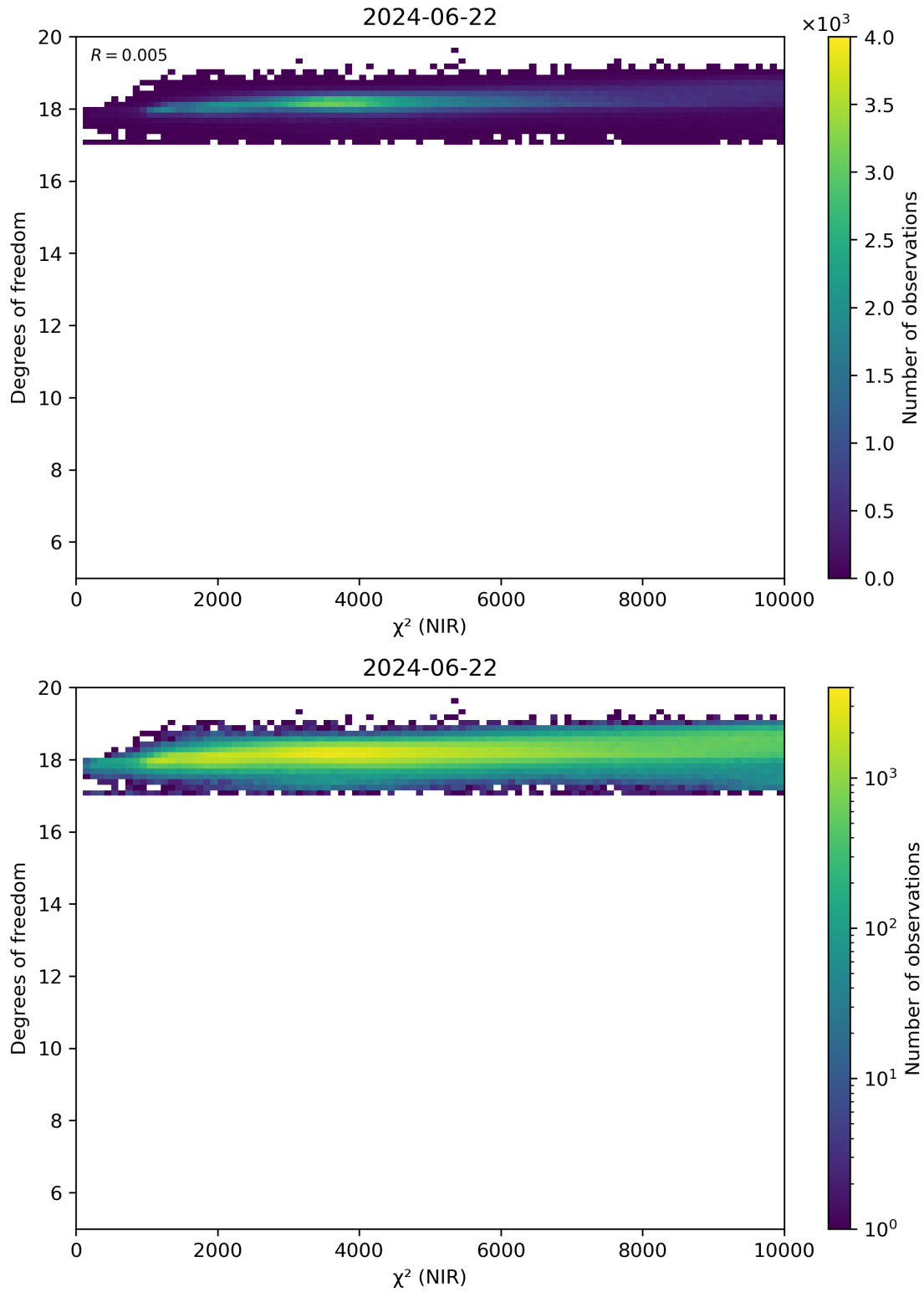
Figure 44: Scatter density plot of “ \chi^2 (NIR)” against “Degrees of freedom” for 2024-06-21 to 2024-06-23.
