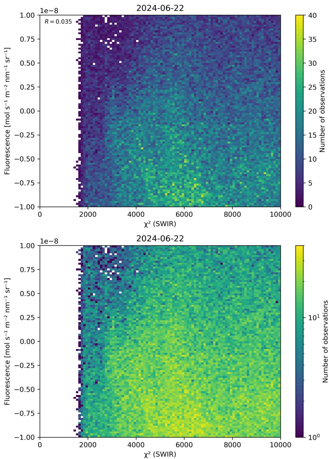
Figure 49: Scatter density plot of “ \chi^2 (SWIR)” against “Fluorescence” for 2024-06-21 to 2024-06-23.
