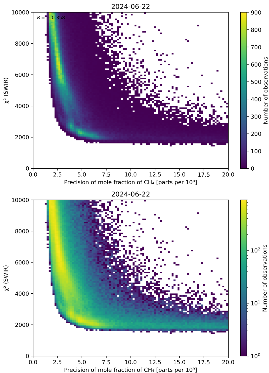
Figure 79: Scatter density plot of “Precision of mole fraction of CH 4 ” against “ \chi^2 (SWIR)” for 2024-06-21 to 2024-06-23.
