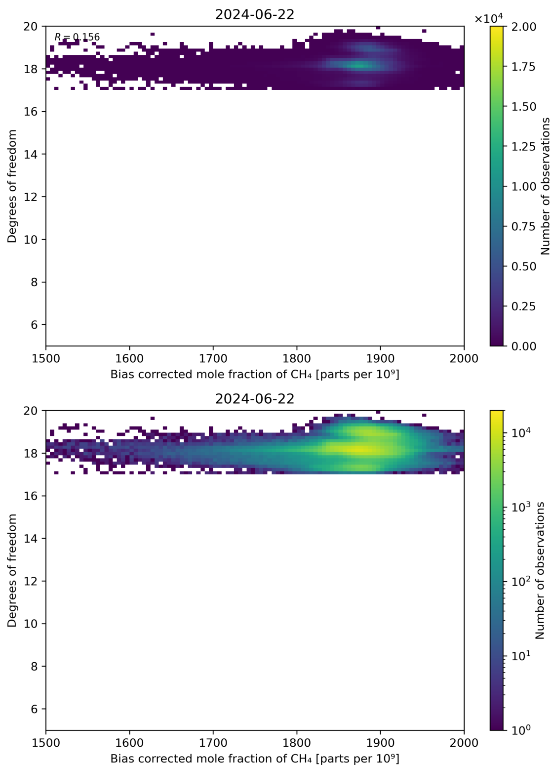
Figure 65: Scatter density plot of “Bias corrected mole fraction of CH 4 ” against “Degrees of freedom” for 2024-06-21 to 2024-06-23.
