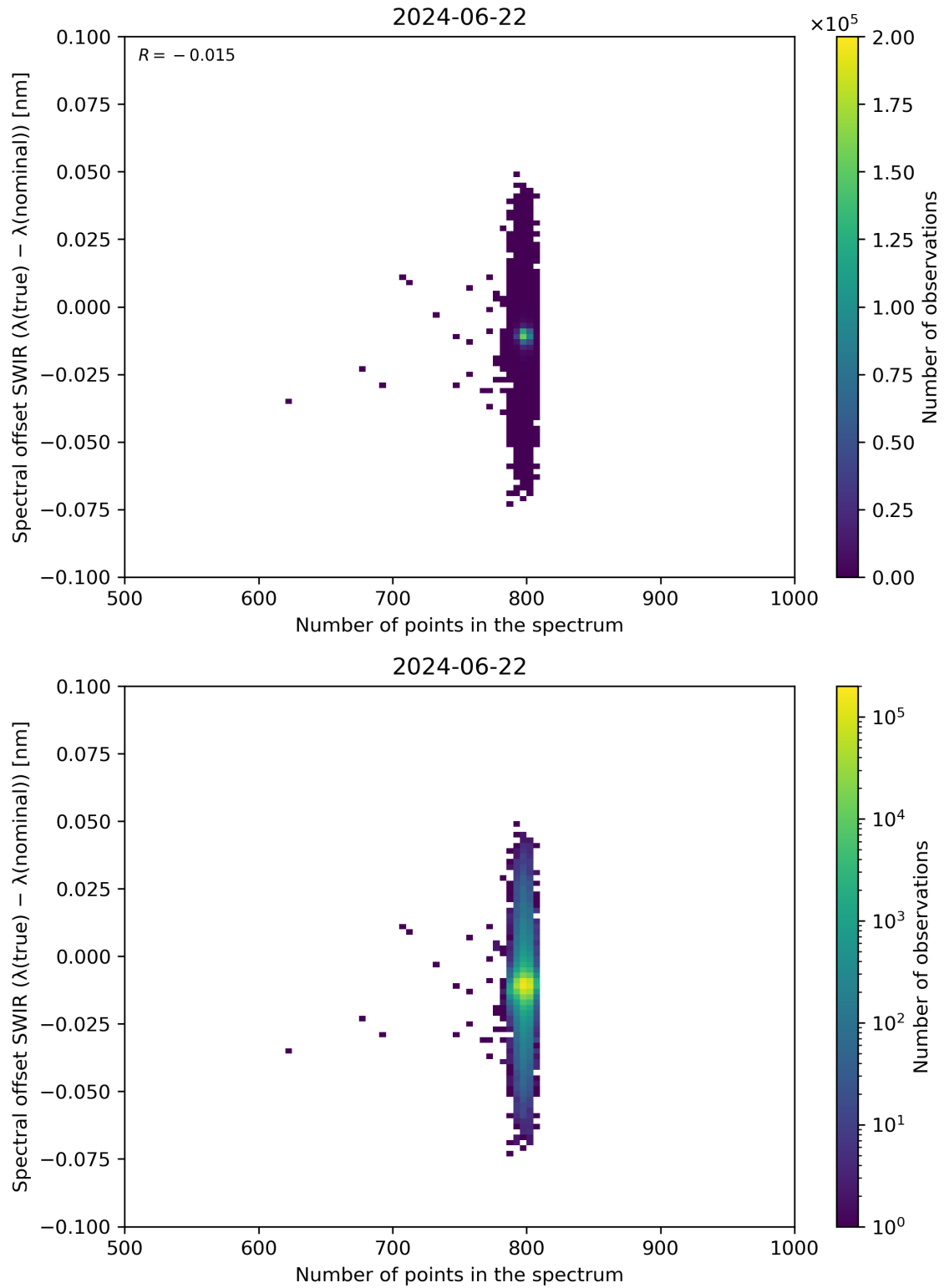
Figure 93: Scatter density plot of “Number of points in the spectrum” against “Spectral offset SWIR ( \lambda(\text{true}) - \lambda(\text{nominal}) )” for 2024-06-21 to 2024-06-23.
