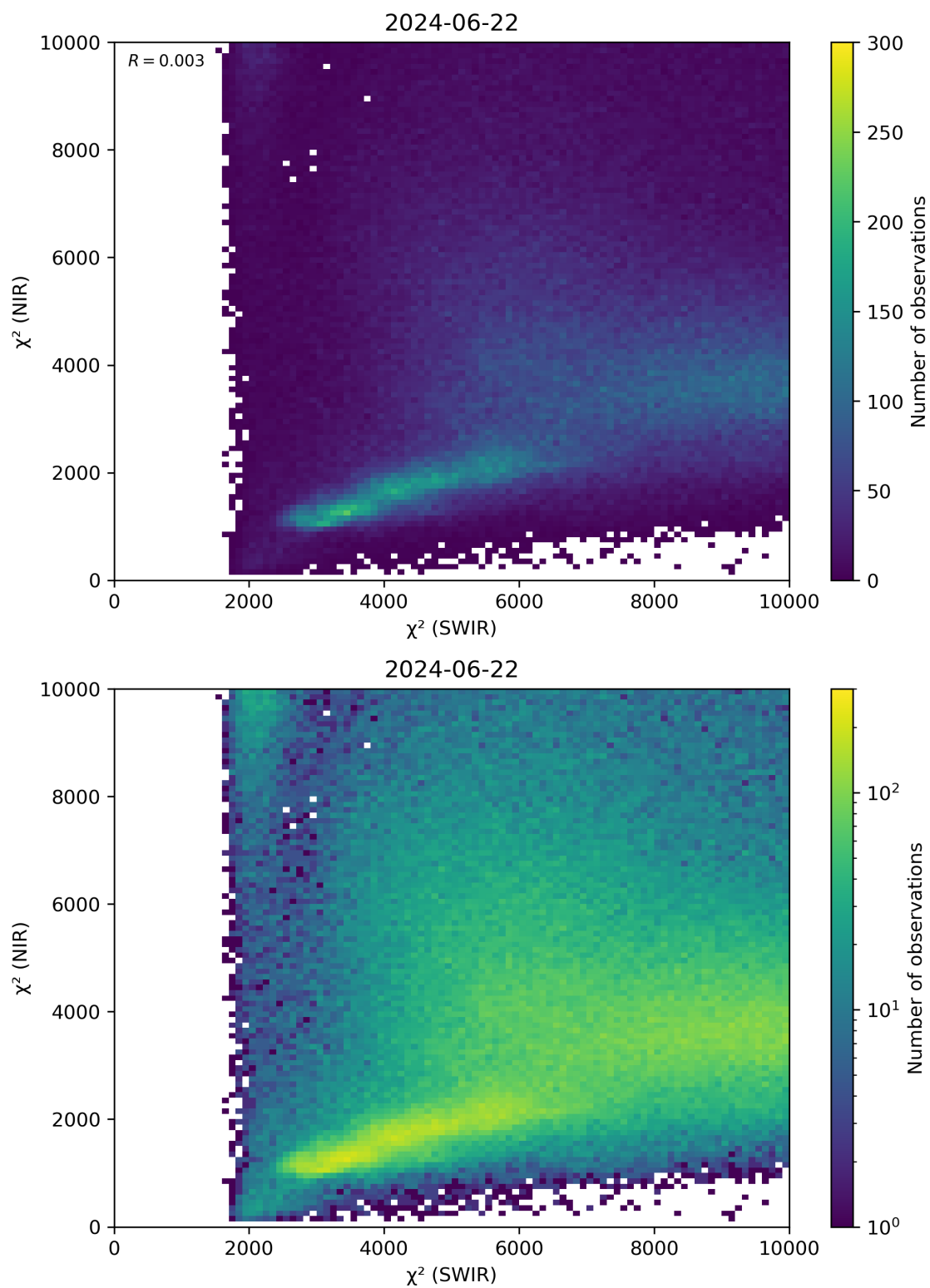
Figure 47: Scatter density plot of “ \chi^2 (SWIR)” against “ \chi^2 (NIR)” for 2024-06-21 to 2024-06-23.
