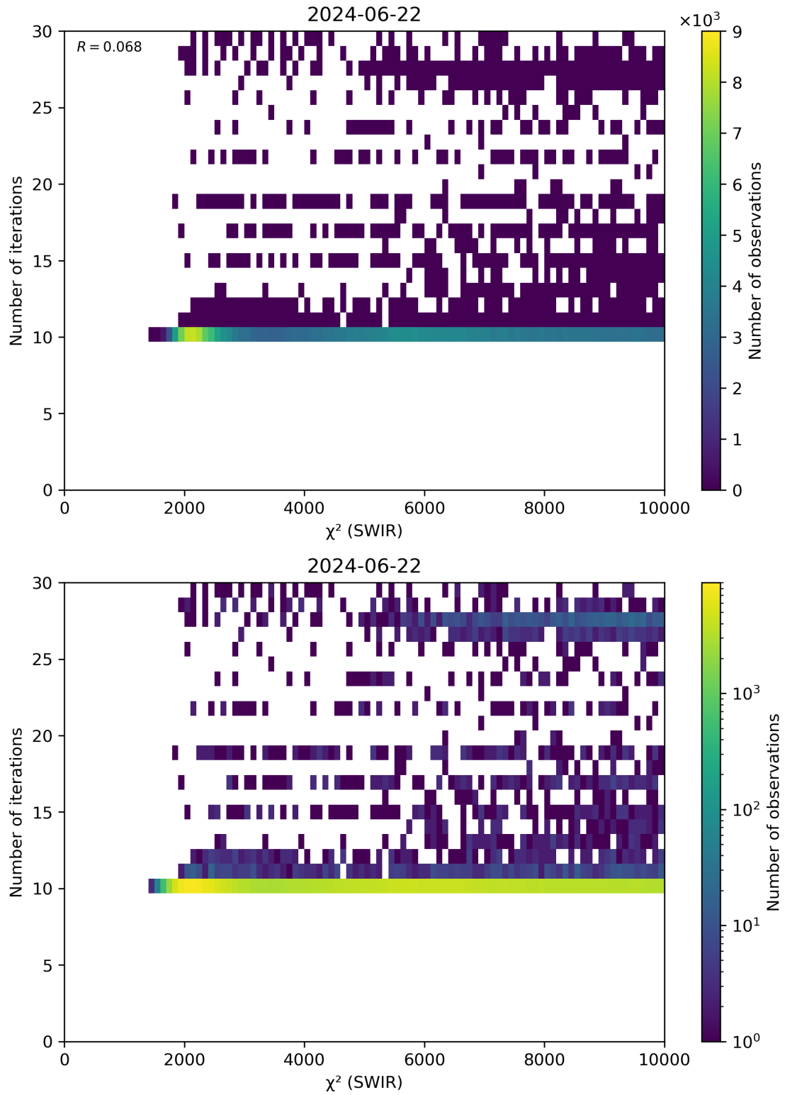
Figure 50: Scatter density plot of “ \chi^2 (SWIR)” against “Number of iterations” for 2024-06-21 to 2024-06-23.
