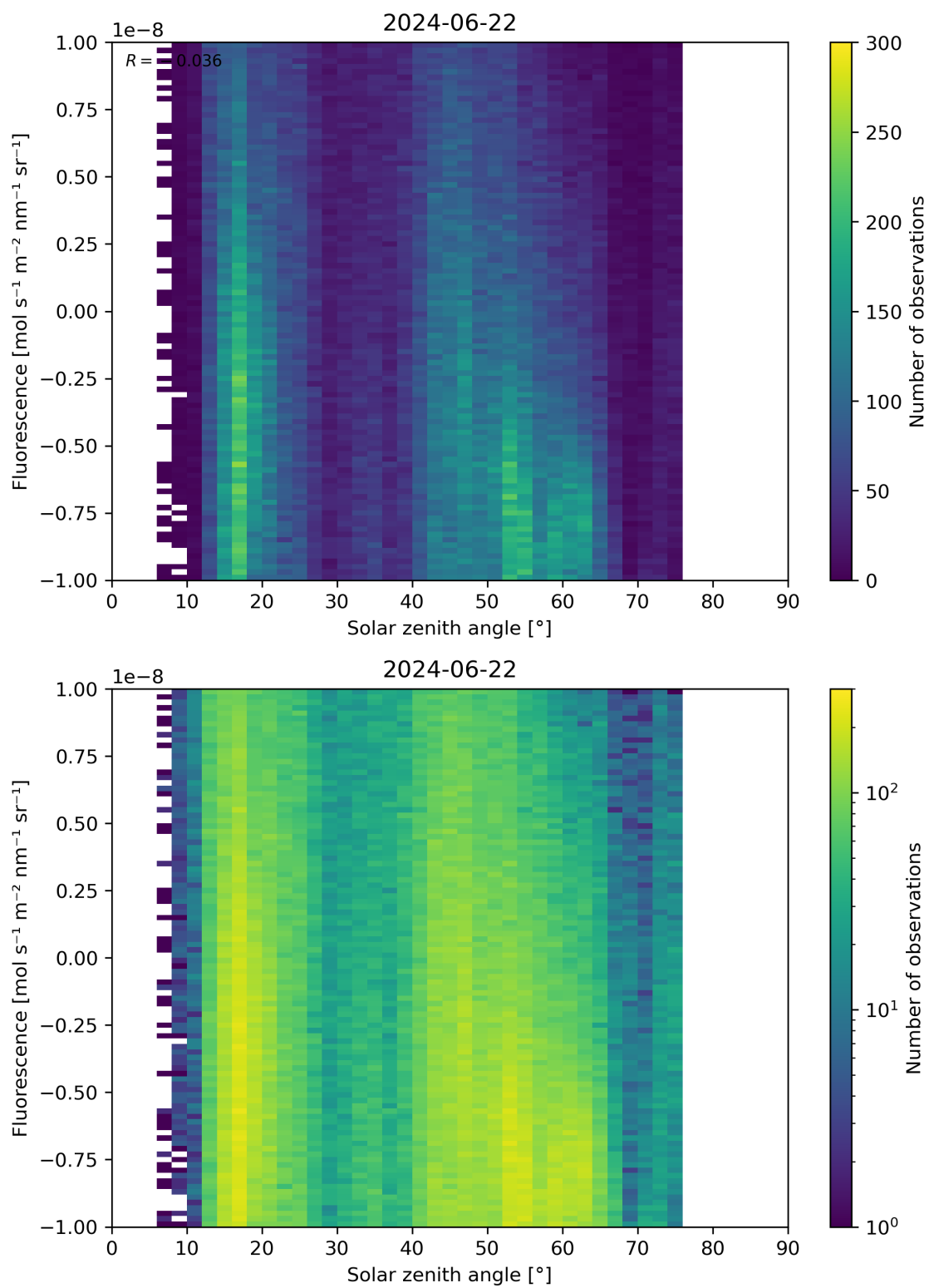
Figure 97: Scatter density plot of “Solar zenith angle” against “Fluorescence” for 2024-06-21 to 2024-06-23.
