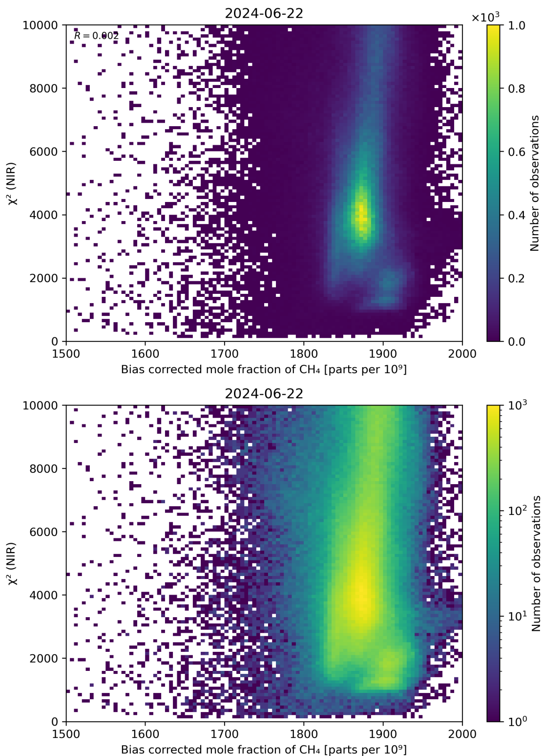
Figure 63: Scatter density plot of “Bias corrected mole fraction of CH 4 ” against “ \chi^2 (NIR)” for 2024-06-21 to 2024-06-23.
