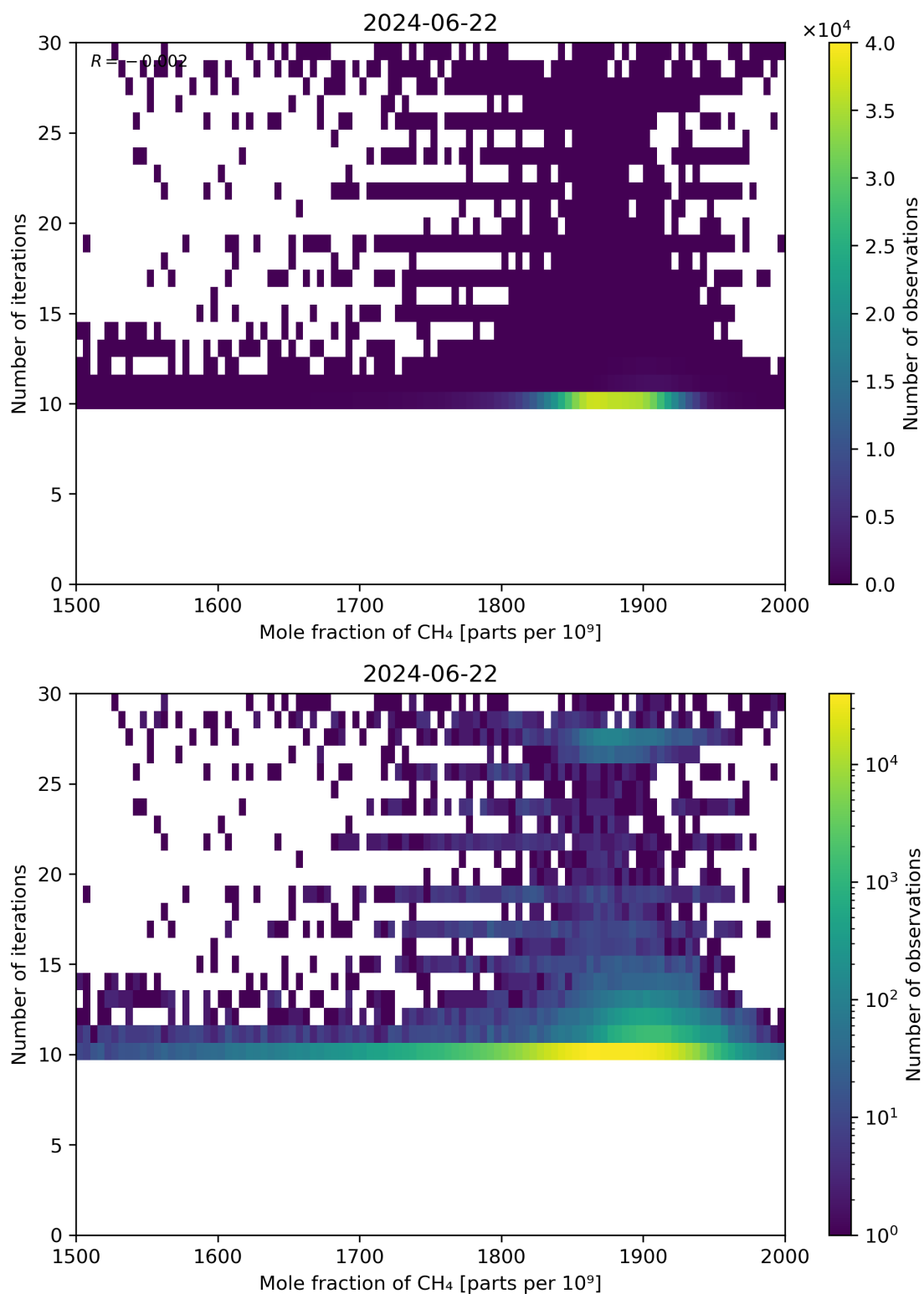
Figure 76: Scatter density plot of “Mole fraction of CH 4 ” against “Number of iterations” for 2024-06-21 to 2024-06-23.
