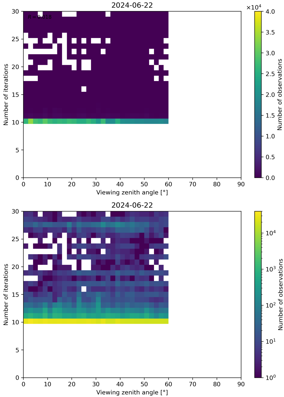
Figure 113: Scatter density plot of “Viewing zenith angle” against “Number of iterations” for 2024-06-21 to 2024-06-23.
