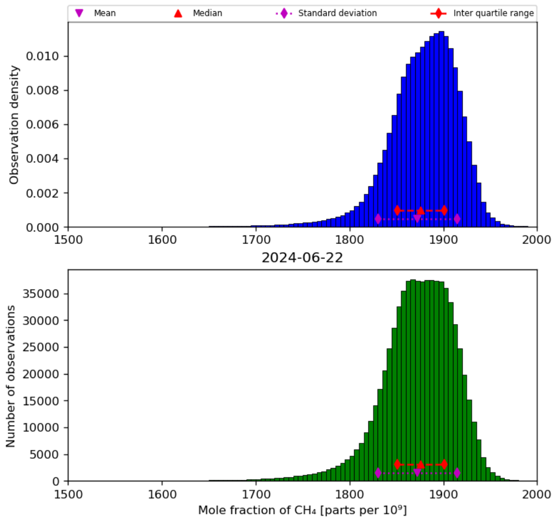
Figure 23: Histogram of “Mole fraction of CH 4 ” for 2024-06-21 to 2024-06-23
