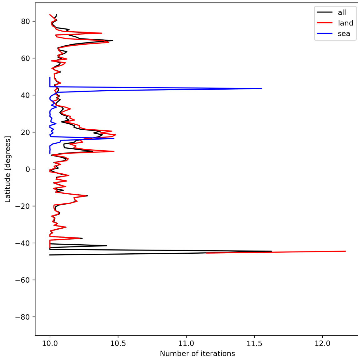
Figure 20: Zonal average of “Number of iterations” for 2024-06-21 to 2024-06-23.
