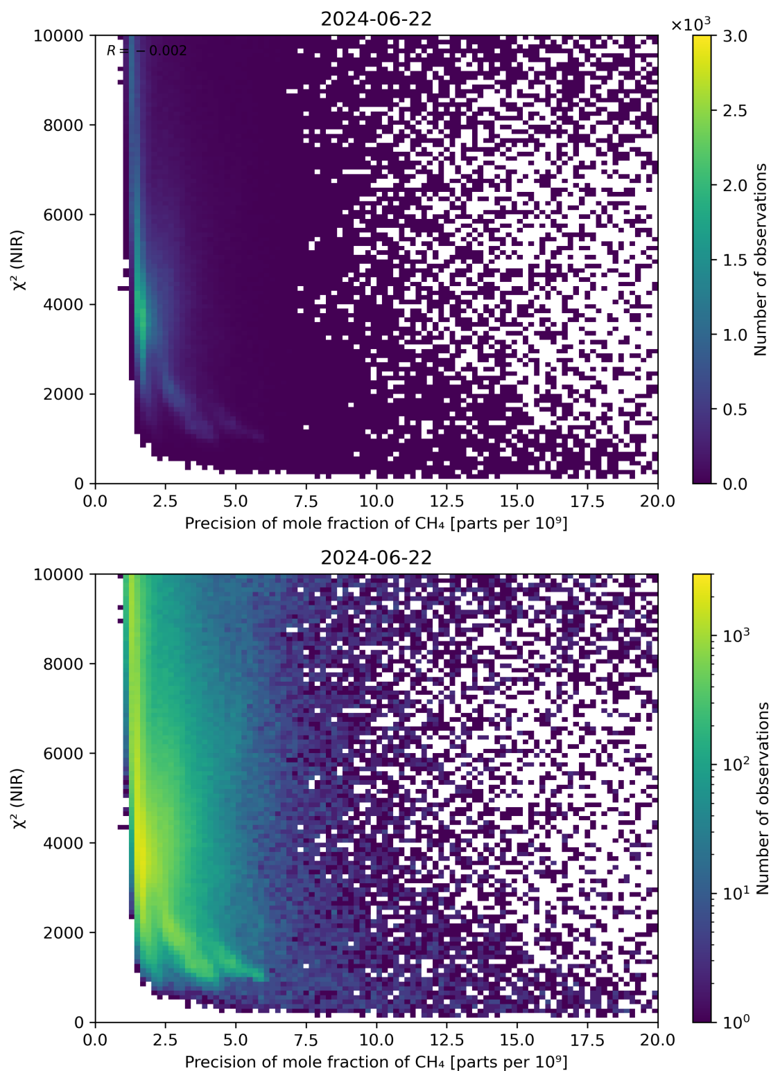
Figure 78: Scatter density plot of “Precision of mole fraction of CH 4 ” against “ \chi^2 (NIR)” for 2024-06-21 to 2024-06-23.
