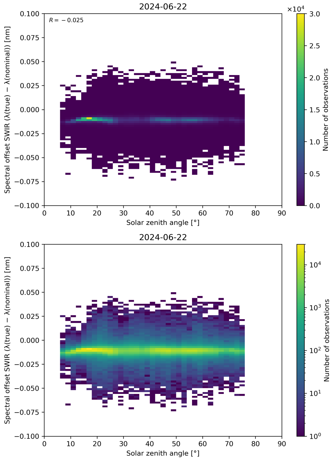
Figure 104: Scatter density plot of “Solar zenith angle” against “Spectral offset SWIR ( \lambda(\text{true}) - \lambda(\text{nominal}) )” for 2024-06-21 to 2024-06-23.
