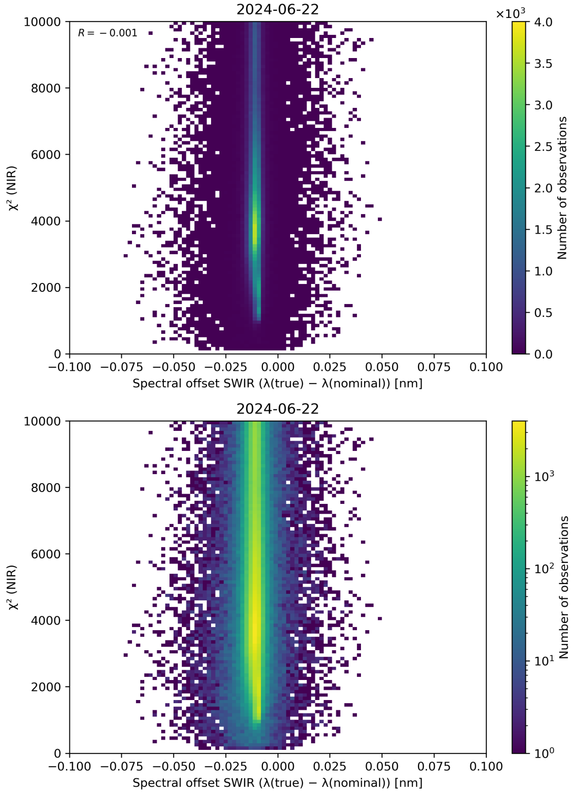
Figure 117: Scatter density plot of “Spectral offset SWIR ( \lambda(\text{true}) - \lambda(\text{nominal}) )” against “ \chi^2 (NIR)” for 2024-06-21 to 2024-06-23.
