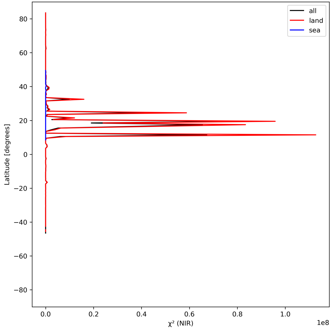
Figure 18: Zonal average of “ \chi^2 (NIR)” for 2024-06-21 to 2024-06-23.
