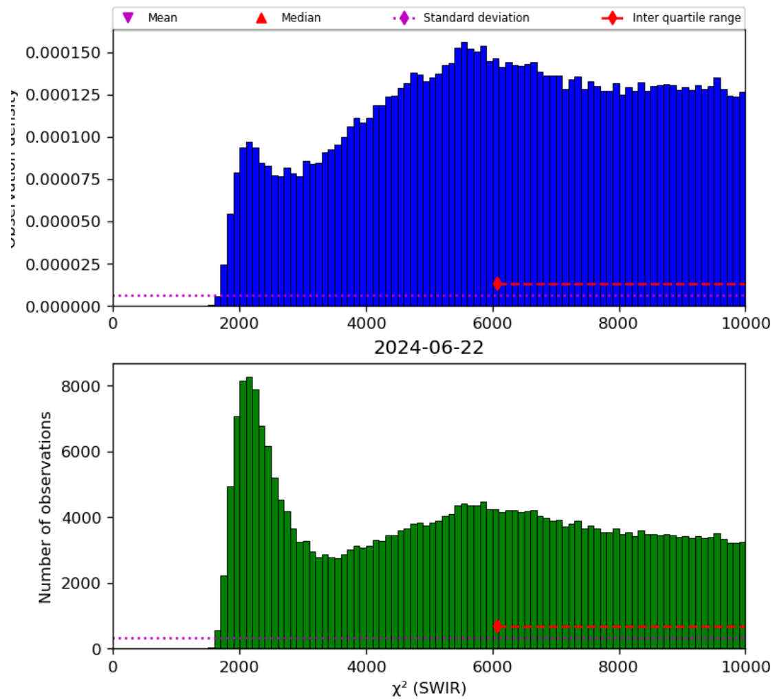
Figure 28: Histogram of “ \chi^2 (SWIR)” for 2024-06-21 to 2024-06-23
