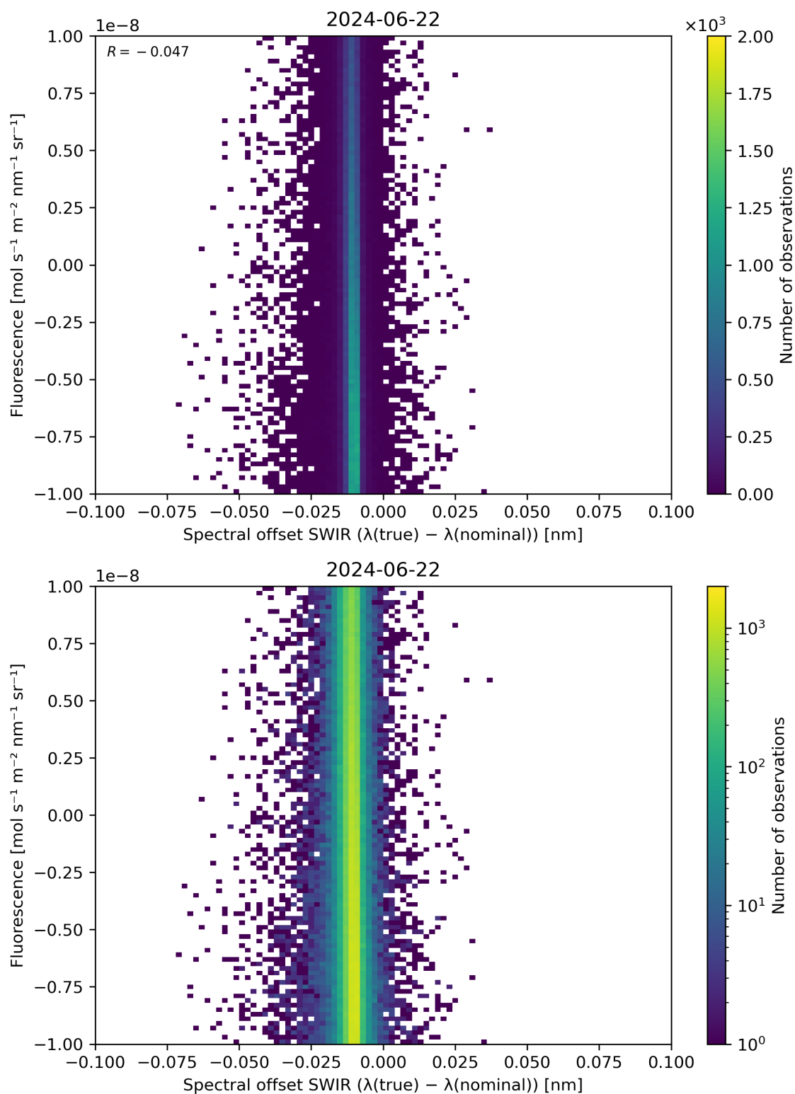
Figure 120: Scatter density plot of “Spectral offset SWIR ( \lambda(\text{true}) - \lambda(\text{nominal}) )” against “Fluorescence” for 2024-06-21 to 2024-06-23.
