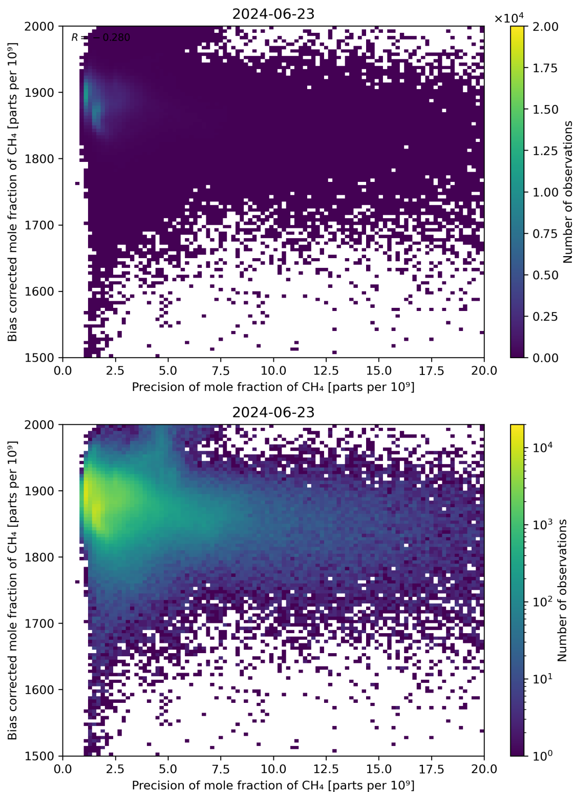
Figure 82: Scatter density plot of “Precision of mole fraction of CH 4 ” against “Bias corrected mole fraction of CH 4 ” for 2024-06-22 to 2024-06-24.
