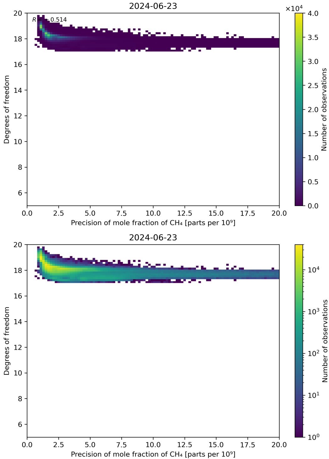
Figure 80: Scatter density plot of “Precision of mole fraction of CH 4 ” against “Degrees of freedom” for 2024-06-22 to 2024-06-24.
