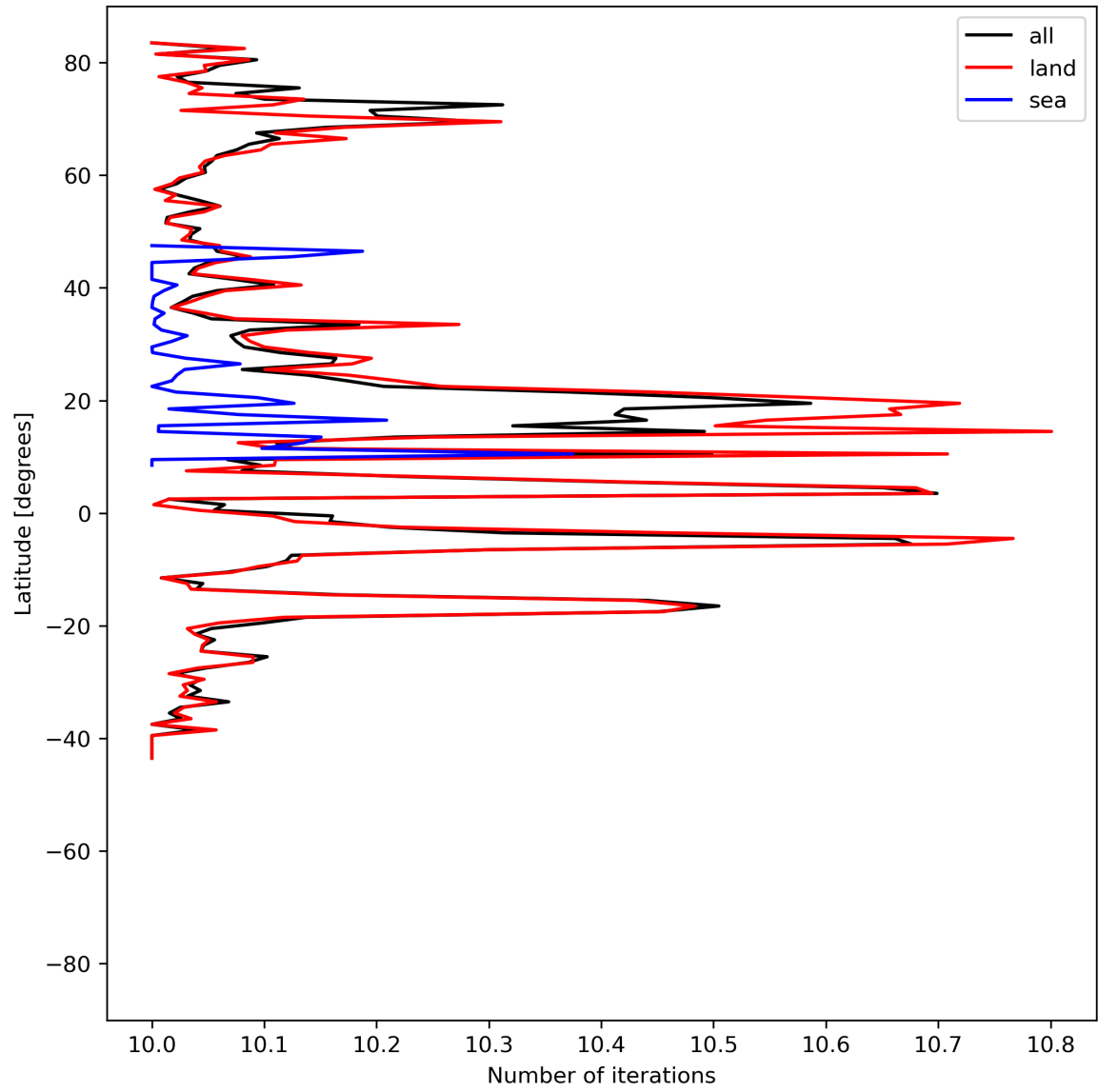
Figure 20: Zonal average of “Number of iterations” for 2024-06-22 to 2024-06-24.
