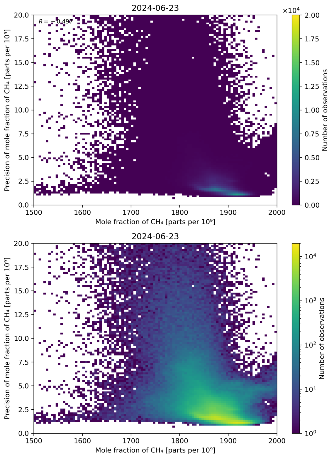
Figure 75: Scatter density plot of “Mole fraction of CH 4 ” against “Precision of mole fraction of CH 4 ” for 2024-06-22 to 2024-06-24.
