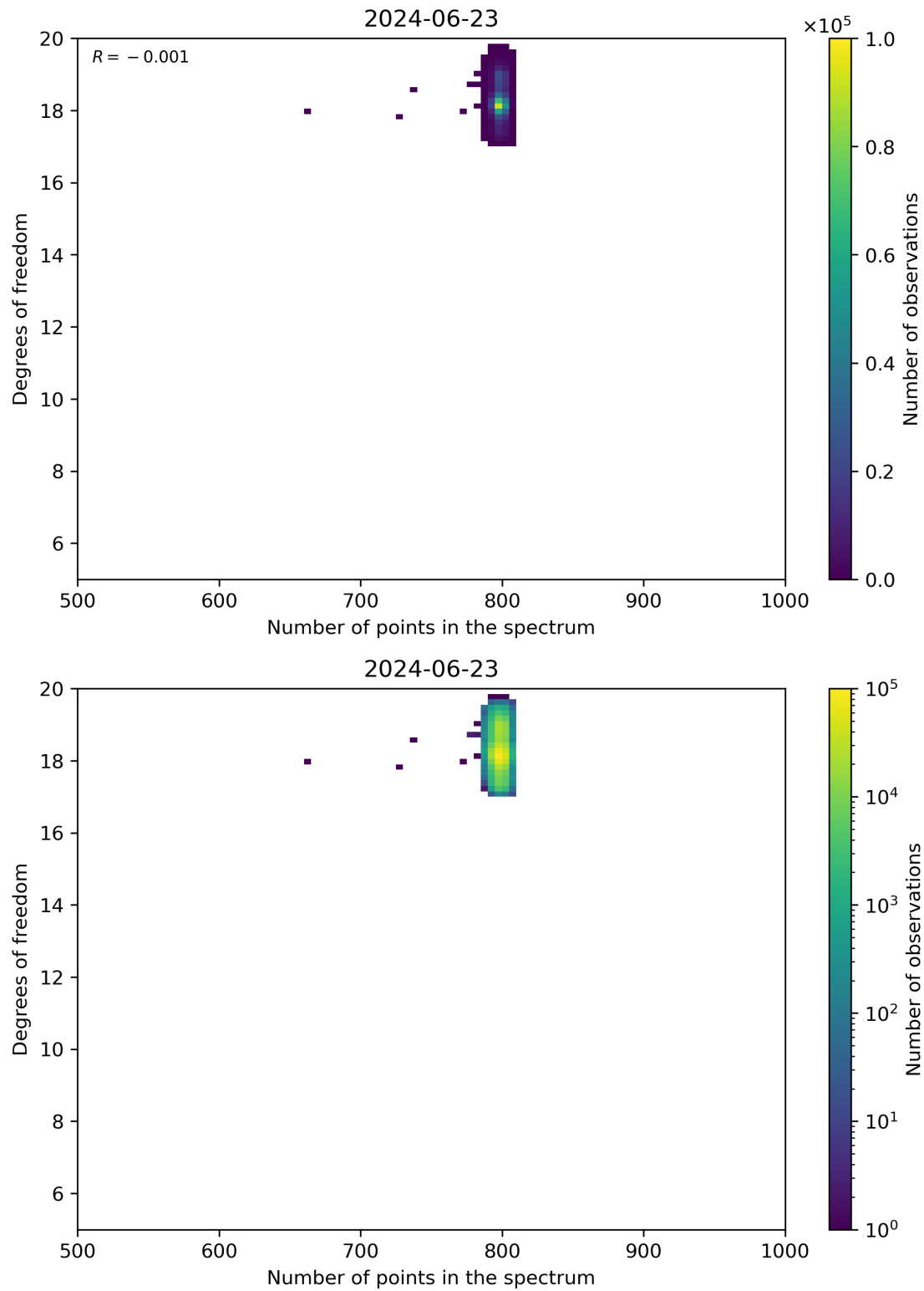
Figure 90: Scatter density plot of “Number of points in the spectrum” against “Degrees of freedom” for 2024-06-22 to 2024-06-24.
