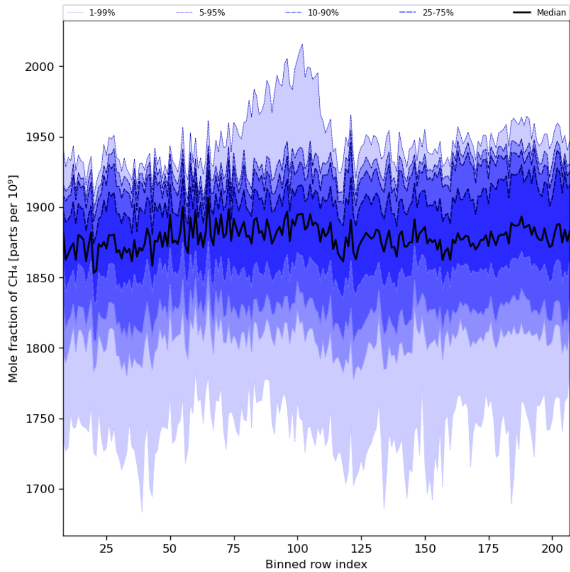
Figure 34: Along track statistics of “Mole fraction of CH 4 ” for 2024-06-22 to 2024-06-24
