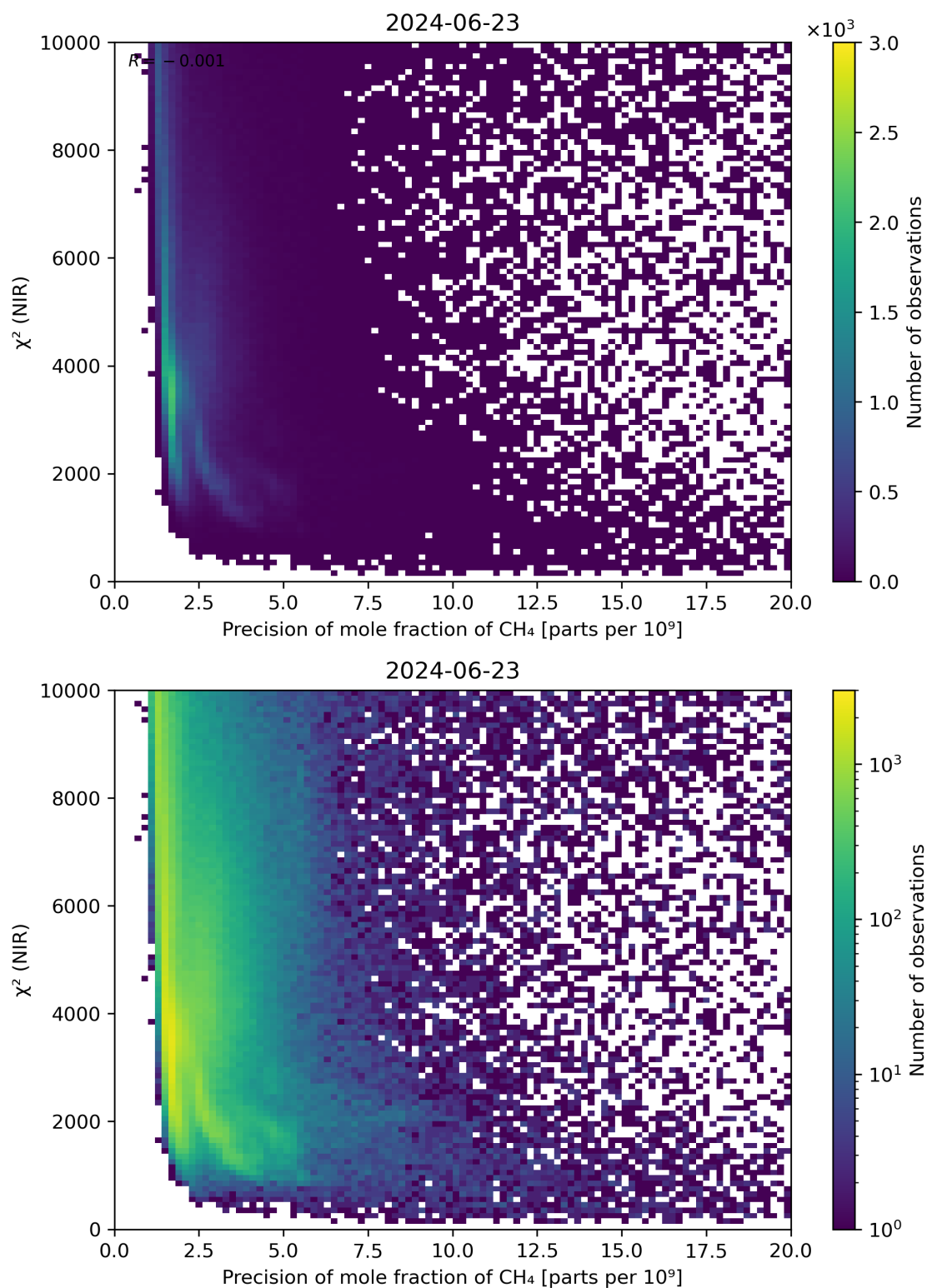
Figure 78: Scatter density plot of “Precision of mole fraction of CH 4 ” against “ \chi^2 (NIR)” for 2024-06-22 to 2024-06-24.
