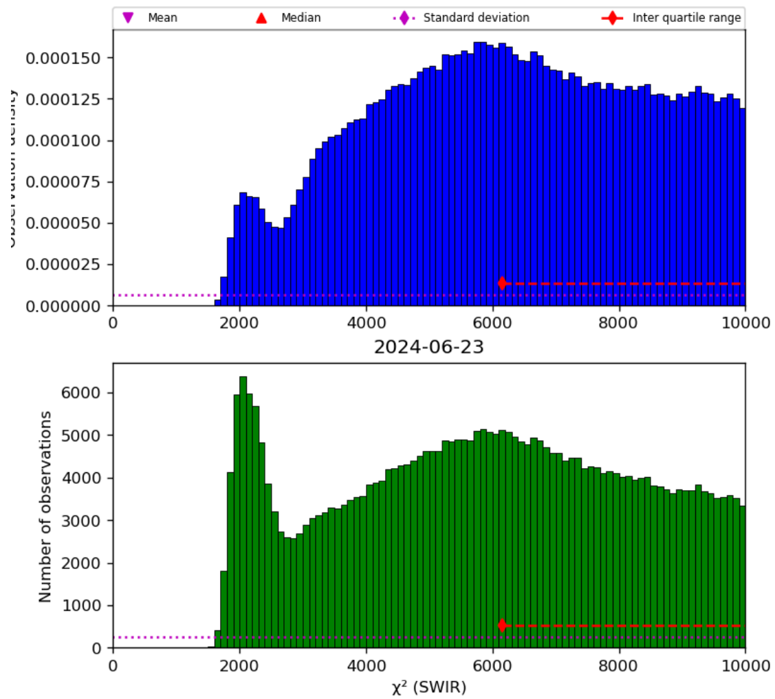
Figure 28: Histogram of “ \chi^2 (SWIR)” for 2024-06-22 to 2024-06-24
