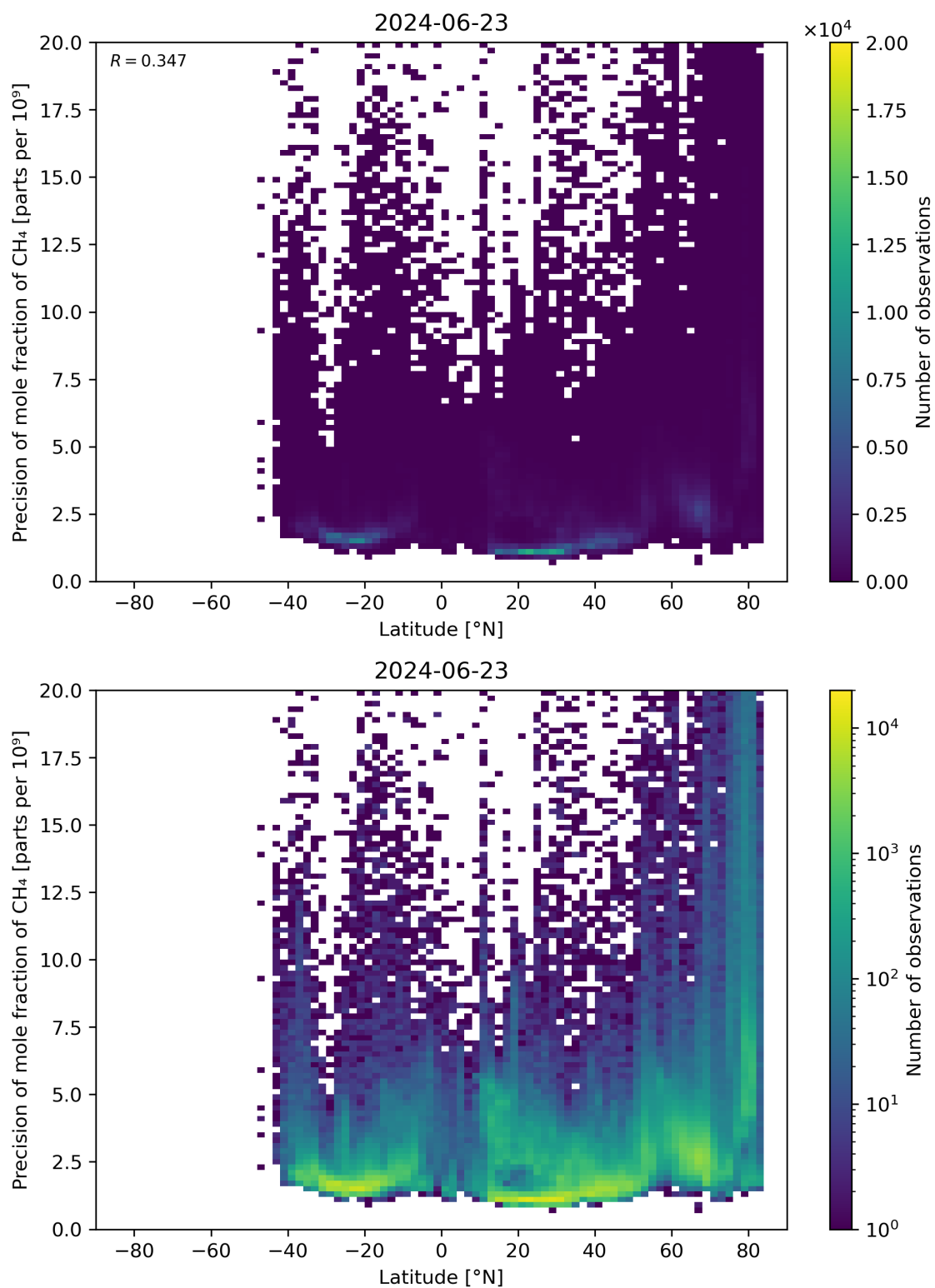
Figure 59: Scatter density plot of “Latitude” against “Precision of mole fraction of \text{CH}_4 ” for 2024-06-22 to 2024-06-24.
