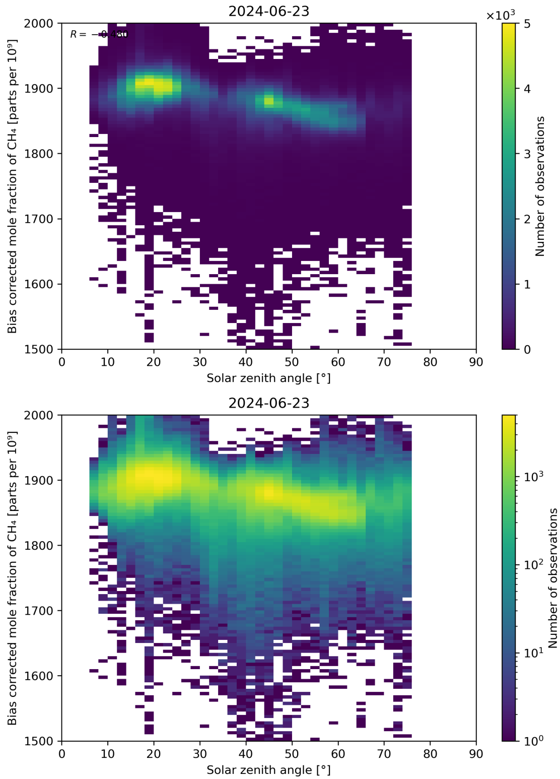
Figure 100: Scatter density plot of “Solar zenith angle” against “Bias corrected mole fraction of \text{CH}_4 ” for 2024-06-22 to 2024-06-24.
