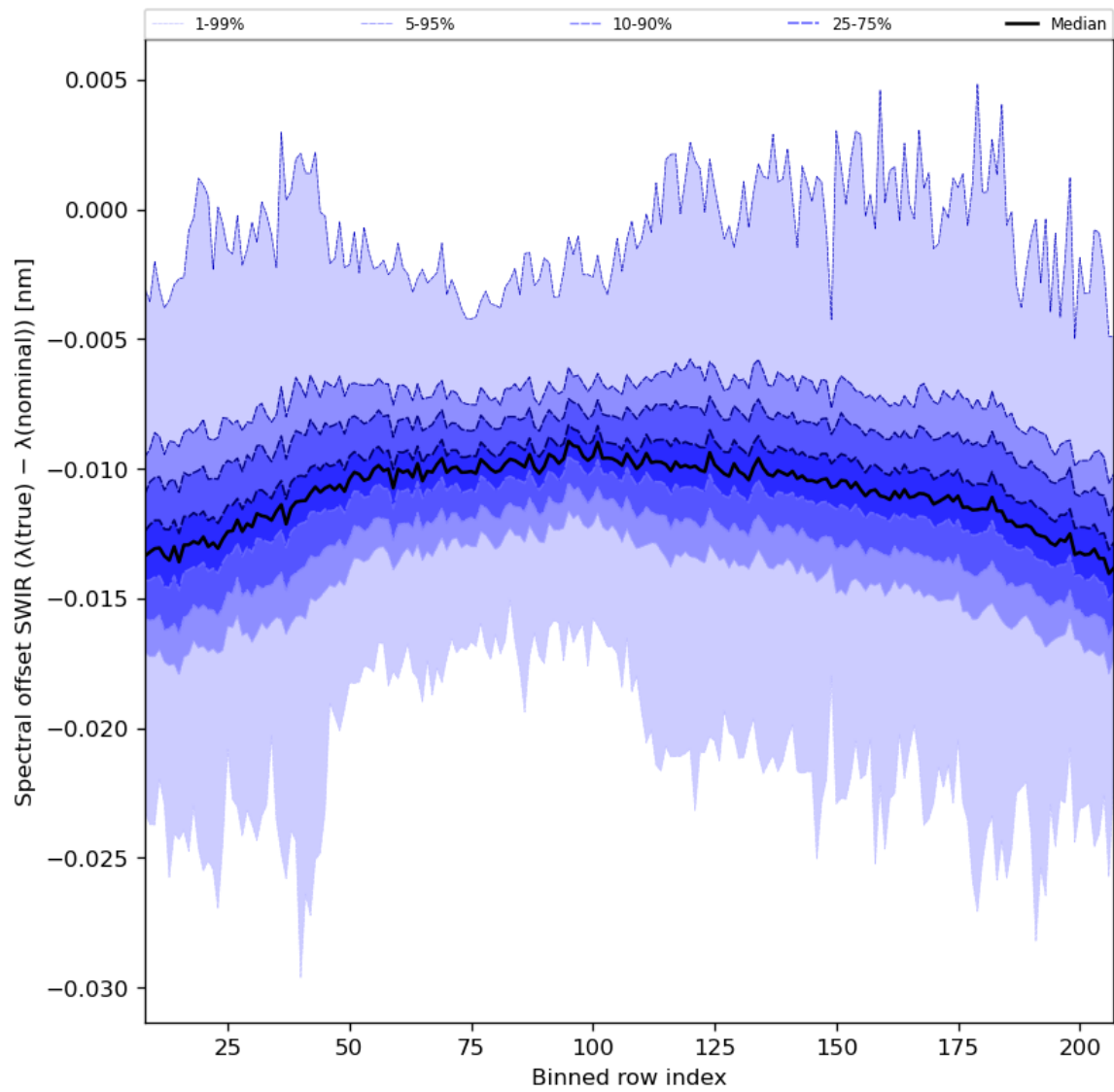
Figure 38: Along track statistics of “Spectral offset SWIR ( \lambda(\text{true}) - \lambda(\text{nominal}) )” for 2024-06-22 to 2024-06-24
