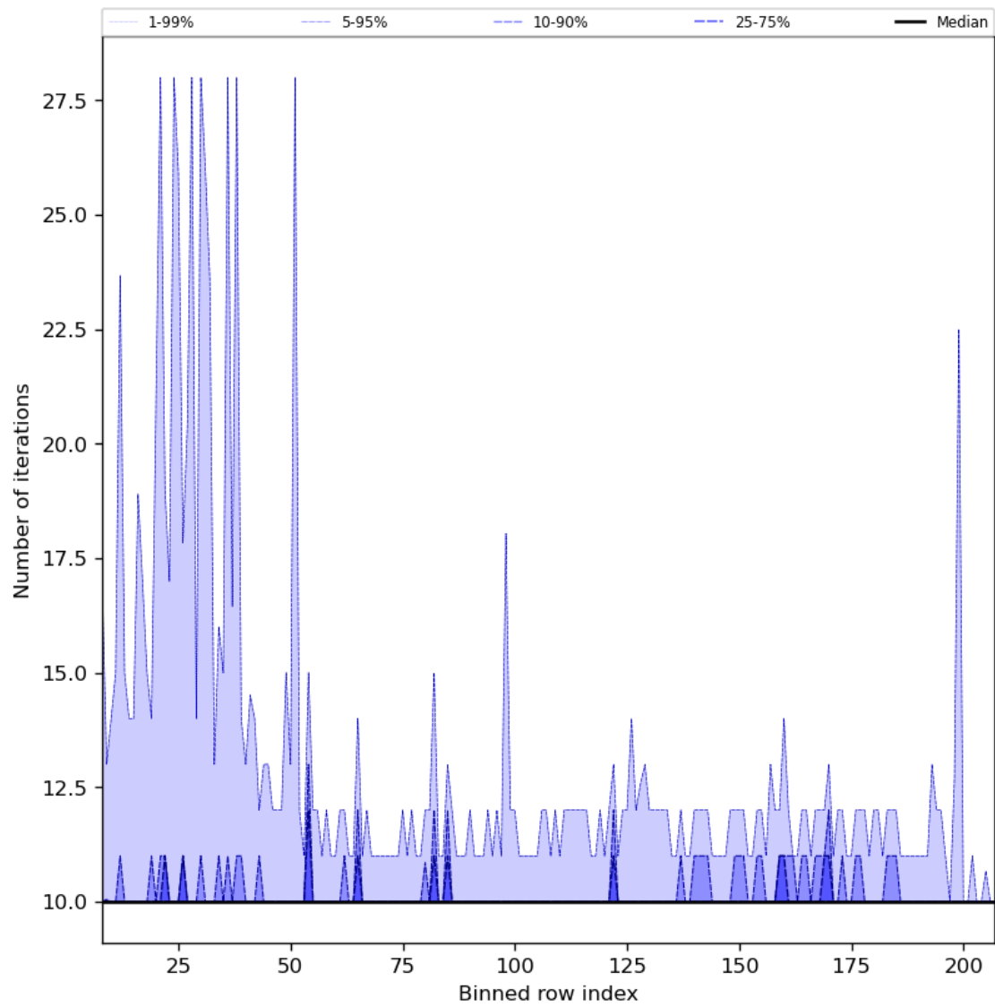
Figure 42: Along track statistics of “Number of iterations” for 2024-06-22 to 2024-06-24
