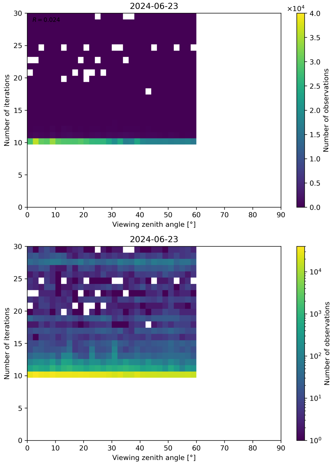
Figure 113: Scatter density plot of “Viewing zenith angle” against “Number of iterations” for 2024-06-22 to 2024-06-24.
