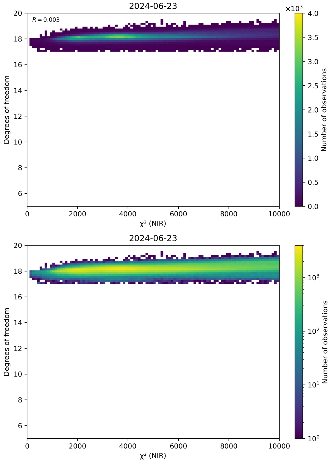
Figure 44: Scatter density plot of “ \chi^2 (NIR)” against “Degrees of freedom” for 2024-06-22 to 2024-06-24.
