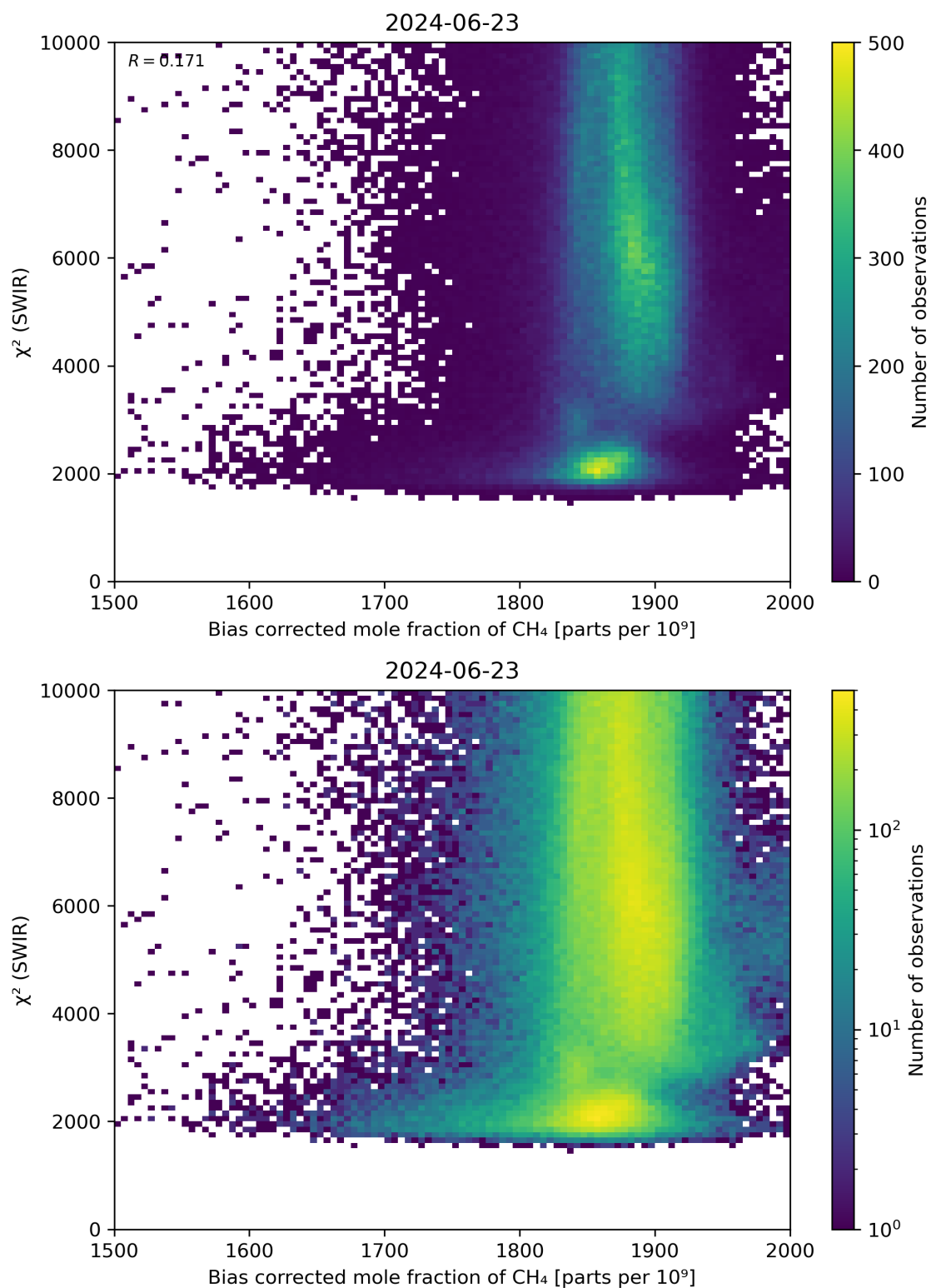
Figure 64: Scatter density plot of “Bias corrected mole fraction of CH 4 ” against “ \chi^2 (SWIR)” for 2024-06-22 to 2024-06-24.
