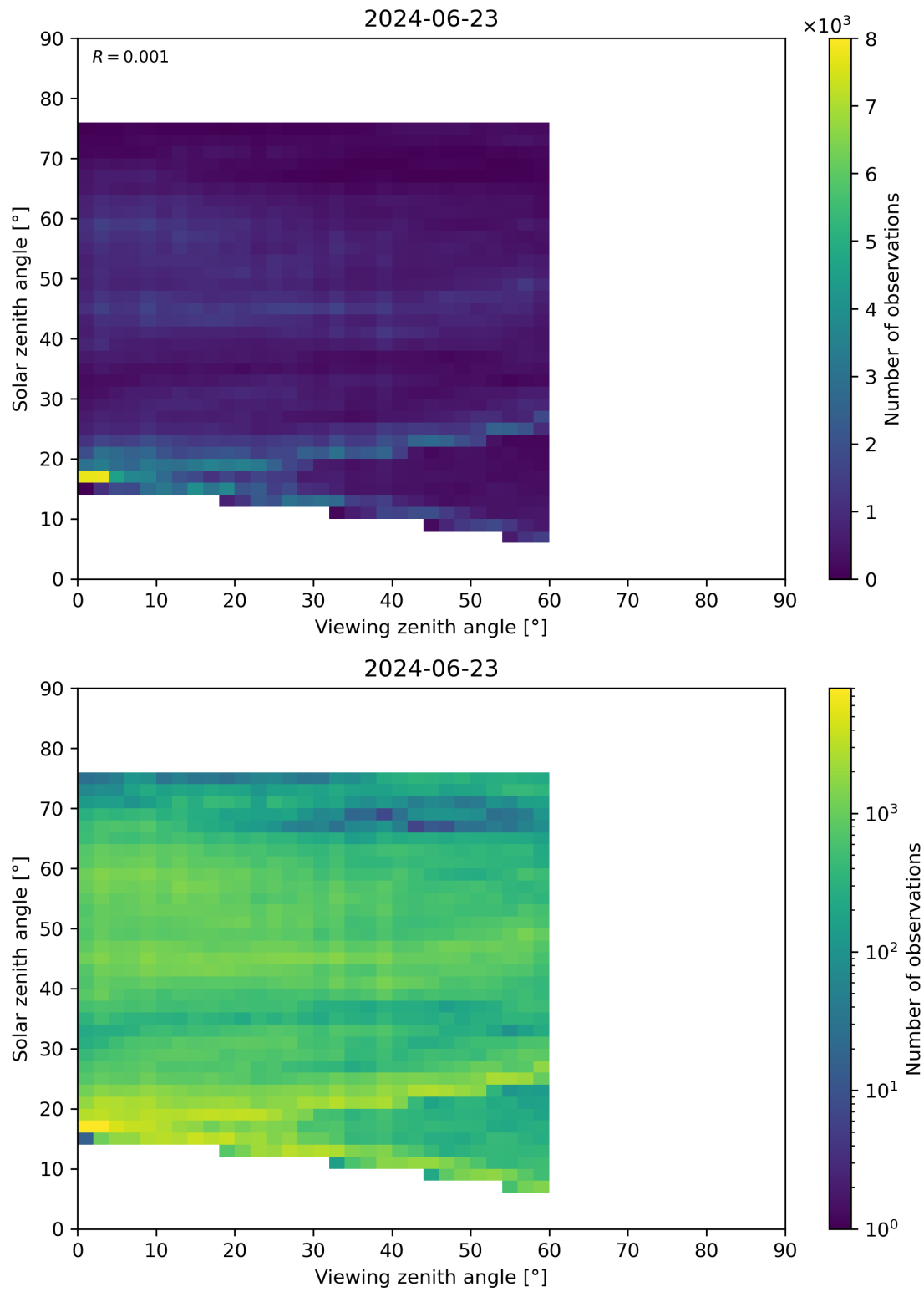
Figure 115: Scatter density plot of “Viewing zenith angle” against “Solar zenith angle” for 2024-06-22 to 2024-06-24.
