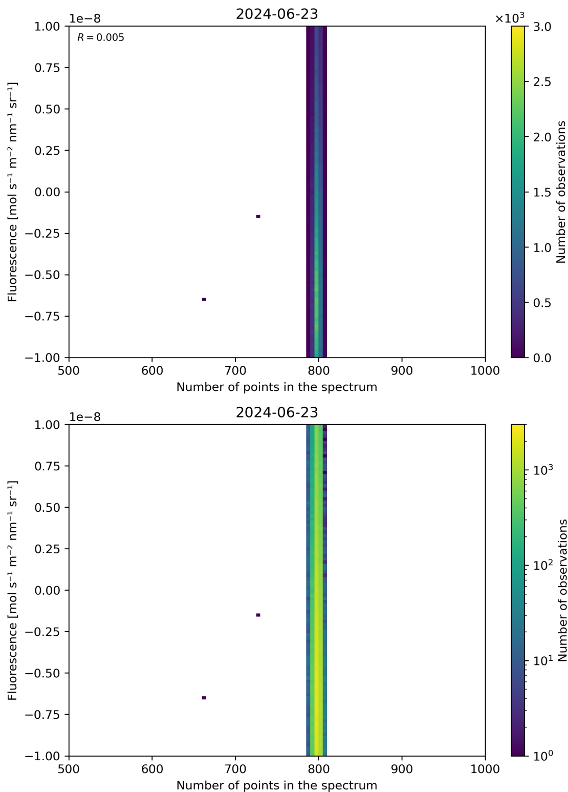
Figure 91: Scatter density plot of “Number of points in the spectrum” against “Fluorescence” for 2024-06-22 to 2024-06-24.
