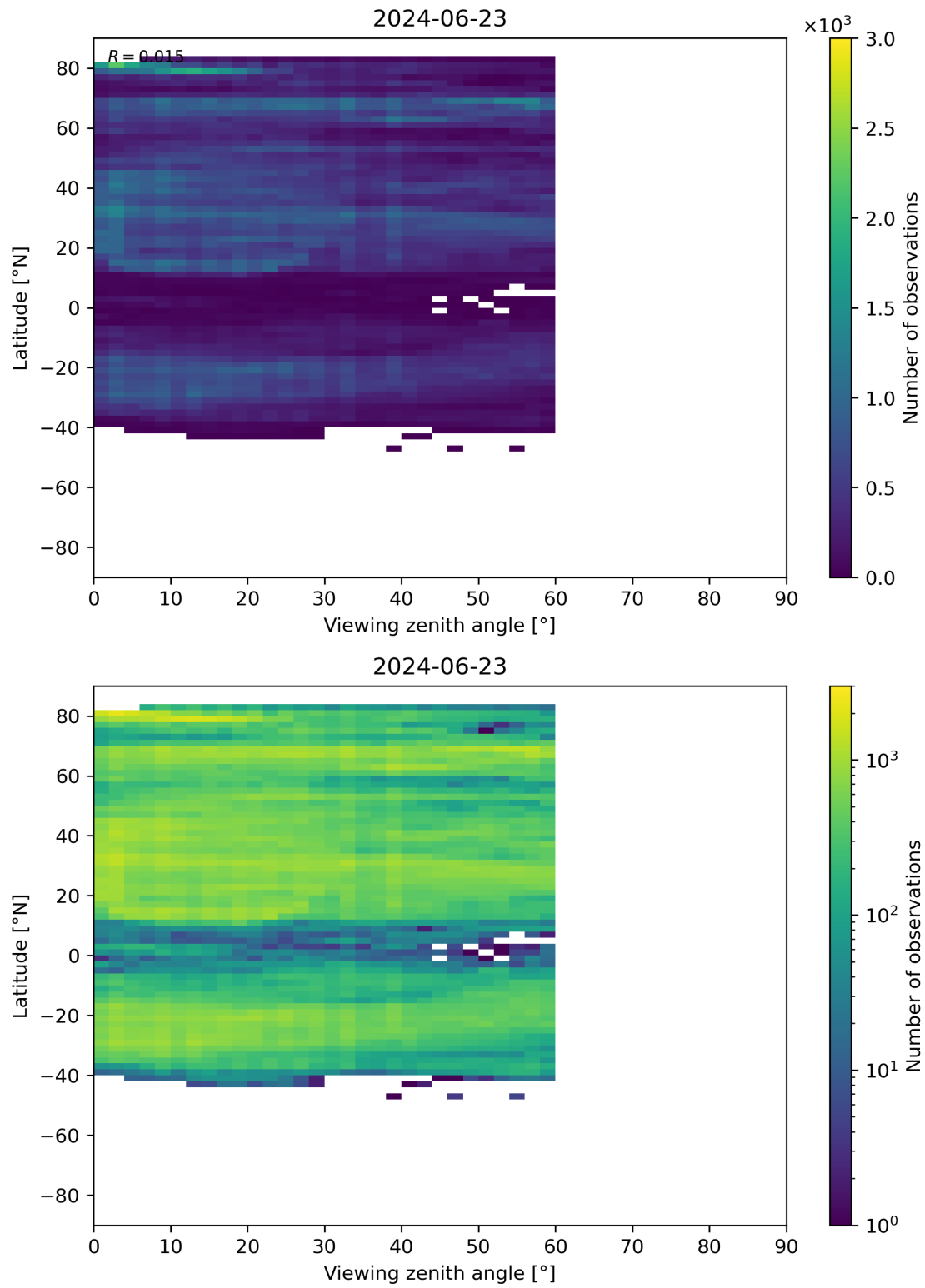
Figure 109: Scatter density plot of “Viewing zenith angle” against “Latitude” for 2024-06-22 to 2024-06-24.
