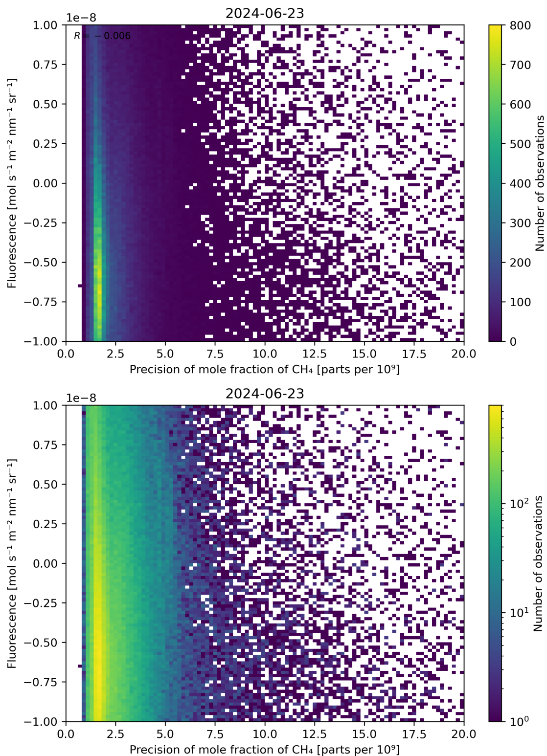
Figure 81: Scatter density plot of “Precision of mole fraction of \text{CH}_4 ” against “Fluorescence” for 2024-06-22 to 2024-06-24.
