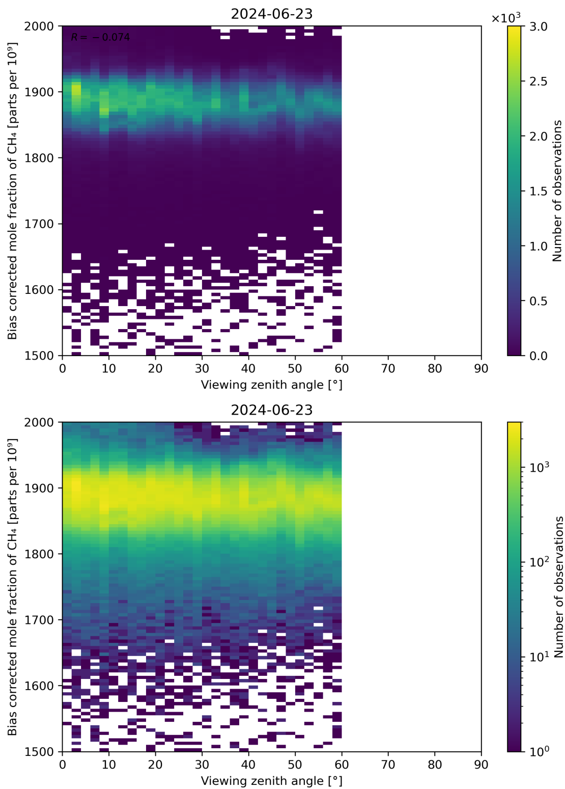
Figure 111: Scatter density plot of “Viewing zenith angle” against “Bias corrected mole fraction of CH 4 ” for 2024-06-22 to 2024-06-24.
