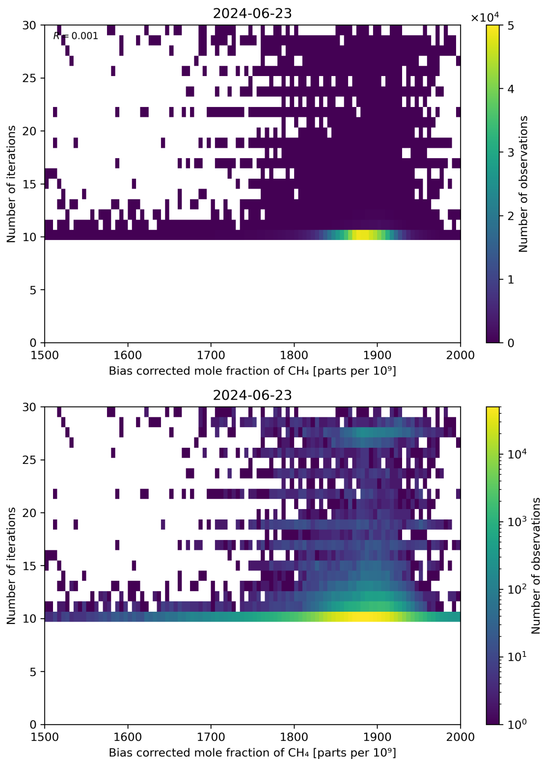
Figure 67: Scatter density plot of “Bias corrected mole fraction of \text{CH}_4 ” against “Number of iterations” for 2024-06-22 to 2024-06-24.
