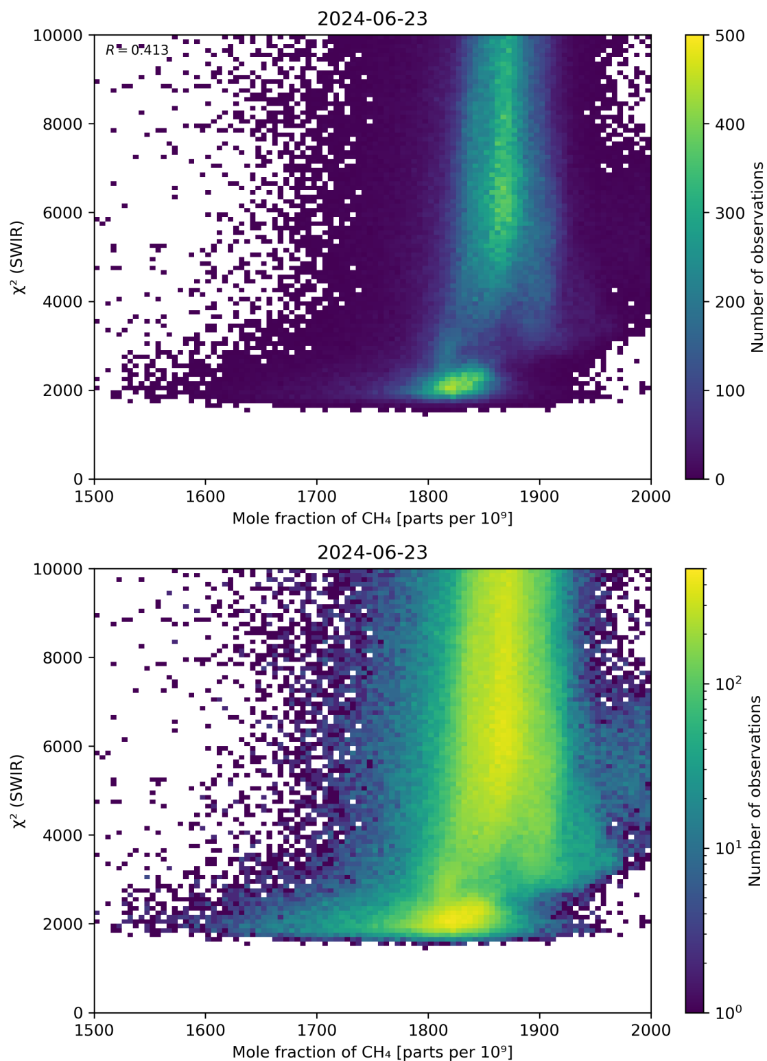
Figure 71: Scatter density plot of “Mole fraction of \text{CH}_4 ” against “ \chi^2 (SWIR)” for 2024-06-22 to 2024-06-24.
