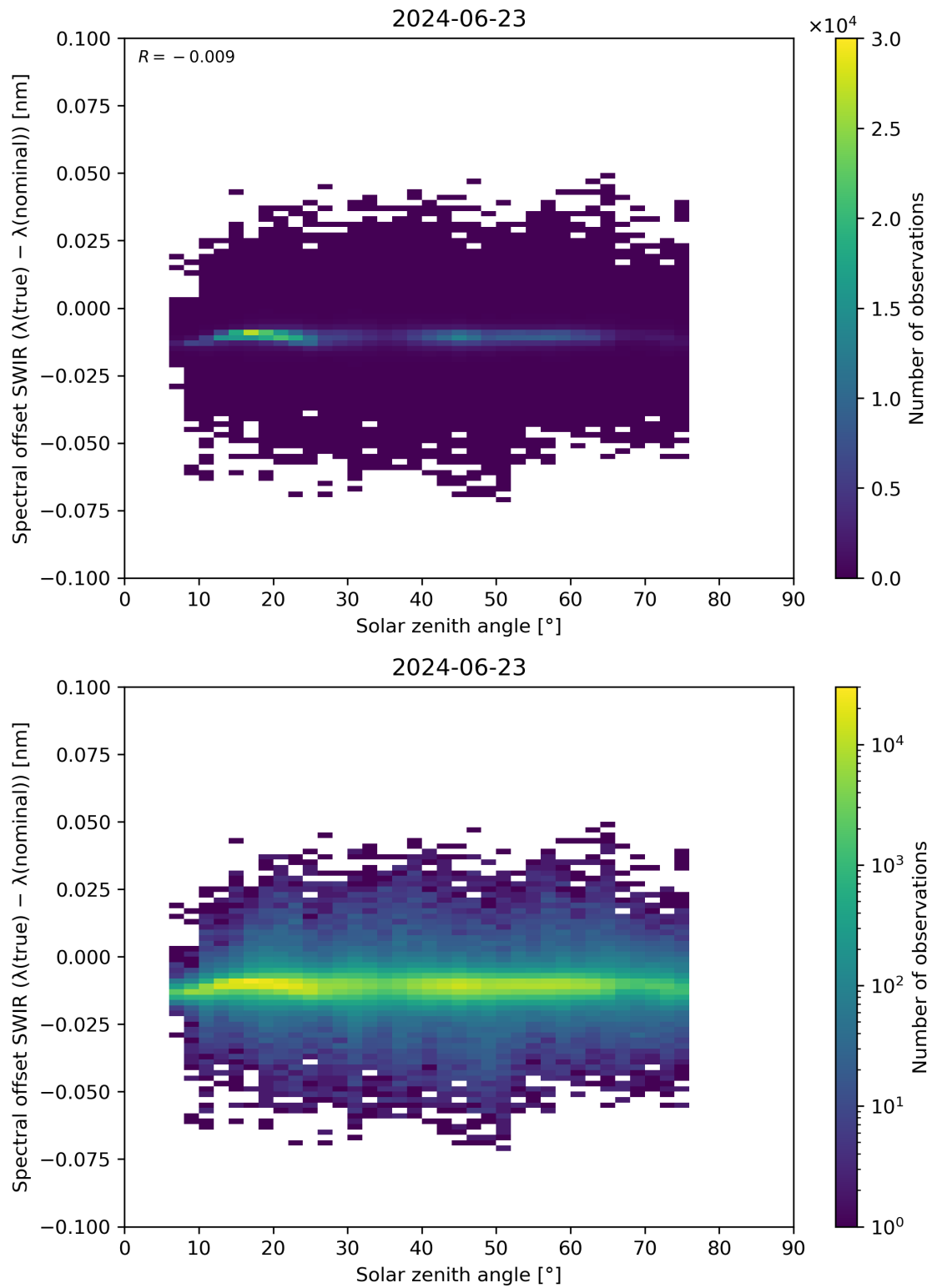
Figure 104: Scatter density plot of “Solar zenith angle” against “Spectral offset SWIR ( \lambda(\text{true}) - \lambda(\text{nominal}) )” for 2024-06-22 to 2024-06-24.
