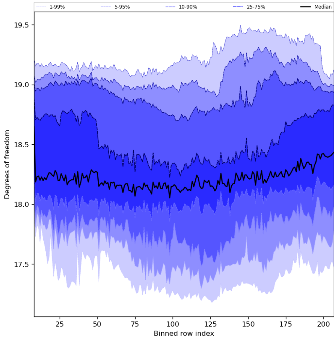
Figure 41: Along track statistics of “Degrees of freedom” for 2024-06-22 to 2024-06-24
