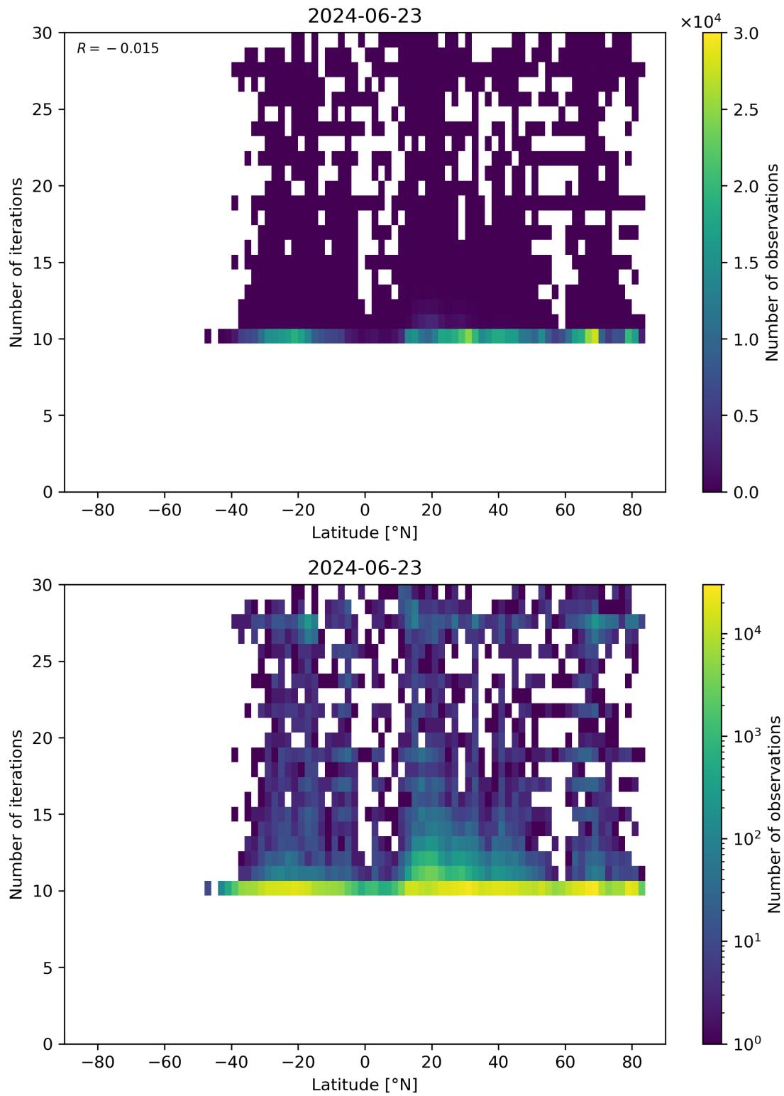
Figure 60: Scatter density plot of “Latitude” against “Number of iterations” for 2024-06-22 to 2024-06-24.
