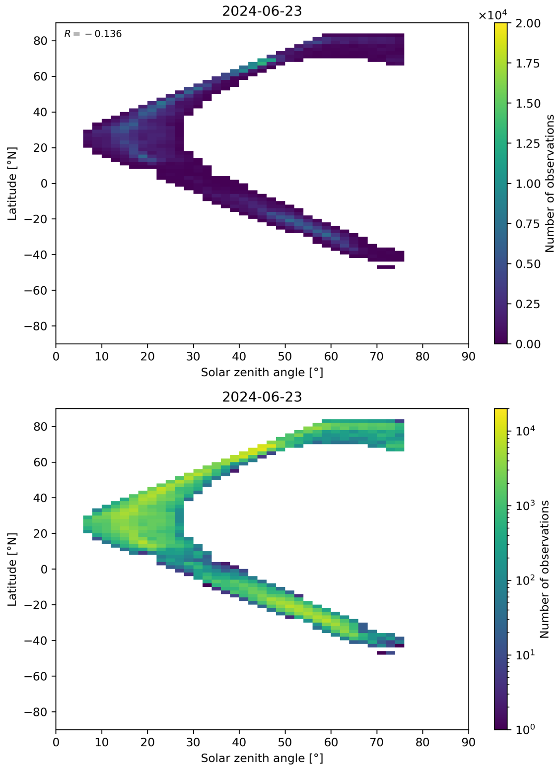
Figure 98: Scatter density plot of “Solar zenith angle” against “Latitude” for 2024-06-22 to 2024-06-24.
