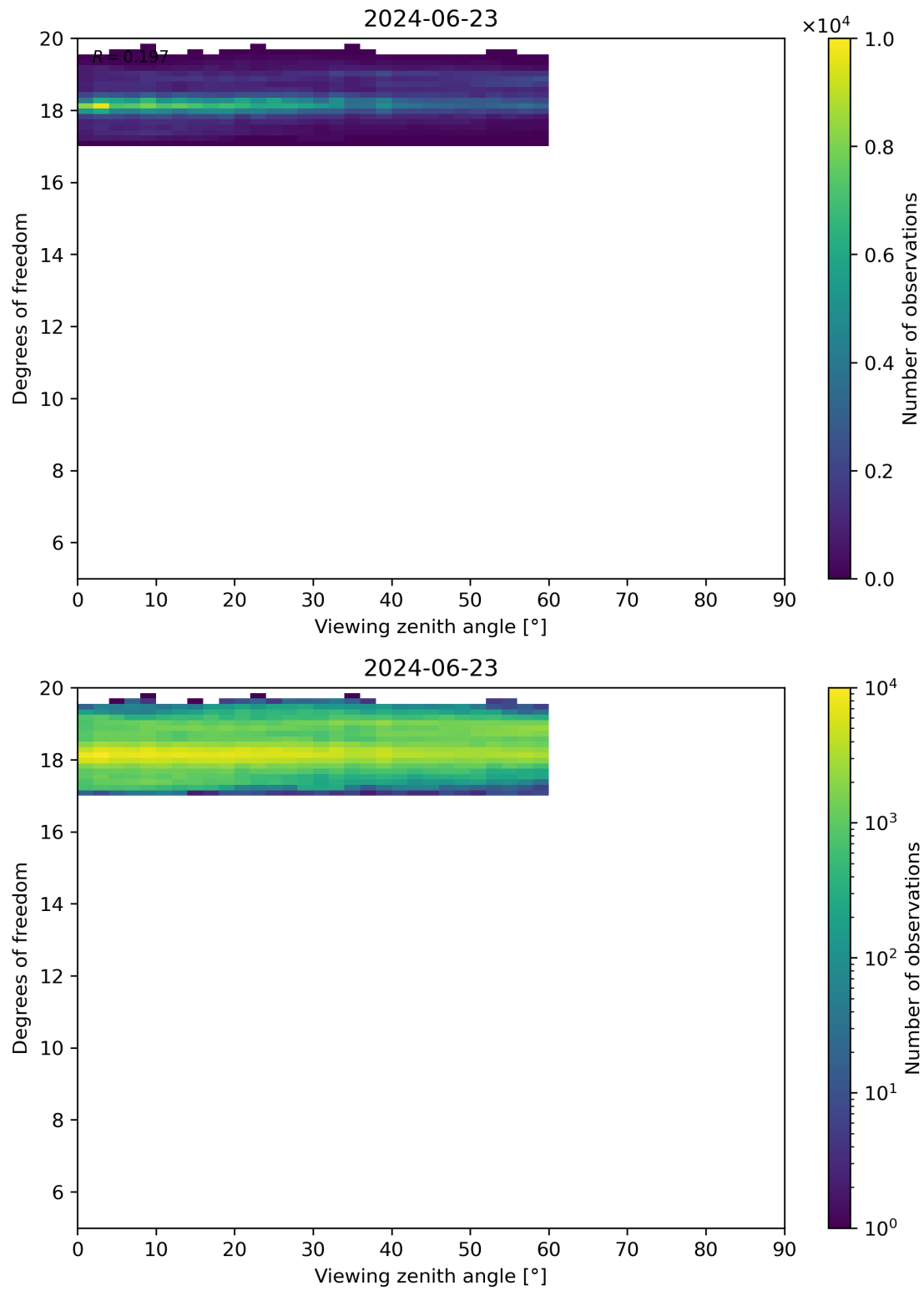
Figure 107: Scatter density plot of “Viewing zenith angle” against “Degrees of freedom” for 2024-06-22 to 2024-06-24.
