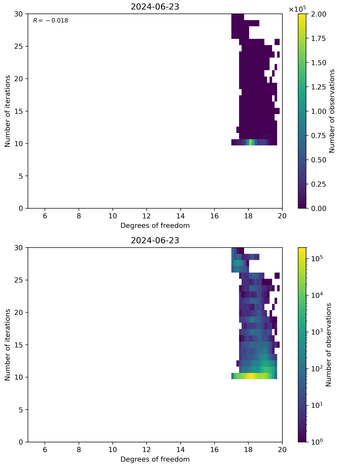
Figure 52: Scatter density plot of “Degrees of freedom” against “Number of iterations” for 2024-06-22 to 2024-06-24.
