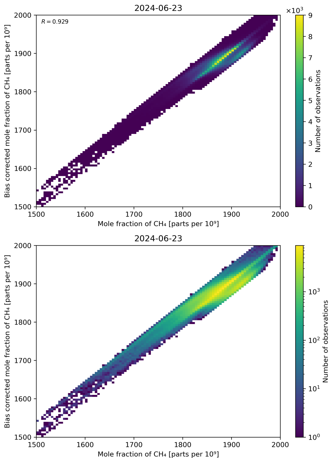
Figure 74: Scatter density plot of “Mole fraction of CH 4 ” against “Bias corrected mole fraction of CH 4 ” for 2024-06-22 to 2024-06-24.
