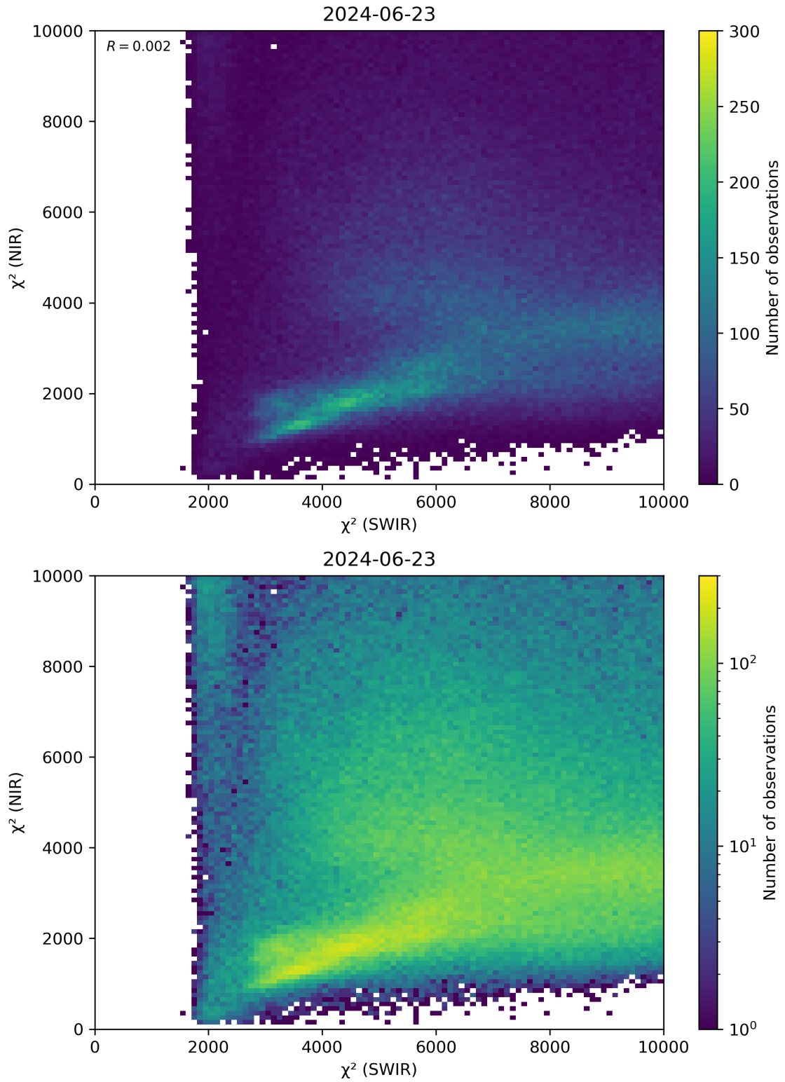
Figure 47: Scatter density plot of “ \chi^2 (SWIR)” against “ \chi^2 (NIR)” for 2024-06-22 to 2024-06-24.
