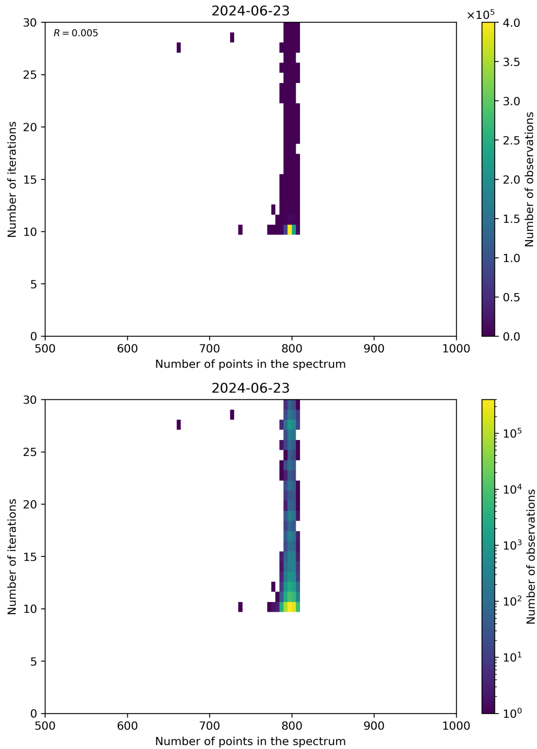
Figure 92: Scatter density plot of “Number of points in the spectrum” against “Number of iterations” for 2024-06-22 to 2024-06-24.
