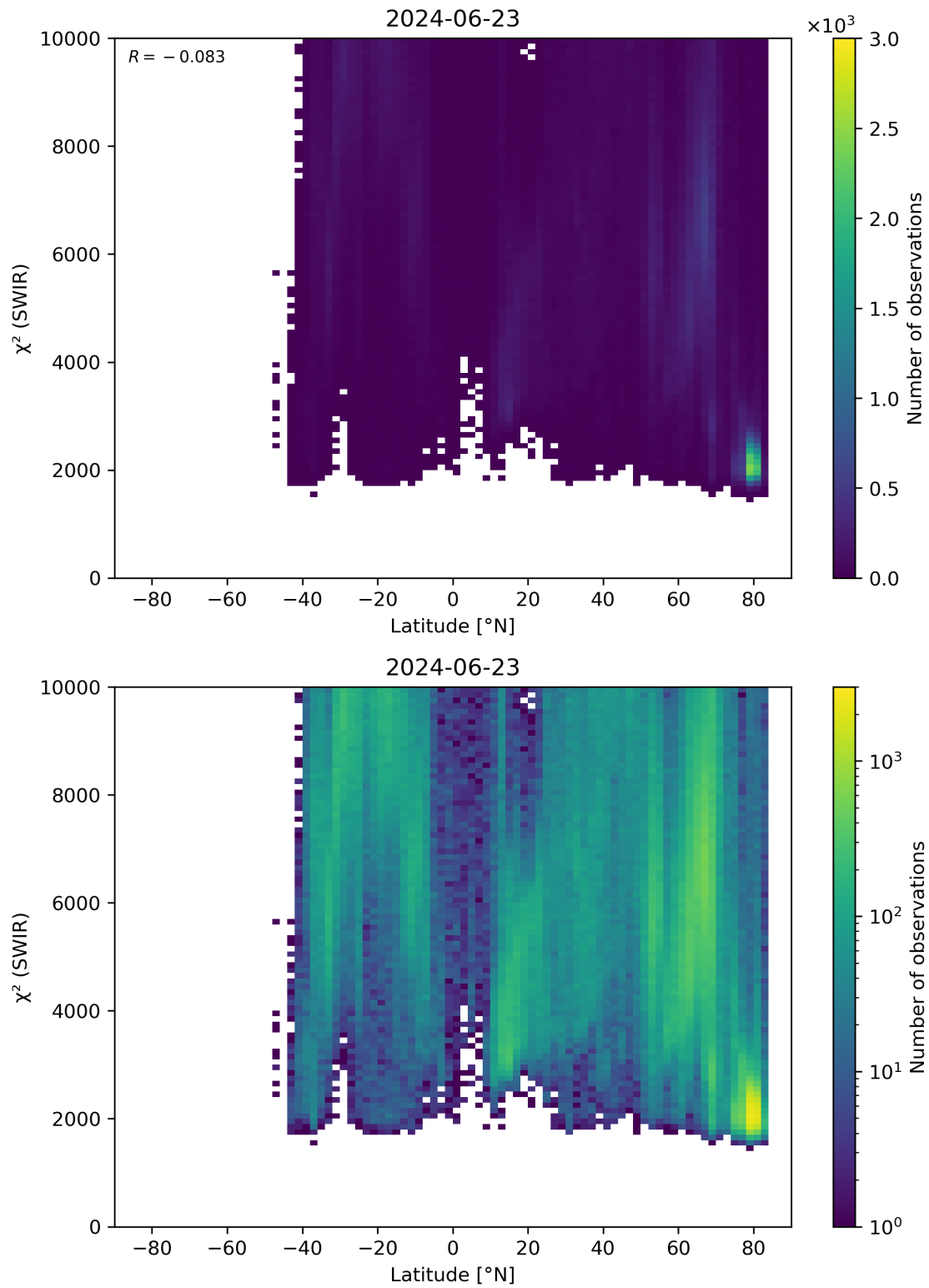
Figure 54: Scatter density plot of “Latitude” against “ \chi^2 (SWIR)” for 2024-06-22 to 2024-06-24.
