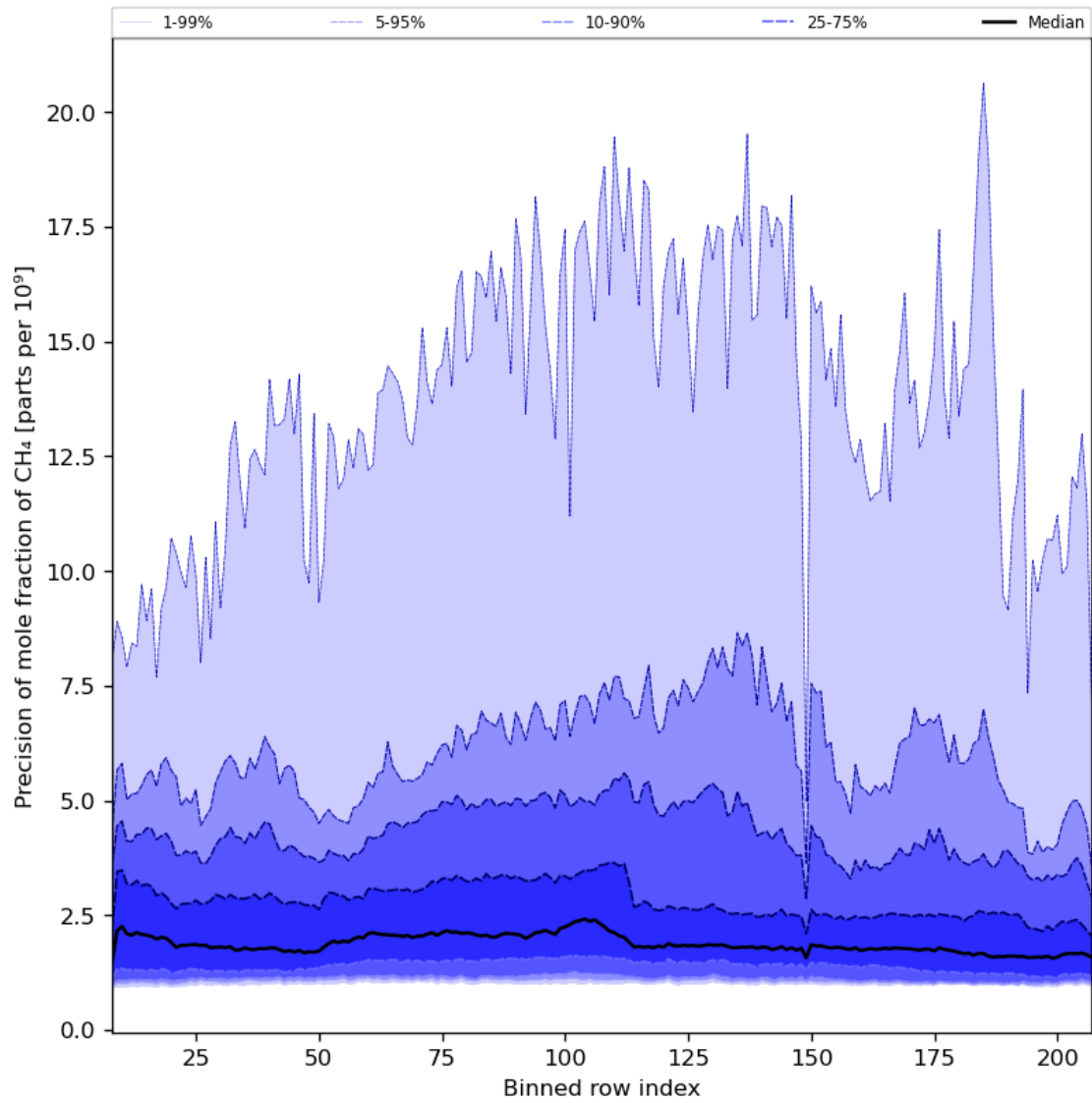
Figure 35: Along track statistics of “Precision of mole fraction of CH 4 ” for 2024-06-22 to 2024-06-24
