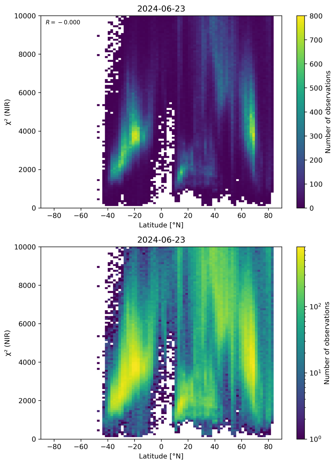
Figure 53: Scatter density plot of “Latitude” against “ \chi^2 (NIR)” for 2024-06-22 to 2024-06-24.
