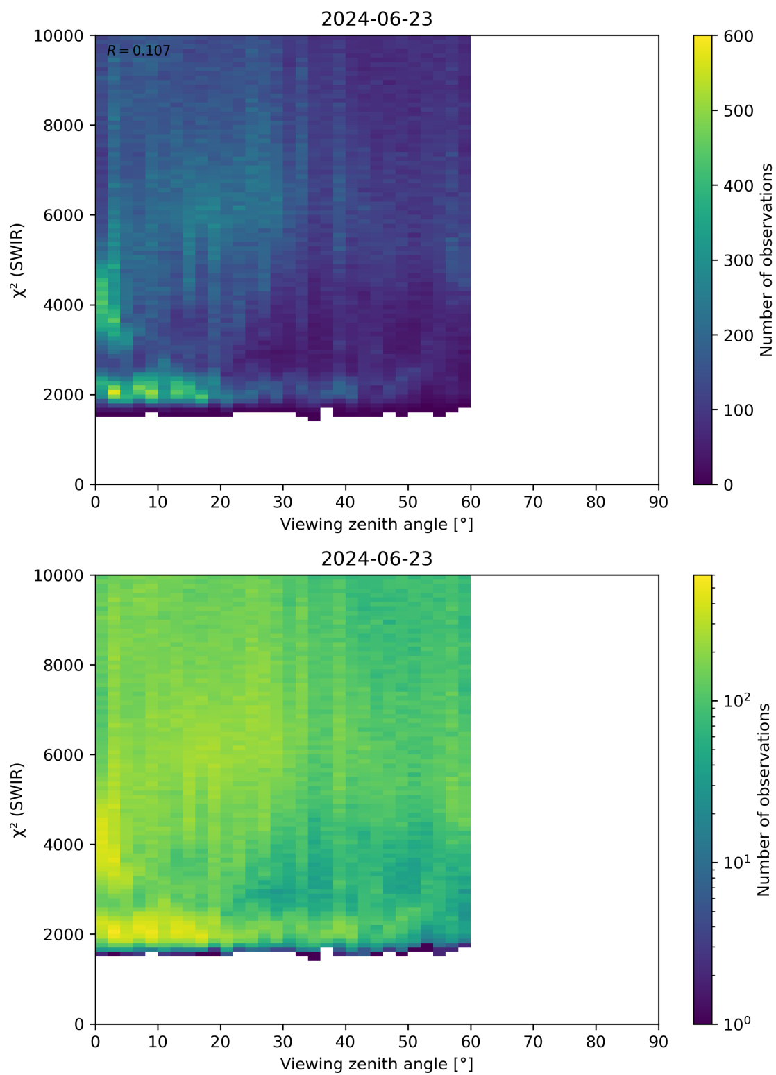
Figure 106: Scatter density plot of “Viewing zenith angle” against “ \chi^2 (SWIR)” for 2024-06-22 to 2024-06-24.
