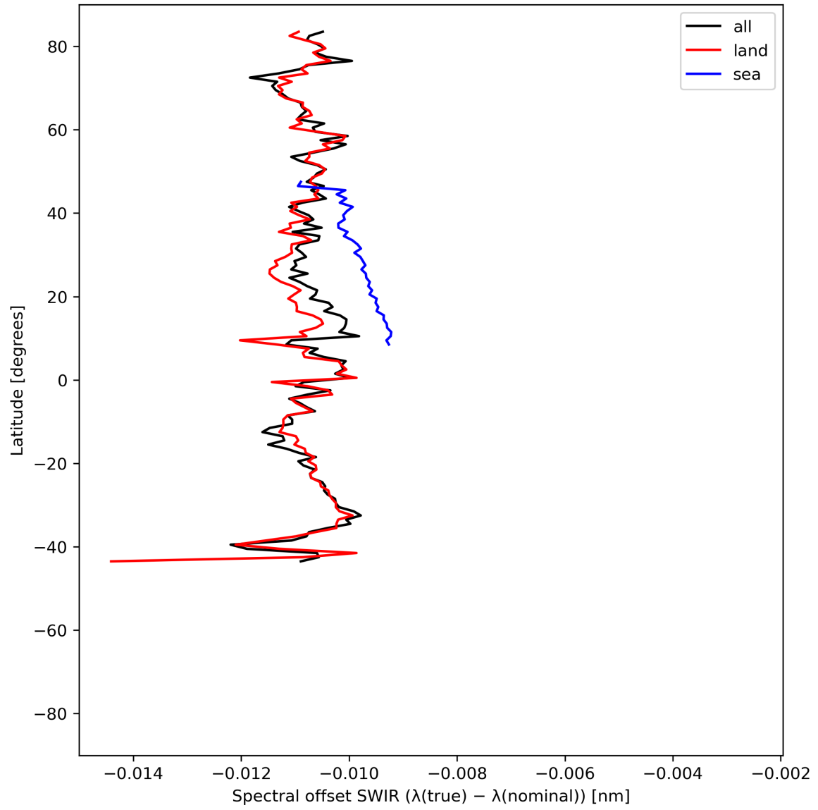
Figure 16: Zonal average of “Spectral offset SWIR ( \lambda(\text{true}) - \lambda(\text{nominal}) )” for 2024-06-22 to 2024-06-24.
