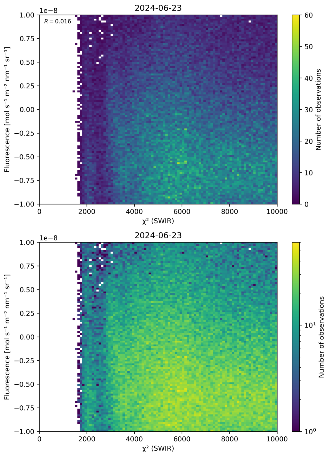
Figure 49: Scatter density plot of “ \chi^2 (SWIR)” against “Fluorescence” for 2024-06-22 to 2024-06-24.
