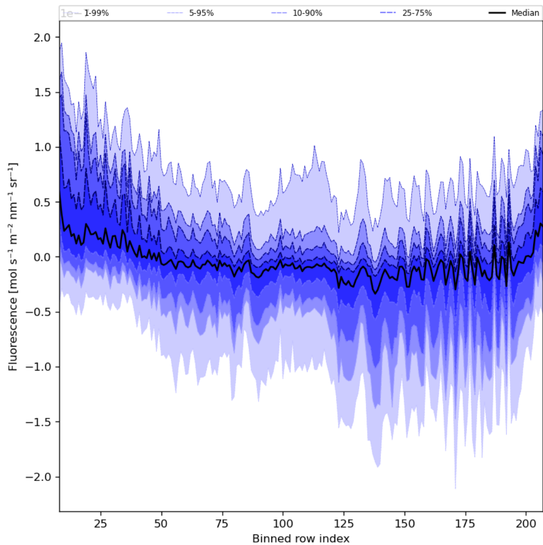
Figure 43: Along track statistics of “Fluorescence” for 2024-06-22 to 2024-06-24
