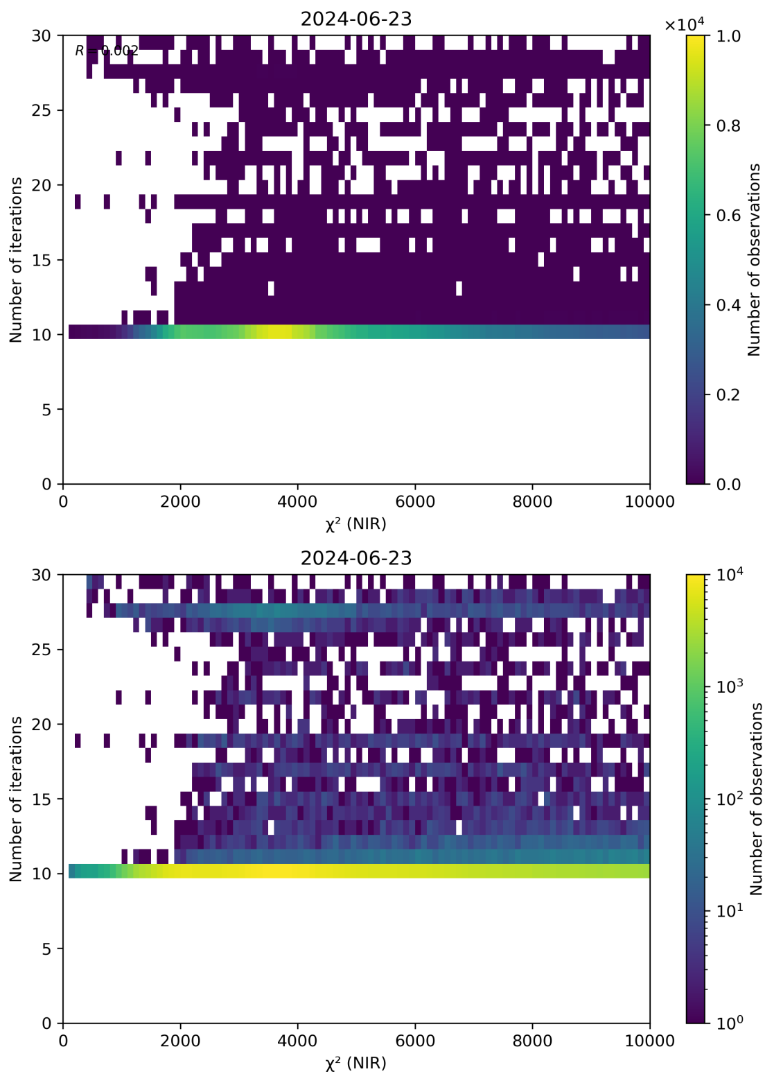
Figure 46: Scatter density plot of “ \chi^2 (NIR)” against “Number of iterations” for 2024-06-22 to 2024-06-24.
