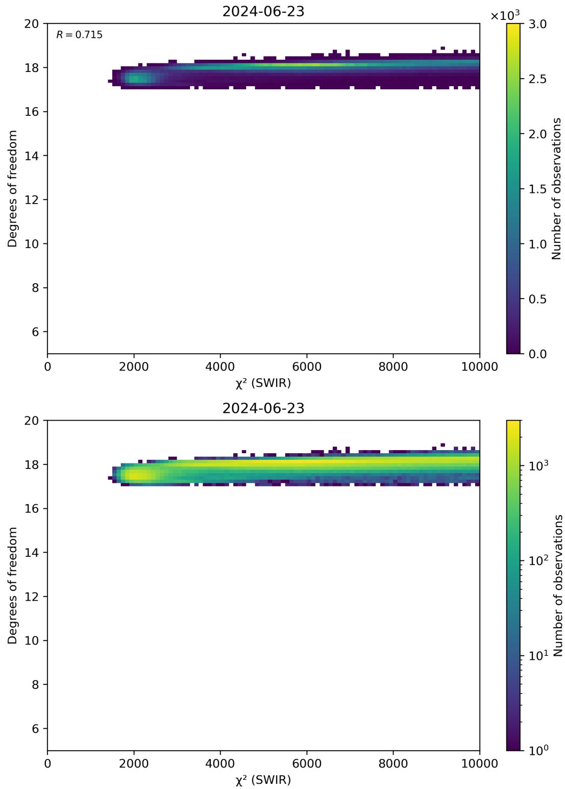
Figure 48: Scatter density plot of “ \chi^2 (SWIR)” against “Degrees of freedom” for 2024-06-22 to 2024-06-24.
