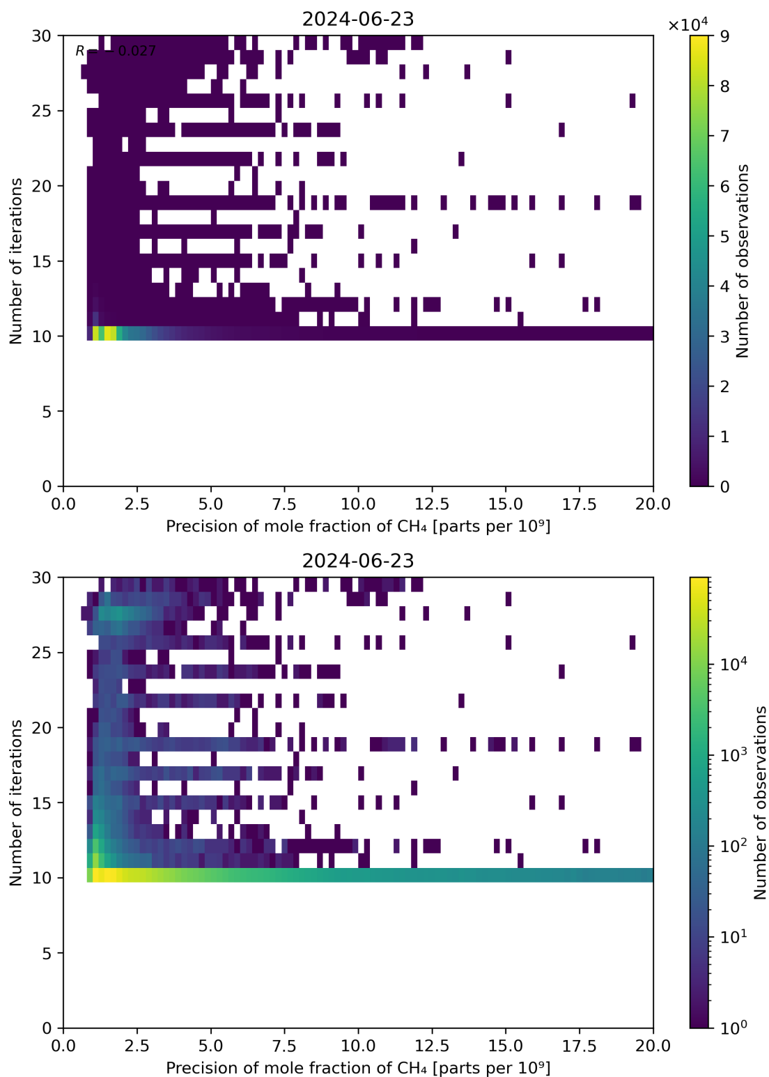
Figure 83: Scatter density plot of “Precision of mole fraction of CH 4 ” against “Number of iterations” for 2024-06-22 to 2024-06-24.
