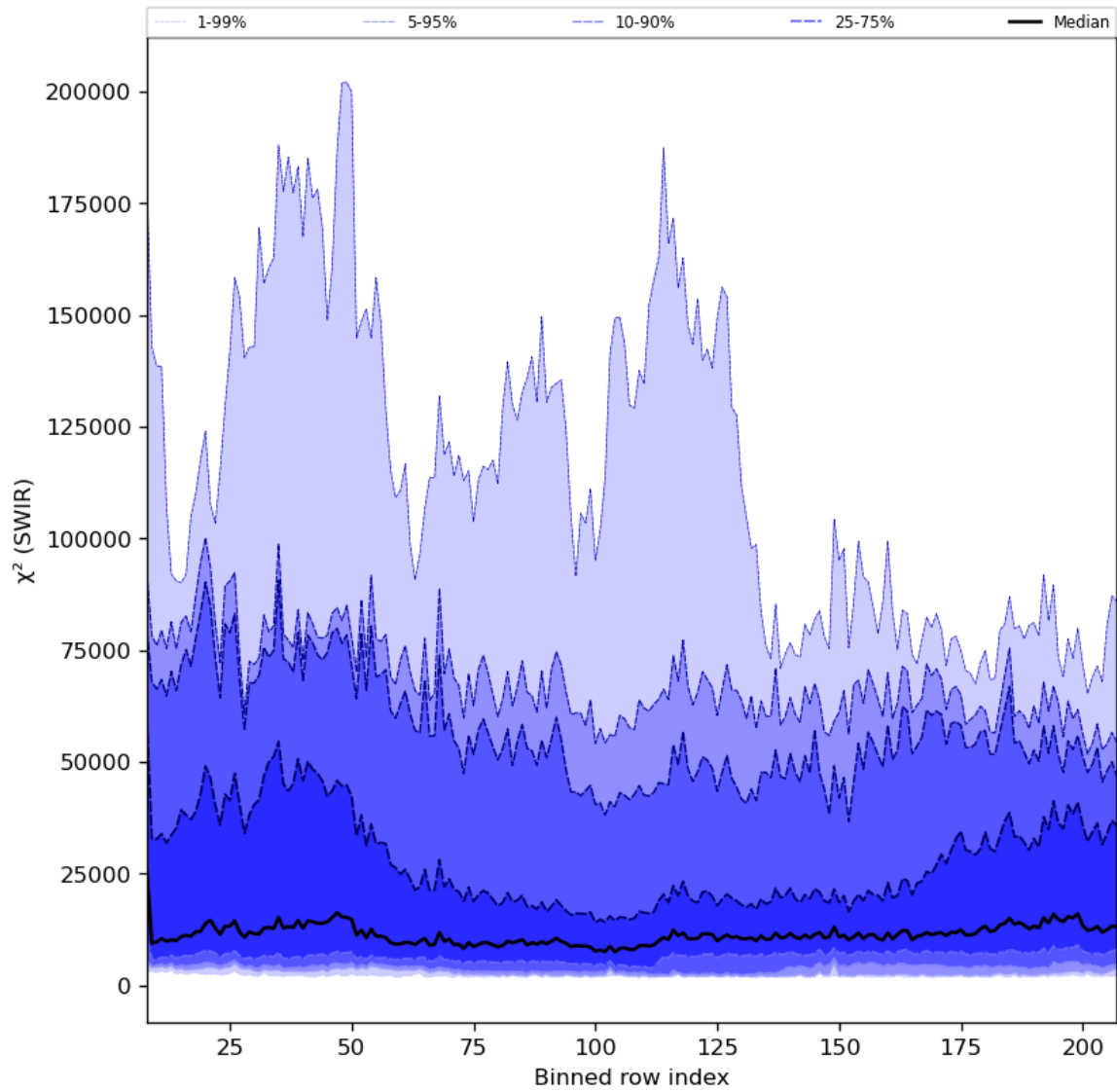
Figure 39: Along track statistics of “ \chi^2 (SWIR)” for 2024-06-22 to 2024-06-24
