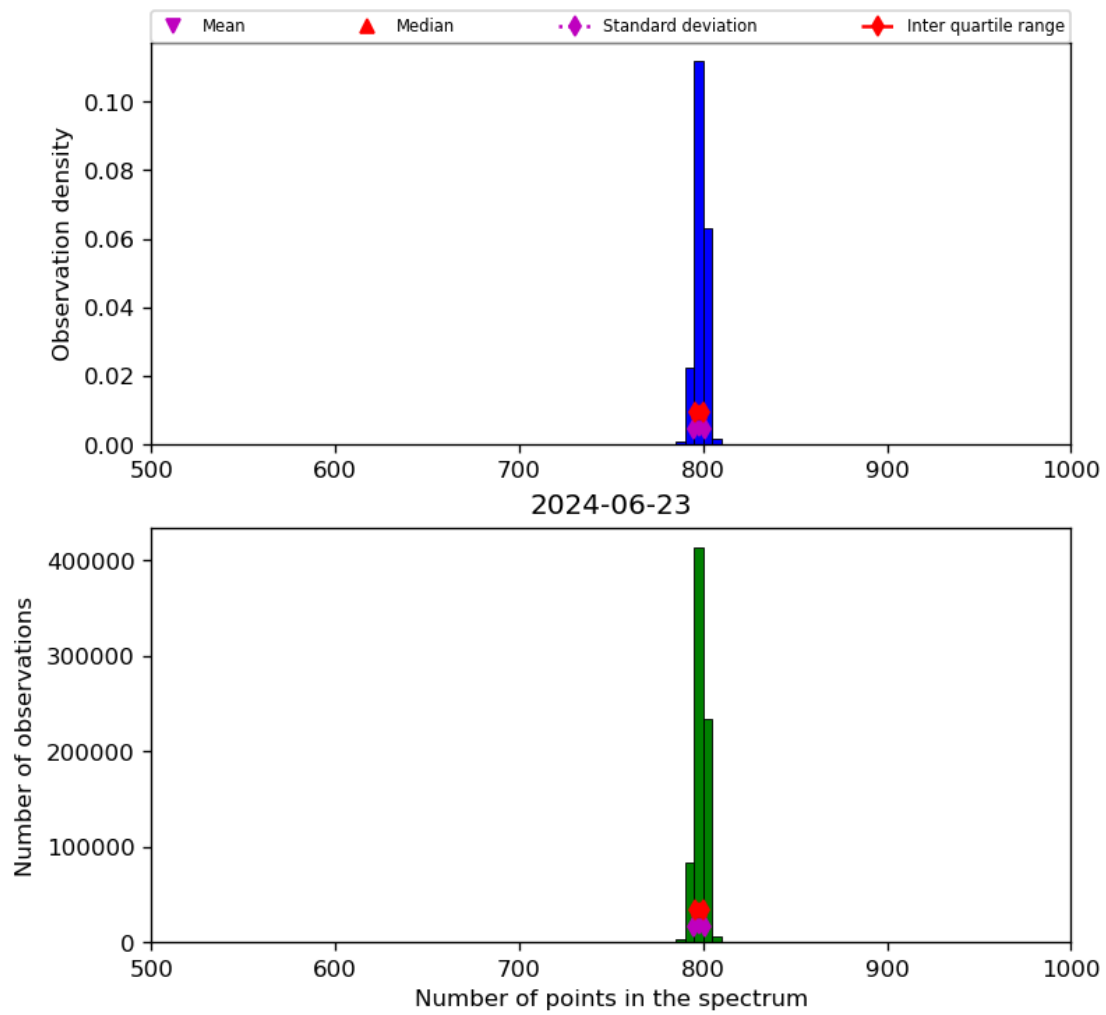
Figure 26: Histogram of “Number of points in the spectrum” for 2024-06-22 to 2024-06-24
