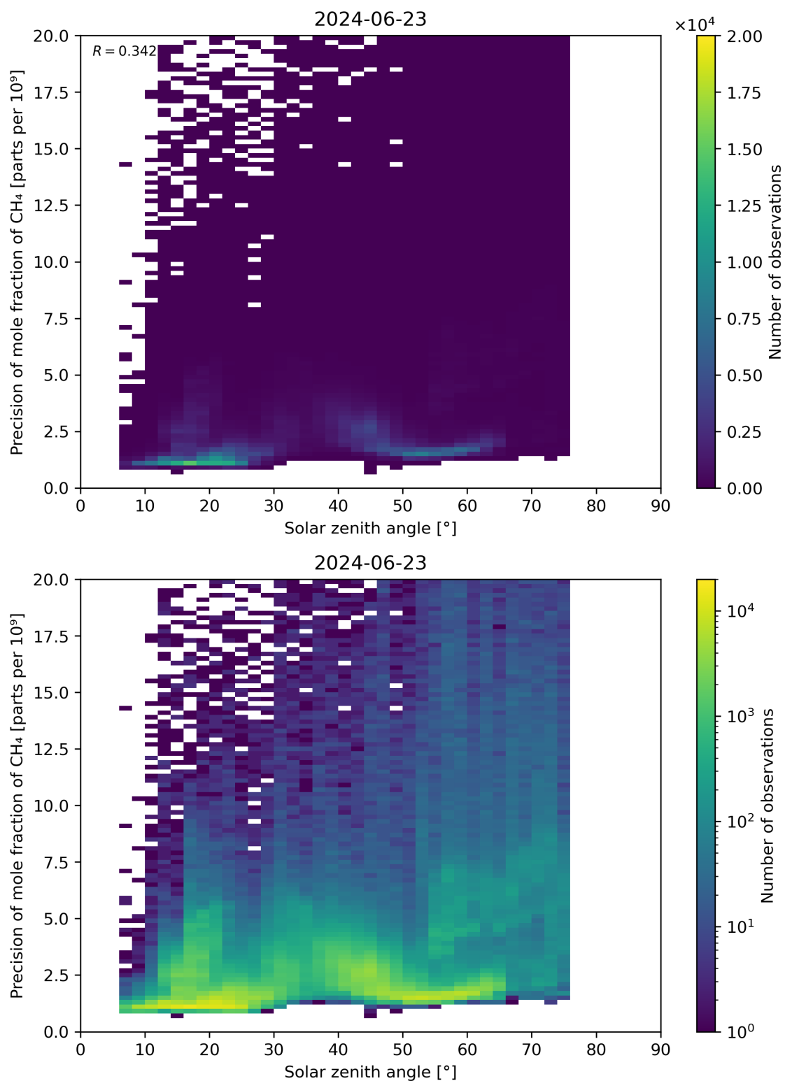
Figure 101: Scatter density plot of “Solar zenith angle” against “Precision of mole fraction of \text{CH}_4 ” for 2024-06-22 to 2024-06-24.
