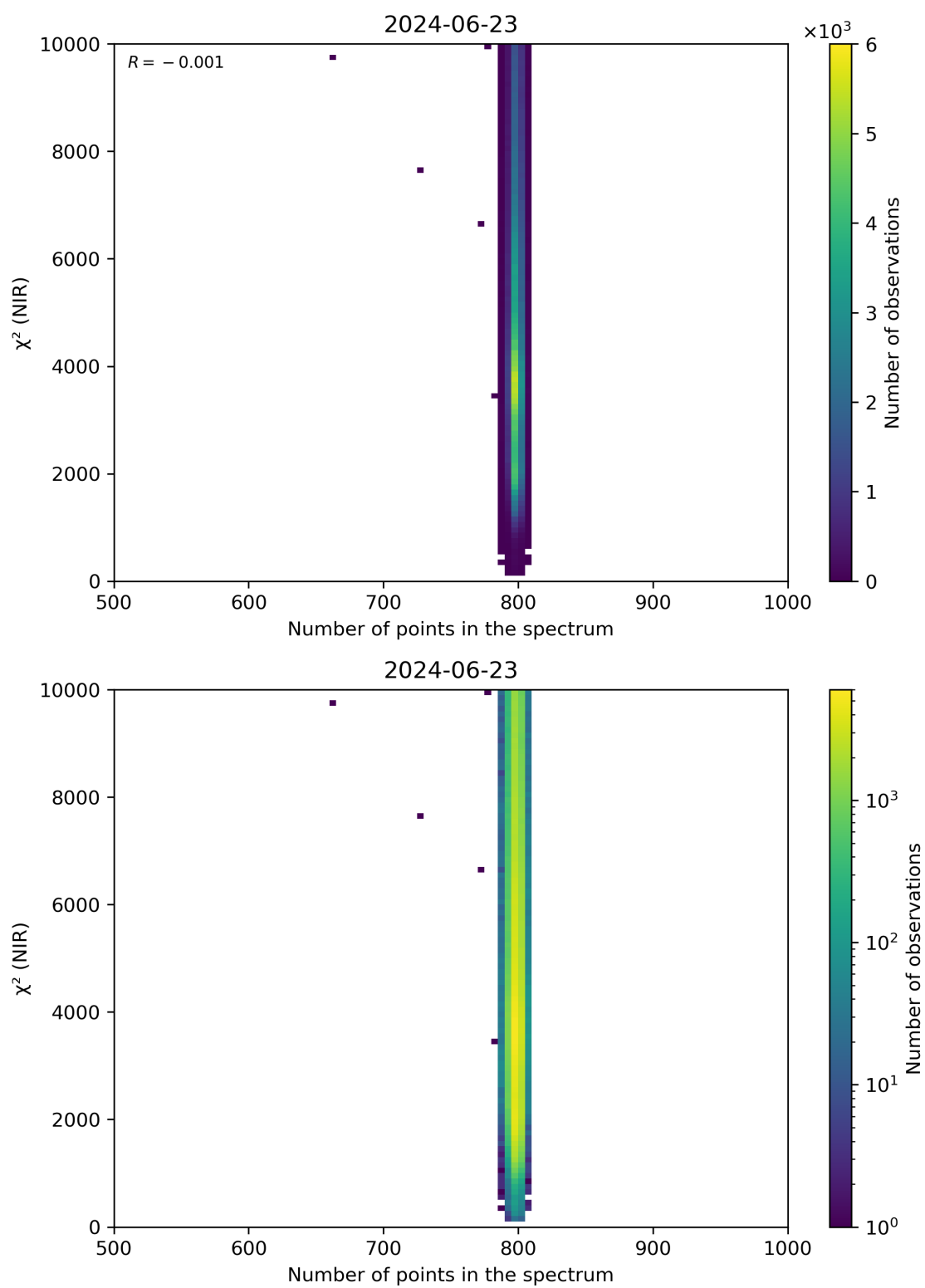
Figure 88: Scatter density plot of “Number of points in the spectrum” against “ \chi^2 (NIR)” for 2024-06-22 to 2024-06-24.
