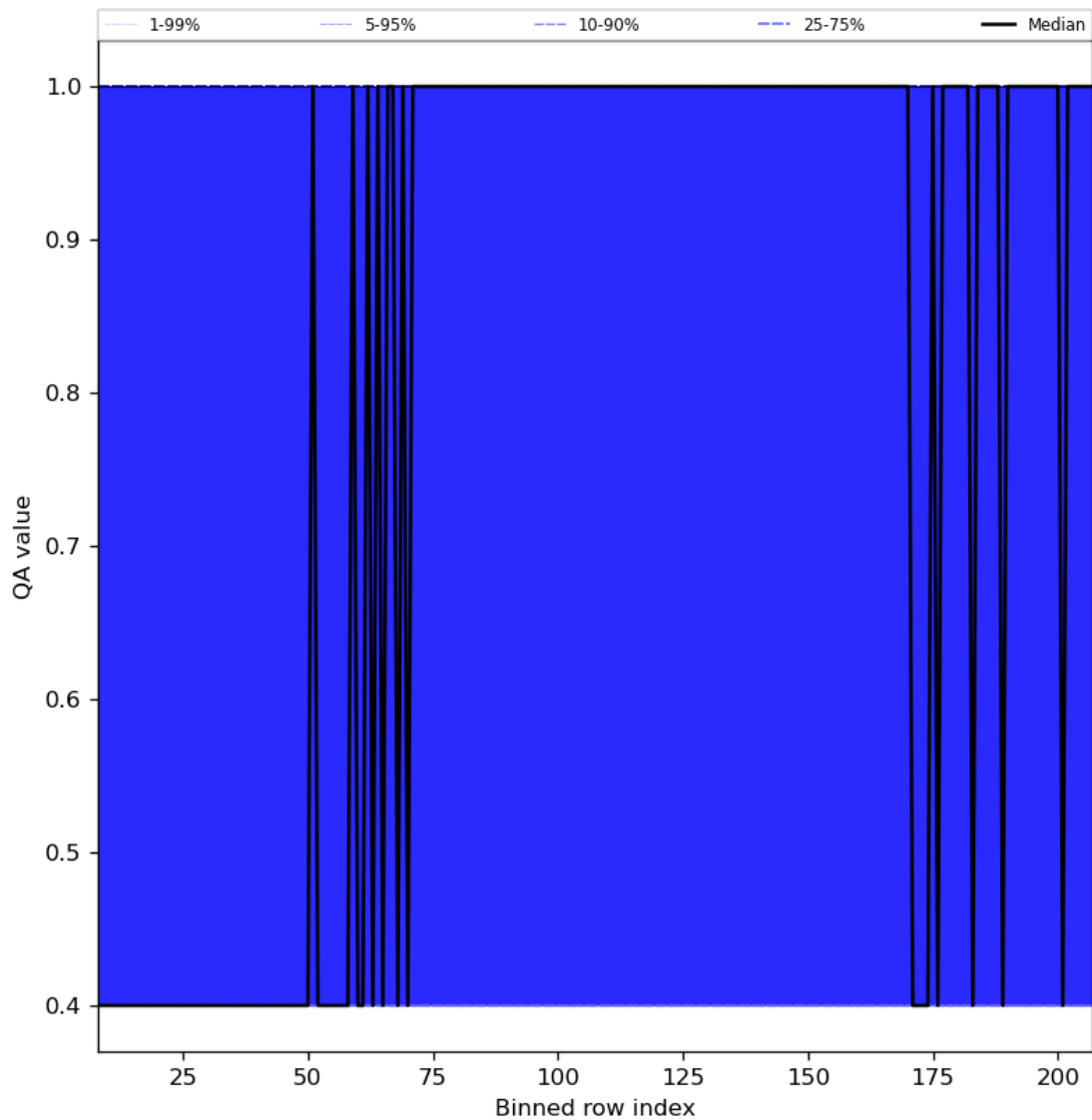
Figure 33: Along track statistics of “QA value” for 2024-06-22 to 2024-06-24
