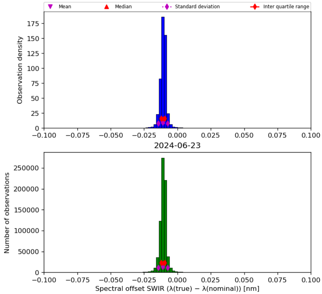
Figure 27: Histogram of “Spectral offset SWIR ( \lambda(\text{true}) - \lambda(\text{nominal}) )” for 2024-06-22 to 2024-06-24
