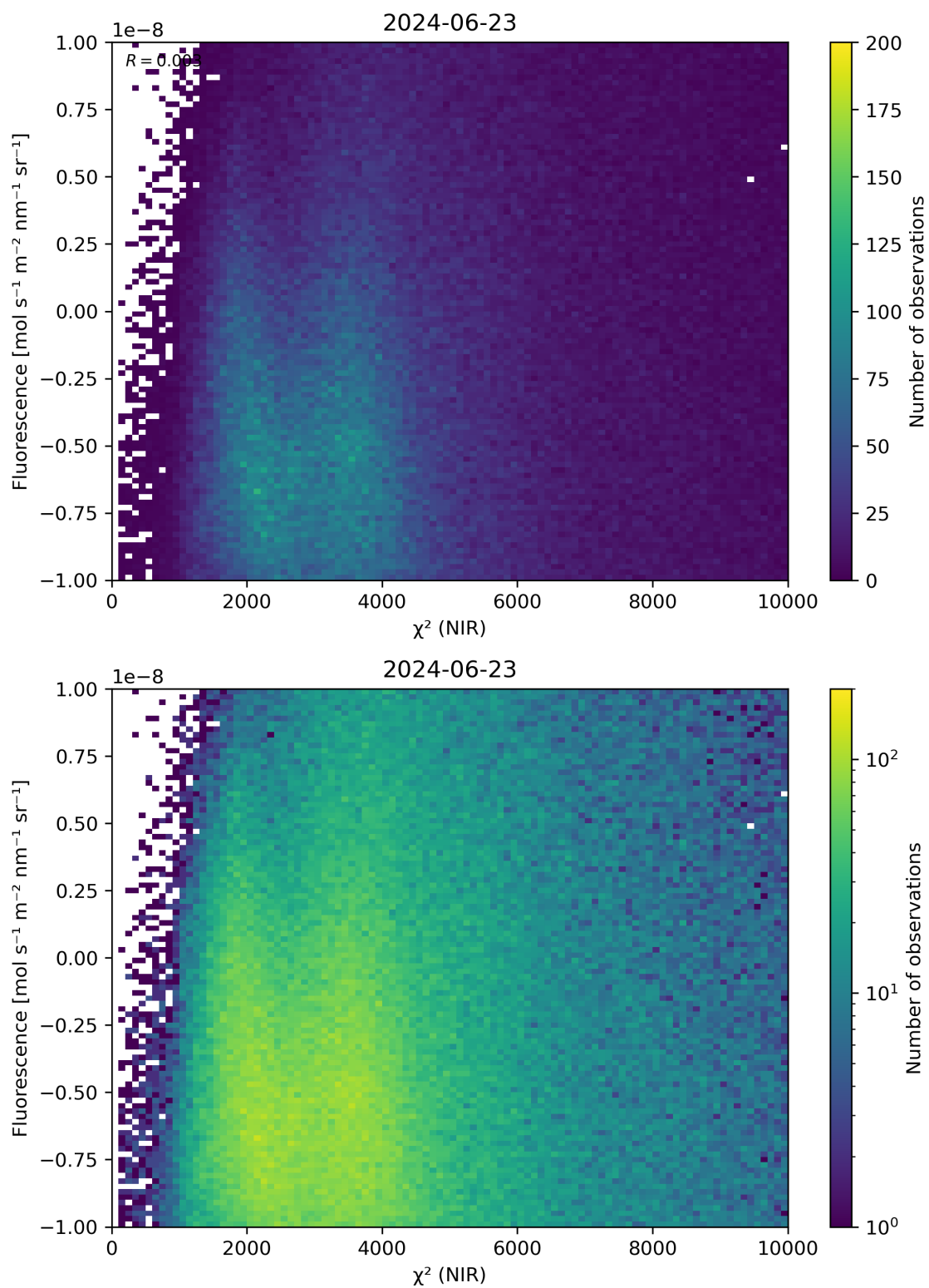
Figure 45: Scatter density plot of “ \chi^2 (NIR)” against “Fluorescence” for 2024-06-22 to 2024-06-24.
