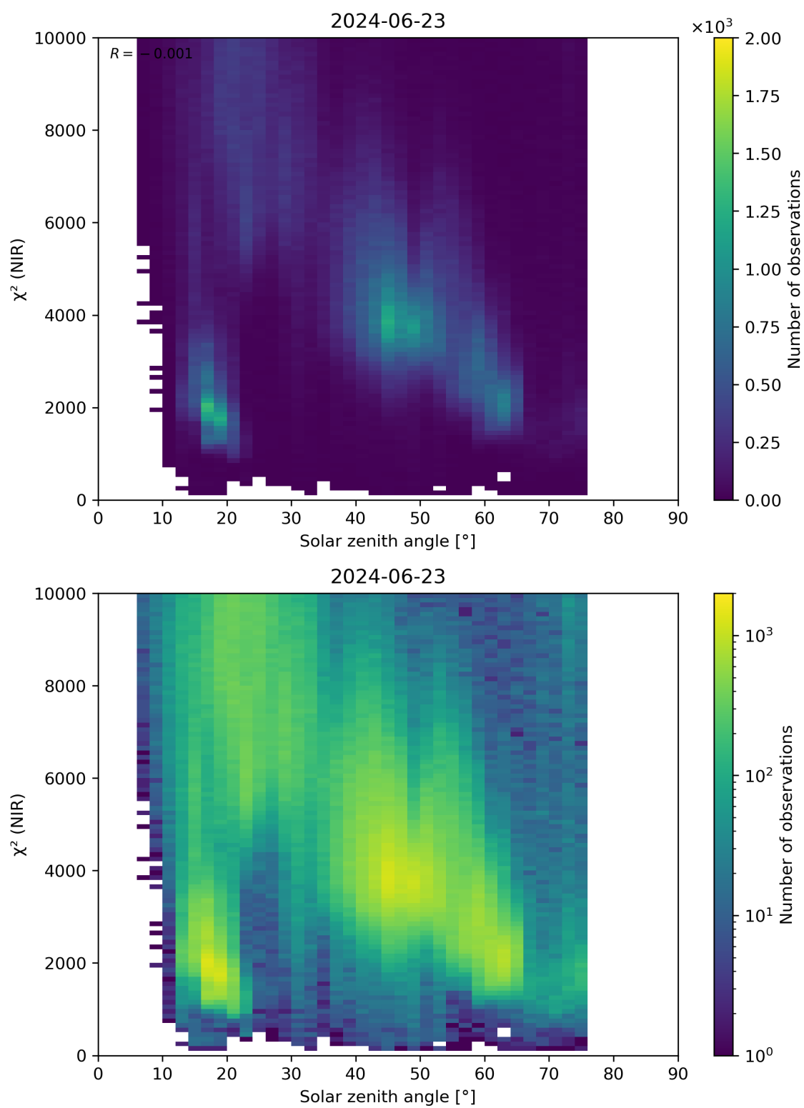
Figure 94: Scatter density plot of “Solar zenith angle” against “ \chi^2 (NIR)” for 2024-06-22 to 2024-06-24.
