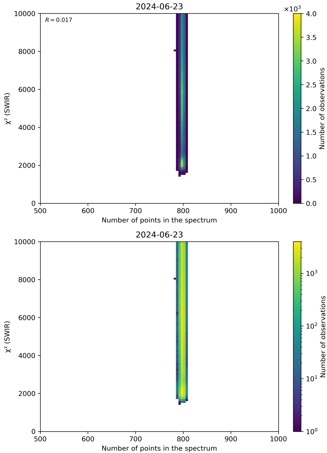
Figure 89: Scatter density plot of “Number of points in the spectrum” against “ \chi^2 (SWIR)” for 2024-06-22 to 2024-06-24.
