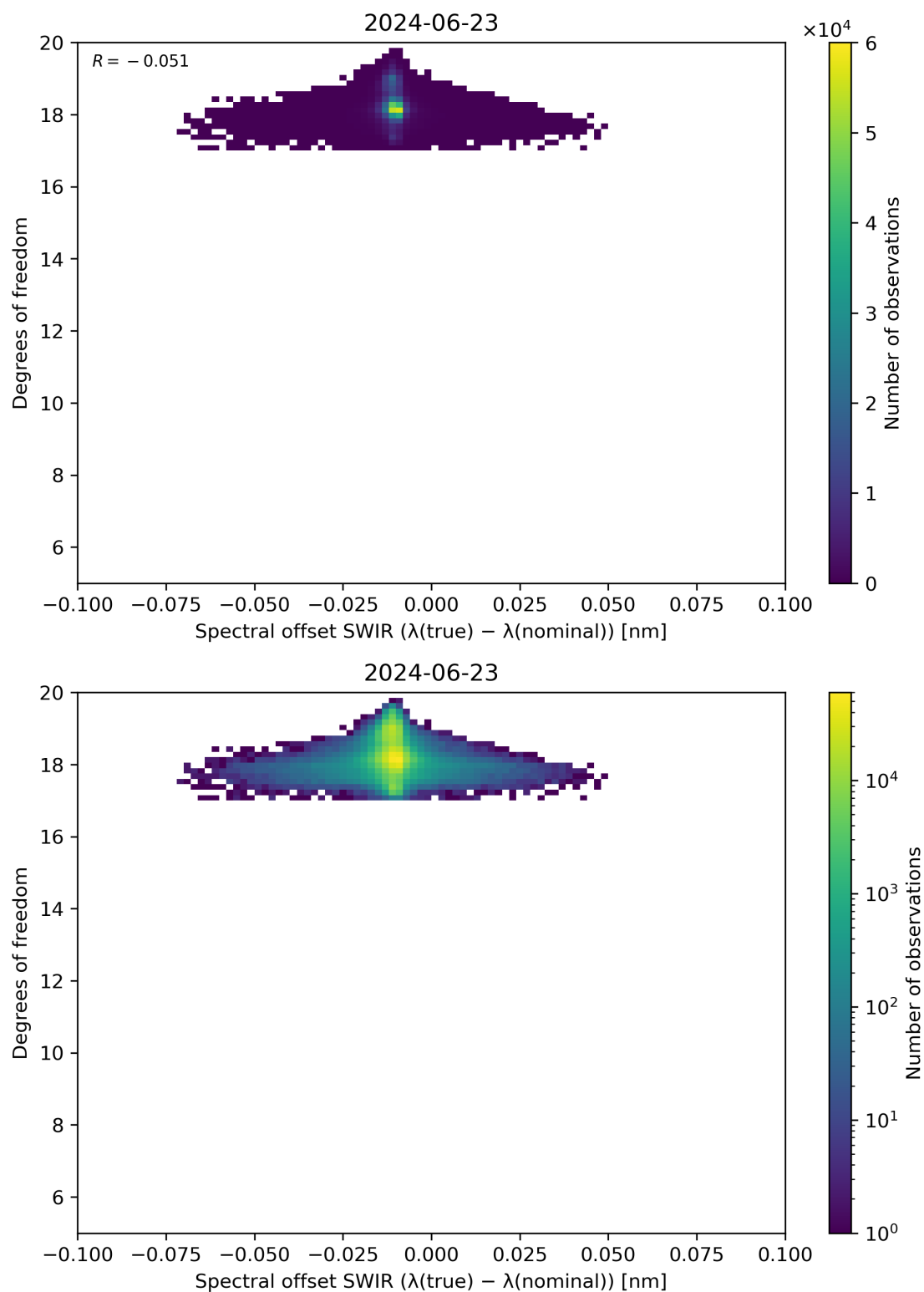
Figure 119: Scatter density plot of “Spectral offset SWIR ( \lambda(\text{true}) - \lambda(\text{nominal}) )” against “Degrees of freedom” for 2024-06-22 to 2024-06-24.
