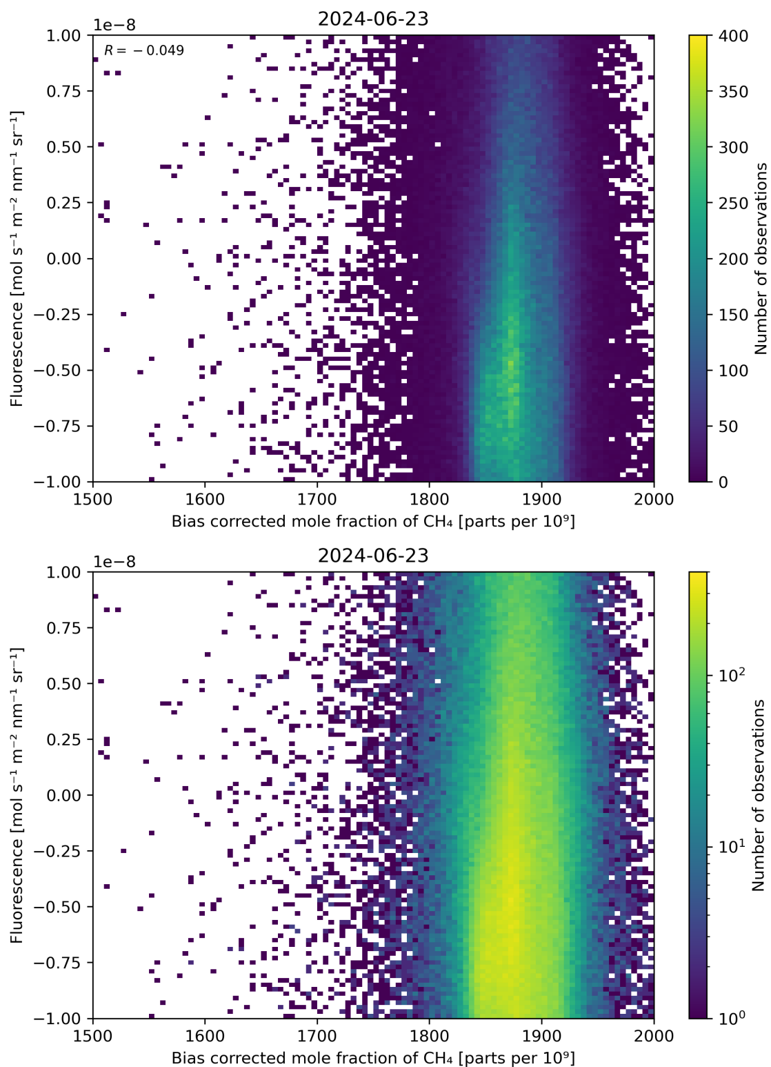
Figure 66: Scatter density plot of “Bias corrected mole fraction of \text{CH}_4 ” against “Fluorescence” for 2024-06-22 to 2024-06-24.
