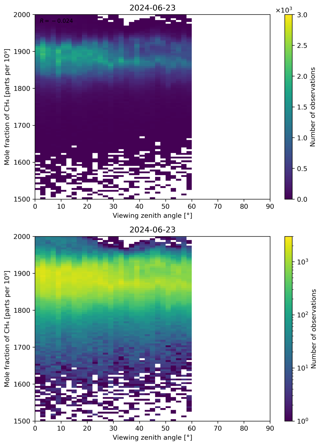
Figure 110: Scatter density plot of “Viewing zenith angle” against “Mole fraction of CH 4 ” for 2024-06-22 to 2024-06-24.
