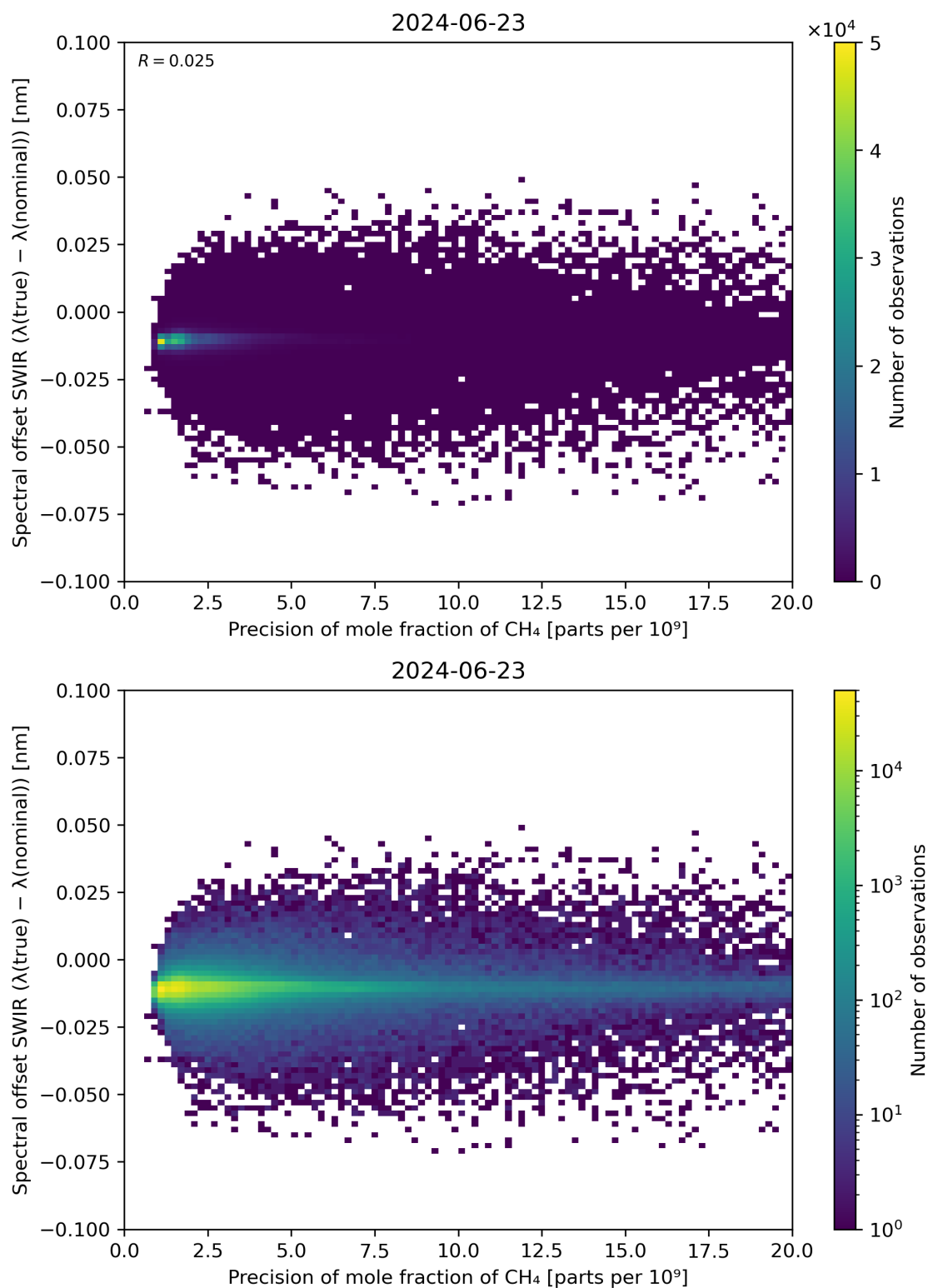
Figure 85: Scatter density plot of “Precision of mole fraction of CH 4 ” against “Spectral offset SWIR ( \lambda(\text{true}) - \lambda(\text{nominal}) )” for 2024-06-22 to 2024-06-24.
