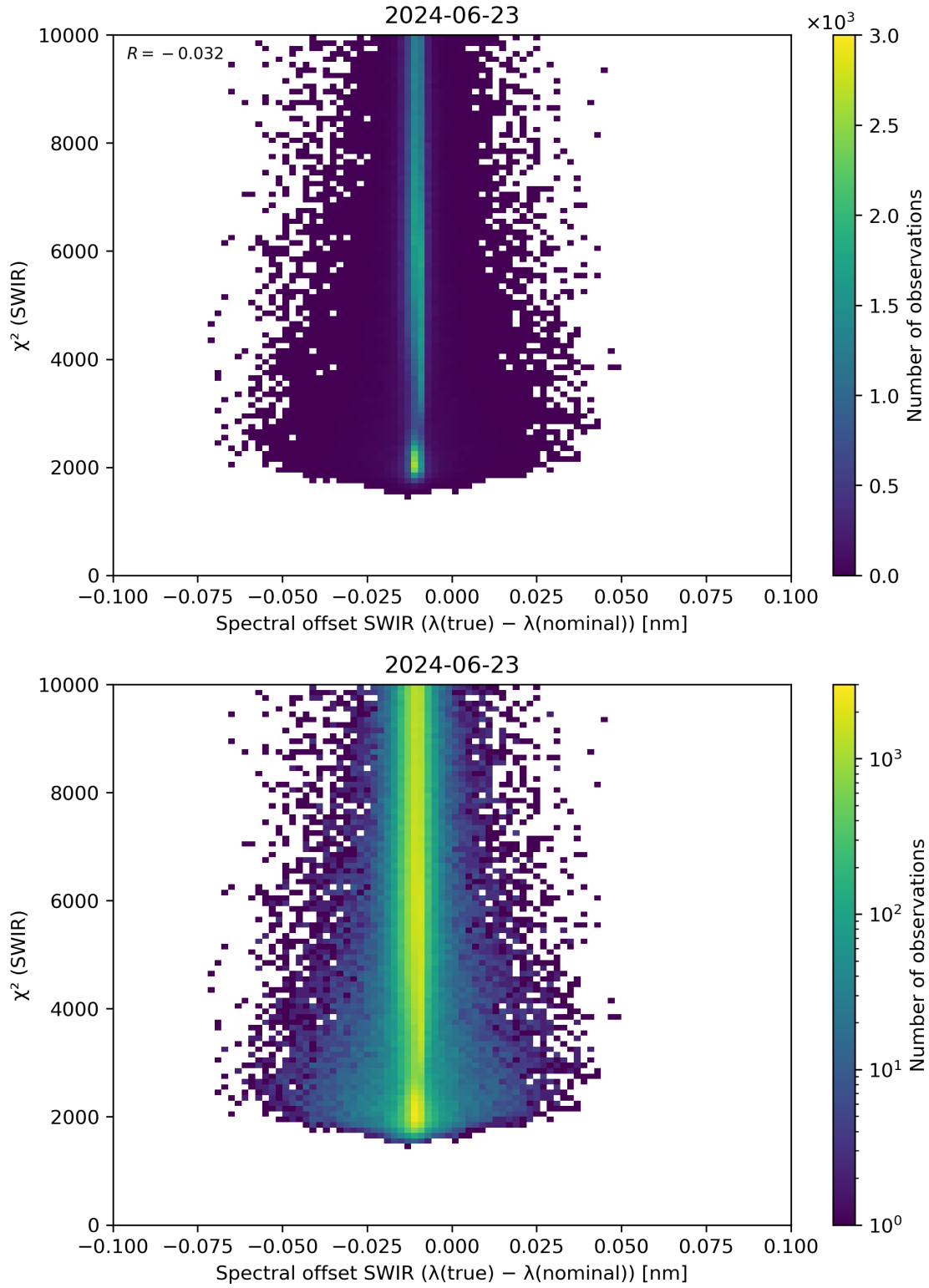
Figure 118: Scatter density plot of “Spectral offset SWIR ( \lambda(\text{true}) - \lambda(\text{nominal}) )” against “ \chi^2 (SWIR)” for 2024-06-22 to 2024-06-24.
