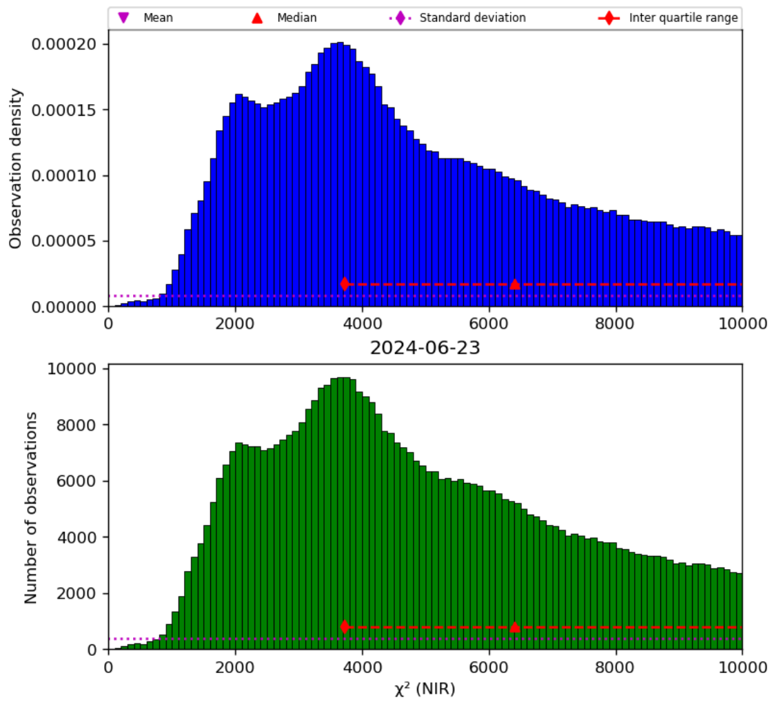
Figure 29: Histogram of " \chi^2 (NIR)" for 2024-06-22 to 2024-06-24
