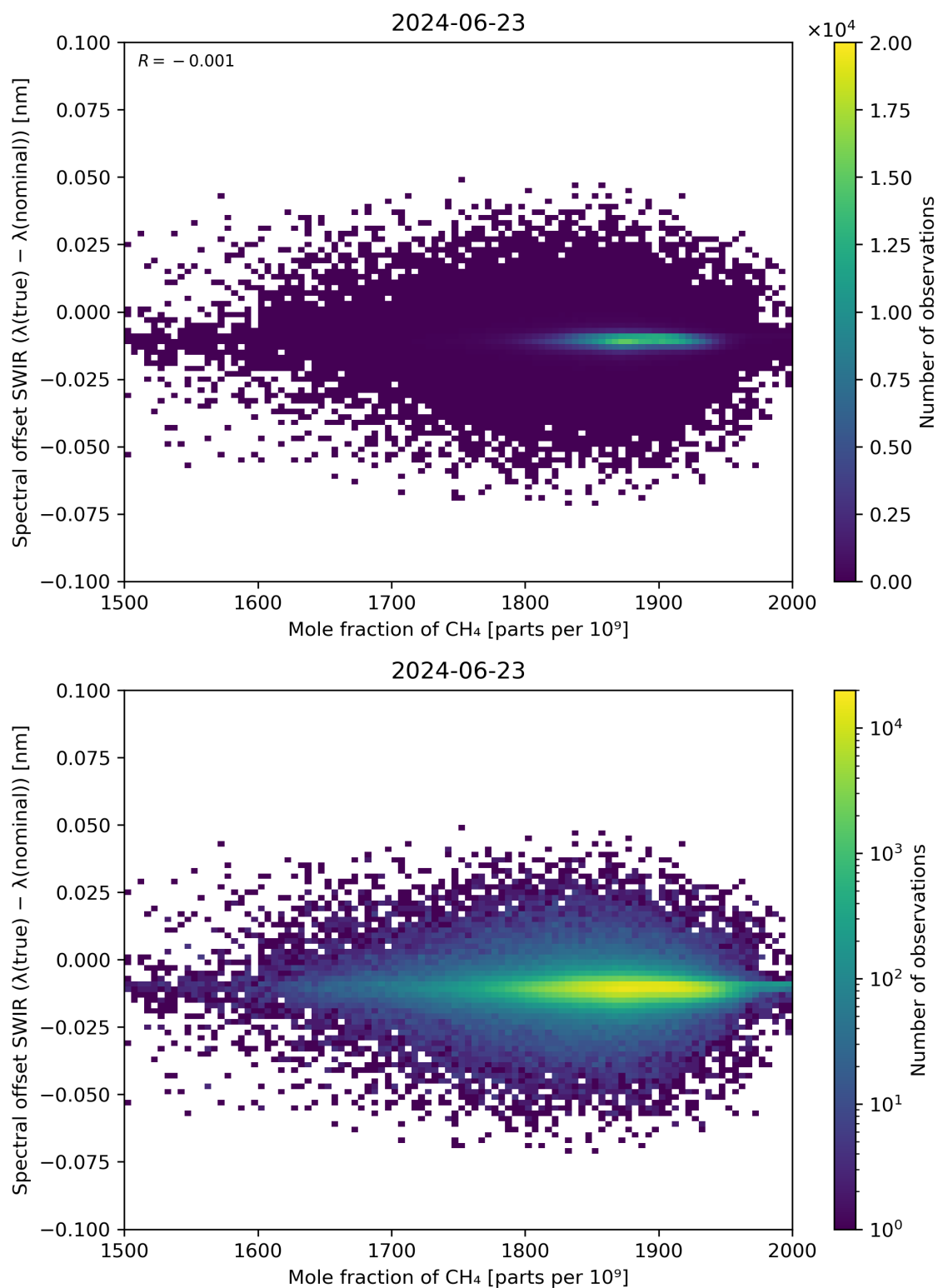
Figure 86: Scatter density plot of “Mole fraction of CH 4 ” against “Spectral offset SWIR ( \lambda(\text{true}) - \lambda(\text{nominal}) )” for 2024-06-22 to 2024-06-24.
