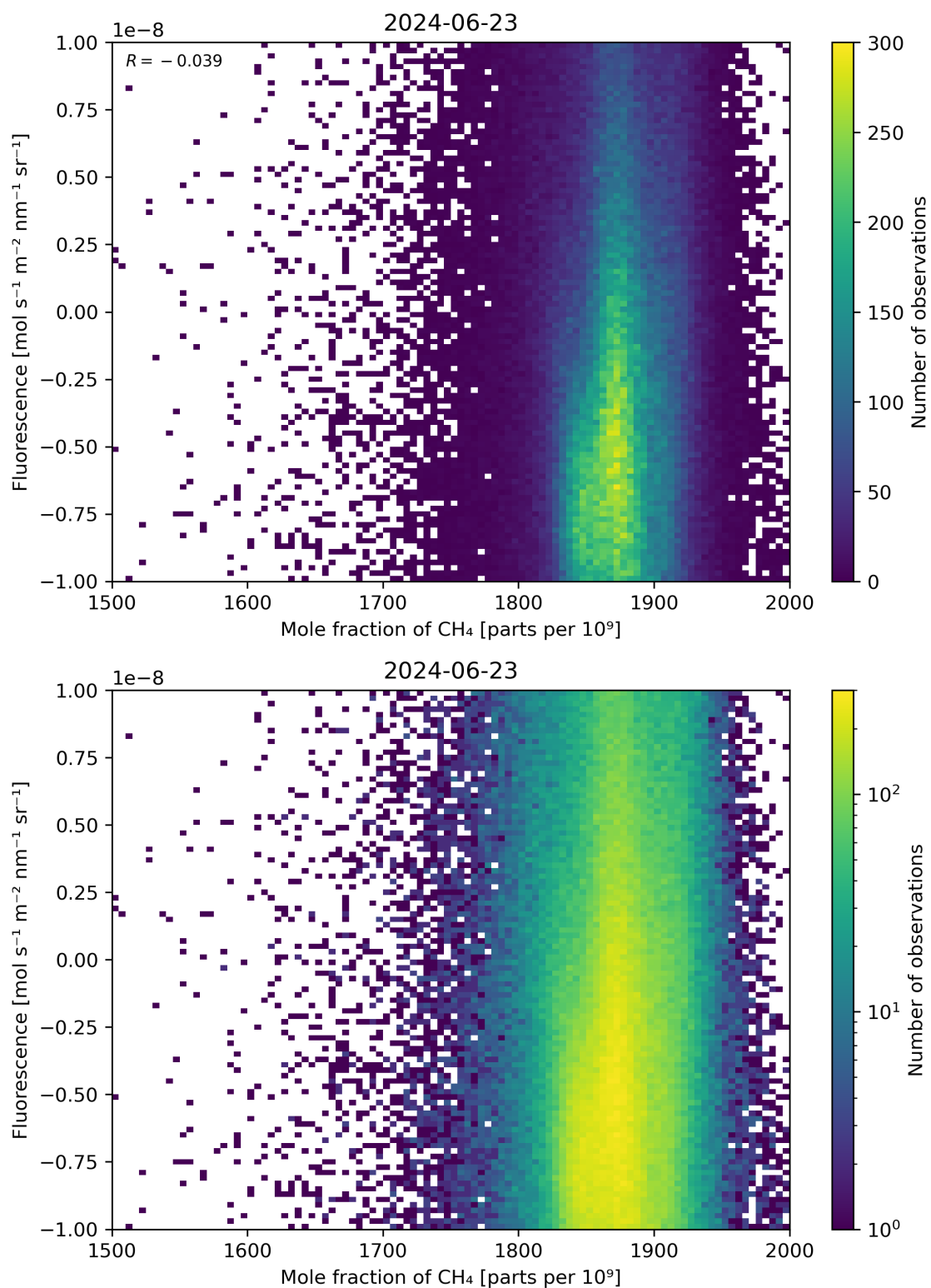
Figure 73: Scatter density plot of “Mole fraction of \text{CH}_4 ” against “Fluorescence” for 2024-06-22 to 2024-06-24.
