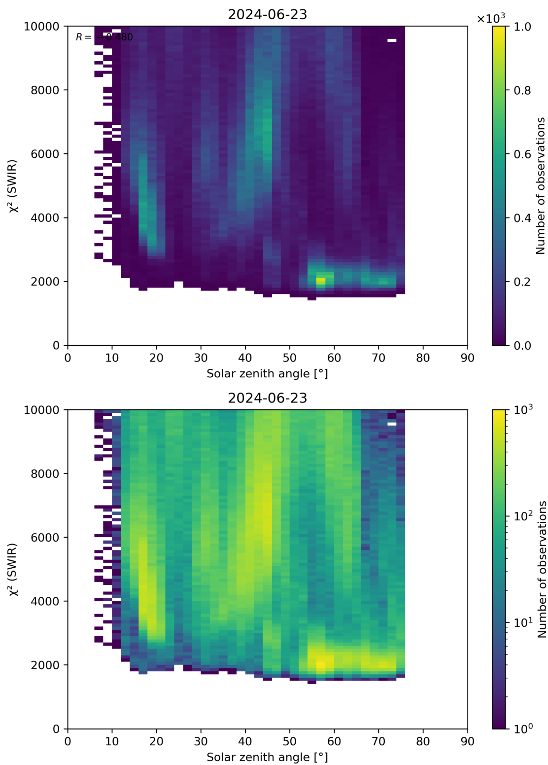
Figure 95: Scatter density plot of “Solar zenith angle” against “ \chi^2 (SWIR)” for 2024-06-22 to 2024-06-24.
