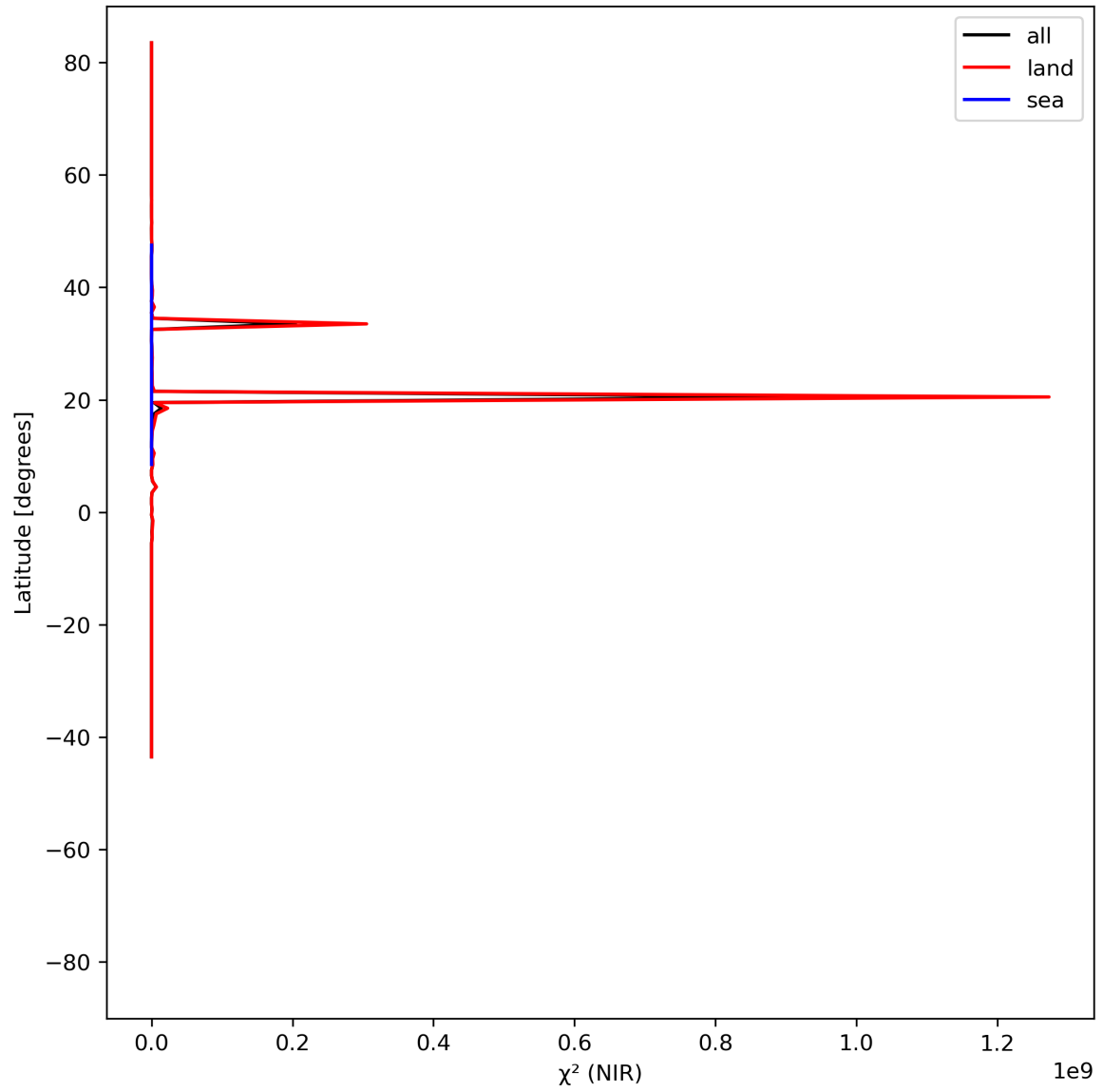
Figure 18: Zonal average of “ \chi^2 (NIR)” for 2024-06-22 to 2024-06-24.
