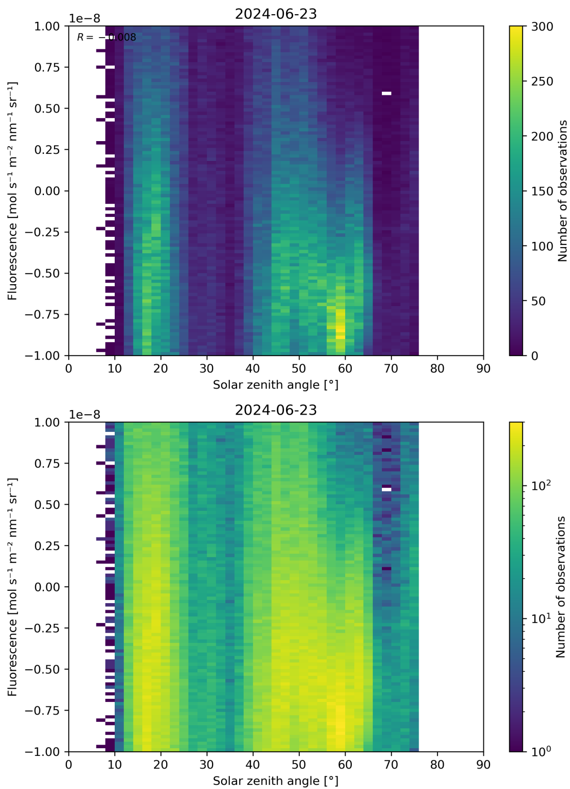
Figure 97: Scatter density plot of “Solar zenith angle” against “Fluorescence” for 2024-06-22 to 2024-06-24.
