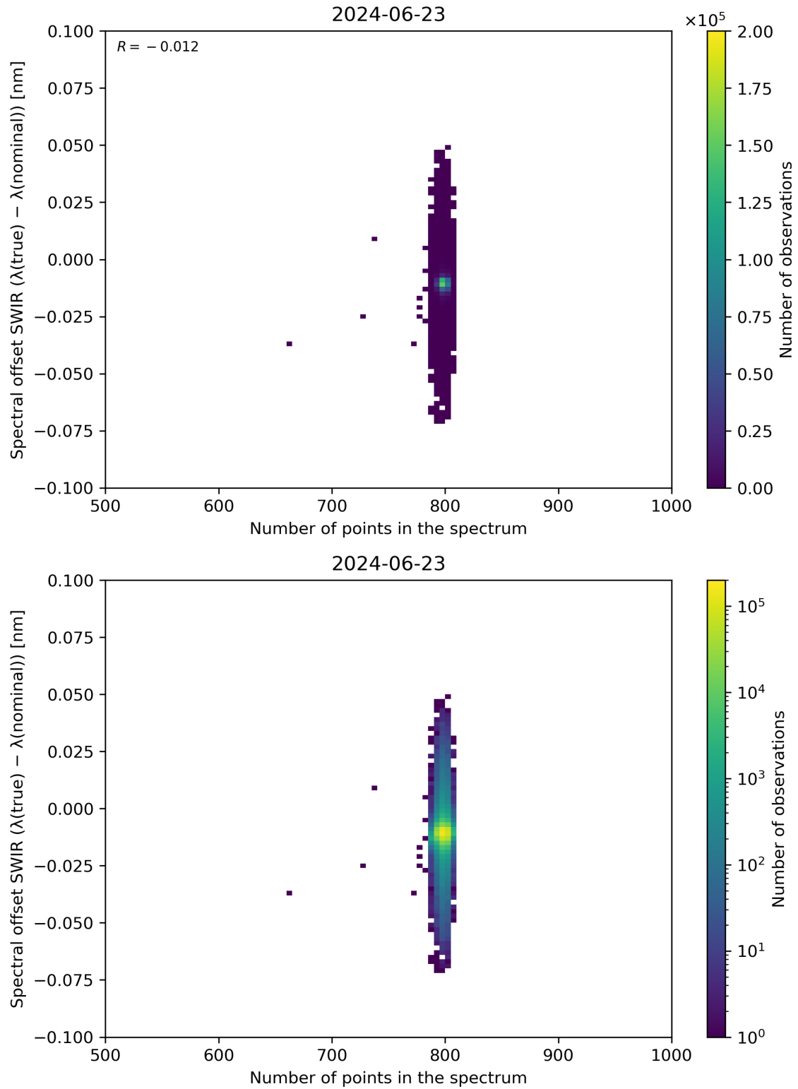
Figure 93: Scatter density plot of “Number of points in the spectrum” against “Spectral offset SWIR ( \lambda(\text{true}) - \lambda(\text{nominal}) )” for 2024-06-22 to 2024-06-24.
