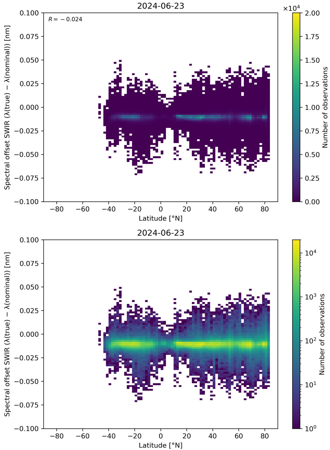
Figure 62: Scatter density plot of “Latitude” against “Spectral offset SWIR ( \lambda(\text{true}) - \lambda(\text{nominal}) )” for 2024-06-22 to 2024-06-24.
