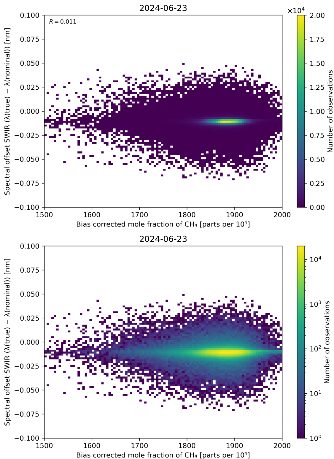
Figure 69: Scatter density plot of “Bias corrected mole fraction of \text{CH}_4 ” against “Spectral offset SWIR ( \lambda(\text{true}) - \lambda(\text{nominal}) )” for 2024-06-22 to 2024-06-24.
