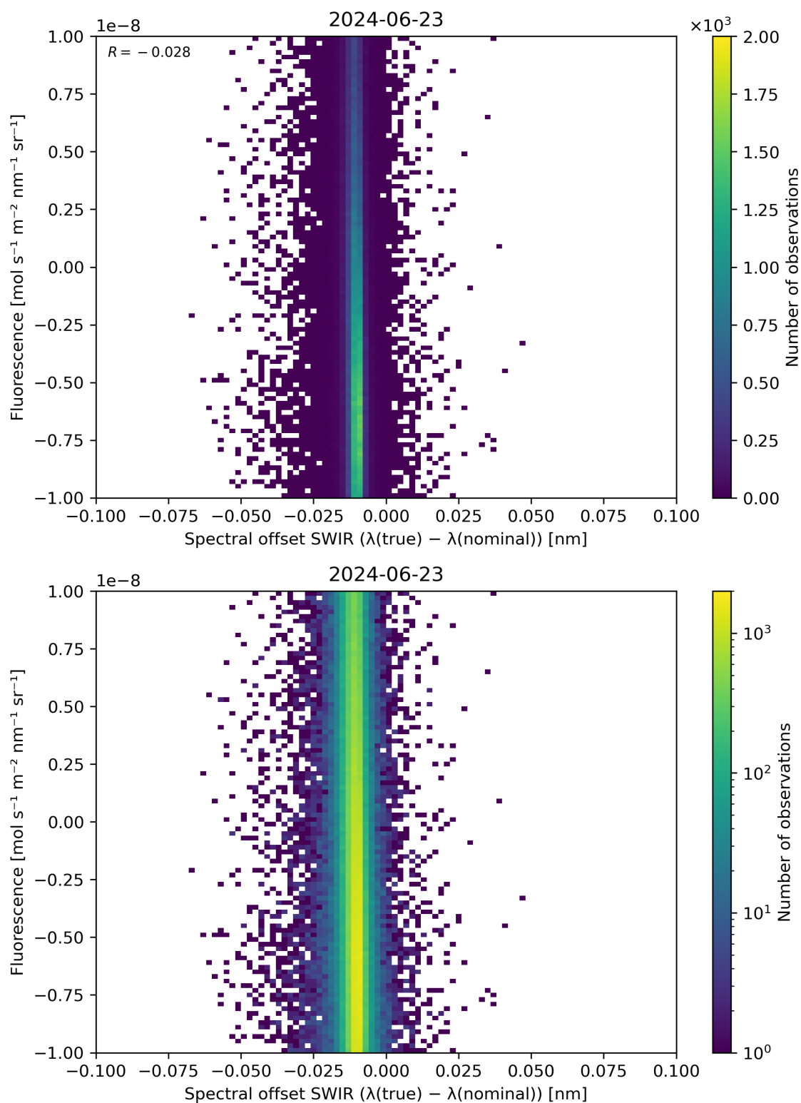
Figure 120: Scatter density plot of “Spectral offset SWIR ( \lambda(\text{true}) - \lambda(\text{nominal}) )” against “Fluorescence” for 2024-06-22 to 2024-06-24.
