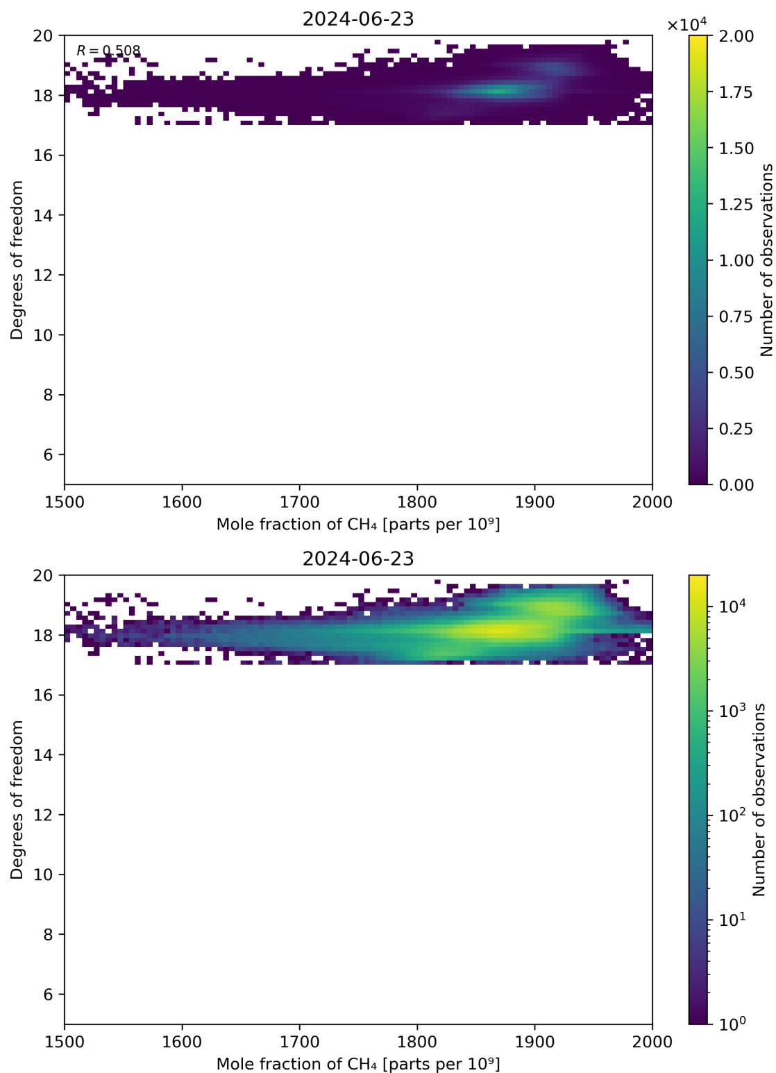
Figure 72: Scatter density plot of “Mole fraction of CH 4 ” against “Degrees of freedom” for 2024-06-22 to 2024-06-24.
