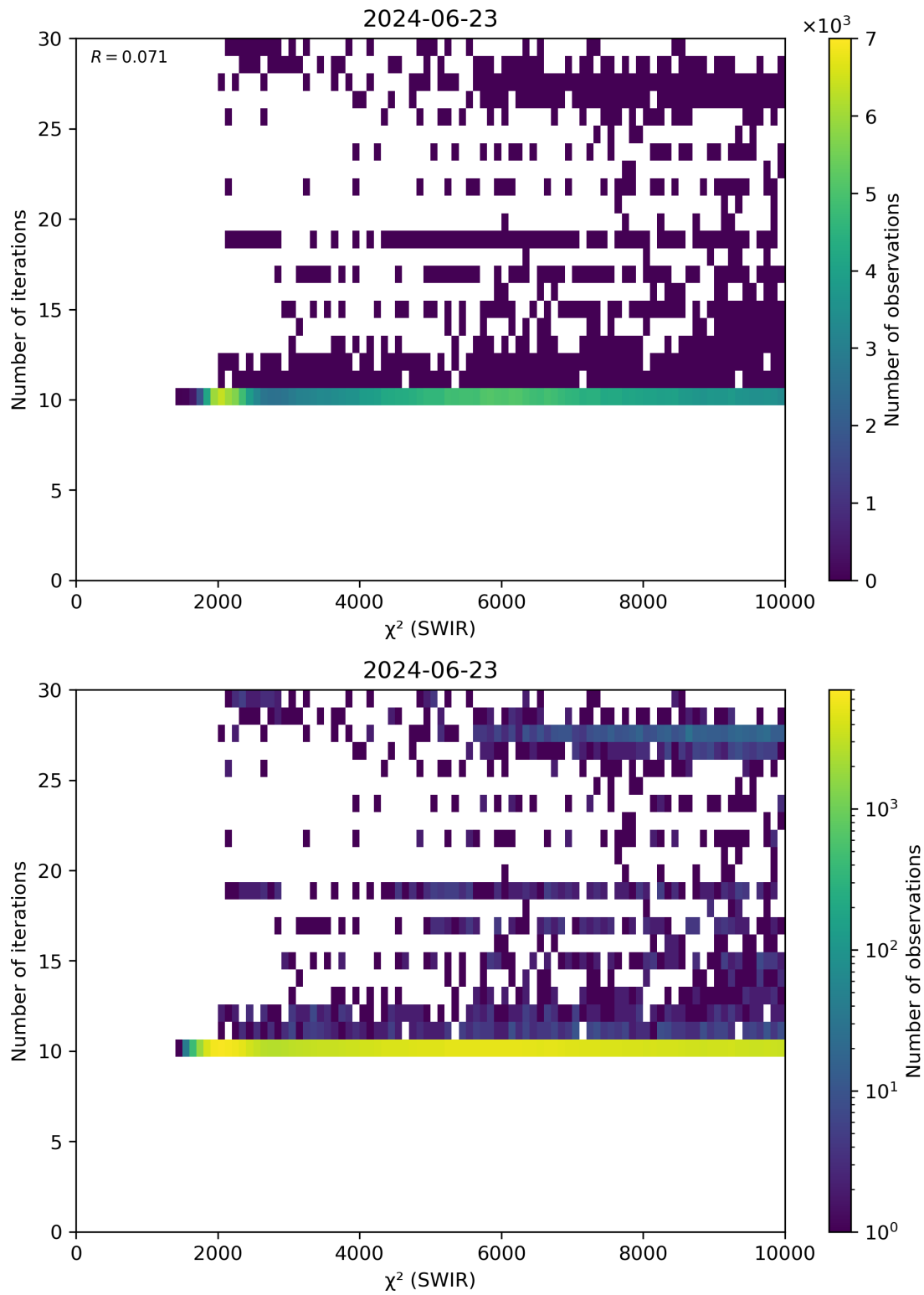
Figure 50: Scatter density plot of “ \chi^2 (SWIR)” against “Number of iterations” for 2024-06-22 to 2024-06-24.
