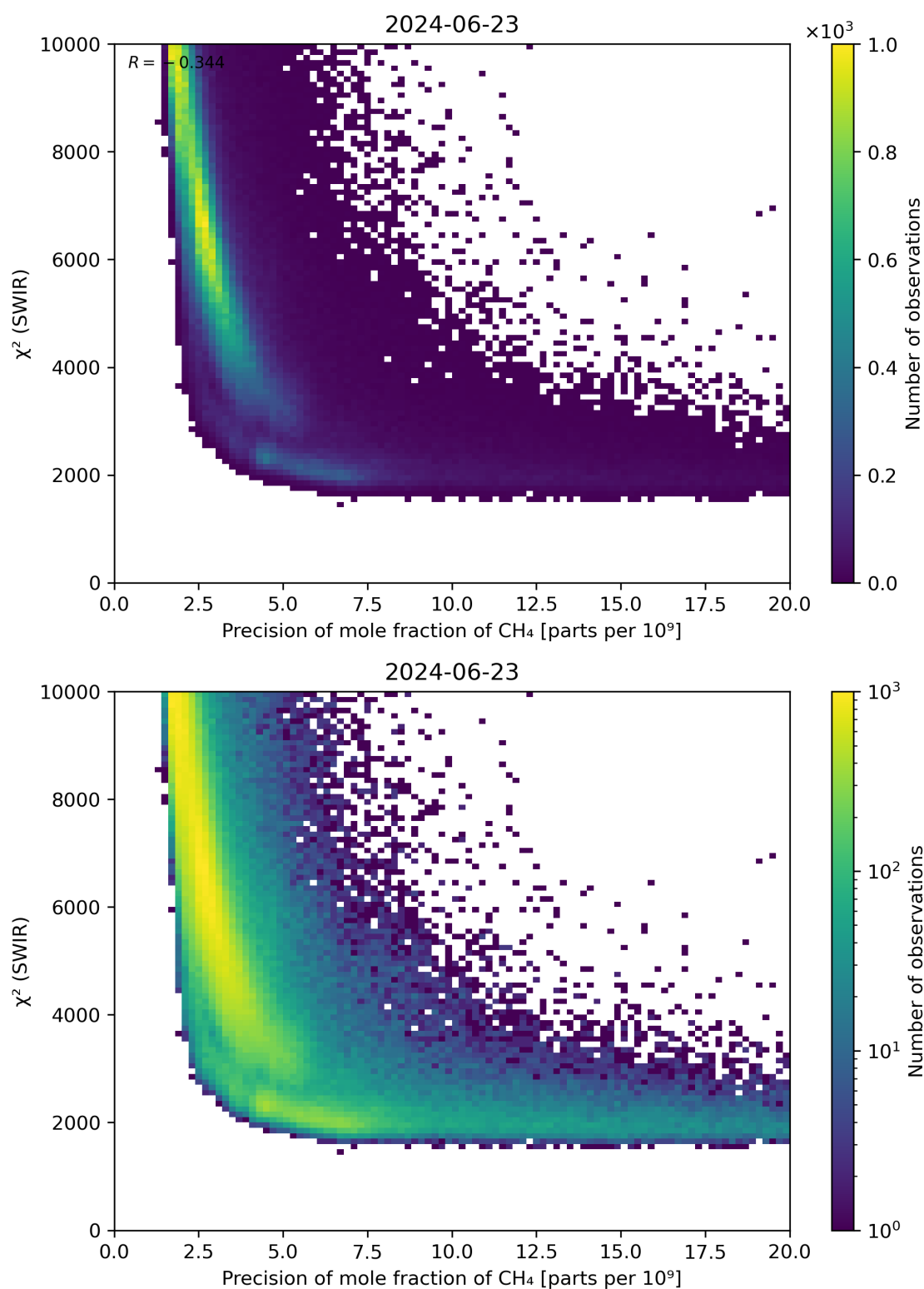
Figure 79: Scatter density plot of “Precision of mole fraction of \text{CH}_4 ” against “ \chi^2 (SWIR)” for 2024-06-22 to 2024-06-24.
