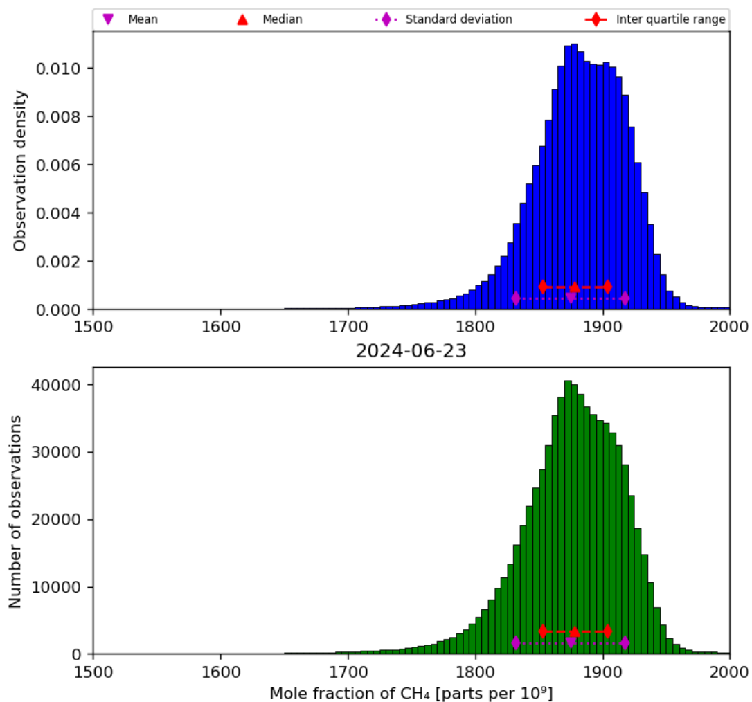
Figure 23: Histogram of “Mole fraction of CH 4 ” for 2024-06-22 to 2024-06-24
