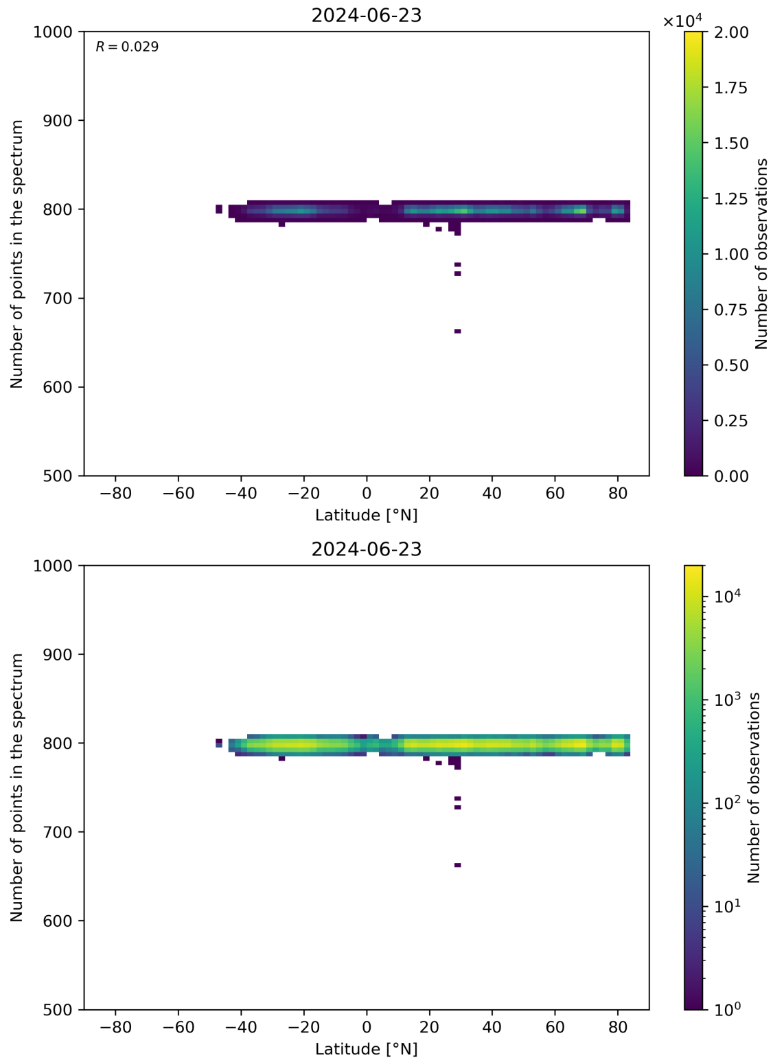
Figure 61: Scatter density plot of “Latitude” against “Number of points in the spectrum” for 2024-06-22 to 2024-06-24.
