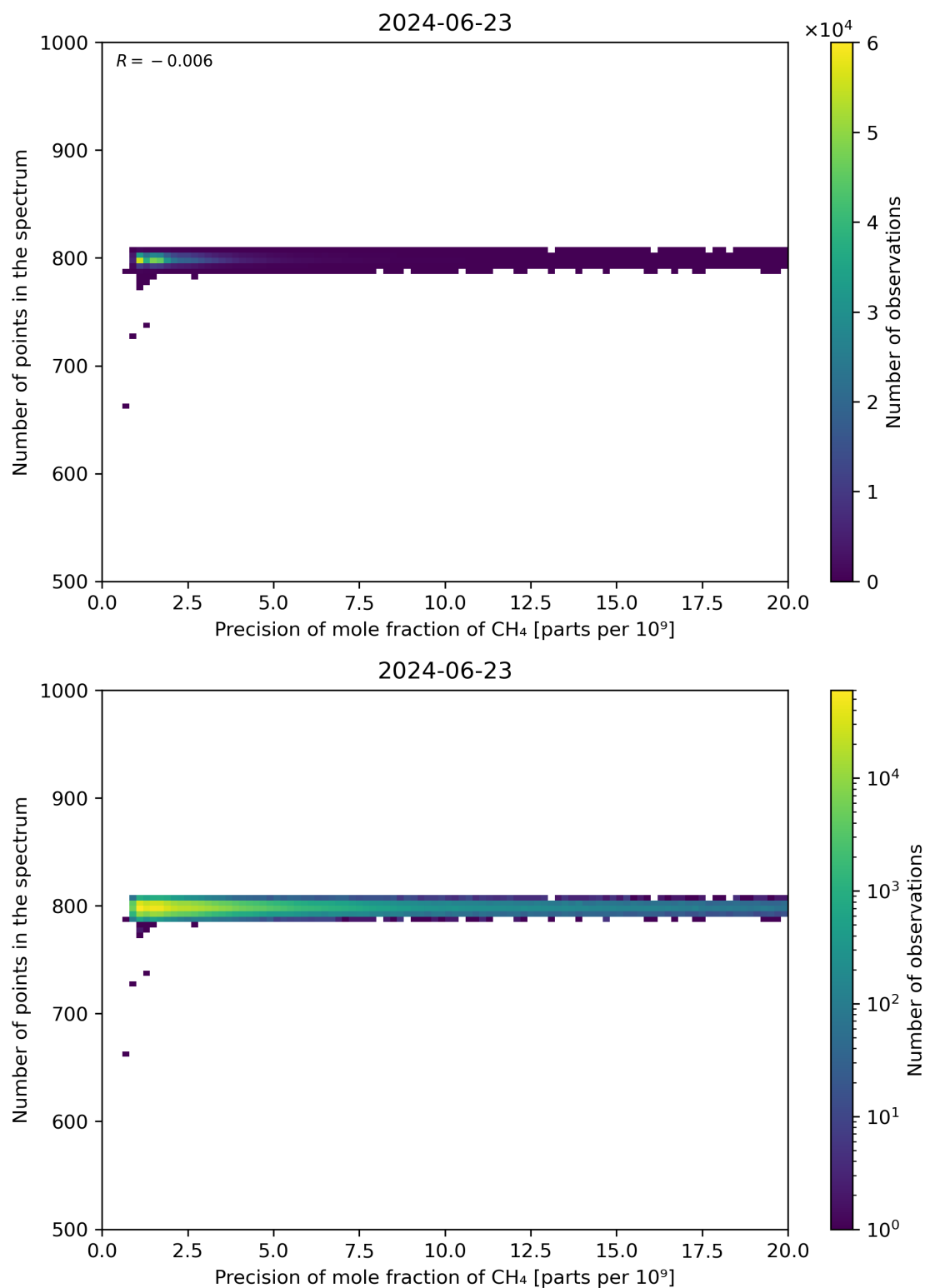
Figure 84: Scatter density plot of “Precision of mole fraction of CH 4 ” against “Number of points in the spectrum” for 2024-06-22 to 2024-06-24.
