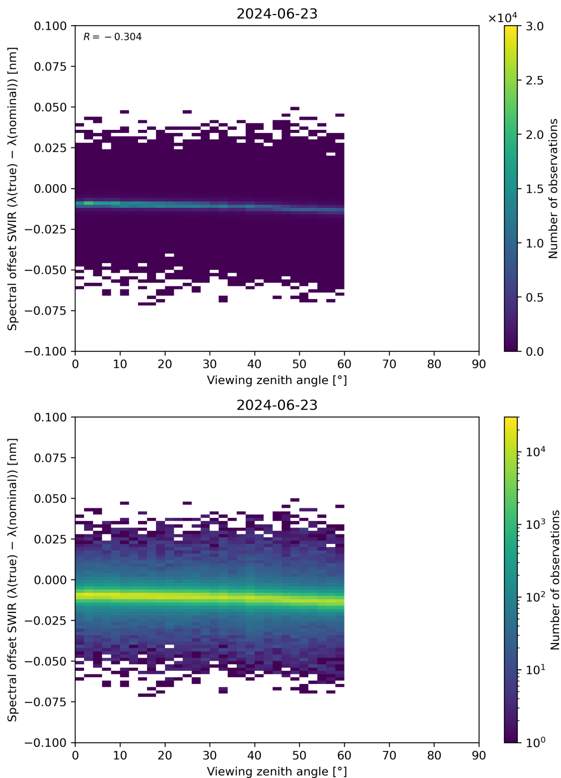
Figure 116: Scatter density plot of “Viewing zenith angle” against “Spectral offset SWIR ( \lambda(\text{true}) - \lambda(\text{nominal}) )” for 2024-06-22 to 2024-06-24.
