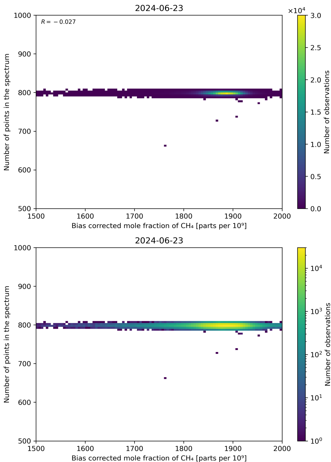
Figure 68: Scatter density plot of “Bias corrected mole fraction of CH 4 ” against “Number of points in the spectrum” for 2024-06-22 to 2024-06-24.
