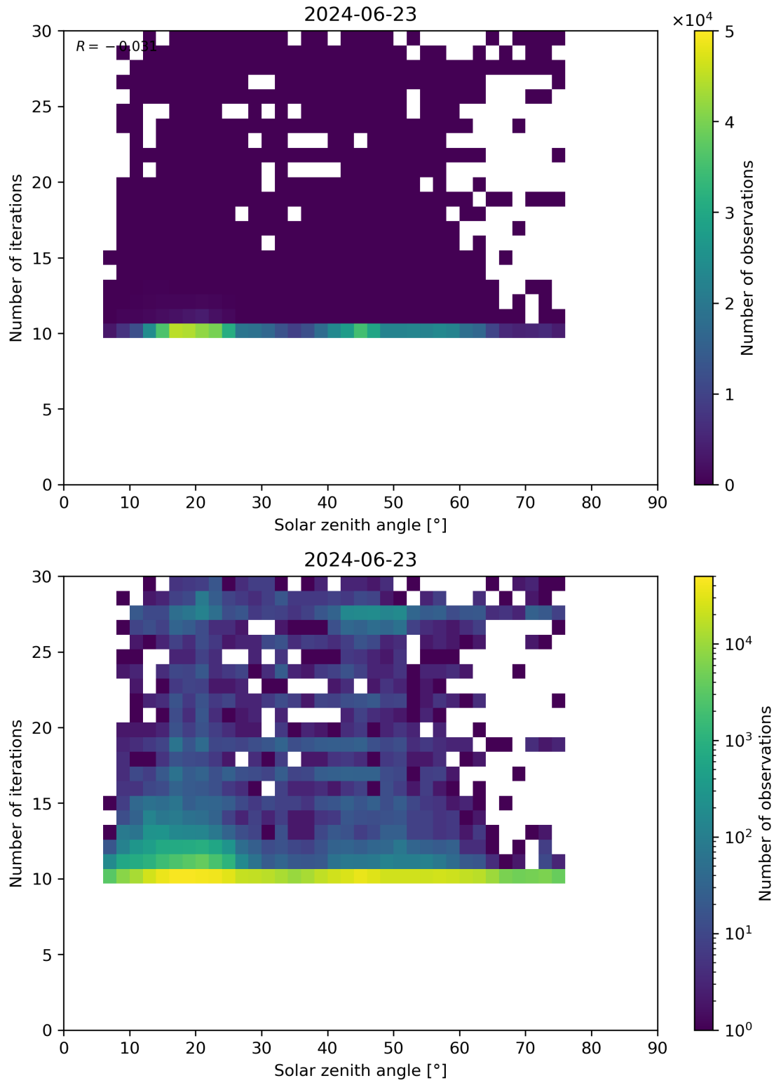
Figure 102: Scatter density plot of “Solar zenith angle” against “Number of iterations” for 2024-06-22 to 2024-06-24.
