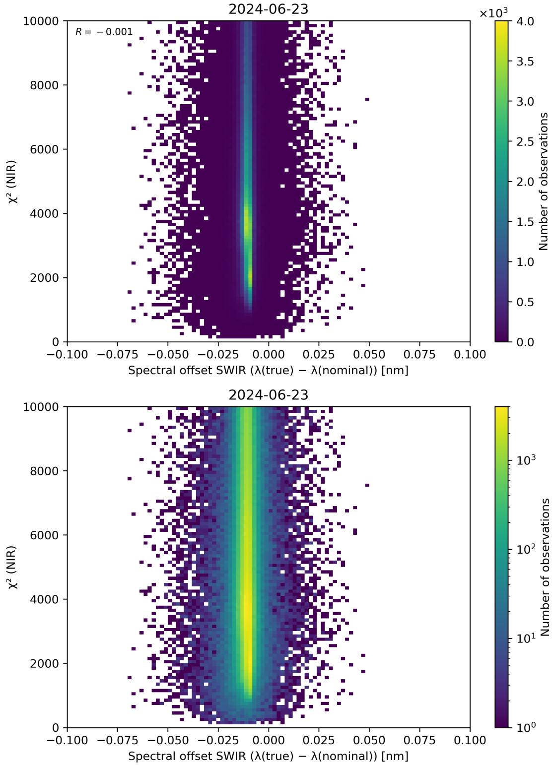
Figure 117: Scatter density plot of “Spectral offset SWIR ( \lambda(\text{true}) - \lambda(\text{nominal}) )” against “ \chi^2 (NIR)” for 2024-06-22 to 2024-06-24.
