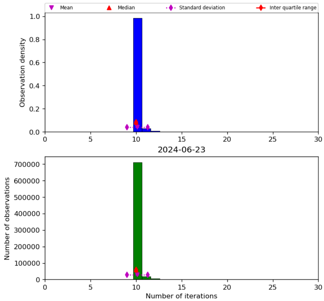
Figure 31: Histogram of “Number of iterations” for 2024-06-22 to 2024-06-24
