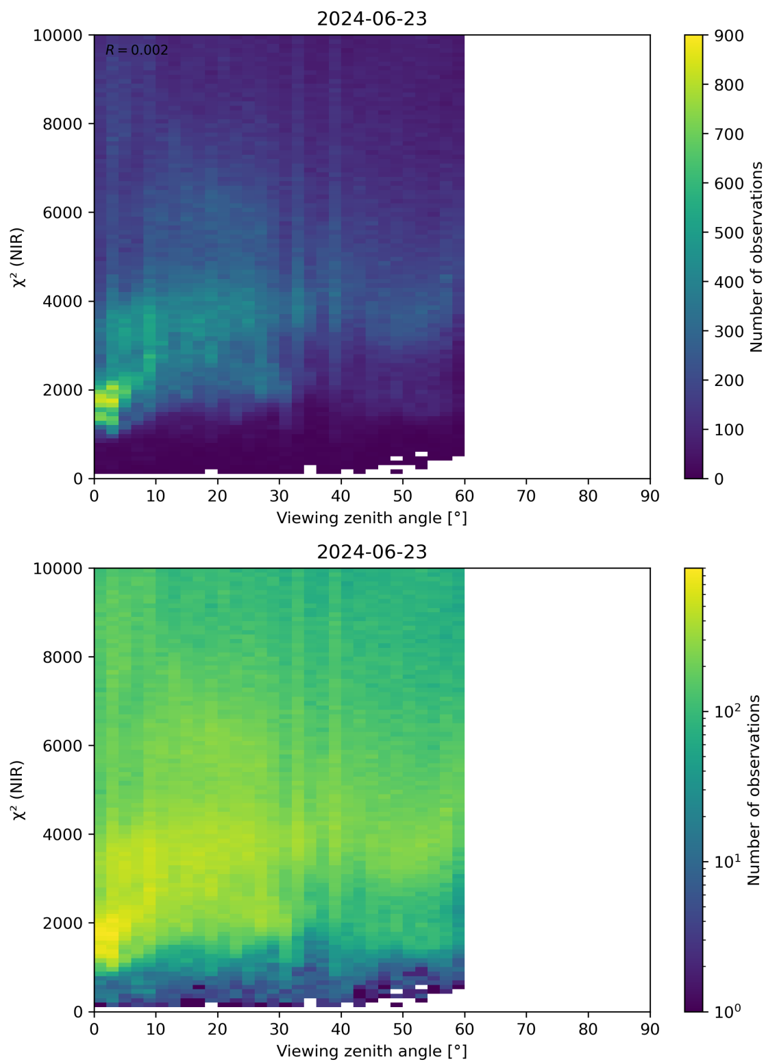
Figure 105: Scatter density plot of “Viewing zenith angle” against “ \chi^2 (NIR)” for 2024-06-22 to 2024-06-24.
