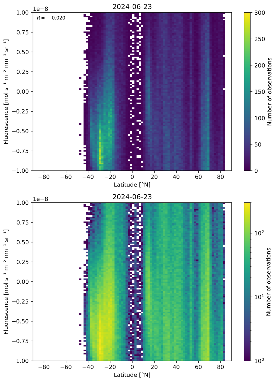
Figure 56: Scatter density plot of “Latitude” against “Fluorescence” for 2024-06-22 to 2024-06-24.
