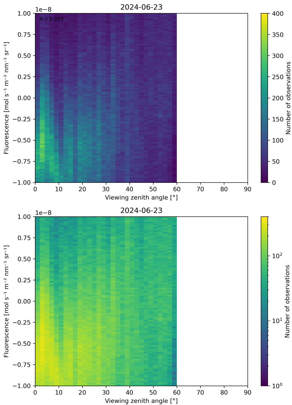
Figure 108: Scatter density plot of “Viewing zenith angle” against “Fluorescence” for 2024-06-22 to 2024-06-24.
