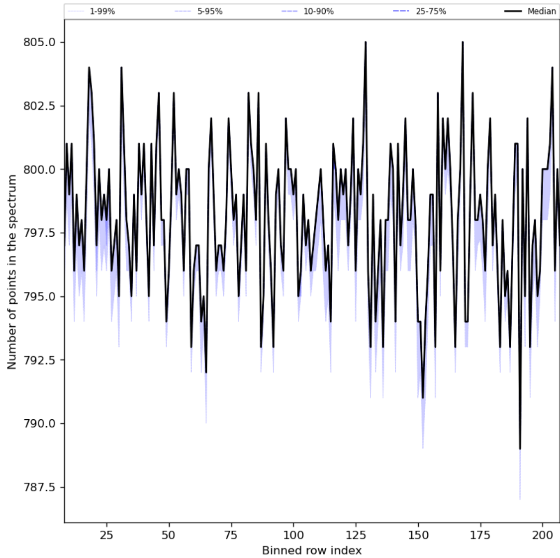
Figure 37: Along track statistics of “Number of points in the spectrum” for 2024-06-22 to 2024-06-24
