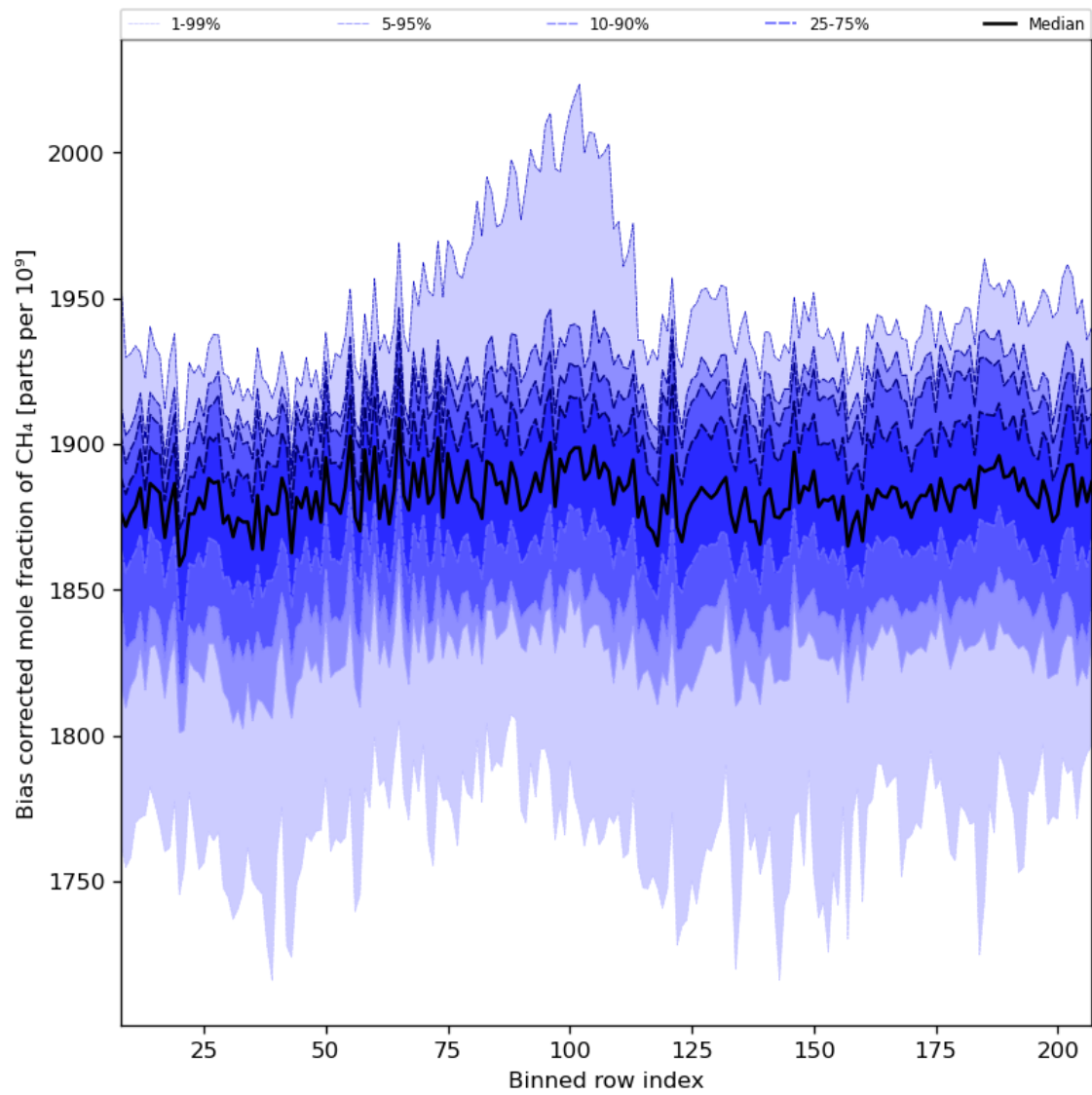
Figure 36: Along track statistics of “Bias corrected mole fraction of CH 4 ” for 2024-06-22 to 2024-06-24
