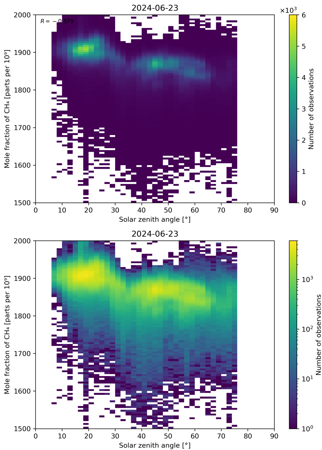
Figure 99: Scatter density plot of “Solar zenith angle” against “Mole fraction of CH 4 ” for 2024-06-22 to 2024-06-24.
