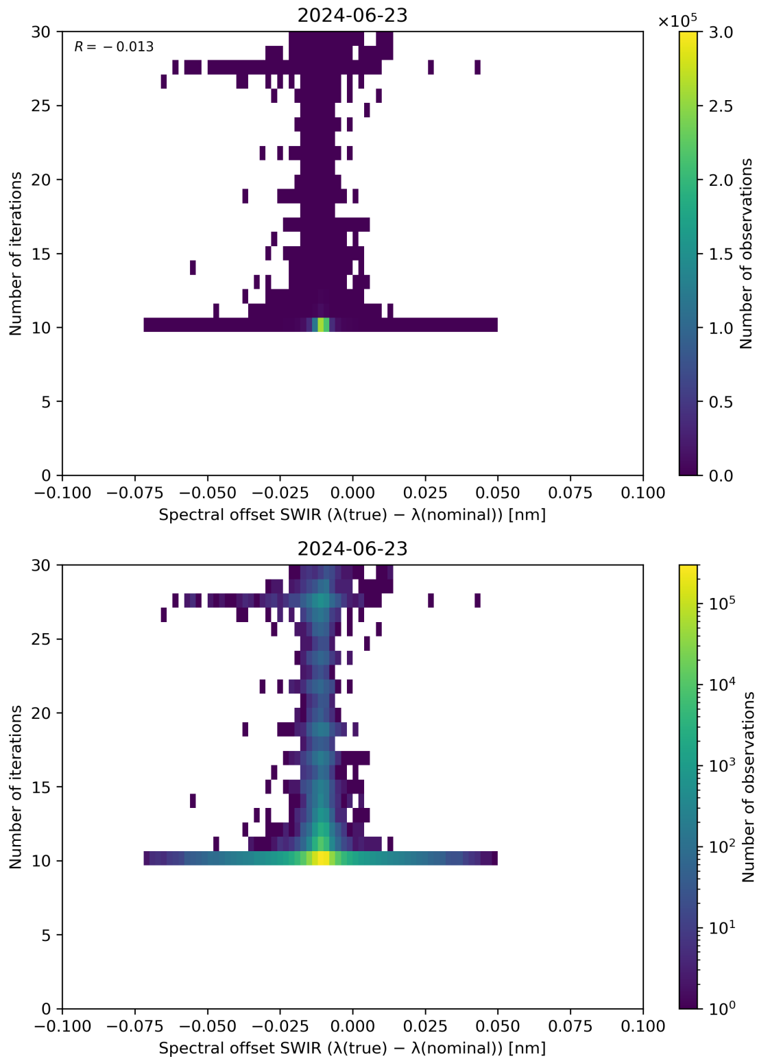
Figure 121: Scatter density plot of “Spectral offset SWIR ( \lambda(\text{true}) - \lambda(\text{nominal}) )” against “Number of iterations” for 2024-06-22 to 2024-06-24.
