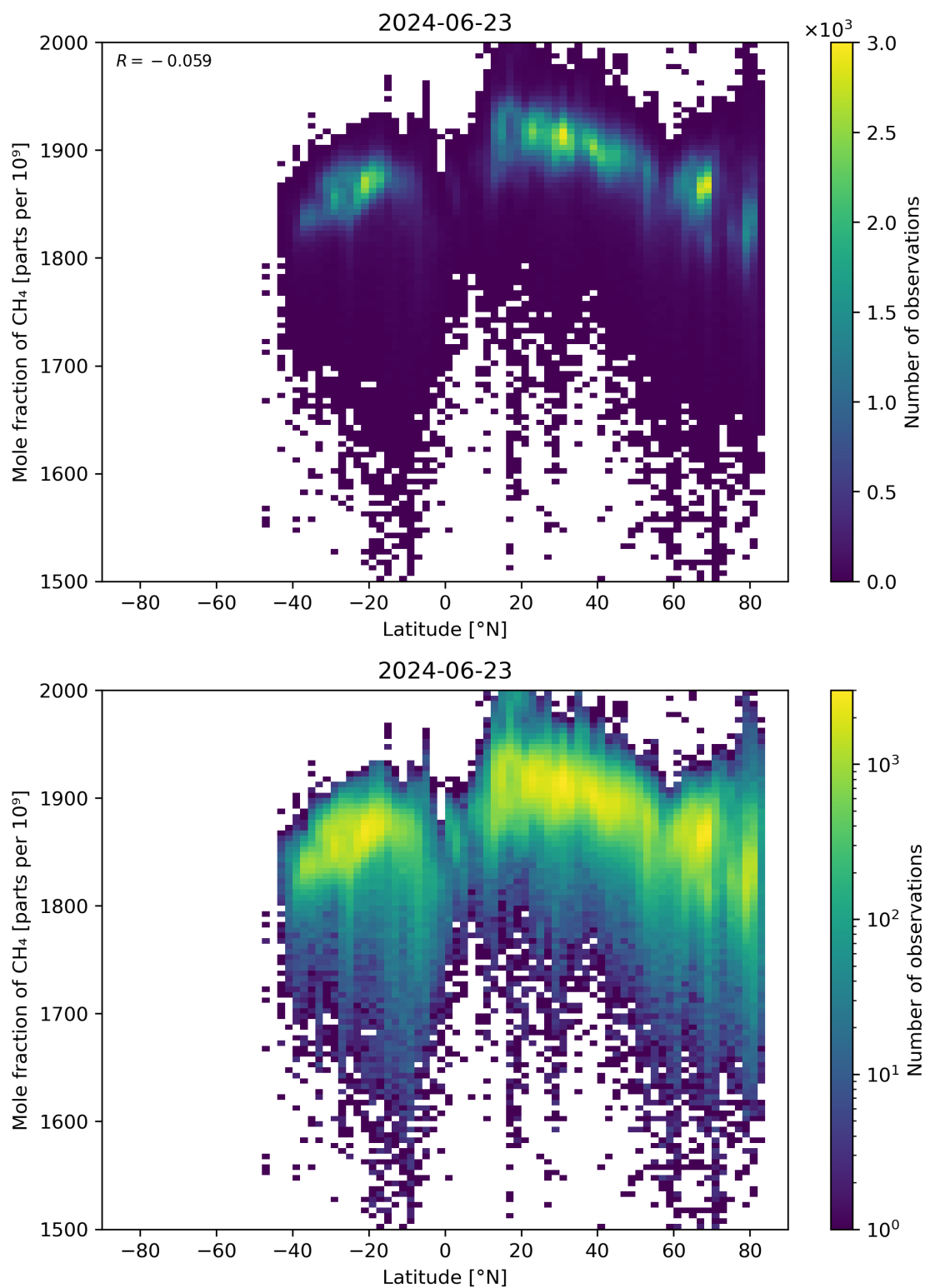
Figure 57: Scatter density plot of “Latitude” against “Mole fraction of \text{CH}_4 ” for 2024-06-22 to 2024-06-24.
