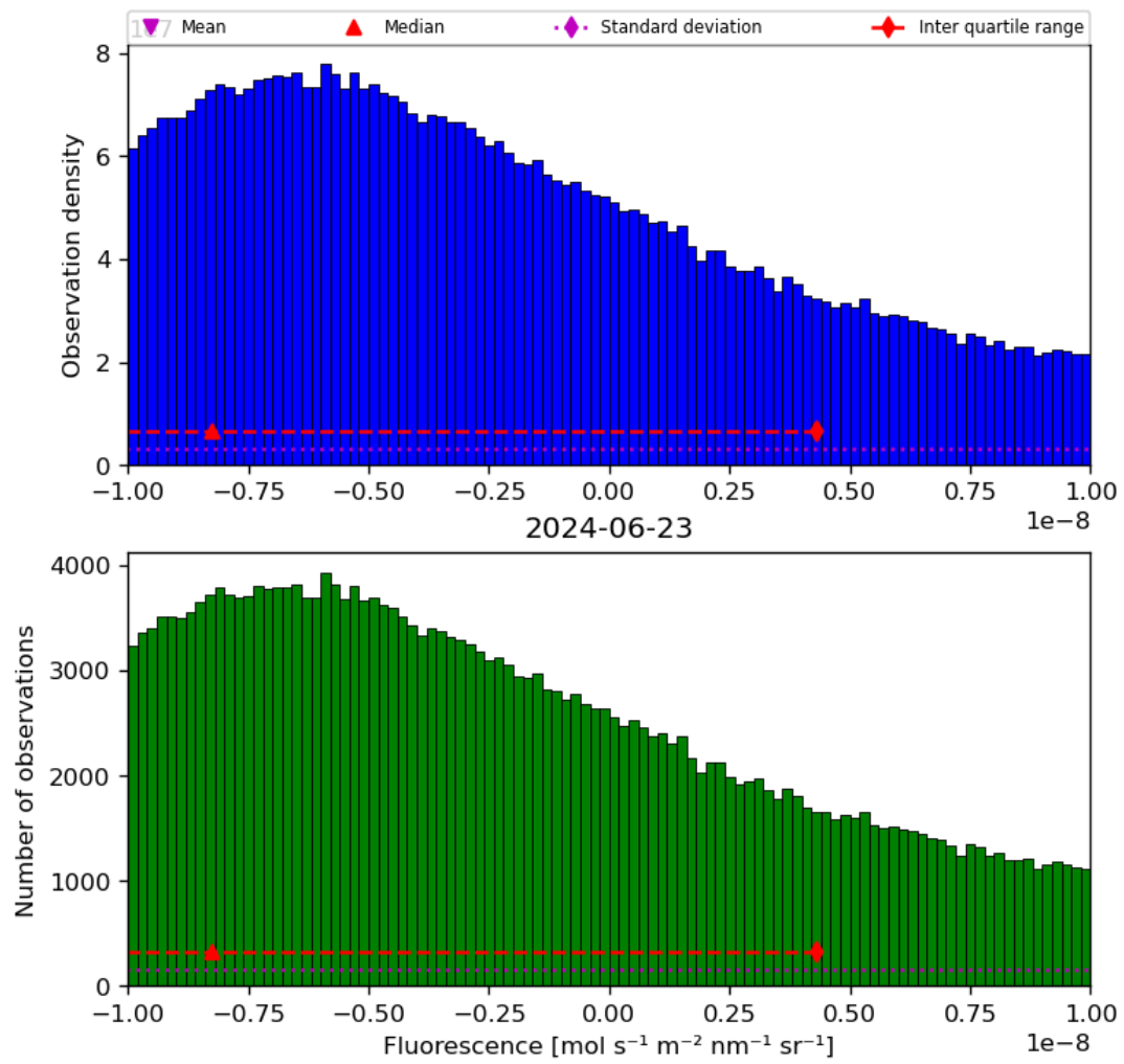
Figure 32: Histogram of “Fluorescence” for 2024-06-22 to 2024-06-24
