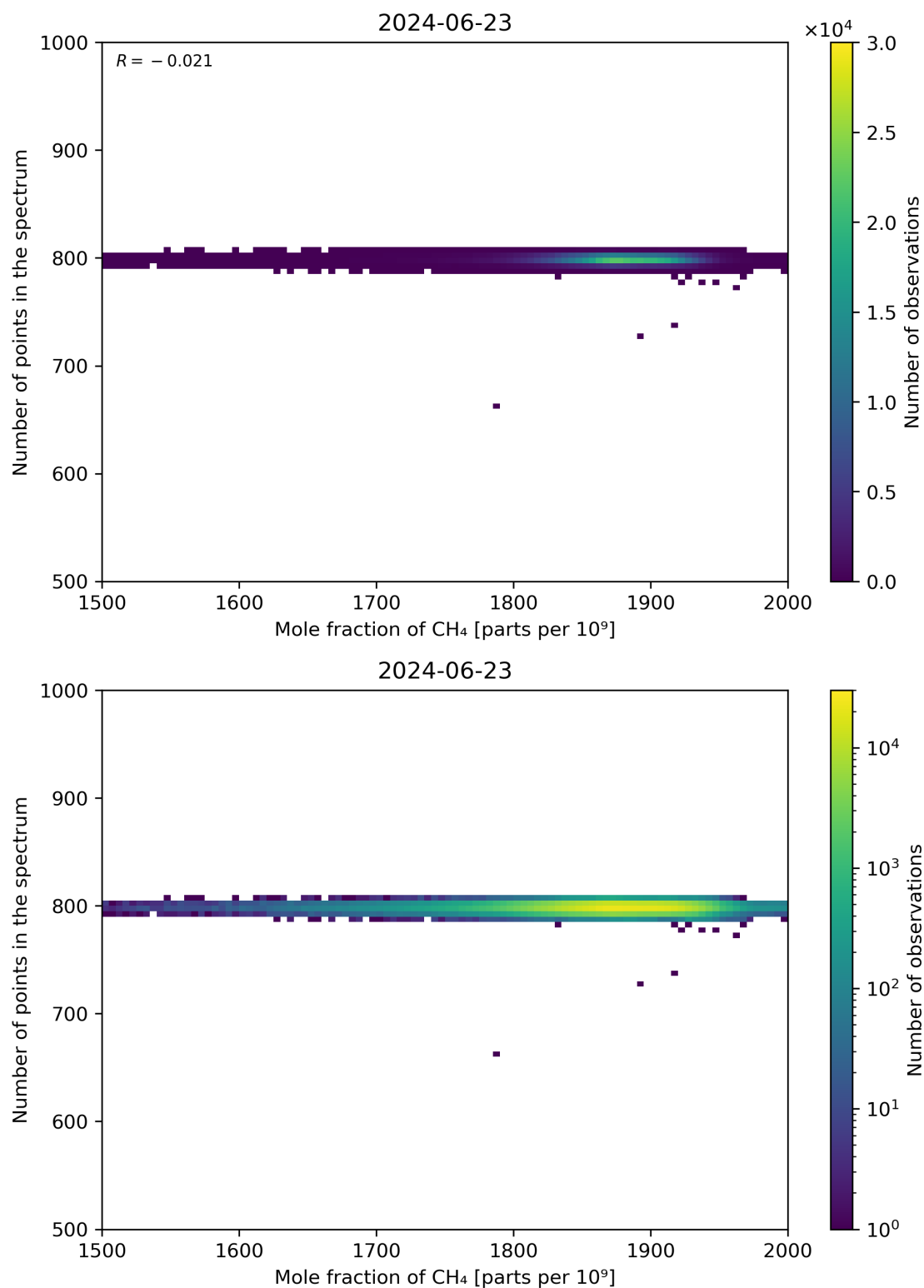
Figure 77: Scatter density plot of “Mole fraction of CH 4 ” against “Number of points in the spectrum” for 2024-06-22 to 2024-06-24.
