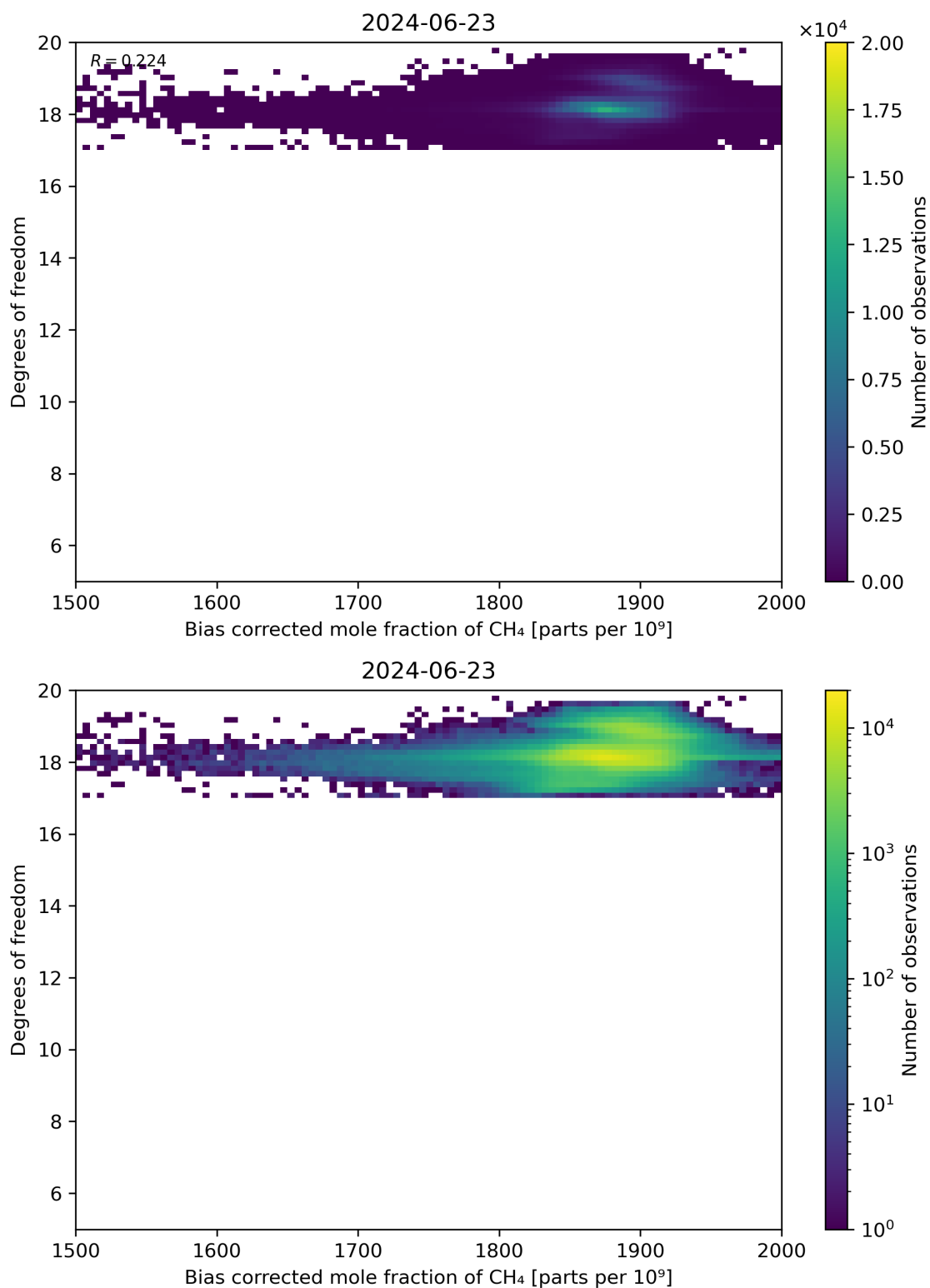
Figure 65: Scatter density plot of “Bias corrected mole fraction of CH 4 ” against “Degrees of freedom” for 2024-06-22 to 2024-06-24.
