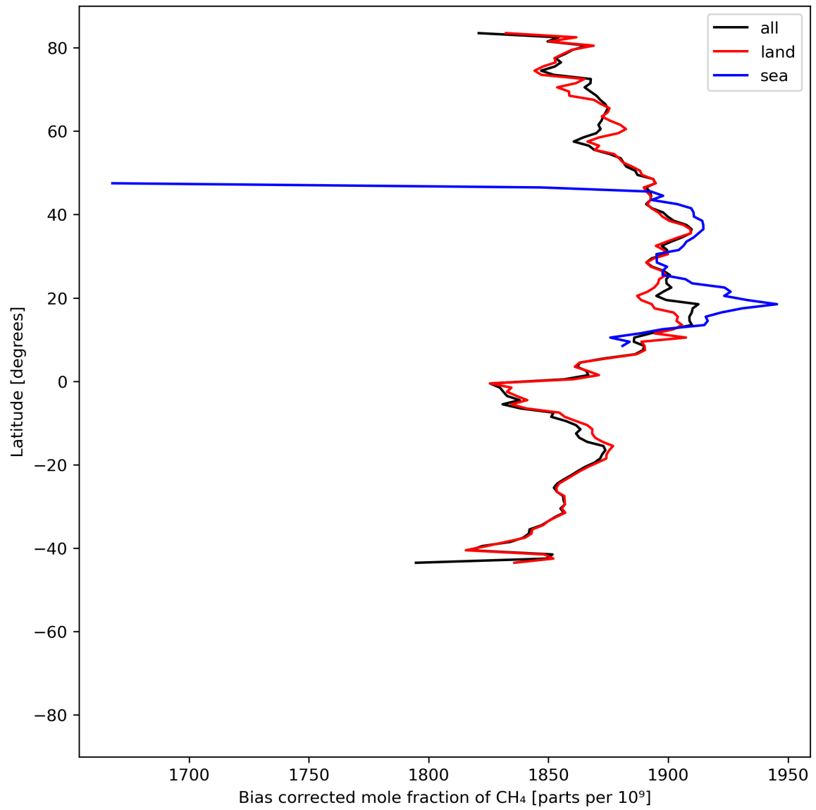
Figure 14: Zonal average of “Bias corrected mole fraction of \text{CH}_4 ” for 2024-06-22 to 2024-06-24.
