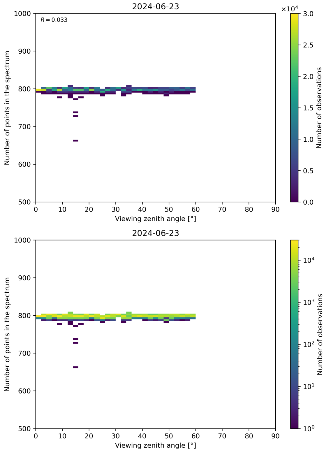
Figure 114: Scatter density plot of “Viewing zenith angle” against “Number of points in the spectrum” for 2024-06-22 to 2024-06-24.
