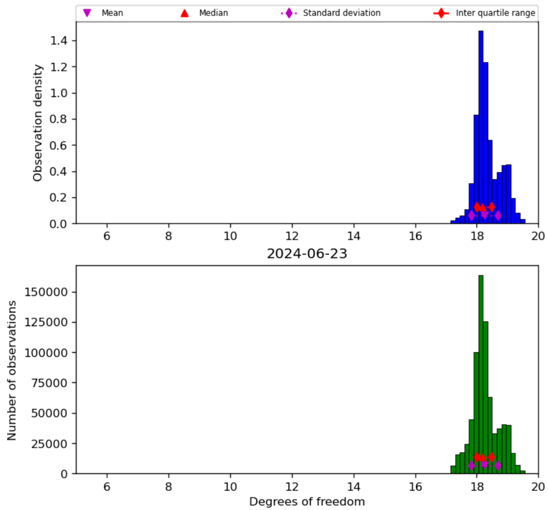
Figure 30: Histogram of “Degrees of freedom” for 2024-06-22 to 2024-06-24
