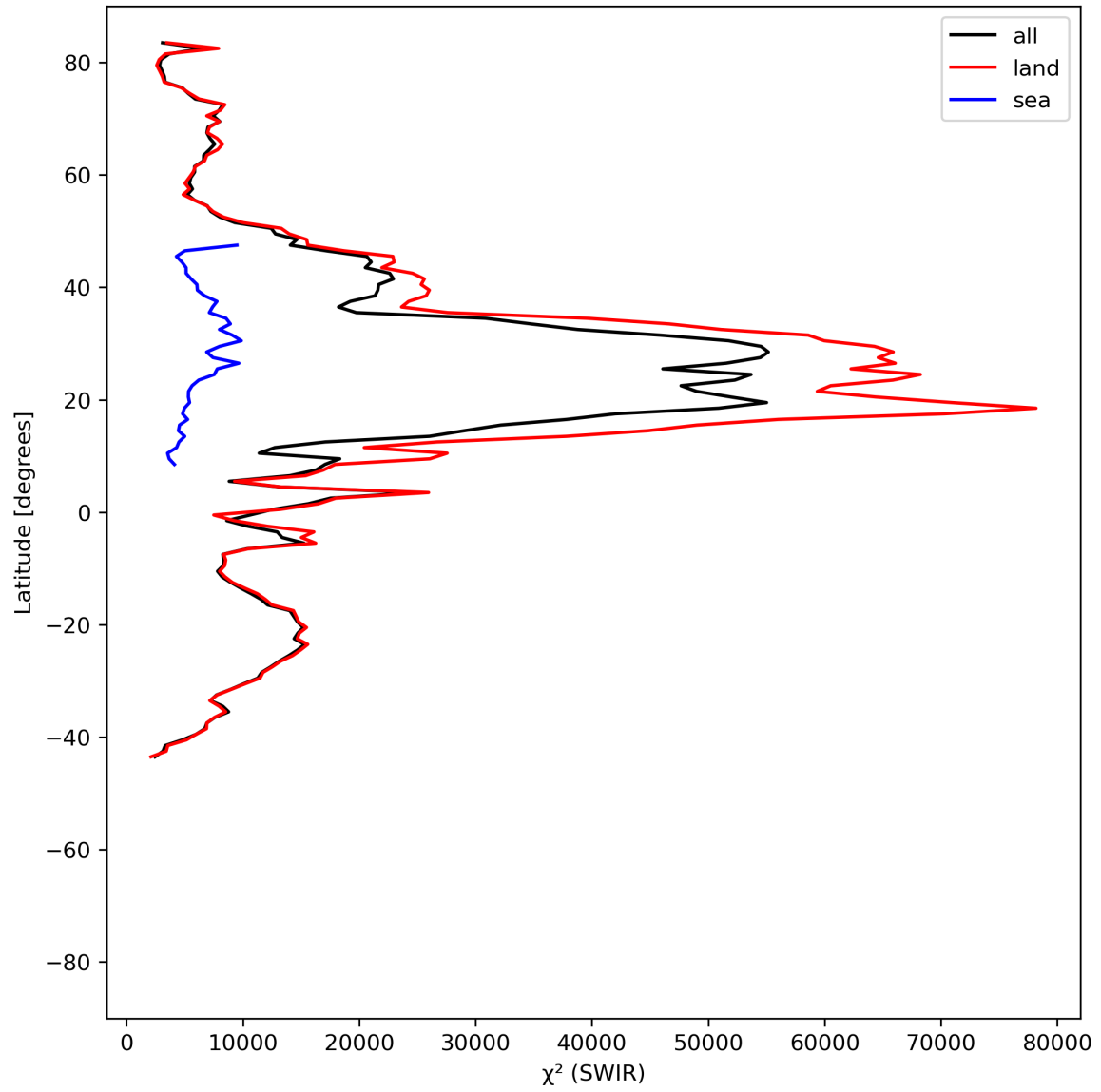
Figure 17: Zonal average of “ \chi^2 (SWIR)” for 2024-06-22 to 2024-06-24.
