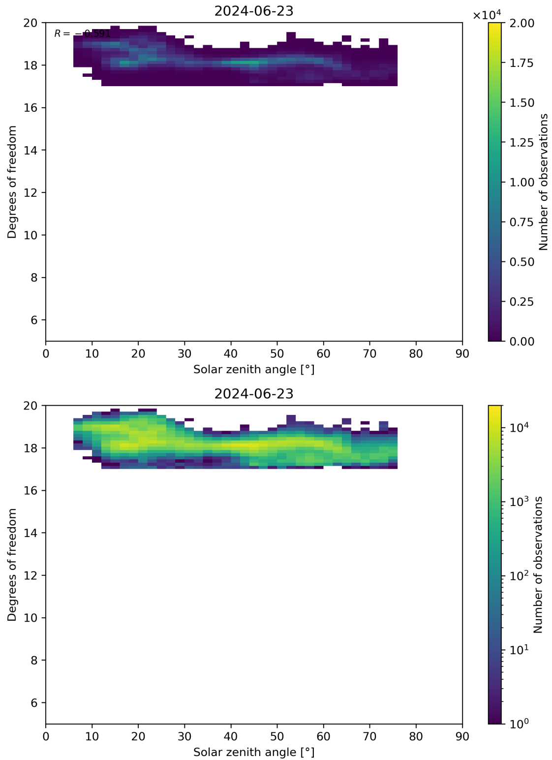
Figure 96: Scatter density plot of “Solar zenith angle” against “Degrees of freedom” for 2024-06-22 to 2024-06-24.
