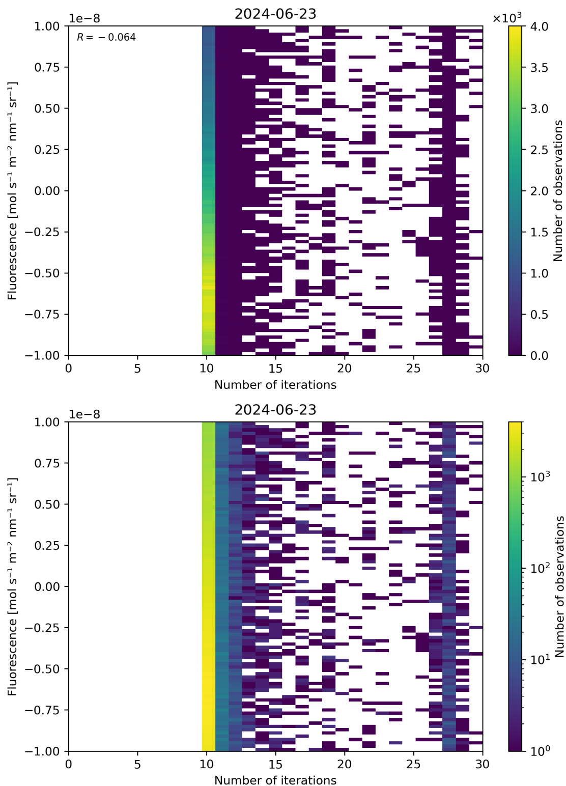
Figure 87: Scatter density plot of “Number of iterations” against “Fluorescence” for 2024-06-22 to 2024-06-24.
