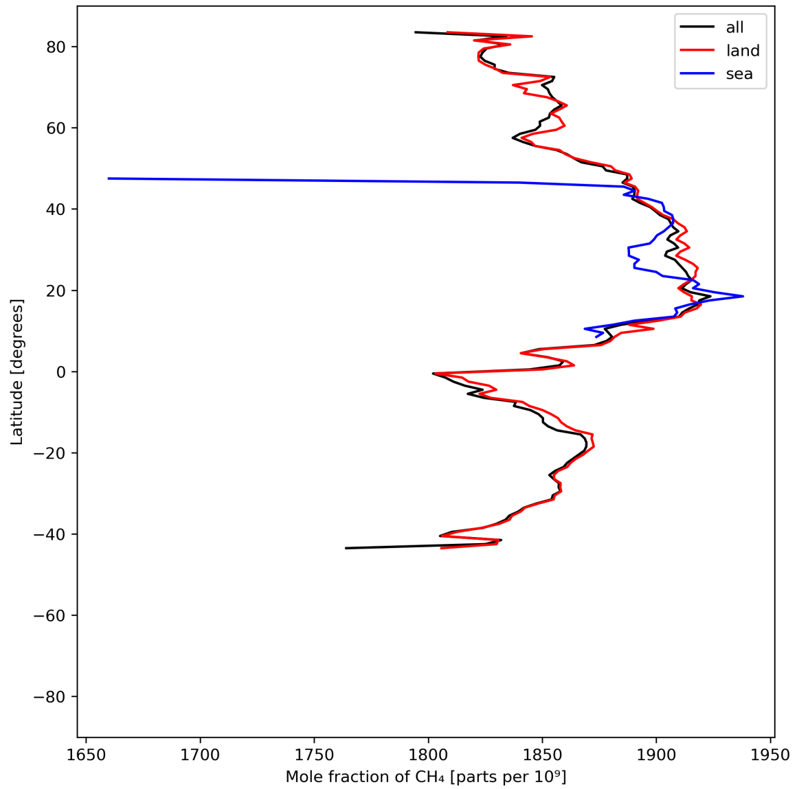
Figure 12: Zonal average of “Mole fraction of \text{CH}_4 ” for 2024-06-22 to 2024-06-24.
