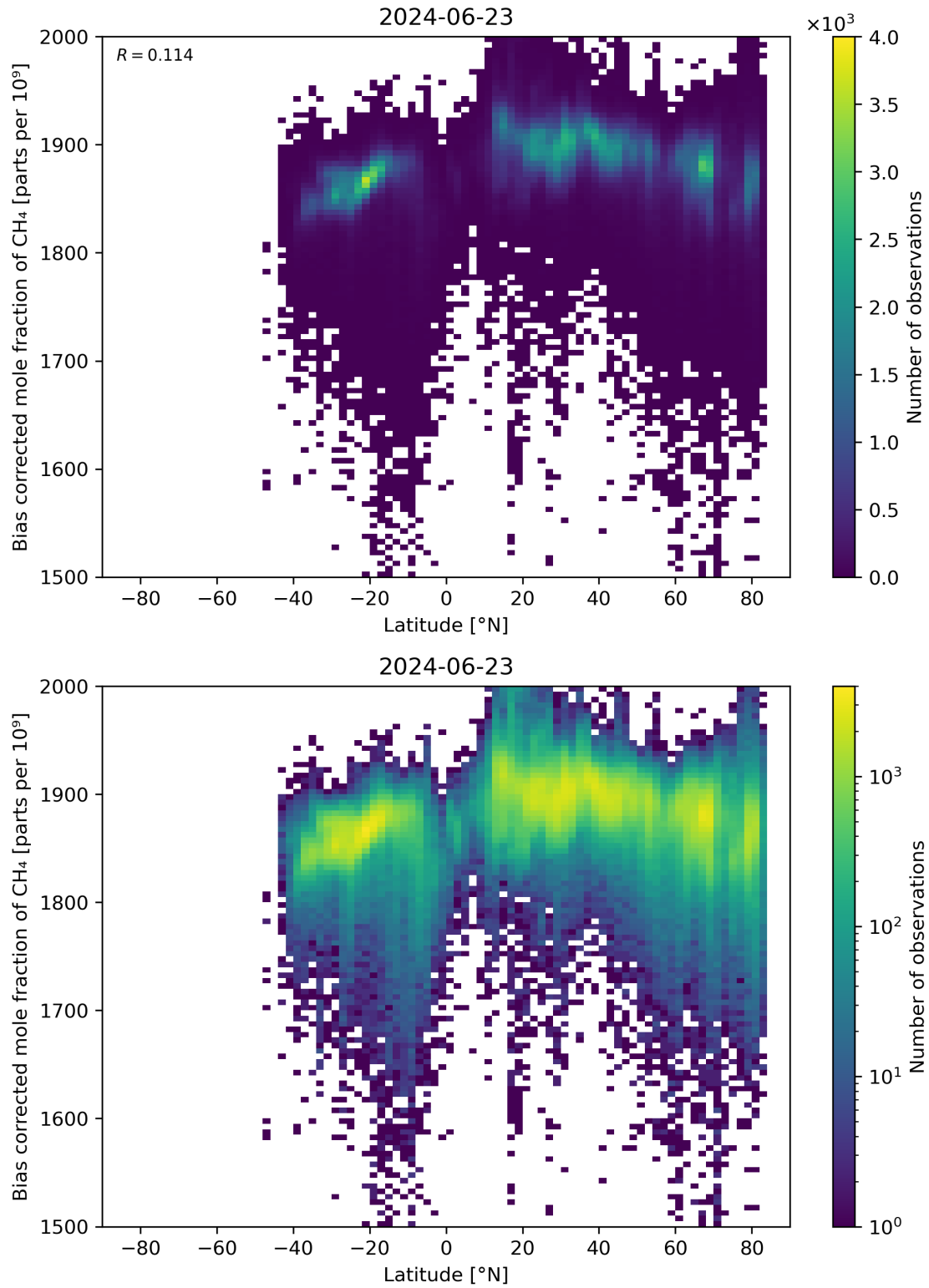
Figure 58: Scatter density plot of “Latitude” against “Bias corrected mole fraction of \text{CH}_4 ” for 2024-06-22 to 2024-06-24.
