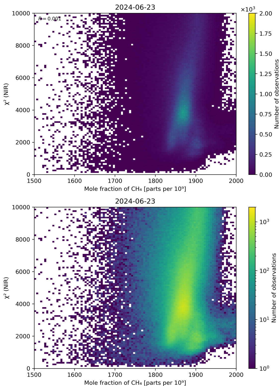
Figure 70: Scatter density plot of “Mole fraction of \text{CH}_4 ” against “ \chi^2 (NIR)” for 2024-06-22 to 2024-06-24.
