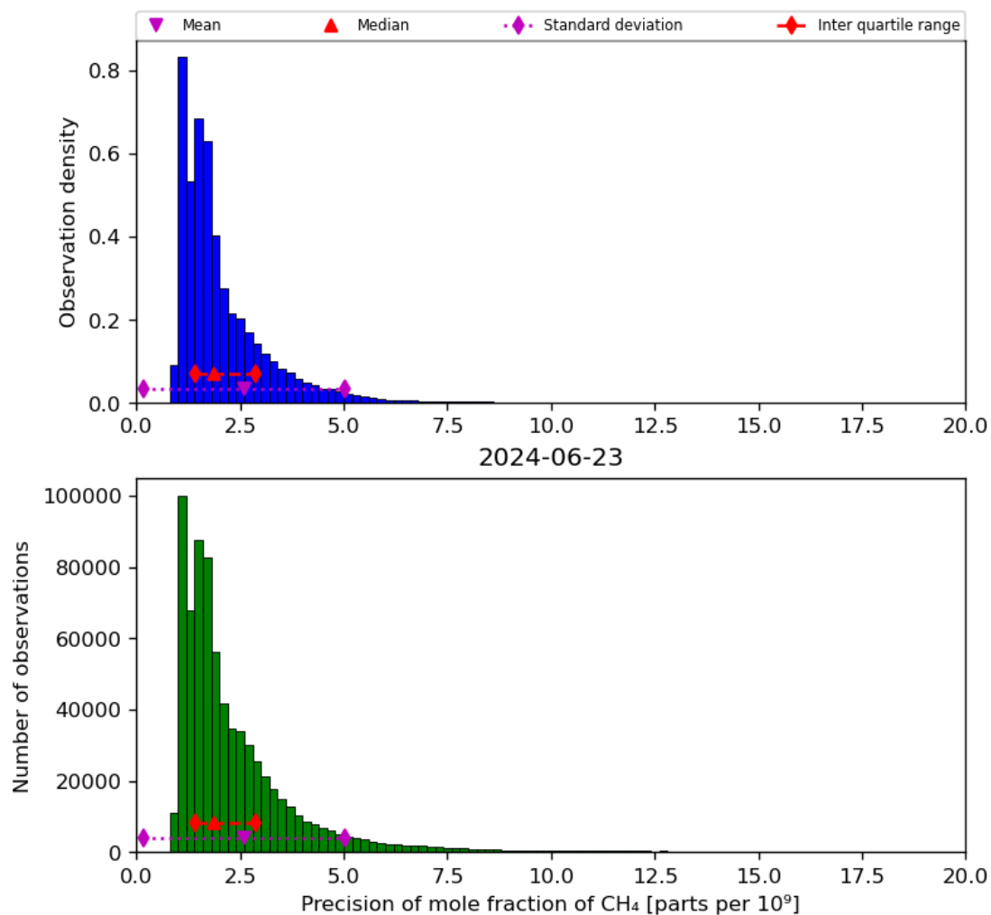
Figure 24: Histogram of “Precision of mole fraction of CH 4 ” for 2024-06-22 to 2024-06-24
