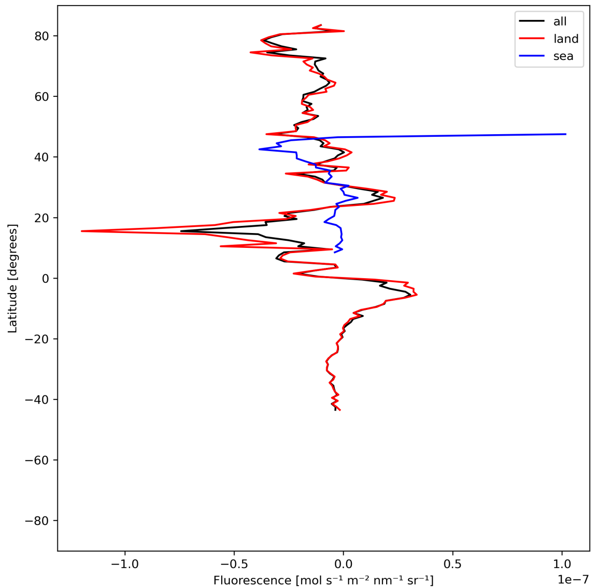
Figure 21: Zonal average of “Fluorescence” for 2024-06-22 to 2024-06-24.
