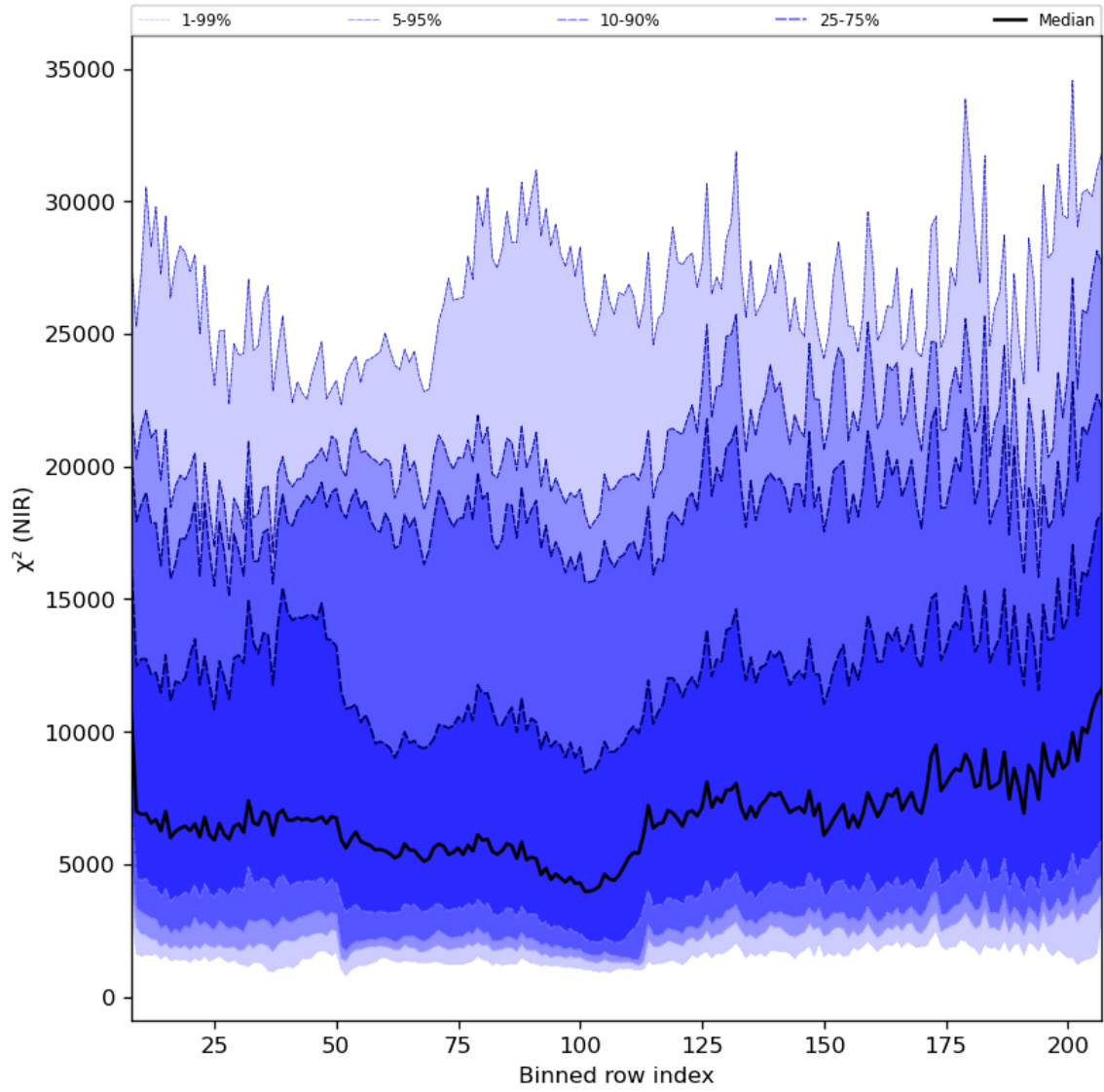
Figure 40: Along track statistics of “ \chi^2 (NIR)” for 2024-06-22 to 2024-06-24
