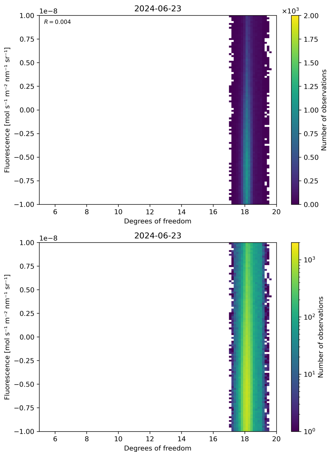
Figure 51: Scatter density plot of “Degrees of freedom” against “Fluorescence” for 2024-06-22 to 2024-06-24.
