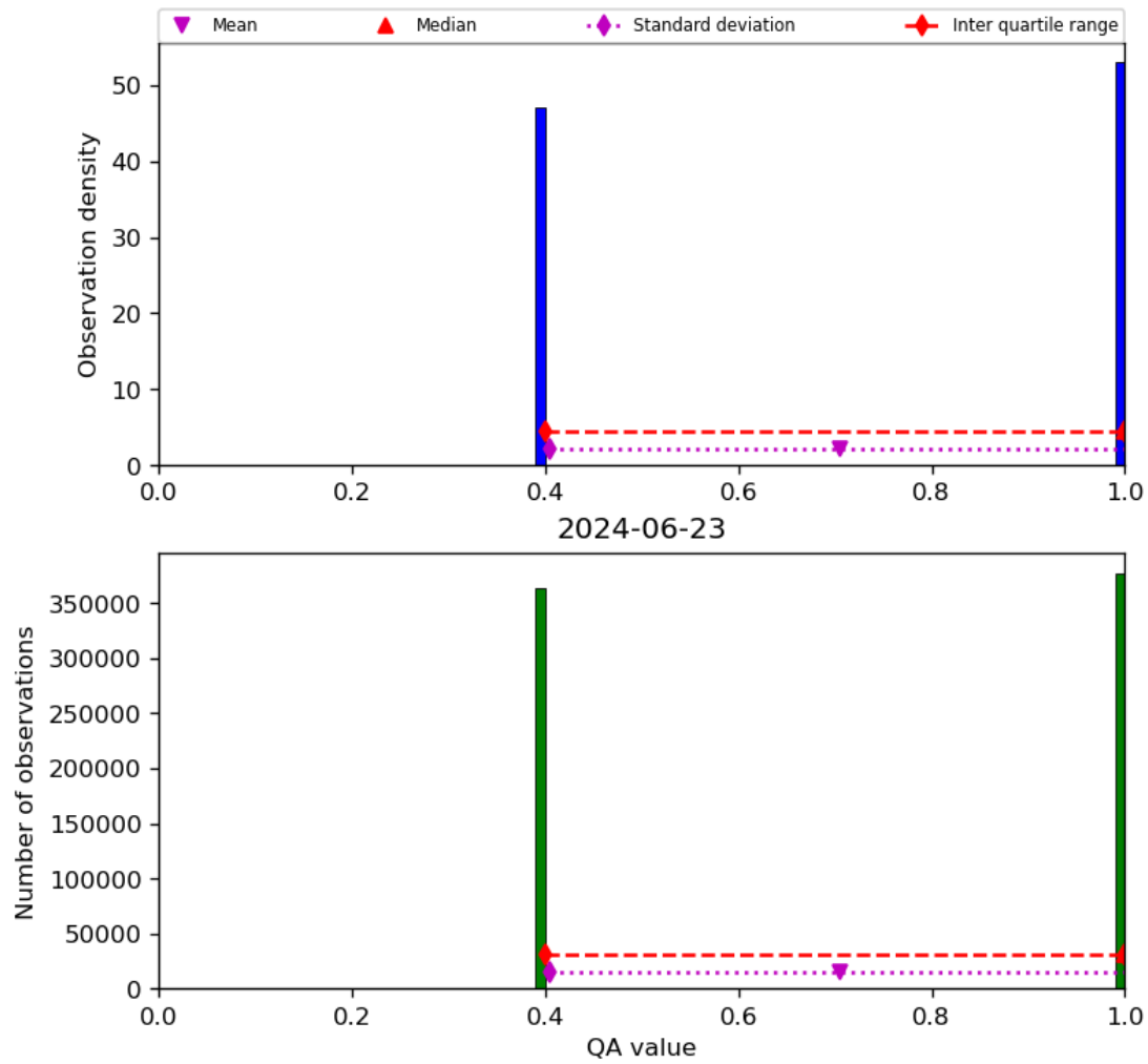
Figure 22: Histogram of “QA value” for 2024-06-22 to 2024-06-24
