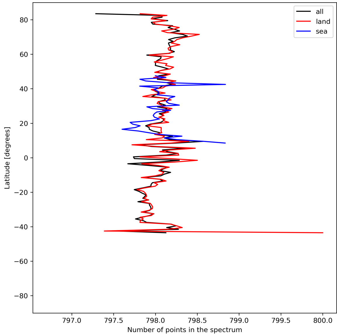
Figure 15: Zonal average of “Number of points in the spectrum” for 2024-06-22 to 2024-06-24.
