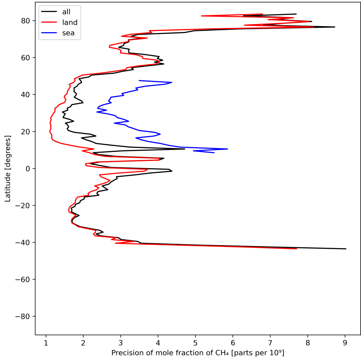
Figure 13: Zonal average of “Precision of mole fraction of CH 4 ” for 2024-06-22 to 2024-06-24.
