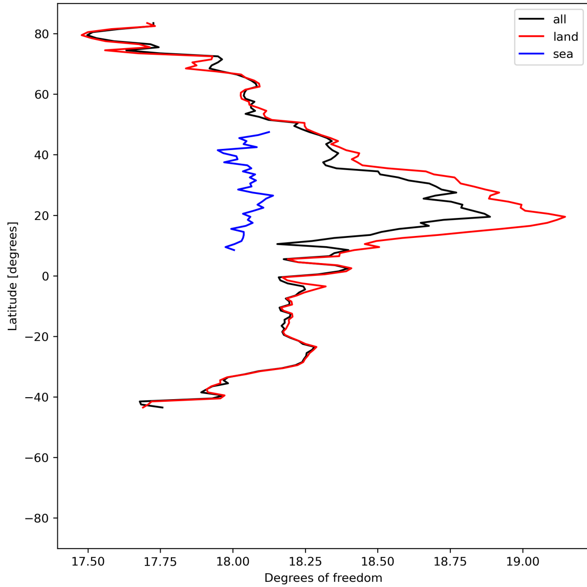
Figure 19: Zonal average of “Degrees of freedom” for 2024-06-22 to 2024-06-24.
