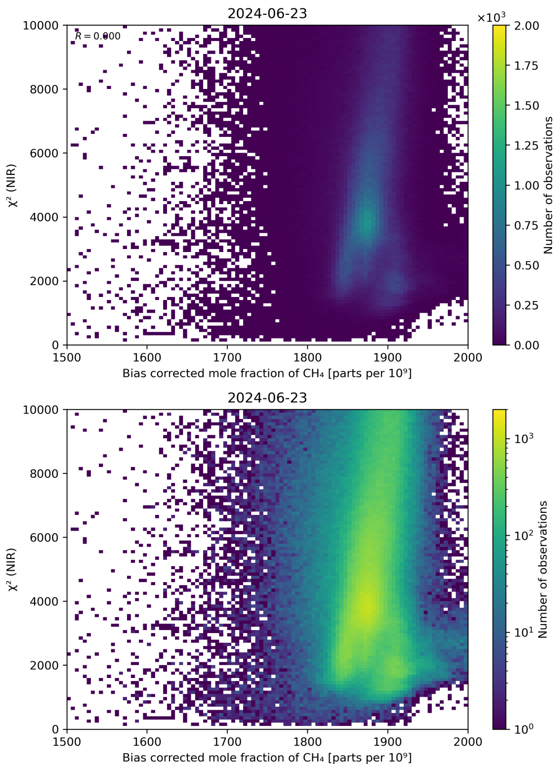
Figure 63: Scatter density plot of “Bias corrected mole fraction of \text{CH}_4 ” against “ \chi^2 (NIR)” for 2024-06-22 to 2024-06-24.
