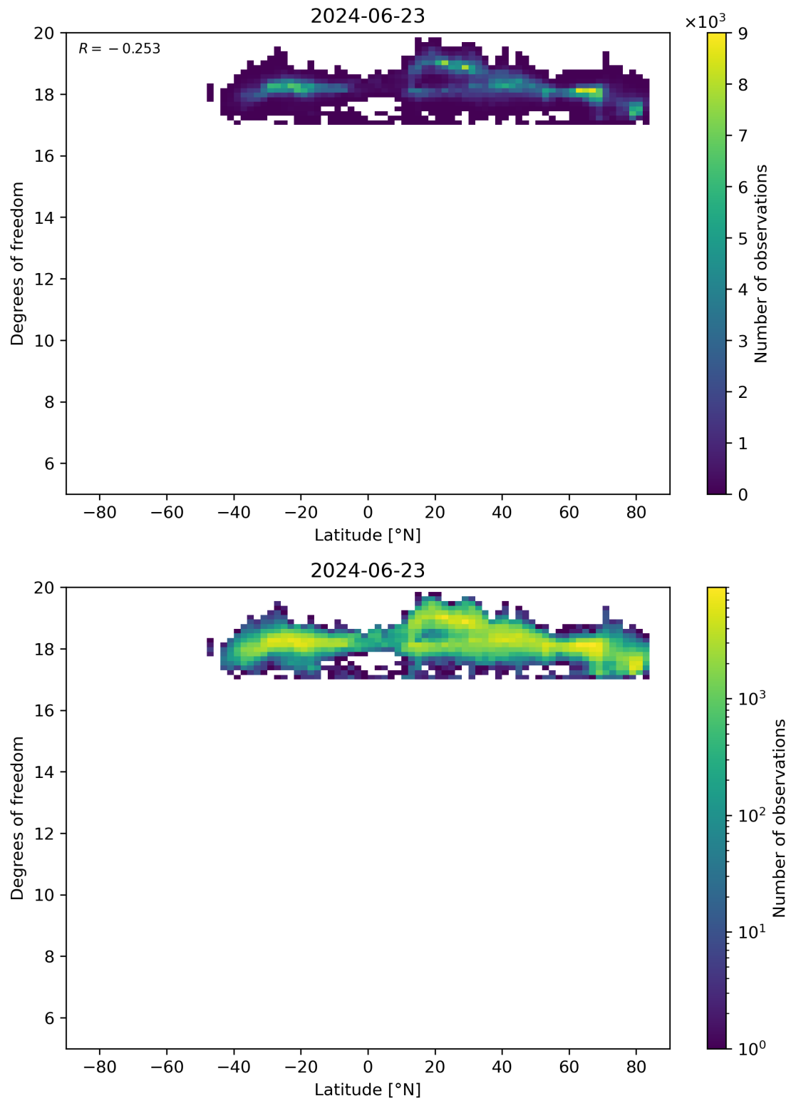
Figure 55: Scatter density plot of “Latitude” against “Degrees of freedom” for 2024-06-22 to 2024-06-24.
