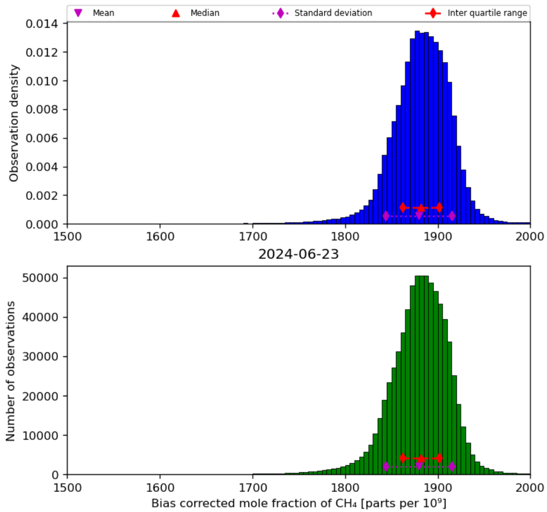
Figure 25: Histogram of “Bias corrected mole fraction of CH 4 ” for 2024-06-22 to 2024-06-24
