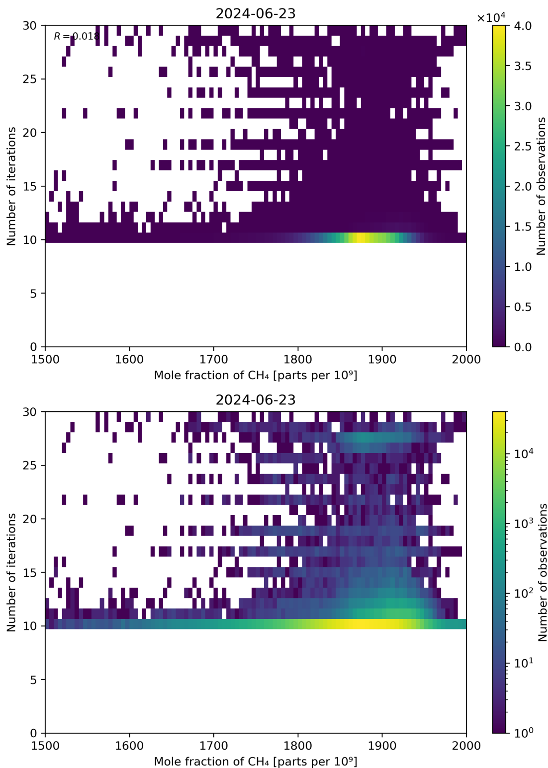
Figure 76: Scatter density plot of “Mole fraction of CH 4 ” against “Number of iterations” for 2024-06-22 to 2024-06-24.
