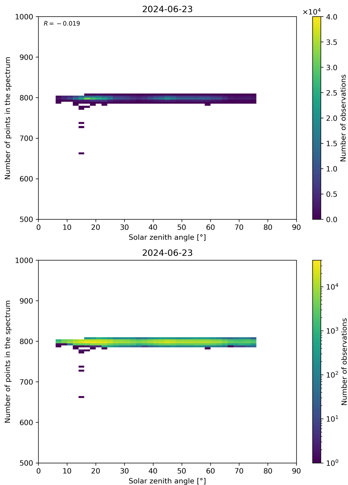
Figure 103: Scatter density plot of “Solar zenith angle” against “Number of points in the spectrum” for 2024-06-22 to 2024-06-24.
