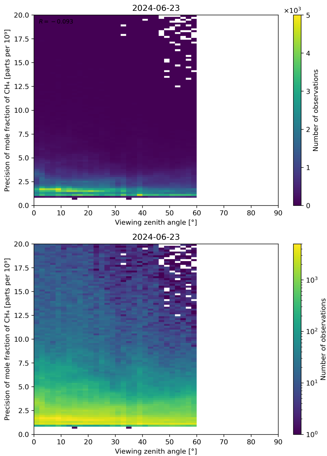
Figure 112: Scatter density plot of “Viewing zenith angle” against “Precision of mole fraction of CH 4 ” for 2024-06-22 to 2024-06-24.
