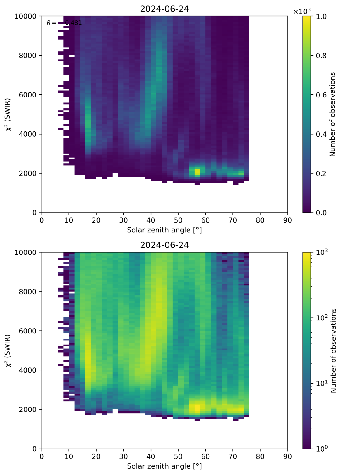
Figure 95: Scatter density plot of “Solar zenith angle” against “ \chi^2 (SWIR)” for 2024-06-24 to 2024-06-25.
