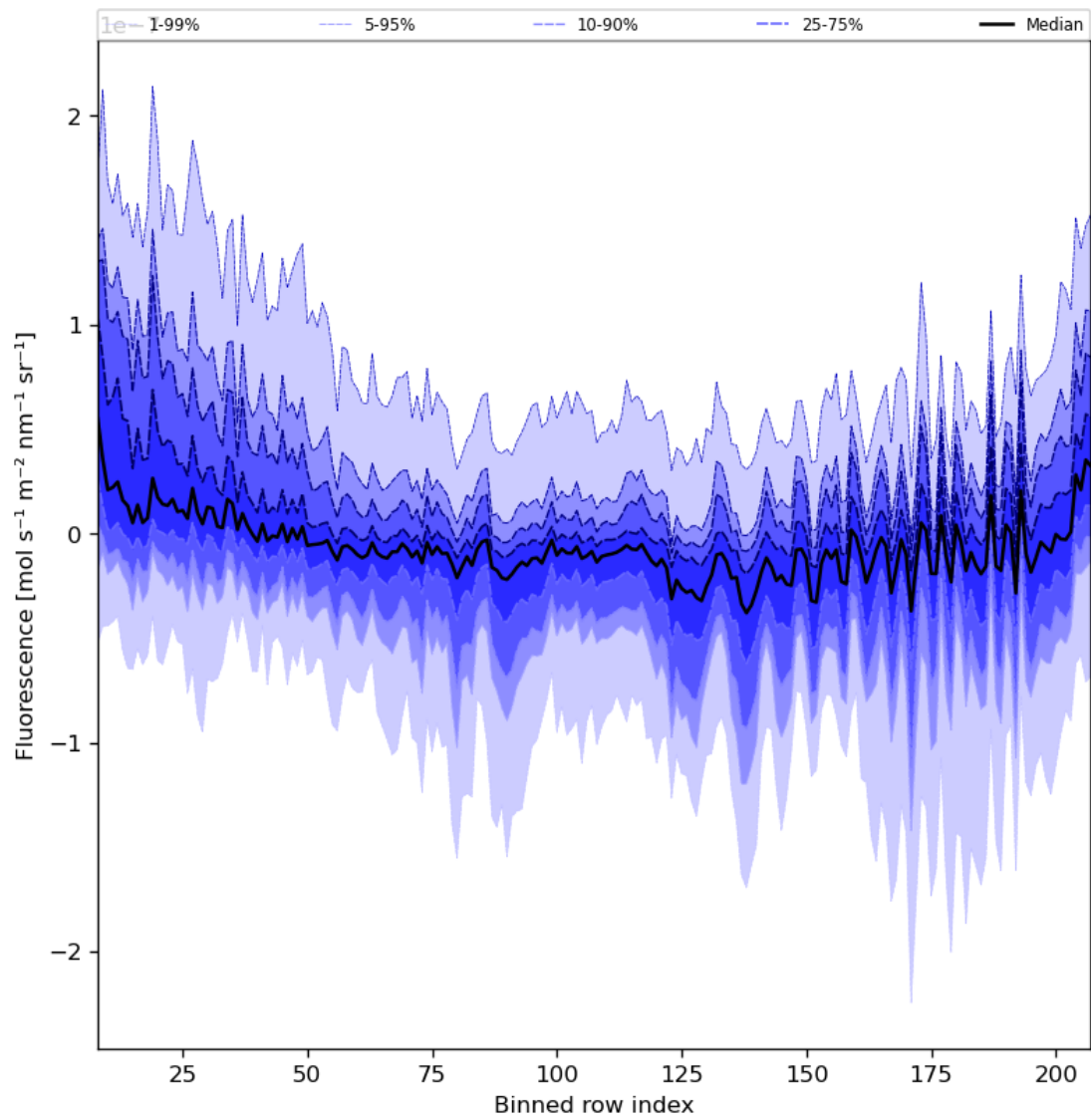
Figure 43: Along track statistics of “Fluorescence” for 2024-06-24 to 2024-06-25
