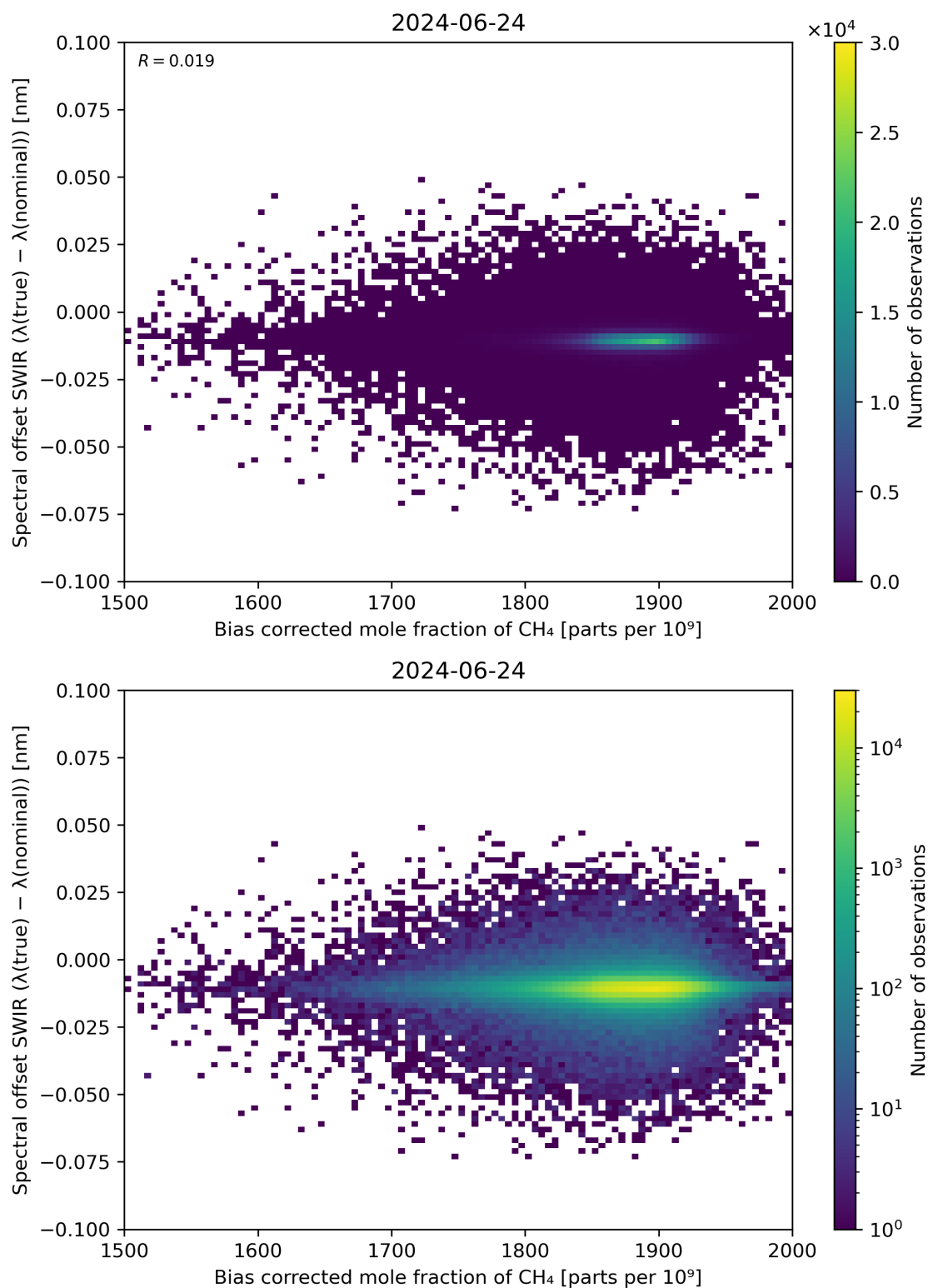
Figure 69: Scatter density plot of “Bias corrected mole fraction of \text{CH}_4 ” against “Spectral offset SWIR ( \lambda(\text{true}) - \lambda(\text{nominal}) )” for 2024-06-24 to 2024-06-25.
