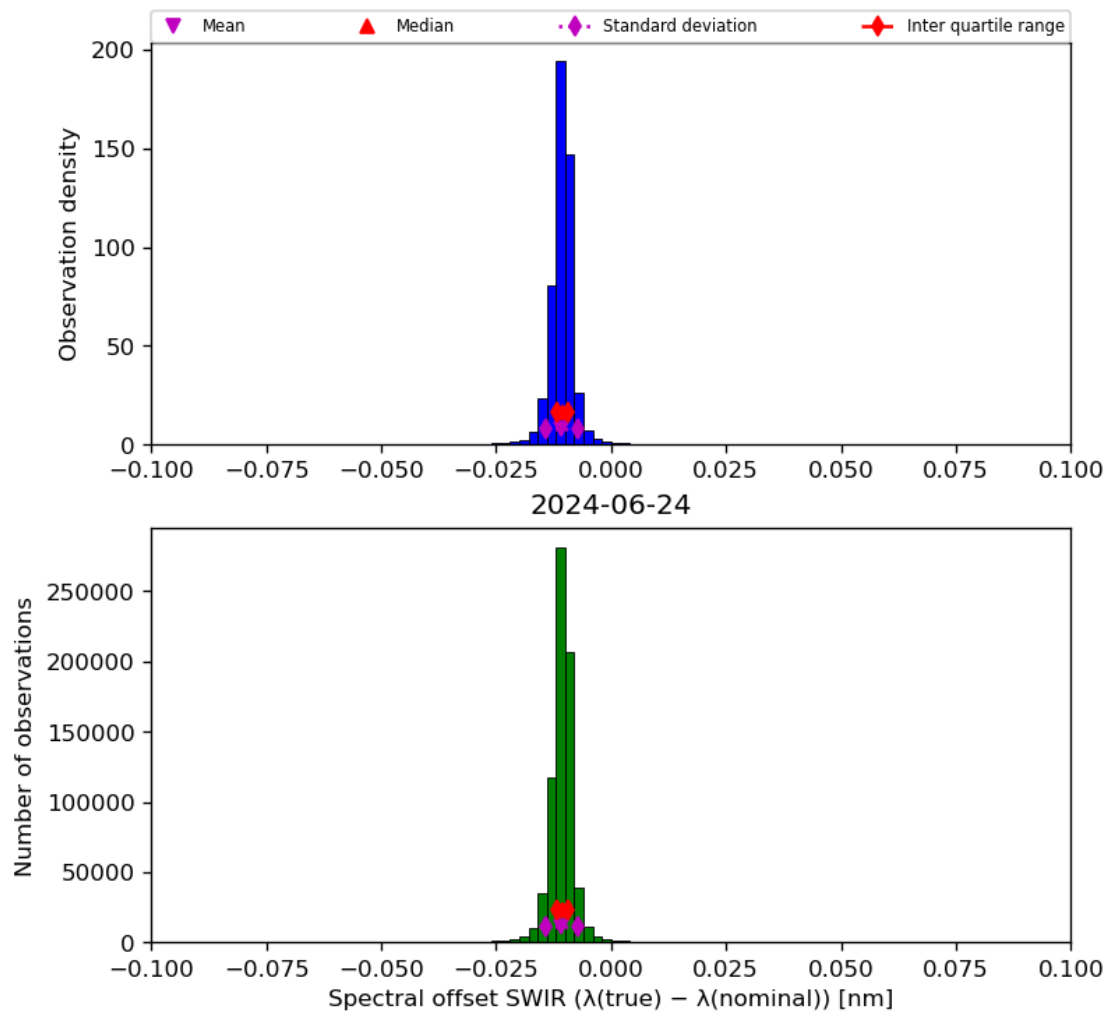
Figure 27: Histogram of “Spectral offset SWIR ( \lambda(\text{true}) - \lambda(\text{nominal}) )” for 2024-06-24 to 2024-06-25
