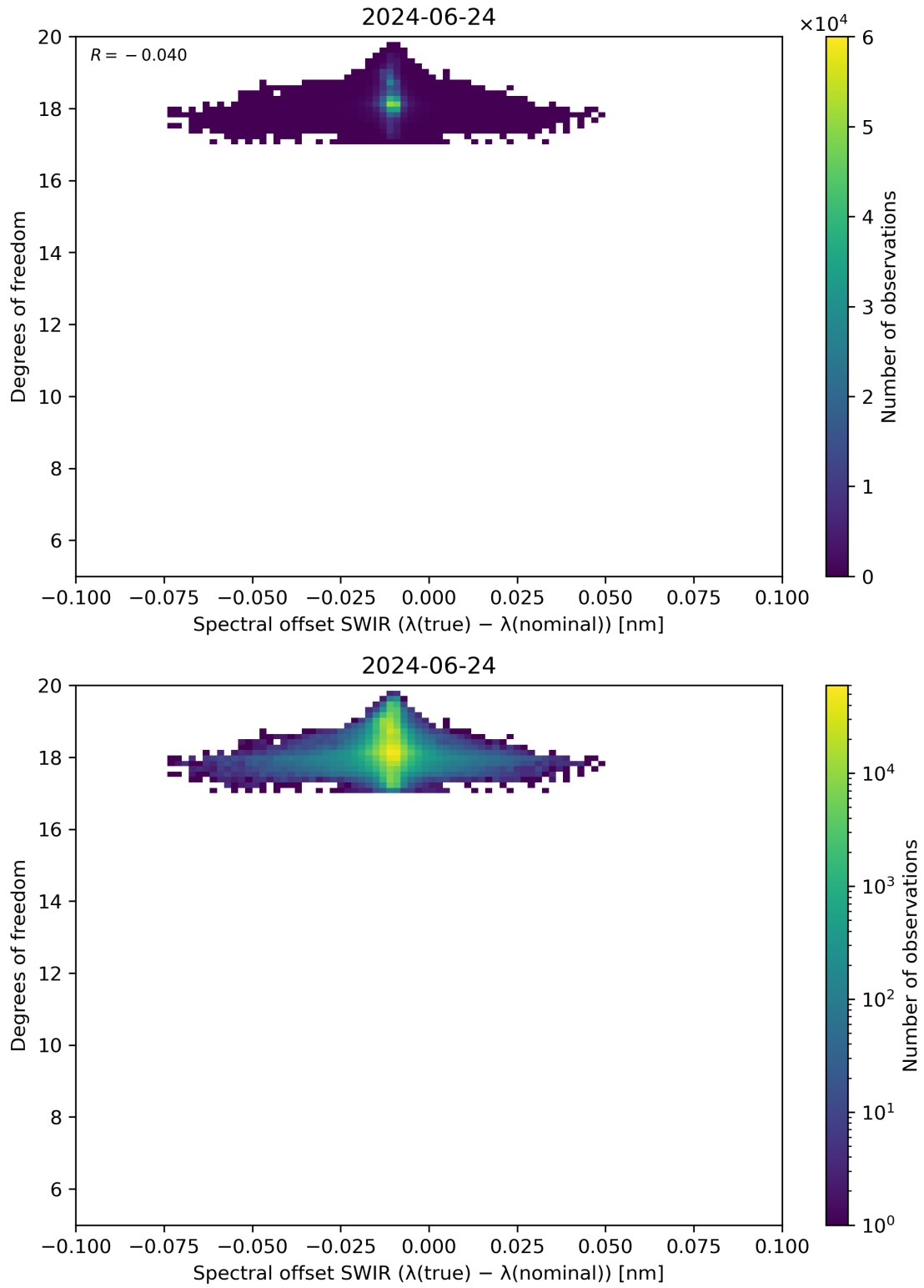
Figure 119: Scatter density plot of “Spectral offset SWIR ( \lambda(\text{true}) - \lambda(\text{nominal}) )” against “Degrees of freedom” for 2024-06-24 to 2024-06-25.
