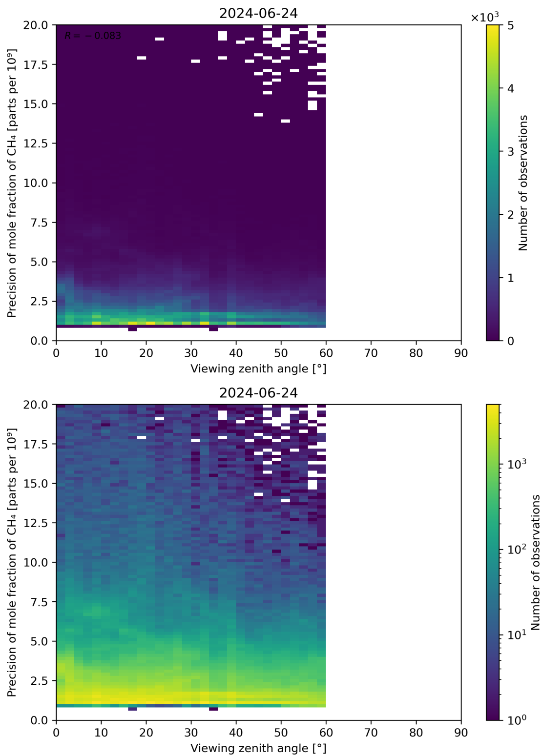
Figure 112: Scatter density plot of “Viewing zenith angle” against “Precision of mole fraction of \text{CH}_4 ” for 2024-06-24 to 2024-06-25.
