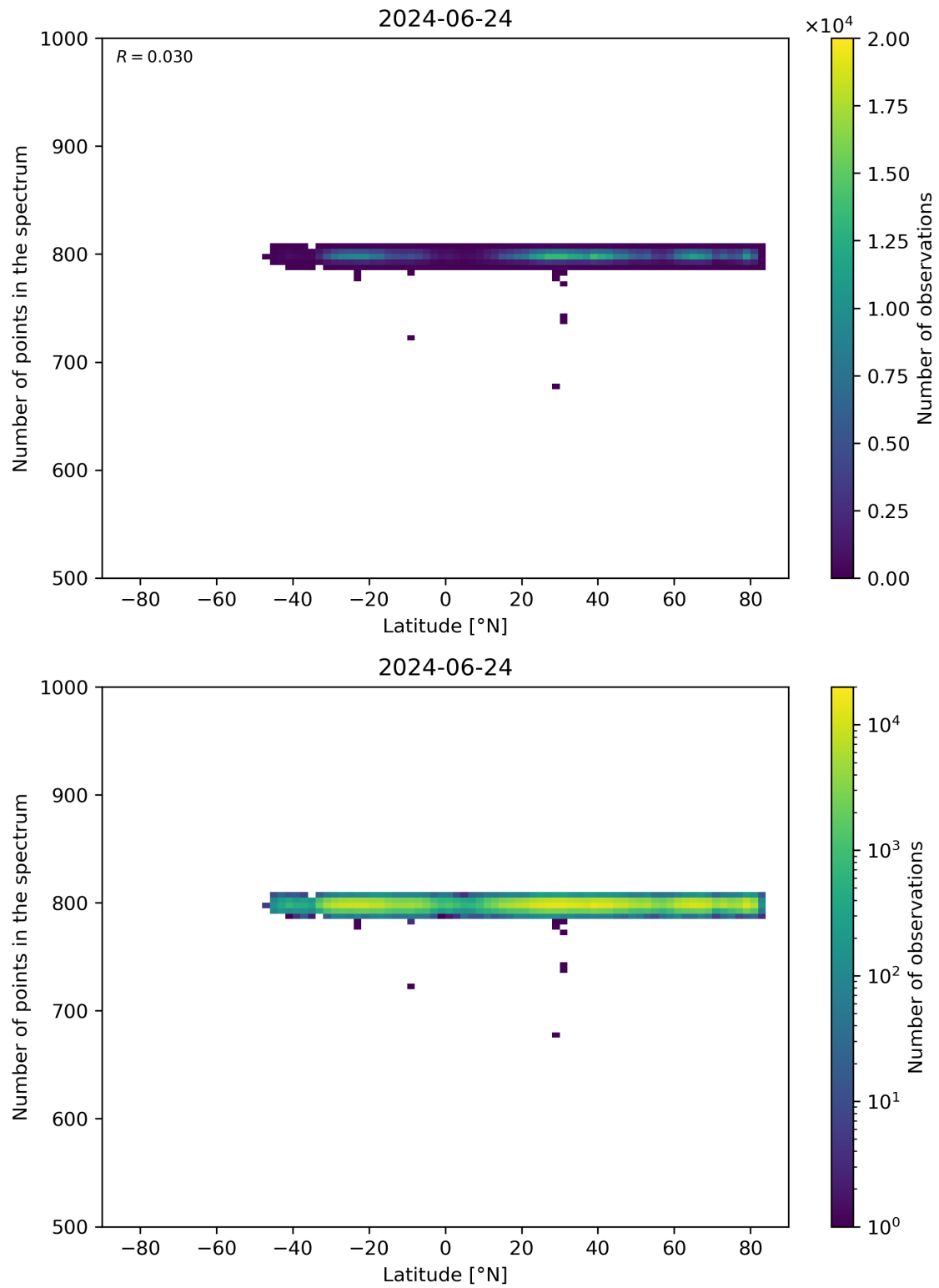
Figure 61: Scatter density plot of “Latitude” against “Number of points in the spectrum” for 2024-06-24 to 2024-06-25.
