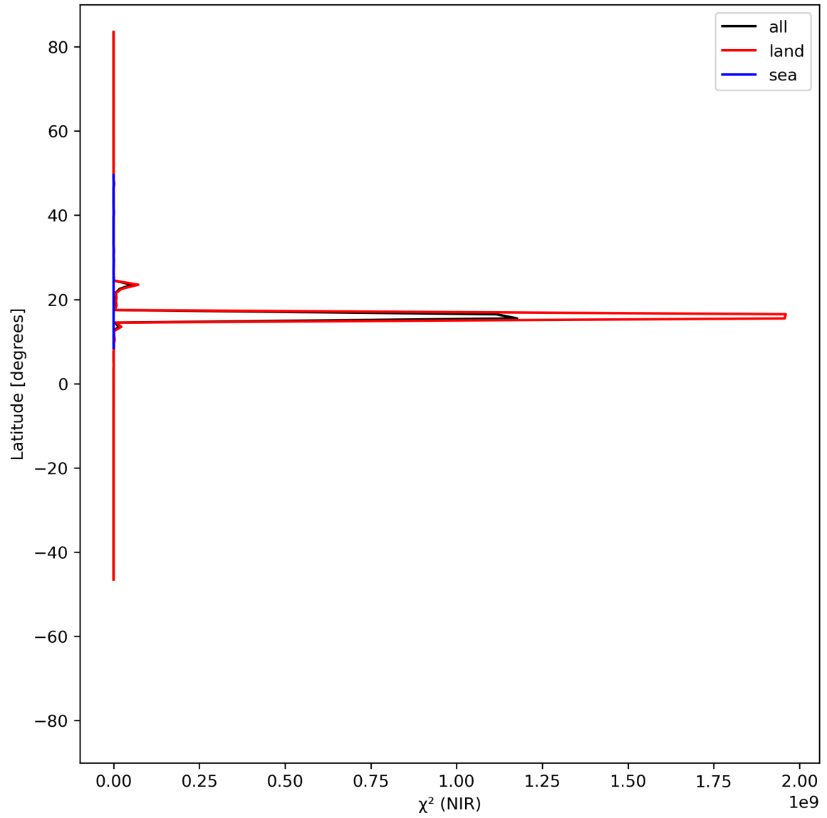
Figure 18: Zonal average of “ \chi^2 (NIR)” for 2024-06-24 to 2024-06-25.
