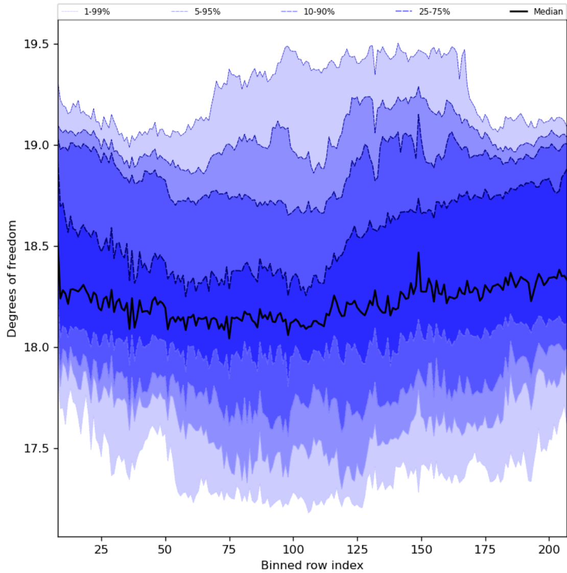
Figure 41: Along track statistics of “Degrees of freedom” for 2024-06-24 to 2024-06-25
