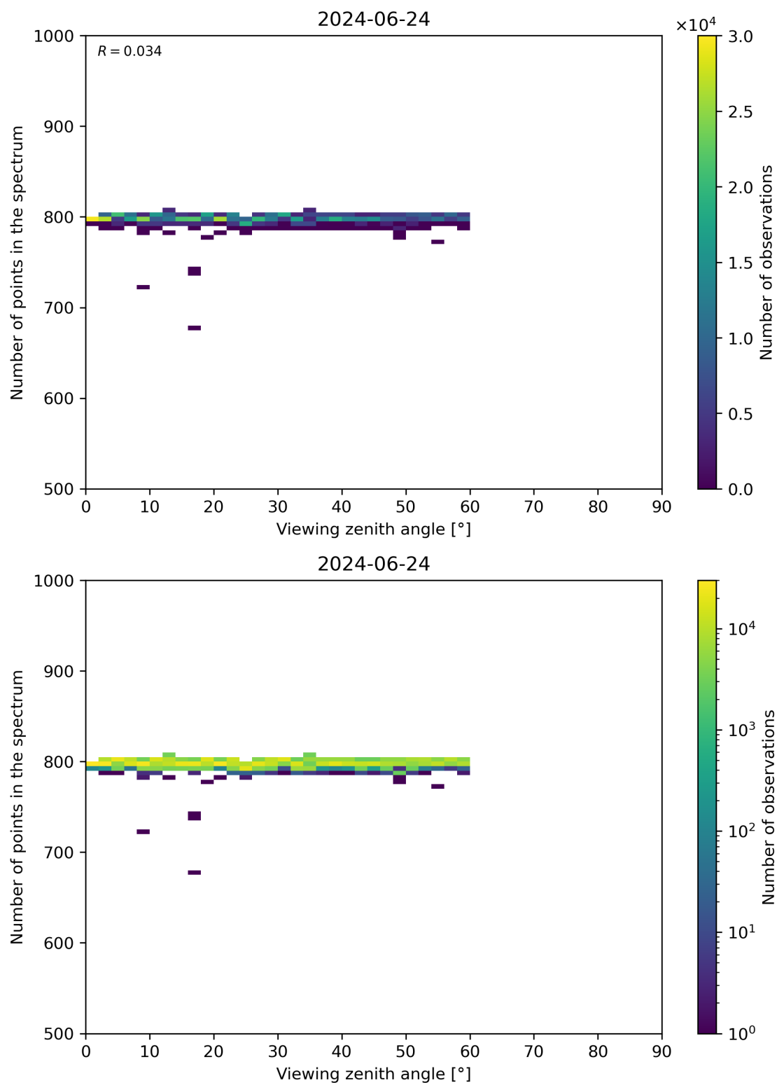
Figure 114: Scatter density plot of “Viewing zenith angle” against “Number of points in the spectrum” for 2024-06-24 to 2024-06-25.
