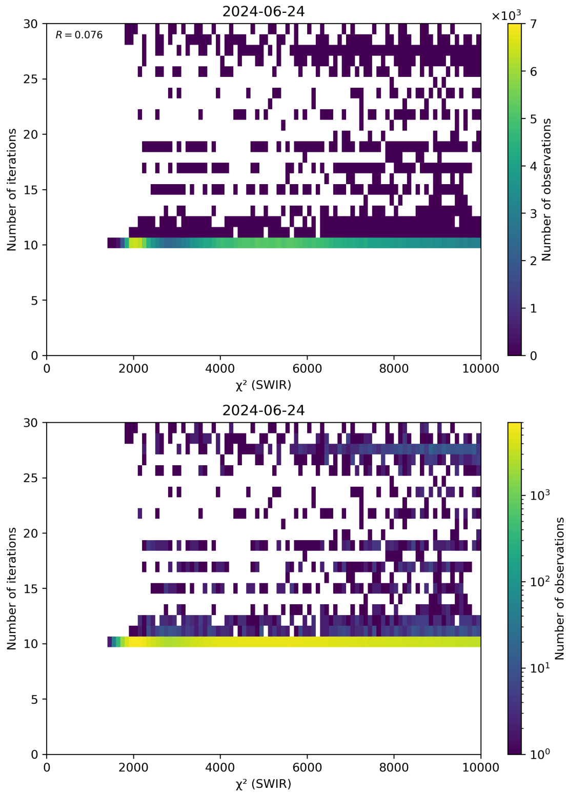
Figure 50: Scatter density plot of “ \chi^2 (SWIR)” against “Number of iterations” for 2024-06-24 to 2024-06-25.
