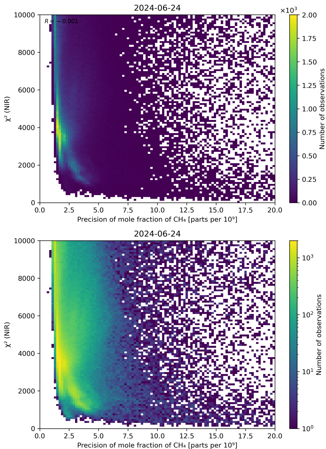
Figure 78: Scatter density plot of “Precision of mole fraction of CH 4 ” against “ \chi^2 (NIR)” for 2024-06-24 to 2024-06-25.
