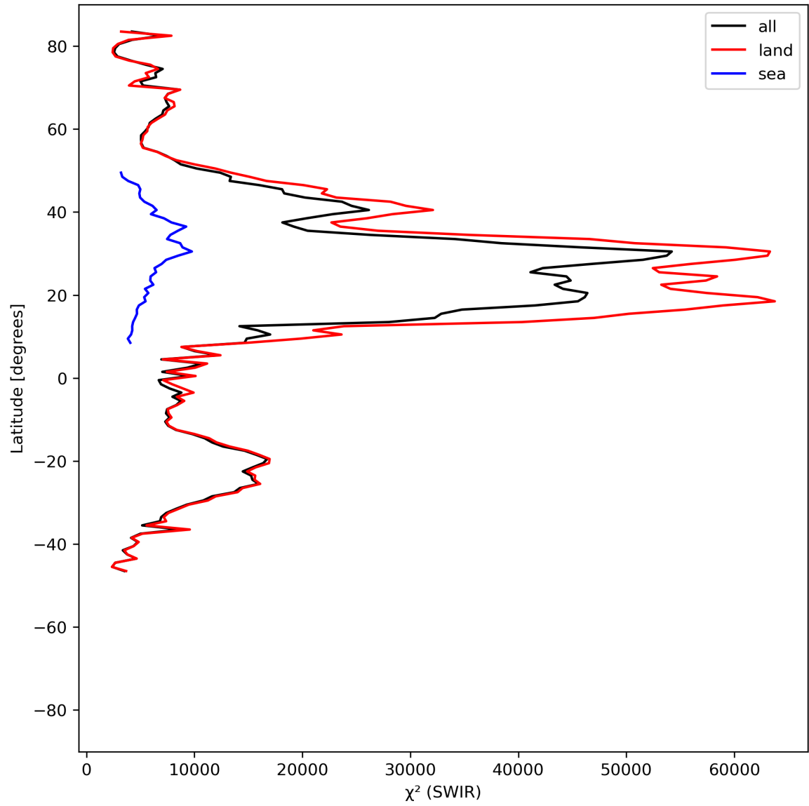
Figure 17: Zonal average of “ \chi^2 (SWIR)” for 2024-06-24 to 2024-06-25.
