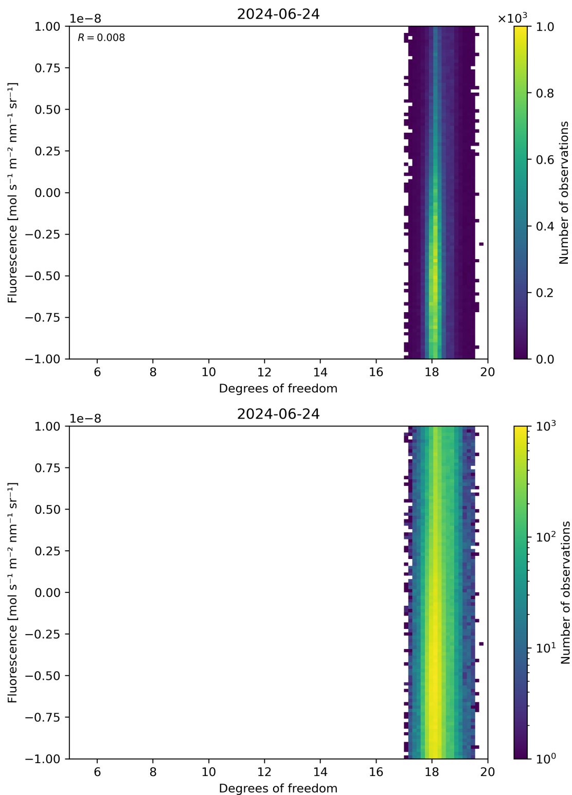
Figure 51: Scatter density plot of “Degrees of freedom” against “Fluorescence” for 2024-06-24 to 2024-06-25.
