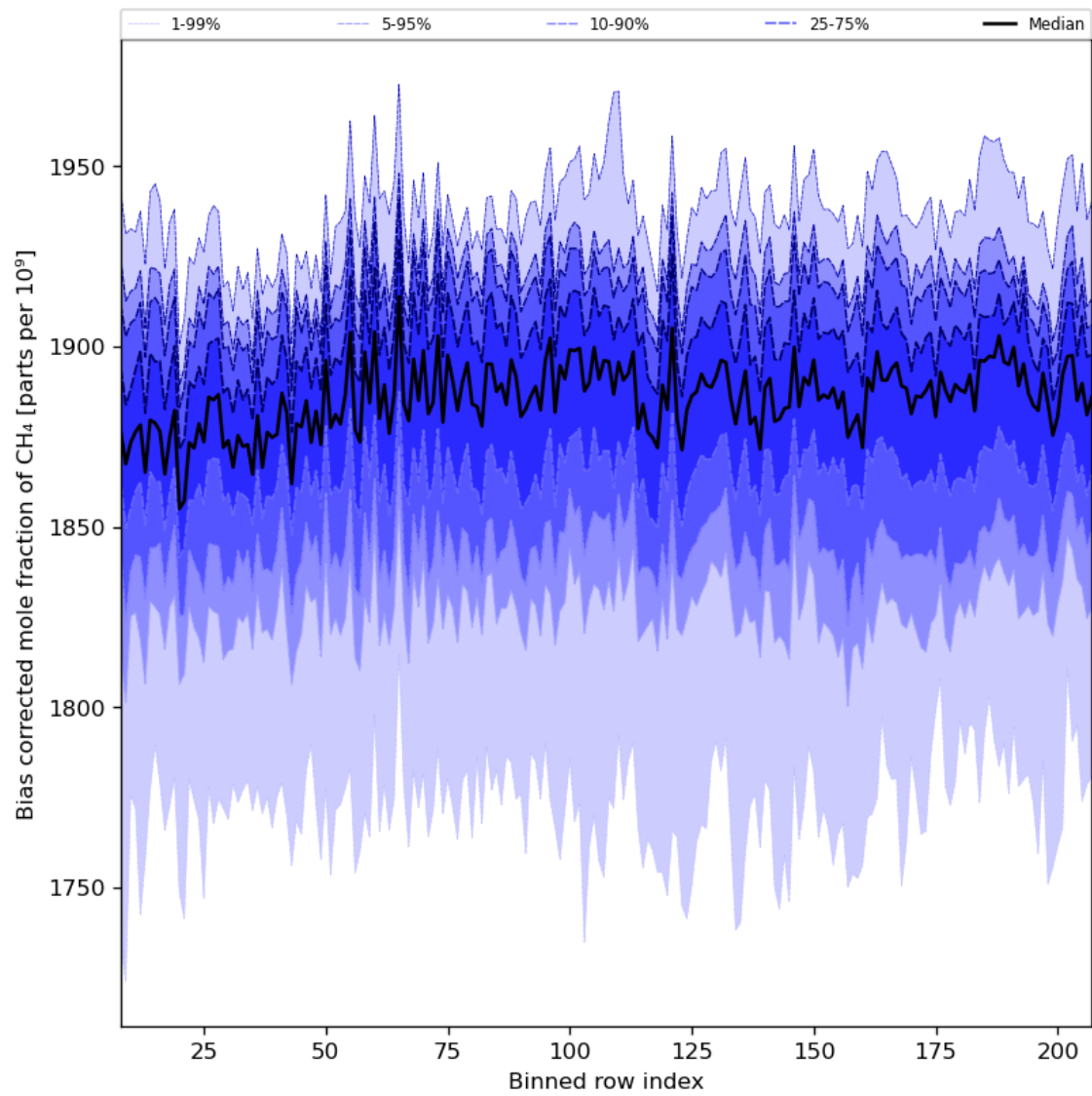
Figure 36: Along track statistics of “Bias corrected mole fraction of CH 4 ” for 2024-06-24 to 2024-06-25
