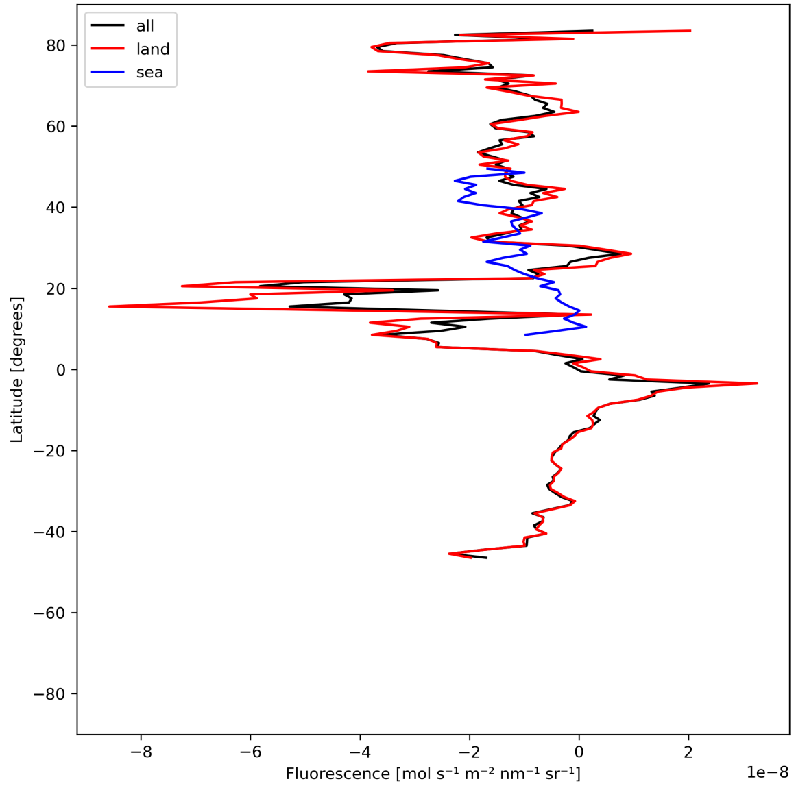
Figure 21: Zonal average of “Fluorescence” for 2024-06-24 to 2024-06-25.
