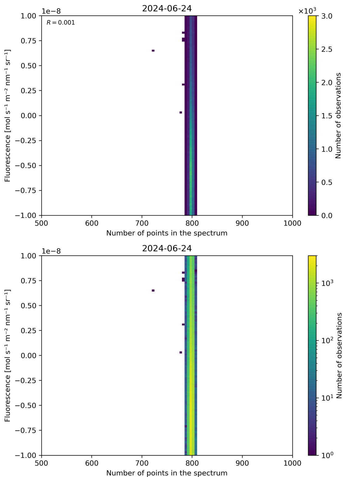
Figure 91: Scatter density plot of “Number of points in the spectrum” against “Fluorescence” for 2024-06-24 to 2024-06-25.
