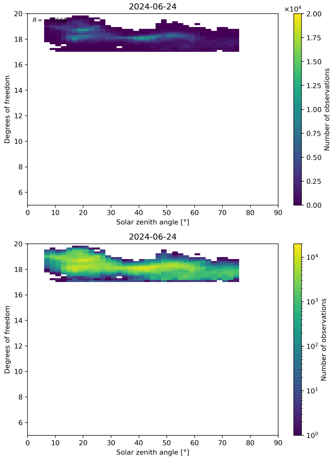
Figure 96: Scatter density plot of “Solar zenith angle” against “Degrees of freedom” for 2024-06-24 to 2024-06-25.
