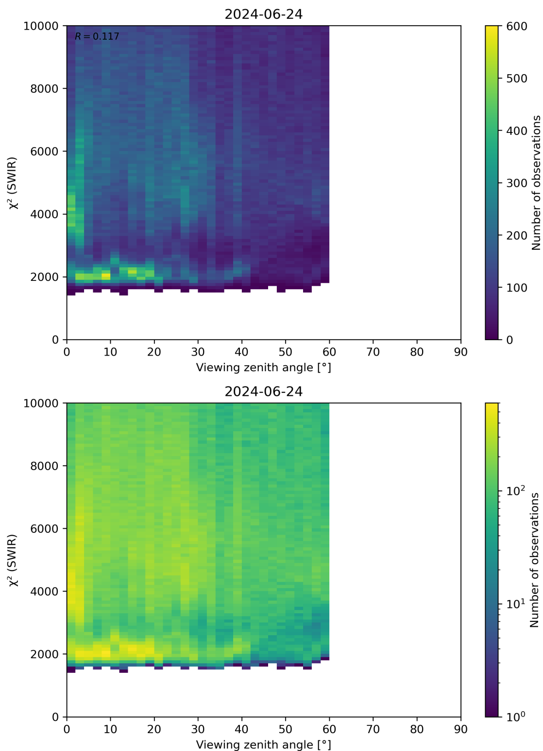
Figure 106: Scatter density plot of “Viewing zenith angle” against “ \chi^2 (SWIR)” for 2024-06-24 to 2024-06-25.
