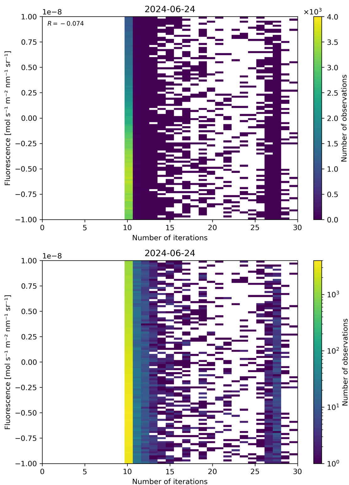
Figure 87: Scatter density plot of “Number of iterations” against “Fluorescence” for 2024-06-24 to 2024-06-25.
