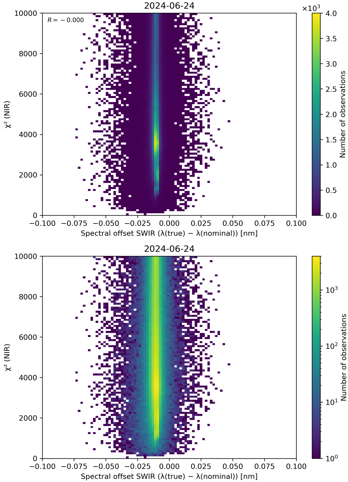
Figure 117: Scatter density plot of “Spectral offset SWIR ( \lambda(\text{true}) - \lambda(\text{nominal}) )” against “ \chi^2 (NIR)” for 2024-06-24 to 2024-06-25.
