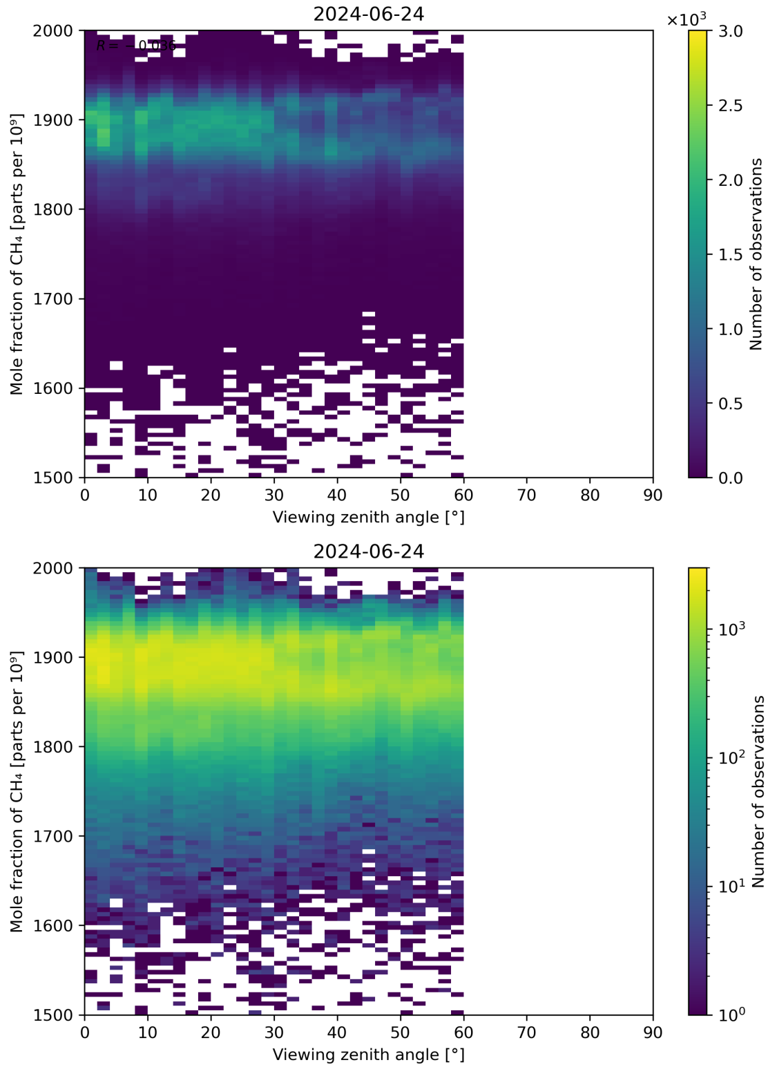
Figure 110: Scatter density plot of “Viewing zenith angle” against “Mole fraction of CH 4 ” for 2024-06-24 to 2024-06-25.
