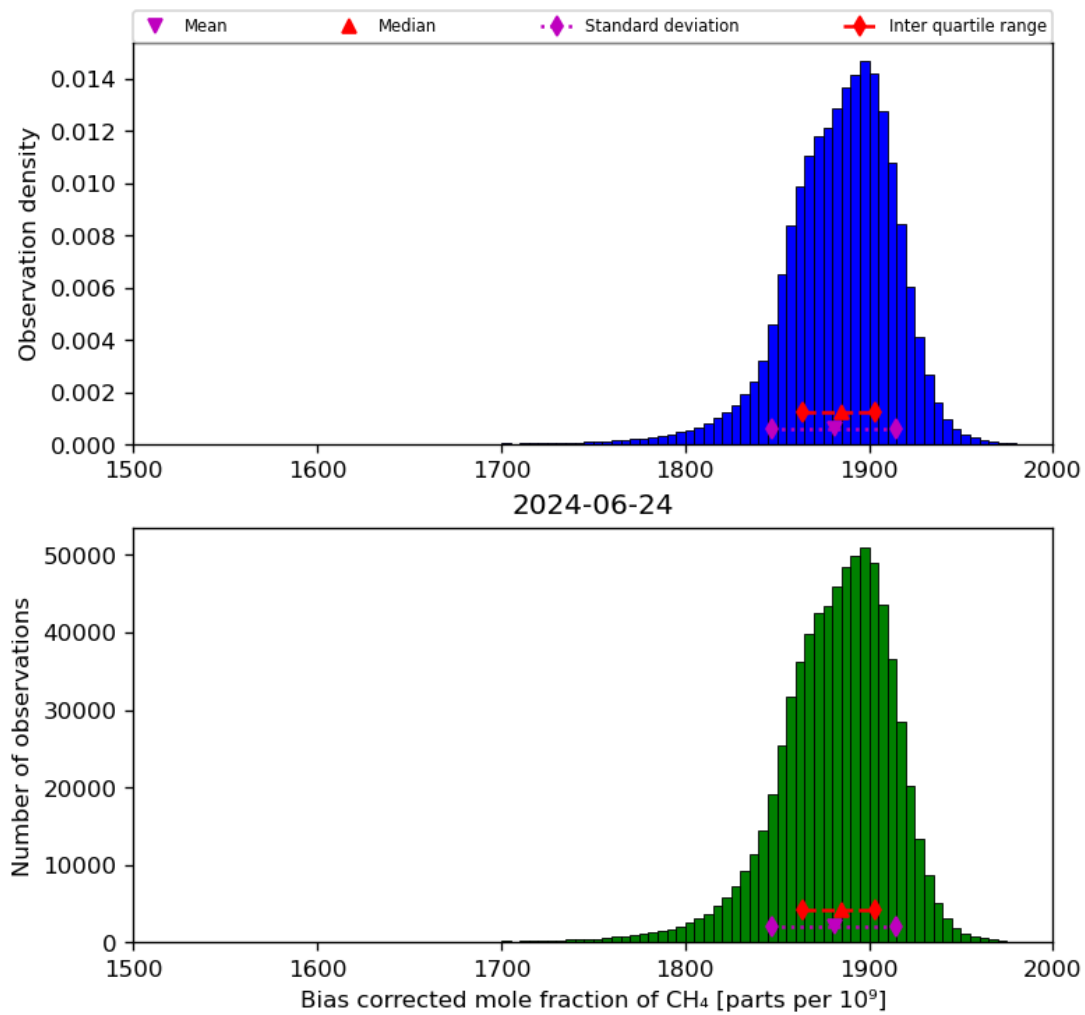
Figure 25: Histogram of “Bias corrected mole fraction of CH 4 ” for 2024-06-24 to 2024-06-25
