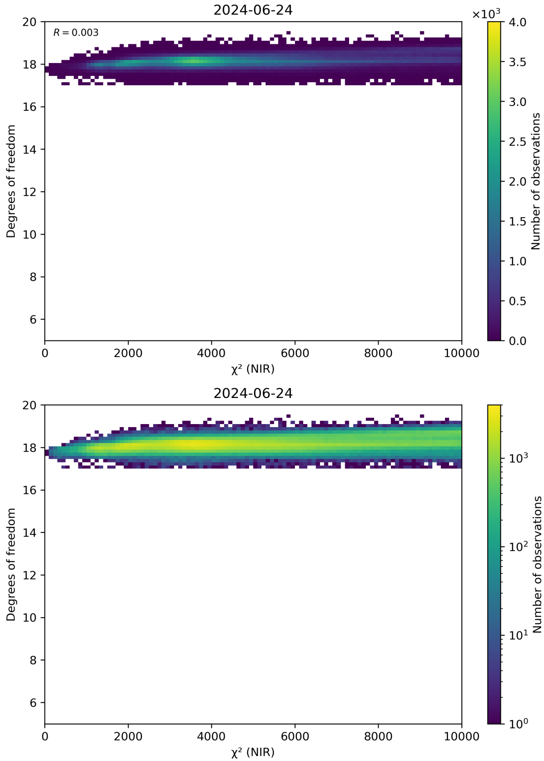
Figure 44: Scatter density plot of “ \chi^2 (NIR)” against “Degrees of freedom” for 2024-06-24 to 2024-06-25.
