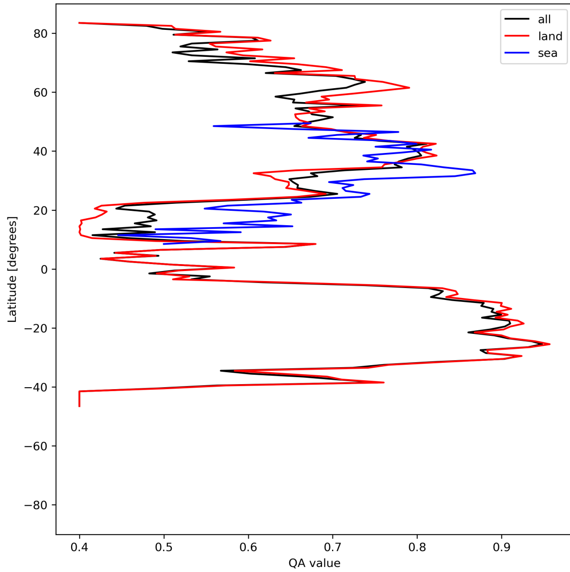
Figure 11: Zonal average of “QA value” for 2024-06-24 to 2024-06-25.
