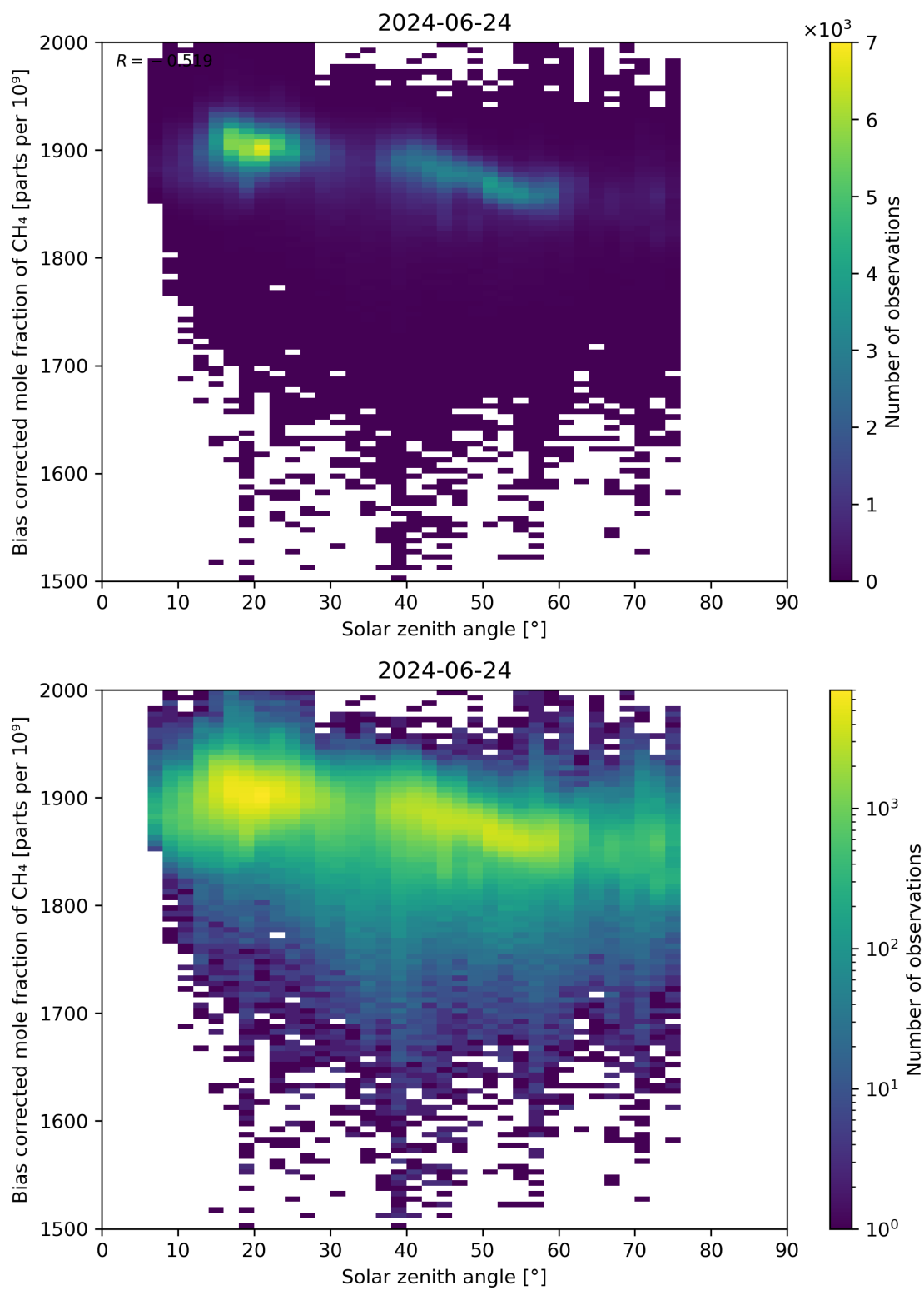
Figure 100: Scatter density plot of “Solar zenith angle” against “Bias corrected mole fraction of CH 4 ” for 2024-06-24 to 2024-06-25.
