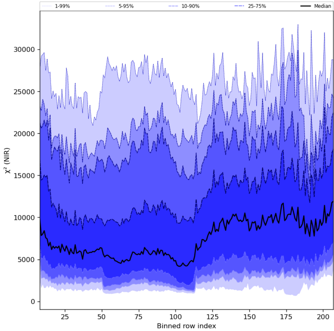
Figure 40: Along track statistics of “ \chi^2 (NIR)” for 2024-06-24 to 2024-06-25
