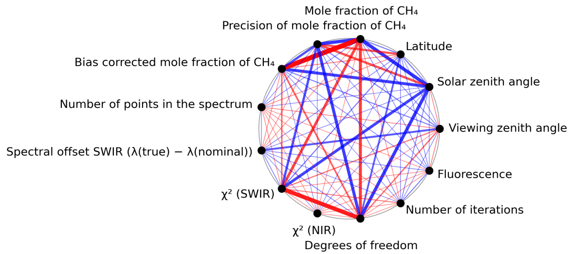
Figure 1: Map of correlation graph for 2024-06-24 to 2024-06-25.
