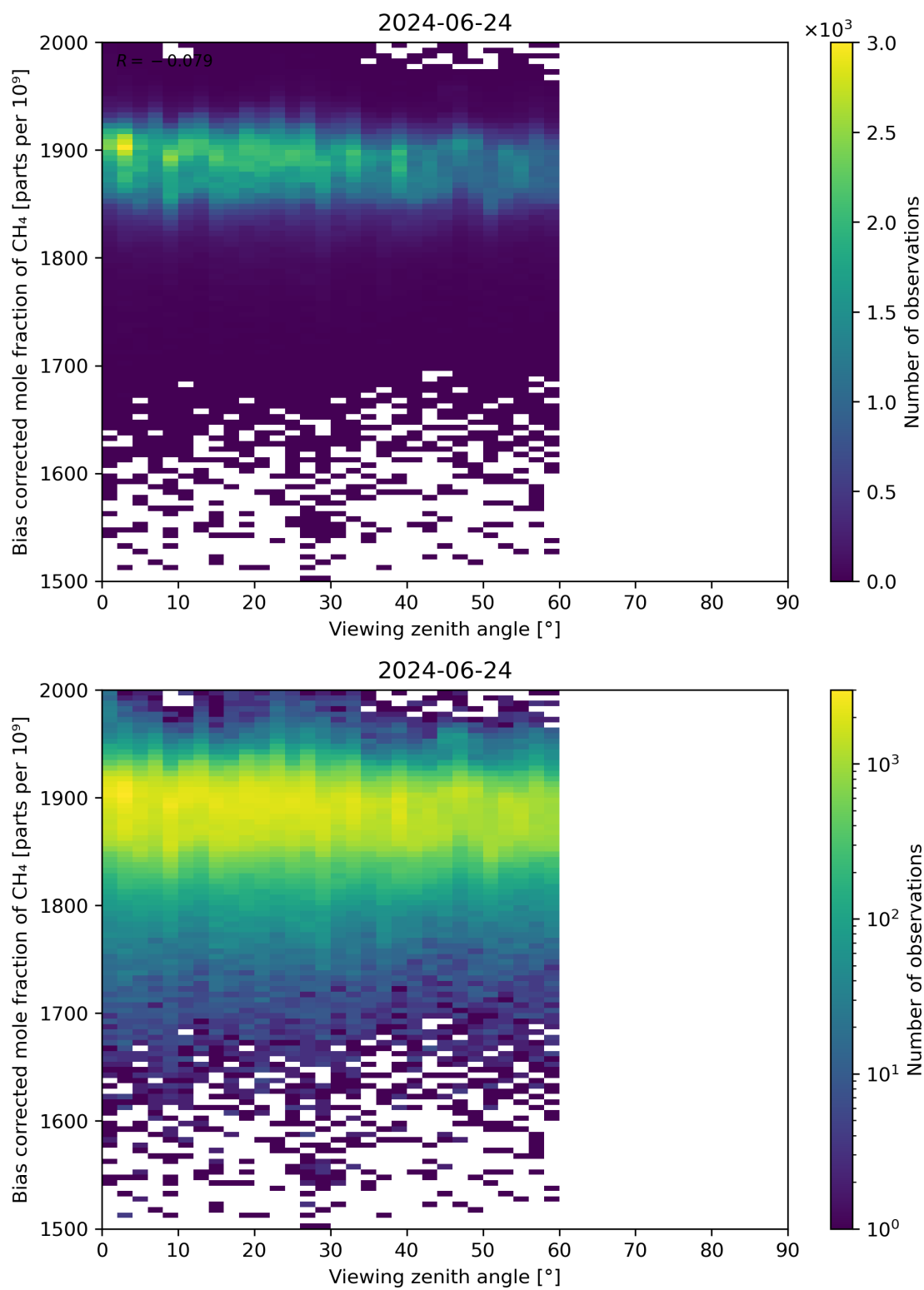
Figure 111: Scatter density plot of “Viewing zenith angle” against “Bias corrected mole fraction of CH 4 ” for 2024-06-24 to 2024-06-25.
