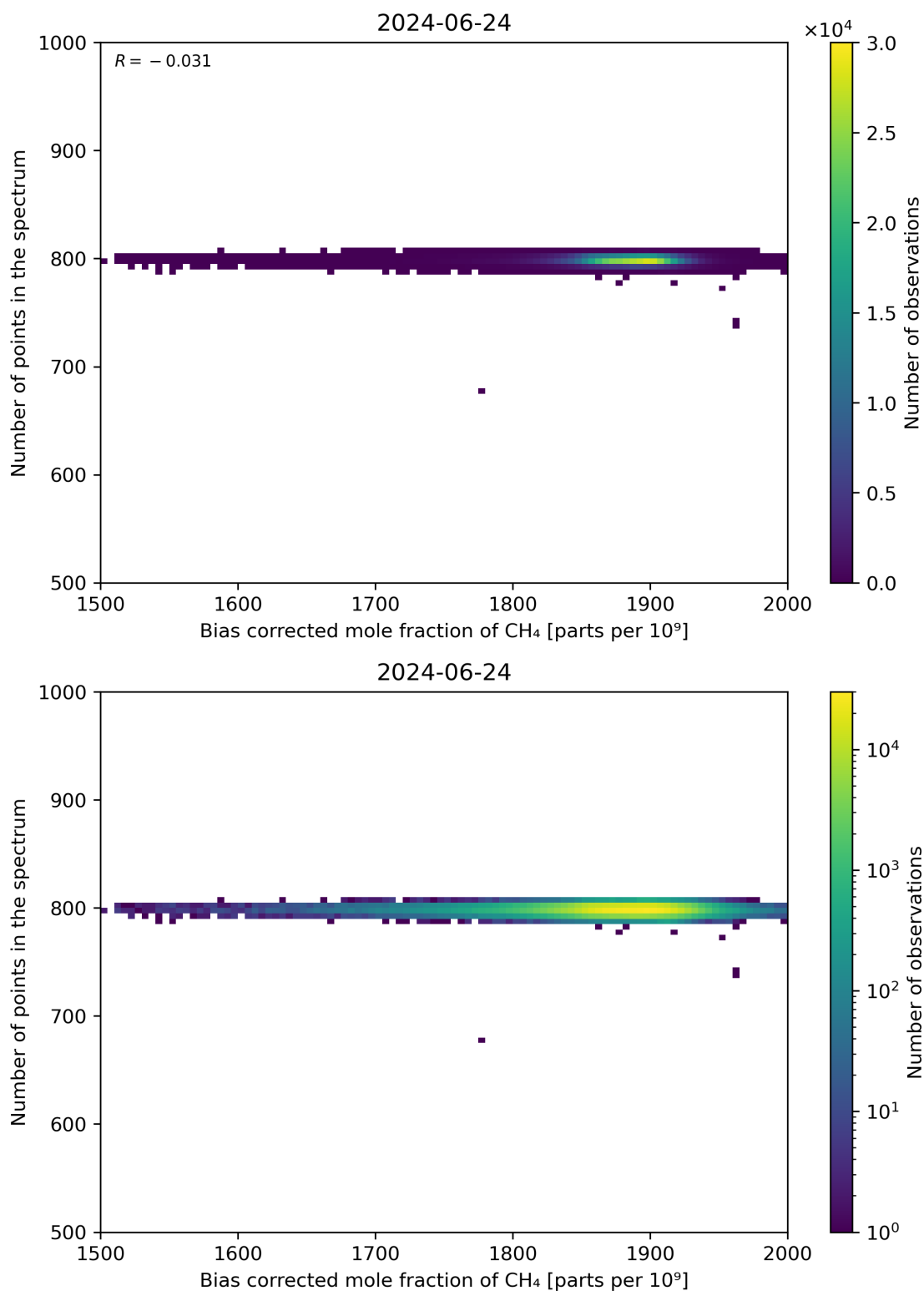
Figure 68: Scatter density plot of “Bias corrected mole fraction of CH 4 ” against “Number of points in the spectrum” for 2024-06-24 to 2024-06-25.
