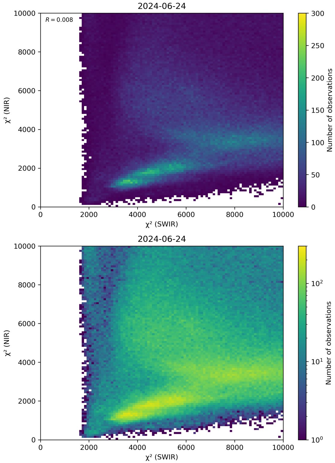
Figure 47: Scatter density plot of “ \chi^2 (SWIR)” against “ \chi^2 (NIR)” for 2024-06-24 to 2024-06-25.
