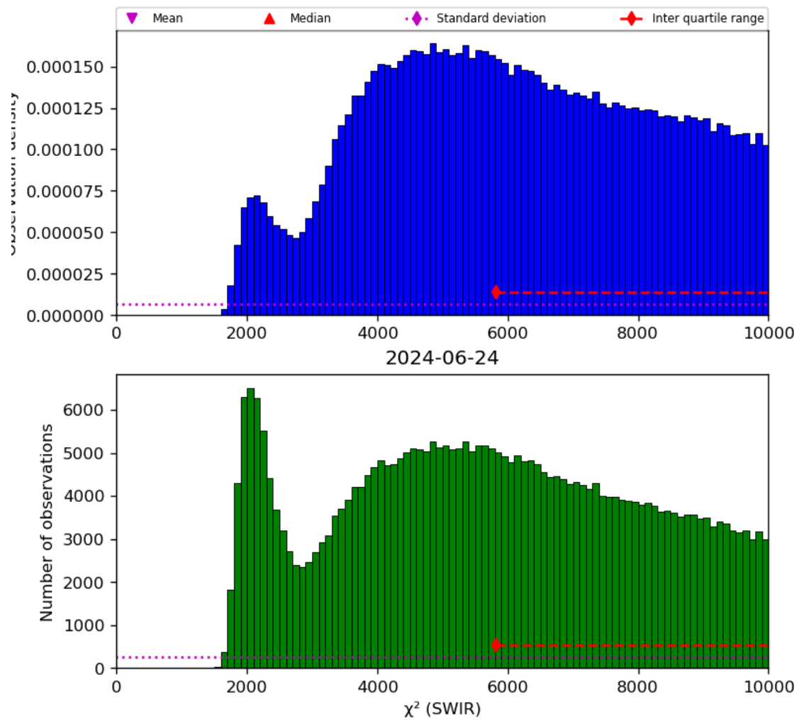
Figure 28: Histogram of “ \chi^2 (SWIR)” for 2024-06-24 to 2024-06-25
