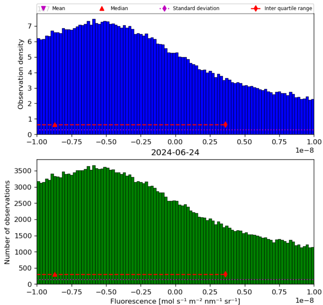
Figure 32: Histogram of “Fluorescence” for 2024-06-24 to 2024-06-25
