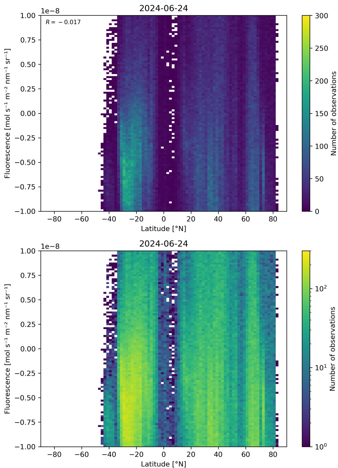
Figure 56: Scatter density plot of “Latitude” against “Fluorescence” for 2024-06-24 to 2024-06-25.
