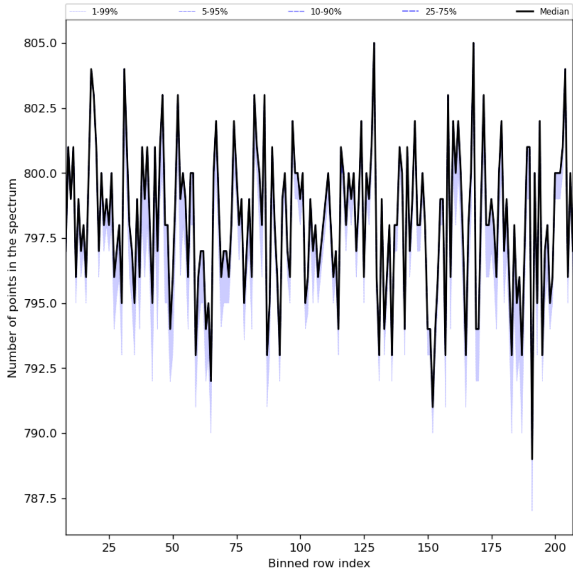
Figure 37: Along track statistics of “Number of points in the spectrum” for 2024-06-24 to 2024-06-25
