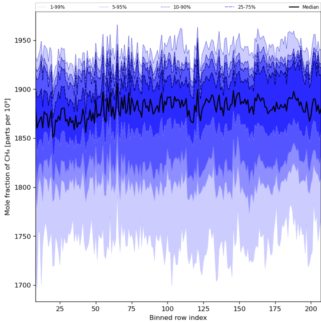
Figure 34: Along track statistics of “Mole fraction of CH 4 ” for 2024-06-24 to 2024-06-25
