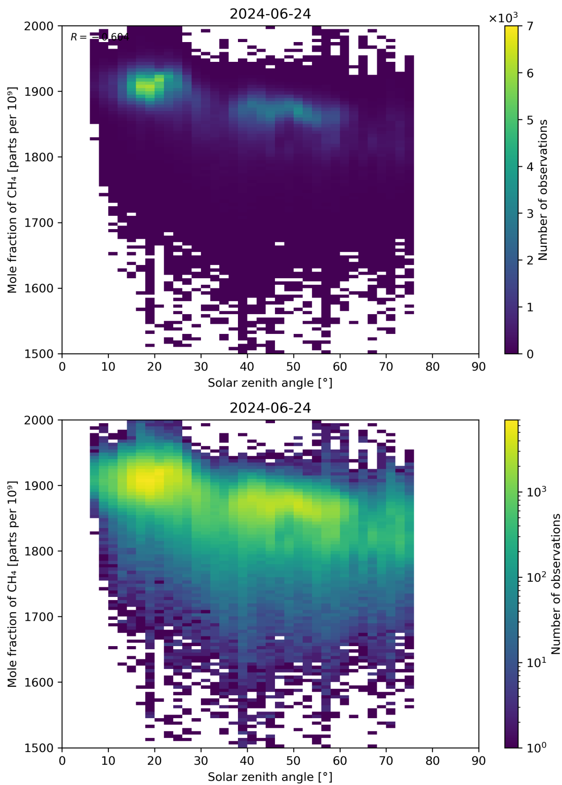
Figure 99: Scatter density plot of “Solar zenith angle” against “Mole fraction of \text{CH}_4 ” for 2024-06-24 to 2024-06-25.
