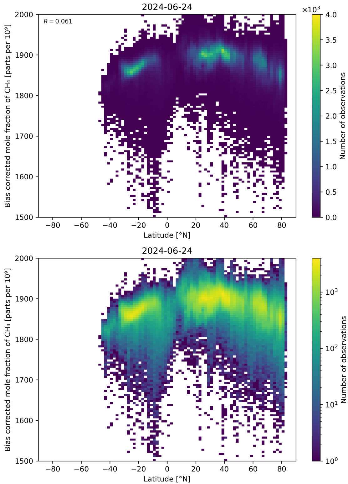
Figure 58: Scatter density plot of “Latitude” against “Bias corrected mole fraction of CH 4 ” for 2024-06-24 to 2024-06-25.
