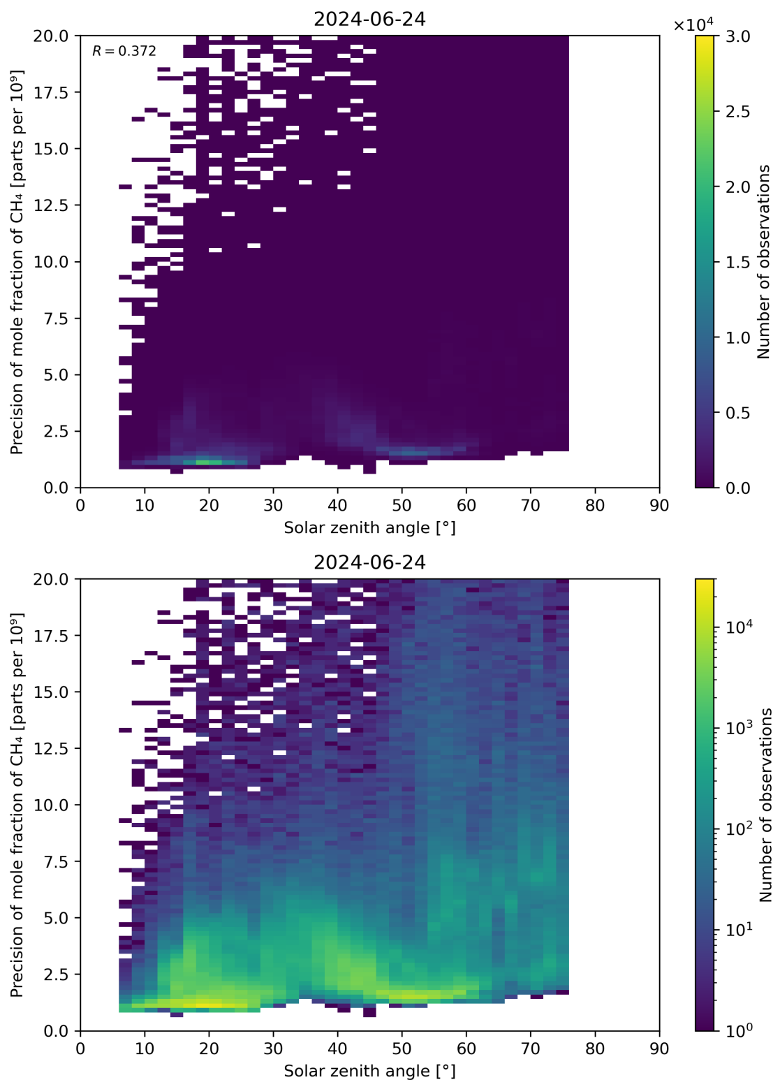
Figure 101: Scatter density plot of “Solar zenith angle” against “Precision of mole fraction of CH 4 ” for 2024-06-24 to 2024-06-25.
