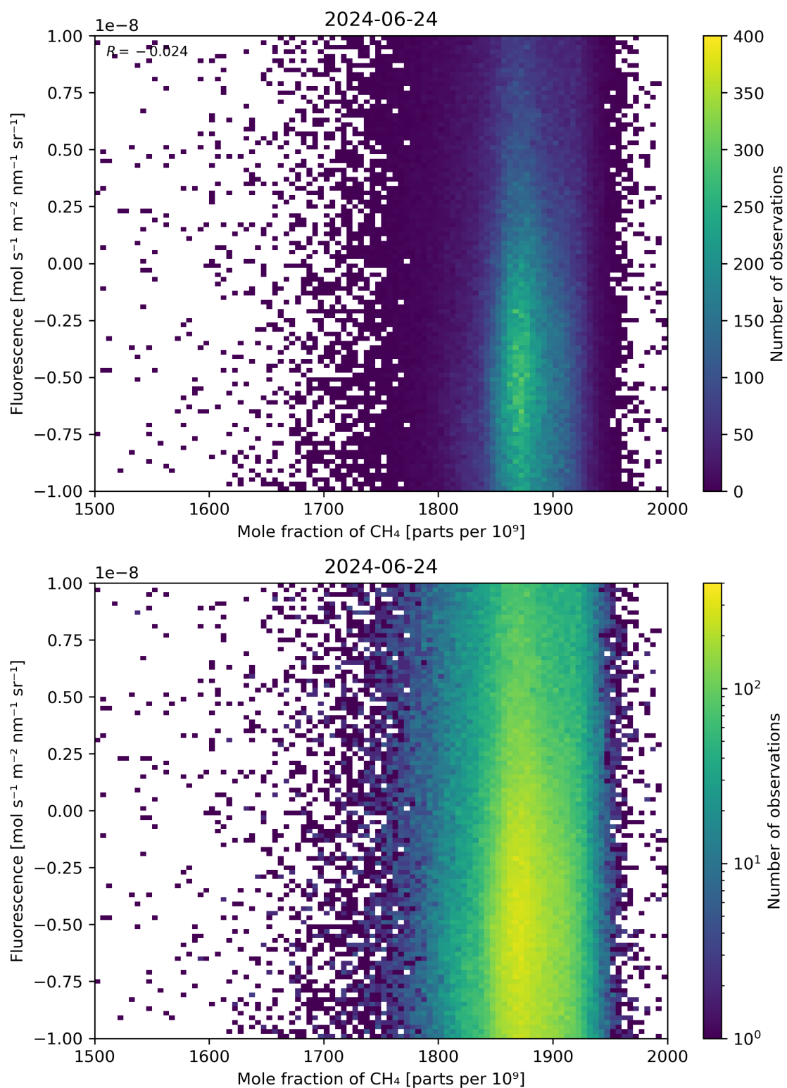
Figure 73: Scatter density plot of “Mole fraction of \text{CH}_4 ” against “Fluorescence” for 2024-06-24 to 2024-06-25.
