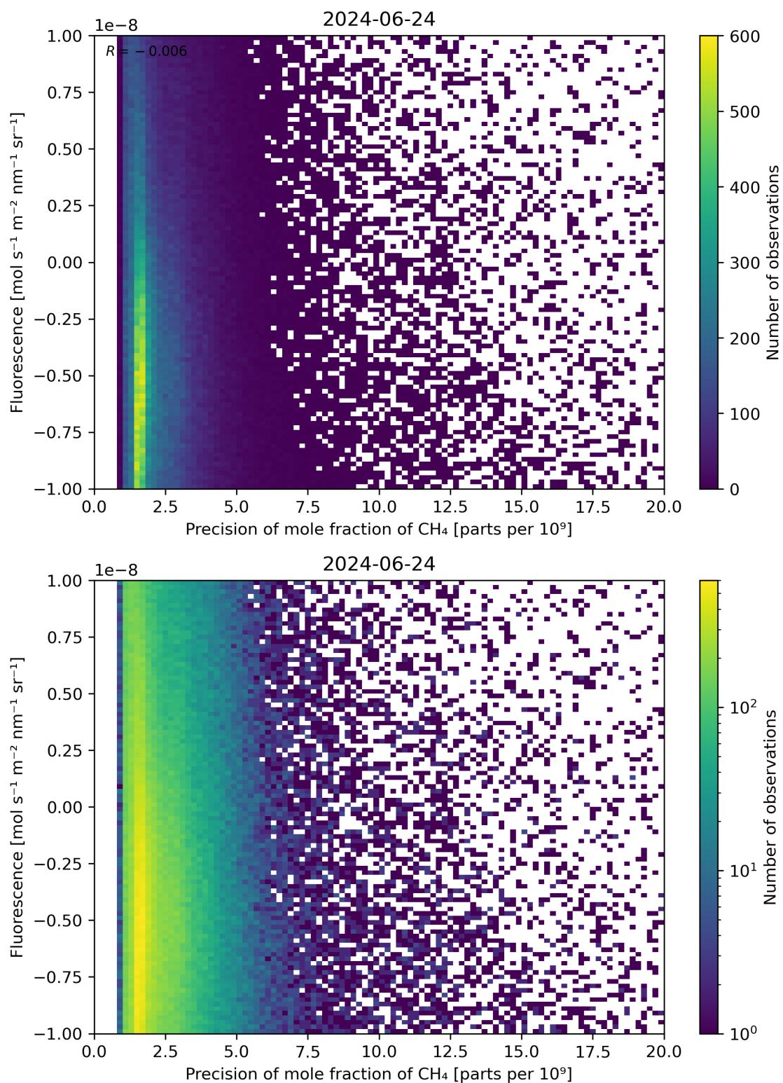
Figure 81: Scatter density plot of “Precision of mole fraction of CH 4 ” against “Fluorescence” for 2024-06-24 to 2024-06-25.
