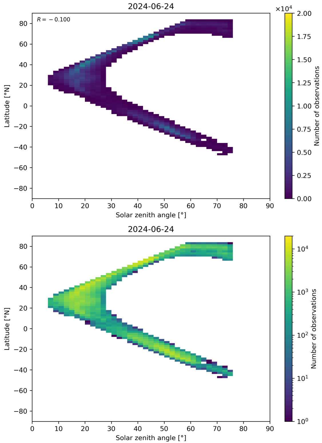
Figure 98: Scatter density plot of “Solar zenith angle” against “Latitude” for 2024-06-24 to 2024-06-25.
