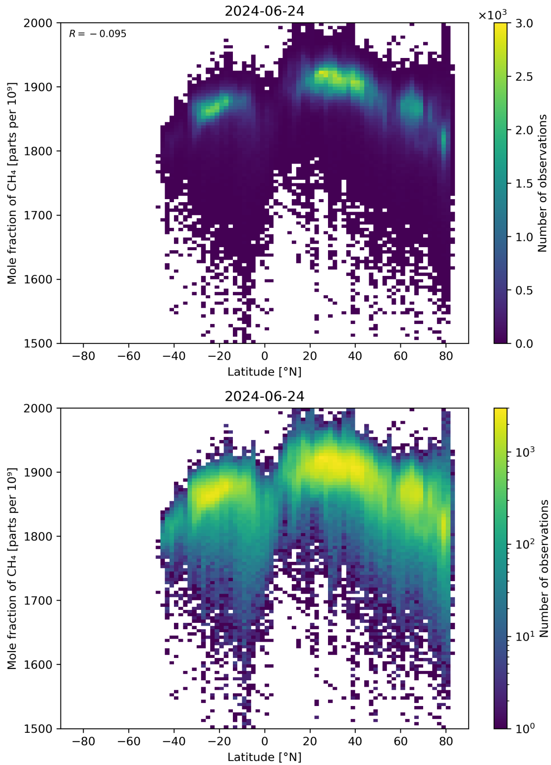
Figure 57: Scatter density plot of “Latitude” against “Mole fraction of CH 4 ” for 2024-06-24 to 2024-06-25.
