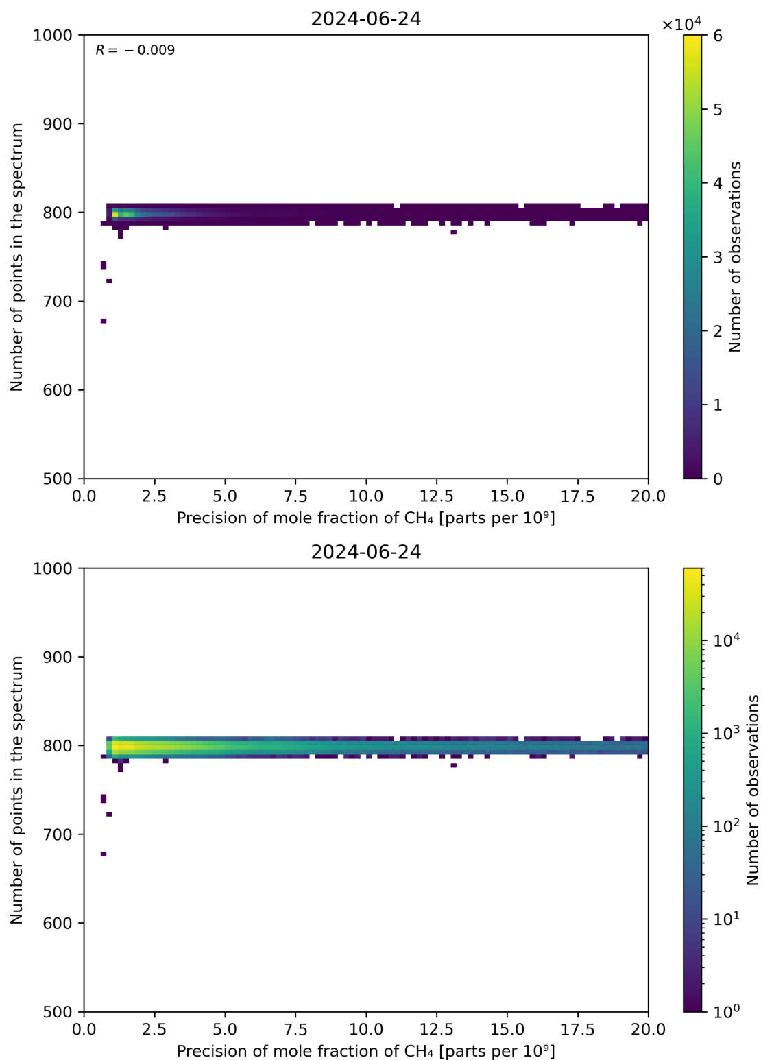
Figure 84: Scatter density plot of “Precision of mole fraction of CH 4 ” against “Number of points in the spectrum” for 2024-06-24 to 2024-06-25.
