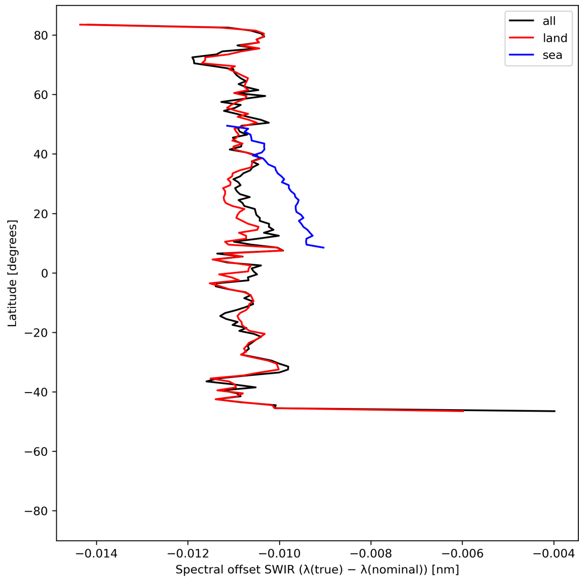
Figure 16: Zonal average of “Spectral offset SWIR ( \lambda(\text{true}) - \lambda(\text{nominal}) )” for 2024-06-24 to 2024-06-25.
