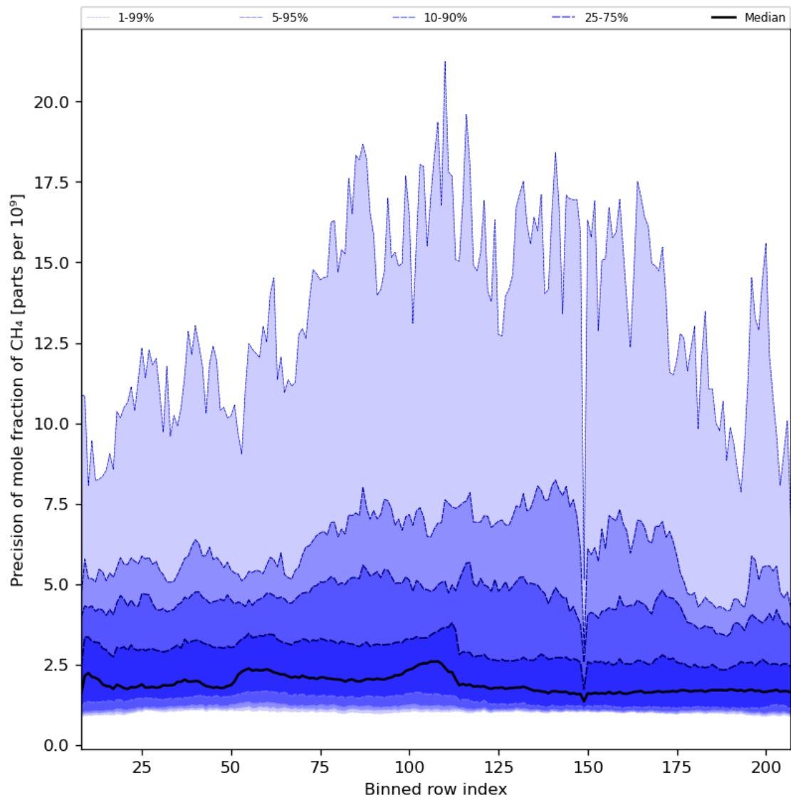
Figure 35: Along track statistics of “Precision of mole fraction of CH 4 ” for 2024-06-24 to 2024-06-25
