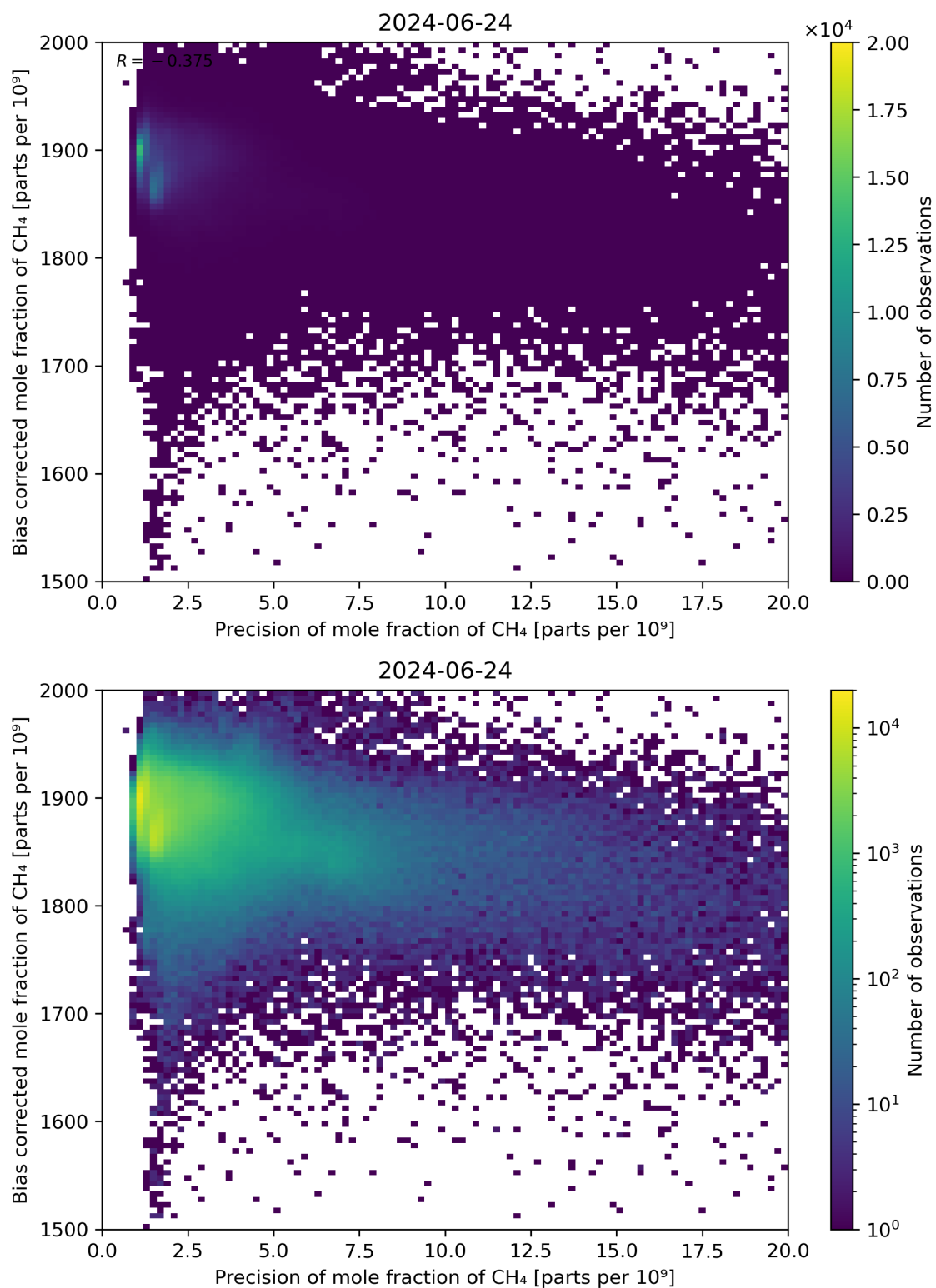
Figure 82: Scatter density plot of “Precision of mole fraction of \text{CH}_4 ” against “Bias corrected mole fraction of \text{CH}_4 ” for 2024-06-24 to 2024-06-25.
