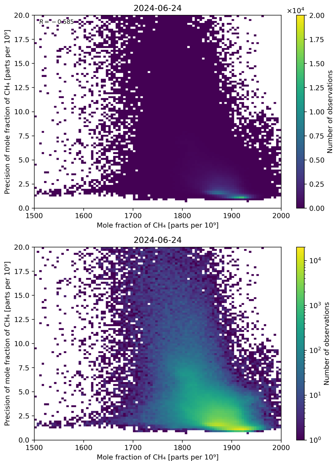
Figure 75: Scatter density plot of “Mole fraction of CH 4 ” against “Precision of mole fraction of CH 4 ” for 2024-06-24 to 2024-06-25.
