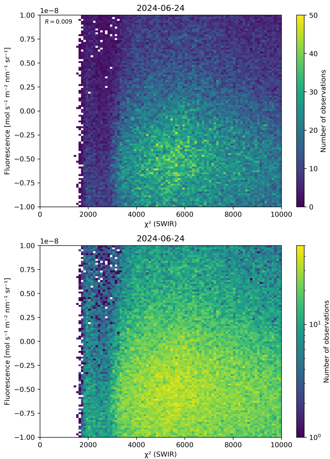
Figure 49: Scatter density plot of “ \chi^2 (SWIR)” against “Fluorescence” for 2024-06-24 to 2024-06-25.
