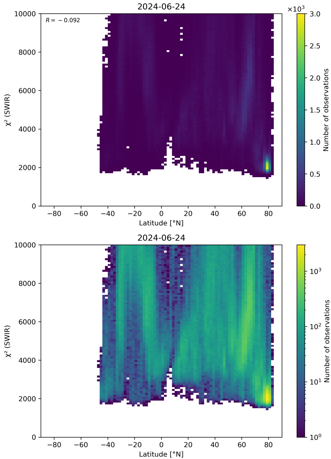
Figure 54: Scatter density plot of “Latitude” against “ \chi^2 (SWIR)” for 2024-06-24 to 2024-06-25.
