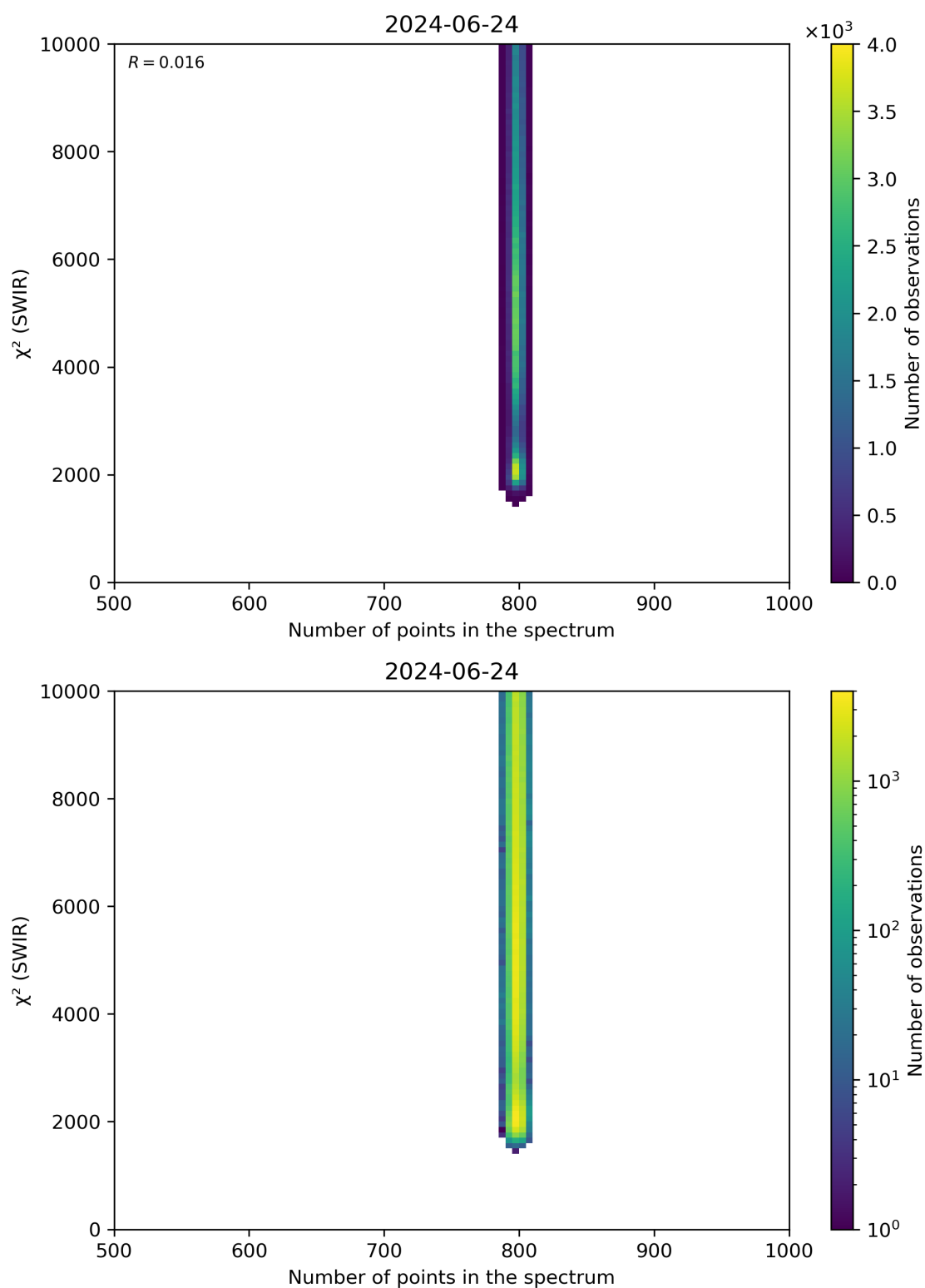
Figure 89: Scatter density plot of “Number of points in the spectrum” against “ \chi^2 (SWIR)” for 2024-06-24 to 2024-06-25.
