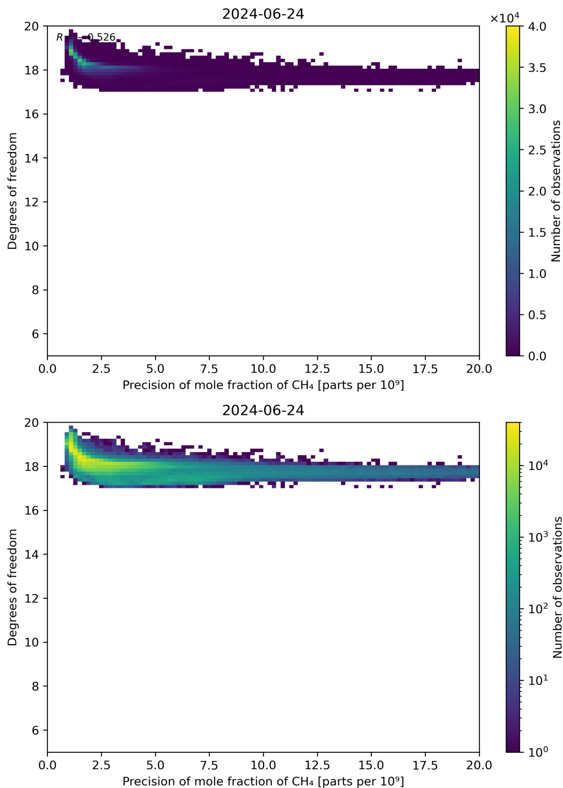
Figure 80: Scatter density plot of “Precision of mole fraction of CH 4 ” against “Degrees of freedom” for 2024-06-24 to 2024-06-25.
