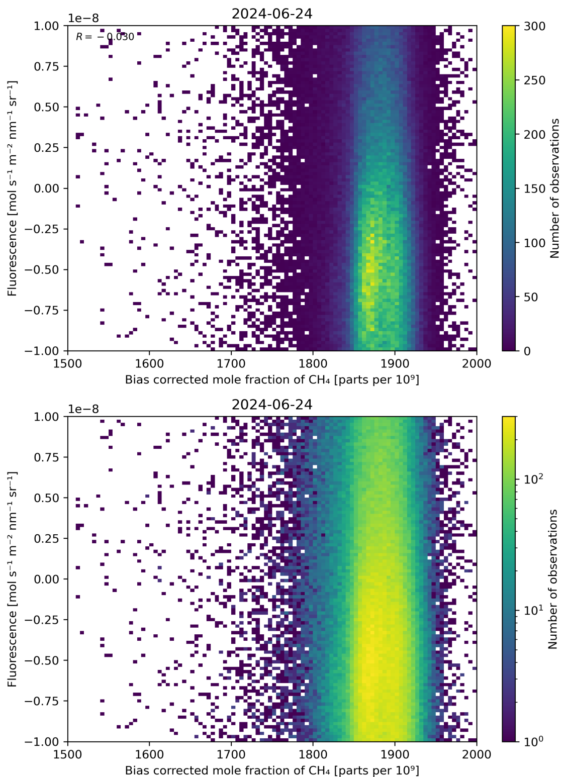
Figure 66: Scatter density plot of “Bias corrected mole fraction of \text{CH}_4 ” against “Fluorescence” for 2024-06-24 to 2024-06-25.
