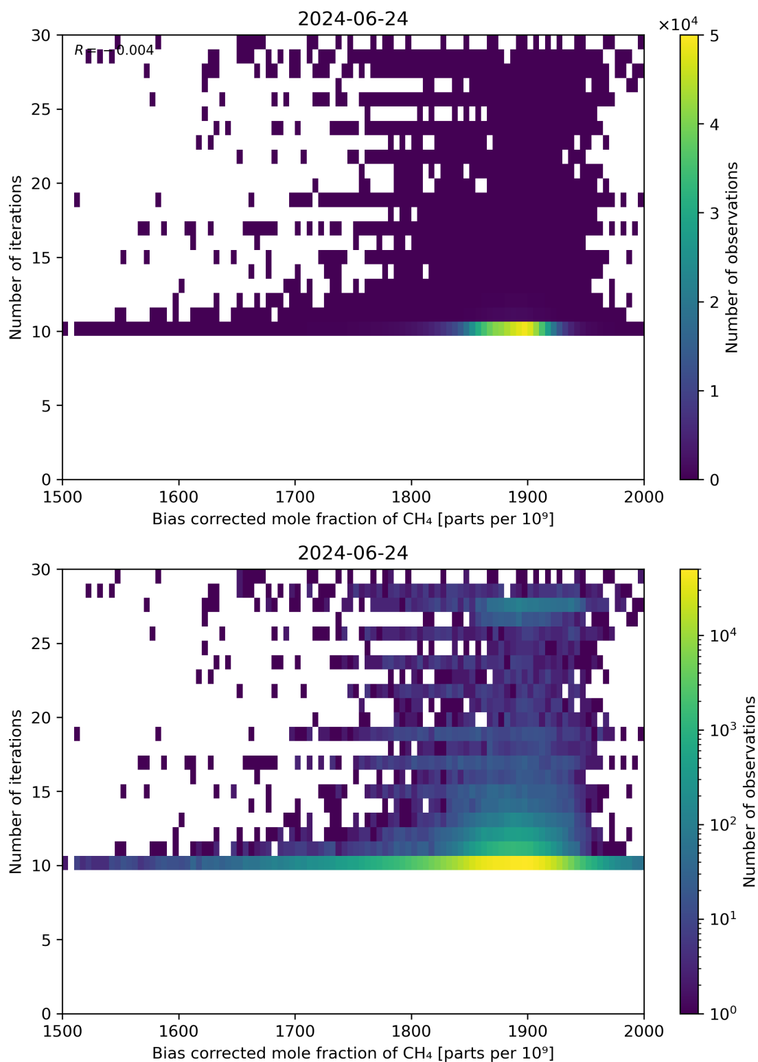
Figure 67: Scatter density plot of “Bias corrected mole fraction of CH 4 ” against “Number of iterations” for 2024-06-24 to 2024-06-25.
