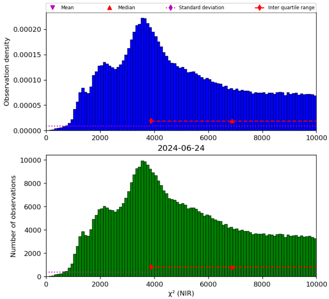
Figure 29: Histogram of “ \chi^2 (NIR)” for 2024-06-24 to 2024-06-25
