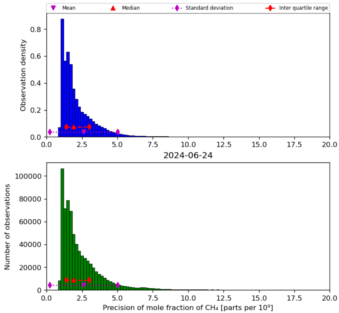
Figure 24: Histogram of “Precision of mole fraction of CH 4 ” for 2024-06-24 to 2024-06-25
