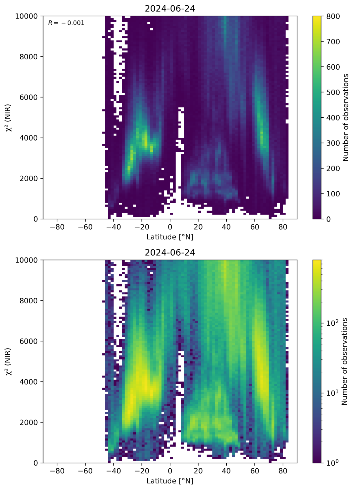
Figure 53: Scatter density plot of “Latitude” against “ \chi^2 (NIR)” for 2024-06-24 to 2024-06-25.
