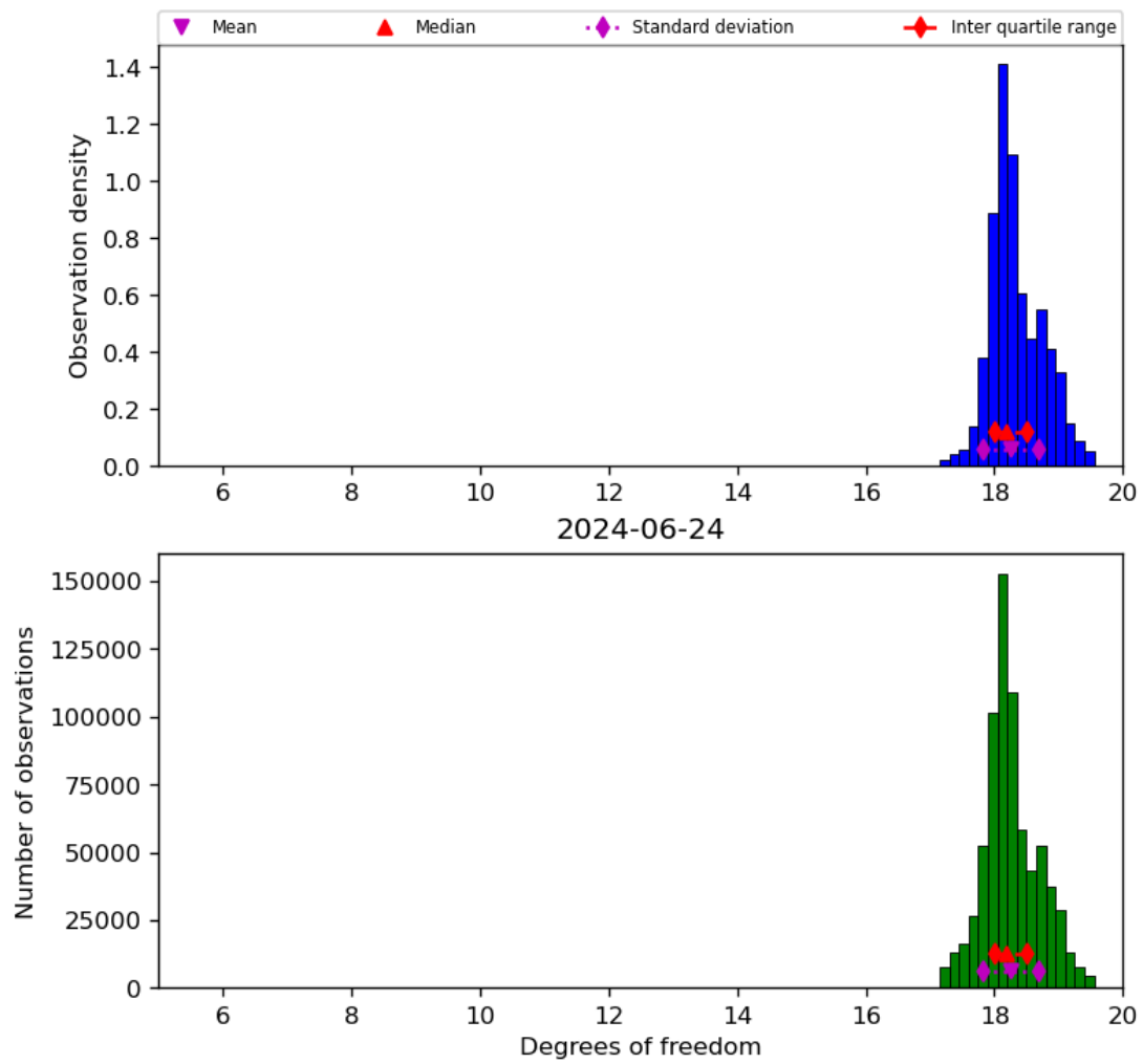
Figure 30: Histogram of “Degrees of freedom” for 2024-06-24 to 2024-06-25
