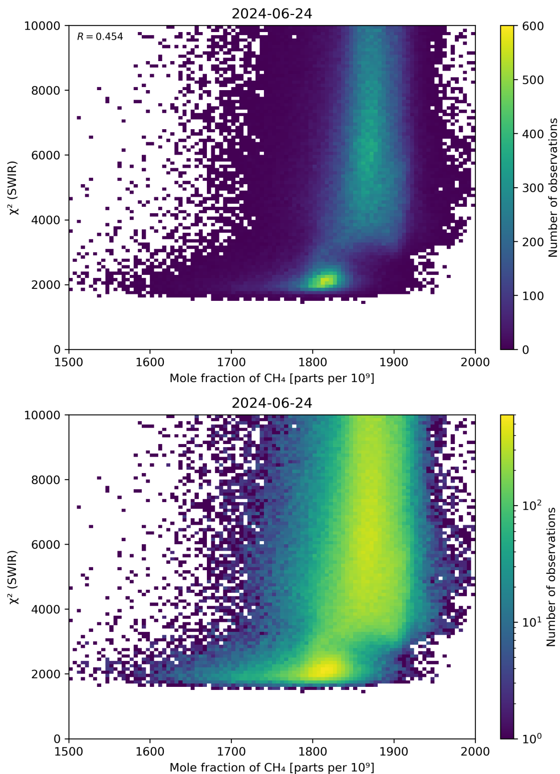
Figure 71: Scatter density plot of “Mole fraction of \text{CH}_4 ” against “ \chi^2 (SWIR)” for 2024-06-24 to 2024-06-25.
