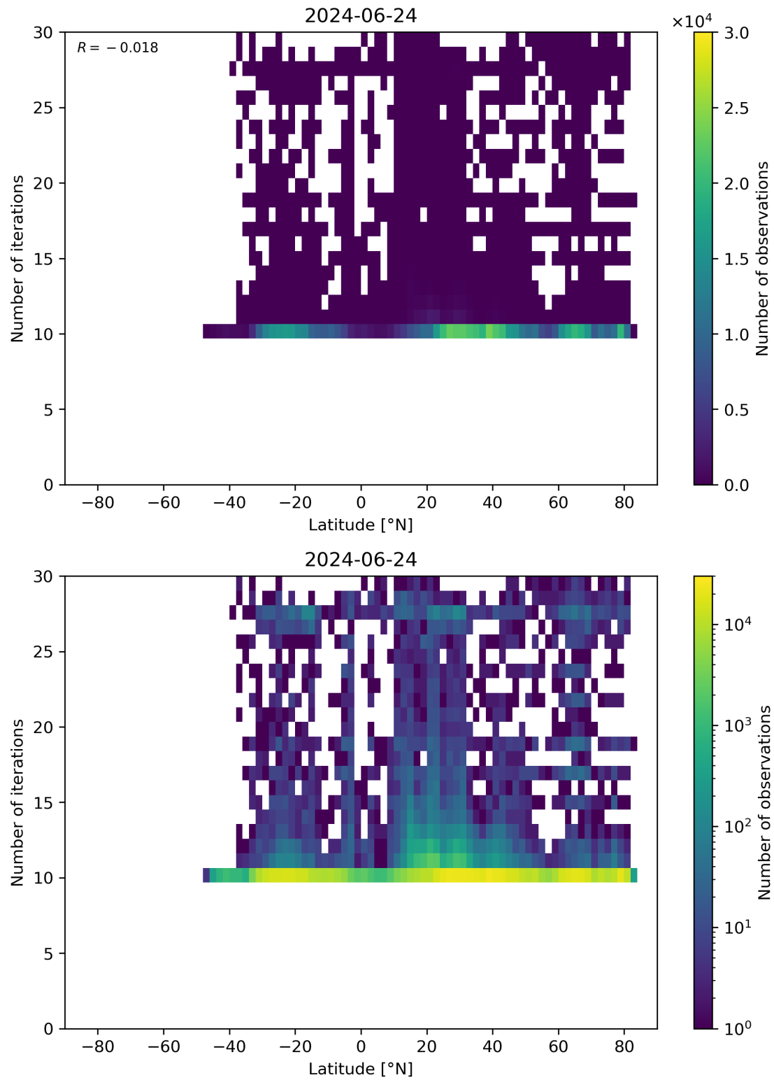
Figure 60: Scatter density plot of “Latitude” against “Number of iterations” for 2024-06-24 to 2024-06-25.
