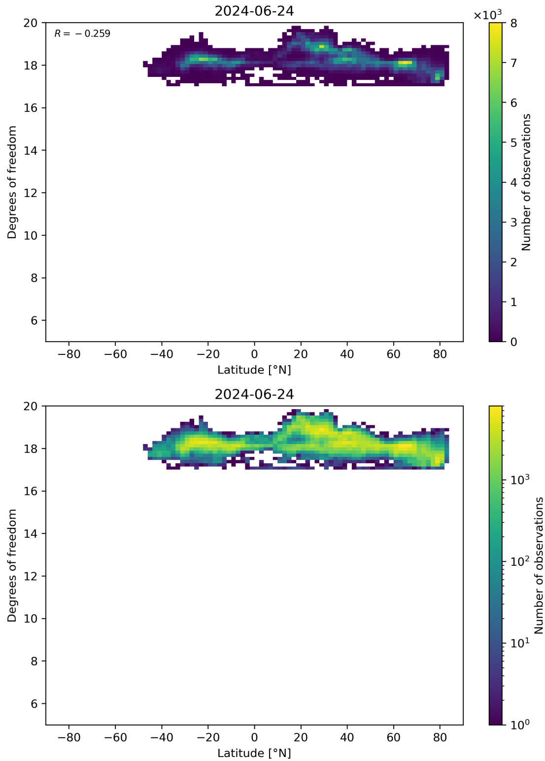
Figure 55: Scatter density plot of “Latitude” against “Degrees of freedom” for 2024-06-24 to 2024-06-25.
