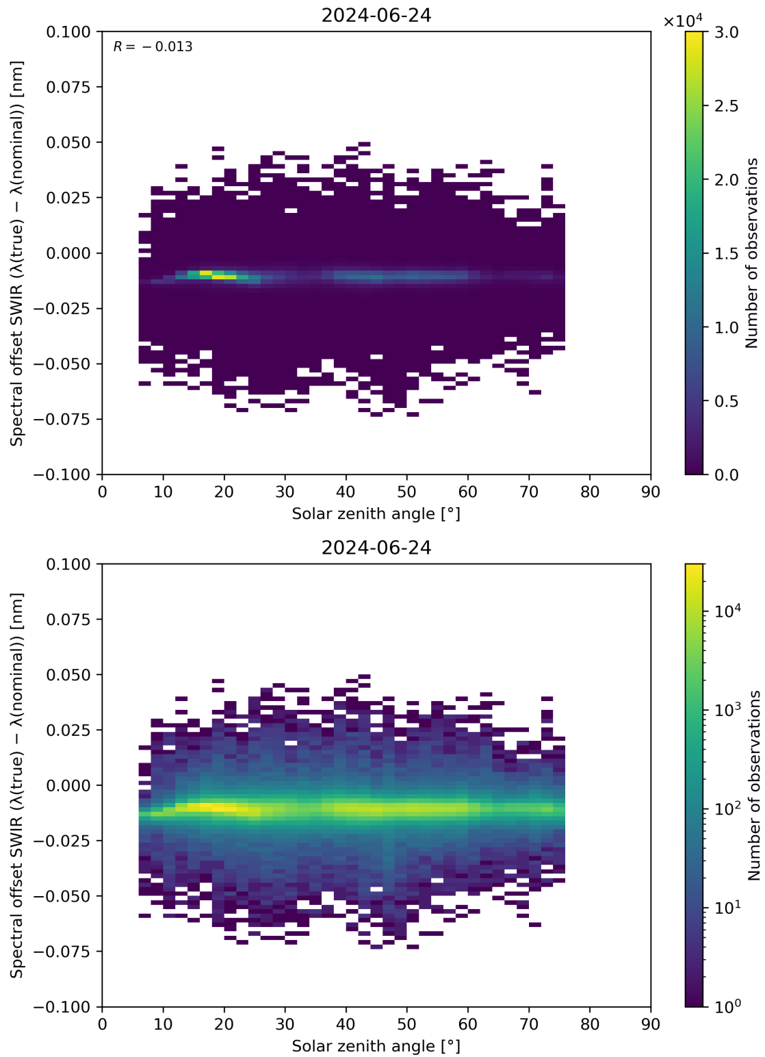
Figure 104: Scatter density plot of “Solar zenith angle” against “Spectral offset SWIR ( \lambda(\text{true}) - \lambda(\text{nominal}) )” for 2024-06-24 to 2024-06-25.
