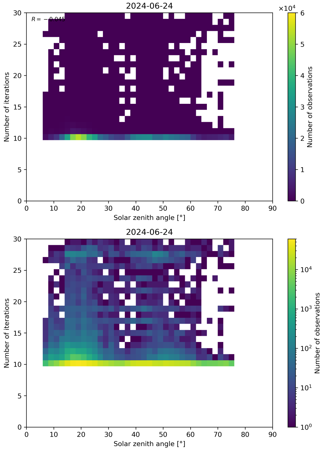
Figure 102: Scatter density plot of “Solar zenith angle” against “Number of iterations” for 2024-06-24 to 2024-06-25.
