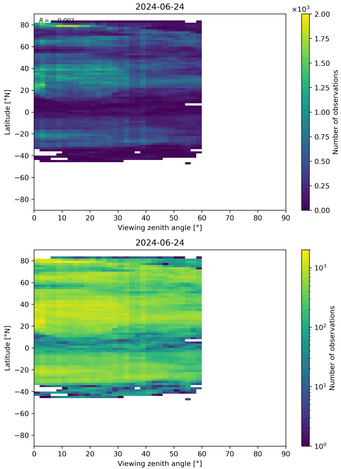
Figure 109: Scatter density plot of “Viewing zenith angle” against “Latitude” for 2024-06-24 to 2024-06-25.
