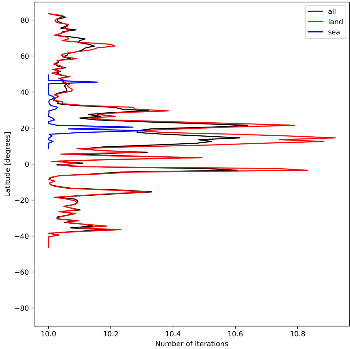
Figure 20: Zonal average of “Number of iterations” for 2024-06-24 to 2024-06-25.
