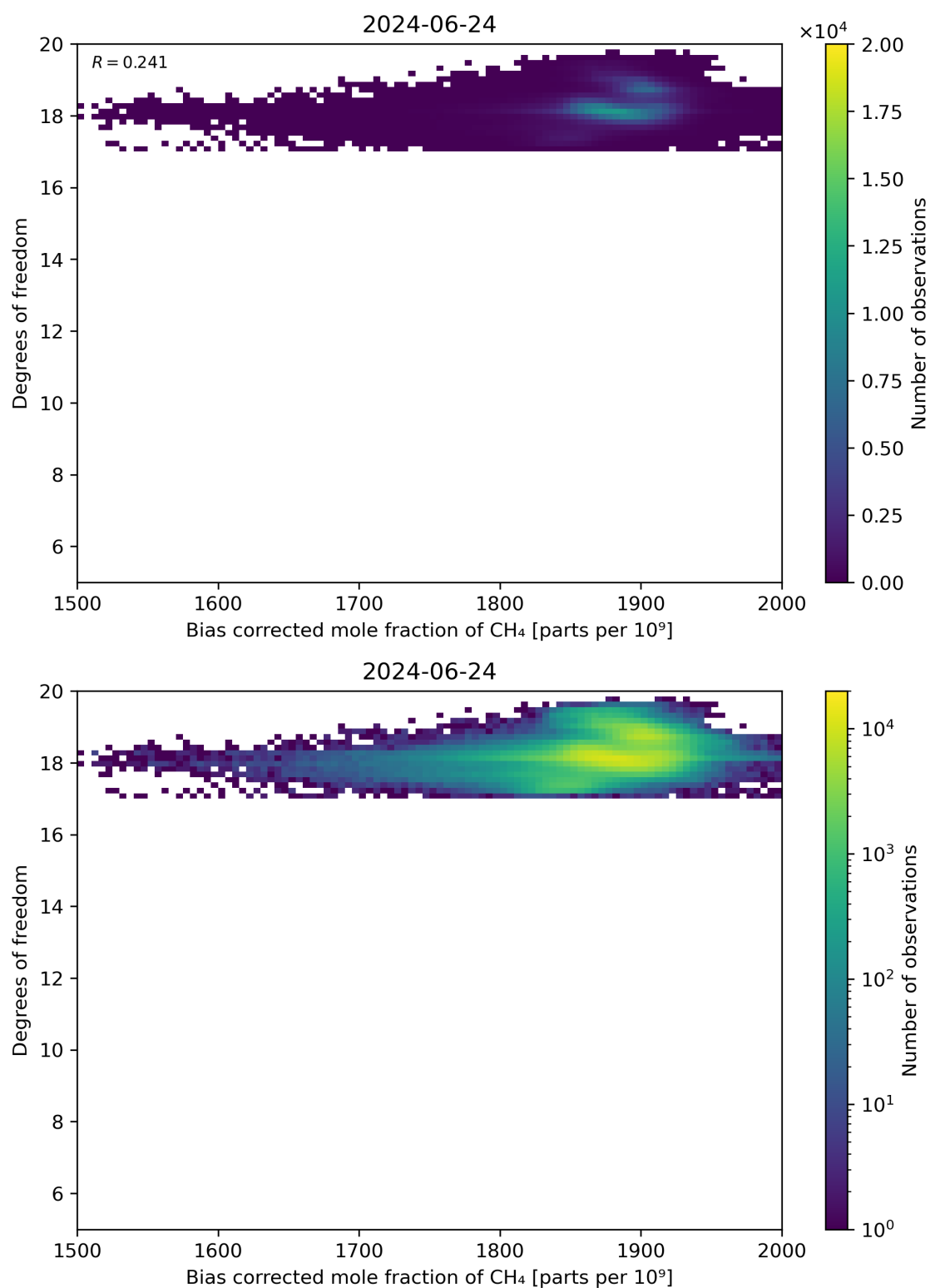
Figure 65: Scatter density plot of “Bias corrected mole fraction of CH 4 ” against “Degrees of freedom” for 2024-06-24 to 2024-06-25.
