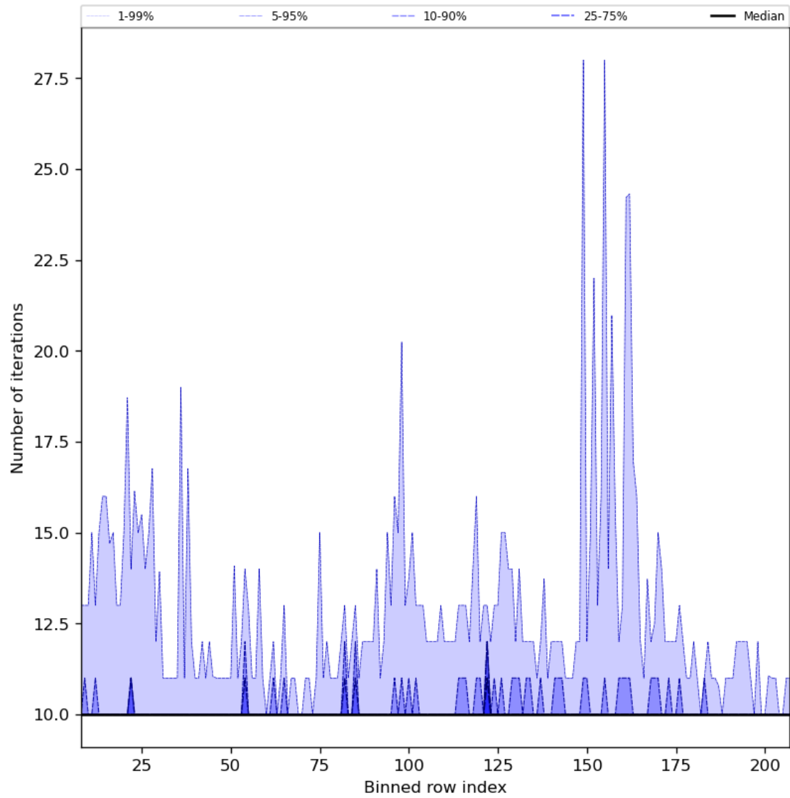
Figure 42: Along track statistics of “Number of iterations” for 2024-06-24 to 2024-06-25
