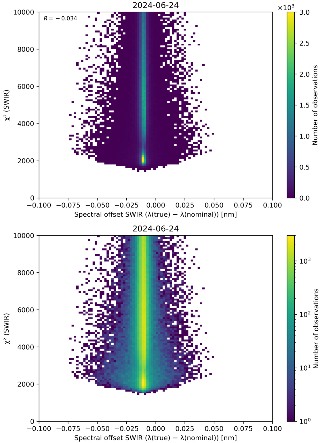
Figure 118: Scatter density plot of “Spectral offset SWIR ( \lambda(\text{true}) - \lambda(\text{nominal}) )” against “ \chi^2 (SWIR)” for 2024-06-24 to 2024-06-25.
