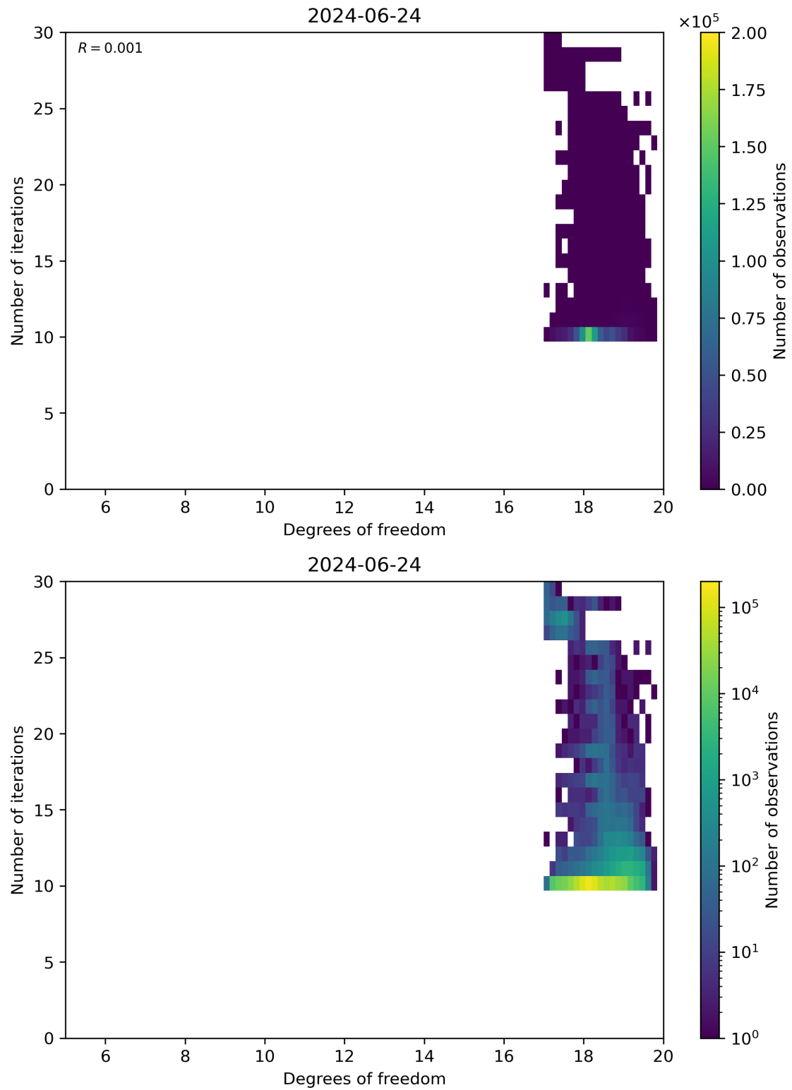
Figure 52: Scatter density plot of “Degrees of freedom” against “Number of iterations” for 2024-06-24 to 2024-06-25.
