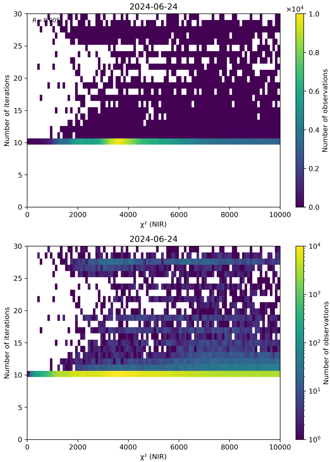
Figure 46: Scatter density plot of “ \chi^2 (NIR)” against “Number of iterations” for 2024-06-24 to 2024-06-25.
