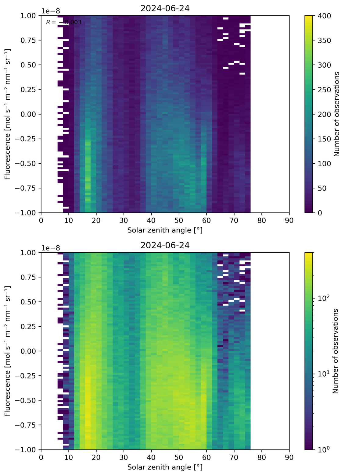
Figure 97: Scatter density plot of “Solar zenith angle” against “Fluorescence” for 2024-06-24 to 2024-06-25.
