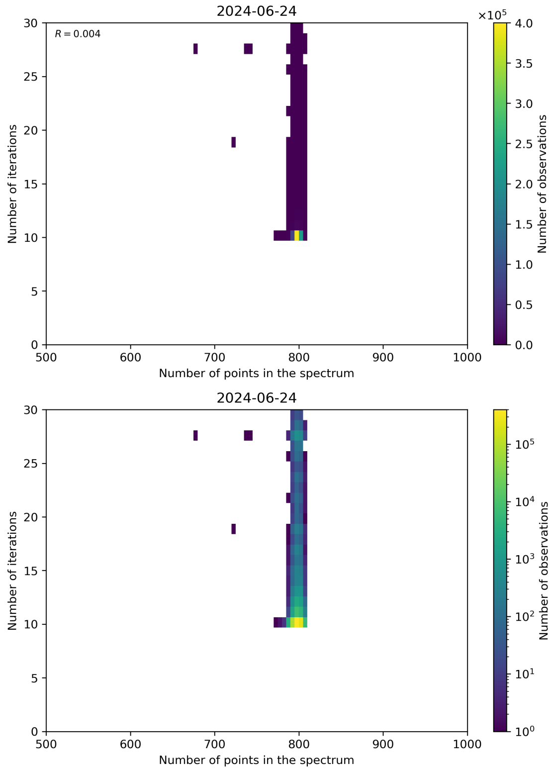
Figure 92: Scatter density plot of “Number of points in the spectrum” against “Number of iterations” for 2024-06-24 to 2024-06-25.
