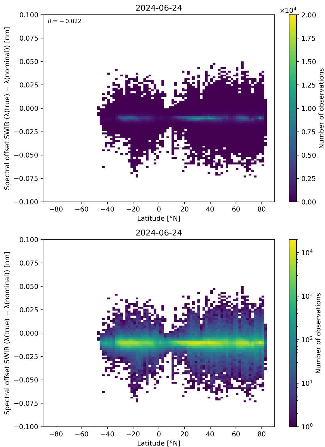
Figure 62: Scatter density plot of “Latitude” against “Spectral offset SWIR ( \lambda(\text{true}) - \lambda(\text{nominal}) )” for 2024-06-24 to 2024-06-25.
