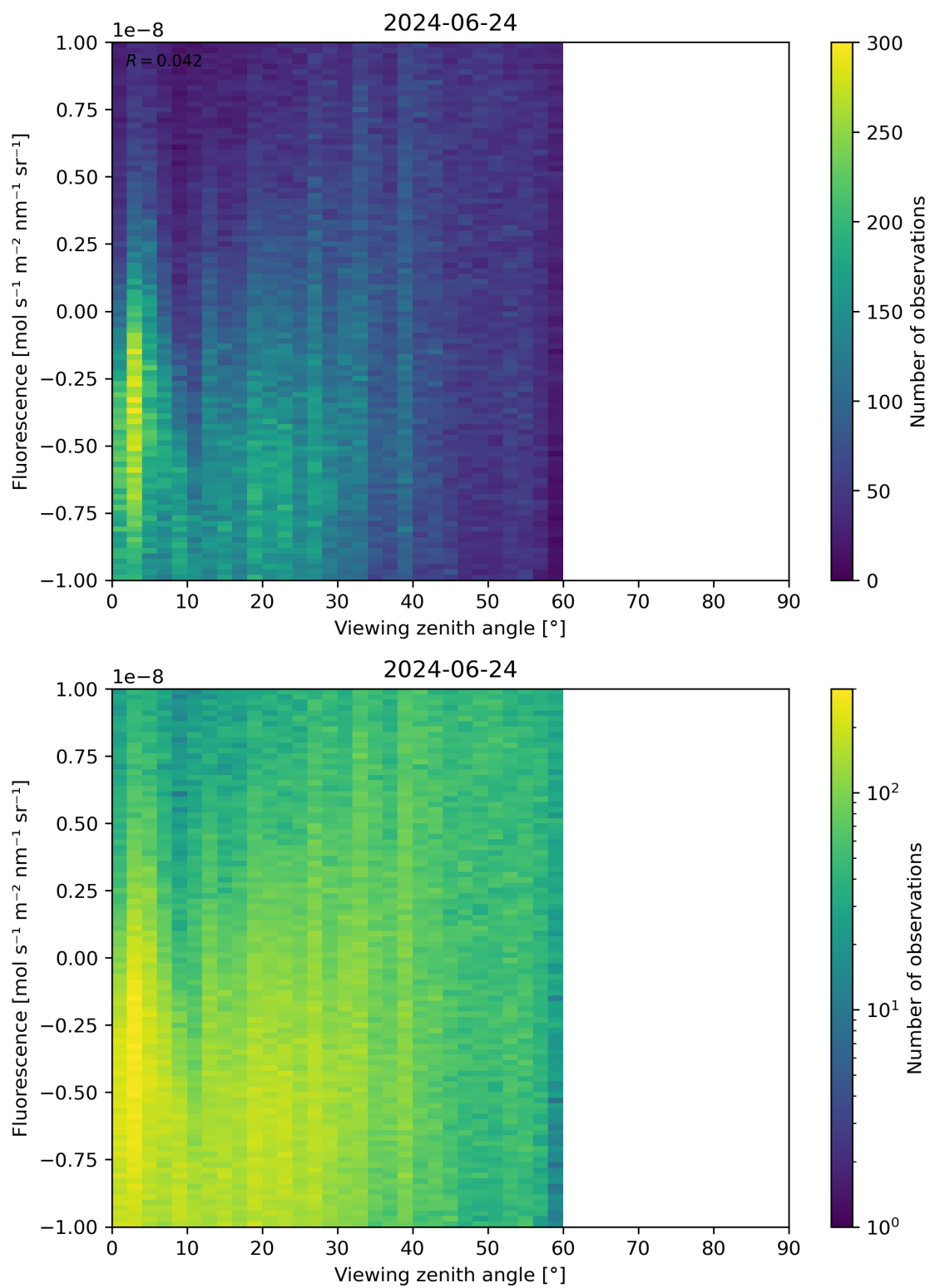
Figure 108: Scatter density plot of “Viewing zenith angle” against “Fluorescence” for 2024-06-24 to 2024-06-25.
