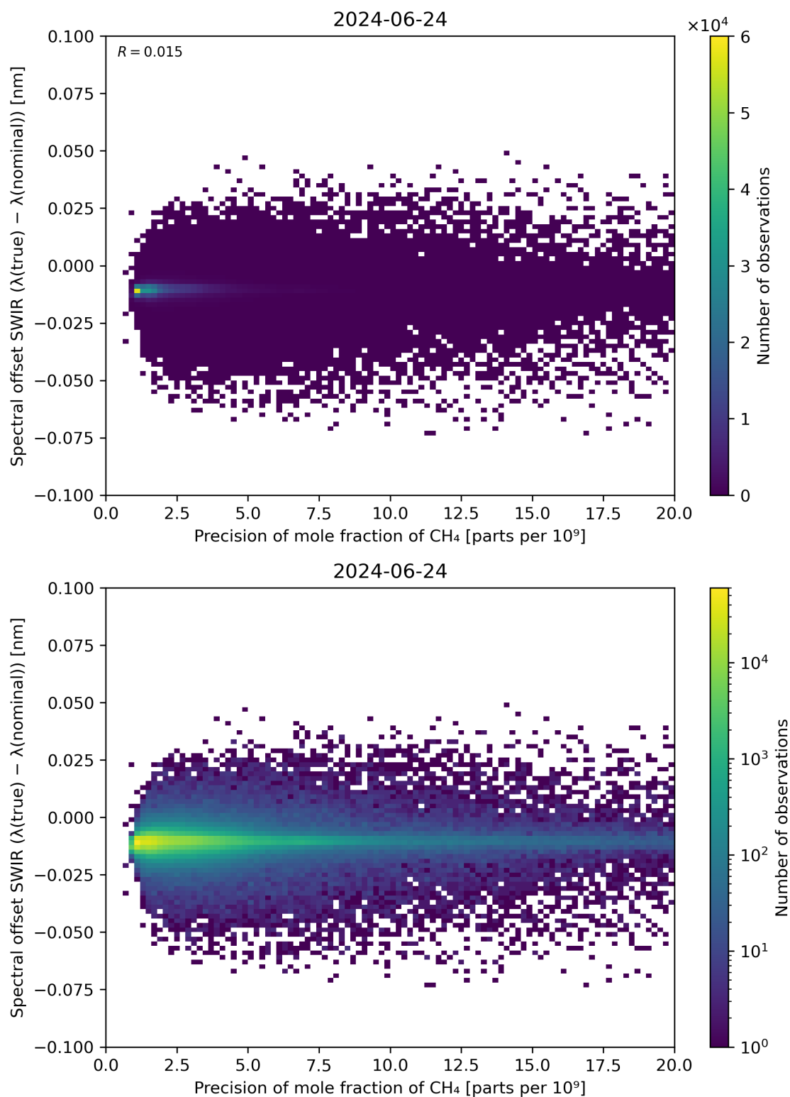
Figure 85: Scatter density plot of “Precision of mole fraction of CH 4 ” against “Spectral offset SWIR ( \lambda(\text{true}) - \lambda(\text{nominal}) )” for 2024-06-24 to 2024-06-25.
