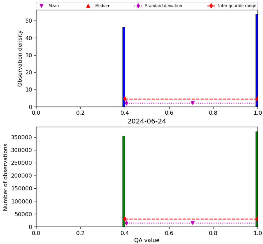
Figure 22: Histogram of “QA value” for 2024-06-24 to 2024-06-25
