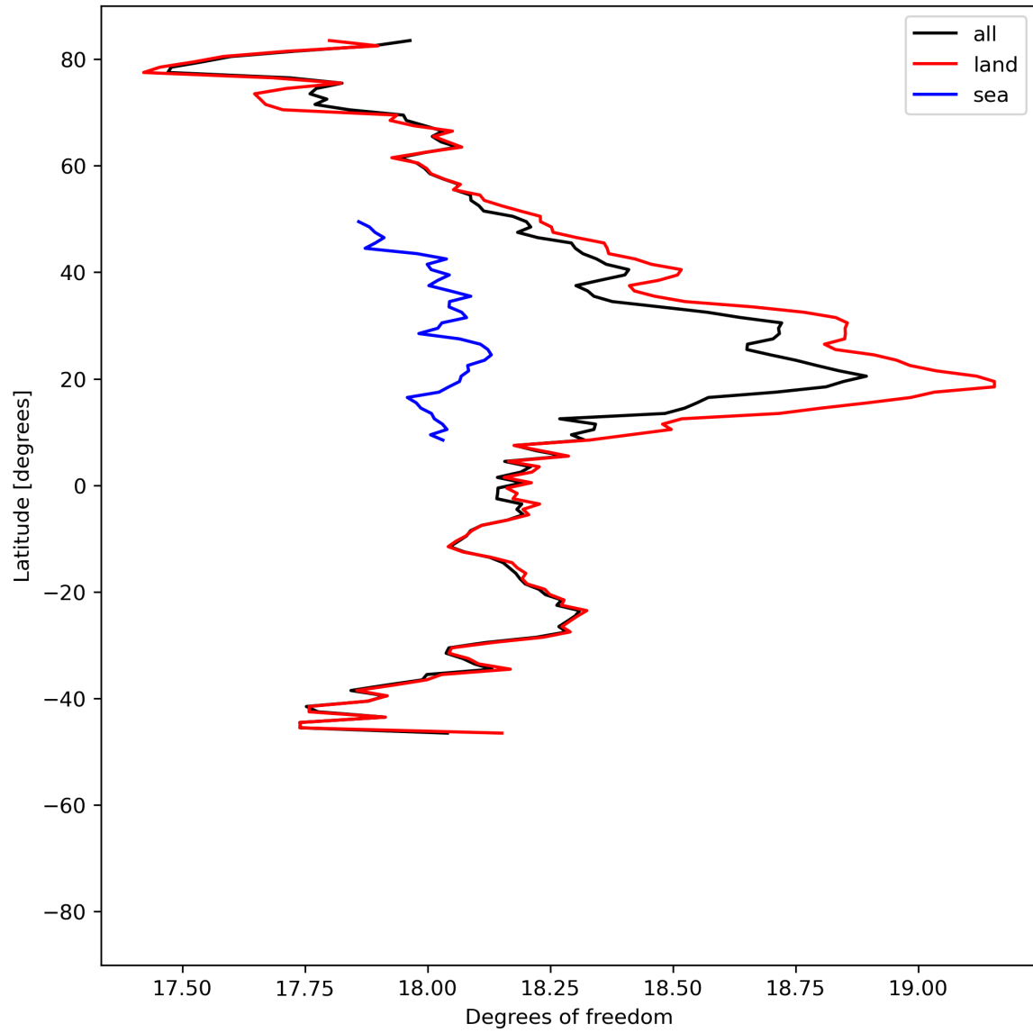
Figure 19: Zonal average of “Degrees of freedom” for 2024-06-24 to 2024-06-25.
