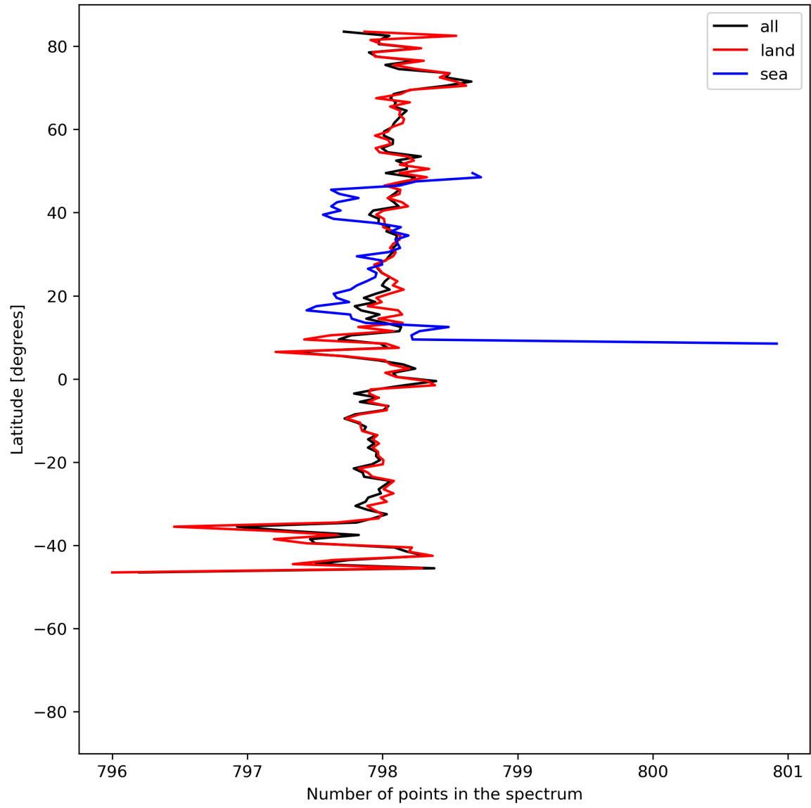
Figure 15: Zonal average of “Number of points in the spectrum” for 2024-06-24 to 2024-06-25.
