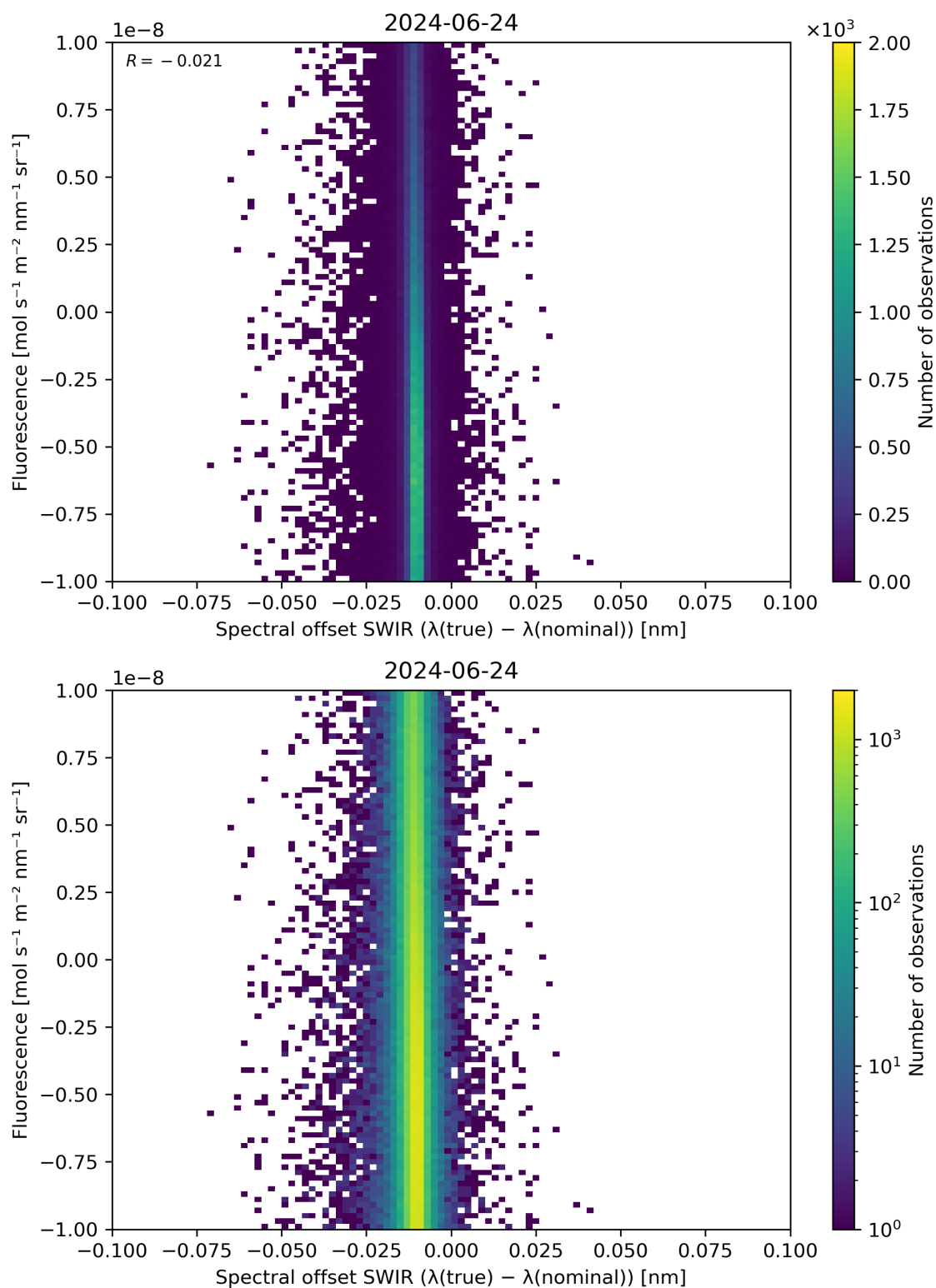
Figure 120: Scatter density plot of “Spectral offset SWIR ( \lambda(\text{true}) - \lambda(\text{nominal}) )” against “Fluorescence” for 2024-06-24 to 2024-06-25.
