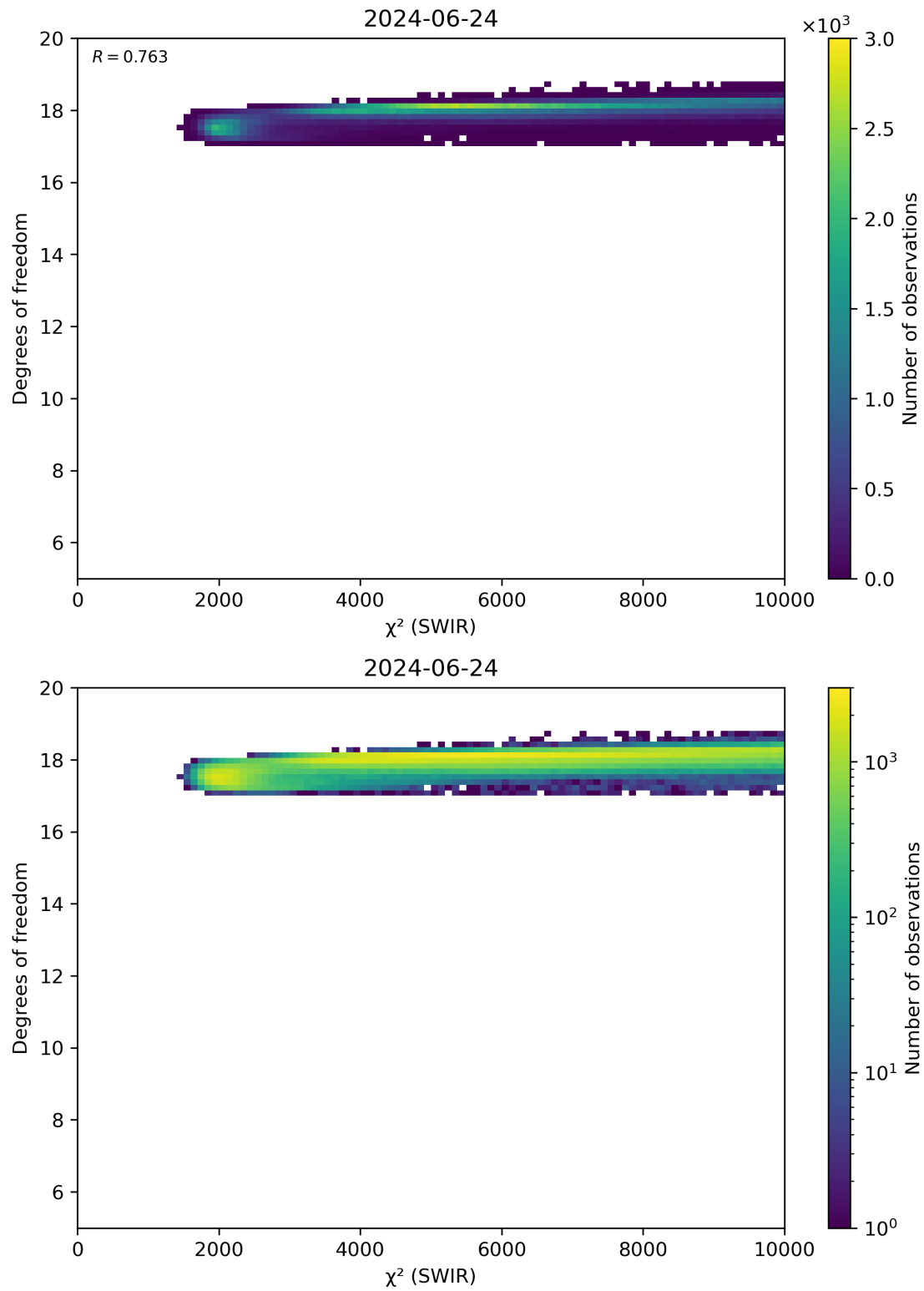
Figure 48: Scatter density plot of “ \chi^2 (SWIR)” against “Degrees of freedom” for 2024-06-24 to 2024-06-25.
