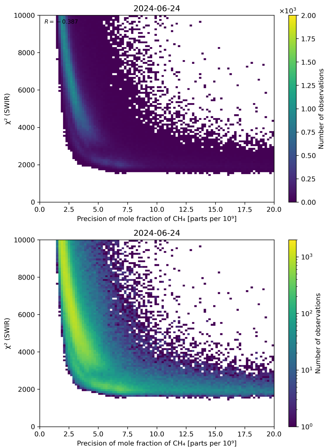
Figure 79: Scatter density plot of “Precision of mole fraction of \text{CH}_4 ” against “ \chi^2 (SWIR)” for 2024-06-24 to 2024-06-25.
