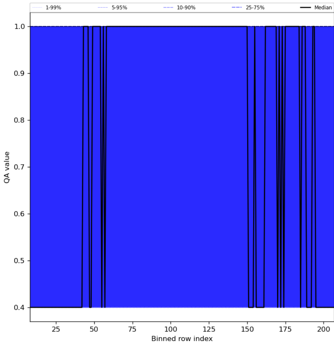
Figure 33: Along track statistics of “QA value” for 2024-06-24 to 2024-06-25
