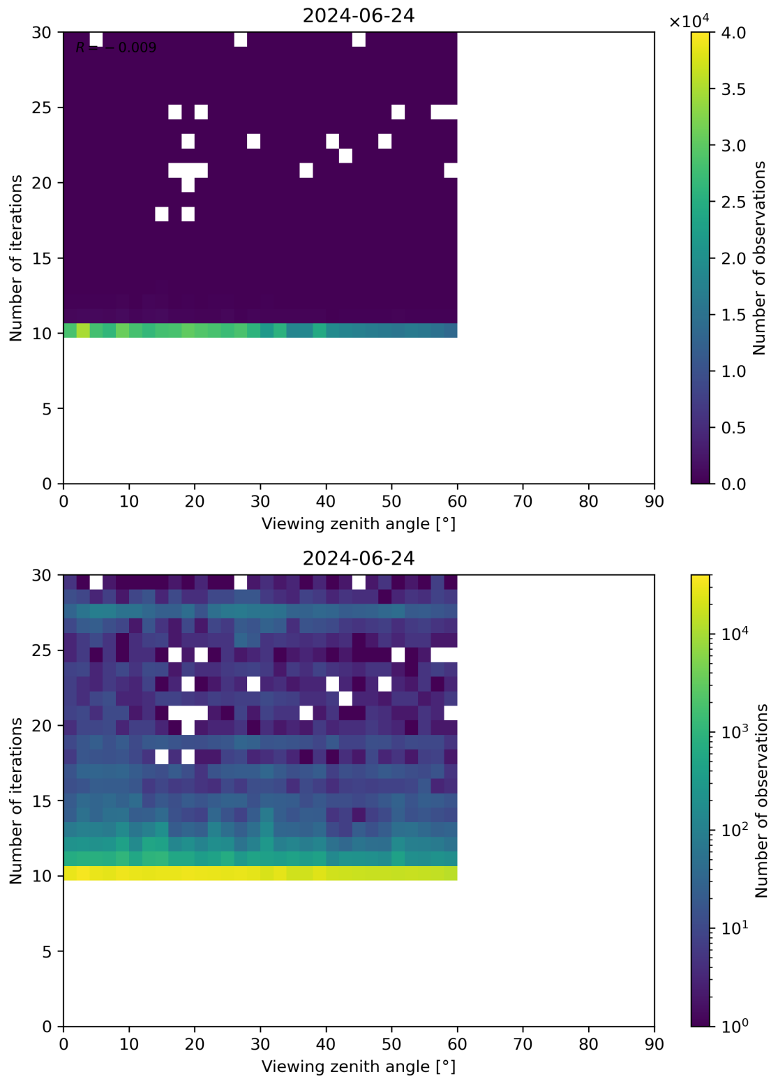
Figure 113: Scatter density plot of “Viewing zenith angle” against “Number of iterations” for 2024-06-24 to 2024-06-25.
