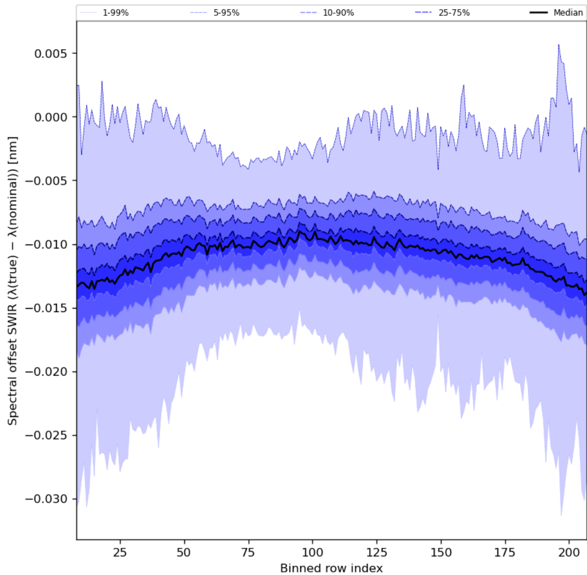
Figure 38: Along track statistics of “Spectral offset SWIR ( \lambda(\text{true}) - \lambda(\text{nominal}) )” for 2024-06-24 to 2024-06-25
