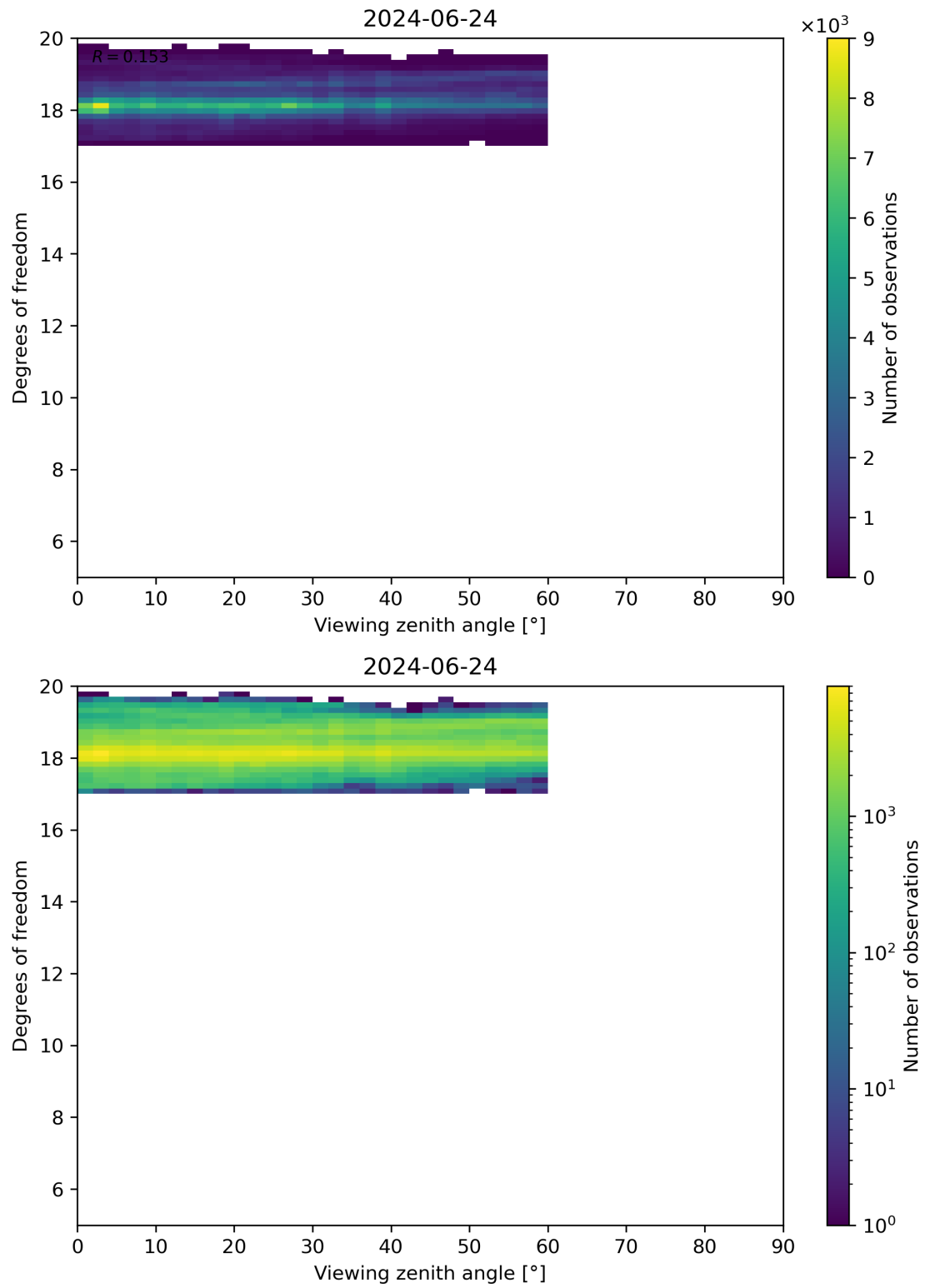
Figure 107: Scatter density plot of “Viewing zenith angle” against “Degrees of freedom” for 2024-06-24 to 2024-06-25.
