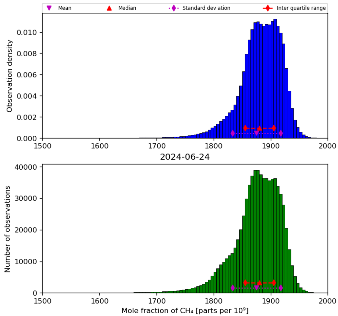
Figure 23: Histogram of “Mole fraction of CH 4 ” for 2024-06-24 to 2024-06-25
