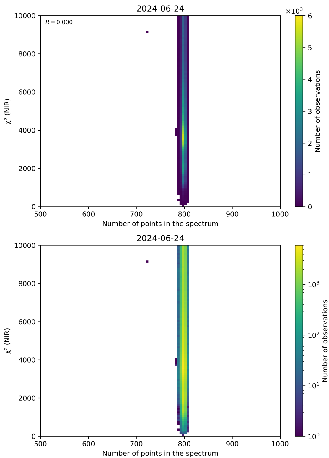
Figure 88: Scatter density plot of “Number of points in the spectrum” against “ \chi^2 (NIR)” for 2024-06-24 to 2024-06-25.
