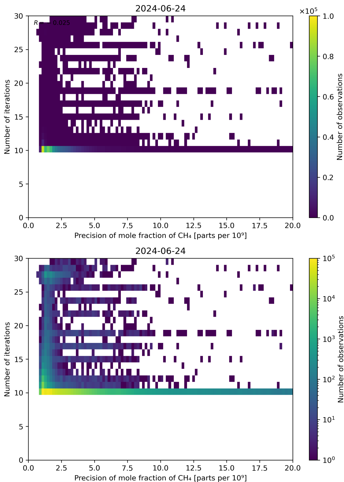
Figure 83: Scatter density plot of “Precision of mole fraction of CH 4 ” against “Number of iterations” for 2024-06-24 to 2024-06-25.
