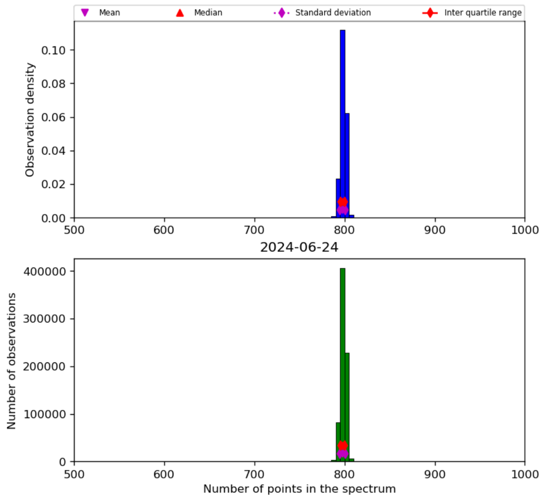
Figure 26: Histogram of “Number of points in the spectrum” for 2024-06-24 to 2024-06-25
