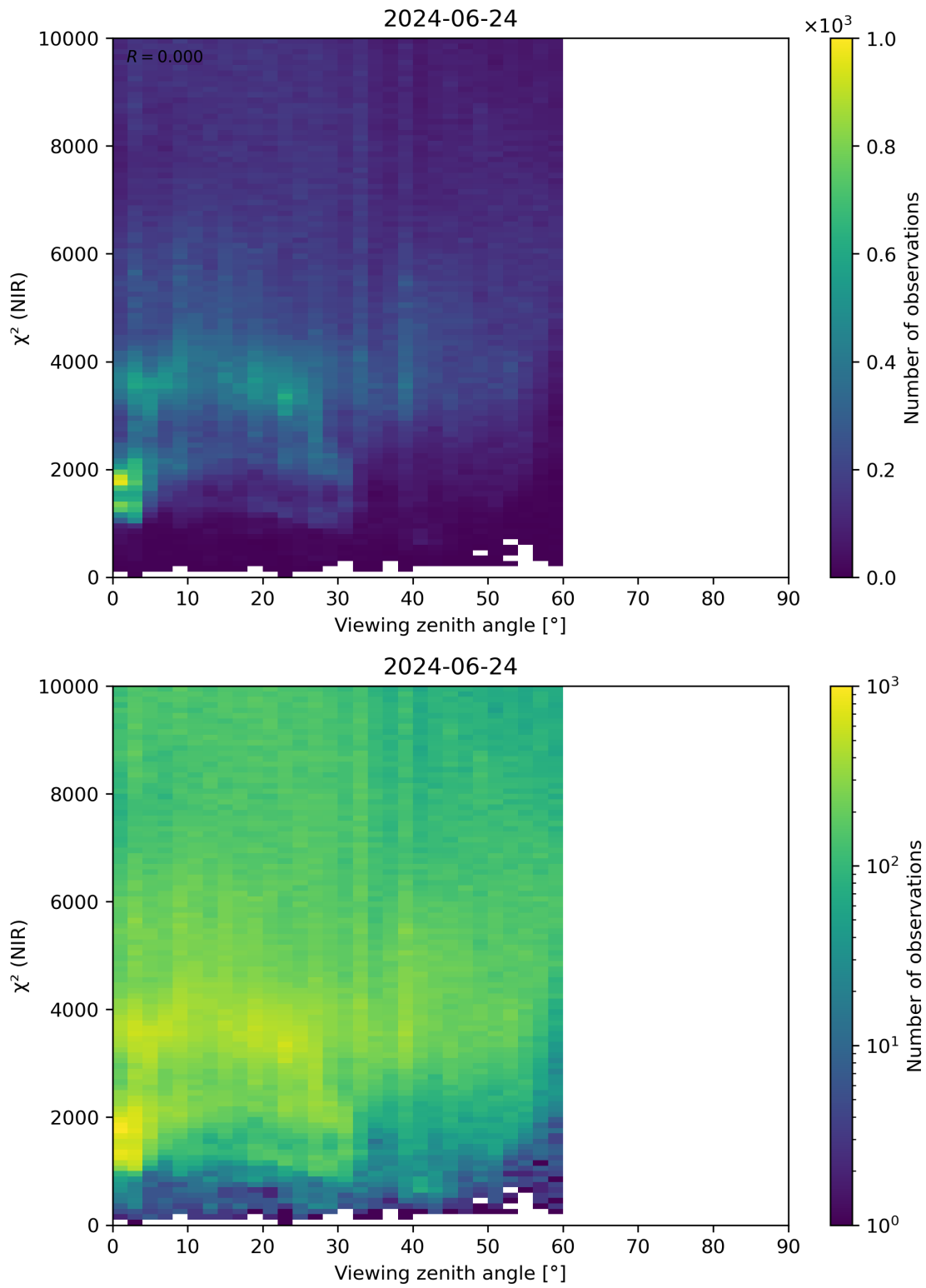
Figure 105: Scatter density plot of “Viewing zenith angle” against “ \chi^2 (NIR)” for 2024-06-24 to 2024-06-25.
