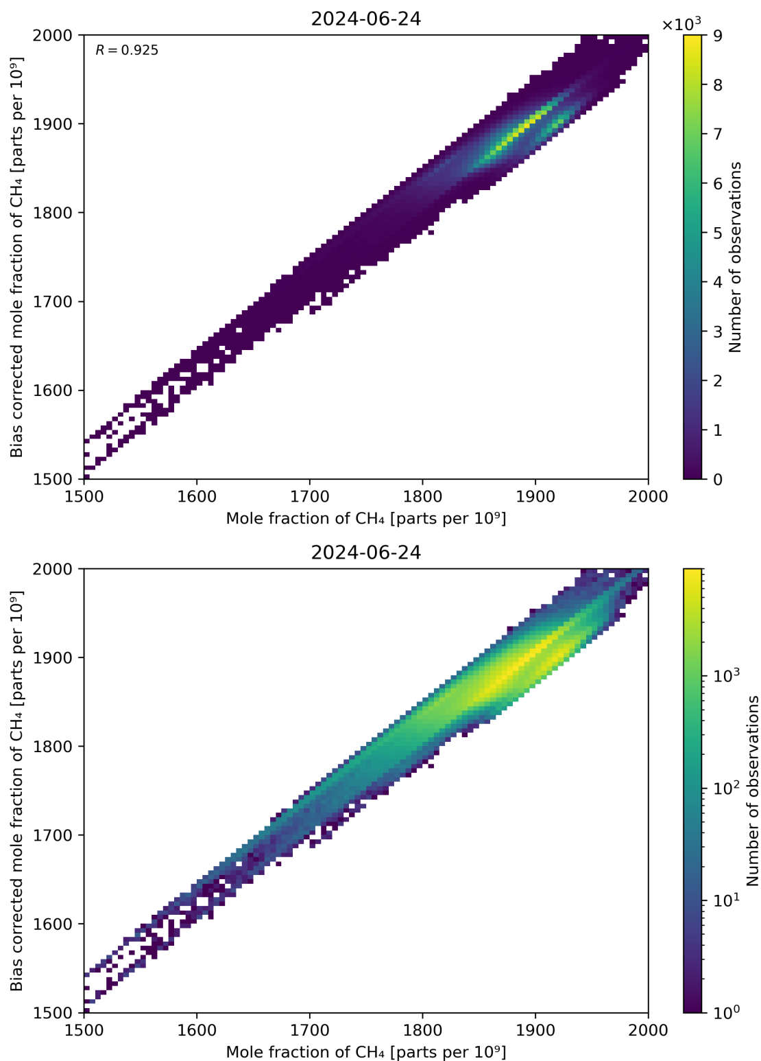
Figure 74: Scatter density plot of “Mole fraction of CH 4 ” against “Bias corrected mole fraction of CH 4 ” for 2024-06-24 to 2024-06-25.
