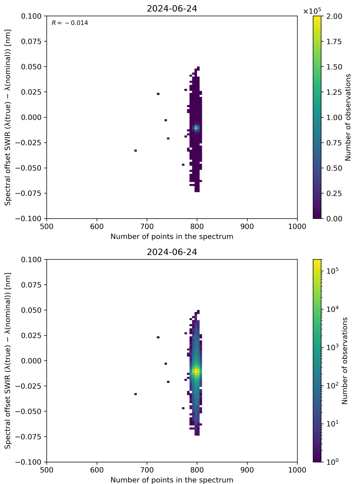
Figure 93: Scatter density plot of “Number of points in the spectrum” against “Spectral offset SWIR ( \lambda(\text{true}) - \lambda(\text{nominal}) )” for 2024-06-24 to 2024-06-25.
