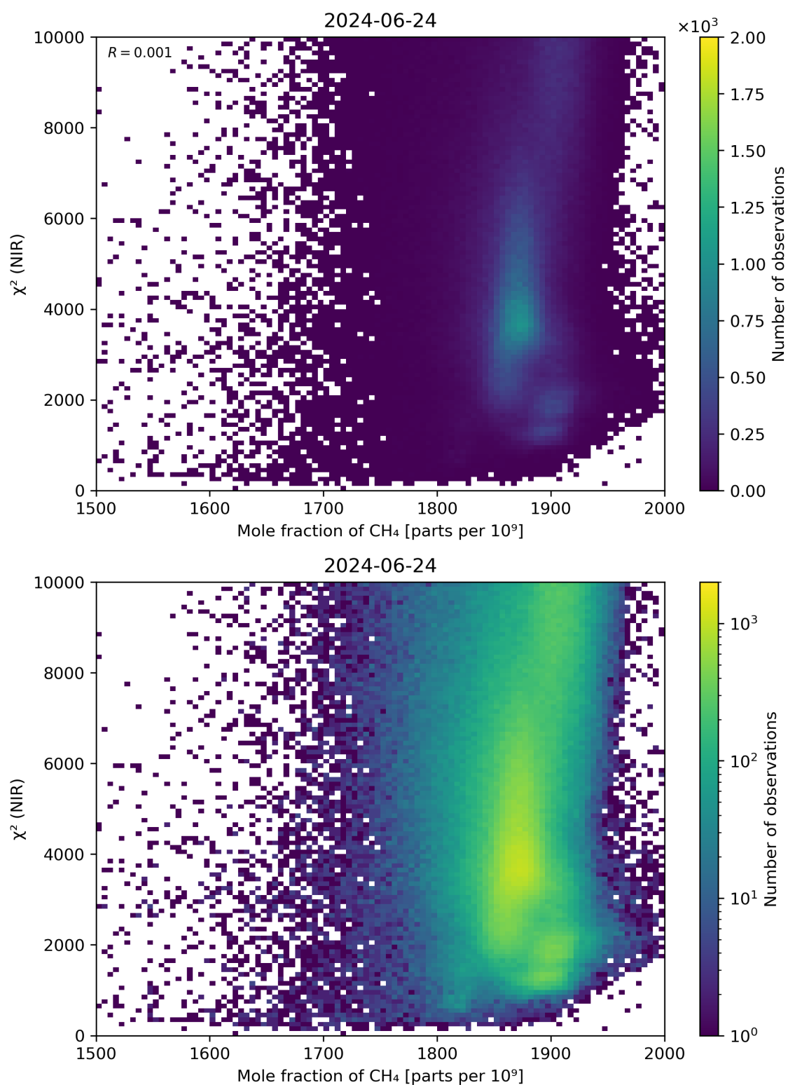
Figure 70: Scatter density plot of “Mole fraction of \text{CH}_4 ” against “ \chi^2 (NIR)” for 2024-06-24 to 2024-06-25.
