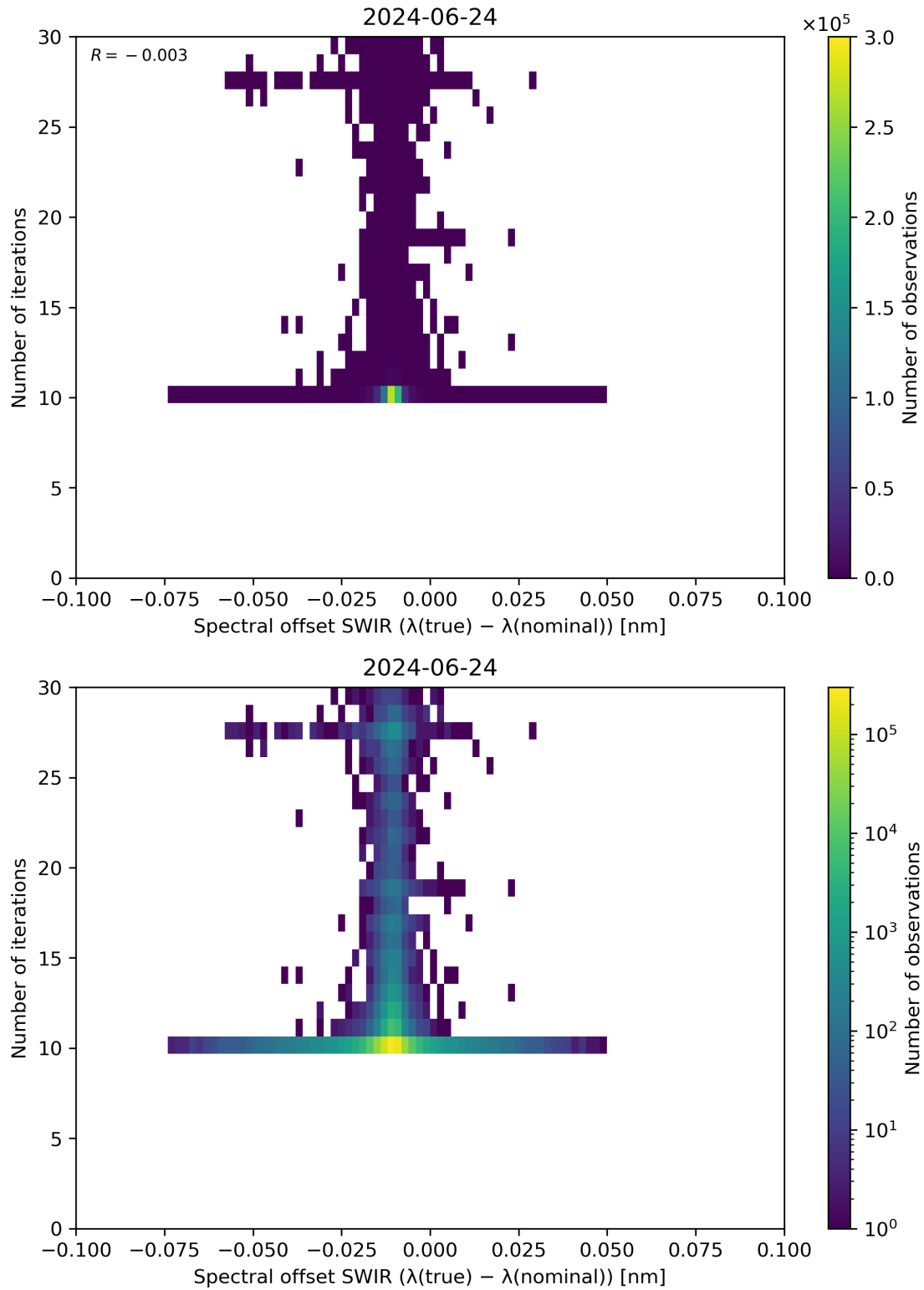
Figure 121: Scatter density plot of “Spectral offset SWIR ( \lambda(\text{true}) - \lambda(\text{nominal}) )” against “Number of iterations” for 2024-06-24 to 2024-06-25.
