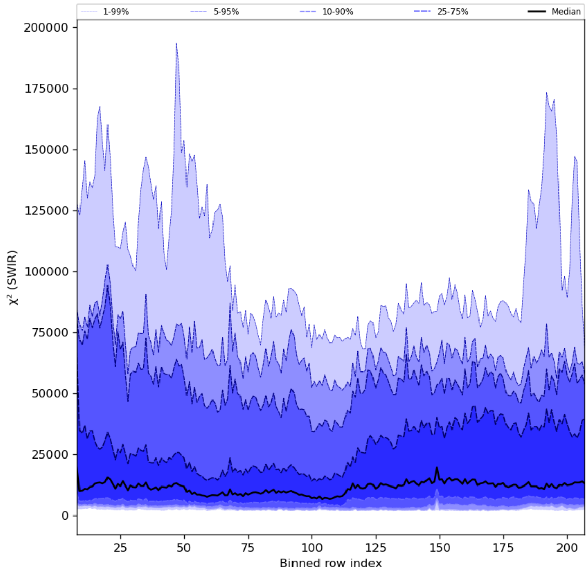
Figure 39: Along track statistics of “ \chi^2 (SWIR)” for 2024-06-24 to 2024-06-25
