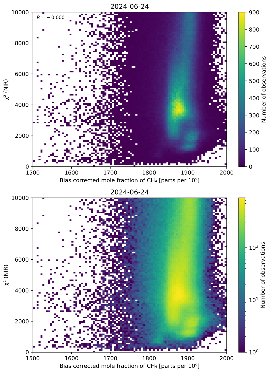
Figure 63: Scatter density plot of “Bias corrected mole fraction of CH 4 ” against “ \chi^2 (NIR)” for 2024-06-24 to 2024-06-25.
