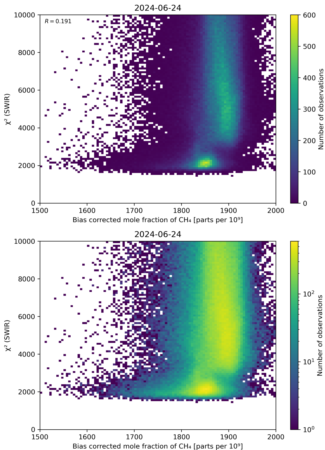
Figure 64: Scatter density plot of “Bias corrected mole fraction of \text{CH}_4 ” against “ \chi^2 (SWIR)” for 2024-06-24 to 2024-06-25.
