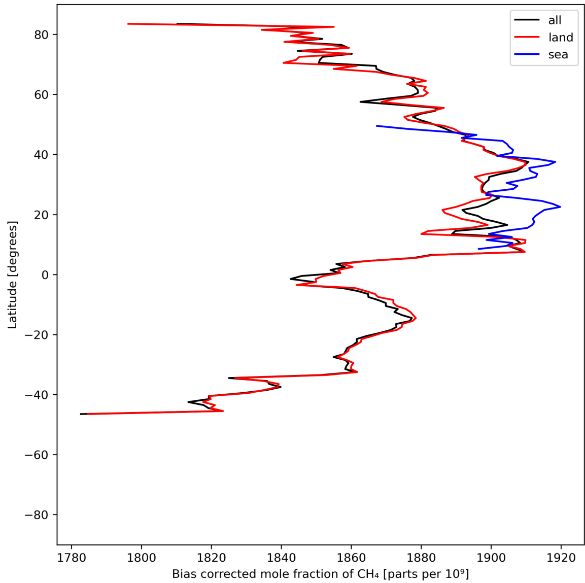
Figure 14: Zonal average of “Bias corrected mole fraction of CH 4 ” for 2024-06-24 to 2024-06-25.
