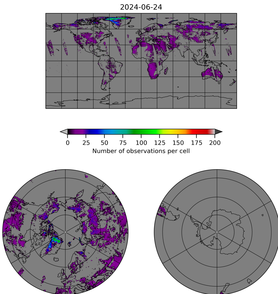
Figure 10: Map of the number of observations for 2024-06-24 to 2024-06-25
