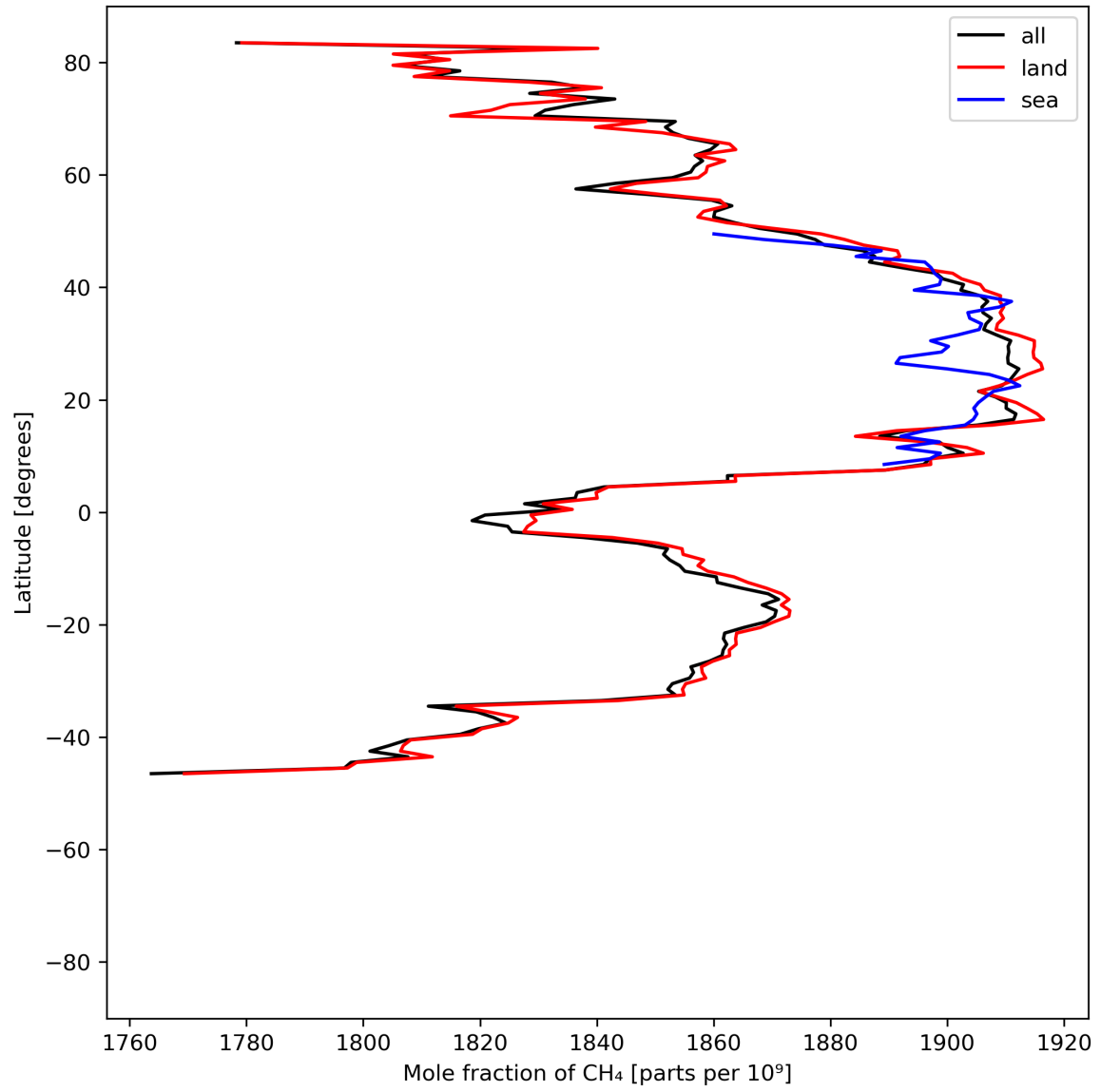
Figure 12: Zonal average of “Mole fraction of \text{CH}_4 ” for 2024-06-24 to 2024-06-25.
