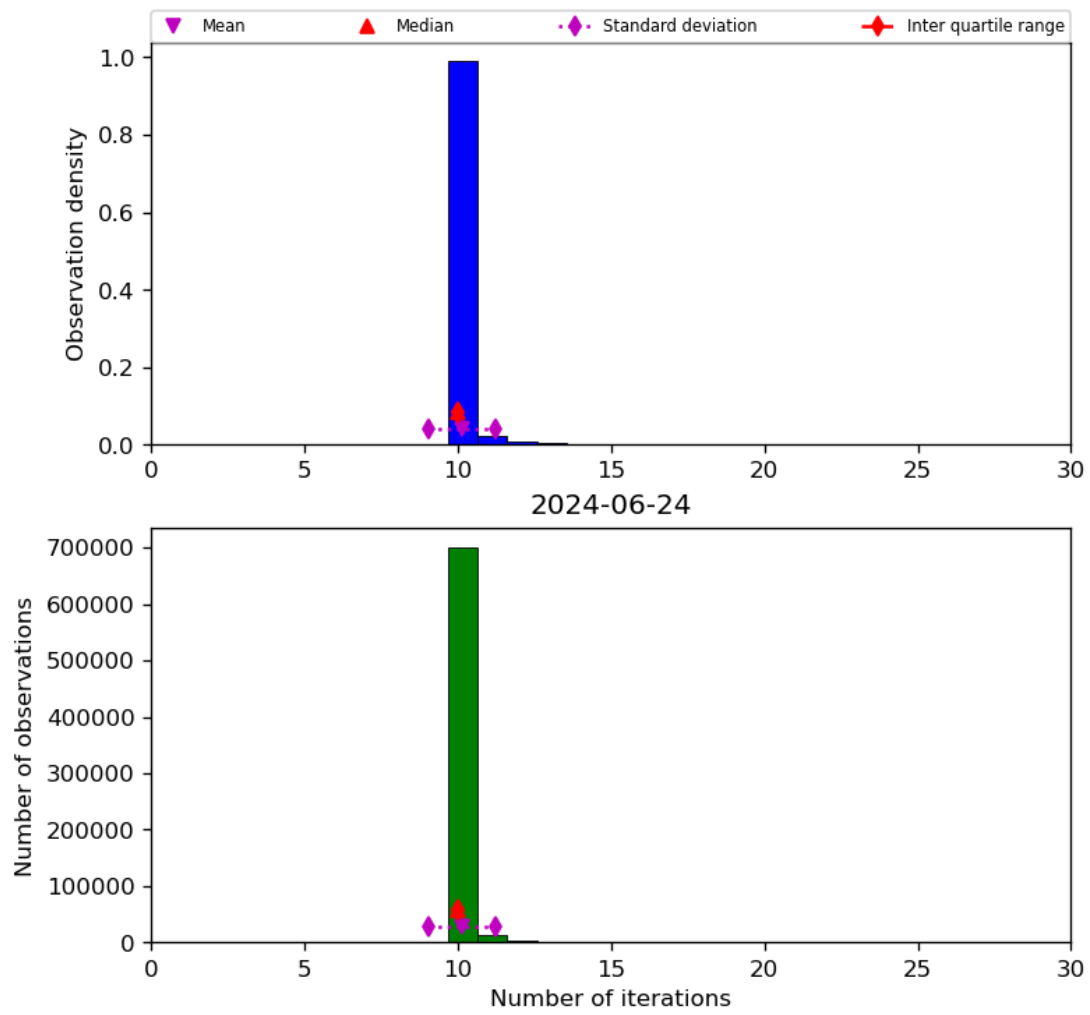
Figure 31: Histogram of “Number of iterations” for 2024-06-24 to 2024-06-25
