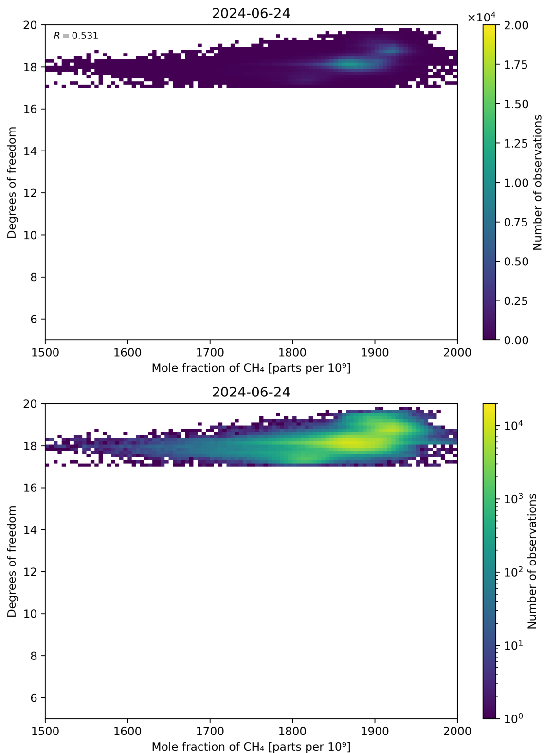
Figure 72: Scatter density plot of “Mole fraction of CH 4 ” against “Degrees of freedom” for 2024-06-24 to 2024-06-25.
