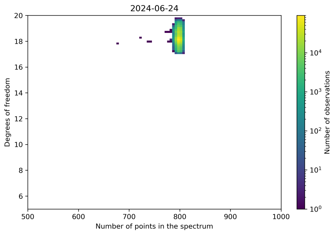
Figure 90: Scatter density plot of “Number of points in the spectrum” against “Degrees of freedom” for 2024-06-24 to 2024-06-25.
