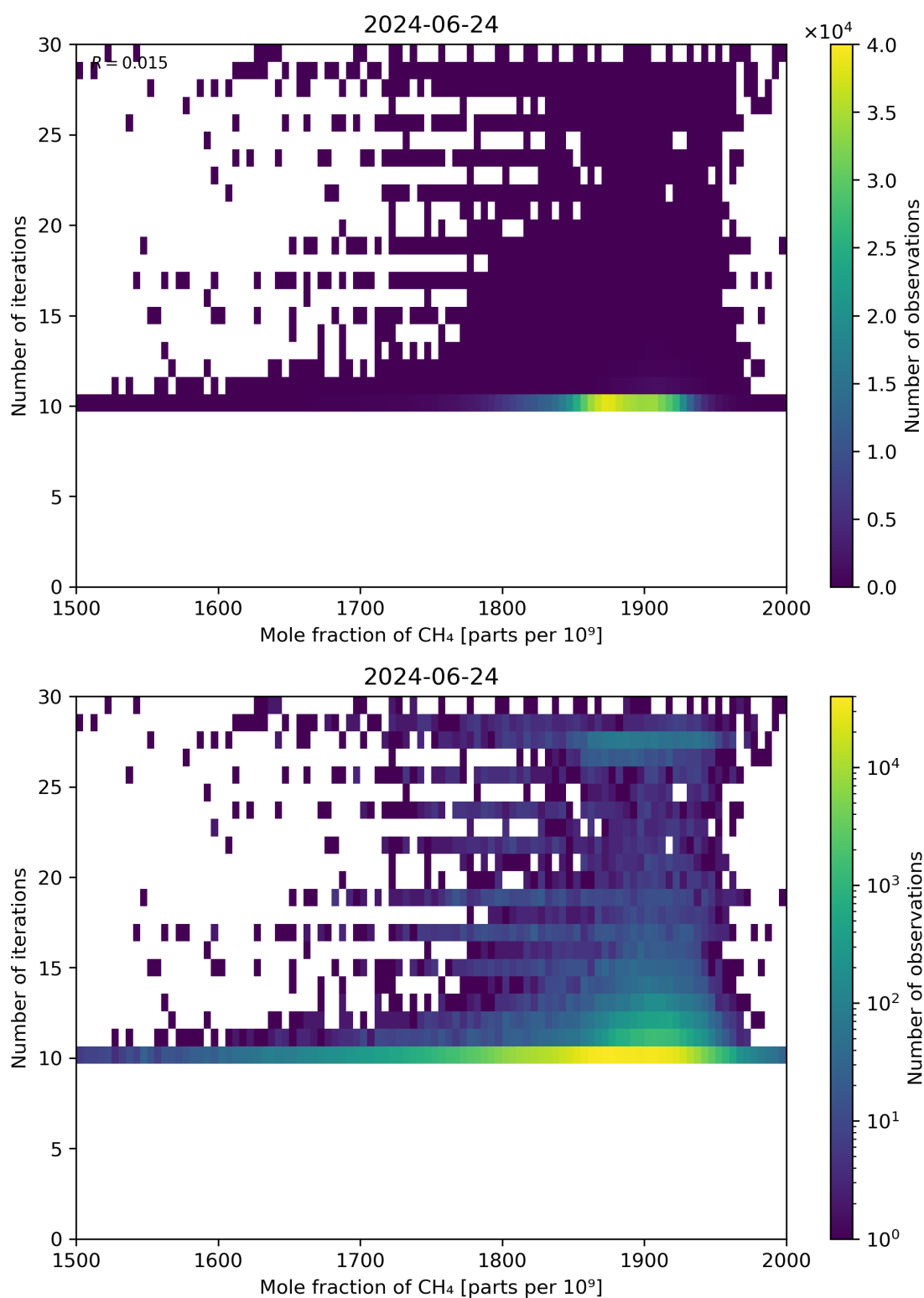
Figure 76: Scatter density plot of “Mole fraction of CH 4 ” against “Number of iterations” for 2024-06-24 to 2024-06-25.
