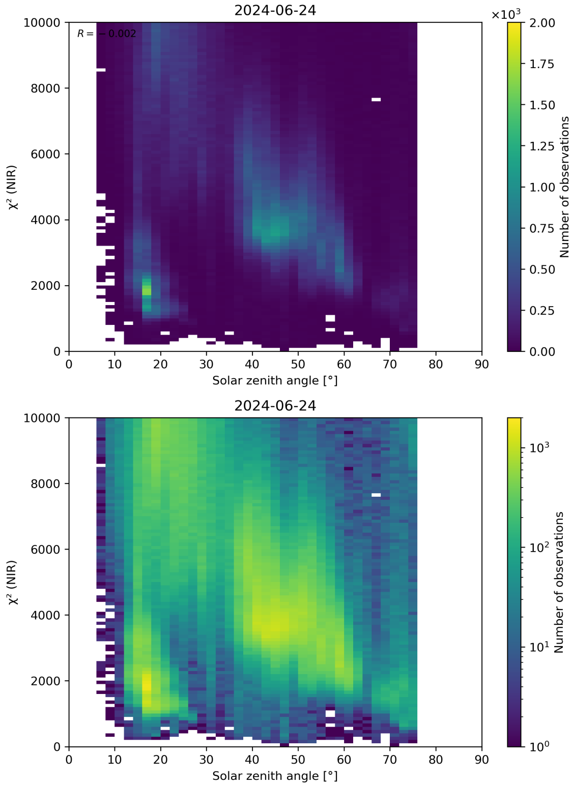
Figure 94: Scatter density plot of “Solar zenith angle” against “ \chi^2 (NIR)” for 2024-06-24 to 2024-06-25.
