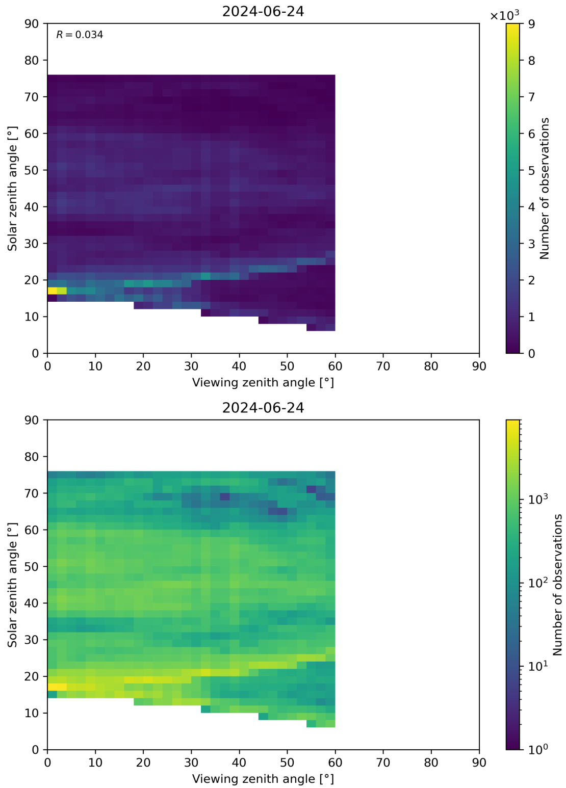
Figure 115: Scatter density plot of “Viewing zenith angle” against “Solar zenith angle” for 2024-06-24 to 2024-06-25.
