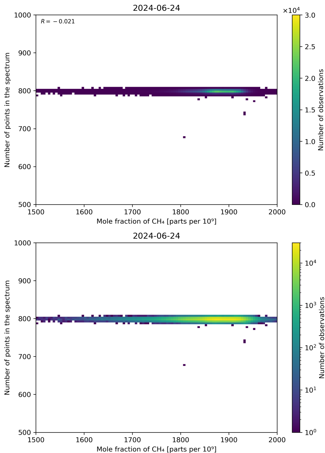
Figure 77: Scatter density plot of “Mole fraction of CH 4 ” against “Number of points in the spectrum” for 2024-06-24 to 2024-06-25.
