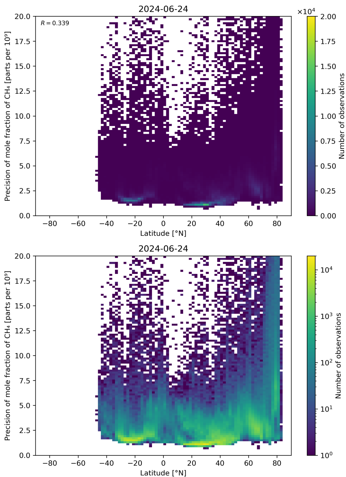
Figure 59: Scatter density plot of “Latitude” against “Precision of mole fraction of \text{CH}_4 ” for 2024-06-24 to 2024-06-25.
