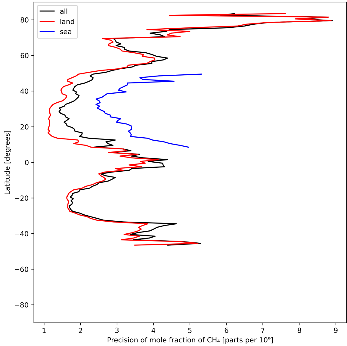
Figure 13: Zonal average of “Precision of mole fraction of CH 4 ” for 2024-06-24 to 2024-06-25.
