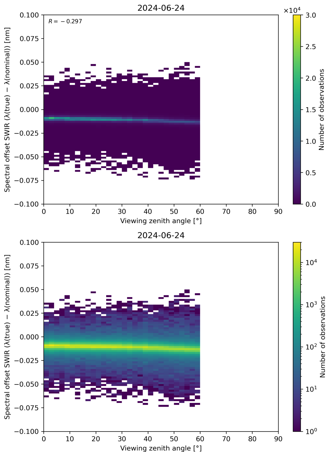
Figure 116: Scatter density plot of “Viewing zenith angle” against “Spectral offset SWIR ( \lambda(\text{true}) - \lambda(\text{nominal}) )” for 2024-06-24 to 2024-06-25.
