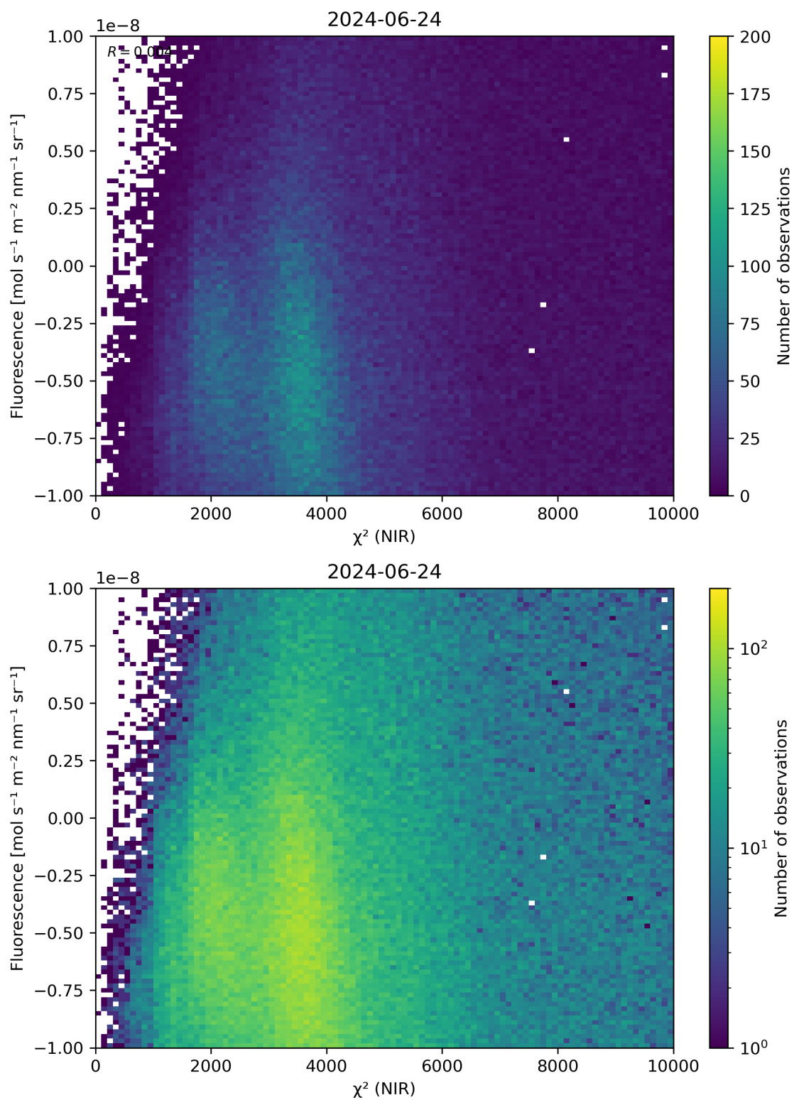
Figure 45: Scatter density plot of “ \chi^2 (NIR)” against “Fluorescence” for 2024-06-24 to 2024-06-25.
