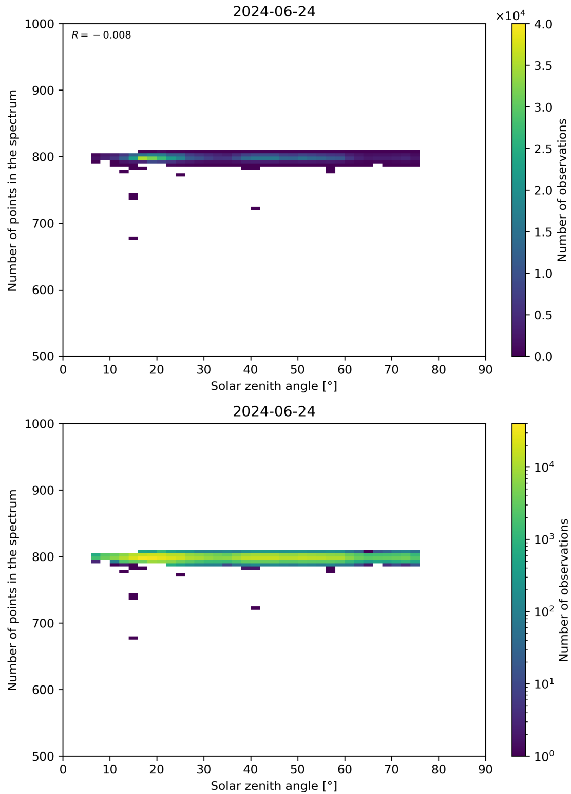
Figure 103: Scatter density plot of “Solar zenith angle” against “Number of points in the spectrum” for 2024-06-24 to 2024-06-25.
