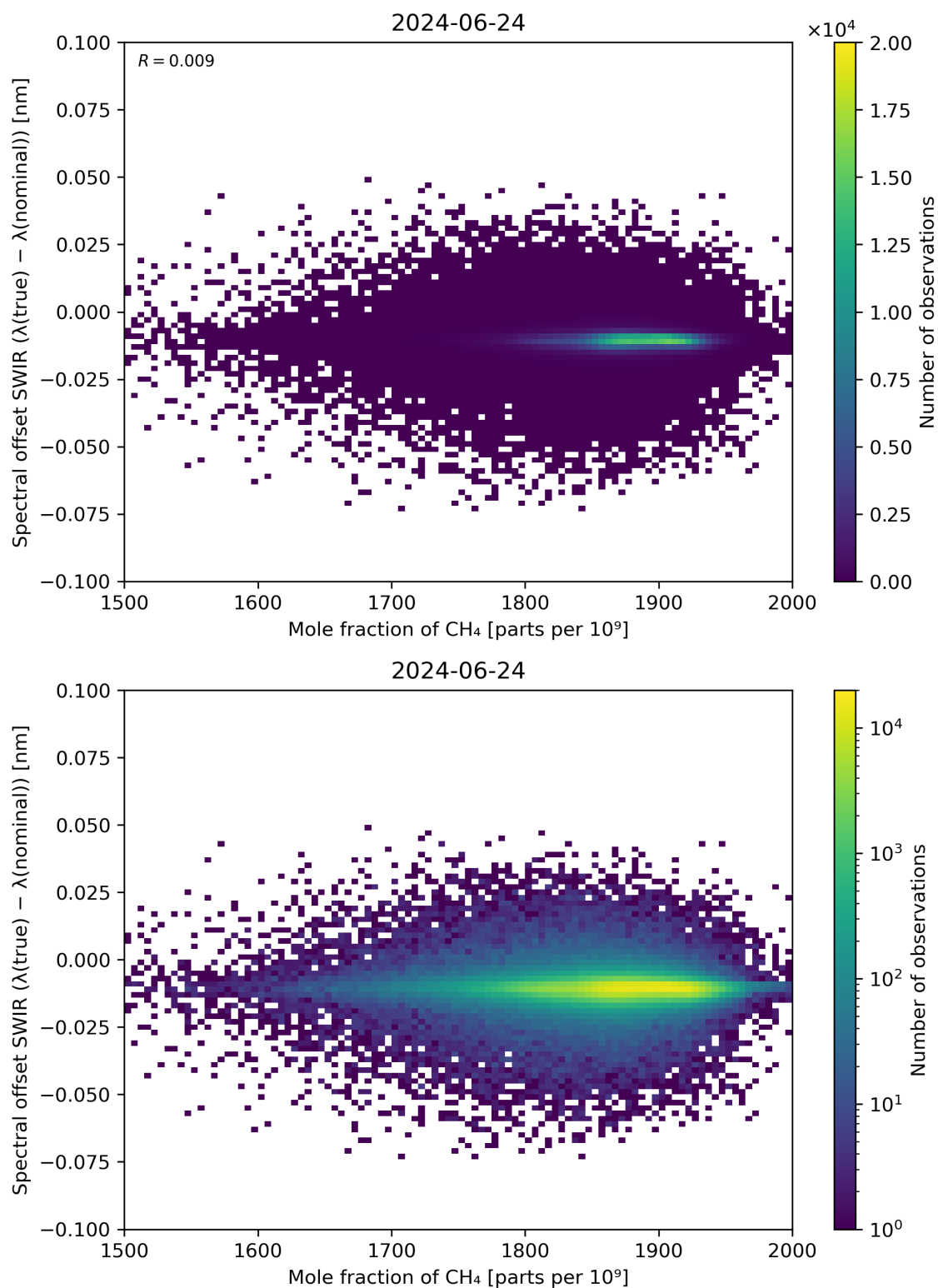
Figure 86: Scatter density plot of “Mole fraction of CH 4 ” against “Spectral offset SWIR ( \lambda(\text{true}) - \lambda(\text{nominal}) )” for 2024-06-24 to 2024-06-25.
