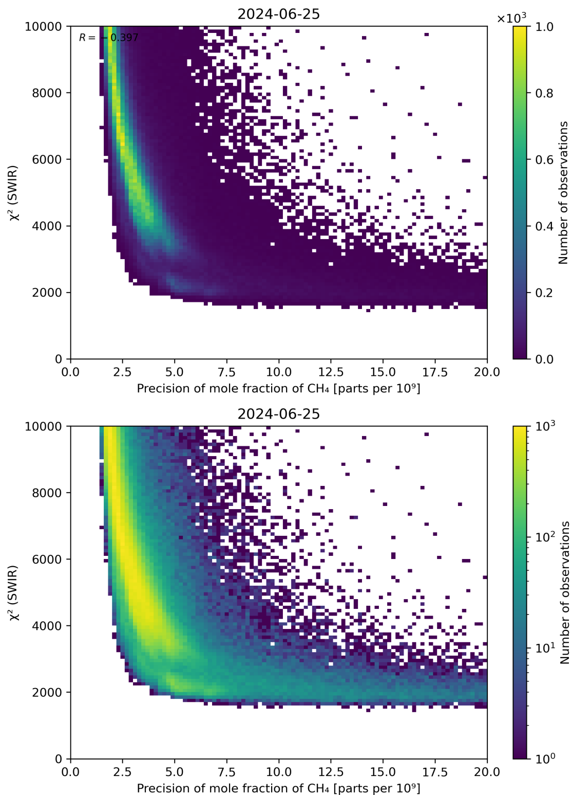
Figure 79: Scatter density plot of “Precision of mole fraction of CH 4 ” against “ \chi^2 (SWIR)” for 2024-06-24 to 2024-06-26.
