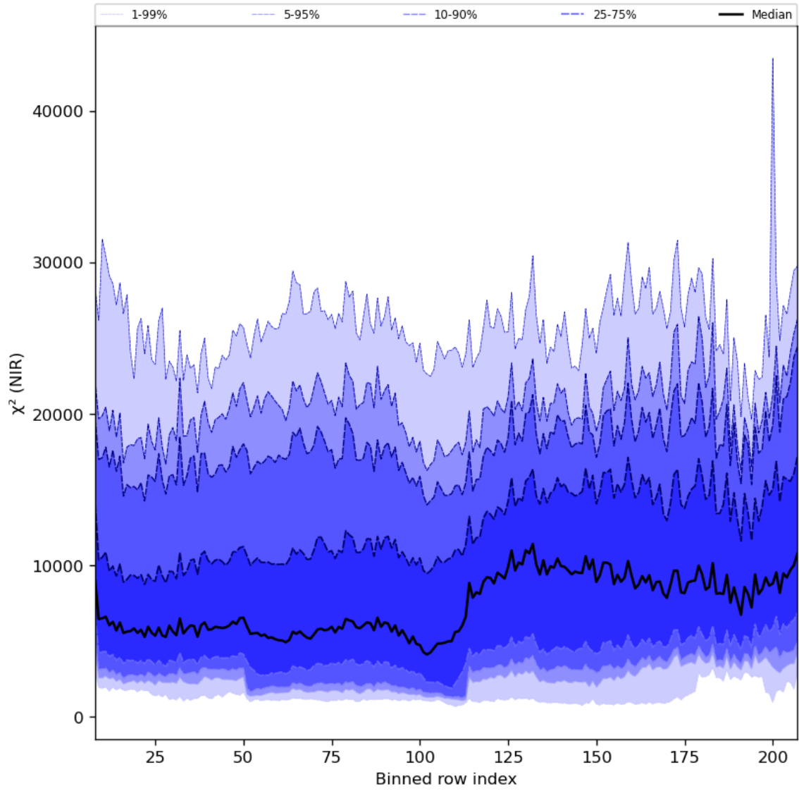
Figure 40: Along track statistics of " \chi^2 (NIR)" for 2024-06-24 to 2024-06-26
