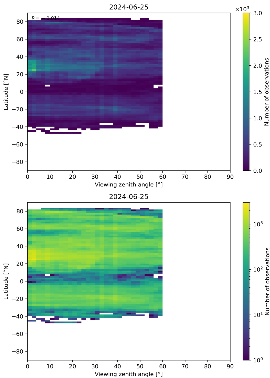
Figure 109: Scatter density plot of “Viewing zenith angle” against “Latitude” for 2024-06-24 to 2024-06-26.
