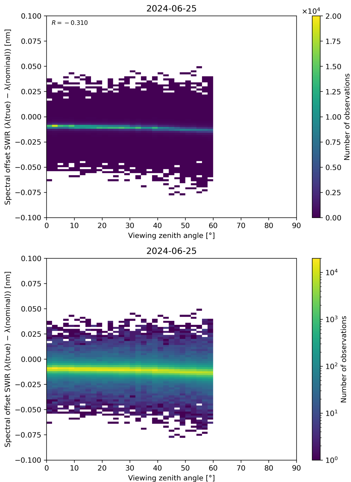
Figure 116: Scatter density plot of “Viewing zenith angle” against “Spectral offset SWIR ( \lambda(\text{true}) - \lambda(\text{nominal}) )” for 2024-06-24 to 2024-06-26.
