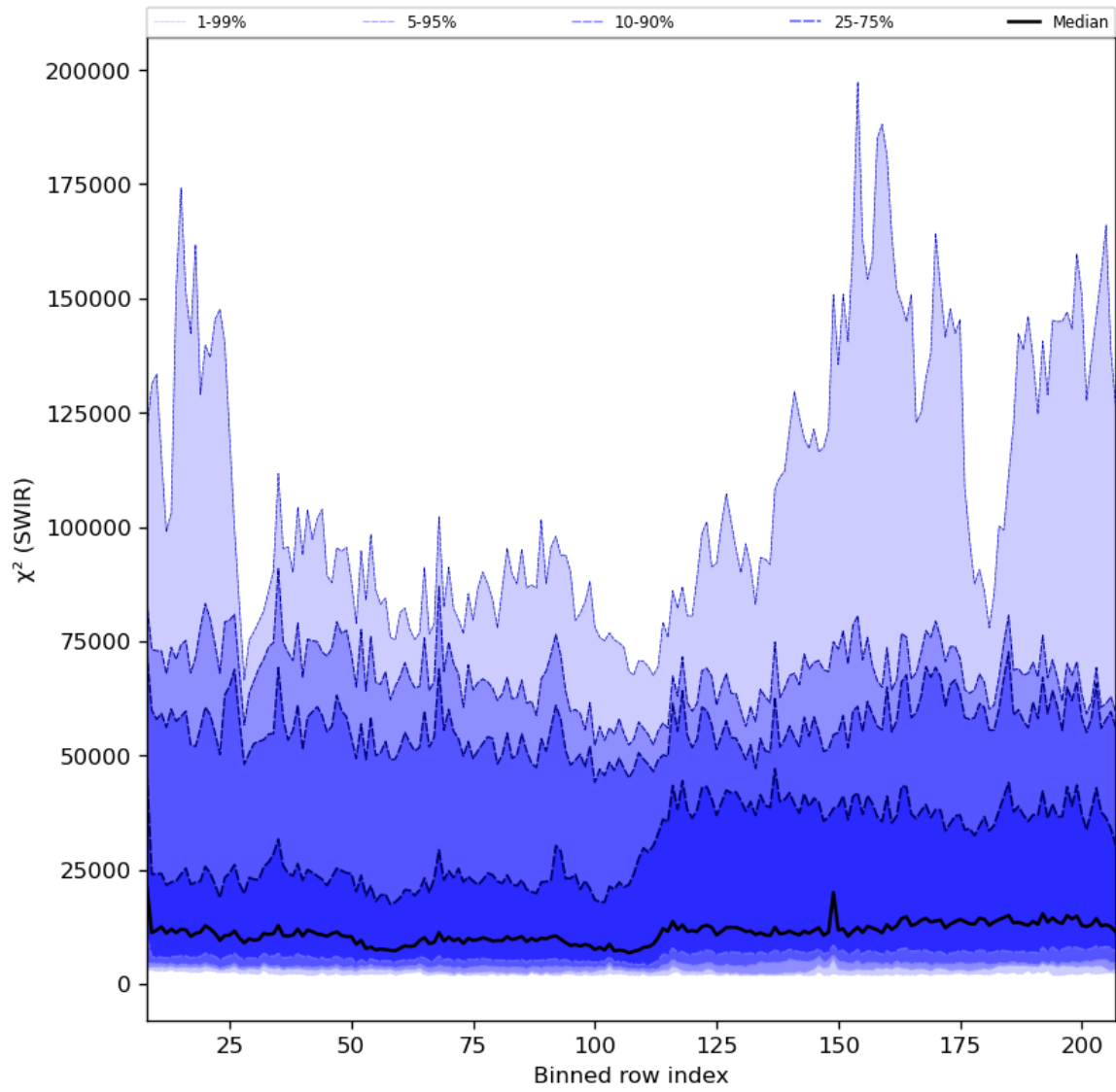
Figure 39: Along track statistics of “ \chi^2 (SWIR)” for 2024-06-24 to 2024-06-26
