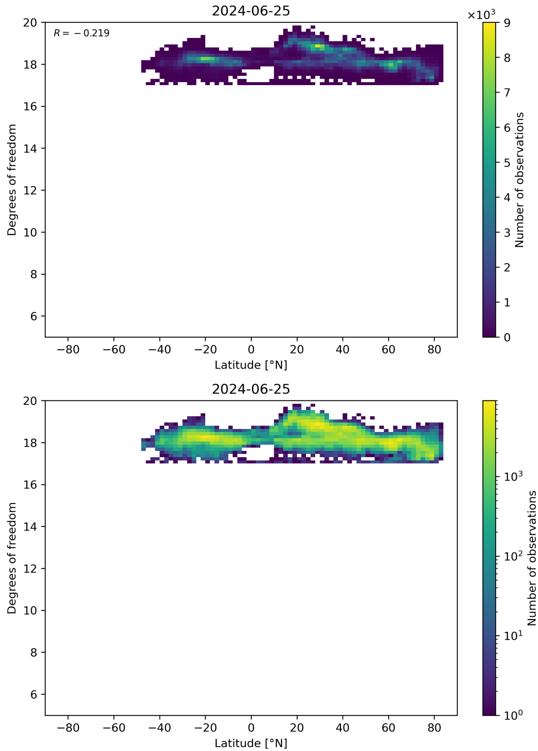
Figure 55: Scatter density plot of “Latitude” against “Degrees of freedom” for 2024-06-24 to 2024-06-26.
