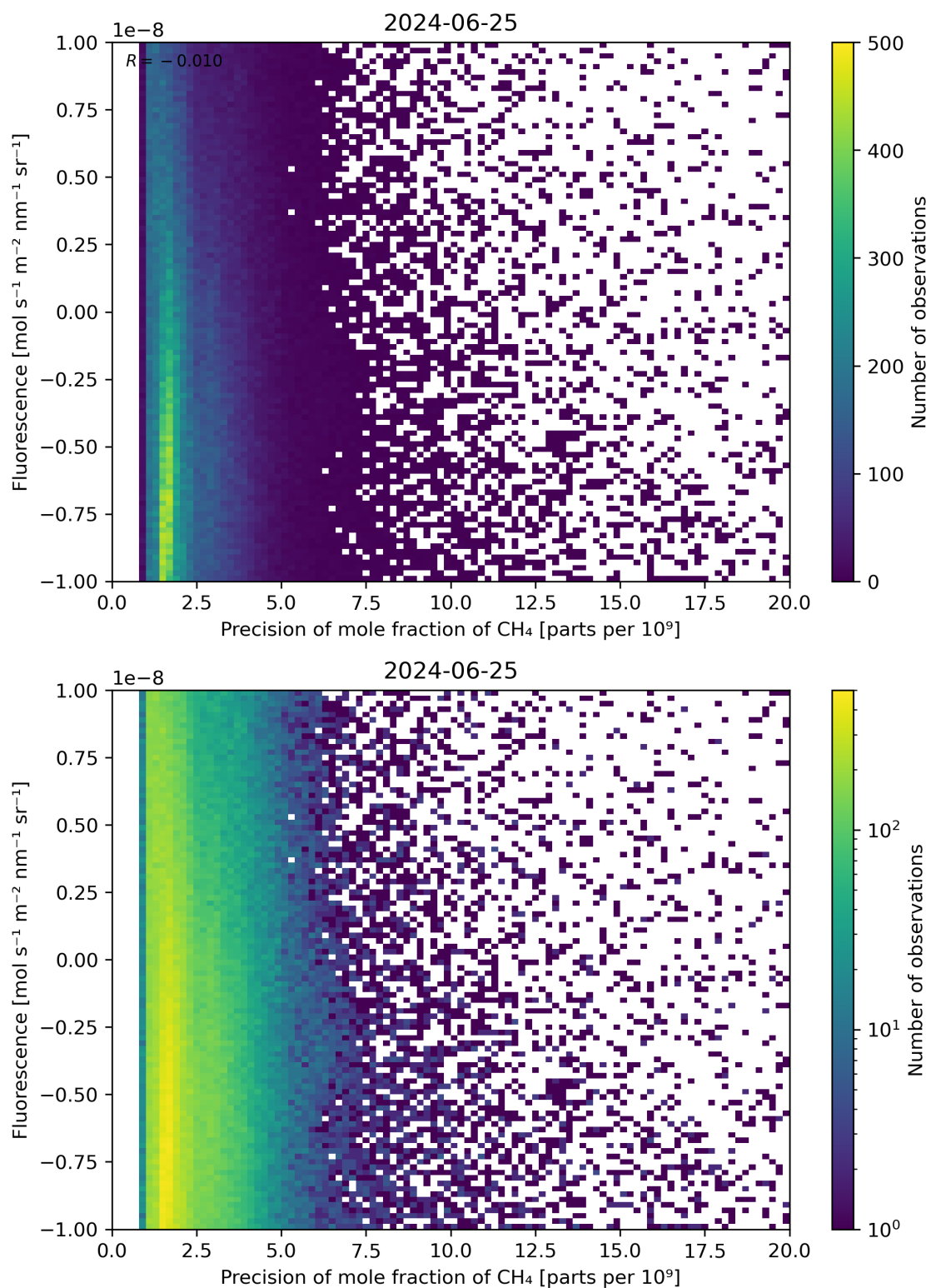
Figure 81: Scatter density plot of “Precision of mole fraction of \text{CH}_4 ” against “Fluorescence” for 2024-06-24 to 2024-06-26.
