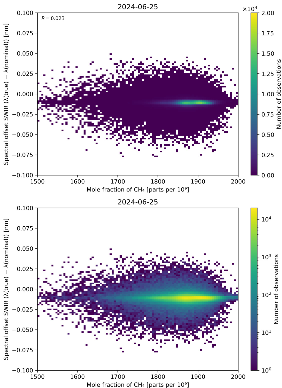
Figure 86: Scatter density plot of “Mole fraction of CH 4 ” against “Spectral offset SWIR ( \lambda(\text{true}) - \lambda(\text{nominal}) )” for 2024-06-24 to 2024-06-26.
