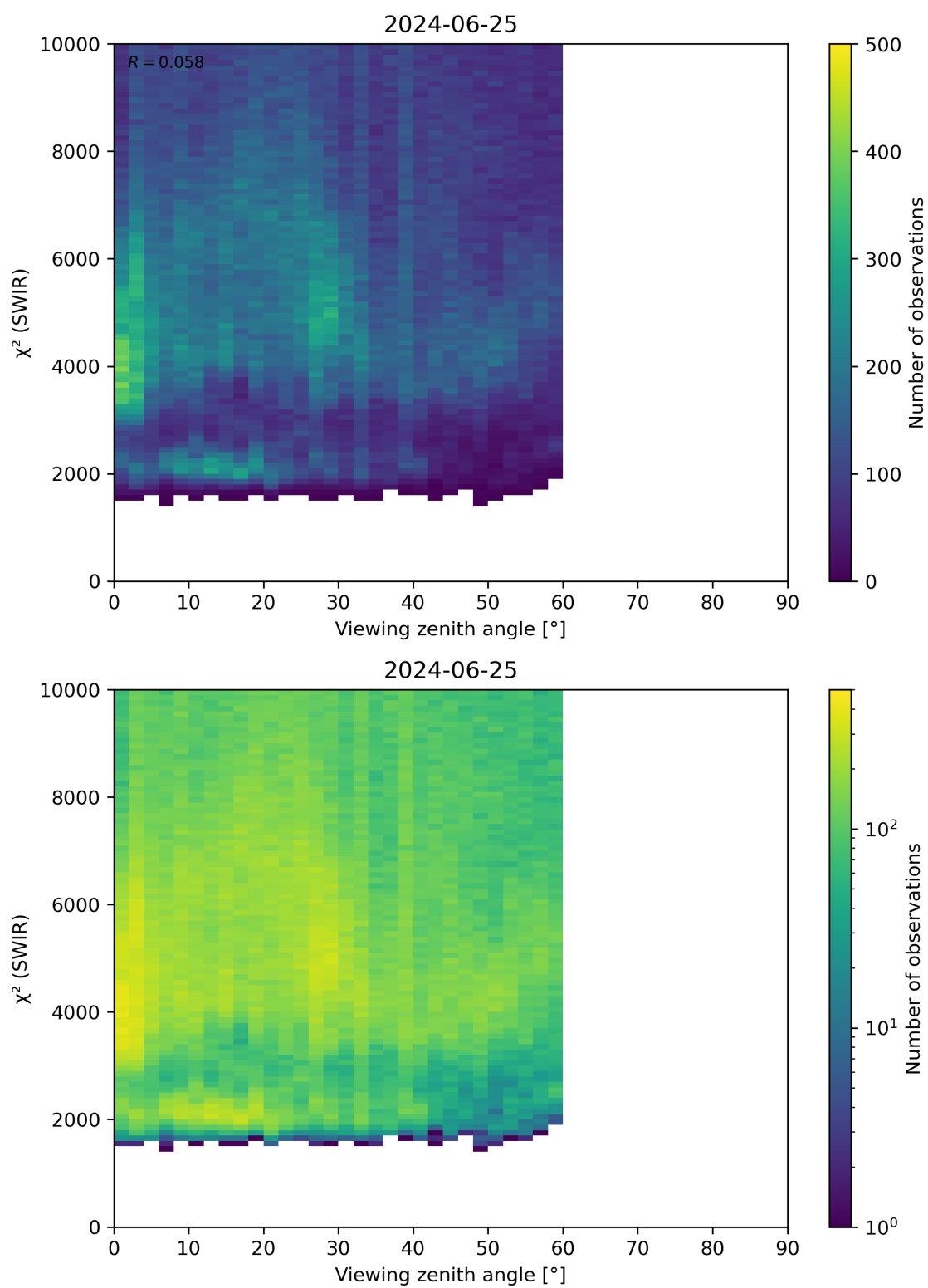
Figure 106: Scatter density plot of “Viewing zenith angle” against “ \chi^2 (SWIR)” for 2024-06-24 to 2024-06-26.
