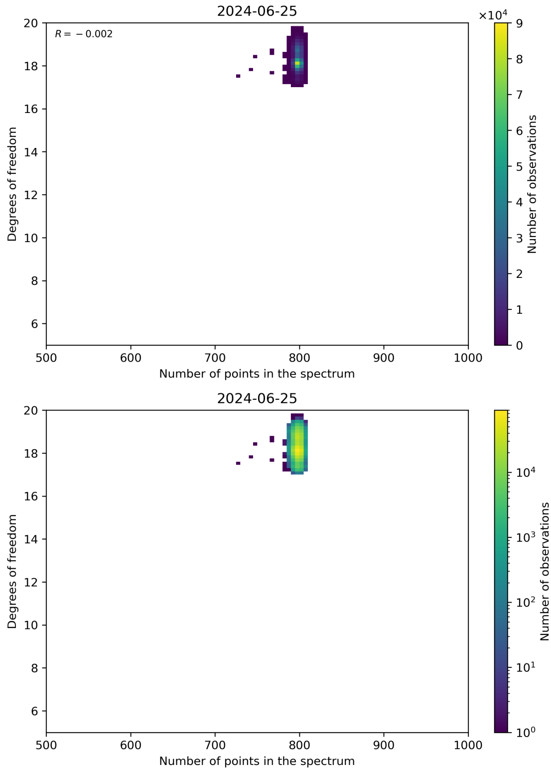
Figure 90: Scatter density plot of “Number of points in the spectrum” against “Degrees of freedom” for 2024-06-24 to 2024-06-26.
