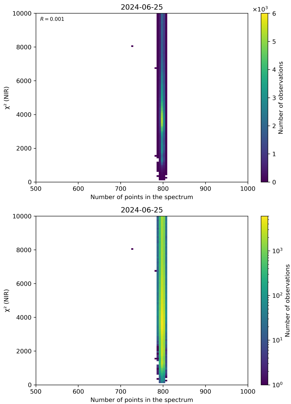
Figure 88: Scatter density plot of “Number of points in the spectrum” against “ \chi^2 (NIR)” for 2024-06-24 to 2024-06-26.
