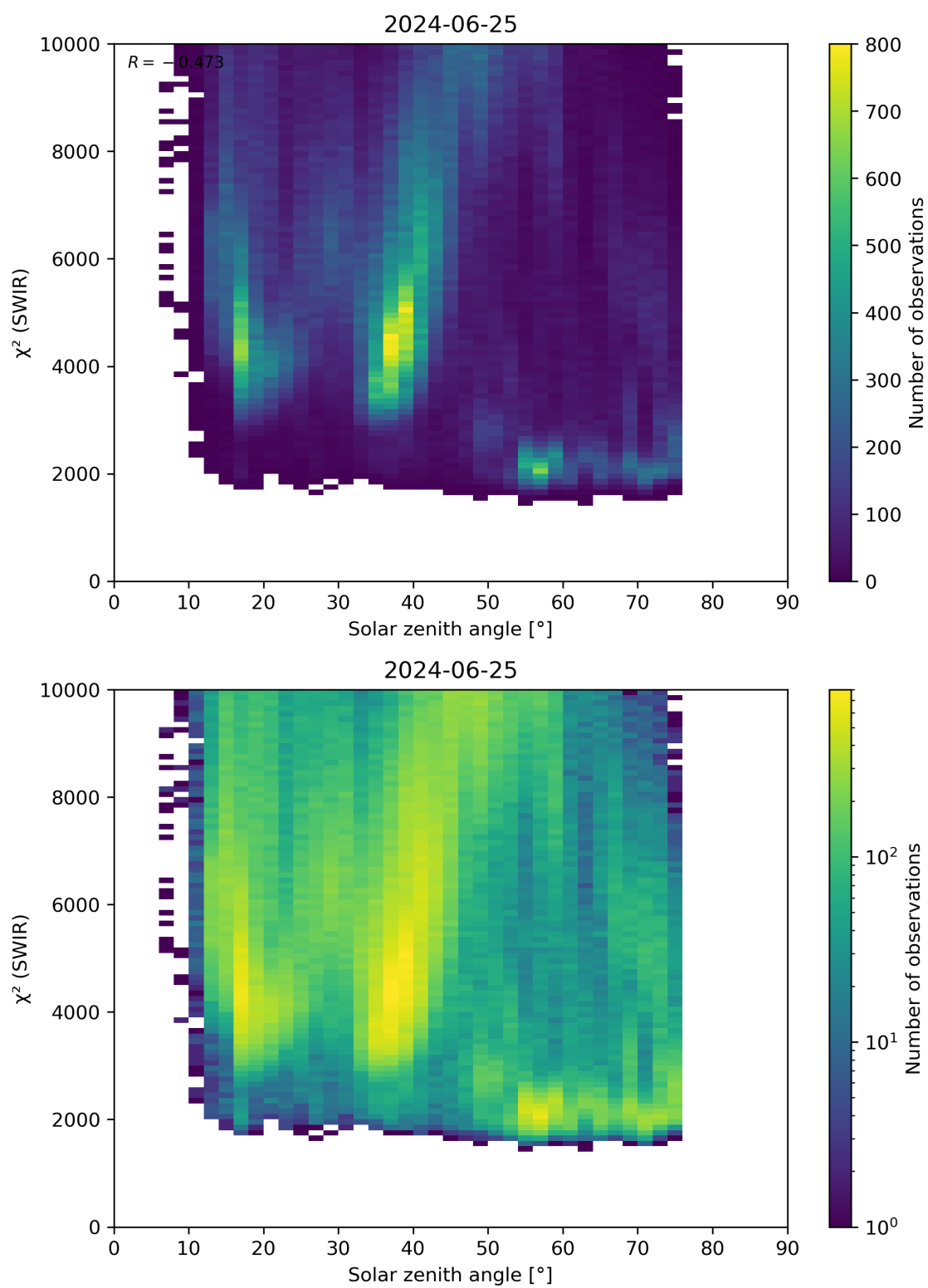
Figure 95: Scatter density plot of “Solar zenith angle” against “ \chi^2 (SWIR)” for 2024-06-24 to 2024-06-26.
