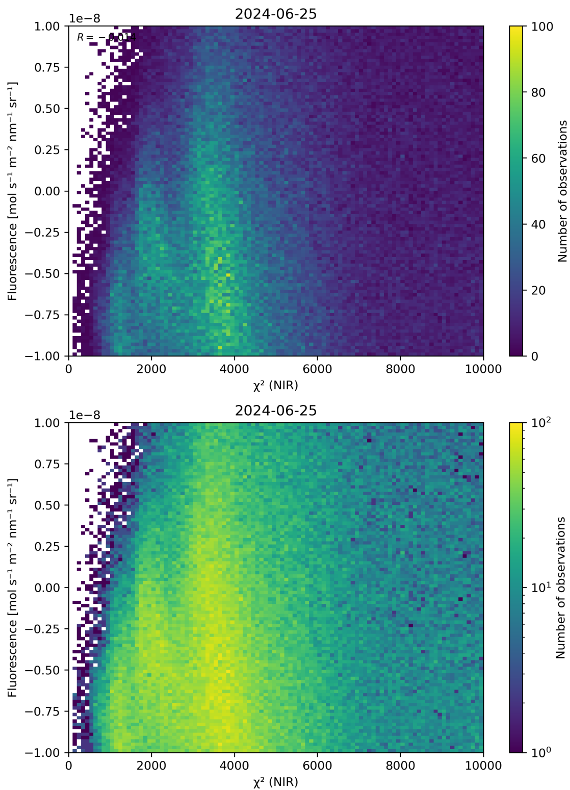
Figure 45: Scatter density plot of “ \chi^2 (NIR)” against “Fluorescence” for 2024-06-24 to 2024-06-26.
