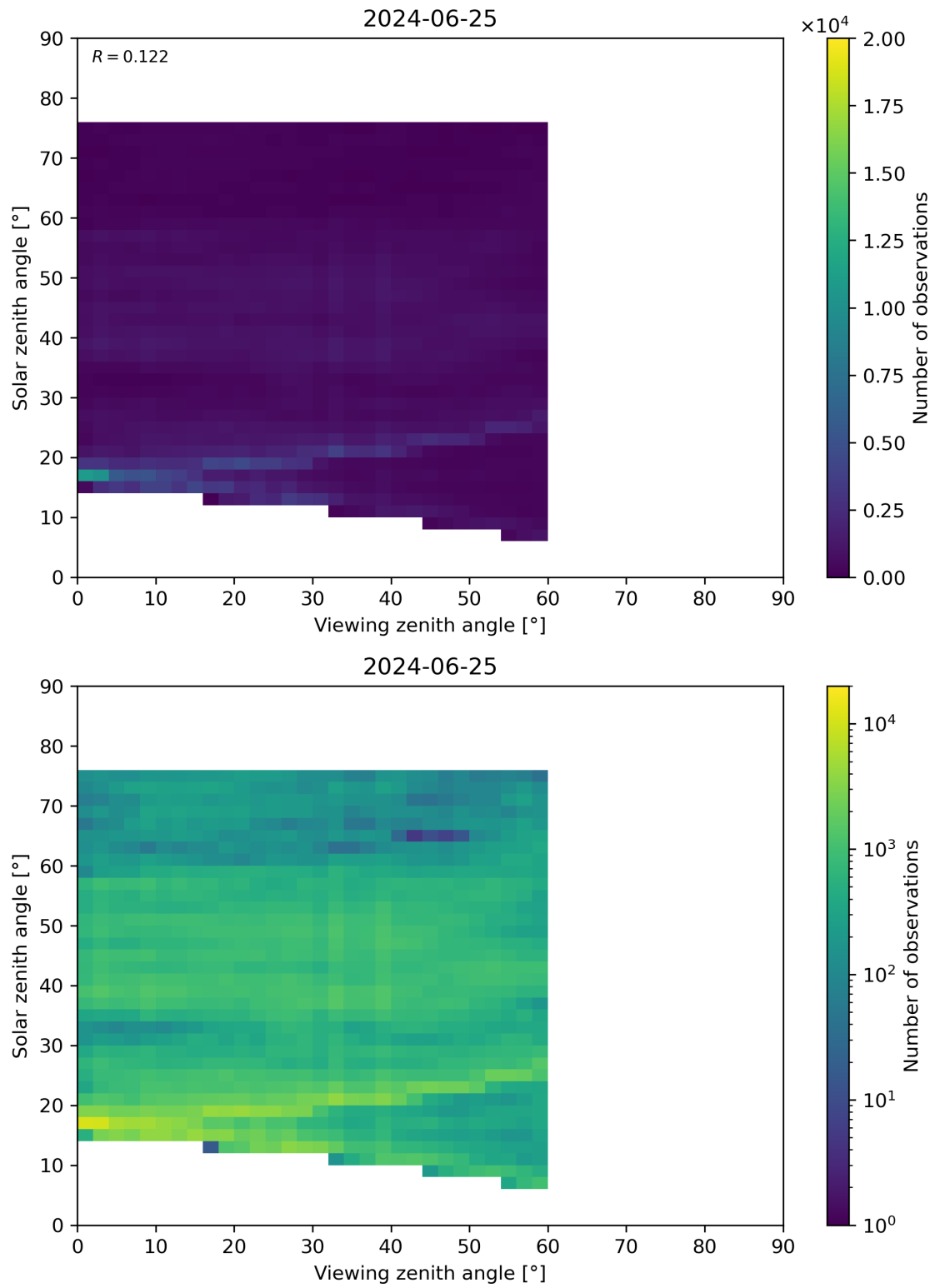
Figure 115: Scatter density plot of “Viewing zenith angle” against “Solar zenith angle” for 2024-06-24 to 2024-06-26.
