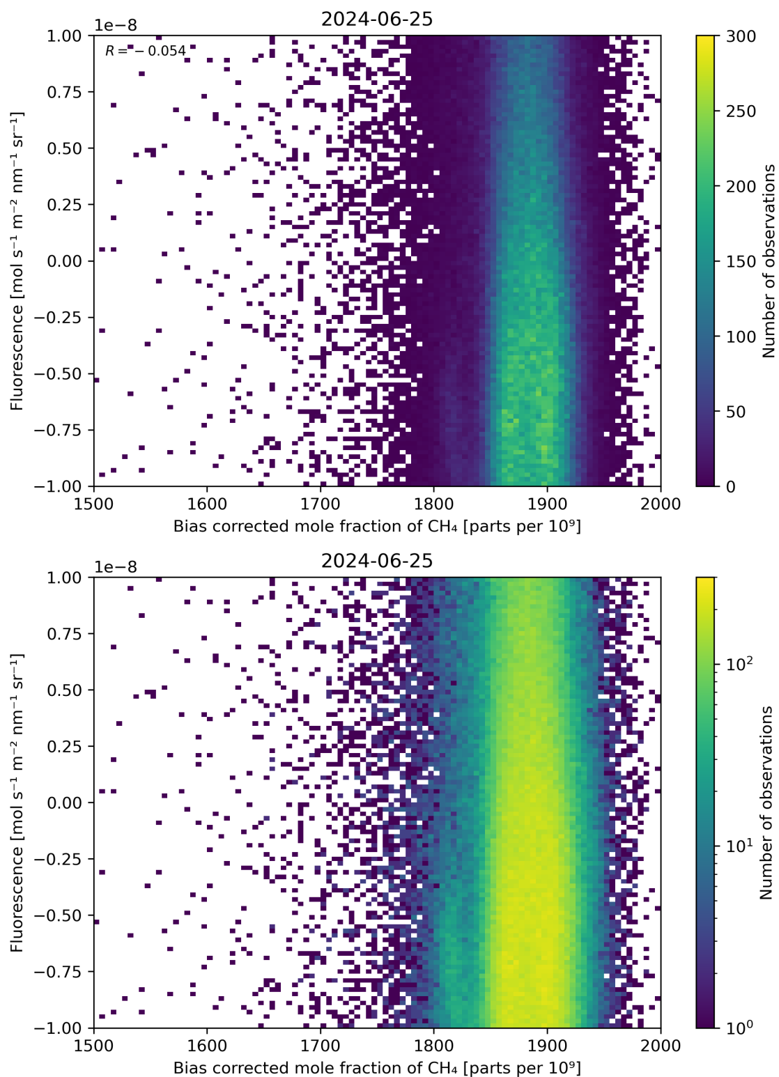
Figure 66: Scatter density plot of “Bias corrected mole fraction of \text{CH}_4 ” against “Fluorescence” for 2024-06-24 to 2024-06-26.
