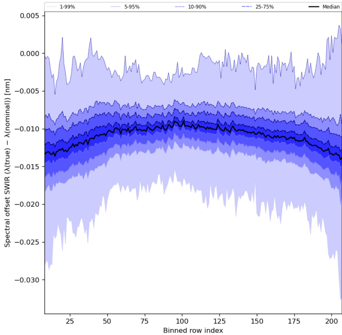
Figure 38: Along track statistics of “Spectral offset SWIR ( \lambda(\text{true}) - \lambda(\text{nominal}) )” for 2024-06-24 to 2024-06-26
