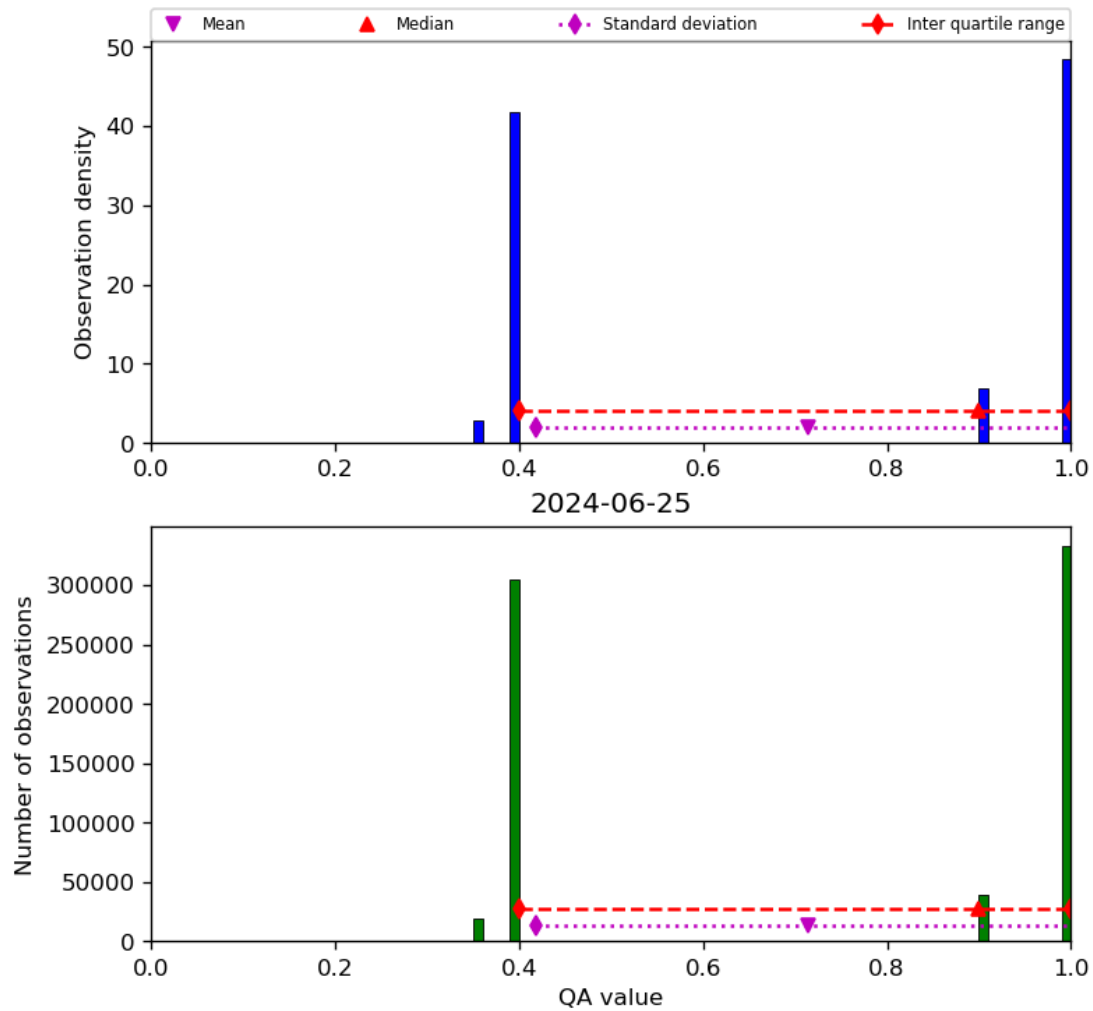
Figure 22: Histogram of “QA value” for 2024-06-24 to 2024-06-26
