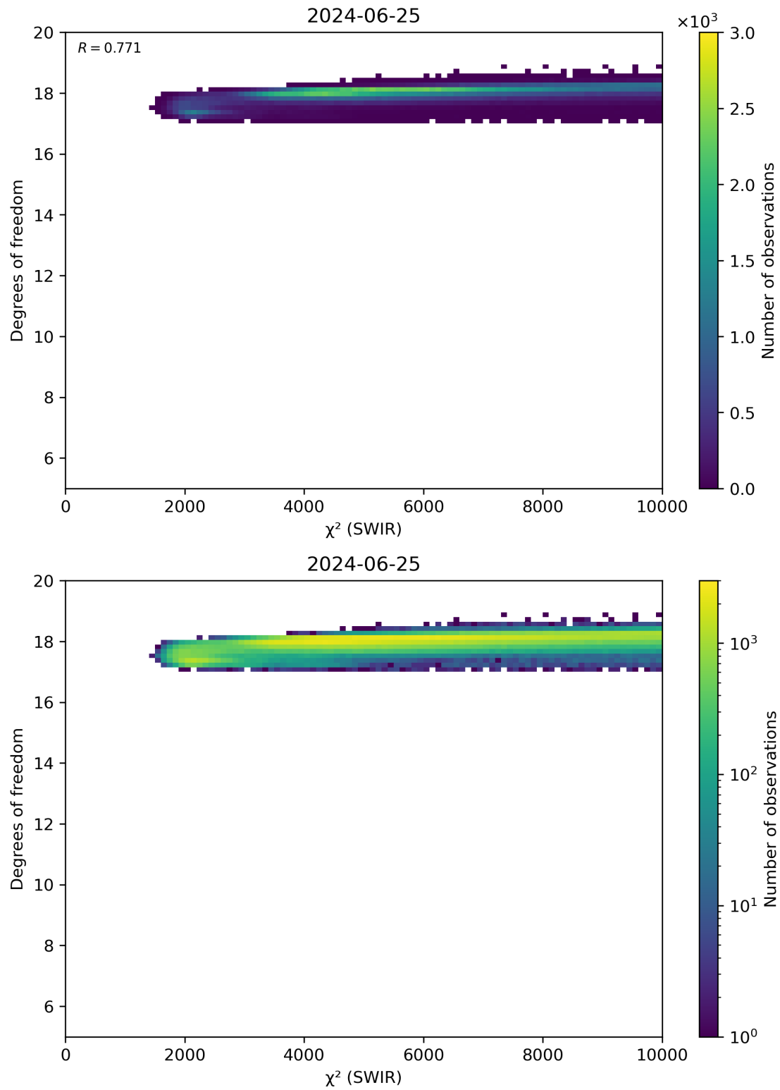
Figure 48: Scatter density plot of “ \chi^2 (SWIR)” against “Degrees of freedom” for 2024-06-24 to 2024-06-26.
