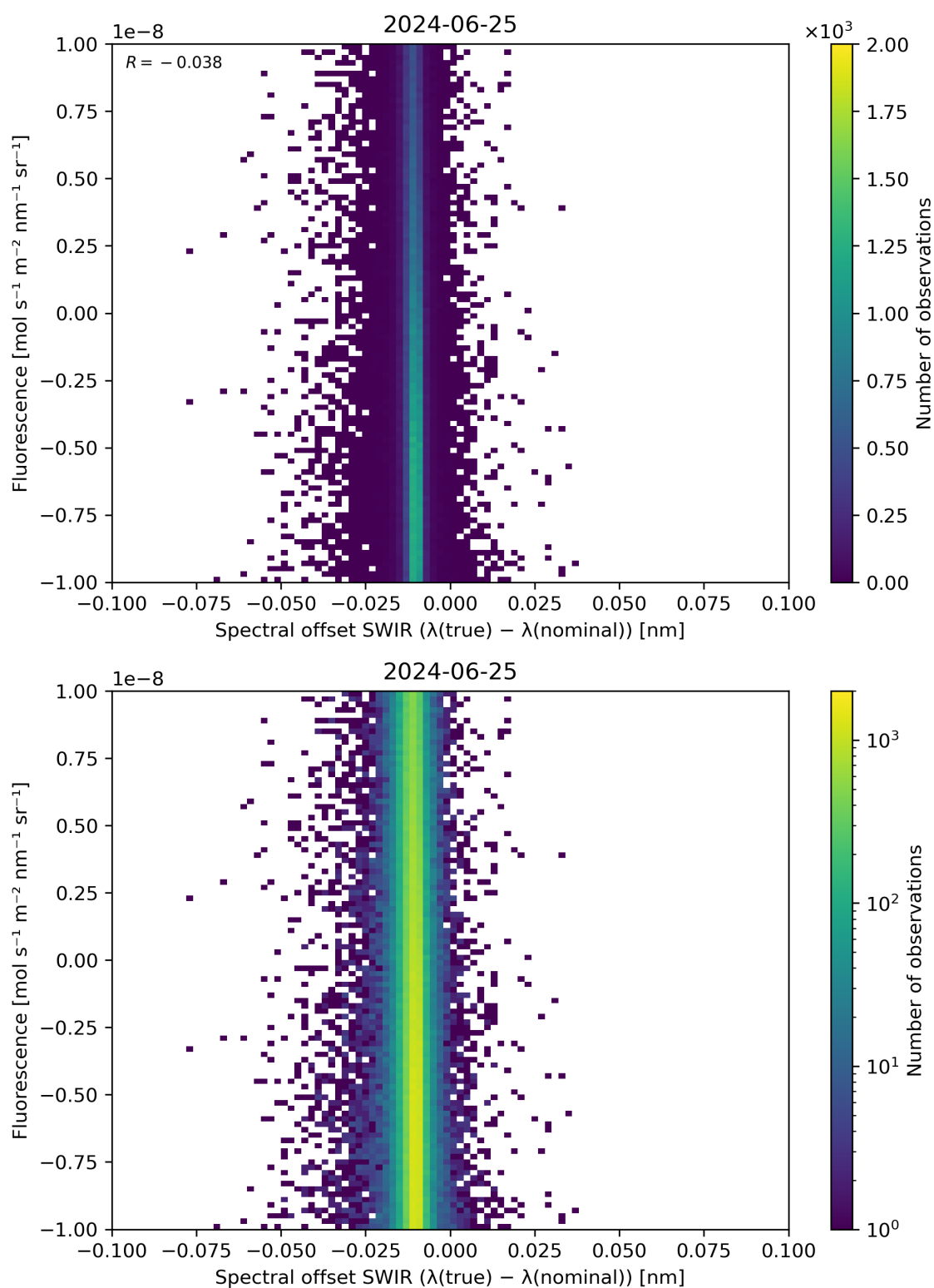
Figure 120: Scatter density plot of “Spectral offset SWIR ( \lambda(\text{true}) - \lambda(\text{nominal}) )” against “Fluorescence” for 2024-06-24 to 2024-06-26.
