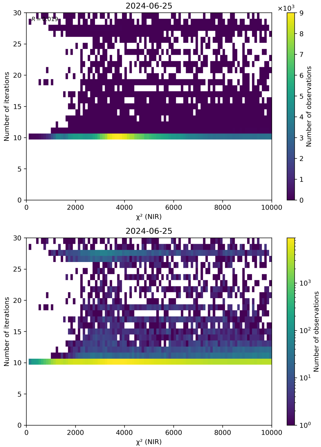
Figure 46: Scatter density plot of “ \chi^2 (NIR)” against “Number of iterations” for 2024-06-24 to 2024-06-26.
