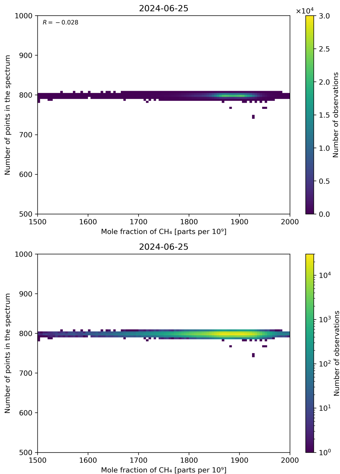
Figure 77: Scatter density plot of “Mole fraction of CH 4 ” against “Number of points in the spectrum” for 2024-06-24 to 2024-06-26.
