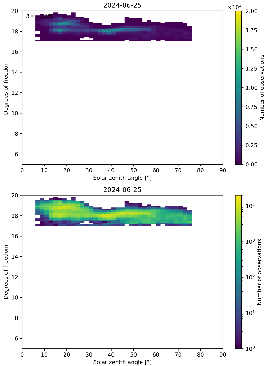
Figure 96: Scatter density plot of “Solar zenith angle” against “Degrees of freedom” for 2024-06-24 to 2024-06-26.
