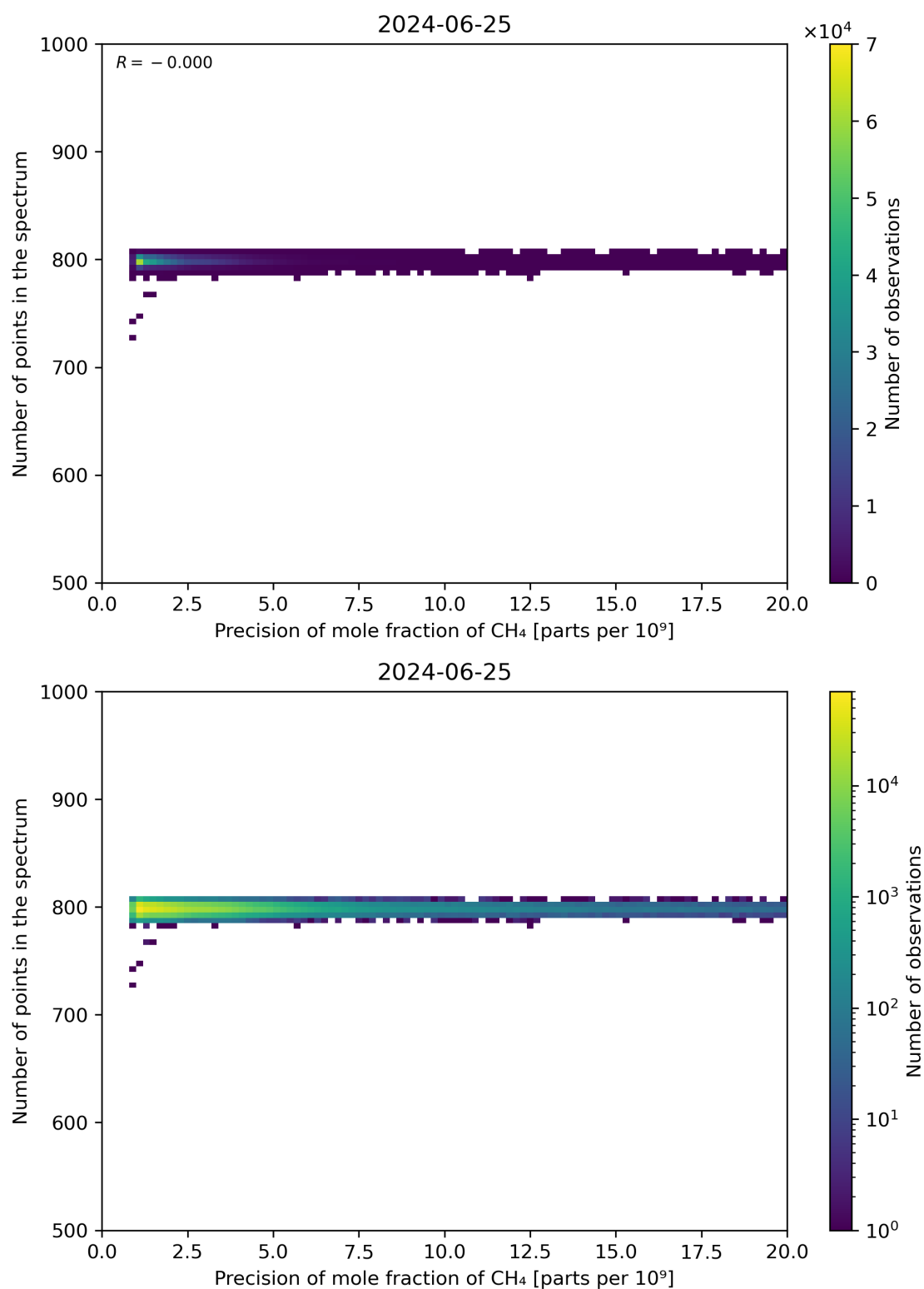
Figure 84: Scatter density plot of “Precision of mole fraction of CH 4 ” against “Number of points in the spectrum” for 2024-06-24 to 2024-06-26.
