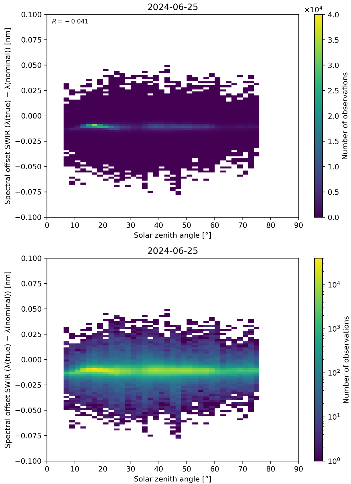
Figure 104: Scatter density plot of “Solar zenith angle” against “Spectral offset SWIR ( \lambda(\text{true}) - \lambda(\text{nominal}) )” for 2024-06-24 to 2024-06-26.
