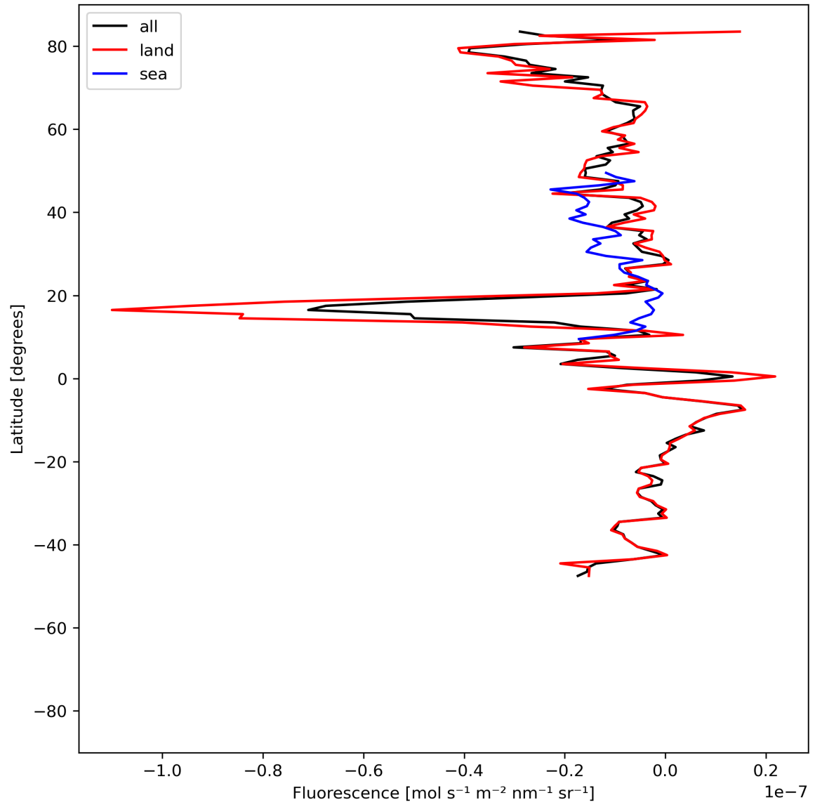
Figure 21: Zonal average of “Fluorescence” for 2024-06-24 to 2024-06-26.
