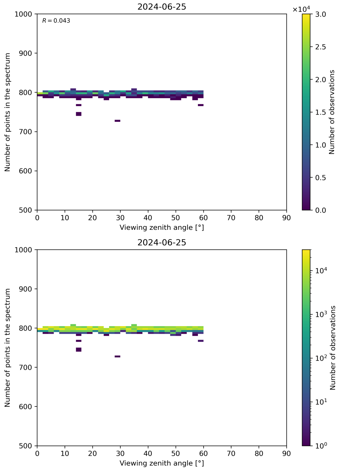
Figure 114: Scatter density plot of “Viewing zenith angle” against “Number of points in the spectrum” for 2024-06-24 to 2024-06-26.
