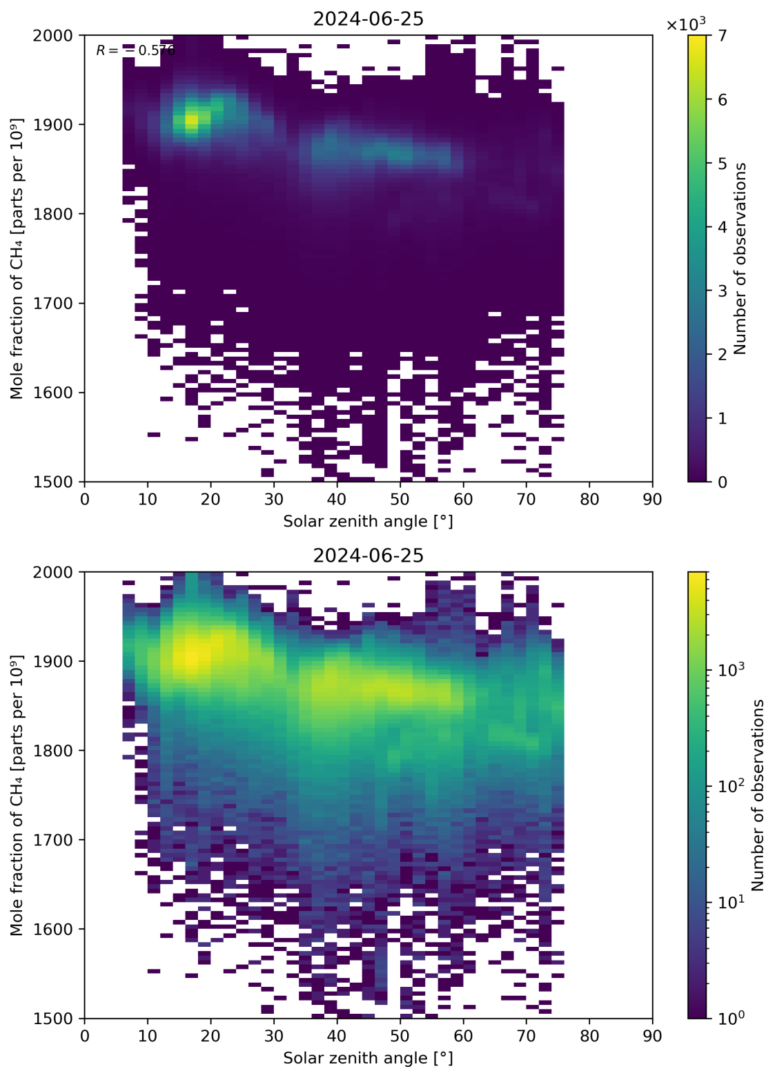
Figure 99: Scatter density plot of “Solar zenith angle” against “Mole fraction of CH 4 ” for 2024-06-24 to 2024-06-26.
