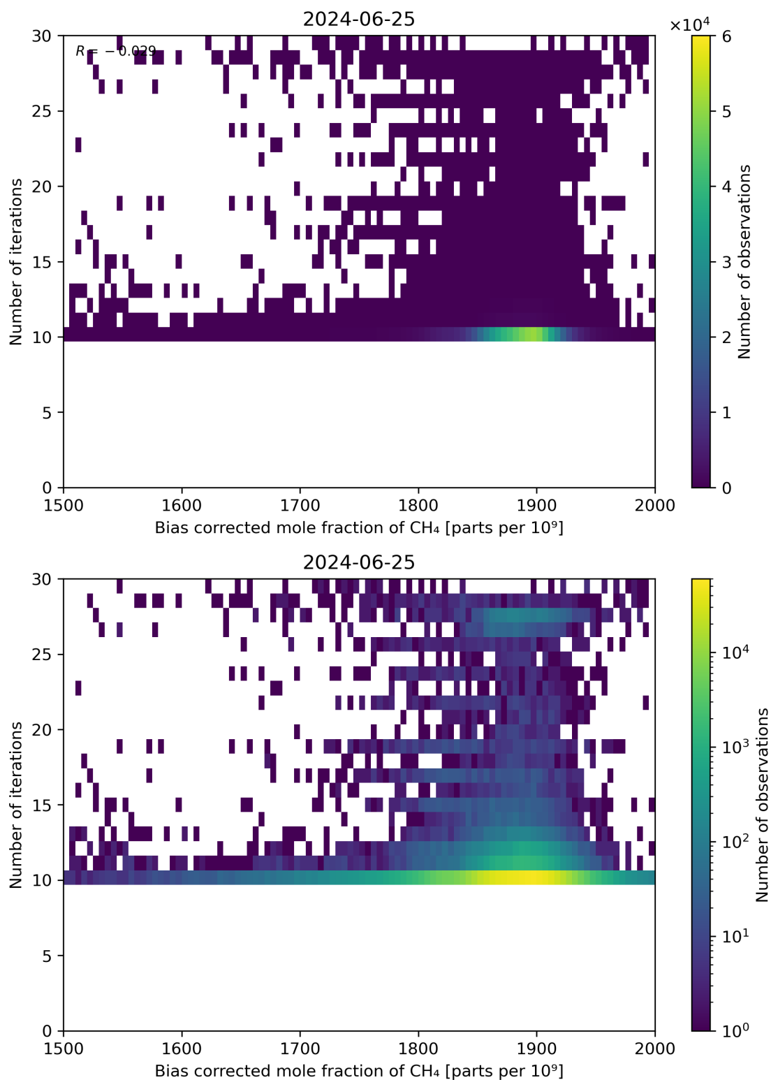
Figure 67: Scatter density plot of “Bias corrected mole fraction of \text{CH}_4 ” against “Number of iterations” for 2024-06-24 to 2024-06-26.
