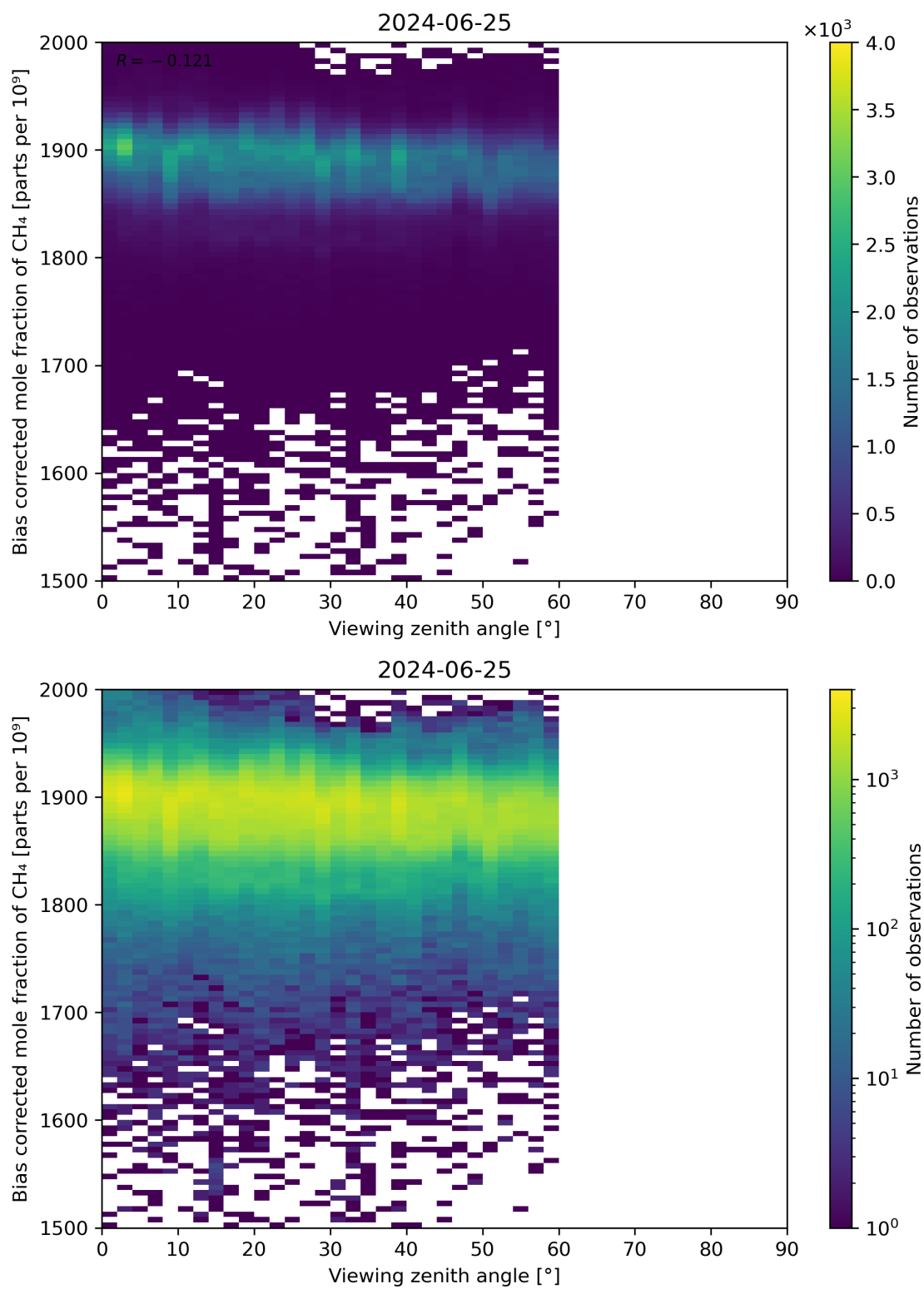
Figure 111: Scatter density plot of “Viewing zenith angle” against “Bias corrected mole fraction of CH 4 ” for 2024-06-24 to 2024-06-26.
