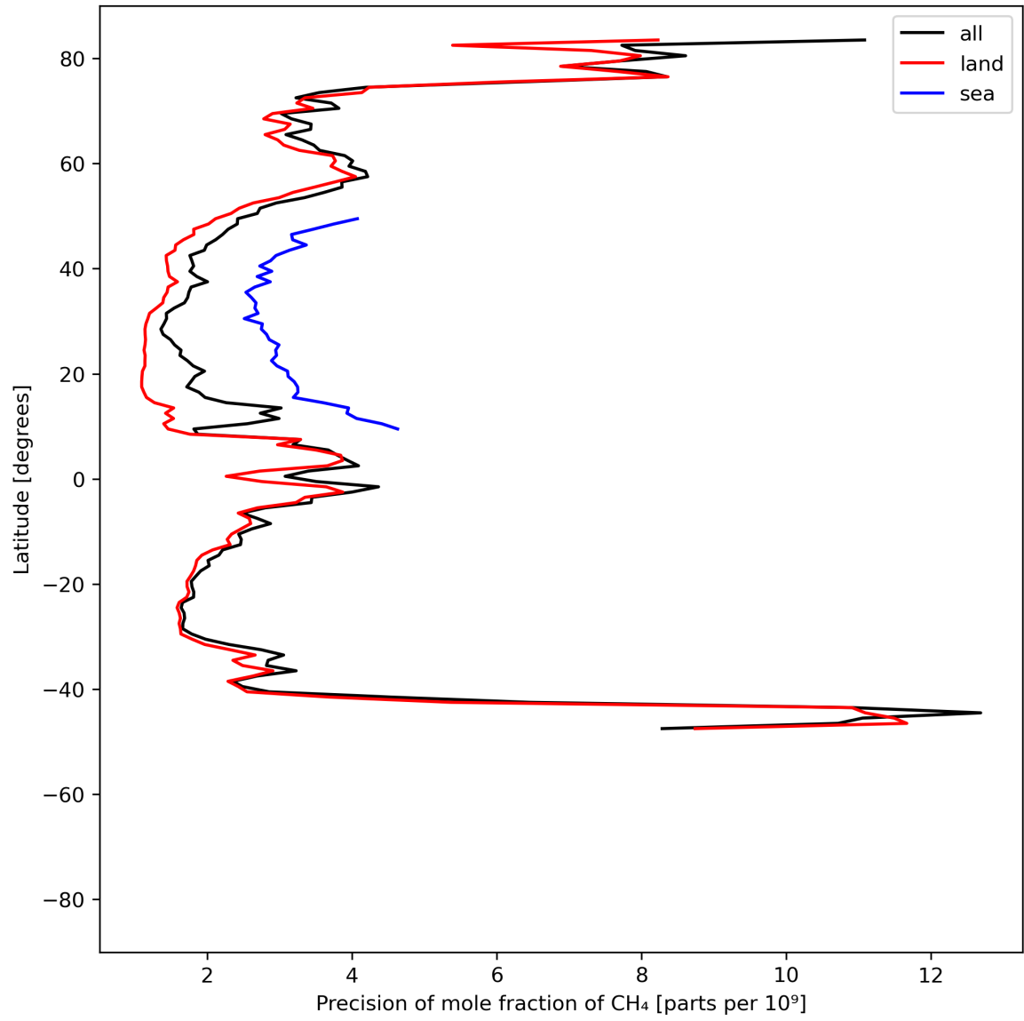
Figure 13: Zonal average of “Precision of mole fraction of CH 4 ” for 2024-06-24 to 2024-06-26.
