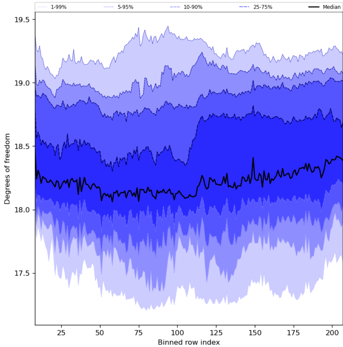
Figure 41: Along track statistics of “Degrees of freedom” for 2024-06-24 to 2024-06-26
