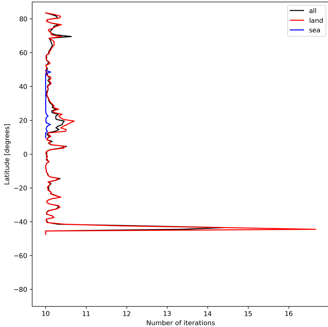
Figure 20: Zonal average of “Number of iterations” for 2024-06-24 to 2024-06-26.
