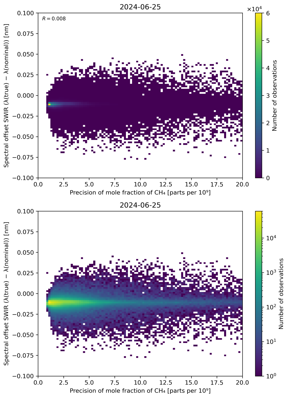
Figure 85: Scatter density plot of “Precision of mole fraction of \text{CH}_4 ” against “Spectral offset SWIR ( \lambda(\text{true}) - \lambda(\text{nominal}) )” for 2024-06-24 to 2024-06-26.
