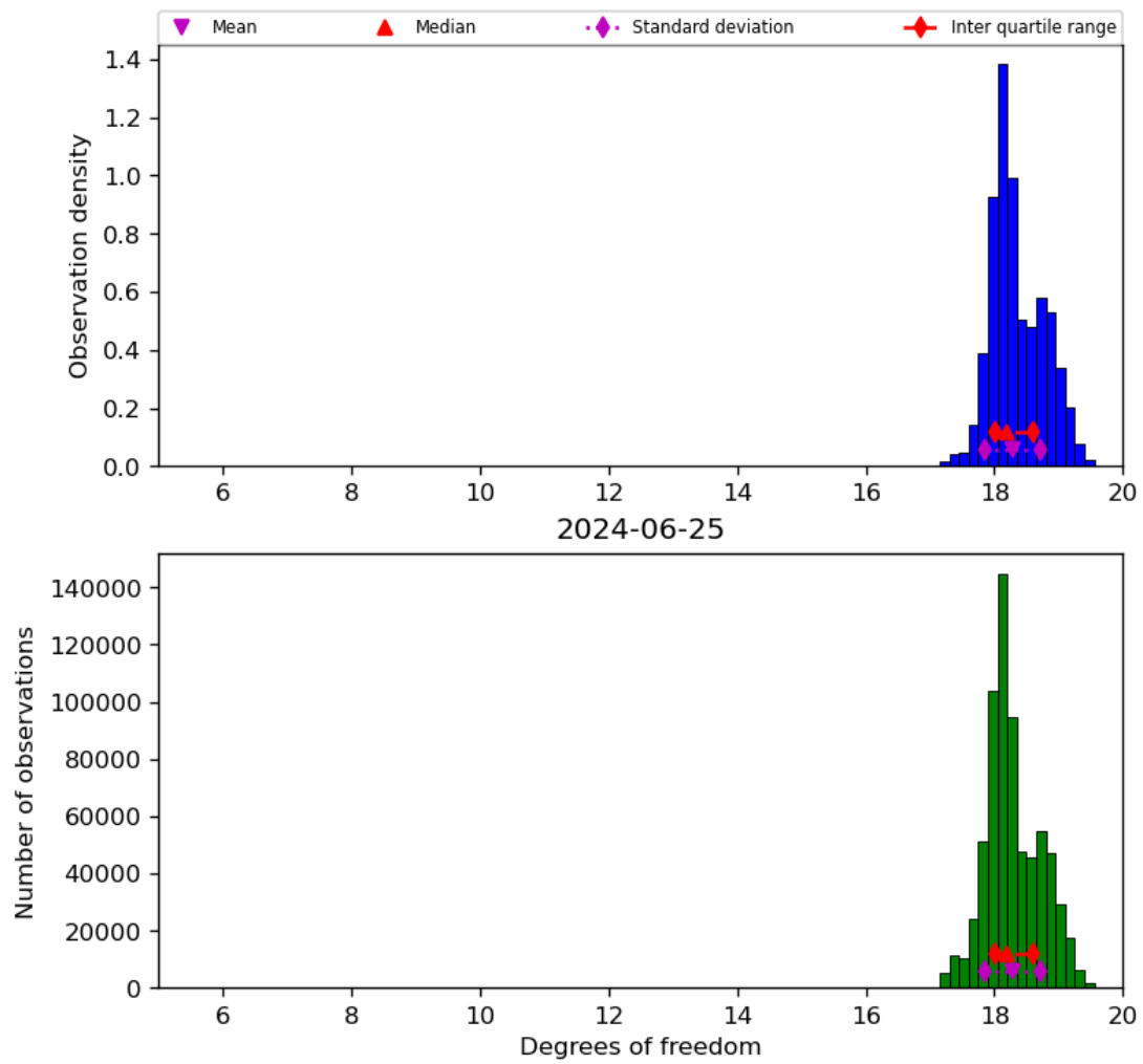
Figure 30: Histogram of “Degrees of freedom” for 2024-06-24 to 2024-06-26
