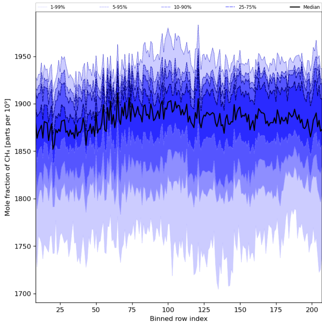
Figure 34: Along track statistics of “Mole fraction of CH 4 ” for 2024-06-24 to 2024-06-26
