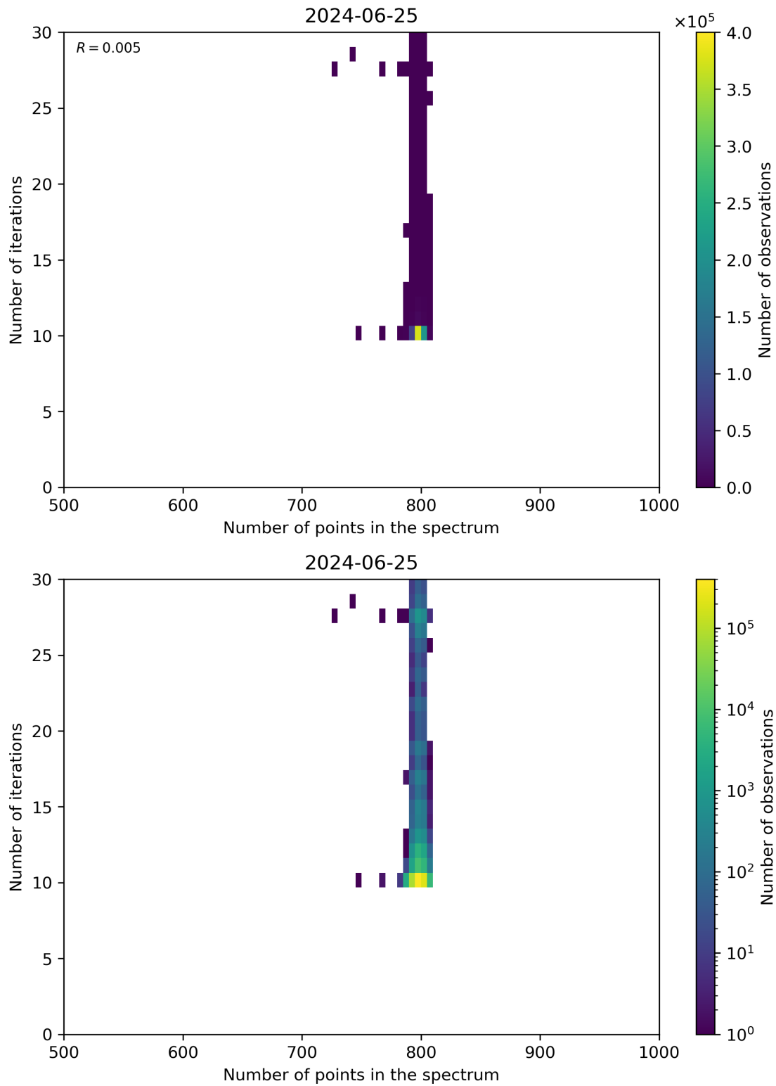
Figure 92: Scatter density plot of “Number of points in the spectrum” against “Number of iterations” for 2024-06-24 to 2024-06-26.
