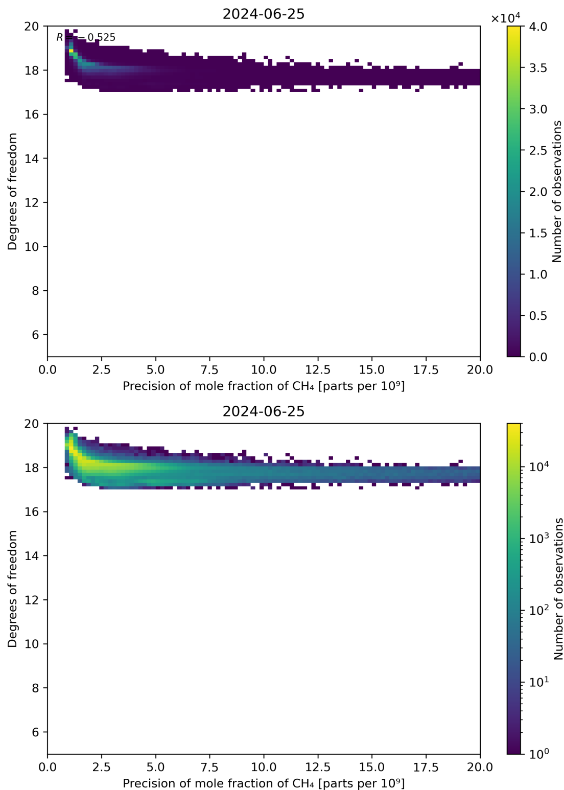
Figure 80: Scatter density plot of “Precision of mole fraction of CH 4 ” against “Degrees of freedom” for 2024-06-24 to 2024-06-26.
