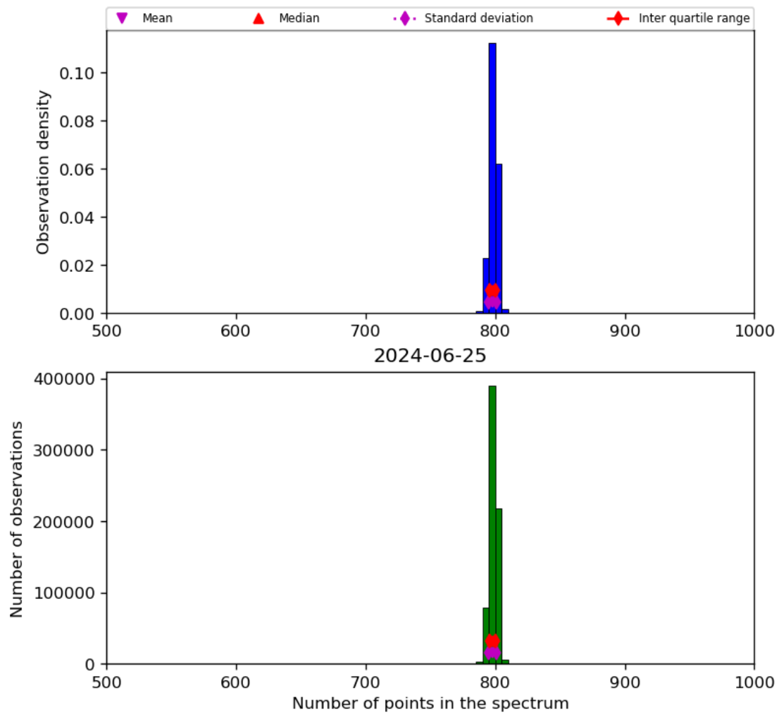
Figure 26: Histogram of “Number of points in the spectrum” for 2024-06-24 to 2024-06-26
