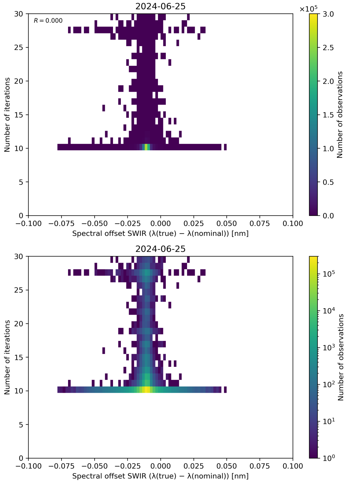
Figure 121: Scatter density plot of “Spectral offset SWIR ( \lambda(\text{true}) - \lambda(\text{nominal}) )” against “Number of iterations” for 2024-06-24 to 2024-06-26.
