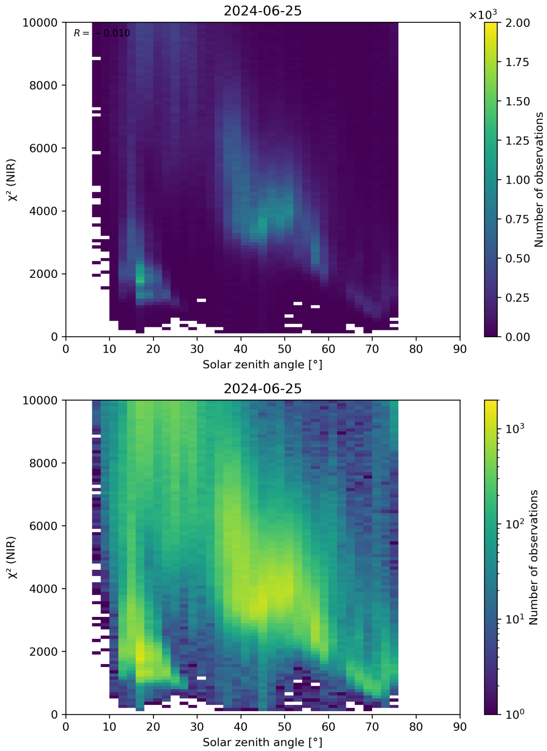
Figure 94: Scatter density plot of “Solar zenith angle” against “ \chi^2 (NIR)” for 2024-06-24 to 2024-06-26.
