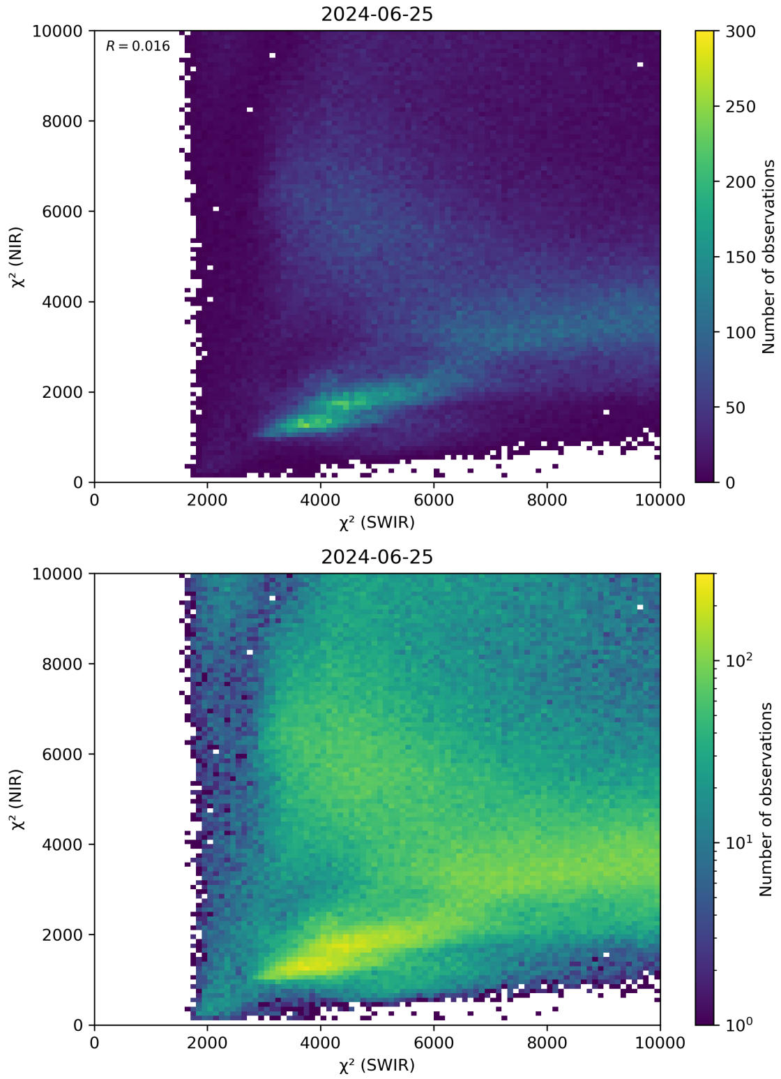
Figure 47: Scatter density plot of “ \chi^2 (SWIR)” against “ \chi^2 (NIR)” for 2024-06-24 to 2024-06-26.
