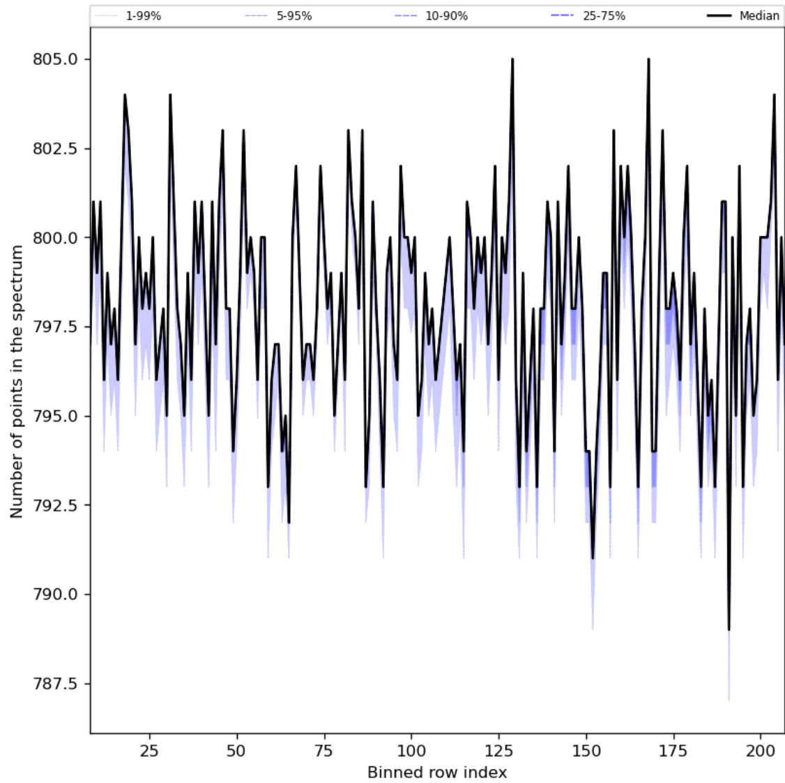
Figure 37: Along track statistics of “Number of points in the spectrum” for 2024-06-24 to 2024-06-26
