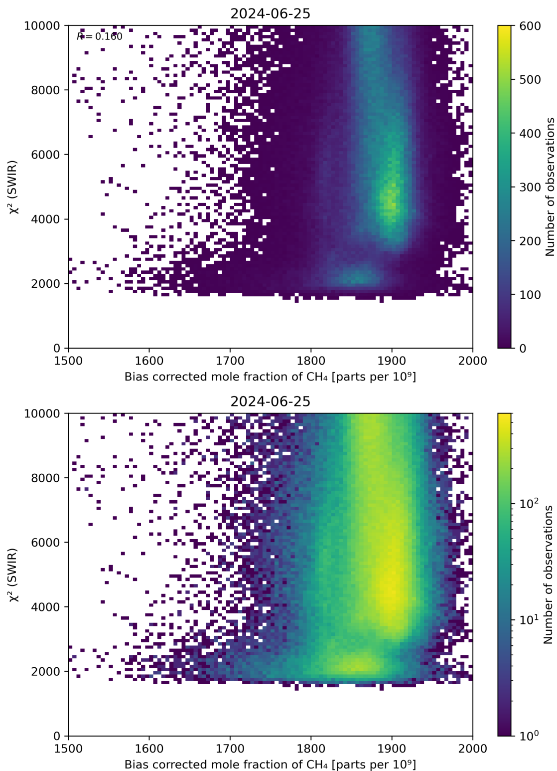
Figure 64: Scatter density plot of “Bias corrected mole fraction of CH 4 ” against “ \chi^2 (SWIR)” for 2024-06-24 to 2024-06-26.
