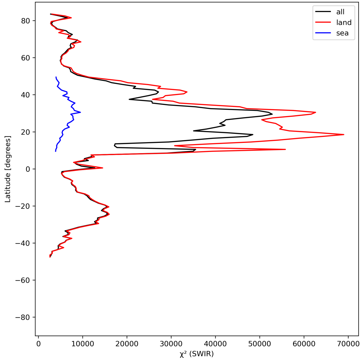
Figure 17: Zonal average of “ \chi^2 (SWIR)” for 2024-06-24 to 2024-06-26.
