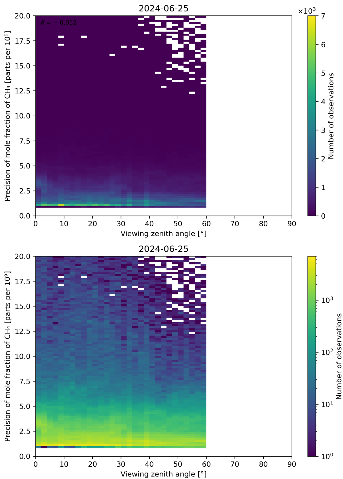
Figure 112: Scatter density plot of “Viewing zenith angle” against “Precision of mole fraction of CH 4 ” for 2024-06-24 to 2024-06-26.
