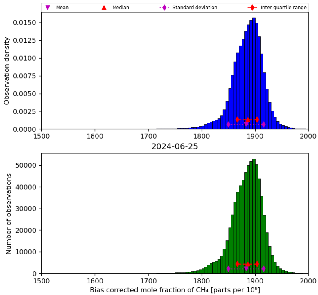
Figure 25: Histogram of “Bias corrected mole fraction of CH 4 ” for 2024-06-24 to 2024-06-26
