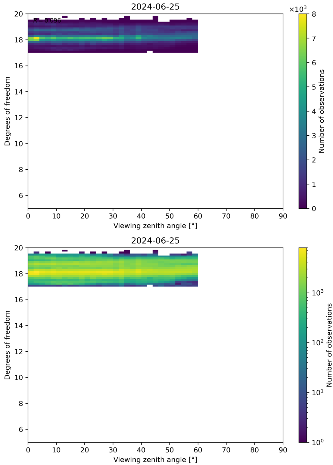
Figure 107: Scatter density plot of “Viewing zenith angle” against “Degrees of freedom” for 2024-06-24 to 2024-06-26.
