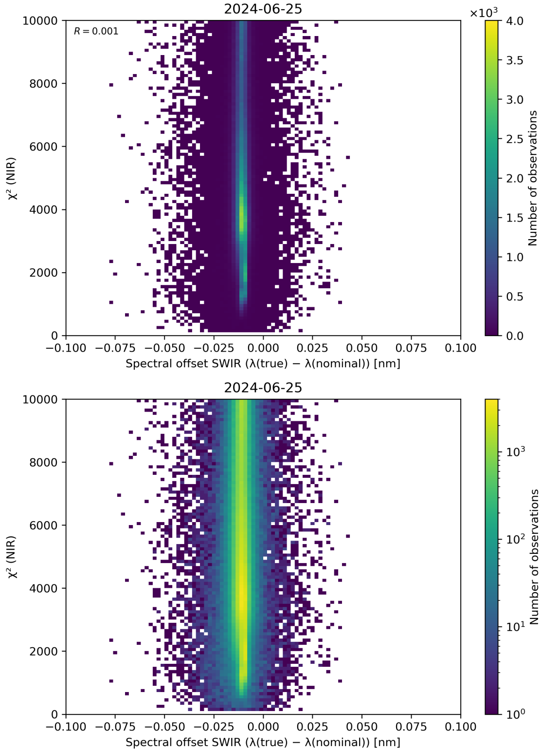
Figure 117: Scatter density plot of “Spectral offset SWIR ( \lambda(\text{true}) - \lambda(\text{nominal}) )” against “ \chi^2 (NIR)” for 2024-06-24 to 2024-06-26.
