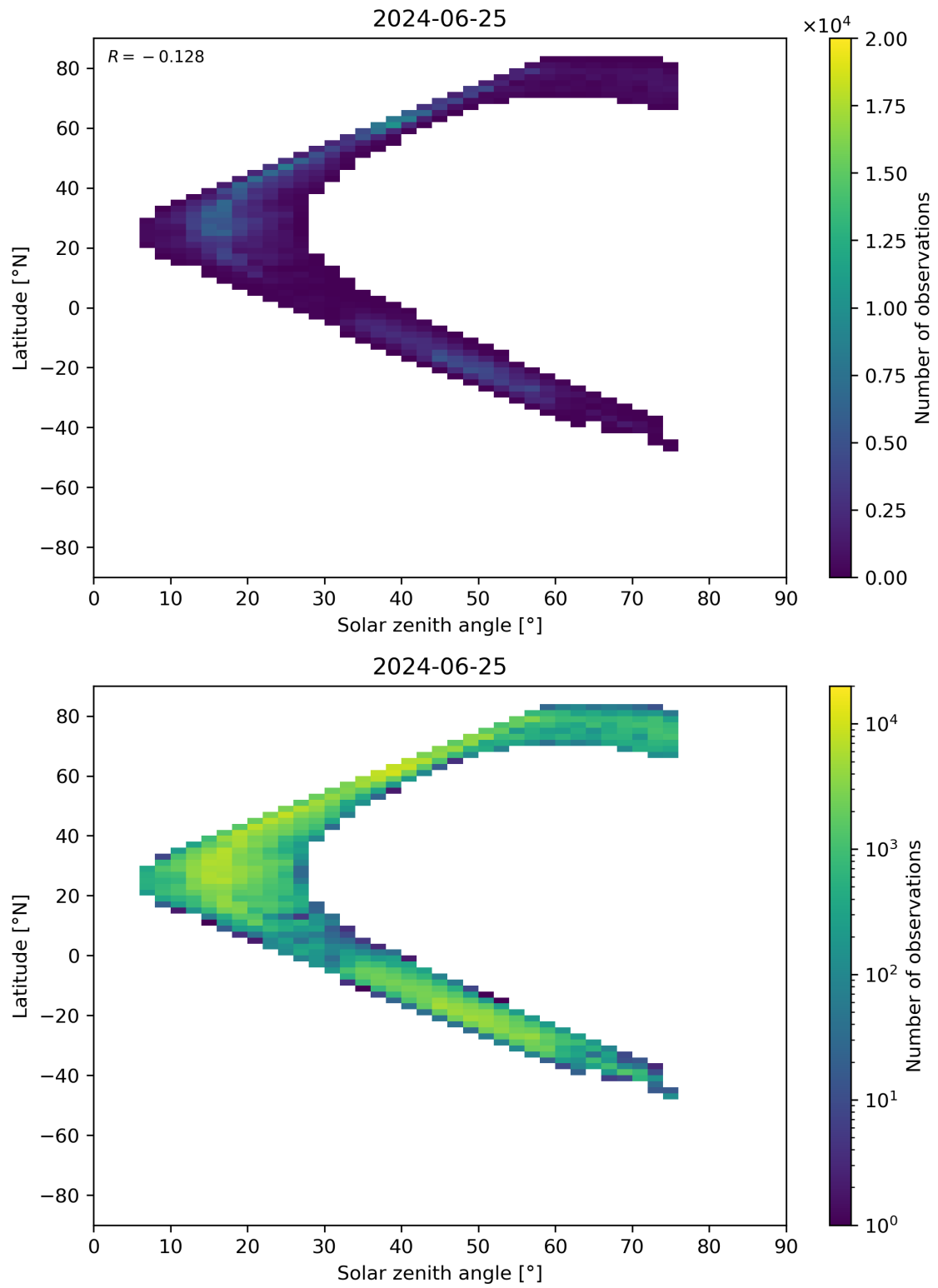
Figure 98: Scatter density plot of “Solar zenith angle” against “Latitude” for 2024-06-24 to 2024-06-26.
