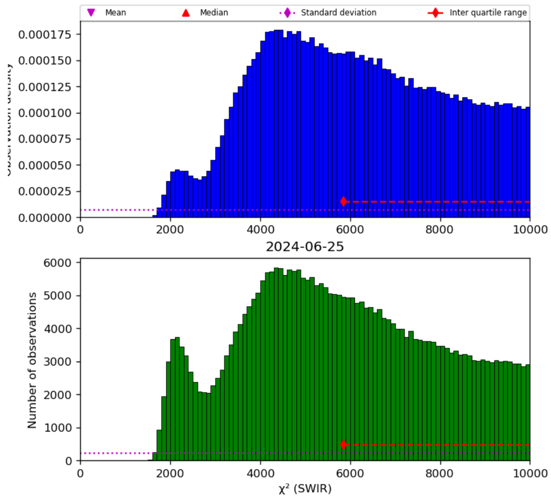
Figure 28: Histogram of “ \chi^2 (SWIR)” for 2024-06-24 to 2024-06-26
