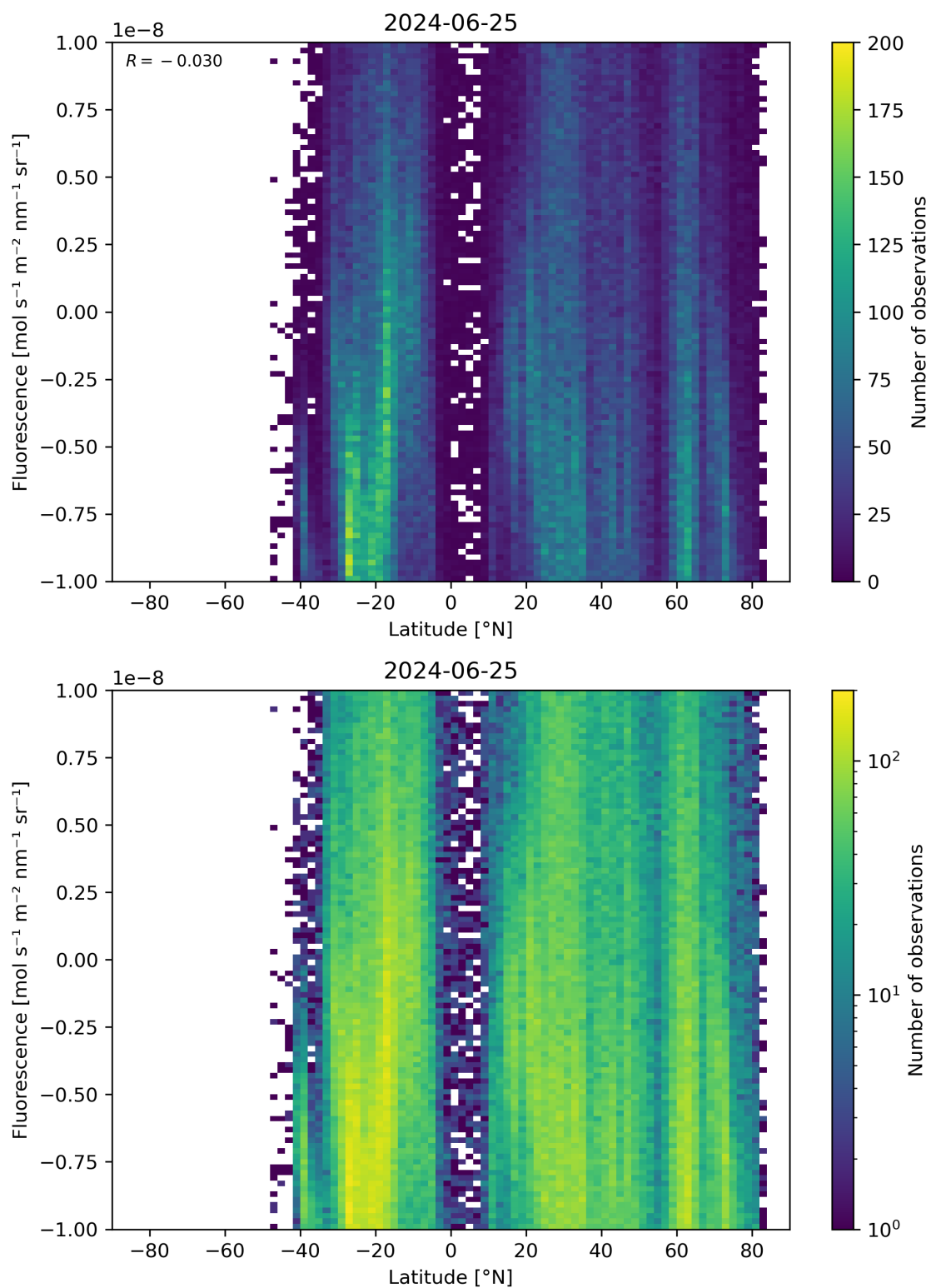
Figure 56: Scatter density plot of “Latitude” against “Fluorescence” for 2024-06-24 to 2024-06-26.
