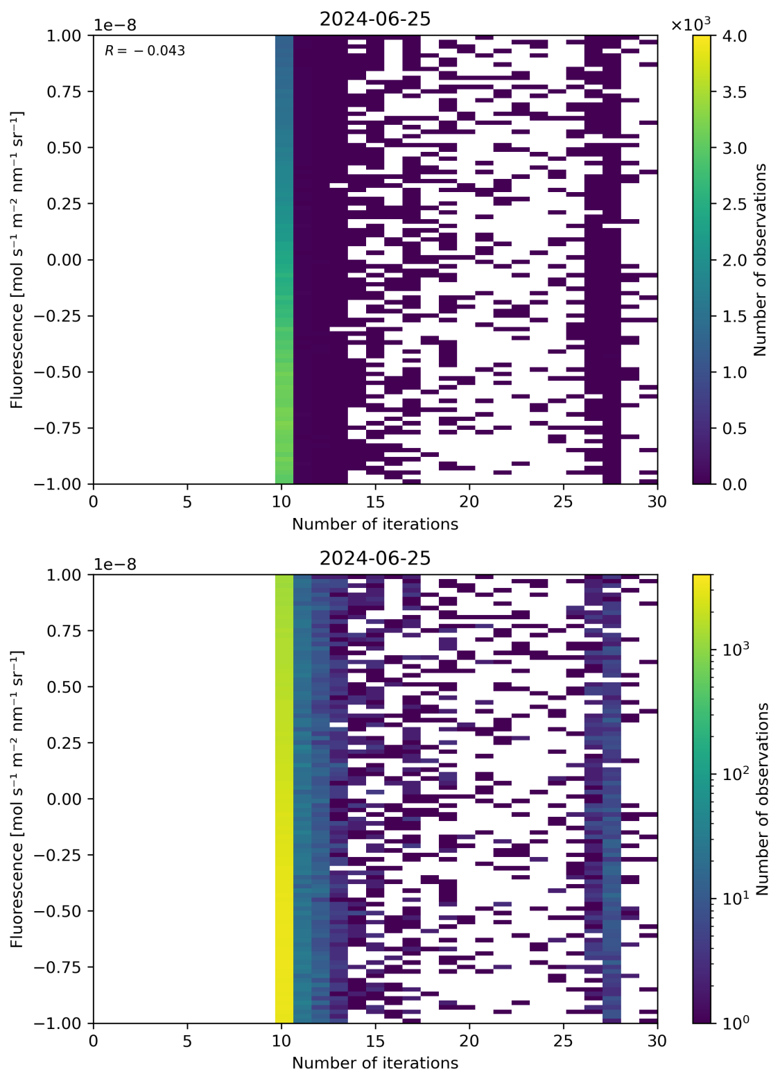
Figure 87: Scatter density plot of “Number of iterations” against “Fluorescence” for 2024-06-24 to 2024-06-26.
