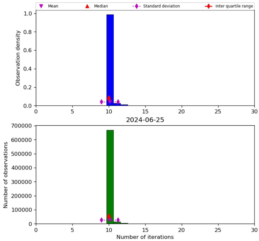
Figure 31: Histogram of “Number of iterations” for 2024-06-24 to 2024-06-26
