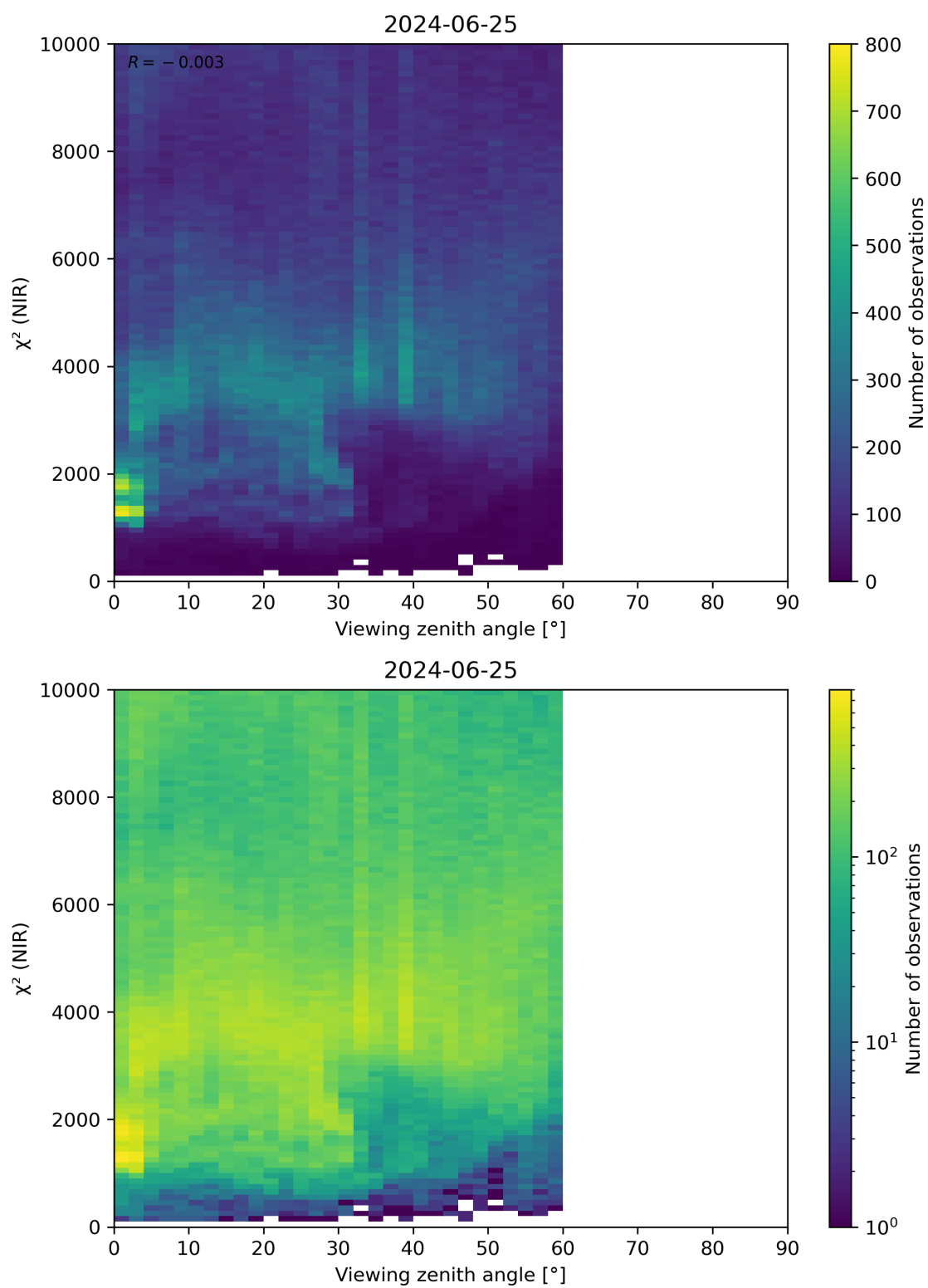
Figure 105: Scatter density plot of “Viewing zenith angle” against “ \chi^2 (NIR)” for 2024-06-24 to 2024-06-26.
