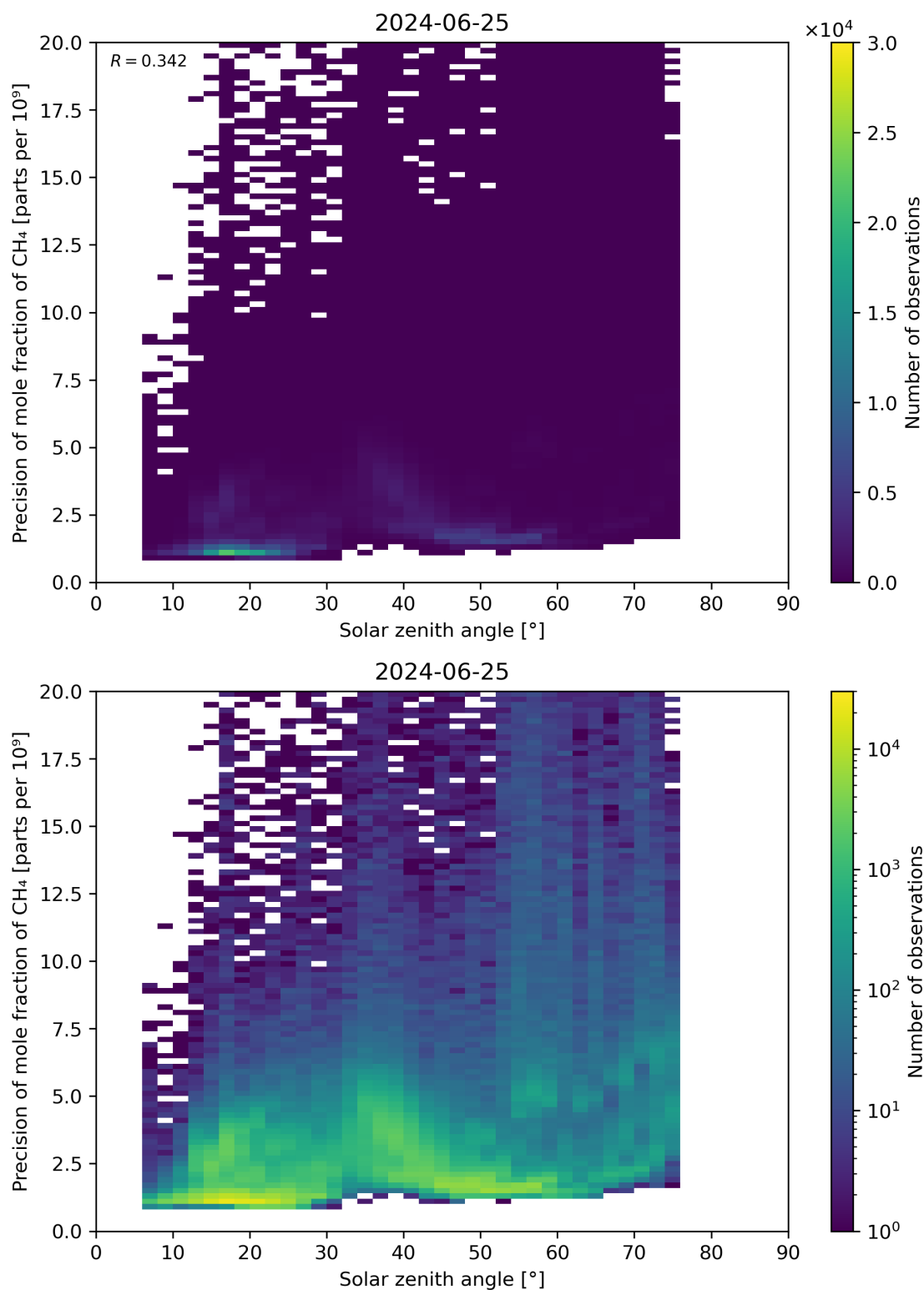
Figure 101: Scatter density plot of “Solar zenith angle” against “Precision of mole fraction of CH 4 ” for 2024-06-24 to 2024-06-26.
