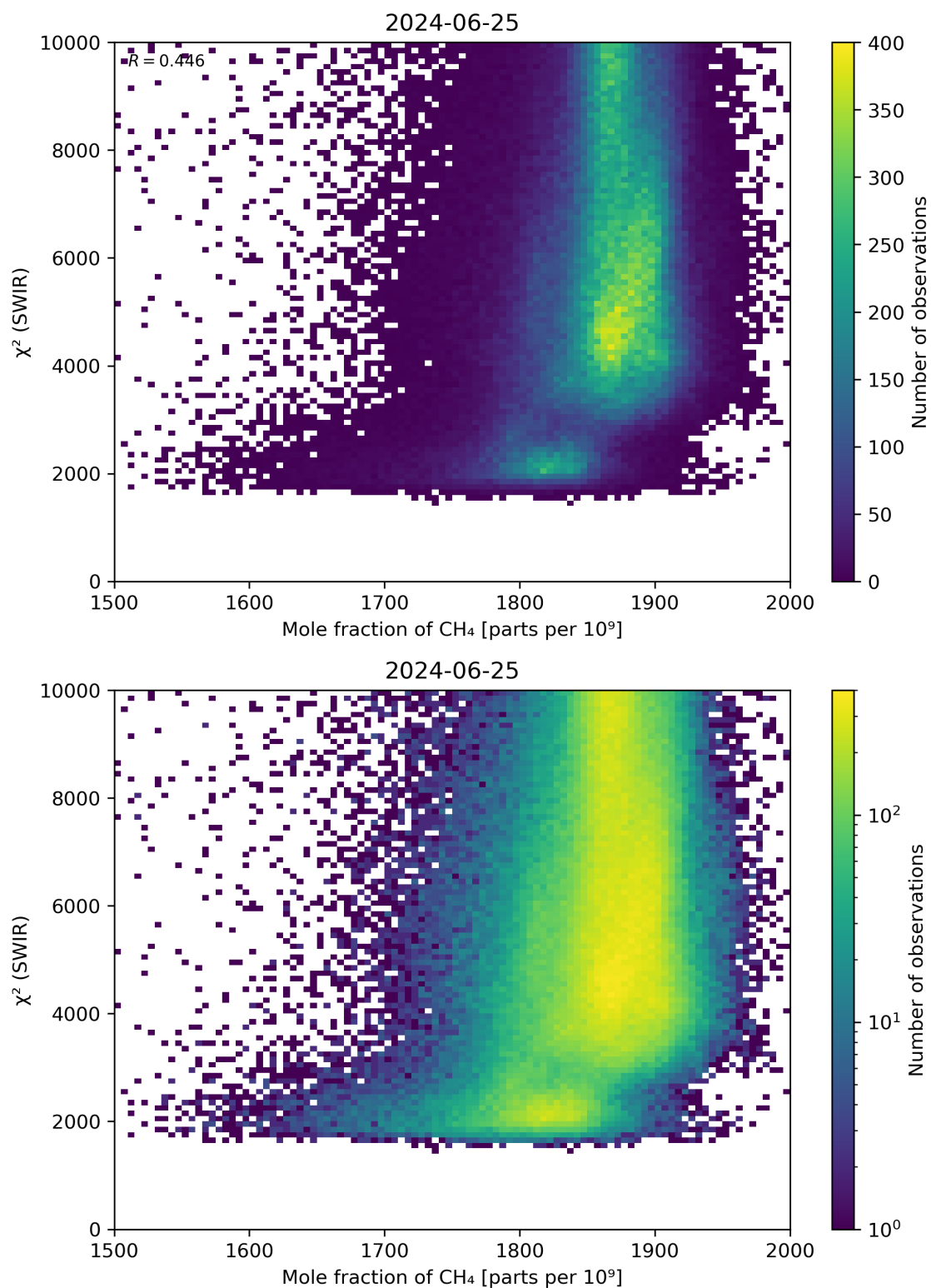
Figure 71: Scatter density plot of “Mole fraction of \text{CH}_4 ” against “ \chi^2 (SWIR)” for 2024-06-24 to 2024-06-26.
