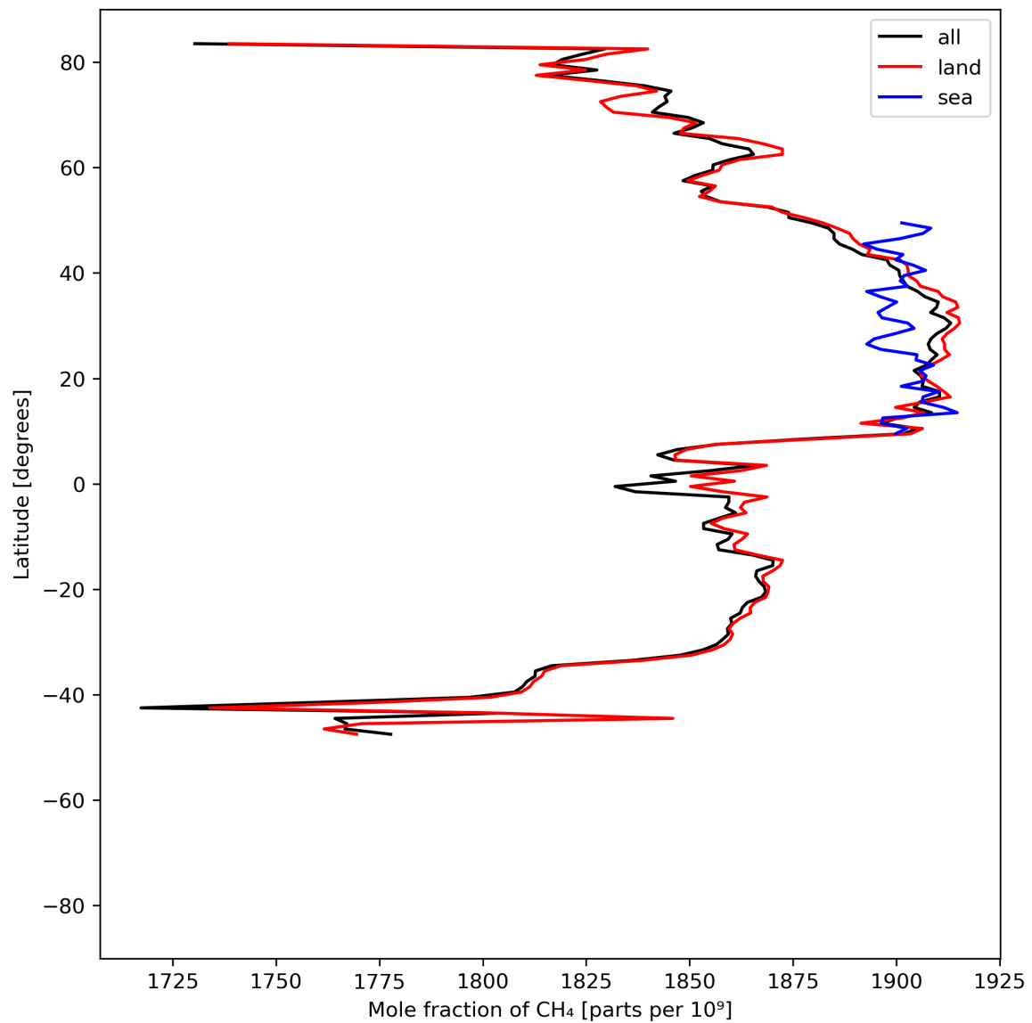
Figure 12: Zonal average of “Mole fraction of \text{CH}_4 ” for 2024-06-24 to 2024-06-26.
