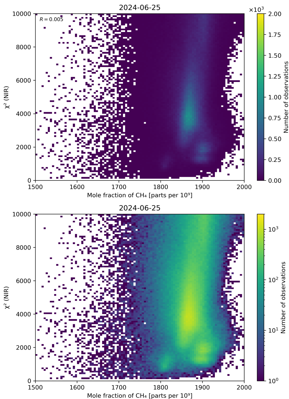
Figure 70: Scatter density plot of “Mole fraction of \text{CH}_4 ” against “ \chi^2 (NIR)” for 2024-06-24 to 2024-06-26.
