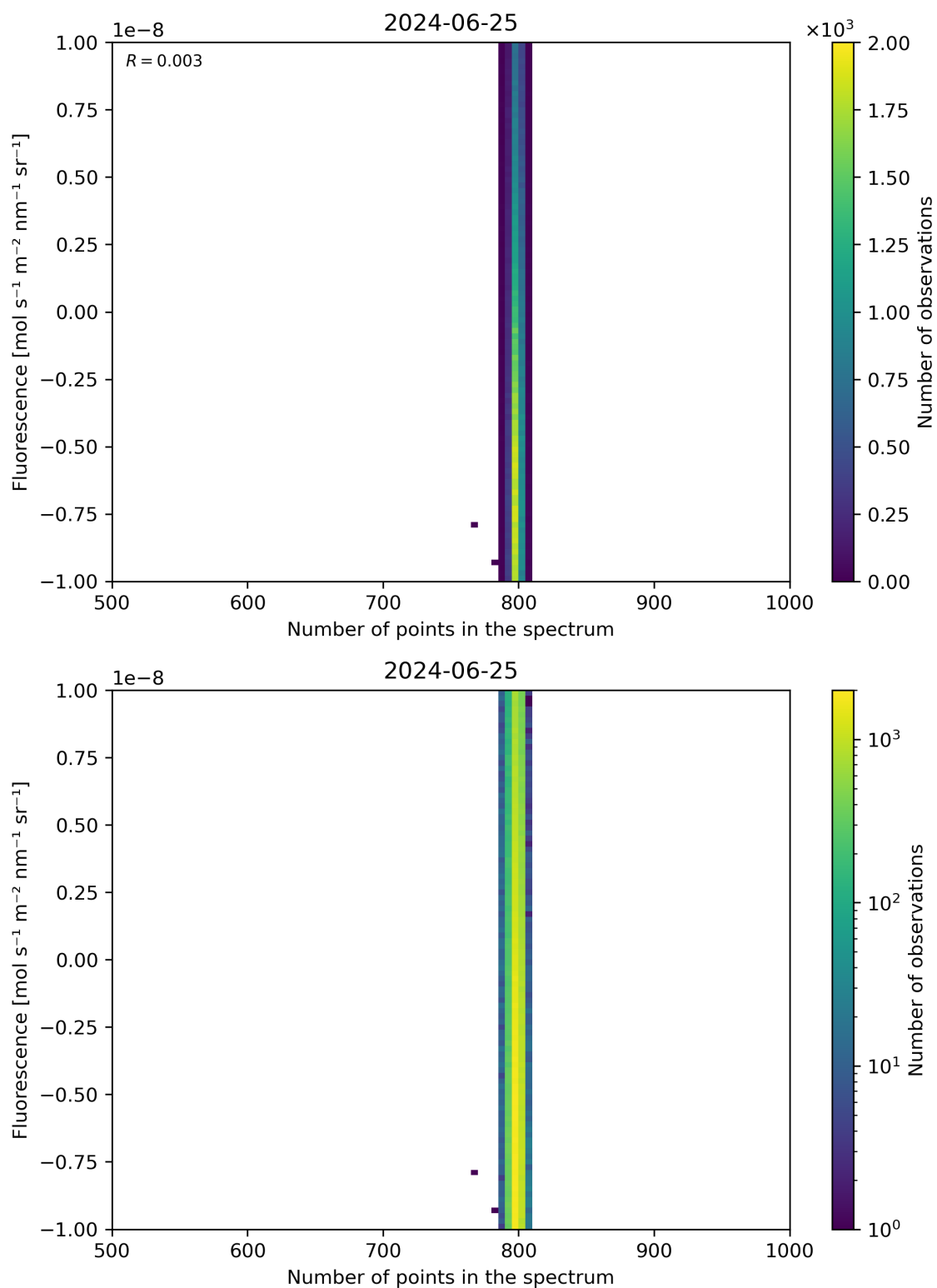
Figure 91: Scatter density plot of “Number of points in the spectrum” against “Fluorescence” for 2024-06-24 to 2024-06-26.
