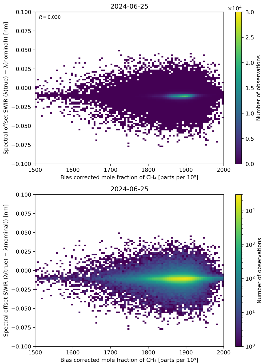
Figure 69: Scatter density plot of “Bias corrected mole fraction of \text{CH}_4 ” against “Spectral offset SWIR ( \lambda(\text{true}) - \lambda(\text{nominal}) )” for 2024-06-24 to 2024-06-26.
