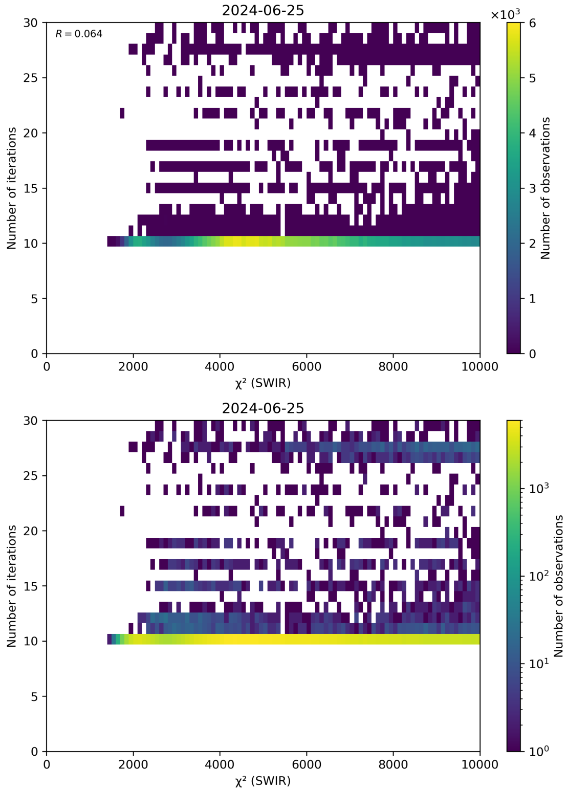
Figure 50: Scatter density plot of “ \chi^2 (SWIR)” against “Number of iterations” for 2024-06-24 to 2024-06-26.
