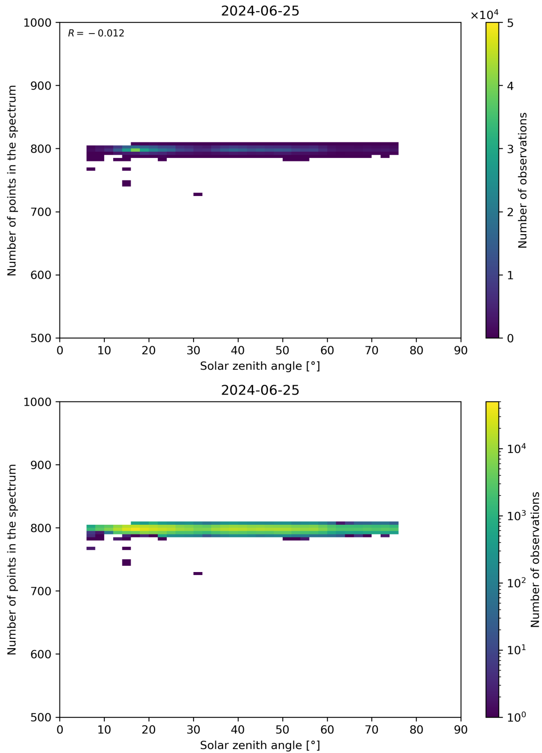
Figure 103: Scatter density plot of “Solar zenith angle” against “Number of points in the spectrum” for 2024-06-24 to 2024-06-26.
