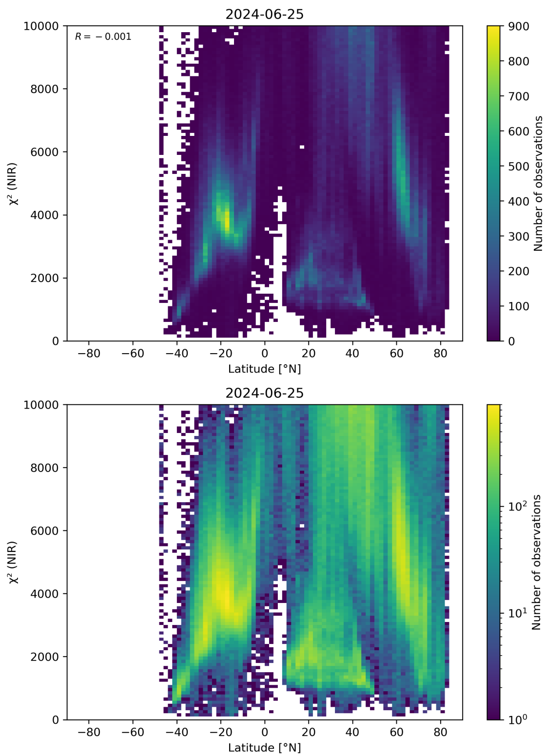
Figure 53: Scatter density plot of “Latitude” against “ \chi^2 (NIR)” for 2024-06-24 to 2024-06-26.
