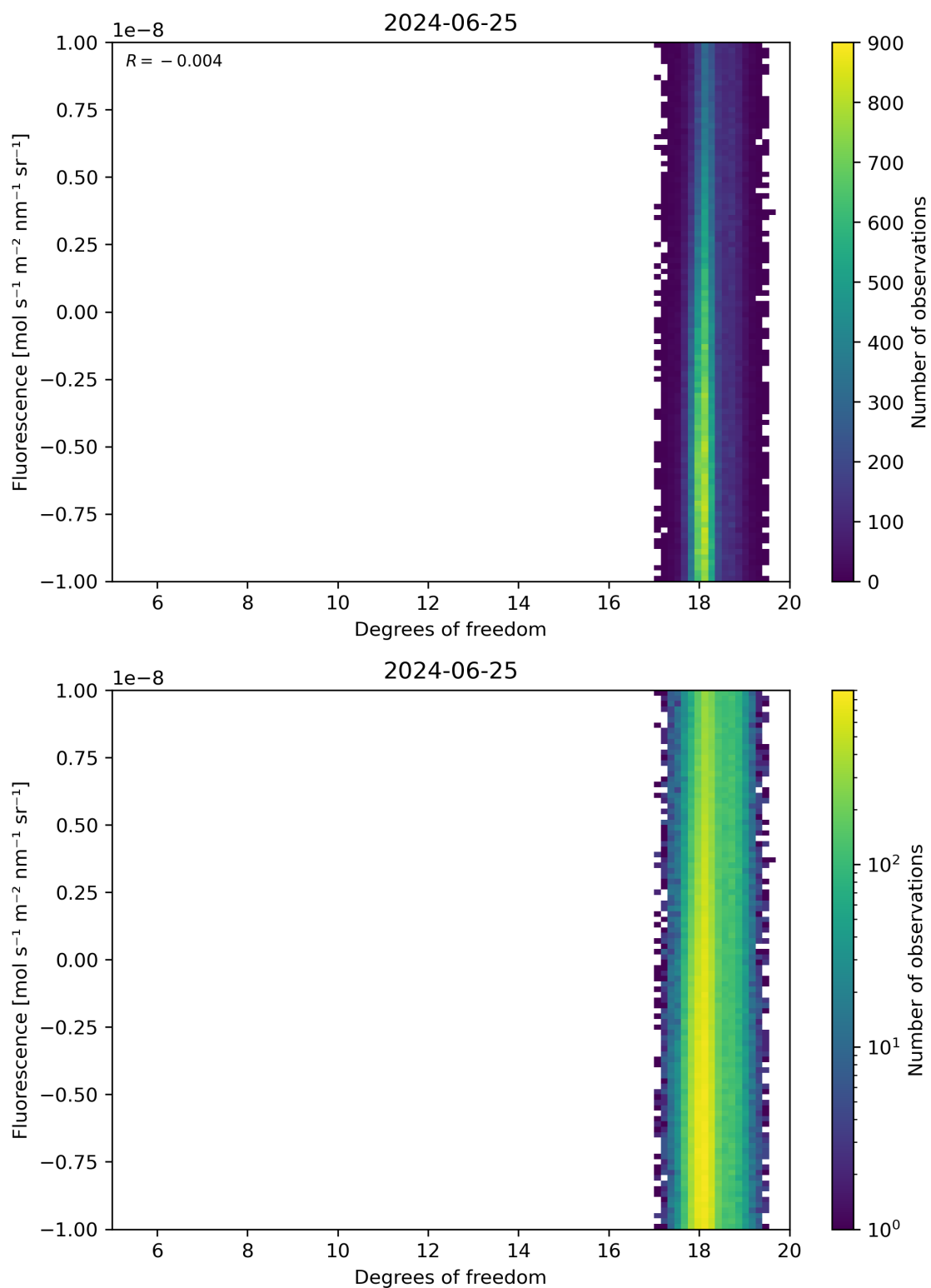
Figure 51: Scatter density plot of “Degrees of freedom” against “Fluorescence” for 2024-06-24 to 2024-06-26.
