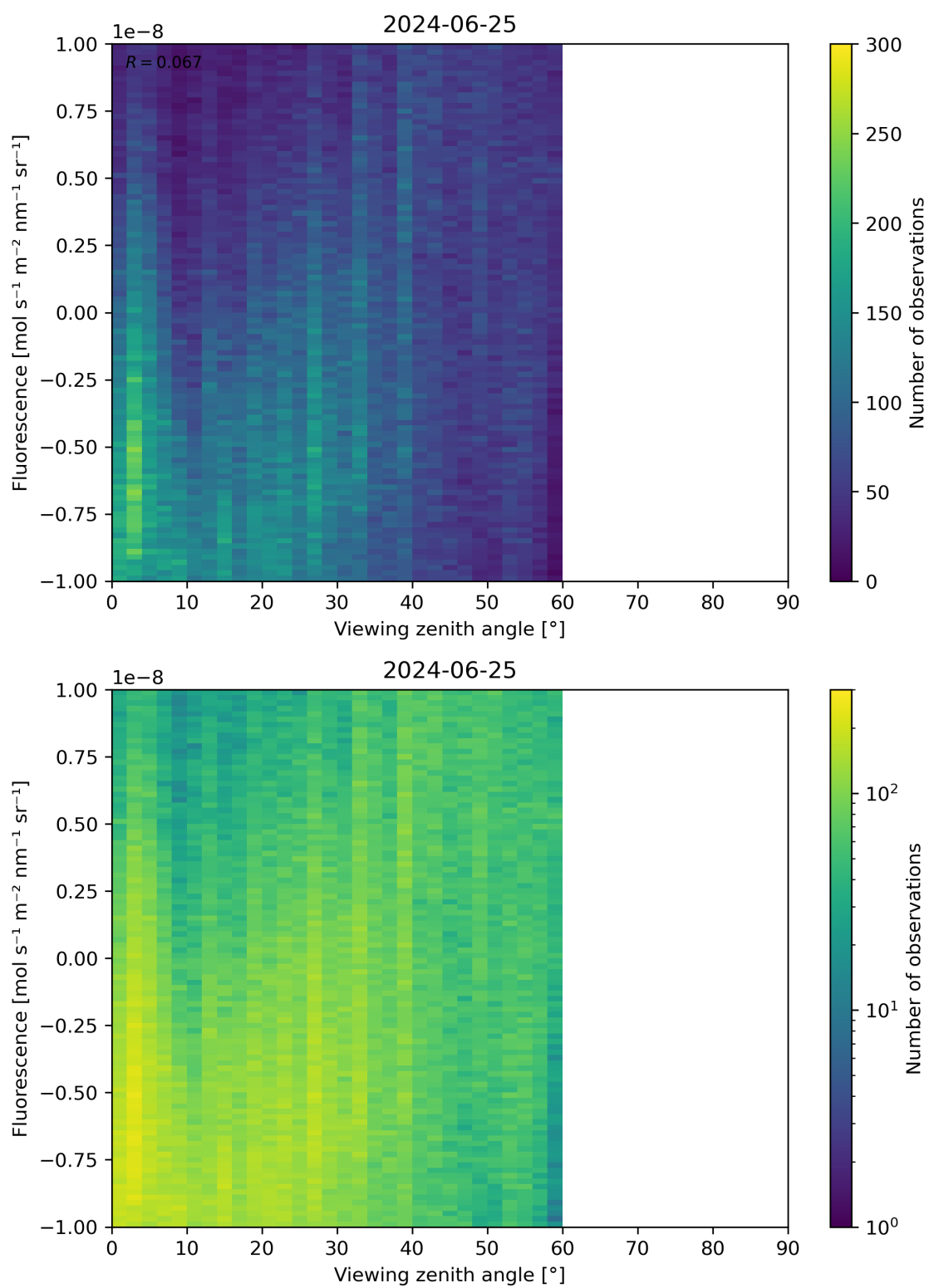
Figure 108: Scatter density plot of “Viewing zenith angle” against “Fluorescence” for 2024-06-24 to 2024-06-26.
