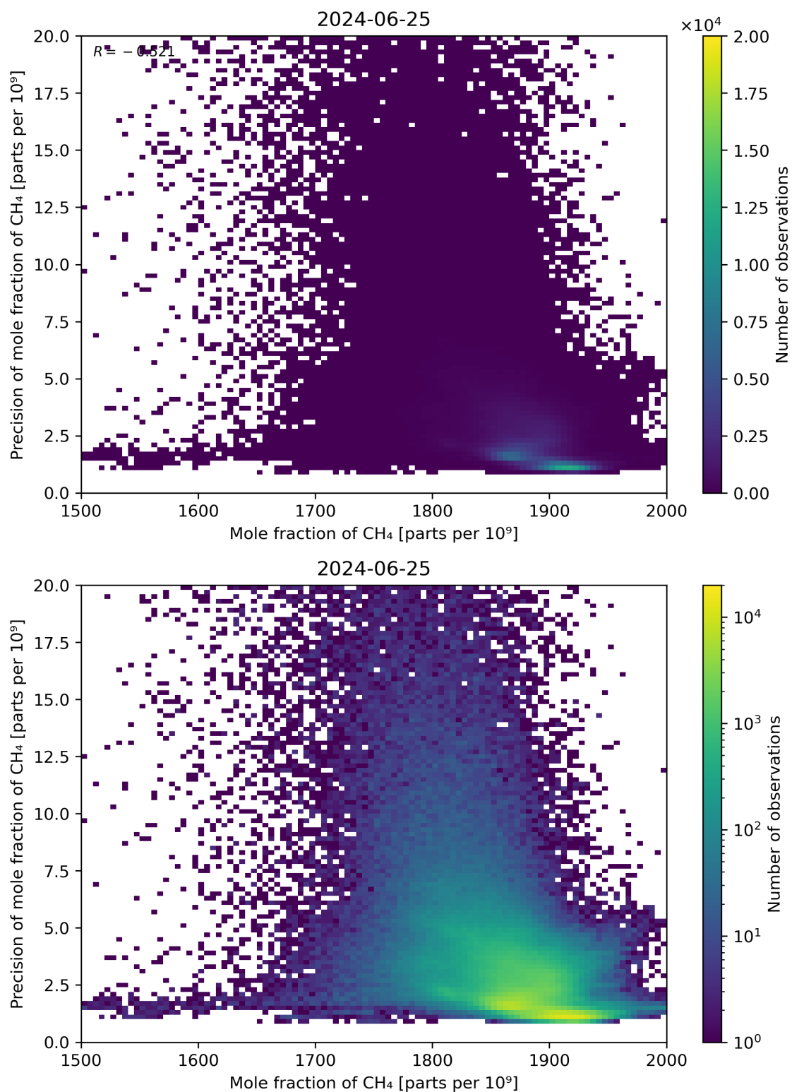
Figure 75: Scatter density plot of “Mole fraction of CH 4 ” against “Precision of mole fraction of CH 4 ” for 2024-06-24 to 2024-06-26.
