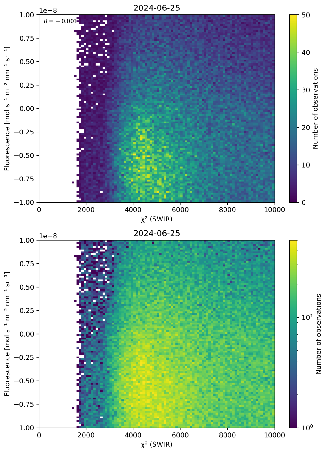
Figure 49: Scatter density plot of “ \chi^2 (SWIR)” against “Fluorescence” for 2024-06-24 to 2024-06-26.
