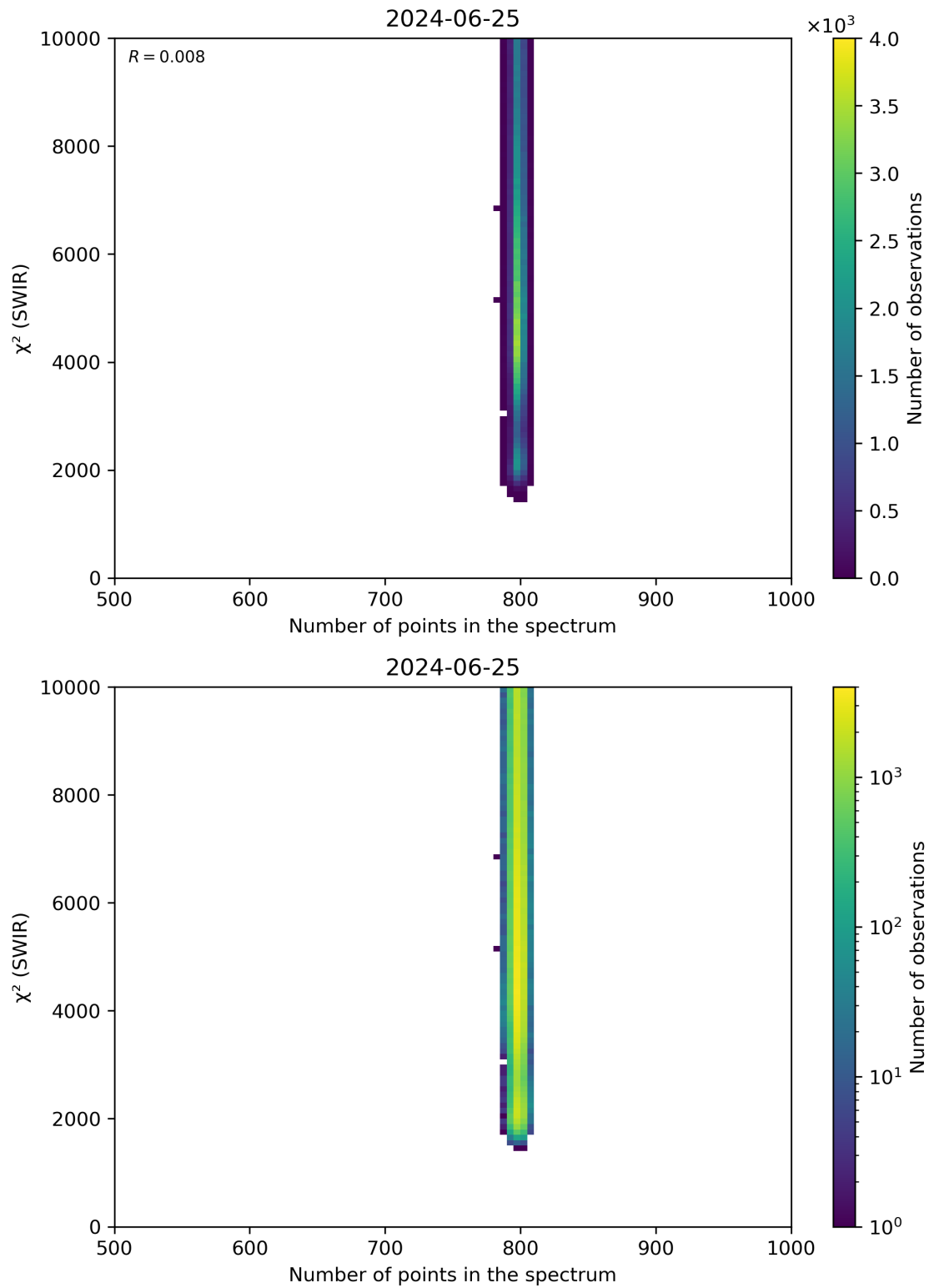
Figure 89: Scatter density plot of “Number of points in the spectrum” against “ \chi^2 (SWIR)” for 2024-06-24 to 2024-06-26.
