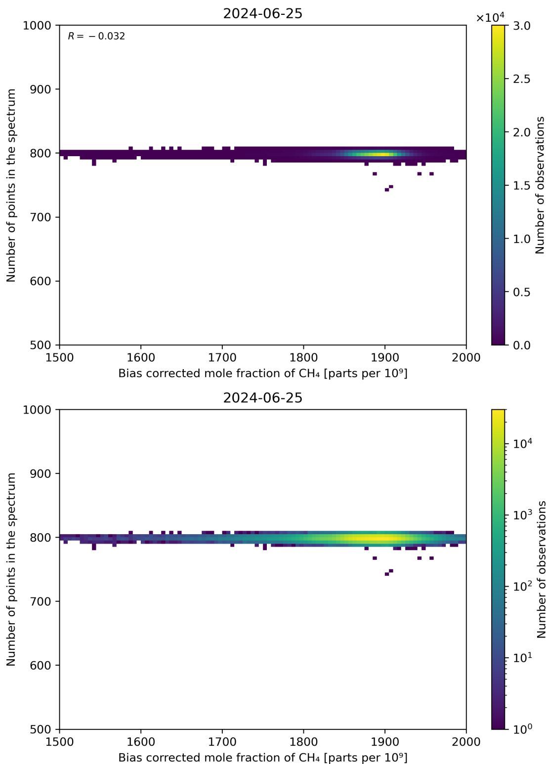
Figure 68: Scatter density plot of “Bias corrected mole fraction of CH 4 ” against “Number of points in the spectrum” for 2024-06-24 to 2024-06-26.
