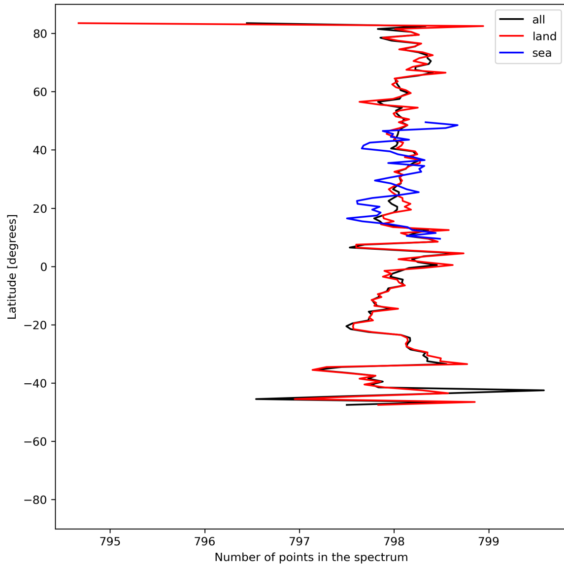
Figure 15: Zonal average of “Number of points in the spectrum” for 2024-06-24 to 2024-06-26.
