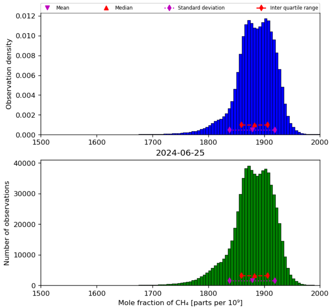
Figure 23: Histogram of “Mole fraction of CH 4 ” for 2024-06-24 to 2024-06-26
