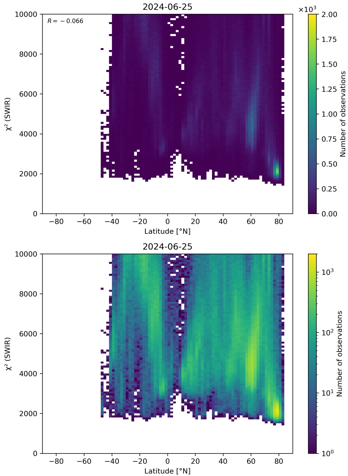
Figure 54: Scatter density plot of “Latitude” against “ \chi^2 (SWIR)” for 2024-06-24 to 2024-06-26.
