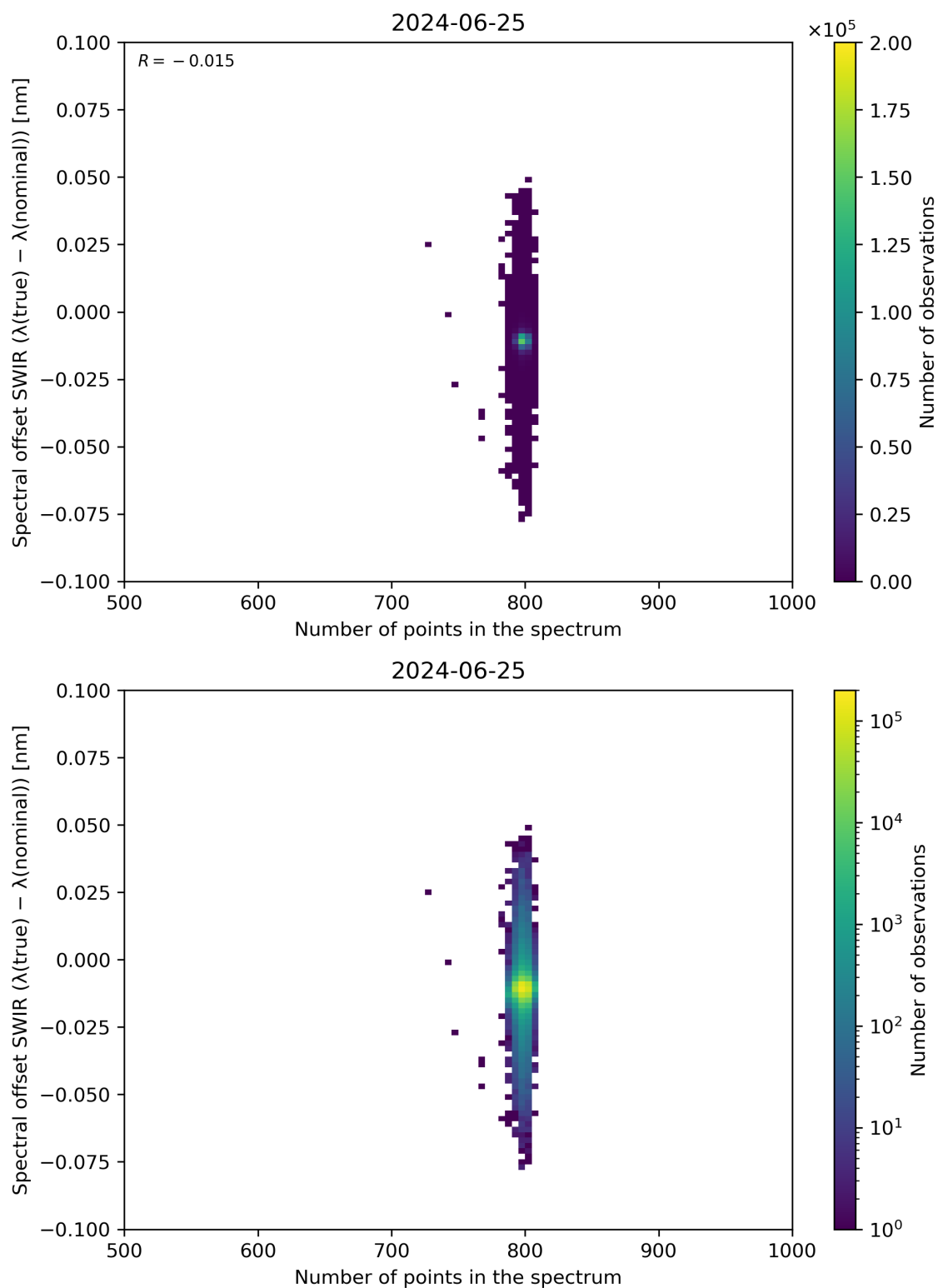
Figure 93: Scatter density plot of “Number of points in the spectrum” against “Spectral offset SWIR ( \lambda(\text{true}) - \lambda(\text{nominal}) )” for 2024-06-24 to 2024-06-26.
