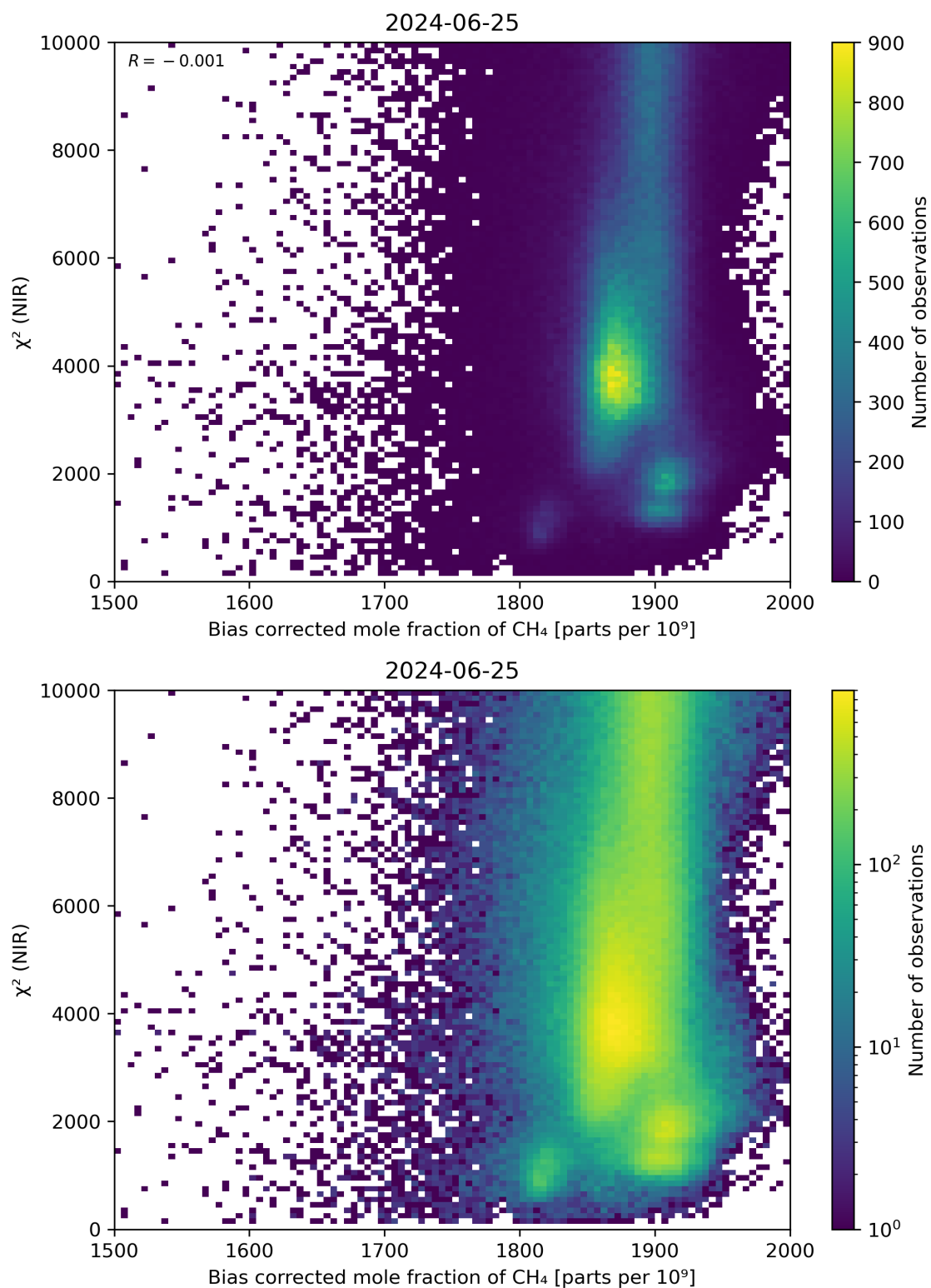
Figure 63: Scatter density plot of “Bias corrected mole fraction of CH 4 ” against “ \chi^2 (NIR)” for 2024-06-24 to 2024-06-26.
