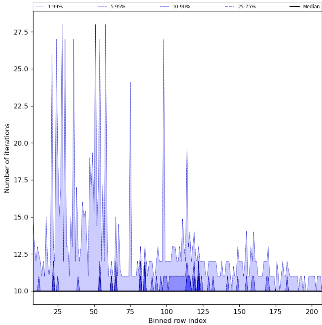
Figure 42: Along track statistics of “Number of iterations” for 2024-06-24 to 2024-06-26
