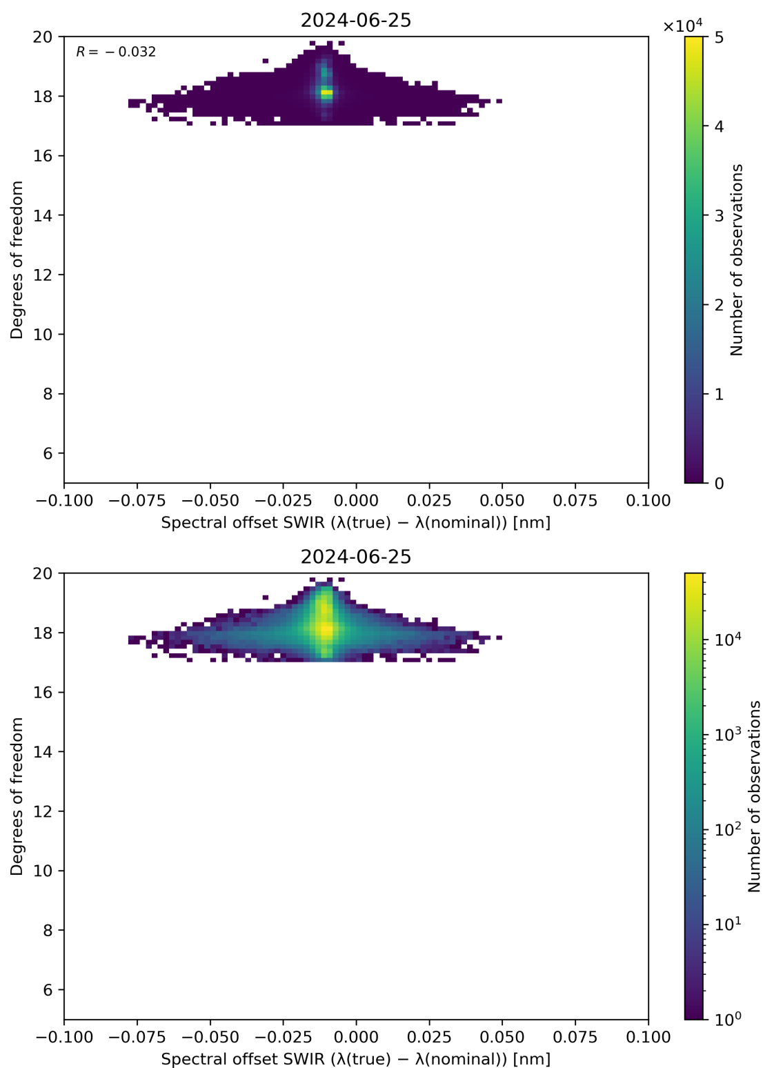
Figure 119: Scatter density plot of “Spectral offset SWIR ( \lambda(\text{true}) - \lambda(\text{nominal}) )” against “Degrees of freedom” for 2024-06-24 to 2024-06-26.
