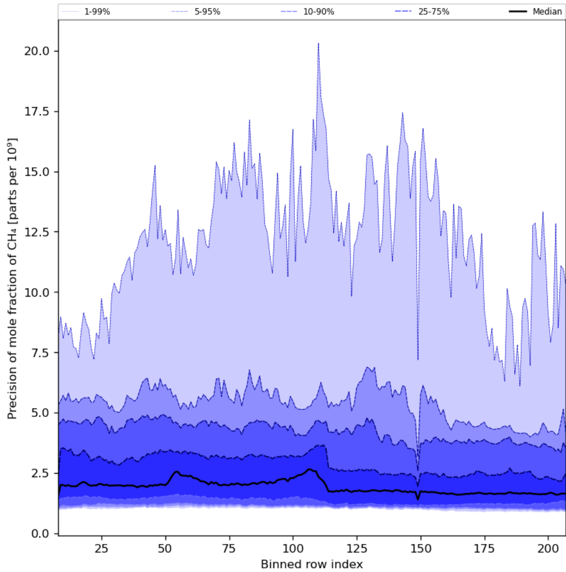
Figure 35: Along track statistics of “Precision of mole fraction of CH 4 ” for 2024-06-24 to 2024-06-26
