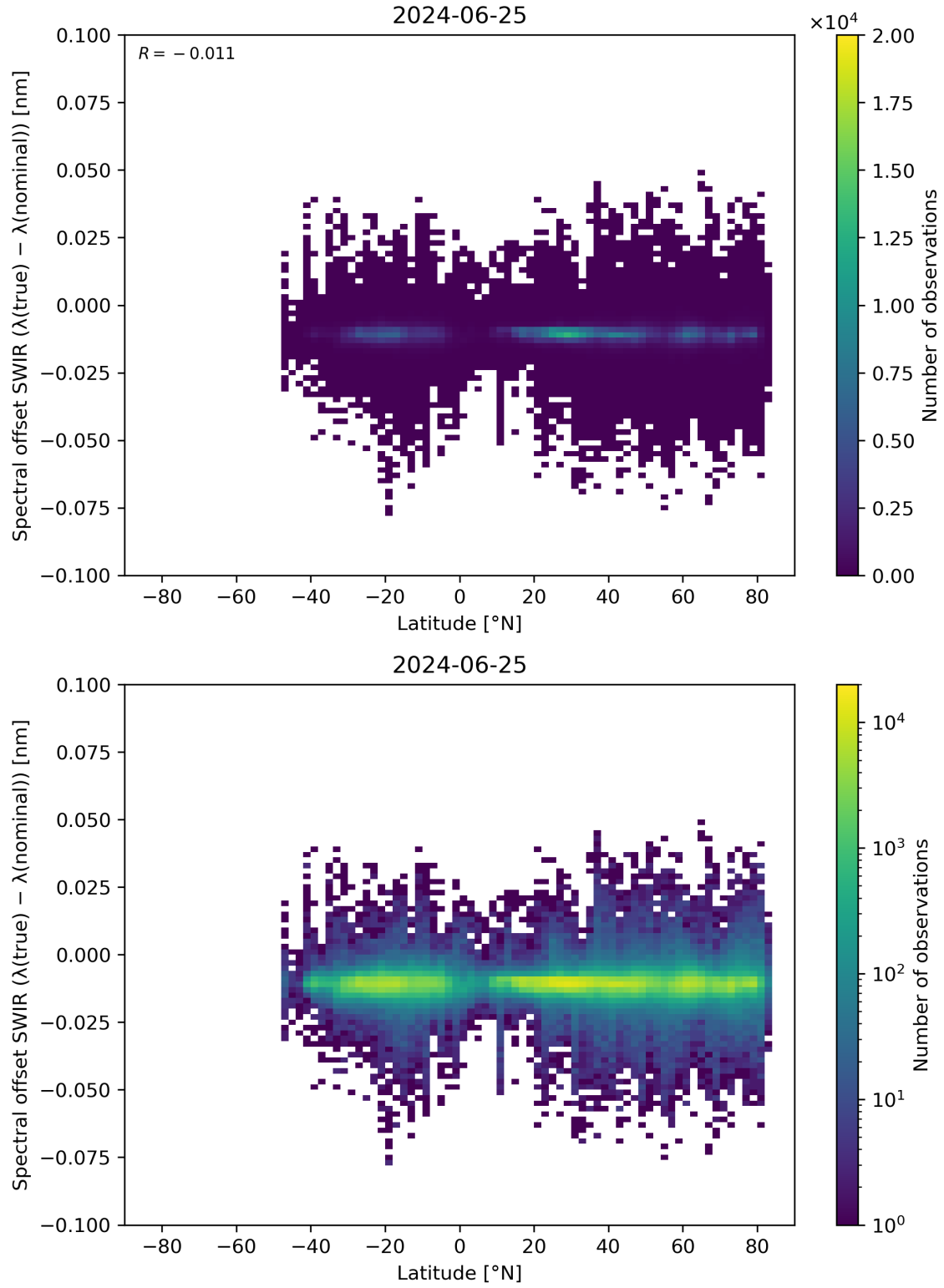
Figure 62: Scatter density plot of “Latitude” against “Spectral offset SWIR ( \lambda(\text{true}) - \lambda(\text{nominal}) )” for 2024-06-24 to 2024-06-26.
