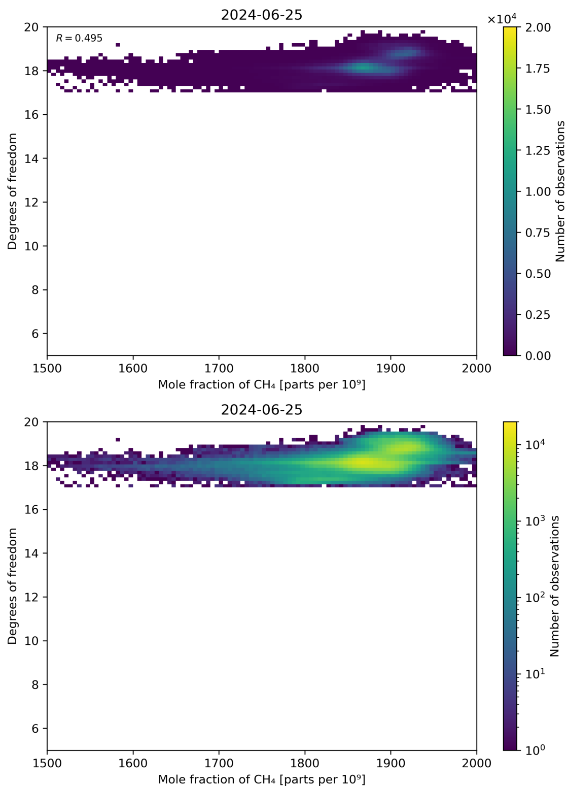
Figure 72: Scatter density plot of “Mole fraction of CH 4 ” against “Degrees of freedom” for 2024-06-24 to 2024-06-26.
