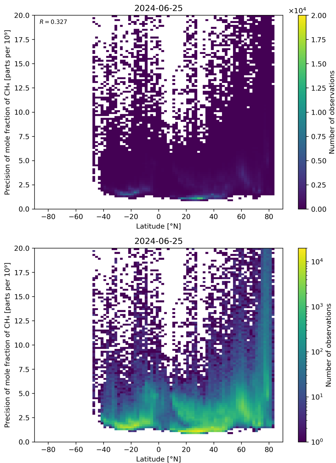
Figure 59: Scatter density plot of “Latitude” against “Precision of mole fraction of CH 4 ” for 2024-06-24 to 2024-06-26.
