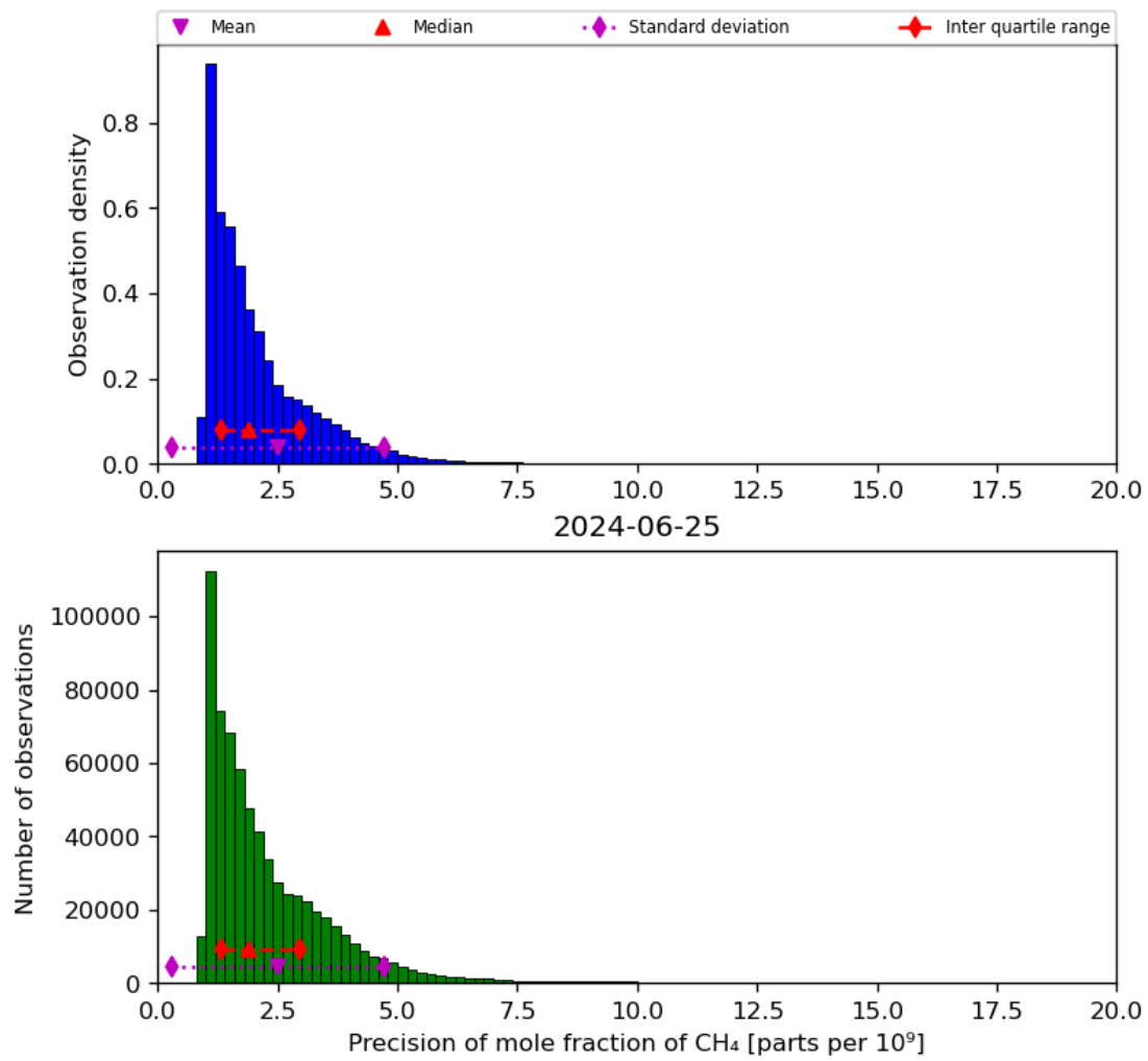
Figure 24: Histogram of “Precision of mole fraction of CH 4 ” for 2024-06-24 to 2024-06-26
