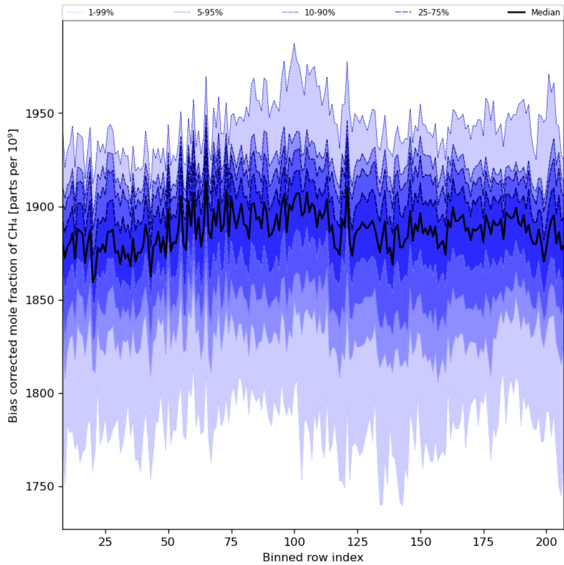
Figure 36: Along track statistics of “Bias corrected mole fraction of CH 4 ” for 2024-06-24 to 2024-06-26
