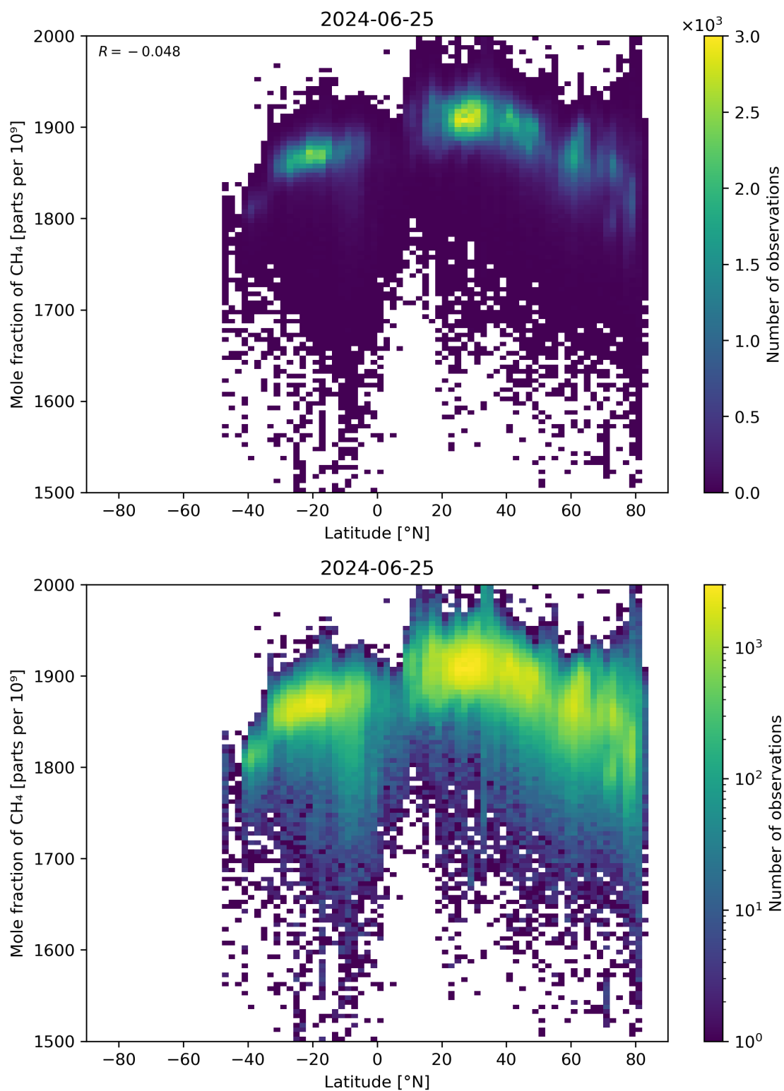
Figure 57: Scatter density plot of “Latitude” against “Mole fraction of CH 4 ” for 2024-06-24 to 2024-06-26.
