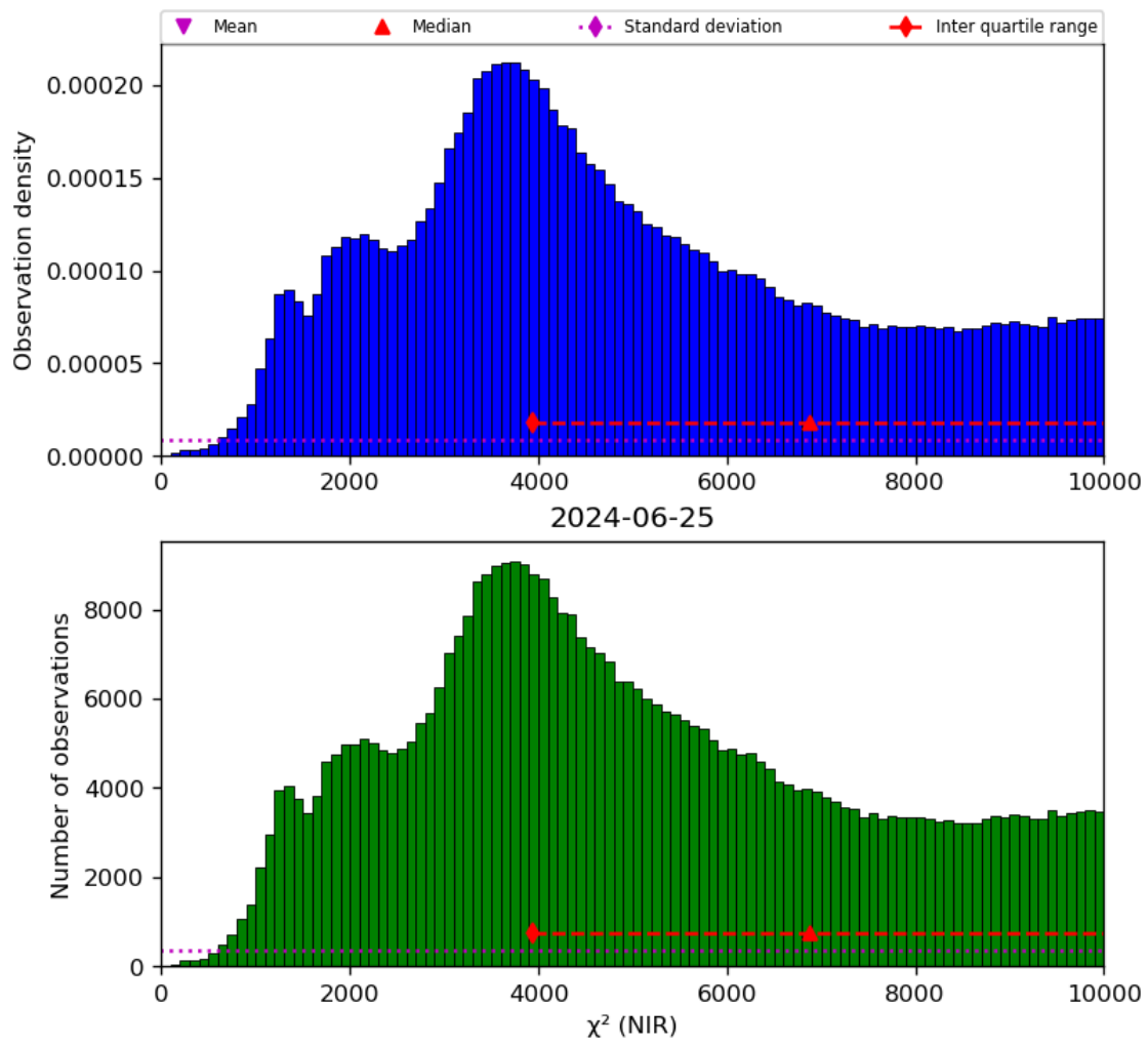
Figure 29: Histogram of “ \chi^2 (NIR)” for 2024-06-24 to 2024-06-26
