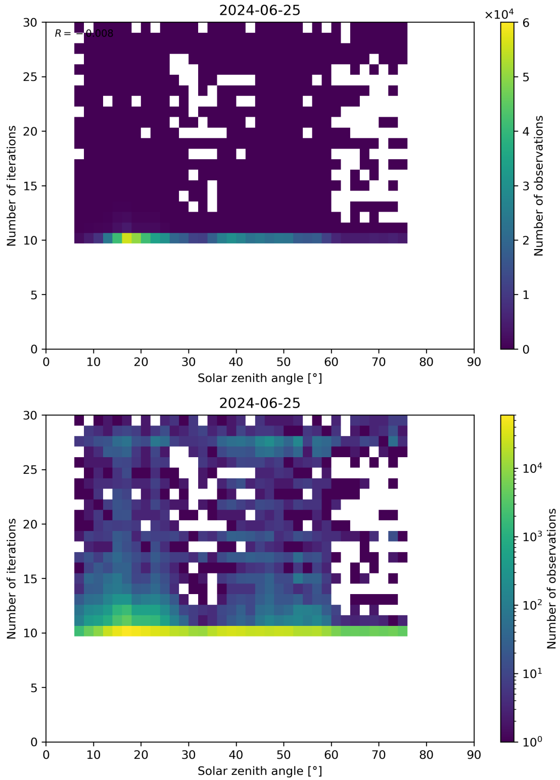
Figure 102: Scatter density plot of “Solar zenith angle” against “Number of iterations” for 2024-06-24 to 2024-06-26.
