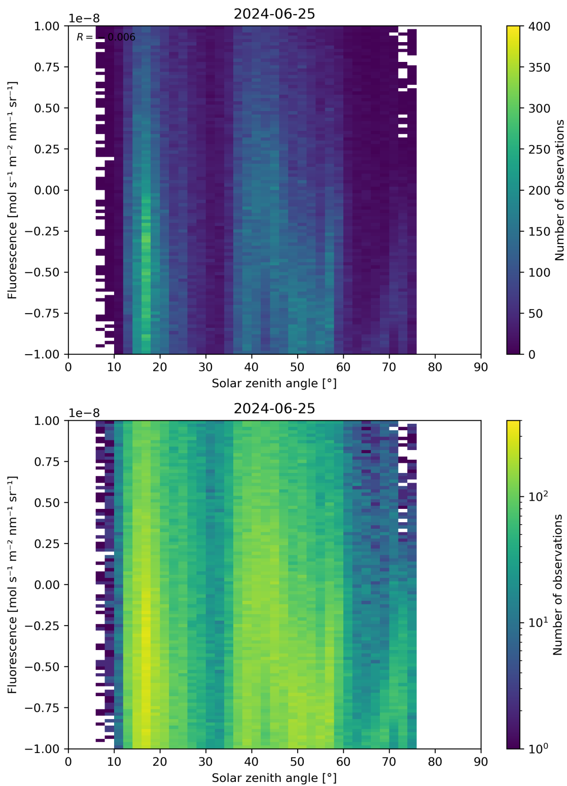
Figure 97: Scatter density plot of “Solar zenith angle” against “Fluorescence” for 2024-06-24 to 2024-06-26.
