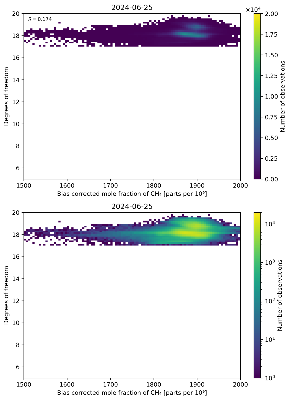
Figure 65: Scatter density plot of “Bias corrected mole fraction of CH 4 ” against “Degrees of freedom” for 2024-06-24 to 2024-06-26.
