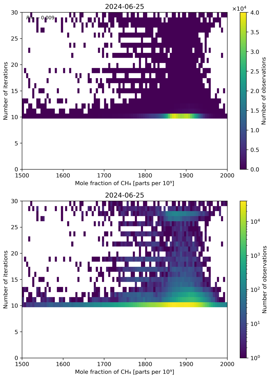
Figure 76: Scatter density plot of “Mole fraction of CH 4 ” against “Number of iterations” for 2024-06-24 to 2024-06-26.
