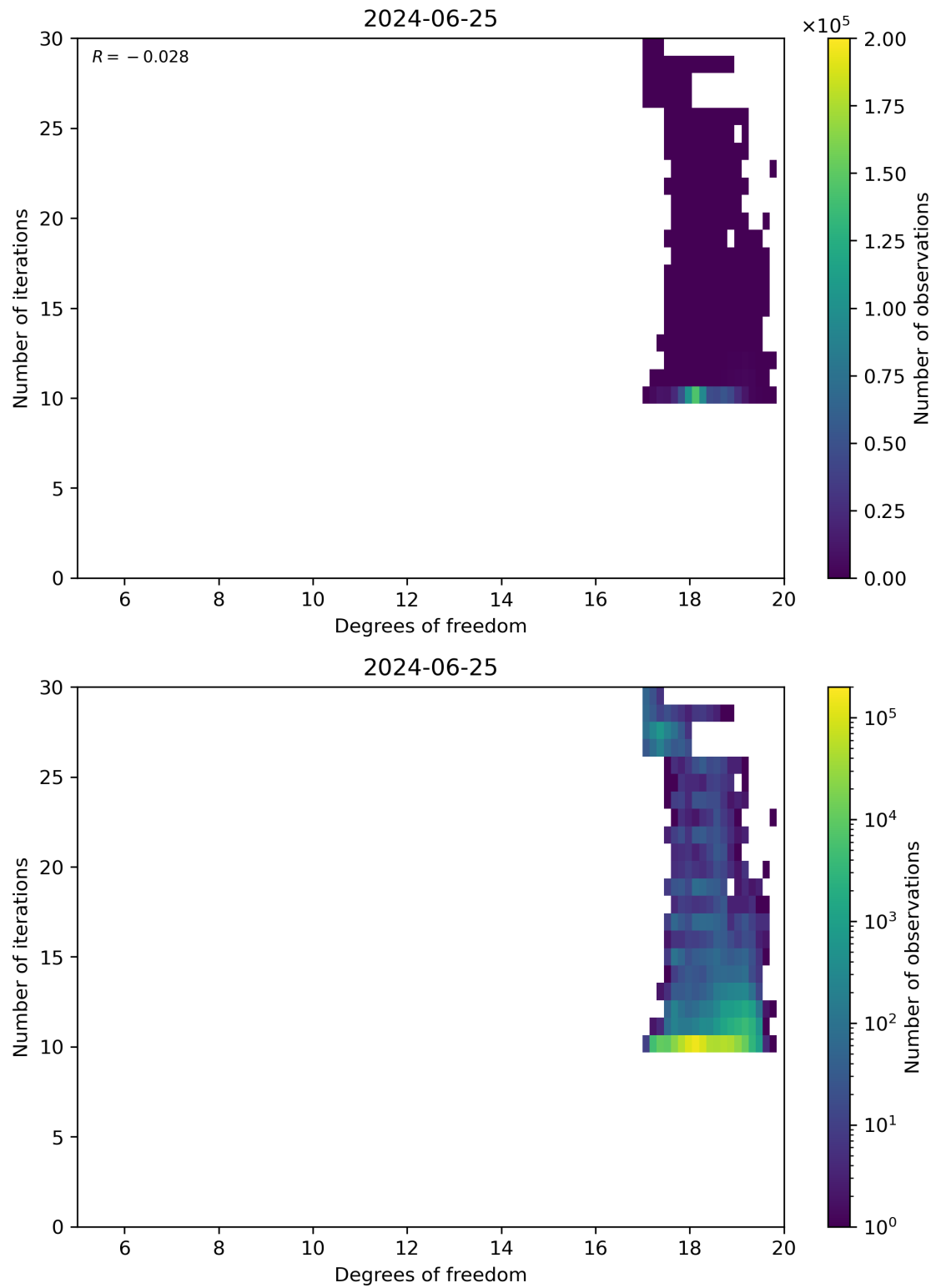
Figure 52: Scatter density plot of “Degrees of freedom” against “Number of iterations” for 2024-06-24 to 2024-06-26.
