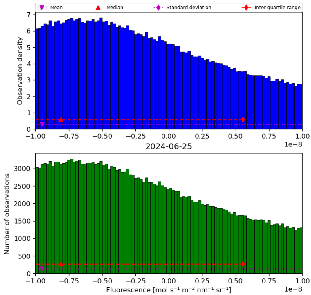
Figure 32: Histogram of “Fluorescence” for 2024-06-24 to 2024-06-26
