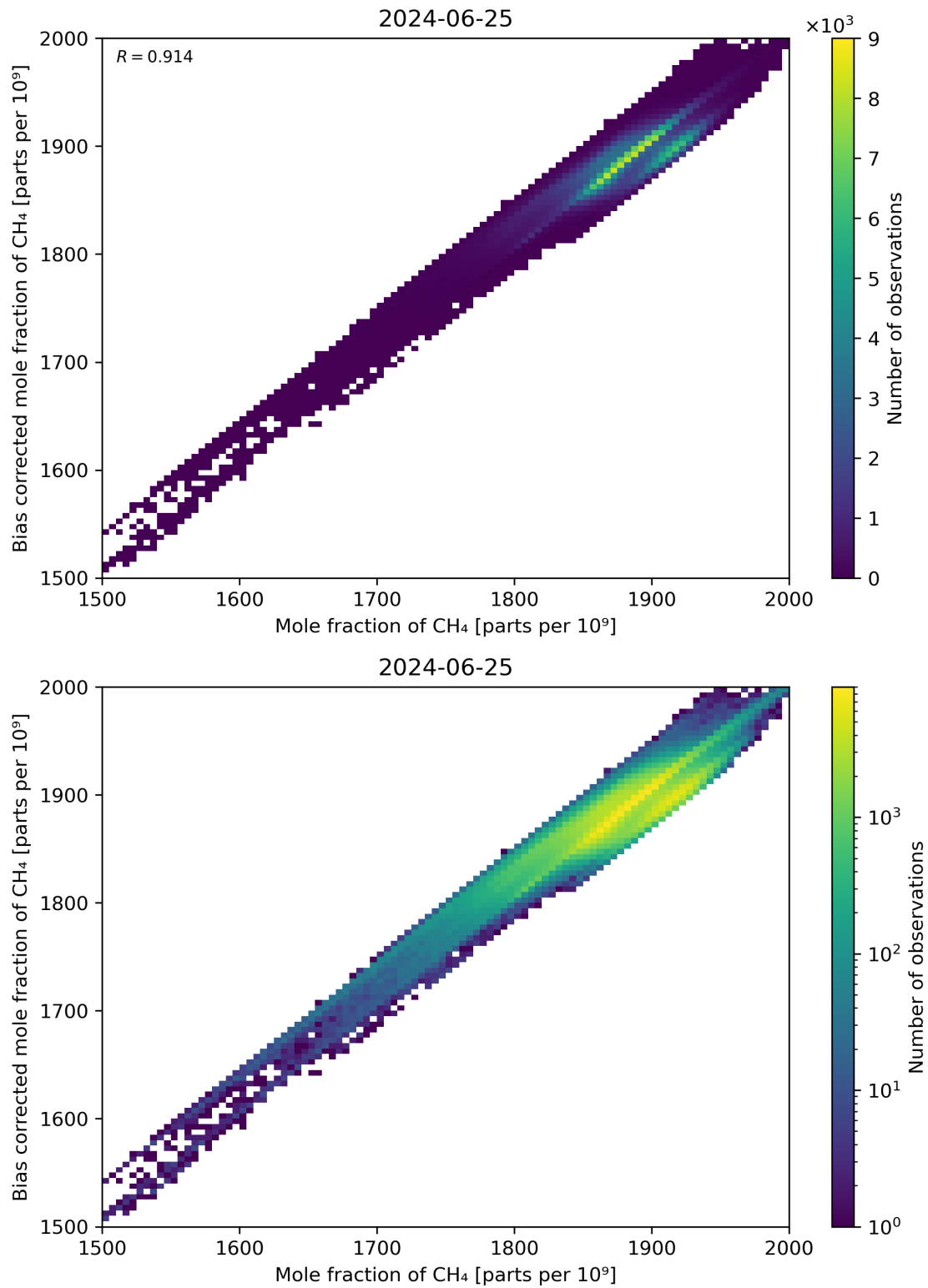
Figure 74: Scatter density plot of “Mole fraction of CH 4 ” against “Bias corrected mole fraction of CH 4 ” for 2024-06-24 to 2024-06-26.
