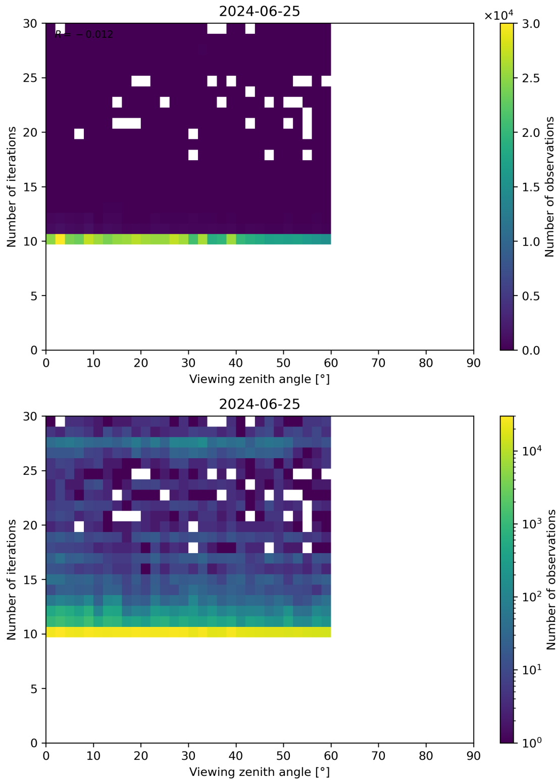
Figure 113: Scatter density plot of “Viewing zenith angle” against “Number of iterations” for 2024-06-24 to 2024-06-26.
