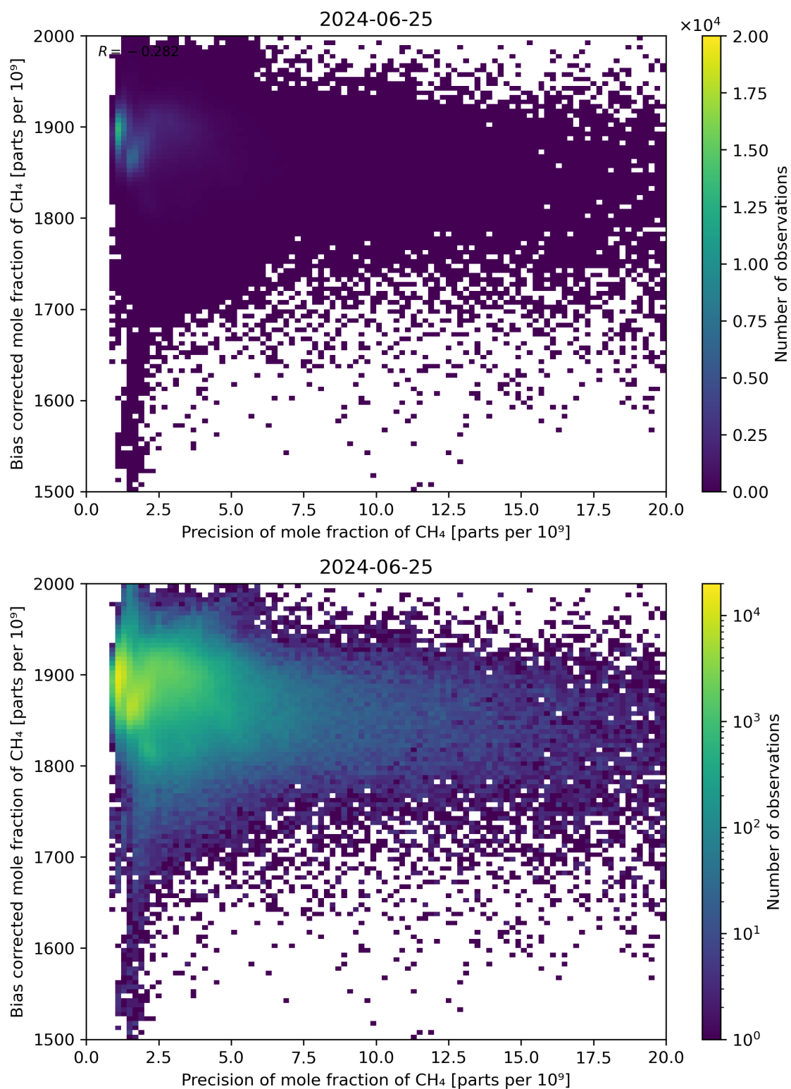
Figure 82: Scatter density plot of “Precision of mole fraction of CH 4 ” against “Bias corrected mole fraction of CH 4 ” for 2024-06-24 to 2024-06-26.
