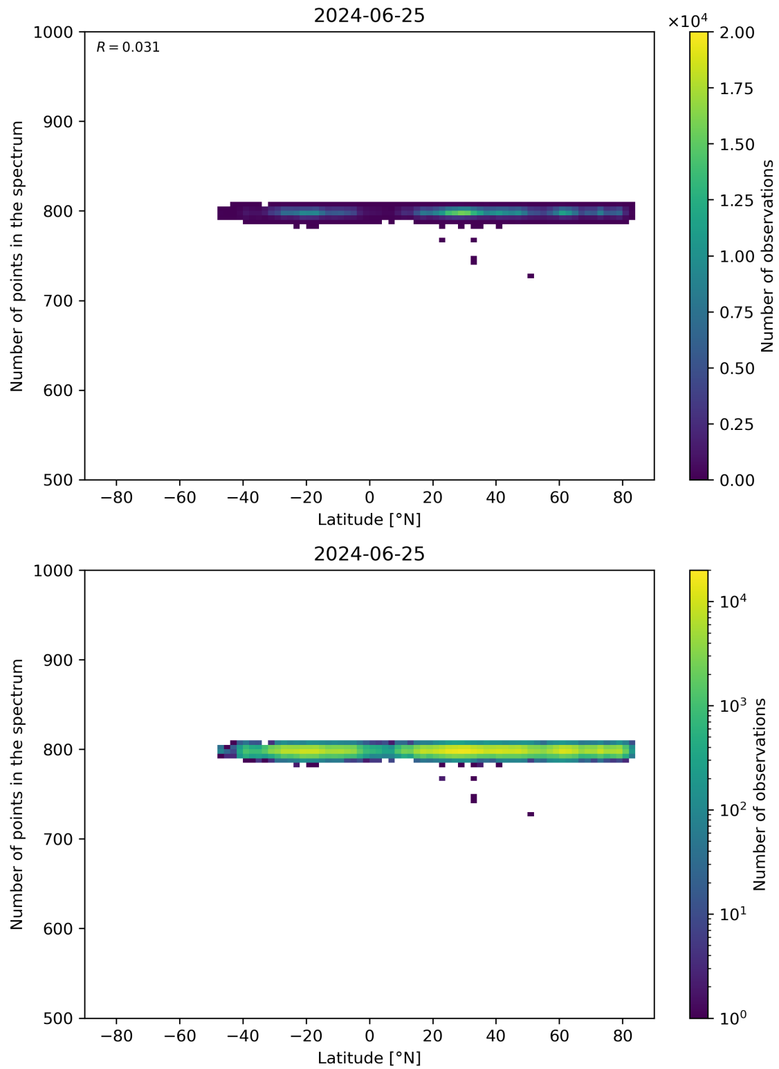
Figure 61: Scatter density plot of “Latitude” against “Number of points in the spectrum” for 2024-06-24 to 2024-06-26.
