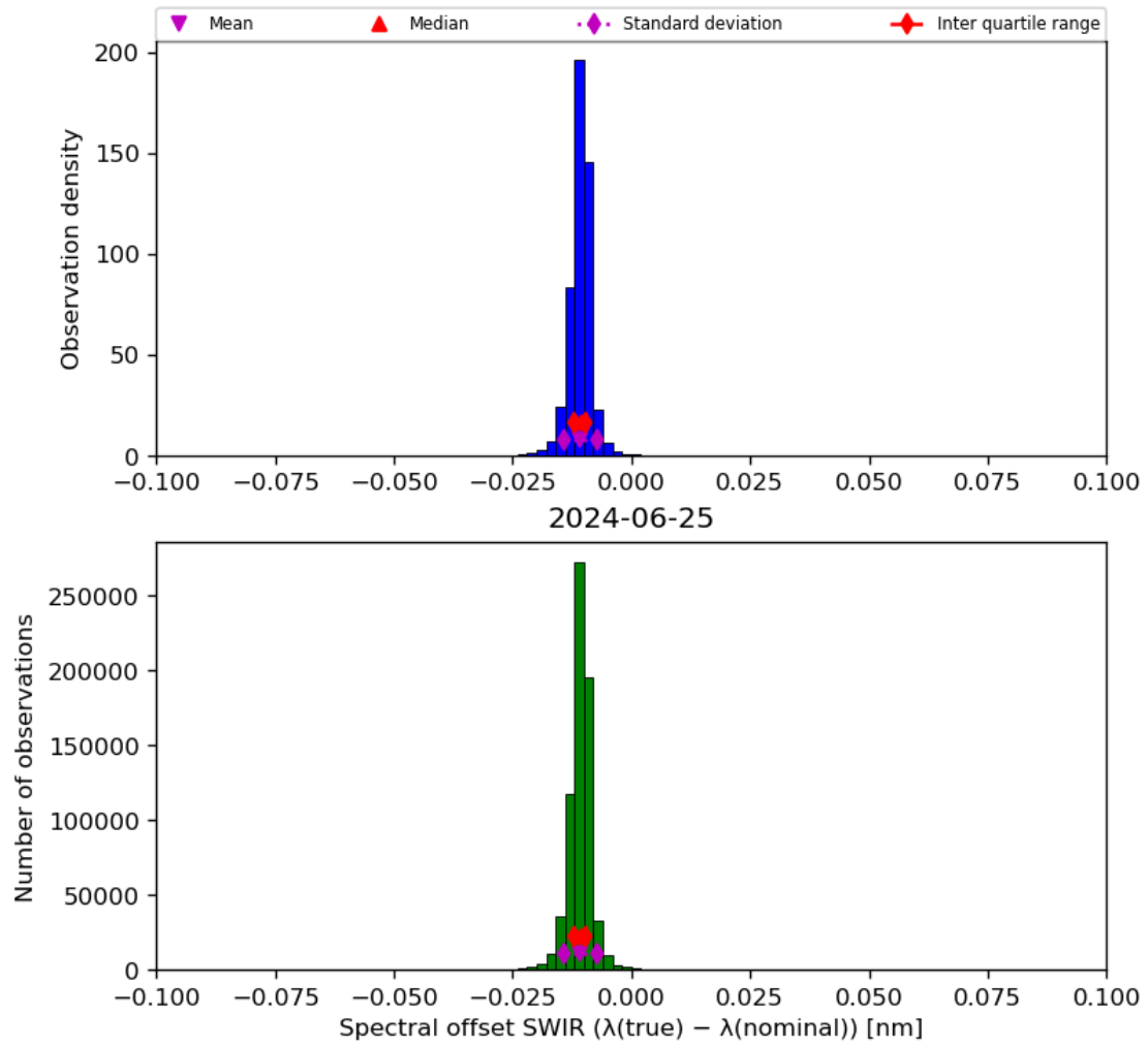
Figure 27: Histogram of “Spectral offset SWIR ( \lambda(\text{true}) - \lambda(\text{nominal}) )” for 2024-06-24 to 2024-06-26
