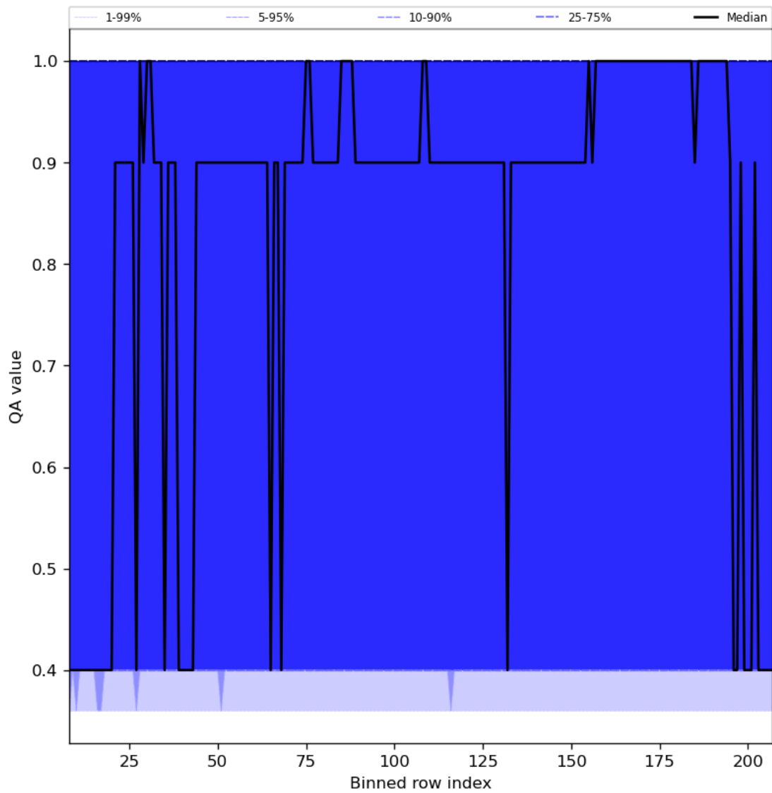
Figure 33: Along track statistics of “QA value” for 2024-06-24 to 2024-06-26
