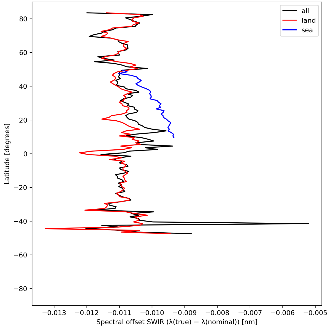
Figure 16: Zonal average of “Spectral offset SWIR ( \lambda(\text{true}) - \lambda(\text{nominal}) )” for 2024-06-24 to 2024-06-26.
