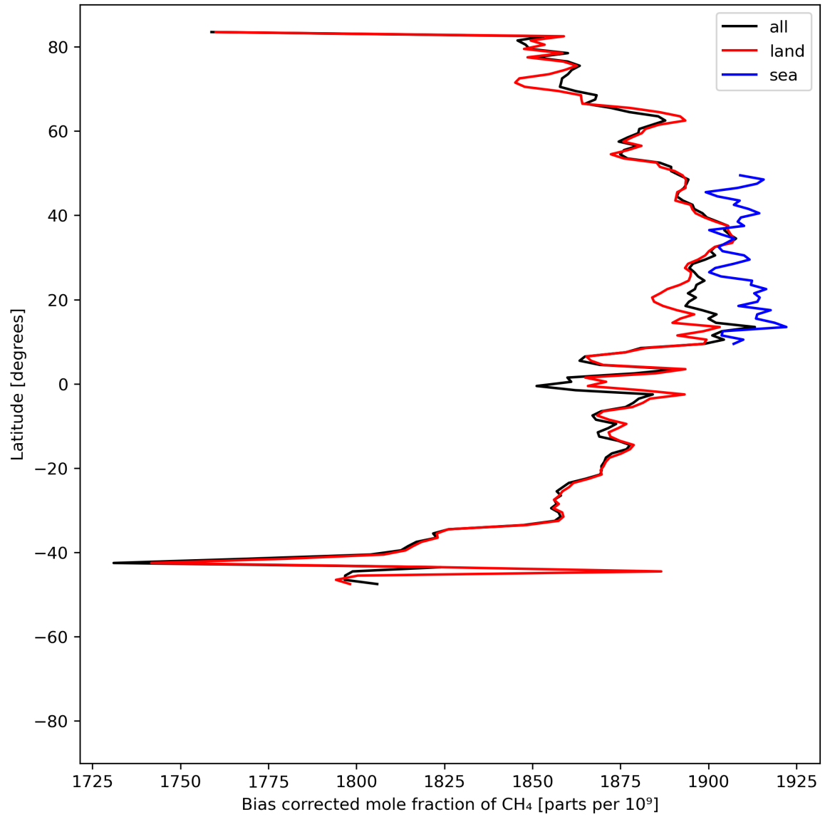
Figure 14: Zonal average of “Bias corrected mole fraction of \text{CH}_4 ” for 2024-06-24 to 2024-06-26.
