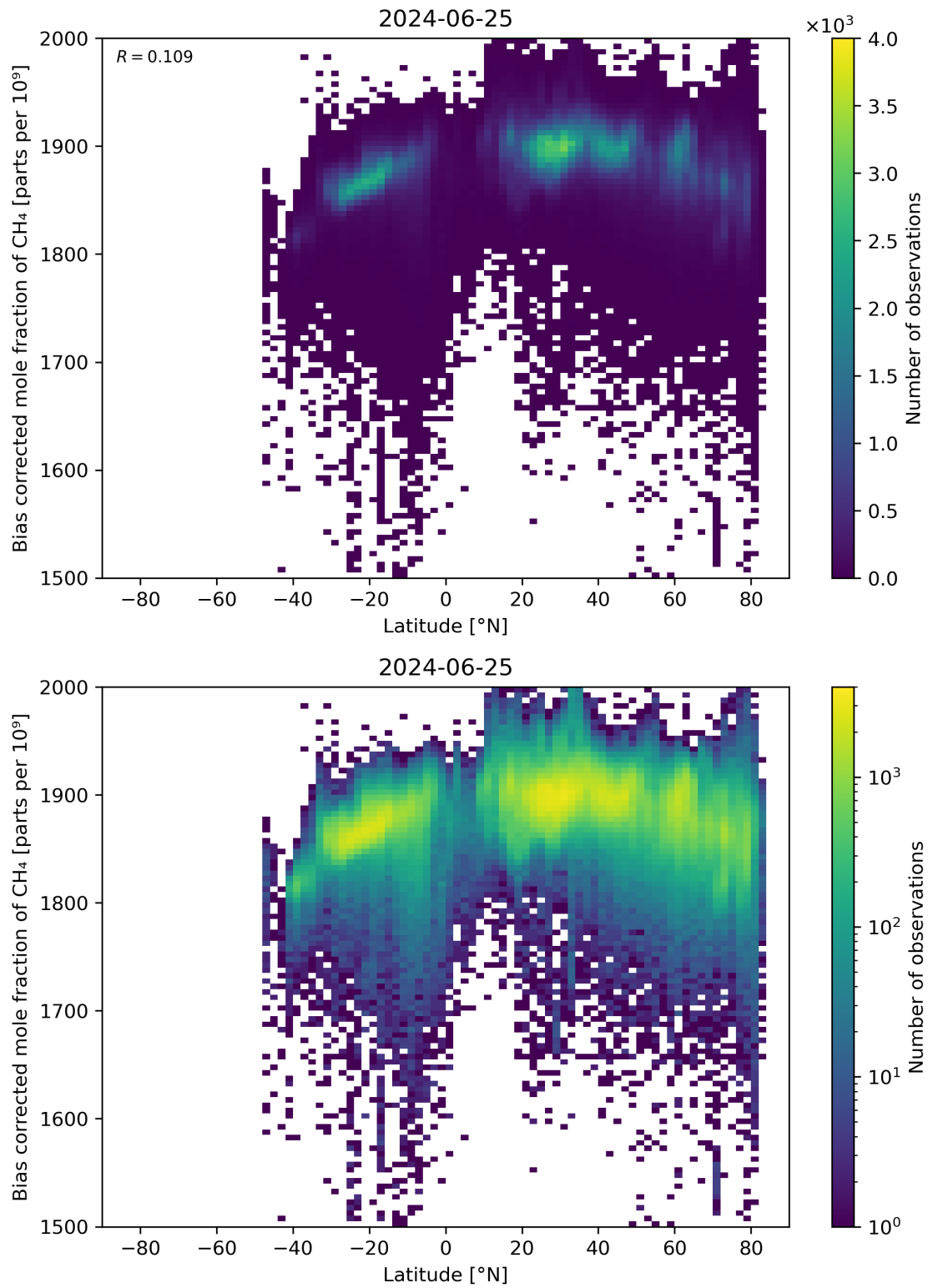
Figure 58: Scatter density plot of “Latitude” against “Bias corrected mole fraction of \text{CH}_4 ” for 2024-06-24 to 2024-06-26.
