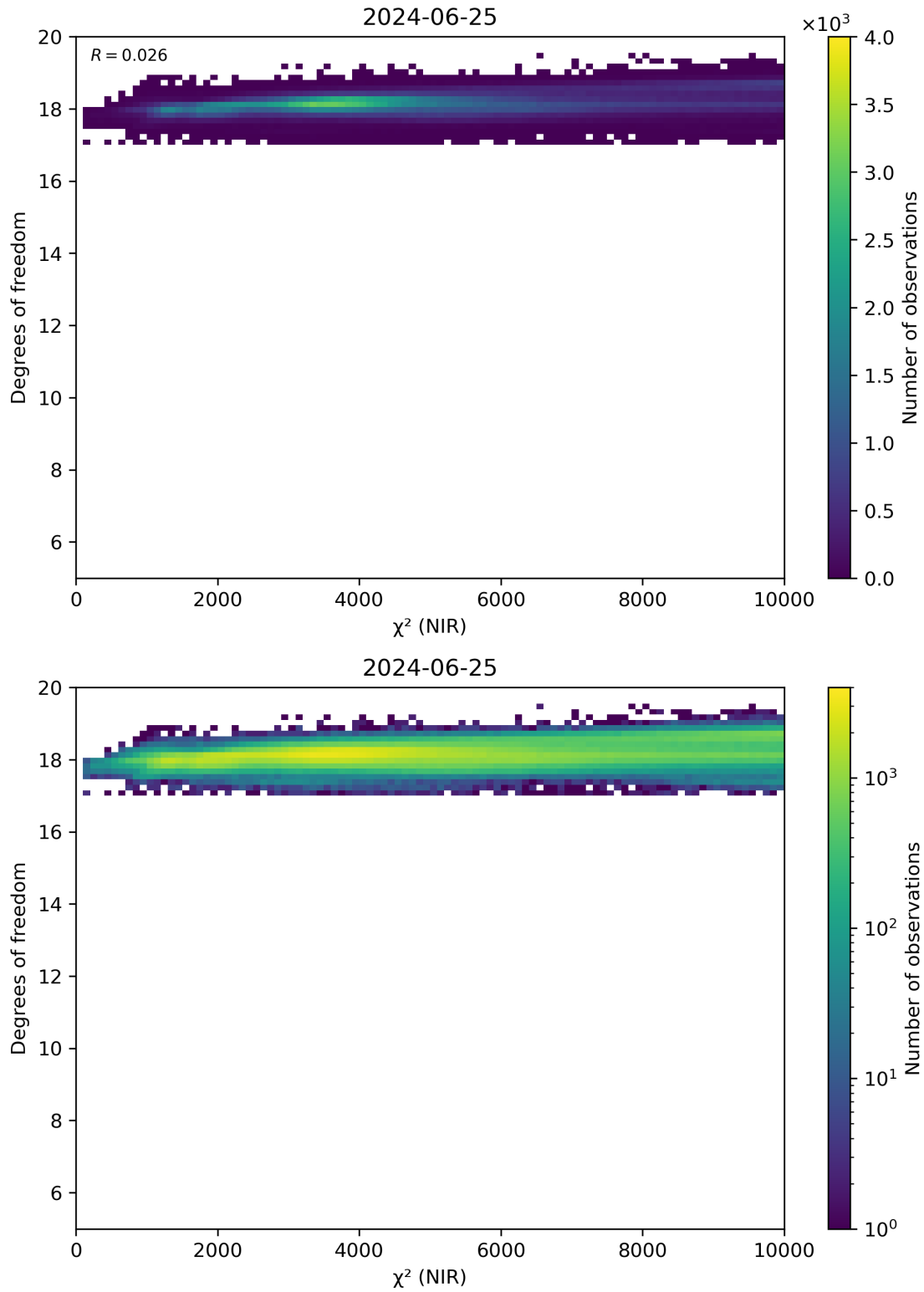
Figure 44: Scatter density plot of “ \chi^2 (NIR)” against “Degrees of freedom” for 2024-06-24 to 2024-06-26.
