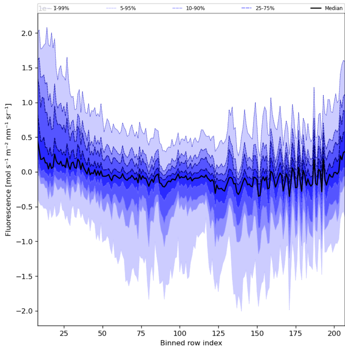
Figure 43: Along track statistics of “Fluorescence” for 2024-06-24 to 2024-06-26
