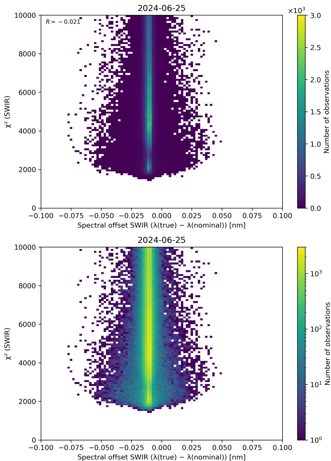
Figure 118: Scatter density plot of “Spectral offset SWIR ( \lambda(\text{true}) - \lambda(\text{nominal}) )” against “ \chi^2 (SWIR)” for 2024-06-24 to 2024-06-26.
