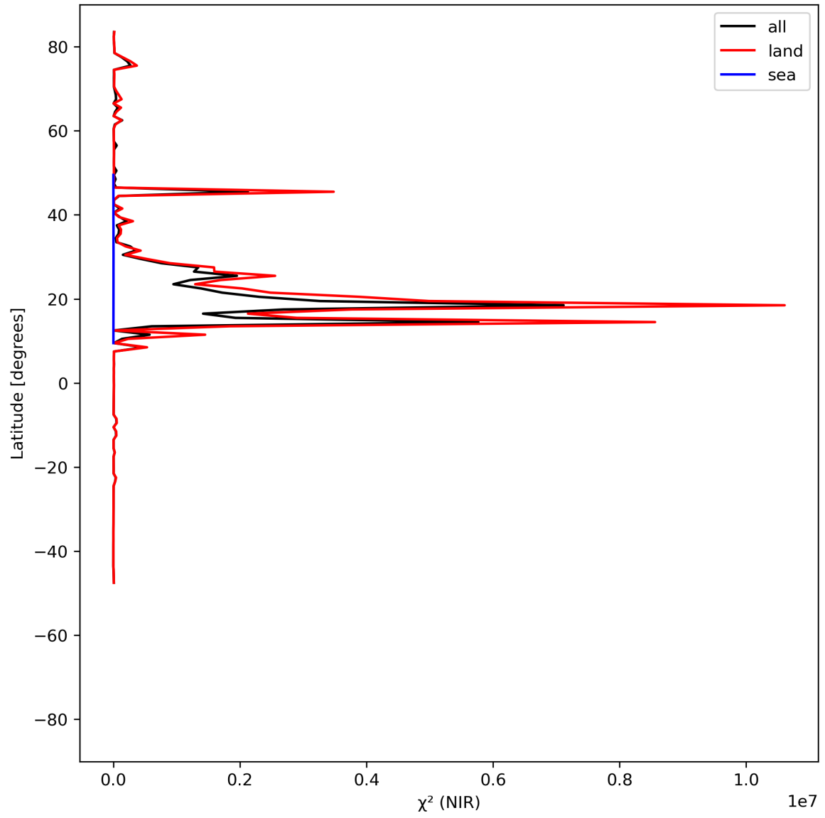
Figure 18: Zonal average of “ \chi^2 (NIR)” for 2024-06-24 to 2024-06-26.
