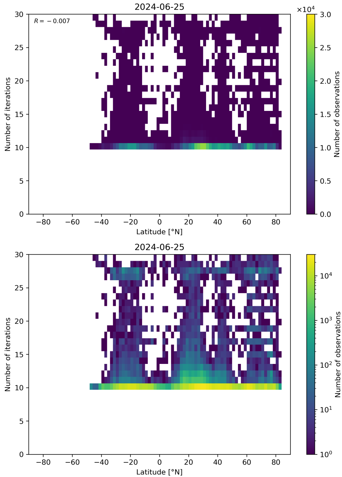
Figure 60: Scatter density plot of “Latitude” against “Number of iterations” for 2024-06-24 to 2024-06-26.
