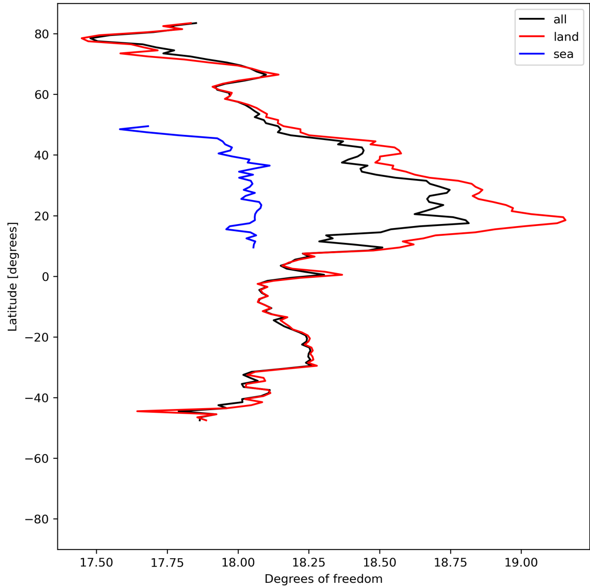
Figure 19: Zonal average of “Degrees of freedom” for 2024-06-24 to 2024-06-26.
