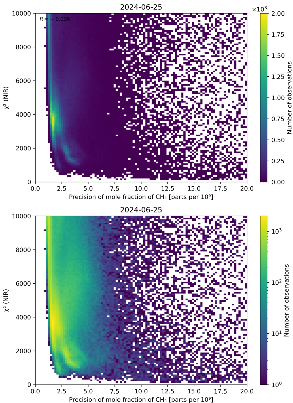
Figure 78: Scatter density plot of “Precision of mole fraction of CH 4 ” against “ \chi^2 (NIR)” for 2024-06-24 to 2024-06-26.
