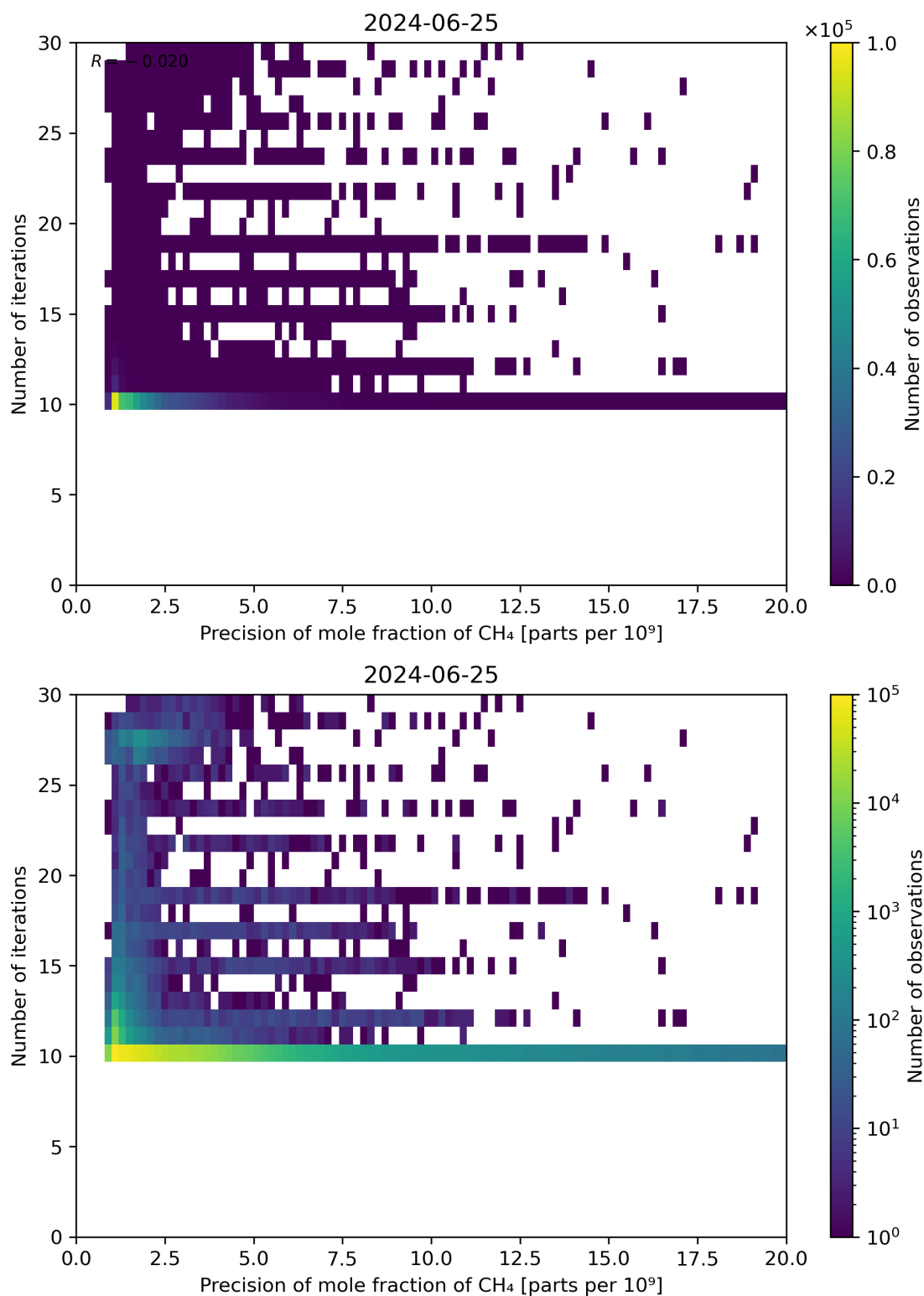
Figure 83: Scatter density plot of “Precision of mole fraction of CH 4 ” against “Number of iterations” for 2024-06-24 to 2024-06-26.
