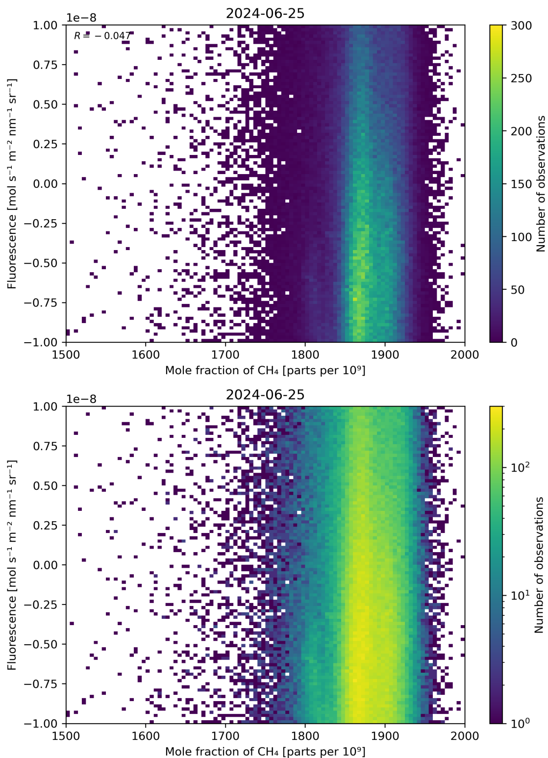
Figure 73: Scatter density plot of “Mole fraction of \text{CH}_4 ” against “Fluorescence” for 2024-06-24 to 2024-06-26.
