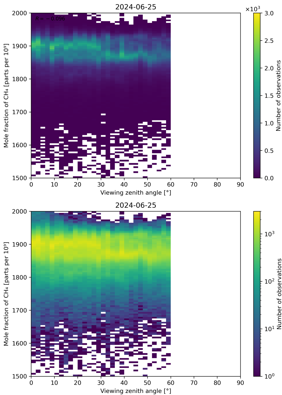
Figure 110: Scatter density plot of “Viewing zenith angle” against “Mole fraction of CH 4 ” for 2024-06-24 to 2024-06-26.
