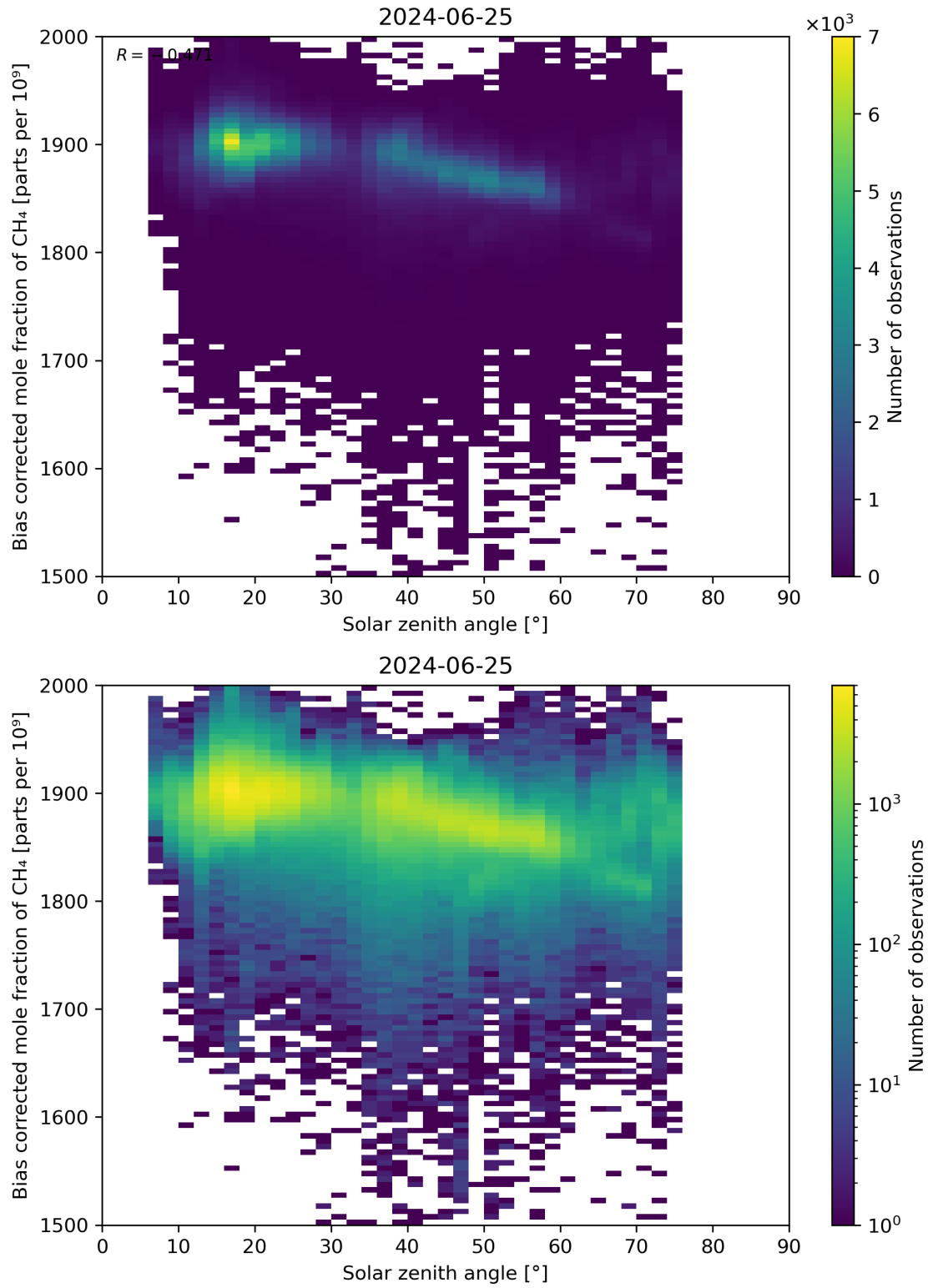
Figure 100: Scatter density plot of “Solar zenith angle” against “Bias corrected mole fraction of CH 4 ” for 2024-06-24 to 2024-06-26.
