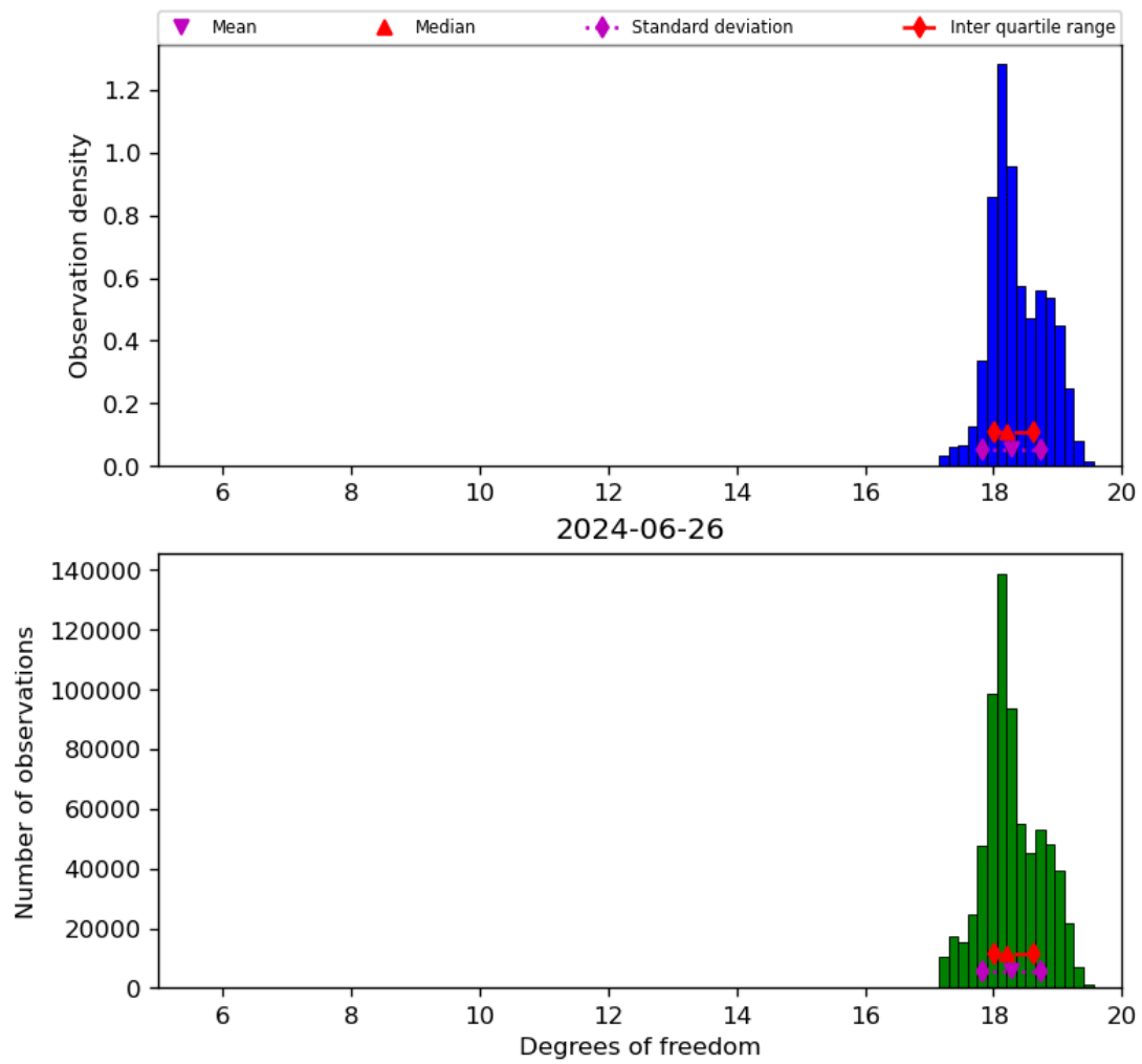
Figure 30: Histogram of “Degrees of freedom” for 2024-06-25 to 2024-06-27
