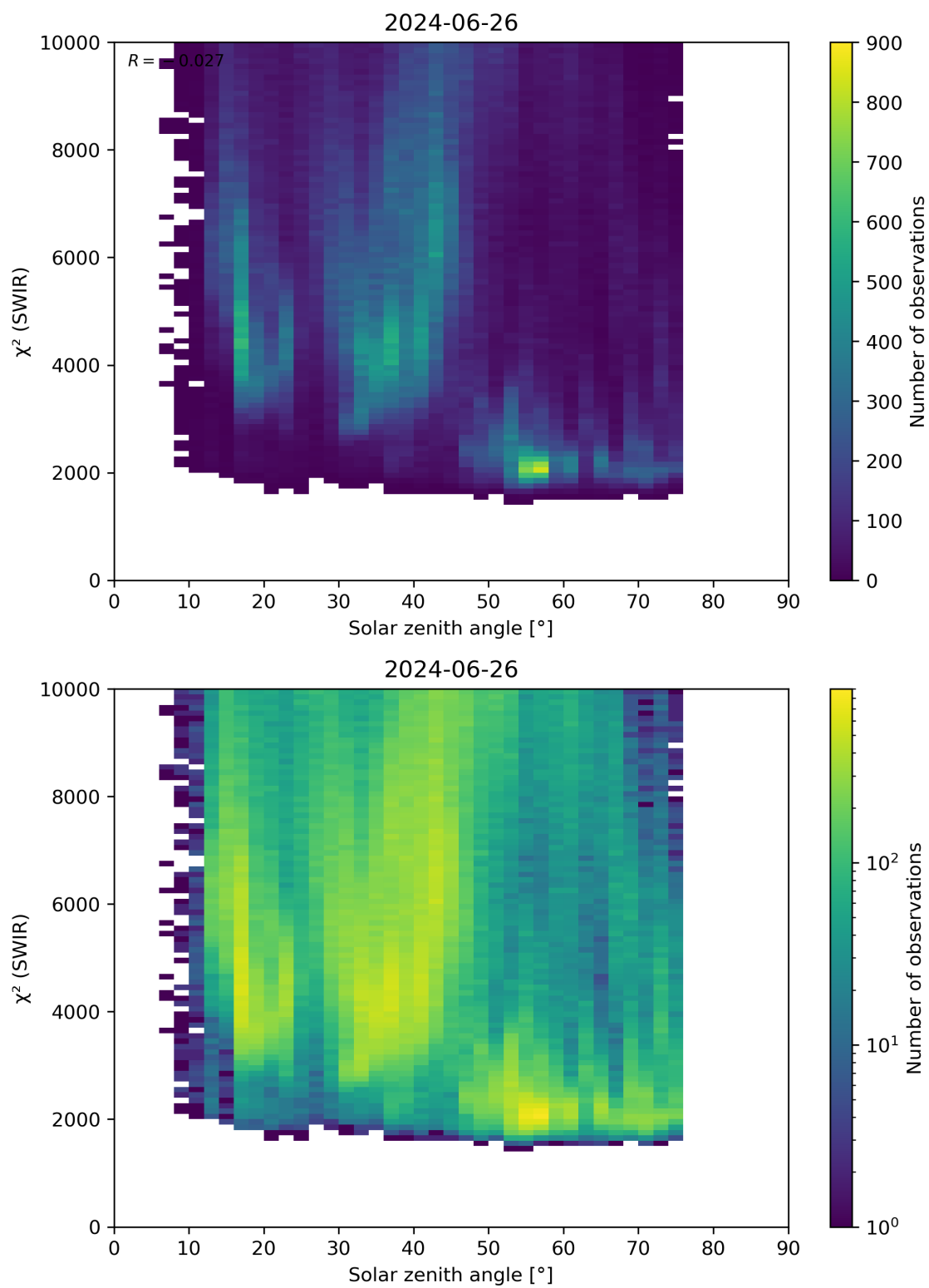
Figure 95: Scatter density plot of “Solar zenith angle” against “ \chi^2 (SWIR)” for 2024-06-25 to 2024-06-27.
