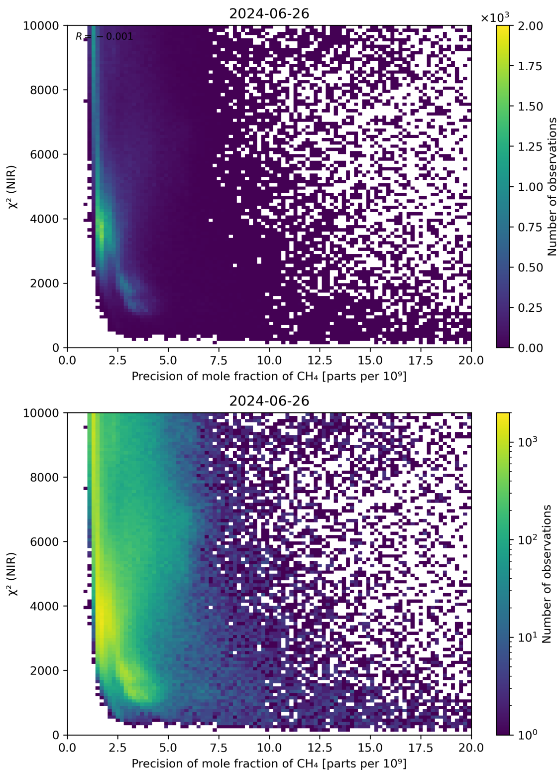
Figure 78: Scatter density plot of “Precision of mole fraction of CH 4 ” against “ \chi^2 (NIR)” for 2024-06-25 to 2024-06-27.
