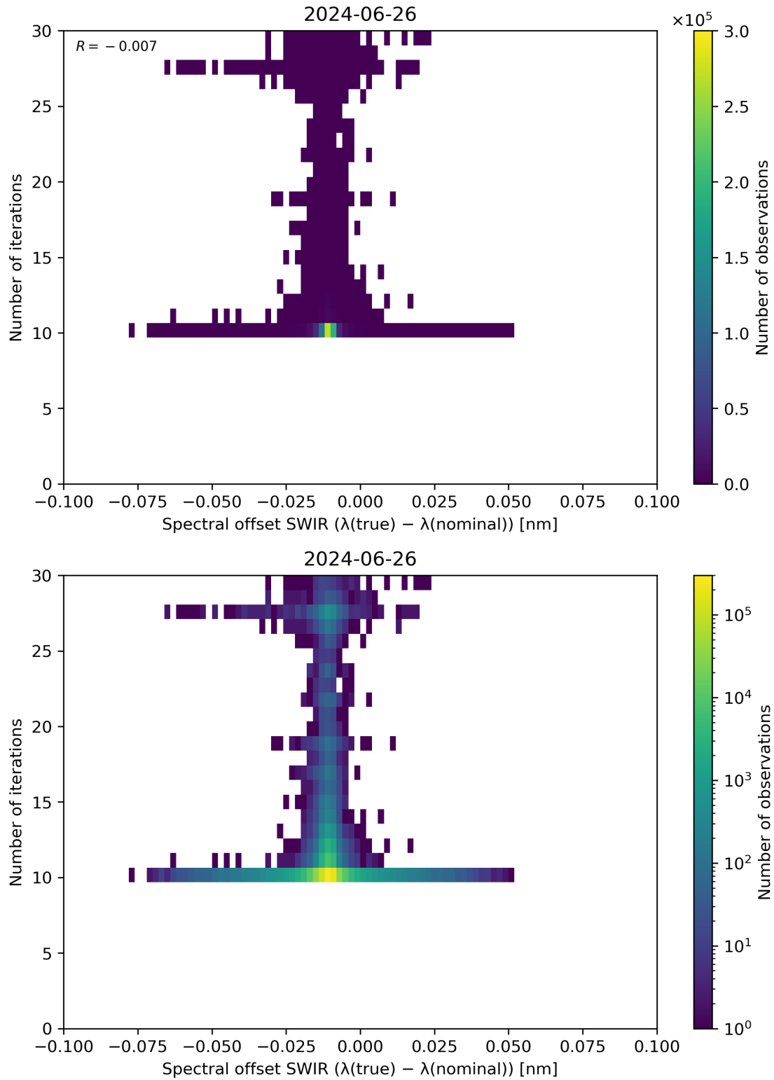
Figure 121: Scatter density plot of “Spectral offset SWIR ( \lambda(\text{true}) - \lambda(\text{nominal}) )” against “Number of iterations” for 2024-06-25 to 2024-06-27.
