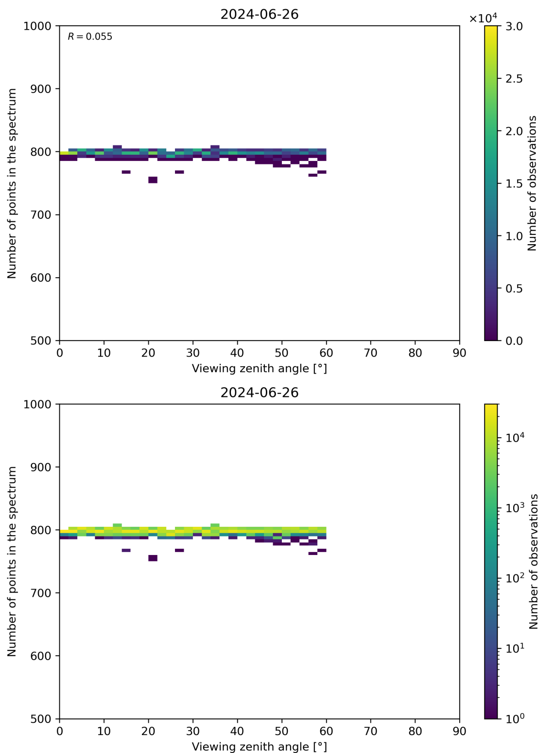
Figure 114: Scatter density plot of “Viewing zenith angle” against “Number of points in the spectrum” for 2024-06-25 to 2024-06-27.
