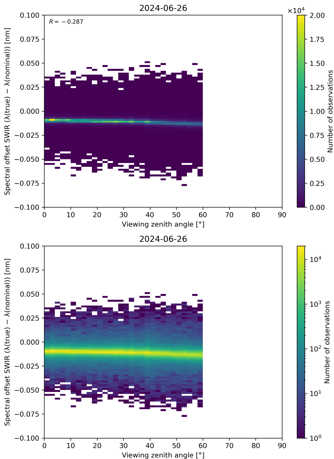
Figure 116: Scatter density plot of “Viewing zenith angle” against “Spectral offset SWIR ( \lambda(\text{true}) - \lambda(\text{nominal}) )” for 2024-06-25 to 2024-06-27.
