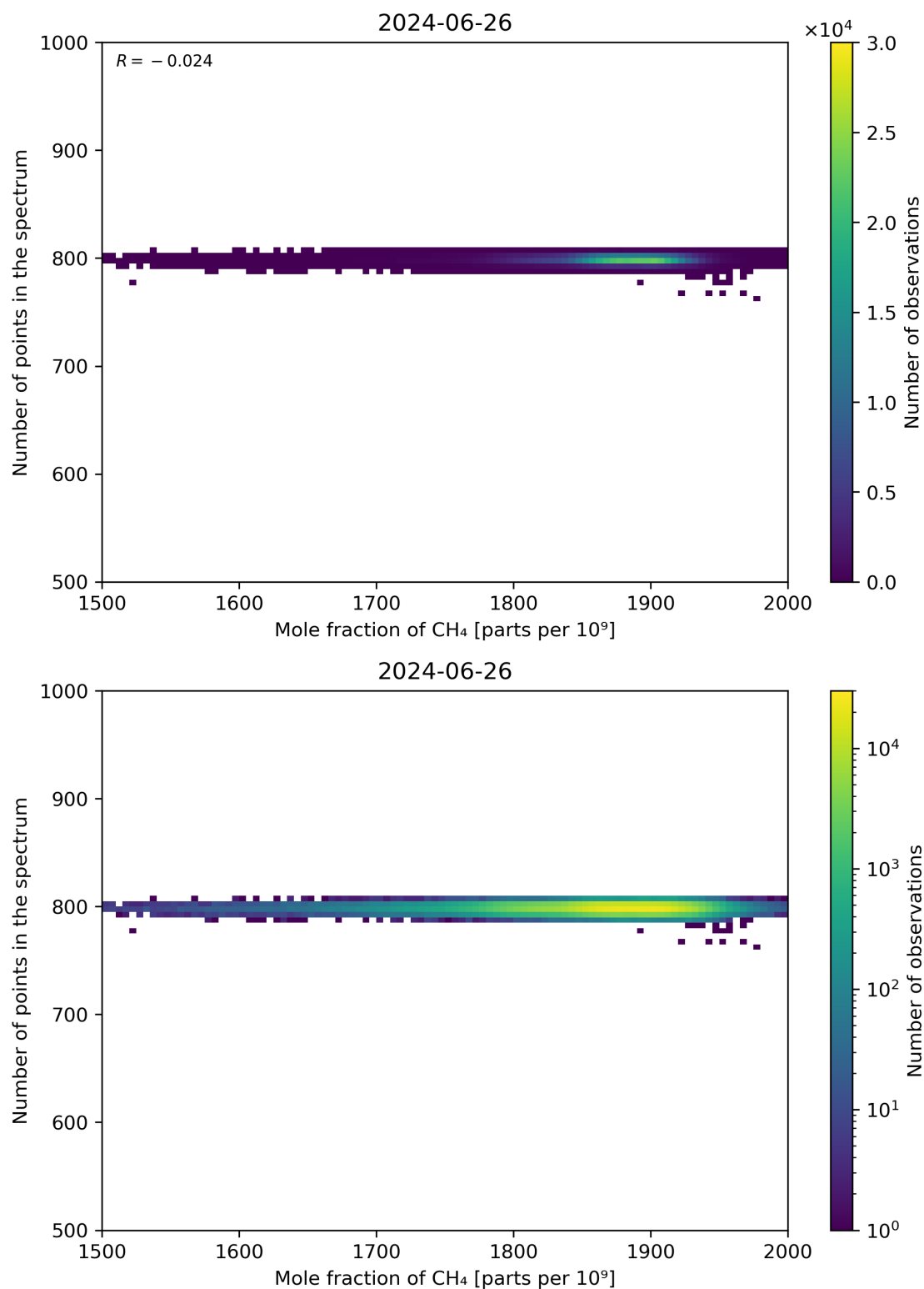
Figure 77: Scatter density plot of “Mole fraction of CH 4 ” against “Number of points in the spectrum” for 2024-06-25 to 2024-06-27.
