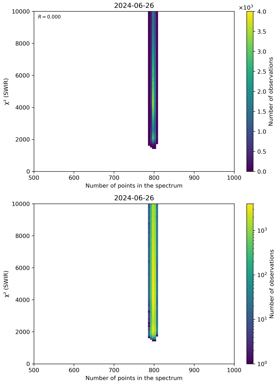
Figure 89: Scatter density plot of “Number of points in the spectrum” against “ \chi^2 (SWIR)” for 2024-06-25 to 2024-06-27.
