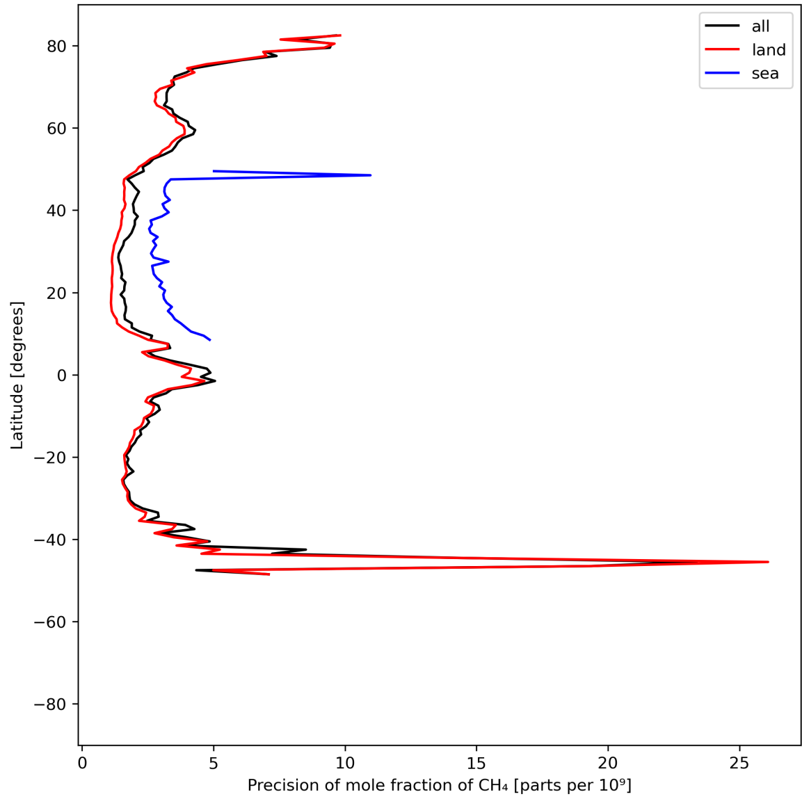
Figure 13: Zonal average of “Precision of mole fraction of CH 4 ” for 2024-06-25 to 2024-06-27.
