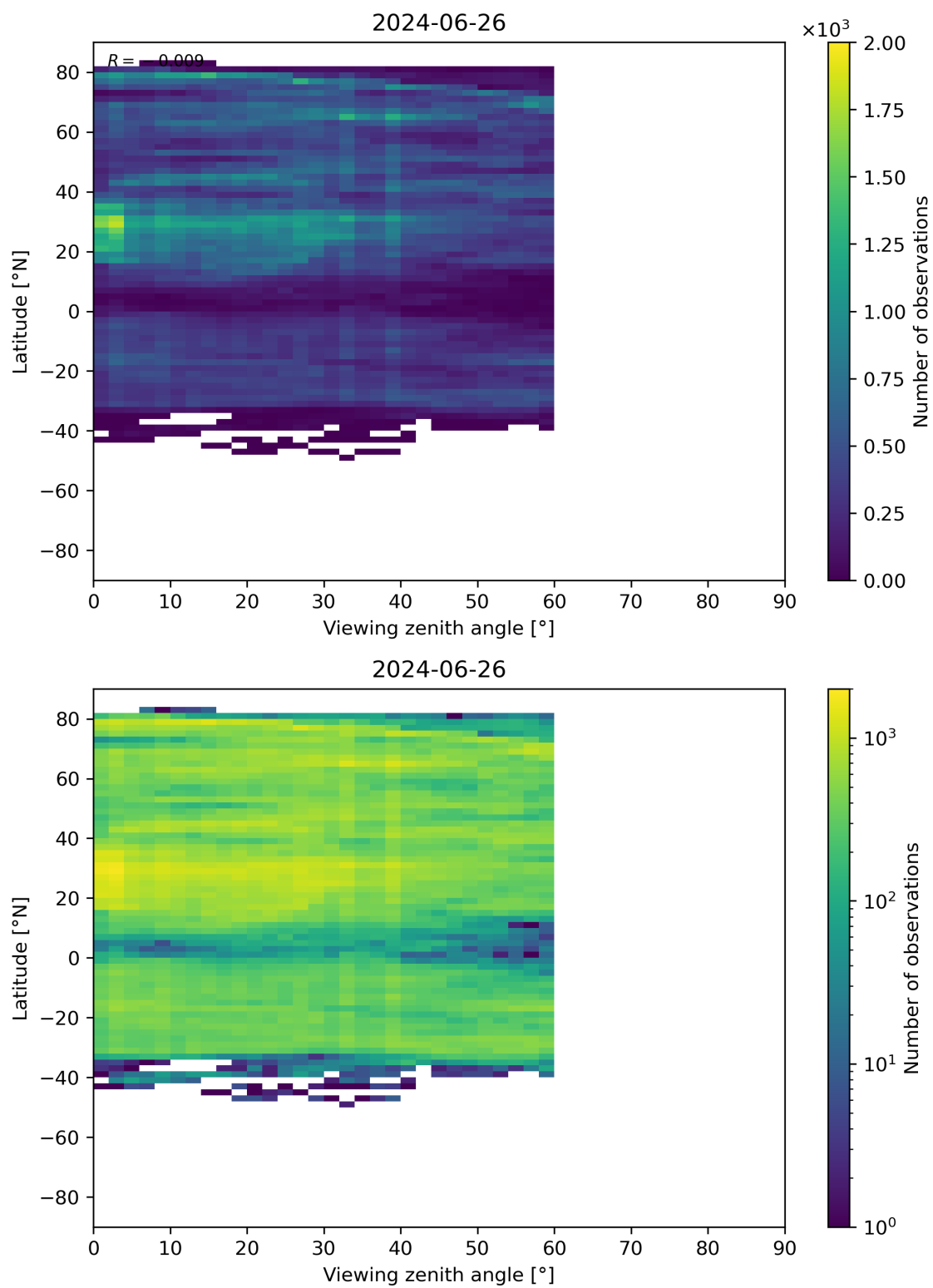
Figure 109: Scatter density plot of “Viewing zenith angle” against “Latitude” for 2024-06-25 to 2024-06-27.
