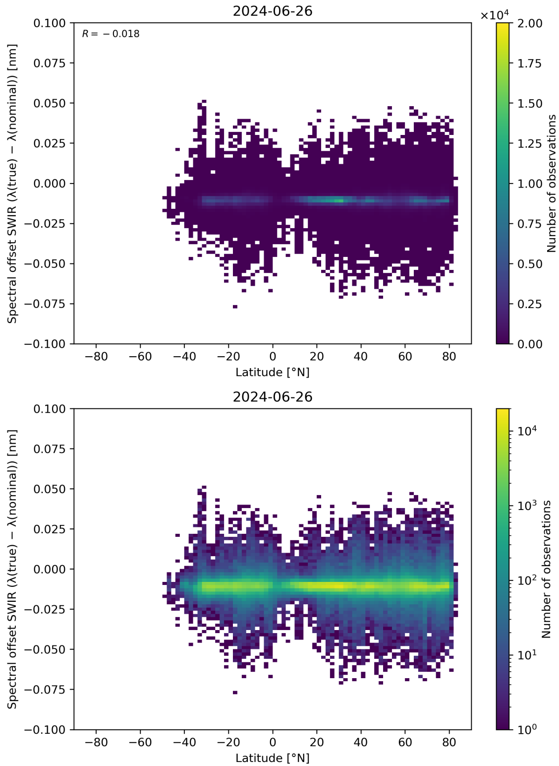
Figure 62: Scatter density plot of “Latitude” against “Spectral offset SWIR ( \lambda(\text{true}) - \lambda(\text{nominal}) )” for 2024-06-25 to 2024-06-27.
