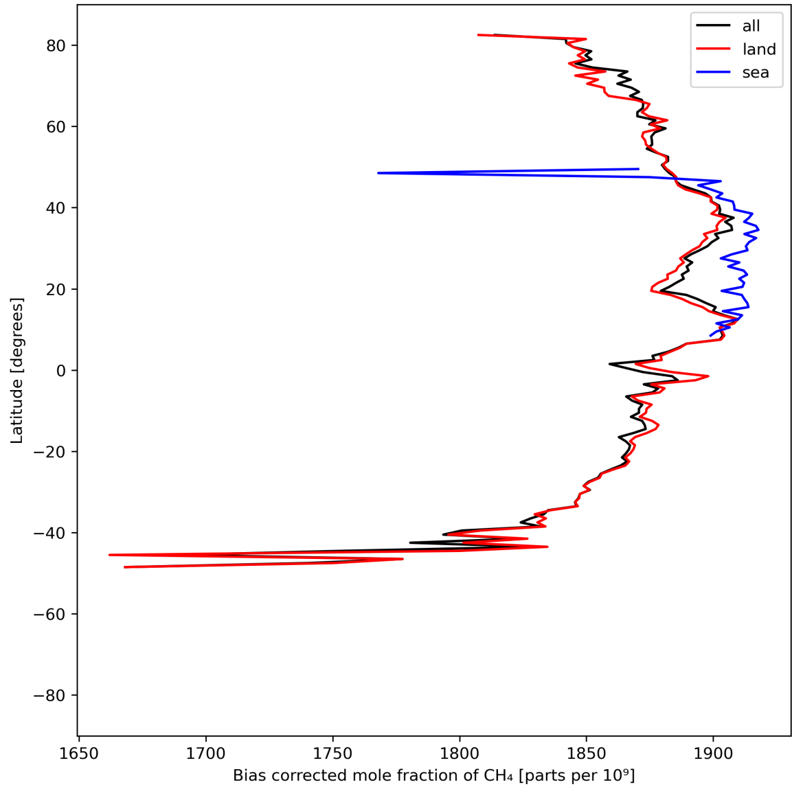
Figure 14: Zonal average of “Bias corrected mole fraction of \text{CH}_4 ” for 2024-06-25 to 2024-06-27.
