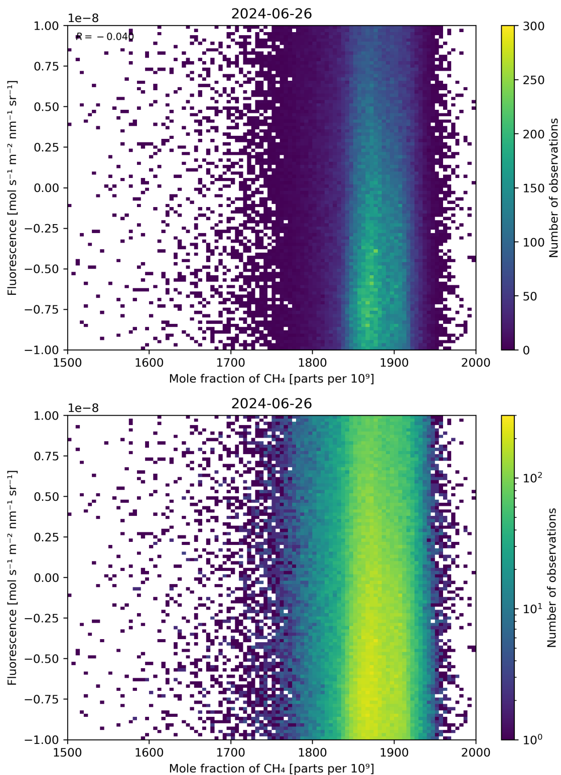
Figure 73: Scatter density plot of “Mole fraction of \text{CH}_4 ” against “Fluorescence” for 2024-06-25 to 2024-06-27.
