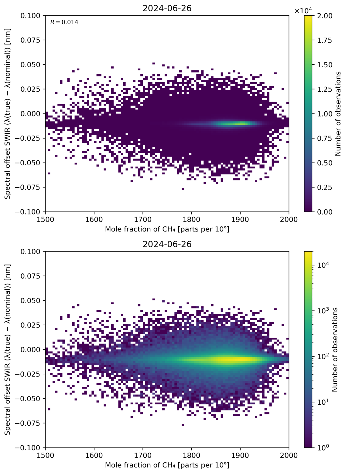
Figure 86: Scatter density plot of “Mole fraction of CH 4 ” against “Spectral offset SWIR ( \lambda(\text{true}) - \lambda(\text{nominal}) )” for 2024-06-25 to 2024-06-27.
