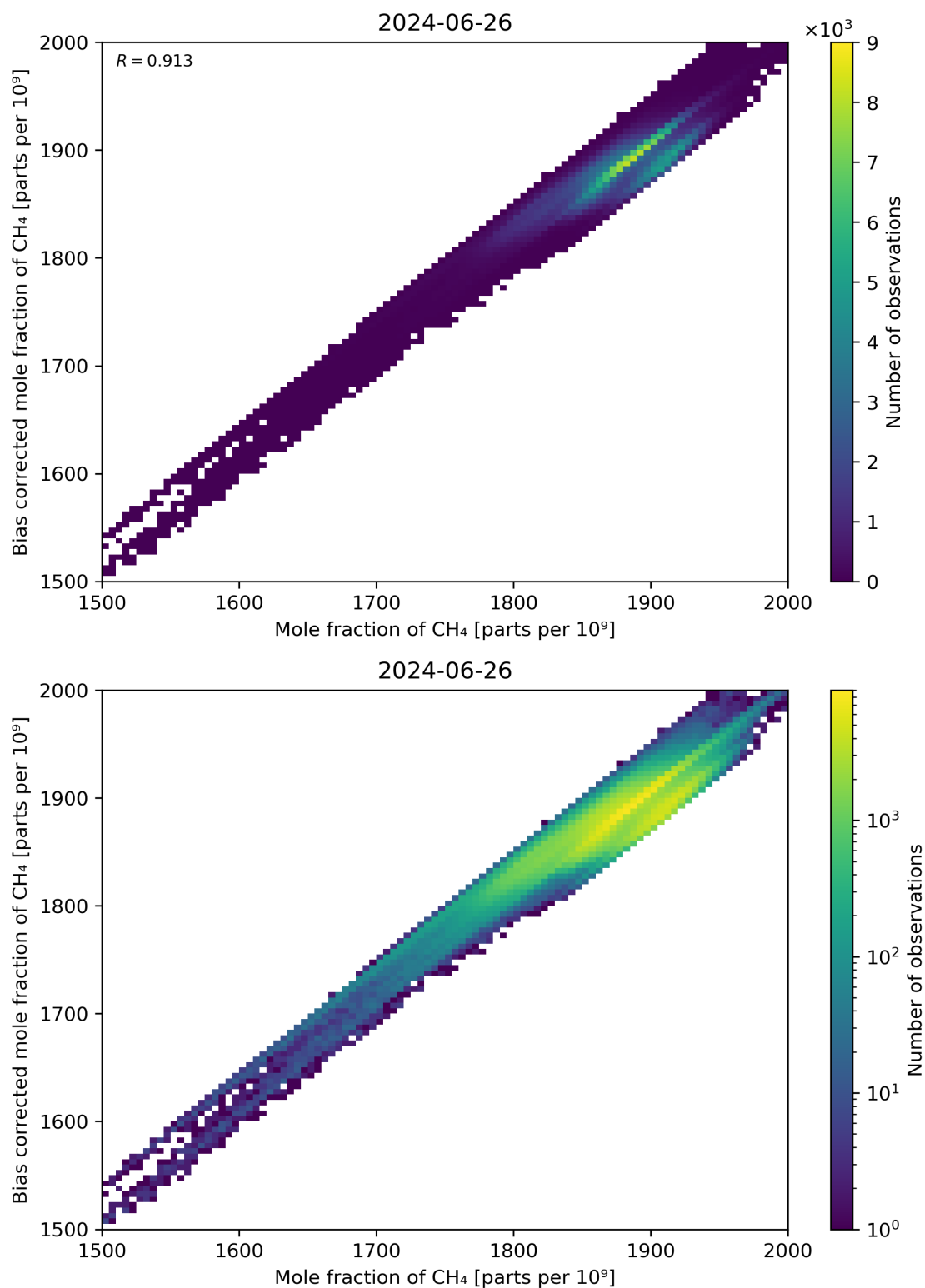
Figure 74: Scatter density plot of “Mole fraction of CH 4 ” against “Bias corrected mole fraction of CH 4 ” for 2024-06-25 to 2024-06-27.
