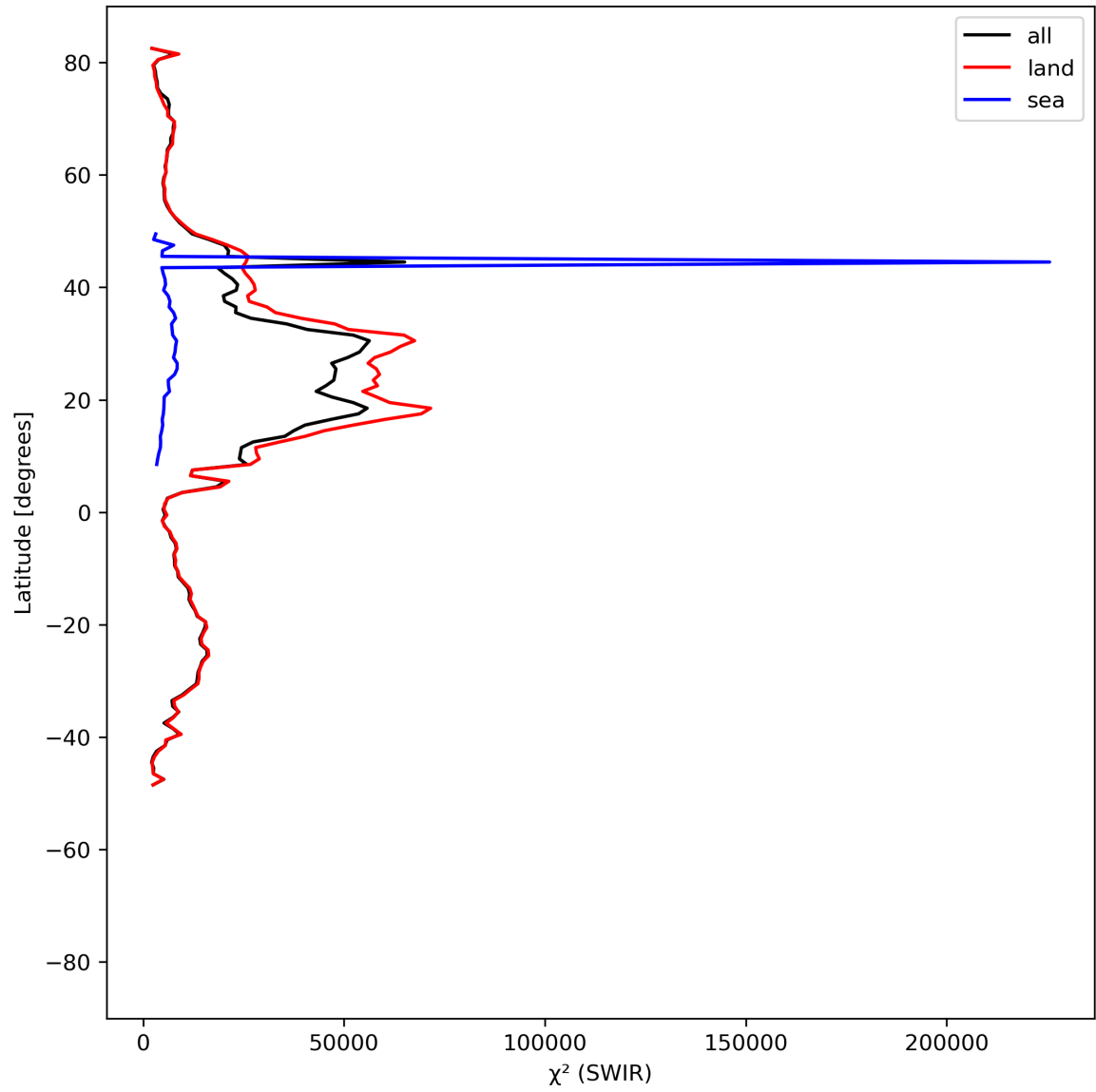
Figure 17: Zonal average of “ \chi^2 (SWIR)” for 2024-06-25 to 2024-06-27.
