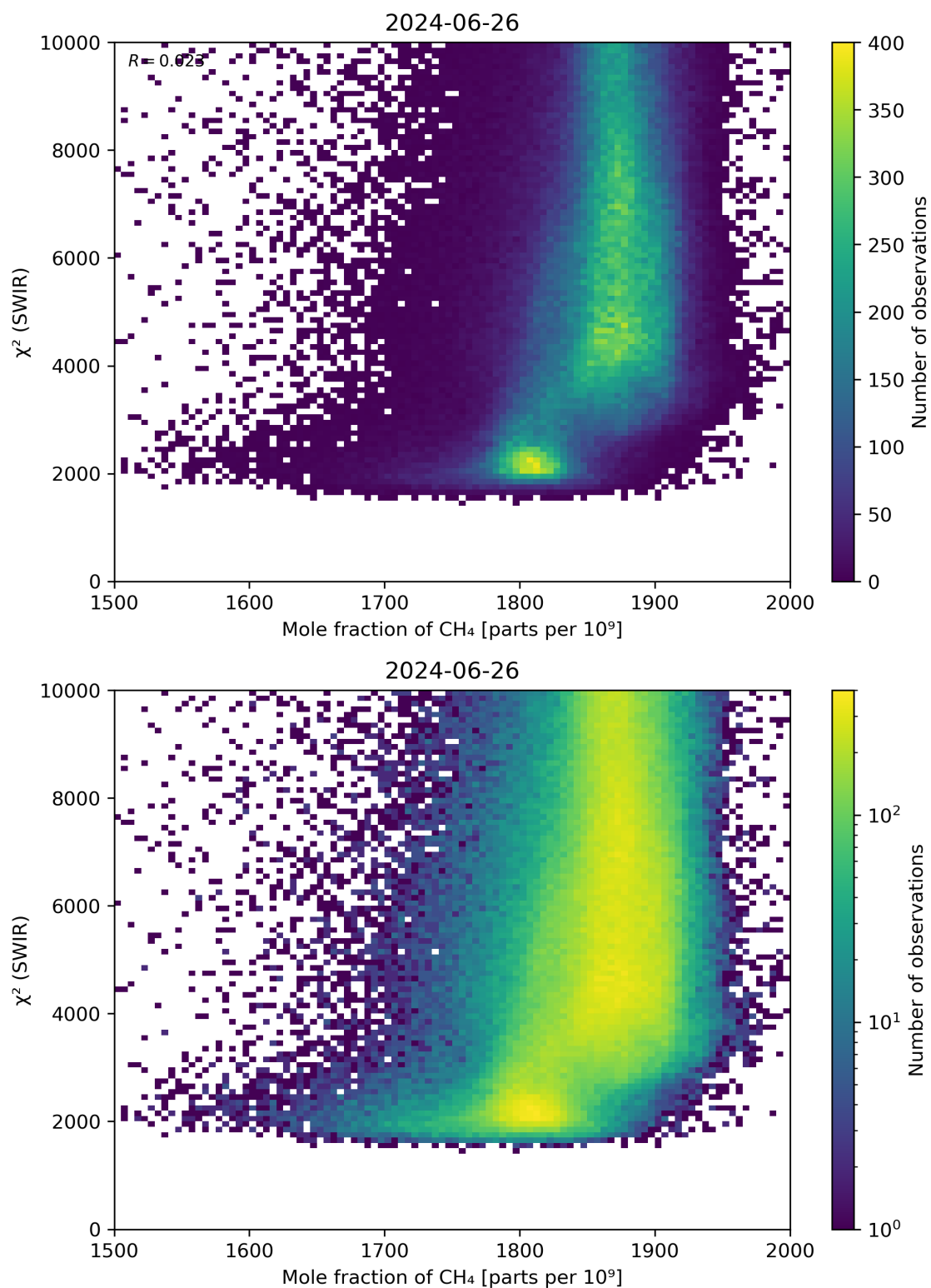
Figure 71: Scatter density plot of “Mole fraction of \text{CH}_4 ” against “ \chi^2 (SWIR)” for 2024-06-25 to 2024-06-27.
