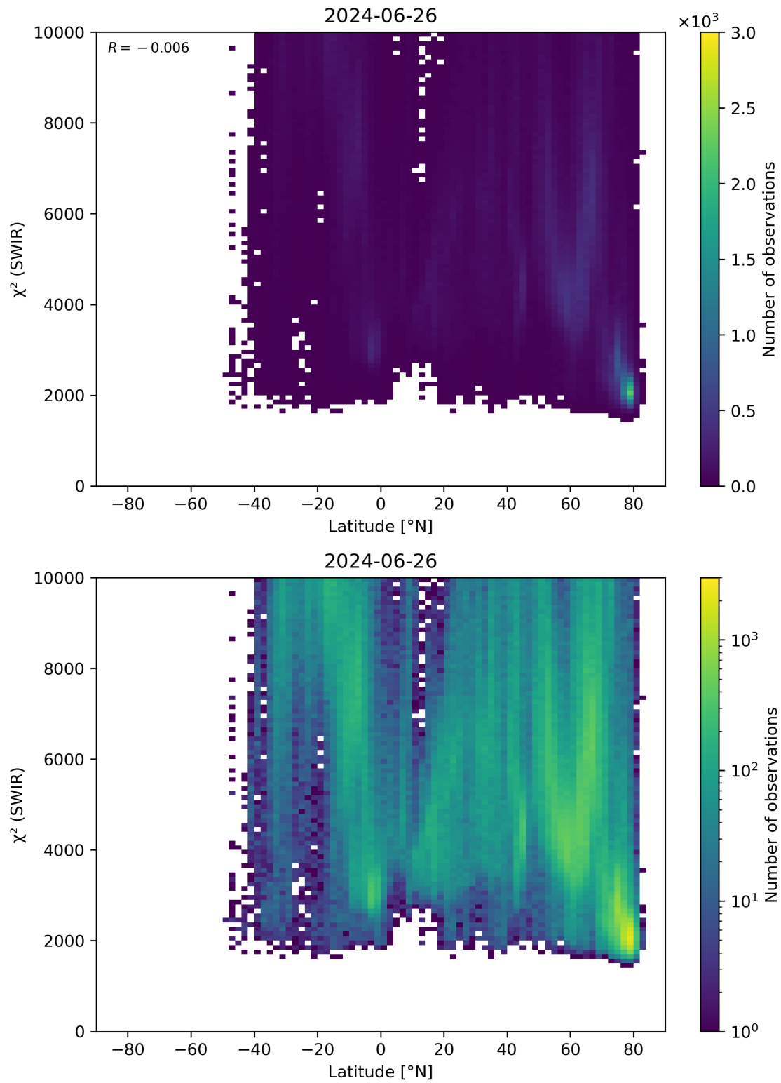
Figure 54: Scatter density plot of “Latitude” against “ \chi^2 (SWIR)” for 2024-06-25 to 2024-06-27.
