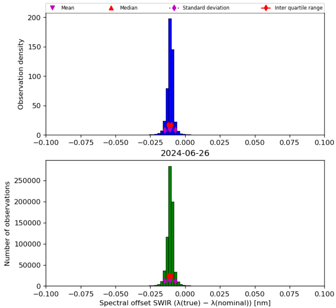
Figure 27: Histogram of “Spectral offset SWIR ( \lambda(\text{true}) - \lambda(\text{nominal}) )” for 2024-06-25 to 2024-06-27
