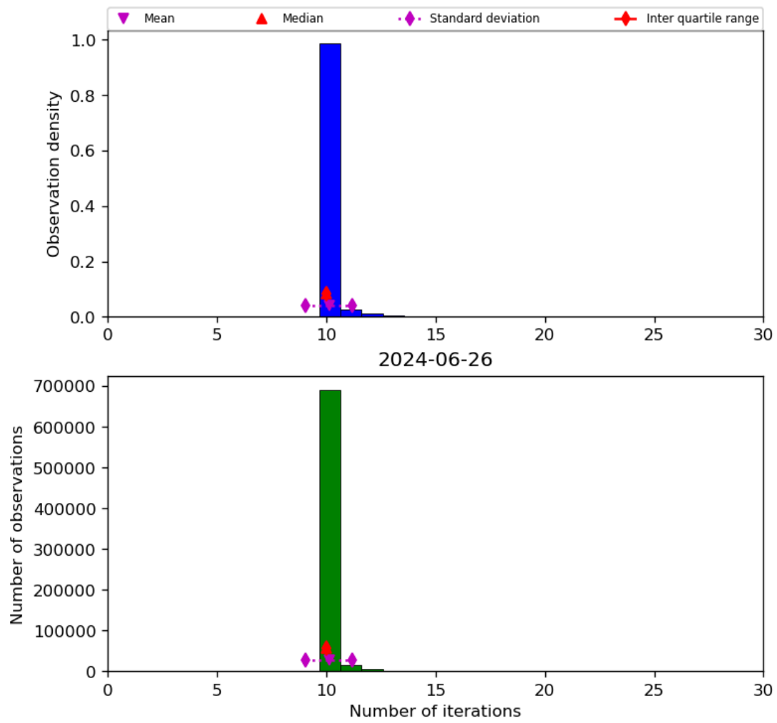
Figure 31: Histogram of “Number of iterations” for 2024-06-25 to 2024-06-27
