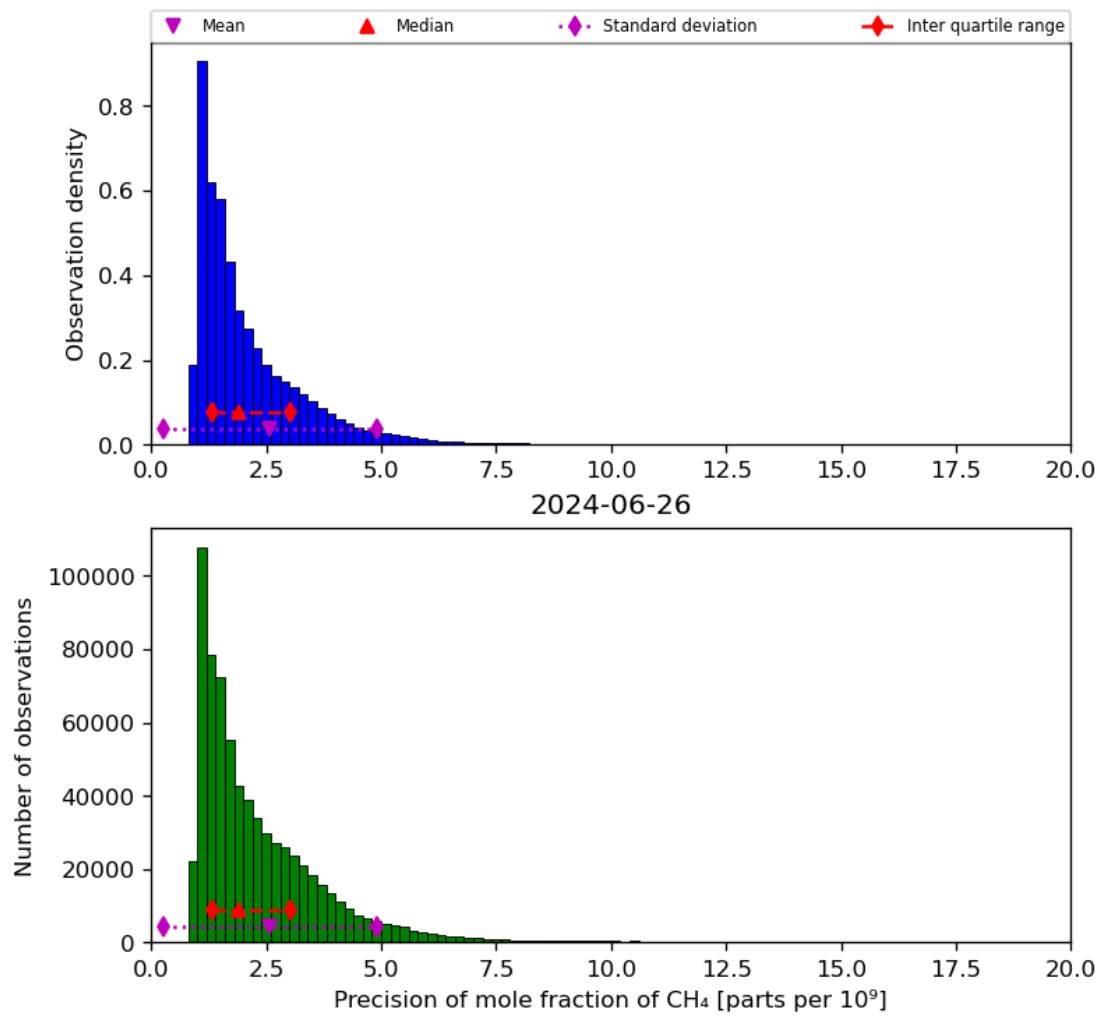
Figure 24: Histogram of “Precision of mole fraction of CH 4 ” for 2024-06-25 to 2024-06-27
