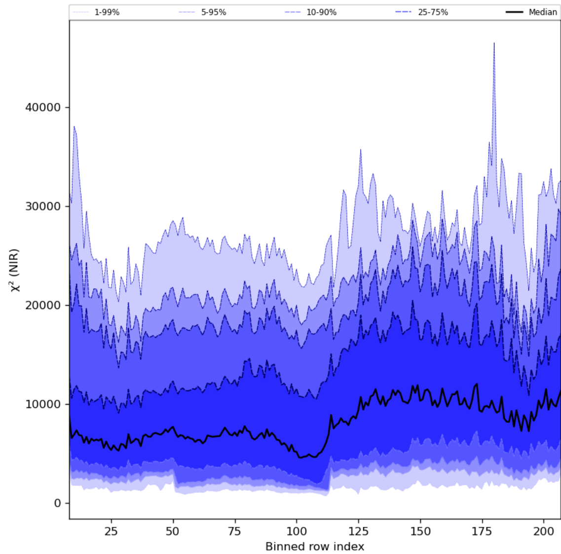
Figure 40: Along track statistics of “ \chi^2 (NIR)” for 2024-06-25 to 2024-06-27
