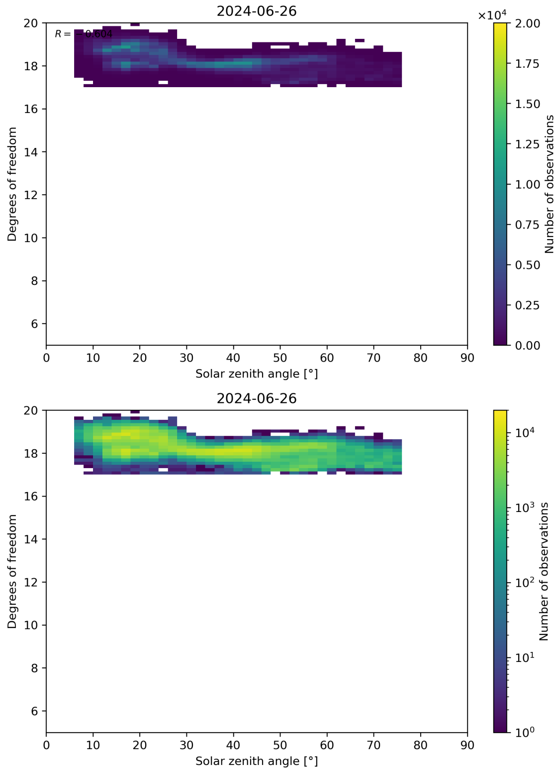
Figure 96: Scatter density plot of “Solar zenith angle” against “Degrees of freedom” for 2024-06-25 to 2024-06-27.
