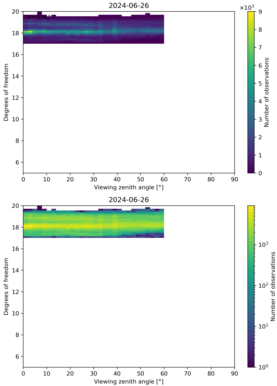
Figure 107: Scatter density plot of “Viewing zenith angle” against “Degrees of freedom” for 2024-06-25 to 2024-06-27.
