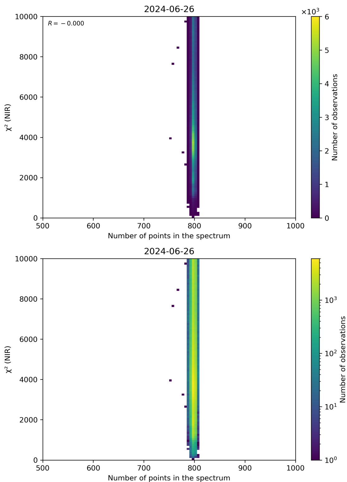
Figure 88: Scatter density plot of “Number of points in the spectrum” against “ \chi^2 (NIR)” for 2024-06-25 to 2024-06-27.
