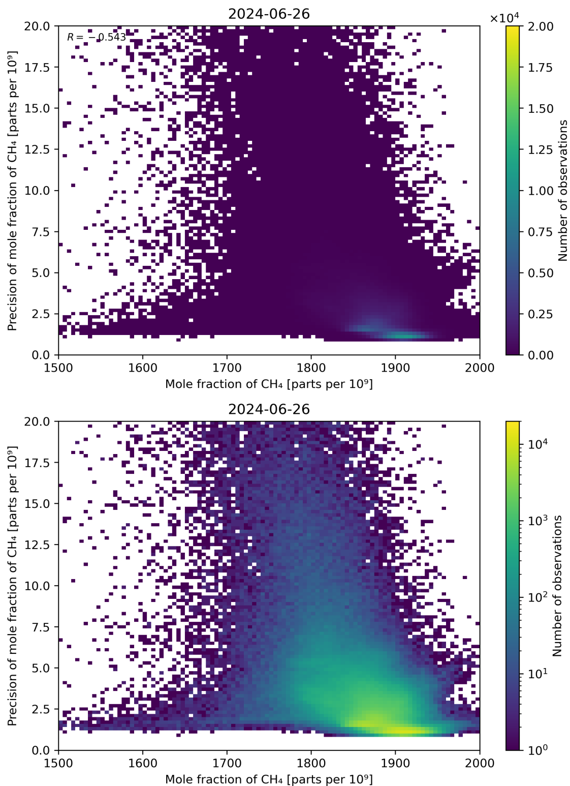
Figure 75: Scatter density plot of “Mole fraction of CH 4 ” against “Precision of mole fraction of CH 4 ” for 2024-06-25 to 2024-06-27.
