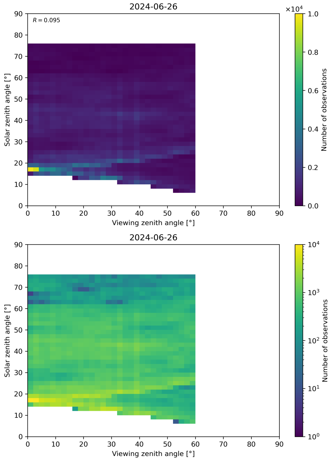
Figure 115: Scatter density plot of “Viewing zenith angle” against “Solar zenith angle” for 2024-06-25 to 2024-06-27.
