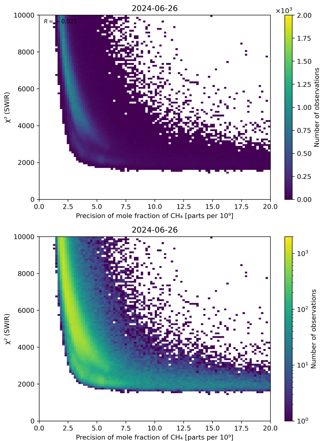
Figure 79: Scatter density plot of “Precision of mole fraction of \text{CH}_4 ” against “ \chi^2 (SWIR)” for 2024-06-25 to 2024-06-27.
