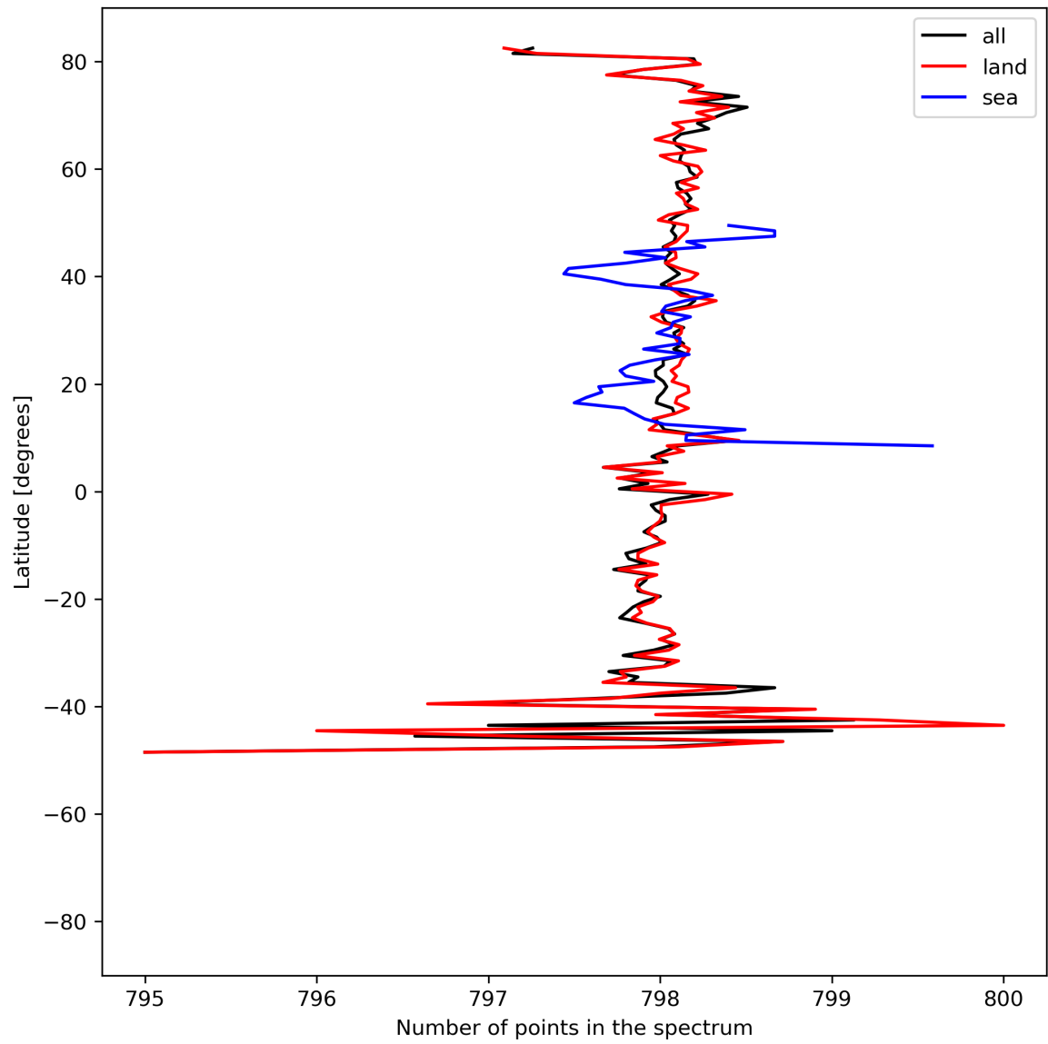
Figure 15: Zonal average of “Number of points in the spectrum” for 2024-06-25 to 2024-06-27.
