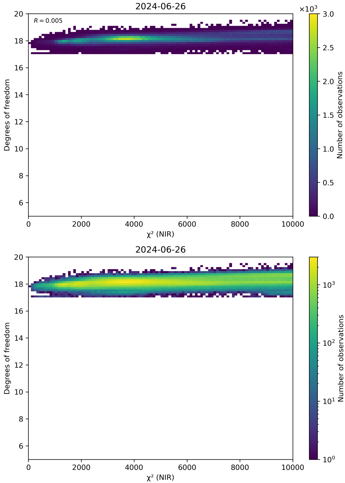
Figure 44: Scatter density plot of “ \chi^2 (NIR)” against “Degrees of freedom” for 2024-06-25 to 2024-06-27.
