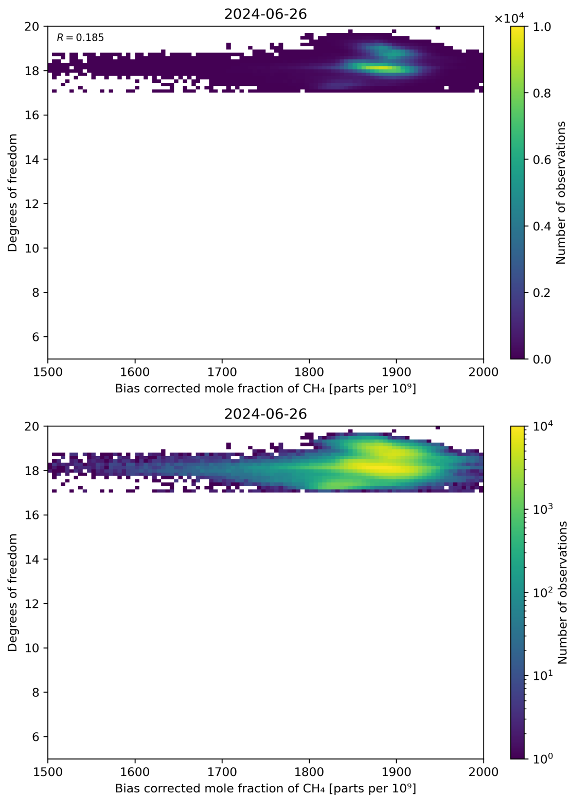
Figure 65: Scatter density plot of “Bias corrected mole fraction of CH 4 ” against “Degrees of freedom” for 2024-06-25 to 2024-06-27.
