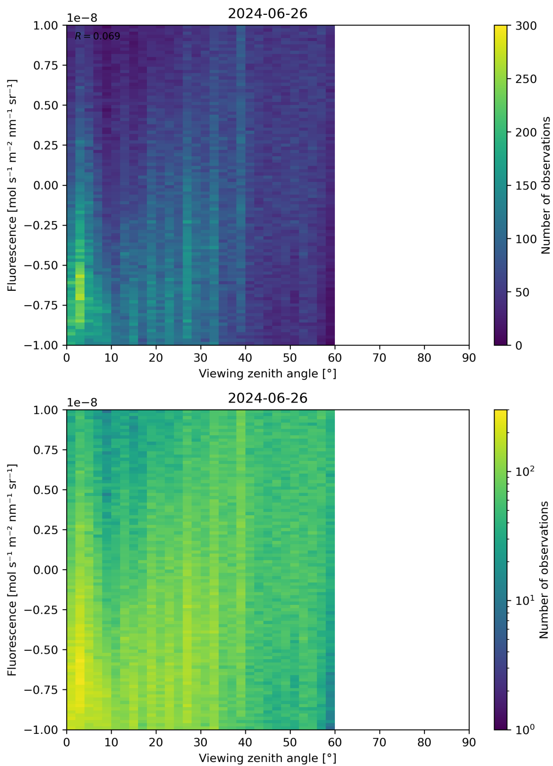
Figure 108: Scatter density plot of “Viewing zenith angle” against “Fluorescence” for 2024-06-25 to 2024-06-27.
