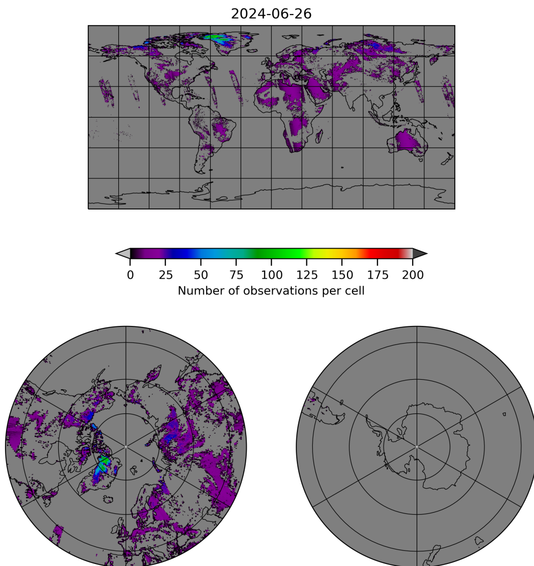
Figure 10: Map of the number of observations for 2024-06-25 to 2024-06-27
