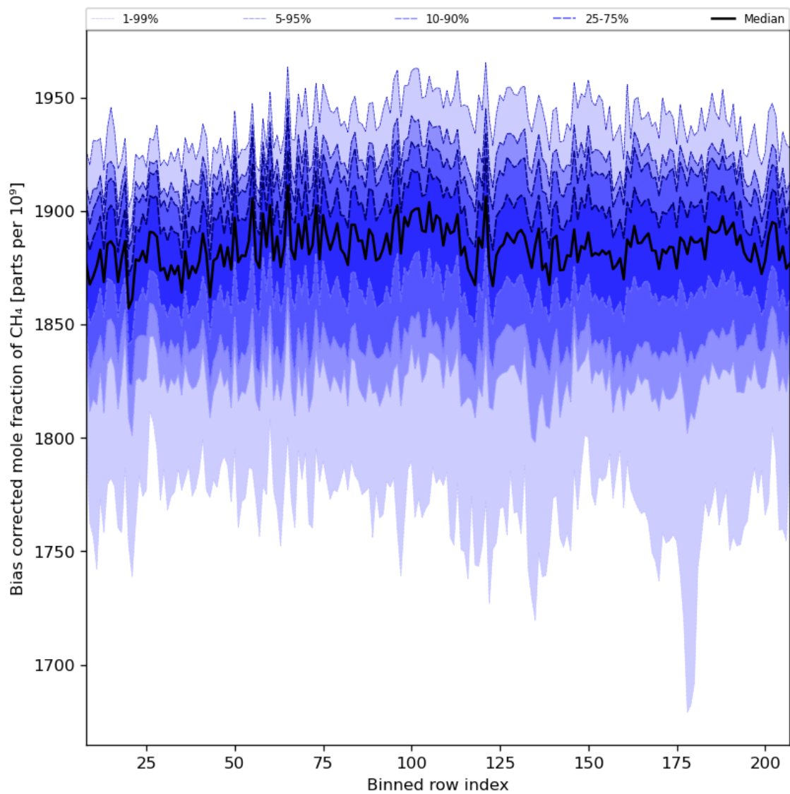
Figure 36: Along track statistics of “Bias corrected mole fraction of CH 4 ” for 2024-06-25 to 2024-06-27
