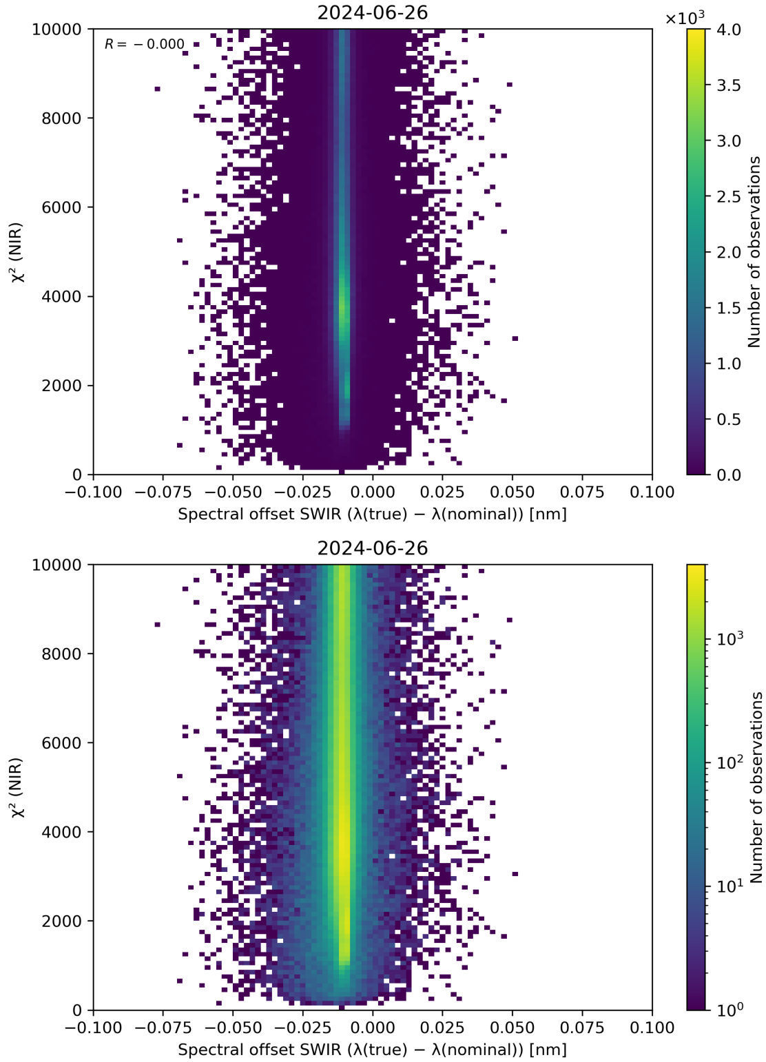
Figure 117: Scatter density plot of “Spectral offset SWIR ( \lambda(\text{true}) - \lambda(\text{nominal}) )” against “ \chi^2 (NIR)” for 2024-06-25 to 2024-06-27.
