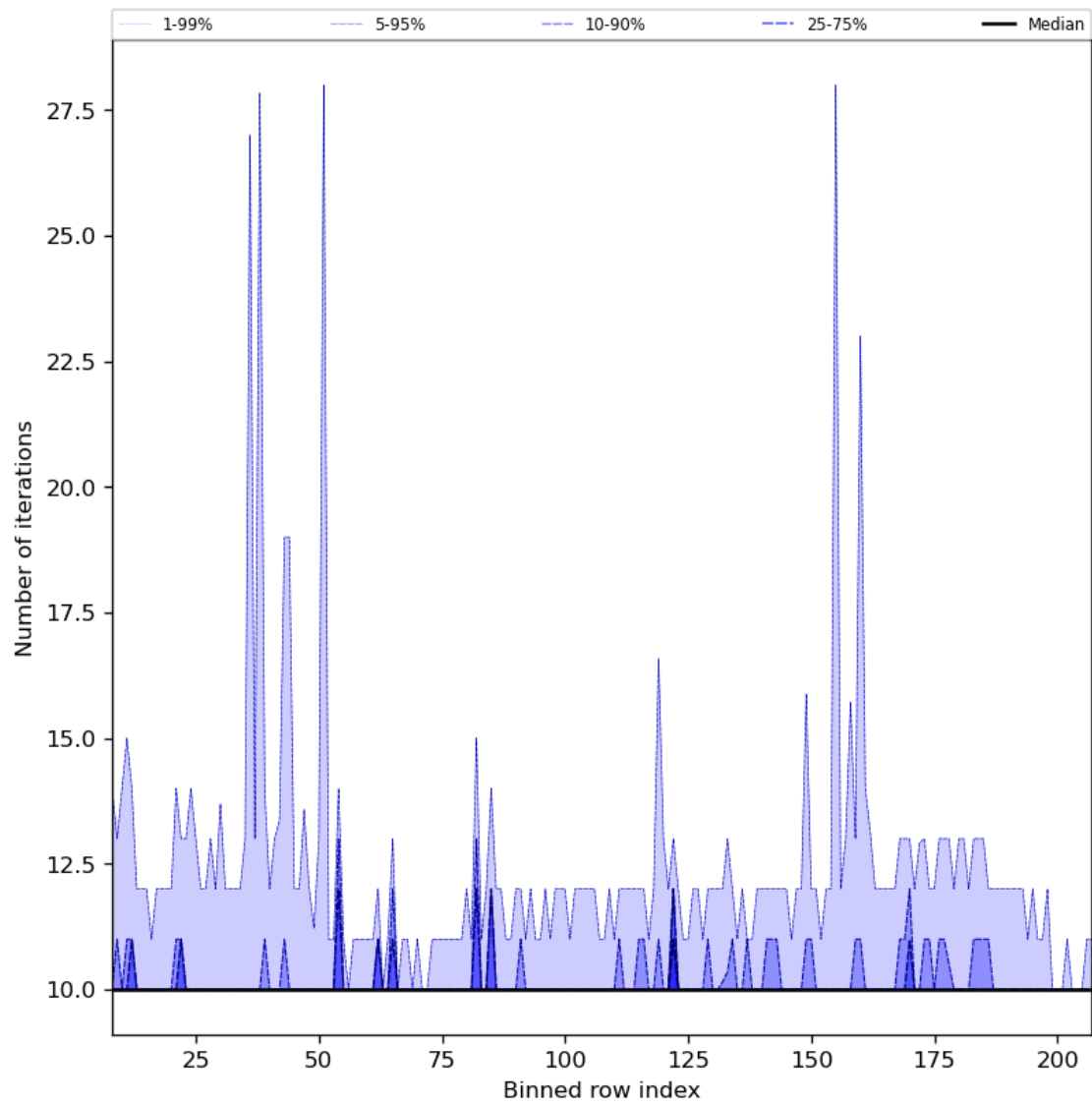
Figure 42: Along track statistics of “Number of iterations” for 2024-06-25 to 2024-06-27
