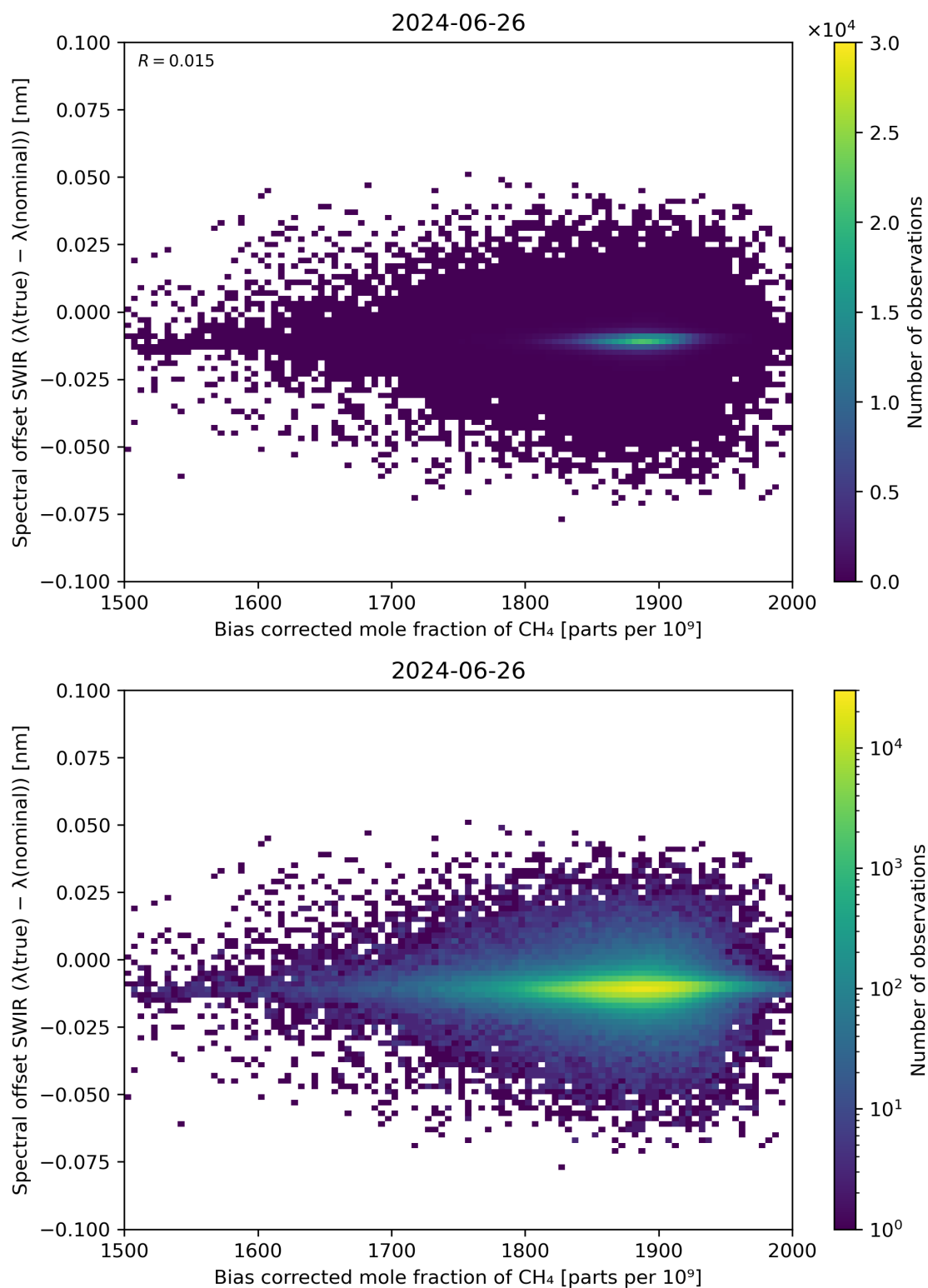
Figure 69: Scatter density plot of “Bias corrected mole fraction of \text{CH}_4 ” against “Spectral offset SWIR ( \lambda(\text{true}) - \lambda(\text{nominal}) )” for 2024-06-25 to 2024-06-27.
