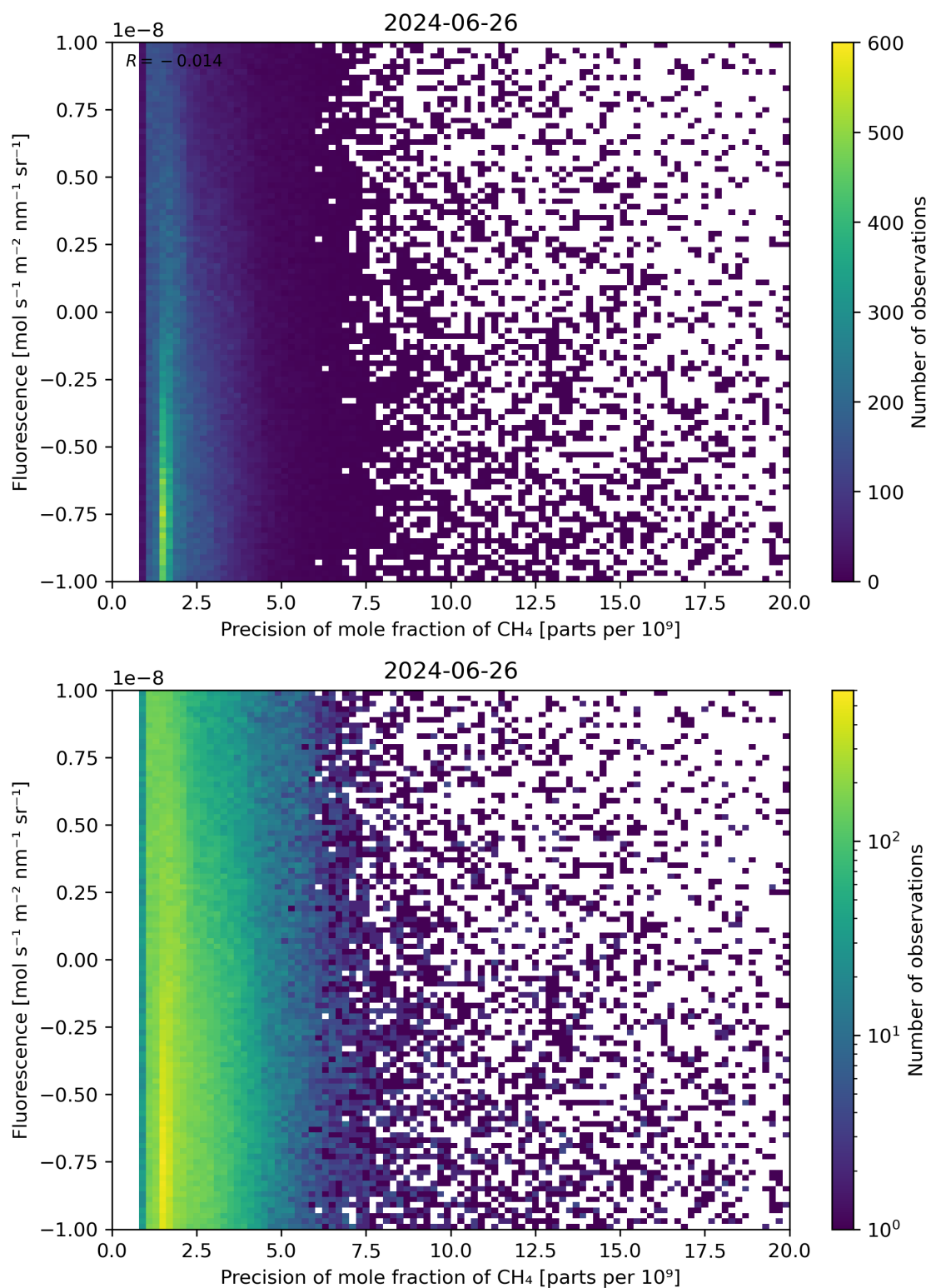
Figure 81: Scatter density plot of “Precision of mole fraction of \text{CH}_4 ” against “Fluorescence” for 2024-06-25 to 2024-06-27.
