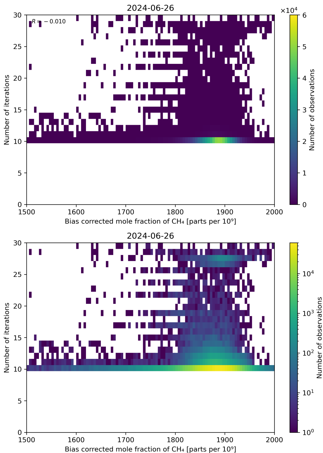
Figure 67: Scatter density plot of “Bias corrected mole fraction of CH 4 ” against “Number of iterations” for 2024-06-25 to 2024-06-27.
