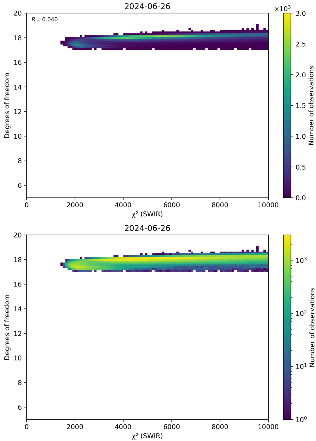
Figure 48: Scatter density plot of “ \chi^2 (SWIR)” against “Degrees of freedom” for 2024-06-25 to 2024-06-27.
