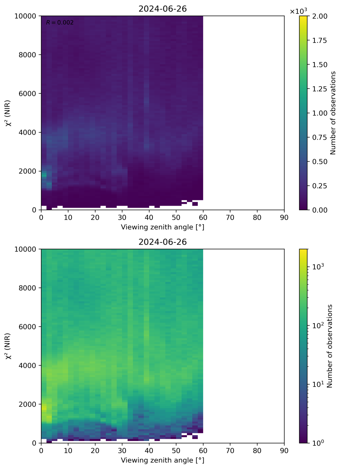
Figure 105: Scatter density plot of “Viewing zenith angle” against “ \chi^2 (NIR)” for 2024-06-25 to 2024-06-27.
