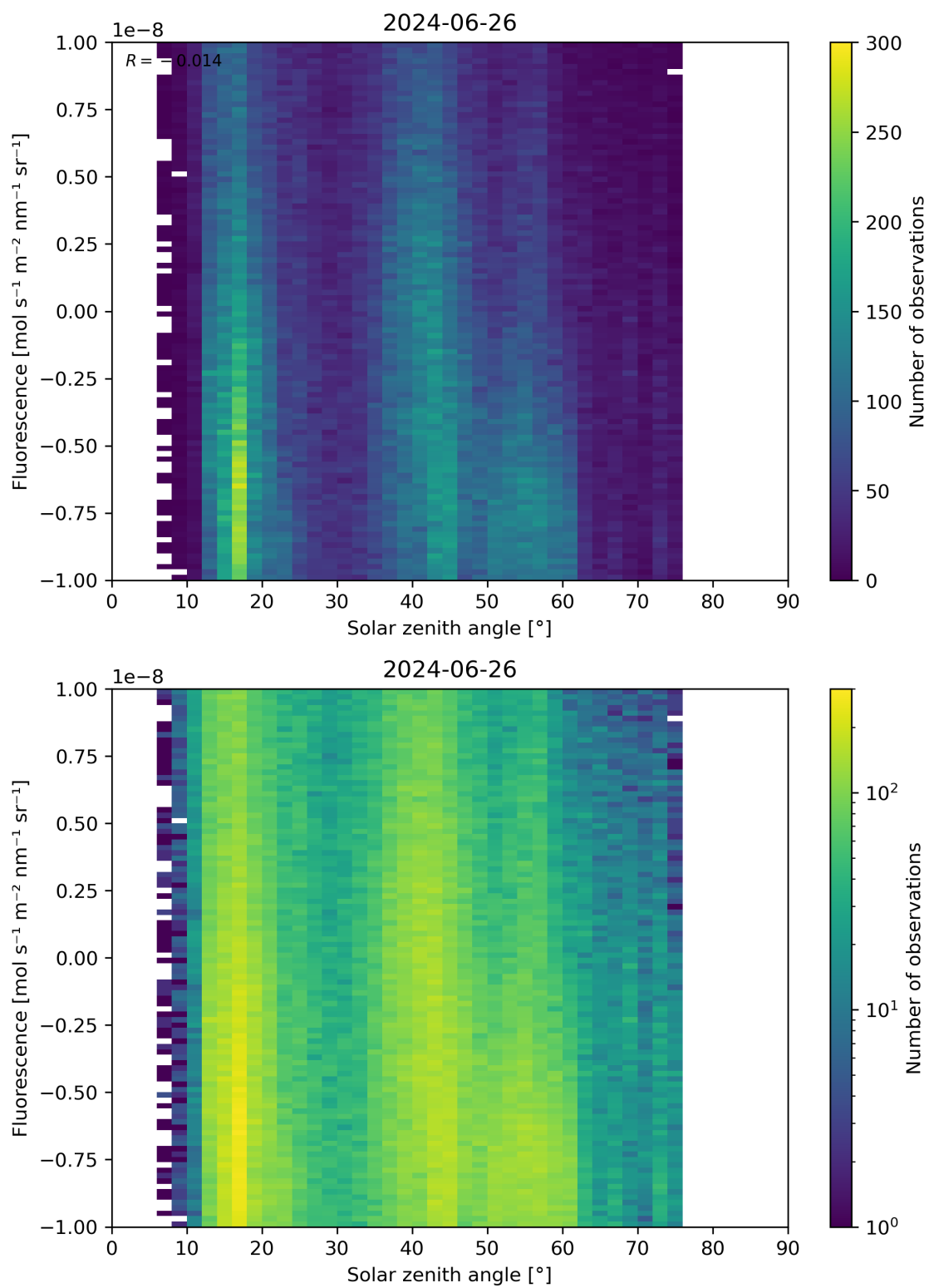
Figure 97: Scatter density plot of “Solar zenith angle” against “Fluorescence” for 2024-06-25 to 2024-06-27.
