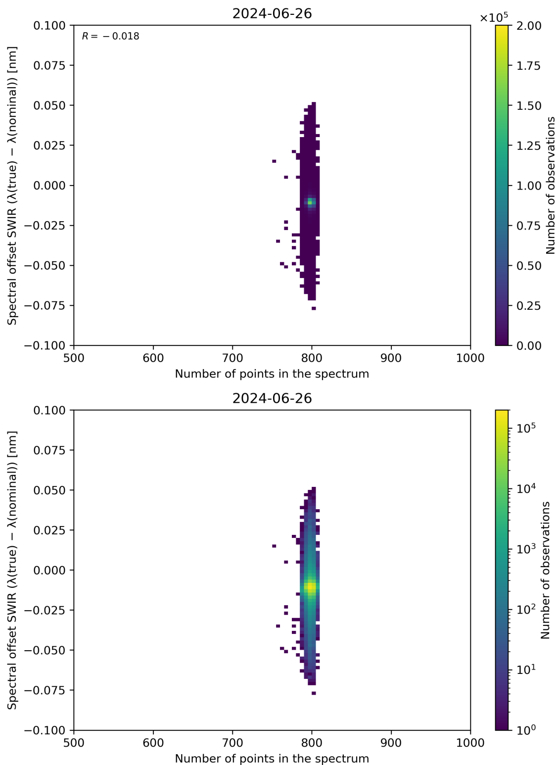
Figure 93: Scatter density plot of “Number of points in the spectrum” against “Spectral offset SWIR ( \lambda(\text{true}) - \lambda(\text{nominal}) )” for 2024-06-25 to 2024-06-27.
