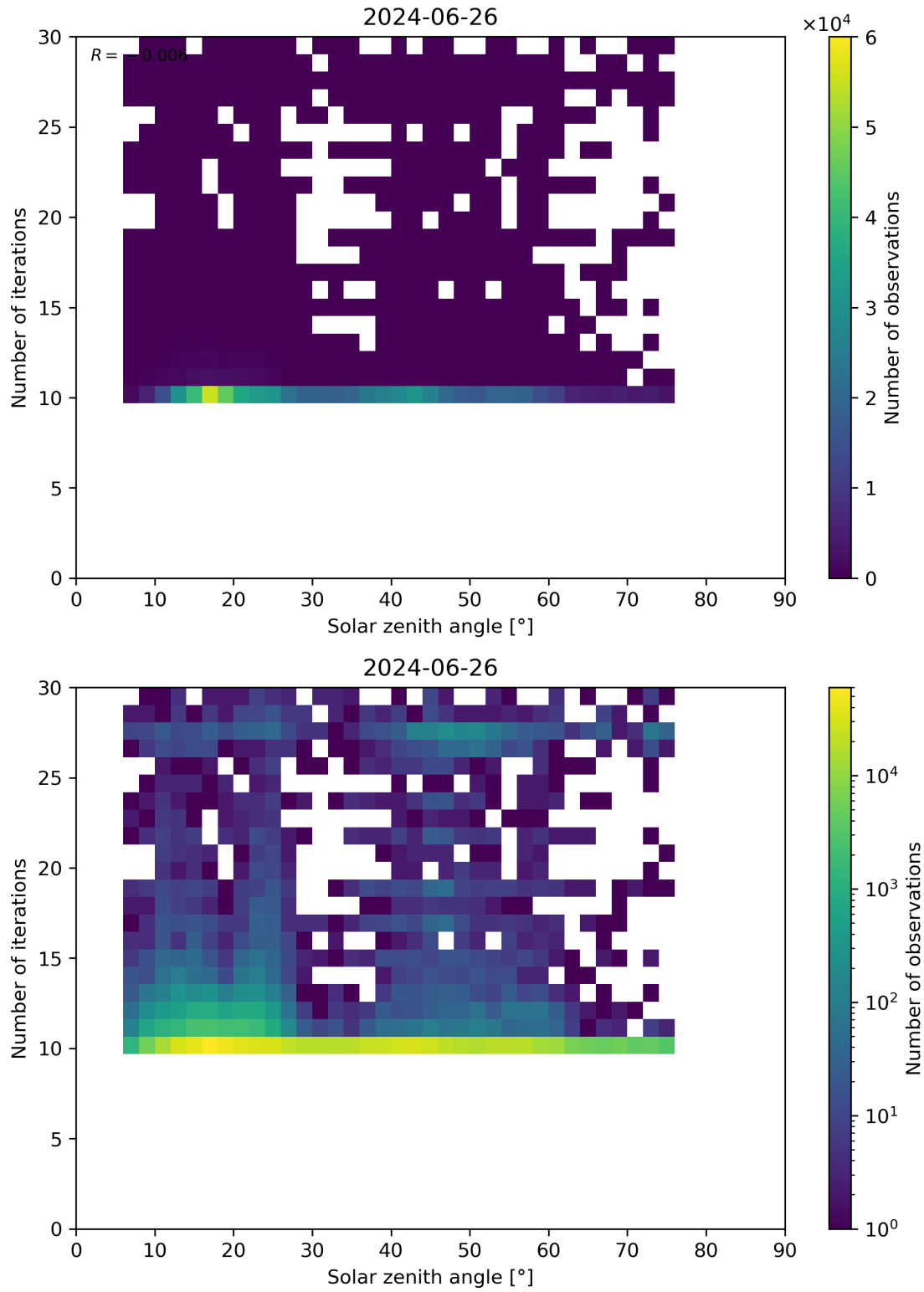
Figure 102: Scatter density plot of “Solar zenith angle” against “Number of iterations” for 2024-06-25 to 2024-06-27.
