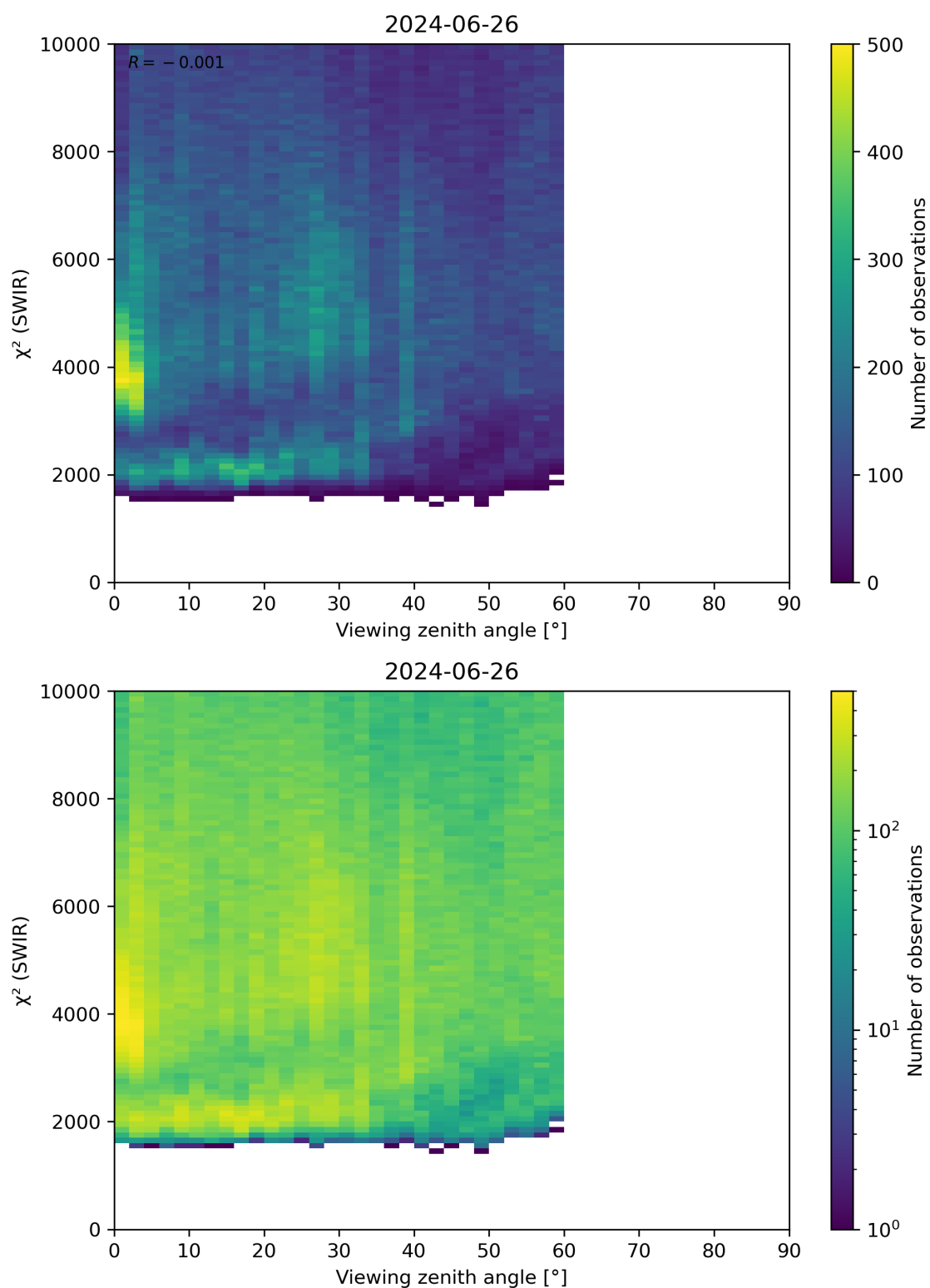
Figure 106: Scatter density plot of “Viewing zenith angle” against “ \chi^2 (SWIR)” for 2024-06-25 to 2024-06-27.
