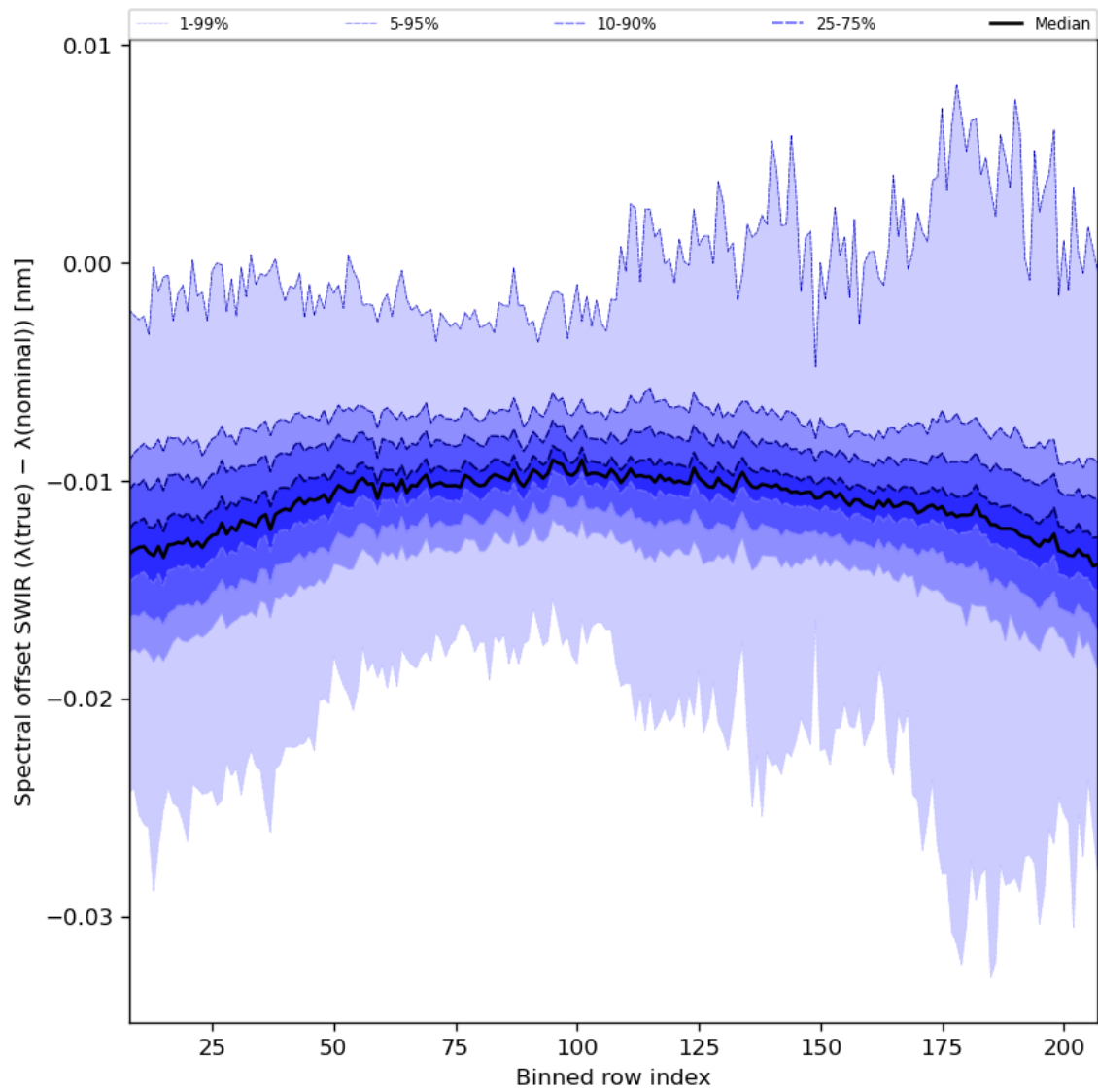
Figure 38: Along track statistics of “Spectral offset SWIR ( \lambda(\text{true}) - \lambda(\text{nominal}) )” for 2024-06-25 to 2024-06-27
