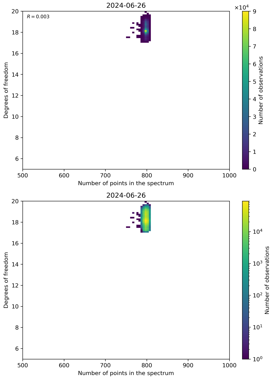
Figure 90: Scatter density plot of “Number of points in the spectrum” against “Degrees of freedom” for 2024-06-25 to 2024-06-27.
