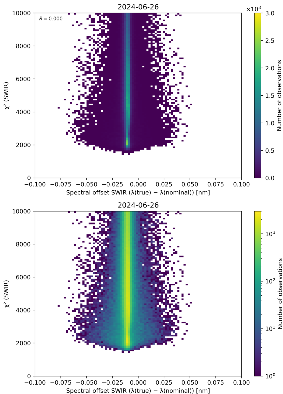
Figure 118: Scatter density plot of “Spectral offset SWIR ( \lambda(\text{true}) - \lambda(\text{nominal}) )” against “ \chi^2 (SWIR)” for 2024-06-25 to 2024-06-27.
