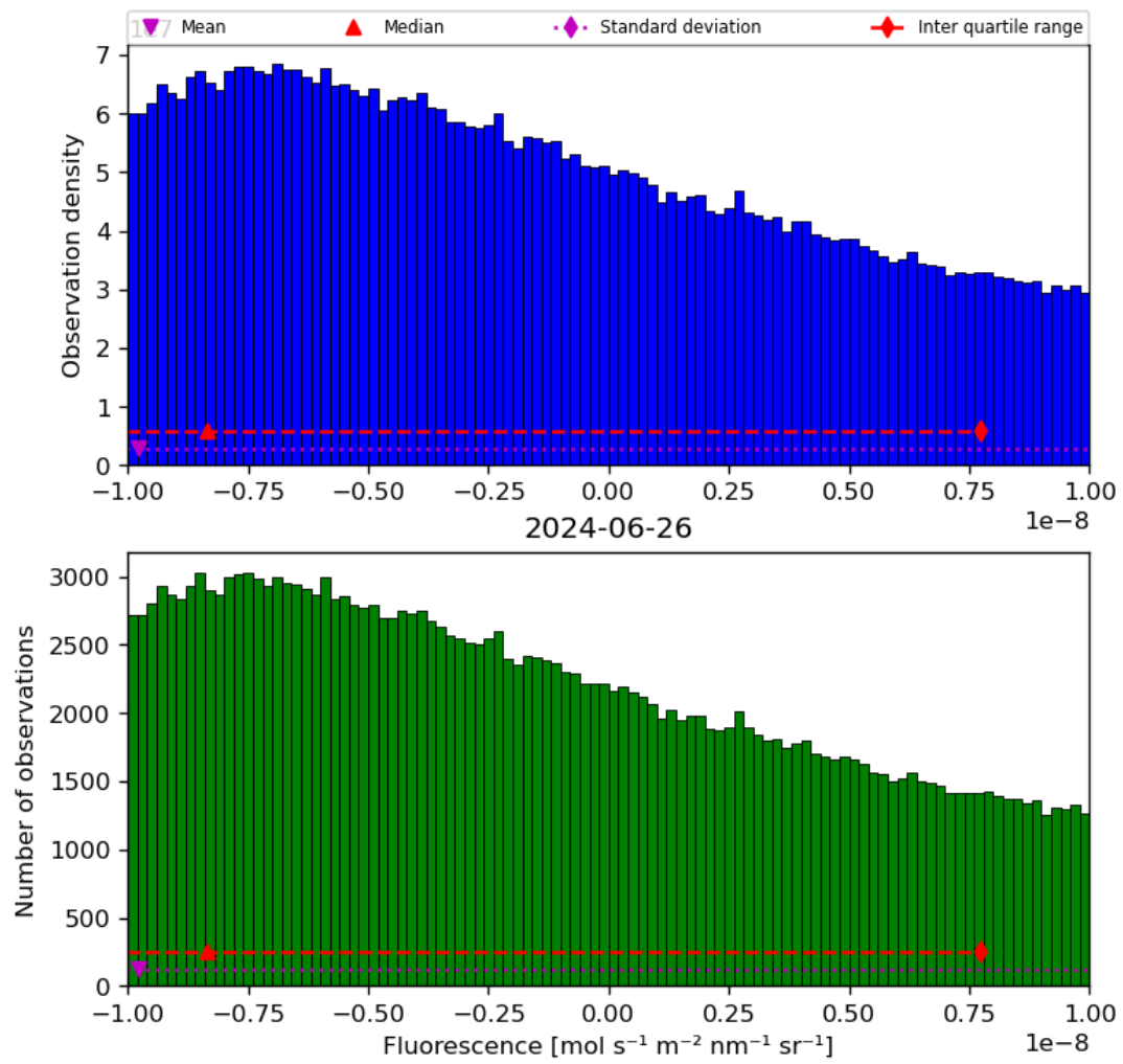
Figure 32: Histogram of “Fluorescence” for 2024-06-25 to 2024-06-27
