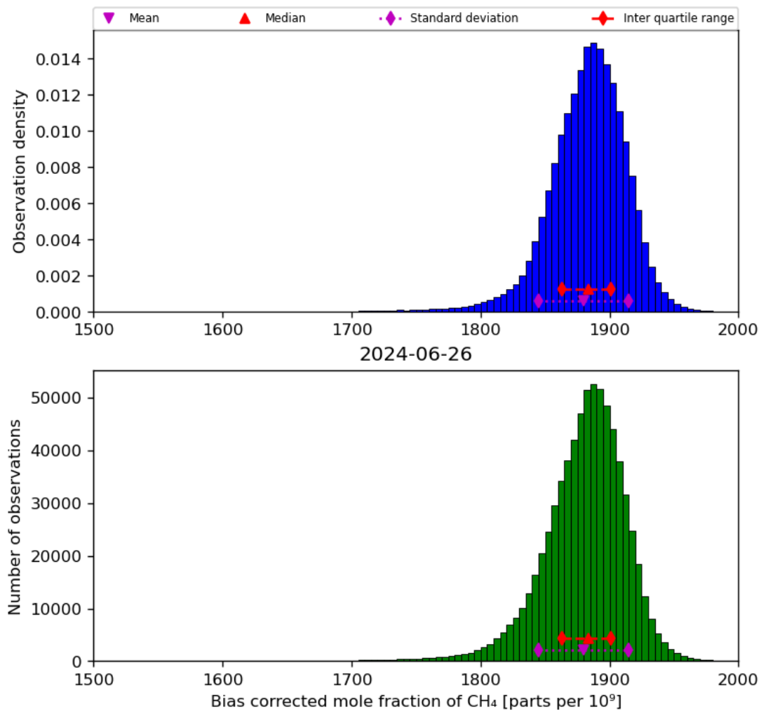
Figure 25: Histogram of “Bias corrected mole fraction of CH 4 ” for 2024-06-25 to 2024-06-27
