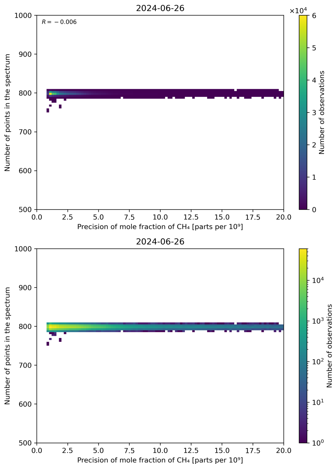
Figure 84: Scatter density plot of “Precision of mole fraction of CH 4 ” against “Number of points in the spectrum” for 2024-06-25 to 2024-06-27.
