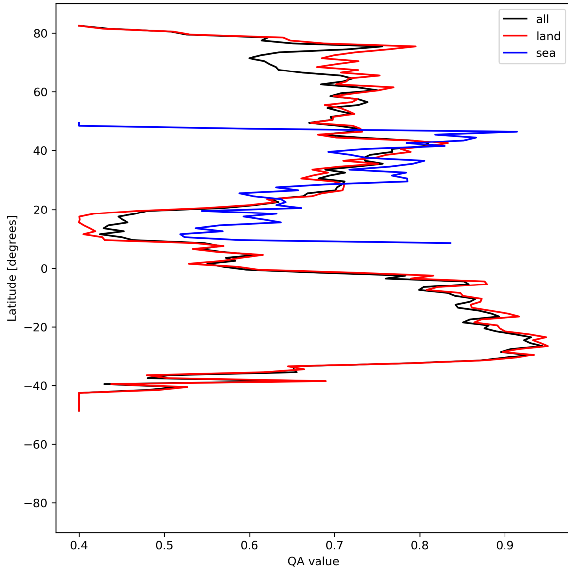
Figure 11: Zonal average of “QA value” for 2024-06-25 to 2024-06-27.
