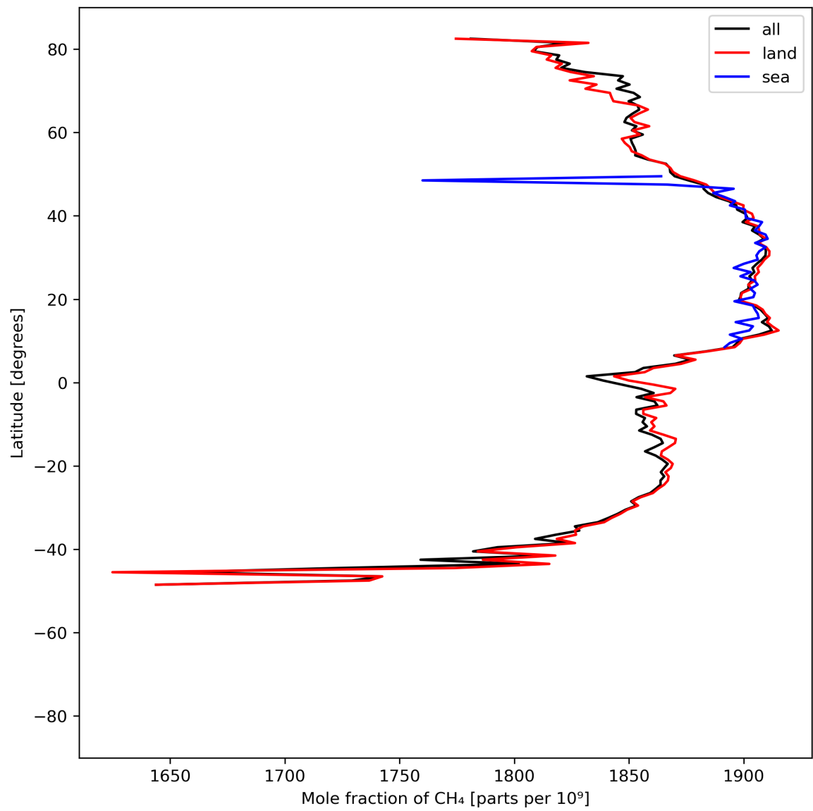
Figure 12: Zonal average of “Mole fraction of \text{CH}_4 ” for 2024-06-25 to 2024-06-27.
