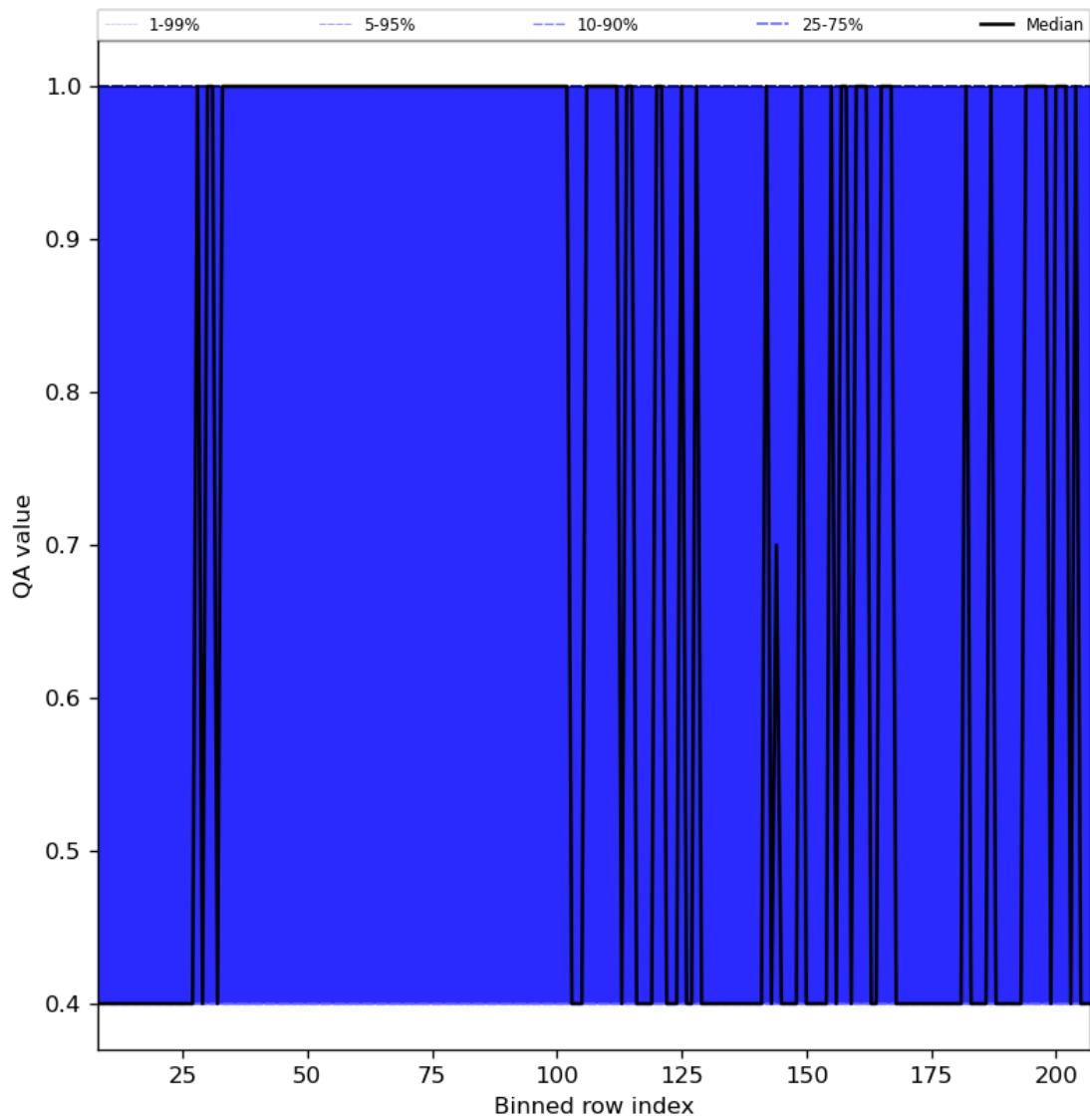
Figure 33: Along track statistics of “QA value” for 2024-06-25 to 2024-06-27
