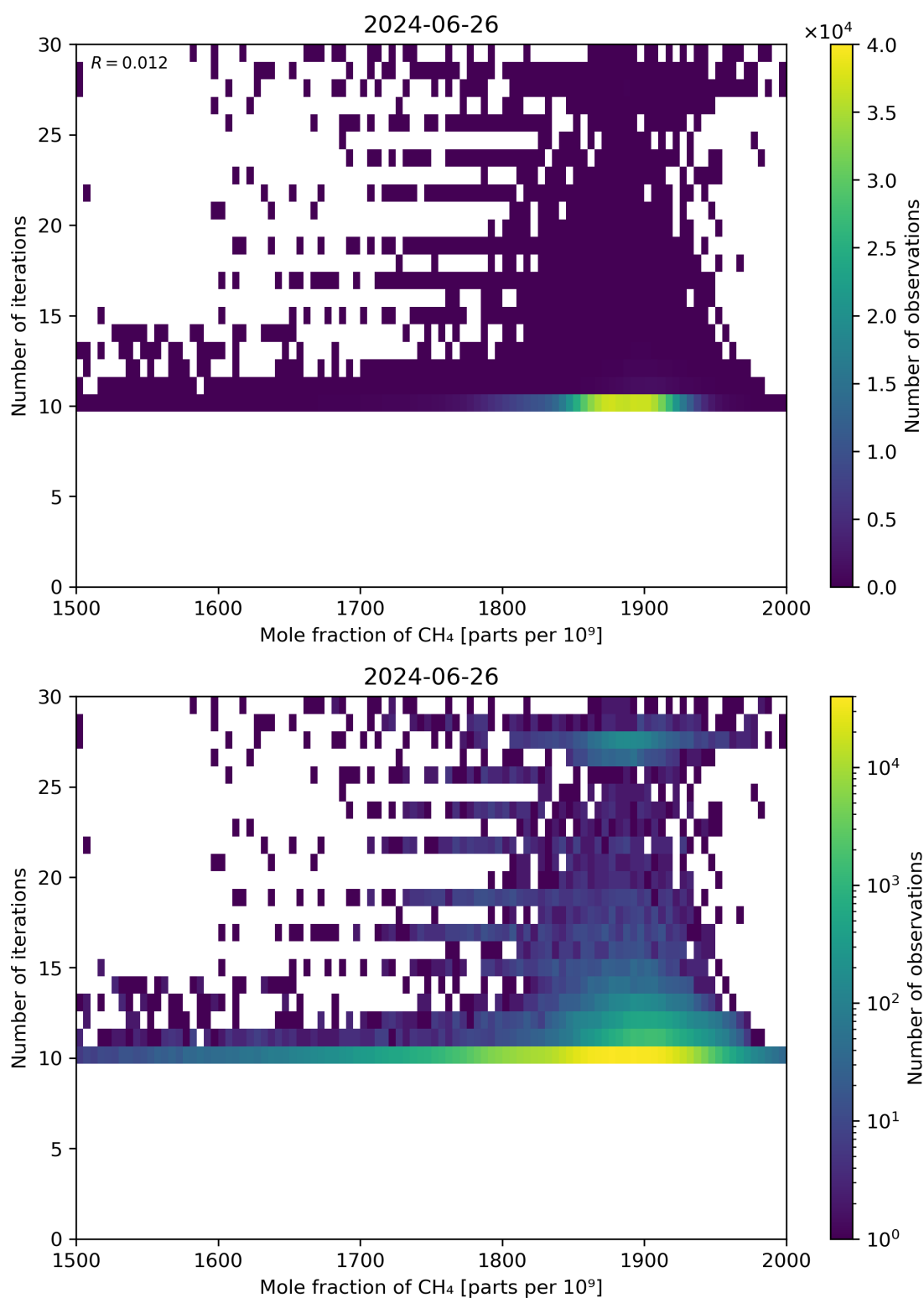
Figure 76: Scatter density plot of “Mole fraction of CH 4 ” against “Number of iterations” for 2024-06-25 to 2024-06-27.
