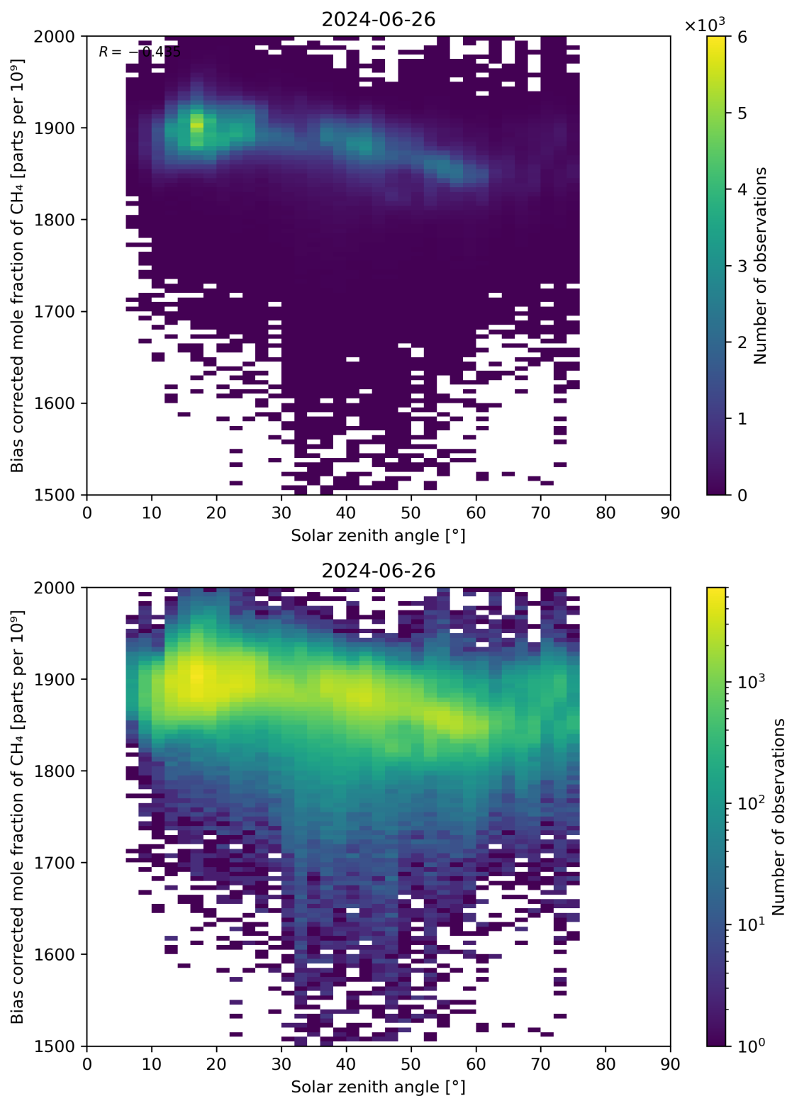
Figure 100: Scatter density plot of “Solar zenith angle” against “Bias corrected mole fraction of CH 4 ” for 2024-06-25 to 2024-06-27.
