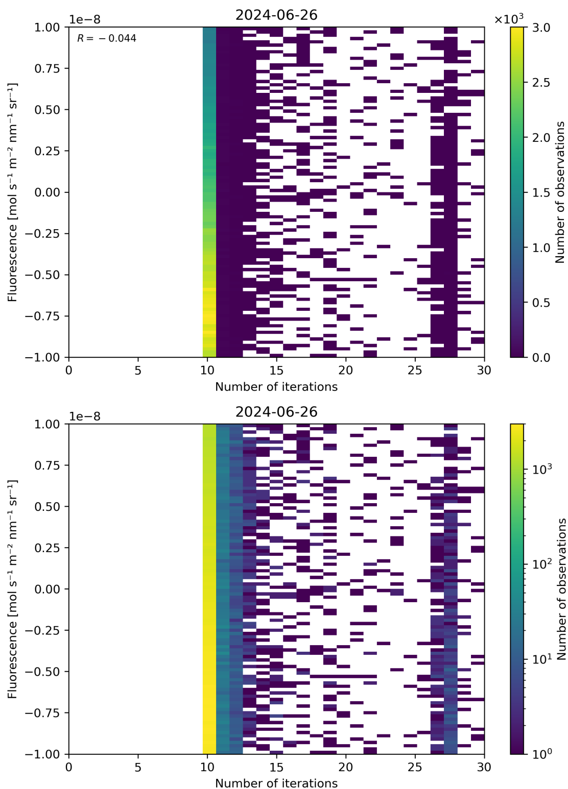
Figure 87: Scatter density plot of “Number of iterations” against “Fluorescence” for 2024-06-25 to 2024-06-27.
