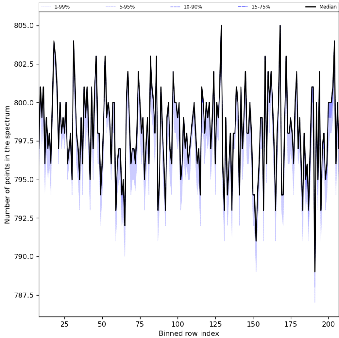
Figure 37: Along track statistics of “Number of points in the spectrum” for 2024-06-25 to 2024-06-27
