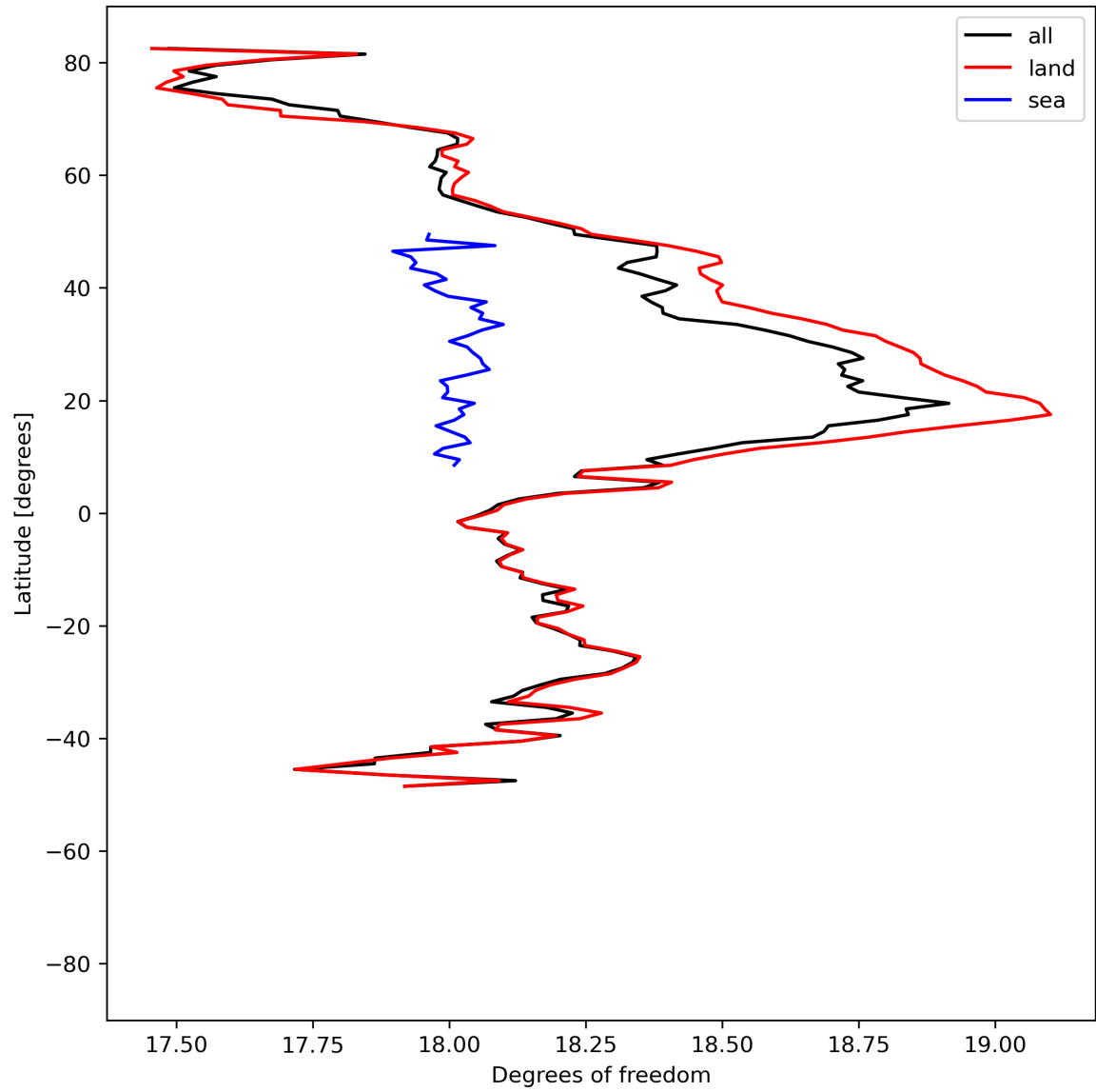
Figure 19: Zonal average of “Degrees of freedom” for 2024-06-25 to 2024-06-27.
