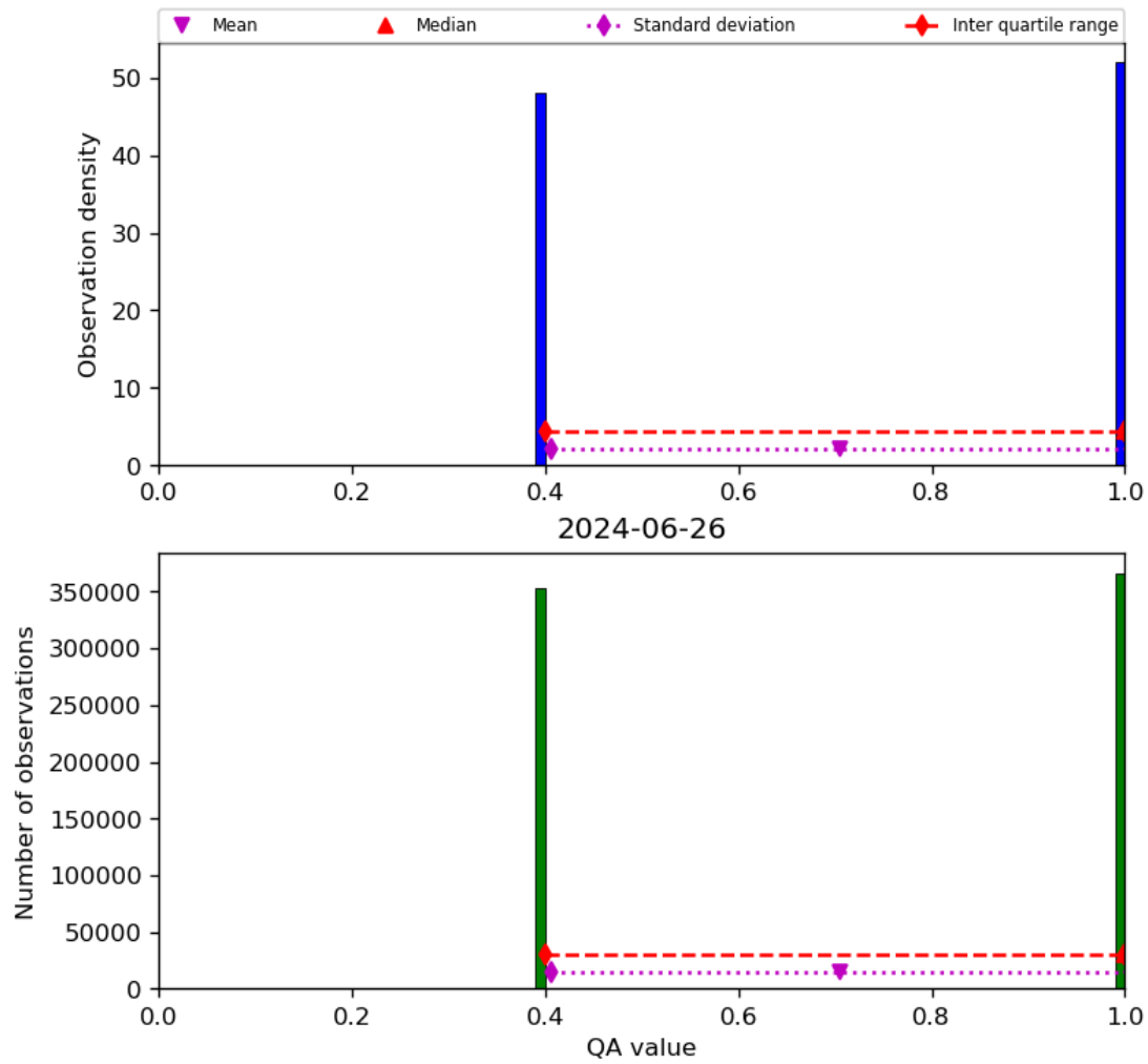
Figure 22: Histogram of “QA value” for 2024-06-25 to 2024-06-27
