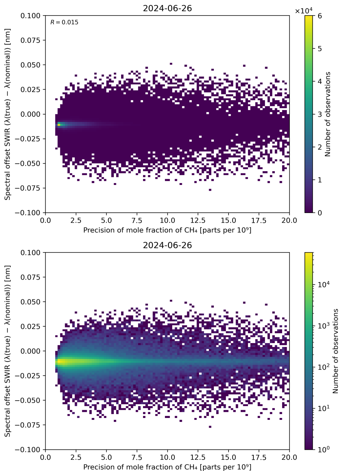
Figure 85: Scatter density plot of “Precision of mole fraction of CH 4 ” against “Spectral offset SWIR ( \lambda(\text{true}) - \lambda(\text{nominal}) )” for 2024-06-25 to 2024-06-27.
