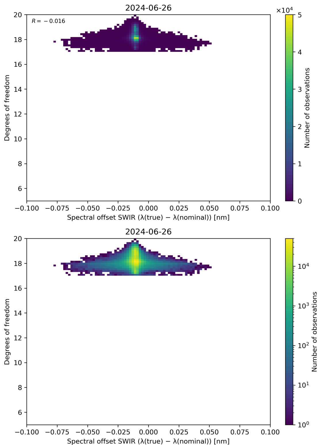
Figure 119: Scatter density plot of “Spectral offset SWIR ( \lambda(\text{true}) - \lambda(\text{nominal}) )” against “Degrees of freedom” for 2024-06-25 to 2024-06-27.
