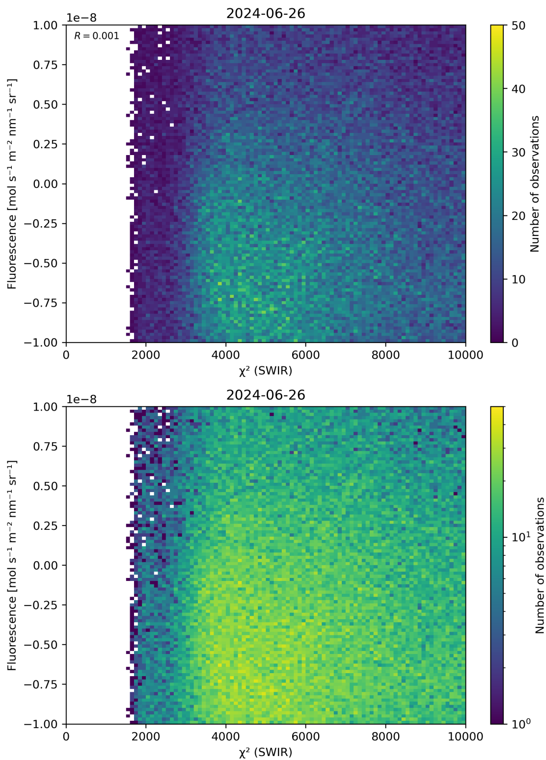
Figure 49: Scatter density plot of “ \chi^2 (SWIR)” against “Fluorescence” for 2024-06-25 to 2024-06-27.
