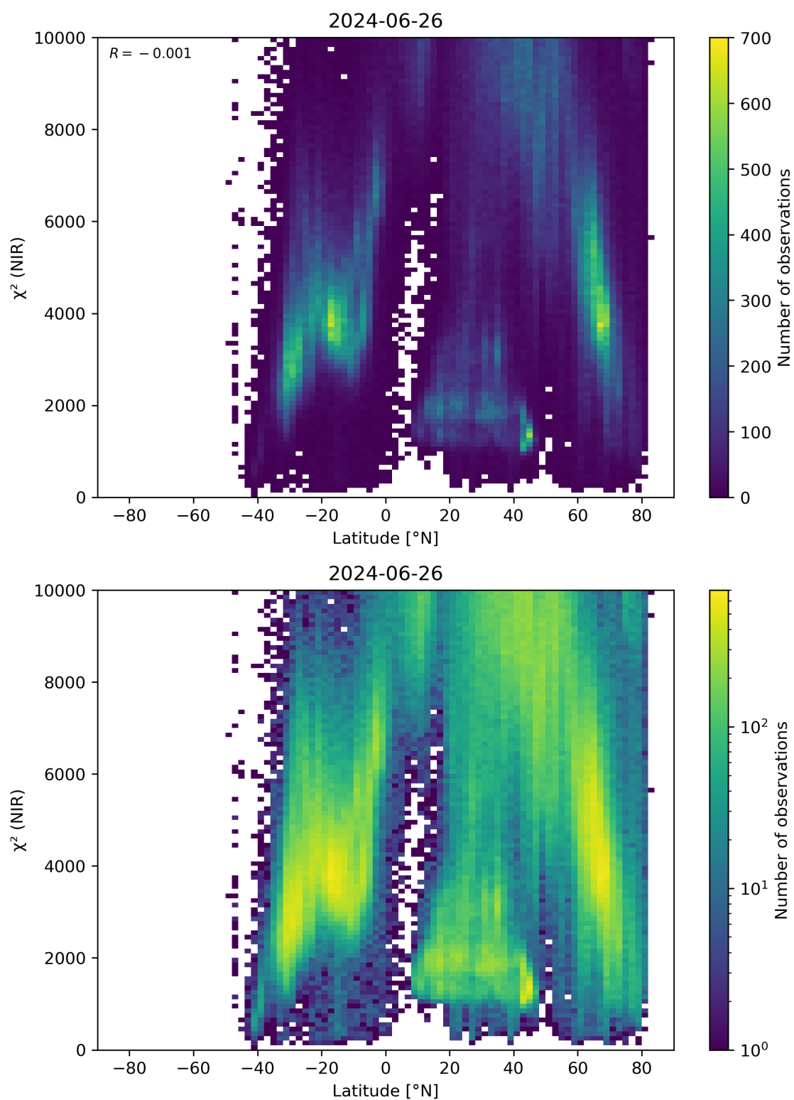
Figure 53: Scatter density plot of “Latitude” against “ \chi^2 (NIR)” for 2024-06-25 to 2024-06-27.
