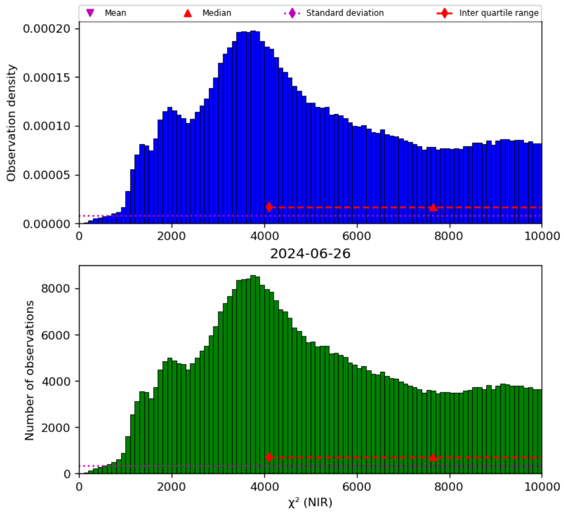
Figure 29: Histogram of “ \chi^2 (NIR)” for 2024-06-25 to 2024-06-27
