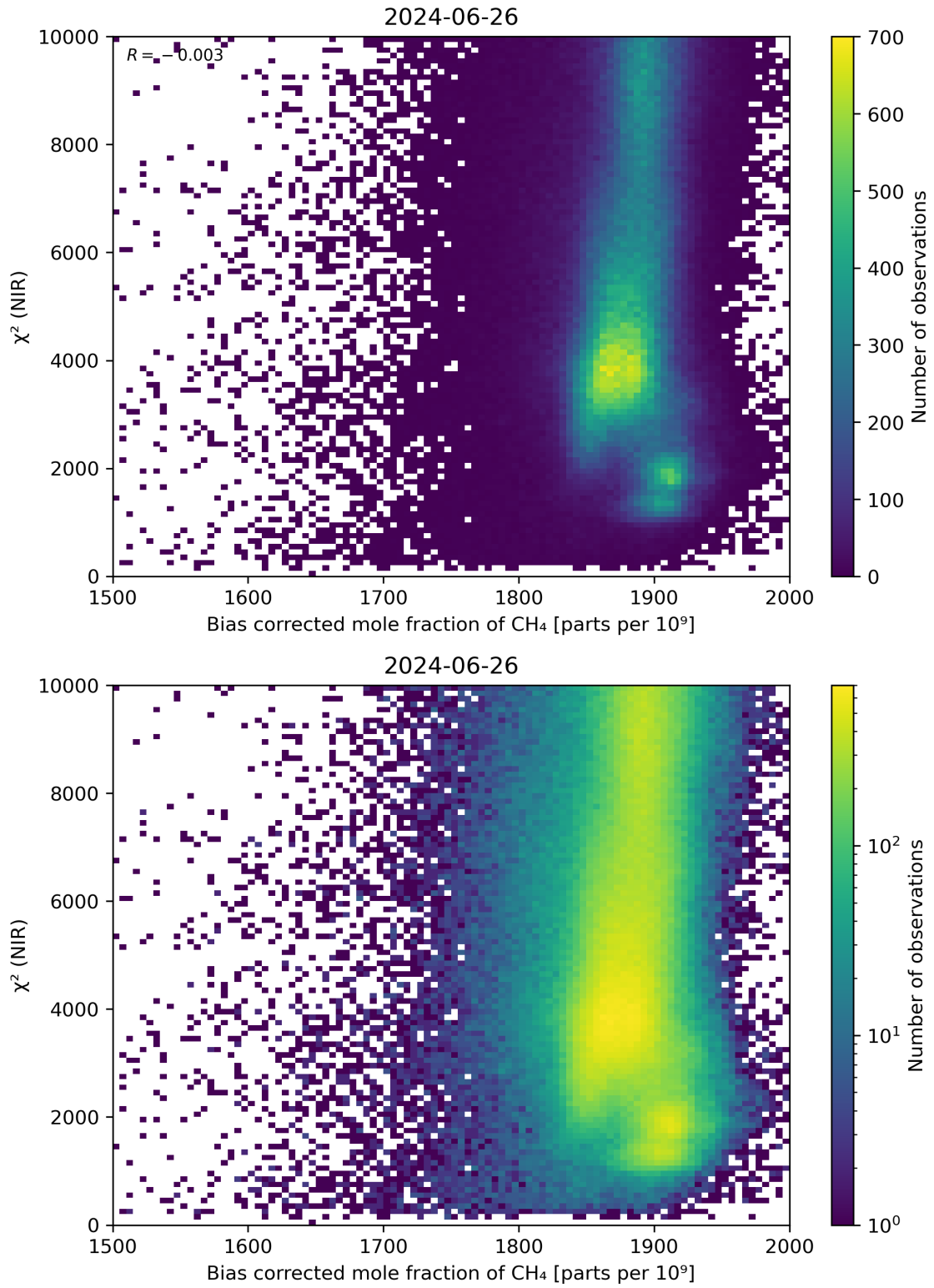
Figure 63: Scatter density plot of “Bias corrected mole fraction of CH 4 ” against “ \chi^2 (NIR)” for 2024-06-25 to 2024-06-27.
