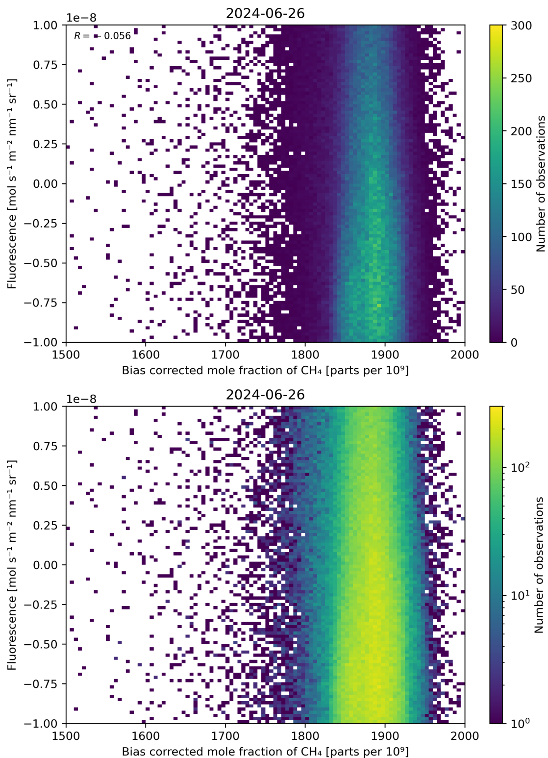
Figure 66: Scatter density plot of “Bias corrected mole fraction of \text{CH}_4 ” against “Fluorescence” for 2024-06-25 to 2024-06-27.
