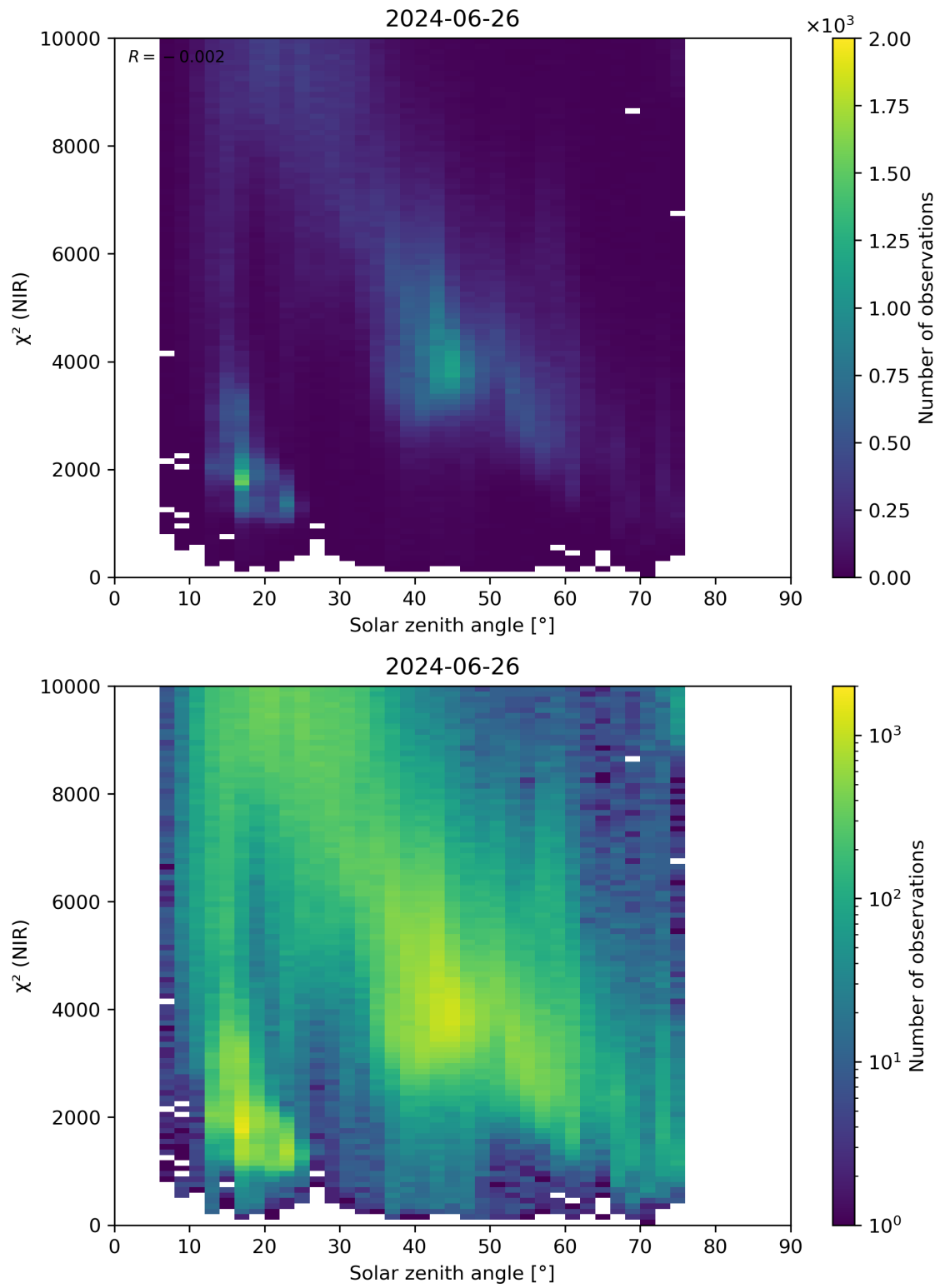
Figure 94: Scatter density plot of “Solar zenith angle” against “ \chi^2 (NIR)” for 2024-06-25 to 2024-06-27.
