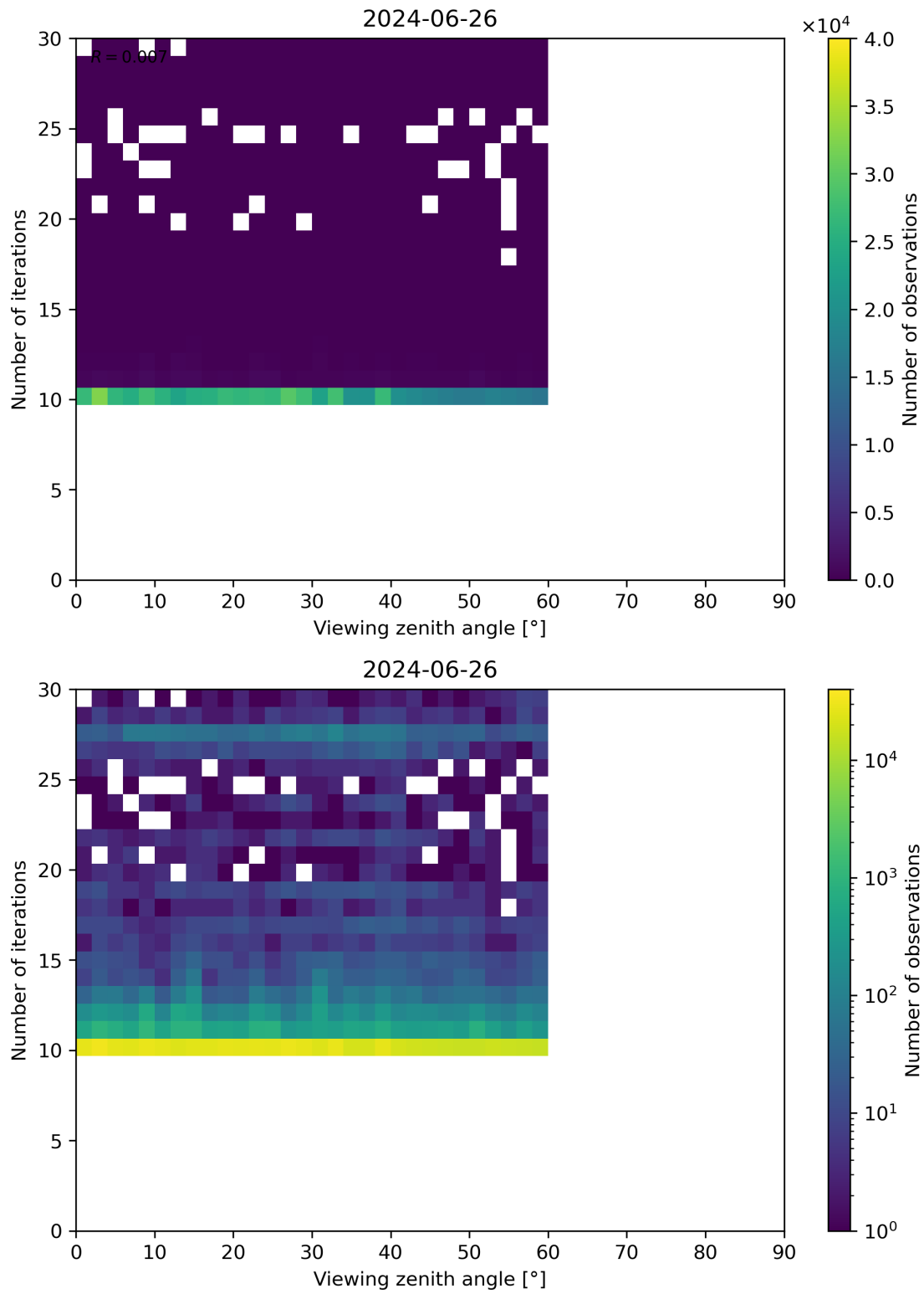
Figure 113: Scatter density plot of “Viewing zenith angle” against “Number of iterations” for 2024-06-25 to 2024-06-27.
