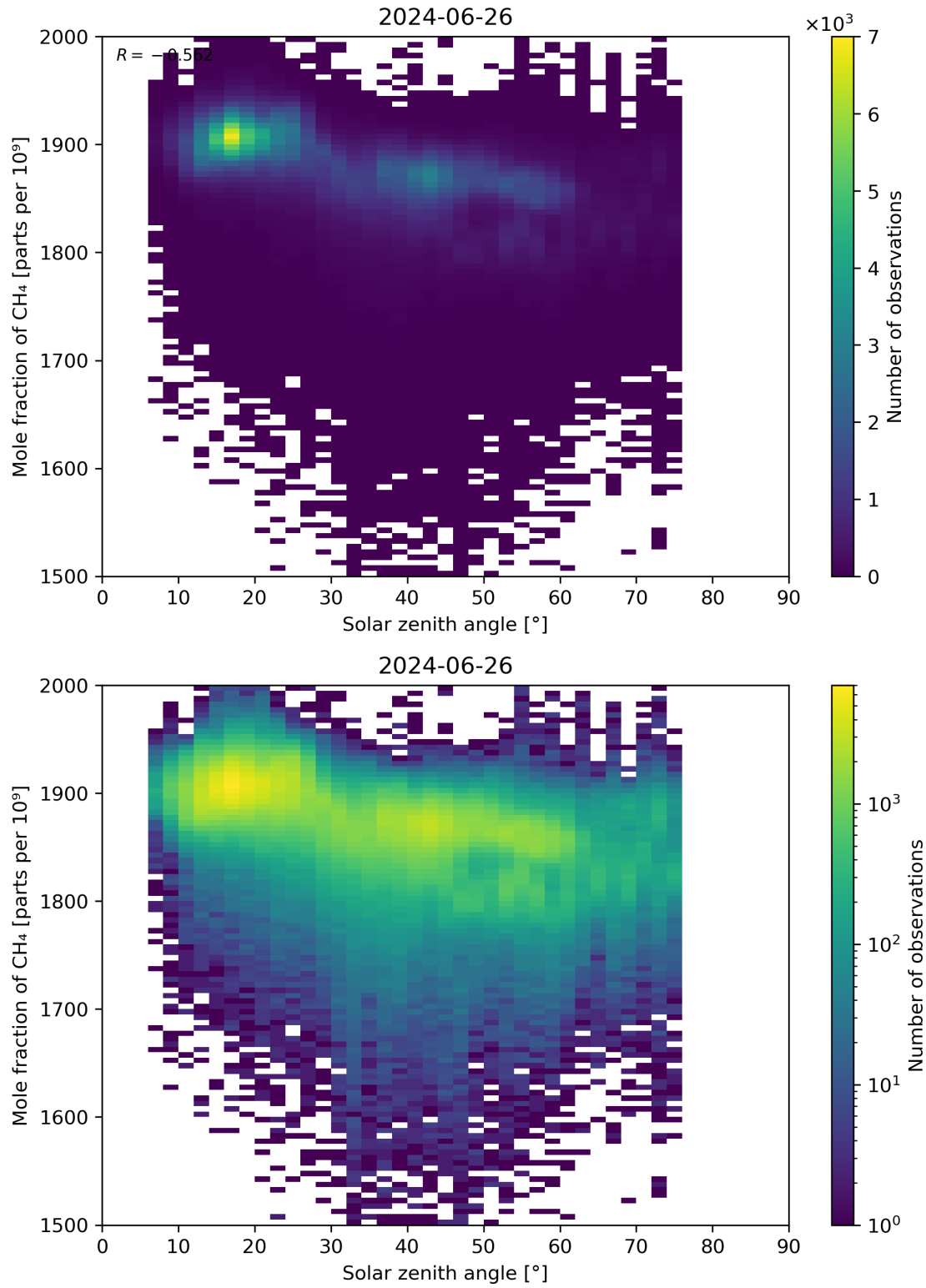
Figure 99: Scatter density plot of “Solar zenith angle” against “Mole fraction of CH 4 ” for 2024-06-25 to 2024-06-27.
