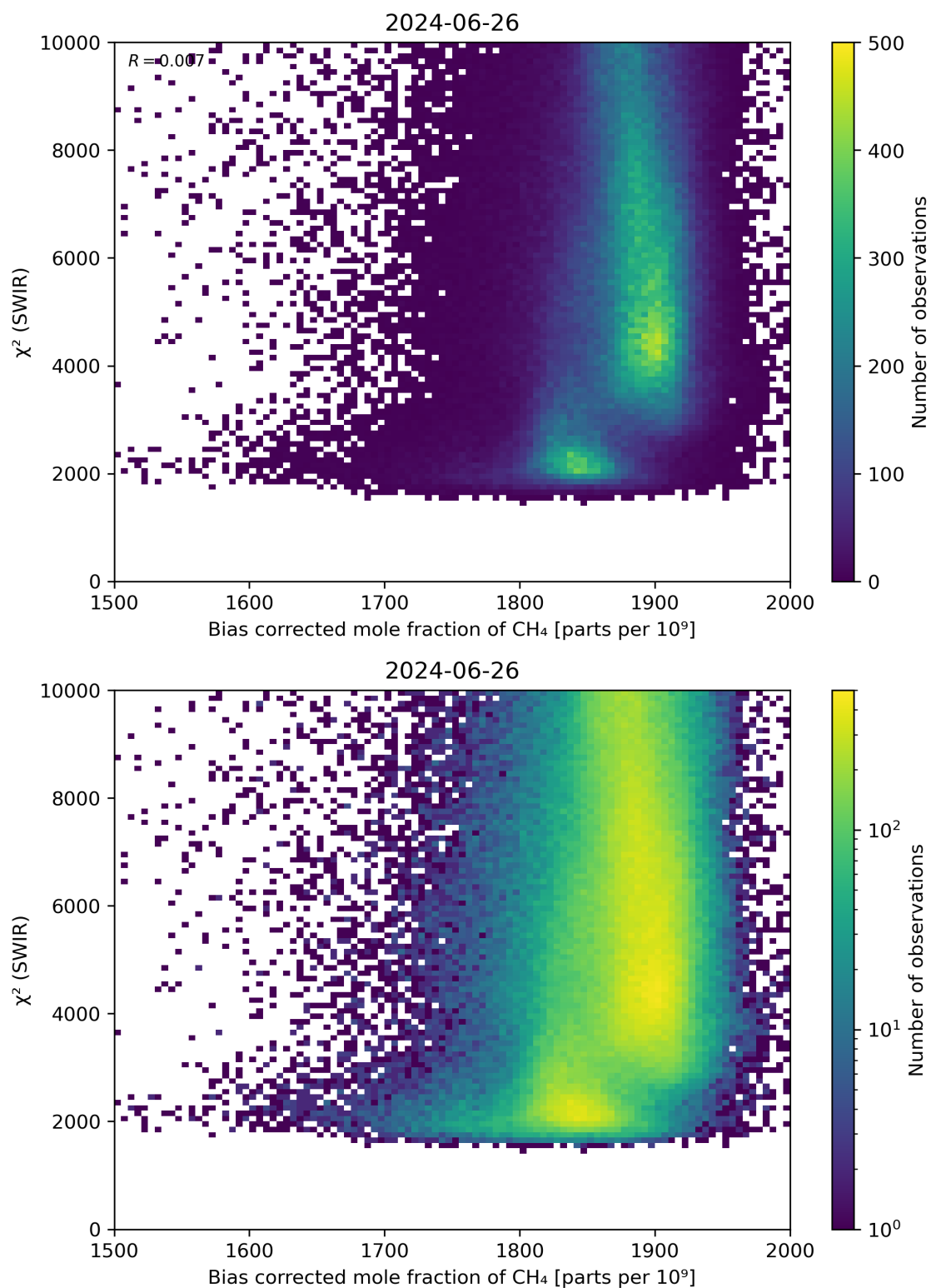
Figure 64: Scatter density plot of “Bias corrected mole fraction of CH 4 ” against “ \chi^2 (SWIR)” for 2024-06-25 to 2024-06-27.
