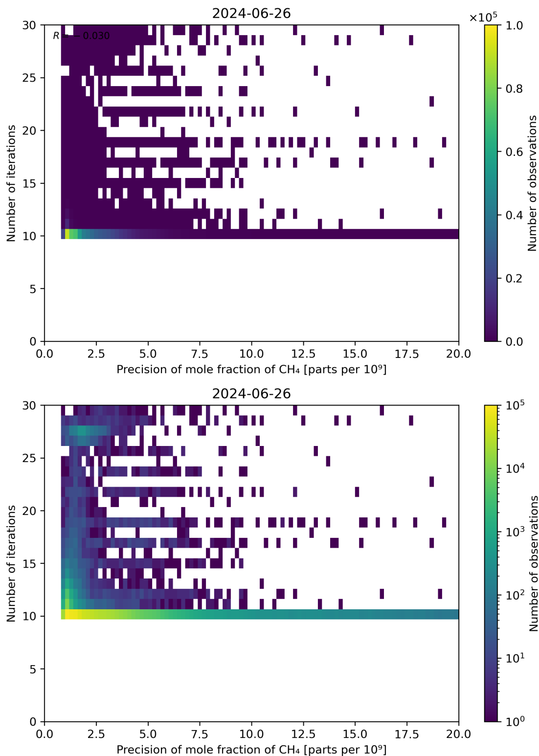
Figure 83: Scatter density plot of “Precision of mole fraction of CH 4 ” against “Number of iterations” for 2024-06-25 to 2024-06-27.
