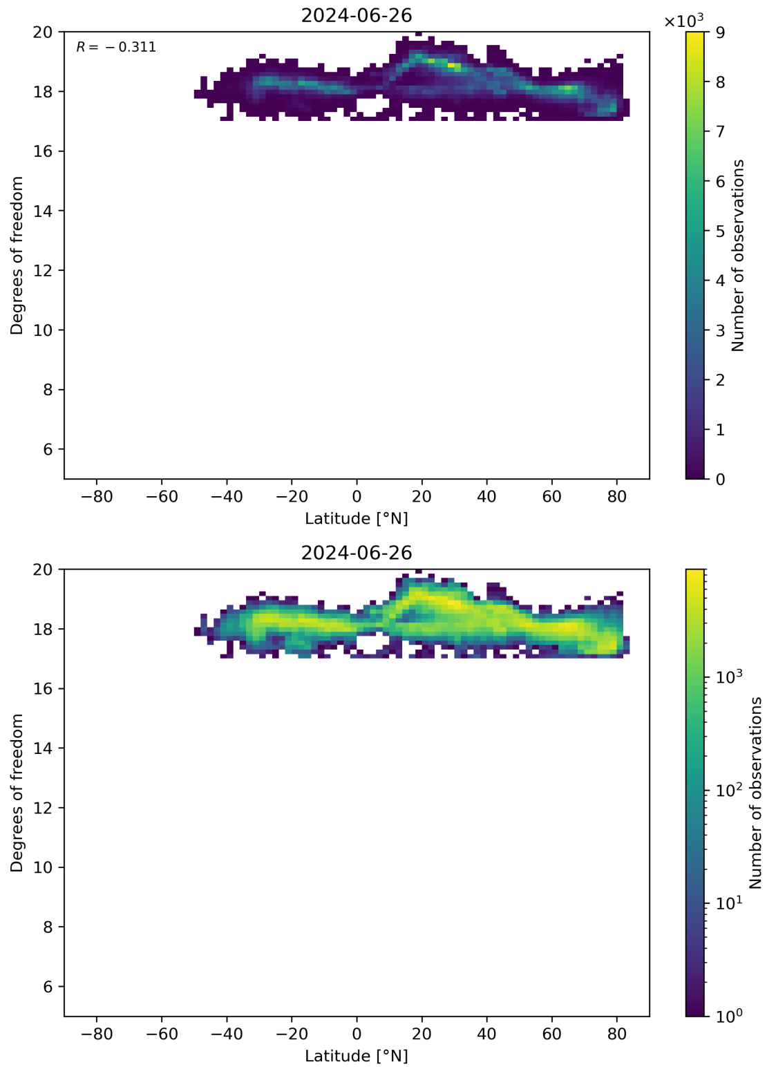
Figure 55: Scatter density plot of “Latitude” against “Degrees of freedom” for 2024-06-25 to 2024-06-27.
