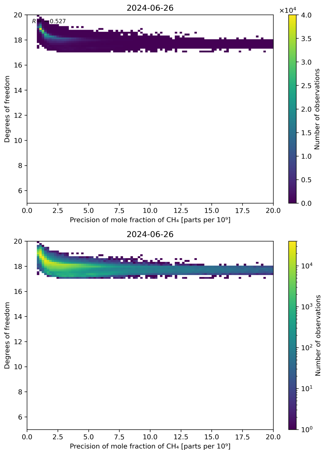
Figure 80: Scatter density plot of “Precision of mole fraction of CH 4 ” against “Degrees of freedom” for 2024-06-25 to 2024-06-27.
