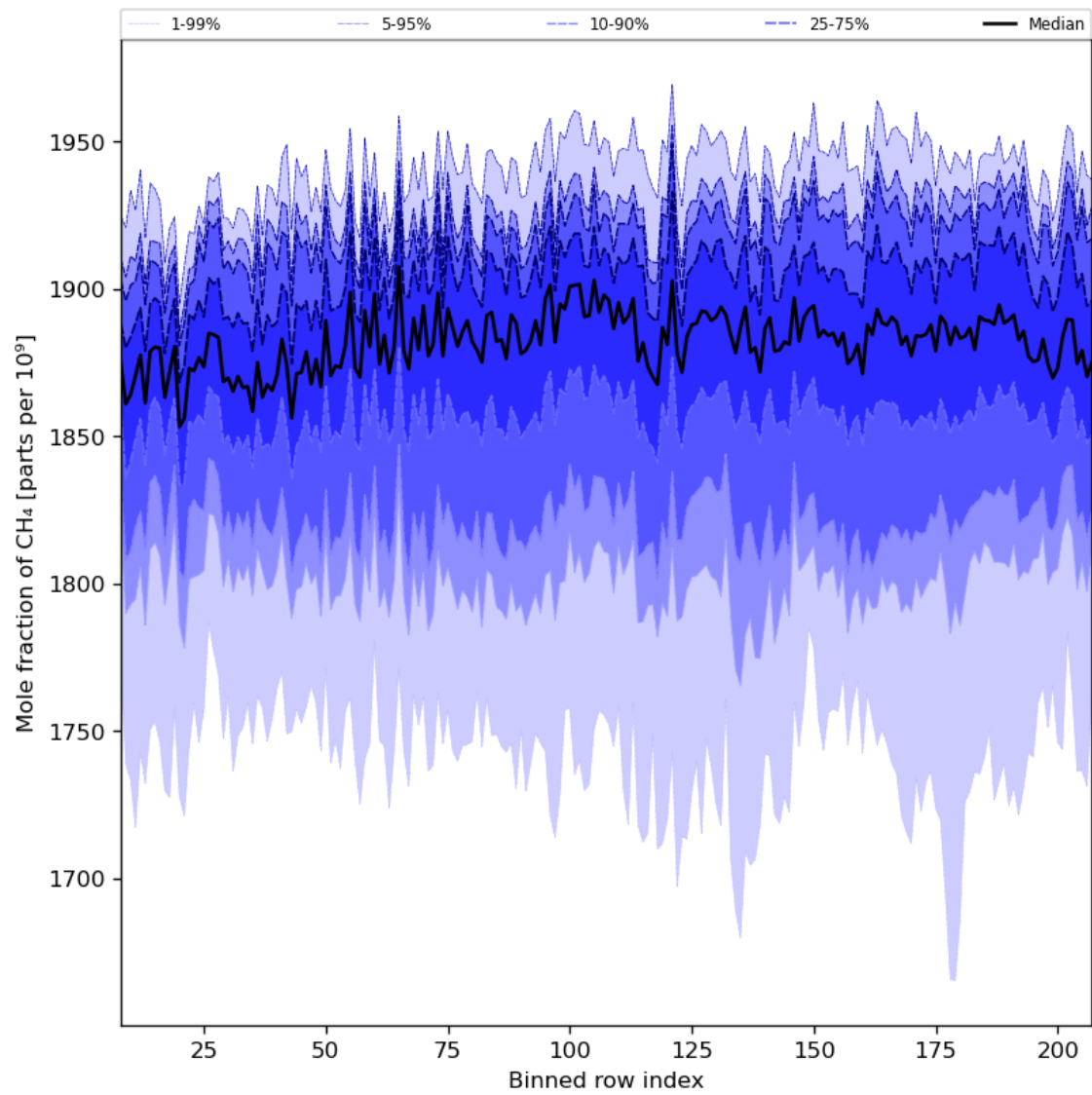
Figure 34: Along track statistics of “Mole fraction of CH 4 ” for 2024-06-25 to 2024-06-27
