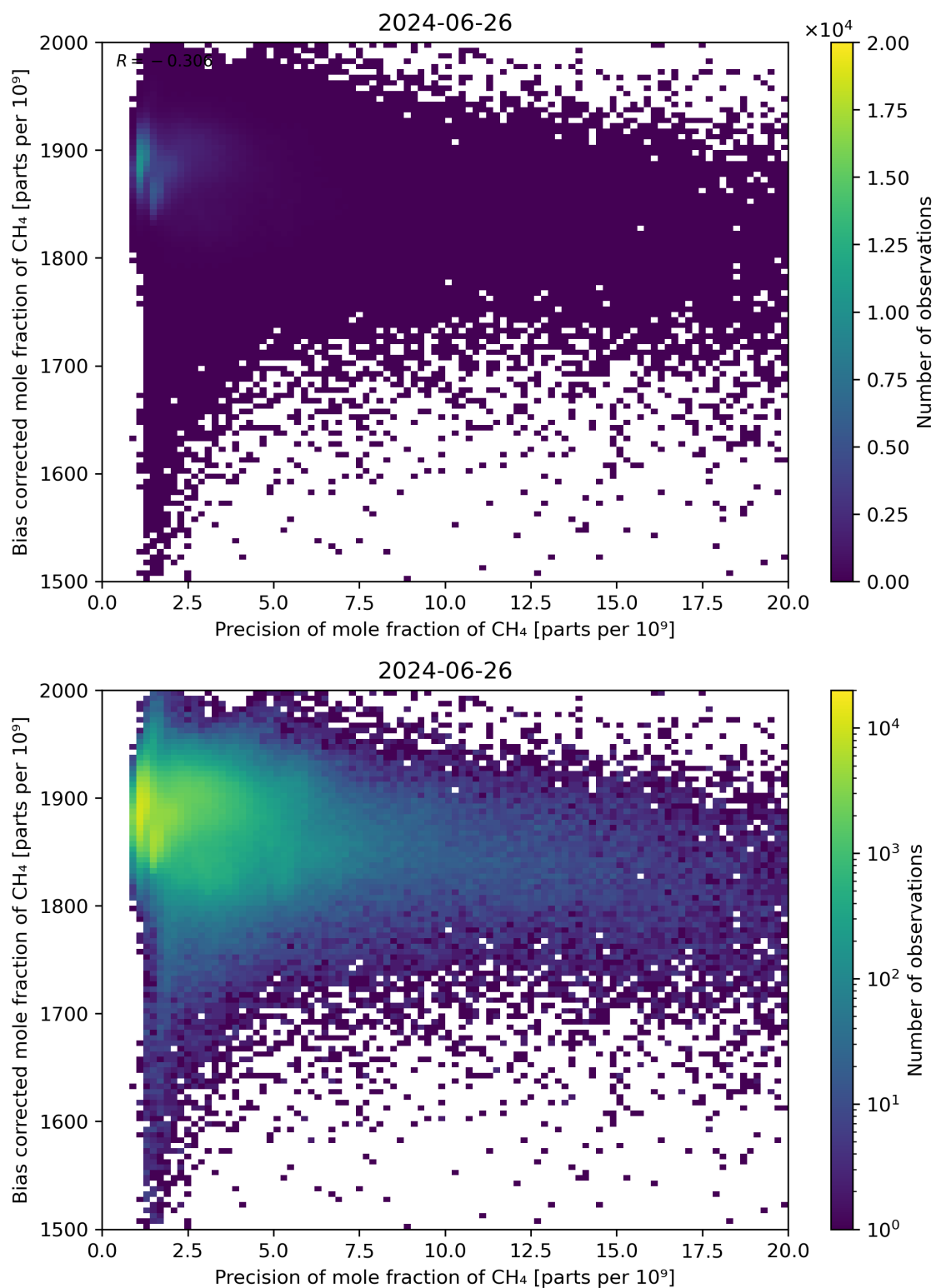
Figure 82: Scatter density plot of “Precision of mole fraction of CH 4 ” against “Bias corrected mole fraction of CH 4 ” for 2024-06-25 to 2024-06-27.
