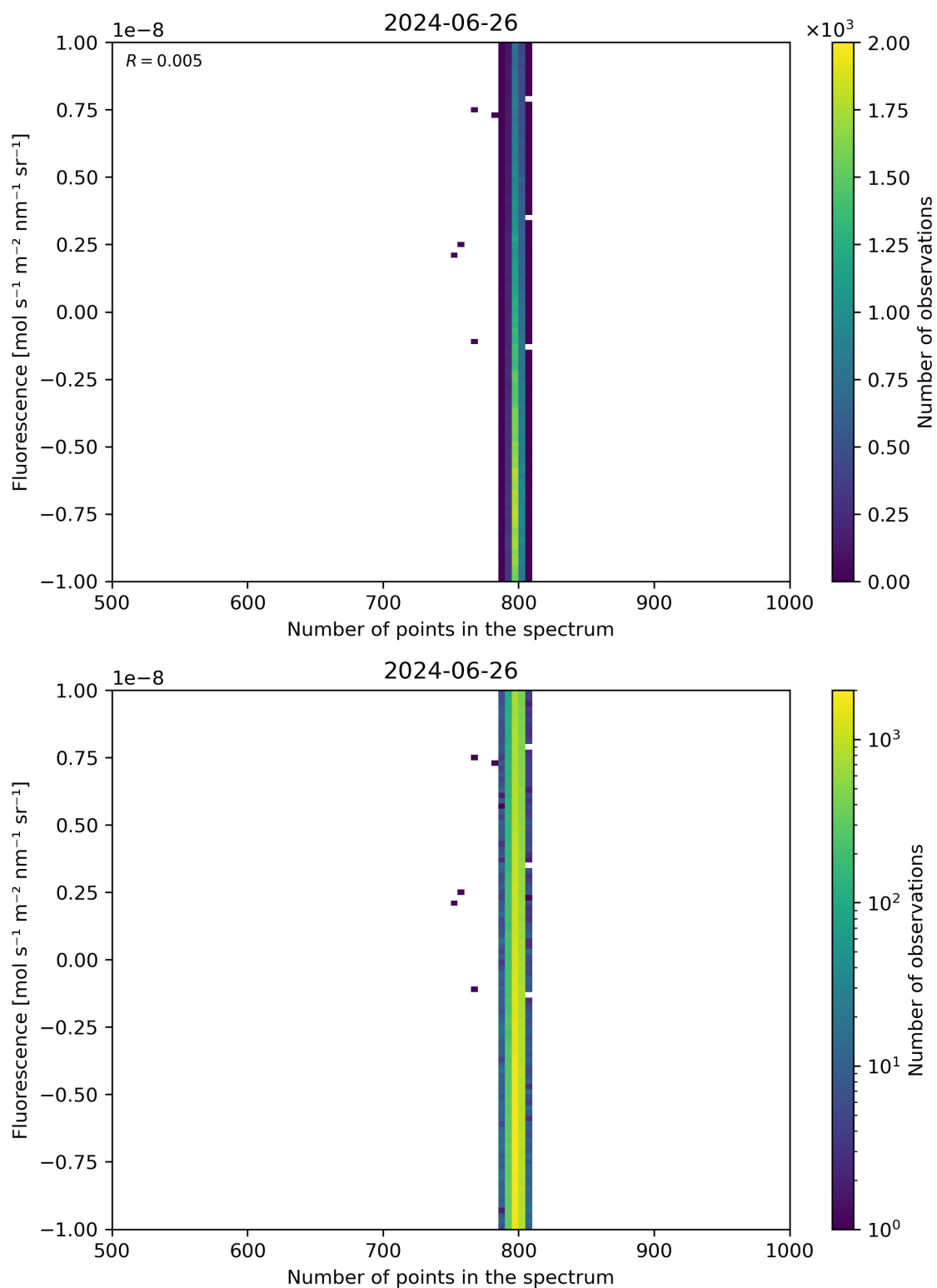
Figure 91: Scatter density plot of “Number of points in the spectrum” against “Fluorescence” for 2024-06-25 to 2024-06-27.
