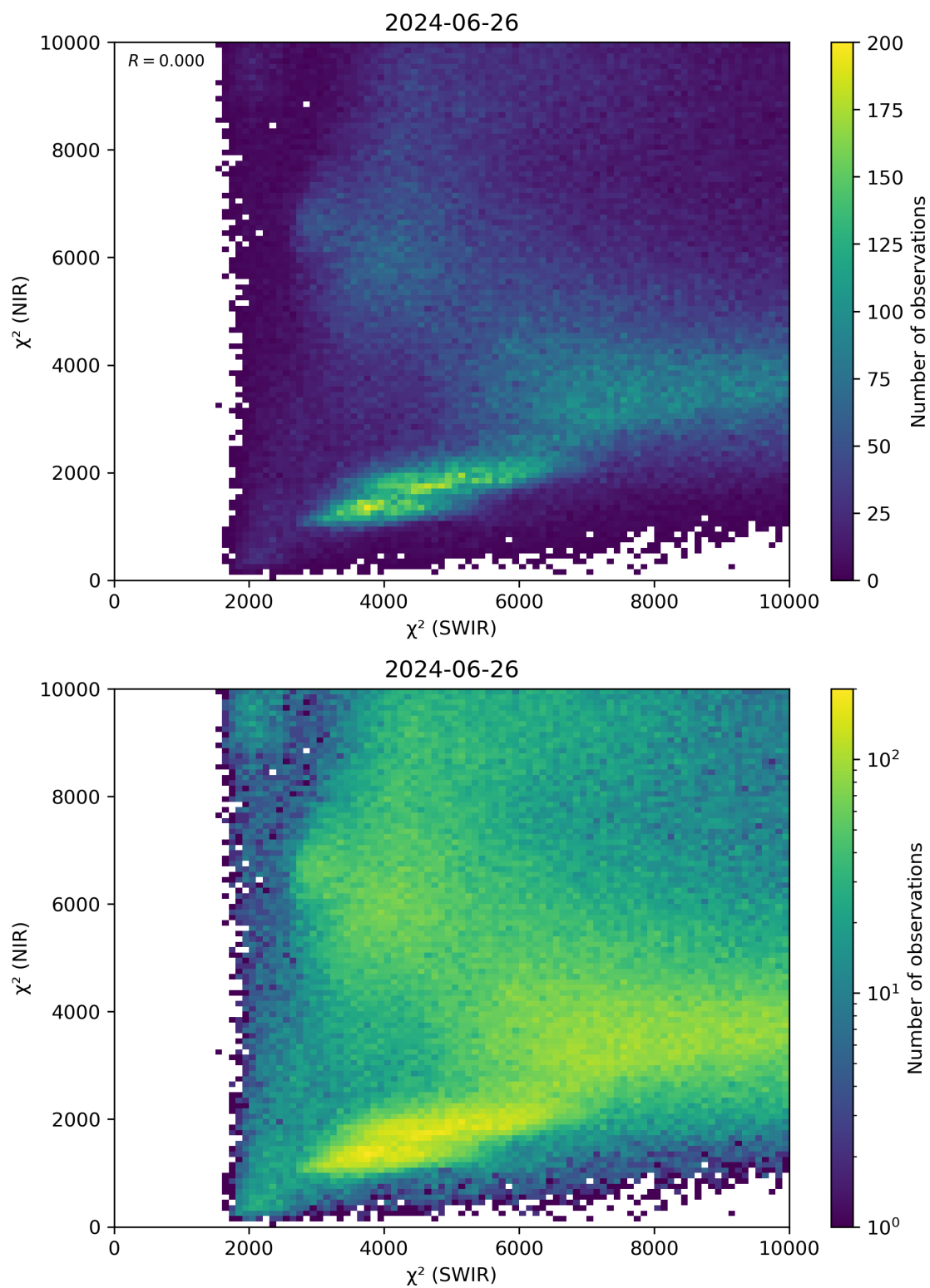
Figure 47: Scatter density plot of “ \chi^2 (SWIR)” against “ \chi^2 (NIR)” for 2024-06-25 to 2024-06-27.
