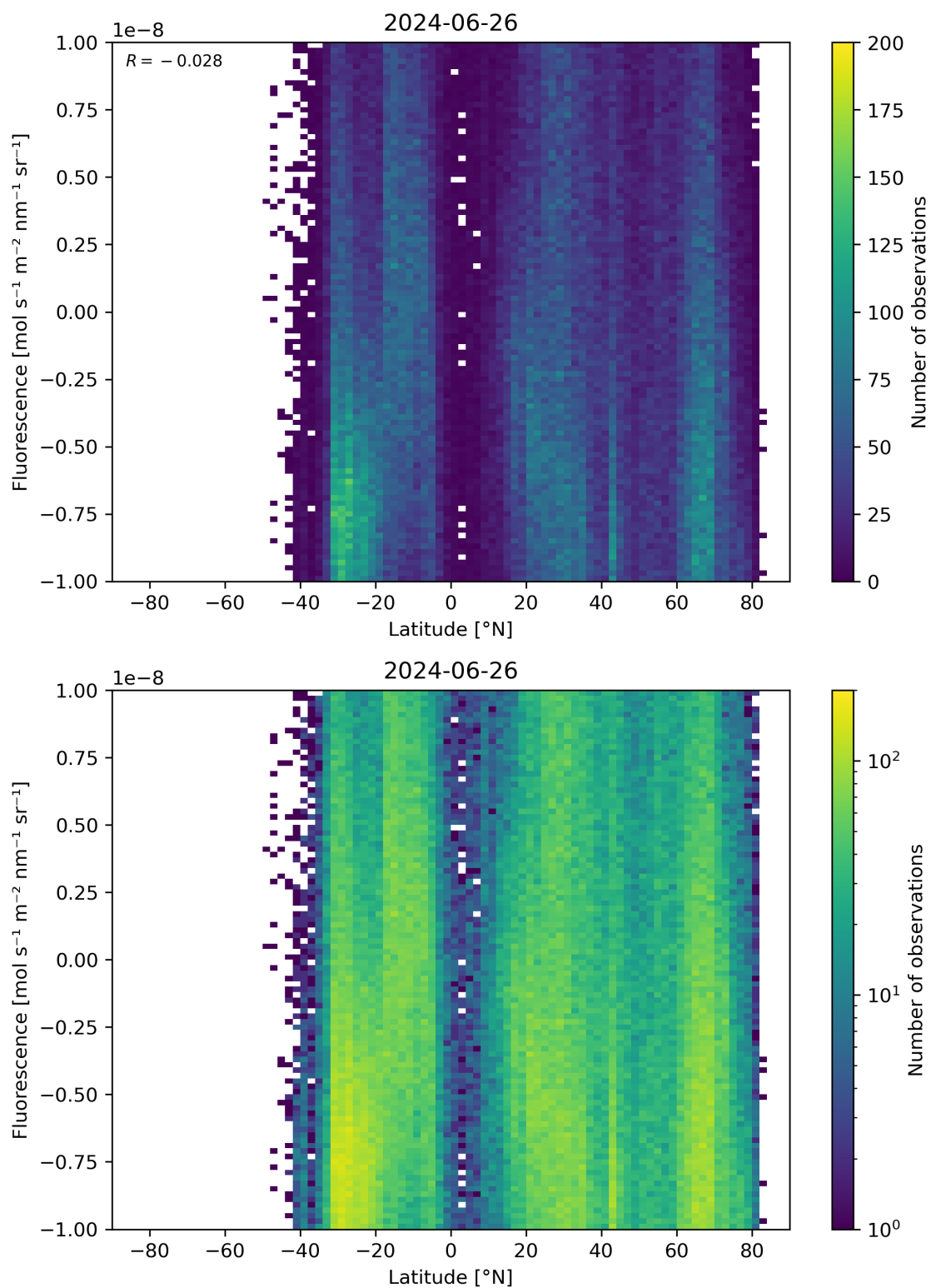
Figure 56: Scatter density plot of “Latitude” against “Fluorescence” for 2024-06-25 to 2024-06-27.
