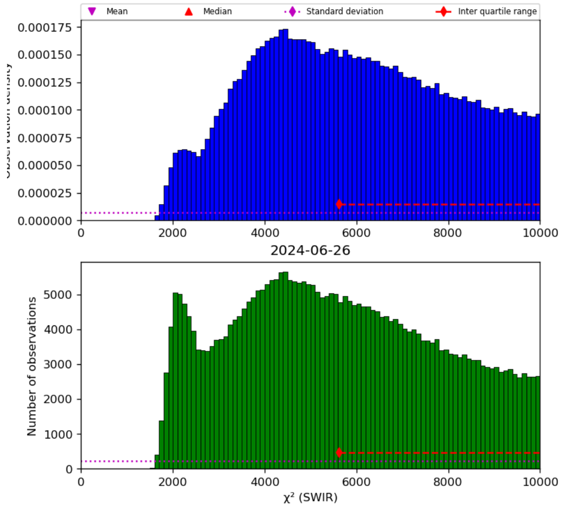
Figure 28: Histogram of “ \chi^2 (SWIR)” for 2024-06-25 to 2024-06-27
