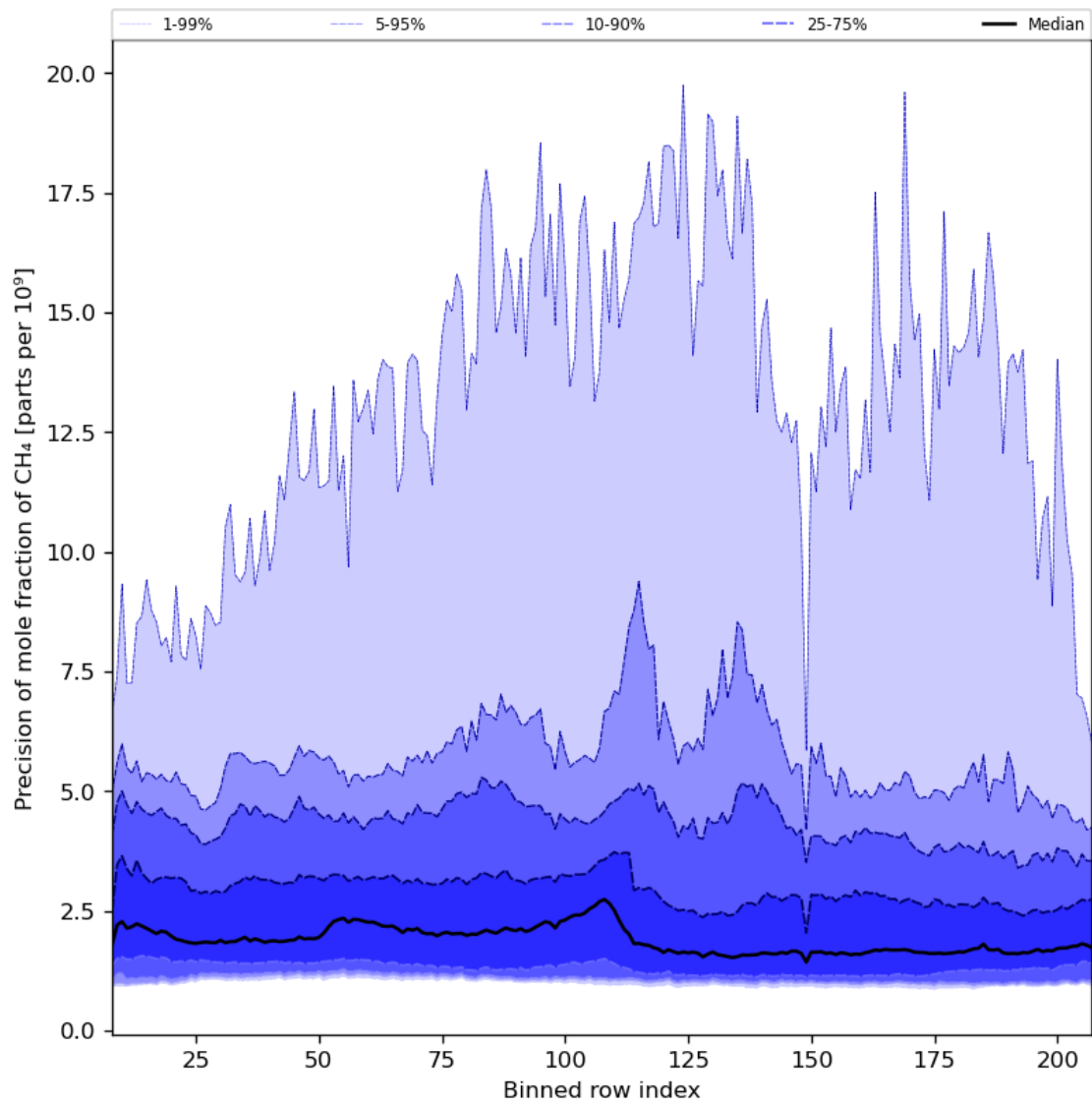
Figure 35: Along track statistics of “Precision of mole fraction of CH 4 ” for 2024-06-25 to 2024-06-27
