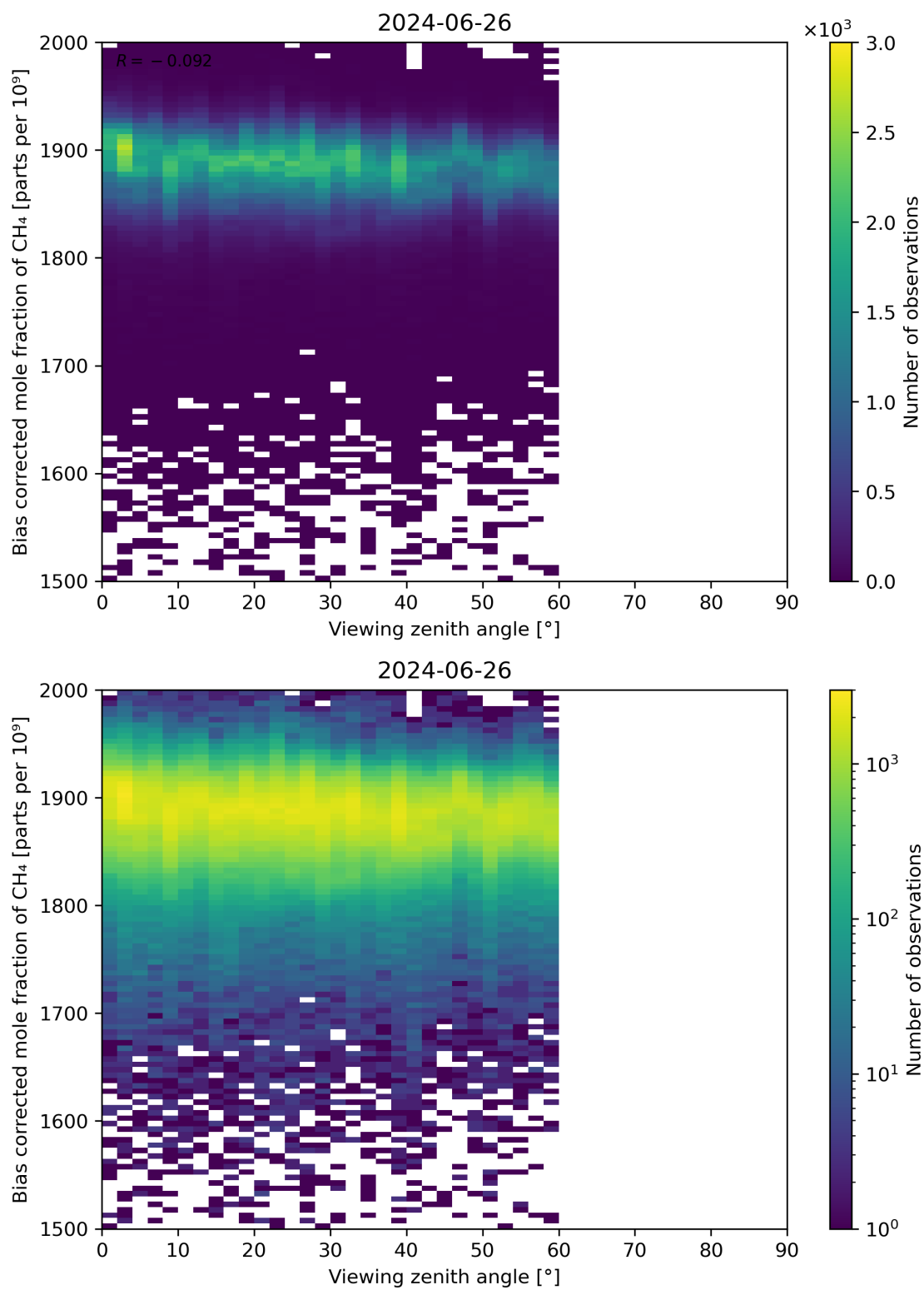
Figure 111: Scatter density plot of “Viewing zenith angle” against “Bias corrected mole fraction of CH 4 ” for 2024-06-25 to 2024-06-27.
