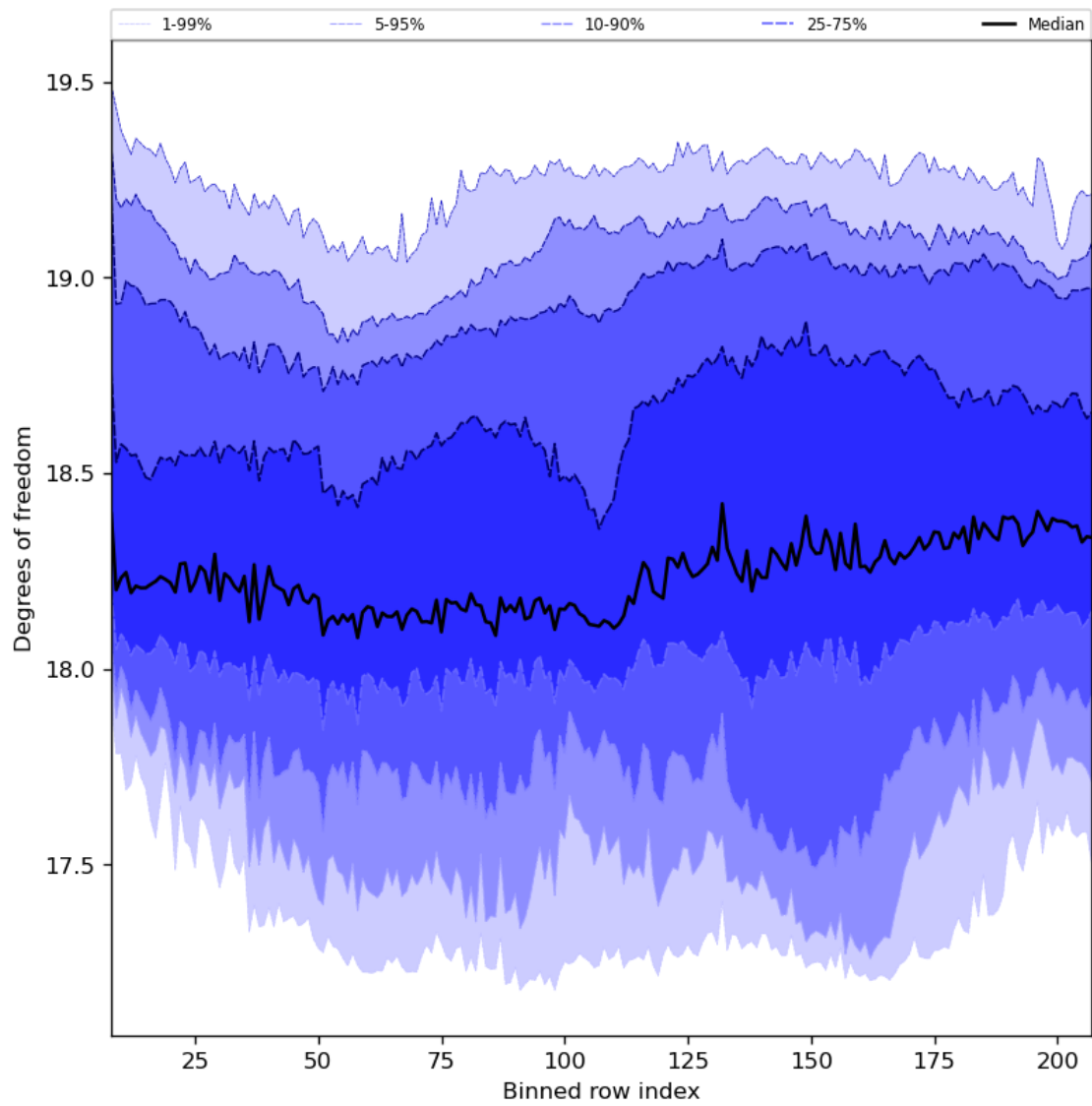
Figure 41: Along track statistics of “Degrees of freedom” for 2024-06-25 to 2024-06-27
