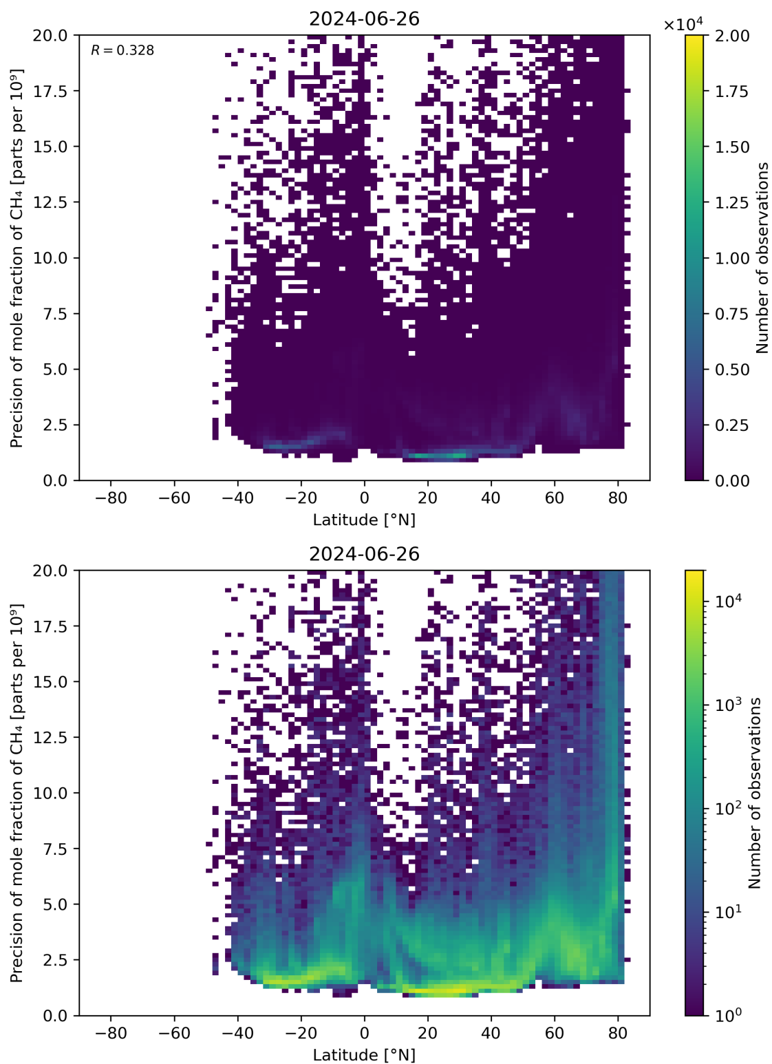
Figure 59: Scatter density plot of “Latitude” against “Precision of mole fraction of \text{CH}_4 ” for 2024-06-25 to 2024-06-27.
