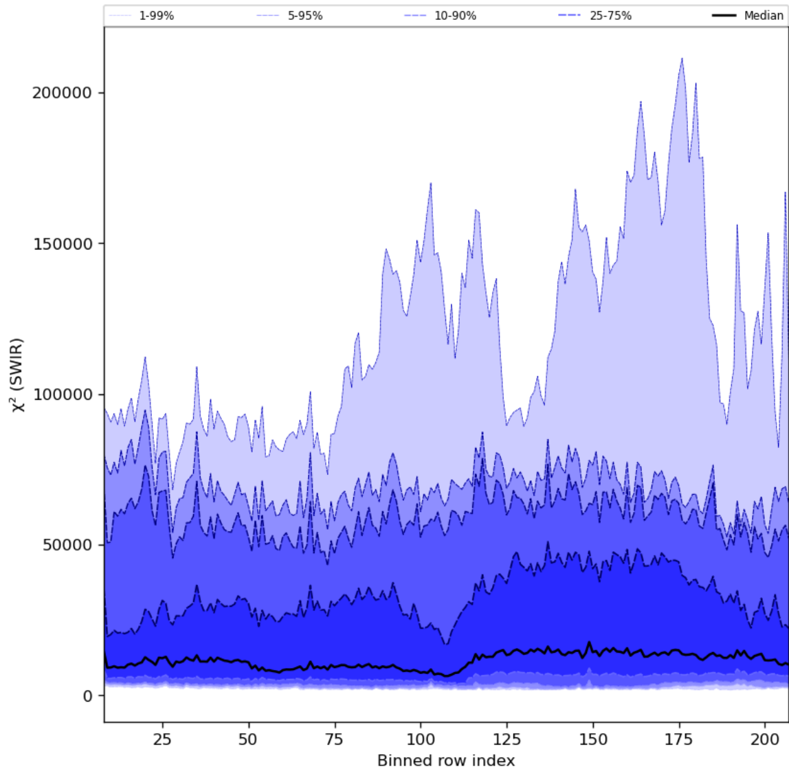
Figure 39: Along track statistics of “ \chi^2 (SWIR)” for 2024-06-25 to 2024-06-27
