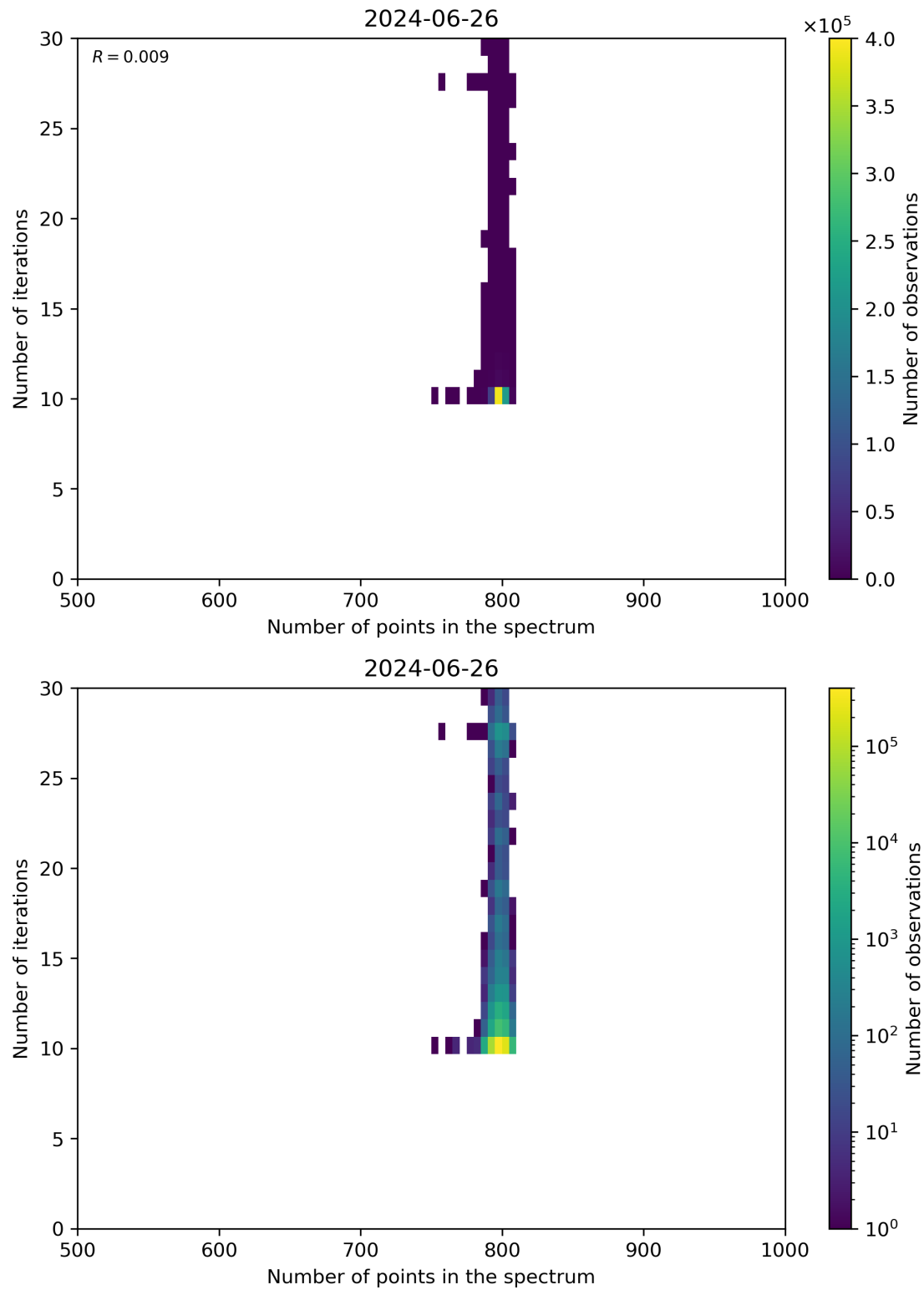
Figure 92: Scatter density plot of “Number of points in the spectrum” against “Number of iterations” for 2024-06-25 to 2024-06-27.
