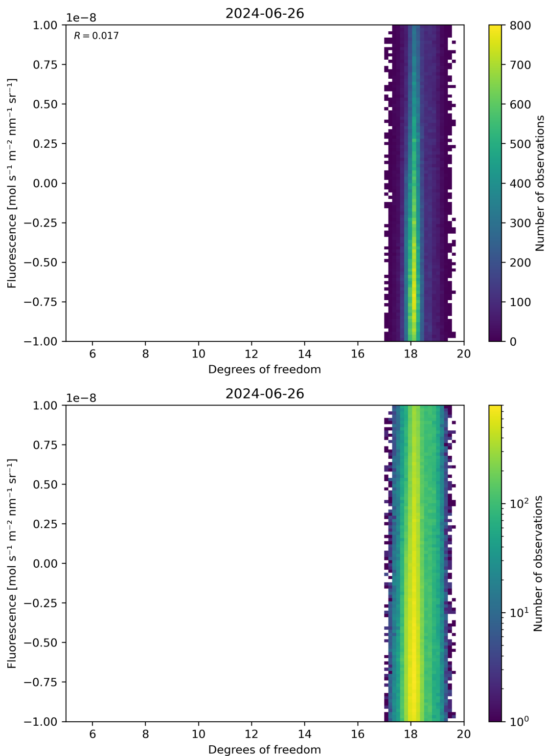
Figure 51: Scatter density plot of “Degrees of freedom” against “Fluorescence” for 2024-06-25 to 2024-06-27.
