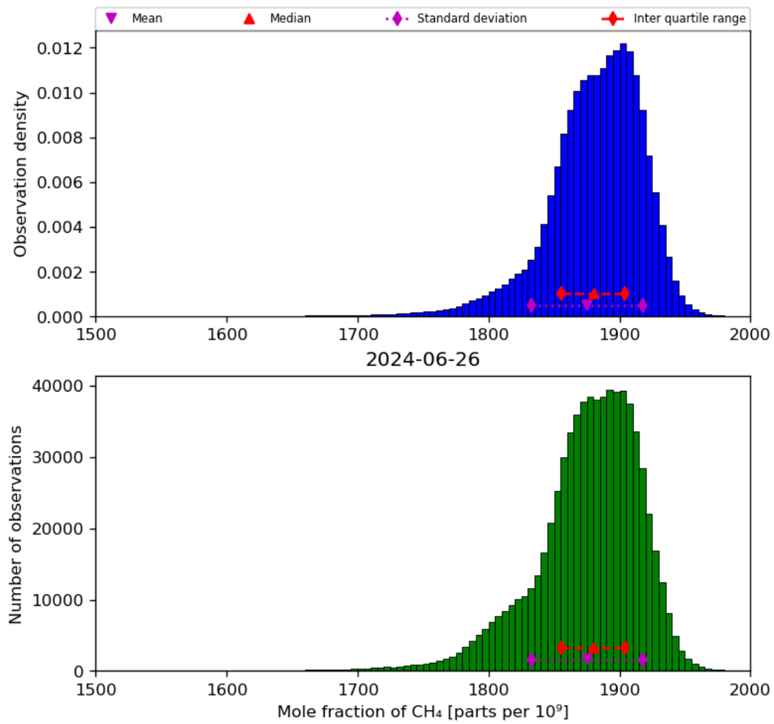
Figure 23: Histogram of “Mole fraction of CH 4 ” for 2024-06-25 to 2024-06-27
