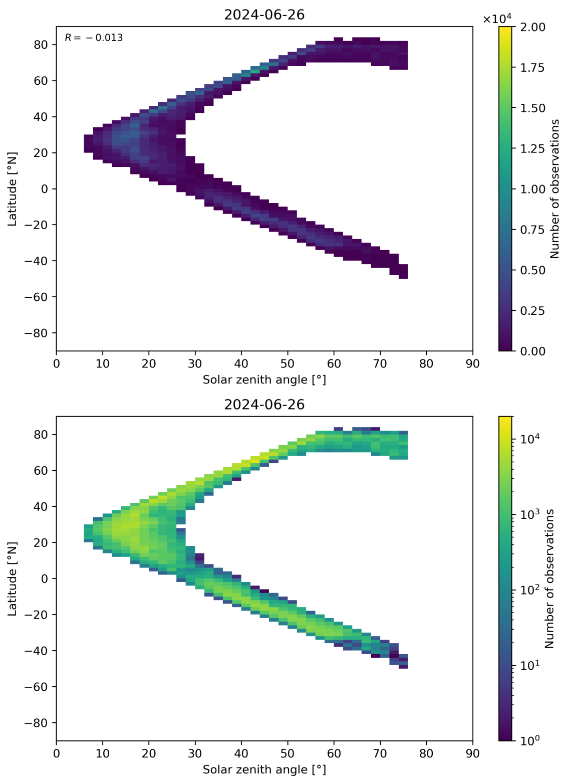
Figure 98: Scatter density plot of “Solar zenith angle” against “Latitude” for 2024-06-25 to 2024-06-27.
