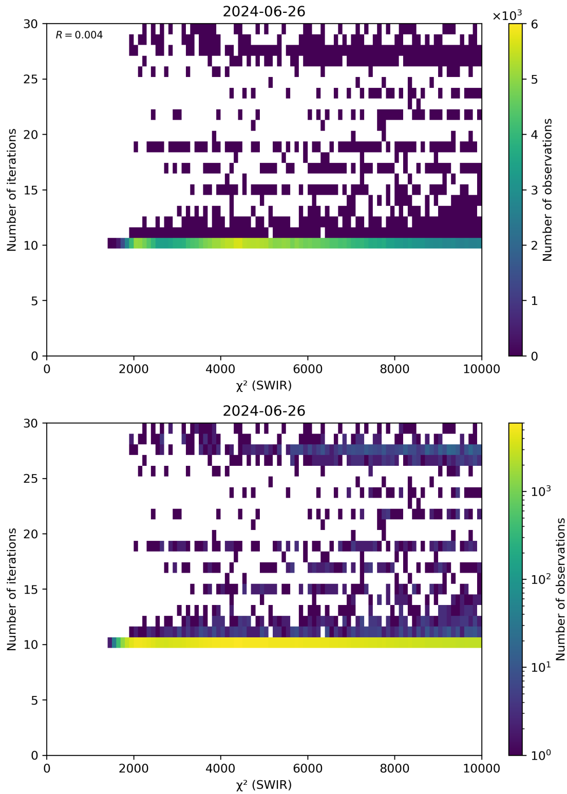
Figure 50: Scatter density plot of “ \chi^2 (SWIR)” against “Number of iterations” for 2024-06-25 to 2024-06-27.
