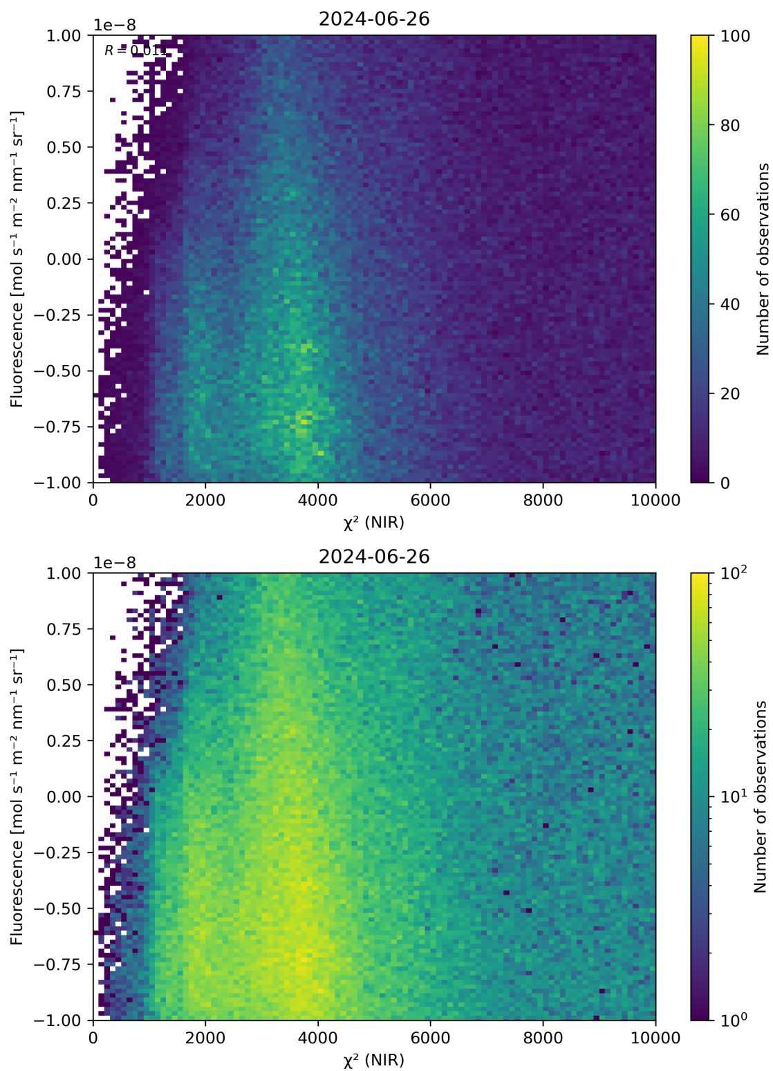
Figure 45: Scatter density plot of “ \chi^2 (NIR)” against “Fluorescence” for 2024-06-25 to 2024-06-27.
