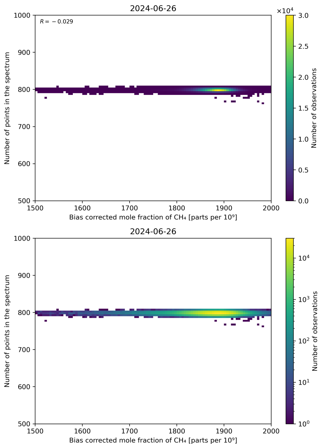
Figure 68: Scatter density plot of “Bias corrected mole fraction of CH 4 ” against “Number of points in the spectrum” for 2024-06-25 to 2024-06-27.
