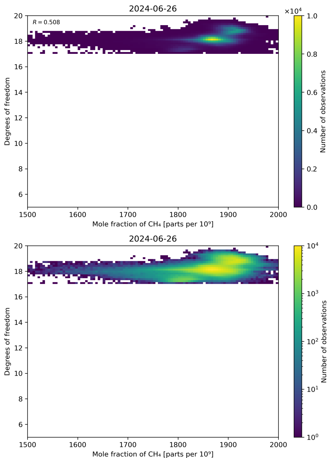
Figure 72: Scatter density plot of “Mole fraction of CH 4 ” against “Degrees of freedom” for 2024-06-25 to 2024-06-27.
