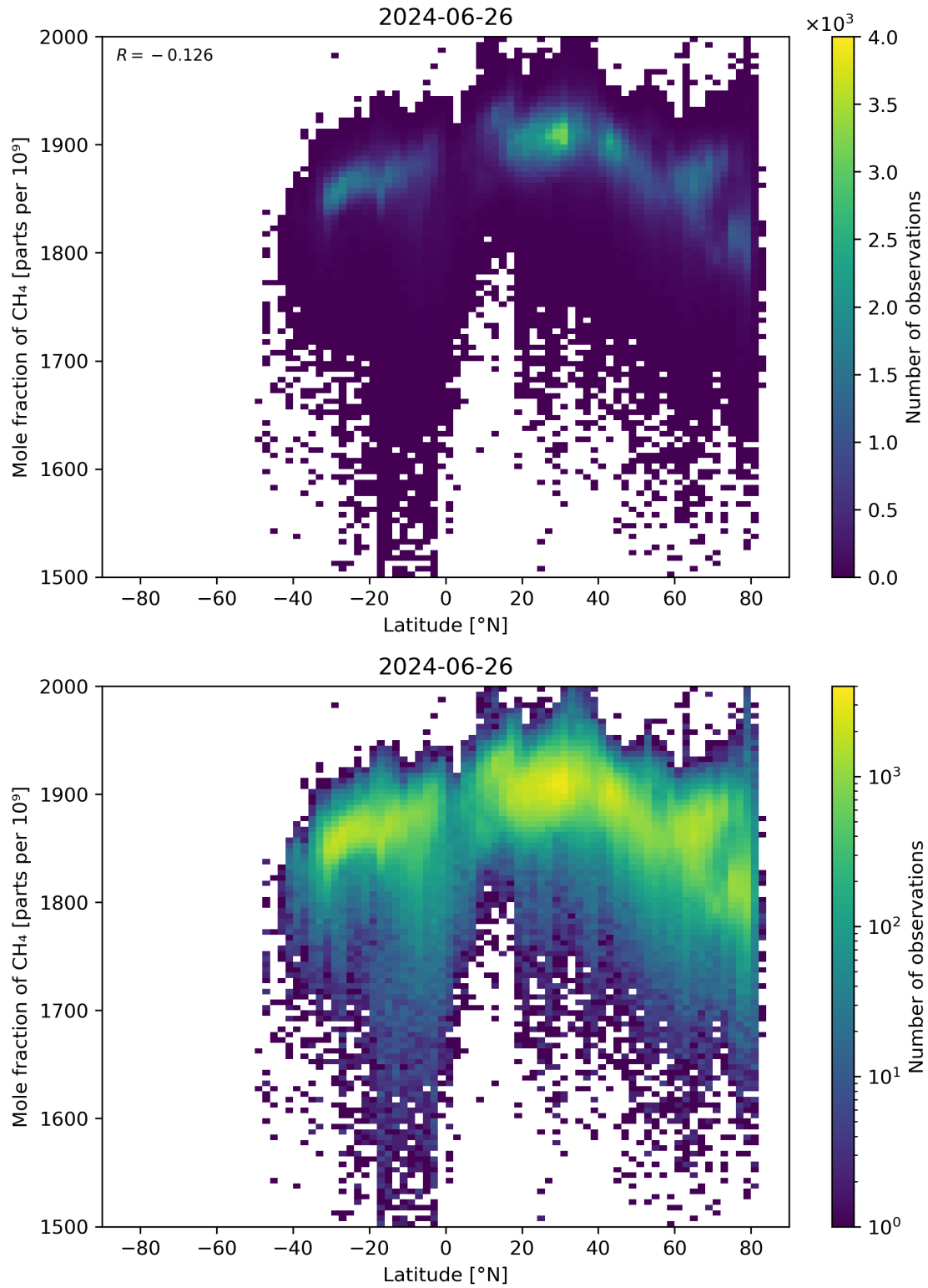
Figure 57: Scatter density plot of “Latitude” against “Mole fraction of CH 4 ” for 2024-06-25 to 2024-06-27.
