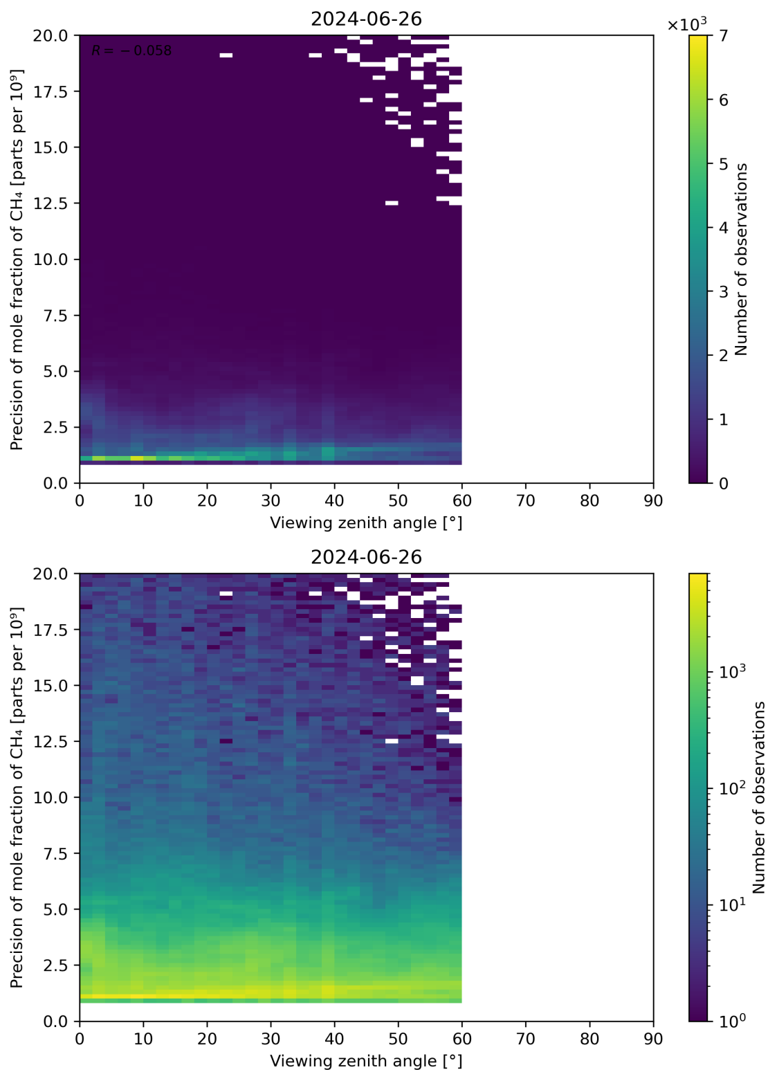
Figure 112: Scatter density plot of “Viewing zenith angle” against “Precision of mole fraction of CH 4 ” for 2024-06-25 to 2024-06-27.
