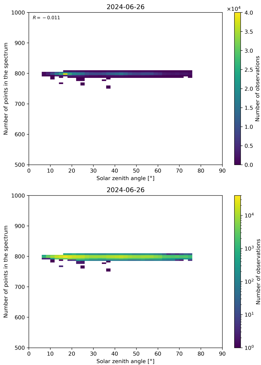
Figure 103: Scatter density plot of “Solar zenith angle” against “Number of points in the spectrum” for 2024-06-25 to 2024-06-27.
