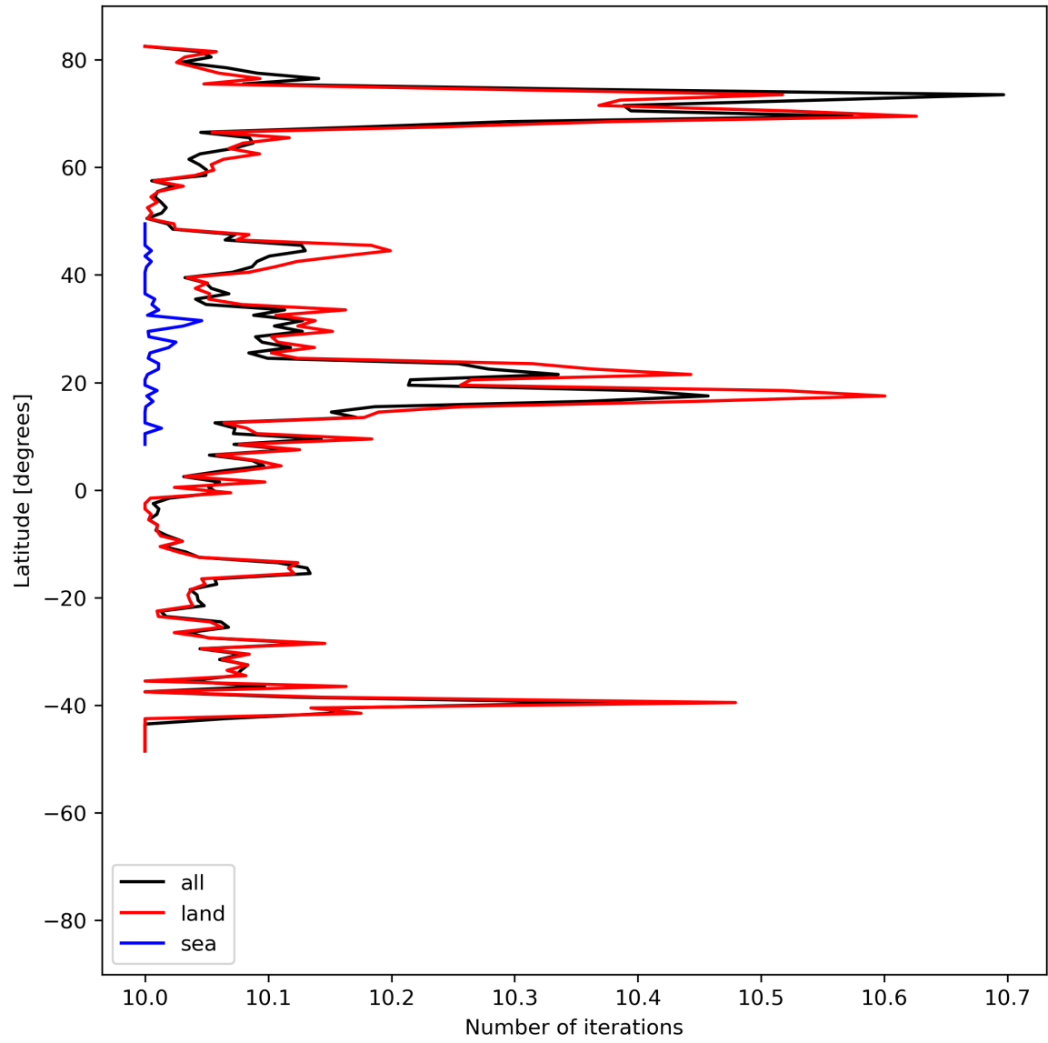
Figure 20: Zonal average of “Number of iterations” for 2024-06-25 to 2024-06-27.
