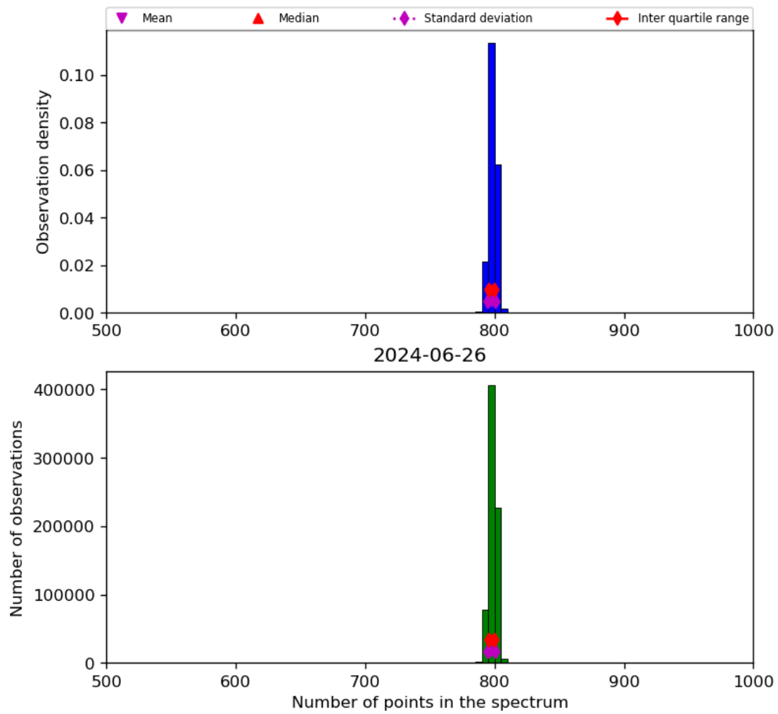
Figure 26: Histogram of “Number of points in the spectrum” for 2024-06-25 to 2024-06-27
