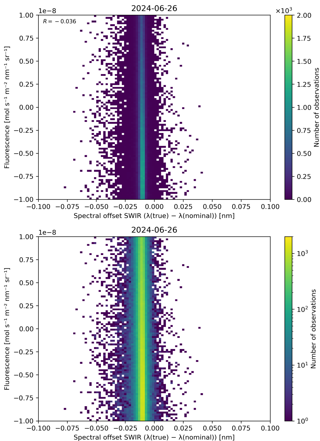
Figure 120: Scatter density plot of “Spectral offset SWIR ( \lambda(\text{true}) - \lambda(\text{nominal}) )” against “Fluorescence” for 2024-06-25 to 2024-06-27.
