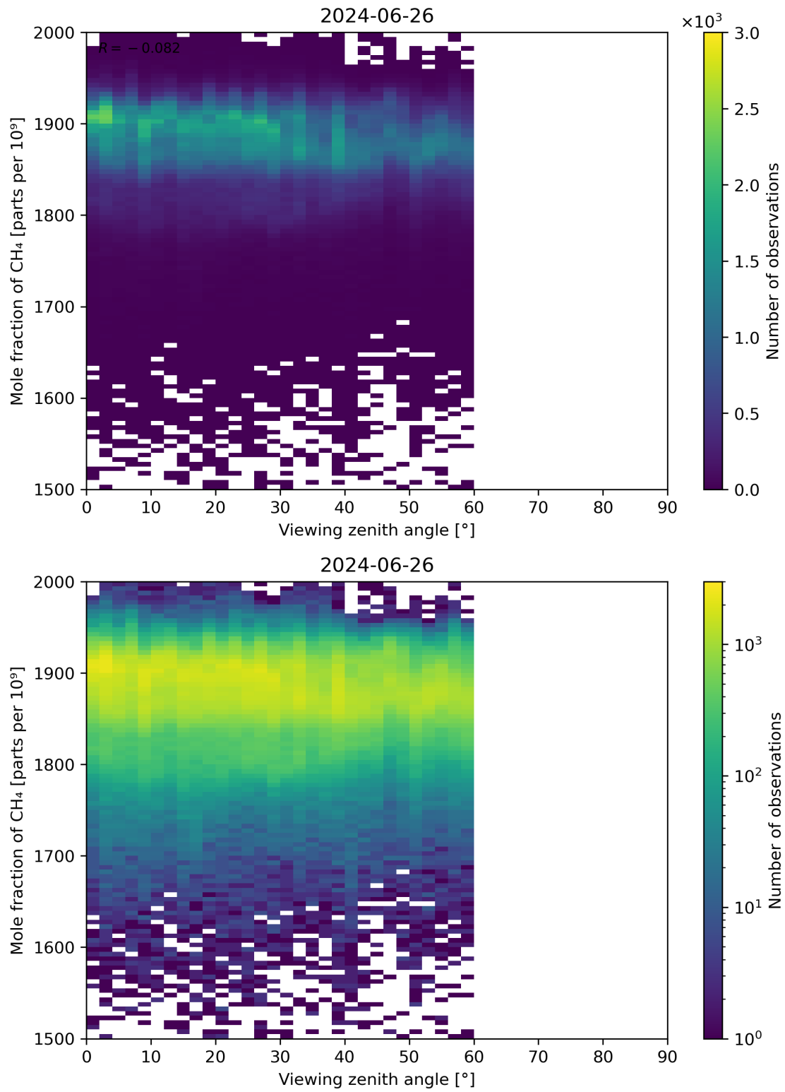
Figure 110: Scatter density plot of “Viewing zenith angle” against “Mole fraction of CH 4 ” for 2024-06-25 to 2024-06-27.
