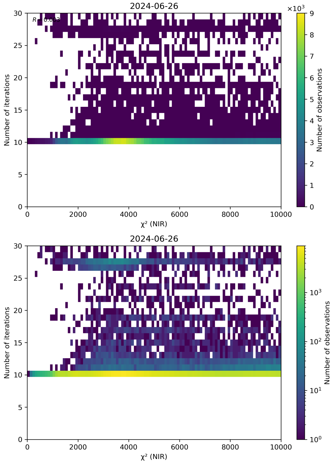
Figure 46: Scatter density plot of “ \chi^2 (NIR)” against “Number of iterations” for 2024-06-25 to 2024-06-27.
