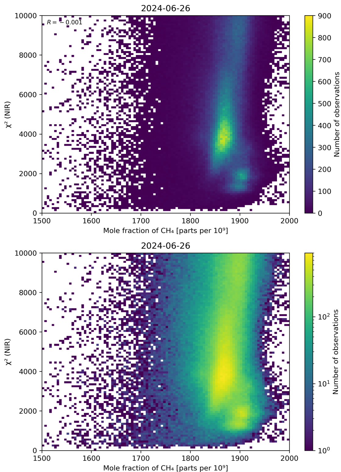
Figure 70: Scatter density plot of “Mole fraction of CH 4 ” against “ \chi^2 (NIR)” for 2024-06-25 to 2024-06-27.
