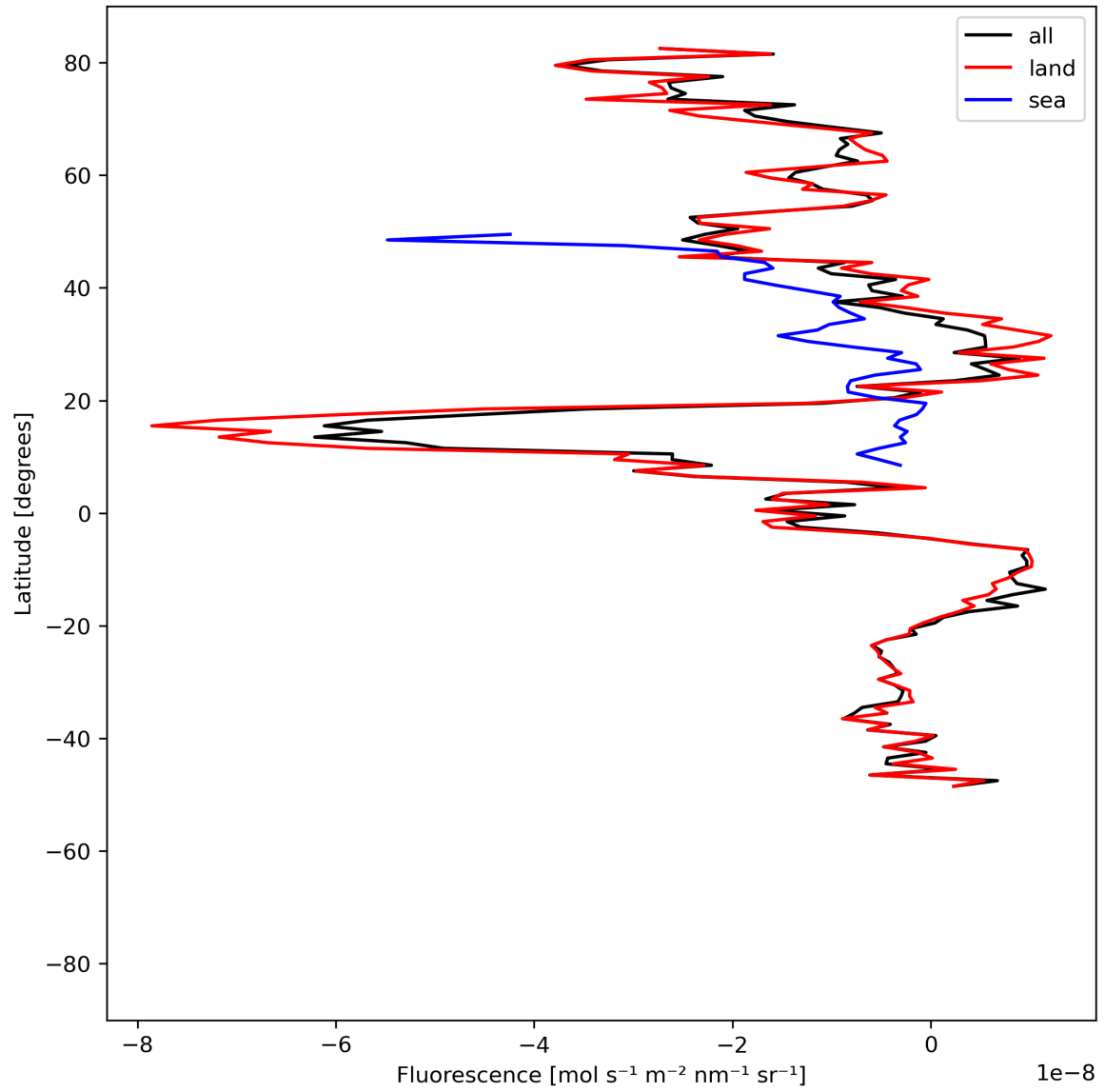
Figure 21: Zonal average of “Fluorescence” for 2024-06-25 to 2024-06-27.
