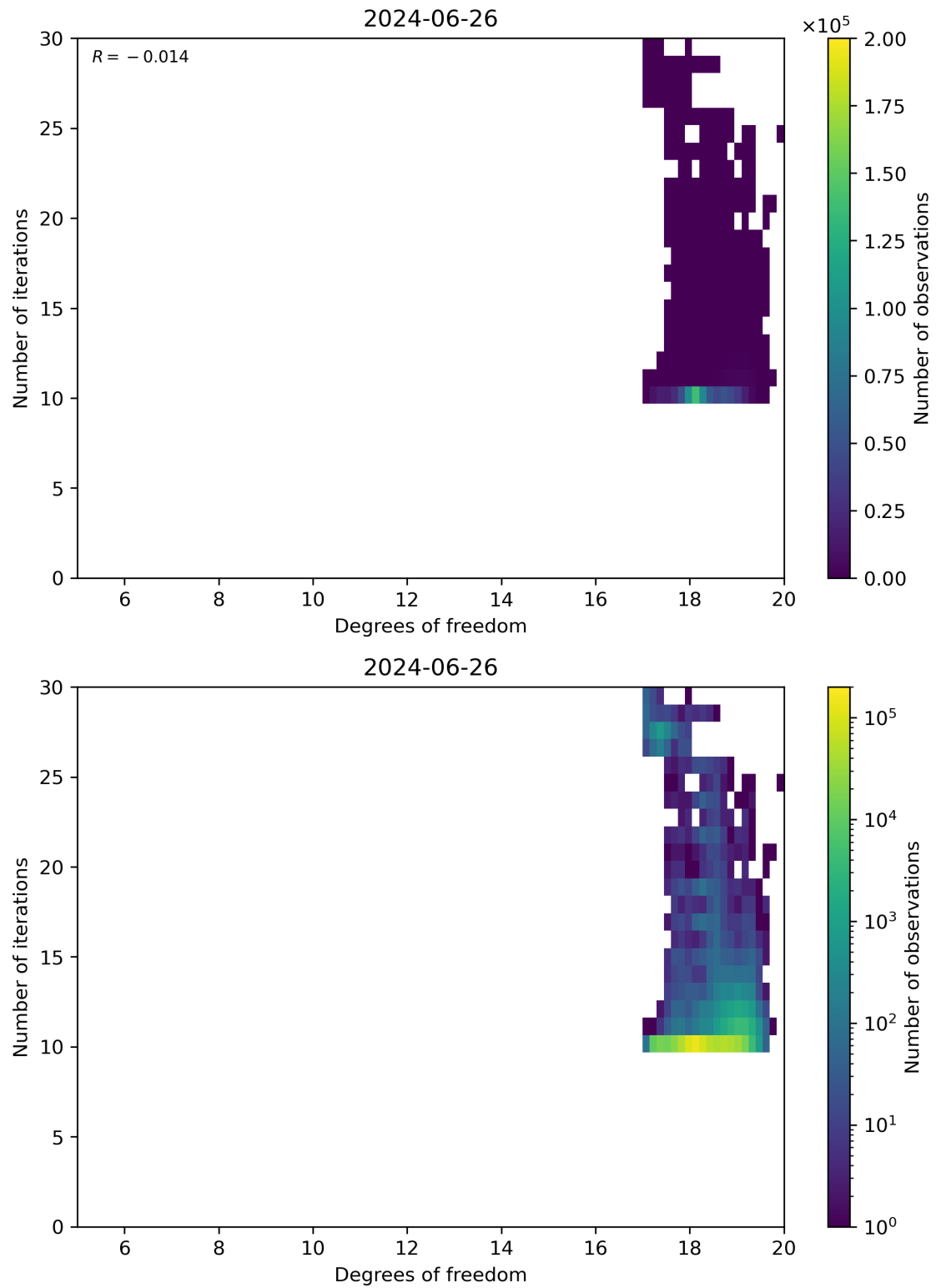
Figure 52: Scatter density plot of “Degrees of freedom” against “Number of iterations” for 2024-06-25 to 2024-06-27.
