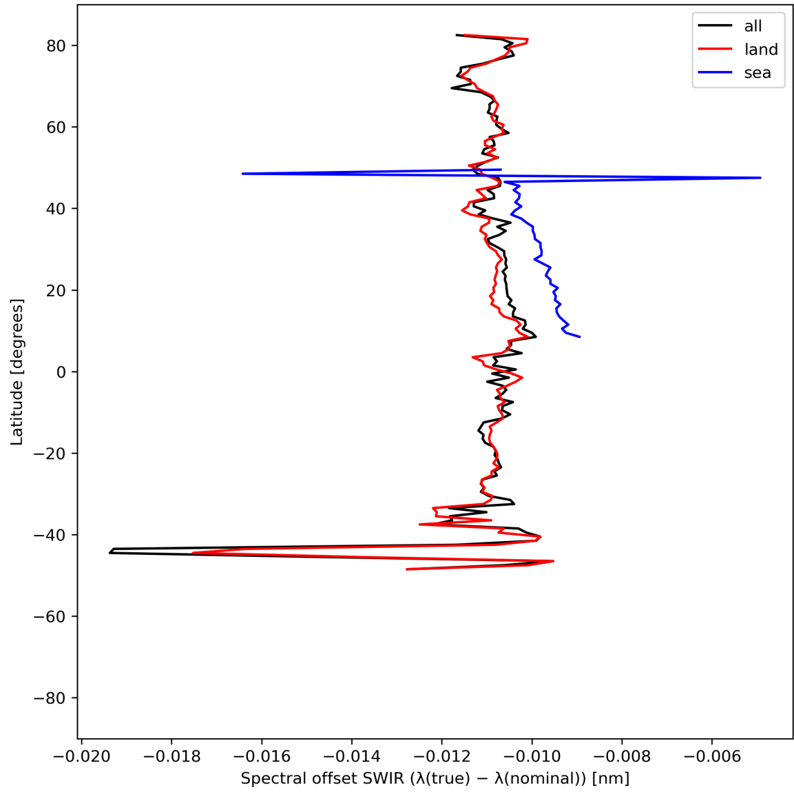
Figure 16: Zonal average of “Spectral offset SWIR ( \lambda(\text{true}) - \lambda(\text{nominal}) )” for 2024-06-25 to 2024-06-27.
