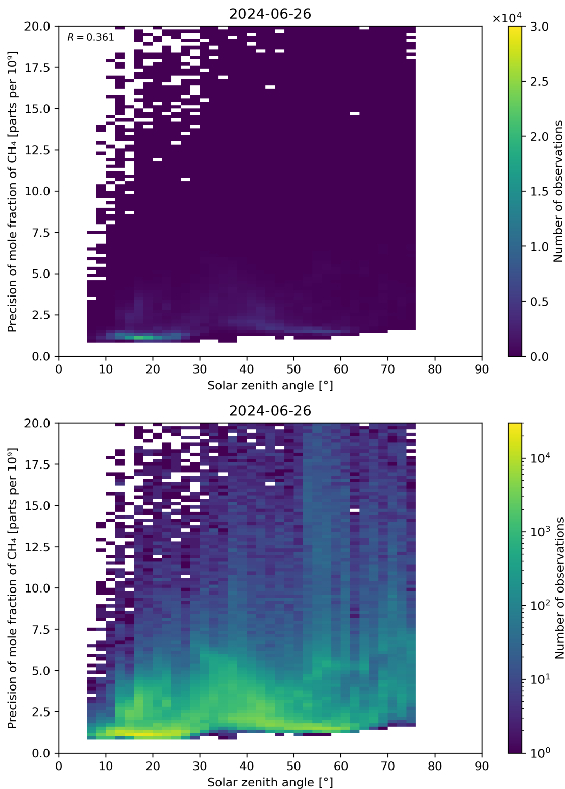
Figure 101: Scatter density plot of “Solar zenith angle” against “Precision of mole fraction of CH 4 ” for 2024-06-25 to 2024-06-27.
