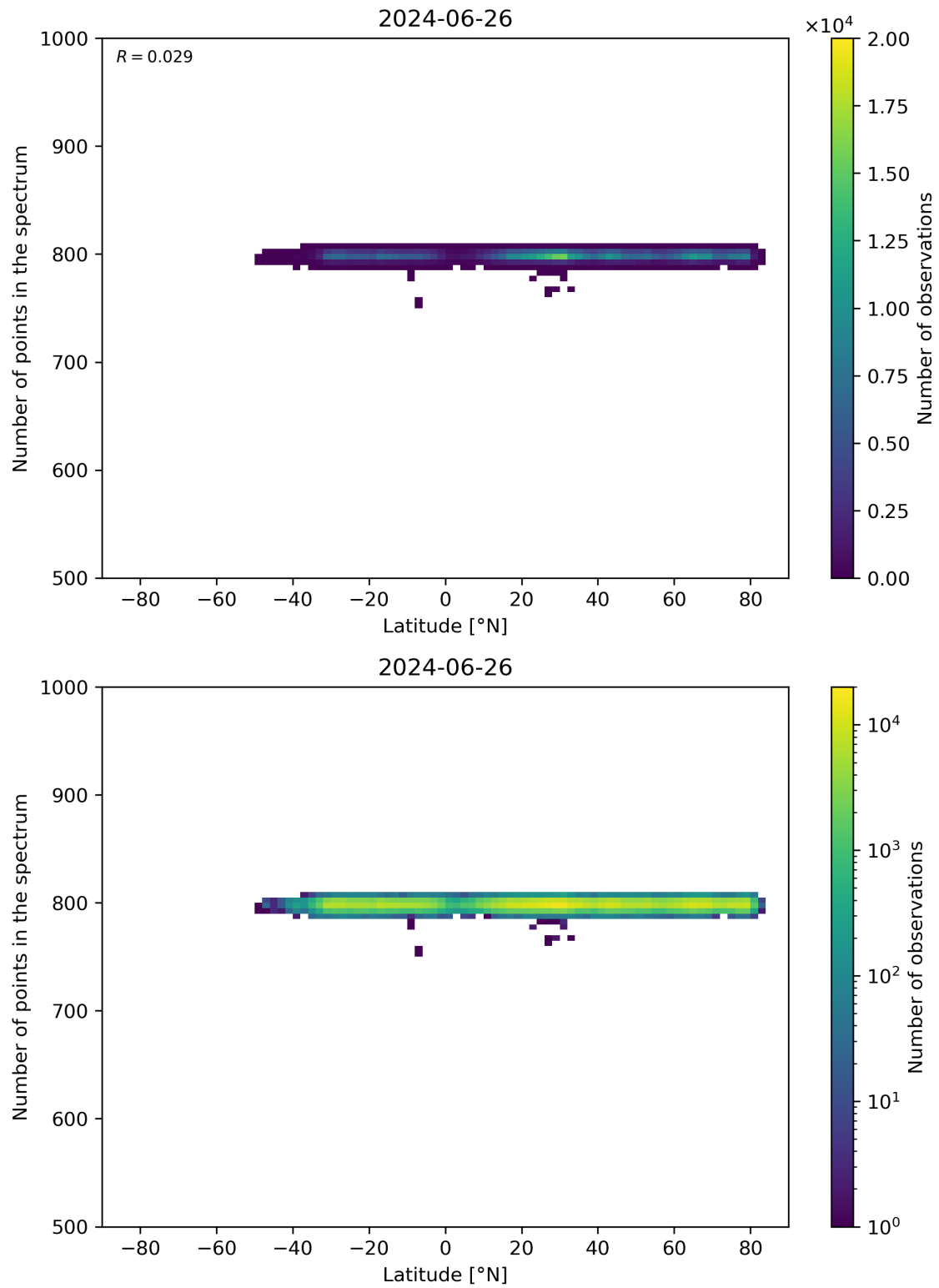
Figure 61: Scatter density plot of “Latitude” against “Number of points in the spectrum” for 2024-06-25 to 2024-06-27.
