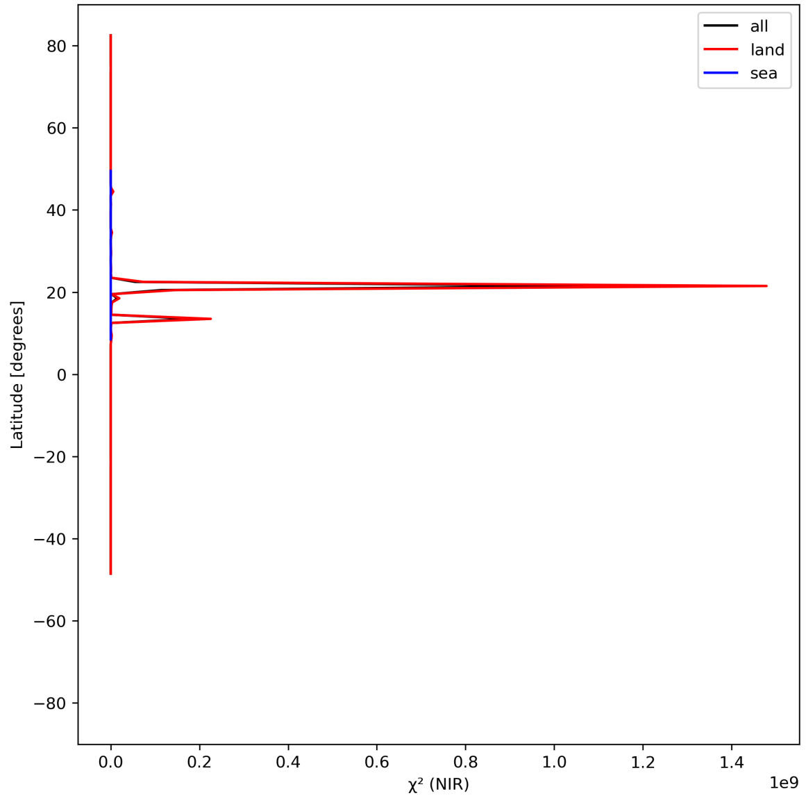
Figure 18: Zonal average of “ \chi^2 (NIR)” for 2024-06-25 to 2024-06-27.
