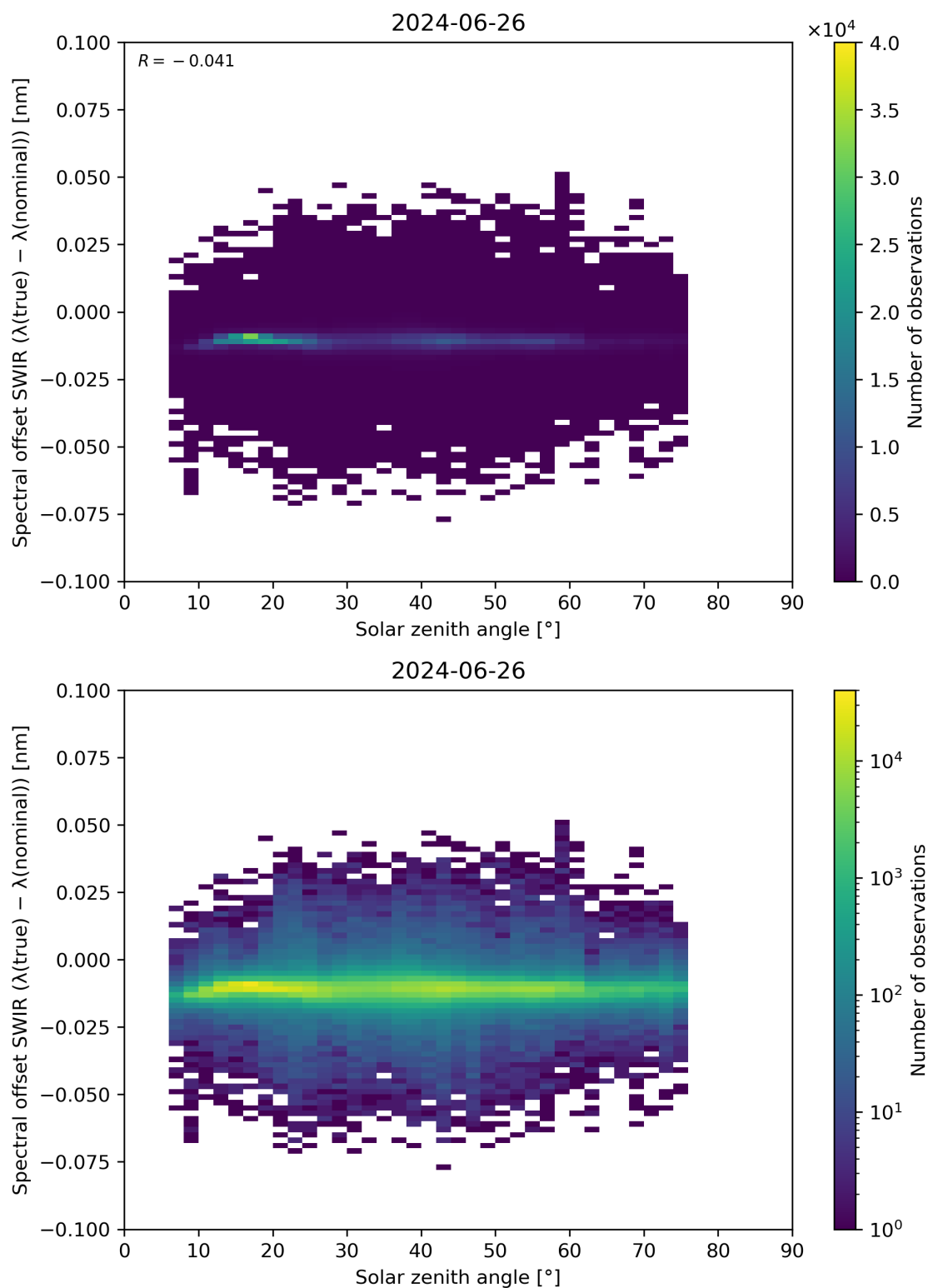
Figure 104: Scatter density plot of “Solar zenith angle” against “Spectral offset SWIR ( \lambda(\text{true}) - \lambda(\text{nominal}) )” for 2024-06-25 to 2024-06-27.
