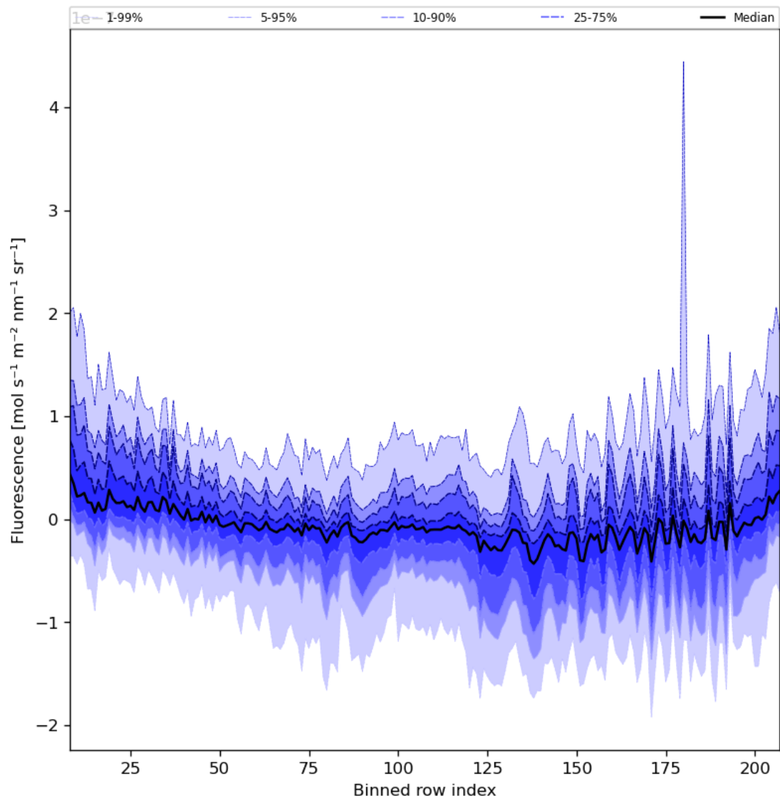
Figure 43: Along track statistics of “Fluorescence” for 2024-06-25 to 2024-06-27
