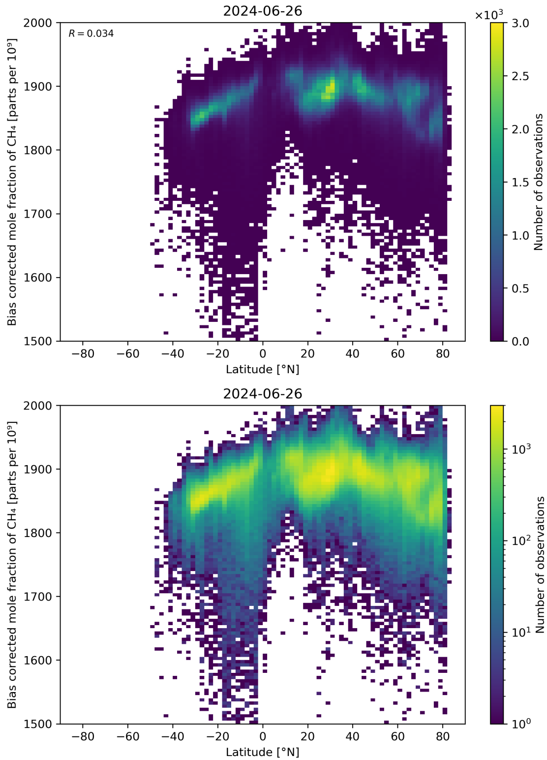
Figure 58: Scatter density plot of “Latitude” against “Bias corrected mole fraction of CH 4 ” for 2024-06-25 to 2024-06-27.
