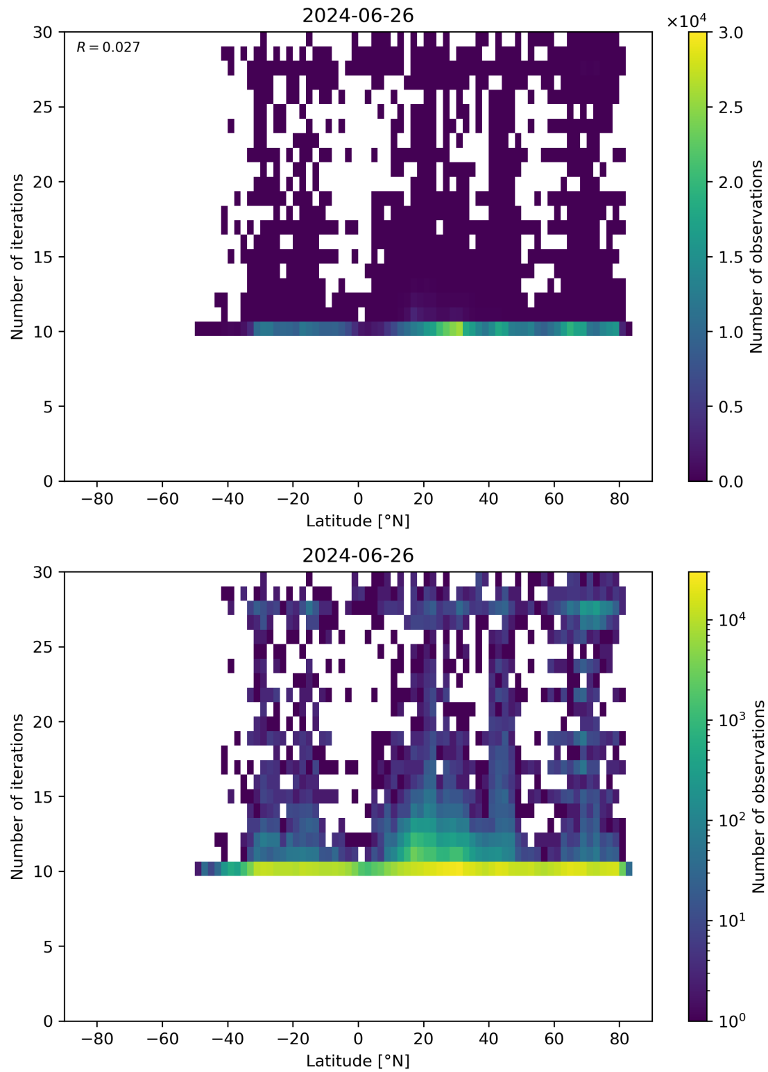
Figure 60: Scatter density plot of “Latitude” against “Number of iterations” for 2024-06-25 to 2024-06-27.
