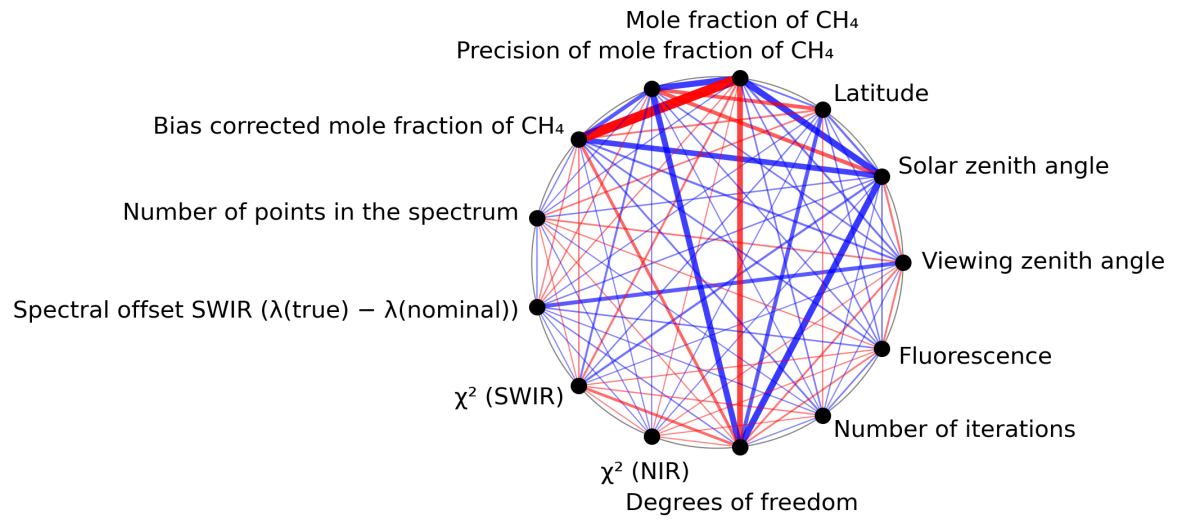
Figure 1: Map of correlation graph for 2024-06-26 to 2024-06-28.
