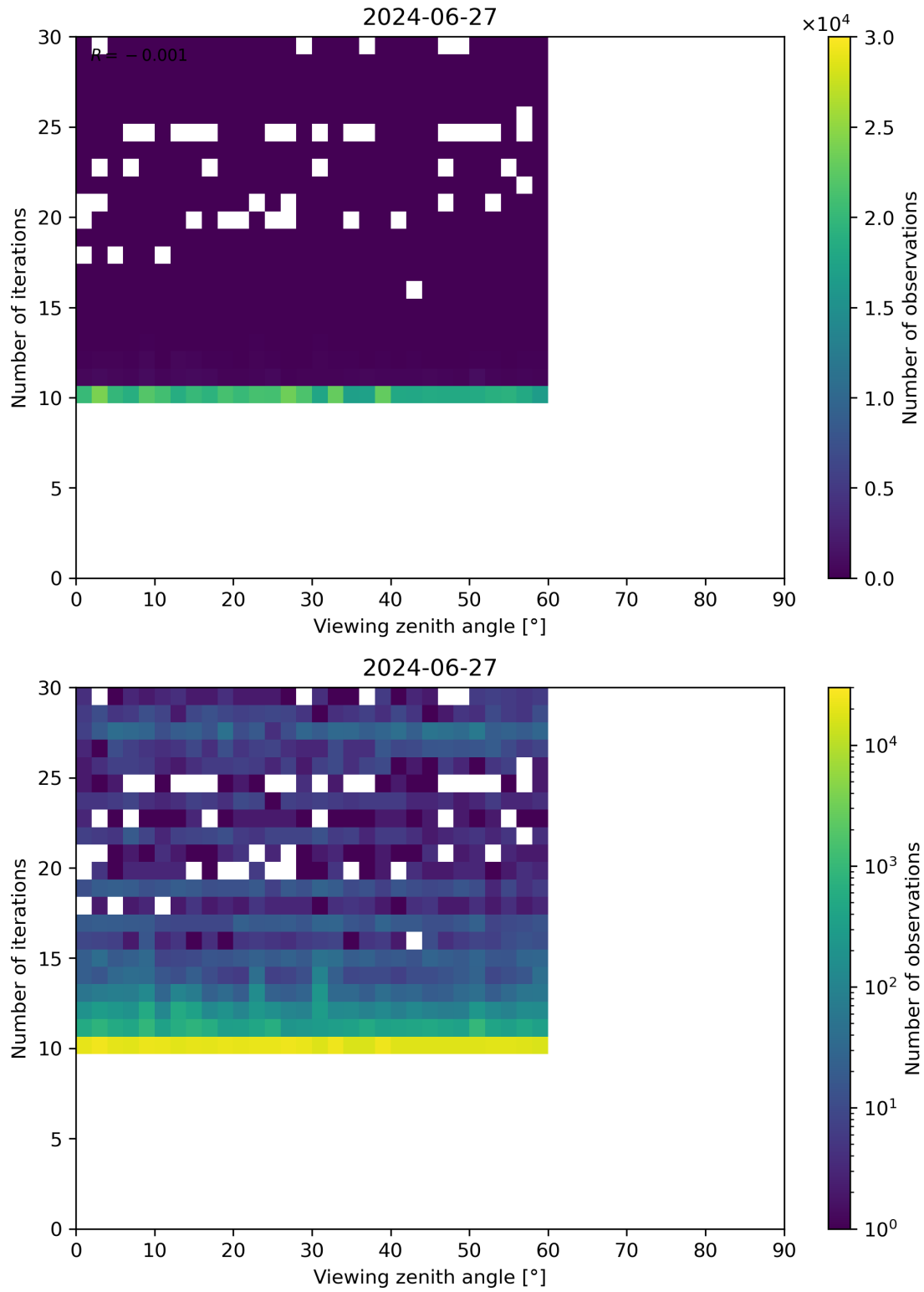
Figure 113: Scatter density plot of “Viewing zenith angle” against “Number of iterations” for 2024-06-26 to 2024-06-28.
