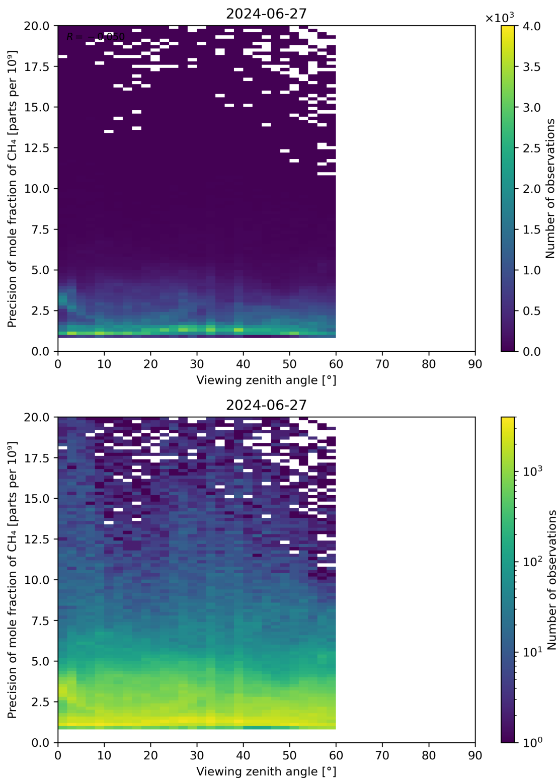
Figure 112: Scatter density plot of “Viewing zenith angle” against “Precision of mole fraction of CH 4 ” for 2024-06-26 to 2024-06-28.
