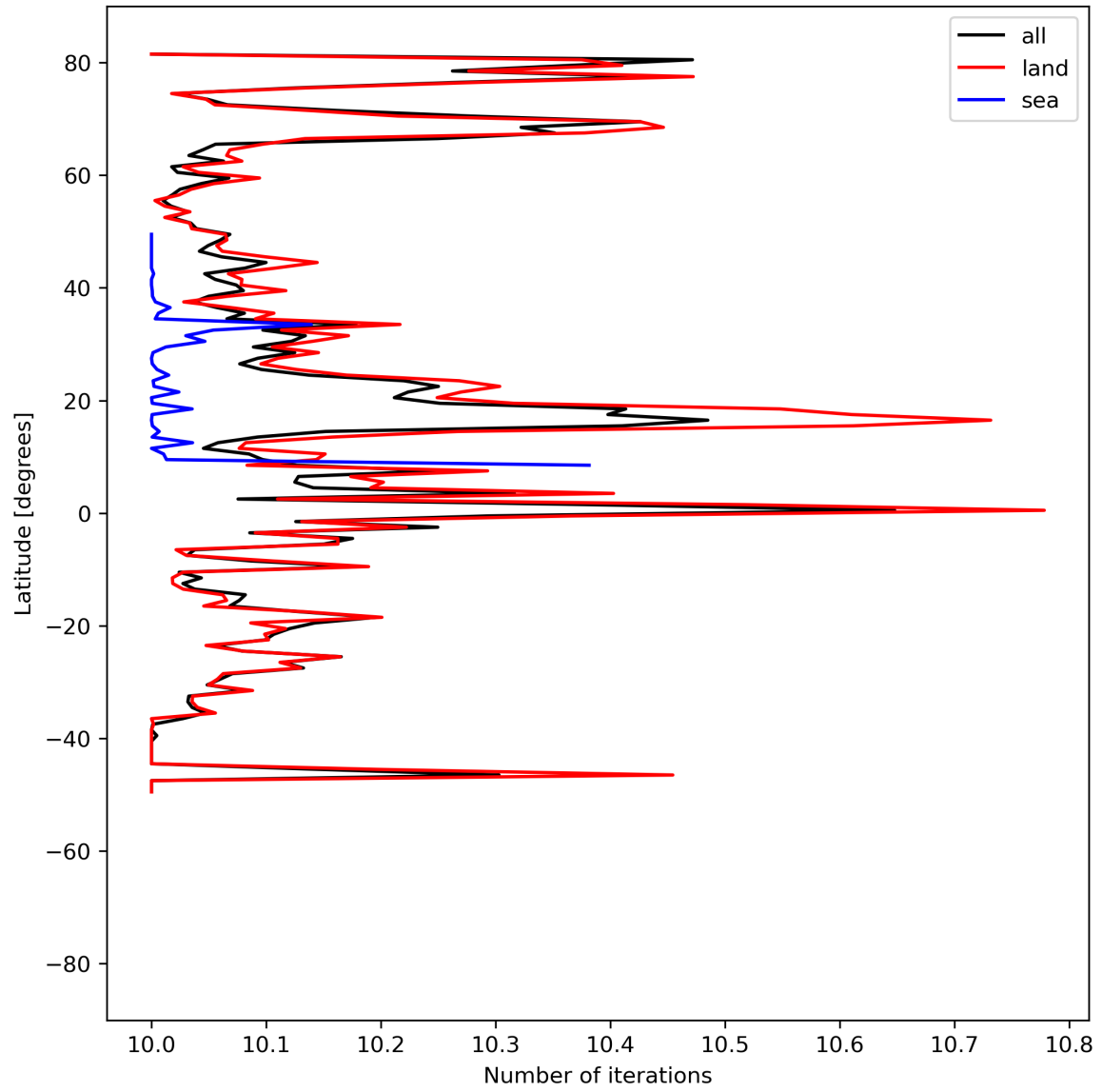
Figure 20: Zonal average of “Number of iterations” for 2024-06-26 to 2024-06-28.
