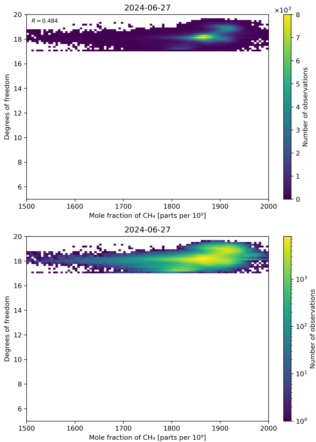
Figure 72: Scatter density plot of “Mole fraction of CH 4 ” against “Degrees of freedom” for 2024-06-26 to 2024-06-28.
