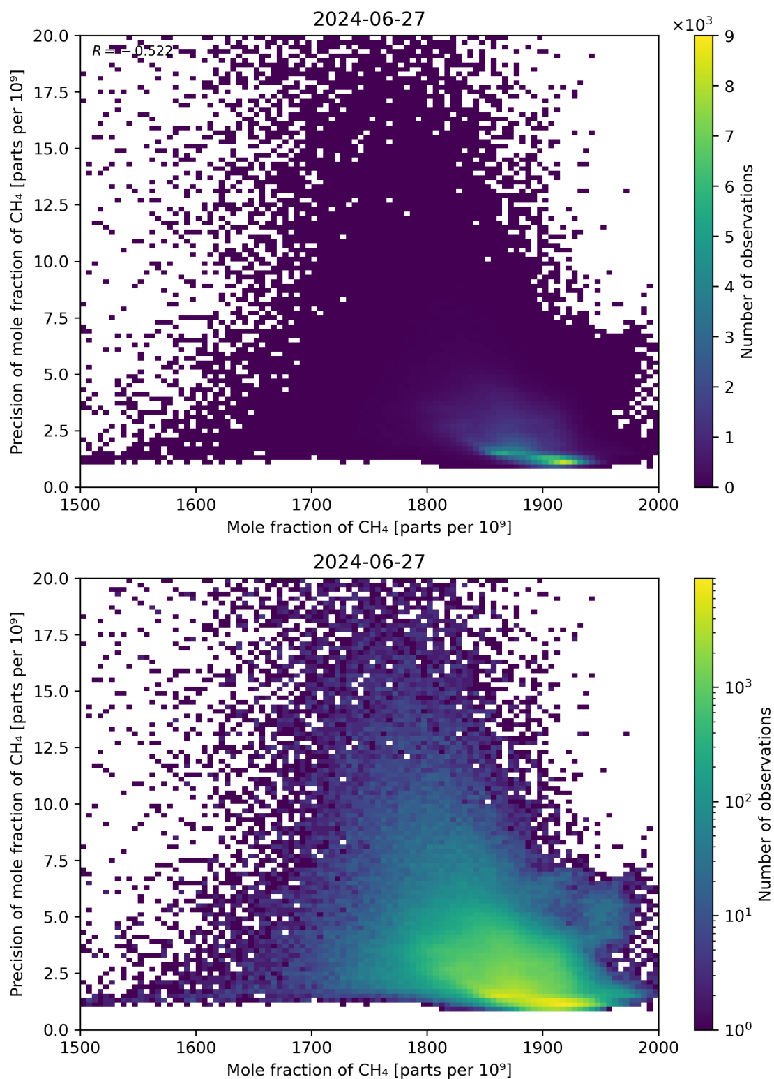
Figure 75: Scatter density plot of “Mole fraction of CH 4 ” against “Precision of mole fraction of CH 4 ” for 2024-06-26 to 2024-06-28.
