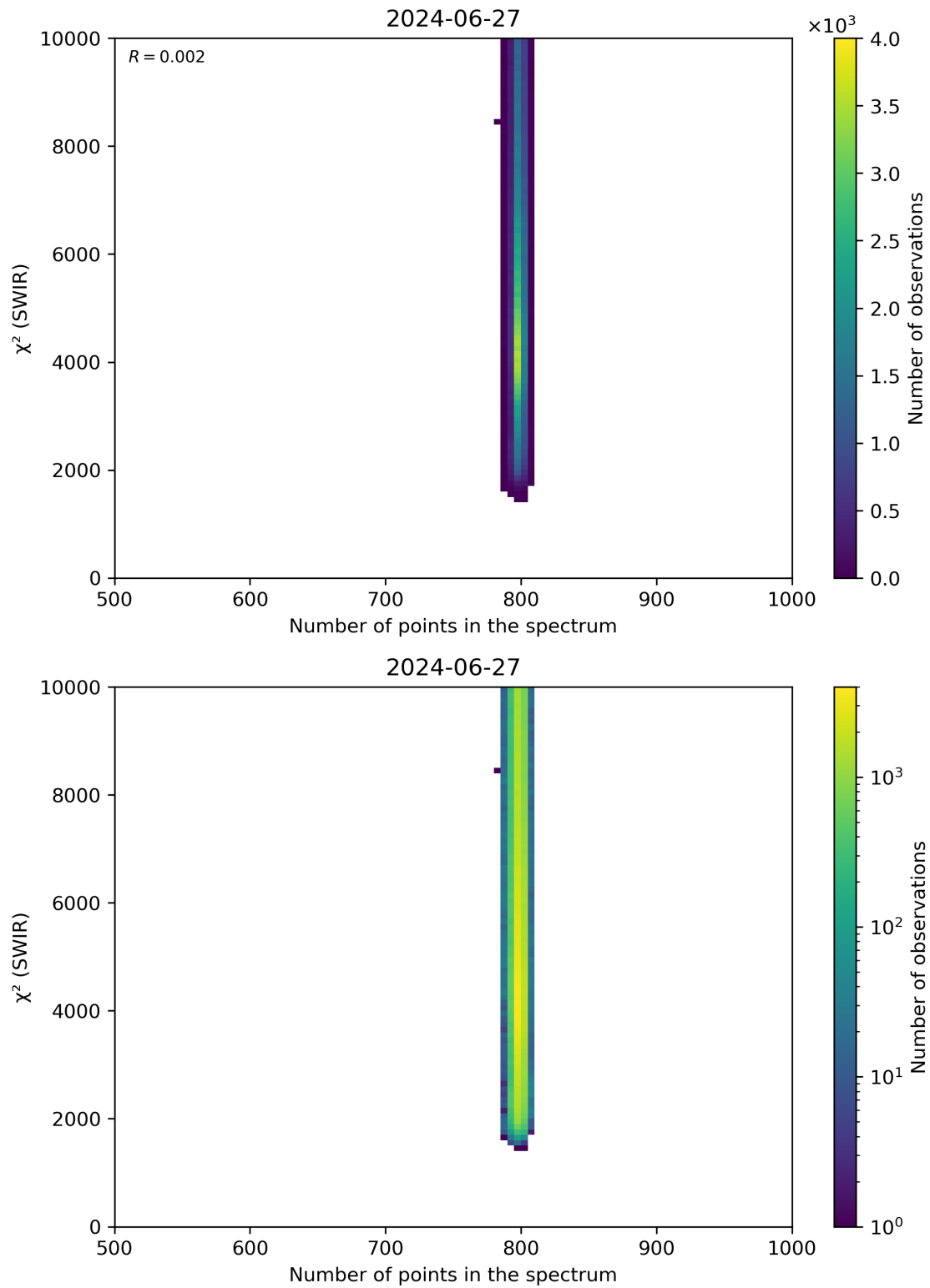
Figure 89: Scatter density plot of “Number of points in the spectrum” against “ \chi^2 (SWIR)” for 2024-06-26 to 2024-06-28.
