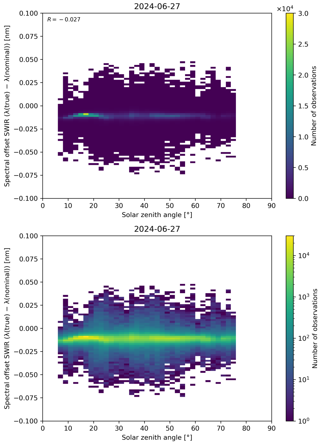
Figure 104: Scatter density plot of “Solar zenith angle” against “Spectral offset SWIR ( \lambda(\text{true}) - \lambda(\text{nominal}) )” for 2024-06-26 to 2024-06-28.
