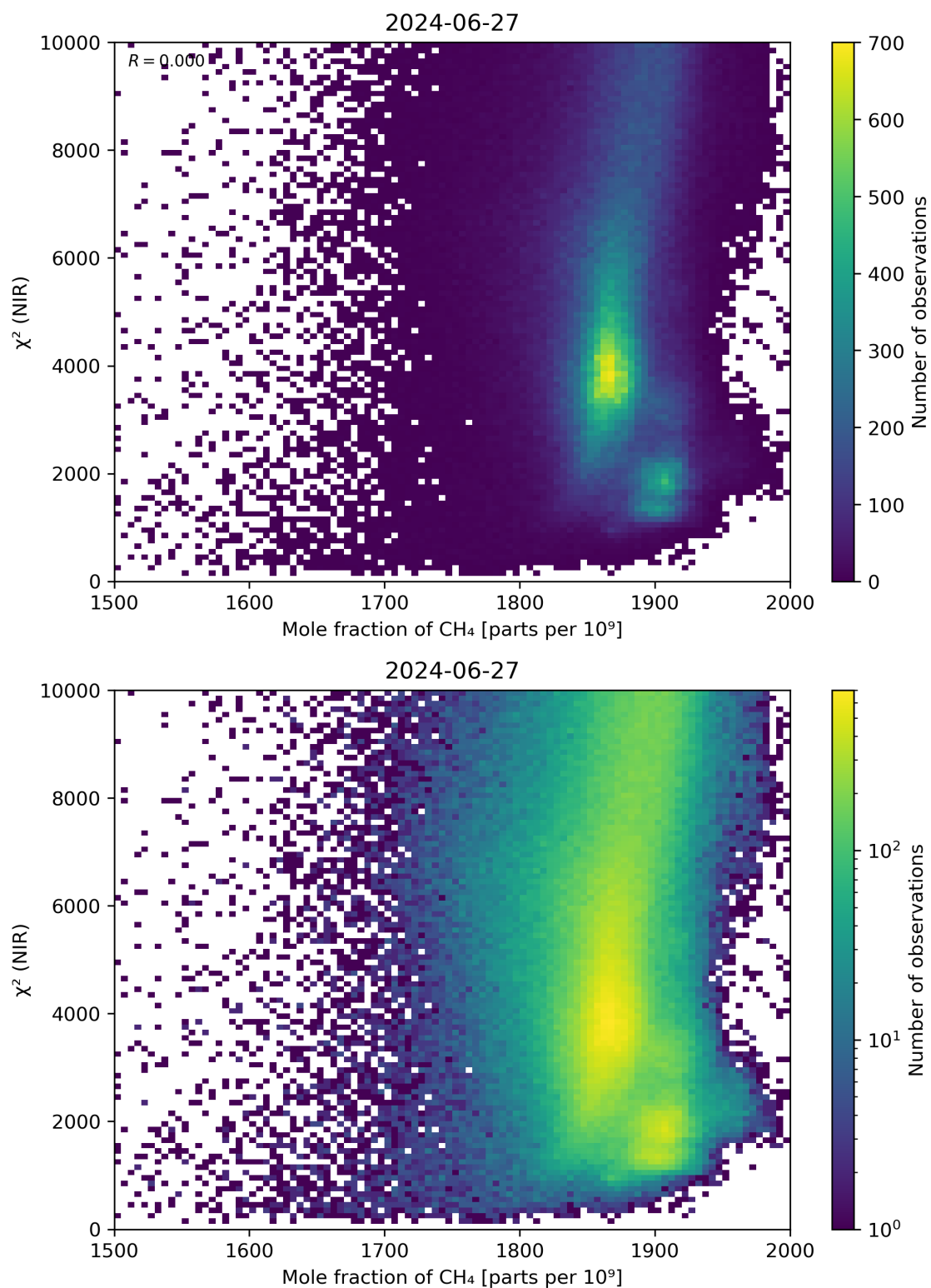
Figure 70: Scatter density plot of “Mole fraction of \text{CH}_4 ” against “ \chi^2 (NIR)” for 2024-06-26 to 2024-06-28.
