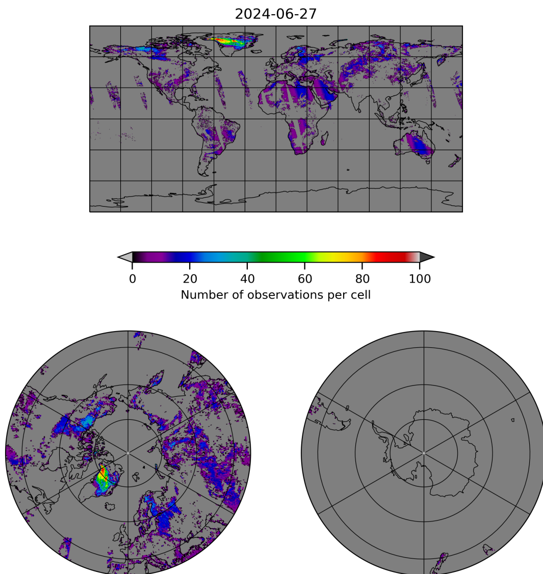
Figure 10: Map of the number of observations for 2024-06-26 to 2024-06-28
