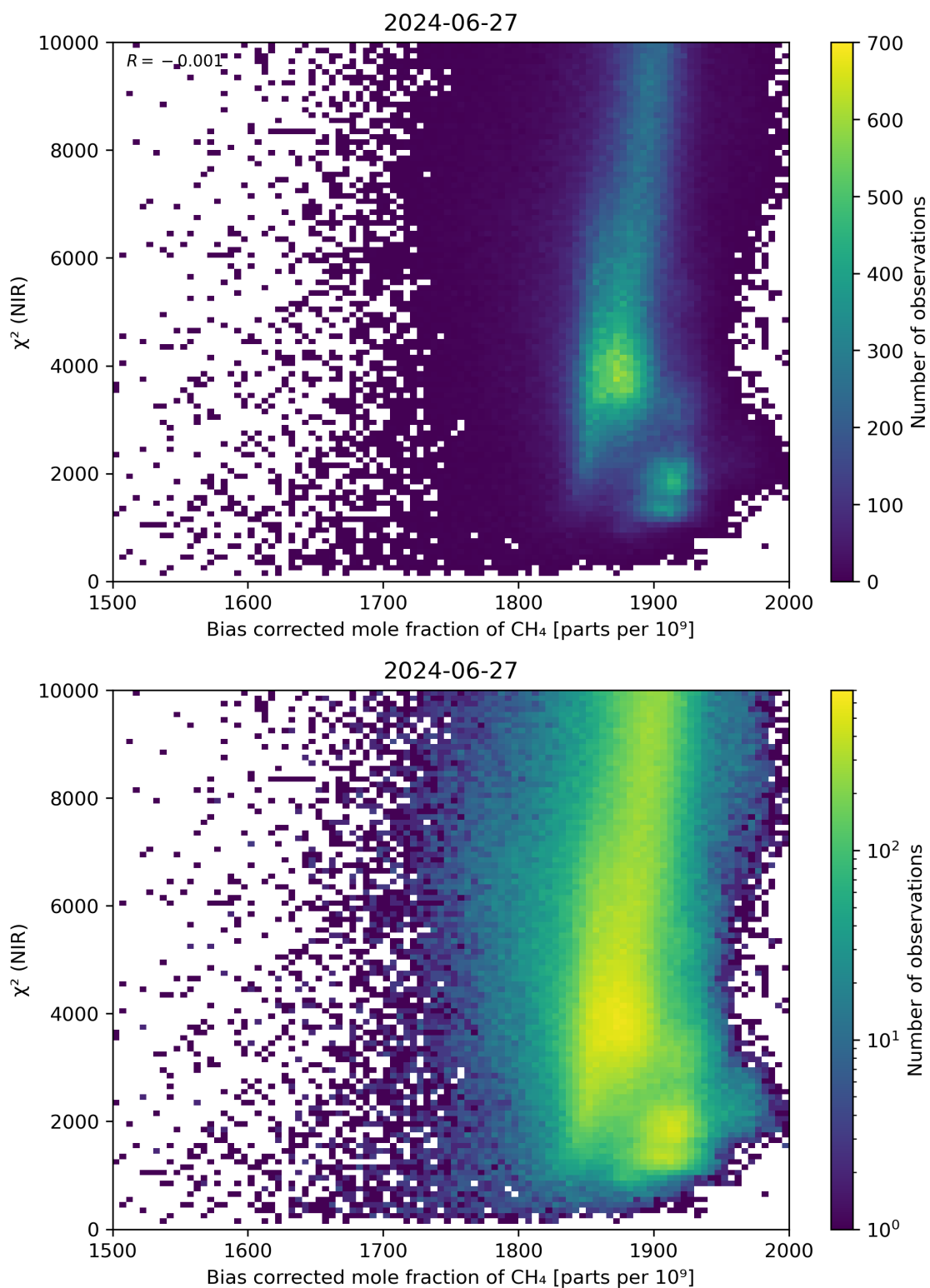
Figure 63: Scatter density plot of “Bias corrected mole fraction of CH 4 ” against “ \chi^2 (NIR)” for 2024-06-26 to 2024-06-28.
