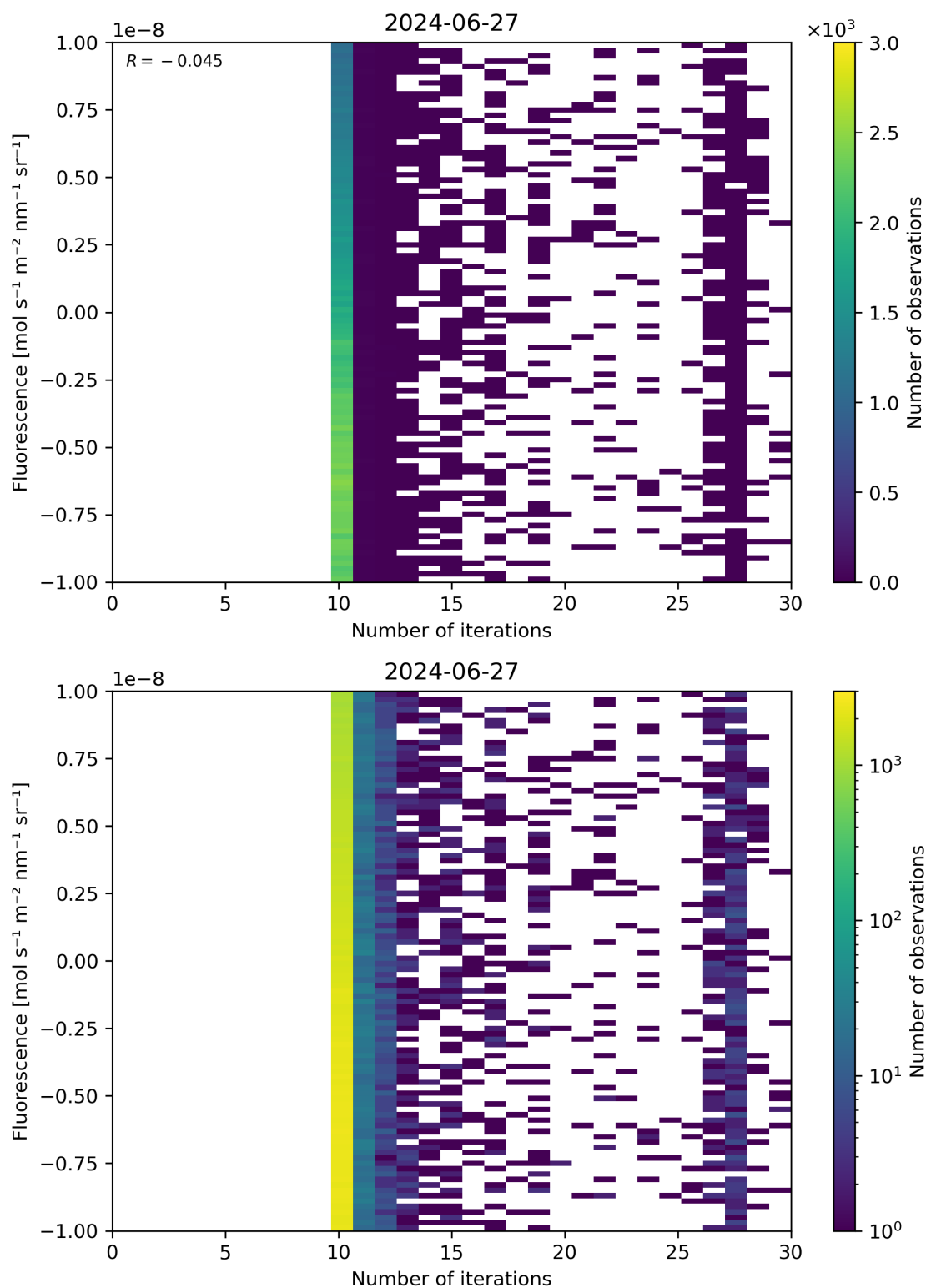
Figure 87: Scatter density plot of “Number of iterations” against “Fluorescence” for 2024-06-26 to 2024-06-28.
