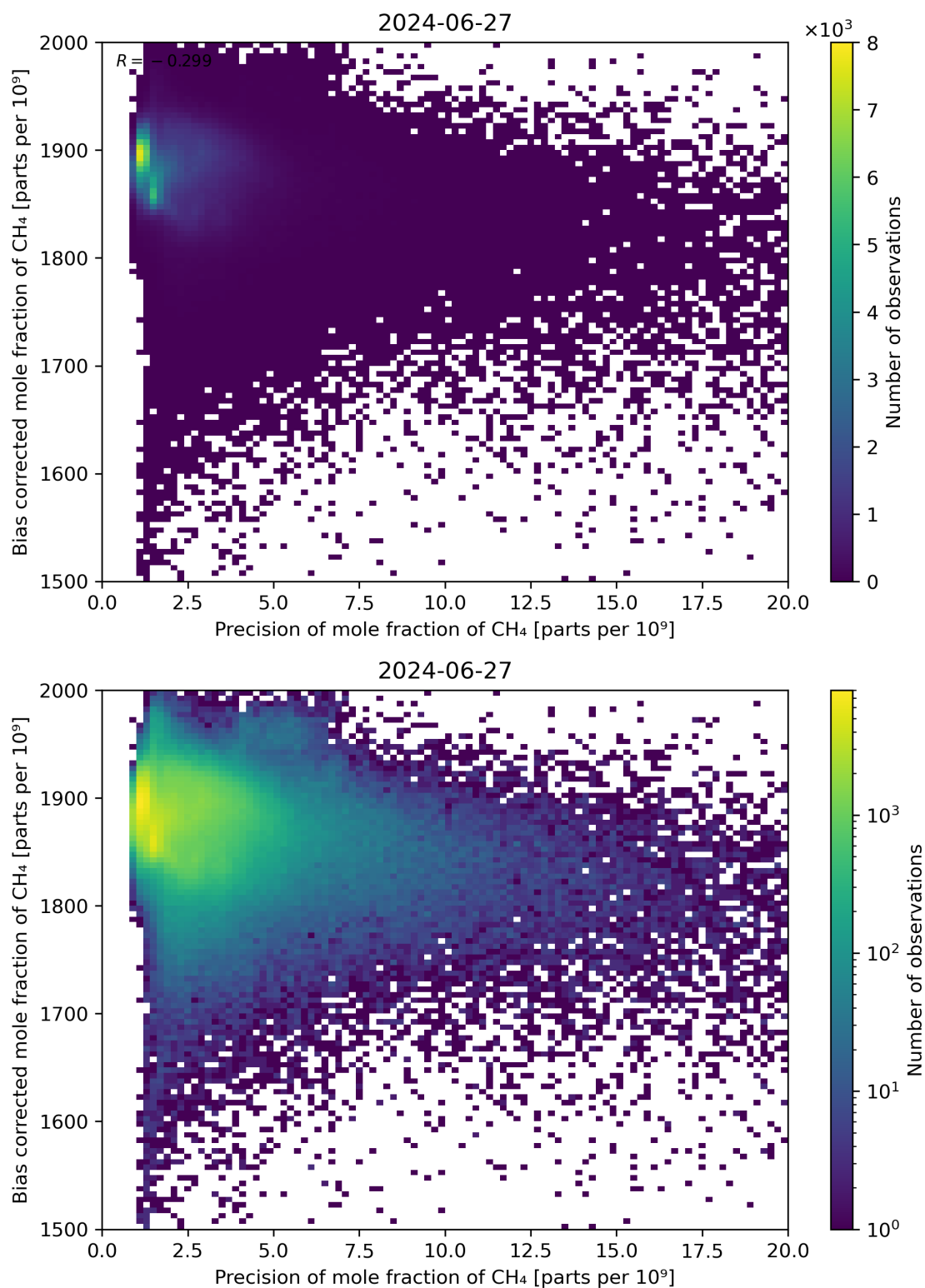
Figure 82: Scatter density plot of “Precision of mole fraction of CH 4 ” against “Bias corrected mole fraction of CH 4 ” for 2024-06-26 to 2024-06-28.
