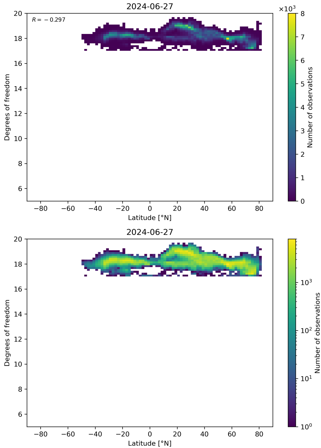
Figure 55: Scatter density plot of “Latitude” against “Degrees of freedom” for 2024-06-26 to 2024-06-28.
