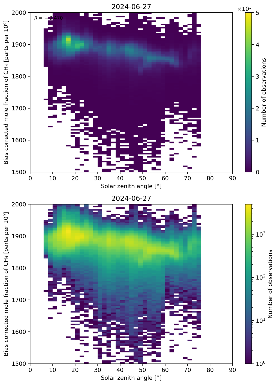
Figure 100: Scatter density plot of “Solar zenith angle” against “Bias corrected mole fraction of CH 4 ” for 2024-06-26 to 2024-06-28.
