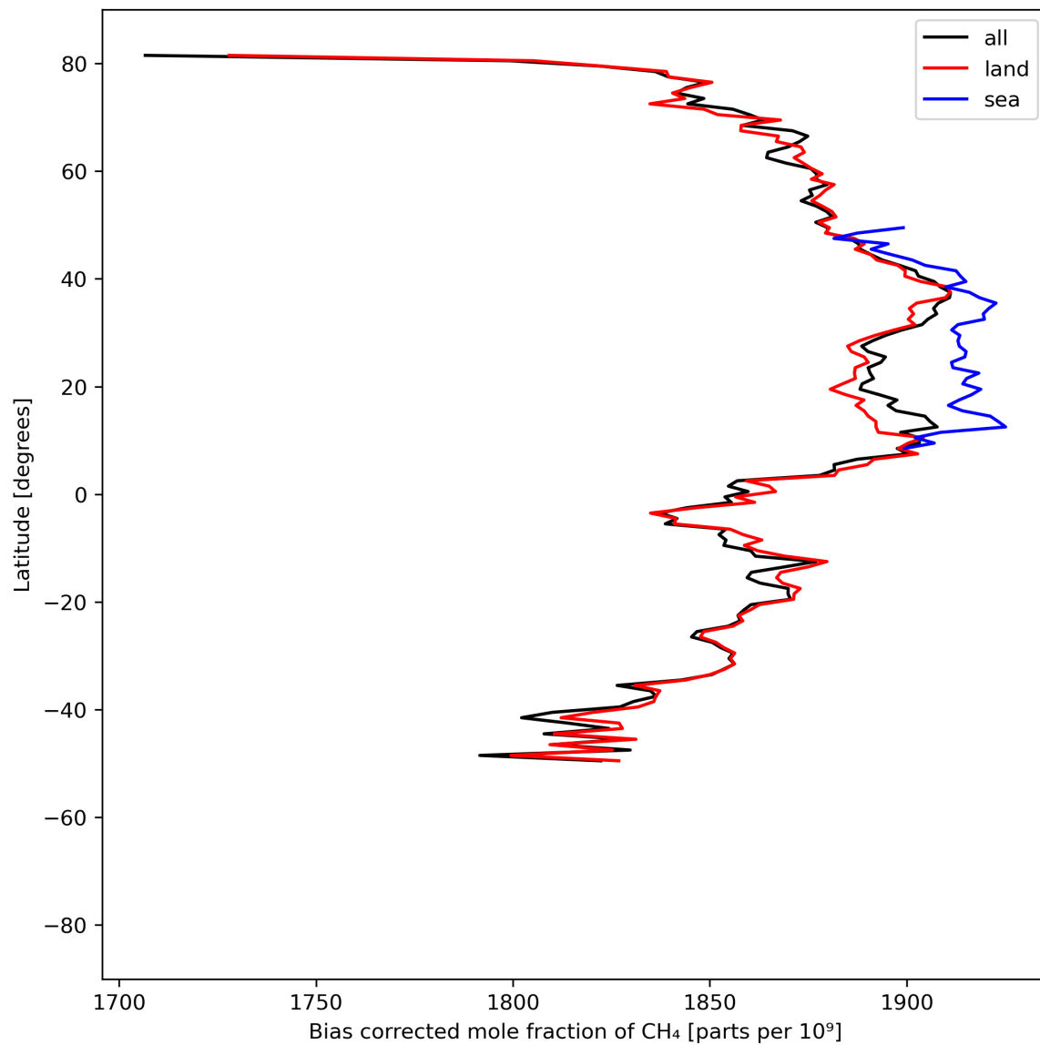
Figure 14: Zonal average of “Bias corrected mole fraction of CH 4 ” for 2024-06-26 to 2024-06-28.
