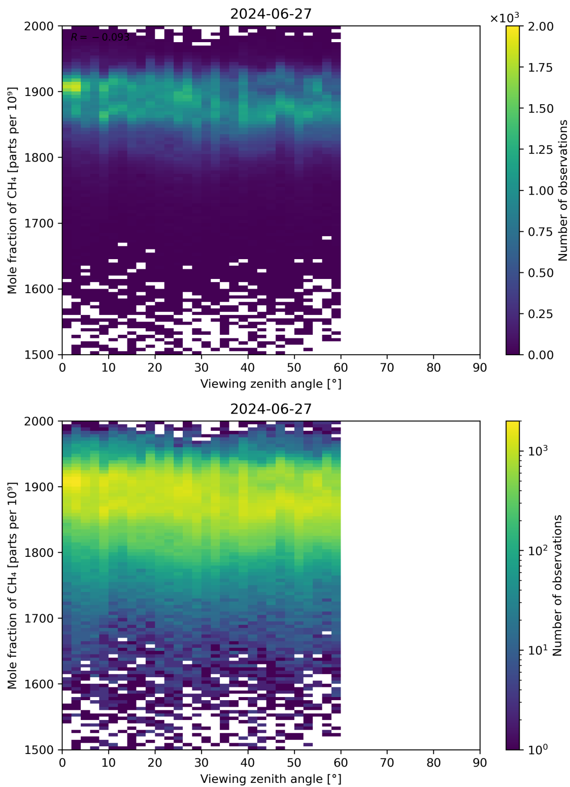
Figure 110: Scatter density plot of “Viewing zenith angle” against “Mole fraction of CH 4 ” for 2024-06-26 to 2024-06-28.
