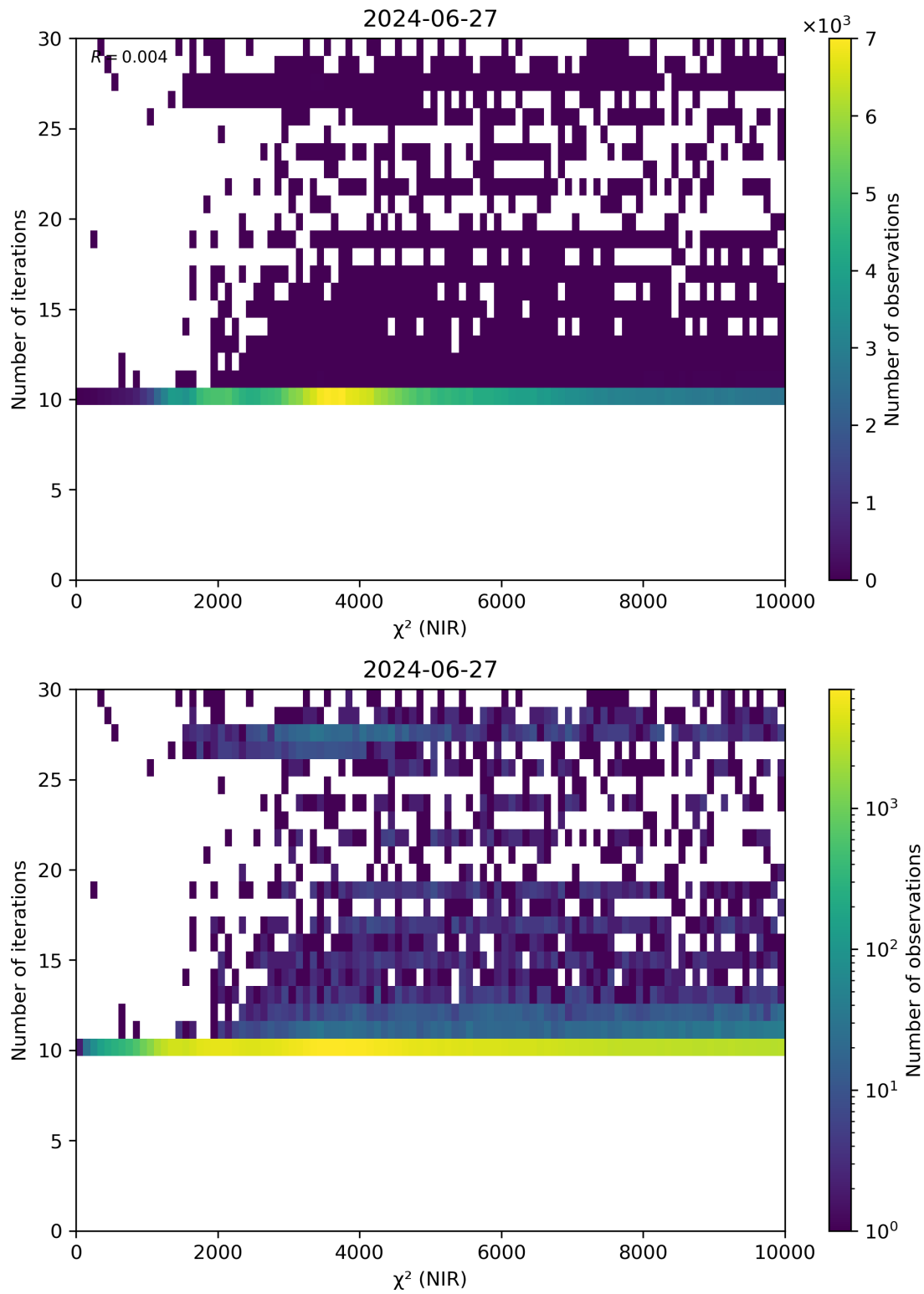
Figure 46: Scatter density plot of “ \chi^2 (NIR)” against “Number of iterations” for 2024-06-26 to 2024-06-28.
