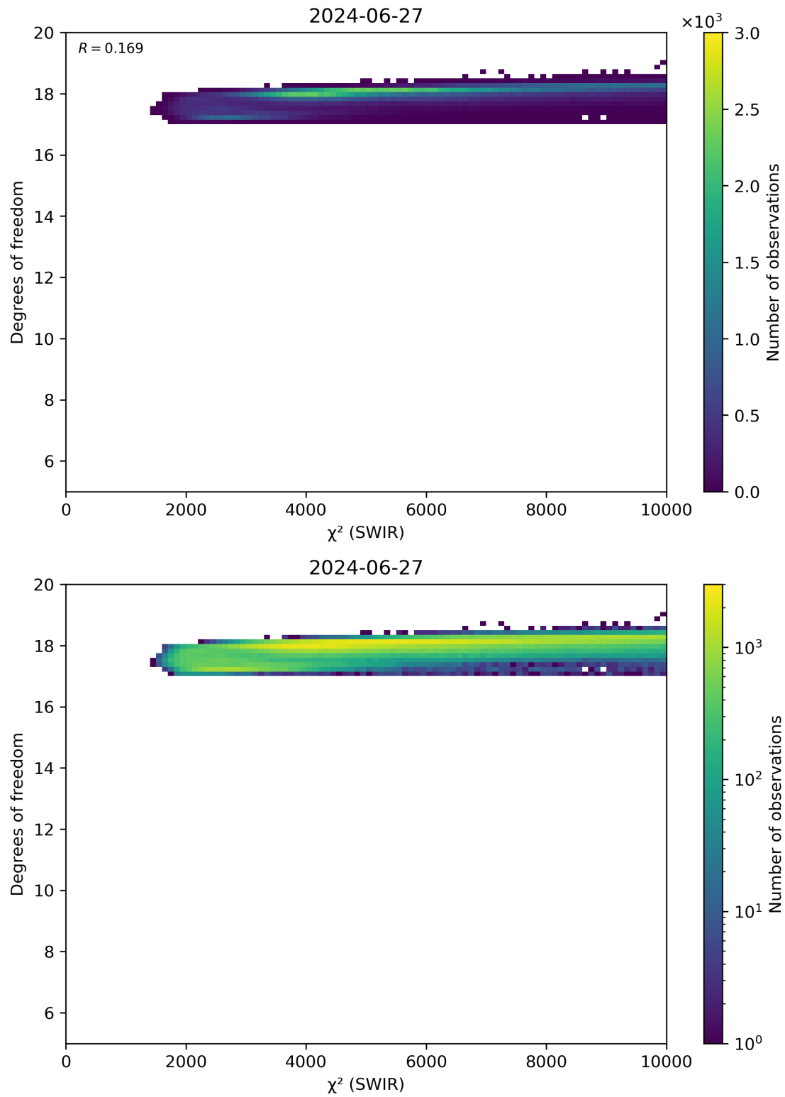
Figure 48: Scatter density plot of “ \chi^2 (SWIR)” against “Degrees of freedom” for 2024-06-26 to 2024-06-28.
