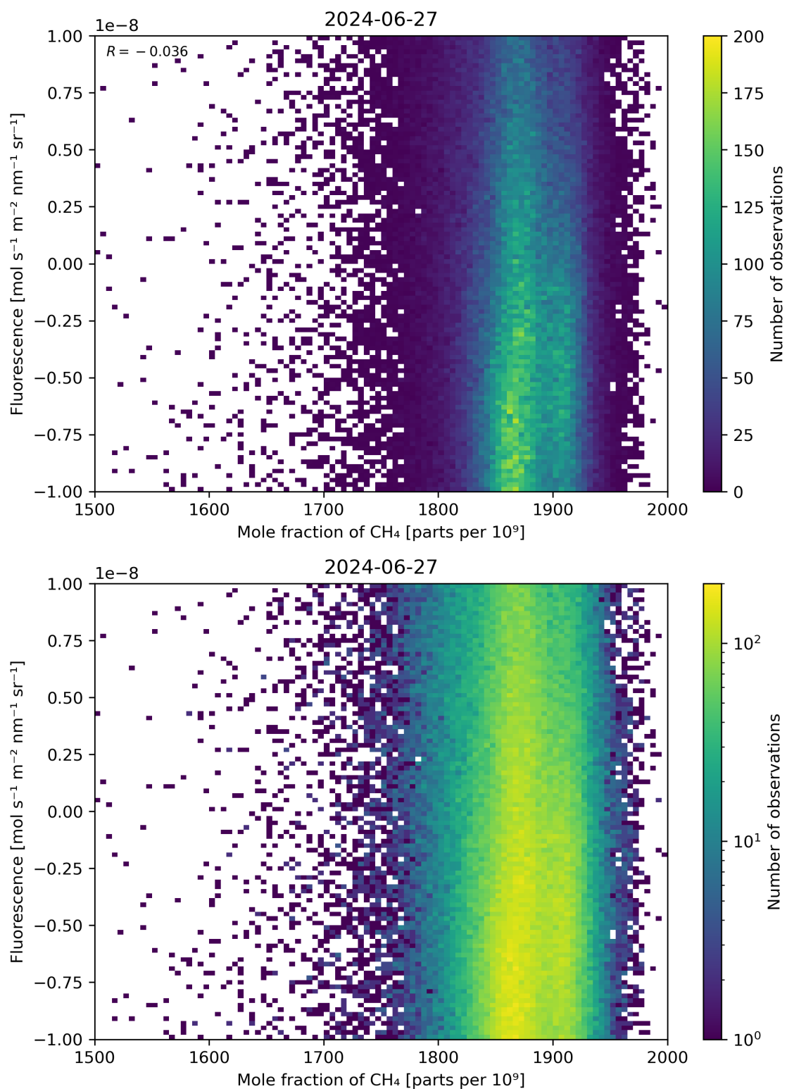
Figure 73: Scatter density plot of “Mole fraction of \text{CH}_4 ” against “Fluorescence” for 2024-06-26 to 2024-06-28.
