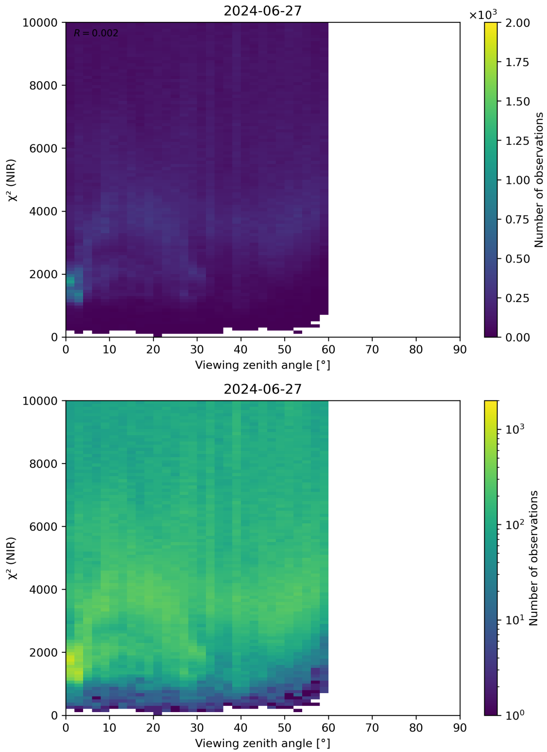
Figure 105: Scatter density plot of “Viewing zenith angle” against “ \chi^2 (NIR)” for 2024-06-26 to 2024-06-28.
