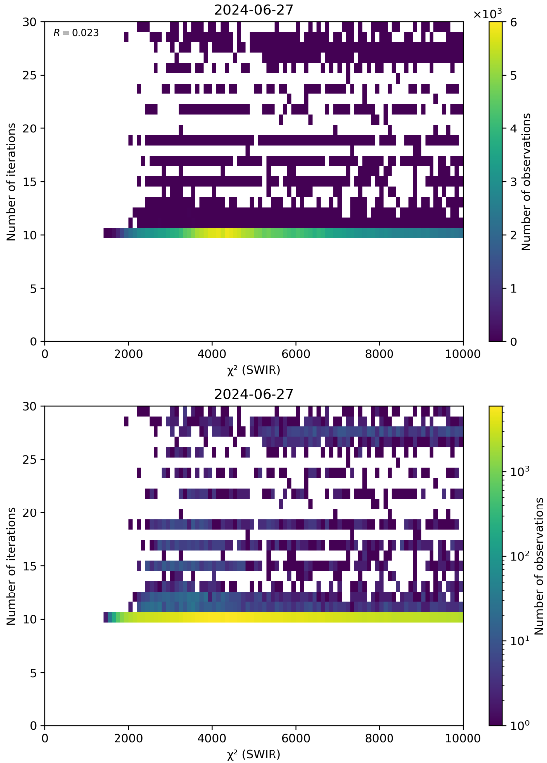
Figure 50: Scatter density plot of “ \chi^2 (SWIR)” against “Number of iterations” for 2024-06-26 to 2024-06-28.
