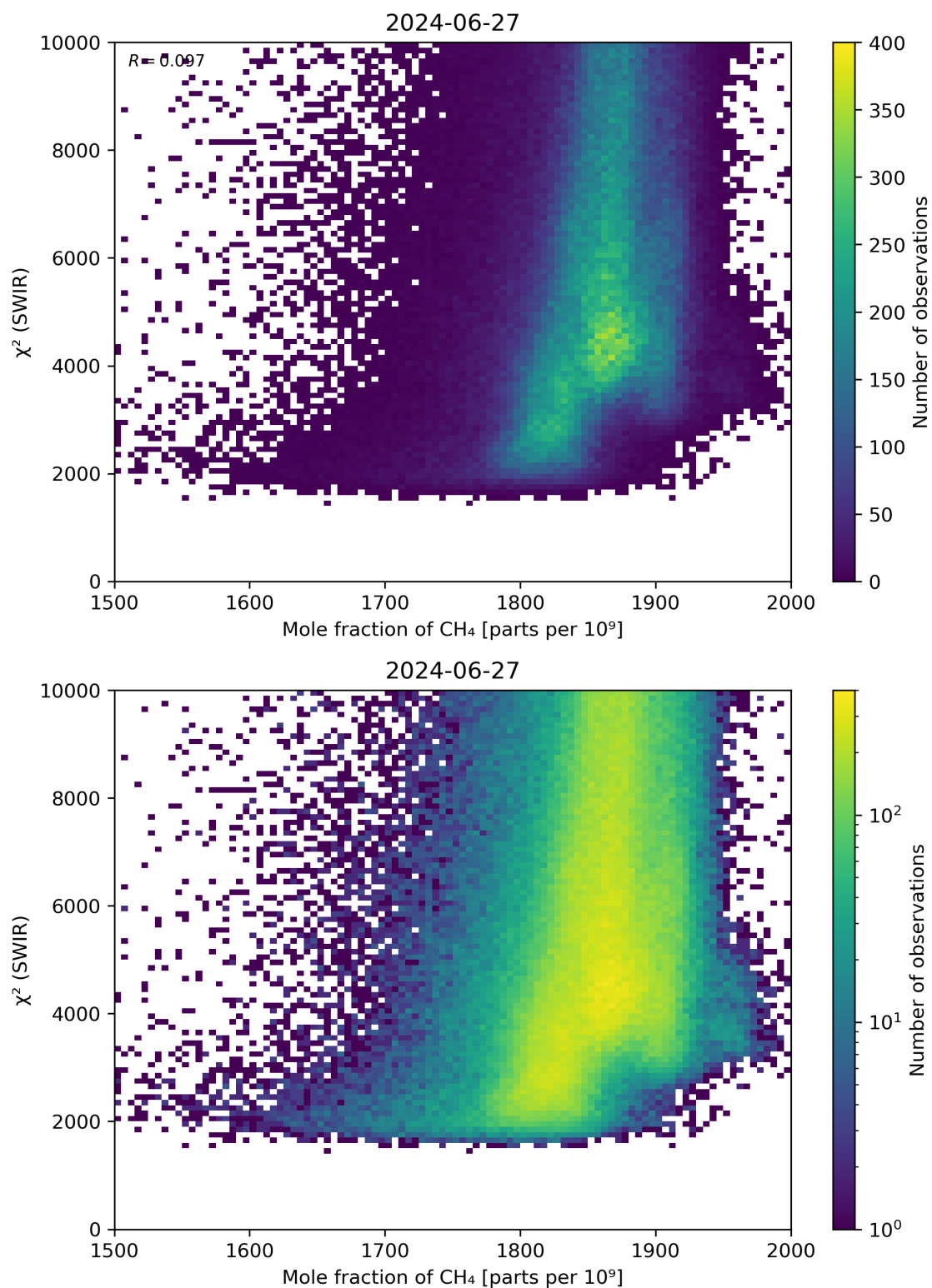
Figure 71: Scatter density plot of “Mole fraction of \text{CH}_4 ” against “ \chi^2 (SWIR)” for 2024-06-26 to 2024-06-28.
