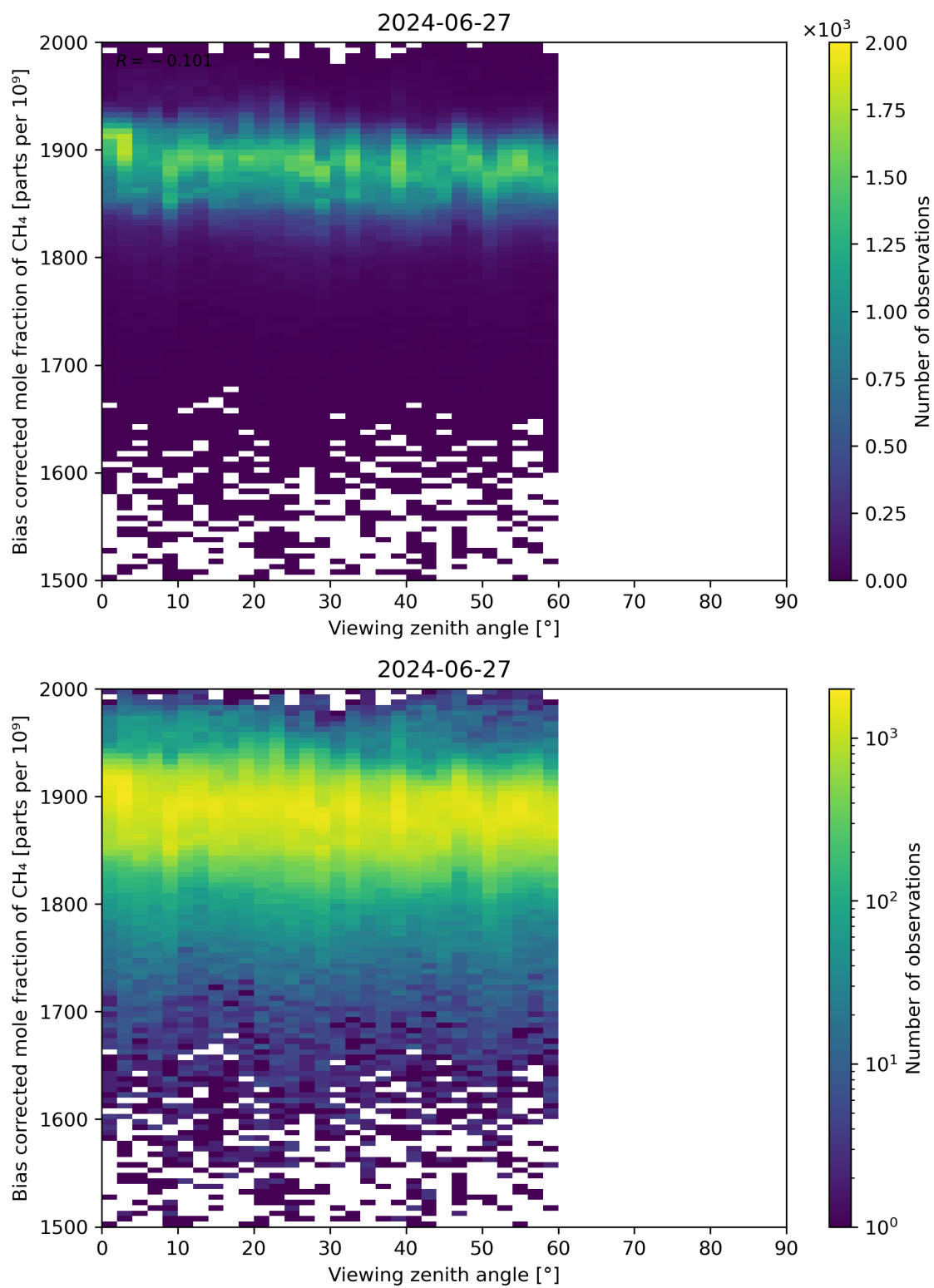
Figure 111: Scatter density plot of “Viewing zenith angle” against “Bias corrected mole fraction of CH 4 ” for 2024-06-26 to 2024-06-28.
