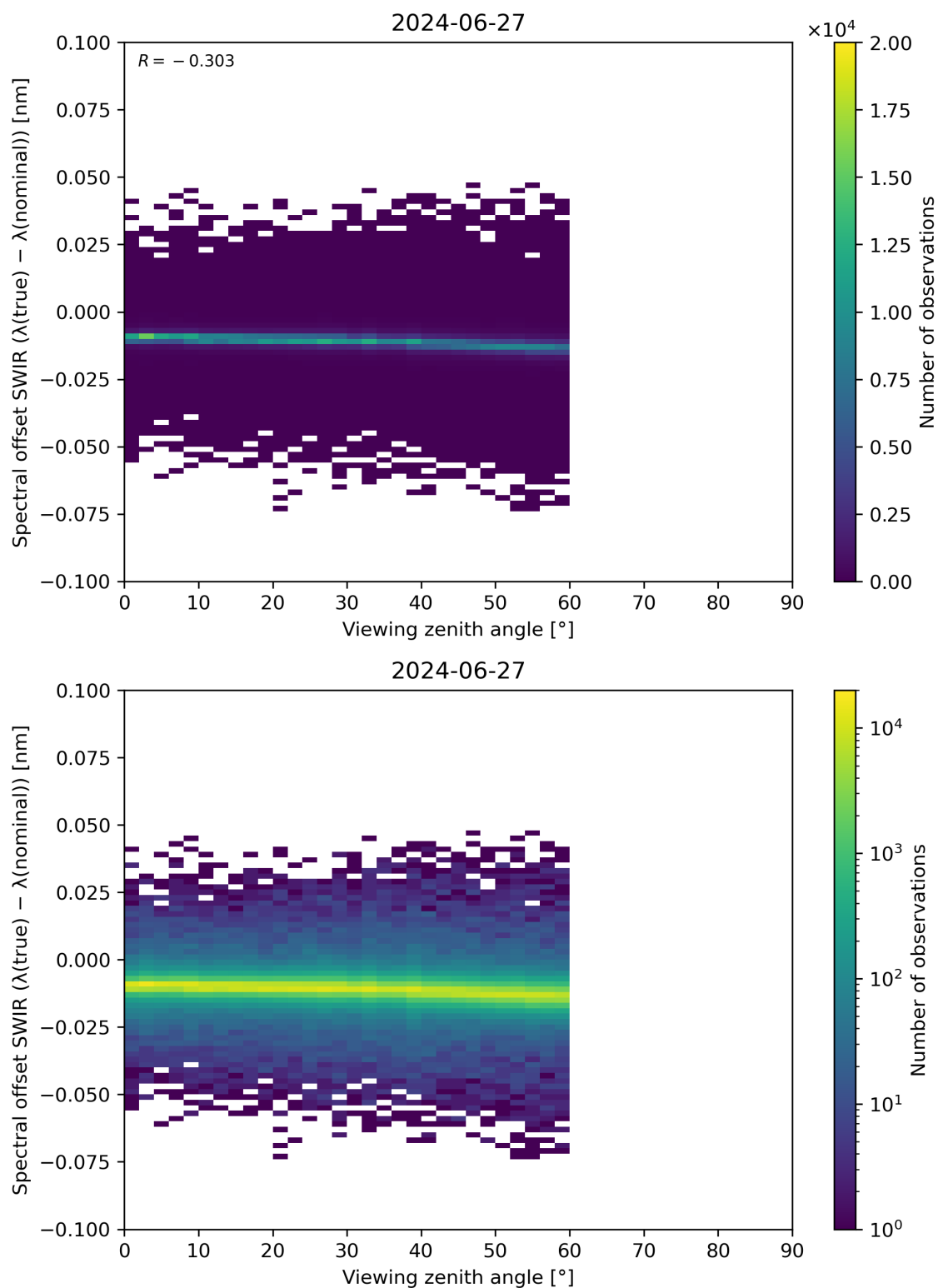
Figure 116: Scatter density plot of “Viewing zenith angle” against “Spectral offset SWIR ( \lambda(\text{true}) - \lambda(\text{nominal}) )” for 2024-06-26 to 2024-06-28.
