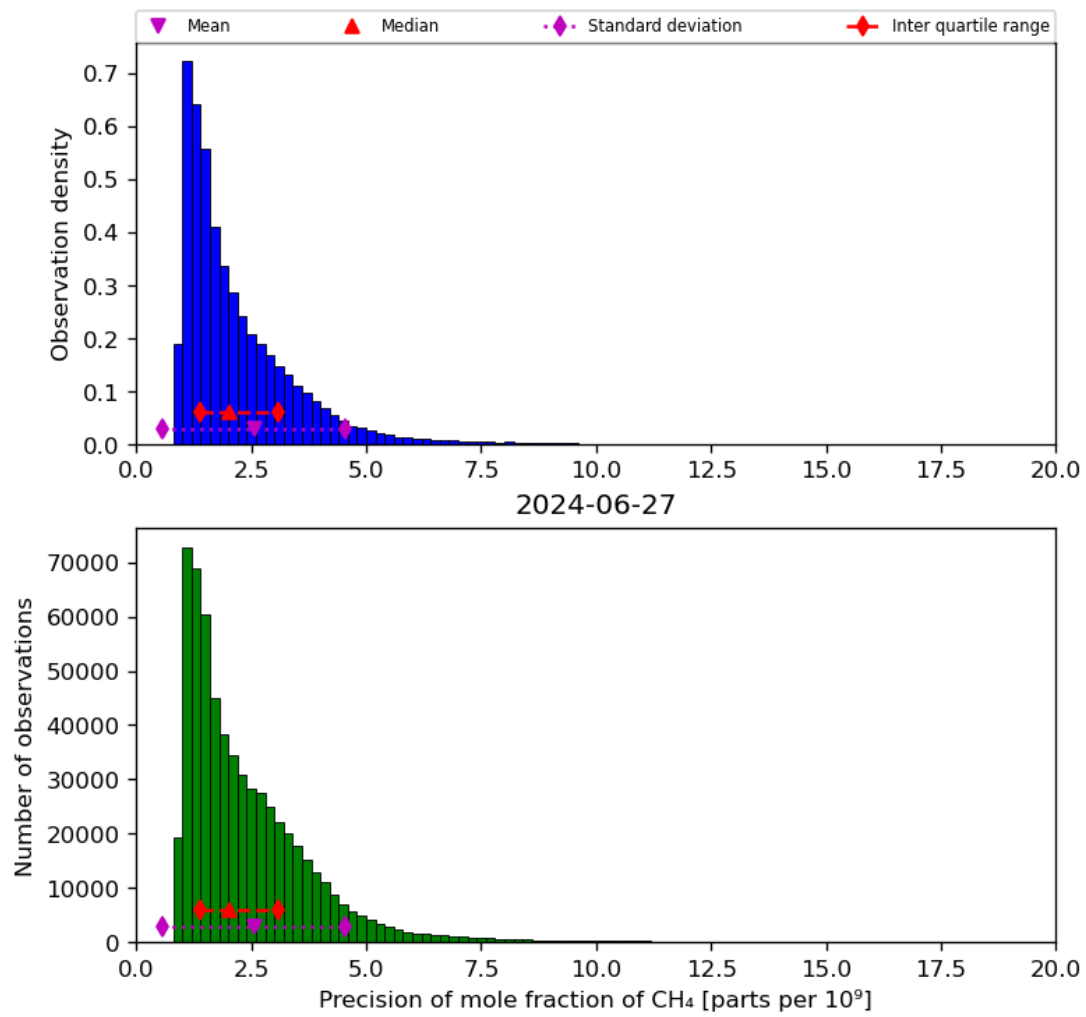
Figure 24: Histogram of “Precision of mole fraction of CH 4 ” for 2024-06-26 to 2024-06-28
