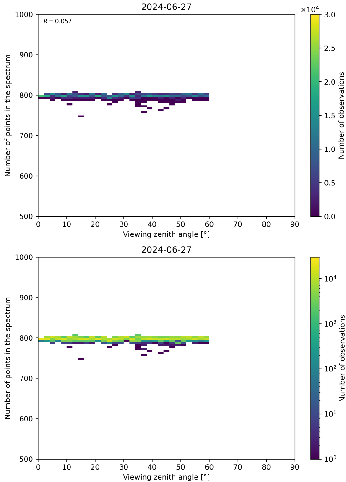
Figure 114: Scatter density plot of “Viewing zenith angle” against “Number of points in the spectrum” for 2024-06-26 to 2024-06-28.
