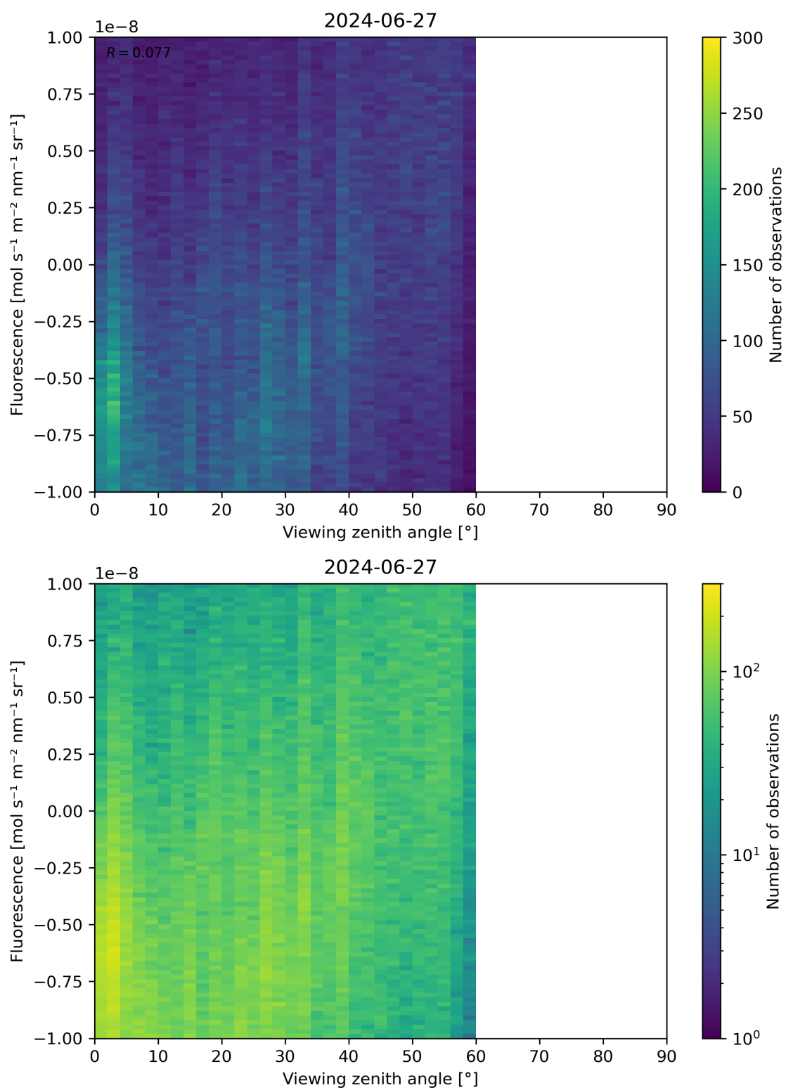
Figure 108: Scatter density plot of “Viewing zenith angle” against “Fluorescence” for 2024-06-26 to 2024-06-28.
