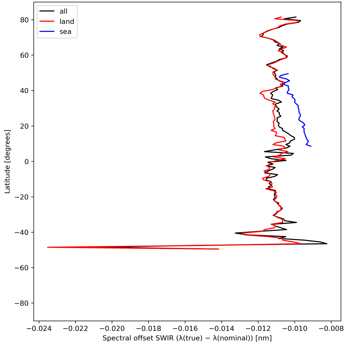
Figure 16: Zonal average of “Spectral offset SWIR ( \lambda(\text{true}) - \lambda(\text{nominal}) )” for 2024-06-26 to 2024-06-28.
