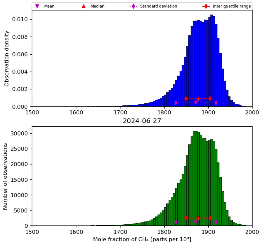
Figure 23: Histogram of “Mole fraction of CH 4 ” for 2024-06-26 to 2024-06-28
