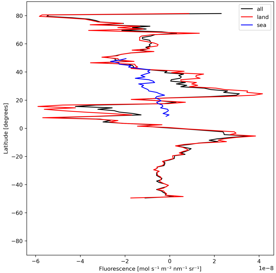
Figure 21: Zonal average of “Fluorescence” for 2024-06-26 to 2024-06-28.
