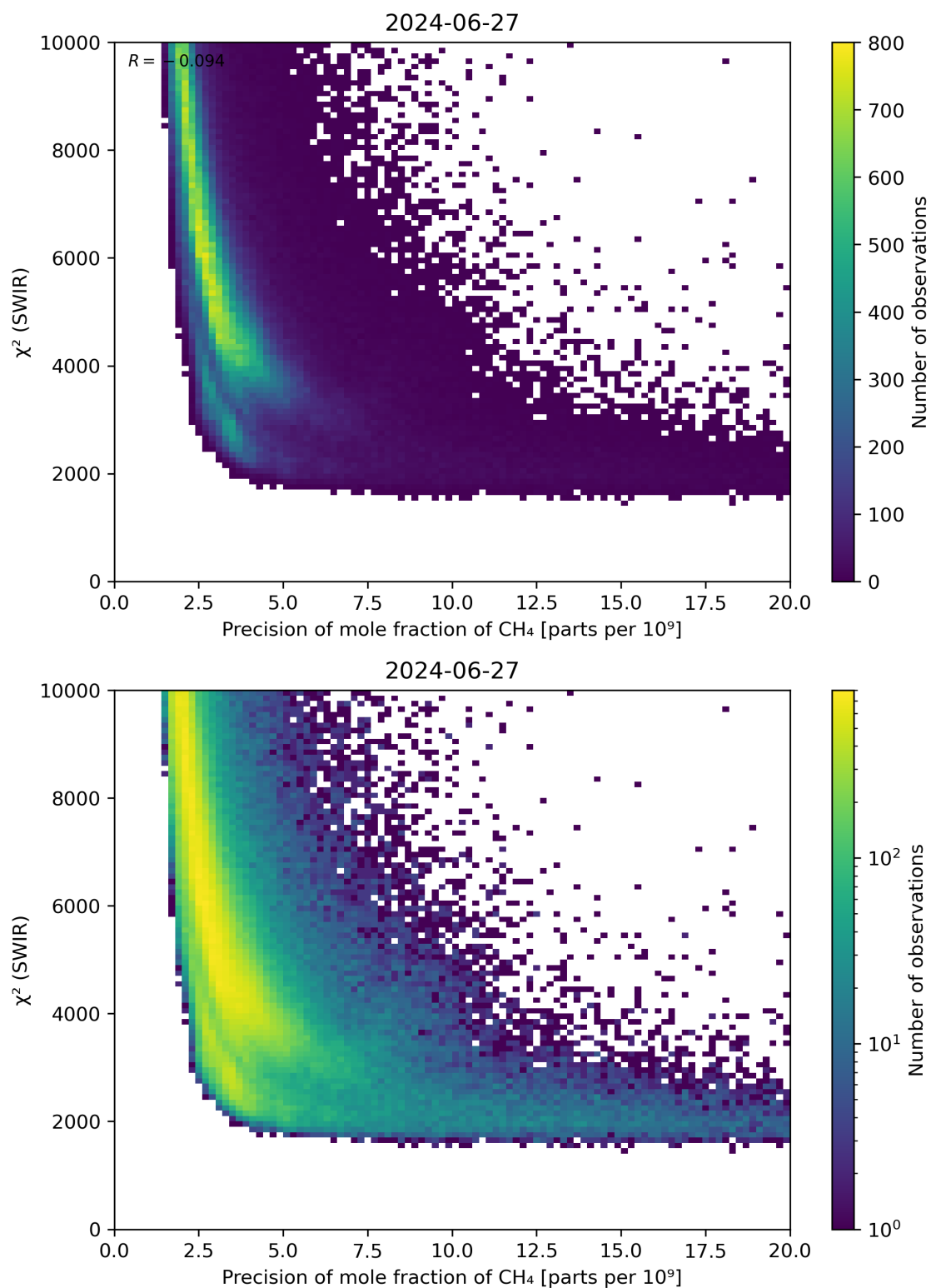
Figure 79: Scatter density plot of “Precision of mole fraction of CH 4 ” against “ \chi^2 (SWIR)” for 2024-06-26 to 2024-06-28.
