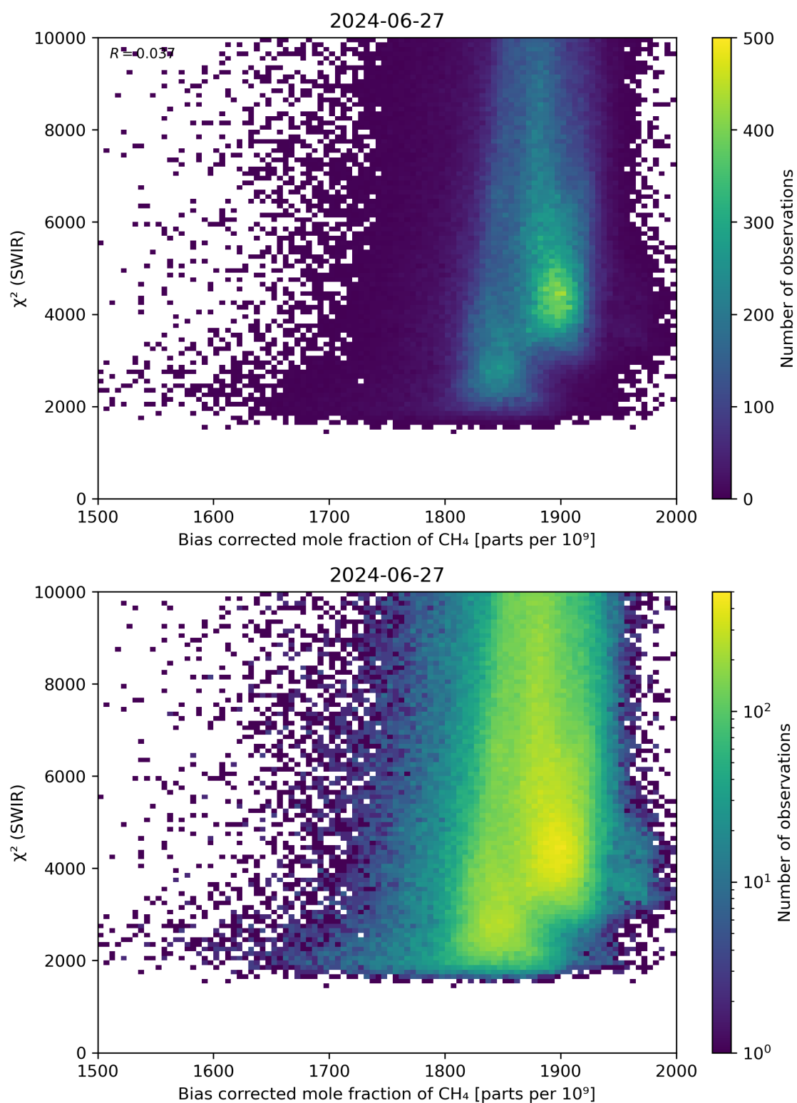
Figure 64: Scatter density plot of “Bias corrected mole fraction of \text{CH}_4 ” against “ \chi^2 (SWIR)” for 2024-06-26 to 2024-06-28.
