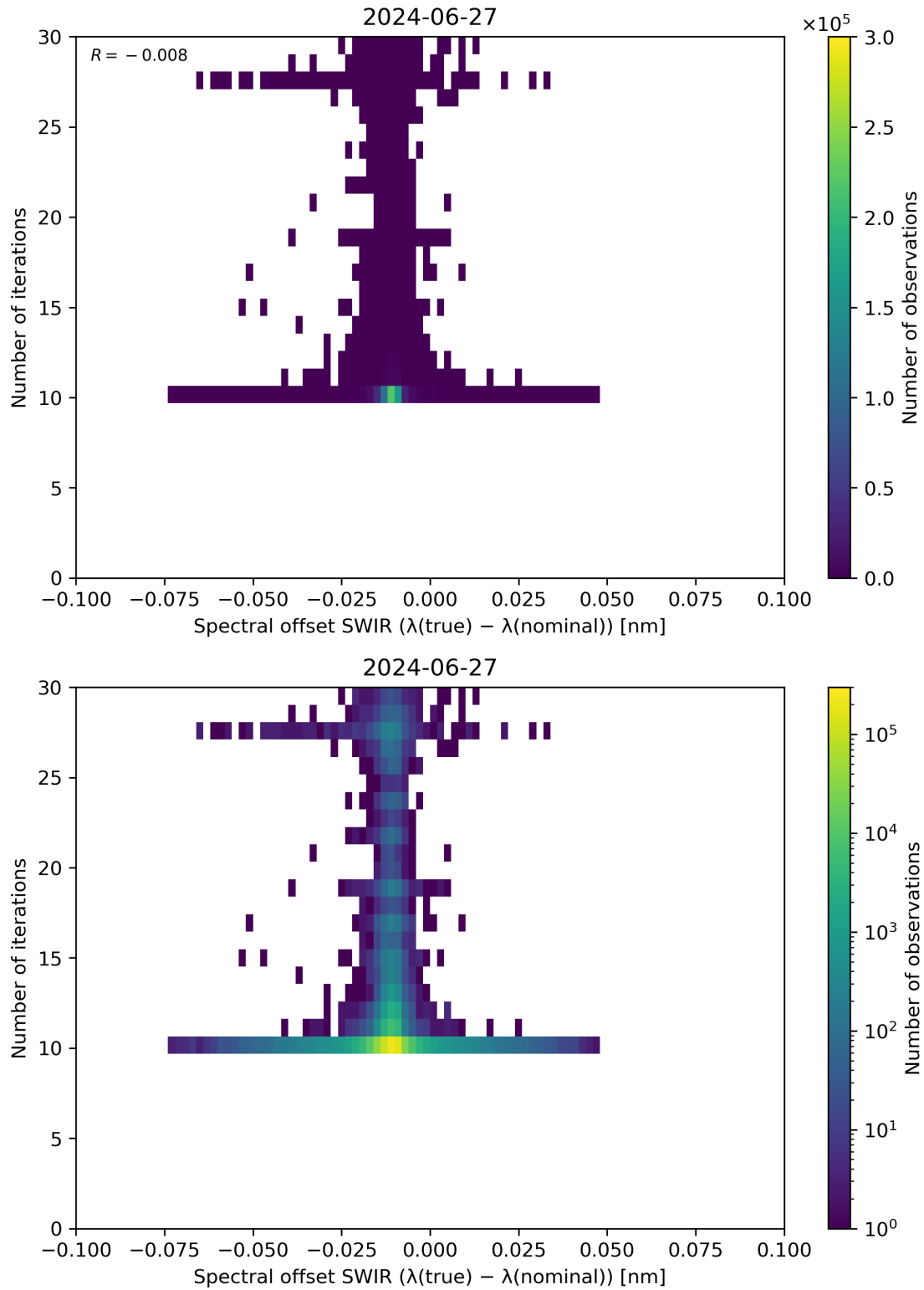
Figure 121: Scatter density plot of “Spectral offset SWIR ( \lambda(\text{true}) - \lambda(\text{nominal}) )” against “Number of iterations” for 2024-06-26 to 2024-06-28.
