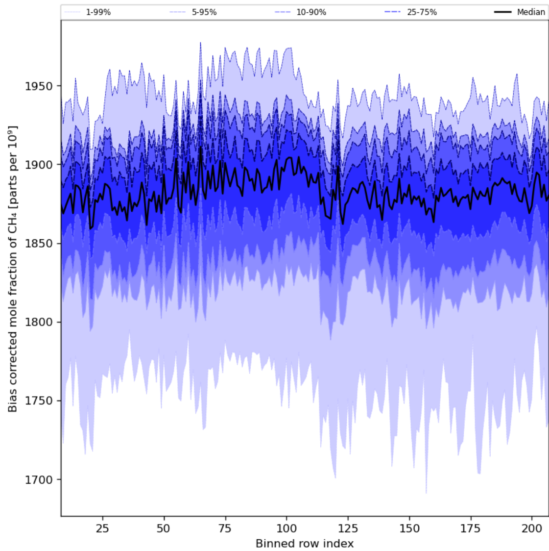
Figure 36: Along track statistics of “Bias corrected mole fraction of CH 4 ” for 2024-06-26 to 2024-06-28
