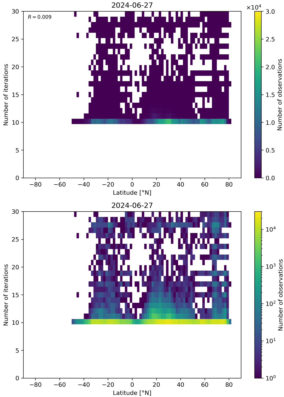
Figure 60: Scatter density plot of “Latitude” against “Number of iterations” for 2024-06-26 to 2024-06-28.
