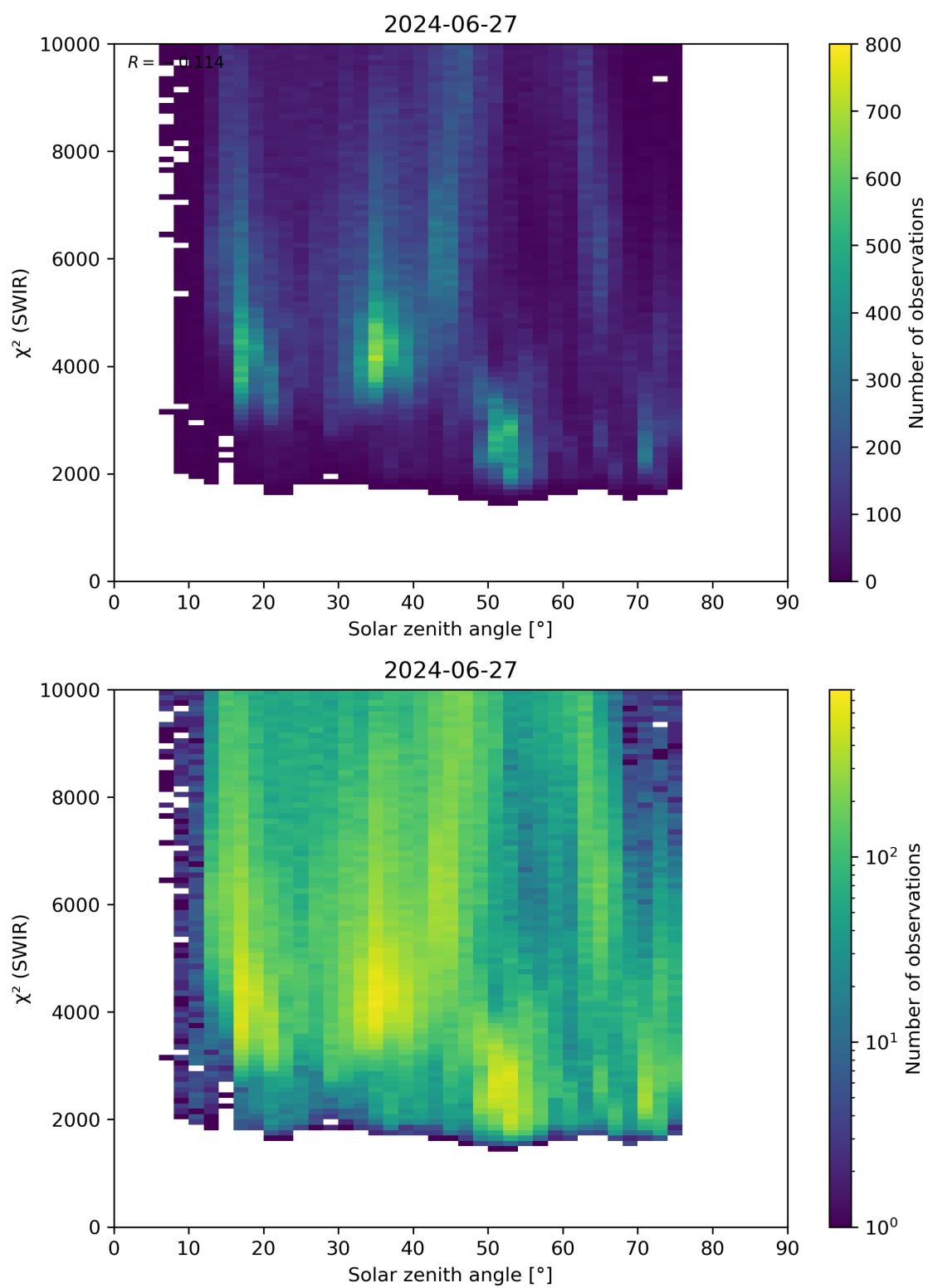
Figure 95: Scatter density plot of “Solar zenith angle” against “ \chi^2 (SWIR)” for 2024-06-26 to 2024-06-28.
