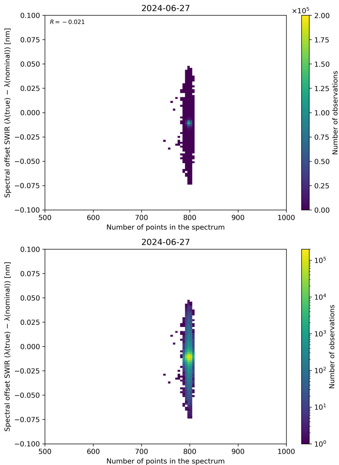
Figure 93: Scatter density plot of “Number of points in the spectrum” against “Spectral offset SWIR ( \lambda(\text{true}) - \lambda(\text{nominal}) )” for 2024-06-26 to 2024-06-28.
