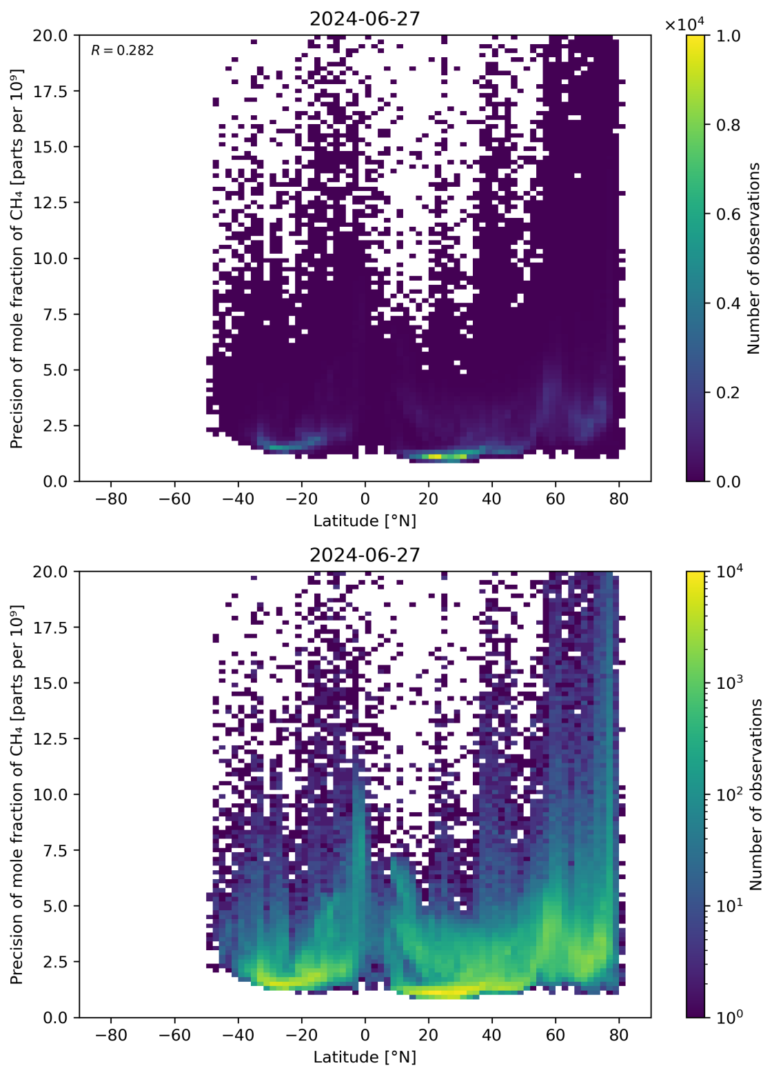
Figure 59: Scatter density plot of “Latitude” against “Precision of mole fraction of \text{CH}_4 ” for 2024-06-26 to 2024-06-28.
