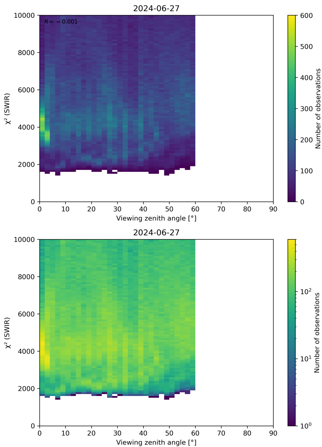
Figure 106: Scatter density plot of “Viewing zenith angle” against “ \chi^2 (SWIR)” for 2024-06-26 to 2024-06-28.
