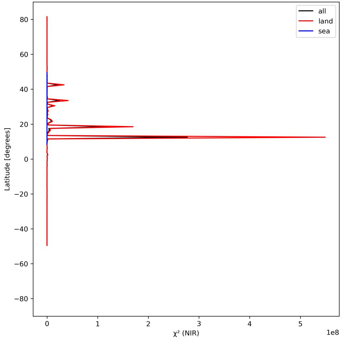
Figure 18: Zonal average of “ \chi^2 (NIR)” for 2024-06-26 to 2024-06-28.
