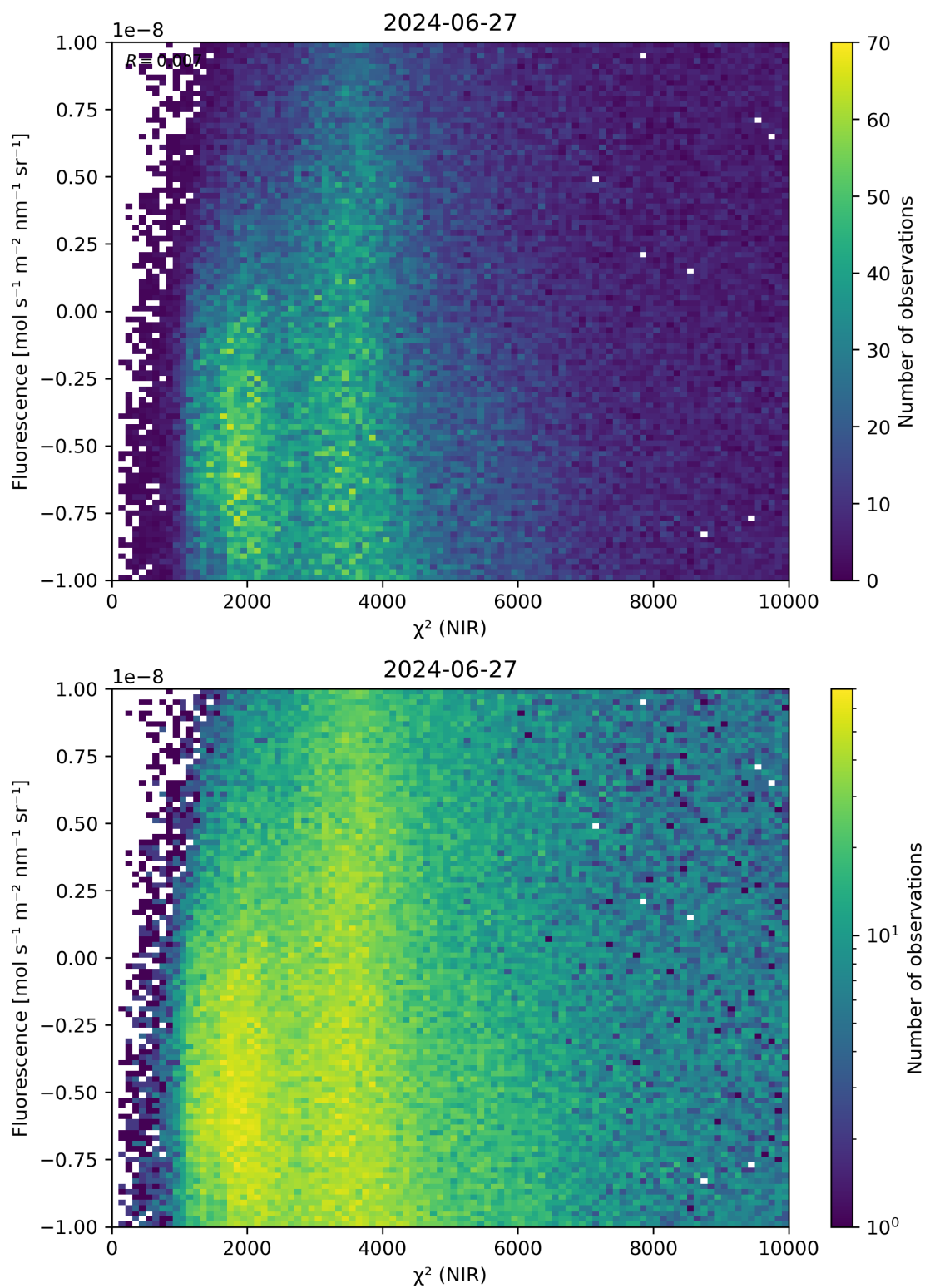
Figure 45: Scatter density plot of “ \chi^2 (NIR)” against “Fluorescence” for 2024-06-26 to 2024-06-28.
