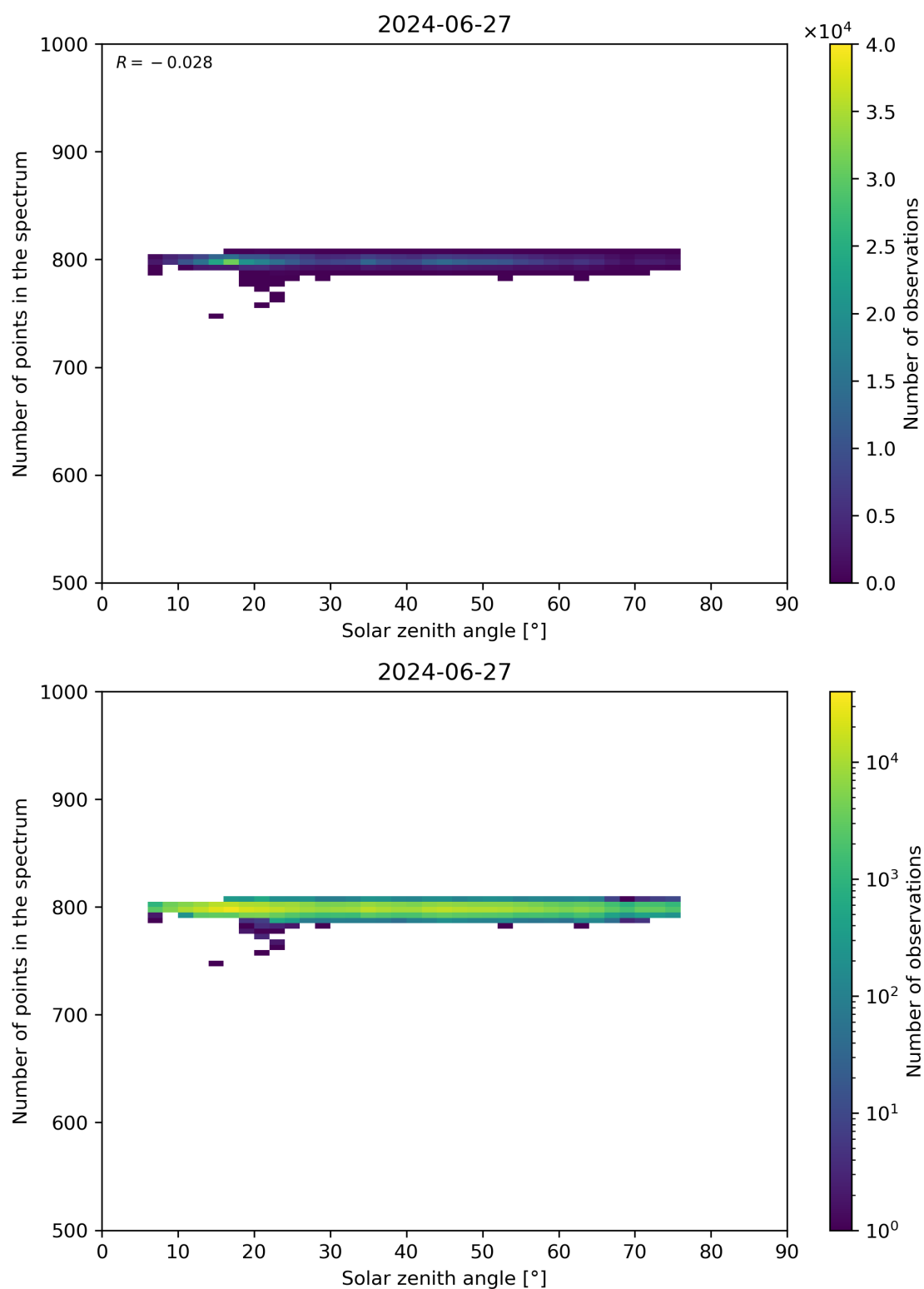
Figure 103: Scatter density plot of “Solar zenith angle” against “Number of points in the spectrum” for 2024-06-26 to 2024-06-28.
