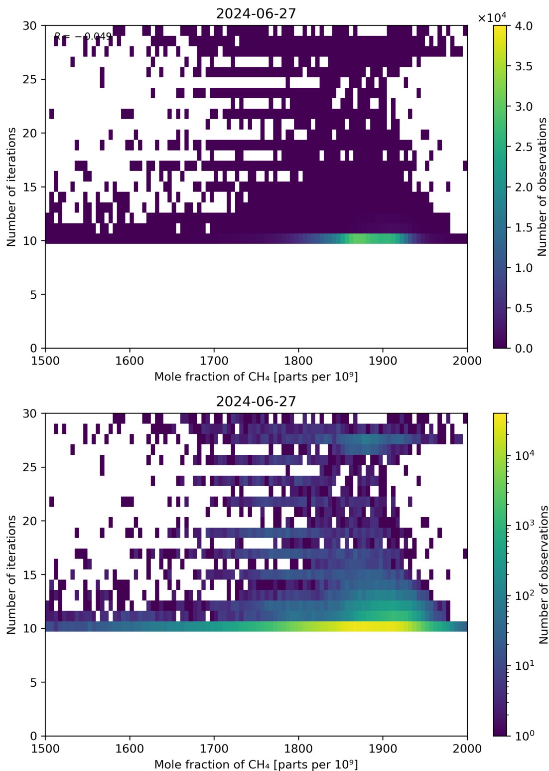
Figure 76: Scatter density plot of “Mole fraction of CH 4 ” against “Number of iterations” for 2024-06-26 to 2024-06-28.
