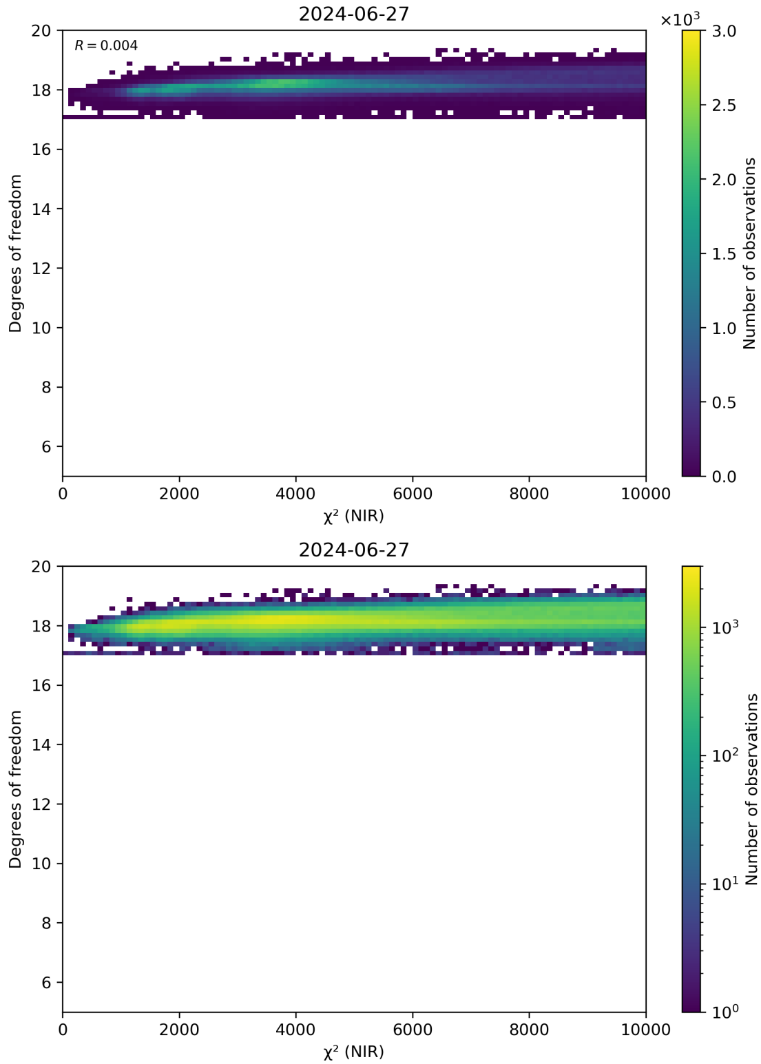
Figure 44: Scatter density plot of “ \chi^2 (NIR)” against “Degrees of freedom” for 2024-06-26 to 2024-06-28.
