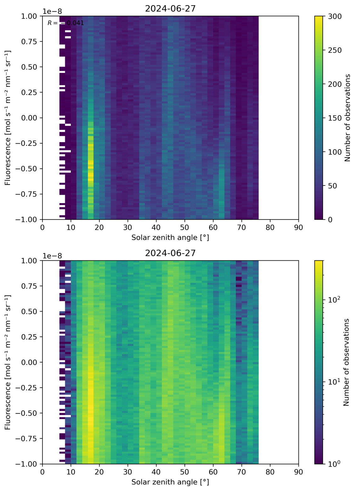
Figure 97: Scatter density plot of “Solar zenith angle” against “Fluorescence” for 2024-06-26 to 2024-06-28.
