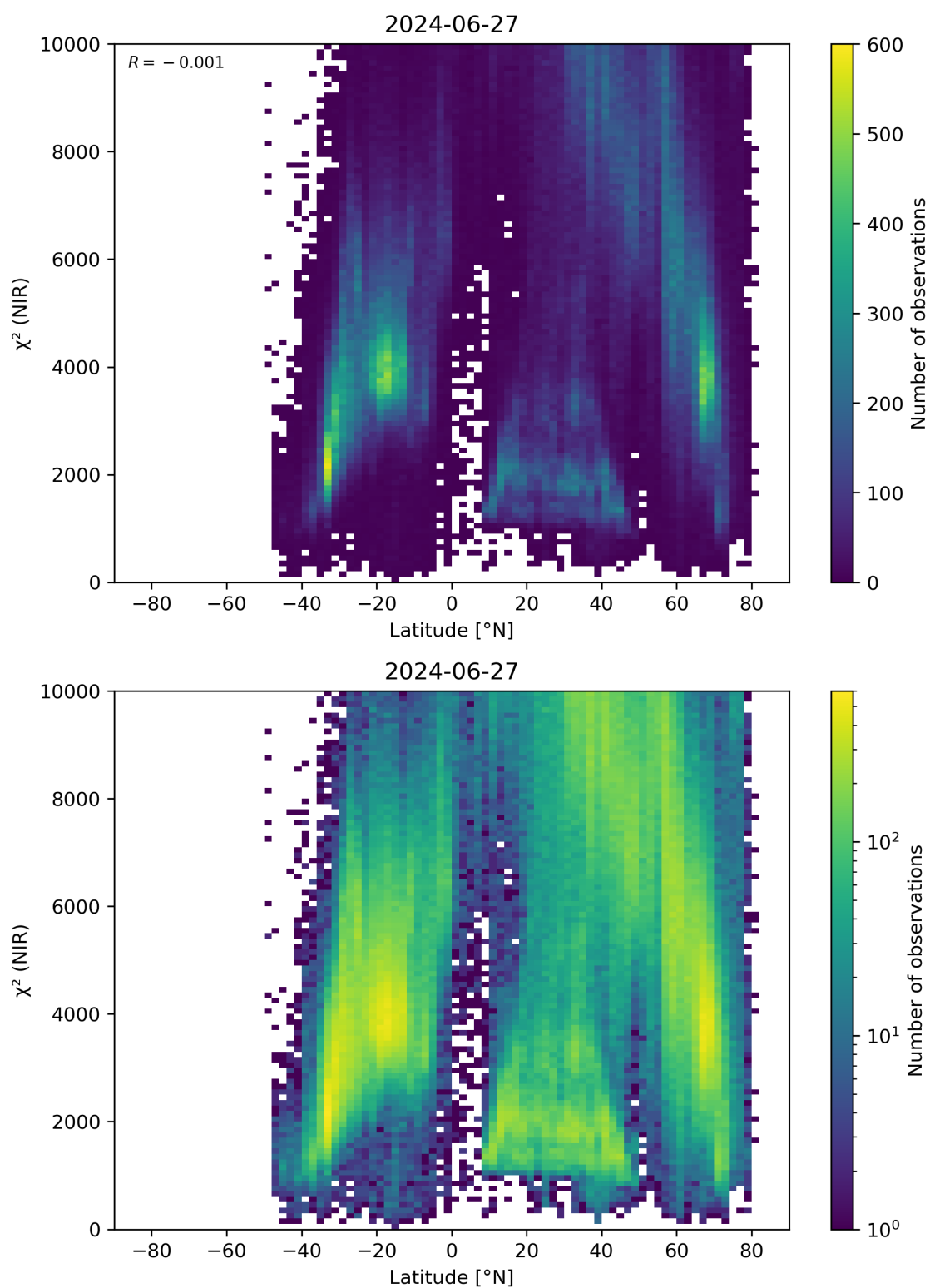
Figure 53: Scatter density plot of “Latitude” against “ \chi^2 (NIR)” for 2024-06-26 to 2024-06-28.
