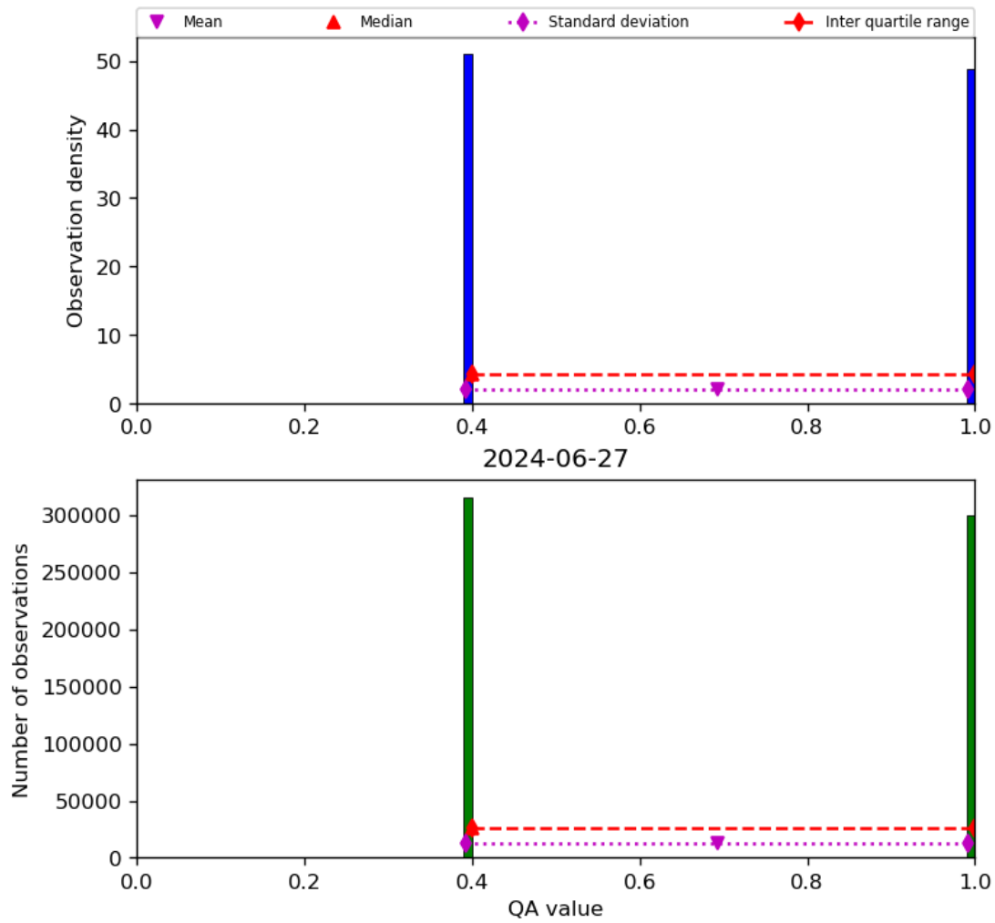
Figure 22: Histogram of “QA value” for 2024-06-26 to 2024-06-28
