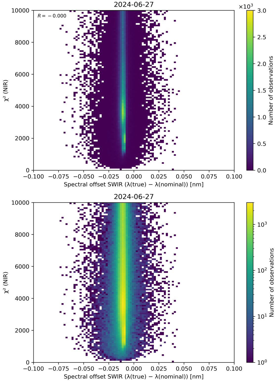
Figure 117: Scatter density plot of “Spectral offset SWIR ( \lambda(\text{true}) - \lambda(\text{nominal}) )” against “ \chi^2 (NIR)” for 2024-06-26 to 2024-06-28.
