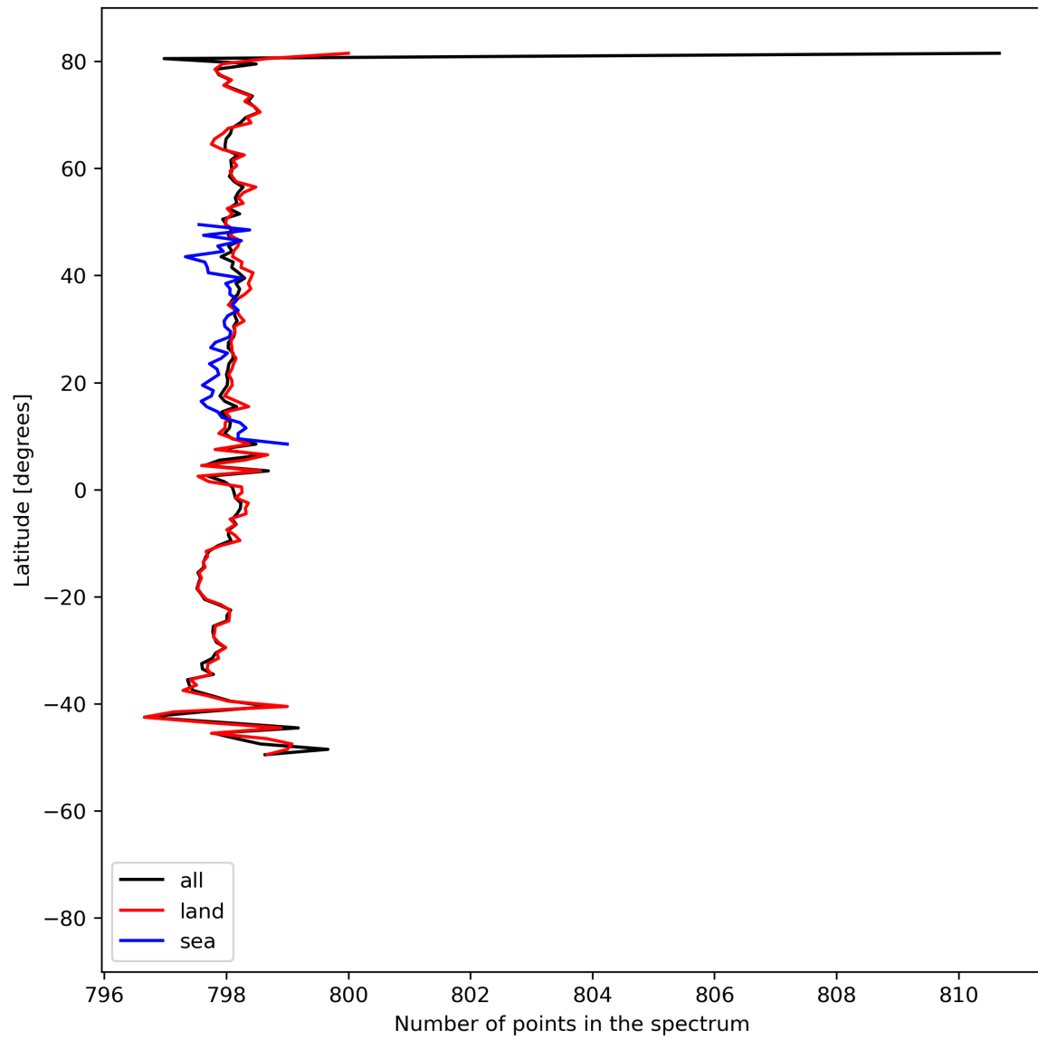
Figure 15: Zonal average of “Number of points in the spectrum” for 2024-06-26 to 2024-06-28.
