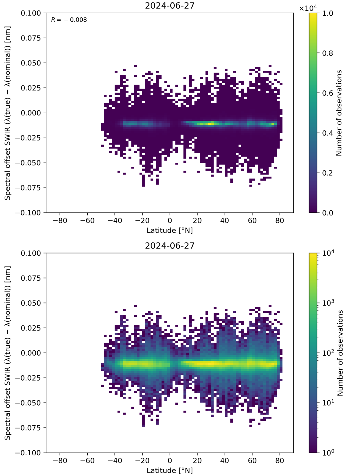
Figure 62: Scatter density plot of “Latitude” against “Spectral offset SWIR ( \lambda(\text{true}) - \lambda(\text{nominal}) )” for 2024-06-26 to 2024-06-28.
