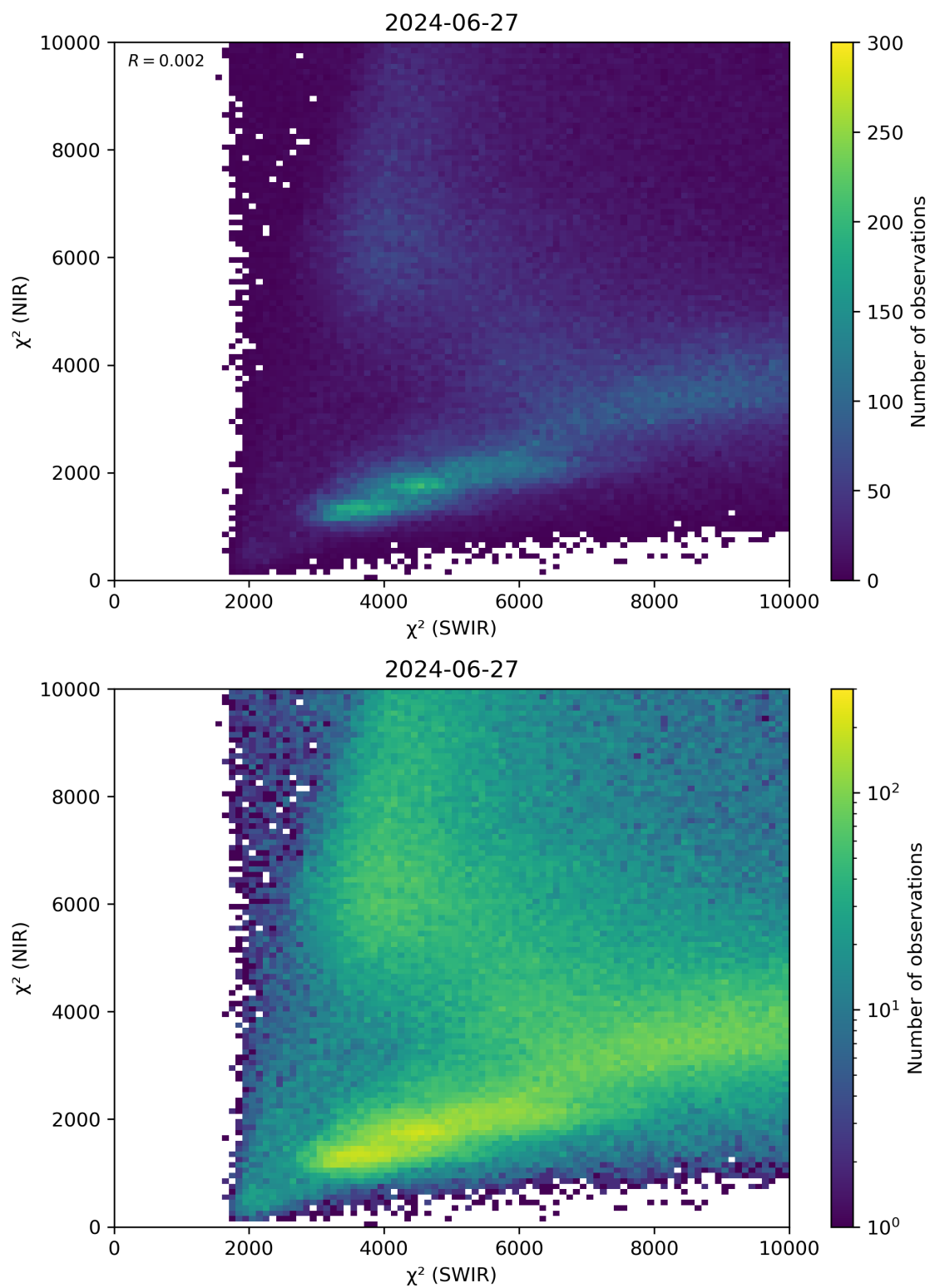
Figure 47: Scatter density plot of “ \chi^2 (SWIR)” against “ \chi^2 (NIR)” for 2024-06-26 to 2024-06-28.
