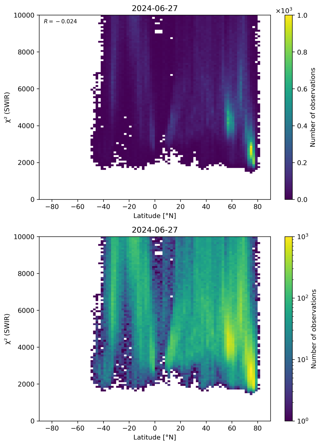
Figure 54: Scatter density plot of “Latitude” against “ \chi^2 (SWIR)” for 2024-06-26 to 2024-06-28.
