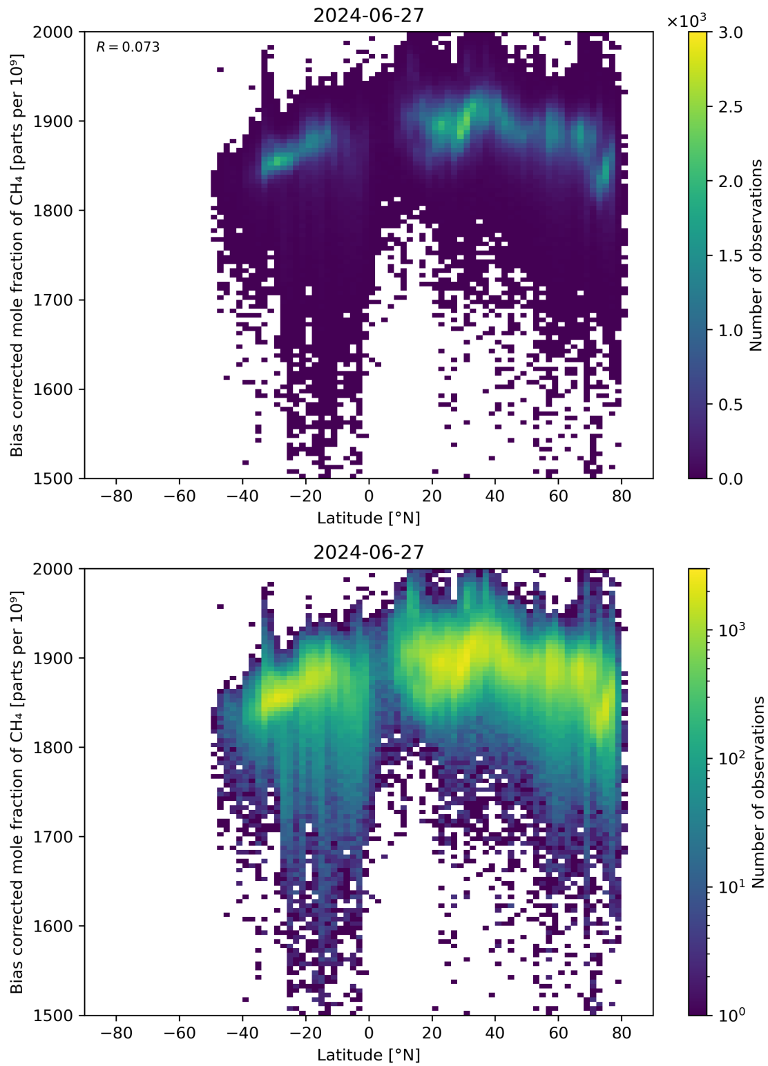
Figure 58: Scatter density plot of “Latitude” against “Bias corrected mole fraction of CH 4 ” for 2024-06-26 to 2024-06-28.
