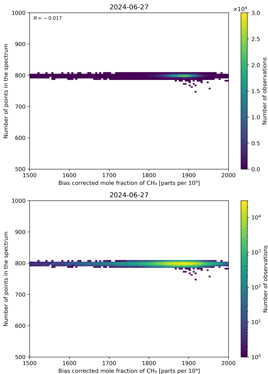
Figure 68: Scatter density plot of “Bias corrected mole fraction of CH 4 ” against “Number of points in the spectrum” for 2024-06-26 to 2024-06-28.
