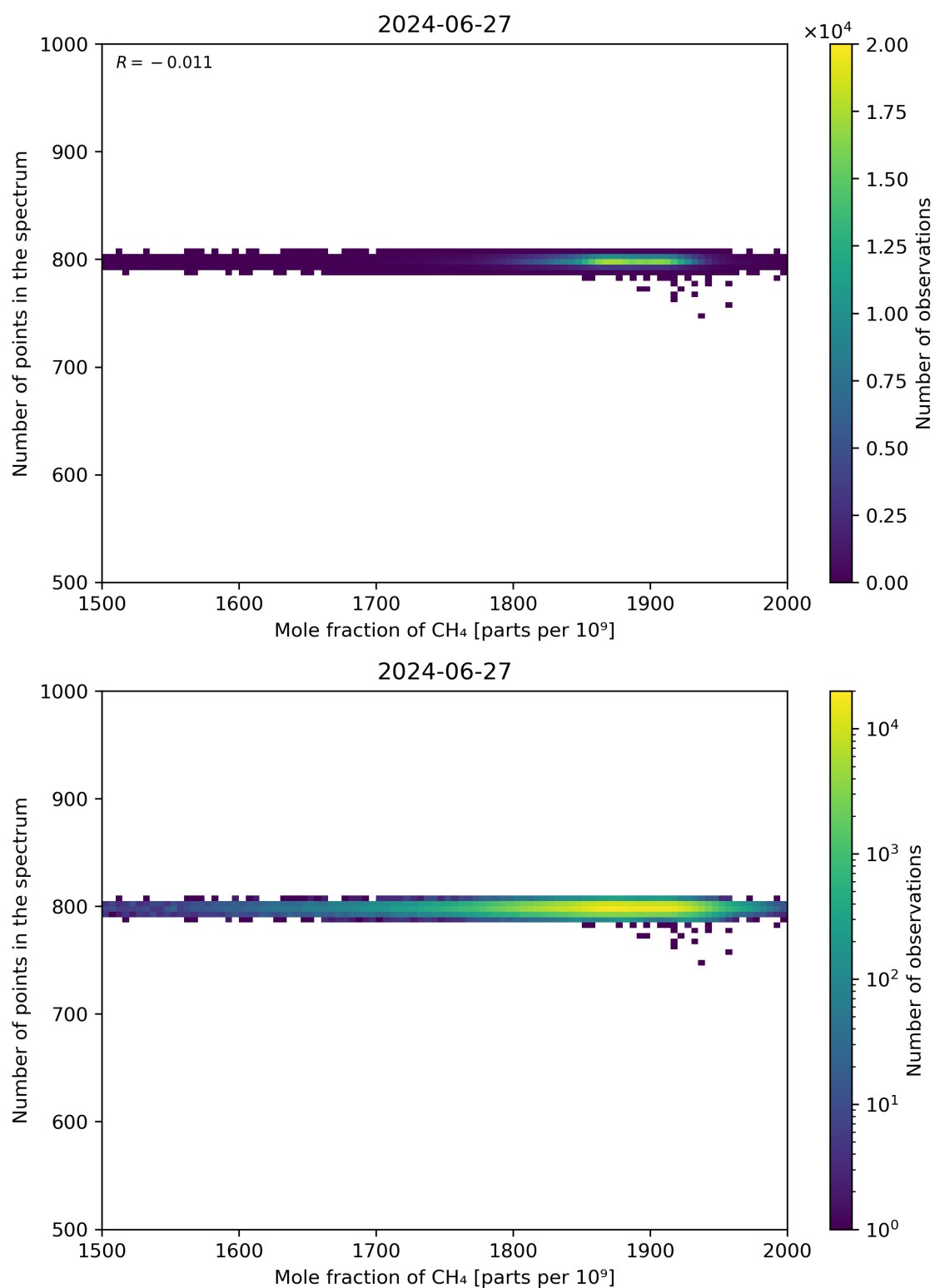
Figure 77: Scatter density plot of “Mole fraction of CH 4 ” against “Number of points in the spectrum” for 2024-06-26 to 2024-06-28.
