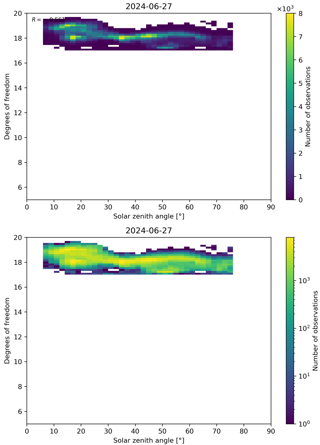
Figure 96: Scatter density plot of “Solar zenith angle” against “Degrees of freedom” for 2024-06-26 to 2024-06-28.
