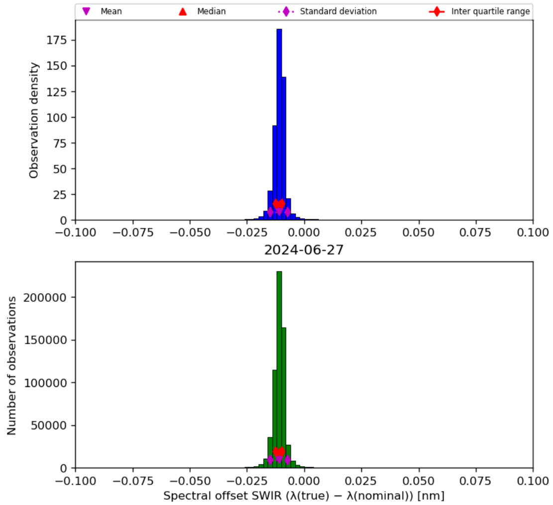
Figure 27: Histogram of “Spectral offset SWIR ( \lambda(\text{true}) - \lambda(\text{nominal}) )” for 2024-06-26 to 2024-06-28
