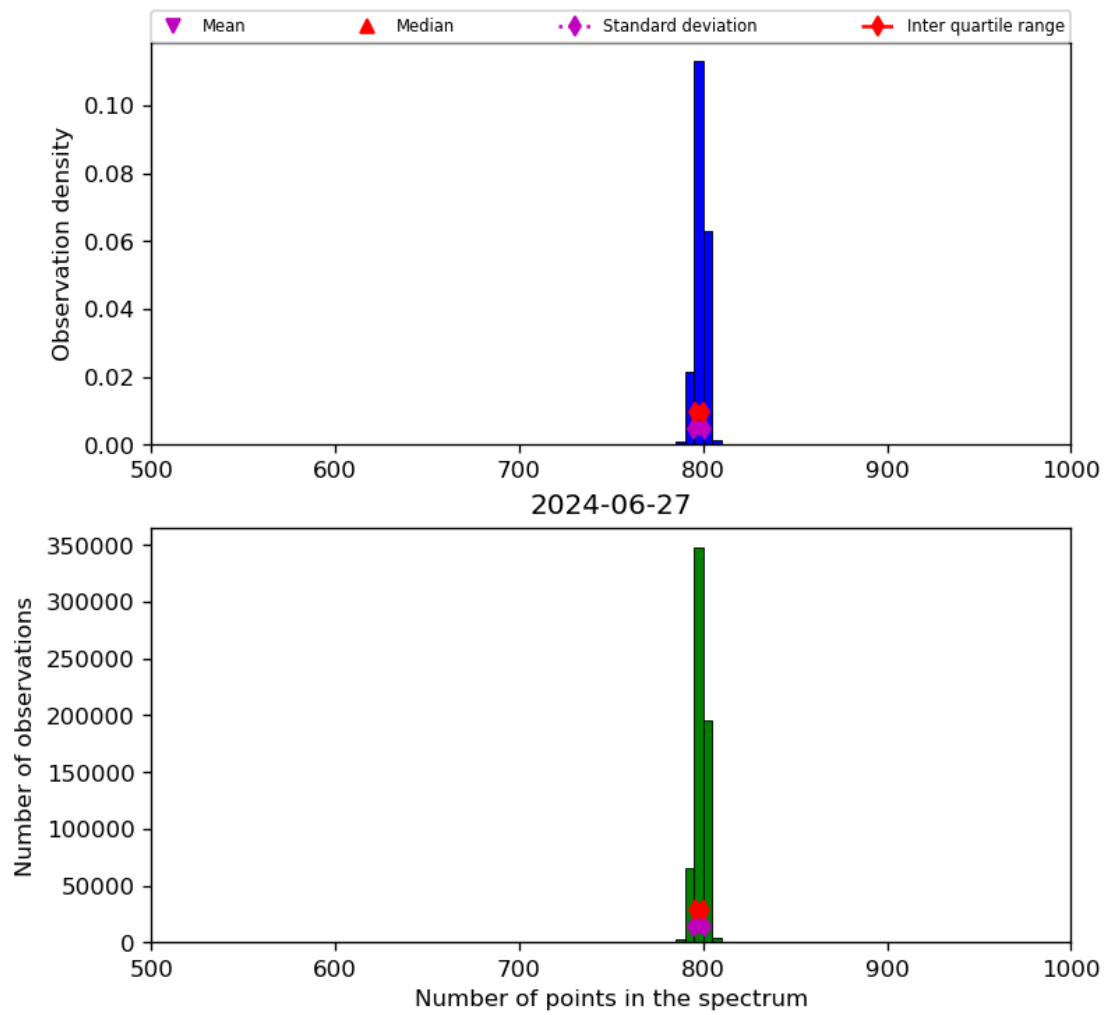
Figure 26: Histogram of “Number of points in the spectrum” for 2024-06-26 to 2024-06-28
