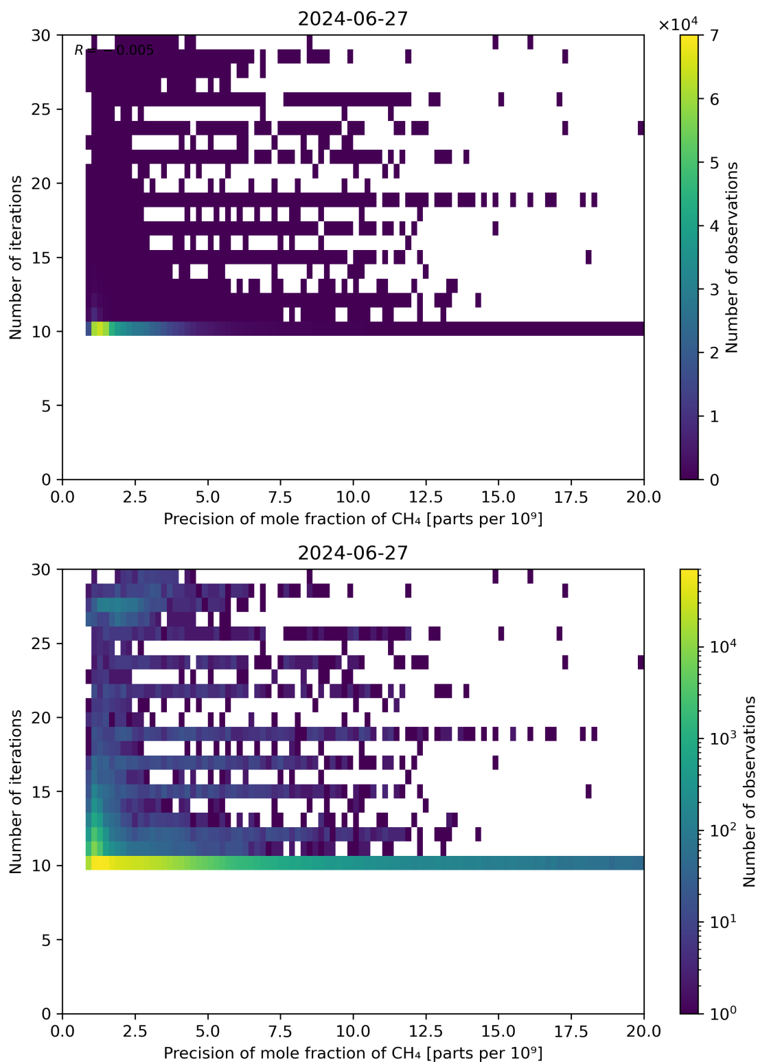
Figure 83: Scatter density plot of “Precision of mole fraction of CH 4 ” against “Number of iterations” for 2024-06-26 to 2024-06-28.
