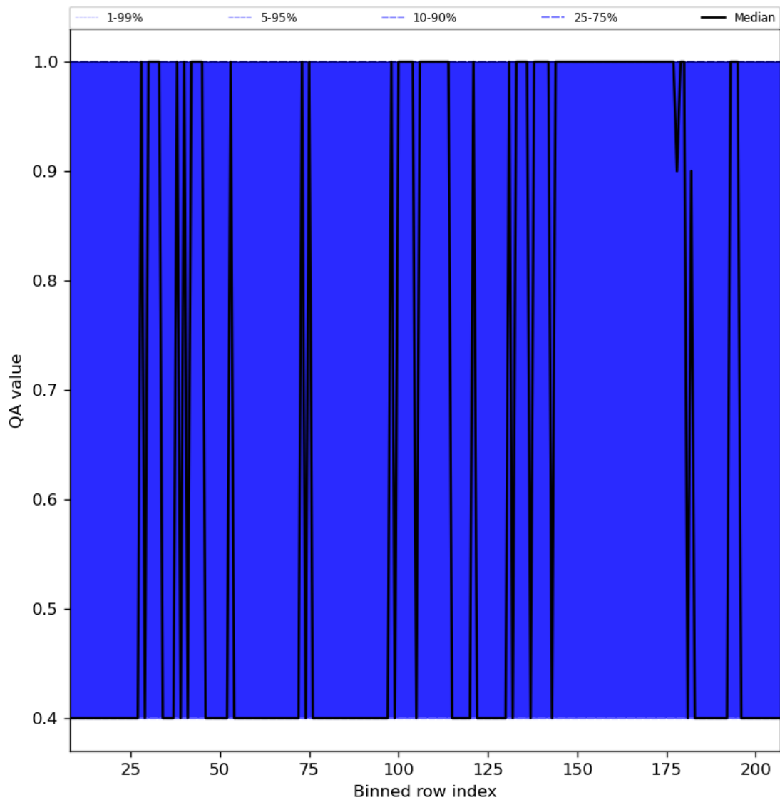
Figure 33: Along track statistics of “QA value” for 2024-06-26 to 2024-06-28
