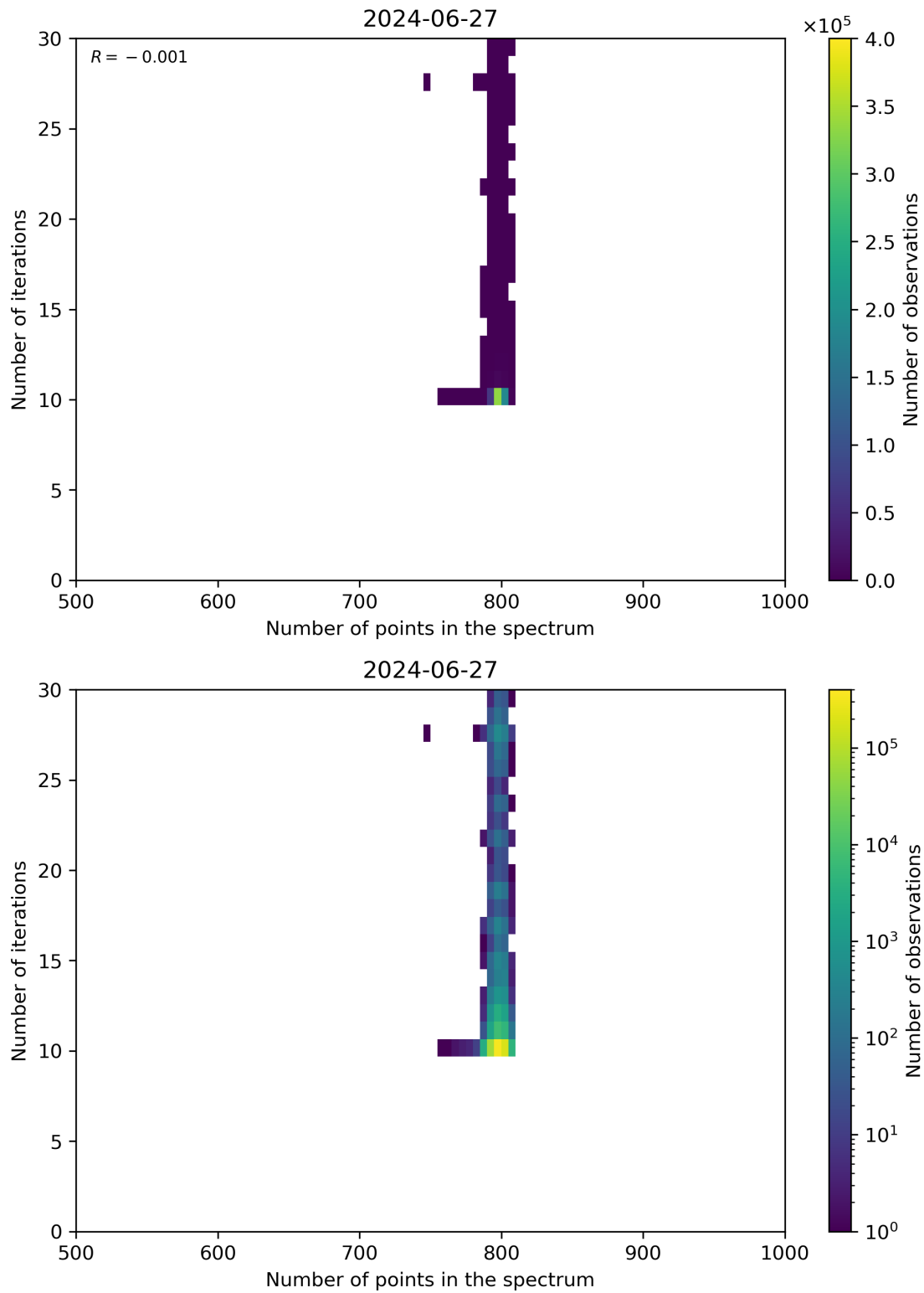
Figure 92: Scatter density plot of “Number of points in the spectrum” against “Number of iterations” for 2024-06-26 to 2024-06-28.
