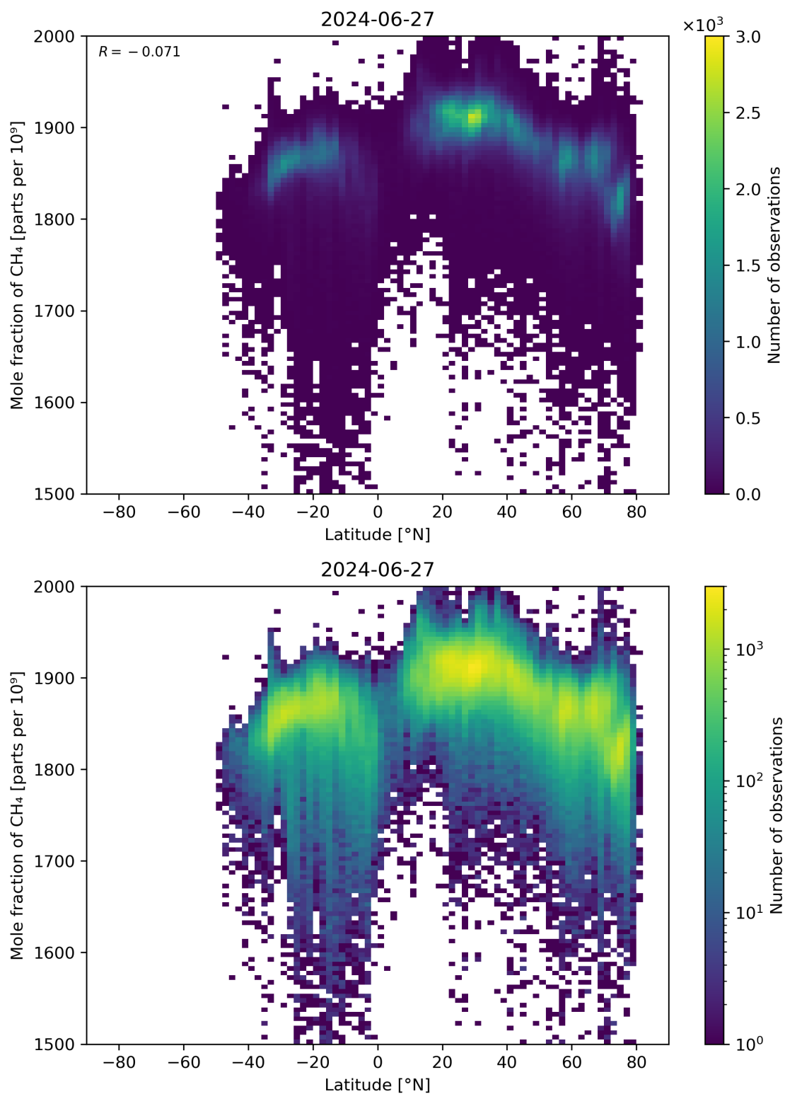
Figure 57: Scatter density plot of “Latitude” against “Mole fraction of \text{CH}_4 ” for 2024-06-26 to 2024-06-28.
