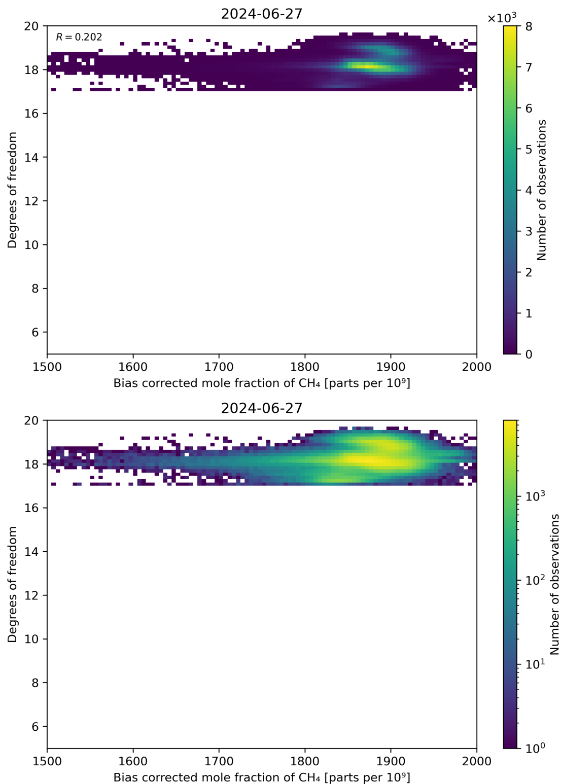
Figure 65: Scatter density plot of “Bias corrected mole fraction of CH 4 ” against “Degrees of freedom” for 2024-06-26 to 2024-06-28.
