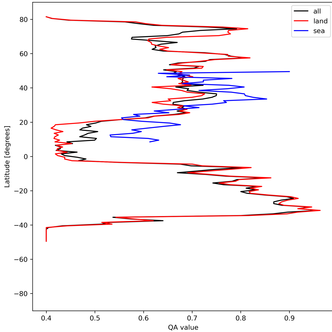
Figure 11: Zonal average of “QA value” for 2024-06-26 to 2024-06-28.
