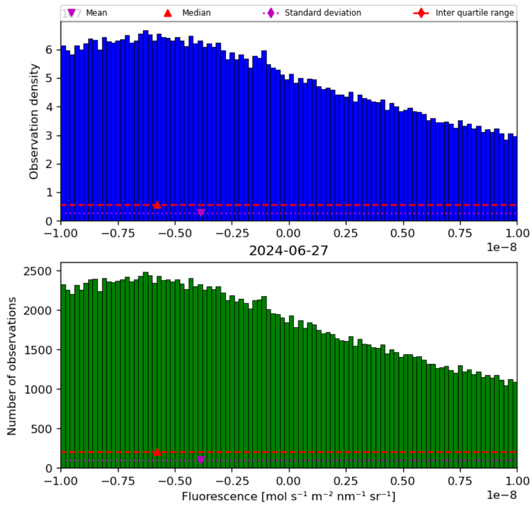
Figure 32: Histogram of “Fluorescence” for 2024-06-26 to 2024-06-28
