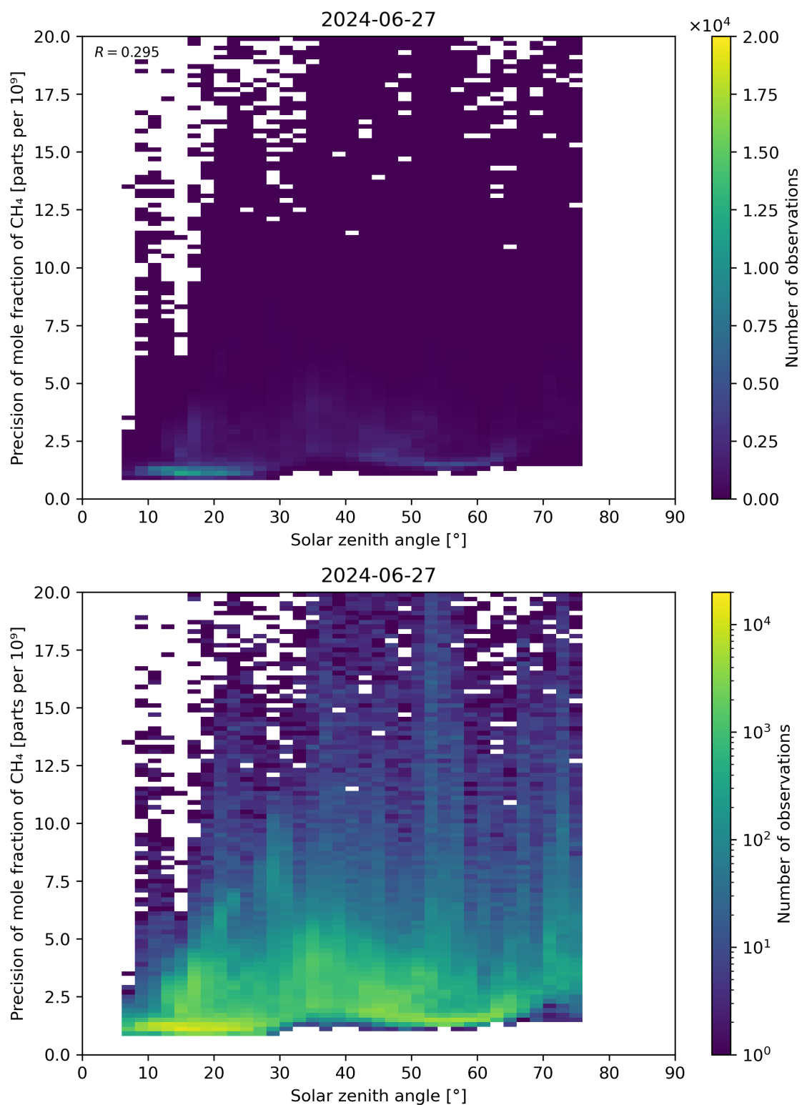
Figure 101: Scatter density plot of “Solar zenith angle” against “Precision of mole fraction of CH 4 ” for 2024-06-26 to 2024-06-28.
