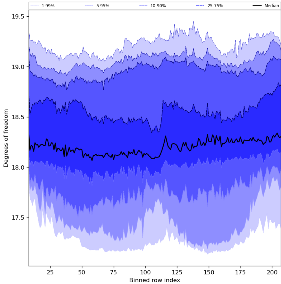
Figure 41: Along track statistics of “Degrees of freedom” for 2024-06-26 to 2024-06-28
