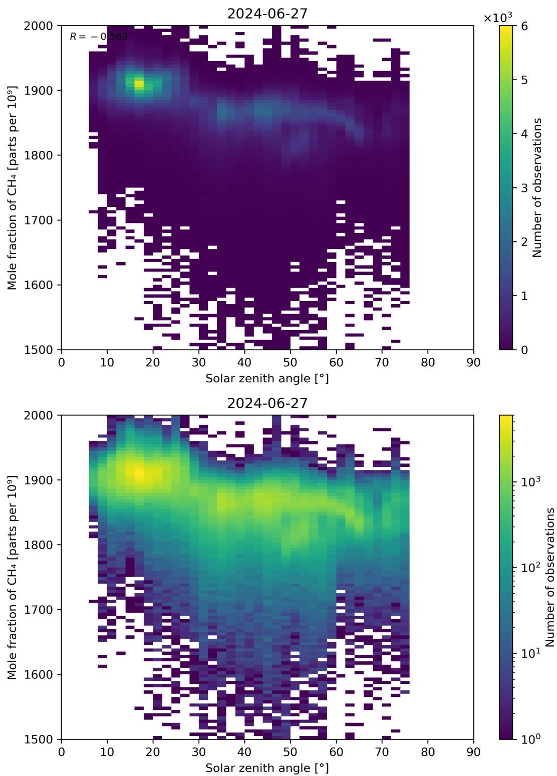
Figure 99: Scatter density plot of “Solar zenith angle” against “Mole fraction of CH 4 ” for 2024-06-26 to 2024-06-28.
