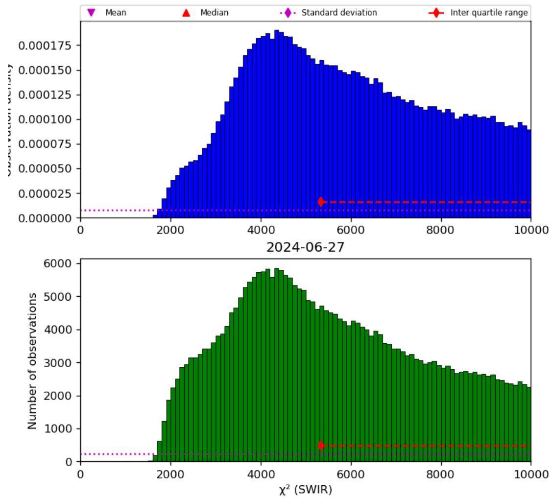
Figure 28: Histogram of “ \chi^2 (SWIR)” for 2024-06-26 to 2024-06-28
