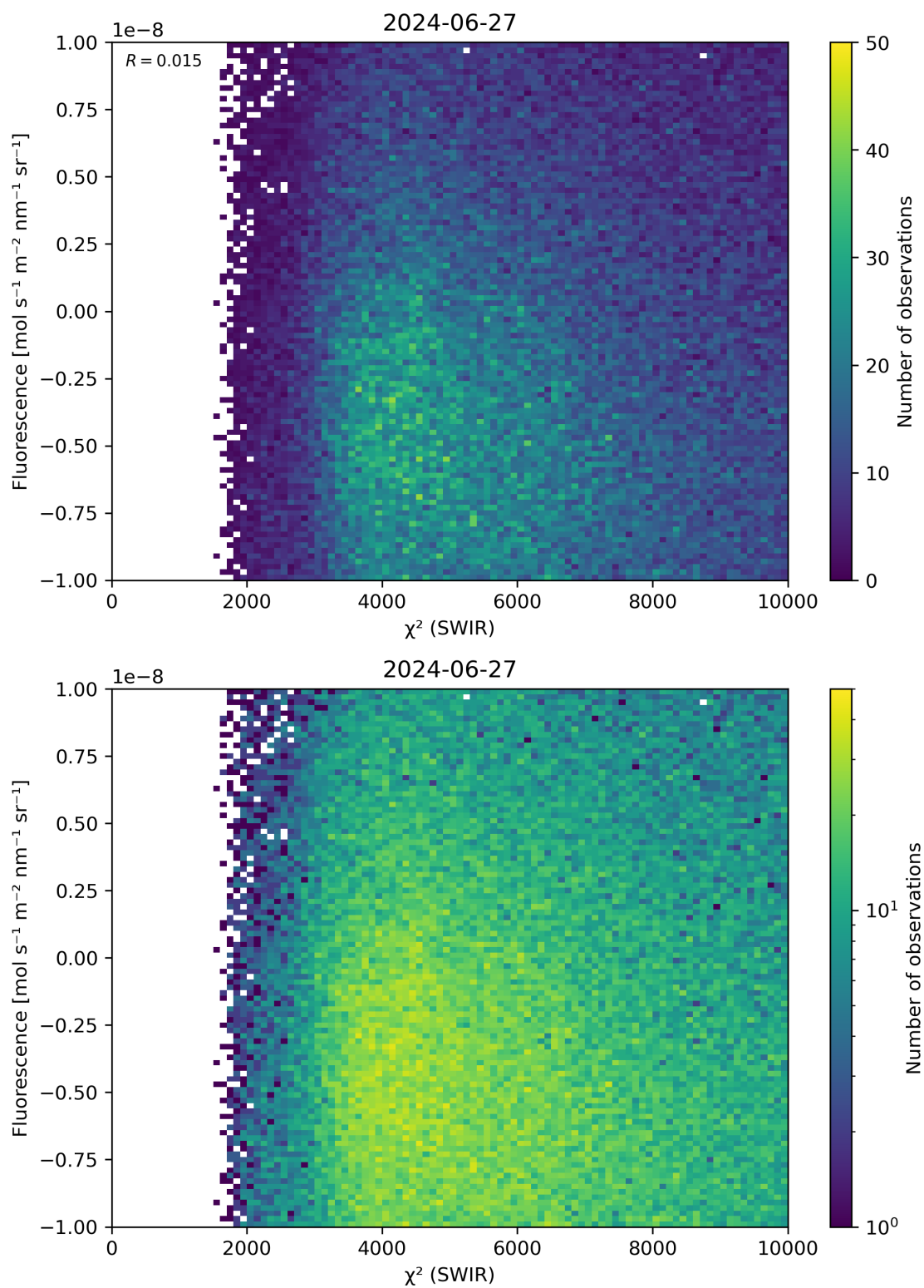
Figure 49: Scatter density plot of “ \chi^2 (SWIR)” against “Fluorescence” for 2024-06-26 to 2024-06-28.
