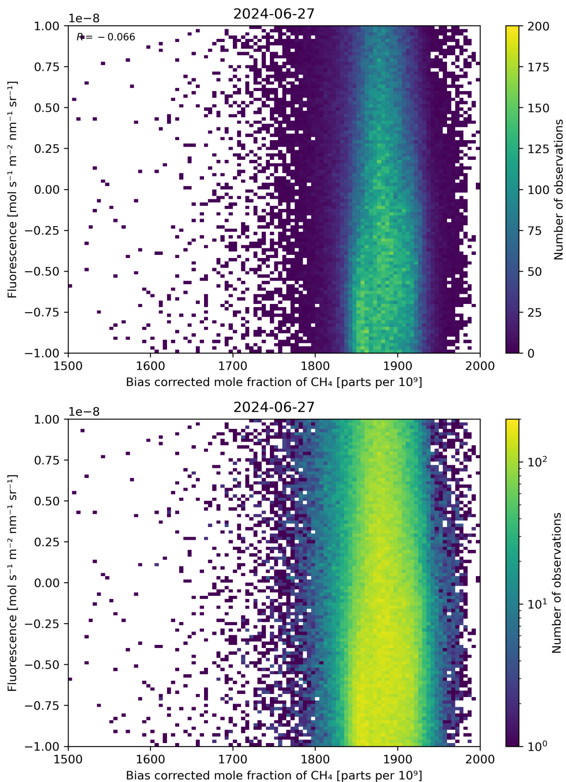
Figure 66: Scatter density plot of “Bias corrected mole fraction of \text{CH}_4 ” against “Fluorescence” for 2024-06-26 to 2024-06-28.
