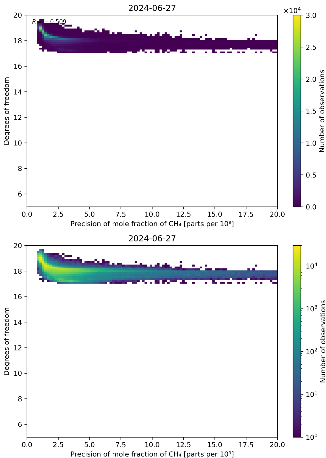
Figure 80: Scatter density plot of “Precision of mole fraction of CH 4 ” against “Degrees of freedom” for 2024-06-26 to 2024-06-28.
