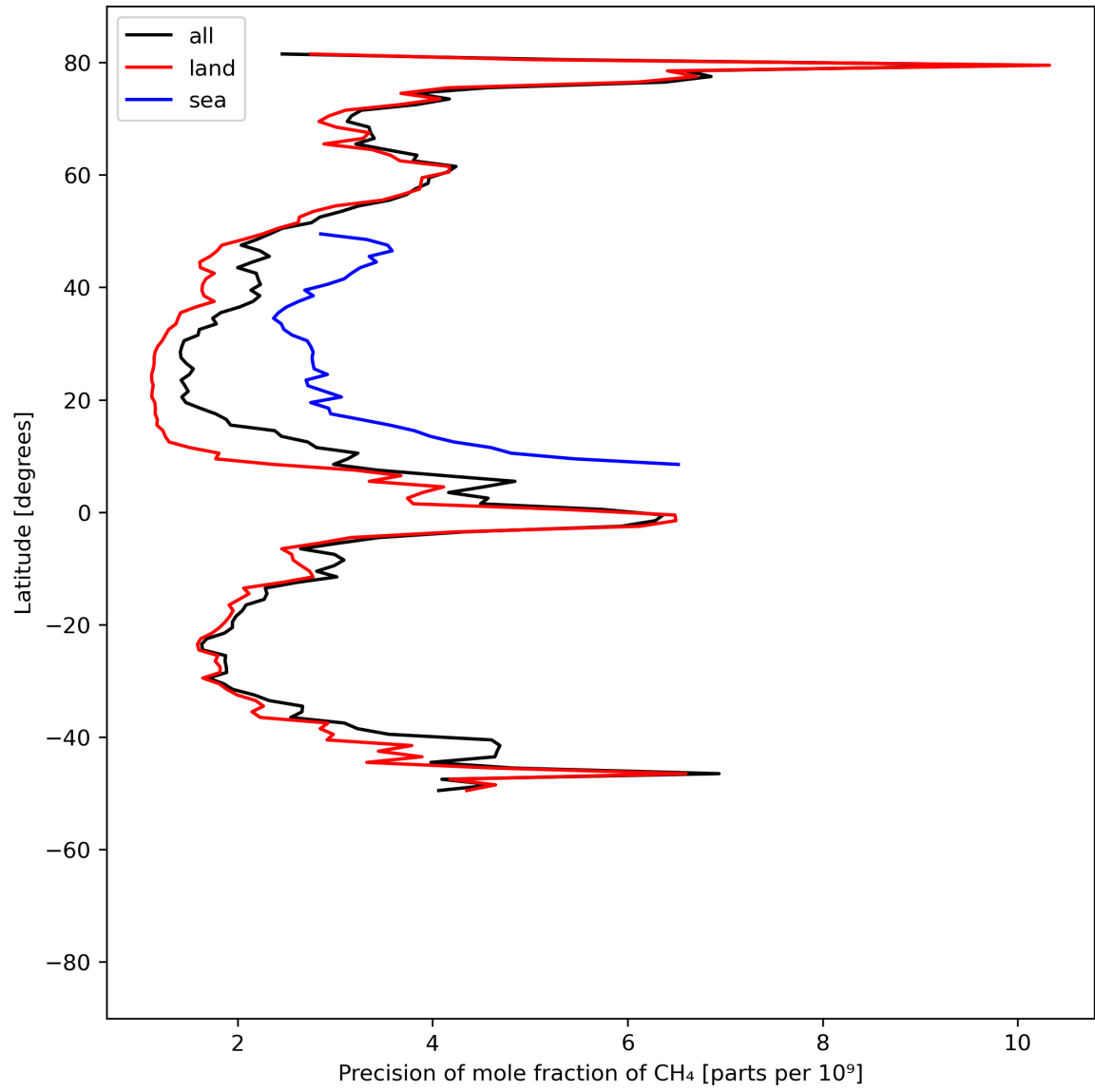
Figure 13: Zonal average of “Precision of mole fraction of CH 4 ” for 2024-06-26 to 2024-06-28.
