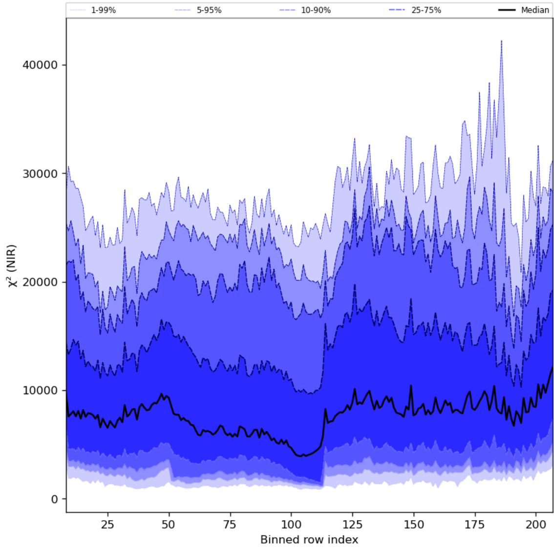
Figure 40: Along track statistics of “ \chi^2 (NIR)” for 2024-06-26 to 2024-06-28
