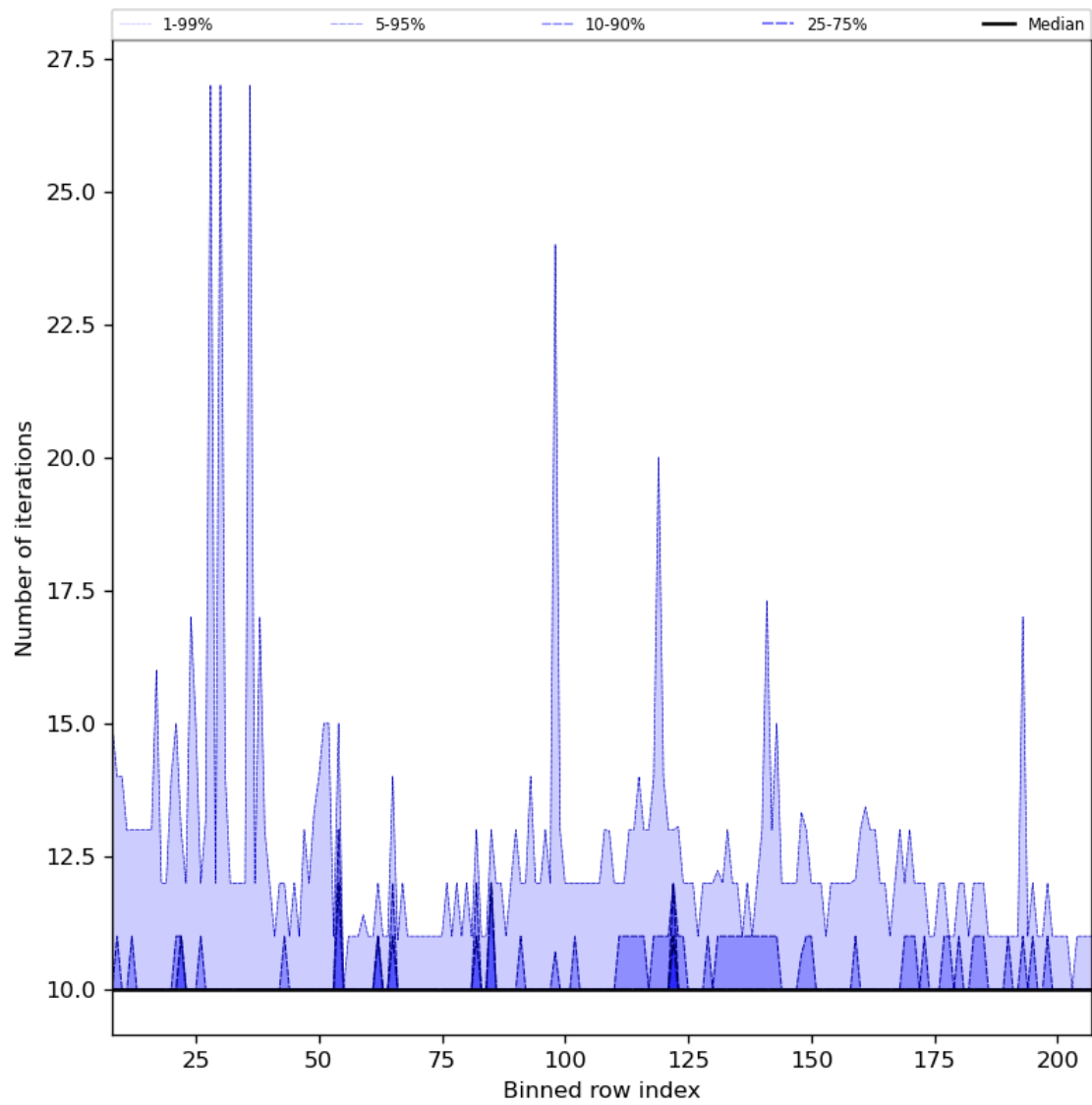
Figure 42: Along track statistics of “Number of iterations” for 2024-06-26 to 2024-06-28
