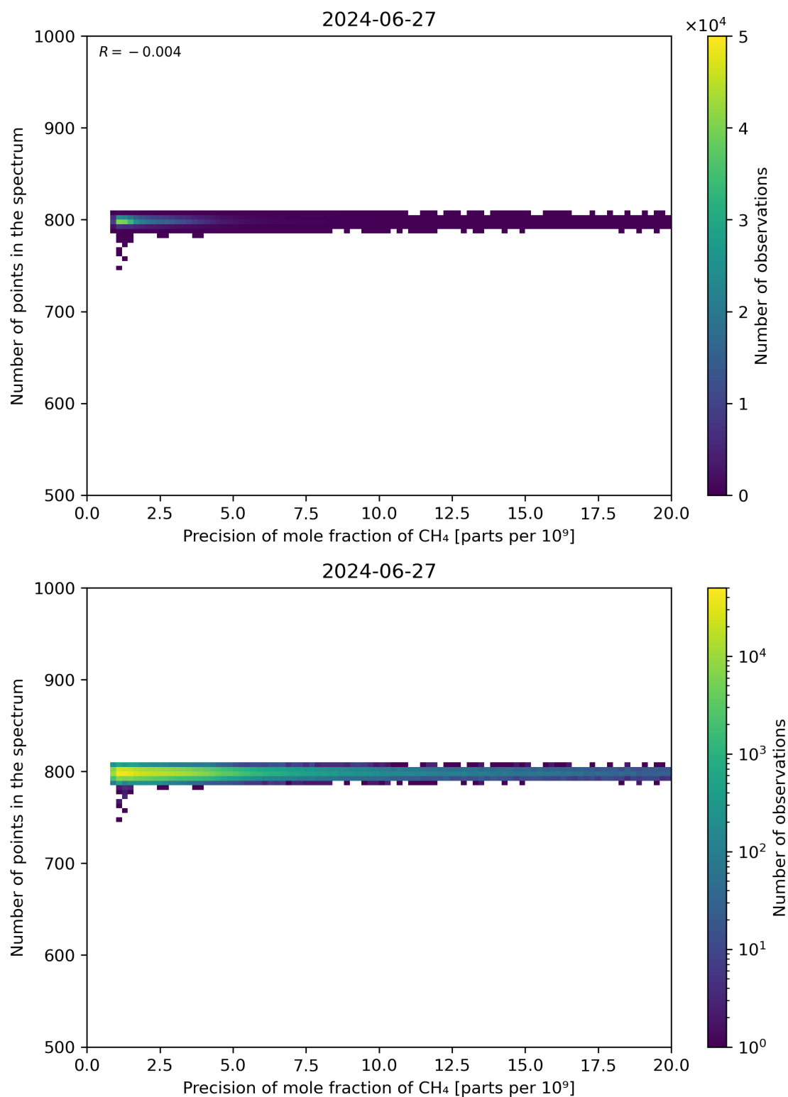
Figure 84: Scatter density plot of “Precision of mole fraction of CH 4 ” against “Number of points in the spectrum” for 2024-06-26 to 2024-06-28.
