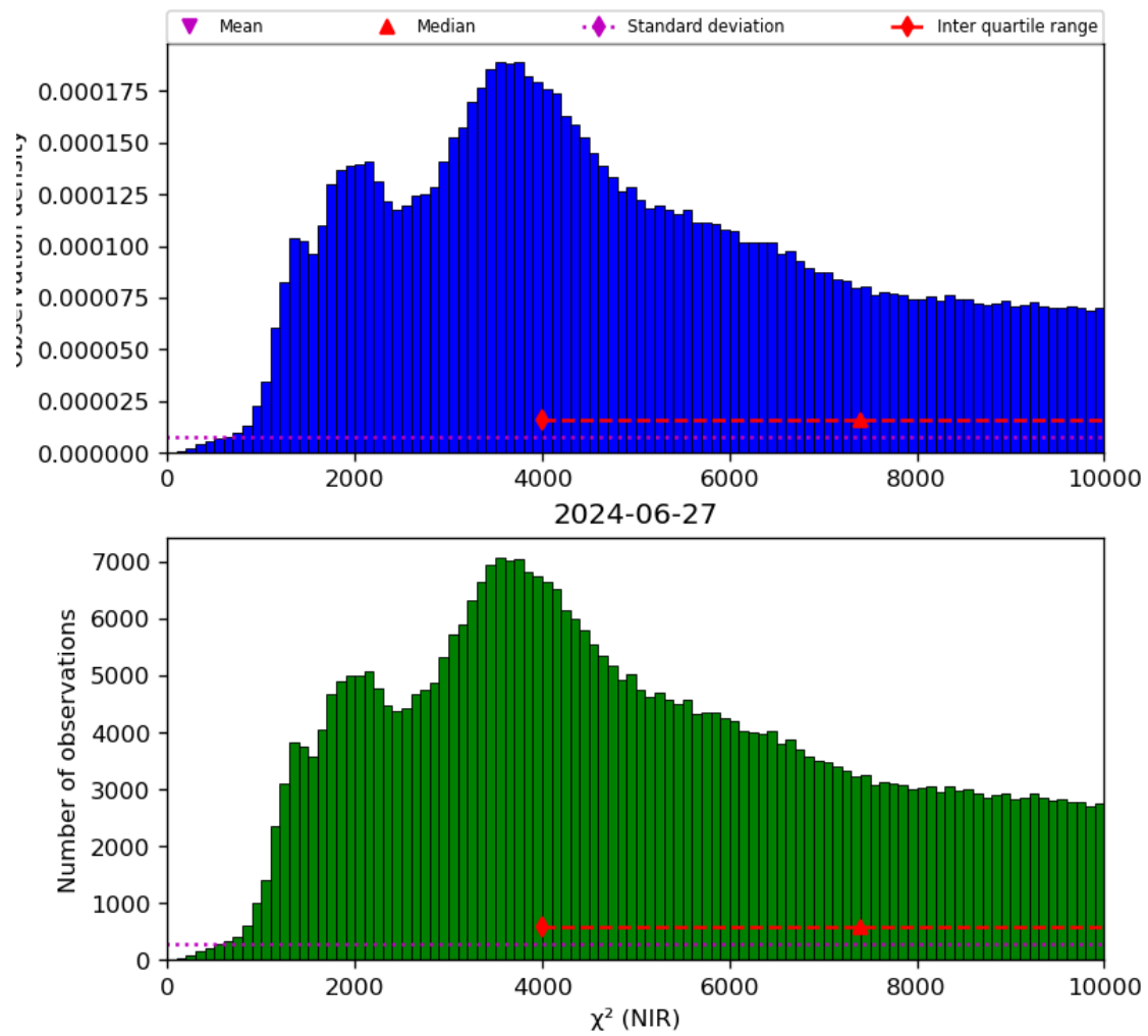
Figure 29: Histogram of “ \chi^2 (NIR)” for 2024-06-26 to 2024-06-28
