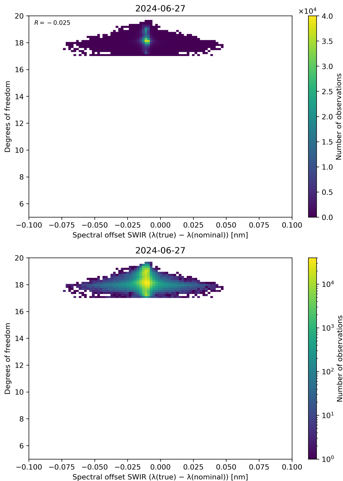
Figure 119: Scatter density plot of “Spectral offset SWIR ( \lambda(\text{true}) - \lambda(\text{nominal}) )” against “Degrees of freedom” for 2024-06-26 to 2024-06-28.
