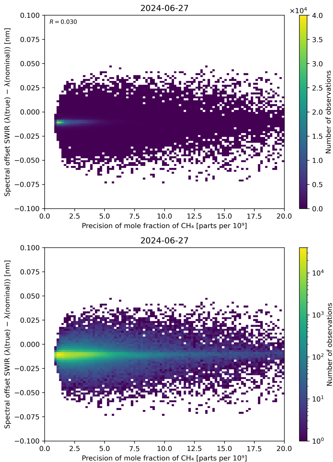
Figure 85: Scatter density plot of “Precision of mole fraction of \text{CH}_4 ” against “Spectral offset SWIR ( \lambda(\text{true}) - \lambda(\text{nominal}) )” for 2024-06-26 to 2024-06-28.
