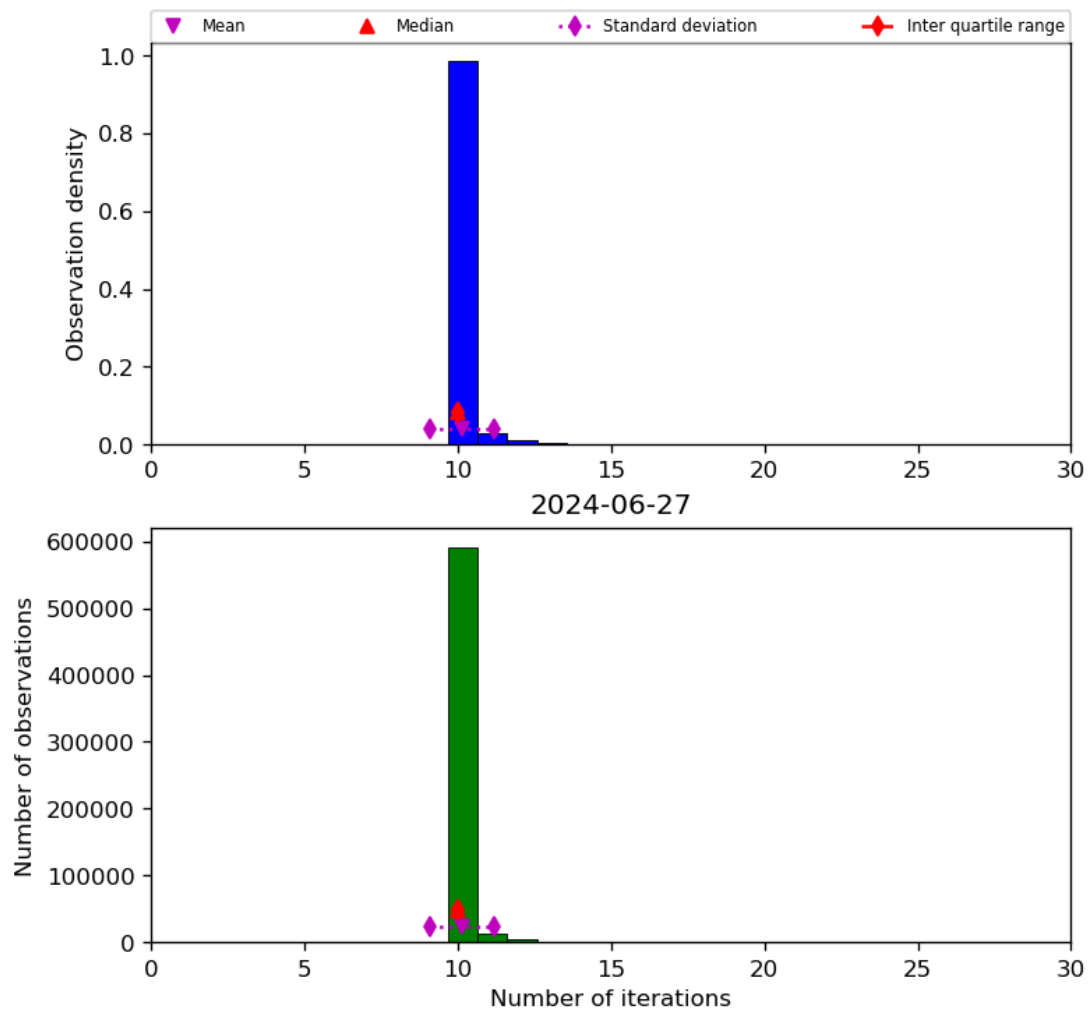
Figure 31: Histogram of “Number of iterations” for 2024-06-26 to 2024-06-28
