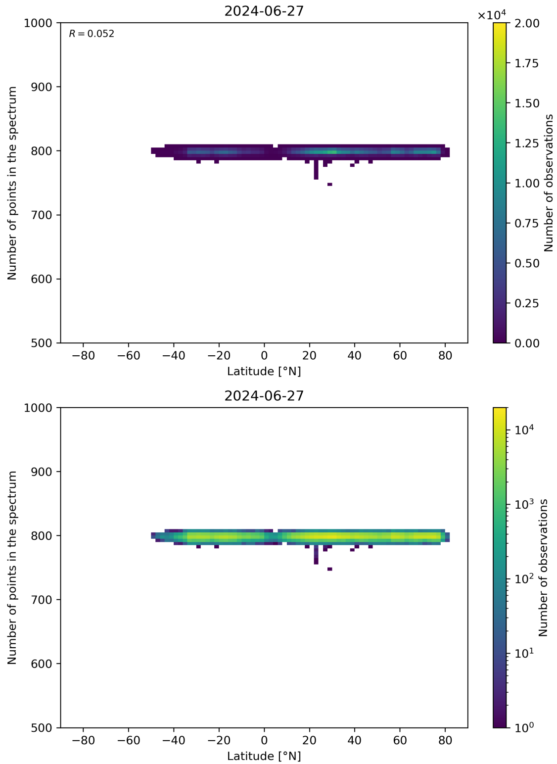
Figure 61: Scatter density plot of “Latitude” against “Number of points in the spectrum” for 2024-06-26 to 2024-06-28.
