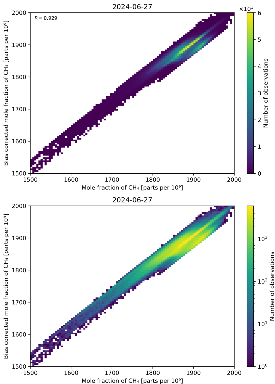
Figure 74: Scatter density plot of “Mole fraction of CH 4 ” against “Bias corrected mole fraction of CH 4 ” for 2024-06-26 to 2024-06-28.
