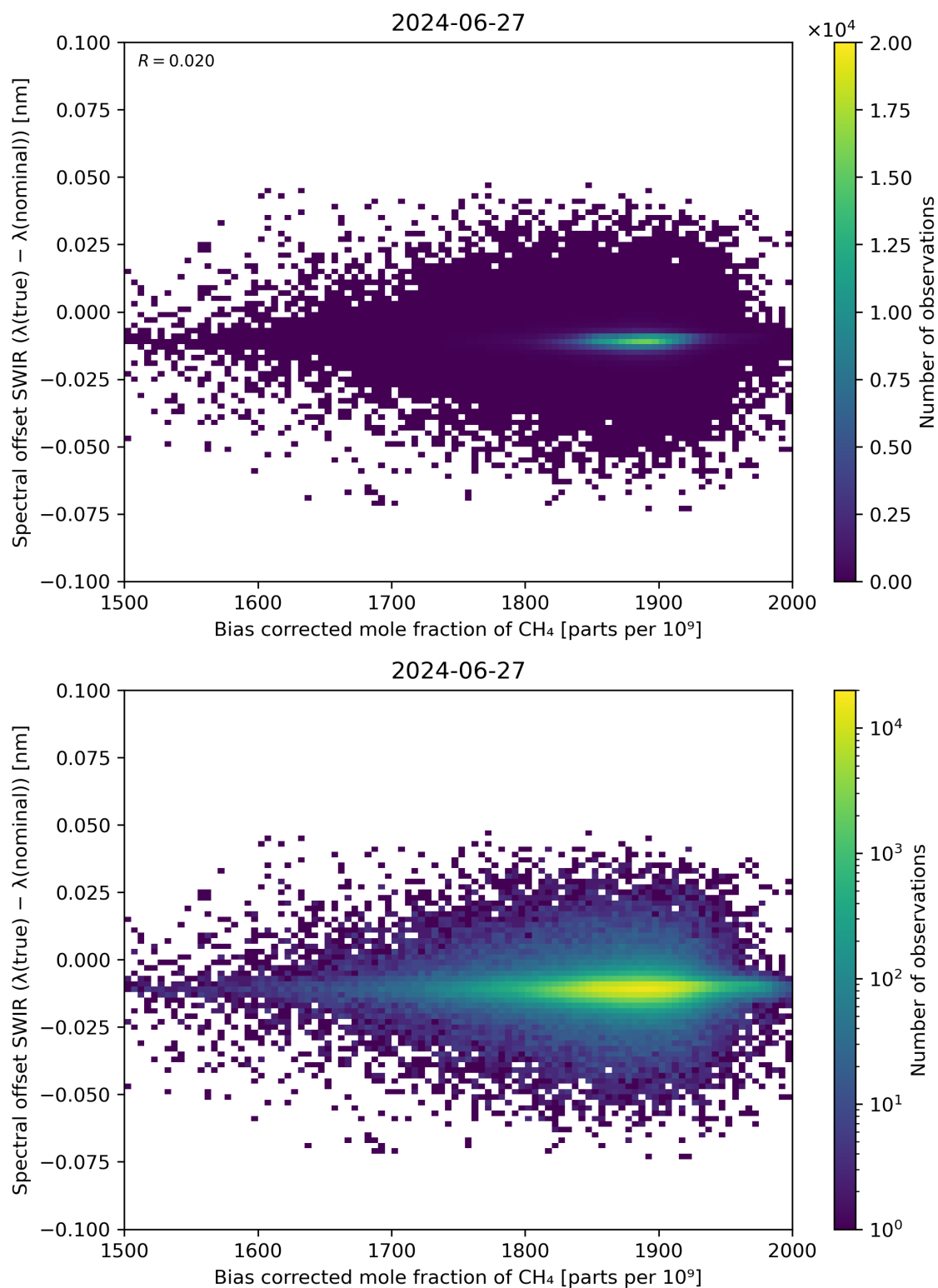
Figure 69: Scatter density plot of “Bias corrected mole fraction of \text{CH}_4 ” against “Spectral offset SWIR ( \lambda(\text{true}) - \lambda(\text{nominal}) )” for 2024-06-26 to 2024-06-28.
