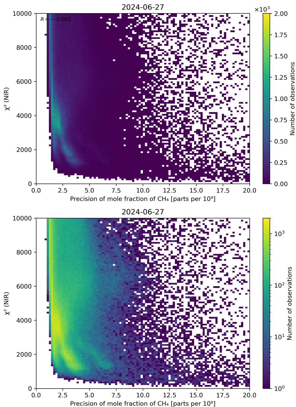
Figure 78: Scatter density plot of “Precision of mole fraction of CH 4 ” against “ \chi^2 (NIR)” for 2024-06-26 to 2024-06-28.
