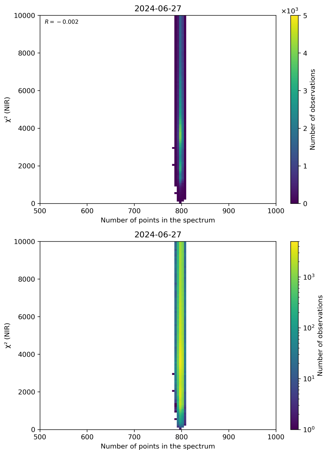
Figure 88: Scatter density plot of “Number of points in the spectrum” against “ \chi^2 (NIR)” for 2024-06-26 to 2024-06-28.
