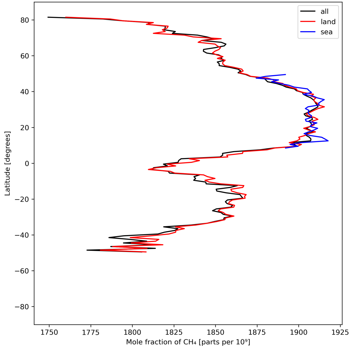
Figure 12: Zonal average of “Mole fraction of \text{CH}_4 ” for 2024-06-26 to 2024-06-28.
