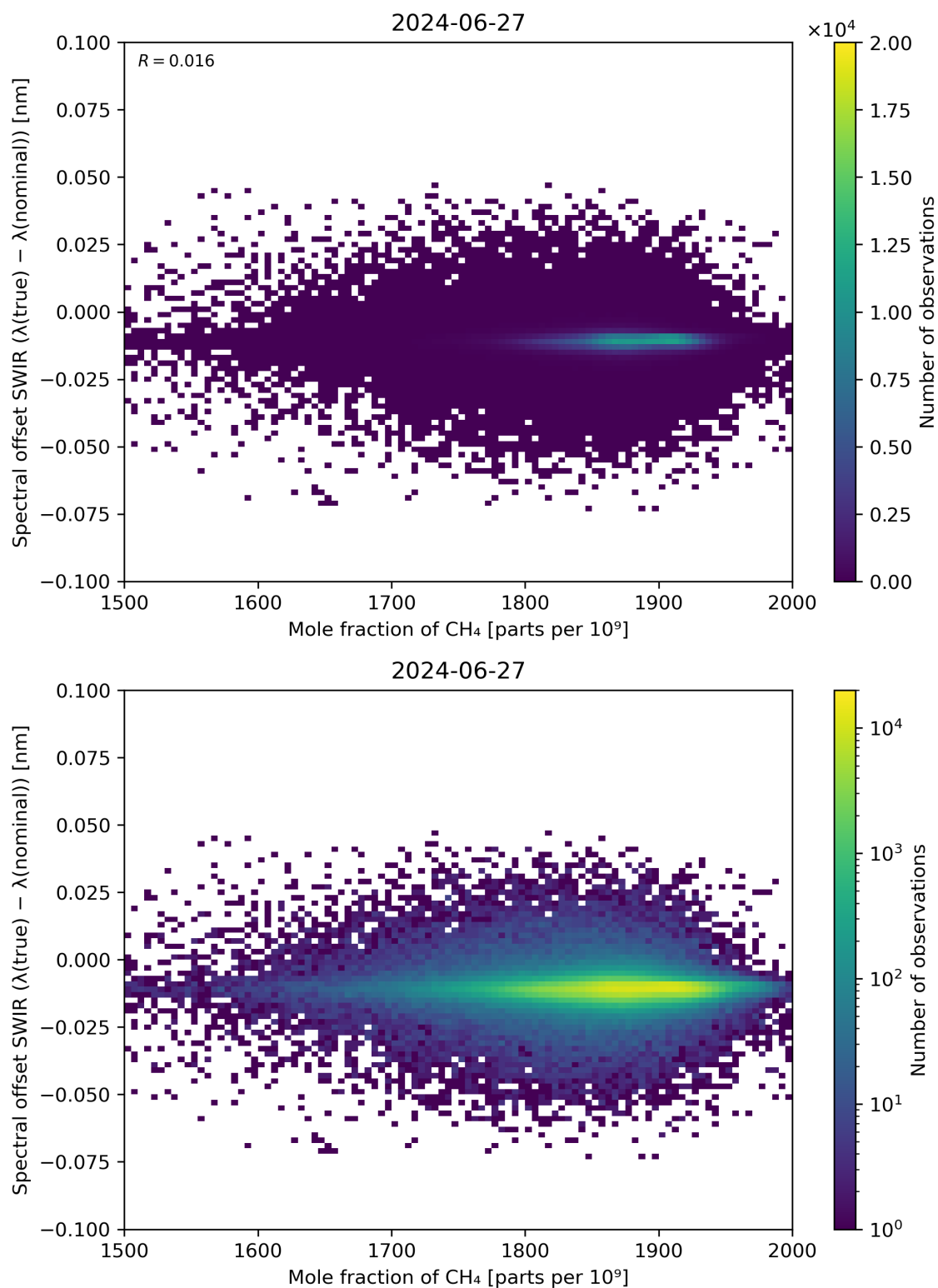
Figure 86: Scatter density plot of “Mole fraction of CH 4 ” against “Spectral offset SWIR ( \lambda(\text{true}) - \lambda(\text{nominal}) )” for 2024-06-26 to 2024-06-28.
