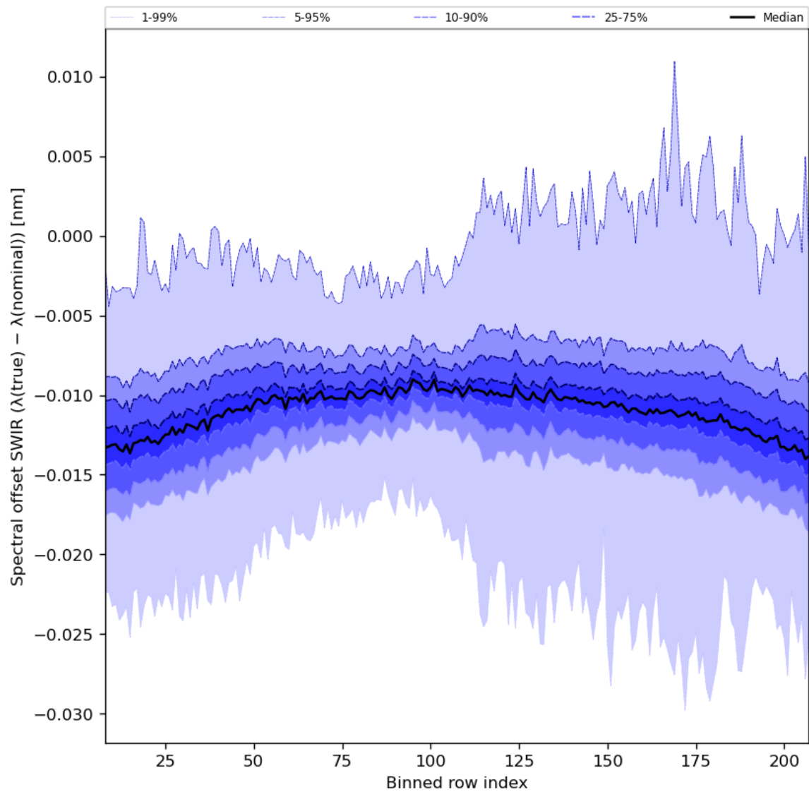
Figure 38: Along track statistics of “Spectral offset SWIR ( \lambda(\text{true}) - \lambda(\text{nominal}) )” for 2024-06-26 to 2024-06-28
