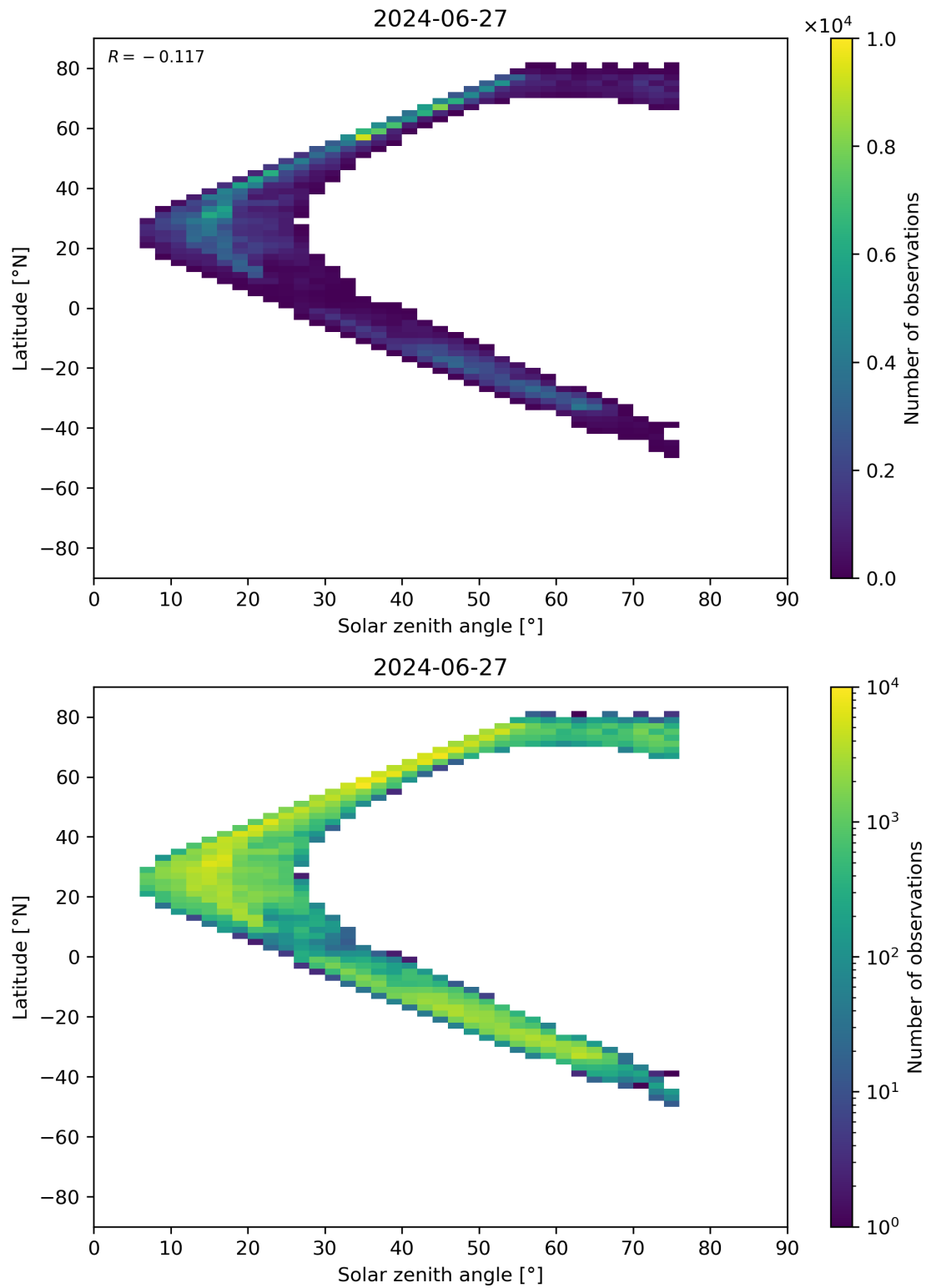
Figure 98: Scatter density plot of “Solar zenith angle” against “Latitude” for 2024-06-26 to 2024-06-28.
