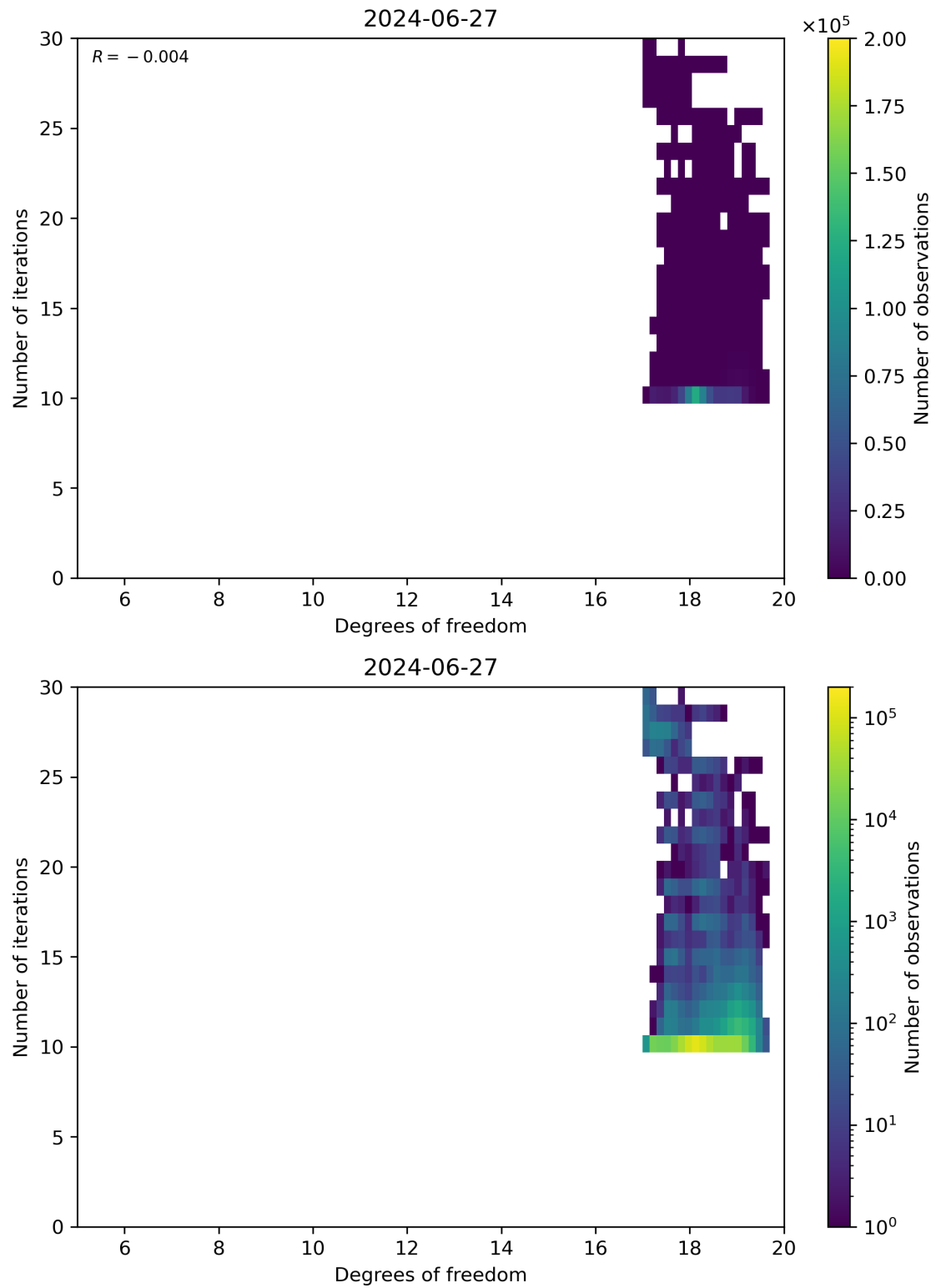
Figure 52: Scatter density plot of “Degrees of freedom” against “Number of iterations” for 2024-06-26 to 2024-06-28.
