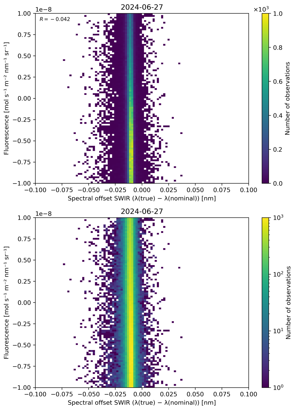
Figure 120: Scatter density plot of “Spectral offset SWIR ( \lambda(\text{true}) - \lambda(\text{nominal}) )” against “Fluorescence” for 2024-06-26 to 2024-06-28.
