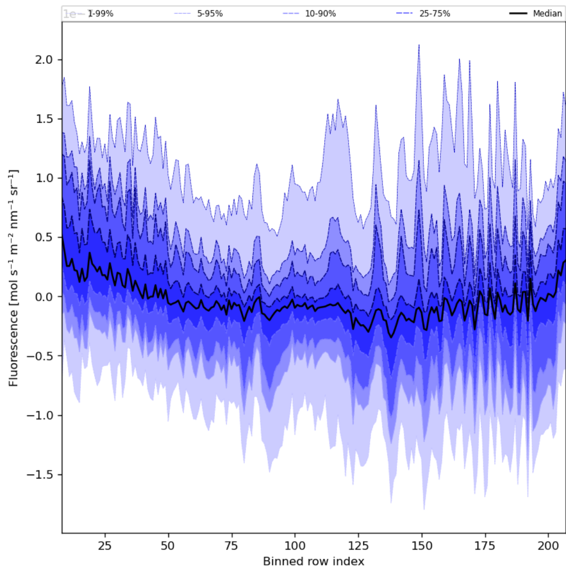
Figure 43: Along track statistics of “Fluorescence” for 2024-06-26 to 2024-06-28
