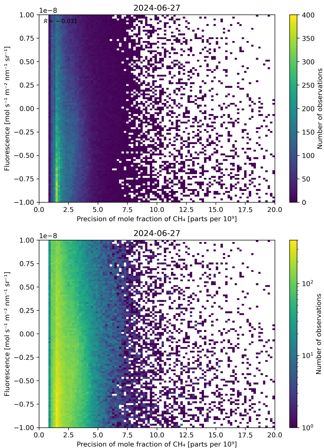
Figure 81: Scatter density plot of “Precision of mole fraction of \text{CH}_4 ” against “Fluorescence” for 2024-06-26 to 2024-06-28.
