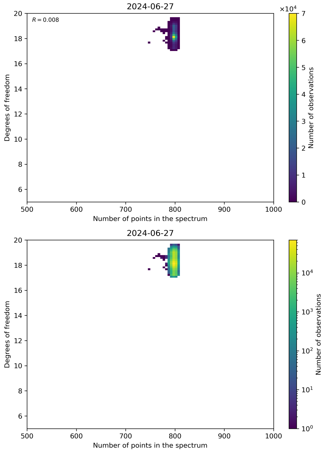
Figure 90: Scatter density plot of “Number of points in the spectrum” against “Degrees of freedom” for 2024-06-26 to 2024-06-28.
