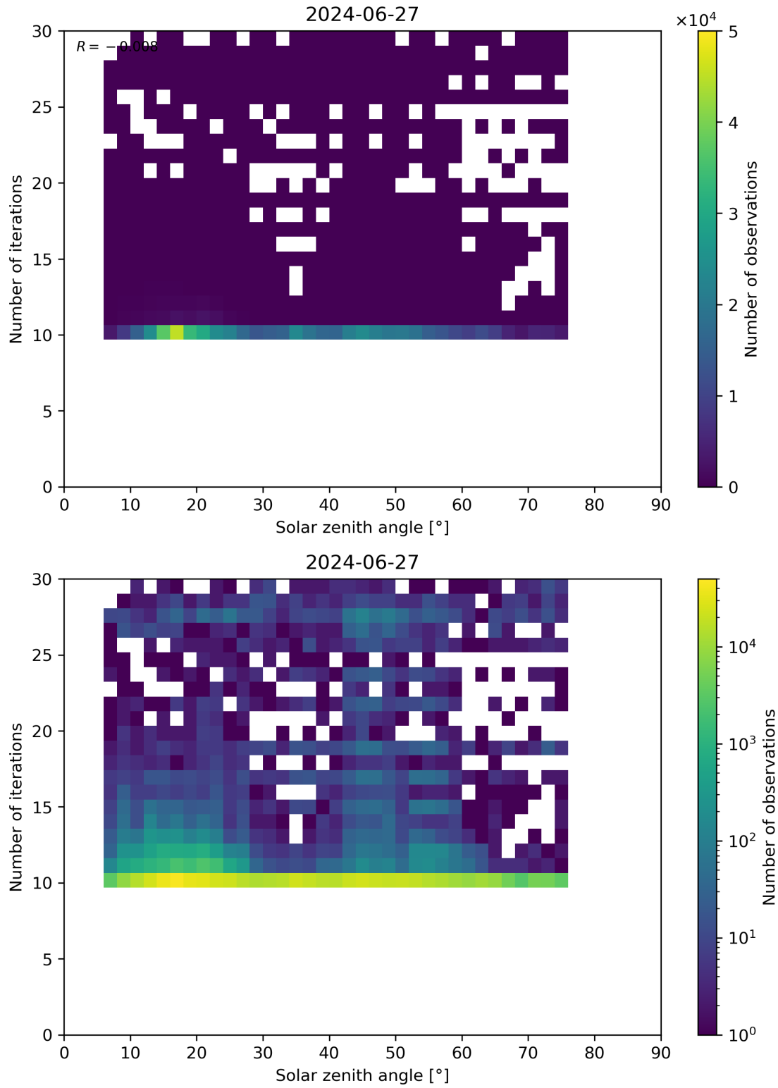
Figure 102: Scatter density plot of “Solar zenith angle” against “Number of iterations” for 2024-06-26 to 2024-06-28.
