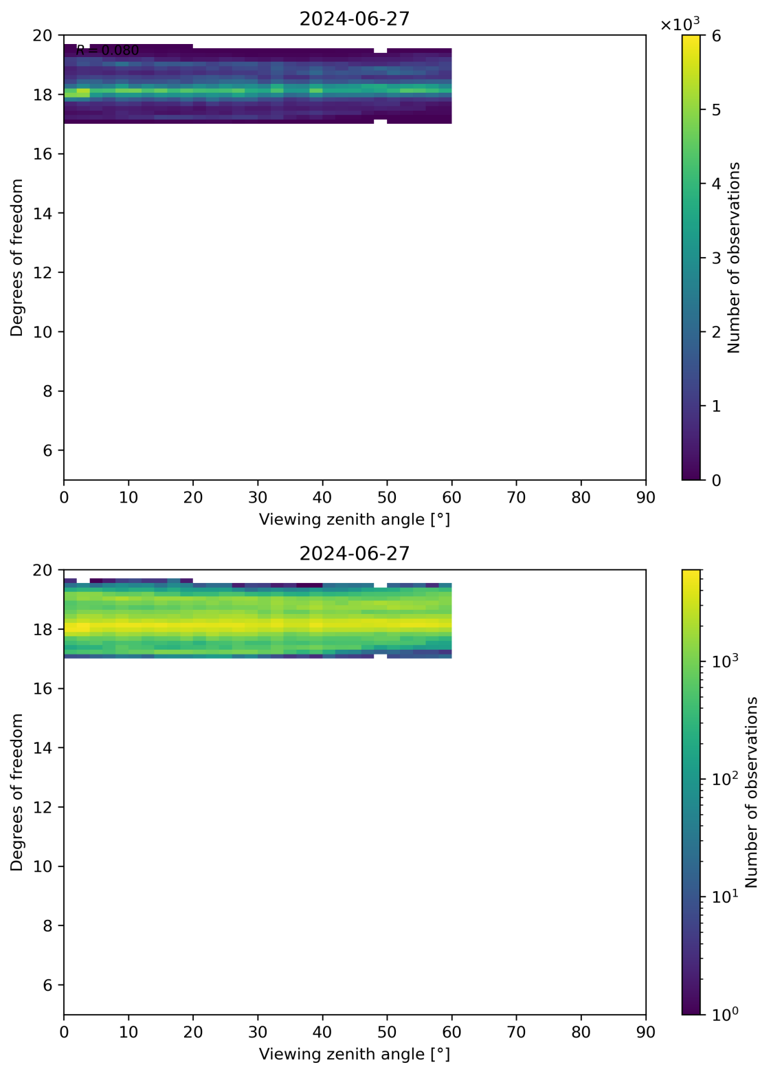
Figure 107: Scatter density plot of “Viewing zenith angle” against “Degrees of freedom” for 2024-06-26 to 2024-06-28.
