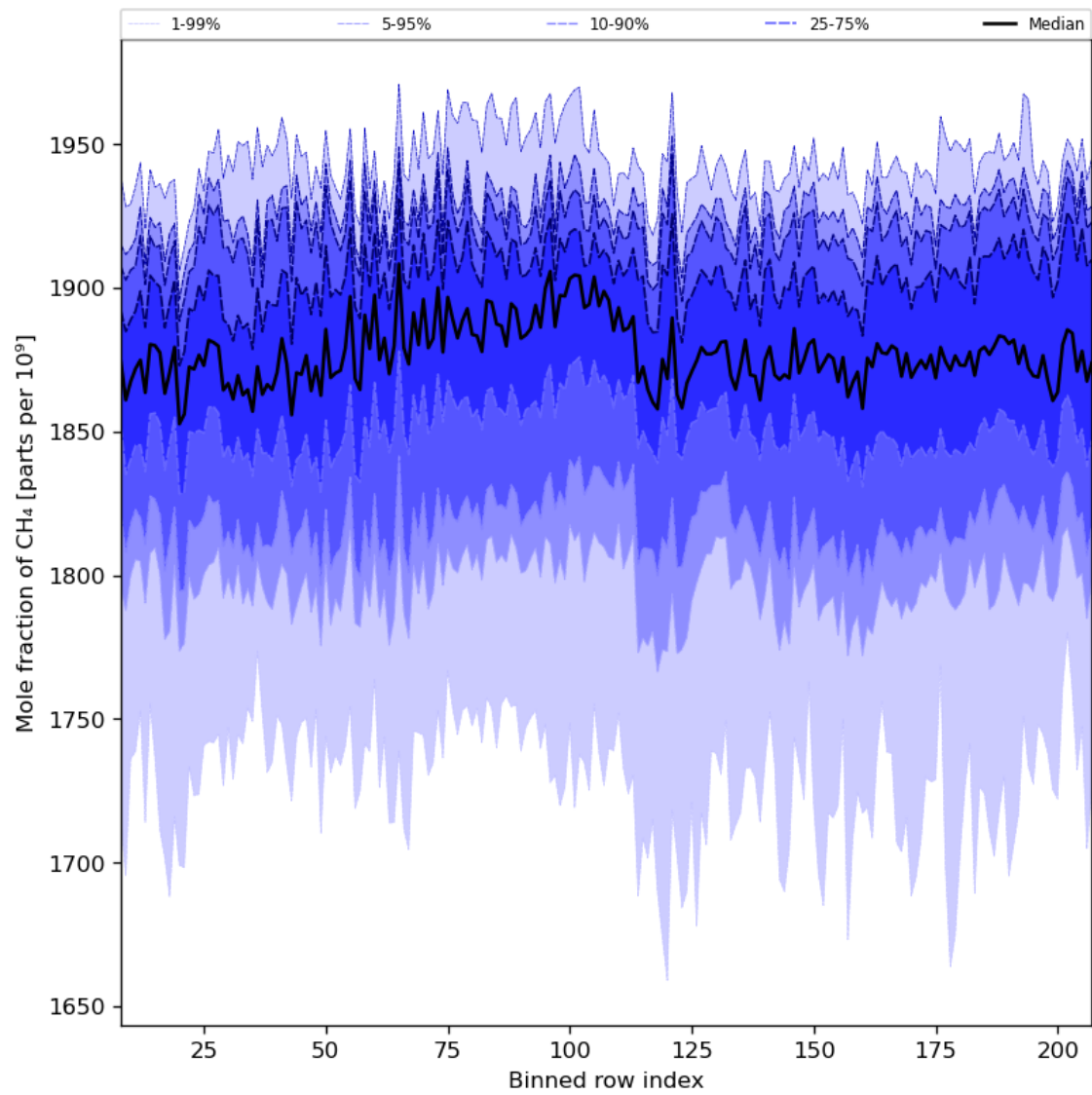
Figure 34: Along track statistics of “Mole fraction of CH 4 ” for 2024-06-26 to 2024-06-28
