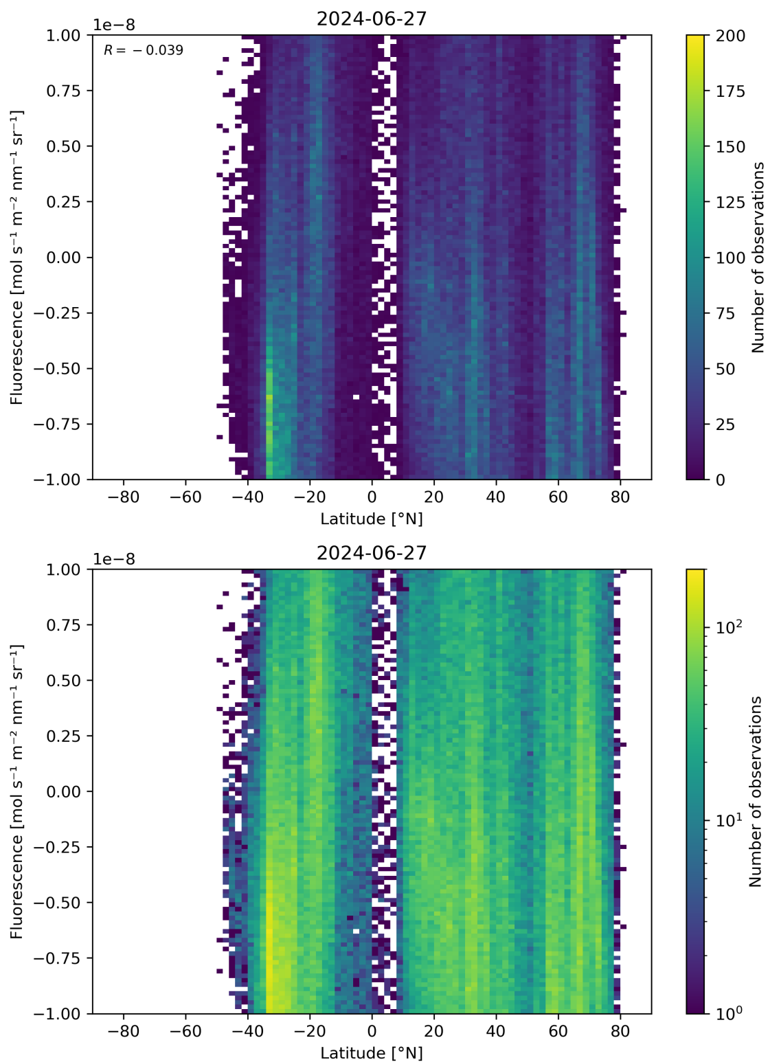
Figure 56: Scatter density plot of “Latitude” against “Fluorescence” for 2024-06-26 to 2024-06-28.
