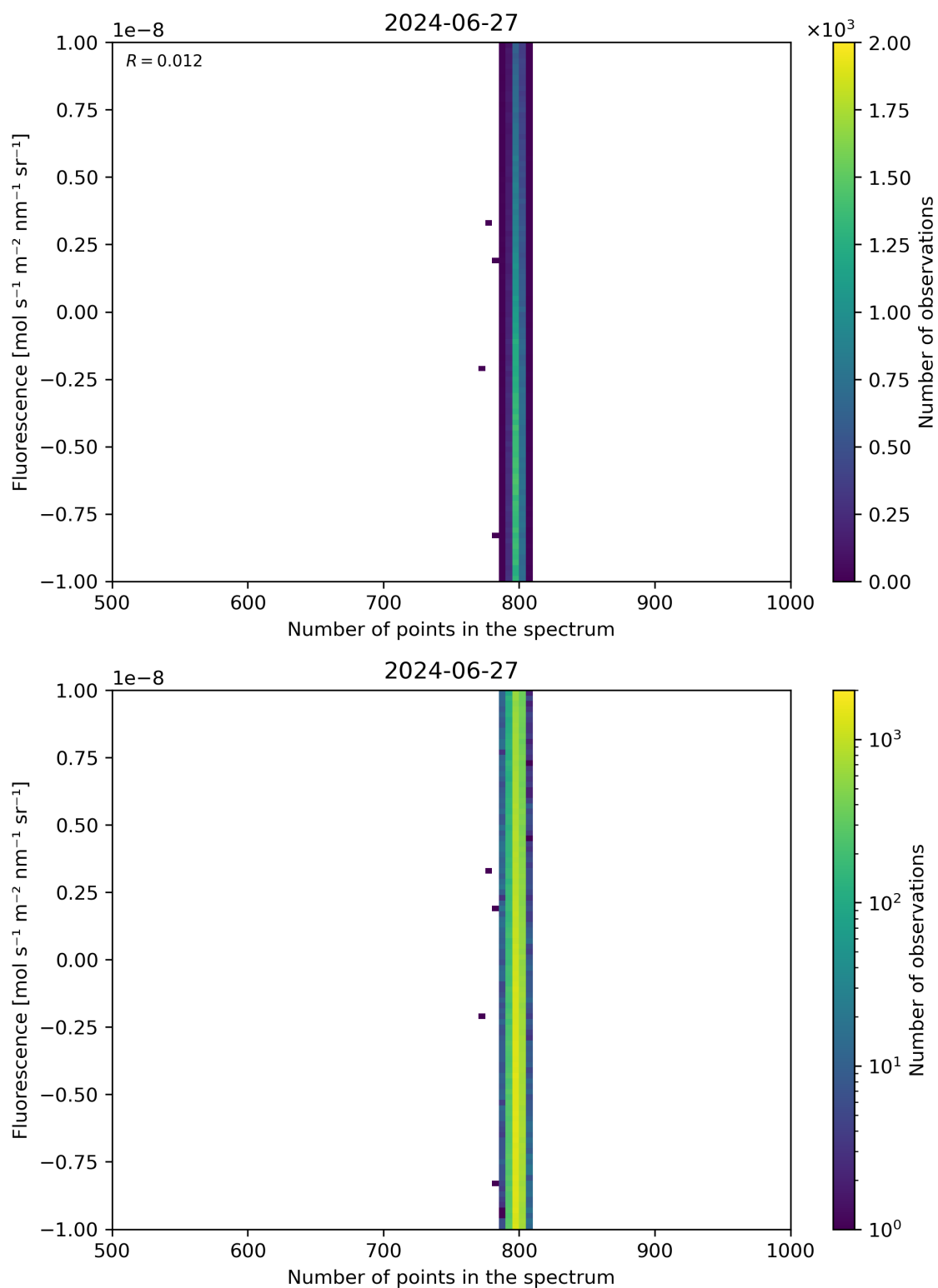
Figure 91: Scatter density plot of “Number of points in the spectrum” against “Fluorescence” for 2024-06-26 to 2024-06-28.
