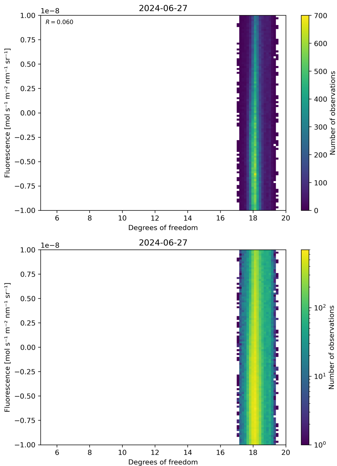
Figure 51: Scatter density plot of “Degrees of freedom” against “Fluorescence” for 2024-06-26 to 2024-06-28.
