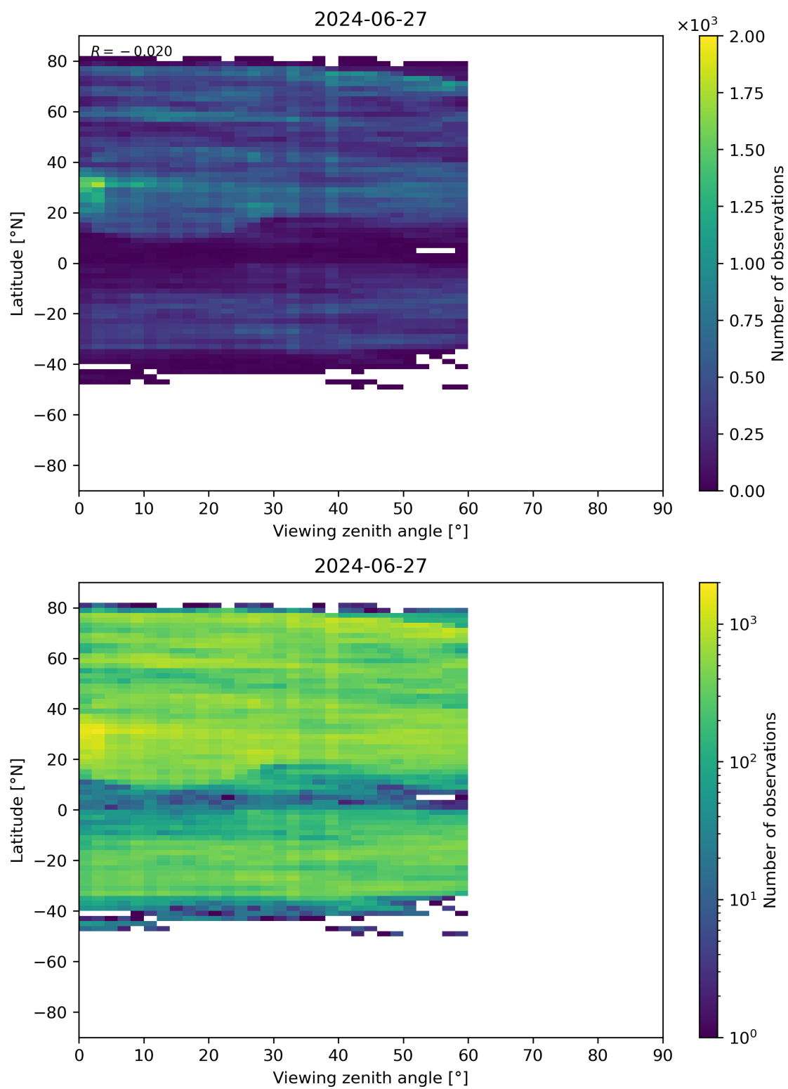
Figure 109: Scatter density plot of “Viewing zenith angle” against “Latitude” for 2024-06-26 to 2024-06-28.
