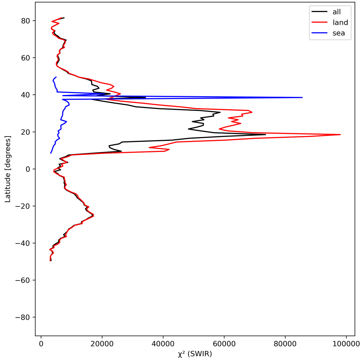
Figure 17: Zonal average of “ \chi^2 (SWIR)” for 2024-06-26 to 2024-06-28.
