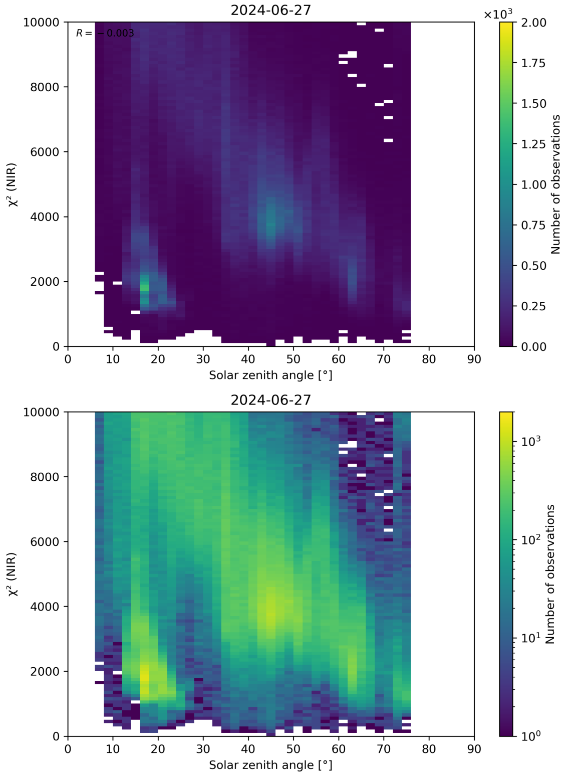
Figure 94: Scatter density plot of “Solar zenith angle” against “ \chi^2 (NIR)” for 2024-06-26 to 2024-06-28.
