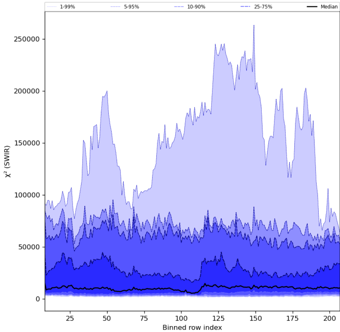
Figure 39: Along track statistics of " \chi^2 (SWIR)" for 2024-06-26 to 2024-06-28
