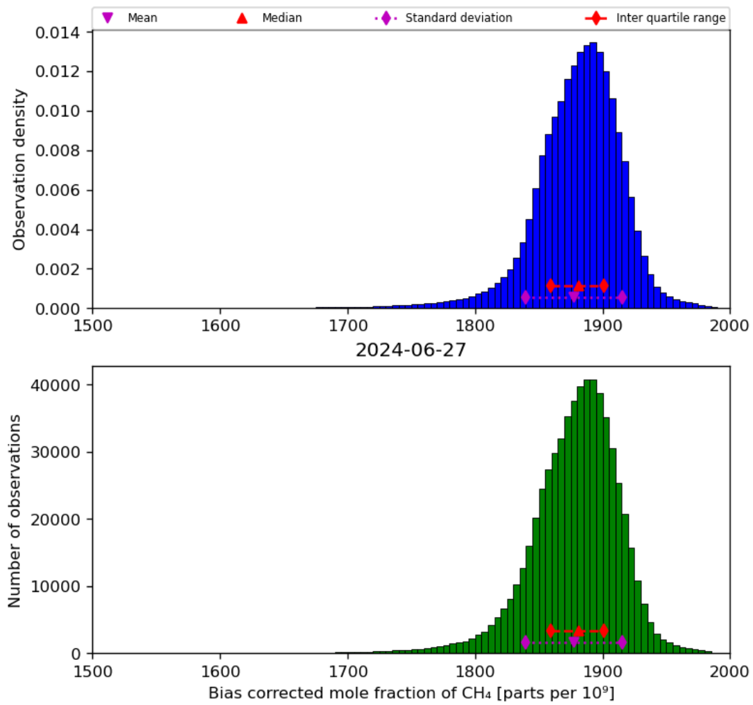
Figure 25: Histogram of “Bias corrected mole fraction of CH 4 ” for 2024-06-26 to 2024-06-28
