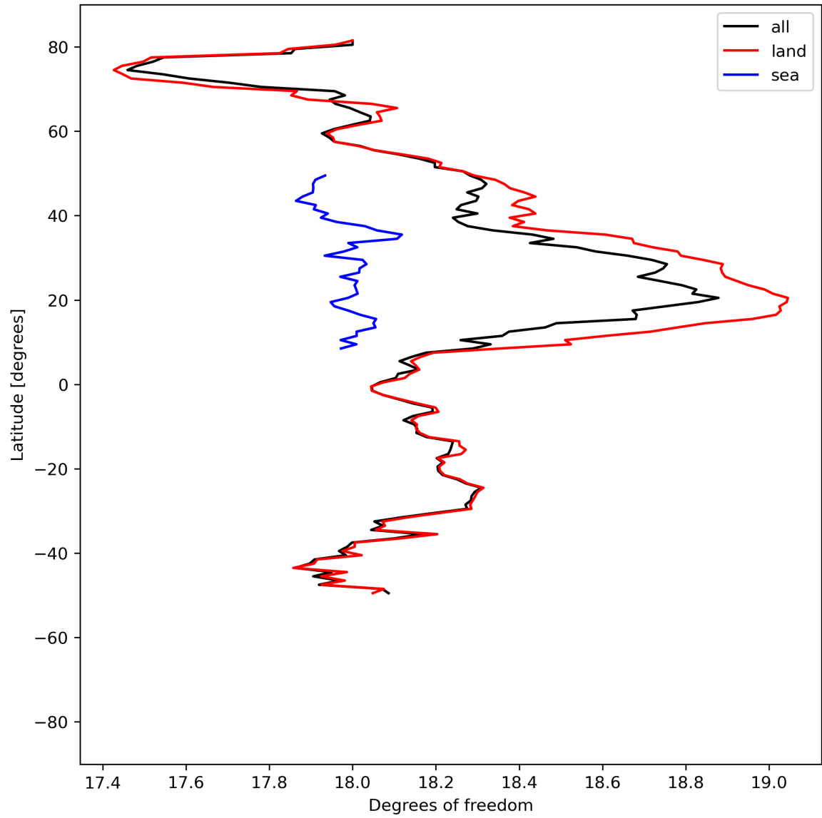
Figure 19: Zonal average of “Degrees of freedom” for 2024-06-26 to 2024-06-28.
