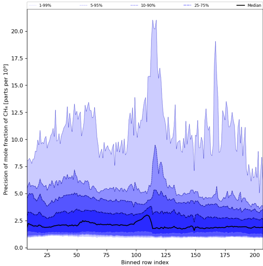
Figure 35: Along track statistics of “Precision of mole fraction of CH 4 ” for 2024-06-26 to 2024-06-28
