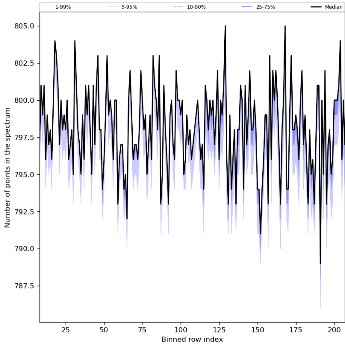
Figure 37: Along track statistics of “Number of points in the spectrum” for 2024-06-26 to 2024-06-28
