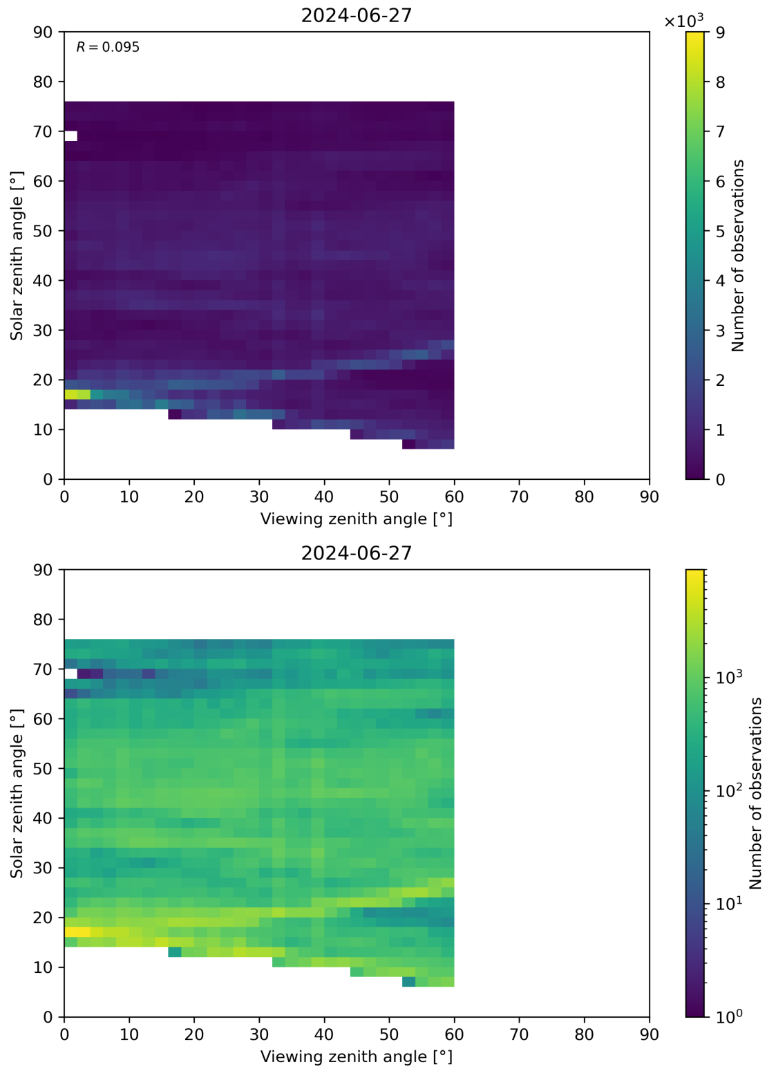
Figure 115: Scatter density plot of “Viewing zenith angle” against “Solar zenith angle” for 2024-06-26 to 2024-06-28.
