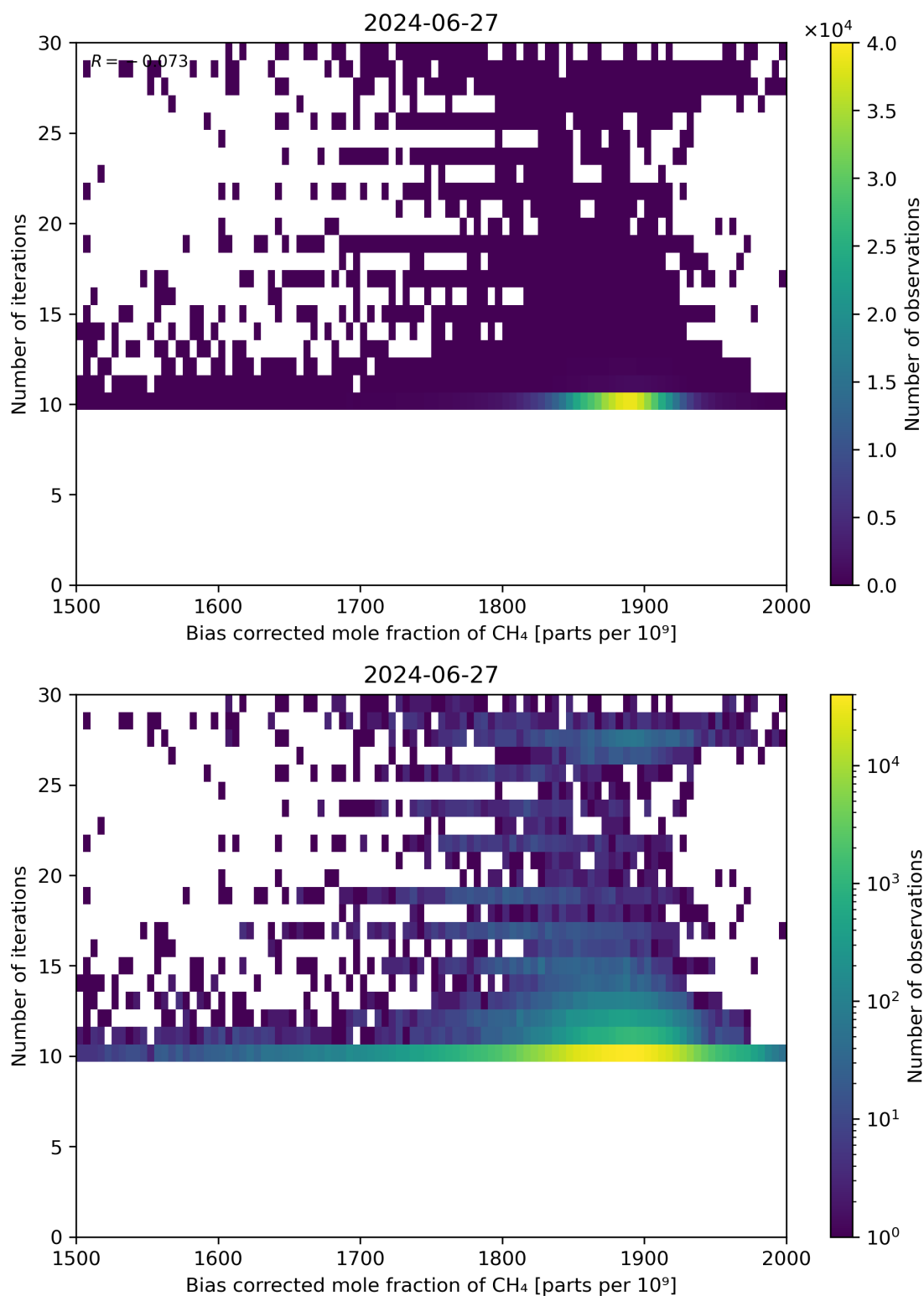
Figure 67: Scatter density plot of “Bias corrected mole fraction of CH 4 ” against “Number of iterations” for 2024-06-26 to 2024-06-28.
