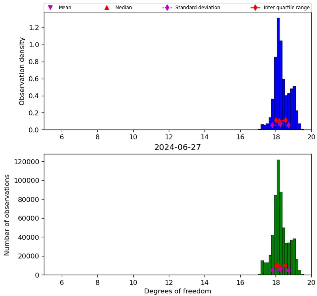
Figure 30: Histogram of “Degrees of freedom” for 2024-06-26 to 2024-06-28
