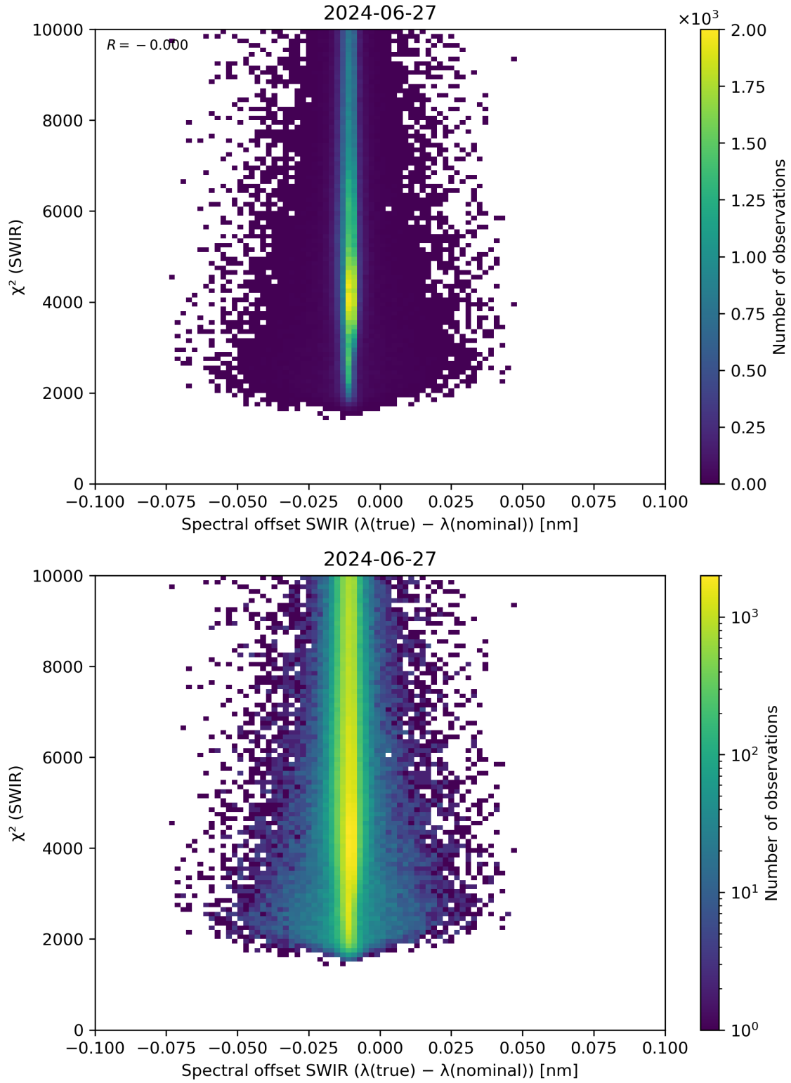
Figure 118: Scatter density plot of “Spectral offset SWIR ( \lambda(\text{true}) - \lambda(\text{nominal}) )” against “ \chi^2 (SWIR)” for 2024-06-26 to 2024-06-28.
