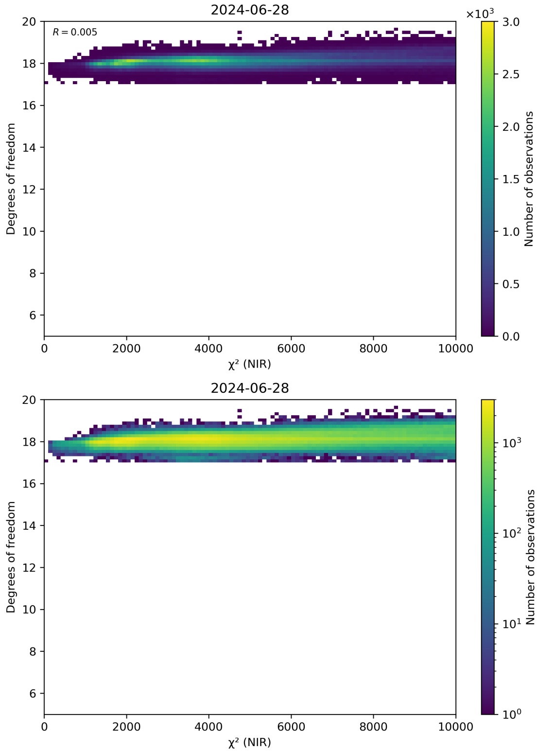
Figure 44: Scatter density plot of “ \chi^2 (NIR)” against “Degrees of freedom” for 2024-06-27 to 2024-06-29.
