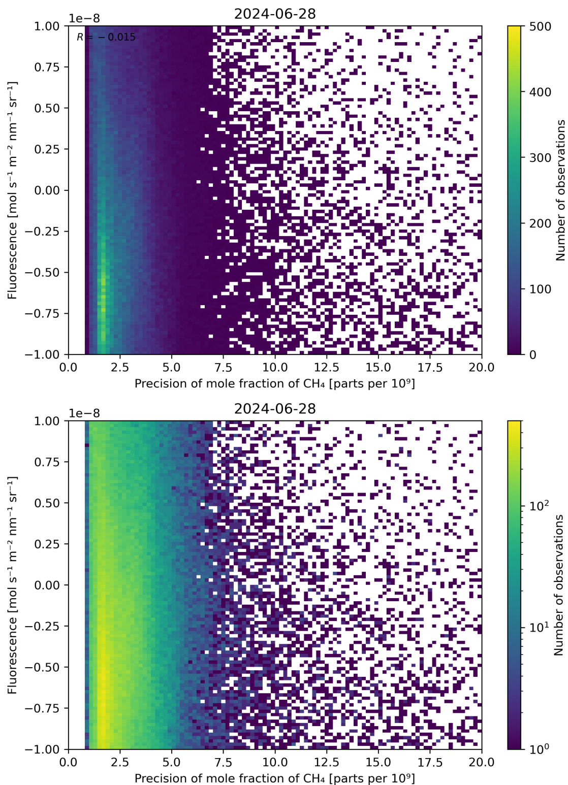
Figure 81: Scatter density plot of “Precision of mole fraction of \text{CH}_4 ” against “Fluorescence” for 2024-06-27 to 2024-06-29.
