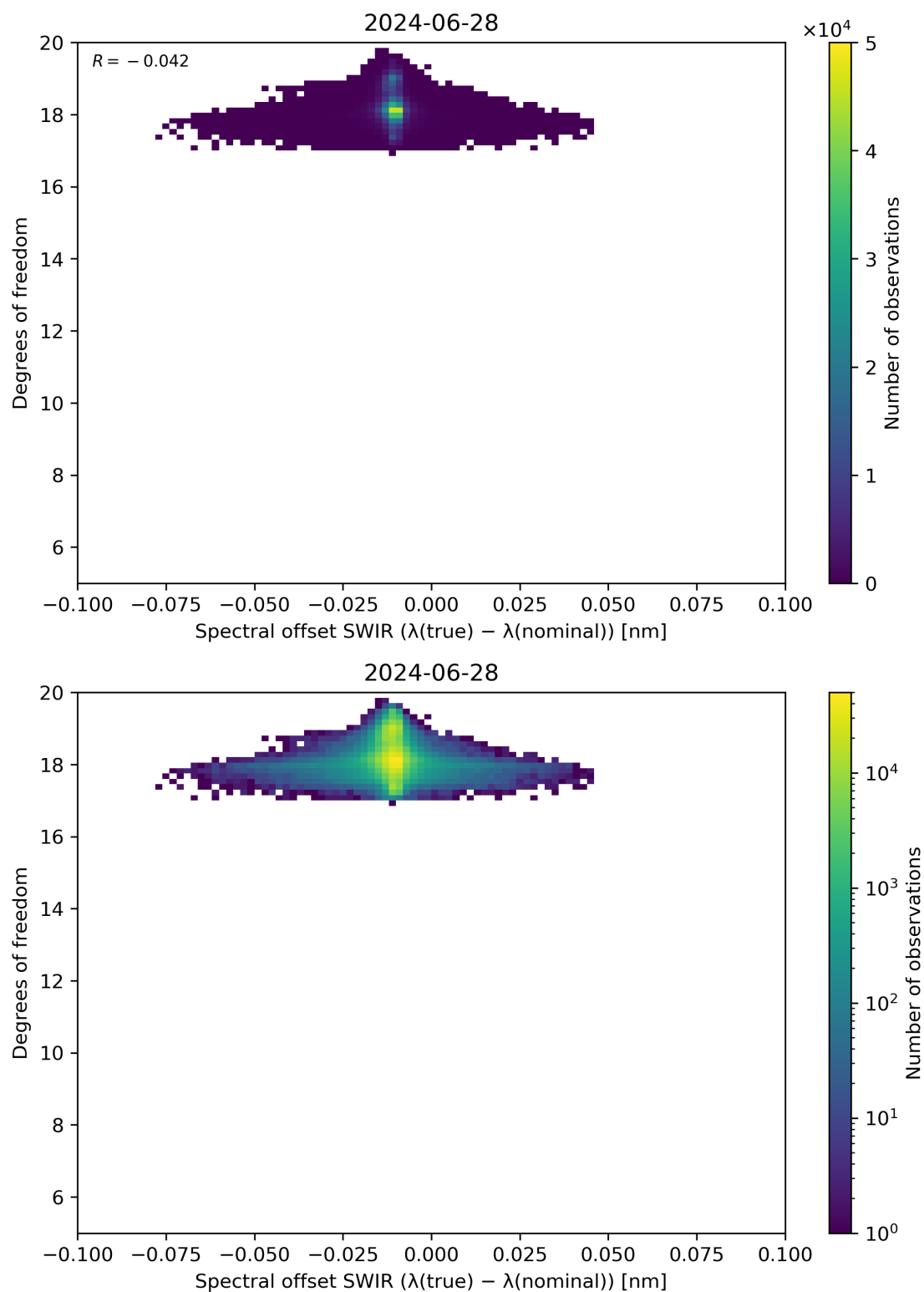
Figure 119: Scatter density plot of “Spectral offset SWIR ( \lambda(\text{true}) - \lambda(\text{nominal}) )” against “Degrees of freedom” for 2024-06-27 to 2024-06-29.
