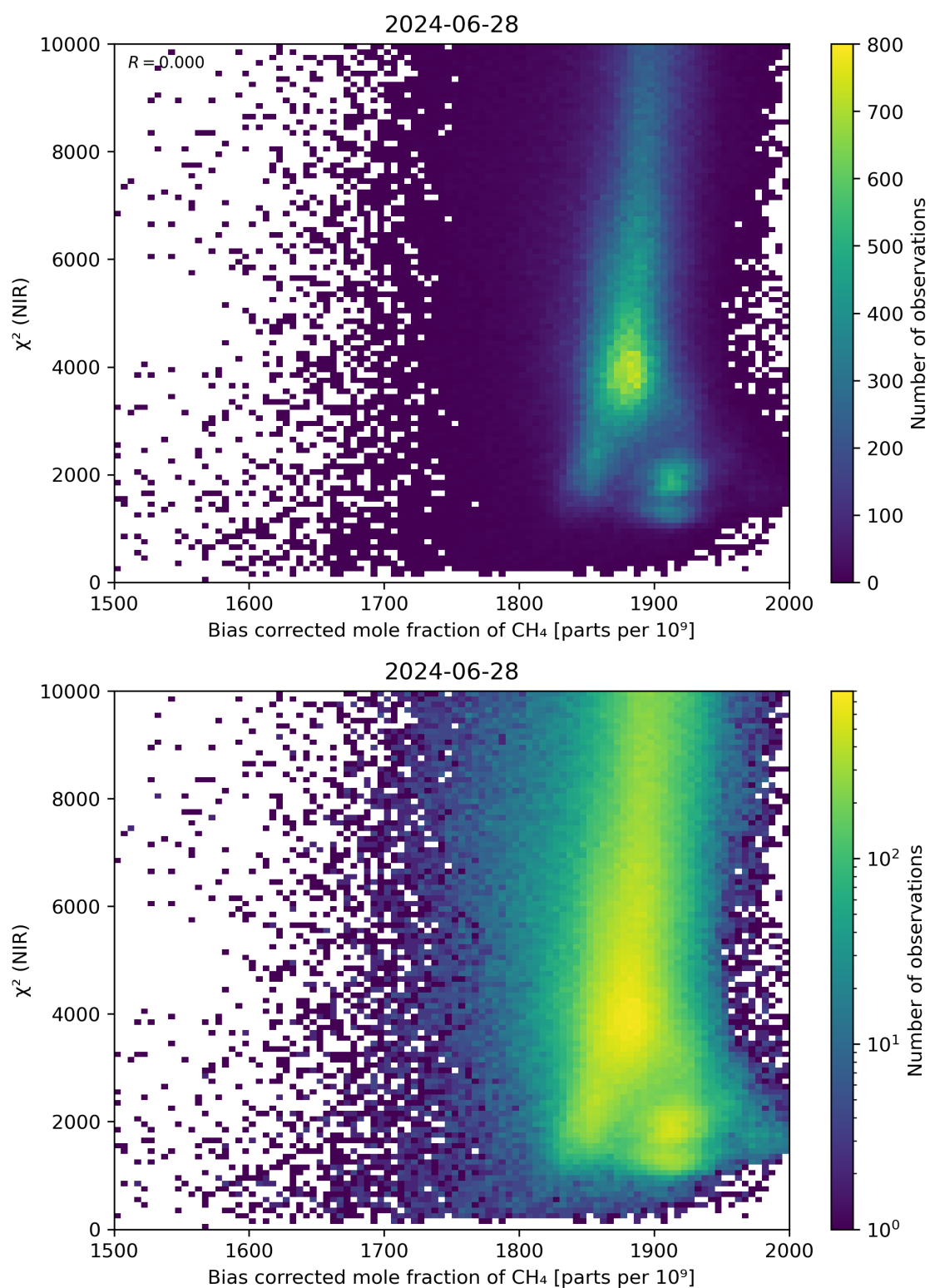
Figure 63: Scatter density plot of “Bias corrected mole fraction of CH 4 ” against “ \chi^2 (NIR)” for 2024-06-27 to 2024-06-29.
