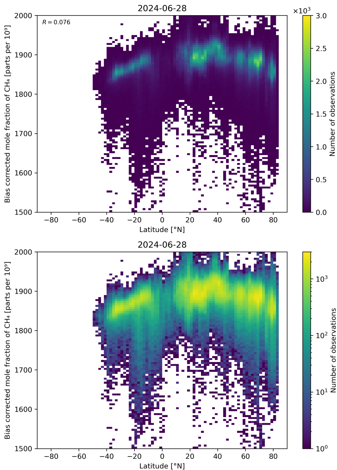
Figure 58: Scatter density plot of “Latitude” against “Bias corrected mole fraction of \text{CH}_4 ” for 2024-06-27 to 2024-06-29.
