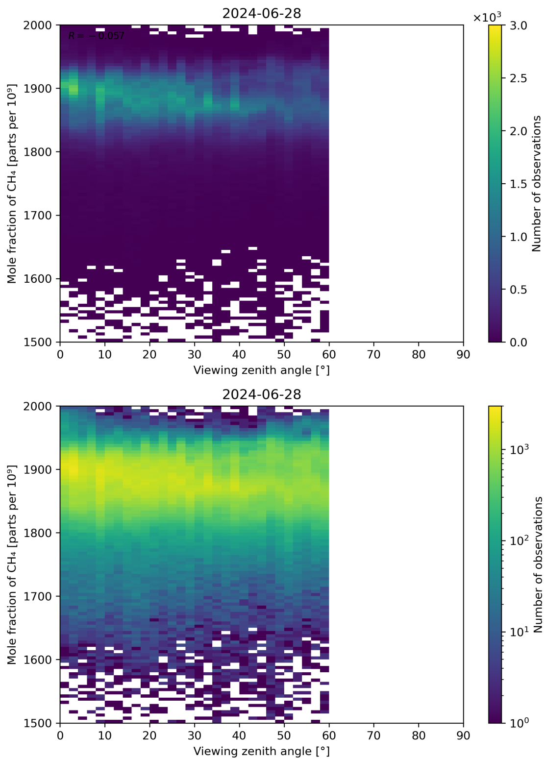
Figure 110: Scatter density plot of “Viewing zenith angle” against “Mole fraction of CH 4 ” for 2024-06-27 to 2024-06-29.
