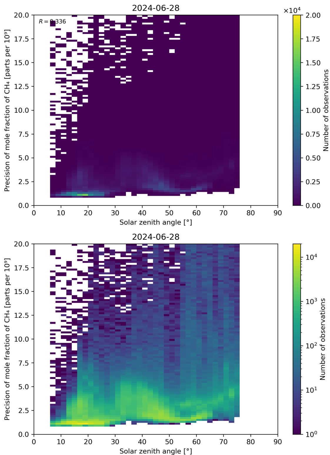
Figure 101: Scatter density plot of “Solar zenith angle” against “Precision of mole fraction of CH 4 ” for 2024-06-27 to 2024-06-29.
