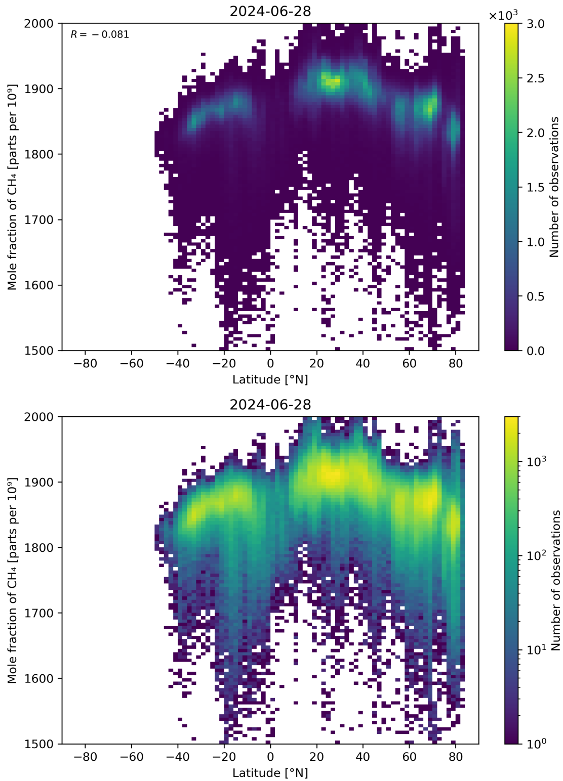
Figure 57: Scatter density plot of “Latitude” against “Mole fraction of \text{CH}_4 ” for 2024-06-27 to 2024-06-29.
