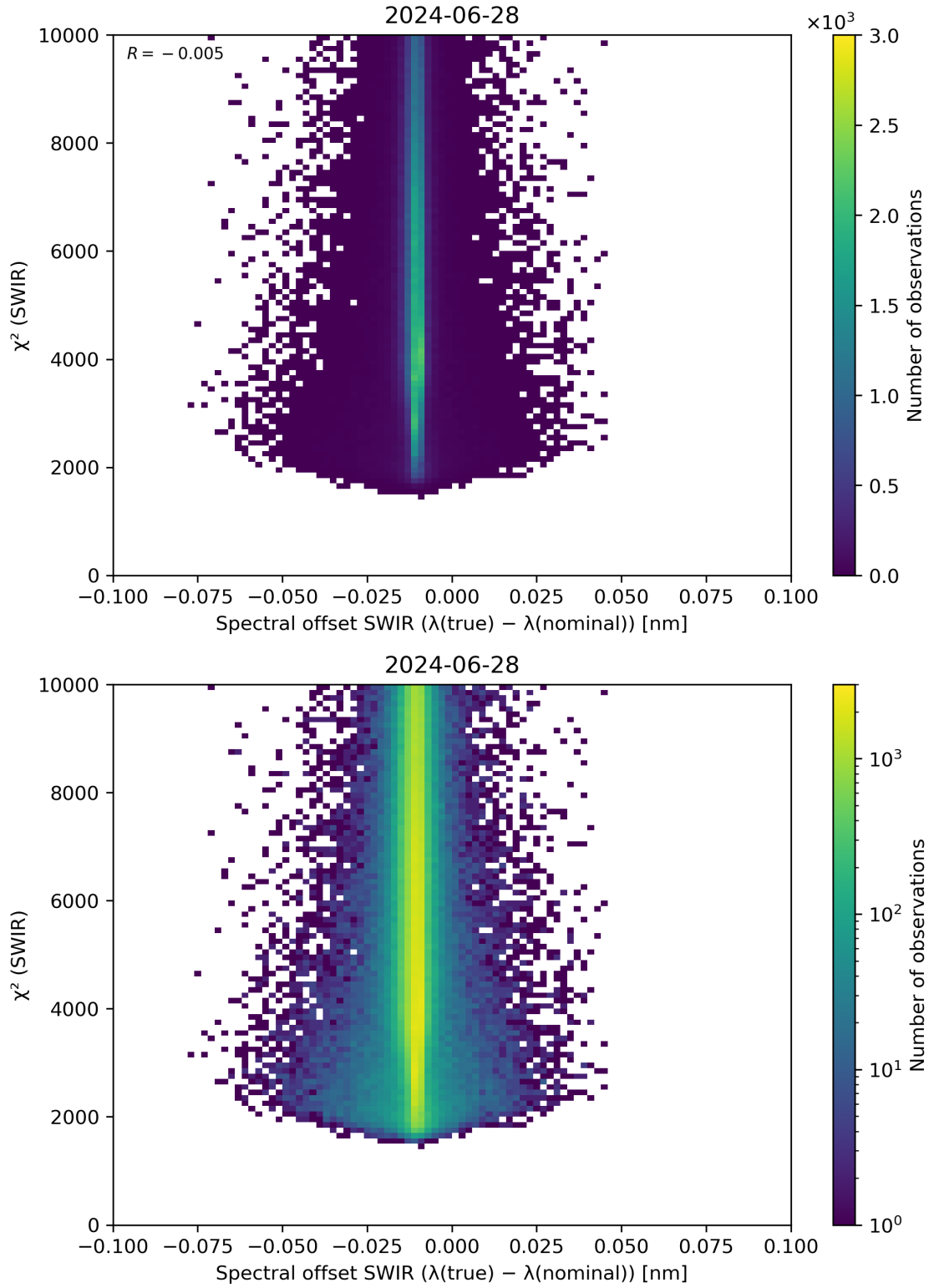
Figure 118: Scatter density plot of “Spectral offset SWIR ( \lambda(\text{true}) - \lambda(\text{nominal}) )” against “ \chi^2 (SWIR)” for 2024-06-27 to 2024-06-29.
