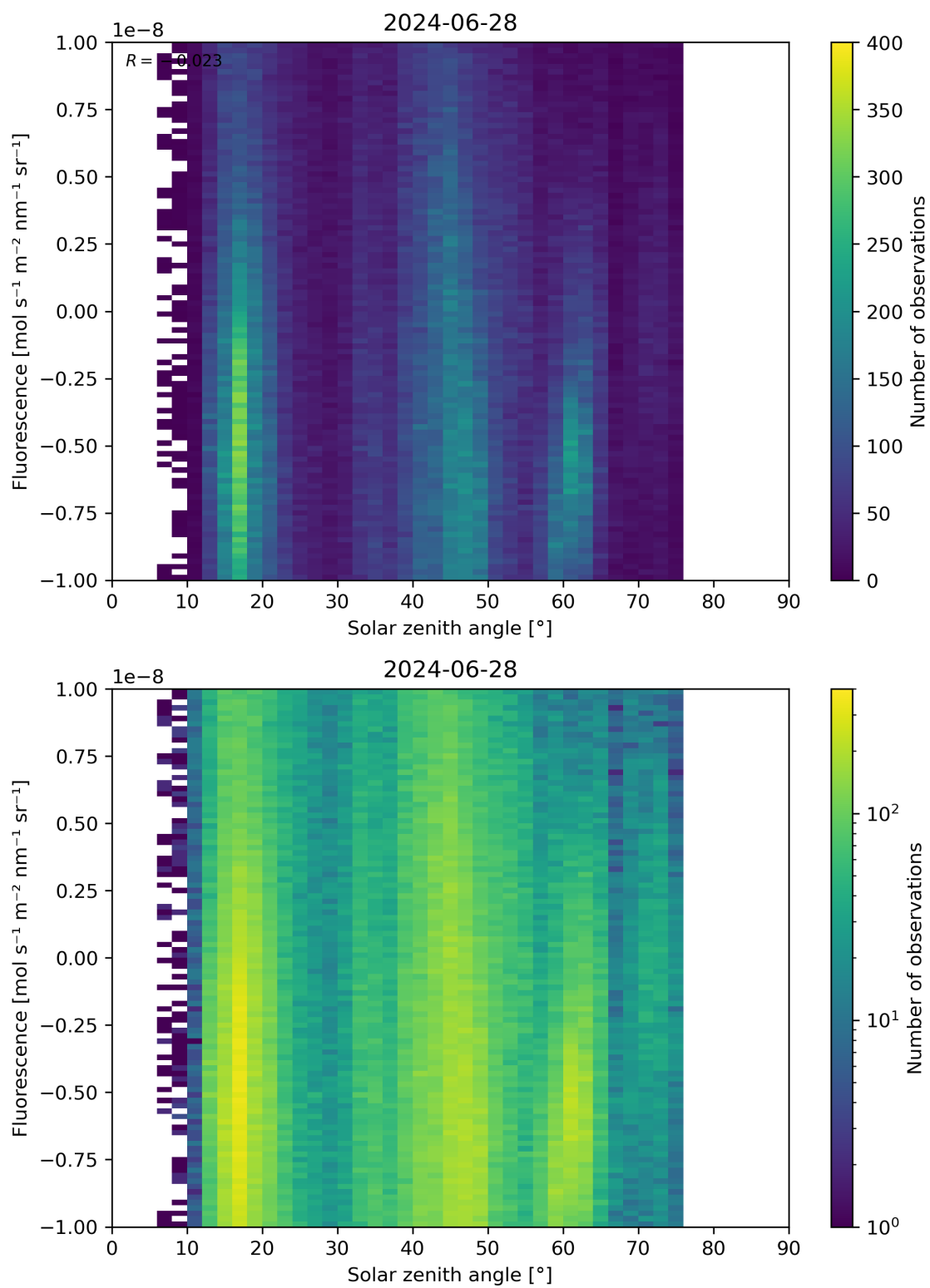
Figure 97: Scatter density plot of “Solar zenith angle” against “Fluorescence” for 2024-06-27 to 2024-06-29.
