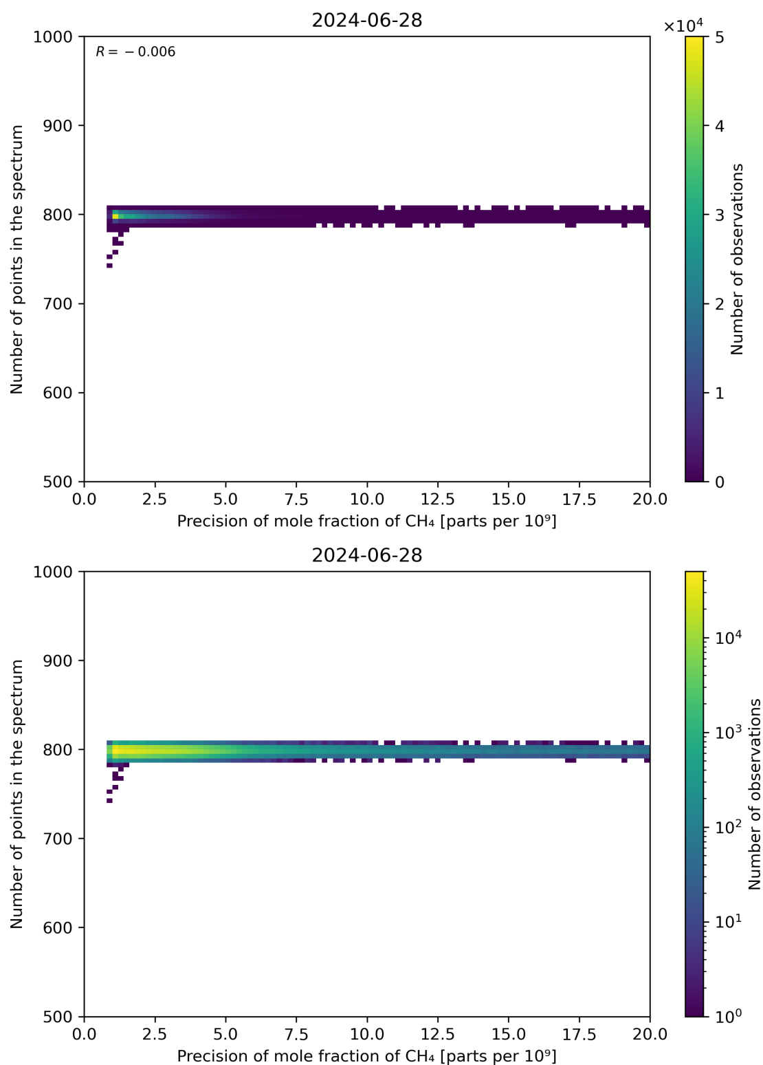
Figure 84: Scatter density plot of “Precision of mole fraction of CH 4 ” against “Number of points in the spectrum” for 2024-06-27 to 2024-06-29.
