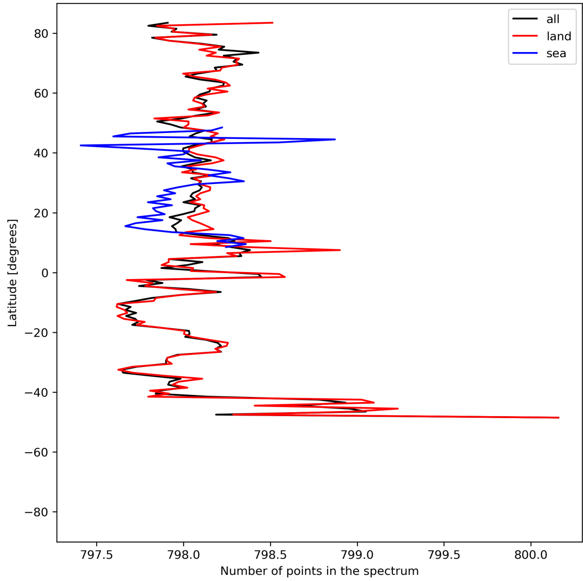
Figure 15: Zonal average of “Number of points in the spectrum” for 2024-06-27 to 2024-06-29.
