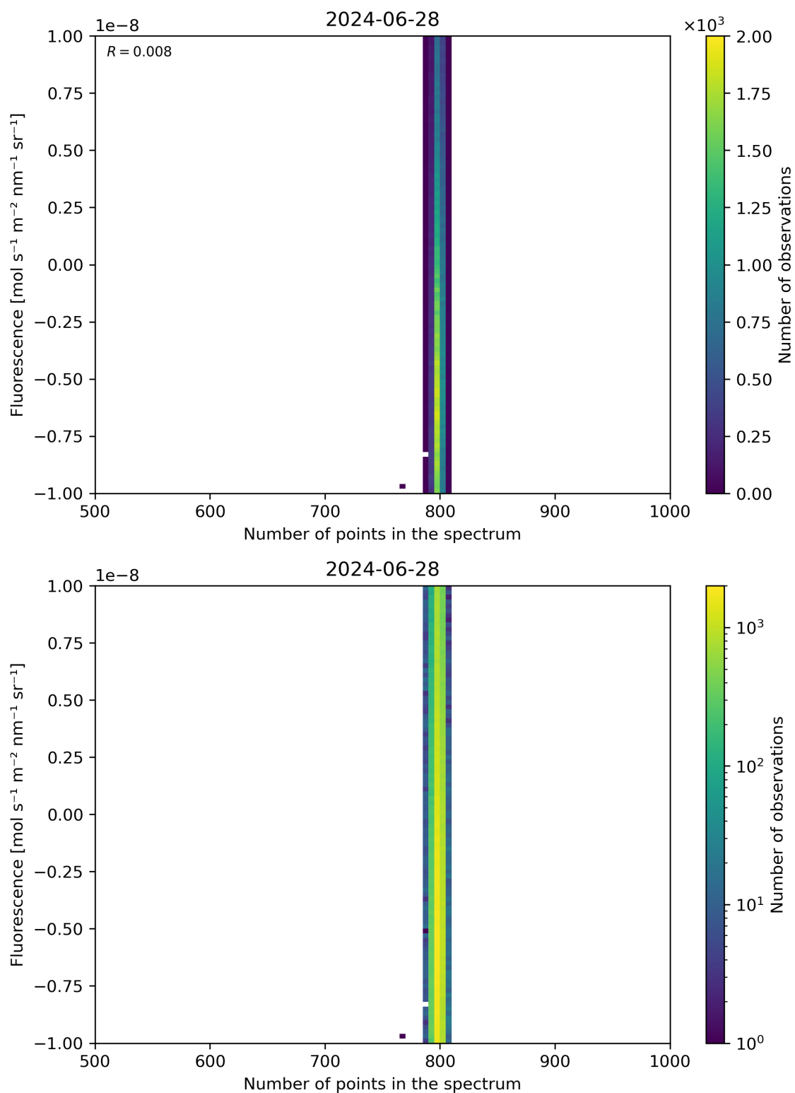
Figure 91: Scatter density plot of “Number of points in the spectrum” against “Fluorescence” for 2024-06-27 to 2024-06-29.
