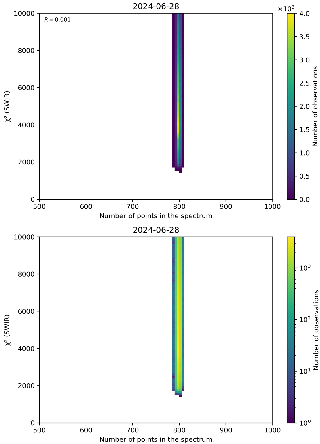
Figure 89: Scatter density plot of “Number of points in the spectrum” against “ \chi^2 (SWIR)” for 2024-06-27 to 2024-06-29.
