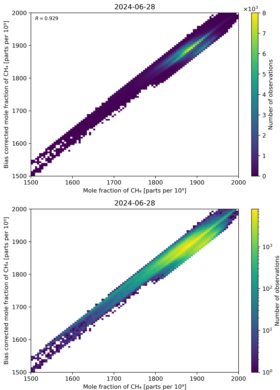
Figure 74: Scatter density plot of “Mole fraction of CH 4 ” against “Bias corrected mole fraction of CH 4 ” for 2024-06-27 to 2024-06-29.
