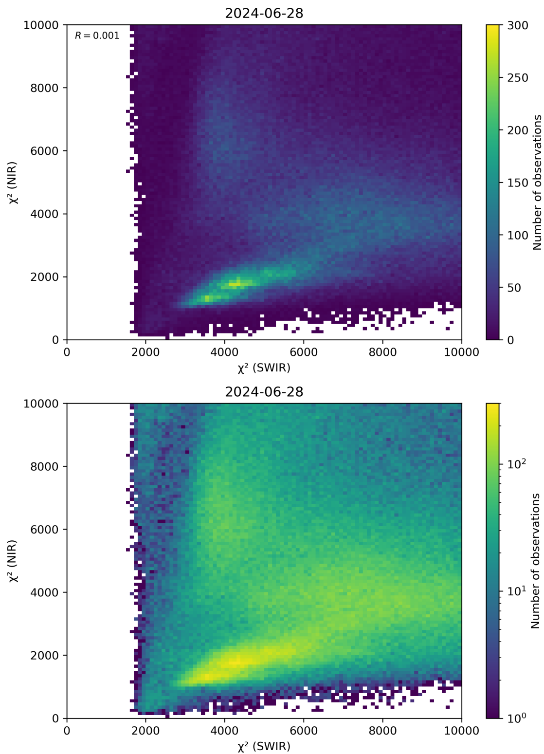
Figure 47: Scatter density plot of “ \chi^2 (SWIR)” against “ \chi^2 (NIR)” for 2024-06-27 to 2024-06-29.
