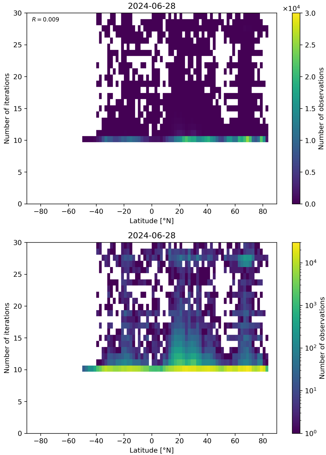
Figure 60: Scatter density plot of “Latitude” against “Number of iterations” for 2024-06-27 to 2024-06-29.
