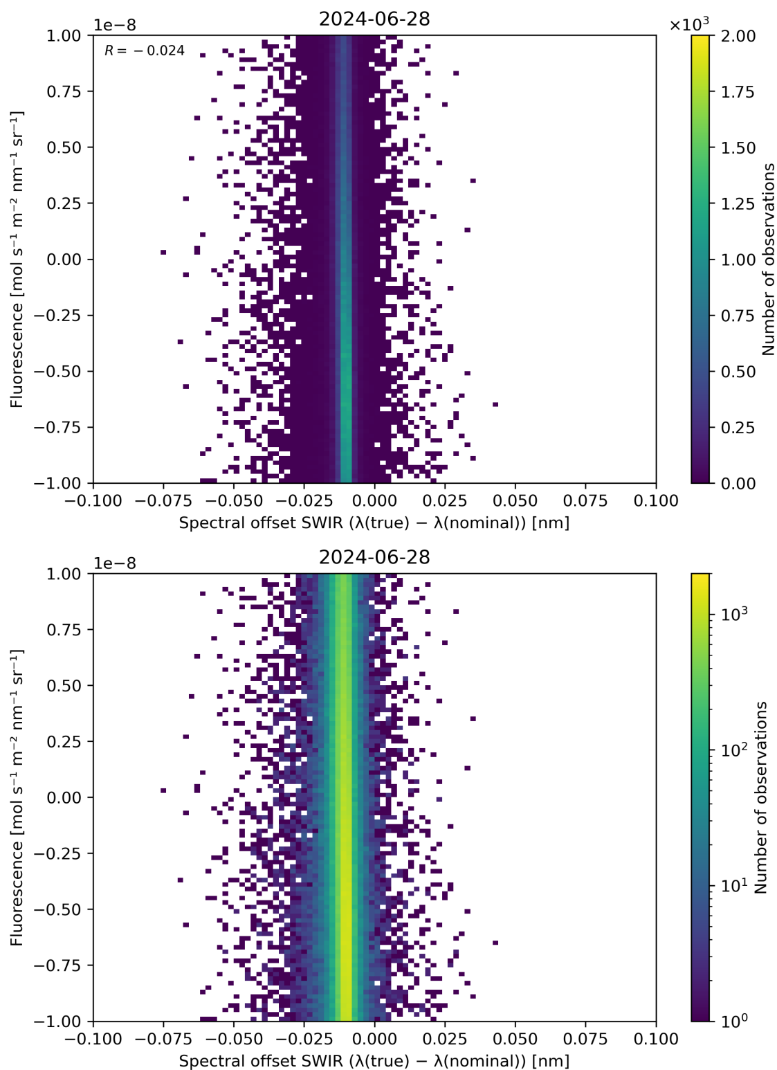
Figure 120: Scatter density plot of “Spectral offset SWIR ( \lambda(\text{true}) - \lambda(\text{nominal}) )” against “Fluorescence” for 2024-06-27 to 2024-06-29.
