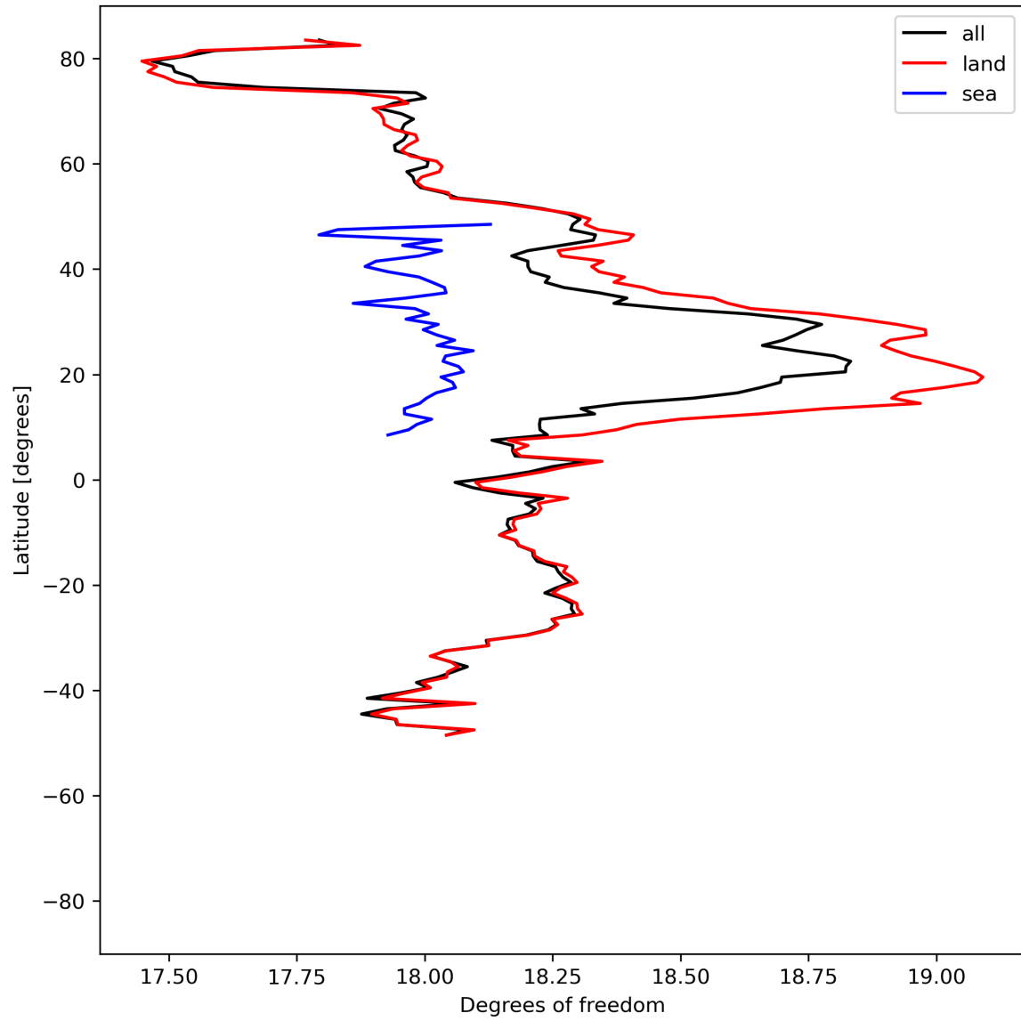
Figure 19: Zonal average of “Degrees of freedom” for 2024-06-27 to 2024-06-29.
