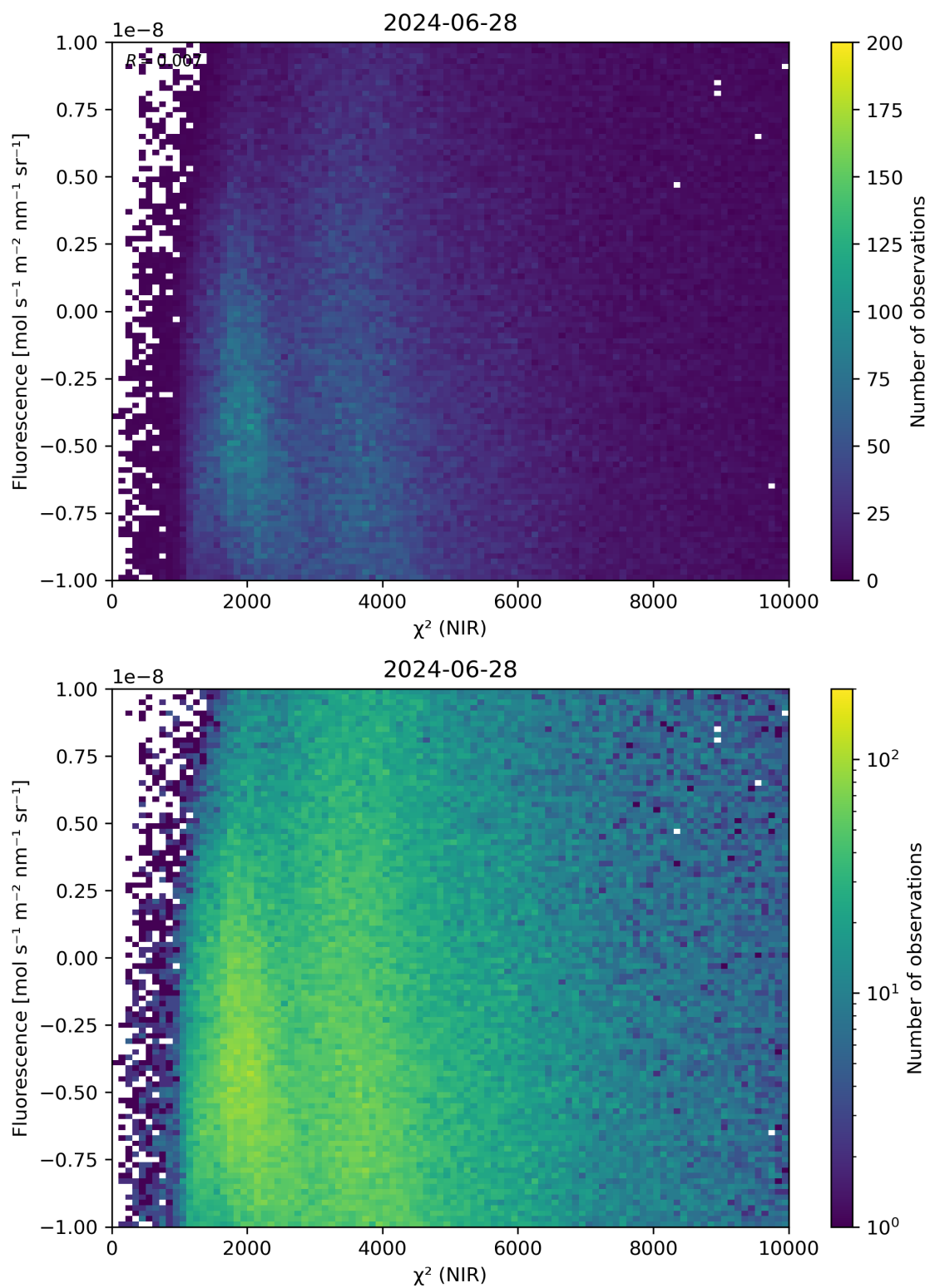
Figure 45: Scatter density plot of “ \chi^2 (NIR)” against “Fluorescence” for 2024-06-27 to 2024-06-29.
