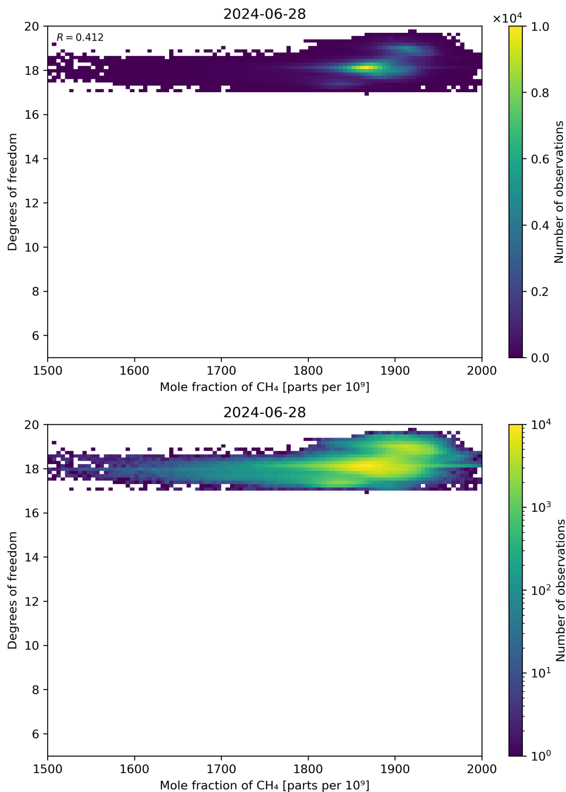
Figure 72: Scatter density plot of “Mole fraction of CH 4 ” against “Degrees of freedom” for 2024-06-27 to 2024-06-29.
