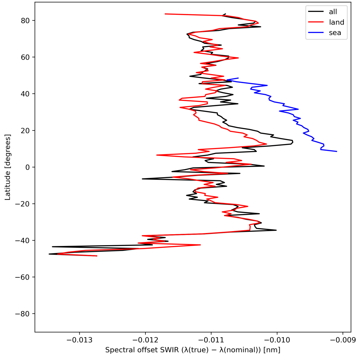
Figure 16: Zonal average of “Spectral offset SWIR ( \lambda(\text{true}) - \lambda(\text{nominal}) )” for 2024-06-27 to 2024-06-29.
