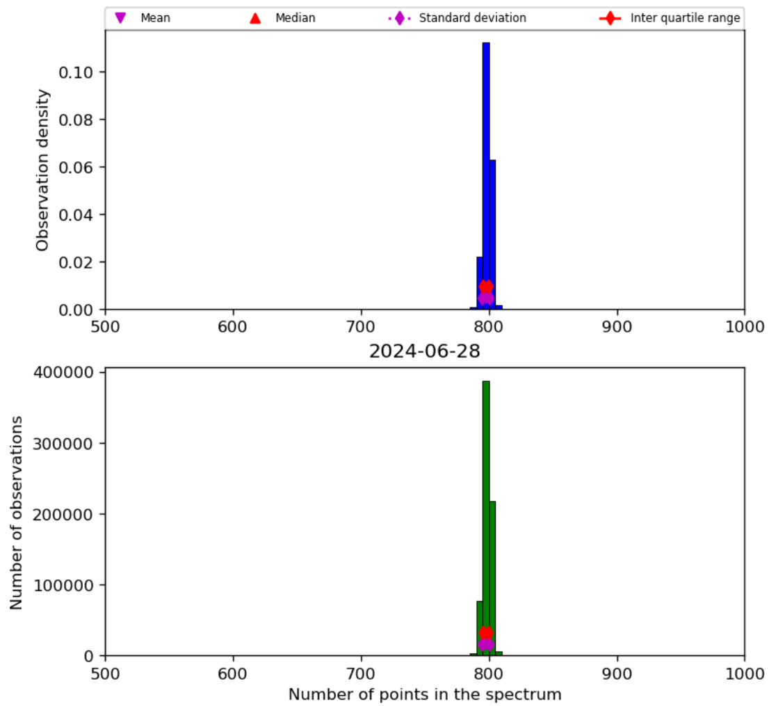
Figure 26: Histogram of “Number of points in the spectrum” for 2024-06-27 to 2024-06-29
