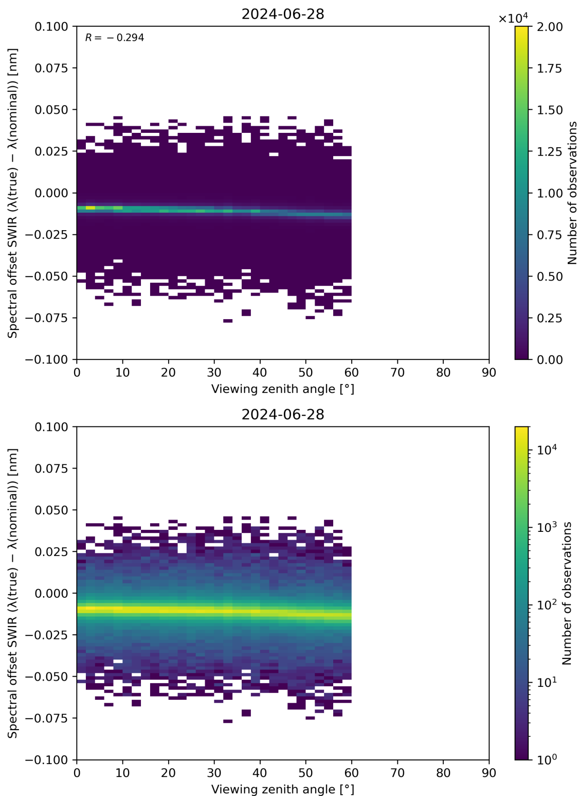
Figure 116: Scatter density plot of “Viewing zenith angle” against “Spectral offset SWIR ( \lambda(\text{true}) - \lambda(\text{nominal}) )” for 2024-06-27 to 2024-06-29.
