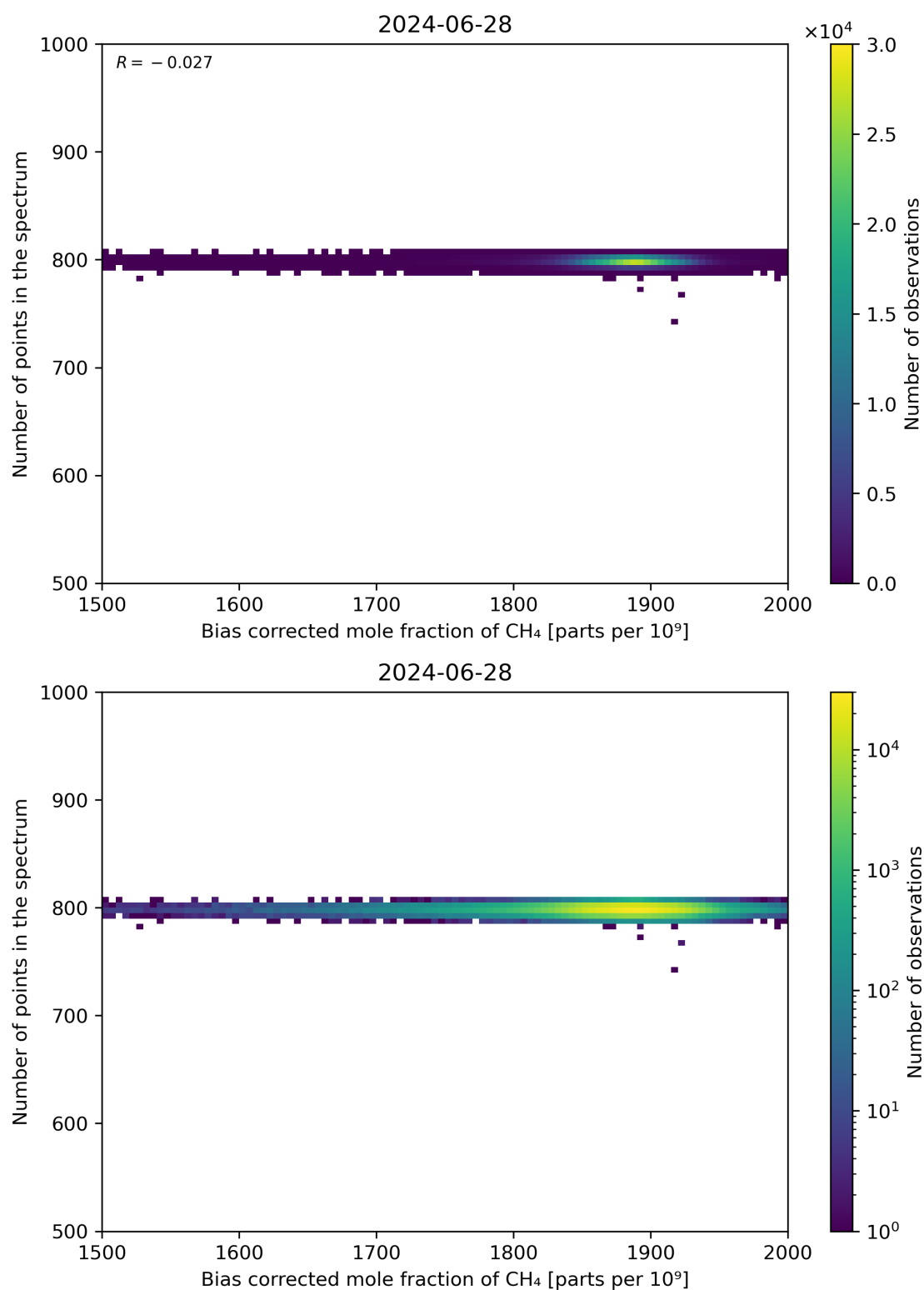
Figure 68: Scatter density plot of “Bias corrected mole fraction of CH 4 ” against “Number of points in the spectrum” for 2024-06-27 to 2024-06-29.
