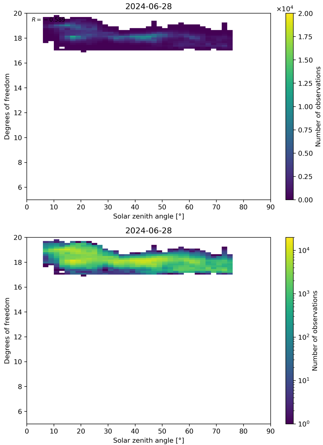
Figure 96: Scatter density plot of “Solar zenith angle” against “Degrees of freedom” for 2024-06-27 to 2024-06-29.
