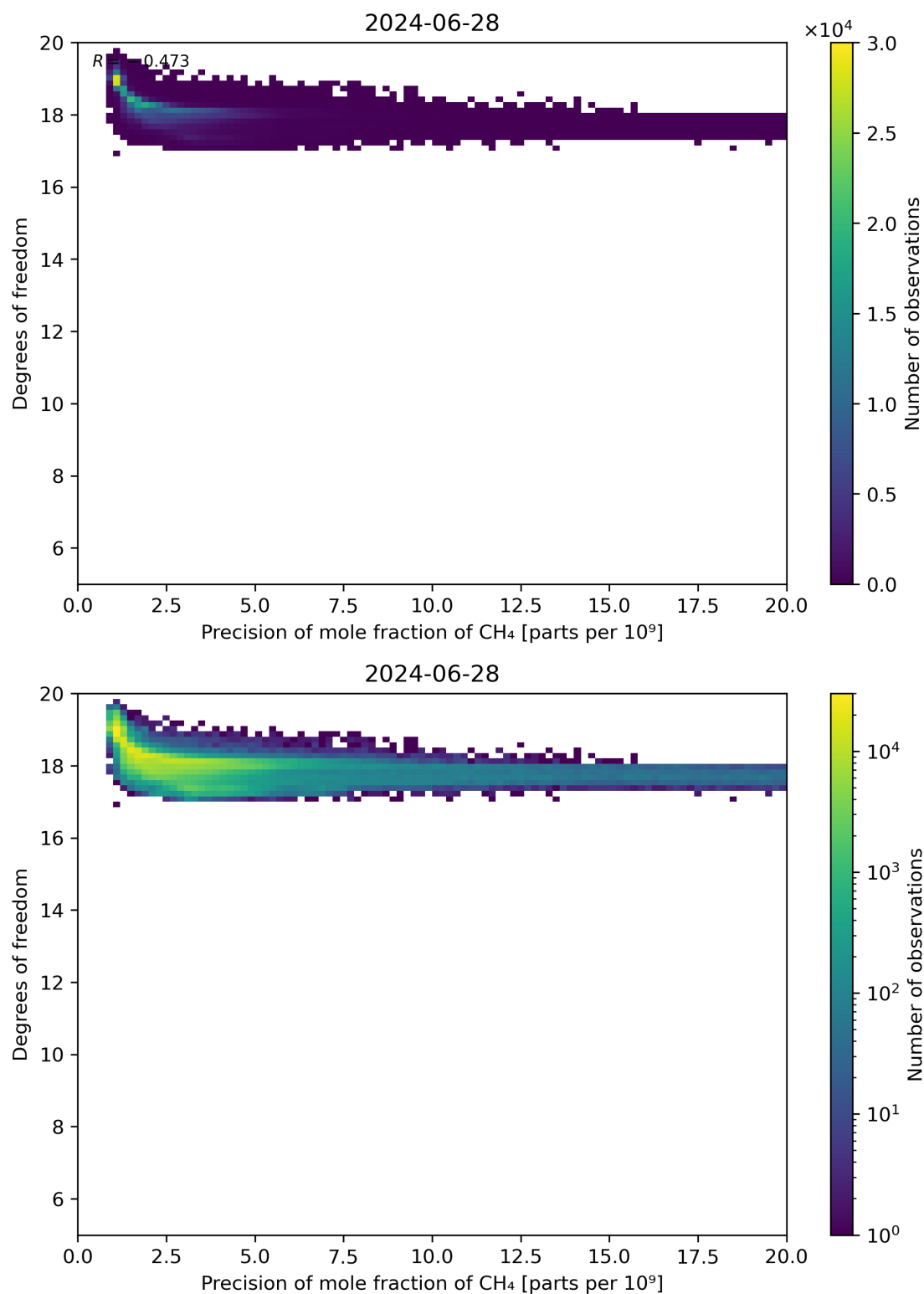
Figure 80: Scatter density plot of “Precision of mole fraction of CH 4 ” against “Degrees of freedom” for 2024-06-27 to 2024-06-29.
