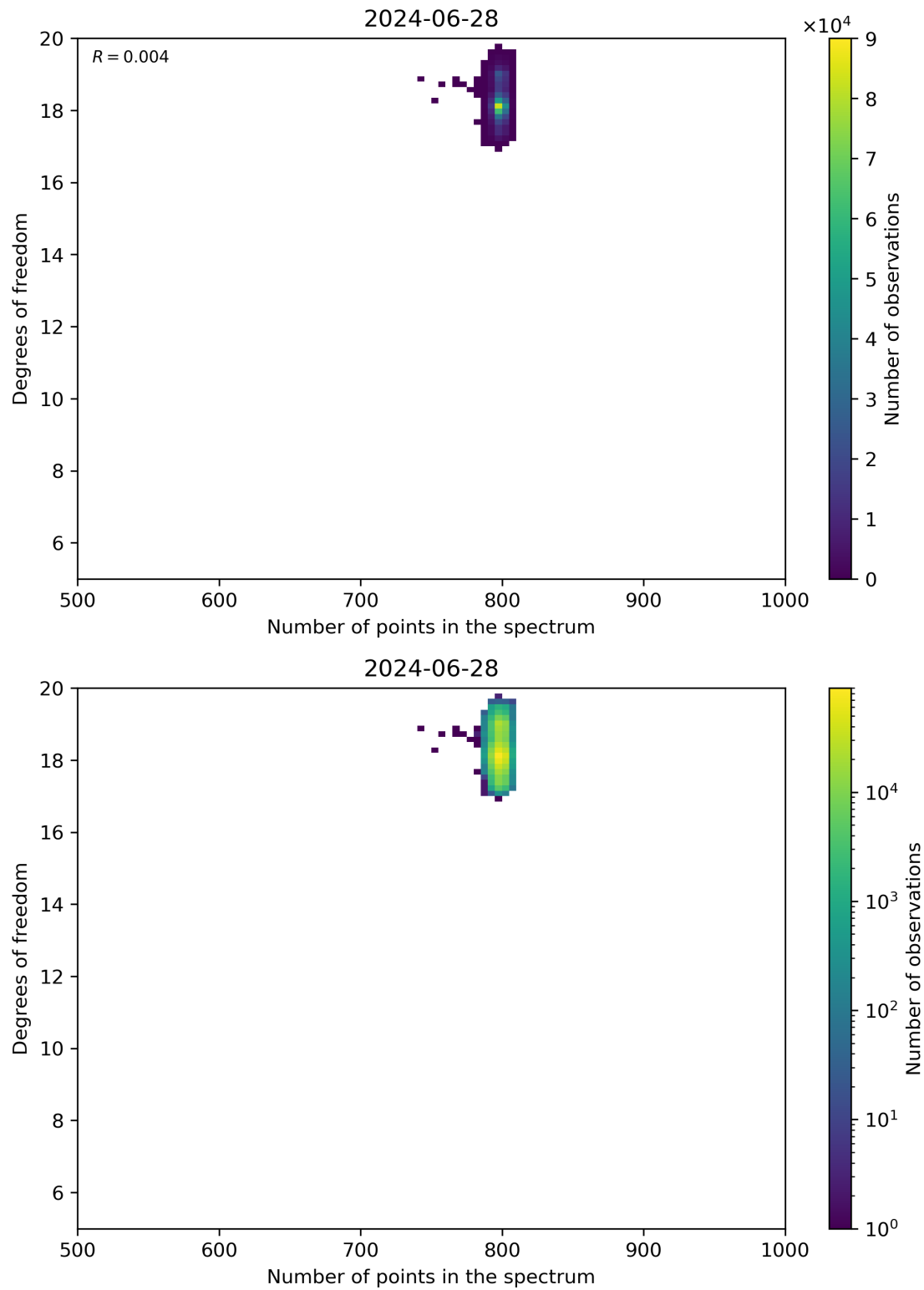
Figure 90: Scatter density plot of “Number of points in the spectrum” against “Degrees of freedom” for 2024-06-27 to 2024-06-29.
