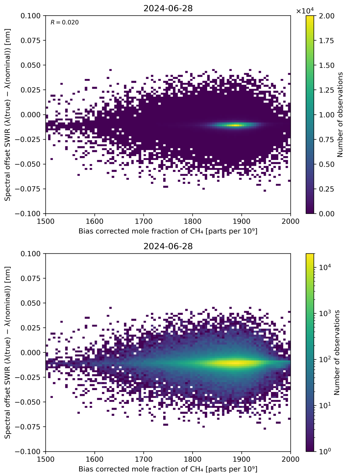
Figure 69: Scatter density plot of “Bias corrected mole fraction of \text{CH}_4 ” against “Spectral offset SWIR ( \lambda(\text{true}) - \lambda(\text{nominal}) )” for 2024-06-27 to 2024-06-29.
