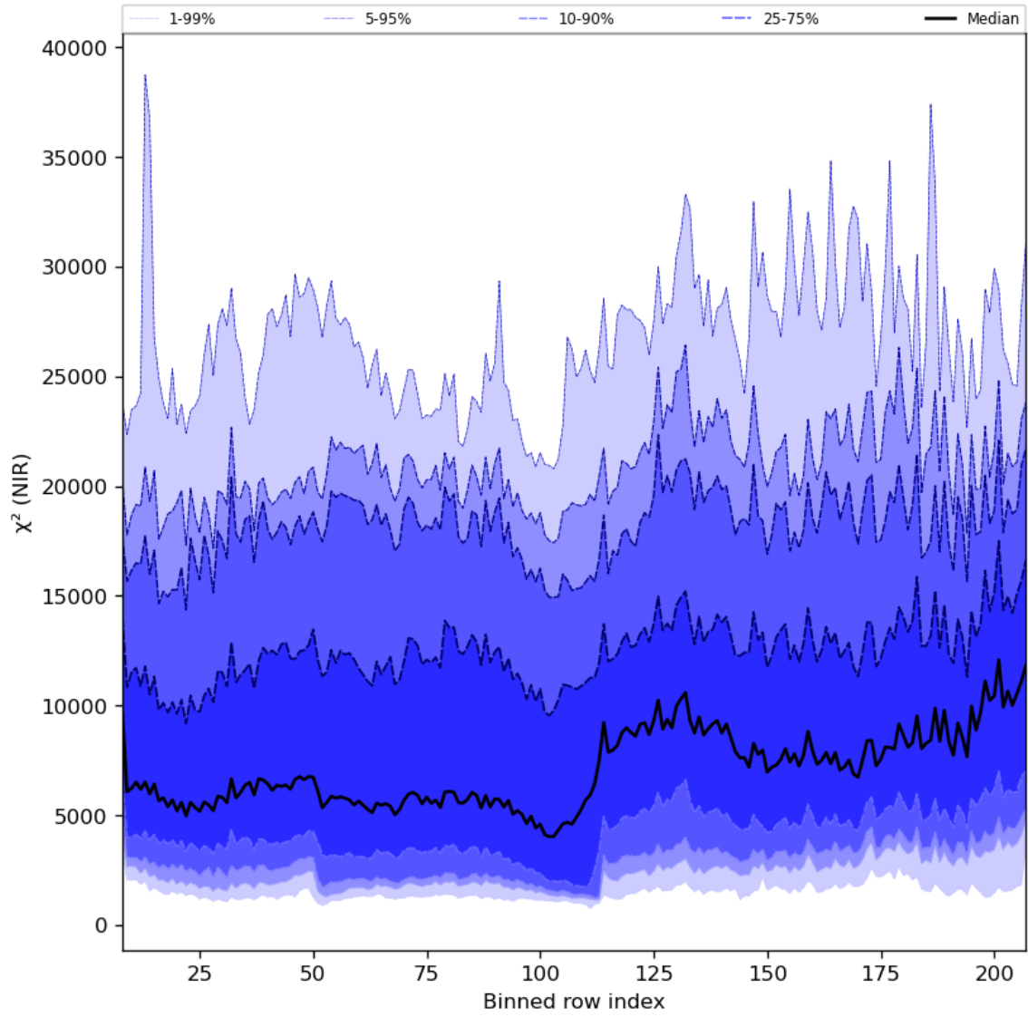
Figure 40: Along track statistics of “ \chi^2 (NIR)” for 2024-06-27 to 2024-06-29
