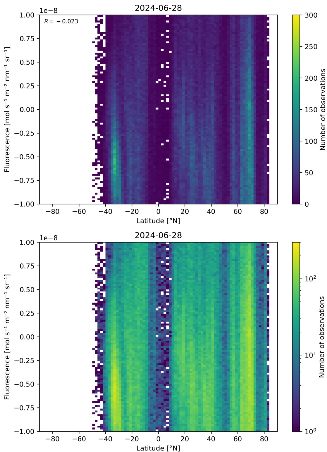
Figure 56: Scatter density plot of “Latitude” against “Fluorescence” for 2024-06-27 to 2024-06-29.
