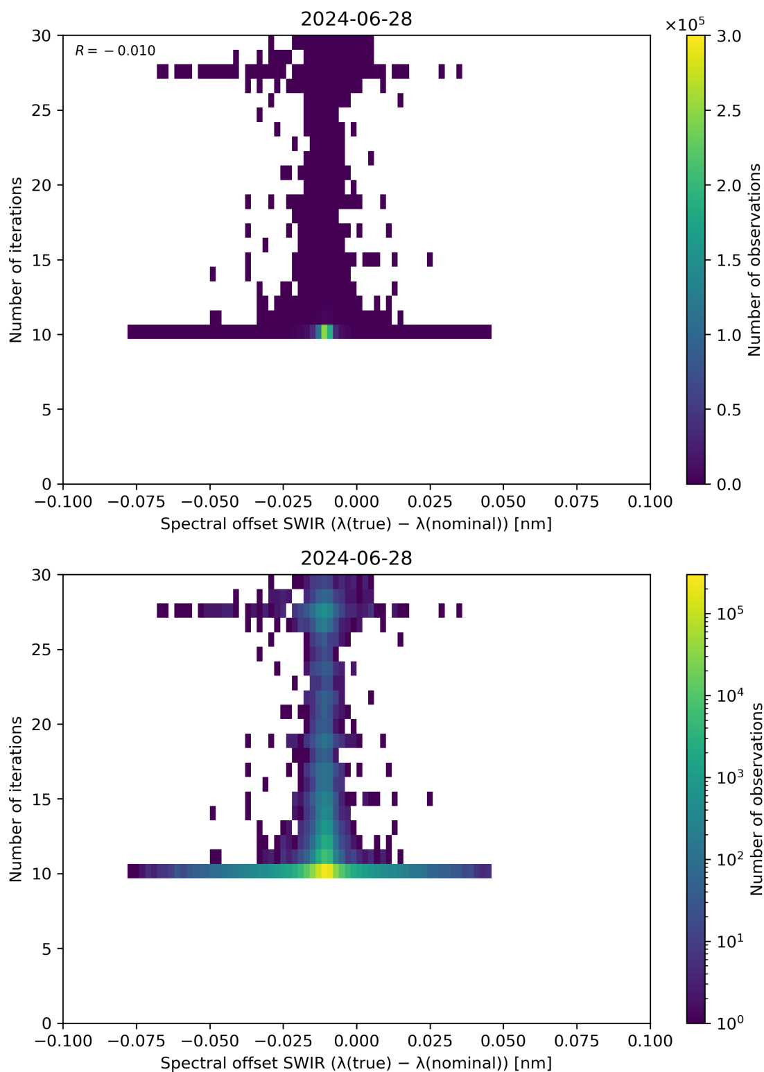
Figure 121: Scatter density plot of “Spectral offset SWIR ( \lambda(\text{true}) - \lambda(\text{nominal}) )” against “Number of iterations” for 2024-06-27 to 2024-06-29.
