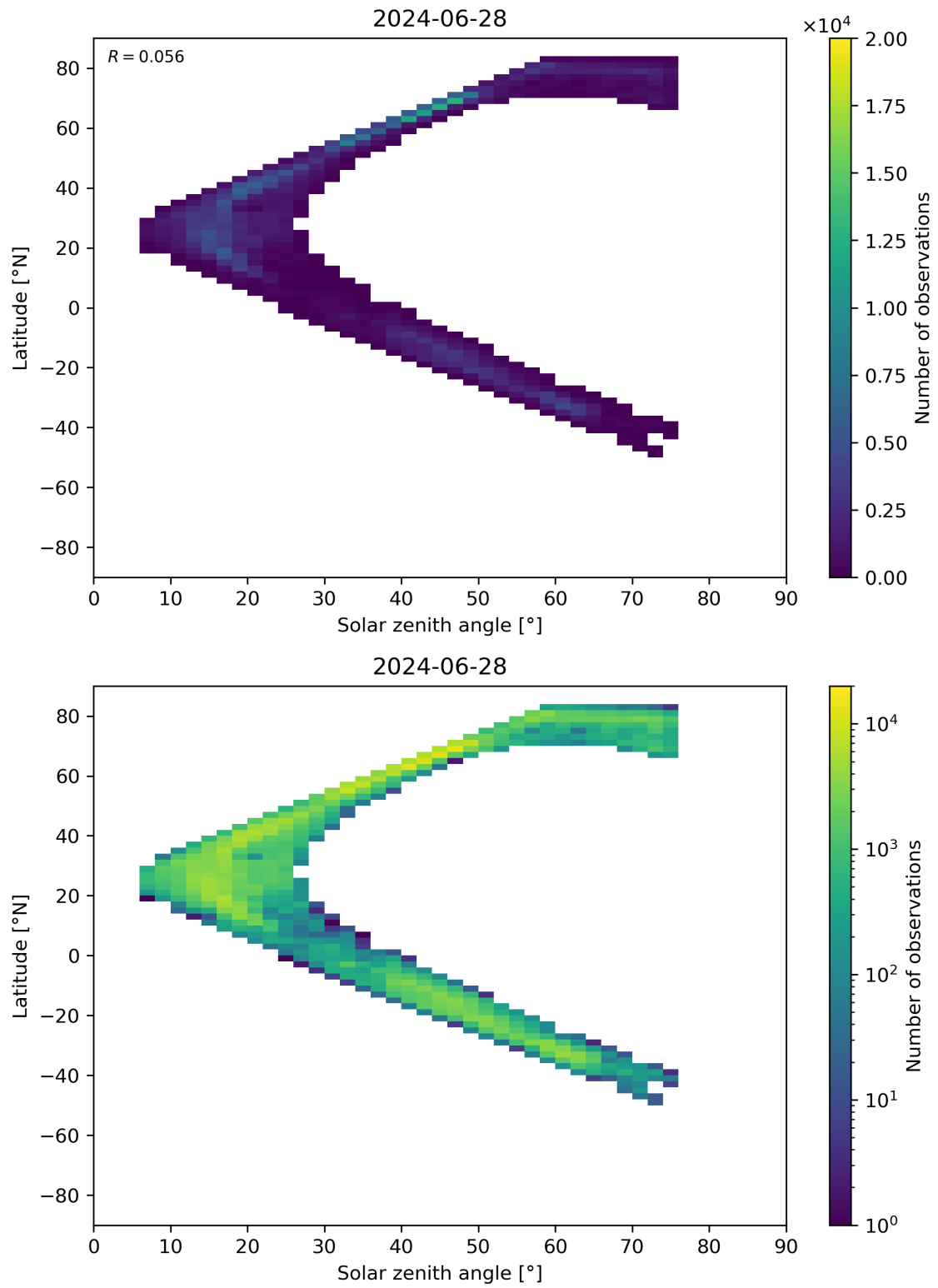
Figure 98: Scatter density plot of “Solar zenith angle” against “Latitude” for 2024-06-27 to 2024-06-29.
