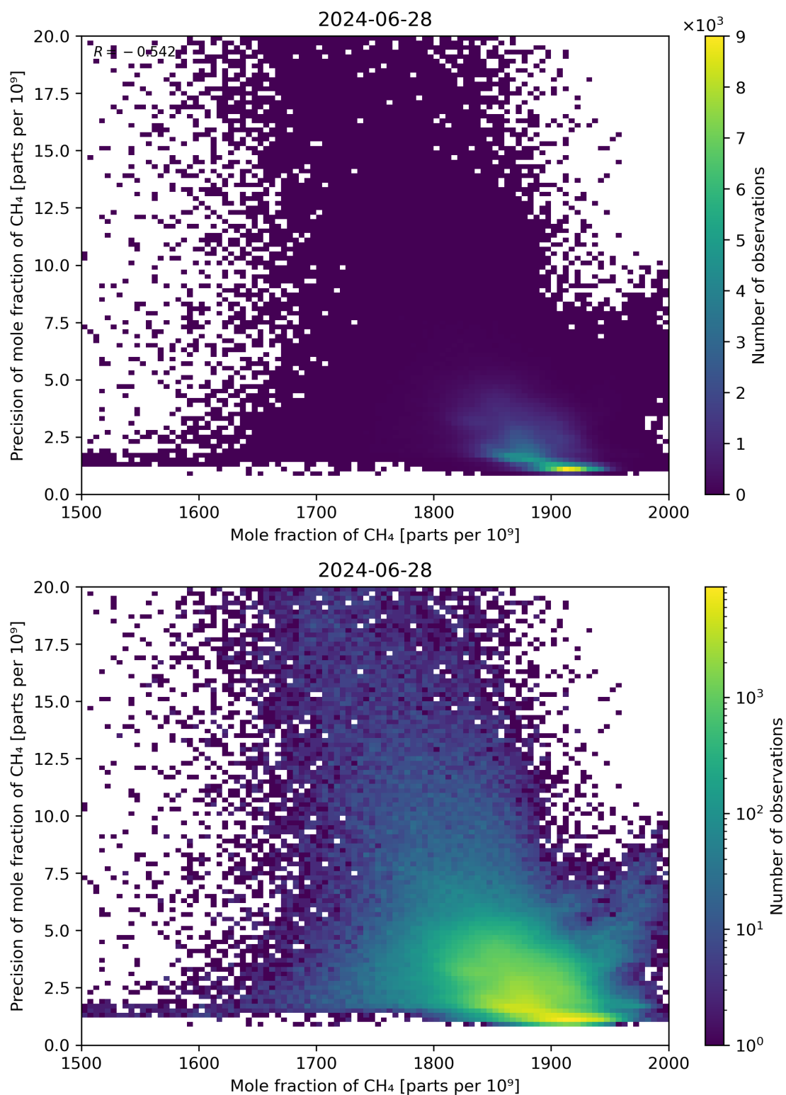
Figure 75: Scatter density plot of “Mole fraction of CH 4 ” against “Precision of mole fraction of CH 4 ” for 2024-06-27 to 2024-06-29.
