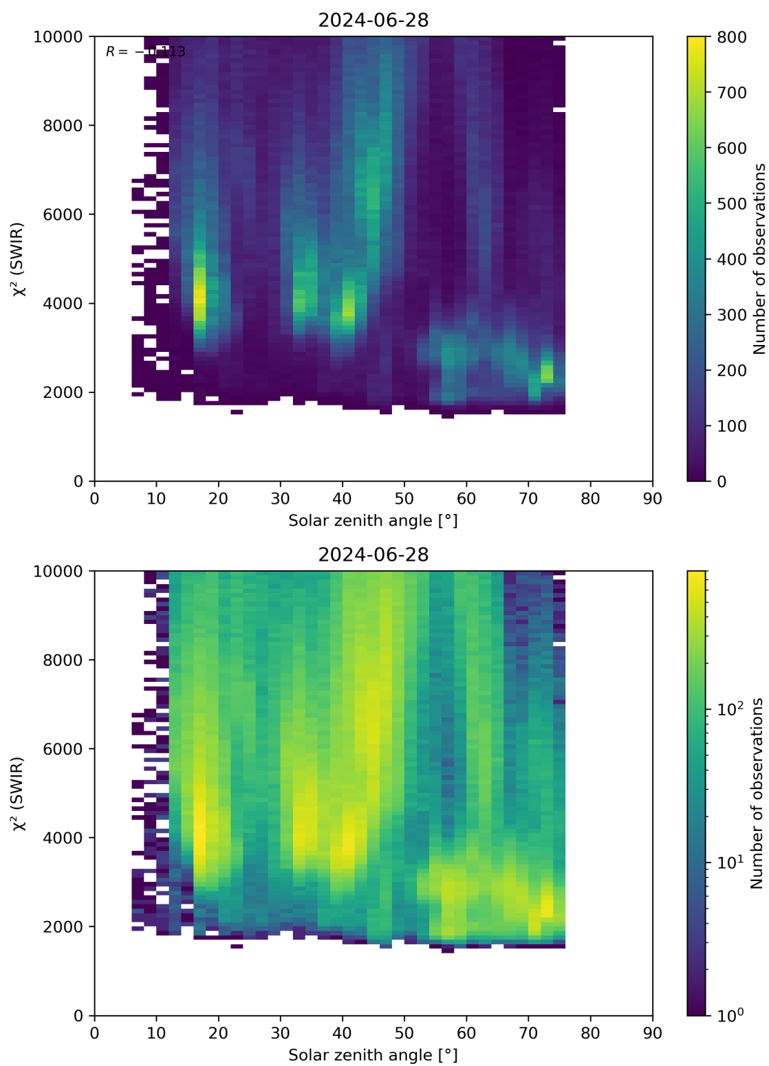
Figure 95: Scatter density plot of “Solar zenith angle” against “ \chi^2 (SWIR)” for 2024-06-27 to 2024-06-29.
