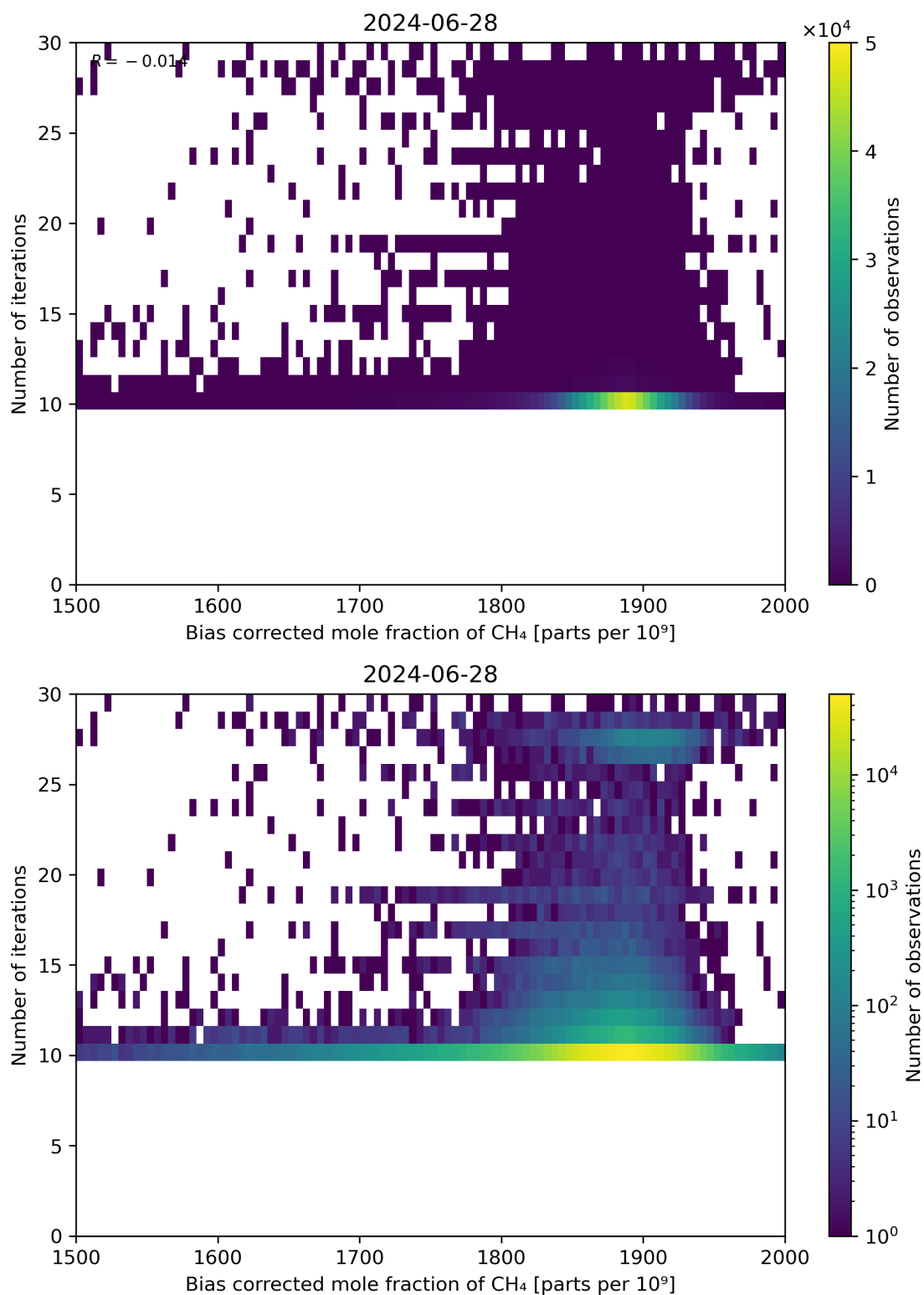
Figure 67: Scatter density plot of “Bias corrected mole fraction of \text{CH}_4 ” against “Number of iterations” for 2024-06-27 to 2024-06-29.
