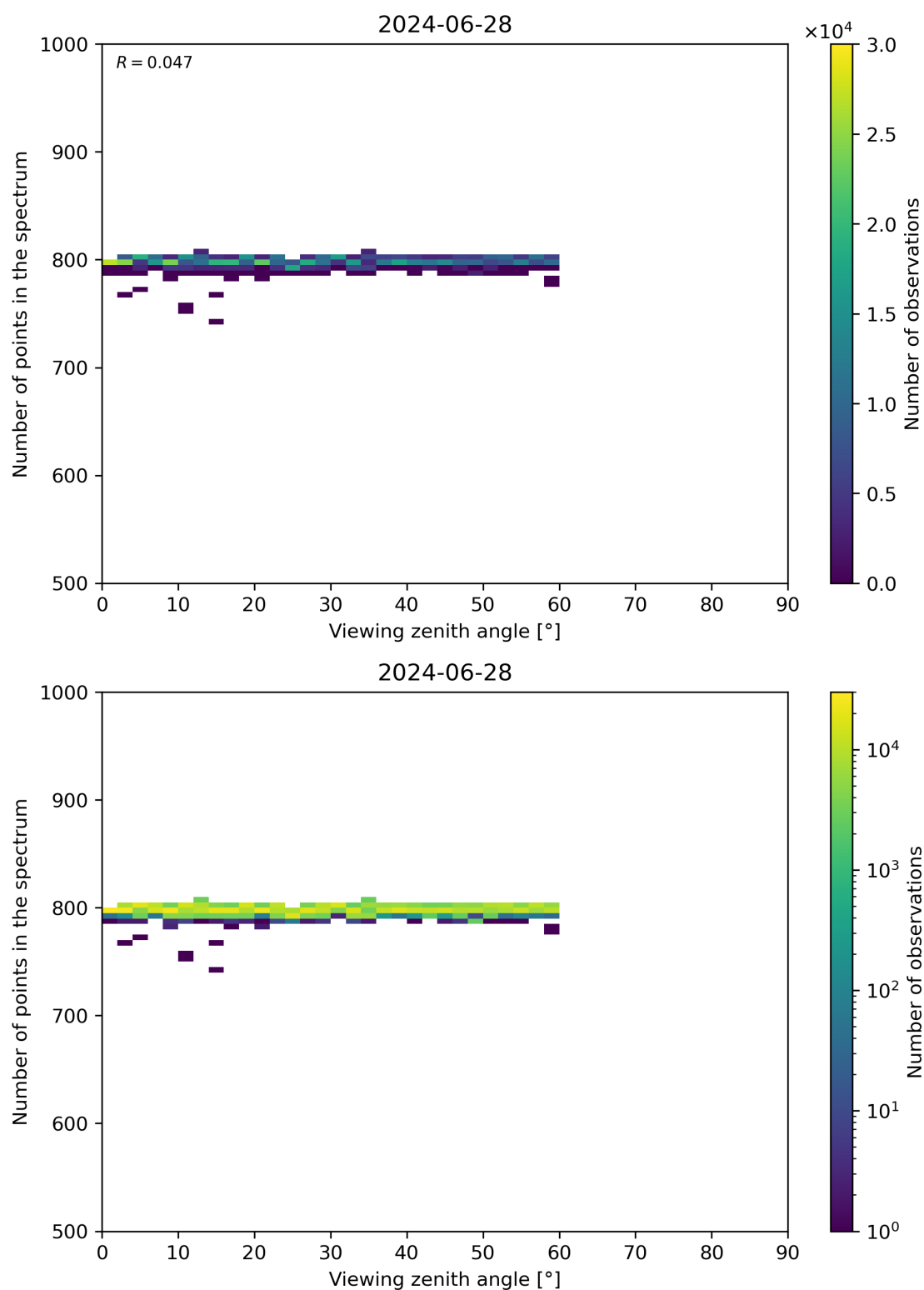
Figure 114: Scatter density plot of “Viewing zenith angle” against “Number of points in the spectrum” for 2024-06-27 to 2024-06-29.
