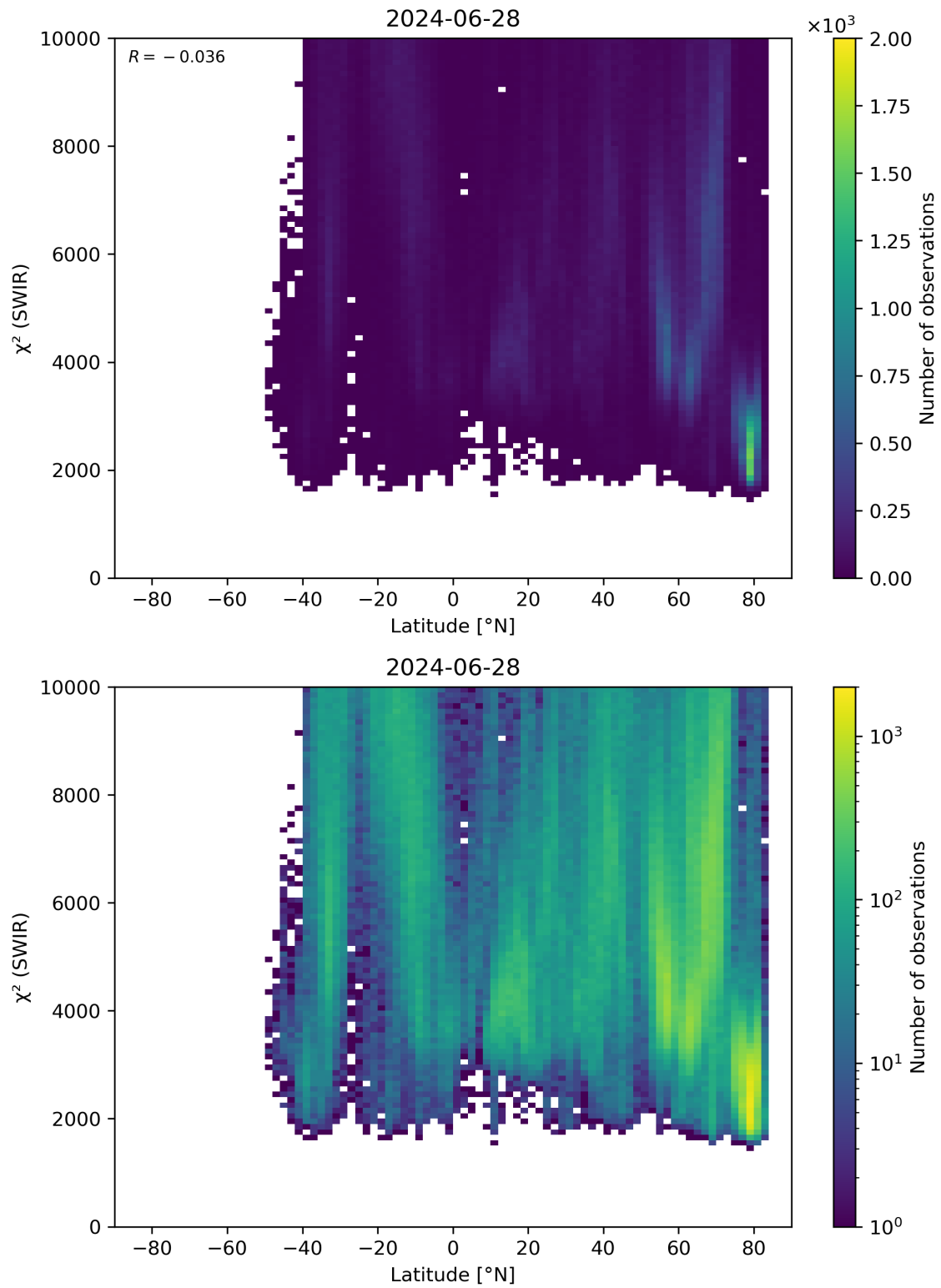
Figure 54: Scatter density plot of “Latitude” against “ \chi^2 (SWIR)” for 2024-06-27 to 2024-06-29.
