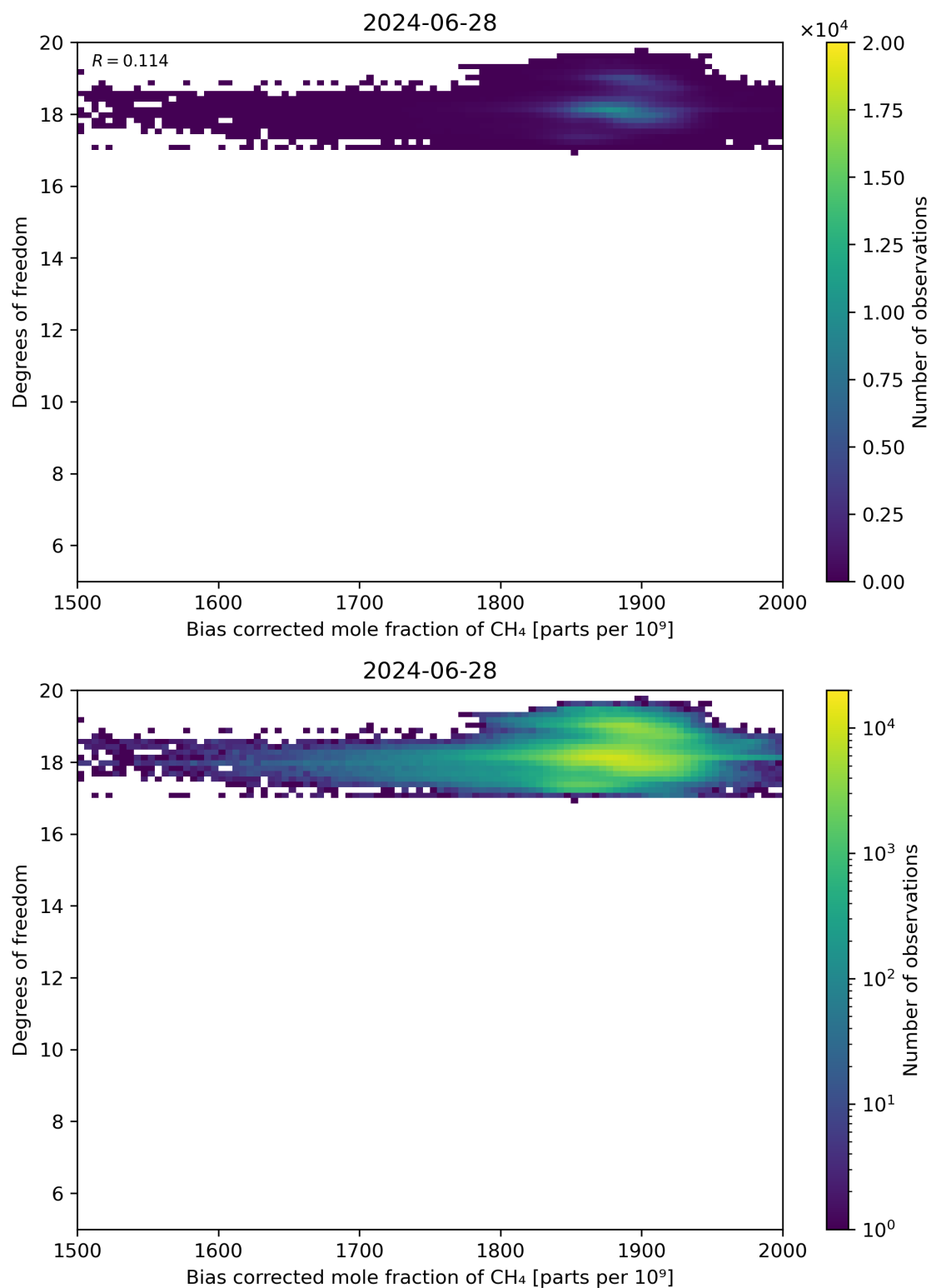
Figure 65: Scatter density plot of “Bias corrected mole fraction of CH 4 ” against “Degrees of freedom” for 2024-06-27 to 2024-06-29.
