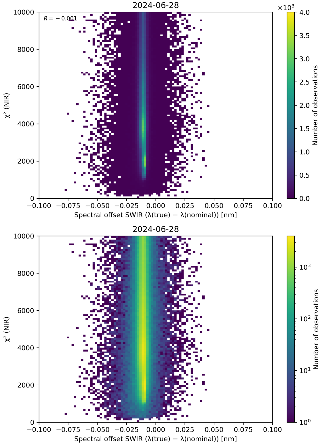
Figure 117: Scatter density plot of “Spectral offset SWIR ( \lambda(\text{true}) - \lambda(\text{nominal}) )” against “ \chi^2 (NIR)” for 2024-06-27 to 2024-06-29.
