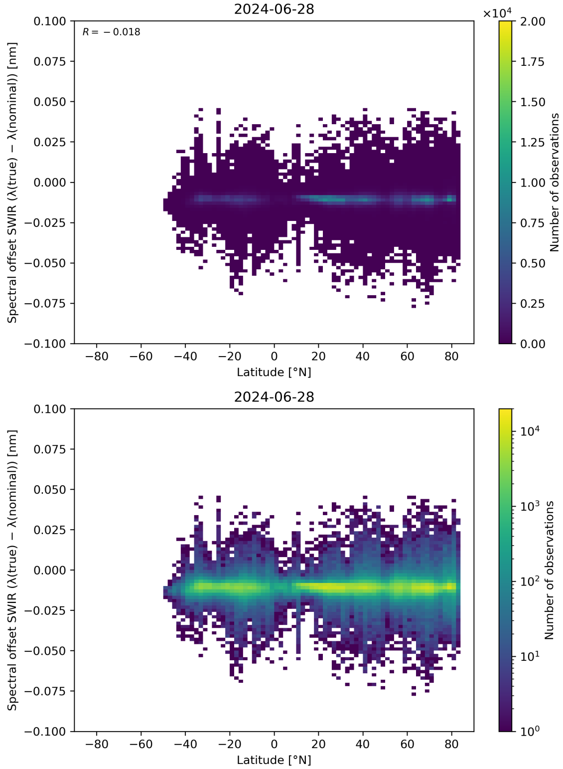
Figure 62: Scatter density plot of “Latitude” against “Spectral offset SWIR ( \lambda(\text{true}) - \lambda(\text{nominal}) )” for 2024-06-27 to 2024-06-29.
