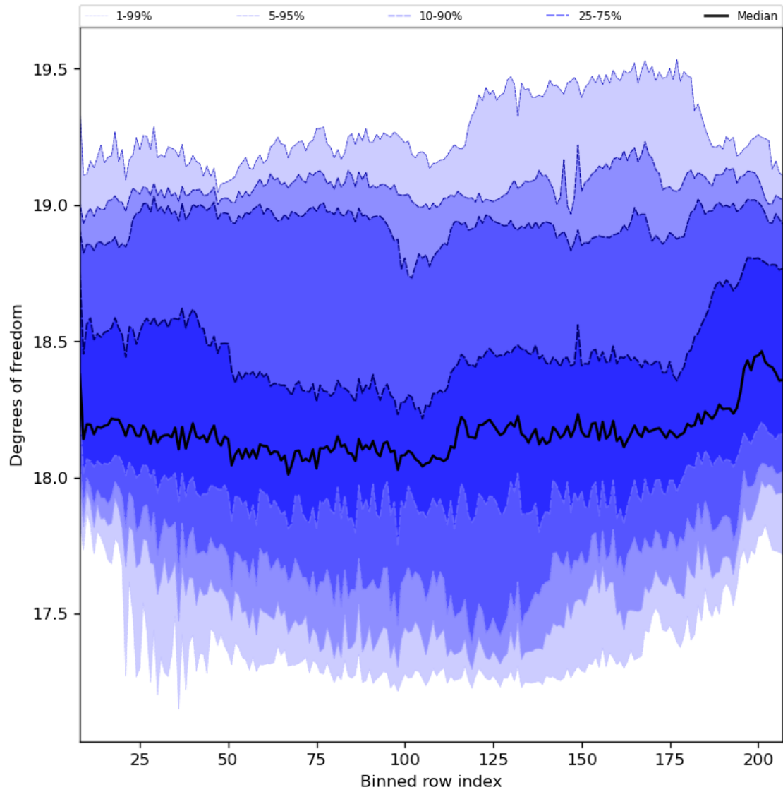
Figure 41: Along track statistics of “Degrees of freedom” for 2024-06-27 to 2024-06-29
