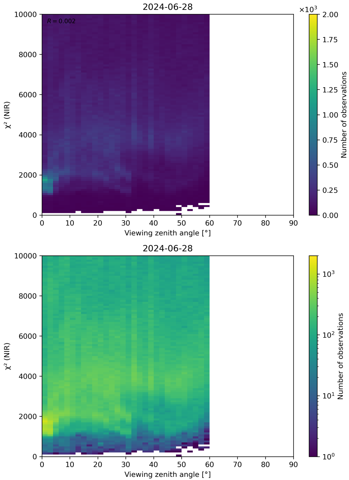
Figure 105: Scatter density plot of “Viewing zenith angle” against “ \chi^2 (NIR)” for 2024-06-27 to 2024-06-29.
