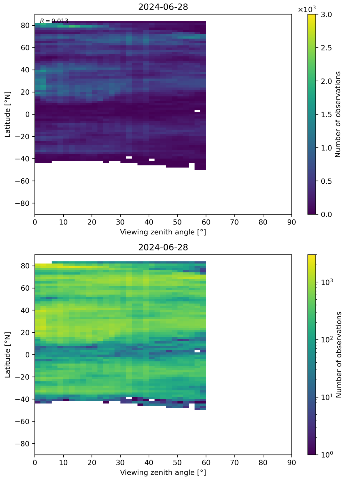
Figure 109: Scatter density plot of “Viewing zenith angle” against “Latitude” for 2024-06-27 to 2024-06-29.
