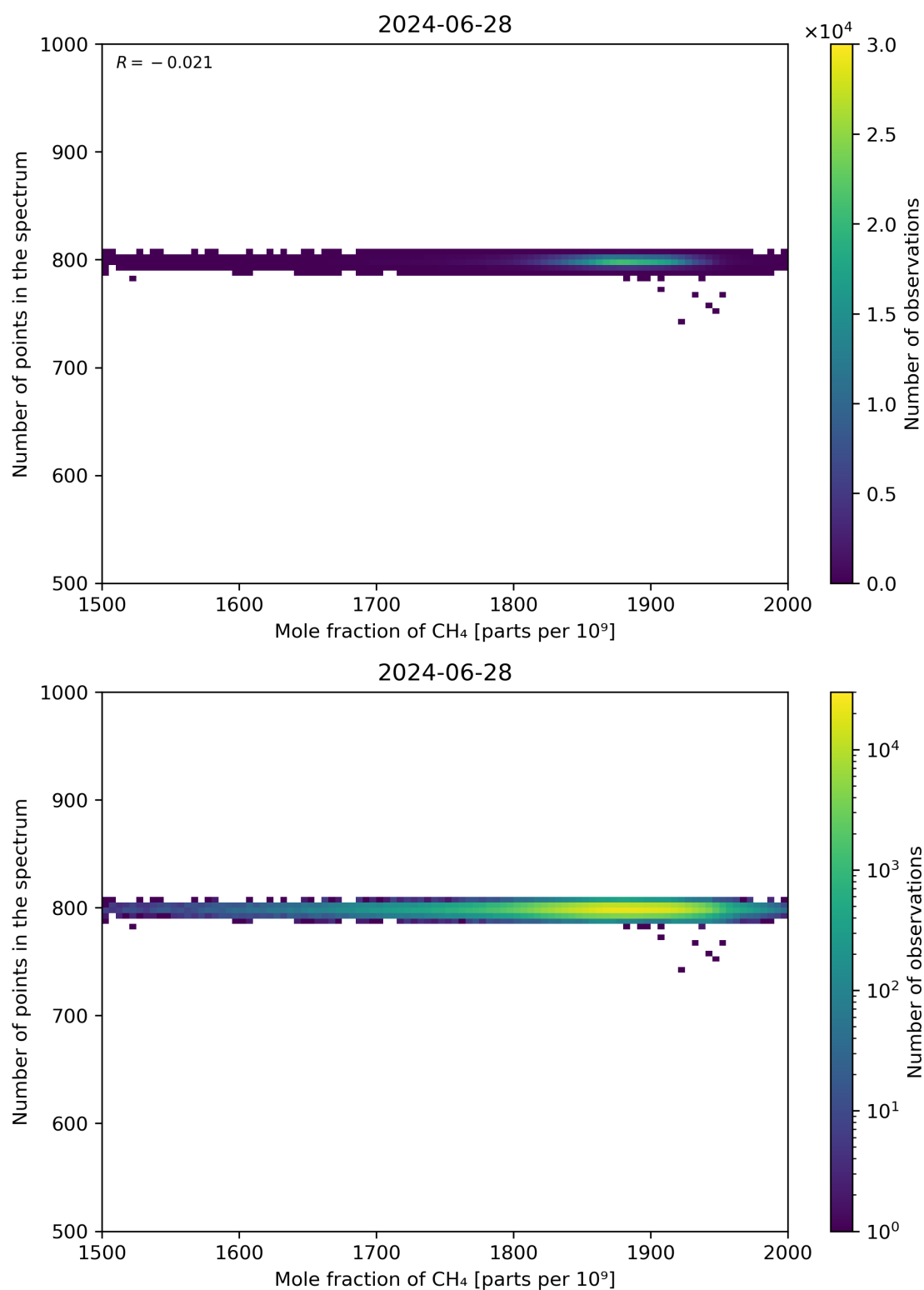
Figure 77: Scatter density plot of “Mole fraction of CH 4 ” against “Number of points in the spectrum” for 2024-06-27 to 2024-06-29.
