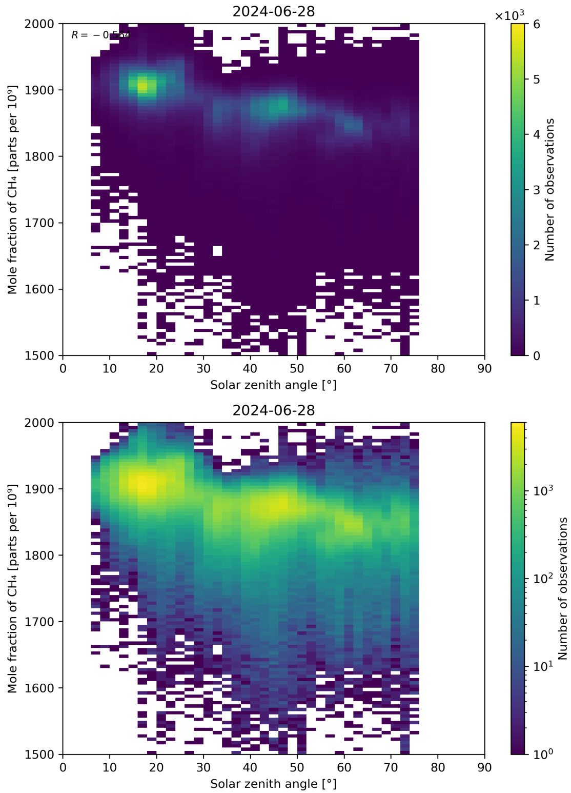
Figure 99: Scatter density plot of “Solar zenith angle” against “Mole fraction of \text{CH}_4 ” for 2024-06-27 to 2024-06-29.
