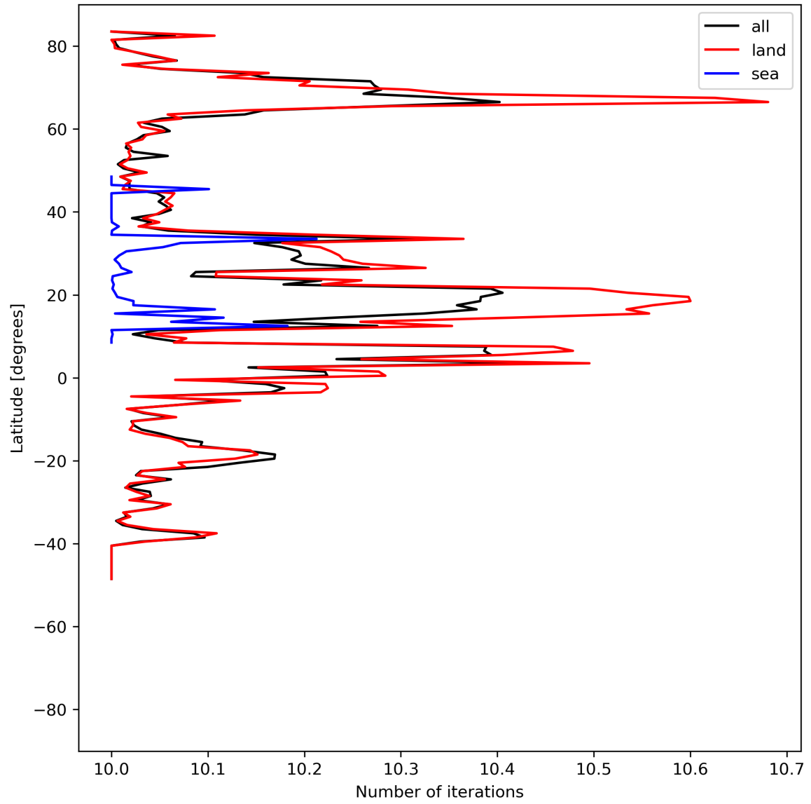
Figure 20: Zonal average of “Number of iterations” for 2024-06-27 to 2024-06-29.
