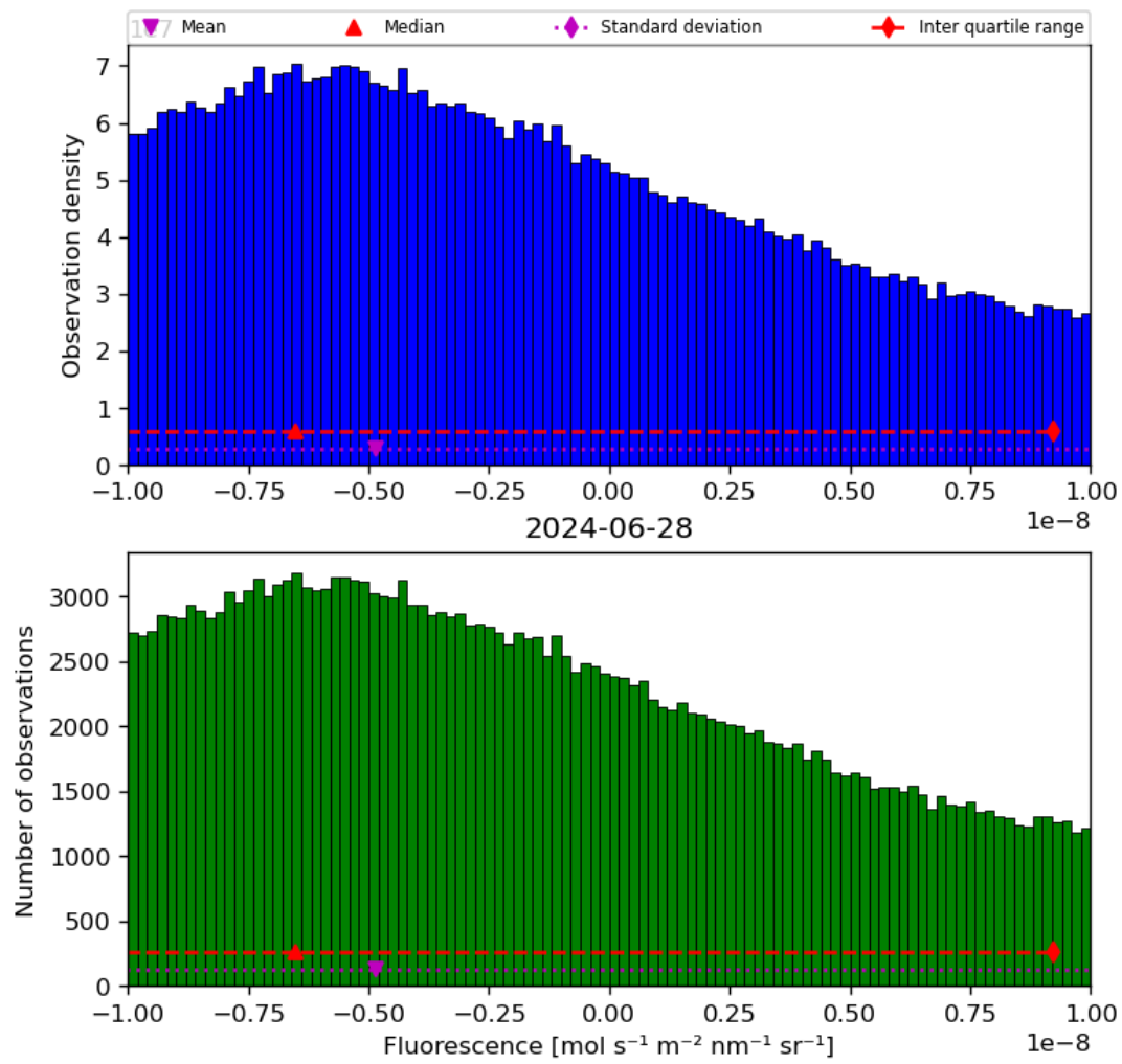
Figure 32: Histogram of “Fluorescence” for 2024-06-27 to 2024-06-29
