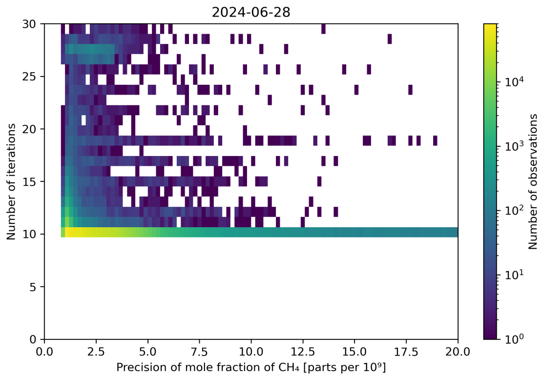
Figure 83: Scatter density plot of “Precision of mole fraction of CH 4 ” against “Number of iterations” for 2024-06-27 to 2024-06-29.
