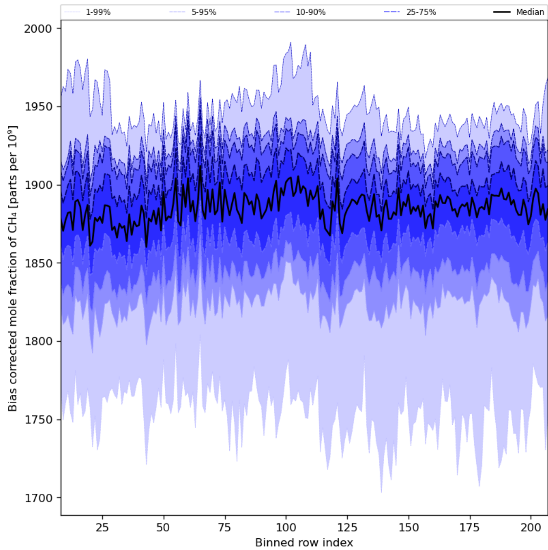
Figure 36: Along track statistics of “Bias corrected mole fraction of CH 4 ” for 2024-06-27 to 2024-06-29
