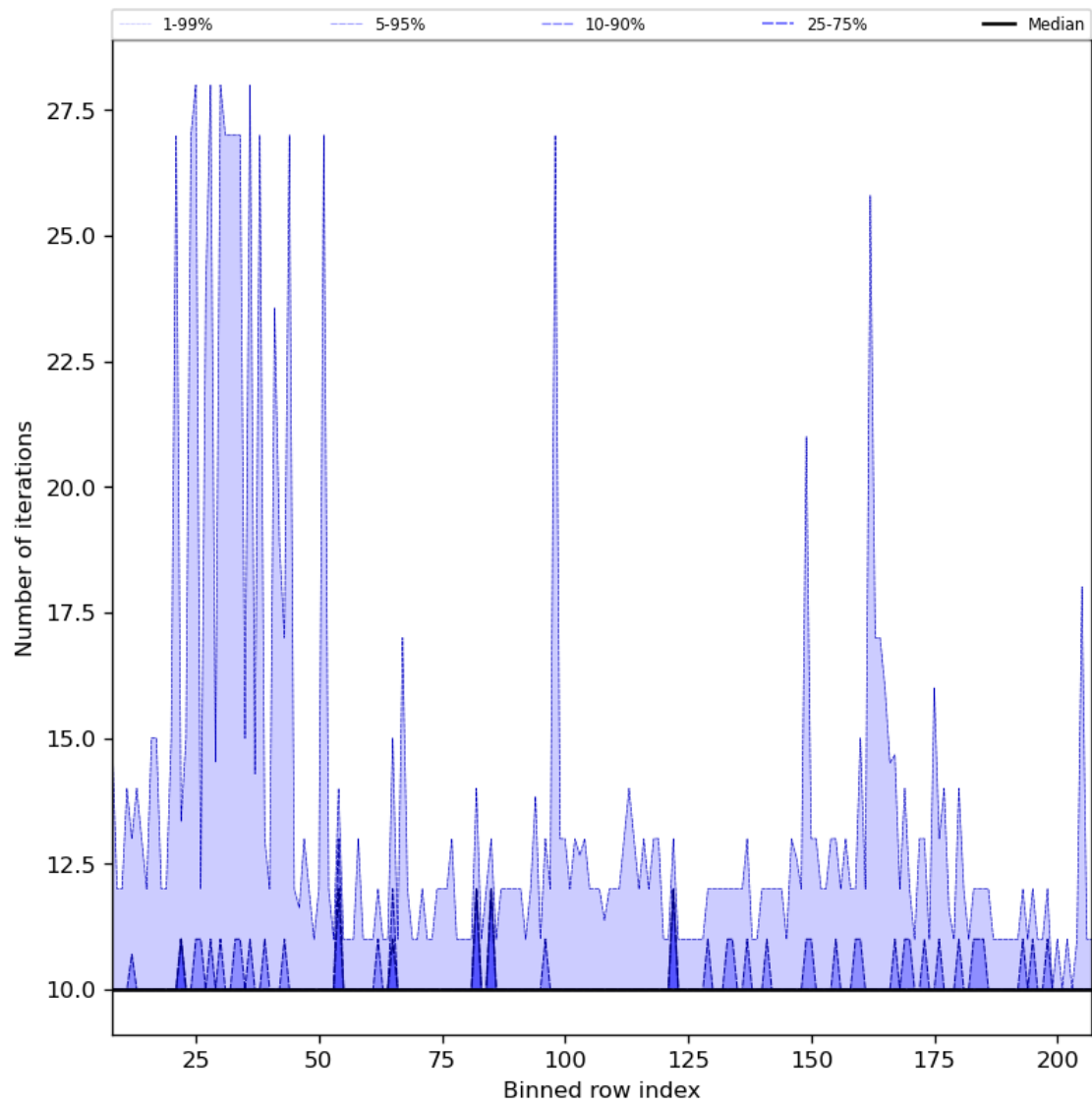
Figure 42: Along track statistics of “Number of iterations” for 2024-06-27 to 2024-06-29
