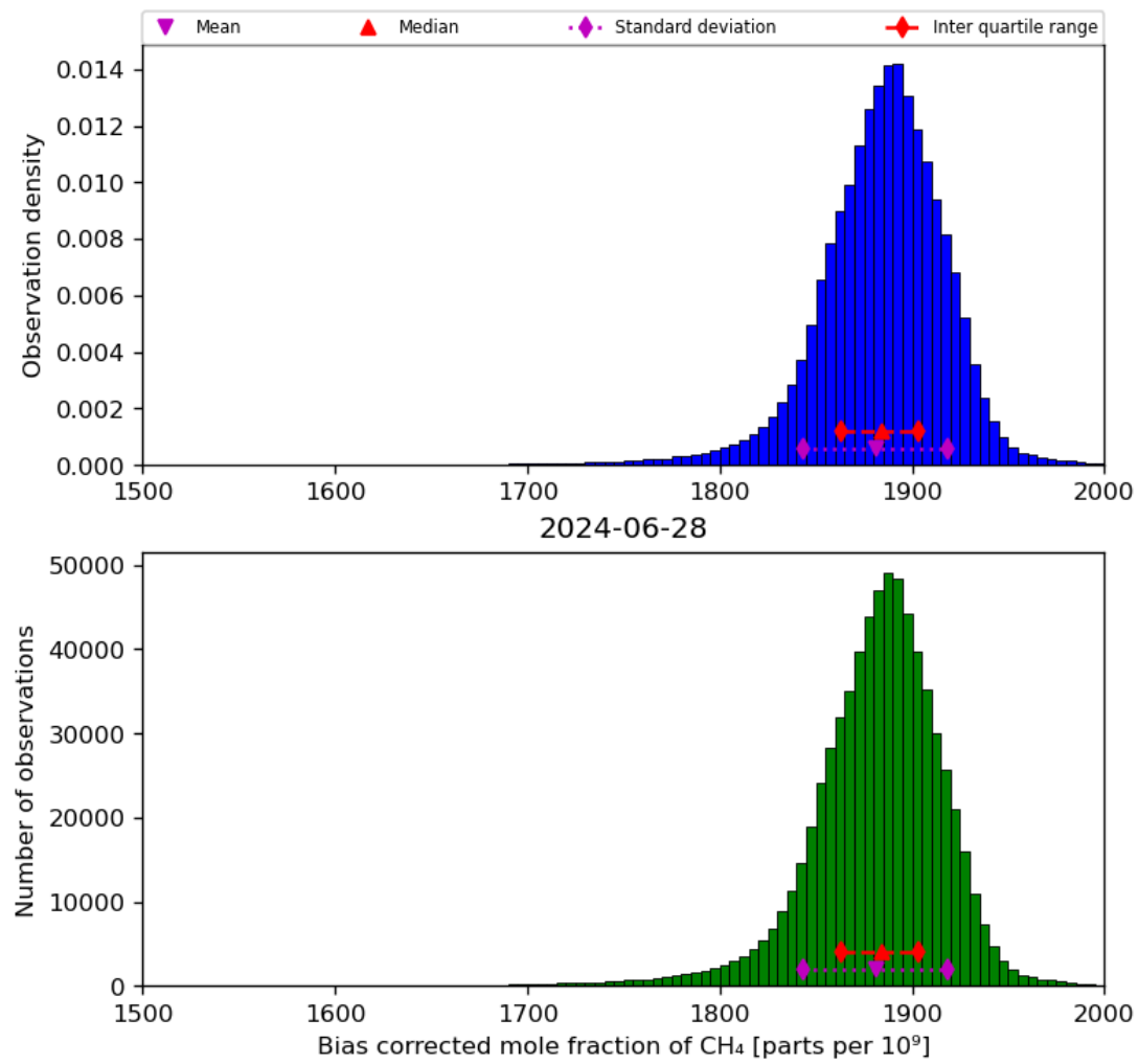
Figure 25: Histogram of “Bias corrected mole fraction of CH 4 ” for 2024-06-27 to 2024-06-29
