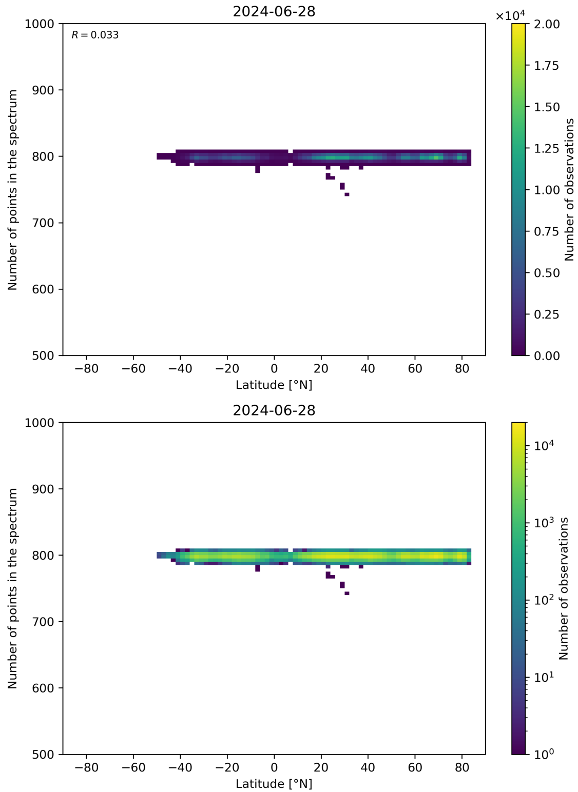
Figure 61: Scatter density plot of “Latitude” against “Number of points in the spectrum” for 2024-06-27 to 2024-06-29.
