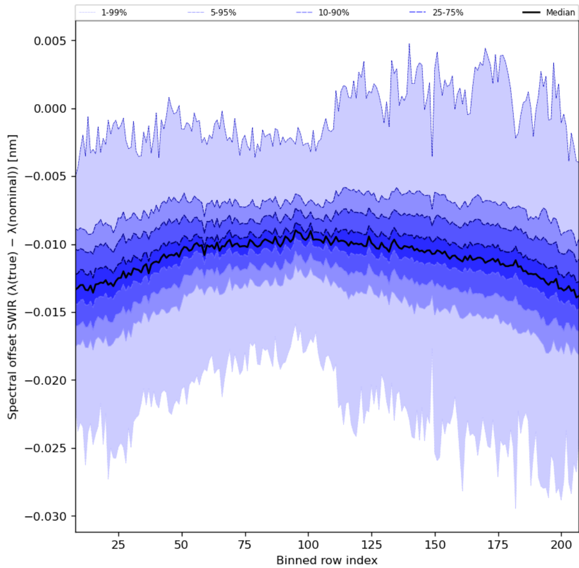
Figure 38: Along track statistics of “Spectral offset SWIR ( \lambda(\text{true}) - \lambda(\text{nominal}) )” for 2024-06-27 to 2024-06-29
