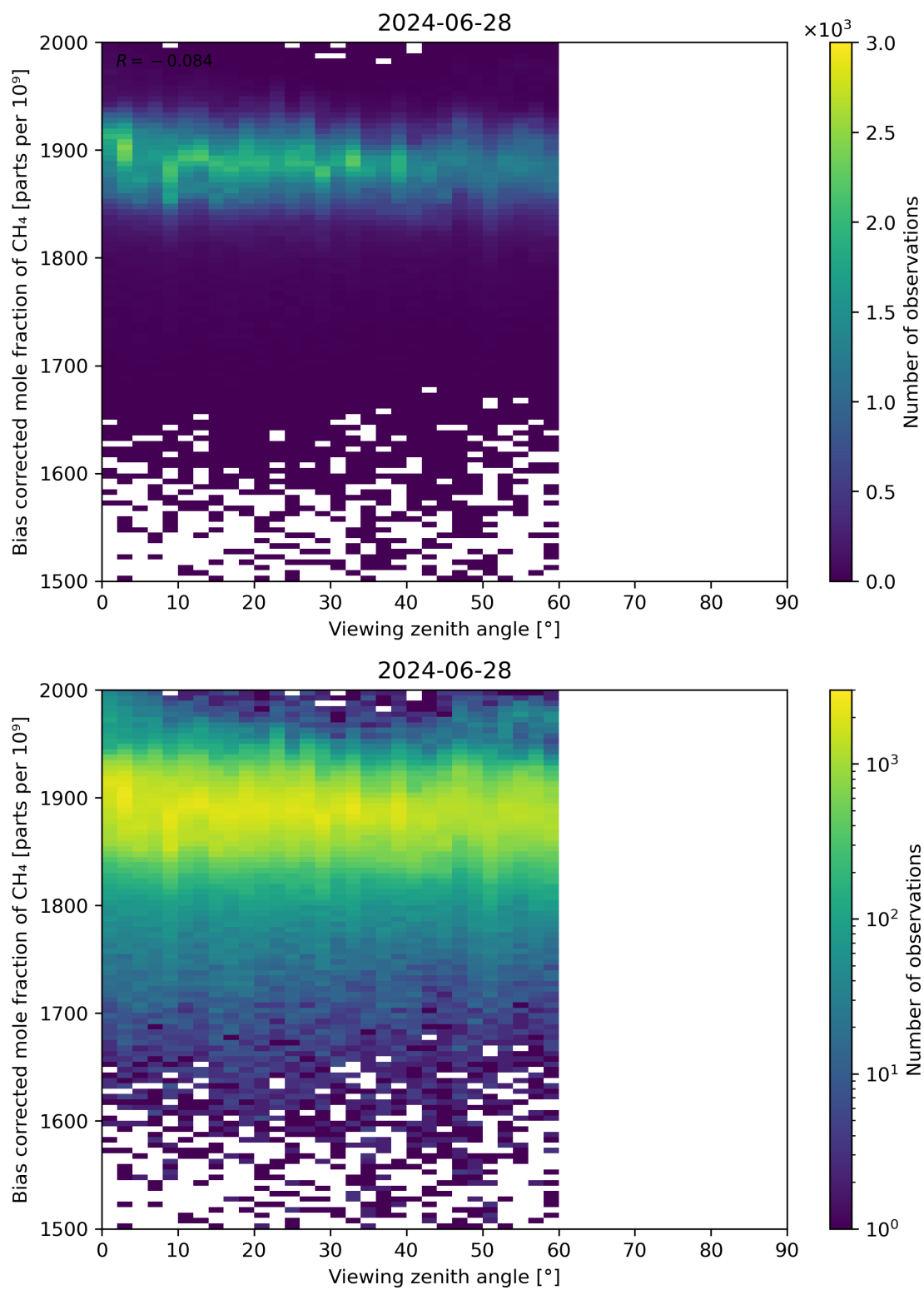
Figure 111: Scatter density plot of “Viewing zenith angle” against “Bias corrected mole fraction of CH 4 ” for 2024-06-27 to 2024-06-29.
