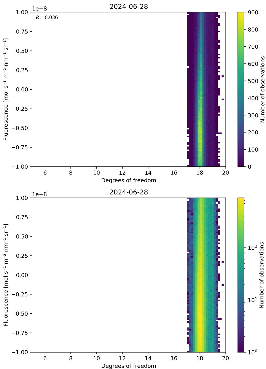
Figure 51: Scatter density plot of “Degrees of freedom” against “Fluorescence” for 2024-06-27 to 2024-06-29.
