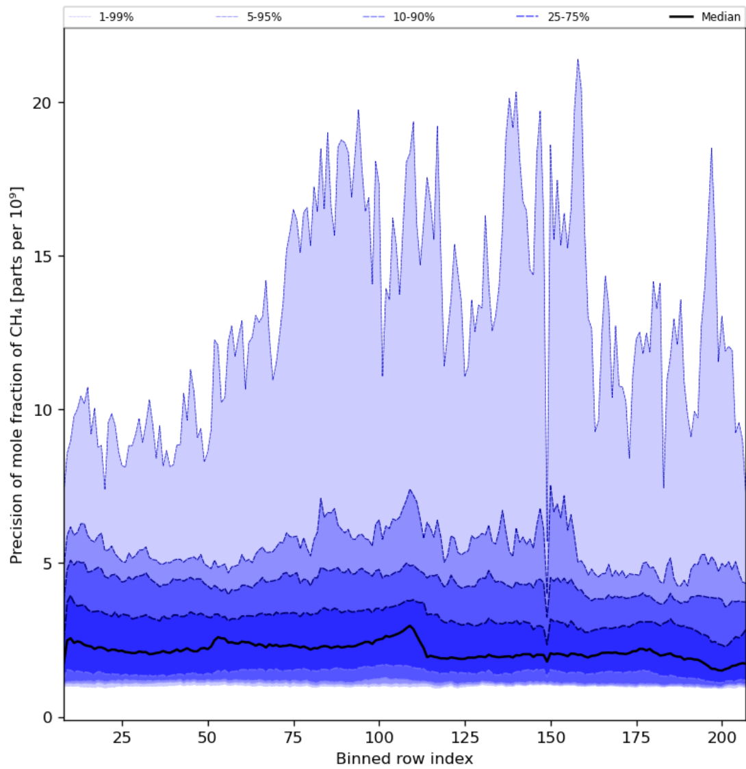
Figure 35: Along track statistics of “Precision of mole fraction of CH 4 ” for 2024-06-27 to 2024-06-29
