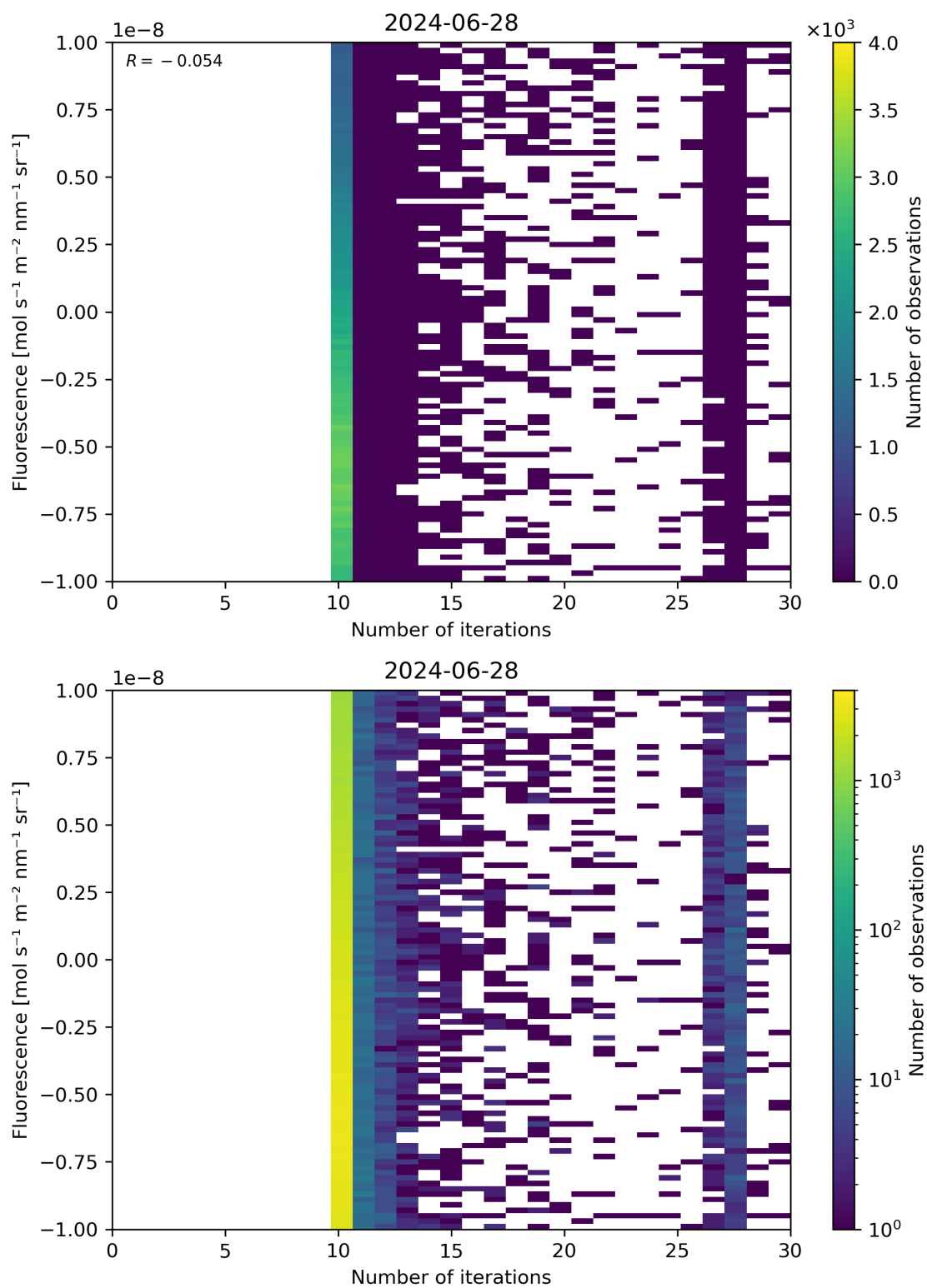
Figure 87: Scatter density plot of “Number of iterations” against “Fluorescence” for 2024-06-27 to 2024-06-29.
