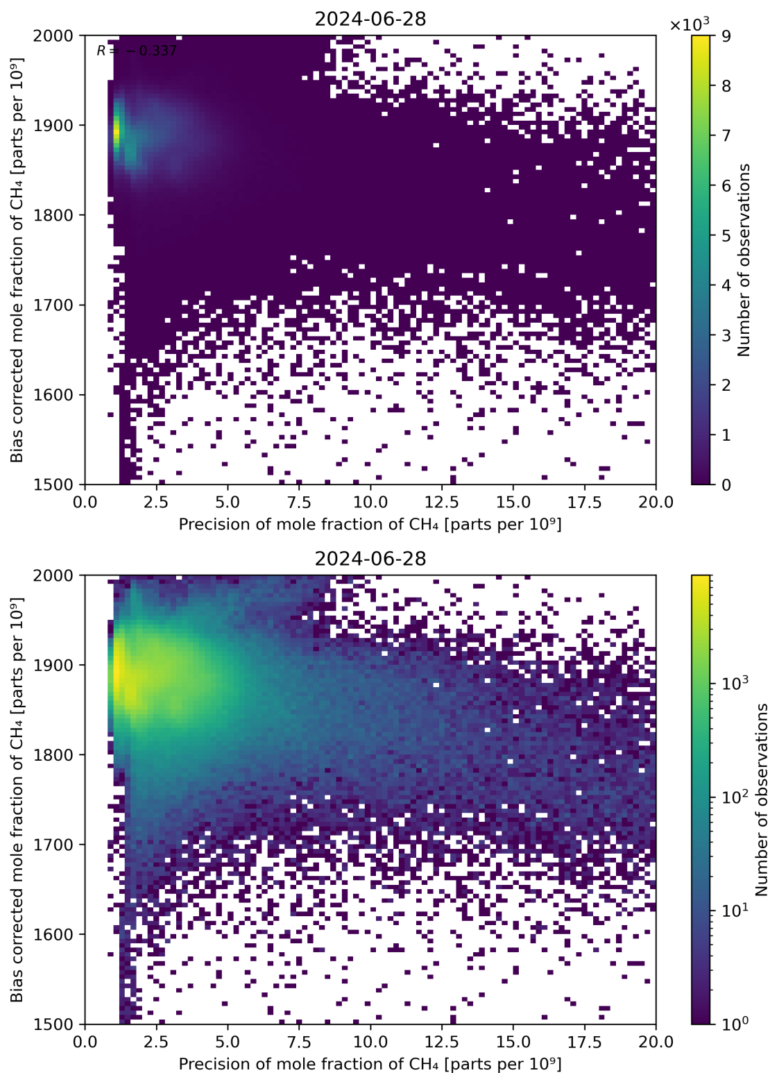
Figure 82: Scatter density plot of “Precision of mole fraction of CH 4 ” against “Bias corrected mole fraction of CH 4 ” for 2024-06-27 to 2024-06-29.
