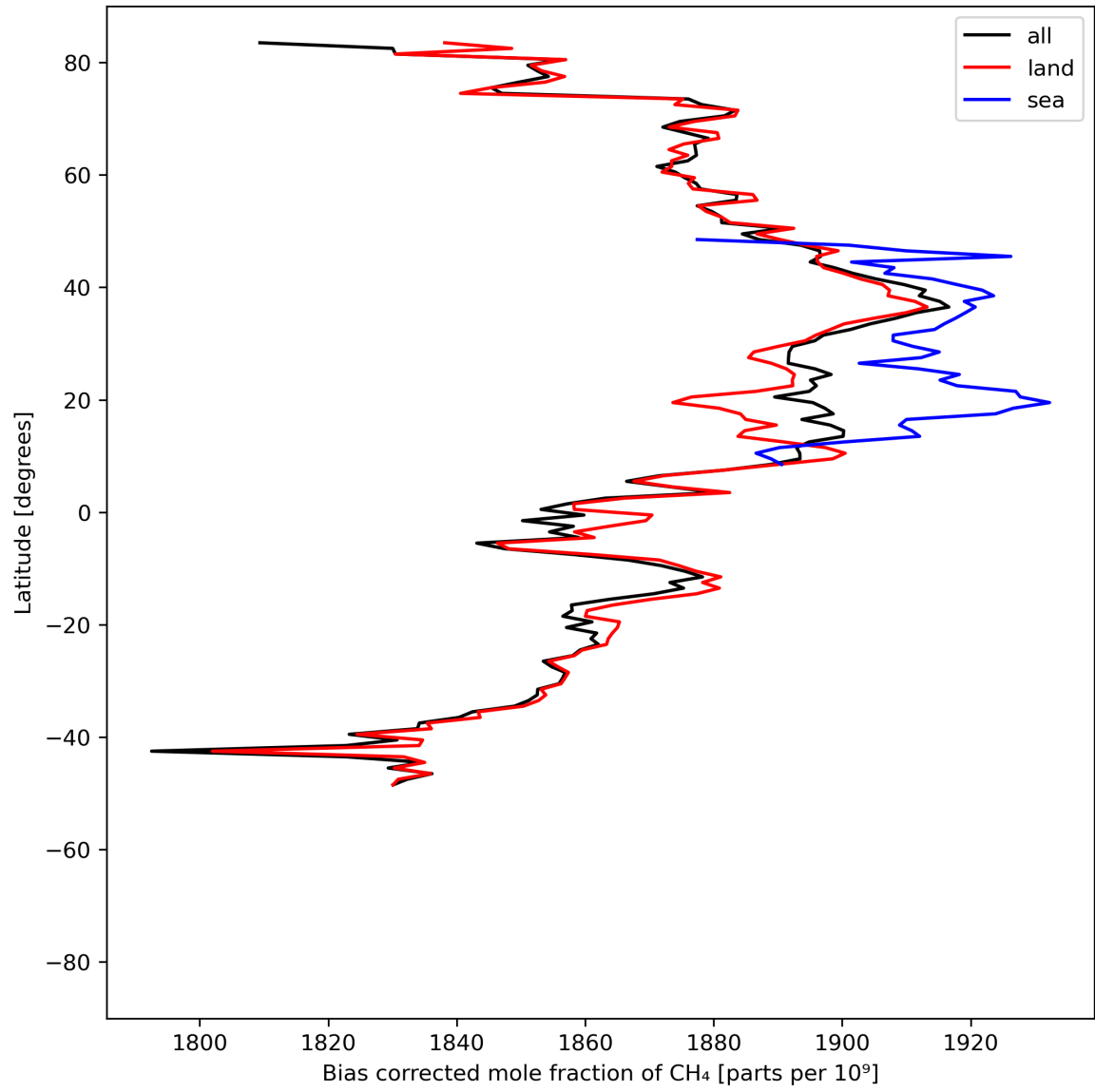
Figure 14: Zonal average of “Bias corrected mole fraction of CH 4 ” for 2024-06-27 to 2024-06-29.
