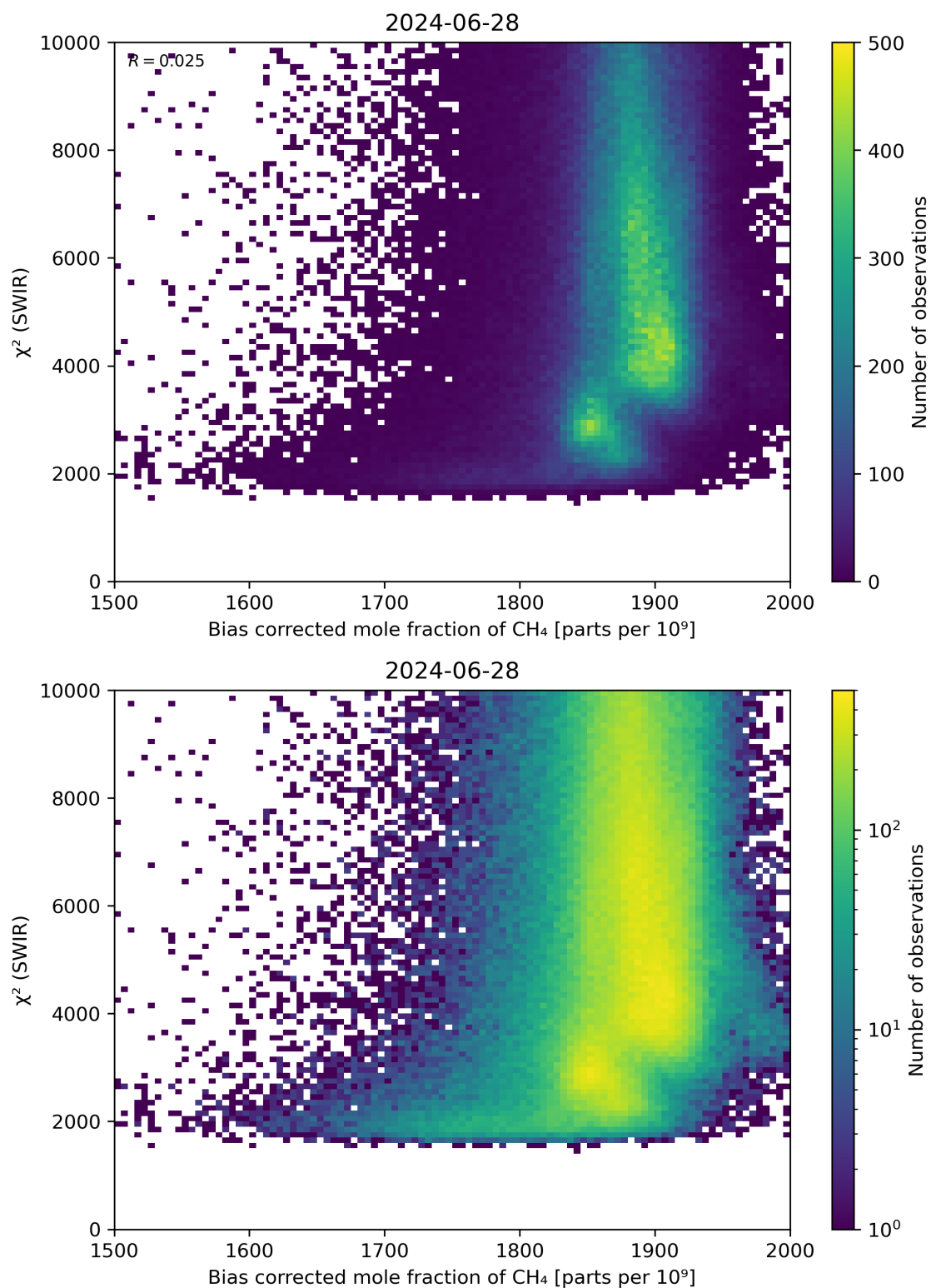
Figure 64: Scatter density plot of “Bias corrected mole fraction of \text{CH}_4 ” against “ \chi^2 (SWIR)” for 2024-06-27 to 2024-06-29.
