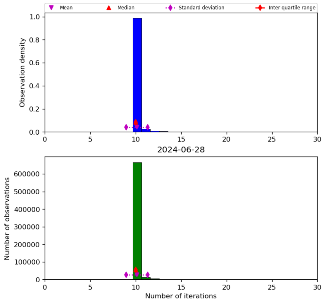
Figure 31: Histogram of “Number of iterations” for 2024-06-27 to 2024-06-29
