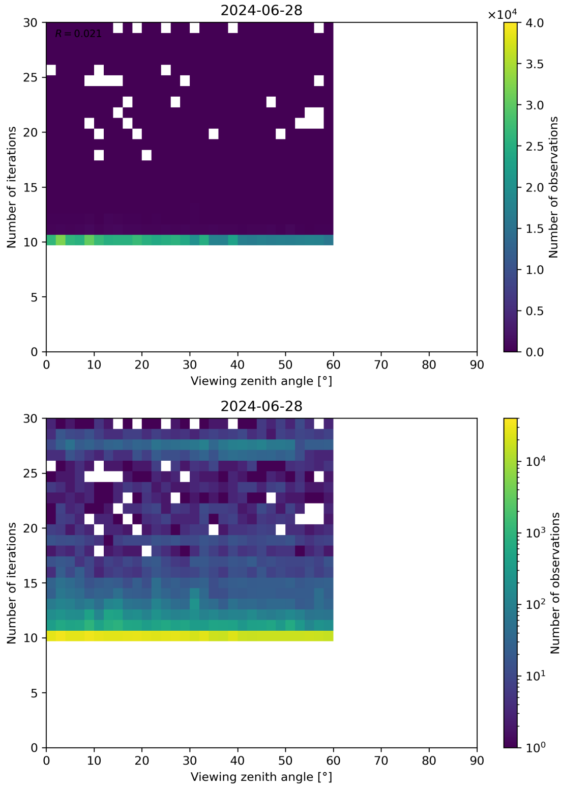
Figure 113: Scatter density plot of “Viewing zenith angle” against “Number of iterations” for 2024-06-27 to 2024-06-29.
