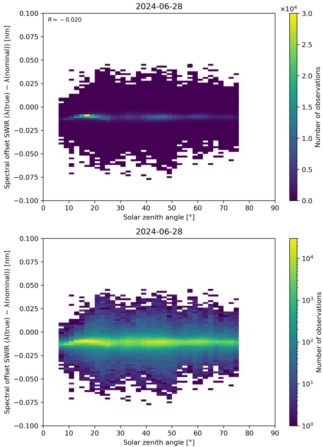
Figure 104: Scatter density plot of “Solar zenith angle” against “Spectral offset SWIR ( \lambda(\text{true}) - \lambda(\text{nominal}) )” for 2024-06-27 to 2024-06-29.
