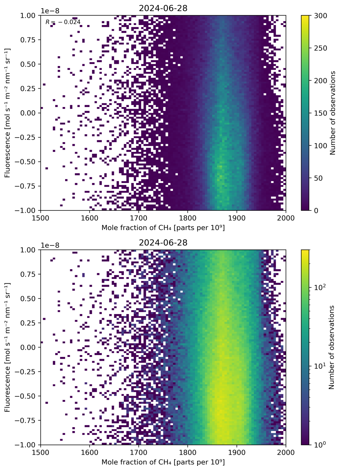
Figure 73: Scatter density plot of “Mole fraction of \text{CH}_4 ” against “Fluorescence” for 2024-06-27 to 2024-06-29.
