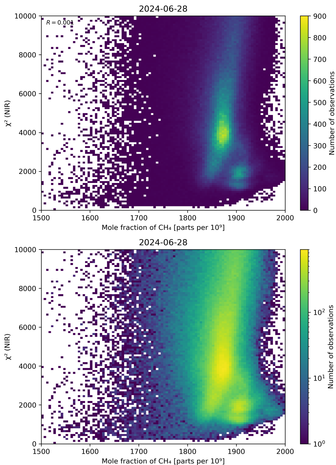
Figure 70: Scatter density plot of “Mole fraction of CH 4 ” against “ \chi^2 (NIR)” for 2024-06-27 to 2024-06-29.
