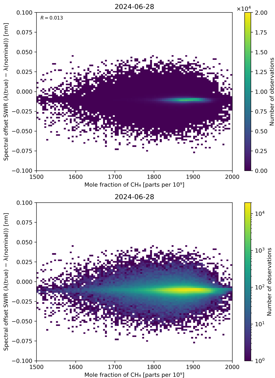
Figure 86: Scatter density plot of “Mole fraction of CH 4 ” against “Spectral offset SWIR ( \lambda(\text{true}) - \lambda(\text{nominal}) )” for 2024-06-27 to 2024-06-29.
