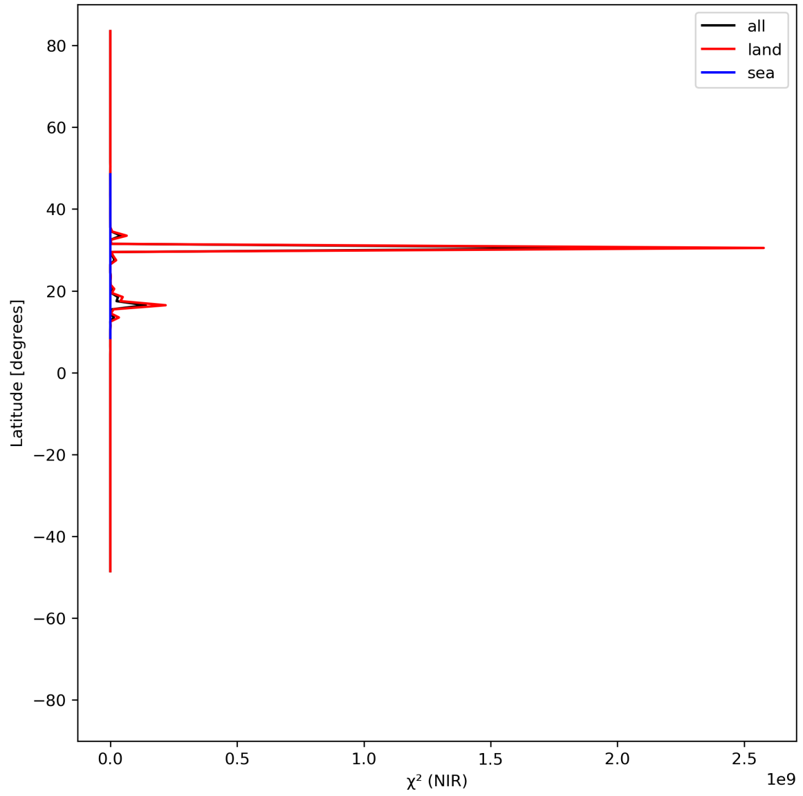
Figure 18: Zonal average of “ \chi^2 (NIR)” for 2024-06-27 to 2024-06-29.
