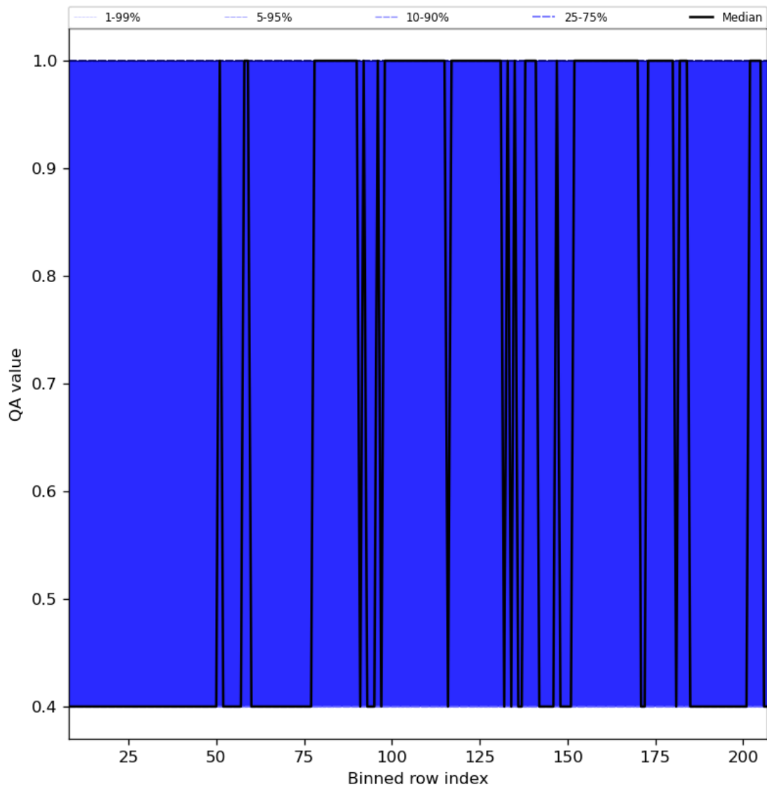
Figure 33: Along track statistics of “QA value” for 2024-06-27 to 2024-06-29
