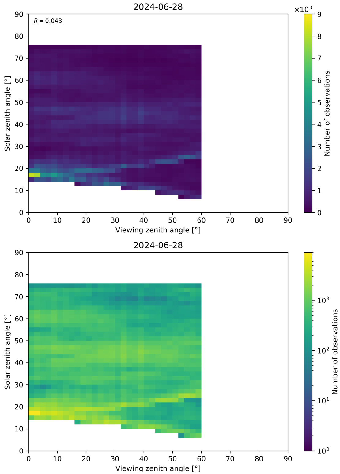
Figure 115: Scatter density plot of “Viewing zenith angle” against “Solar zenith angle” for 2024-06-27 to 2024-06-29.
