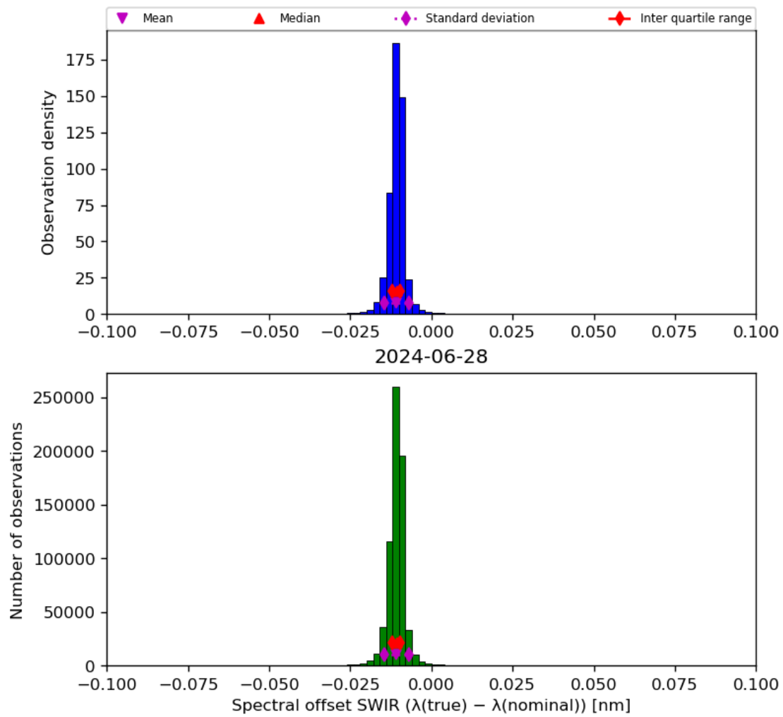
Figure 27: Histogram of “Spectral offset SWIR ( \lambda(\text{true}) - \lambda(\text{nominal}) )” for 2024-06-27 to 2024-06-29
