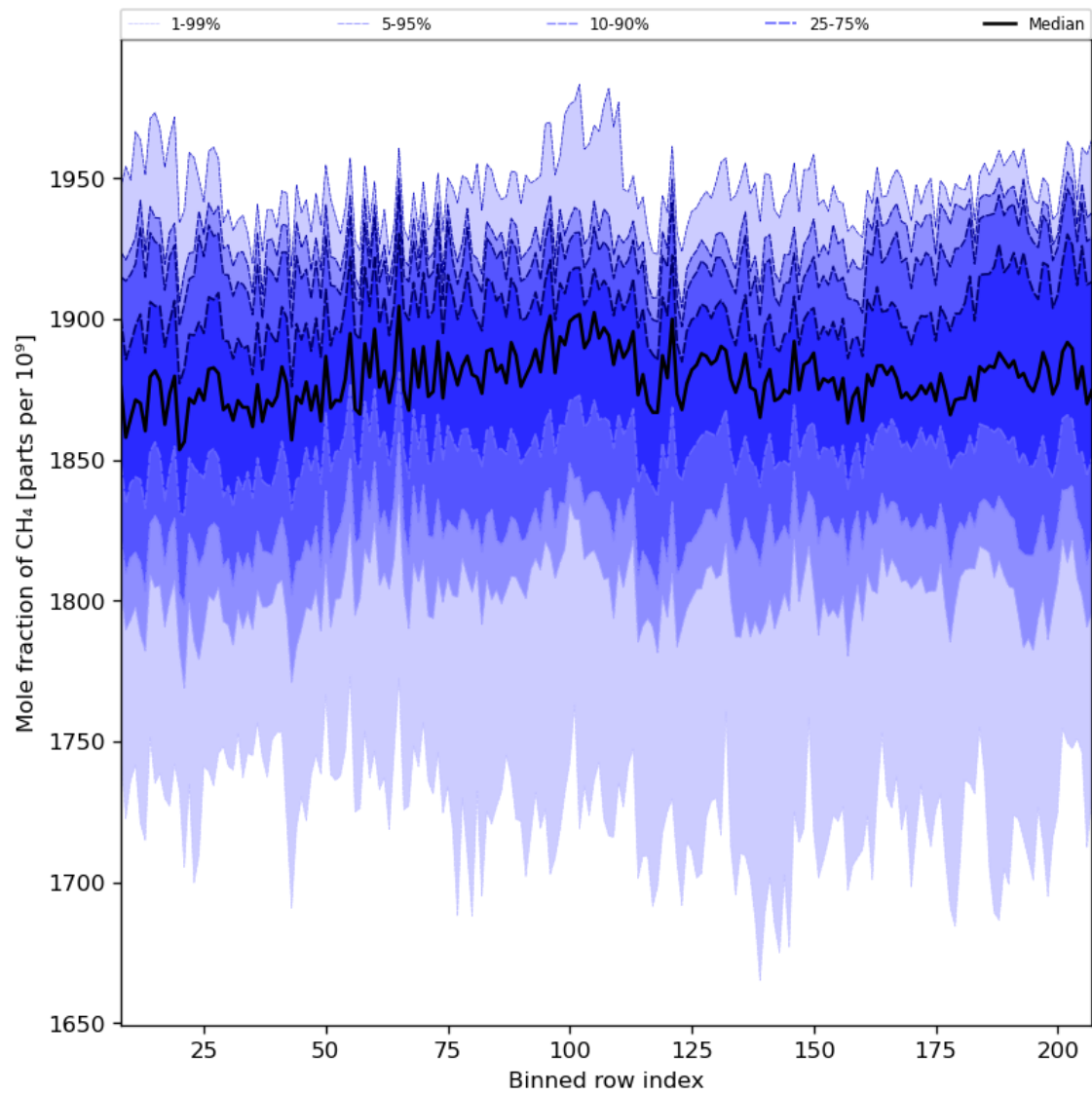
Figure 34: Along track statistics of “Mole fraction of CH 4 ” for 2024-06-27 to 2024-06-29
