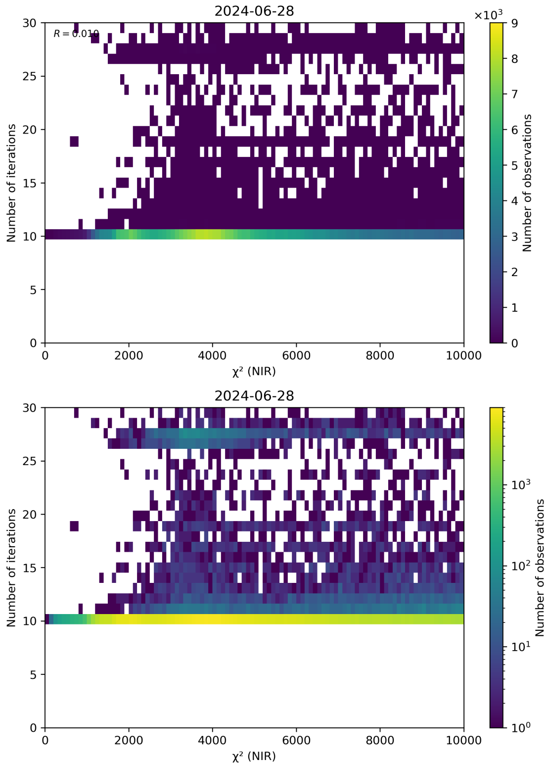
Figure 46: Scatter density plot of “ \chi^2 (NIR)” against “Number of iterations” for 2024-06-27 to 2024-06-29.
