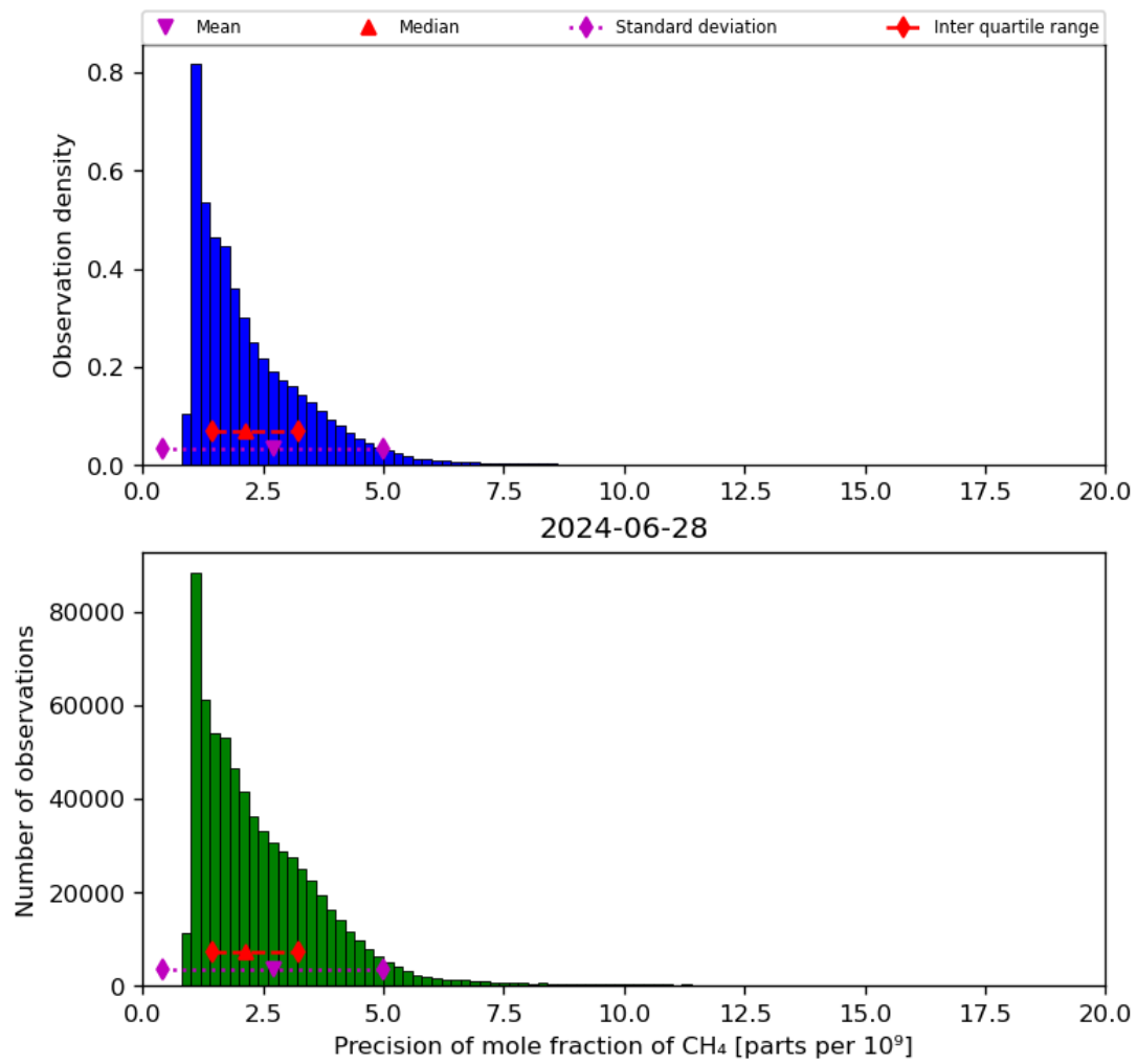
Figure 24: Histogram of “Precision of mole fraction of CH 4 ” for 2024-06-27 to 2024-06-29
