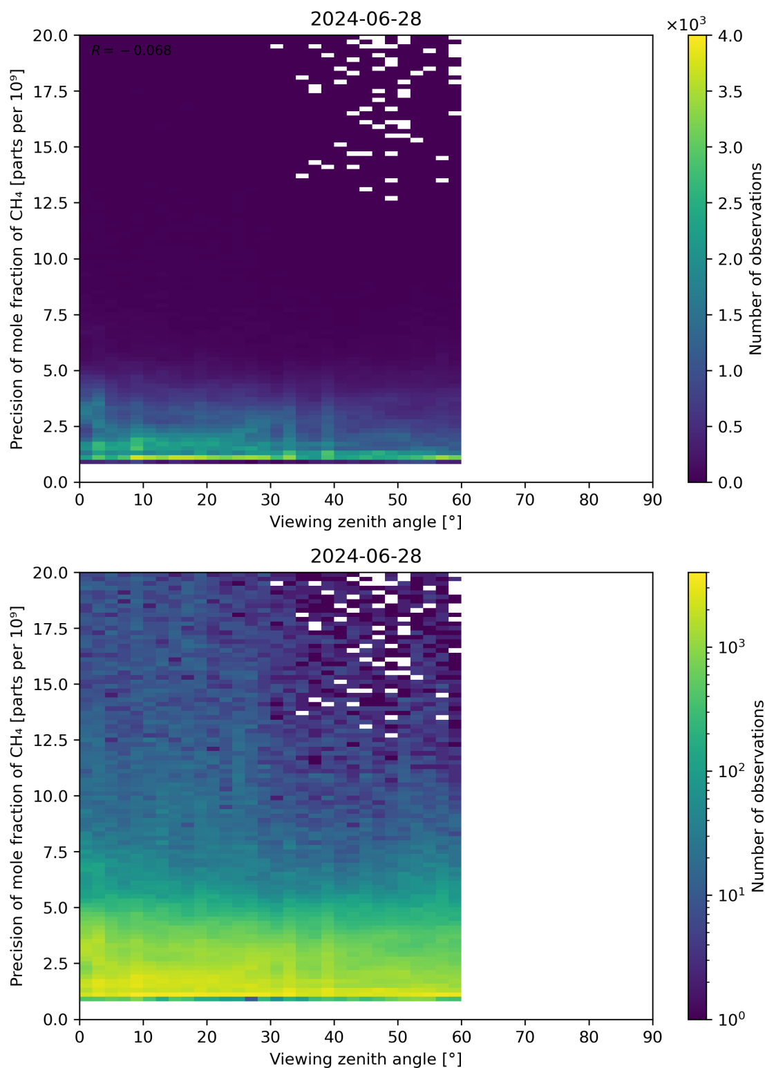
Figure 112: Scatter density plot of “Viewing zenith angle” against “Precision of mole fraction of CH 4 ” for 2024-06-27 to 2024-06-29.
