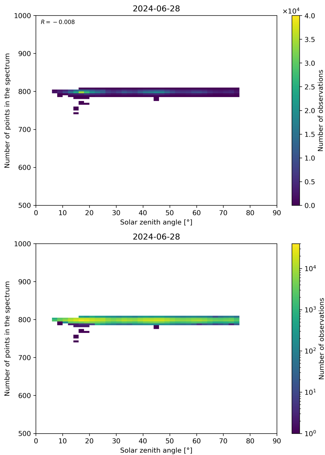
Figure 103: Scatter density plot of “Solar zenith angle” against “Number of points in the spectrum” for 2024-06-27 to 2024-06-29.
