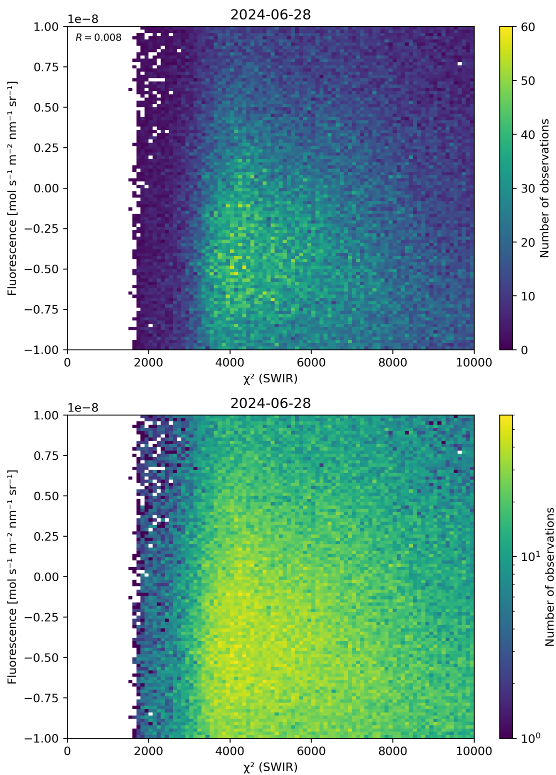
Figure 49: Scatter density plot of “ \chi^2 (SWIR)” against “Fluorescence” for 2024-06-27 to 2024-06-29.
