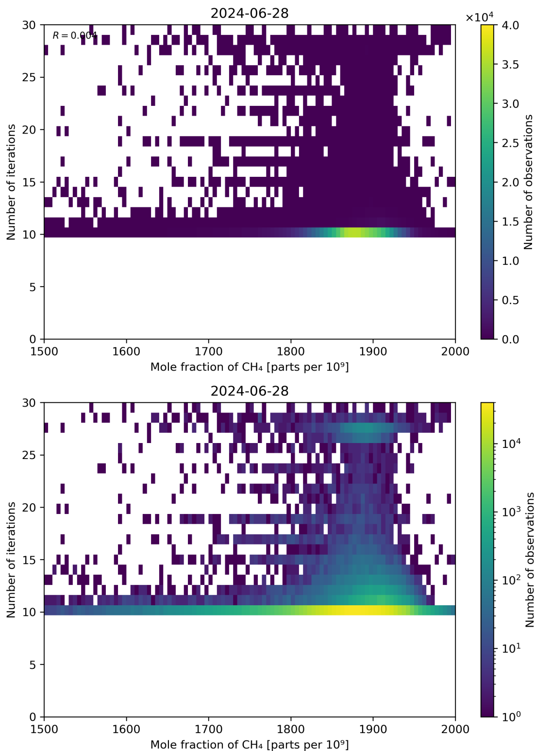
Figure 76: Scatter density plot of “Mole fraction of CH 4 ” against “Number of iterations” for 2024-06-27 to 2024-06-29.
