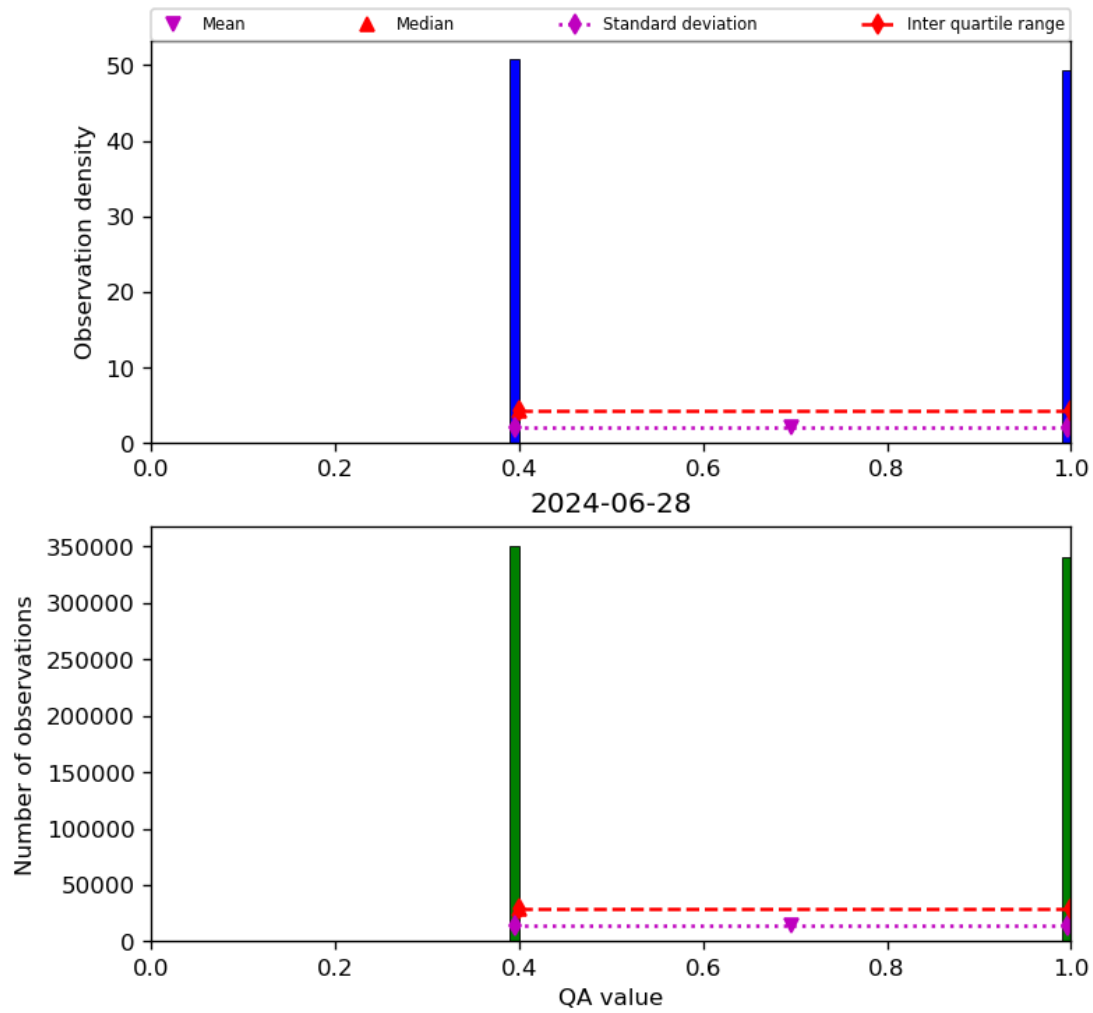
Figure 22: Histogram of “QA value” for 2024-06-27 to 2024-06-29
