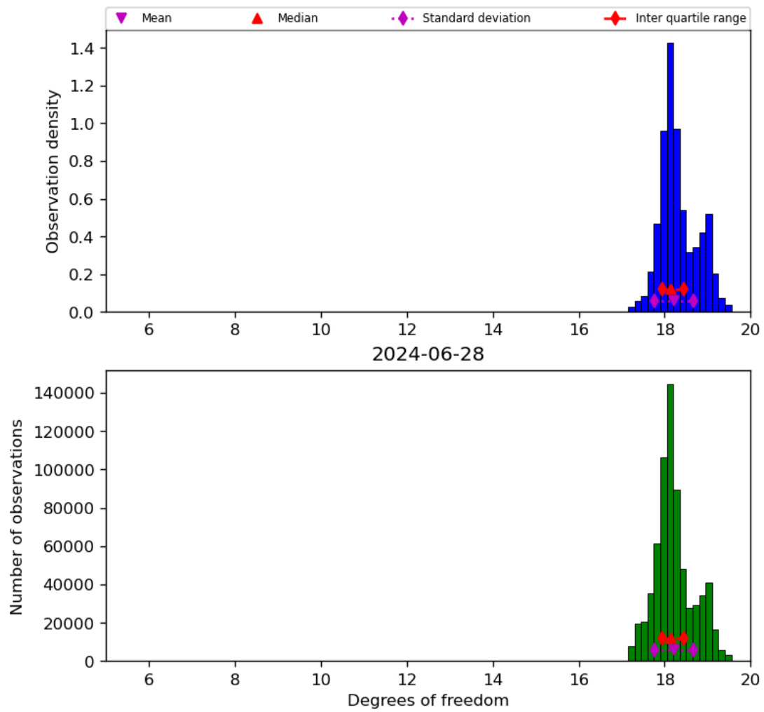
Figure 30: Histogram of “Degrees of freedom” for 2024-06-27 to 2024-06-29
