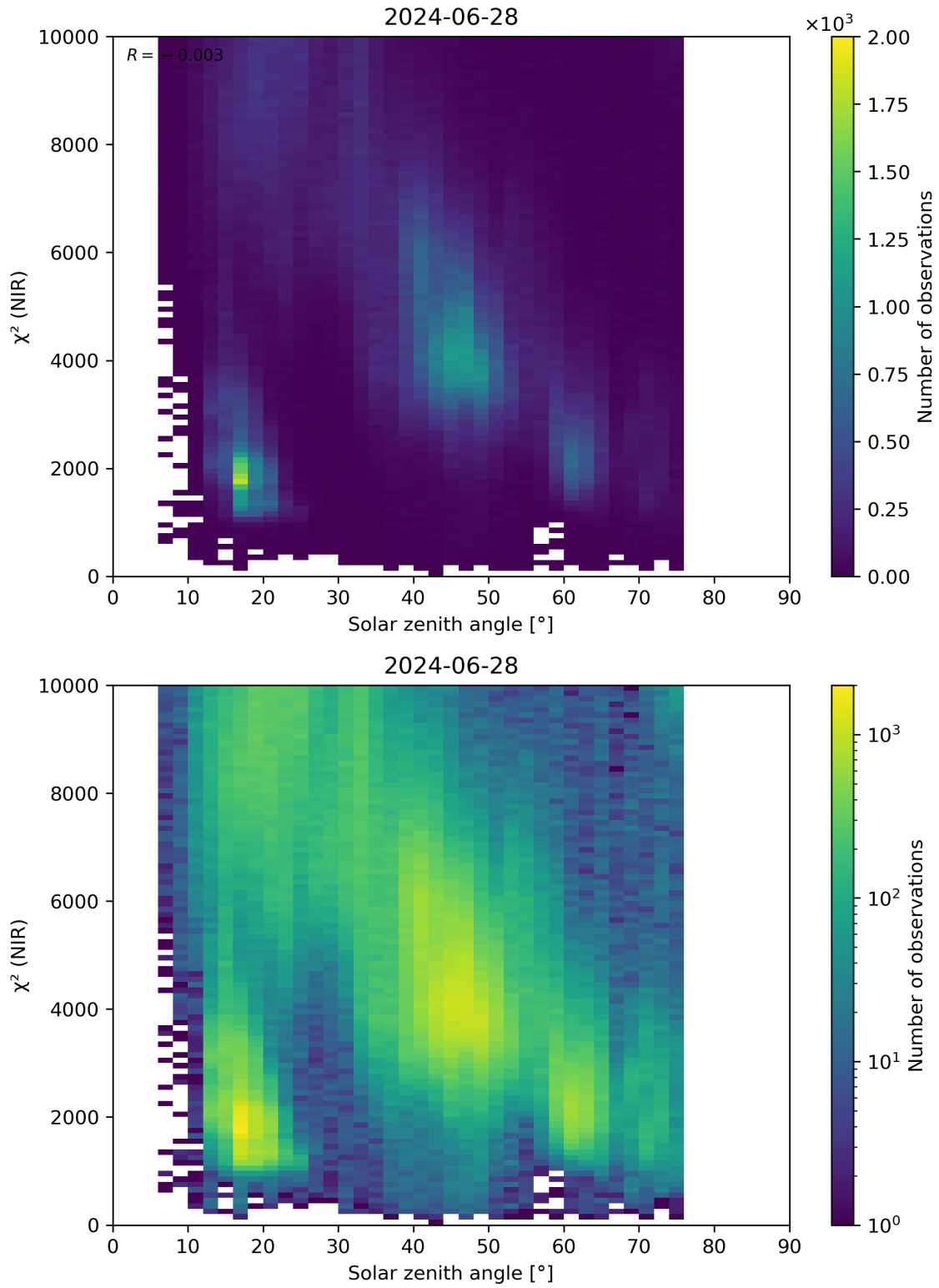
Figure 94: Scatter density plot of “Solar zenith angle” against “ \chi^2 (NIR)” for 2024-06-27 to 2024-06-29.
