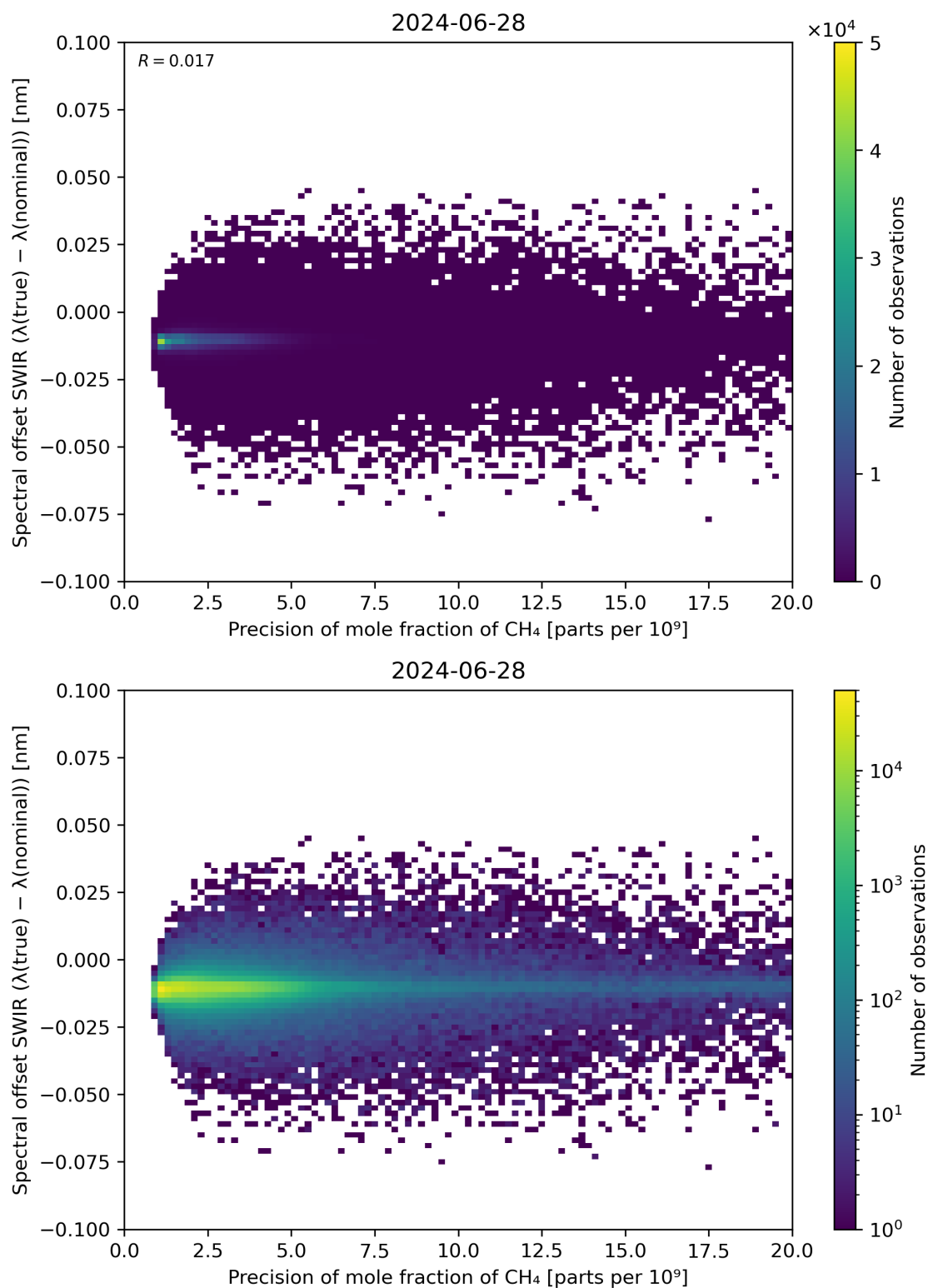
Figure 85: Scatter density plot of “Precision of mole fraction of \text{CH}_4 ” against “Spectral offset SWIR ( \lambda(\text{true}) - \lambda(\text{nominal}) )” for 2024-06-27 to 2024-06-29.
