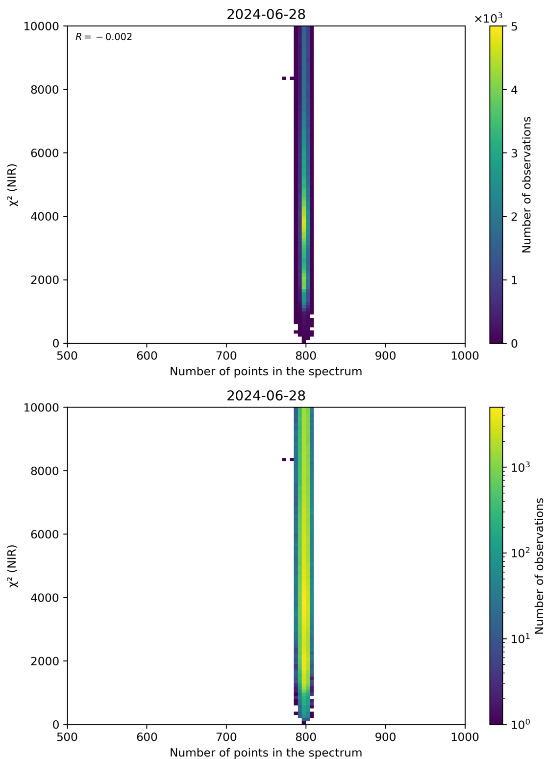
Figure 88: Scatter density plot of “Number of points in the spectrum” against “ \chi^2 (NIR)” for 2024-06-27 to 2024-06-29.
