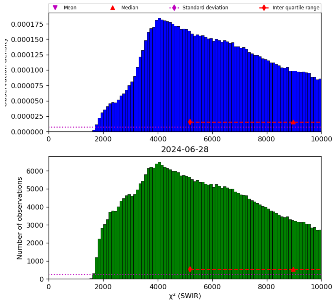
Figure 28: Histogram of “ \chi^2 (SWIR)” for 2024-06-27 to 2024-06-29
