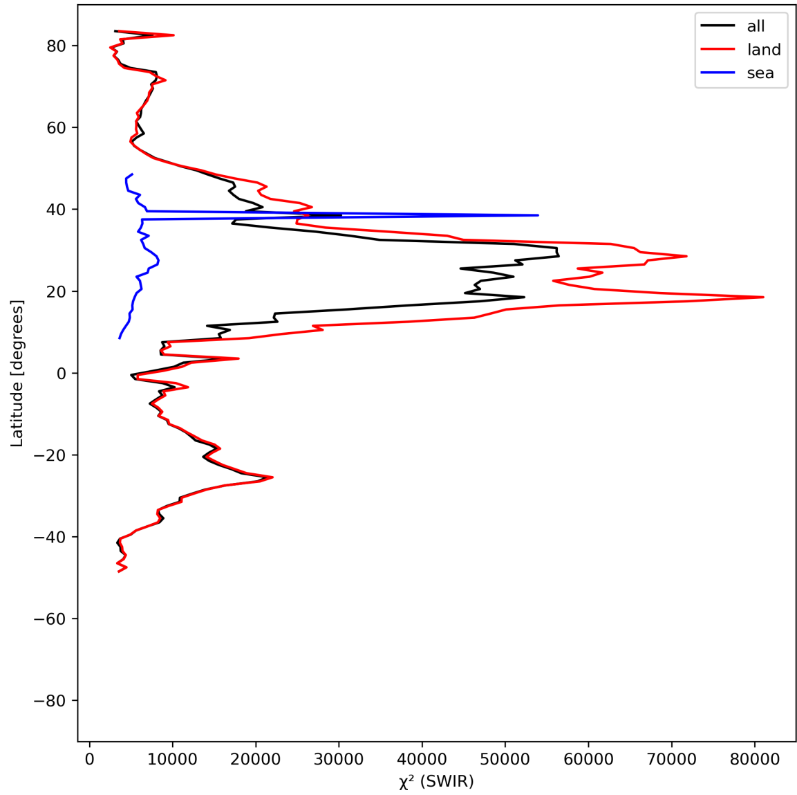
Figure 17: Zonal average of “ \chi^2 (SWIR)” for 2024-06-27 to 2024-06-29.
