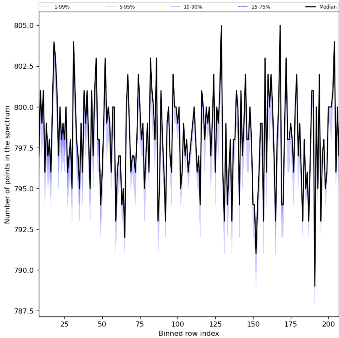
Figure 37: Along track statistics of “Number of points in the spectrum” for 2024-06-27 to 2024-06-29
