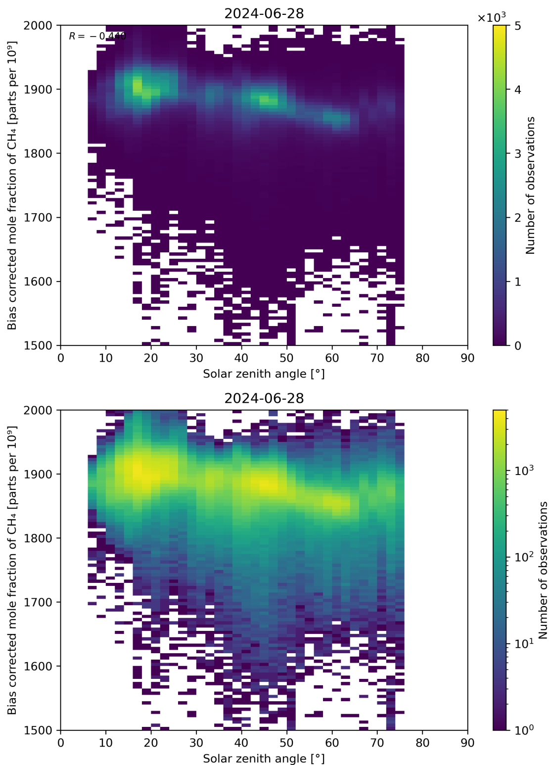
Figure 100: Scatter density plot of “Solar zenith angle” against “Bias corrected mole fraction of CH 4 ” for 2024-06-27 to 2024-06-29.
