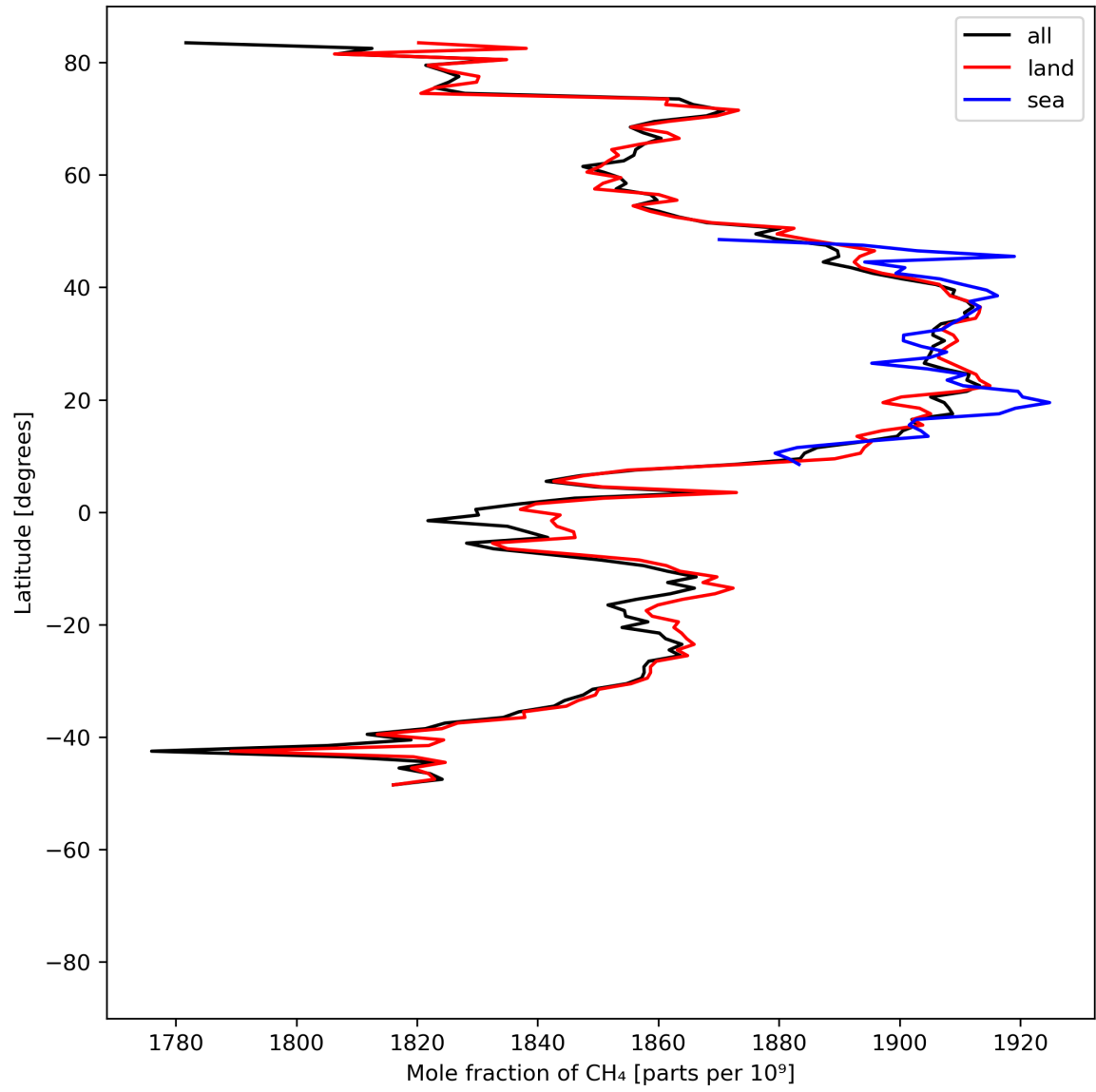
Figure 12: Zonal average of “Mole fraction of \text{CH}_4 ” for 2024-06-27 to 2024-06-29.
