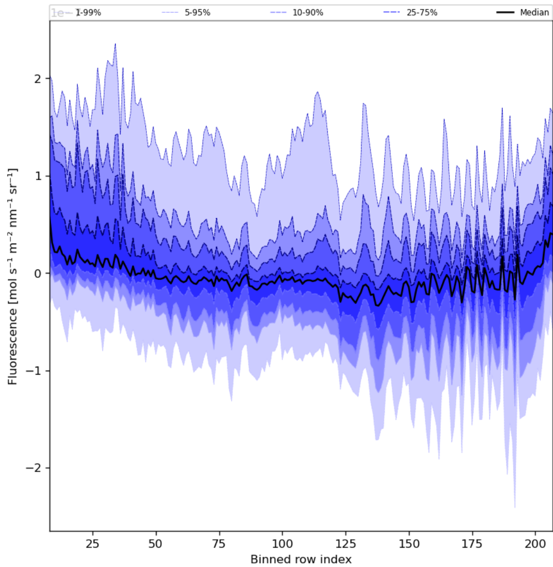
Figure 43: Along track statistics of “Fluorescence” for 2024-06-27 to 2024-06-29
