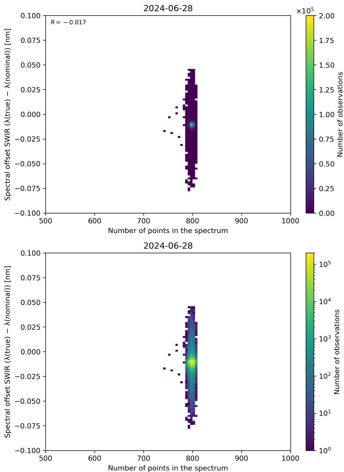
Figure 93: Scatter density plot of “Number of points in the spectrum” against “Spectral offset SWIR ( \lambda(\text{true}) - \lambda(\text{nominal}) )” for 2024-06-27 to 2024-06-29.
