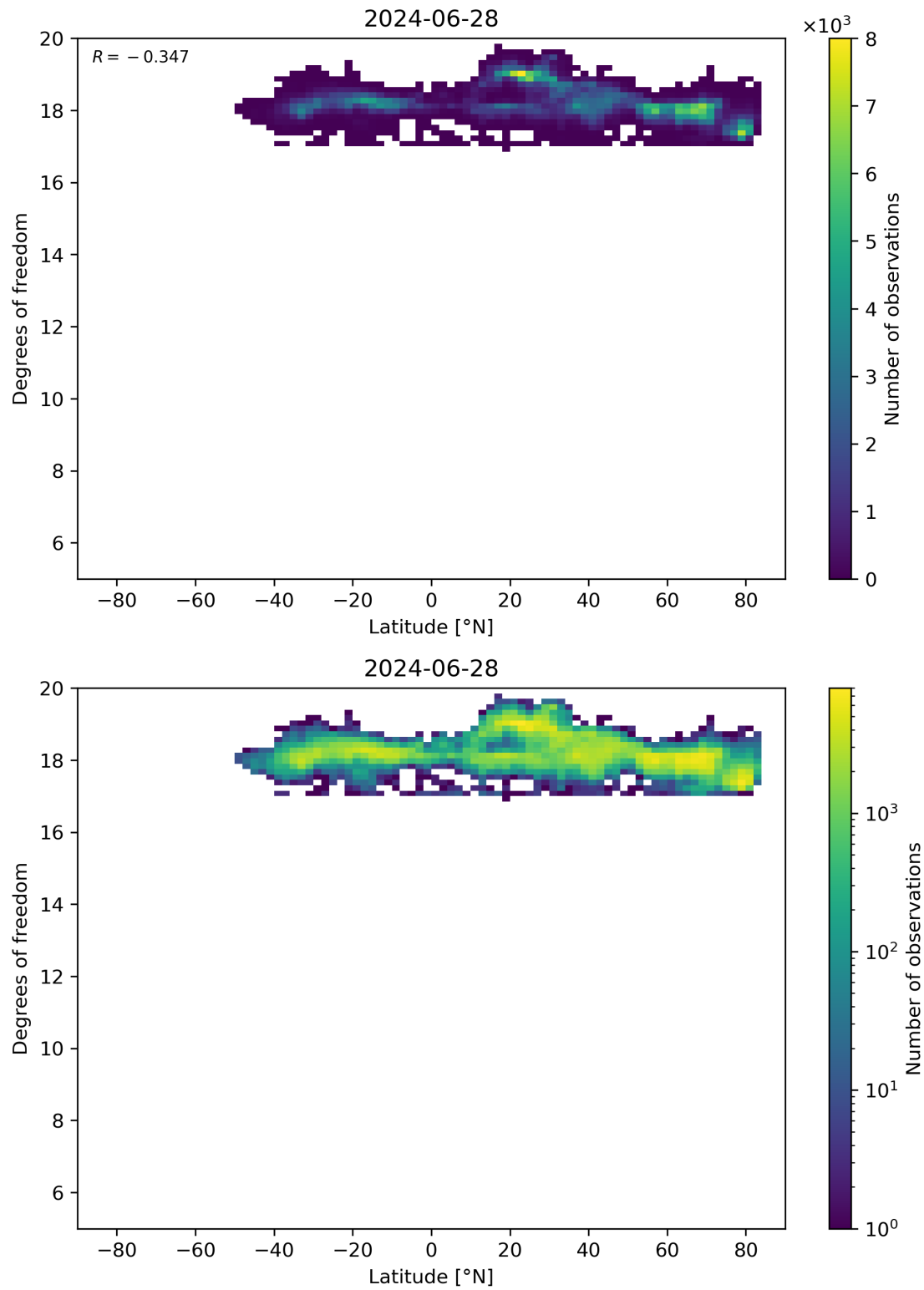
Figure 55: Scatter density plot of “Latitude” against “Degrees of freedom” for 2024-06-27 to 2024-06-29.
