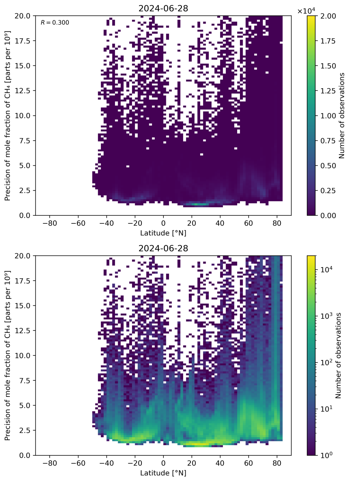
Figure 59: Scatter density plot of “Latitude” against “Precision of mole fraction of \text{CH}_4 ” for 2024-06-27 to 2024-06-29.
