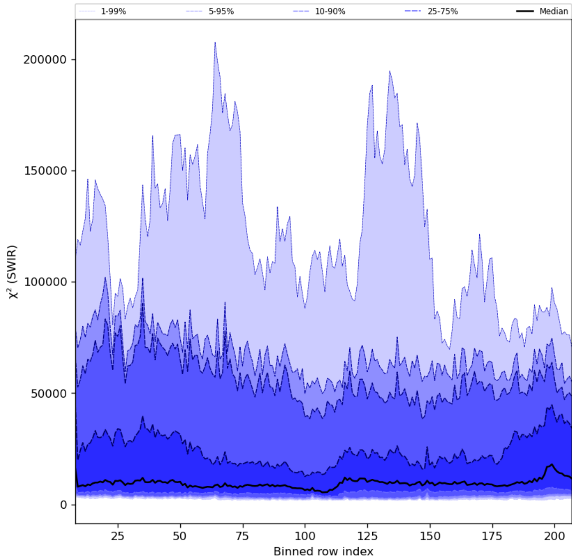
Figure 39: Along track statistics of “ \chi^2 (SWIR)” for 2024-06-27 to 2024-06-29
