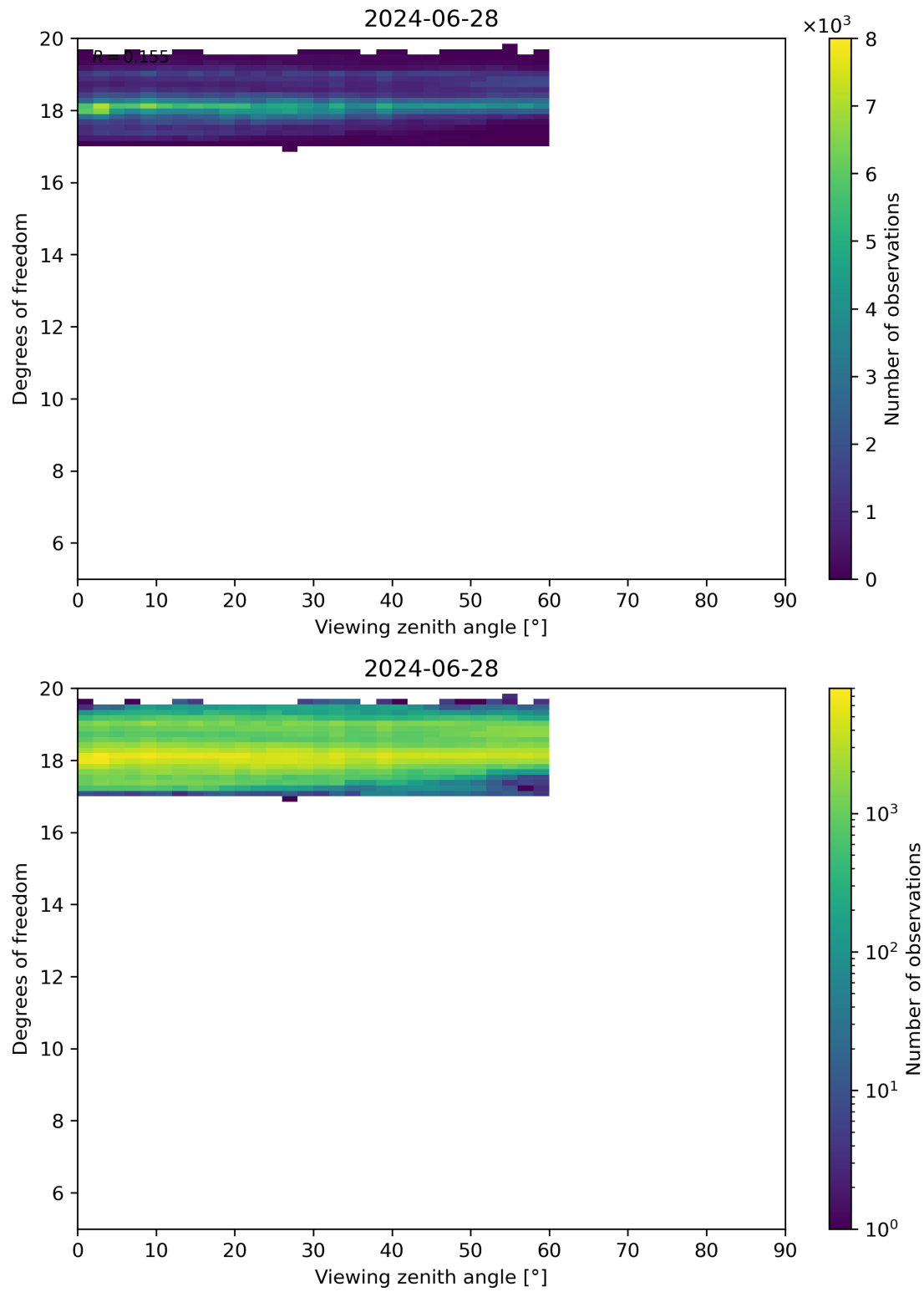
Figure 107: Scatter density plot of “Viewing zenith angle” against “Degrees of freedom” for 2024-06-27 to 2024-06-29.
