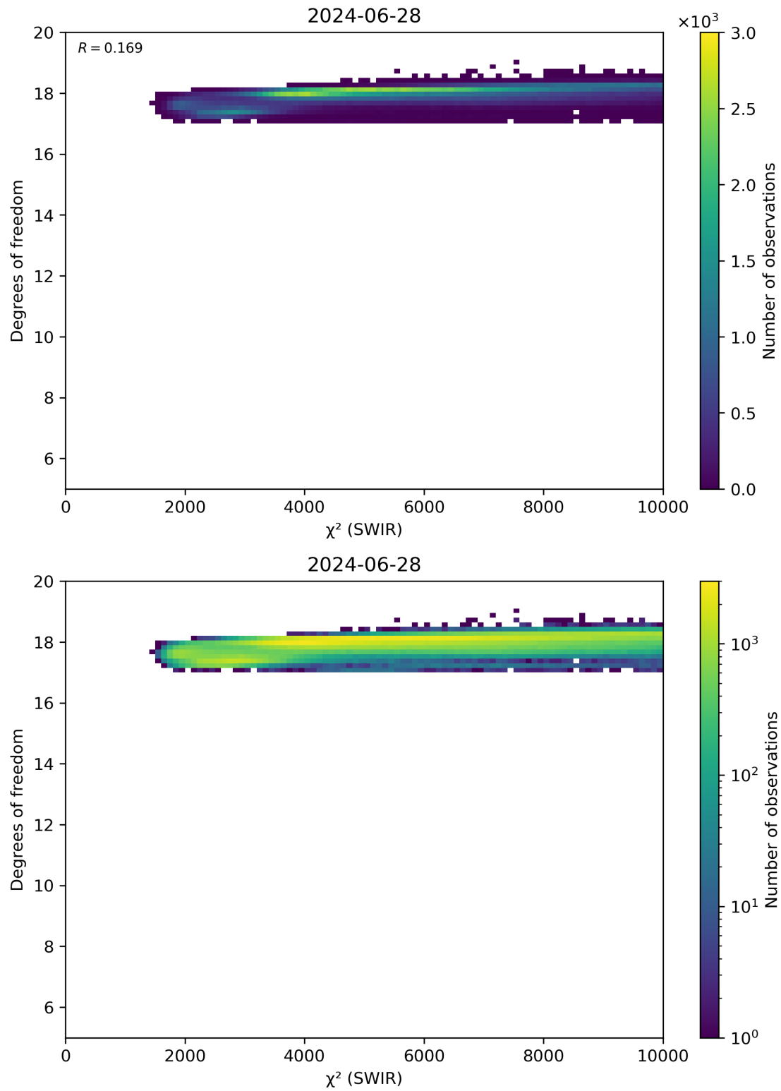
Figure 48: Scatter density plot of “ \chi^2 (SWIR)” against “Degrees of freedom” for 2024-06-27 to 2024-06-29.
