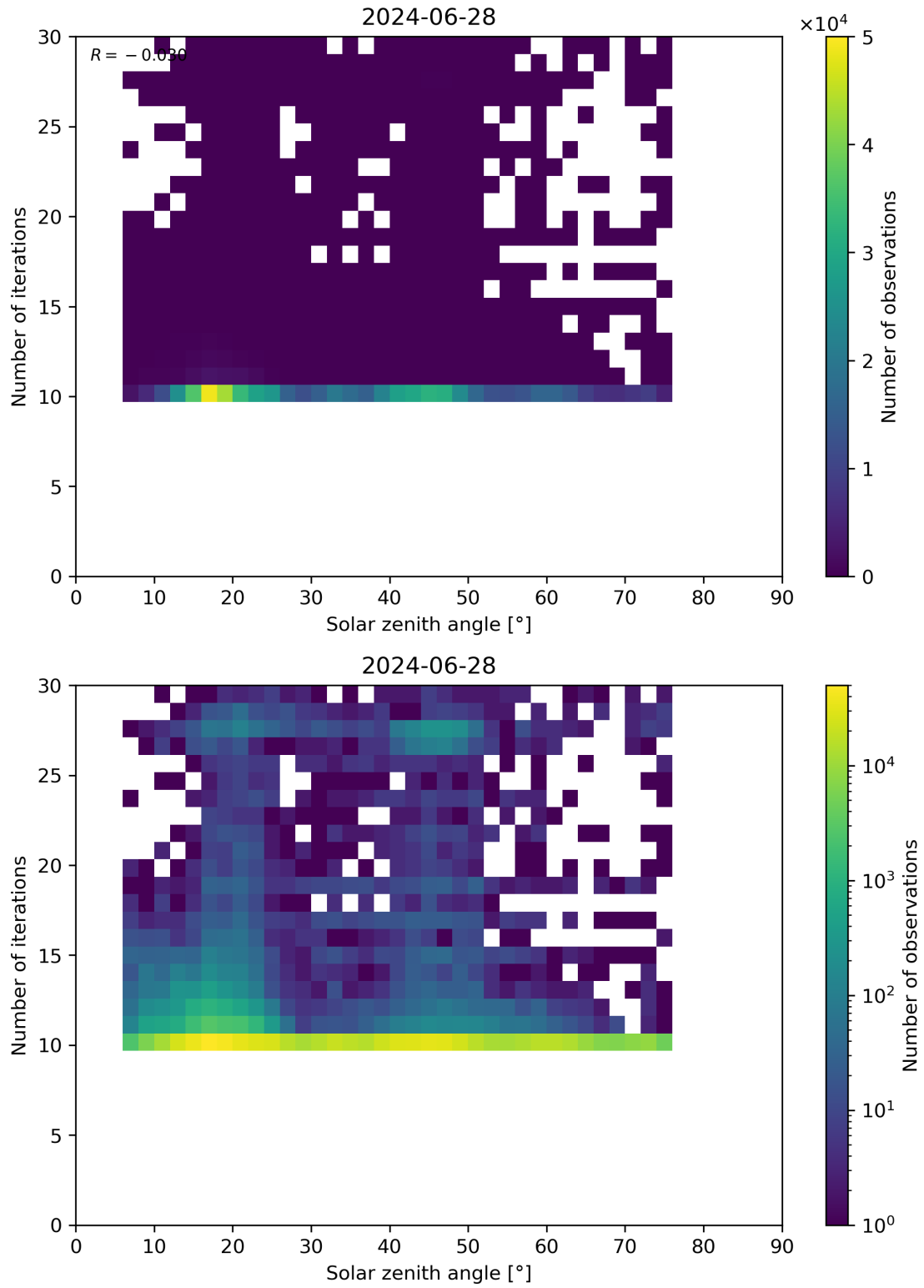
Figure 102: Scatter density plot of “Solar zenith angle” against “Number of iterations” for 2024-06-27 to 2024-06-29.
