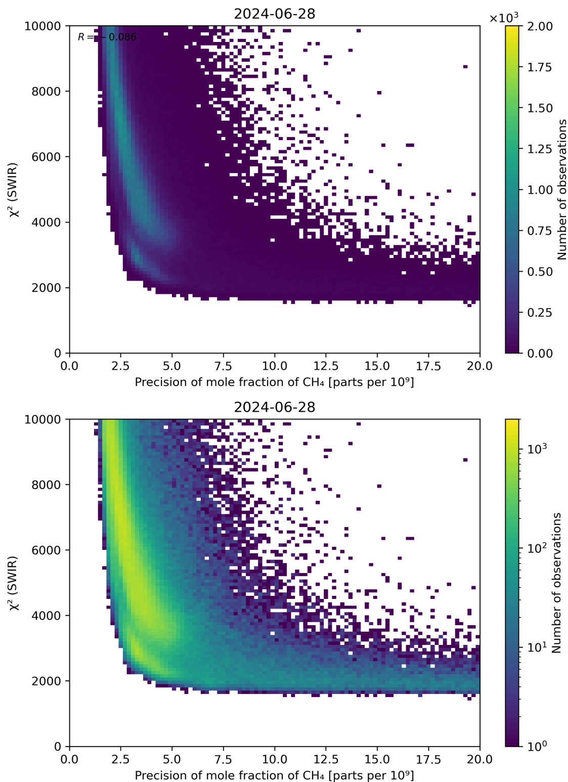
Figure 79: Scatter density plot of “Precision of mole fraction of \text{CH}_4 ” against “ \chi^2 (SWIR)” for 2024-06-27 to 2024-06-29.
