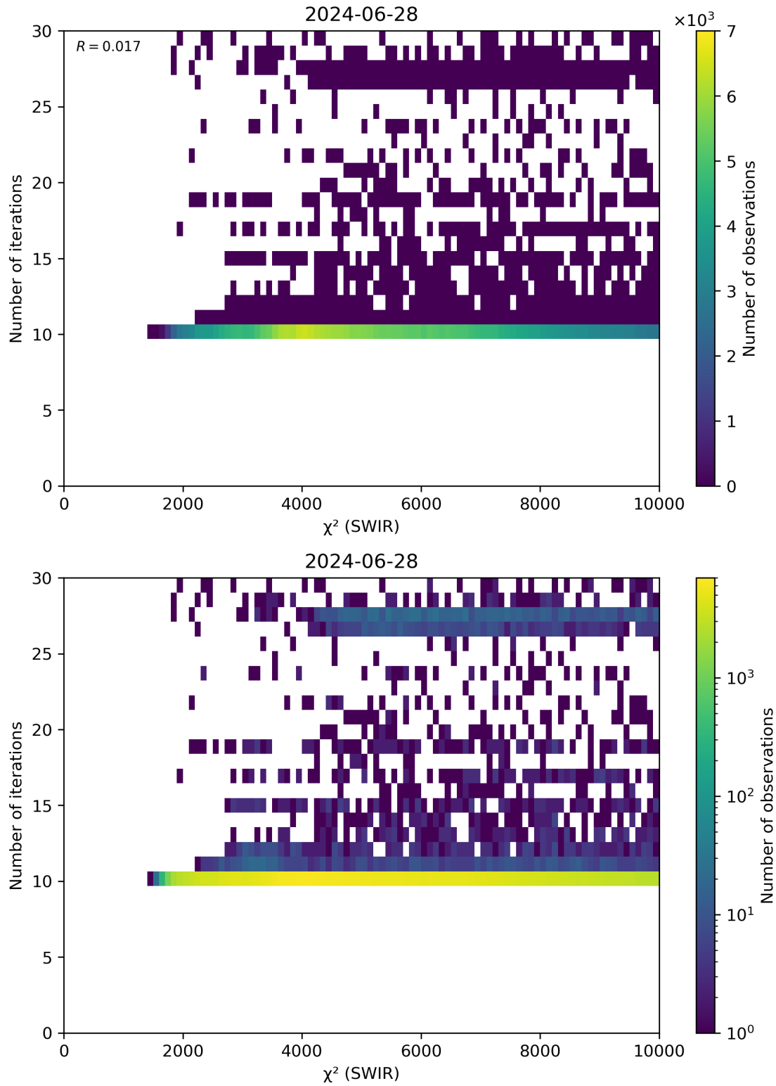
Figure 50: Scatter density plot of “ \chi^2 (SWIR)” against “Number of iterations” for 2024-06-27 to 2024-06-29.
