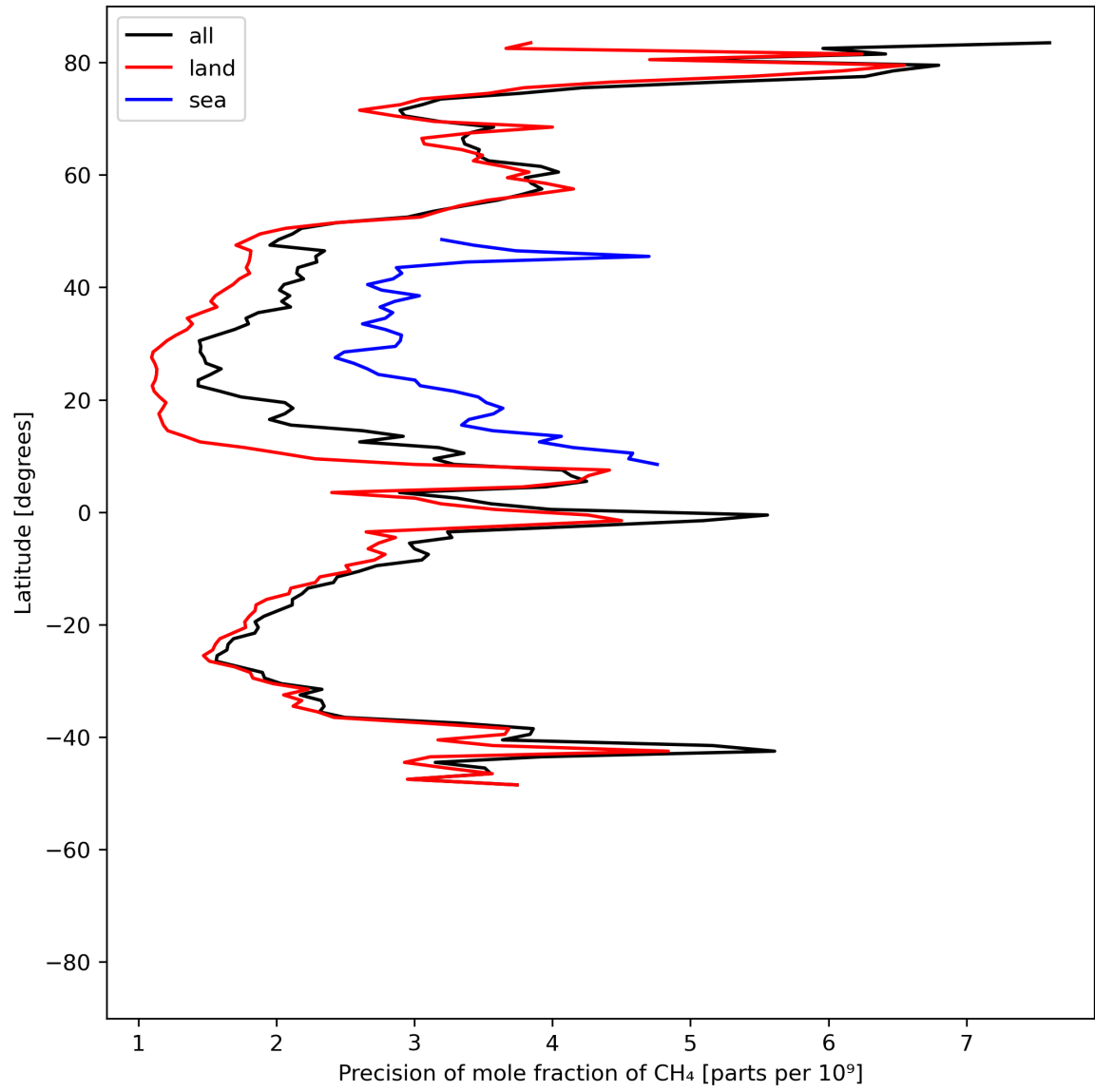
Figure 13: Zonal average of “Precision of mole fraction of CH 4 ” for 2024-06-27 to 2024-06-29.
