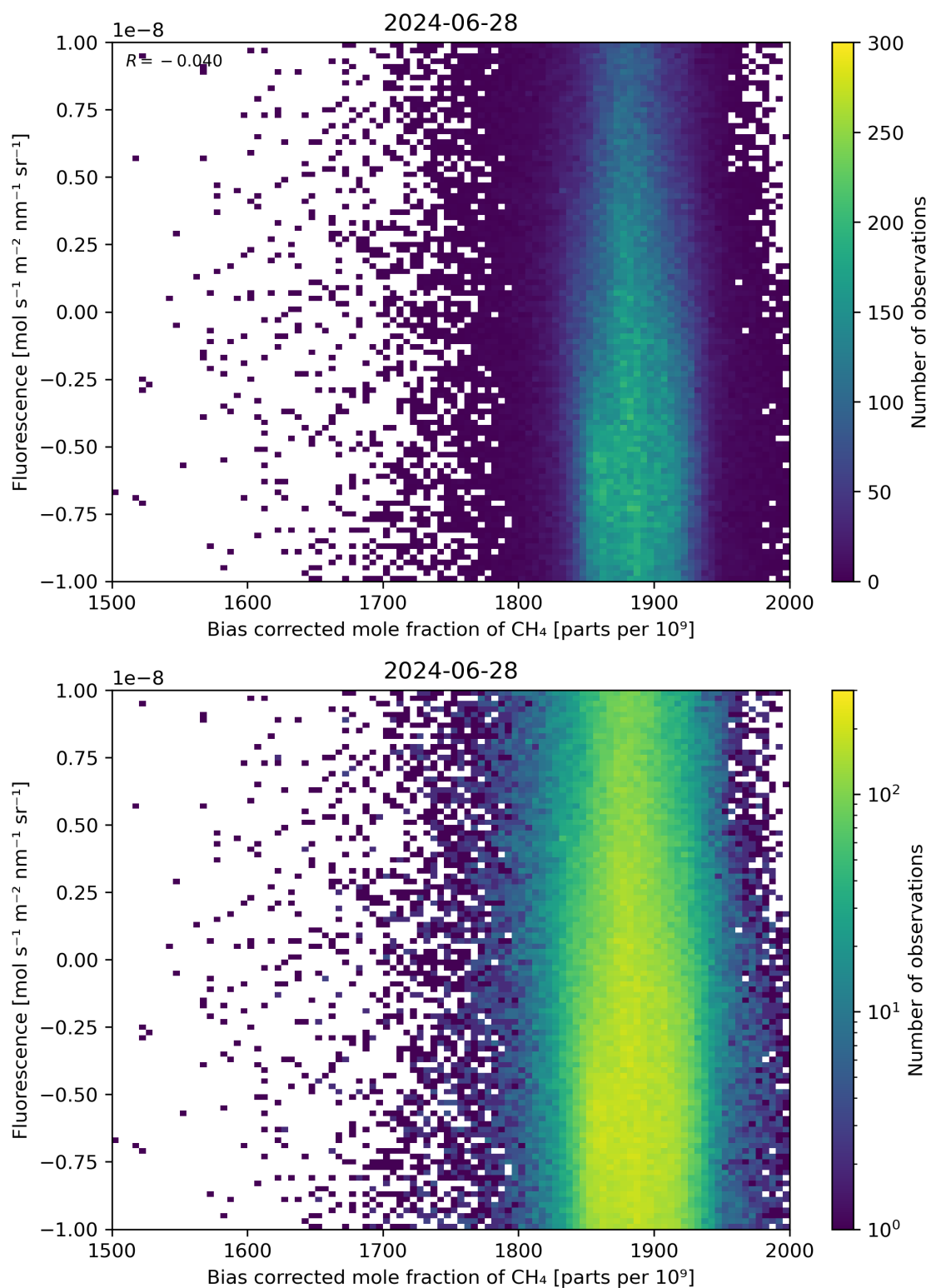
Figure 66: Scatter density plot of “Bias corrected mole fraction of \text{CH}_4 ” against “Fluorescence” for 2024-06-27 to 2024-06-29.
