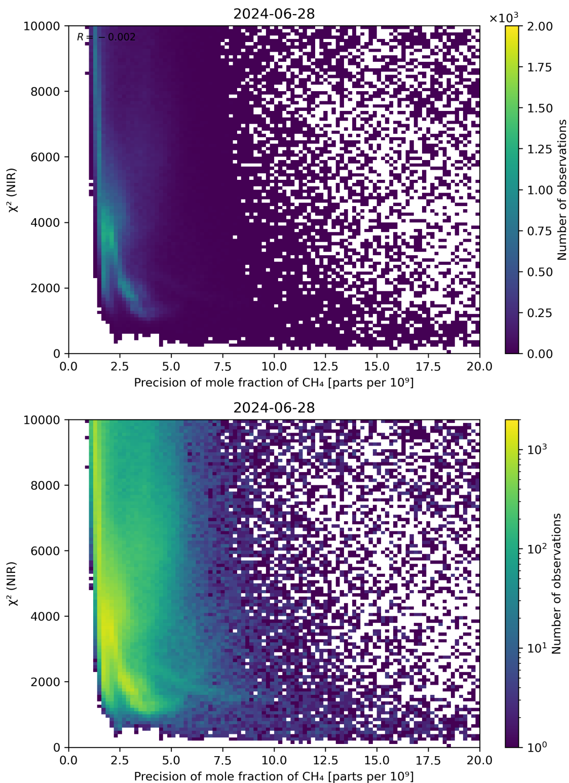
Figure 78: Scatter density plot of “Precision of mole fraction of CH 4 ” against “ \chi^2 (NIR)” for 2024-06-27 to 2024-06-29.
