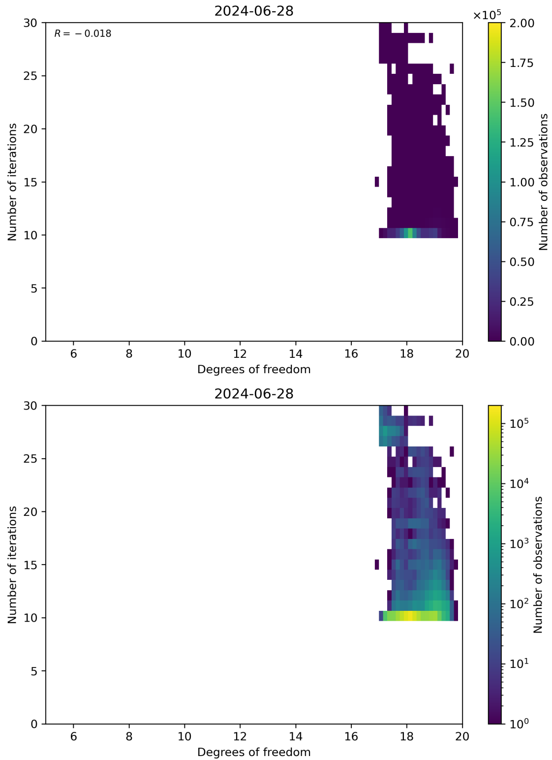
Figure 52: Scatter density plot of “Degrees of freedom” against “Number of iterations” for 2024-06-27 to 2024-06-29.
