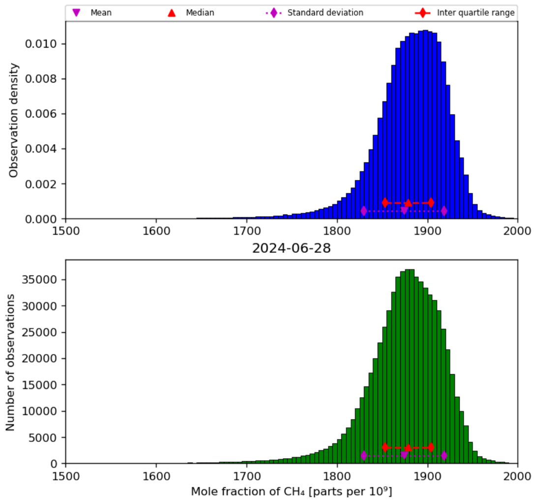
Figure 23: Histogram of “Mole fraction of CH 4 ” for 2024-06-27 to 2024-06-29
