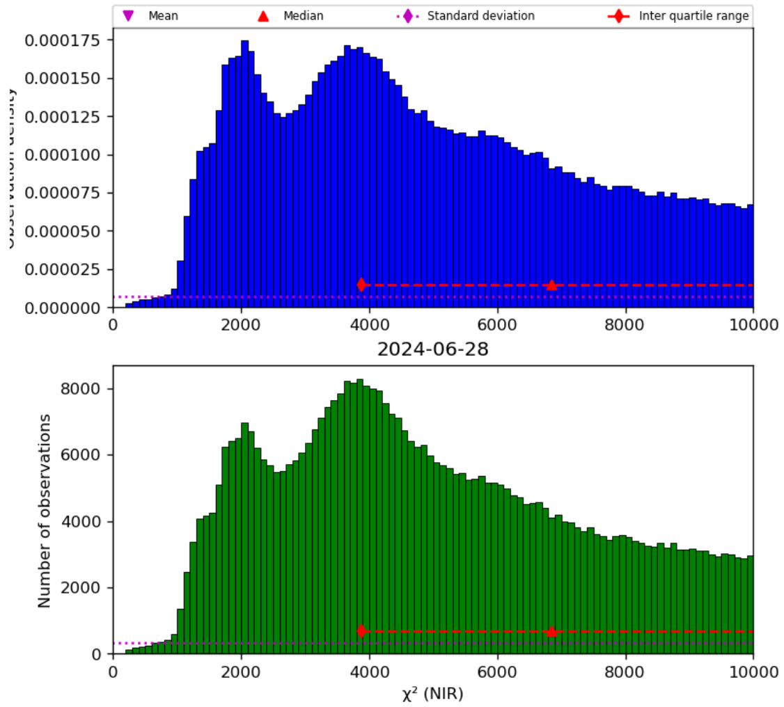
Figure 29: Histogram of “ \chi^2 (NIR)” for 2024-06-27 to 2024-06-29
