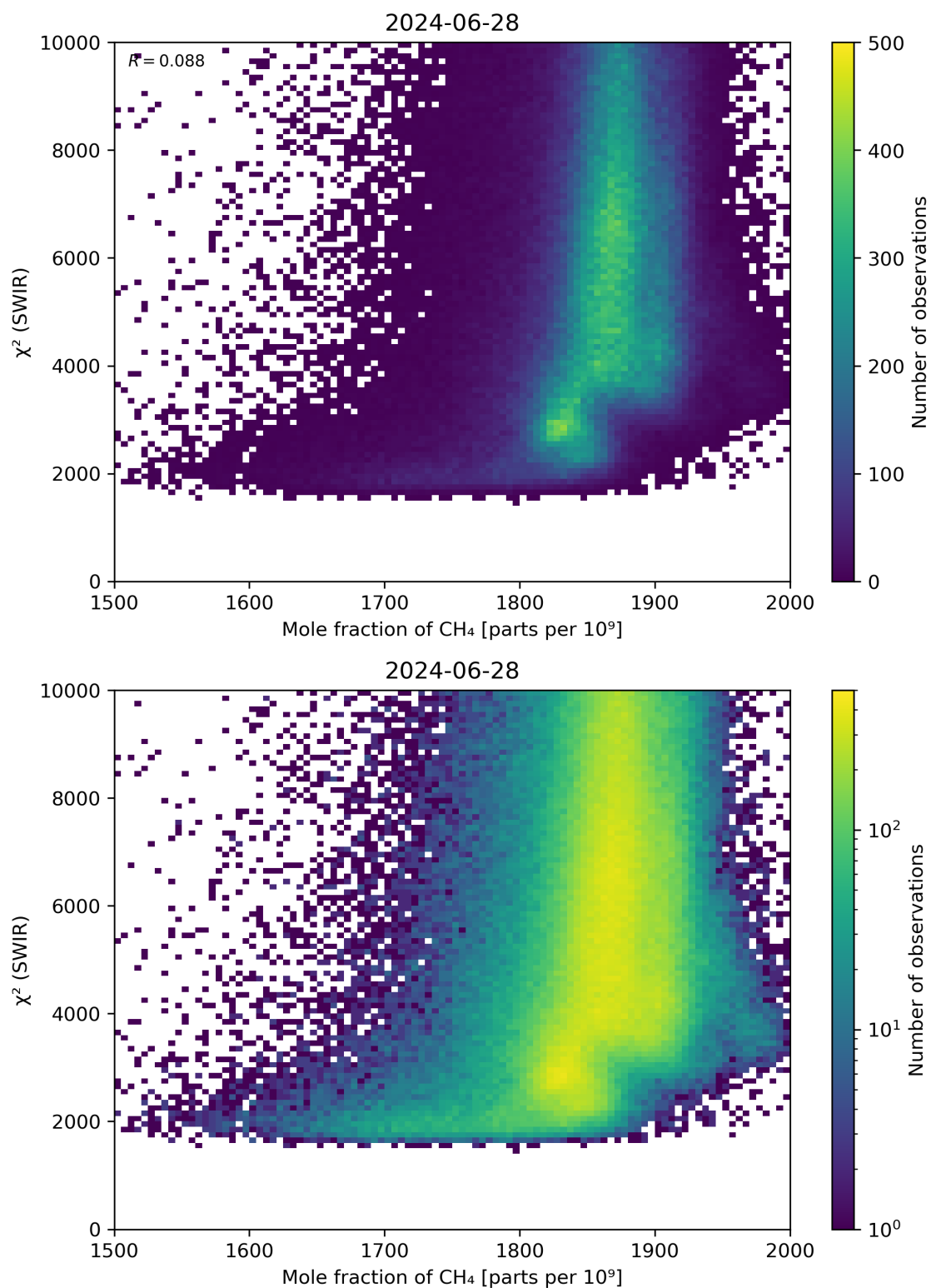
Figure 71: Scatter density plot of “Mole fraction of \text{CH}_4 ” against “ \chi^2 (SWIR)” for 2024-06-27 to 2024-06-29.
