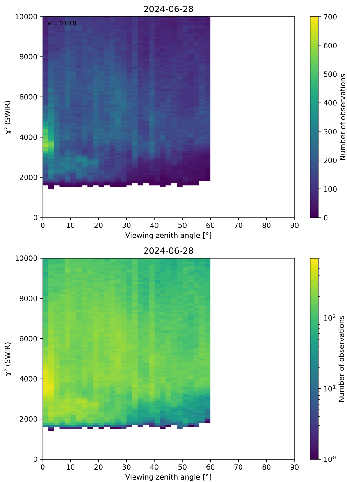
Figure 106: Scatter density plot of “Viewing zenith angle” against “ \chi^2 (SWIR)” for 2024-06-27 to 2024-06-29.
