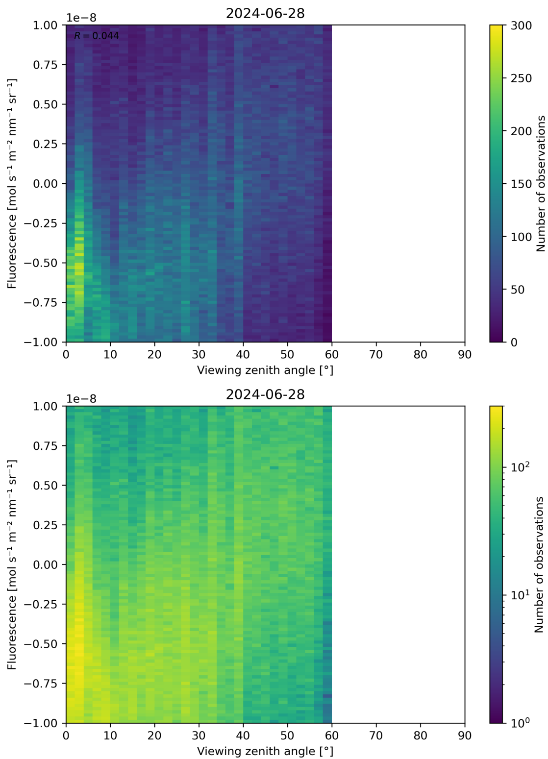
Figure 108: Scatter density plot of “Viewing zenith angle” against “Fluorescence” for 2024-06-27 to 2024-06-29.
