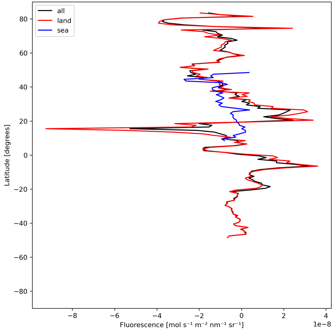
Figure 21: Zonal average of “Fluorescence” for 2024-06-27 to 2024-06-29.
