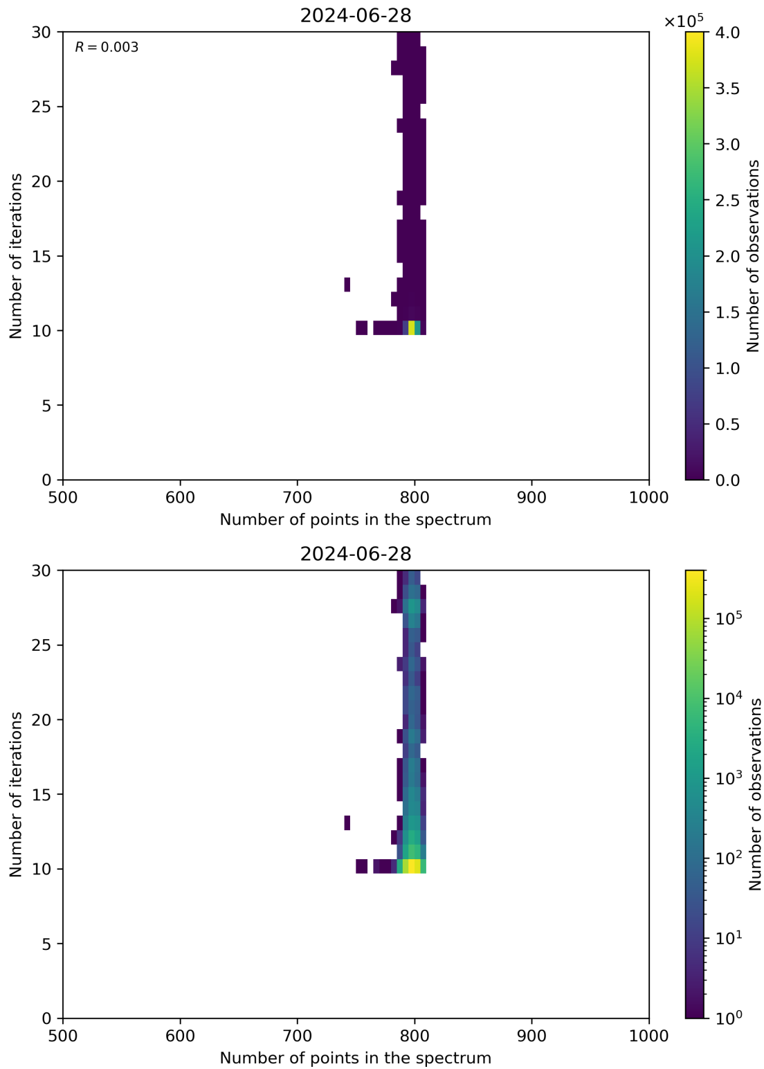
Figure 92: Scatter density plot of “Number of points in the spectrum” against “Number of iterations” for 2024-06-27 to 2024-06-29.
