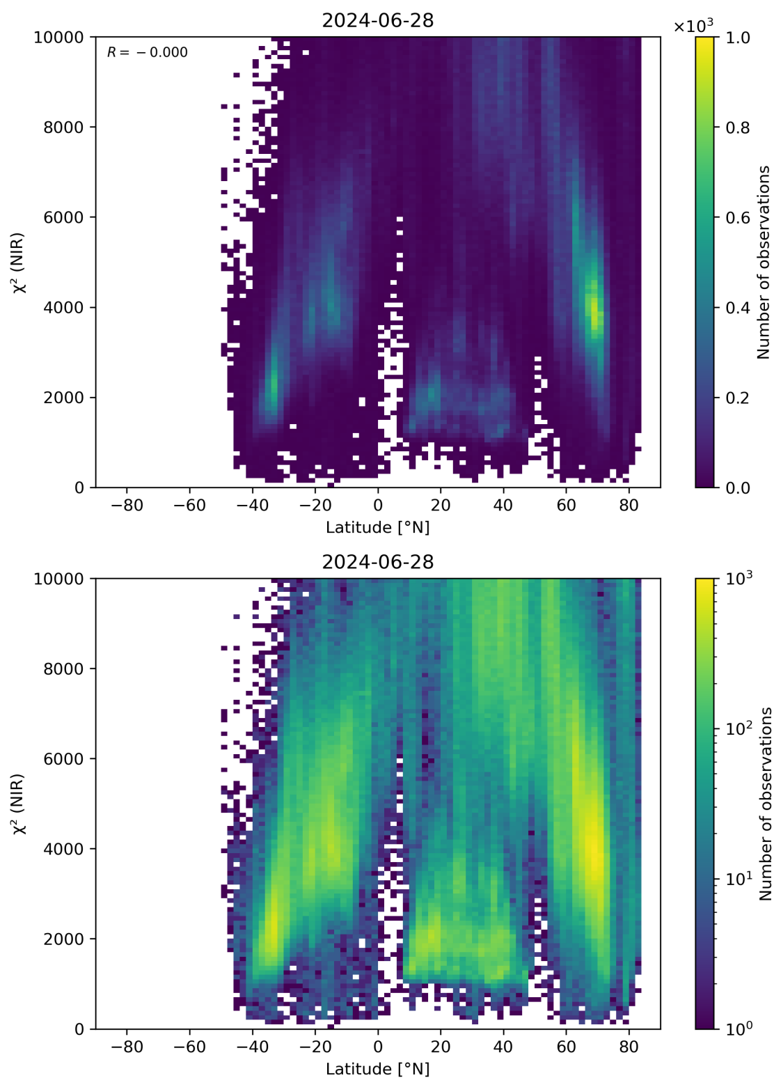
Figure 53: Scatter density plot of “Latitude” against “ \chi^2 (NIR)” for 2024-06-27 to 2024-06-29.
