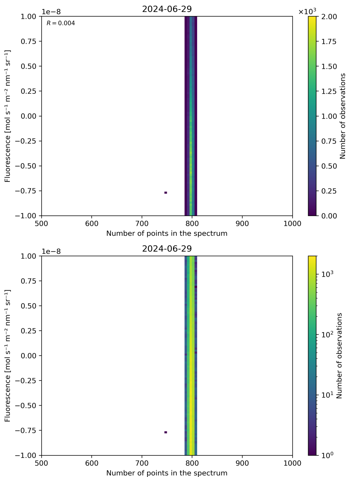
Figure 91: Scatter density plot of “Number of points in the spectrum” against “Fluorescence” for 2024-06-29 to 2024-06-30.
