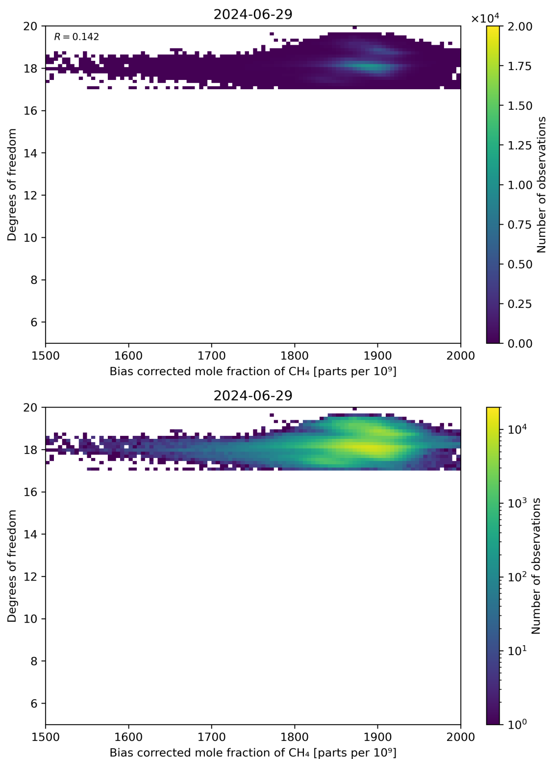
Figure 65: Scatter density plot of “Bias corrected mole fraction of CH 4 ” against “Degrees of freedom” for 2024-06-29 to 2024-06-30.
