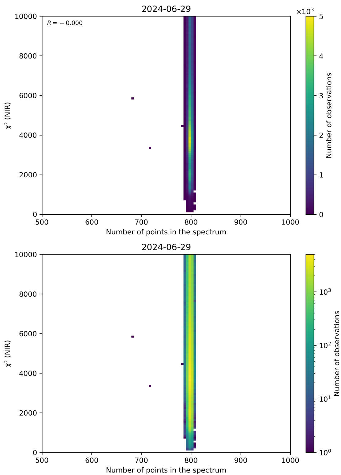
Figure 88: Scatter density plot of “Number of points in the spectrum” against “ \chi^2 (NIR)” for 2024-06-29 to 2024-06-30.
