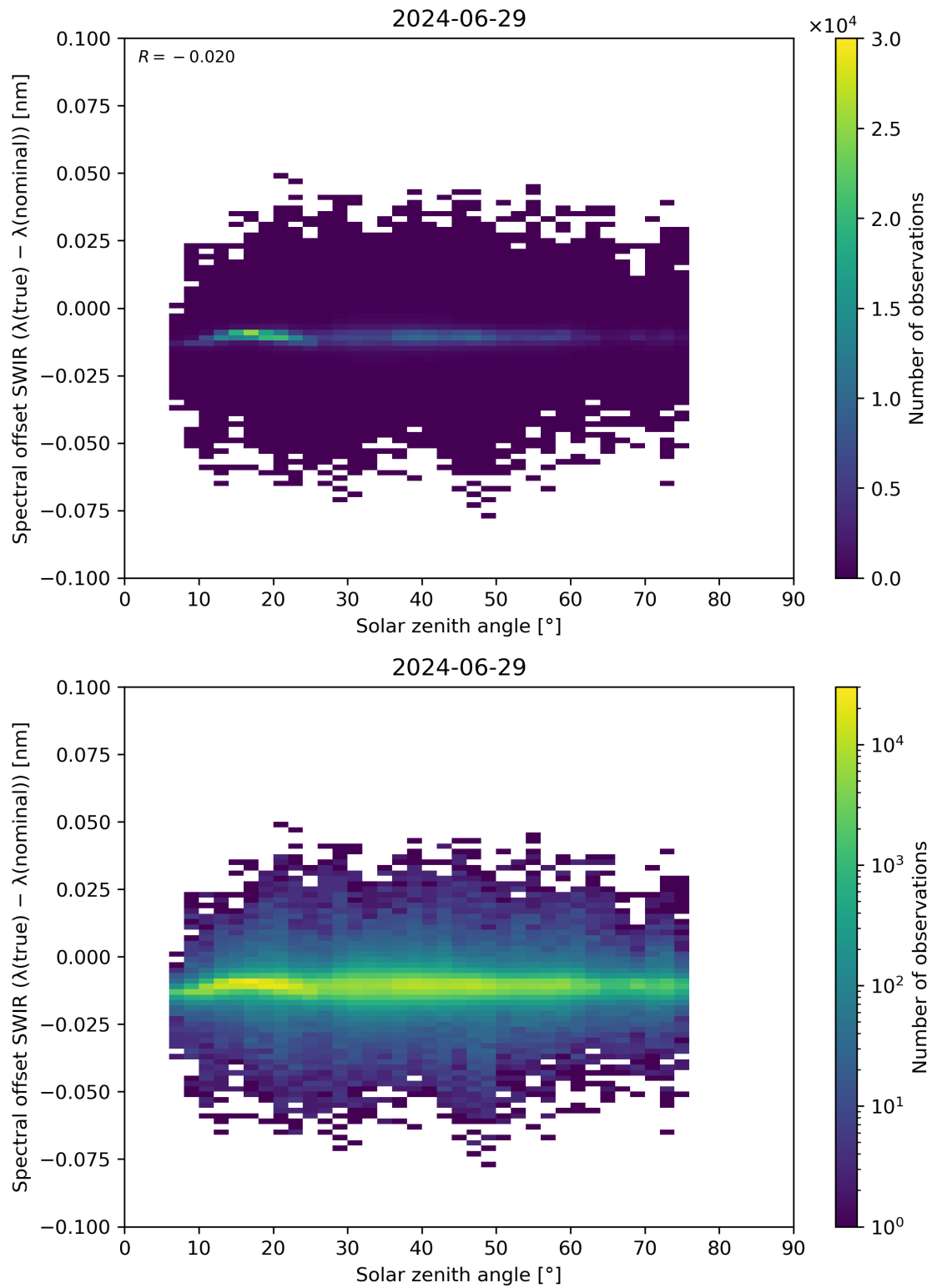
Figure 104: Scatter density plot of “Solar zenith angle” against “Spectral offset SWIR ( \lambda(\text{true}) - \lambda(\text{nominal}) )” for 2024-06-29 to 2024-06-30.
