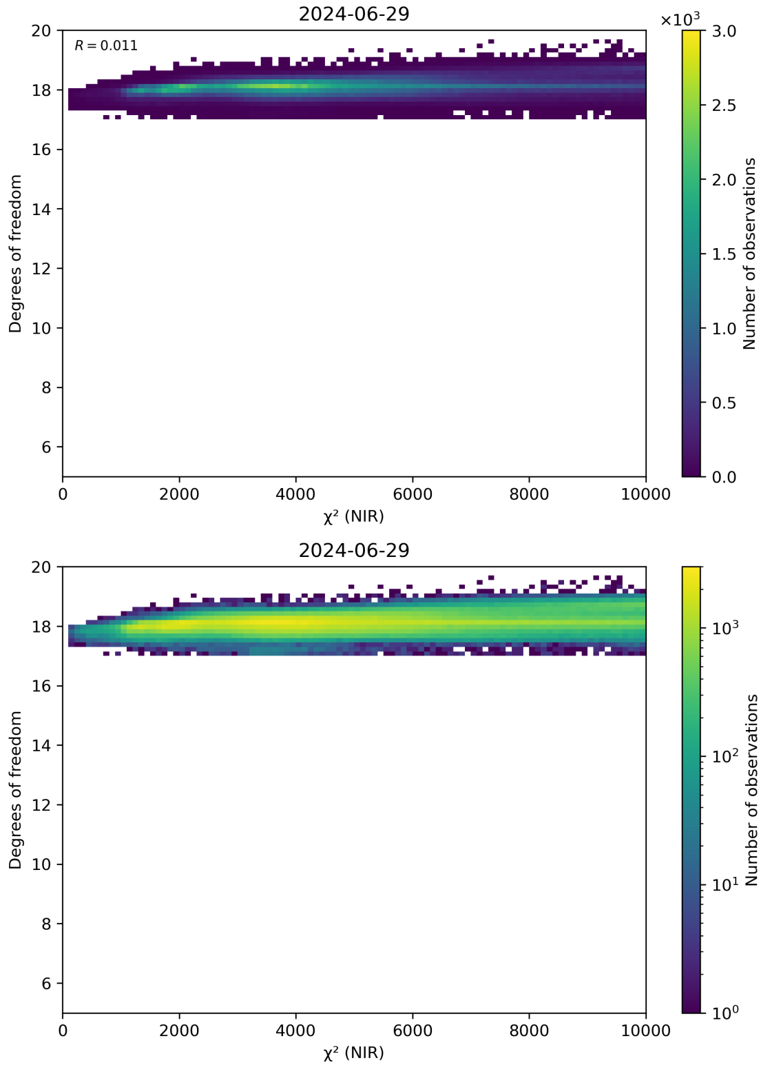
Figure 44: Scatter density plot of “ \chi^2 (NIR)” against “Degrees of freedom” for 2024-06-29 to 2024-06-30.
