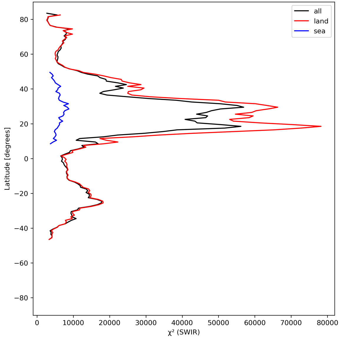
Figure 17: Zonal average of “ \chi^2 (SWIR)” for 2024-06-29 to 2024-06-30.
