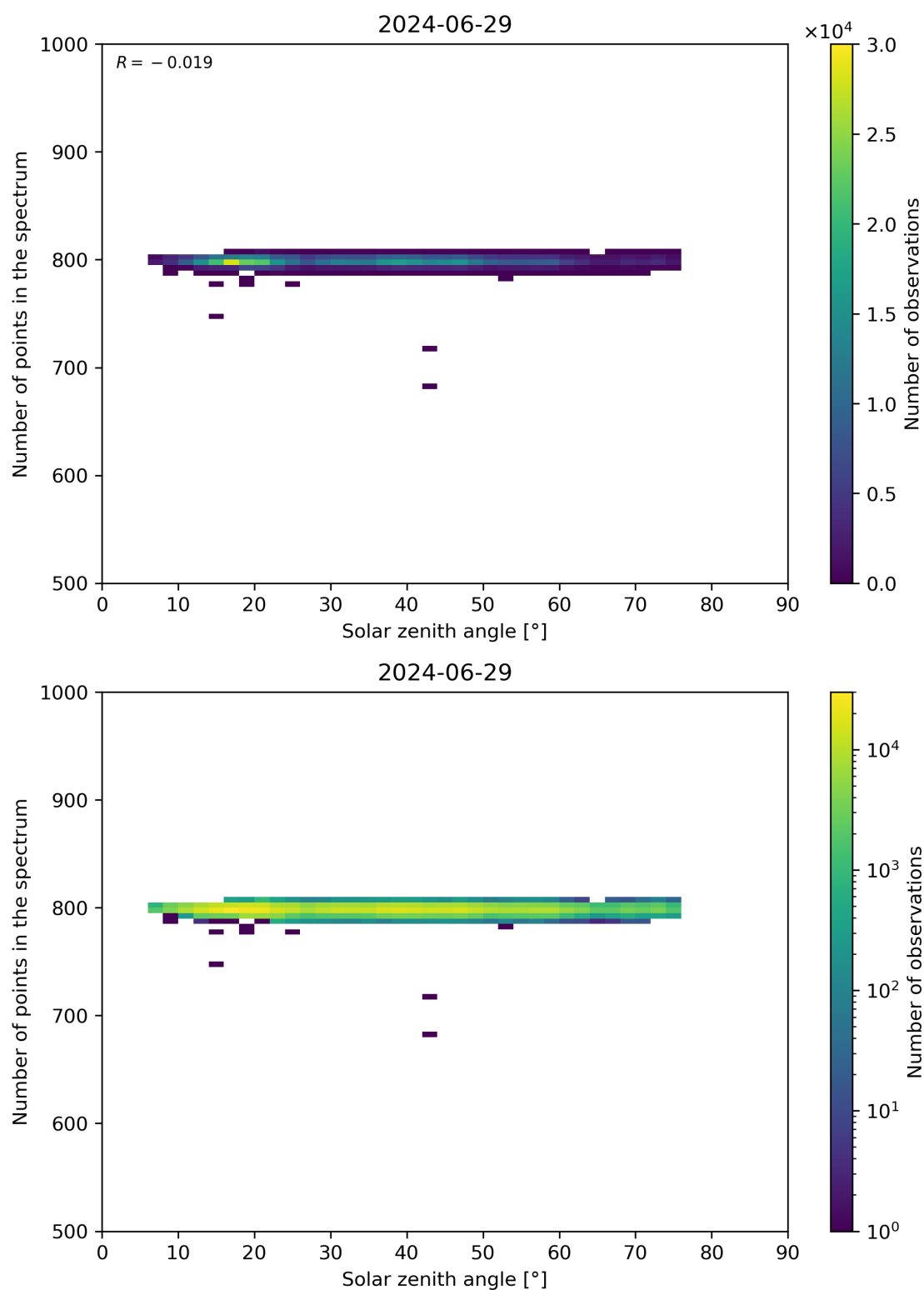
Figure 103: Scatter density plot of “Solar zenith angle” against “Number of points in the spectrum” for 2024-06-29 to 2024-06-30.
