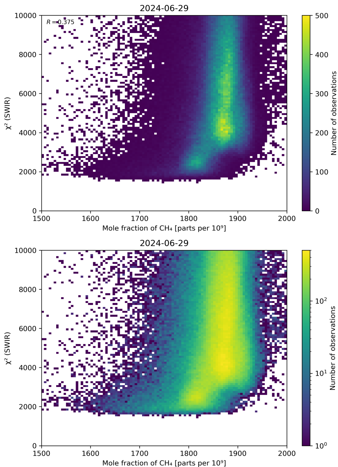
Figure 71: Scatter density plot of “Mole fraction of \text{CH}_4 ” against “ \chi^2 (SWIR)” for 2024-06-29 to 2024-06-30.
