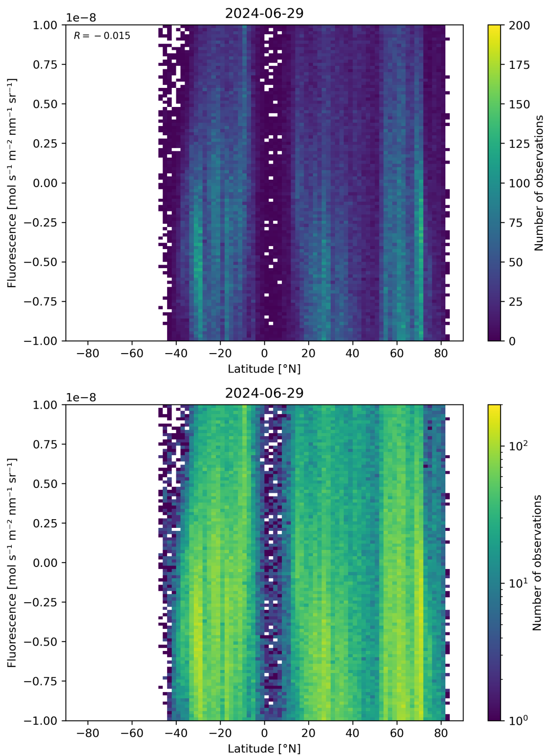
Figure 56: Scatter density plot of “Latitude” against “Fluorescence” for 2024-06-29 to 2024-06-30.
