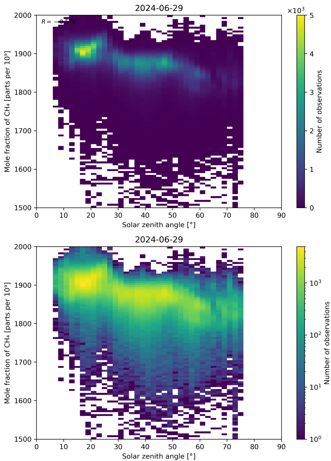
Figure 99: Scatter density plot of “Solar zenith angle” against “Mole fraction of CH 4 ” for 2024-06-29 to 2024-06-30.
