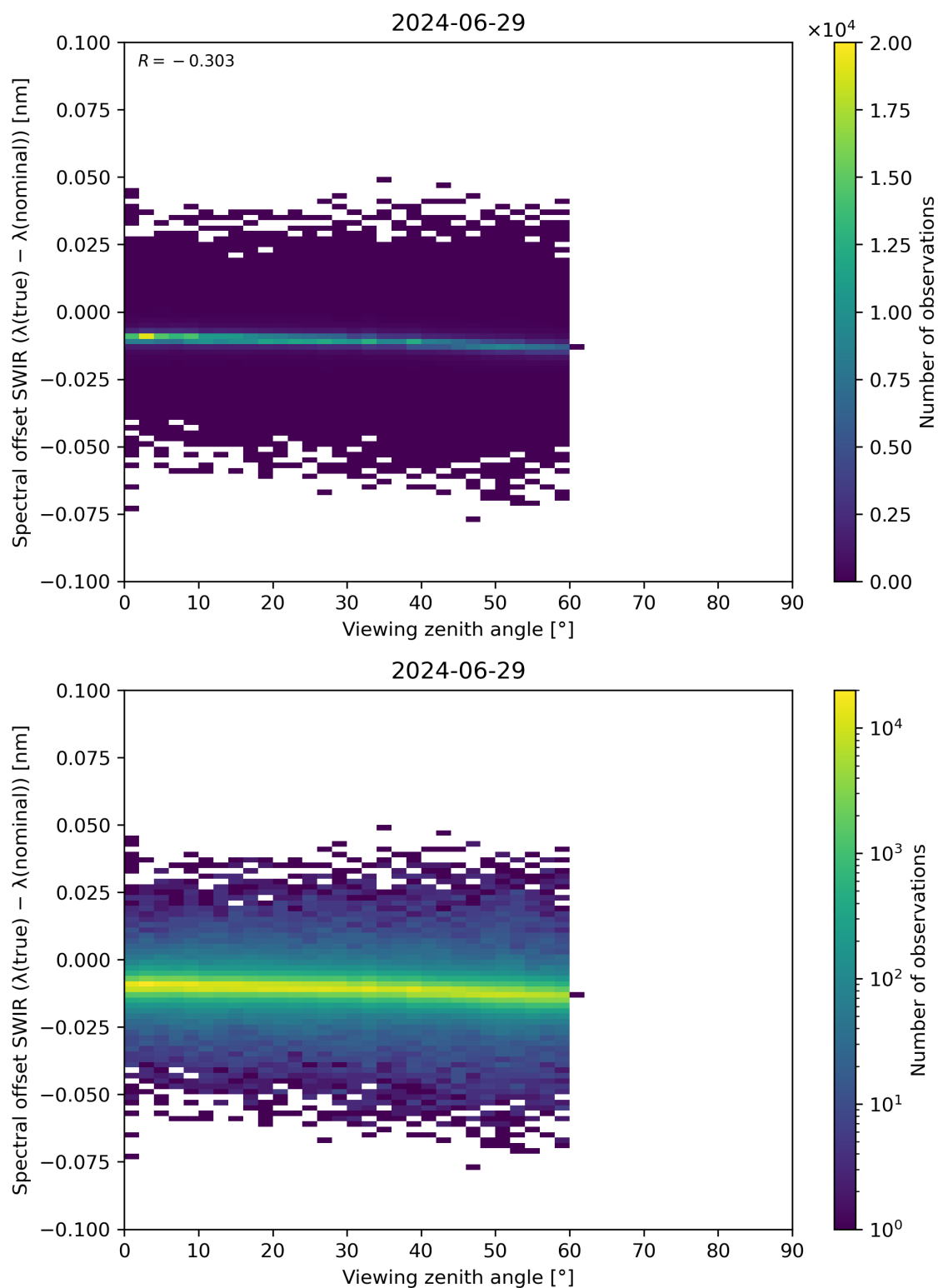
Figure 116: Scatter density plot of “Viewing zenith angle” against “Spectral offset SWIR ( \lambda(\text{true}) - \lambda(\text{nominal}) )” for 2024-06-29 to 2024-06-30.
