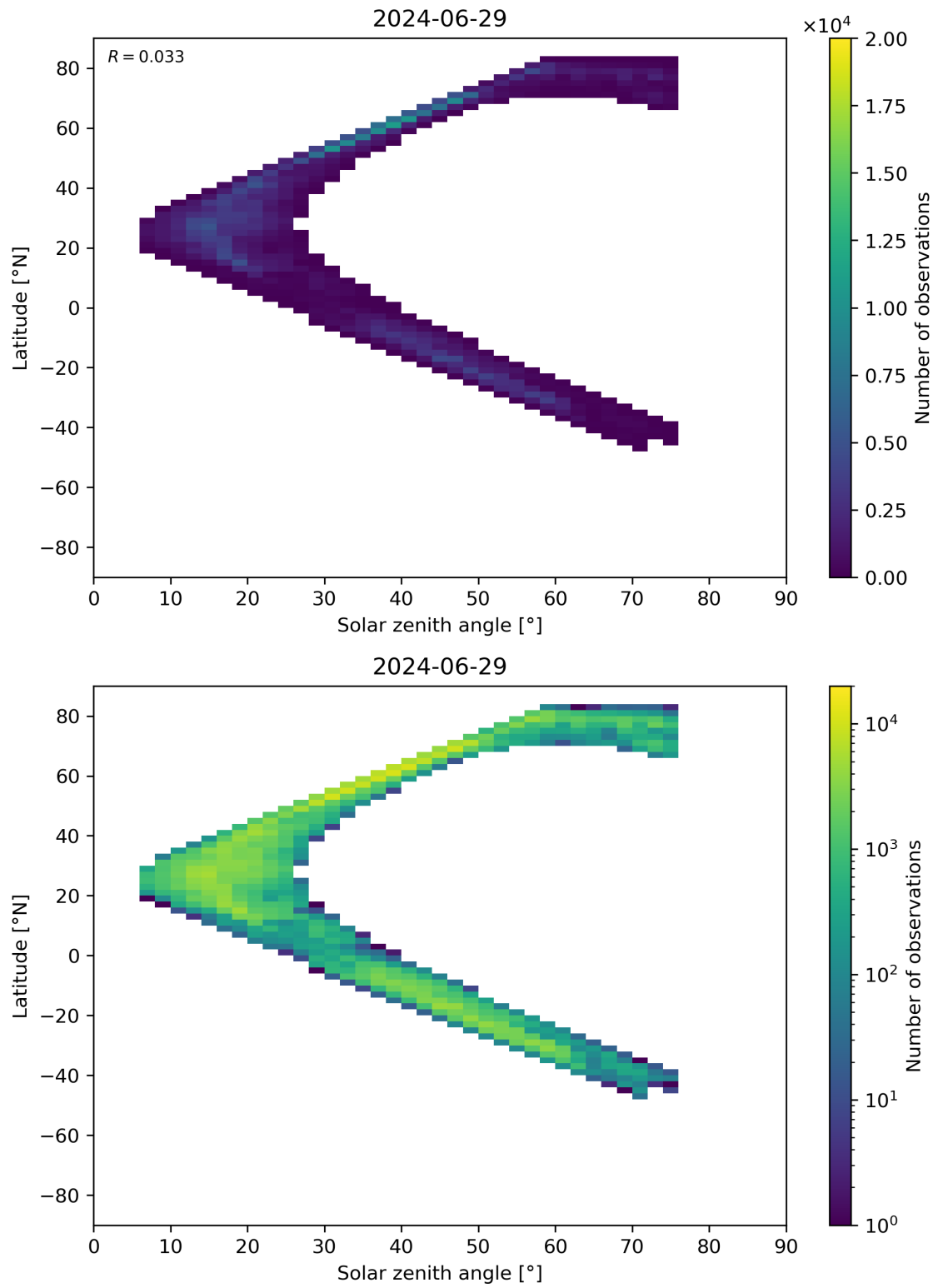
Figure 98: Scatter density plot of “Solar zenith angle” against “Latitude” for 2024-06-29 to 2024-06-30.
