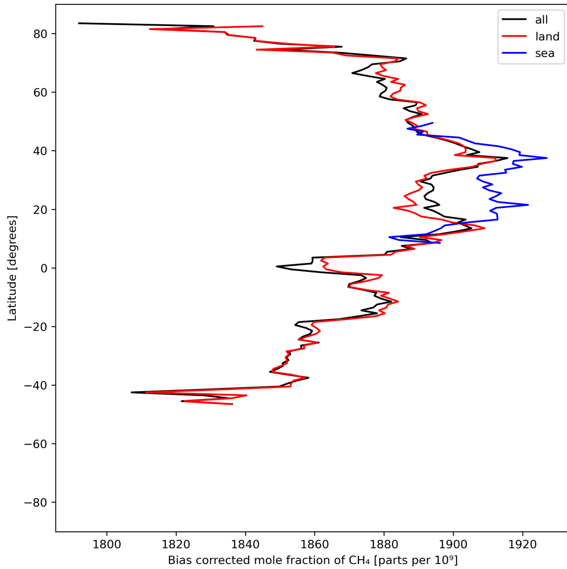
Figure 14: Zonal average of “Bias corrected mole fraction of CH 4 ” for 2024-06-29 to 2024-06-30.
