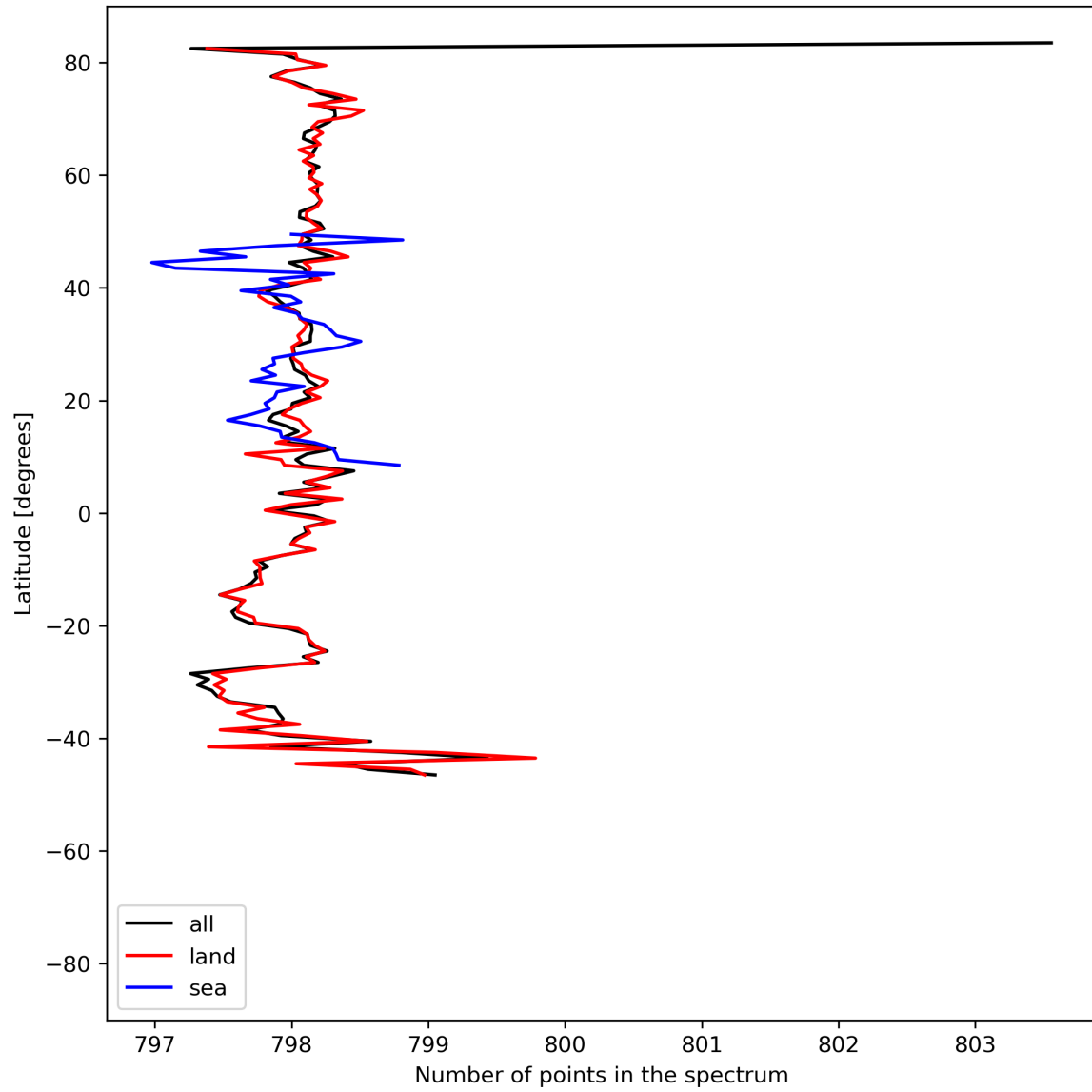
Figure 15: Zonal average of “Number of points in the spectrum” for 2024-06-29 to 2024-06-30.
