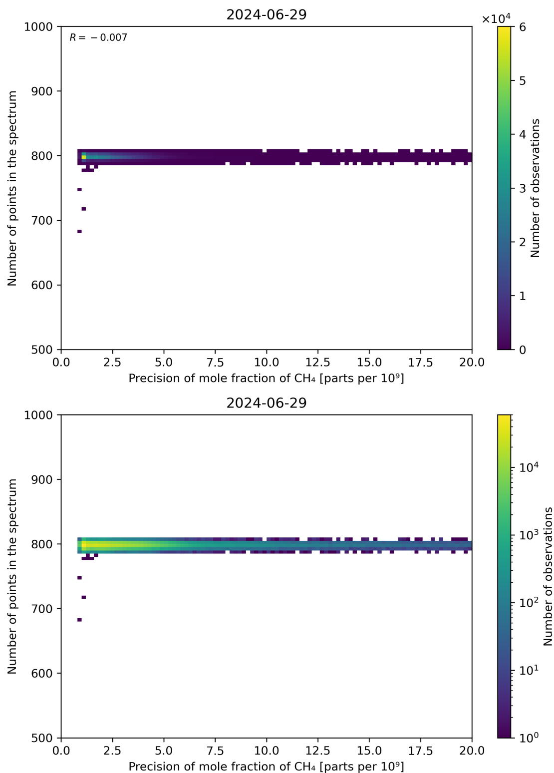
Figure 84: Scatter density plot of “Precision of mole fraction of CH 4 ” against “Number of points in the spectrum” for 2024-06-29 to 2024-06-30.
