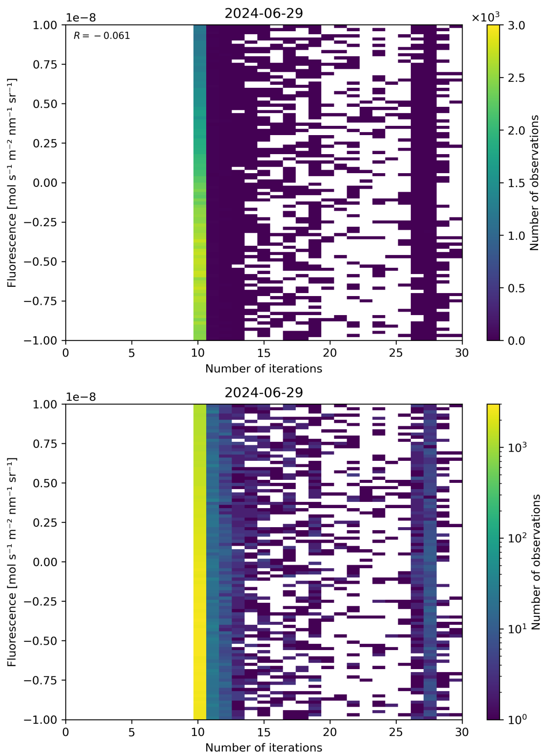
Figure 87: Scatter density plot of “Number of iterations” against “Fluorescence” for 2024-06-29 to 2024-06-30.
