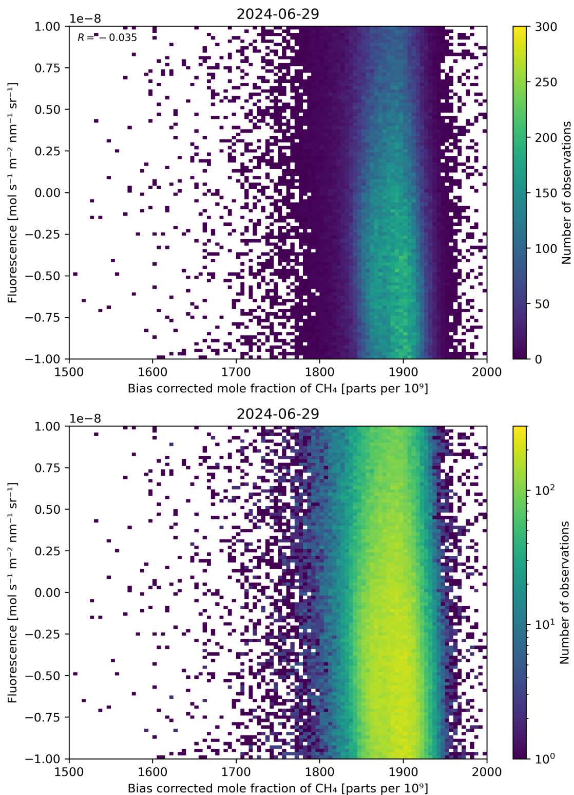
Figure 66: Scatter density plot of “Bias corrected mole fraction of \text{CH}_4 ” against “Fluorescence” for 2024-06-29 to 2024-06-30.
