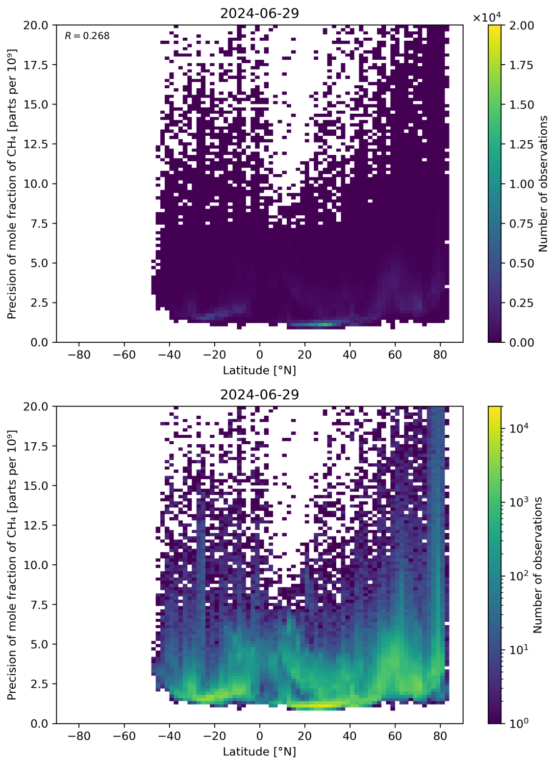
Figure 59: Scatter density plot of “Latitude” against “Precision of mole fraction of \text{CH}_4 ” for 2024-06-29 to 2024-06-30.
