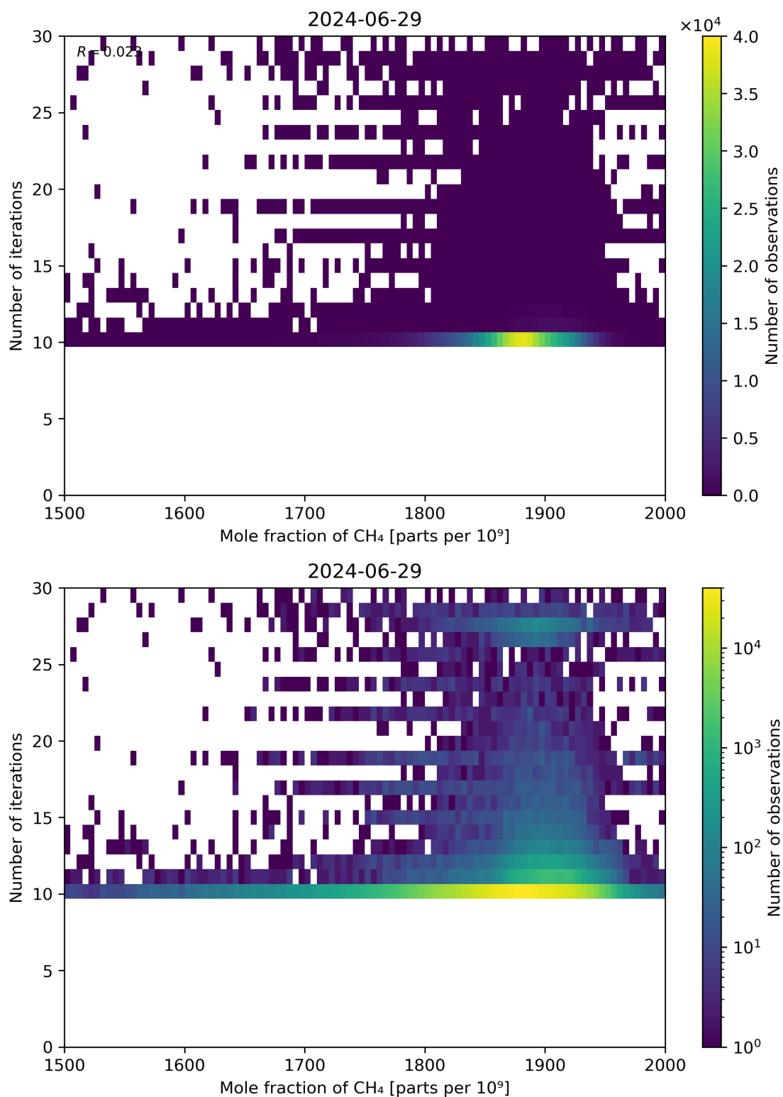
Figure 76: Scatter density plot of “Mole fraction of CH 4 ” against “Number of iterations” for 2024-06-29 to 2024-06-30.
