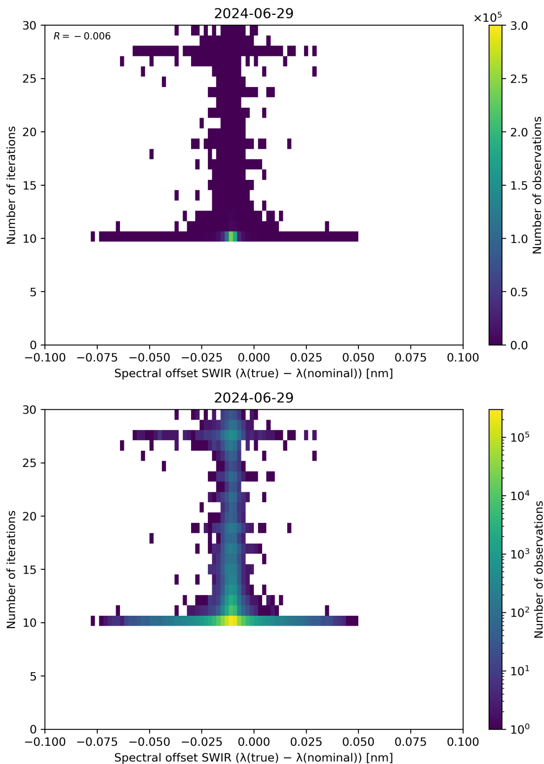
Figure 121: Scatter density plot of “Spectral offset SWIR ( \lambda(\text{true}) - \lambda(\text{nominal}) )” against “Number of iterations” for 2024-06-29 to 2024-06-30.
