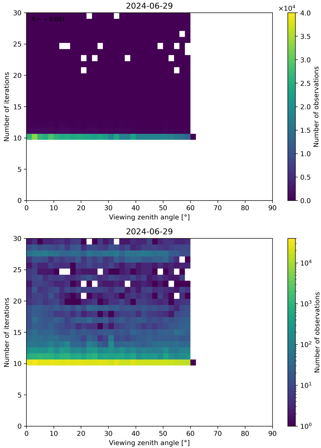
Figure 113: Scatter density plot of “Viewing zenith angle” against “Number of iterations” for 2024-06-29 to 2024-06-30.
