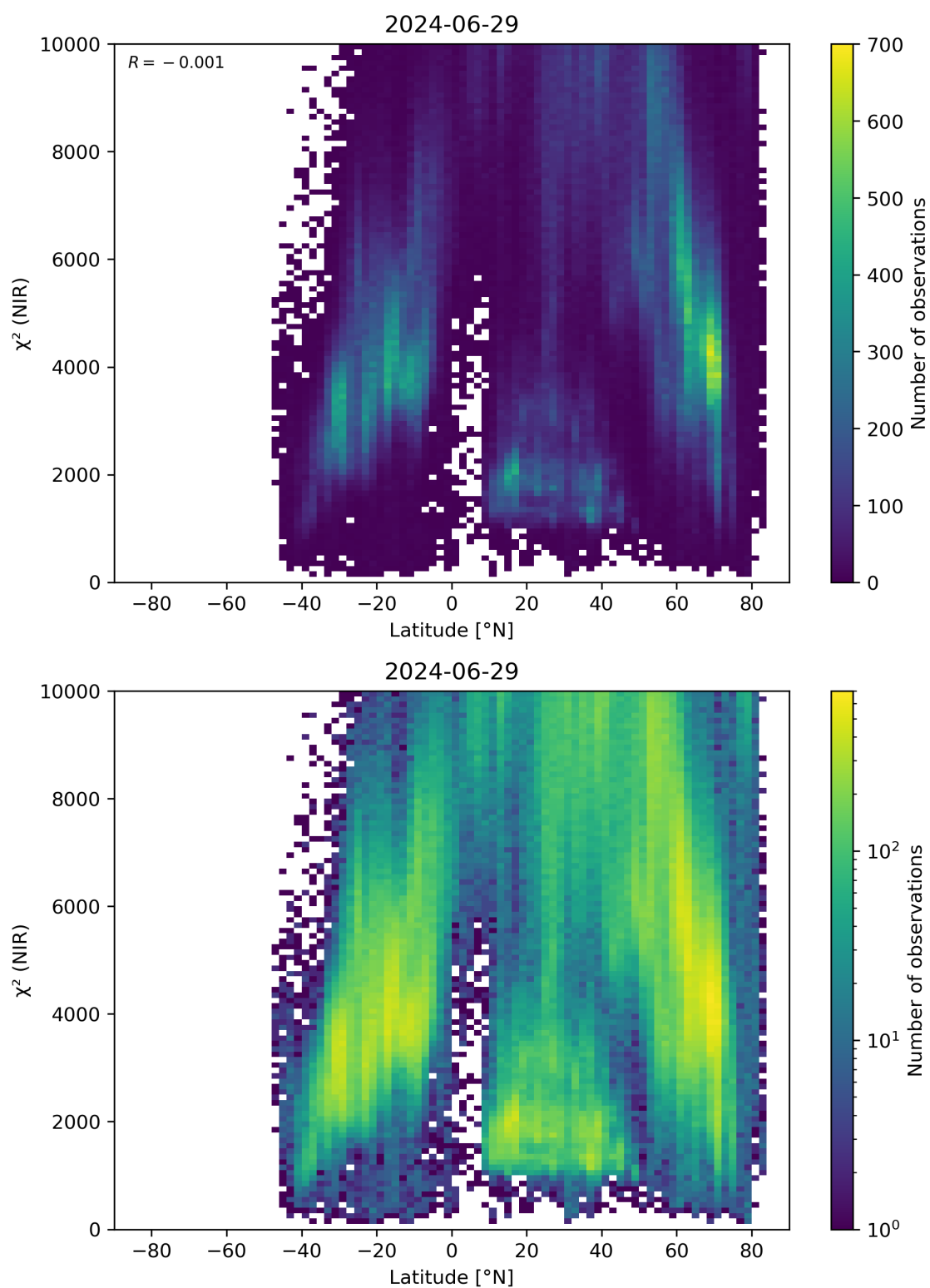
Figure 53: Scatter density plot of “Latitude” against “ \chi^2 (NIR)” for 2024-06-29 to 2024-06-30.
