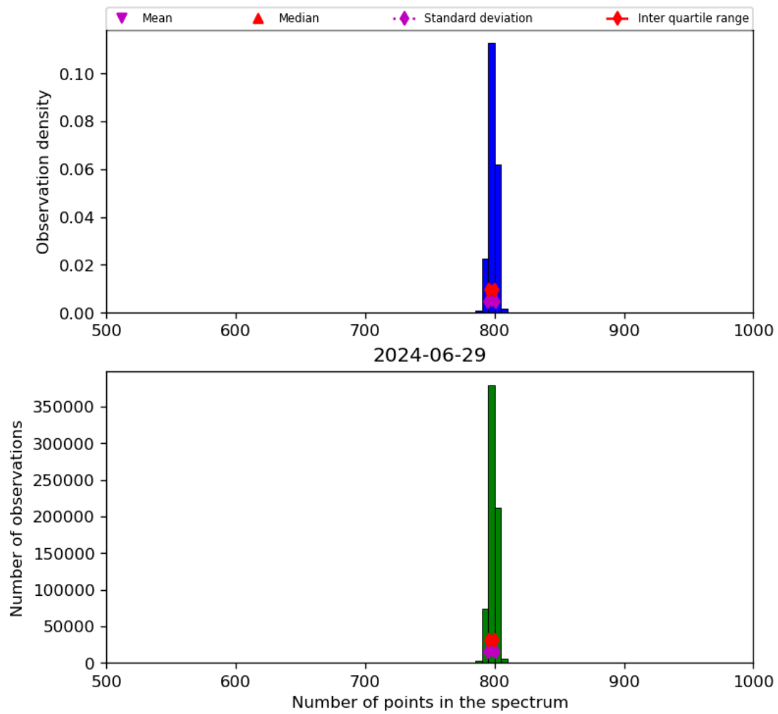
Figure 26: Histogram of “Number of points in the spectrum” for 2024-06-29 to 2024-06-30
