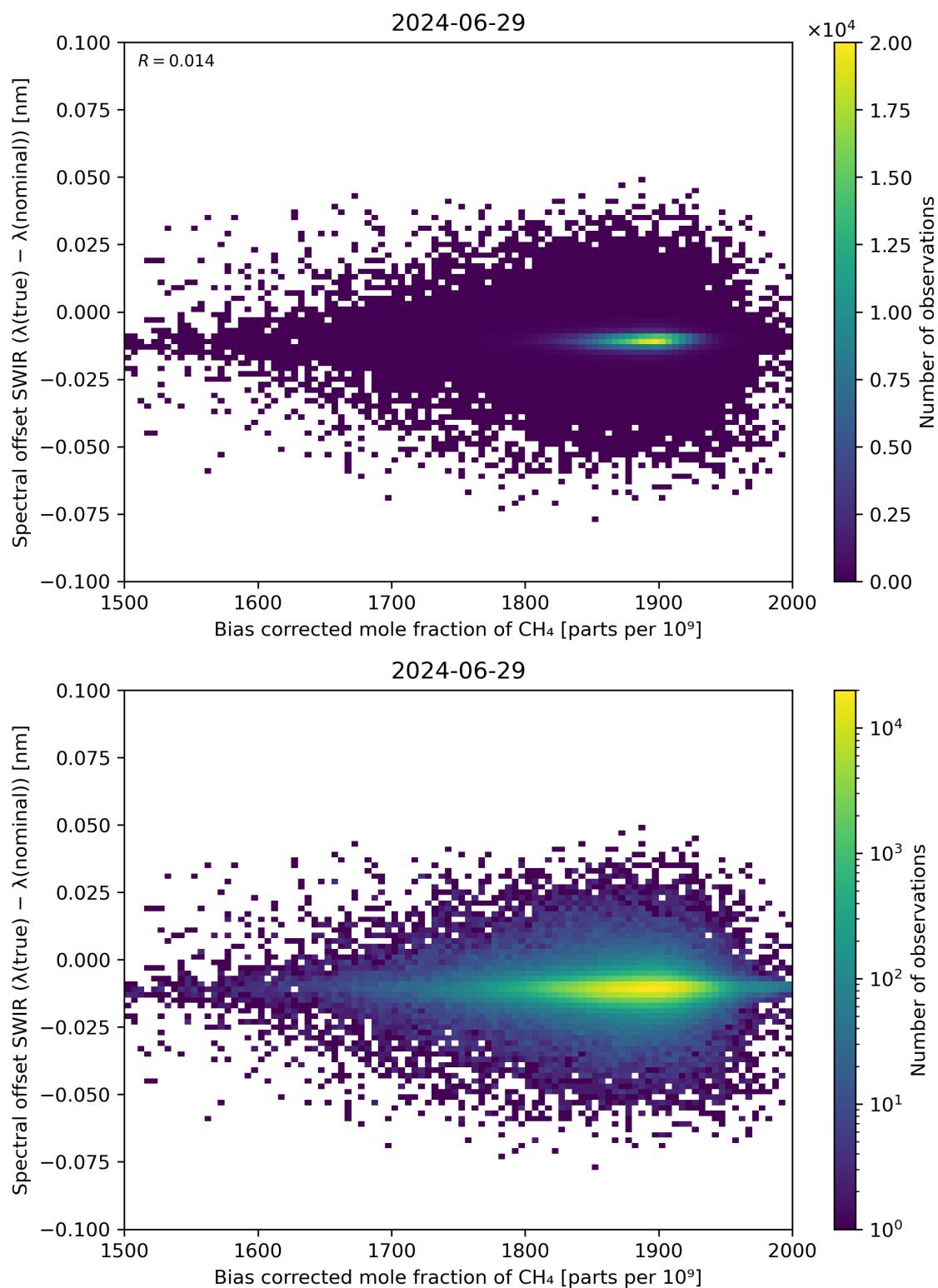
Figure 69: Scatter density plot of “Bias corrected mole fraction of \text{CH}_4 ” against “Spectral offset SWIR ( \lambda(\text{true}) - \lambda(\text{nominal}) )” for 2024-06-29 to 2024-06-30.
