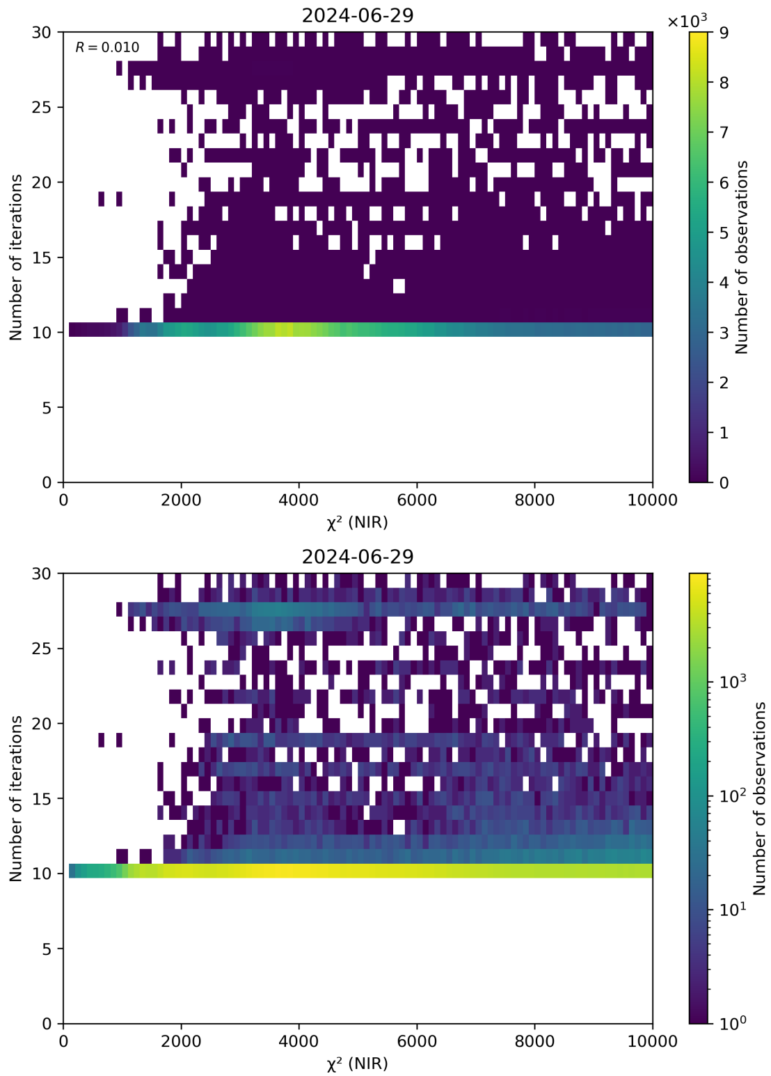
Figure 46: Scatter density plot of “ \chi^2 (NIR)” against “Number of iterations” for 2024-06-29 to 2024-06-30.
