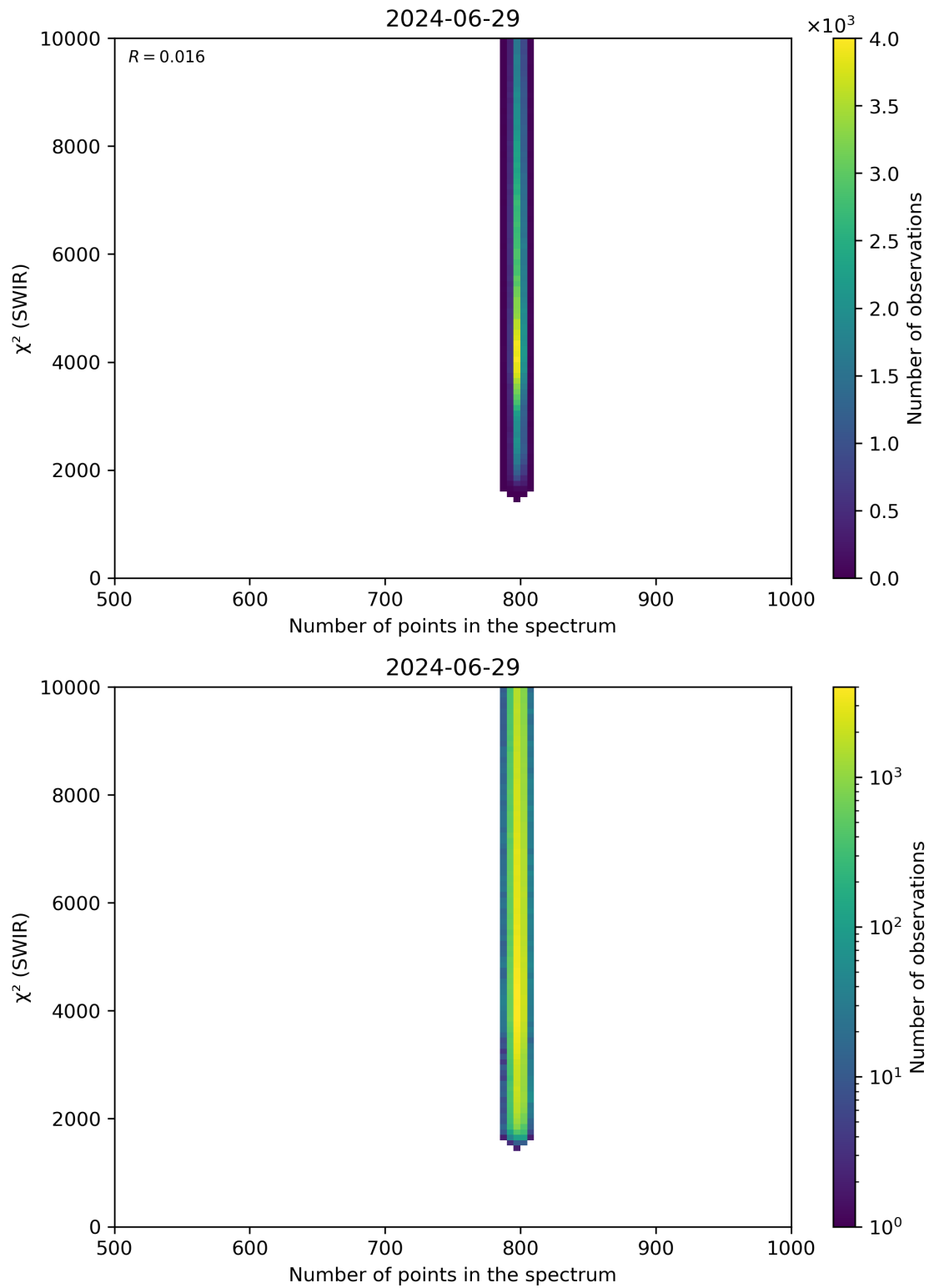
Figure 89: Scatter density plot of “Number of points in the spectrum” against “ \chi^2 (SWIR)” for 2024-06-29 to 2024-06-30.
