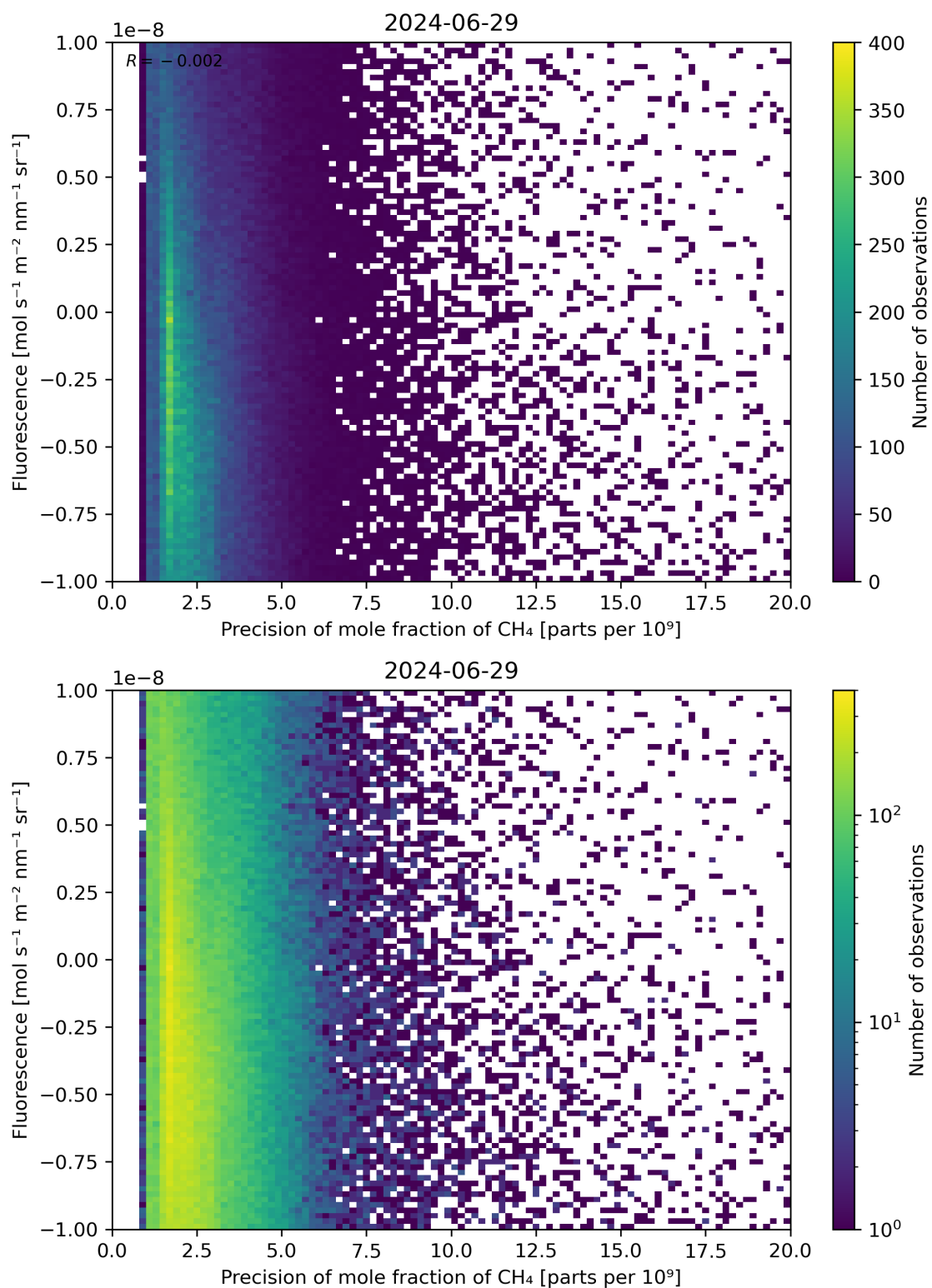
Figure 81: Scatter density plot of “Precision of mole fraction of CH 4 ” against “Fluorescence” for 2024-06-29 to 2024-06-30.
