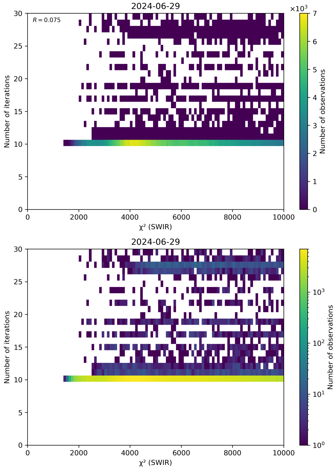
Figure 50: Scatter density plot of " \chi^2 (SWIR)" against "Number of iterations" for 2024-06-29 to 2024-06-30.
