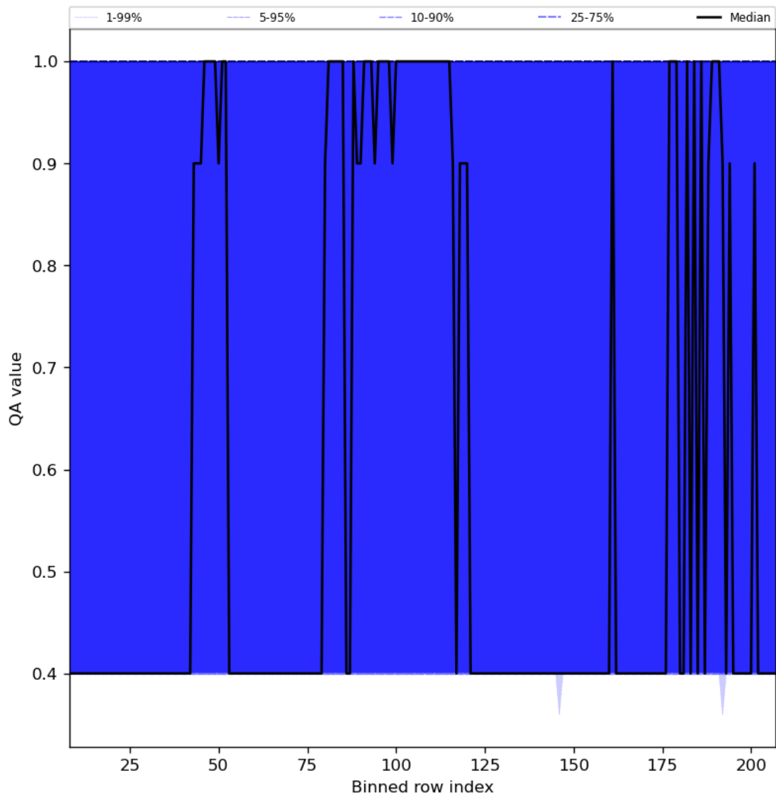
Figure 33: Along track statistics of “QA value” for 2024-06-29 to 2024-06-30
