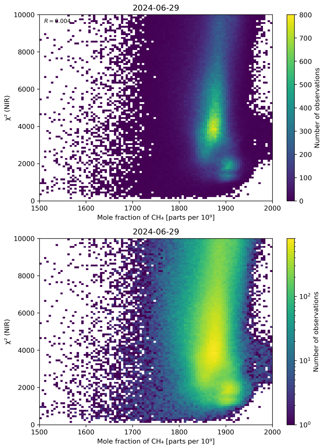
Figure 70: Scatter density plot of “Mole fraction of \text{CH}_4 ” against “ \chi^2 (NIR)” for 2024-06-29 to 2024-06-30.
