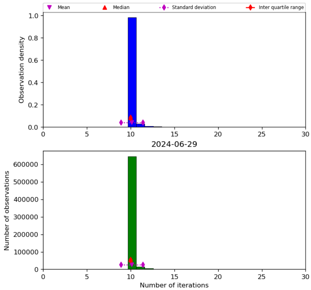
Figure 31: Histogram of “Number of iterations” for 2024-06-29 to 2024-06-30
