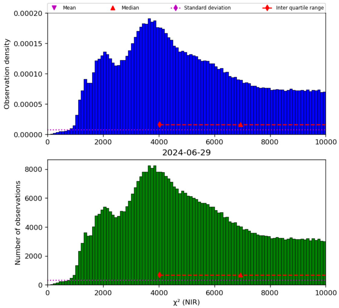
Figure 29: Histogram of “ \chi^2 (NIR)” for 2024-06-29 to 2024-06-30
