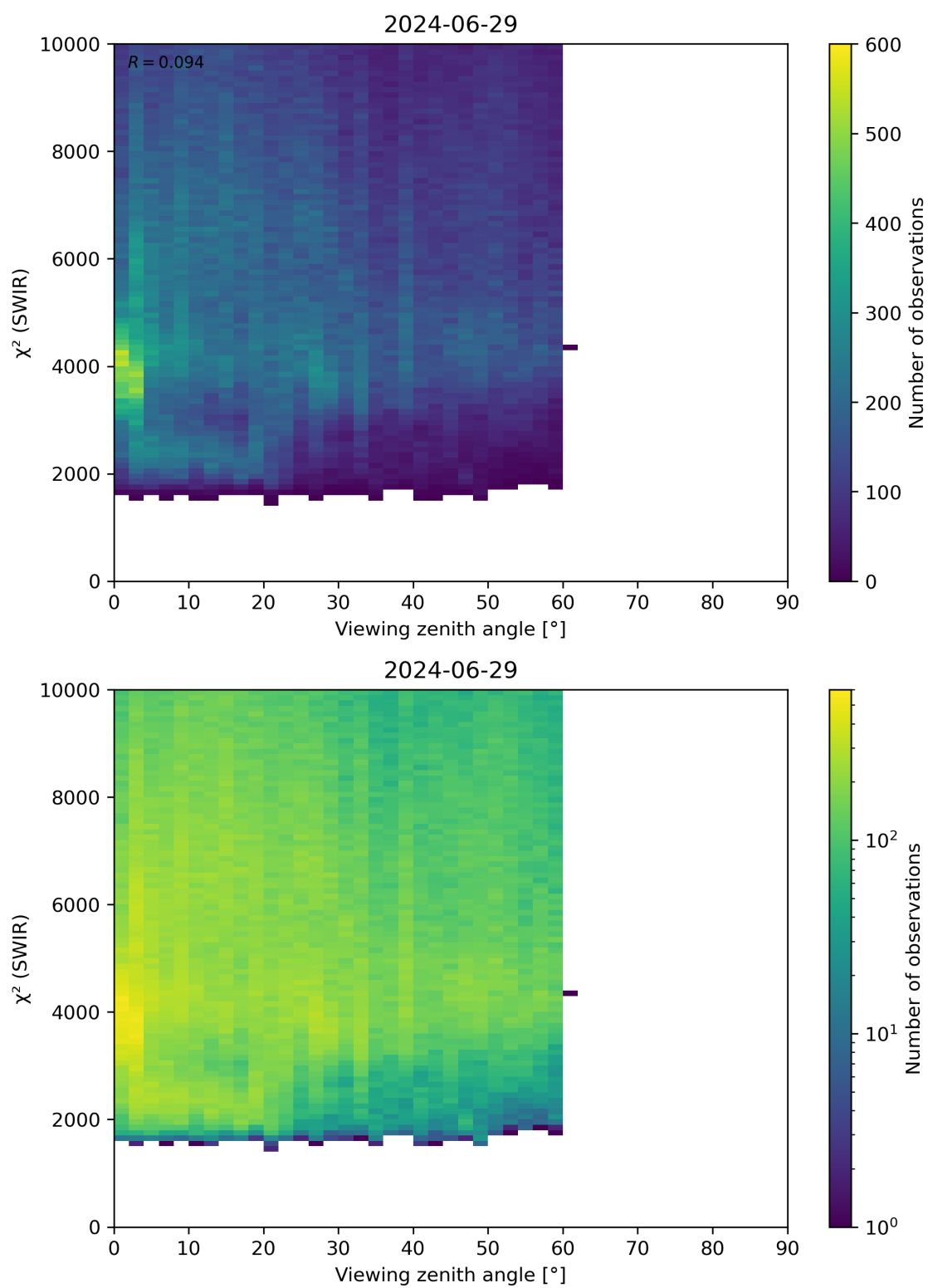
Figure 106: Scatter density plot of “Viewing zenith angle” against “ \chi^2 (SWIR)” for 2024-06-29 to 2024-06-30.
