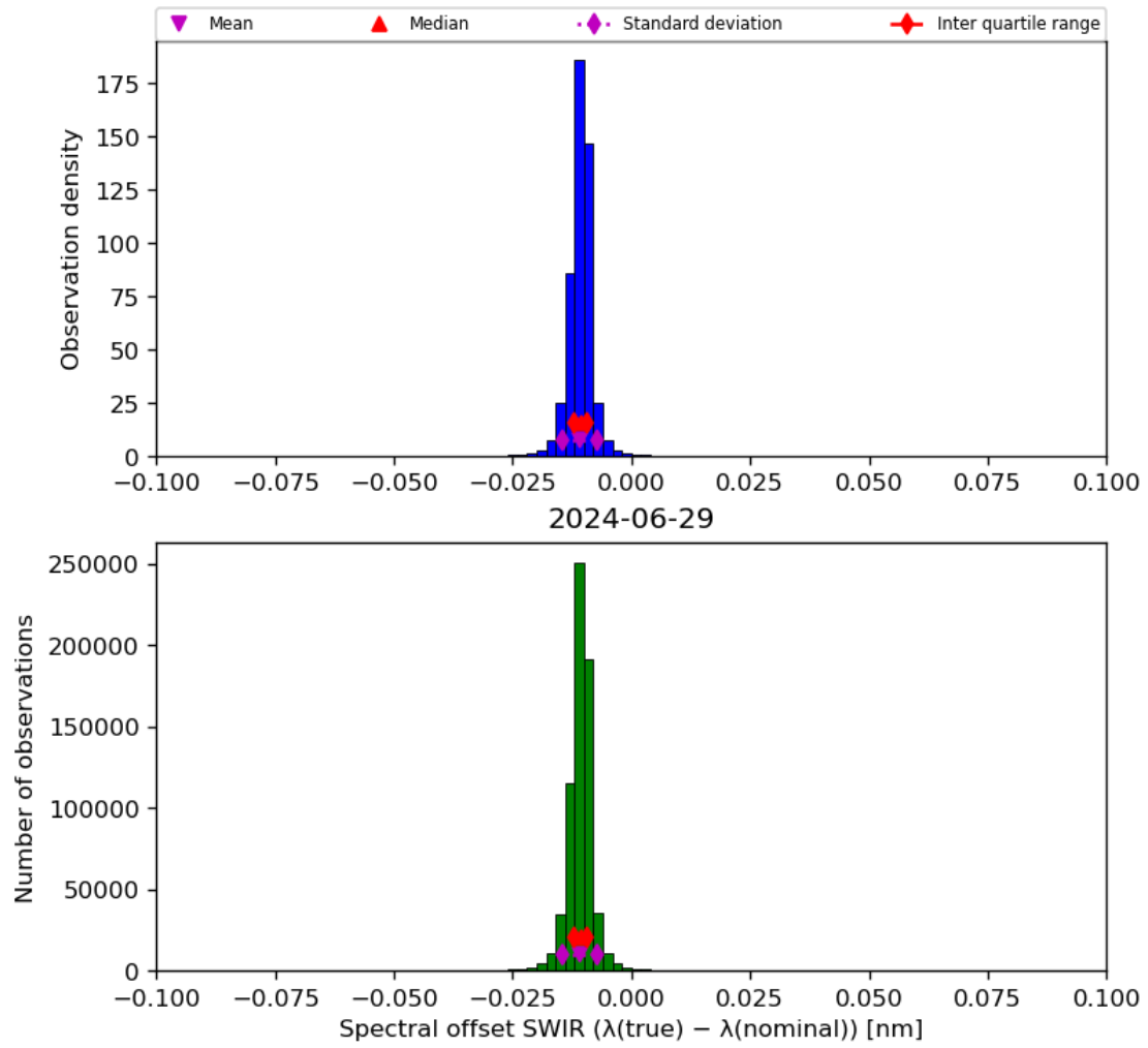
Figure 27: Histogram of “Spectral offset SWIR ( \lambda(\text{true}) - \lambda(\text{nominal}) )” for 2024-06-29 to 2024-06-30
