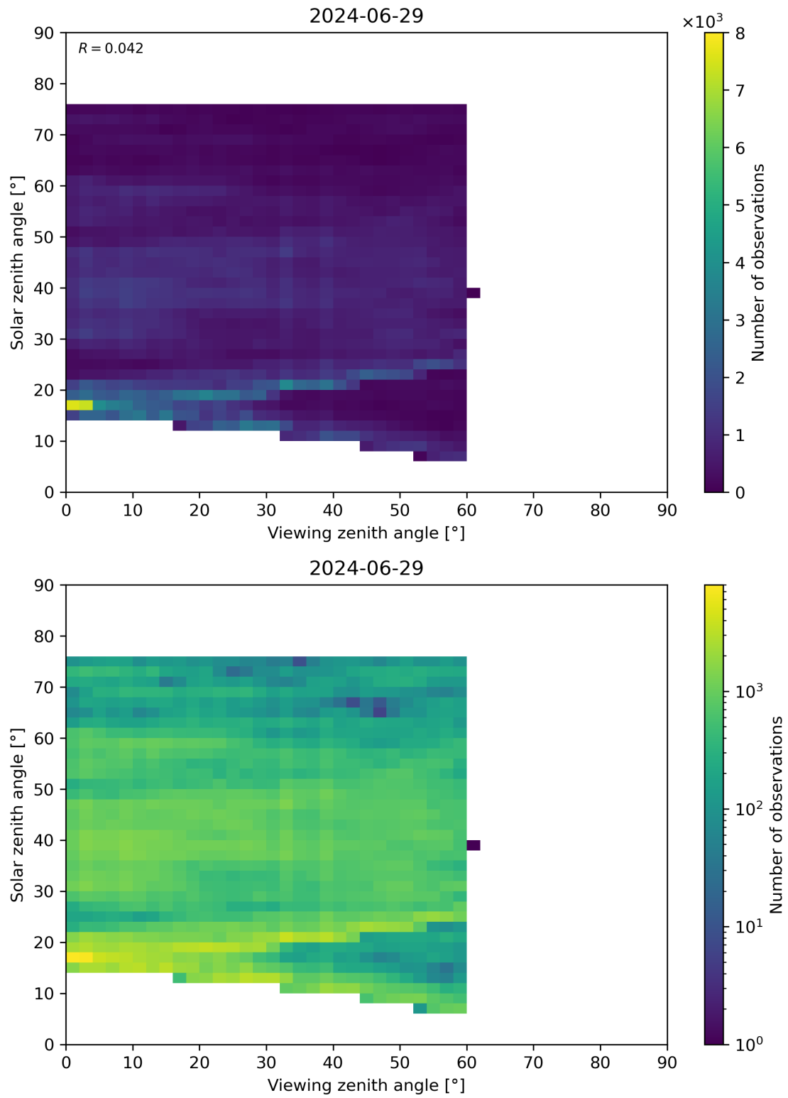
Figure 115: Scatter density plot of “Viewing zenith angle” against “Solar zenith angle” for 2024-06-29 to 2024-06-30.
