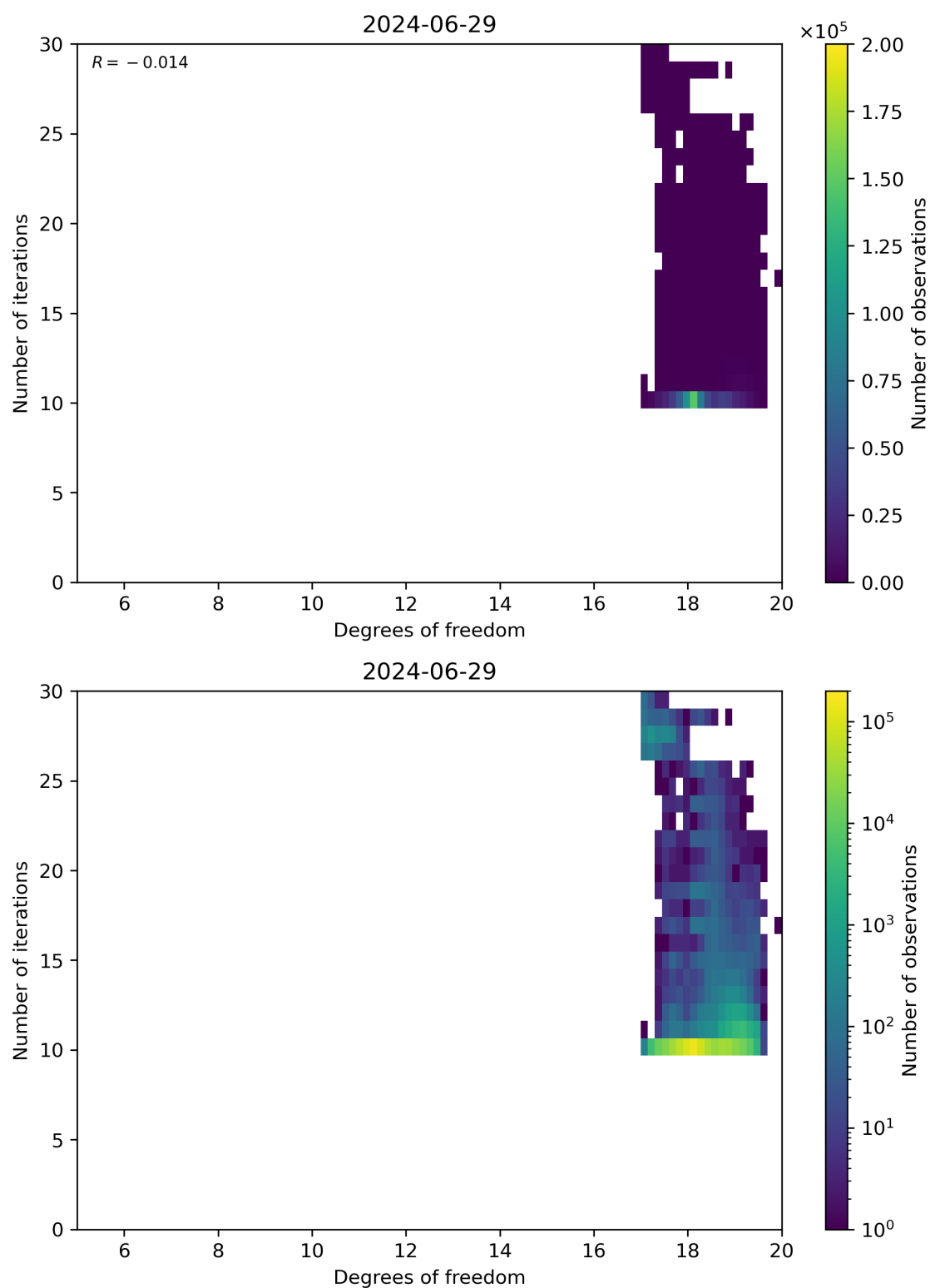
Figure 52: Scatter density plot of “Degrees of freedom” against “Number of iterations” for 2024-06-29 to 2024-06-30.
