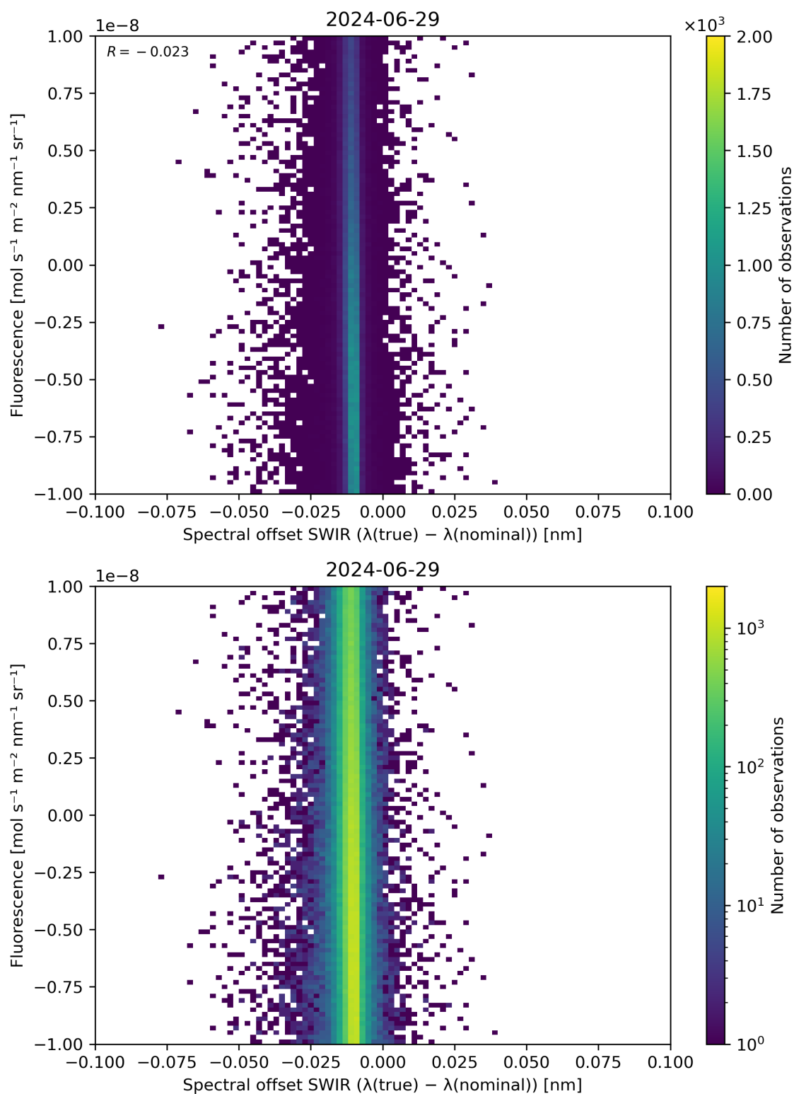
Figure 120: Scatter density plot of “Spectral offset SWIR ( \lambda(\text{true}) - \lambda(\text{nominal}) )” against “Fluorescence” for 2024-06-29 to 2024-06-30.
