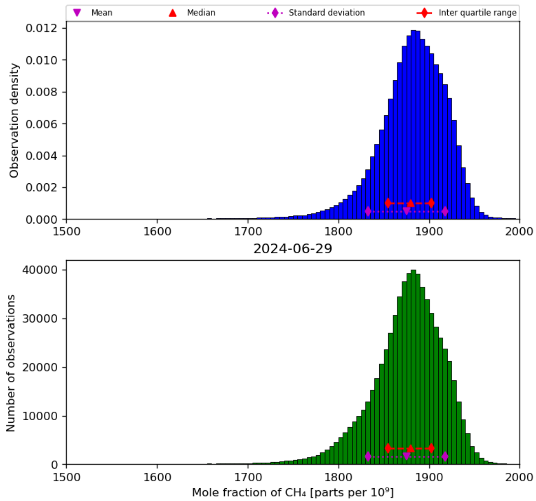
Figure 23: Histogram of “Mole fraction of CH 4 ” for 2024-06-29 to 2024-06-30
