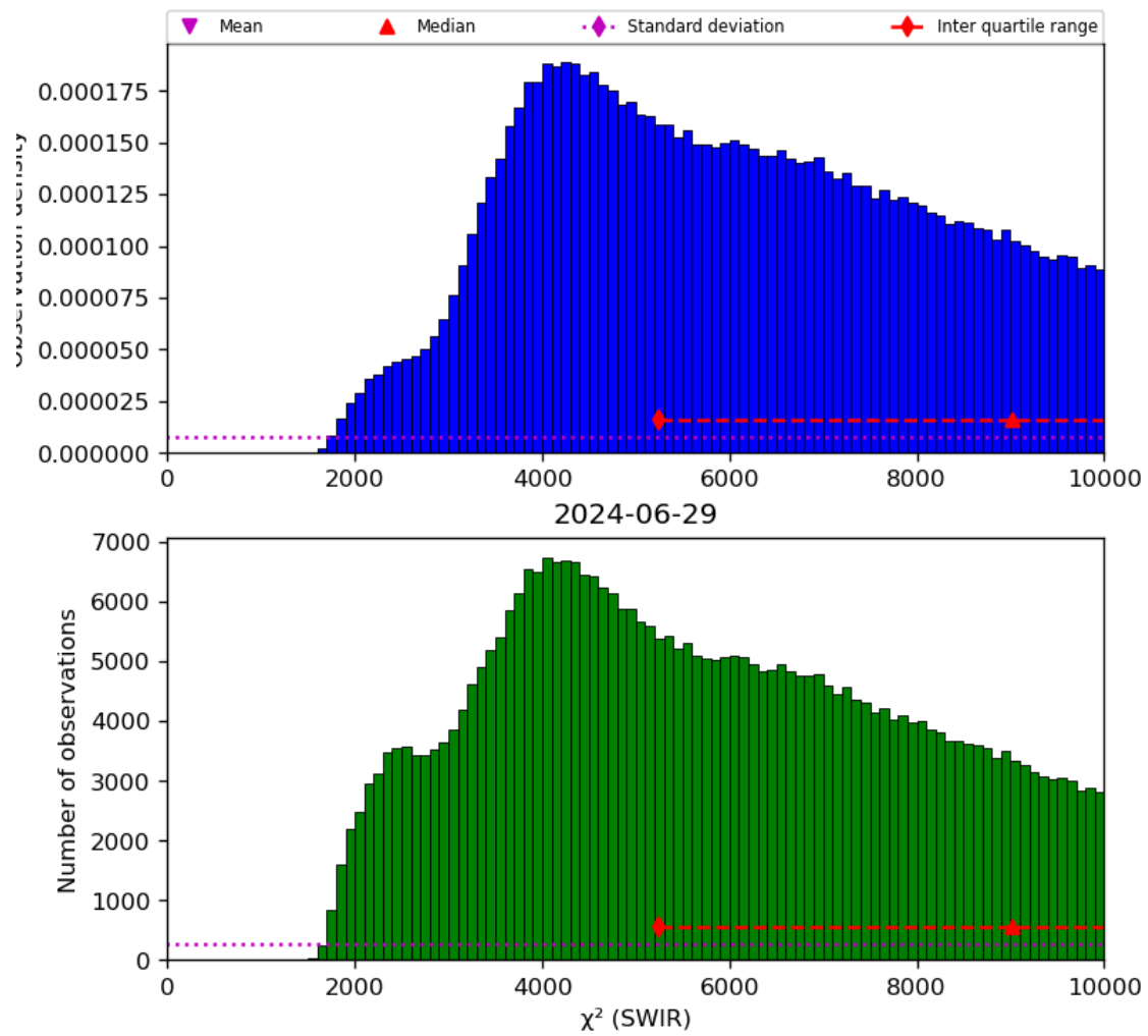
Figure 28: Histogram of “ \chi^2 (SWIR)” for 2024-06-29 to 2024-06-30
