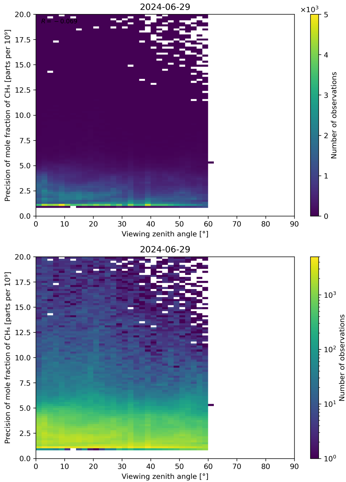
Figure 112: Scatter density plot of “Viewing zenith angle” against “Precision of mole fraction of CH 4 ” for 2024-06-29 to 2024-06-30.
