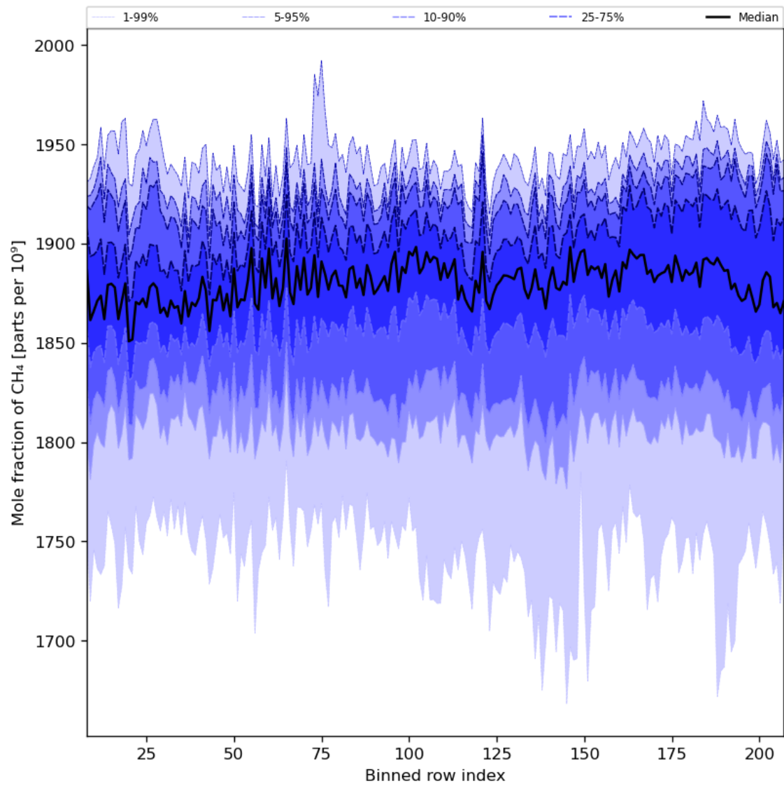
Figure 34: Along track statistics of “Mole fraction of CH 4 ” for 2024-06-29 to 2024-06-30
