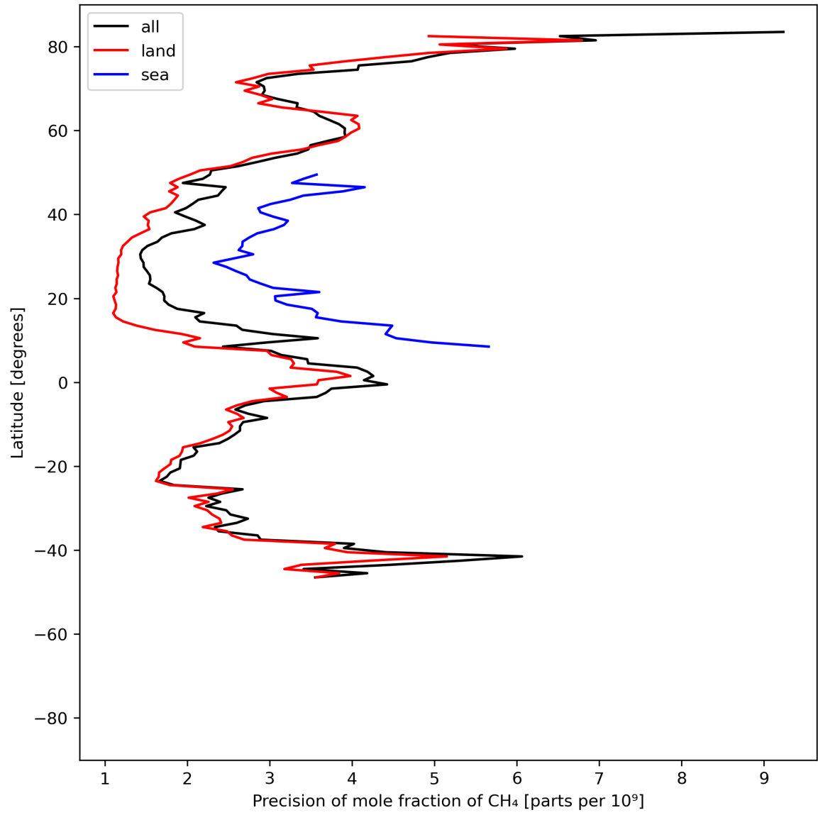
Figure 13: Zonal average of “Precision of mole fraction of CH 4 ” for 2024-06-29 to 2024-06-30.
