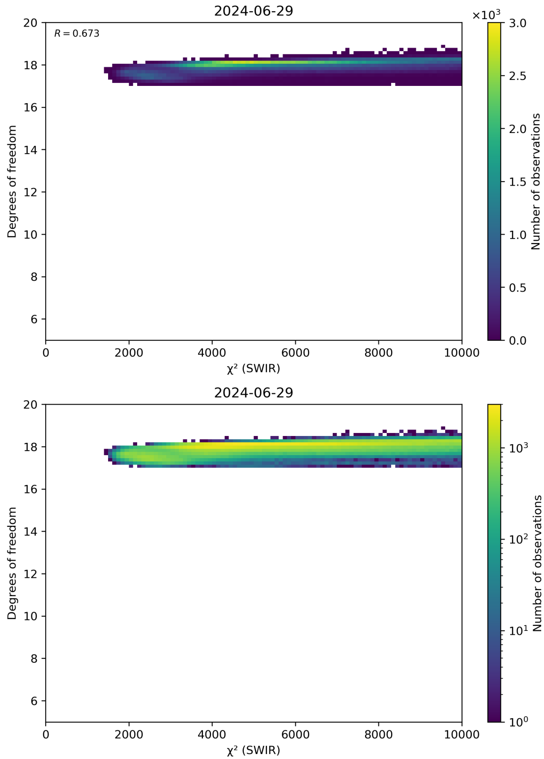
Figure 48: Scatter density plot of " \chi^2 (SWIR)" against "Degrees of freedom" for 2024-06-29 to 2024-06-30.
