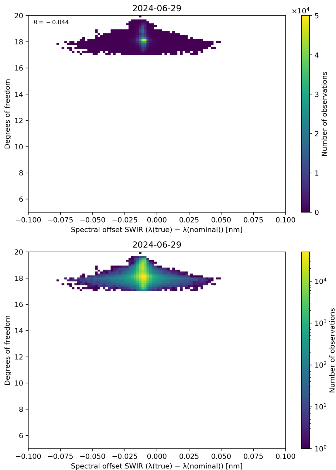
Figure 119: Scatter density plot of “Spectral offset SWIR ( \lambda(\text{true}) - \lambda(\text{nominal}) )” against “Degrees of freedom” for 2024-06-29 to 2024-06-30.
