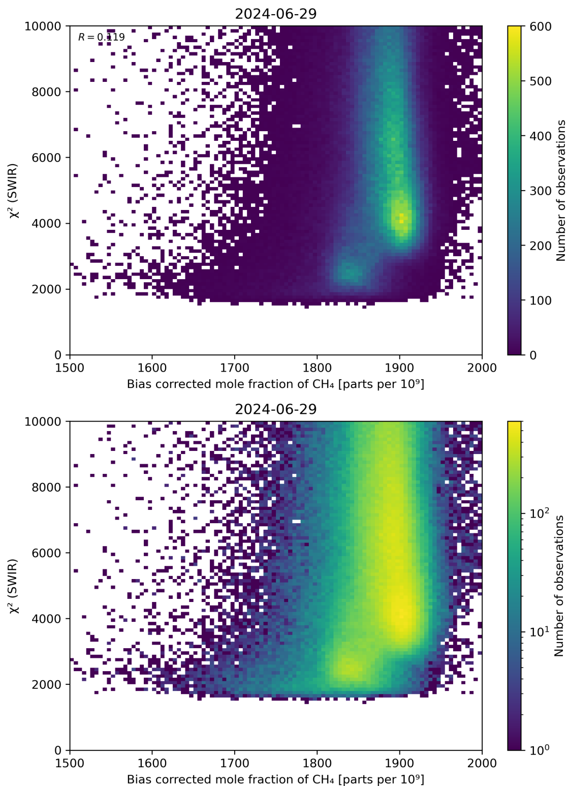
Figure 64: Scatter density plot of “Bias corrected mole fraction of CH 4 ” against “ \chi^2 (SWIR)” for 2024-06-29 to 2024-06-30.
