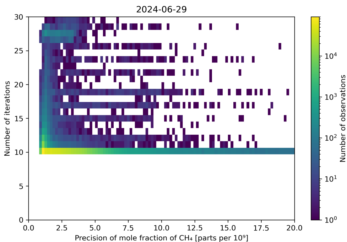
Figure 83: Scatter density plot of “Precision of mole fraction of CH 4 ” against “Number of iterations” for 2024-06-29 to 2024-06-30.
