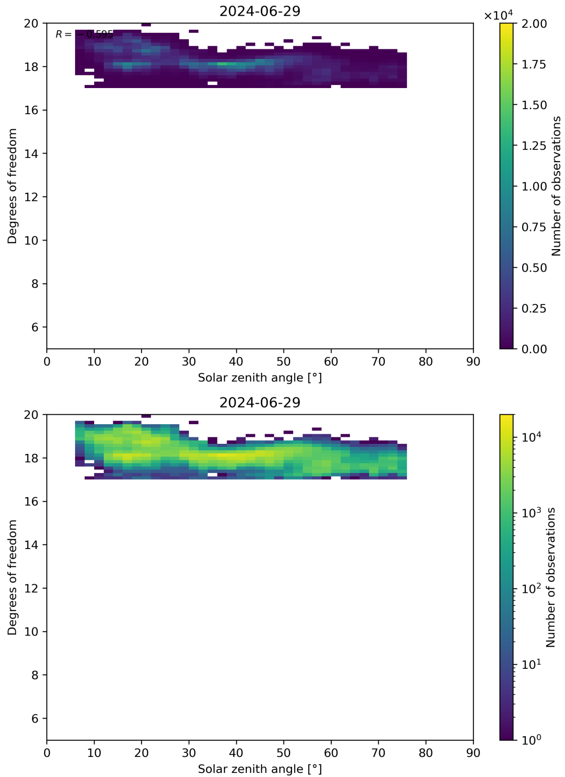
Figure 96: Scatter density plot of “Solar zenith angle” against “Degrees of freedom” for 2024-06-29 to 2024-06-30.
