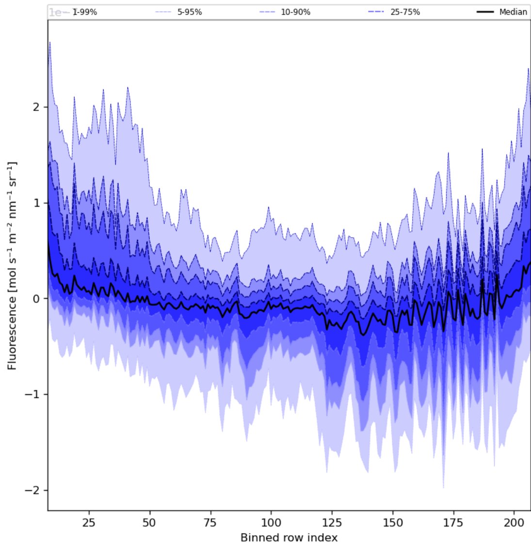
Figure 43: Along track statistics of “Fluorescence” for 2024-06-29 to 2024-06-30
