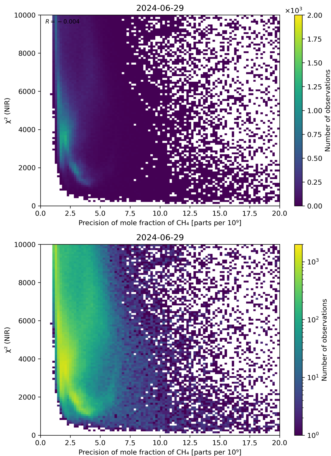
Figure 78: Scatter density plot of “Precision of mole fraction of CH 4 ” against “ \chi^2 (NIR)” for 2024-06-29 to 2024-06-30.
