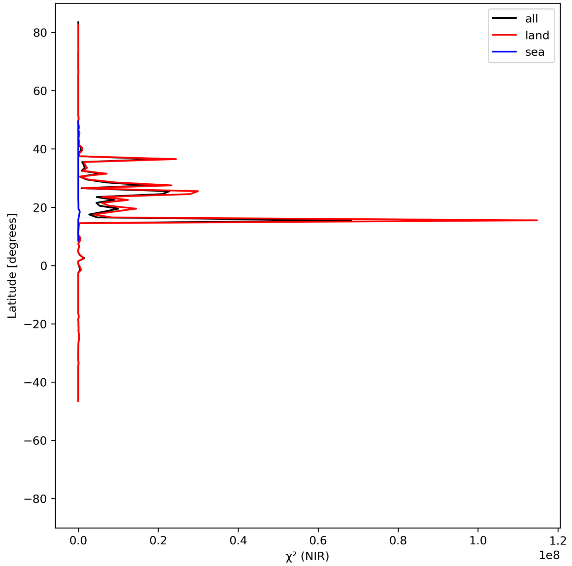
Figure 18: Zonal average of “ \chi^2 (NIR)” for 2024-06-29 to 2024-06-30.
