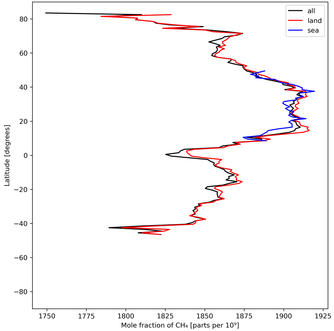
Figure 12: Zonal average of “Mole fraction of \text{CH}_4 ” for 2024-06-29 to 2024-06-30.
