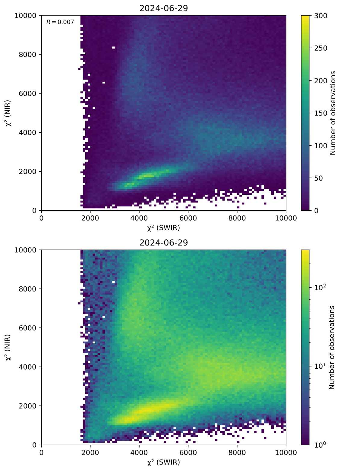
Figure 47: Scatter density plot of “ \chi^2 (SWIR)” against “ \chi^2 (NIR)” for 2024-06-29 to 2024-06-30.
