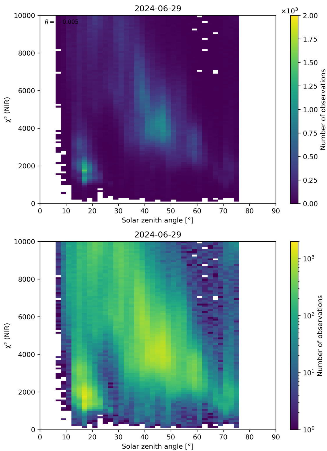
Figure 94: Scatter density plot of “Solar zenith angle” against “ \chi^2 (NIR)” for 2024-06-29 to 2024-06-30.
