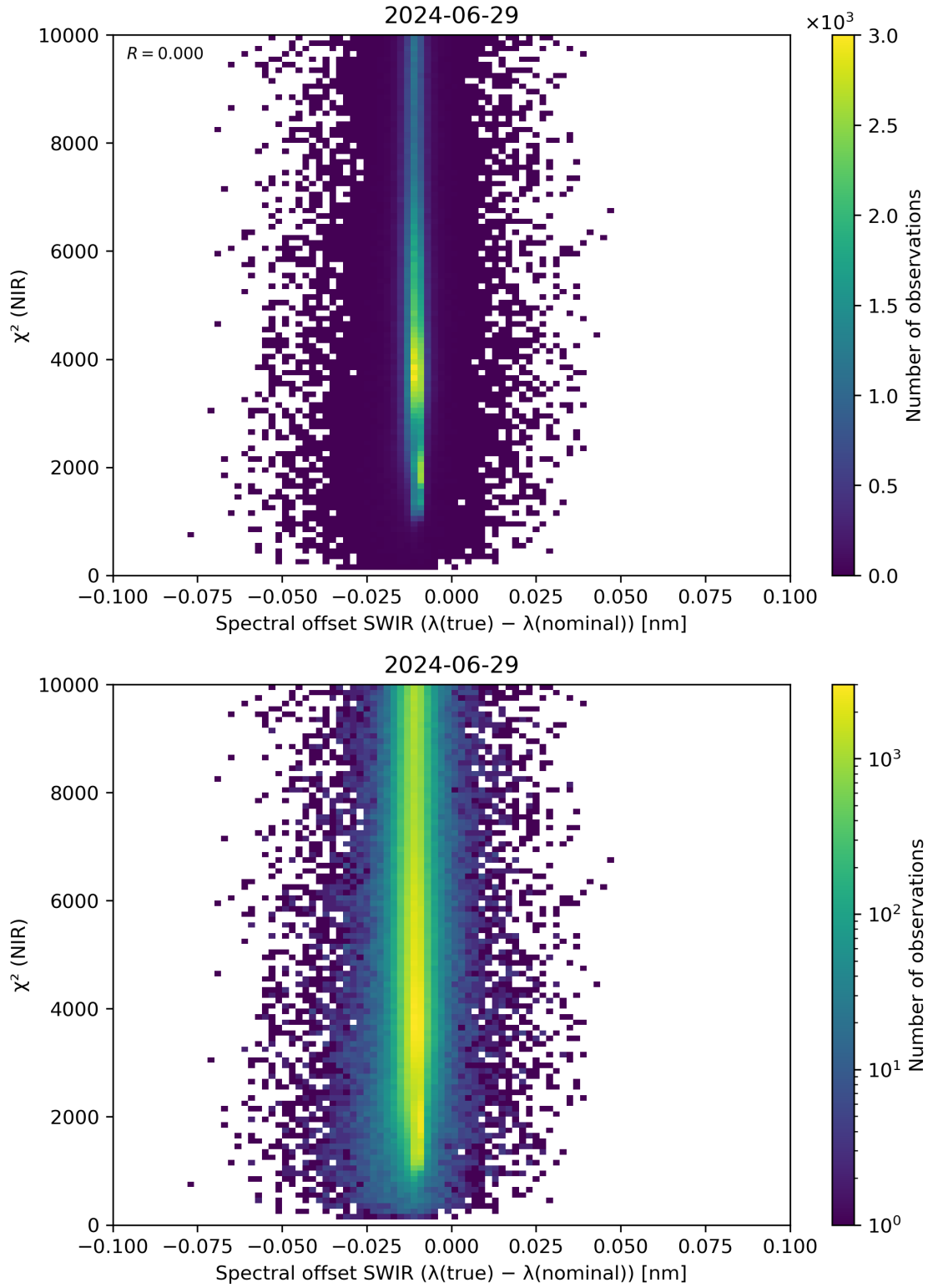
Figure 117: Scatter density plot of “Spectral offset SWIR ( \lambda(\text{true}) - \lambda(\text{nominal}) )” against “ \chi^2 (NIR)” for 2024-06-29 to 2024-06-30.
