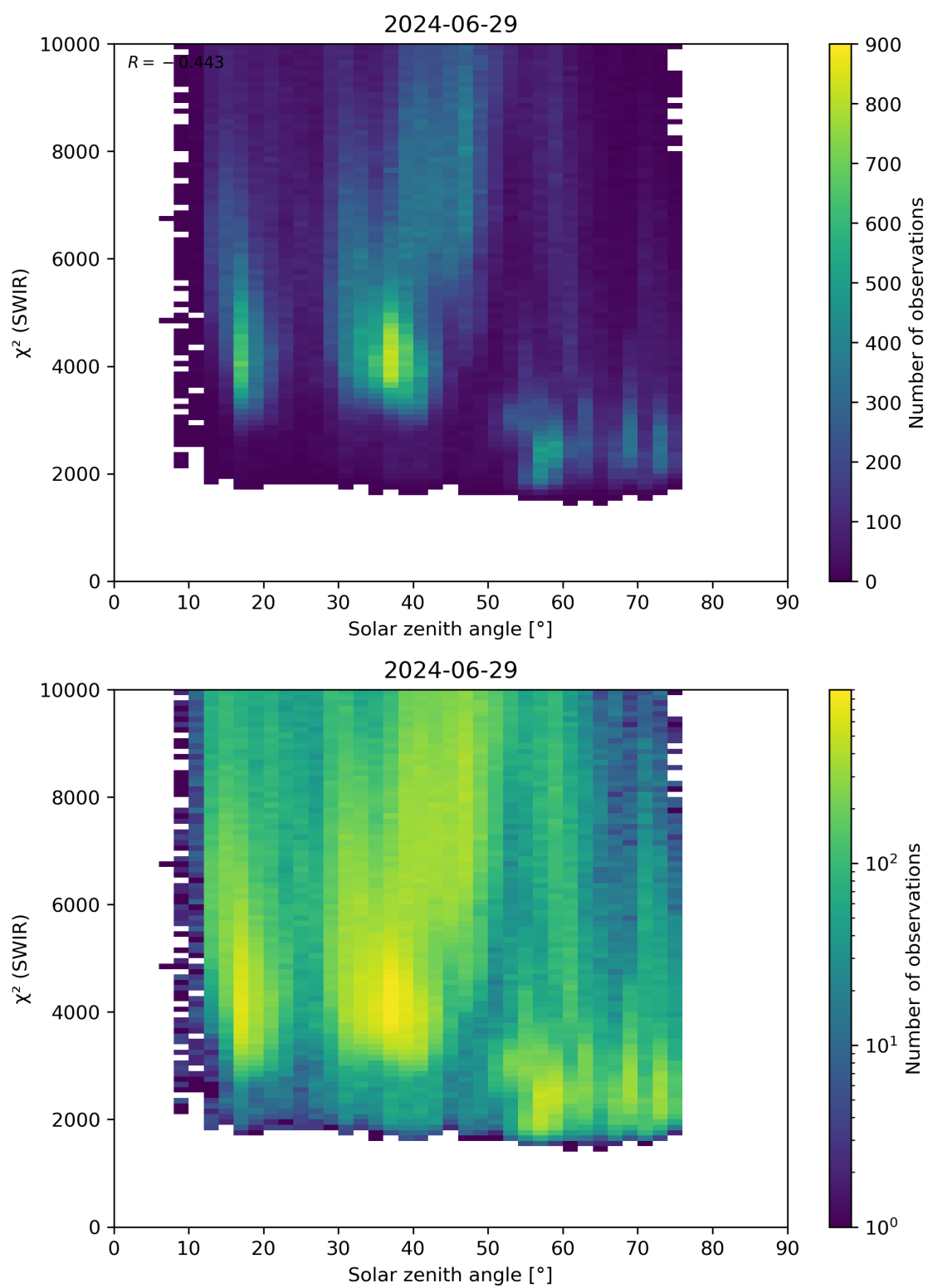
Figure 95: Scatter density plot of “Solar zenith angle” against “ \chi^2 (SWIR)” for 2024-06-29 to 2024-06-30.
