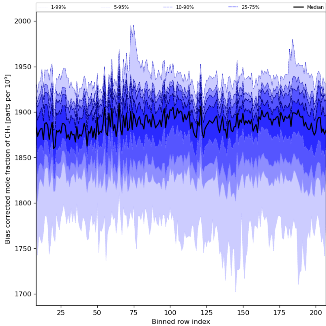
Figure 36: Along track statistics of “Bias corrected mole fraction of CH 4 ” for 2024-06-29 to 2024-06-30
