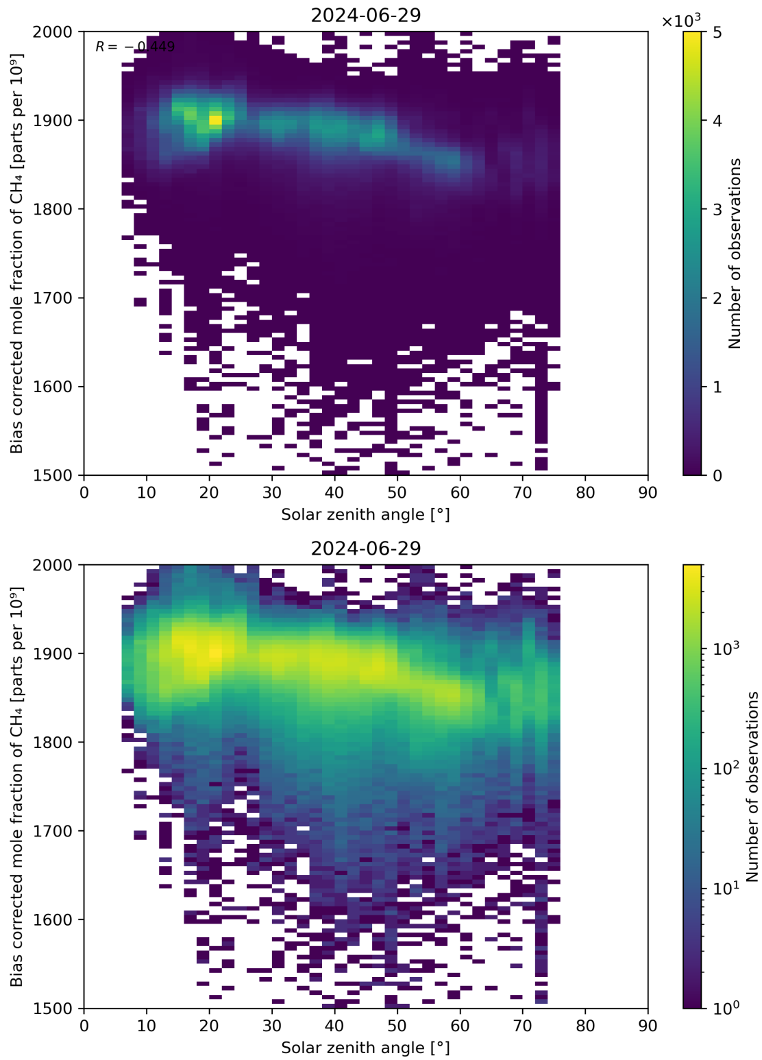
Figure 100: Scatter density plot of “Solar zenith angle” against “Bias corrected mole fraction of CH 4 ” for 2024-06-29 to 2024-06-30.
