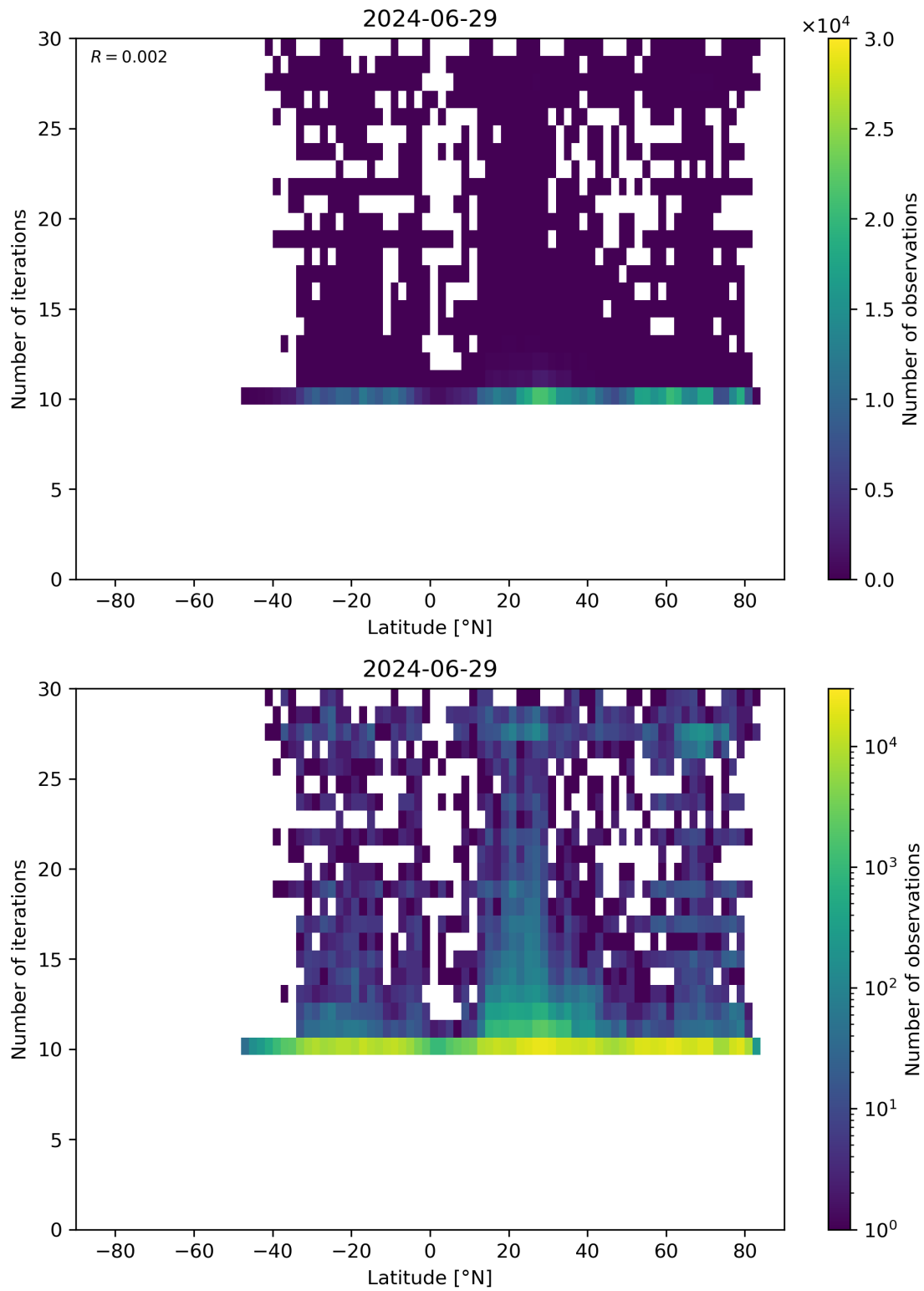
Figure 60: Scatter density plot of “Latitude” against “Number of iterations” for 2024-06-29 to 2024-06-30.
