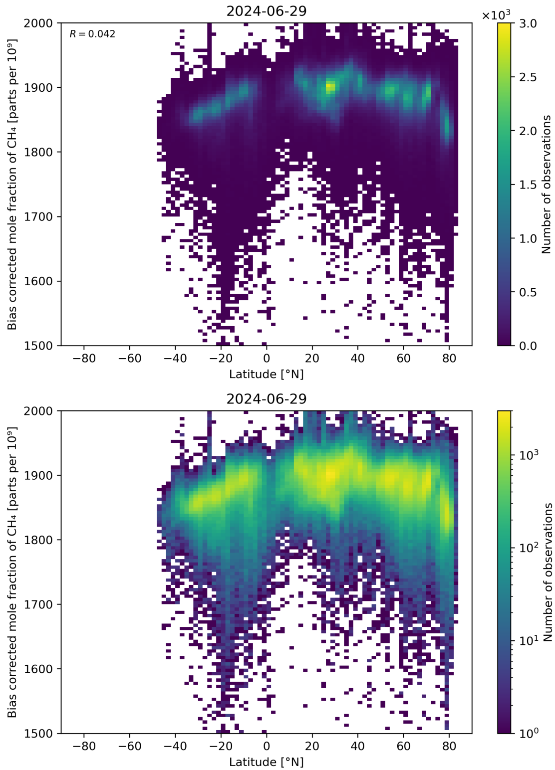
Figure 58: Scatter density plot of “Latitude” against “Bias corrected mole fraction of CH 4 ” for 2024-06-29 to 2024-06-30.
