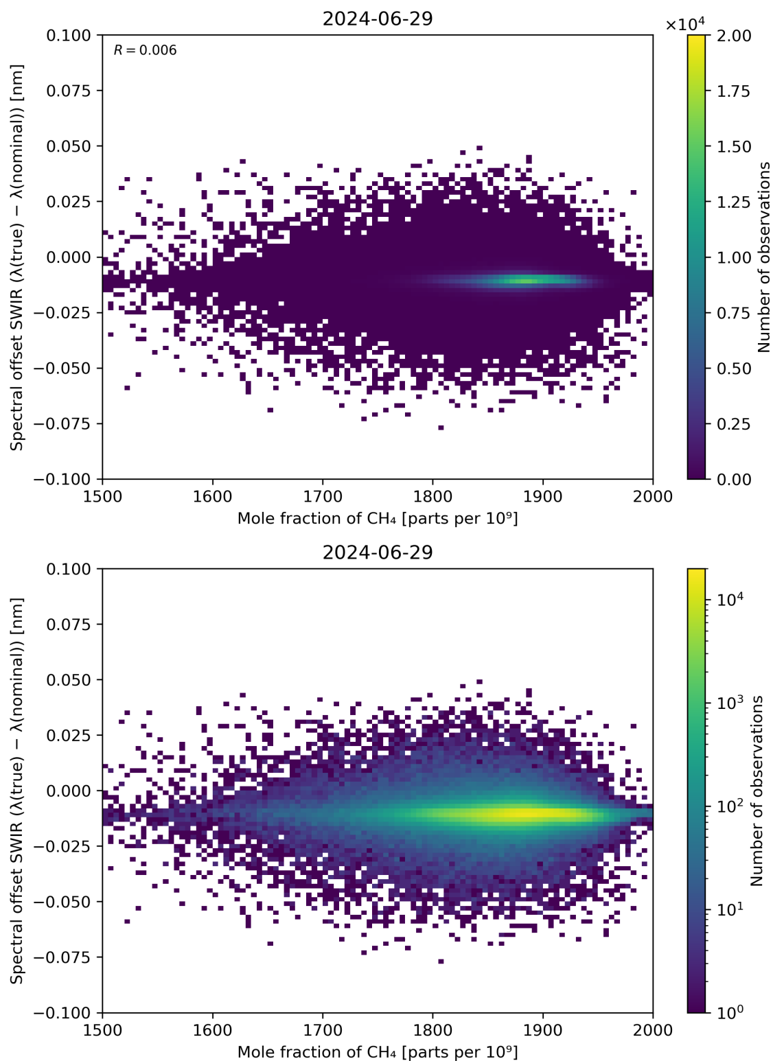
Figure 86: Scatter density plot of “Mole fraction of CH 4 ” against “Spectral offset SWIR ( \lambda(\text{true}) - \lambda(\text{nominal}) )” for 2024-06-29 to 2024-06-30.
