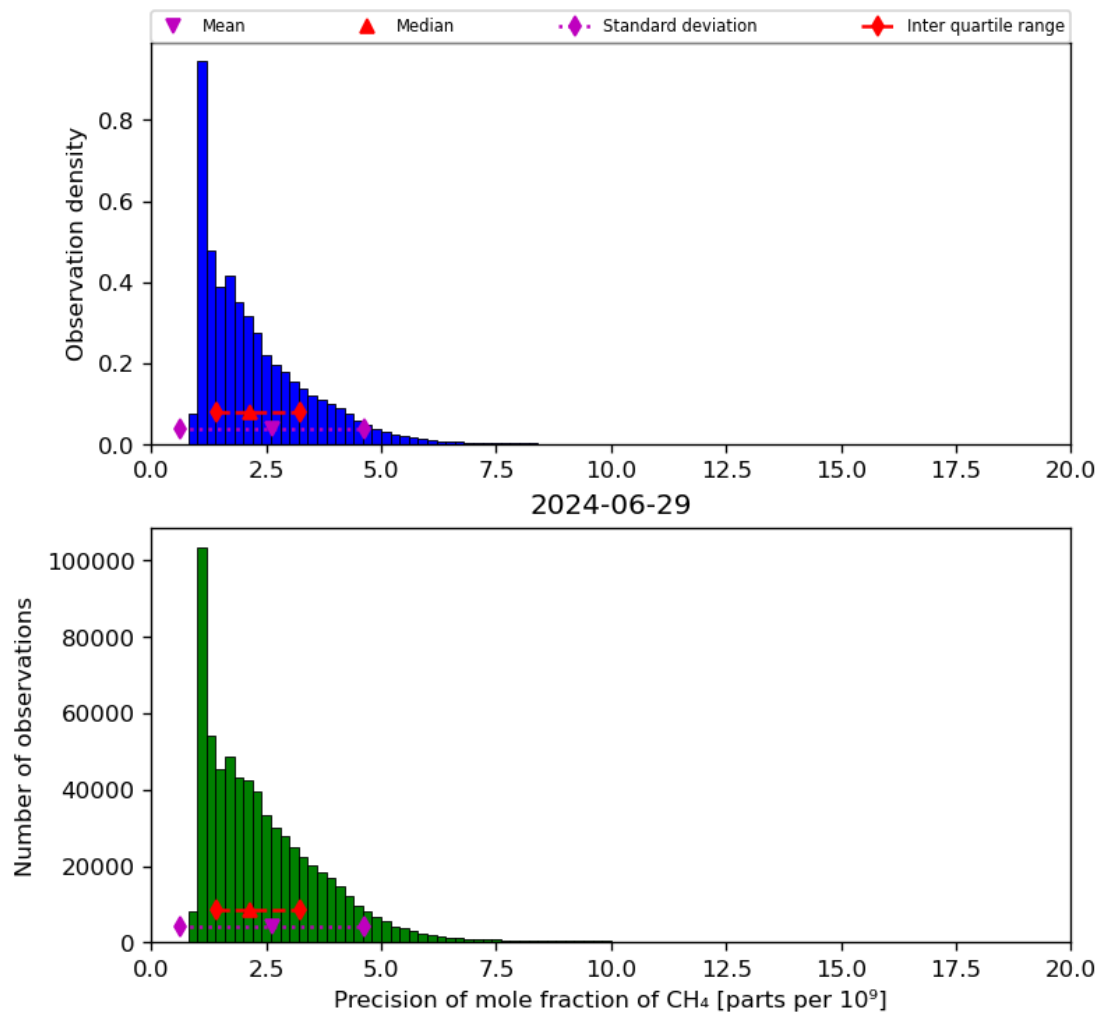
Figure 24: Histogram of “Precision of mole fraction of CH 4 ” for 2024-06-29 to 2024-06-30
