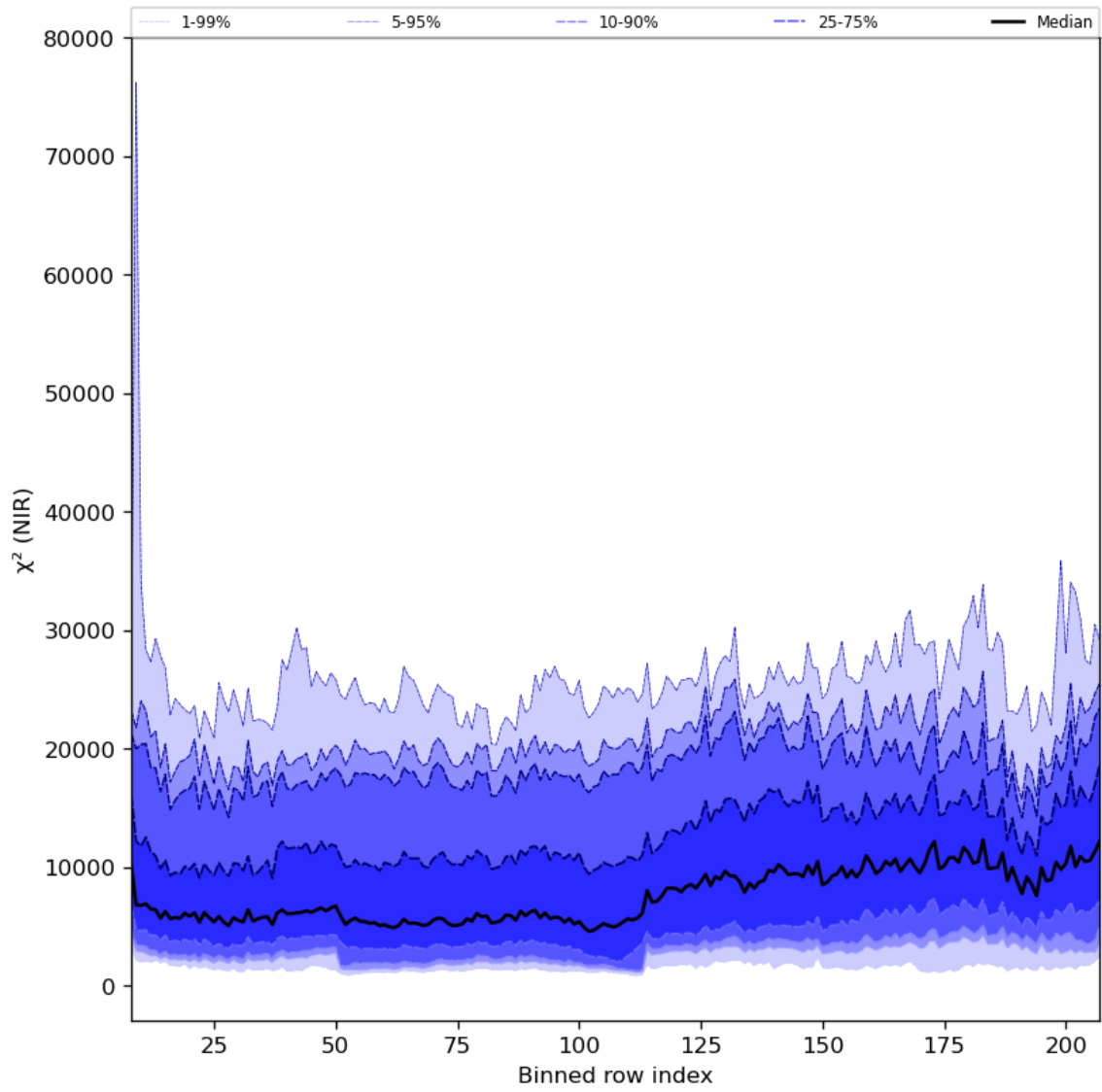
Figure 40: Along track statistics of “ \chi^2 (NIR)” for 2024-06-29 to 2024-06-30
