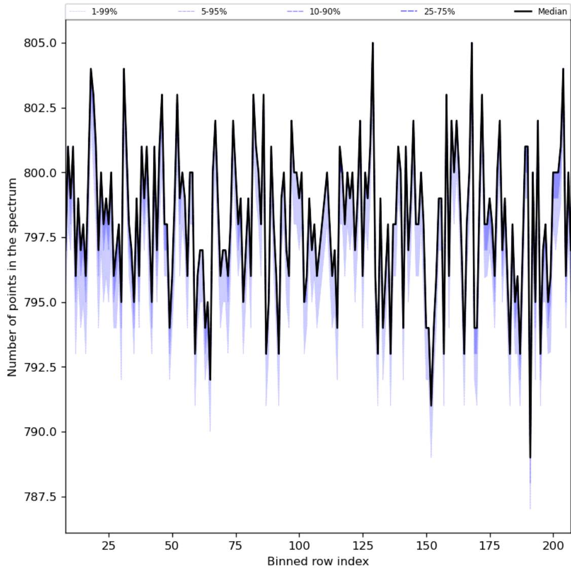
Figure 37: Along track statistics of “Number of points in the spectrum” for 2024-06-29 to 2024-06-30
