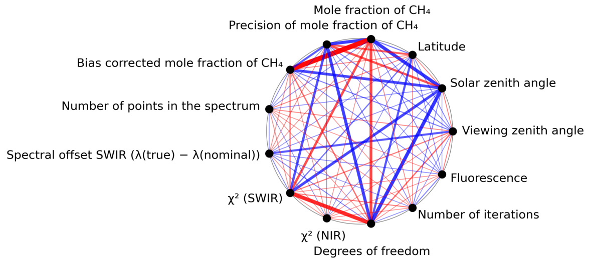
Figure 1: Map of correlation graph for 2024-06-29 to 2024-06-30.
