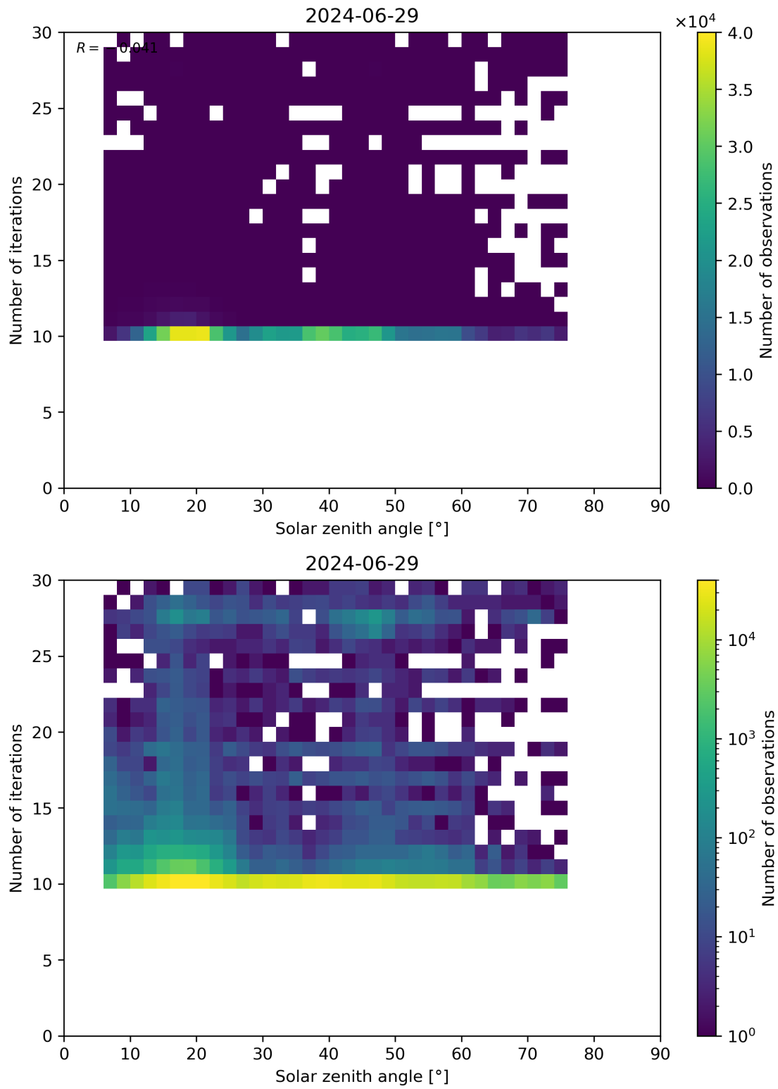
Figure 102: Scatter density plot of “Solar zenith angle” against “Number of iterations” for 2024-06-29 to 2024-06-30.
