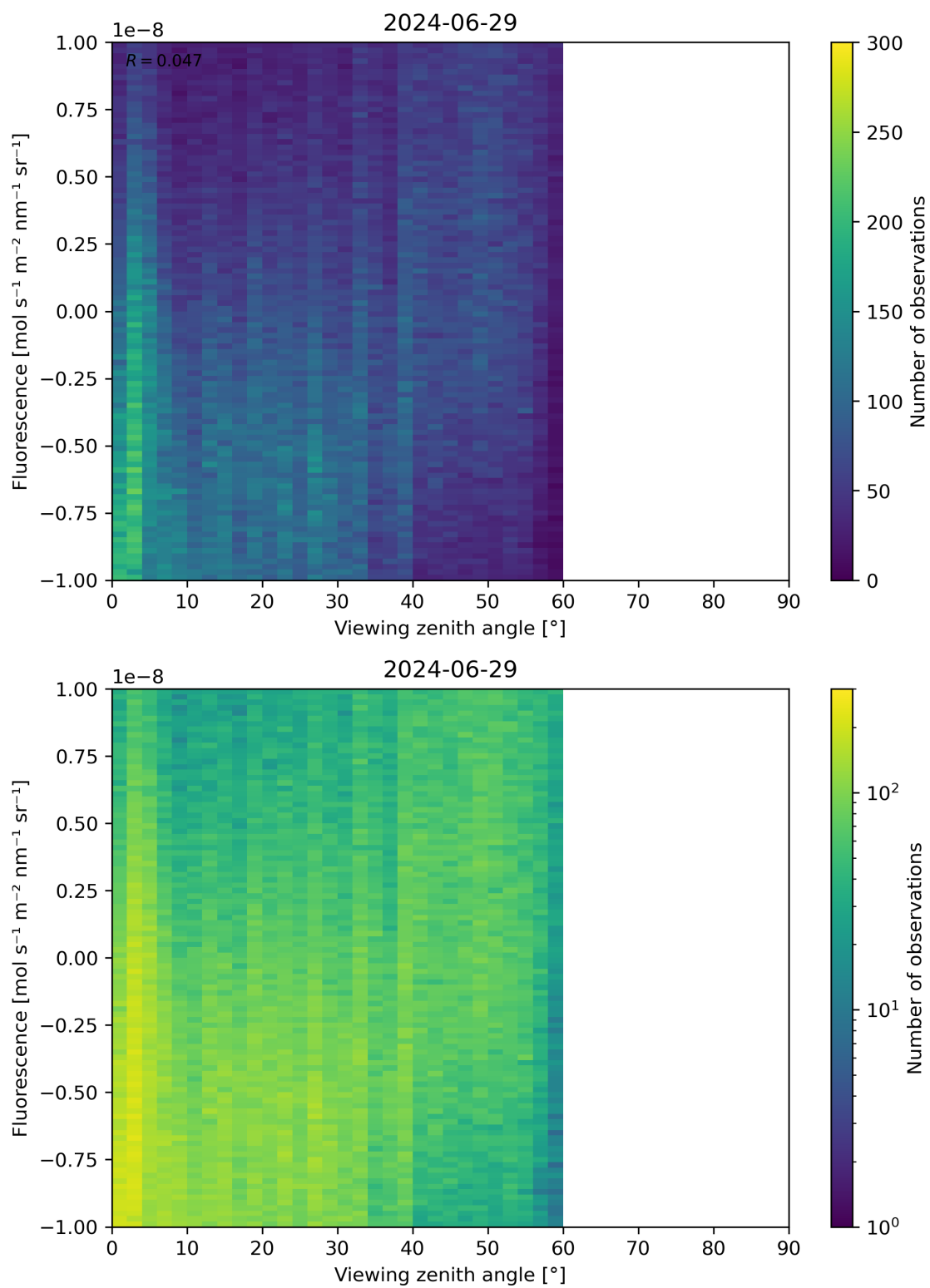
Figure 108: Scatter density plot of “Viewing zenith angle” against “Fluorescence” for 2024-06-29 to 2024-06-30.
