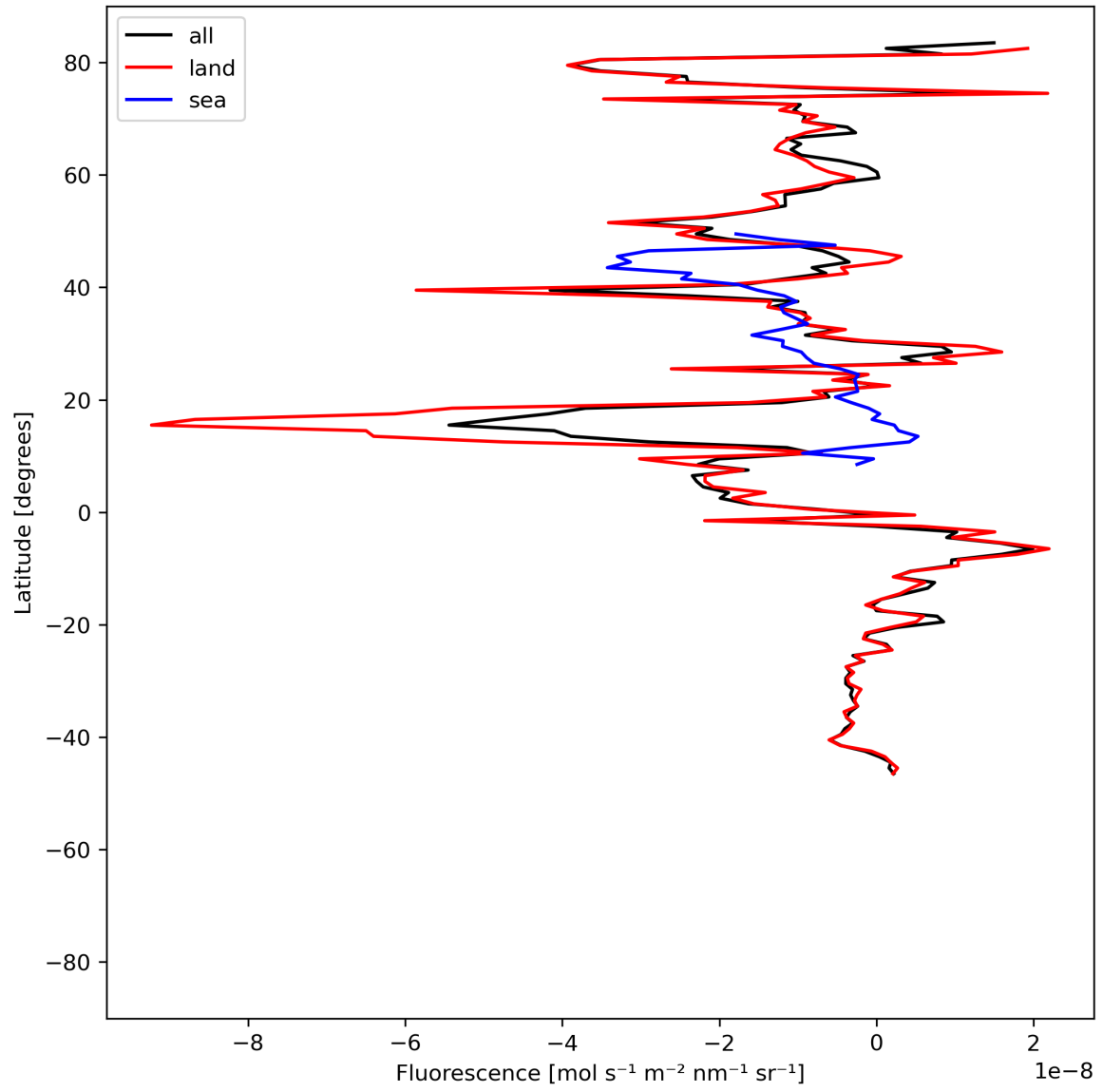
Figure 21: Zonal average of “Fluorescence” for 2024-06-29 to 2024-06-30.
