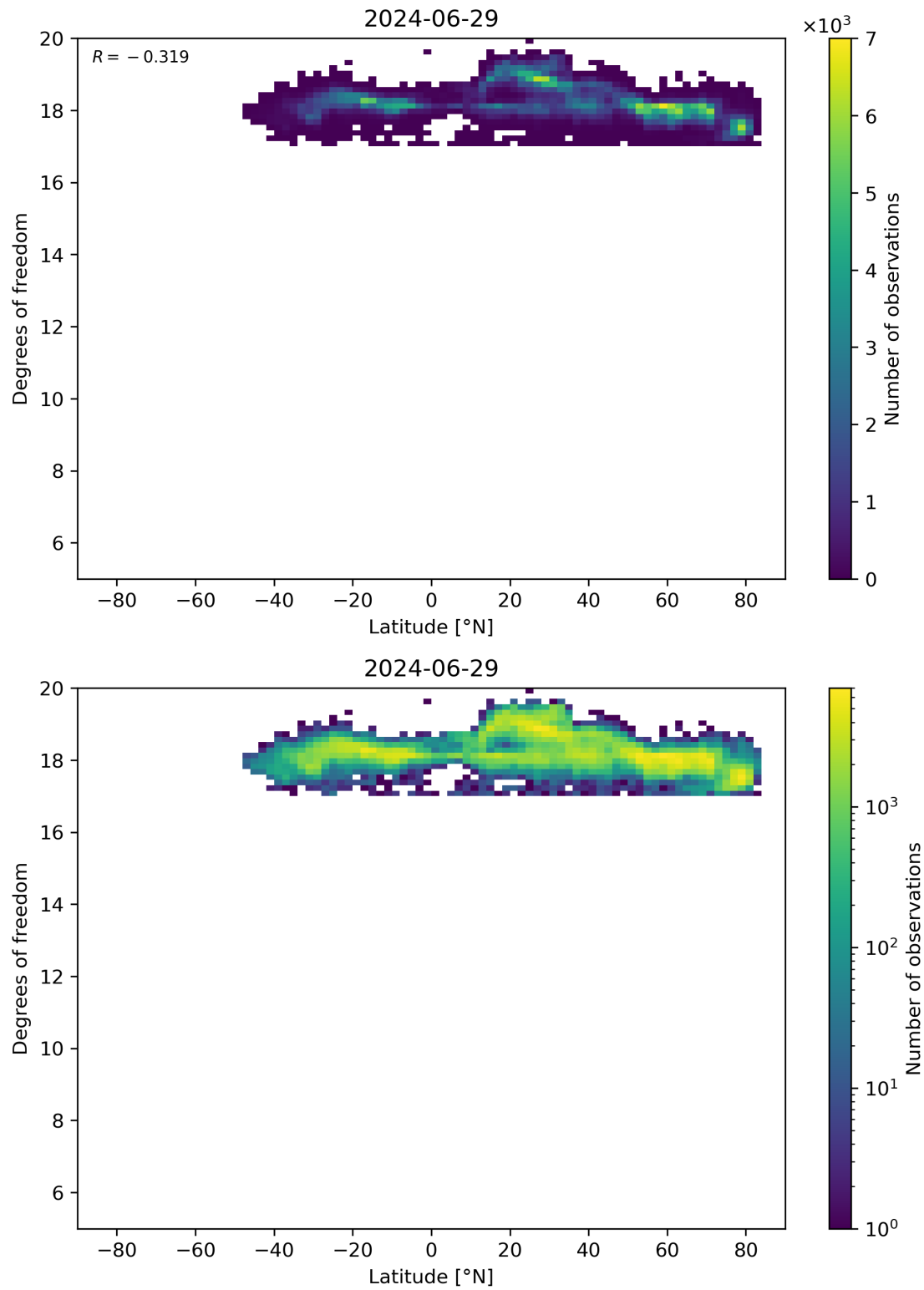
Figure 55: Scatter density plot of “Latitude” against “Degrees of freedom” for 2024-06-29 to 2024-06-30.
