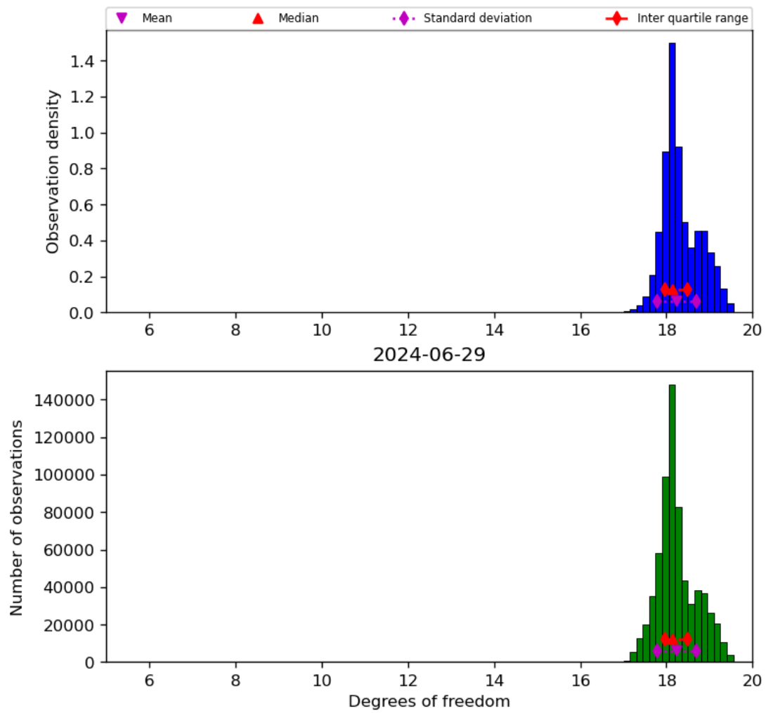
Figure 30: Histogram of “Degrees of freedom” for 2024-06-29 to 2024-06-30
