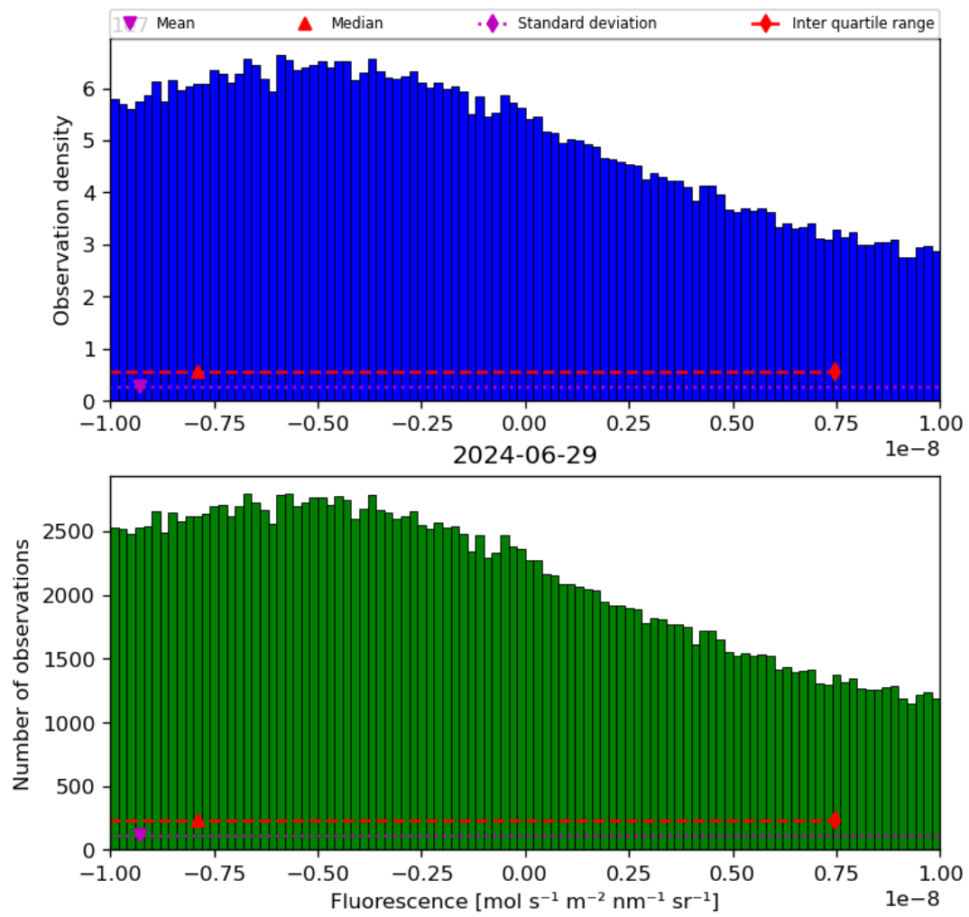
Figure 32: Histogram of “Fluorescence” for 2024-06-29 to 2024-06-30
