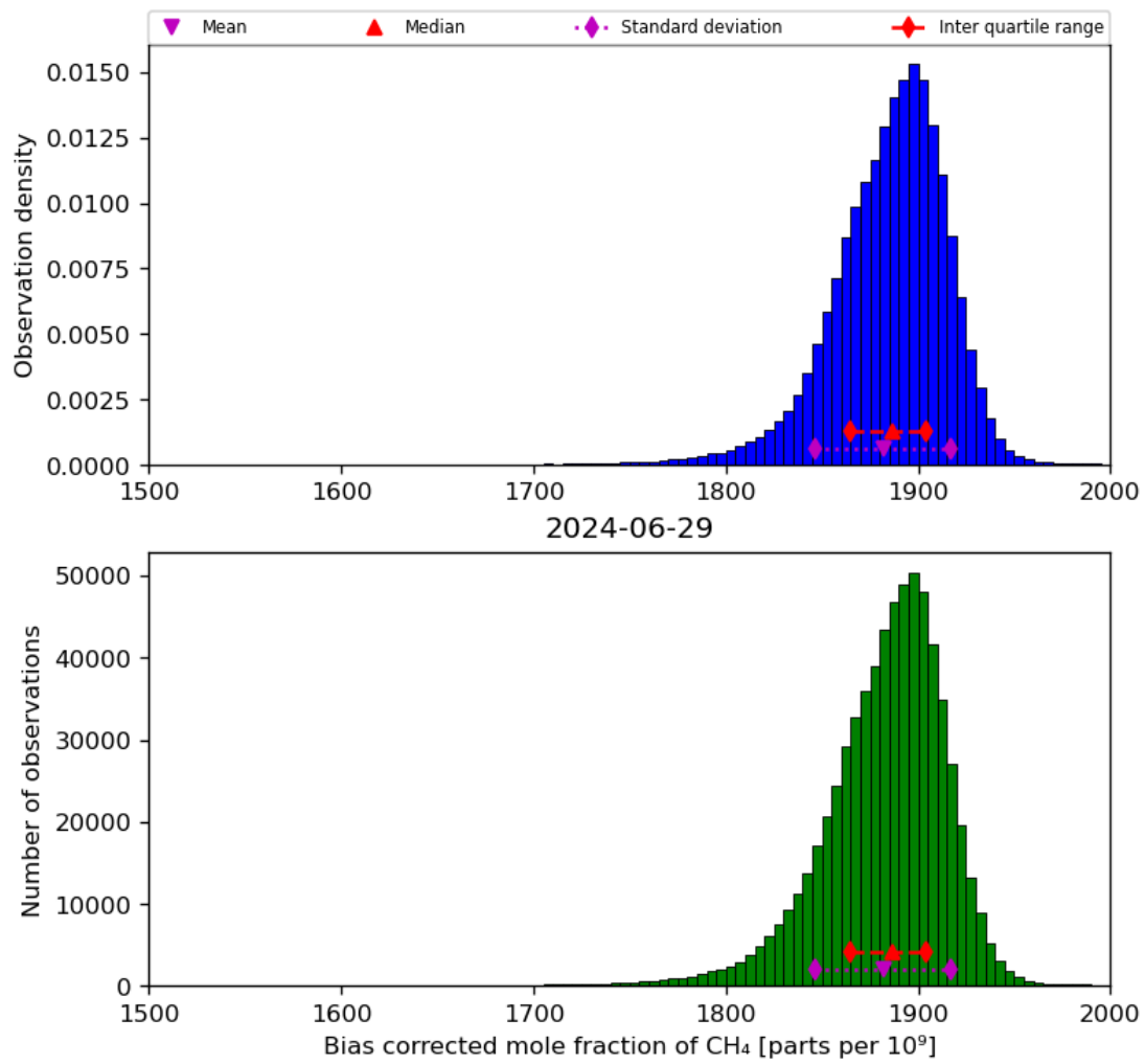
Figure 25: Histogram of “Bias corrected mole fraction of CH 4 ” for 2024-06-29 to 2024-06-30
