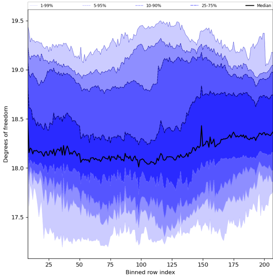
Figure 41: Along track statistics of “Degrees of freedom” for 2024-06-29 to 2024-06-30
