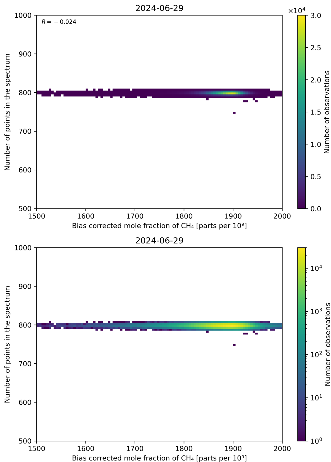
Figure 68: Scatter density plot of “Bias corrected mole fraction of CH 4 ” against “Number of points in the spectrum” for 2024-06-29 to 2024-06-30.
