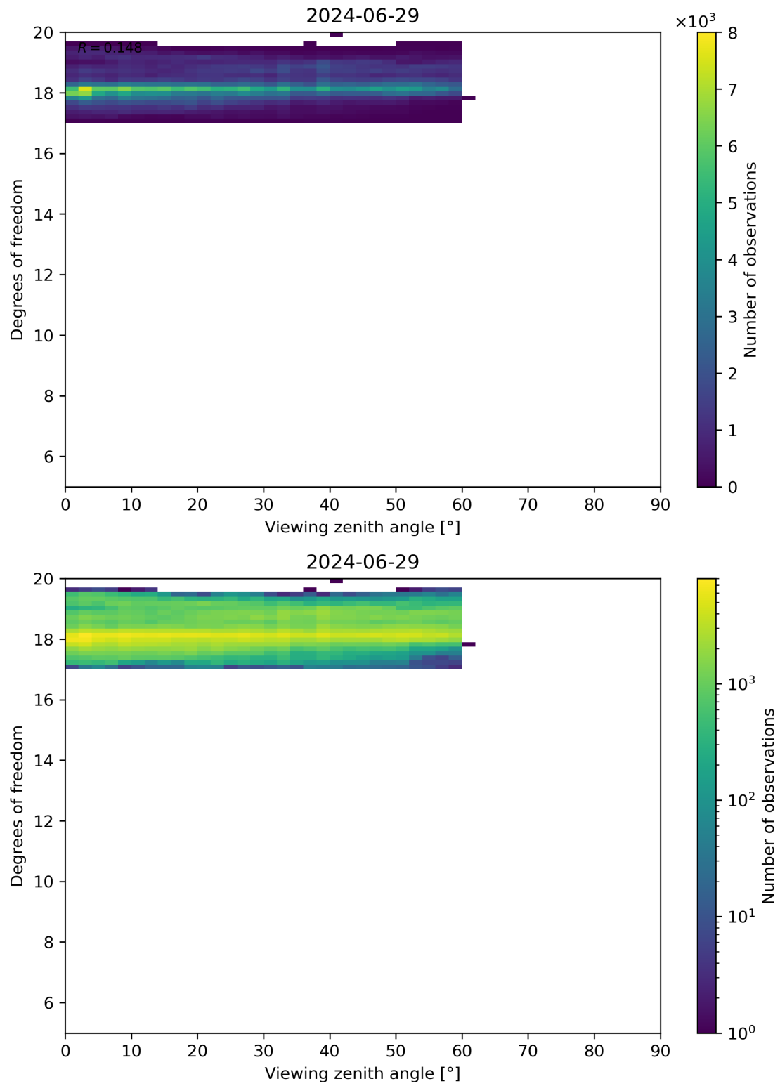
Figure 107: Scatter density plot of “Viewing zenith angle” against “Degrees of freedom” for 2024-06-29 to 2024-06-30.
