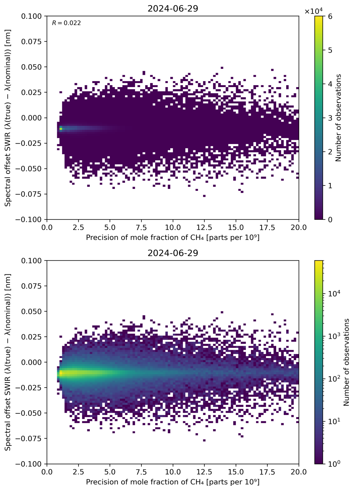
Figure 85: Scatter density plot of “Precision of mole fraction of \text{CH}_4 ” against “Spectral offset SWIR ( \lambda(\text{true}) - \lambda(\text{nominal}) )” for 2024-06-29 to 2024-06-30.
