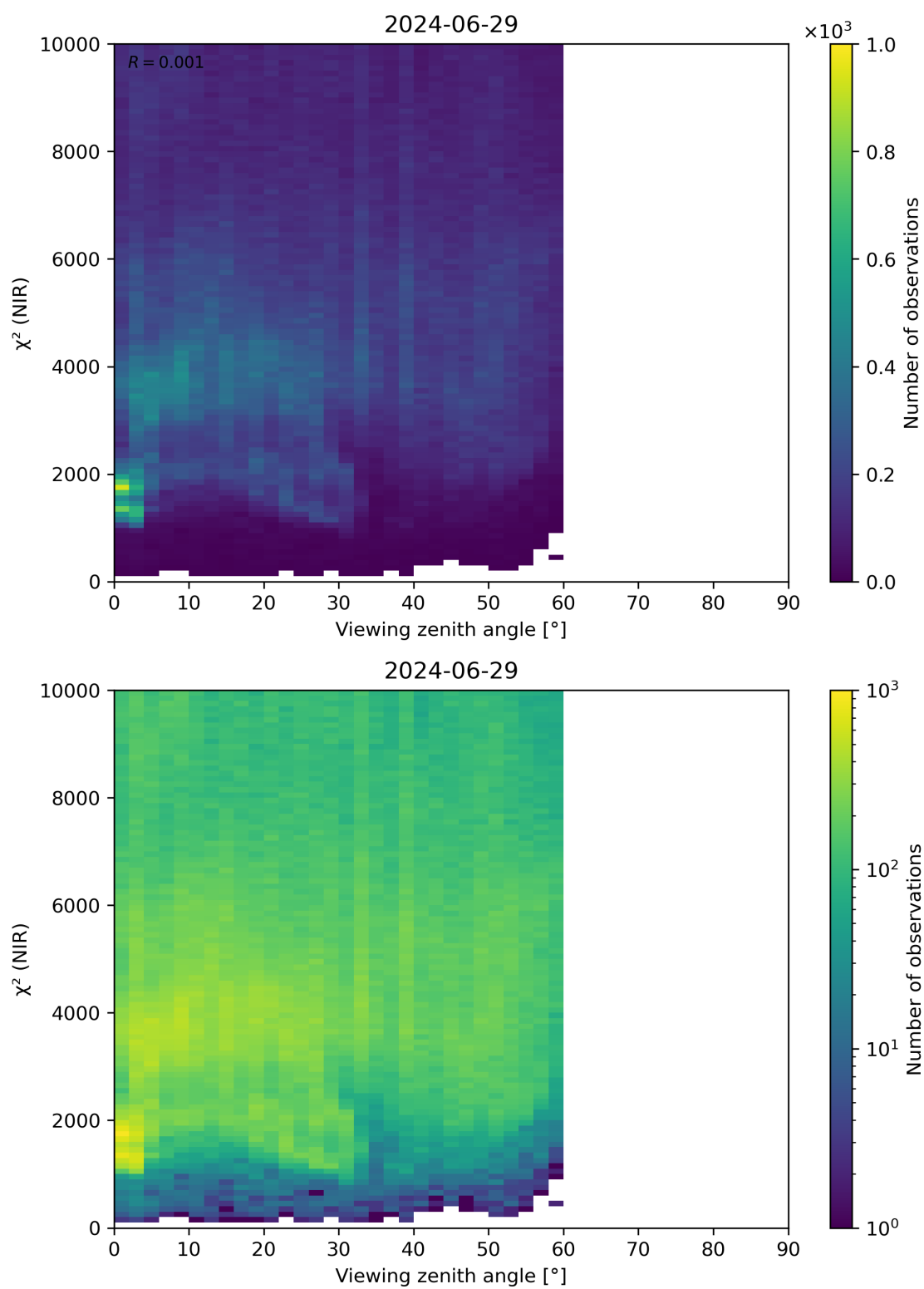
Figure 105: Scatter density plot of “Viewing zenith angle” against “ \chi^2 (NIR)” for 2024-06-29 to 2024-06-30.
