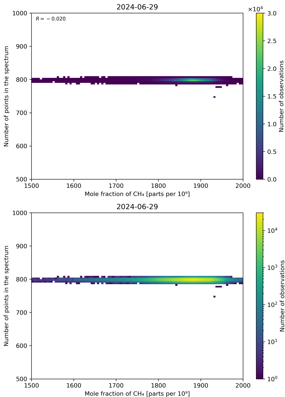
Figure 77: Scatter density plot of “Mole fraction of CH 4 ” against “Number of points in the spectrum” for 2024-06-29 to 2024-06-30.
