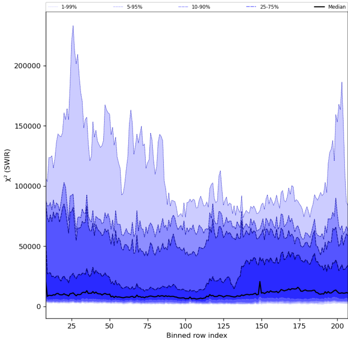
Figure 39: Along track statistics of " \chi^2 (SWIR)" for 2024-06-29 to 2024-06-30
