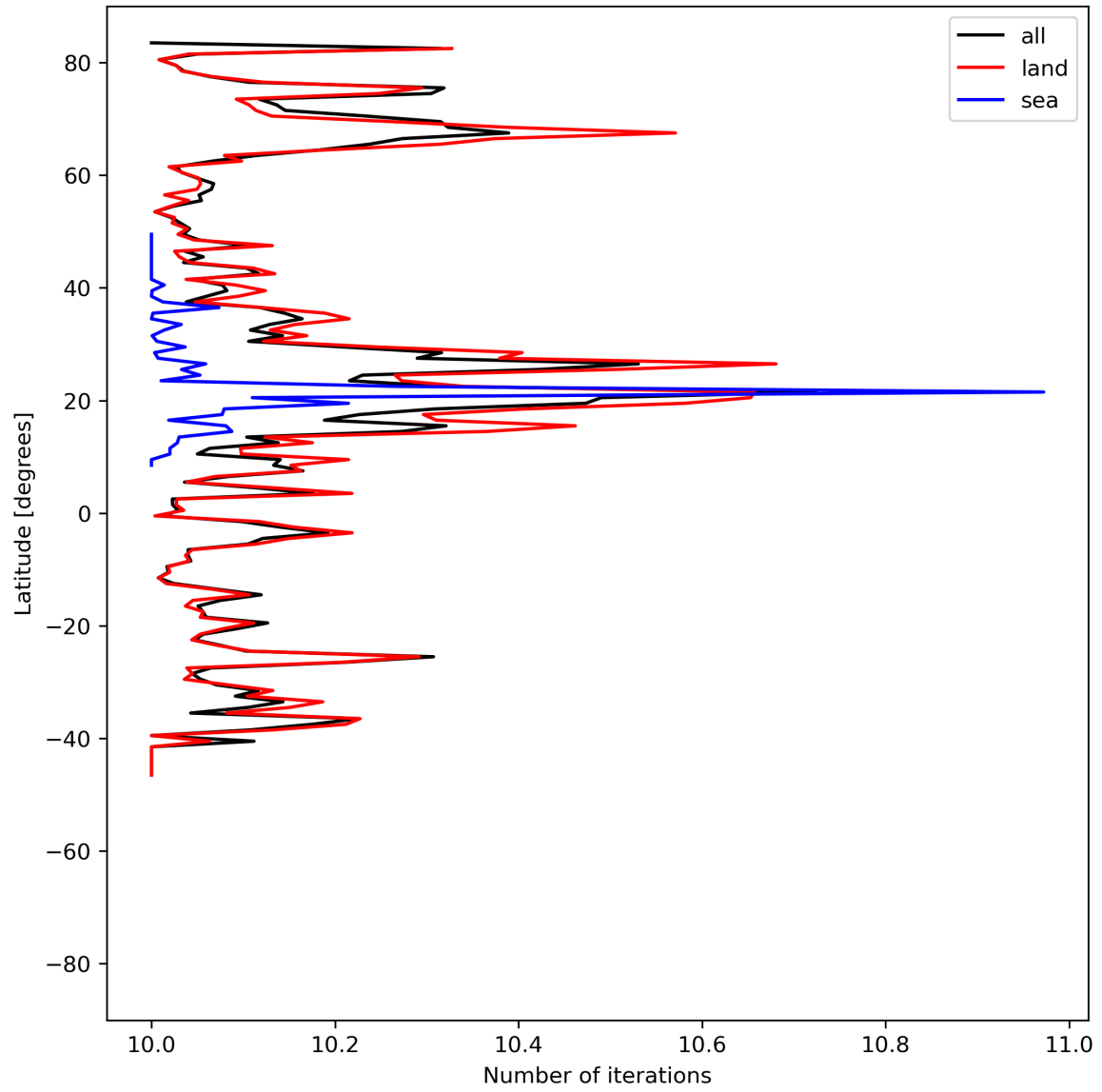
Figure 20: Zonal average of “Number of iterations” for 2024-06-29 to 2024-06-30.
