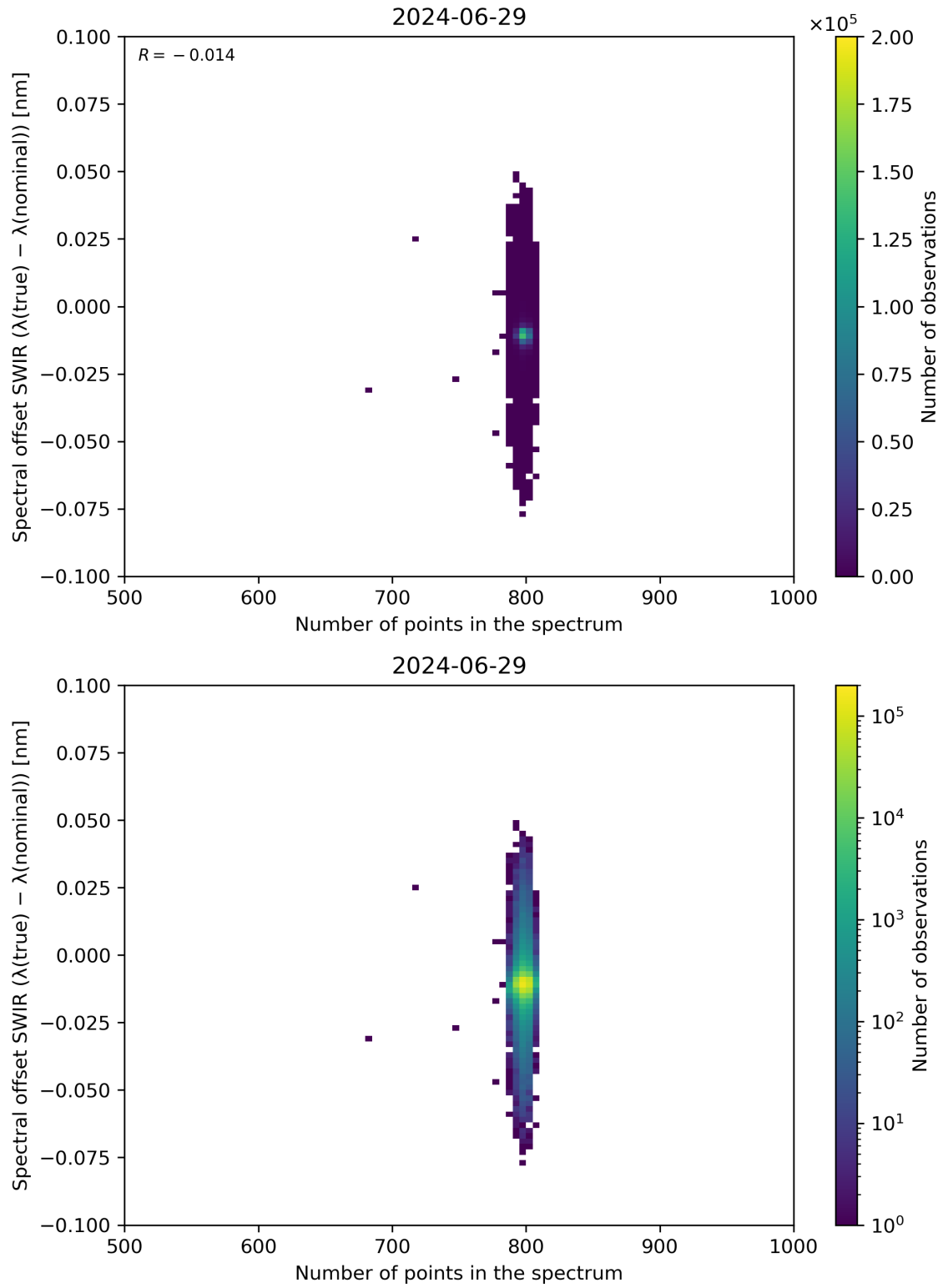
Figure 93: Scatter density plot of “Number of points in the spectrum” against “Spectral offset SWIR ( \lambda(\text{true}) - \lambda(\text{nominal}) )” for 2024-06-29 to 2024-06-30.
