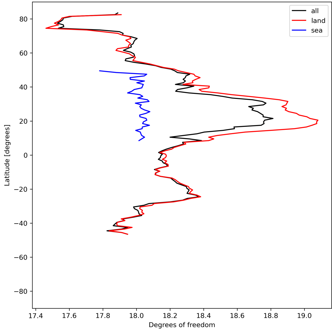
Figure 19: Zonal average of “Degrees of freedom” for 2024-06-29 to 2024-06-30.
