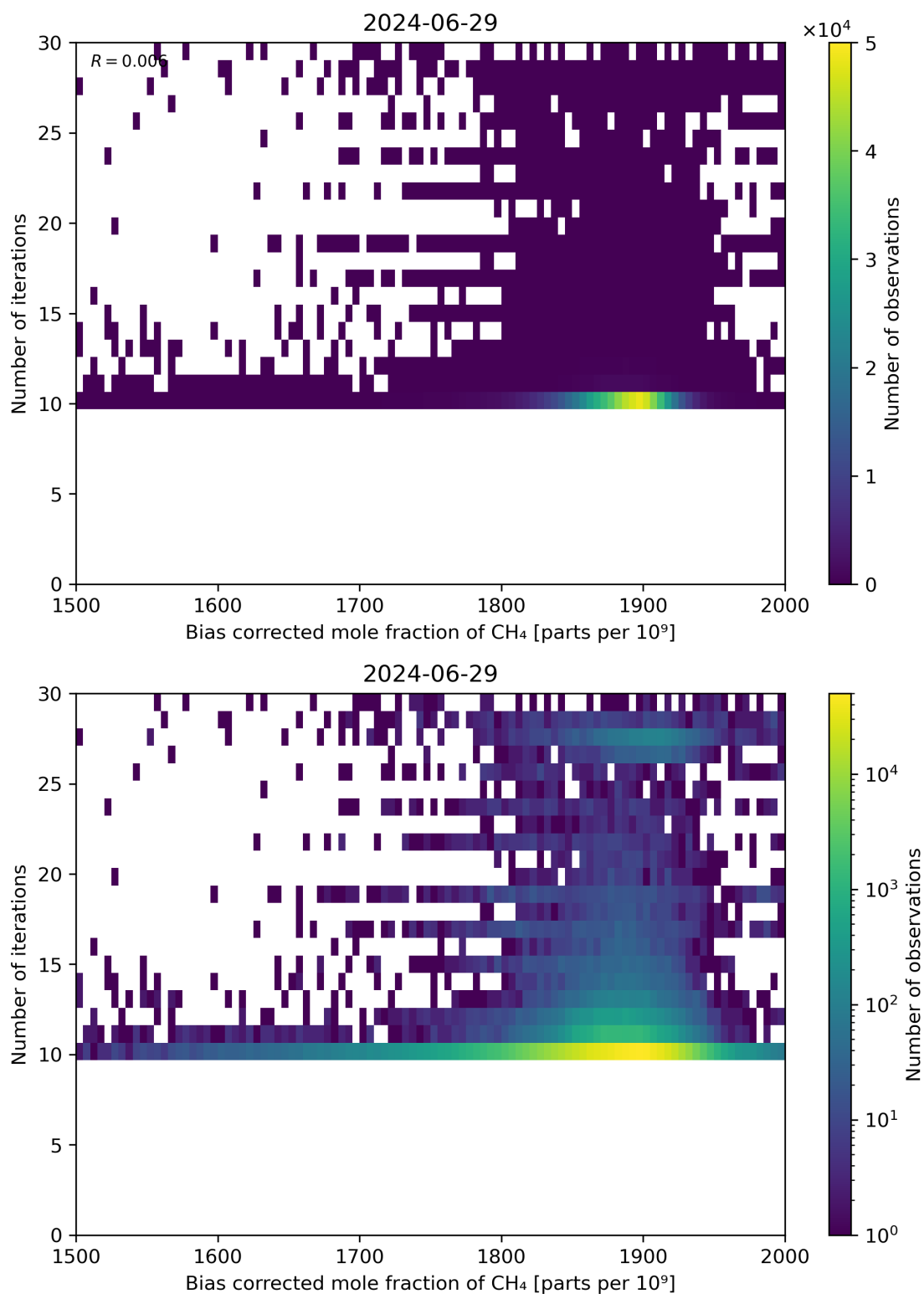
Figure 67: Scatter density plot of “Bias corrected mole fraction of \text{CH}_4 ” against “Number of iterations” for 2024-06-29 to 2024-06-30.
