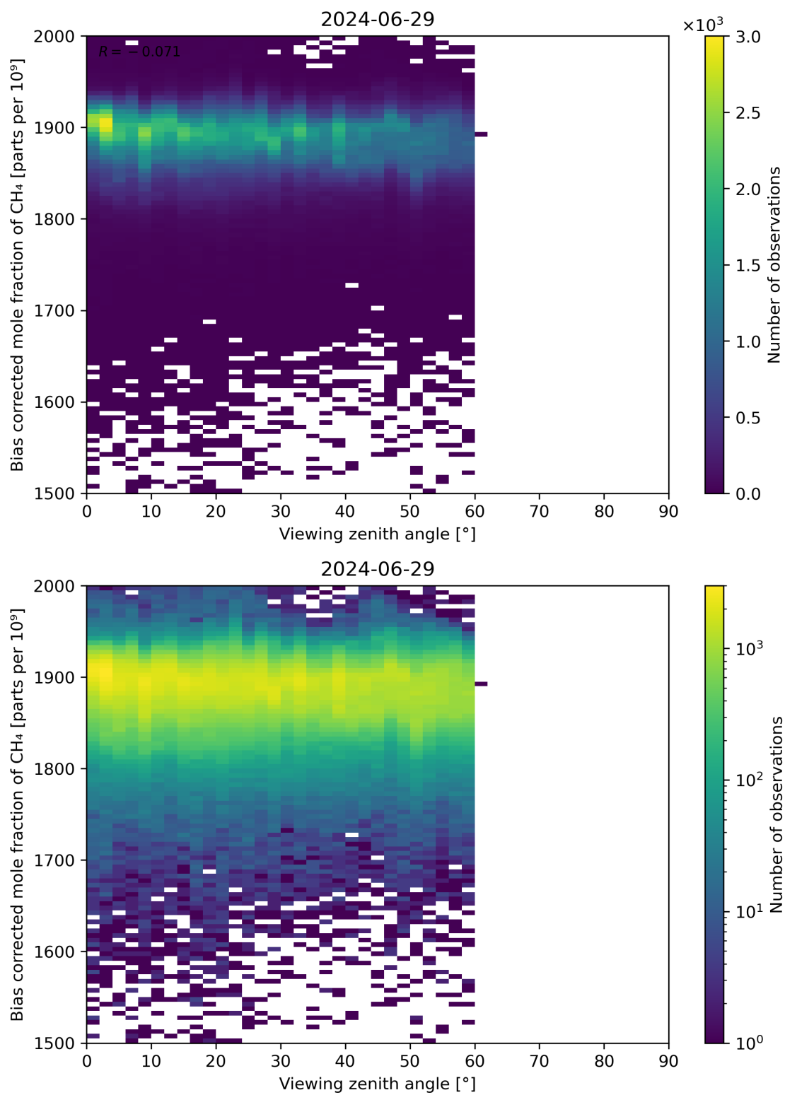
Figure 111: Scatter density plot of “Viewing zenith angle” against “Bias corrected mole fraction of CH 4 ” for 2024-06-29 to 2024-06-30.
