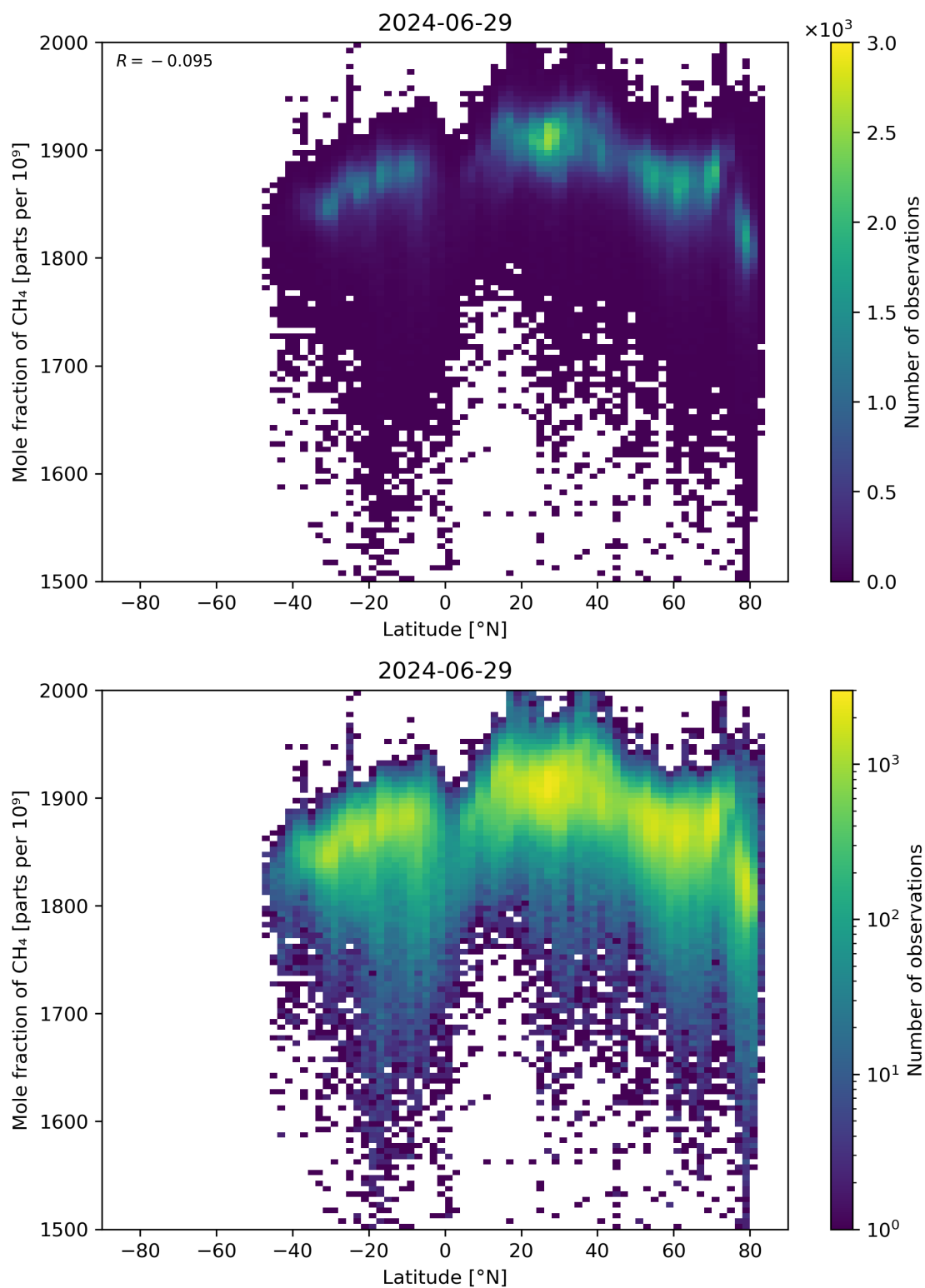
Figure 57: Scatter density plot of “Latitude” against “Mole fraction of \text{CH}_4 ” for 2024-06-29 to 2024-06-30.
