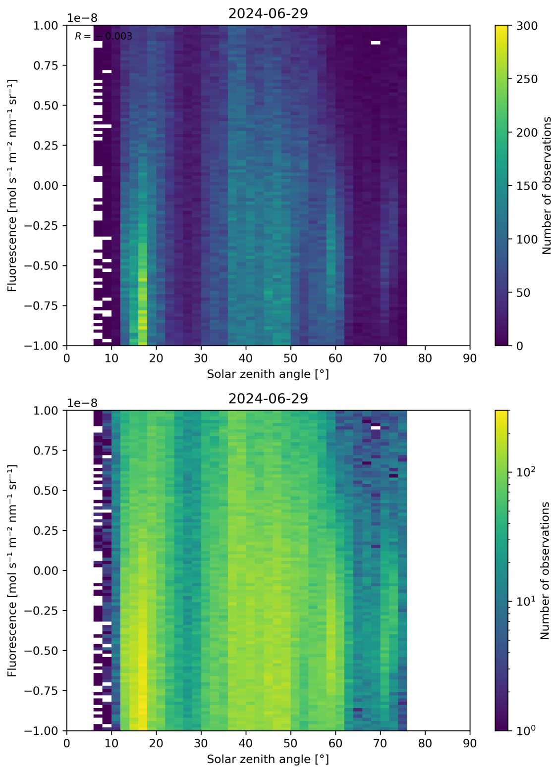
Figure 97: Scatter density plot of “Solar zenith angle” against “Fluorescence” for 2024-06-29 to 2024-06-30.
