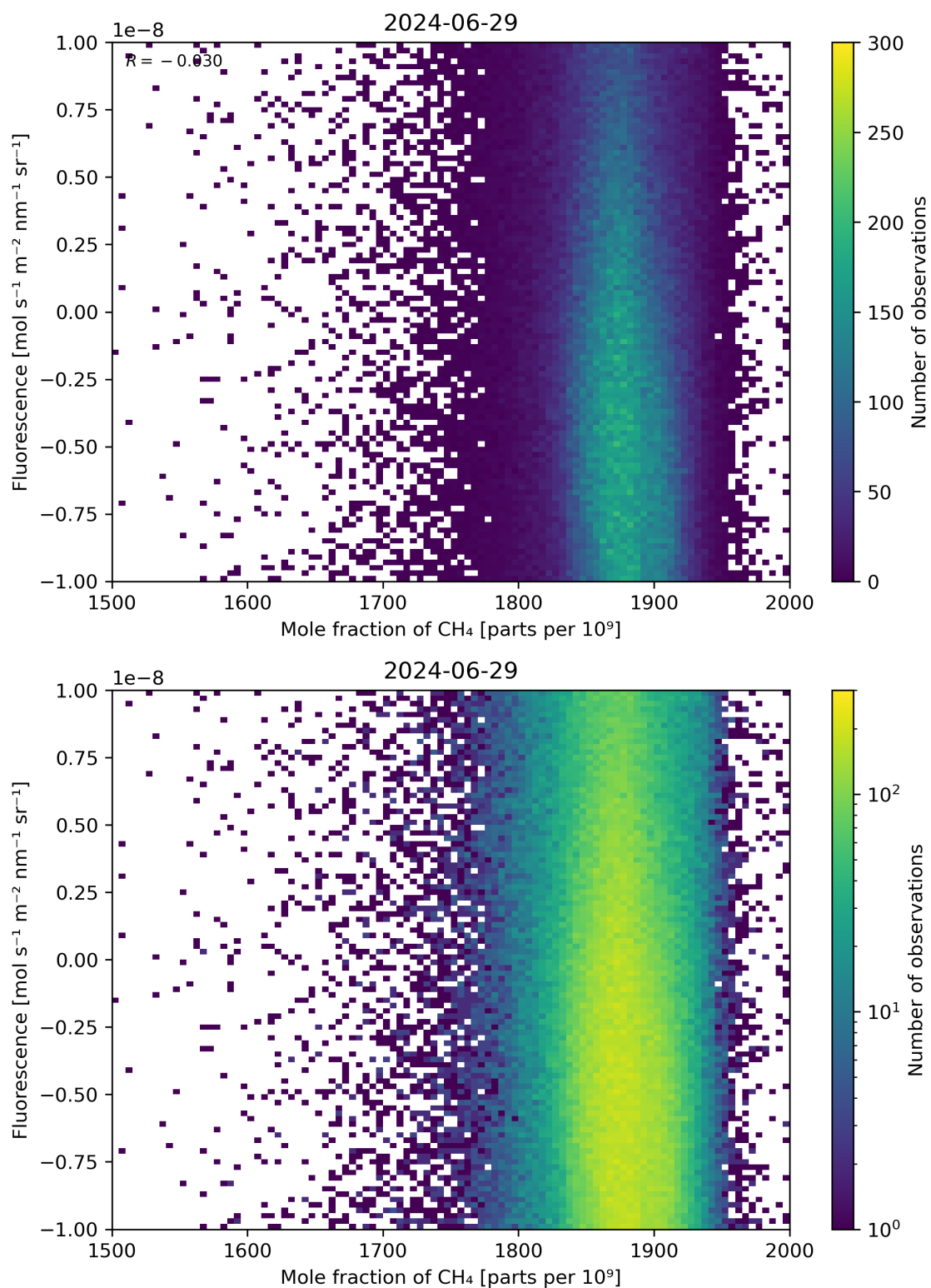
Figure 73: Scatter density plot of “Mole fraction of \text{CH}_4 ” against “Fluorescence” for 2024-06-29 to 2024-06-30.
