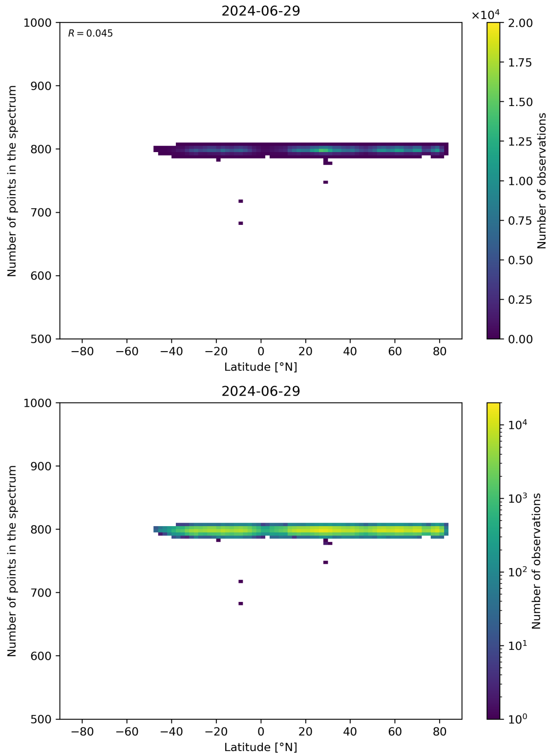
Figure 61: Scatter density plot of “Latitude” against “Number of points in the spectrum” for 2024-06-29 to 2024-06-30.
