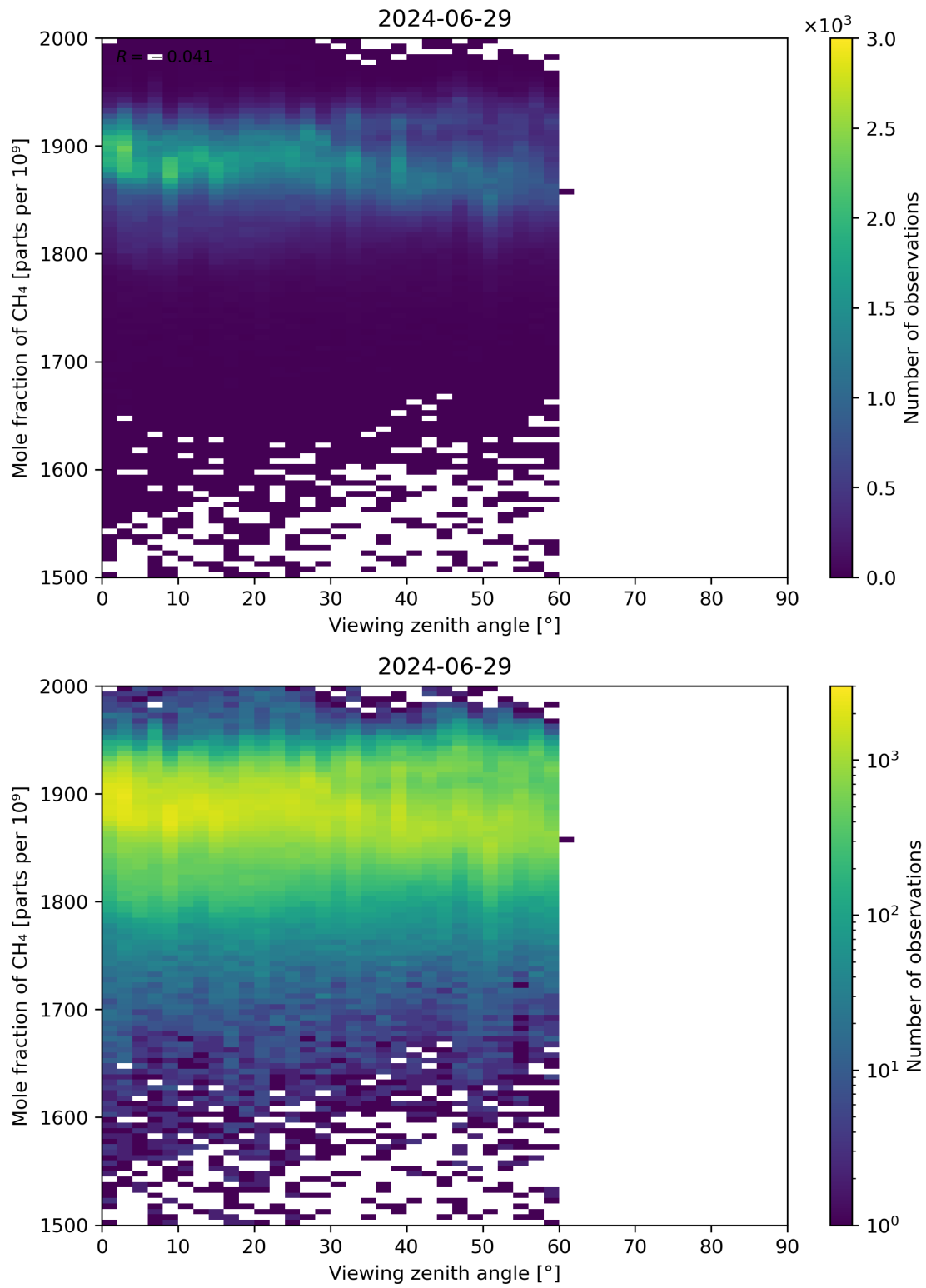
Figure 110: Scatter density plot of “Viewing zenith angle” against “Mole fraction of CH 4 ” for 2024-06-29 to 2024-06-30.
