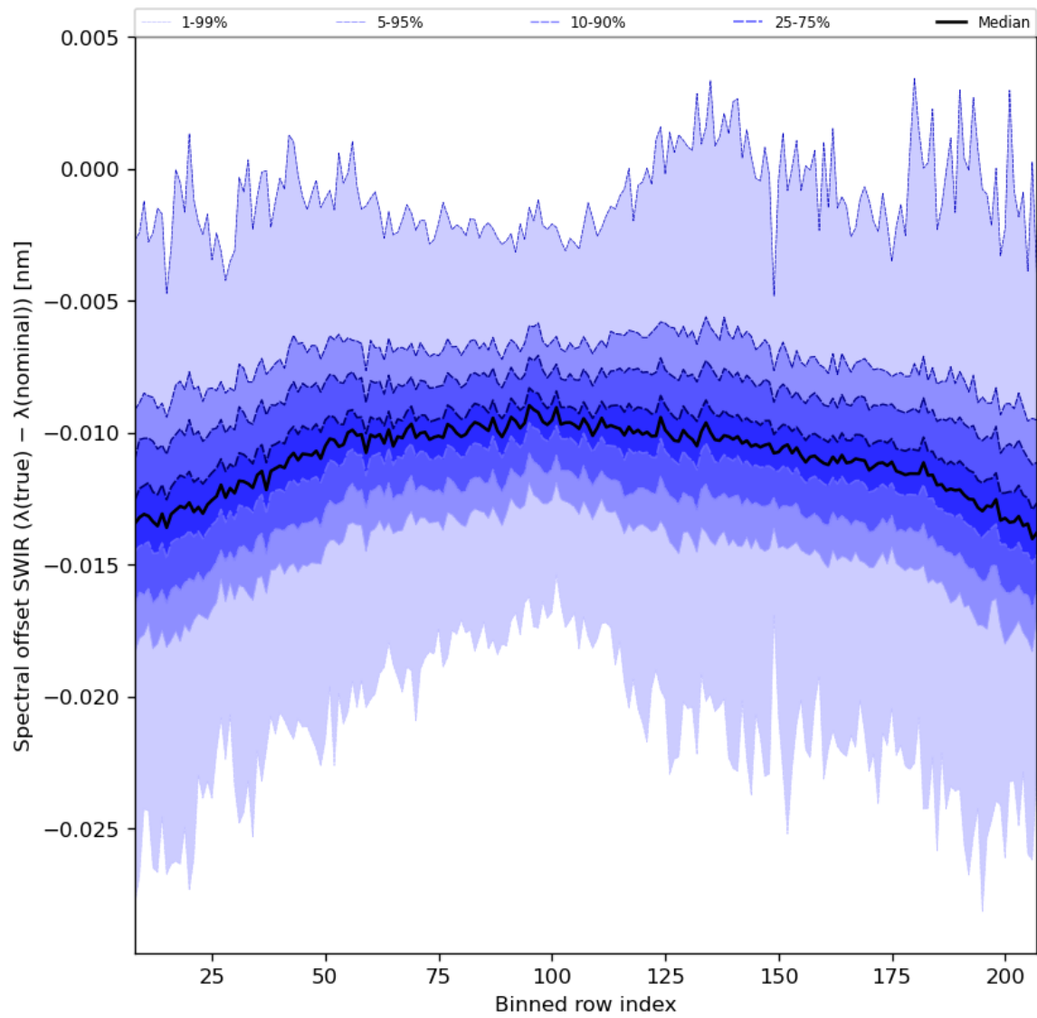
Figure 38: Along track statistics of “Spectral offset SWIR ( \lambda(\text{true}) - \lambda(\text{nominal}) )” for 2024-06-29 to 2024-06-30
