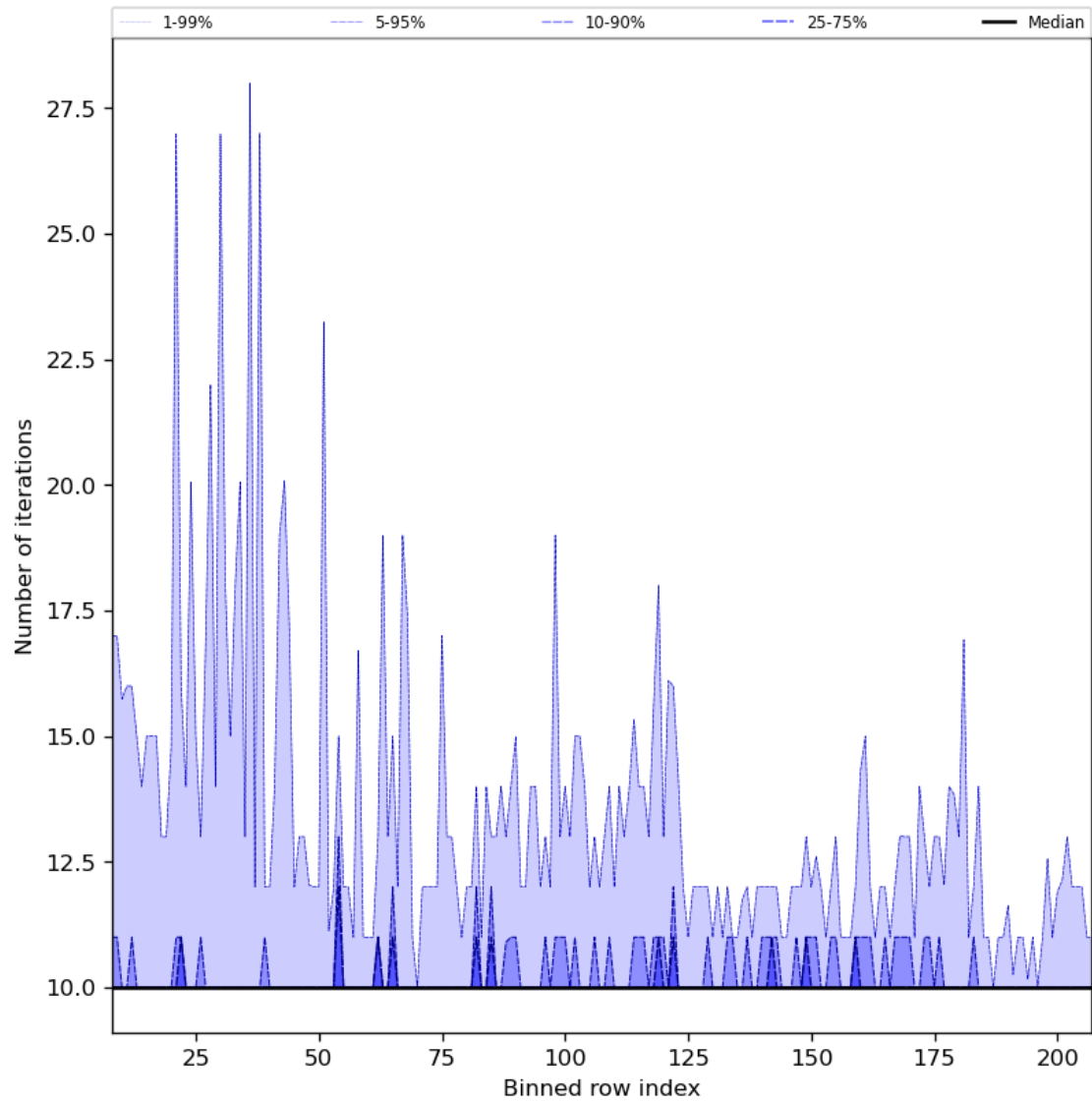
Figure 42: Along track statistics of “Number of iterations” for 2024-06-29 to 2024-06-30
