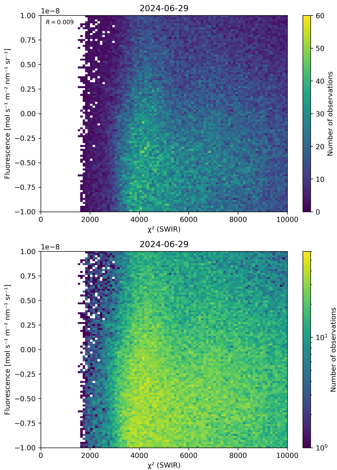
Figure 49: Scatter density plot of “ \chi^2 (SWIR)” against “Fluorescence” for 2024-06-29 to 2024-06-30.
