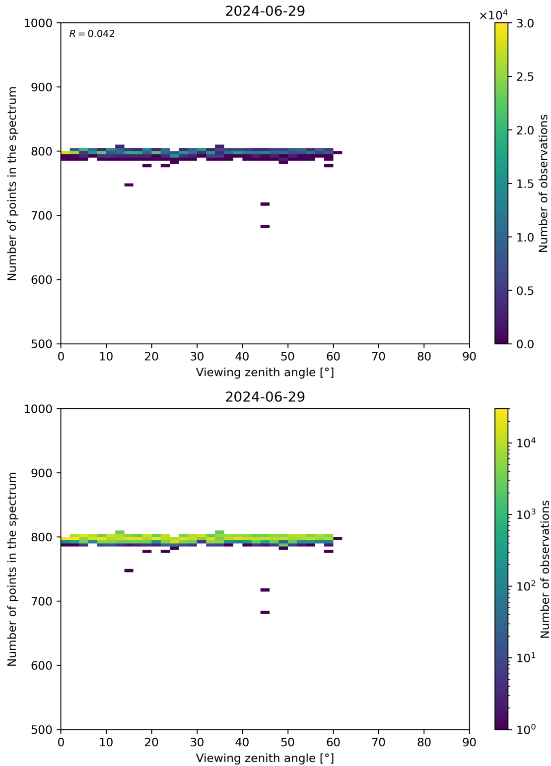
Figure 114: Scatter density plot of “Viewing zenith angle” against “Number of points in the spectrum” for 2024-06-29 to 2024-06-30.
