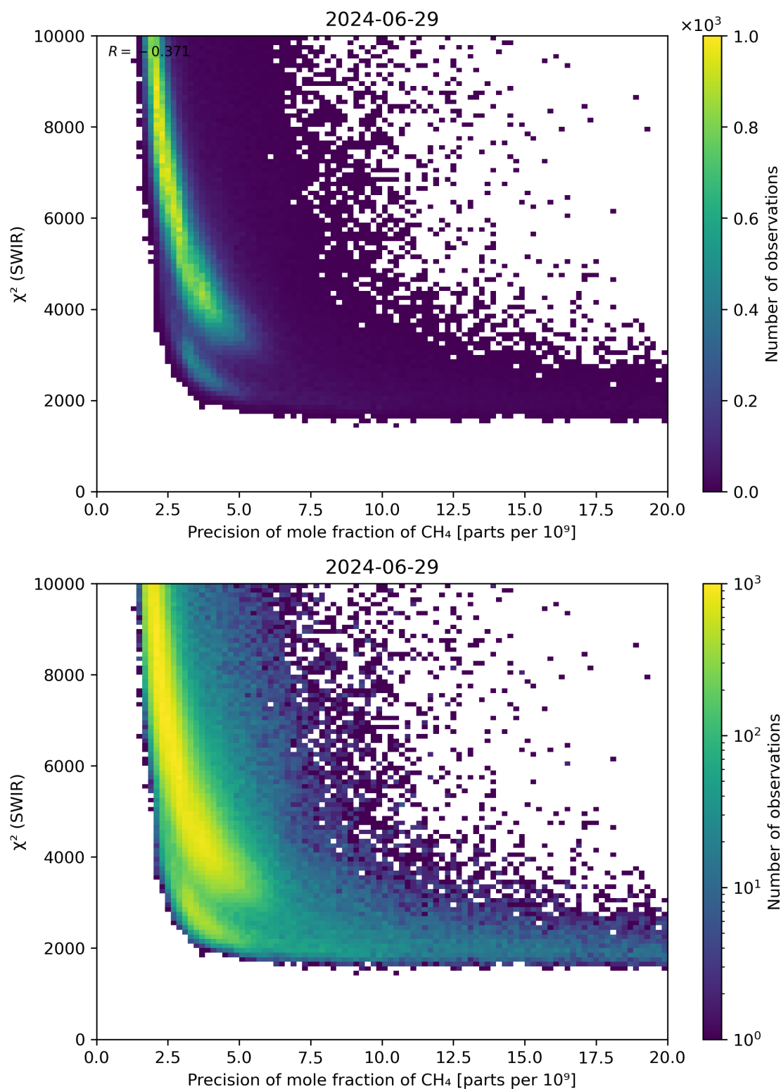
Figure 79: Scatter density plot of “Precision of mole fraction of CH 4 ” against “ \chi^2 (SWIR)” for 2024-06-29 to 2024-06-30.
