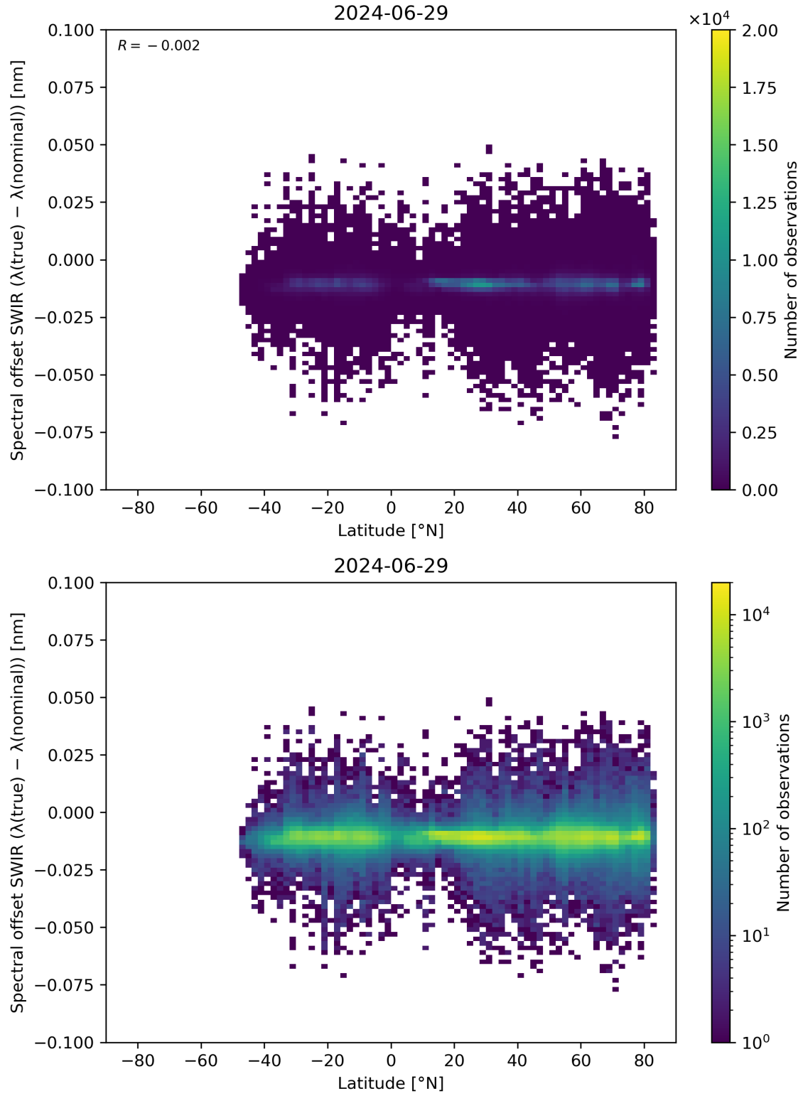
Figure 62: Scatter density plot of “Latitude” against “Spectral offset SWIR ( \lambda(\text{true}) - \lambda(\text{nominal}) )” for 2024-06-29 to 2024-06-30.
