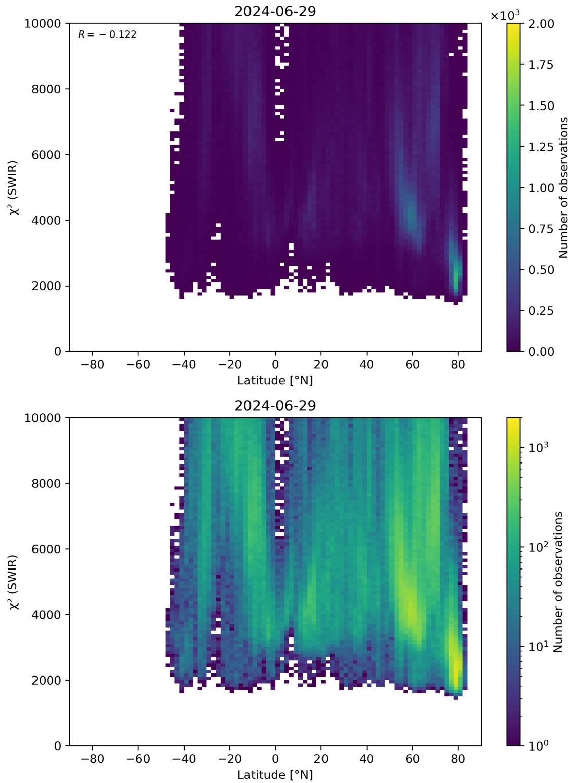
Figure 54: Scatter density plot of “Latitude” against “ \chi^2 (SWIR)” for 2024-06-29 to 2024-06-30.
