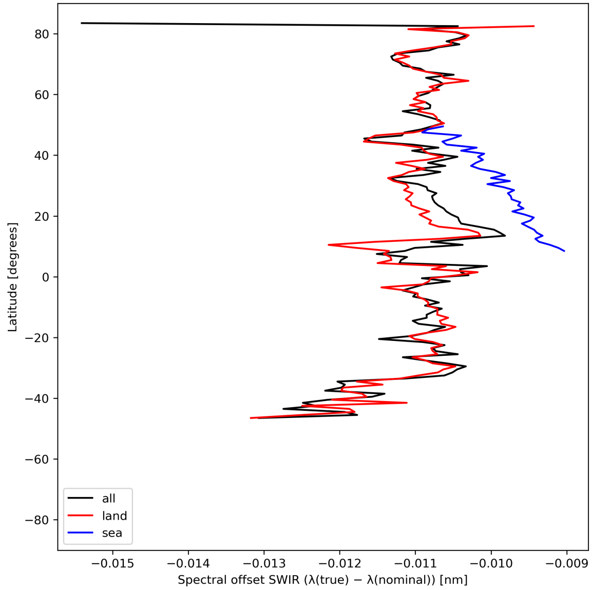
Figure 16: Zonal average of “Spectral offset SWIR ( \lambda(\text{true}) - \lambda(\text{nominal}) )” for 2024-06-29 to 2024-06-30.
