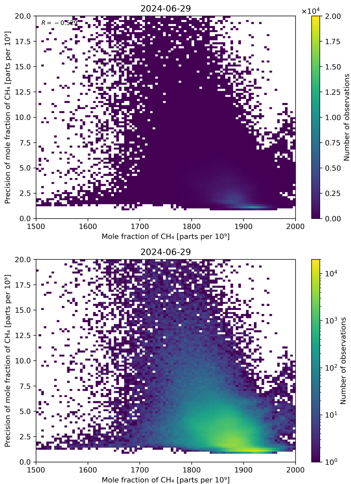
Figure 75: Scatter density plot of “Mole fraction of CH 4 ” against “Precision of mole fraction of CH 4 ” for 2024-06-29 to 2024-06-30.
