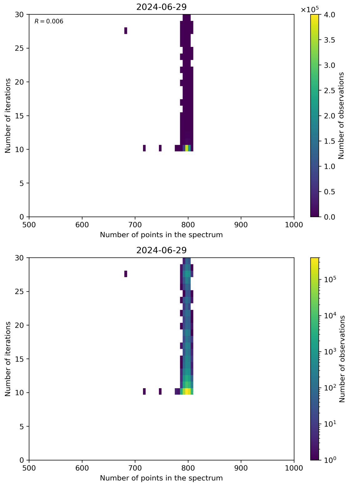
Figure 92: Scatter density plot of “Number of points in the spectrum” against “Number of iterations” for 2024-06-29 to 2024-06-30.
