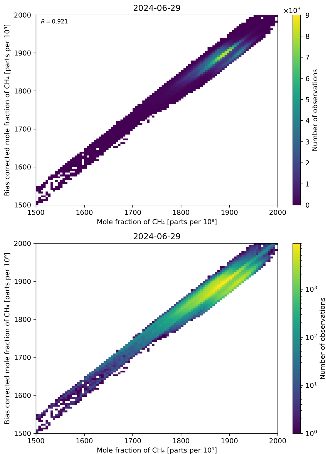
Figure 74: Scatter density plot of “Mole fraction of CH 4 ” against “Bias corrected mole fraction of CH 4 ” for 2024-06-29 to 2024-06-30.
