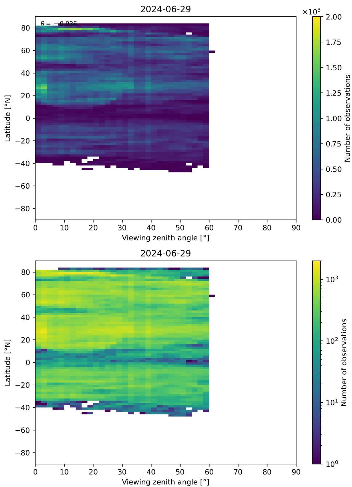
Figure 109: Scatter density plot of “Viewing zenith angle” against “Latitude” for 2024-06-29 to 2024-06-30.
