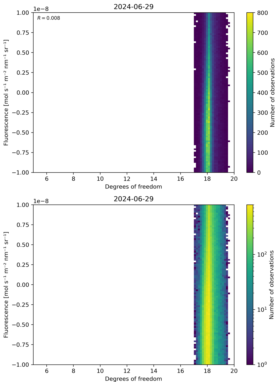
Figure 51: Scatter density plot of “Degrees of freedom” against “Fluorescence” for 2024-06-29 to 2024-06-30.
