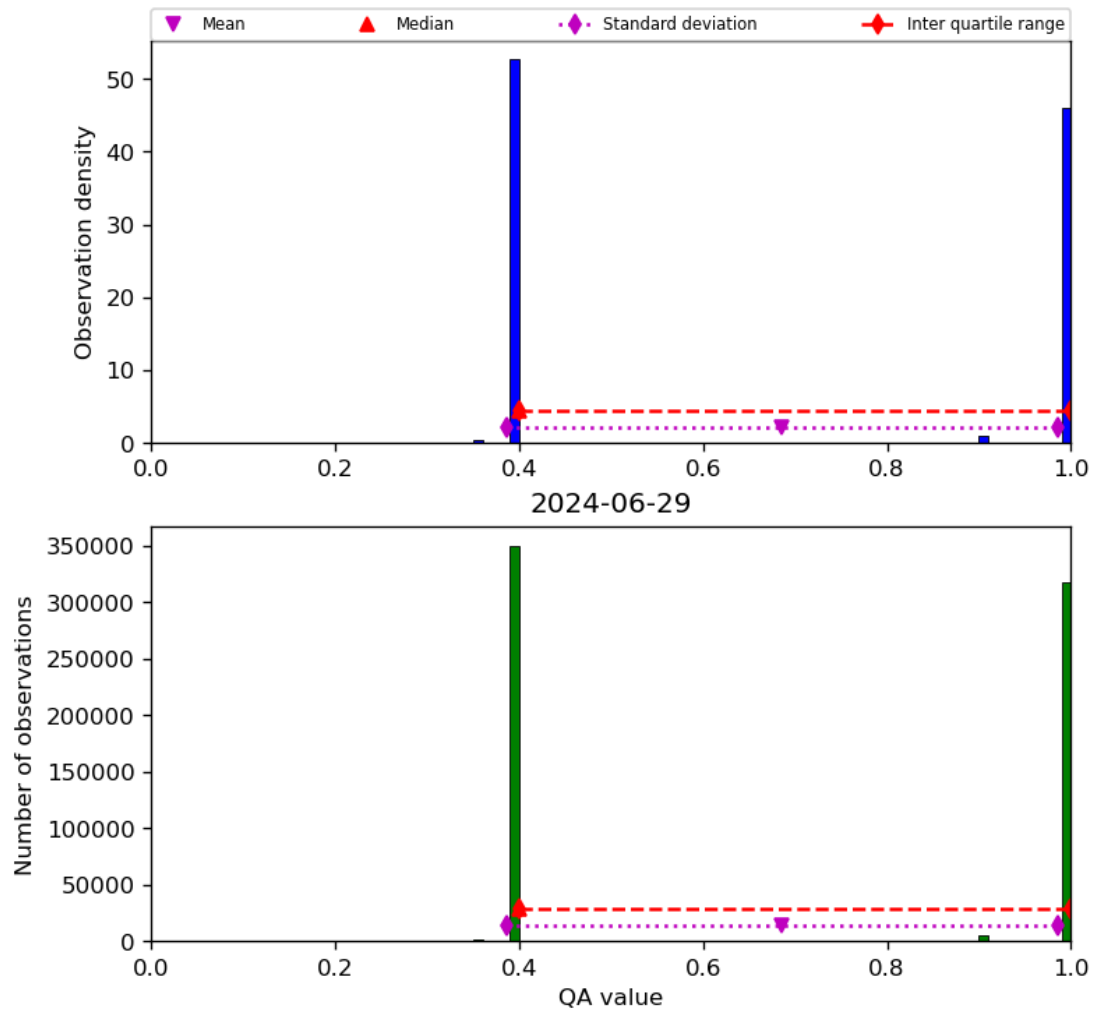
Figure 22: Histogram of “QA value” for 2024-06-29 to 2024-06-30
