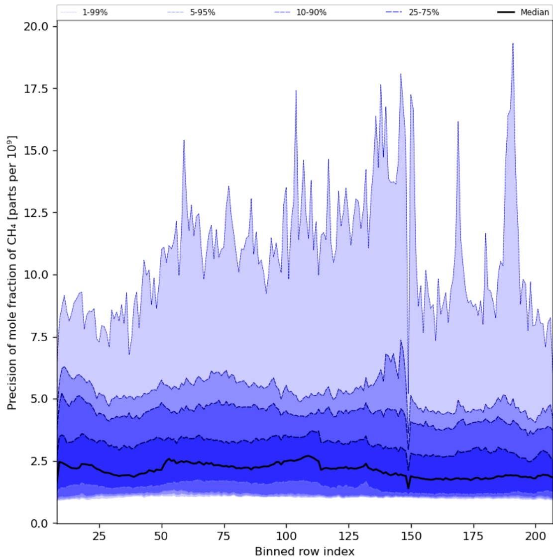
Figure 35: Along track statistics of “Precision of mole fraction of CH 4 ” for 2024-06-29 to 2024-06-30
