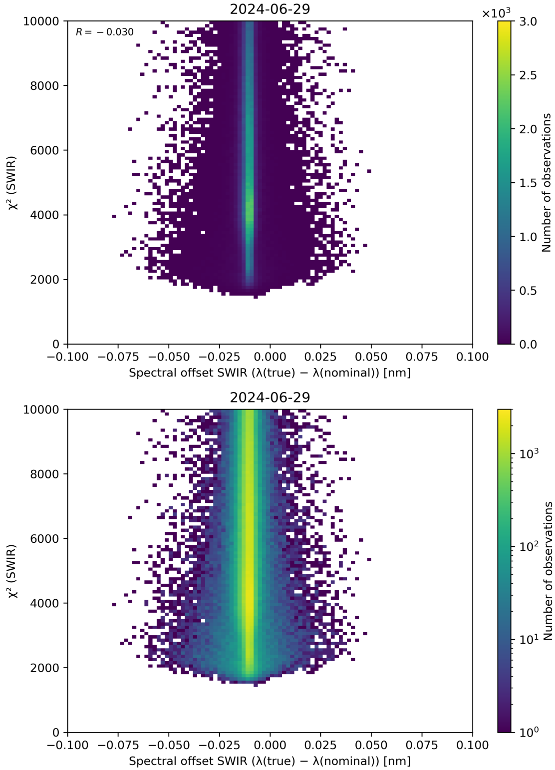
Figure 118: Scatter density plot of “Spectral offset SWIR ( \lambda(\text{true}) - \lambda(\text{nominal}) )” against “ \chi^2 (SWIR)” for 2024-06-29 to 2024-06-30.
