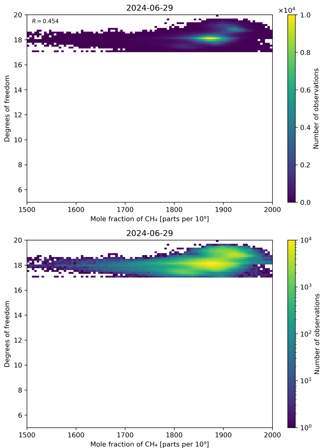
Figure 72: Scatter density plot of “Mole fraction of CH 4 ” against “Degrees of freedom” for 2024-06-29 to 2024-06-30.
