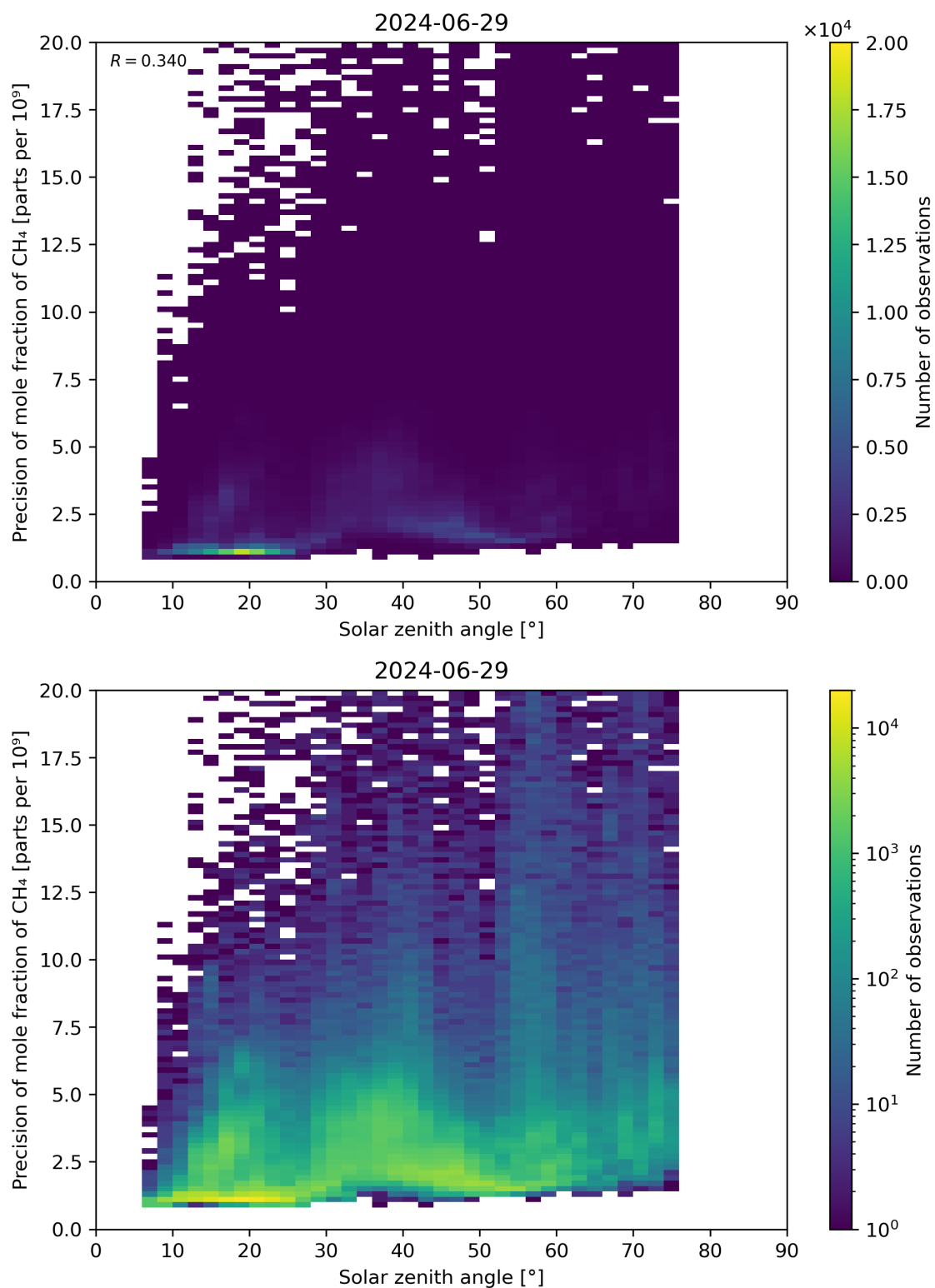
Figure 101: Scatter density plot of “Solar zenith angle” against “Precision of mole fraction of \text{CH}_4 ” for 2024-06-29 to 2024-06-30.
