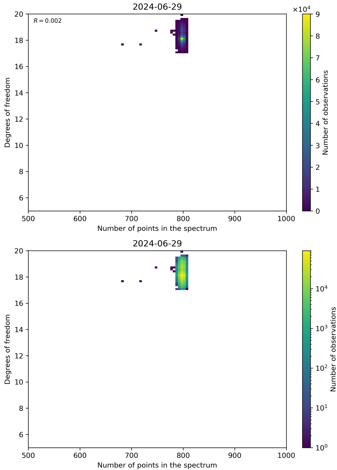
Figure 90: Scatter density plot of “Number of points in the spectrum” against “Degrees of freedom” for 2024-06-29 to 2024-06-30.
