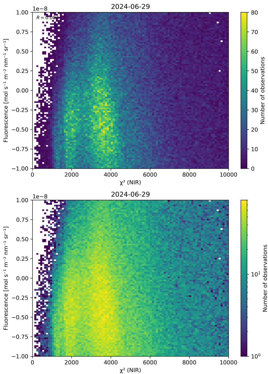
Figure 45: Scatter density plot of “ \chi^2 (NIR)” against “Fluorescence” for 2024-06-29 to 2024-06-30.
