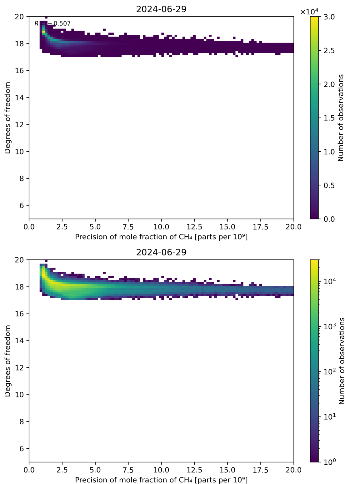
Figure 80: Scatter density plot of “Precision of mole fraction of CH 4 ” against “Degrees of freedom” for 2024-06-29 to 2024-06-30.
