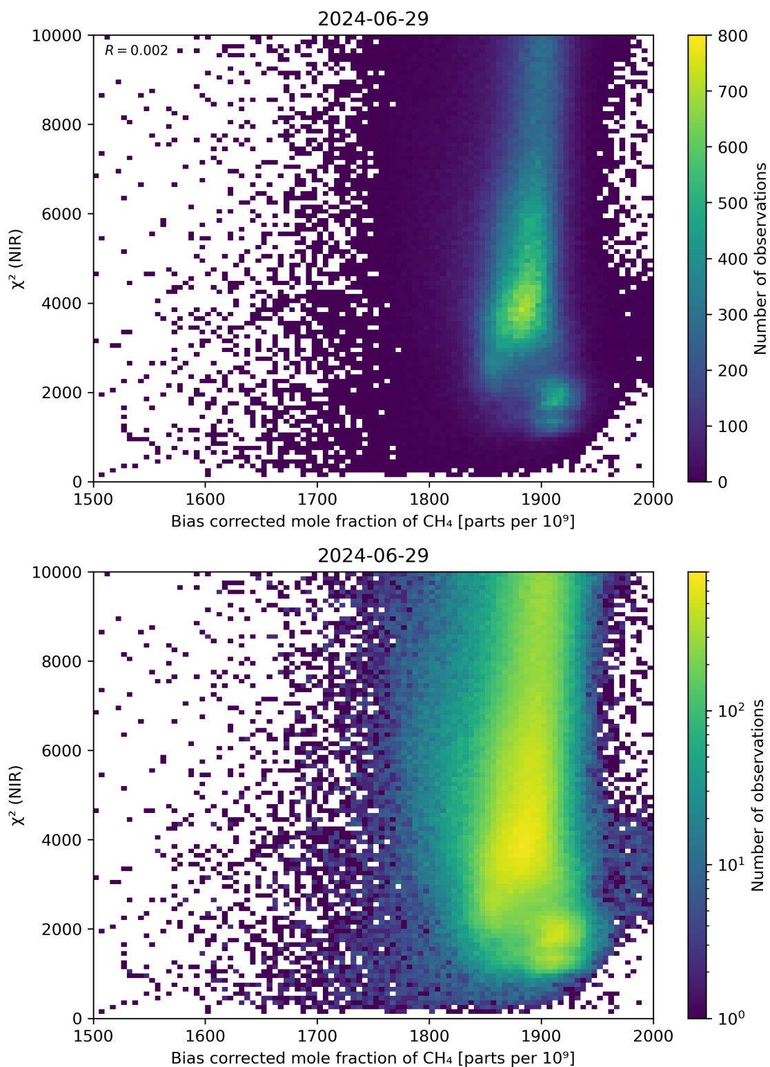
Figure 63: Scatter density plot of “Bias corrected mole fraction of CH 4 ” against “ \chi^2 (NIR)” for 2024-06-29 to 2024-06-30.
