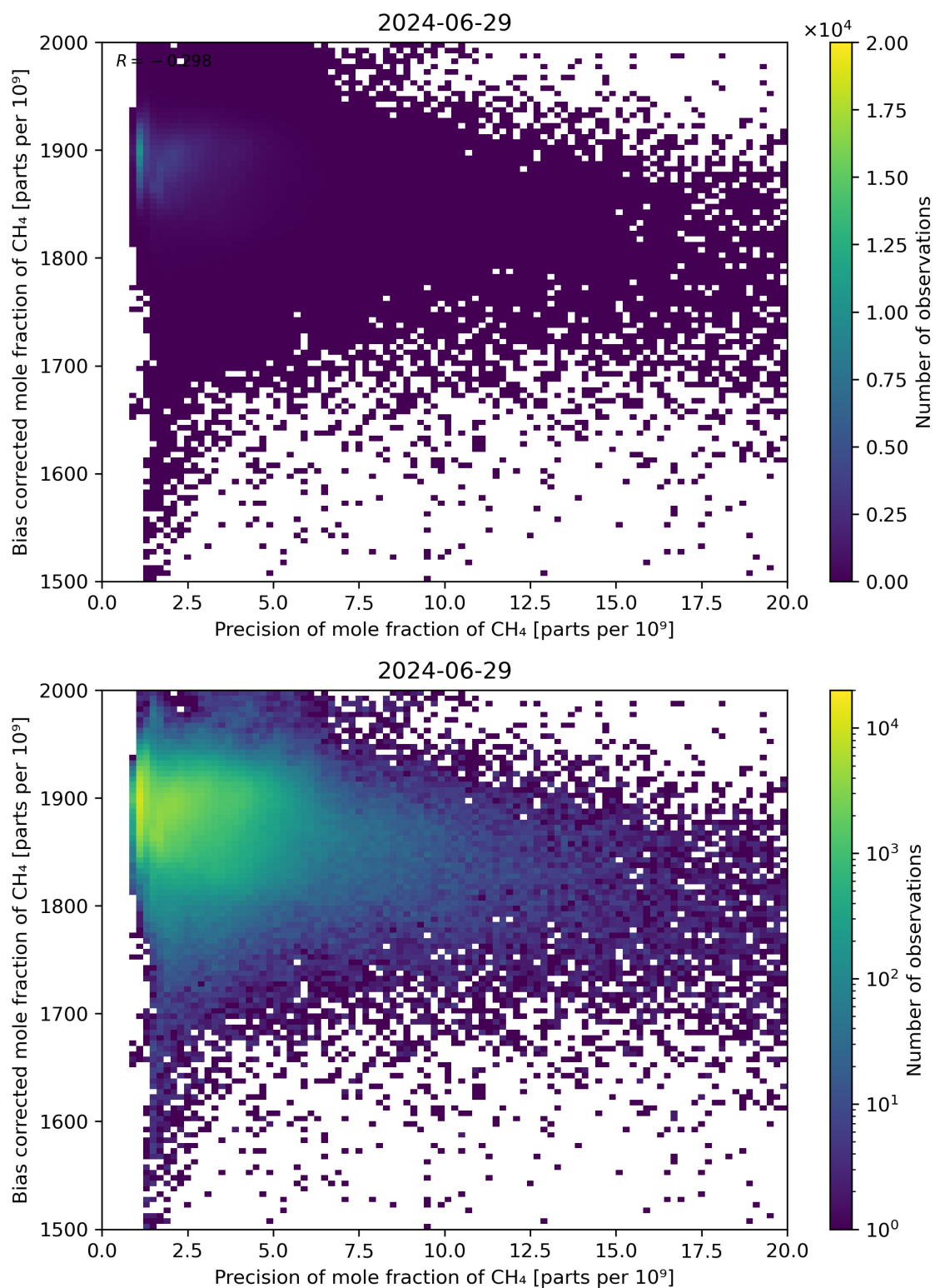
Figure 82: Scatter density plot of “Precision of mole fraction of CH 4 ” against “Bias corrected mole fraction of CH 4 ” for 2024-06-29 to 2024-06-30.
