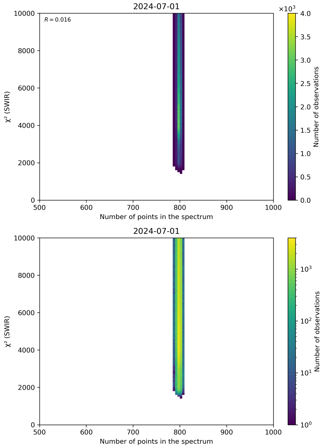
Figure 89: Scatter density plot of “Number of points in the spectrum” against “ \chi^2 (SWIR)” for 2024-06-30 to 2024-07-02.
