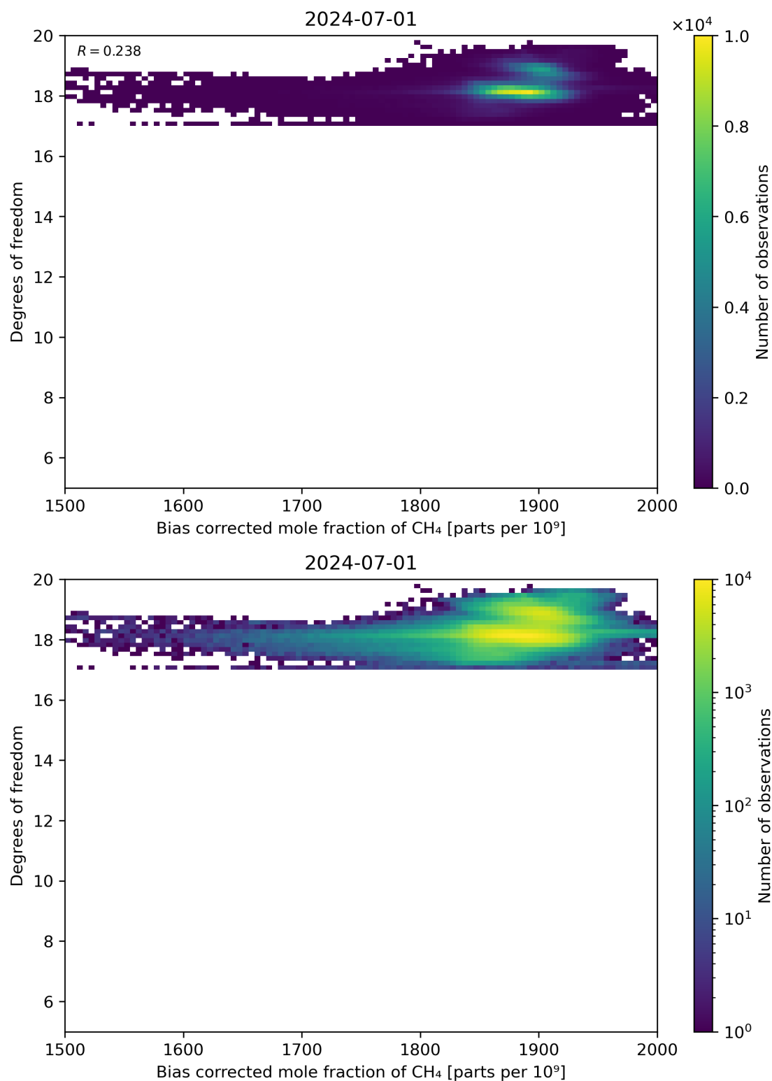
Figure 65: Scatter density plot of “Bias corrected mole fraction of CH 4 ” against “Degrees of freedom” for 2024-06-30 to 2024-07-02.
