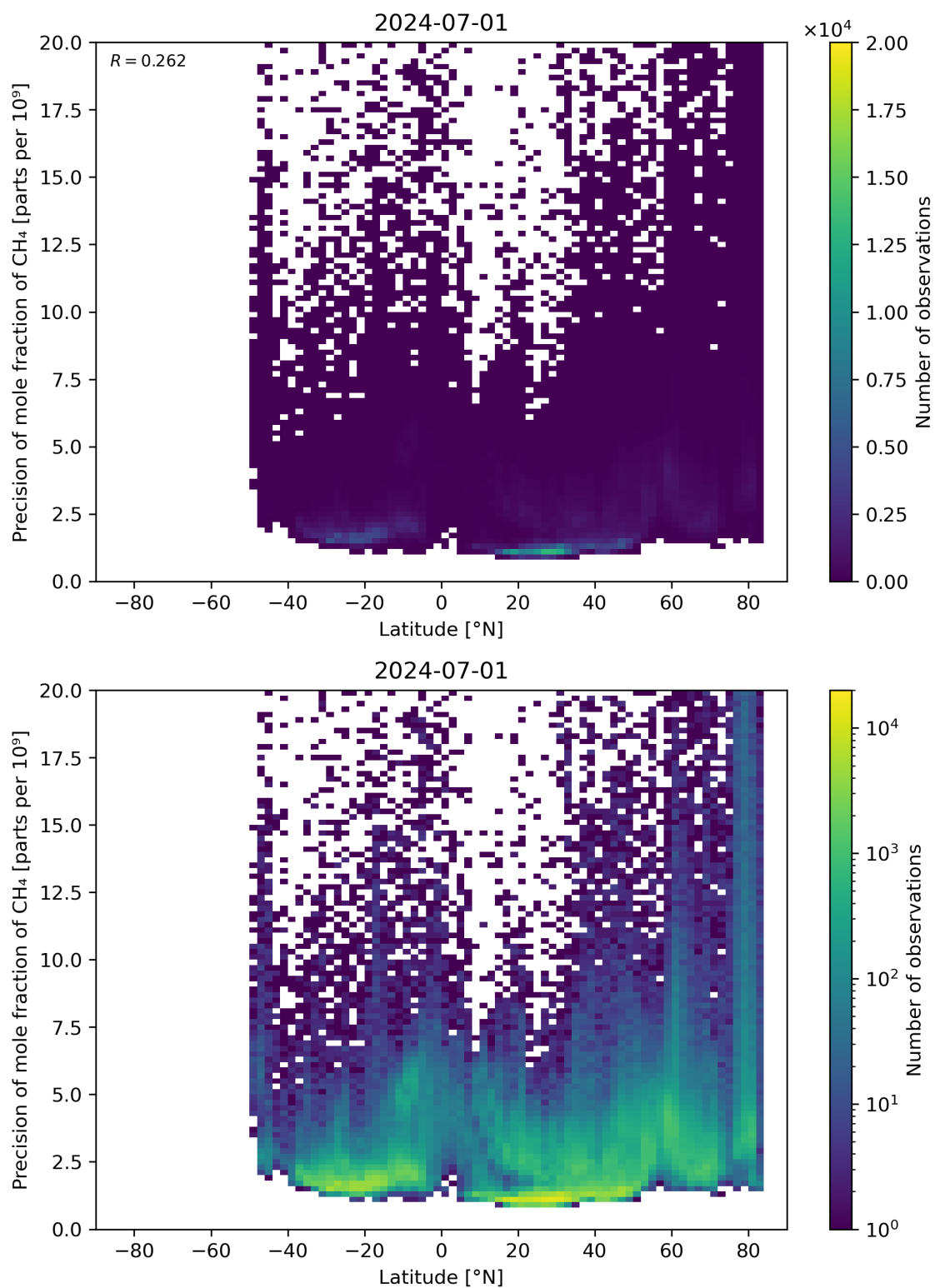
Figure 59: Scatter density plot of “Latitude” against “Precision of mole fraction of \text{CH}_4 ” for 2024-06-30 to 2024-07-02.
