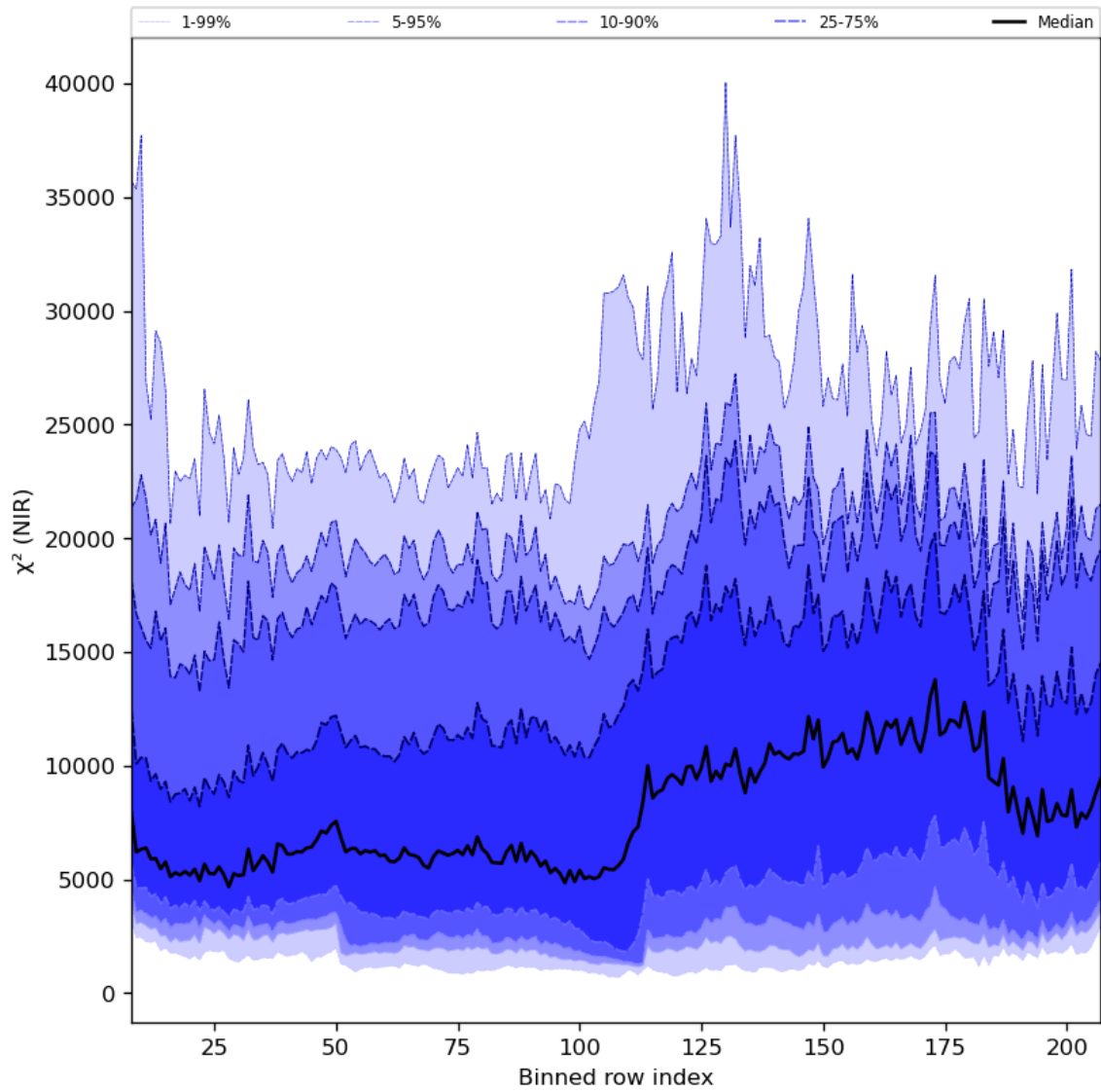
Figure 40: Along track statistics of “ \chi^2 (NIR)” for 2024-06-30 to 2024-07-02
