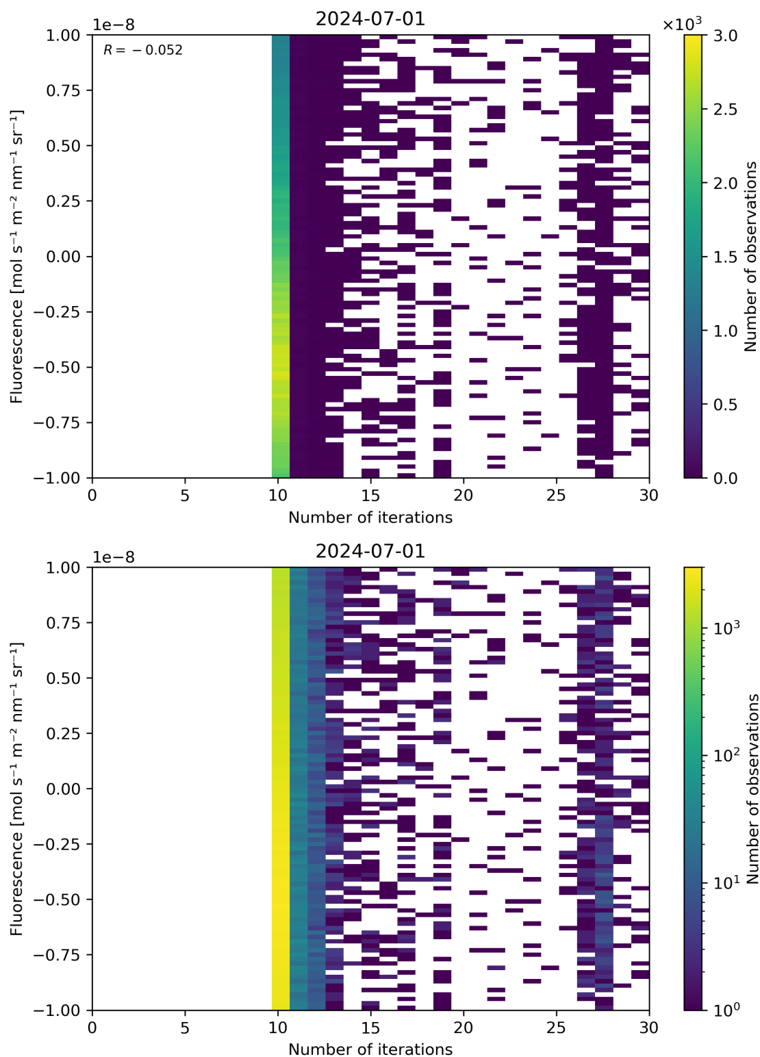
Figure 87: Scatter density plot of “Number of iterations” against “Fluorescence” for 2024-06-30 to 2024-07-02.
