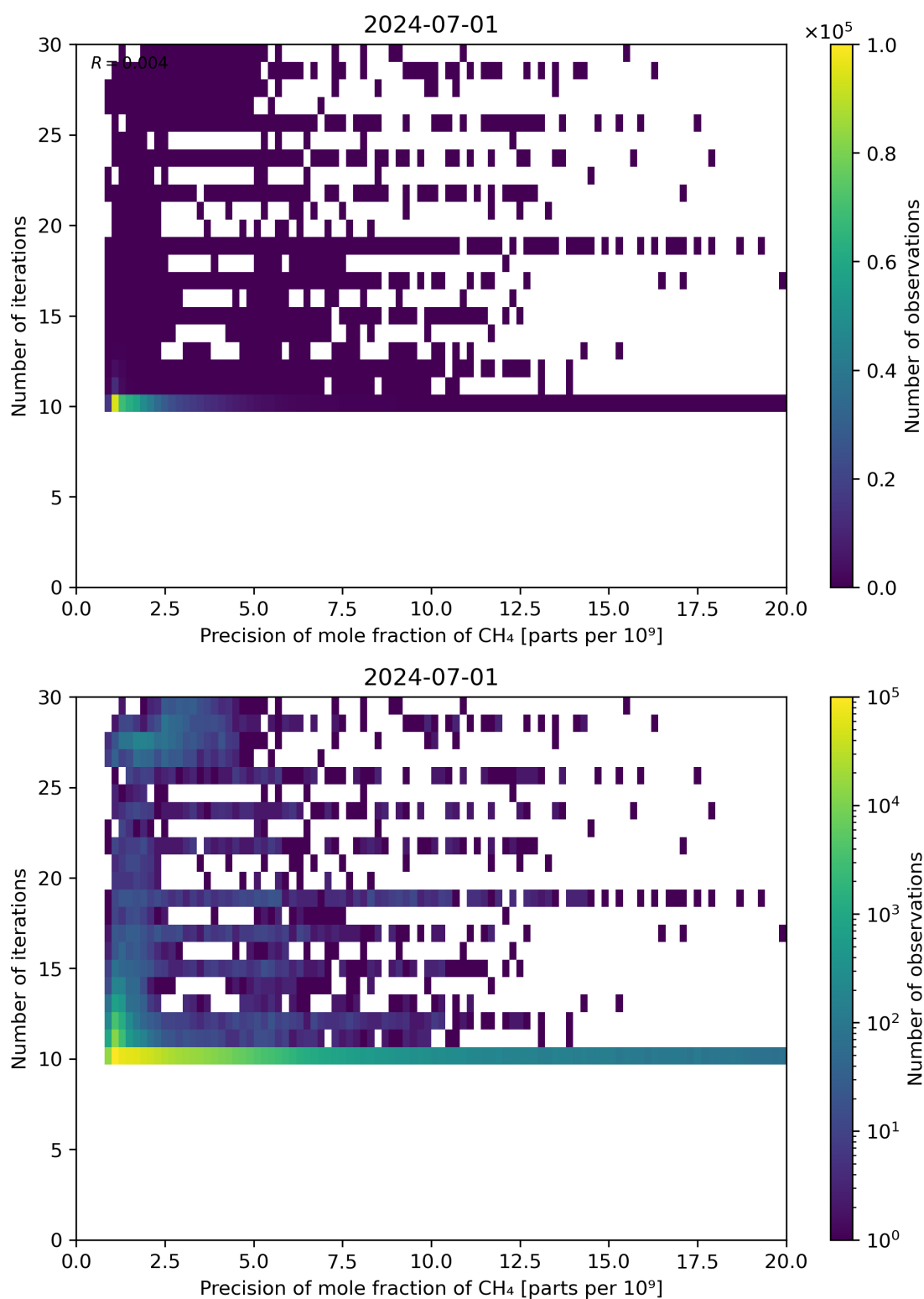
Figure 83: Scatter density plot of “Precision of mole fraction of CH 4 ” against “Number of iterations” for 2024-06-30 to 2024-07-02.
