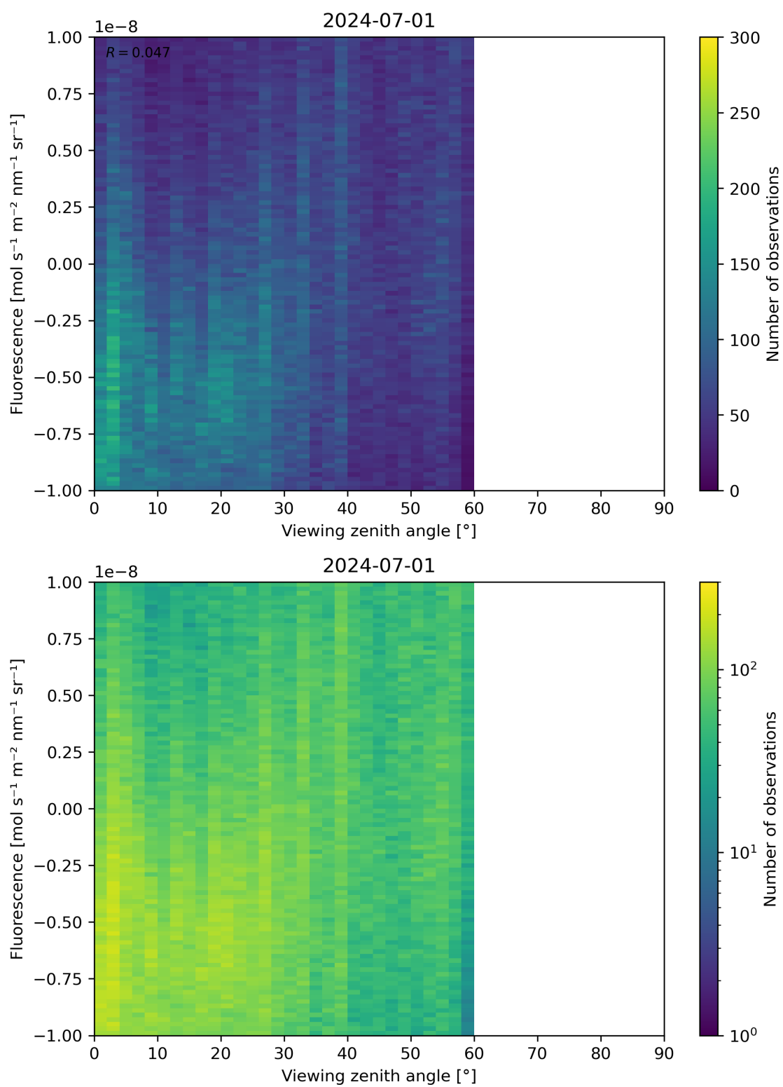
Figure 108: Scatter density plot of “Viewing zenith angle” against “Fluorescence” for 2024-06-30 to 2024-07-02.
