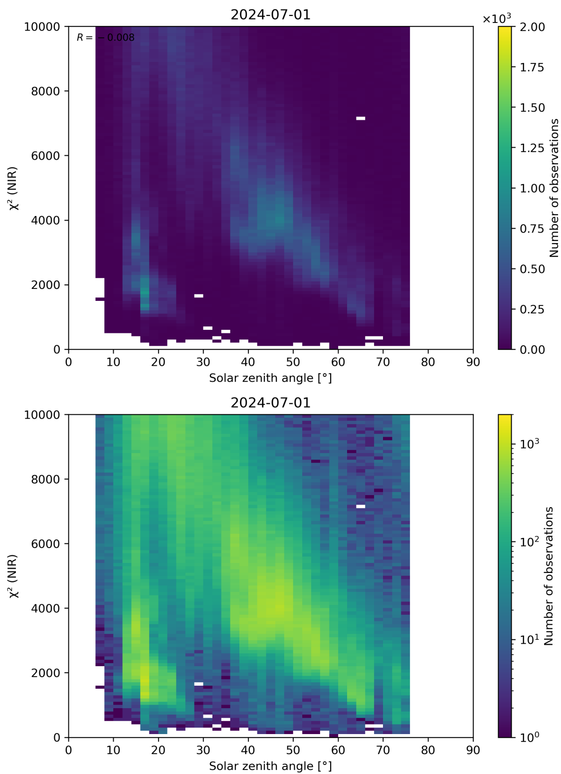
Figure 94: Scatter density plot of “Solar zenith angle” against “ \chi^2 (NIR)” for 2024-06-30 to 2024-07-02.
