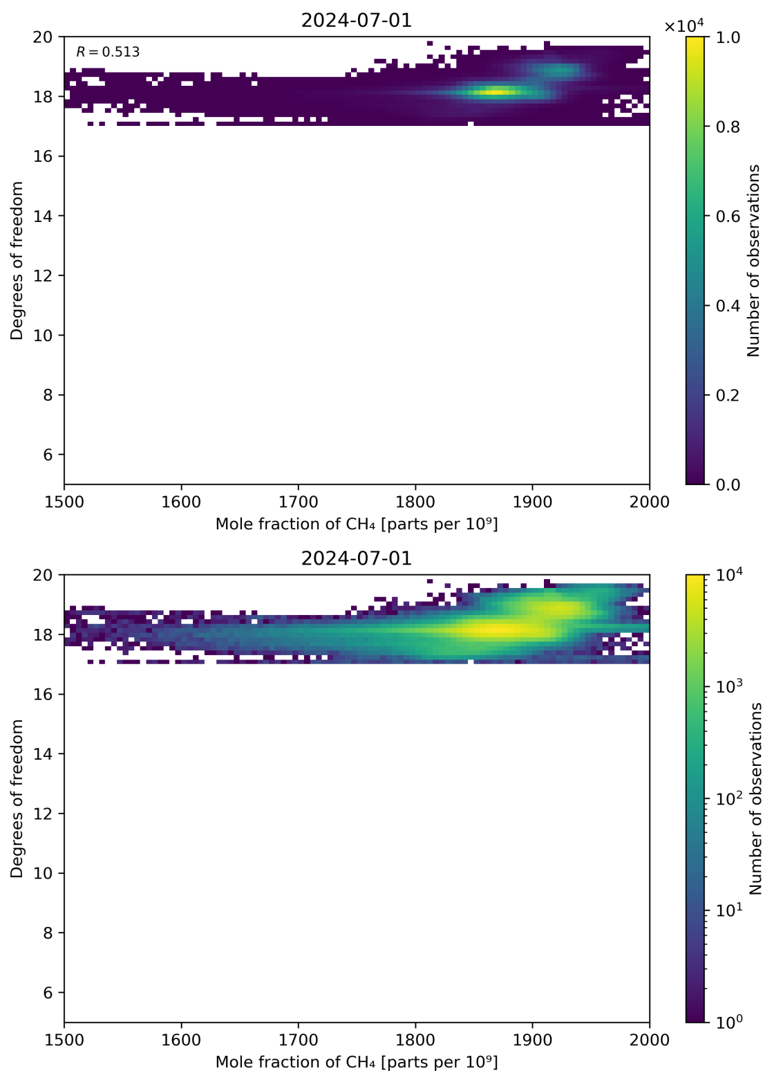
Figure 72: Scatter density plot of “Mole fraction of CH 4 ” against “Degrees of freedom” for 2024-06-30 to 2024-07-02.
