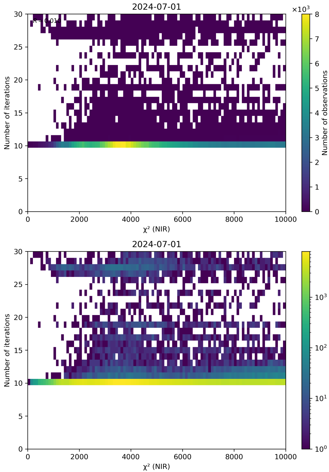
Figure 46: Scatter density plot of “ \chi^2 (NIR)” against “Number of iterations” for 2024-06-30 to 2024-07-02.
