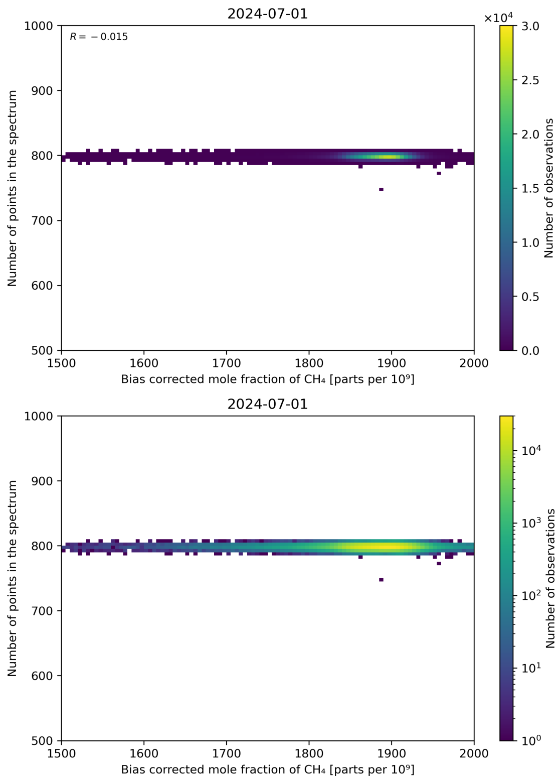
Figure 68: Scatter density plot of “Bias corrected mole fraction of CH 4 ” against “Number of points in the spectrum” for 2024-06-30 to 2024-07-02.
