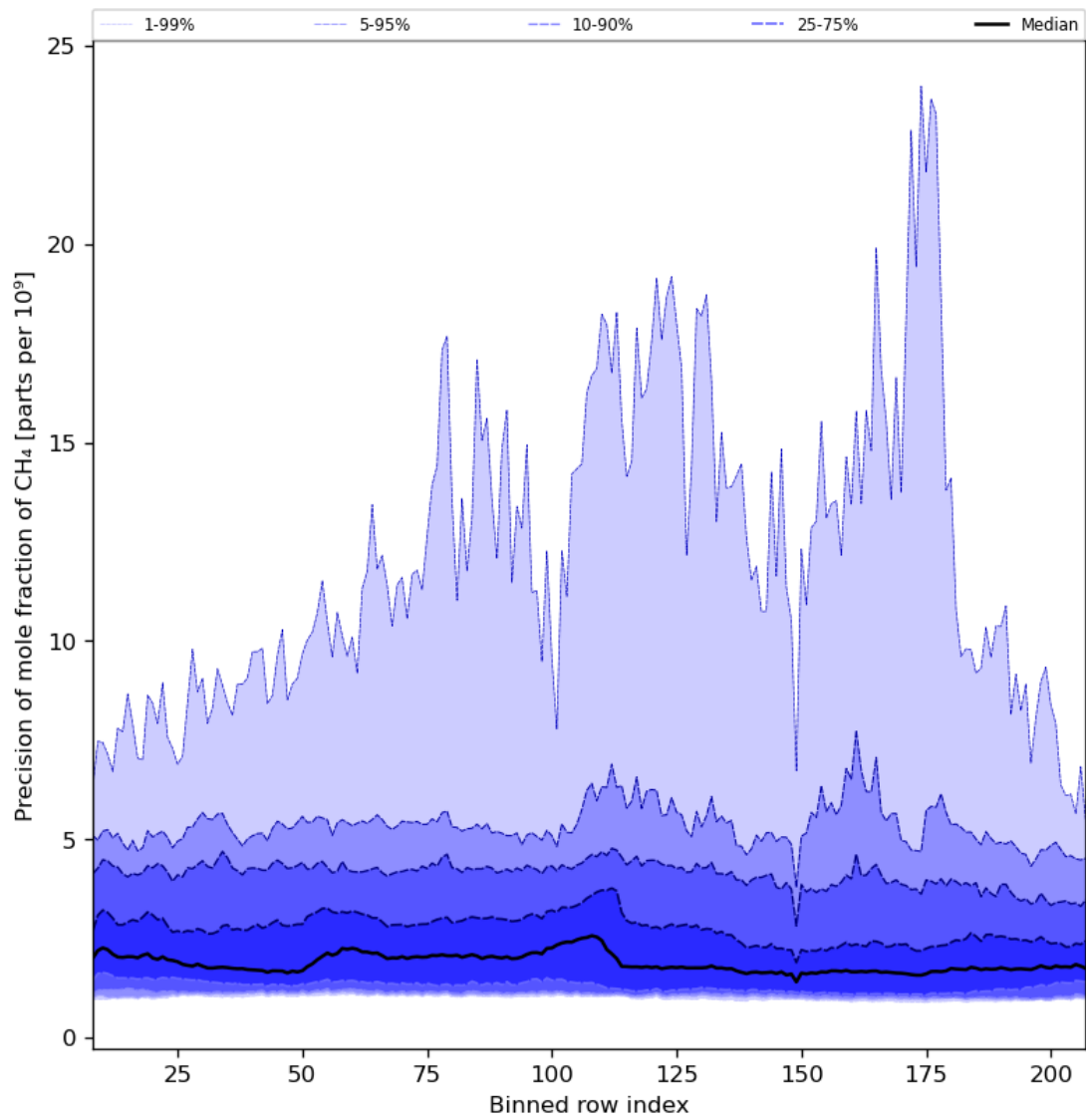
Figure 35: Along track statistics of “Precision of mole fraction of CH 4 ” for 2024-06-30 to 2024-07-02
