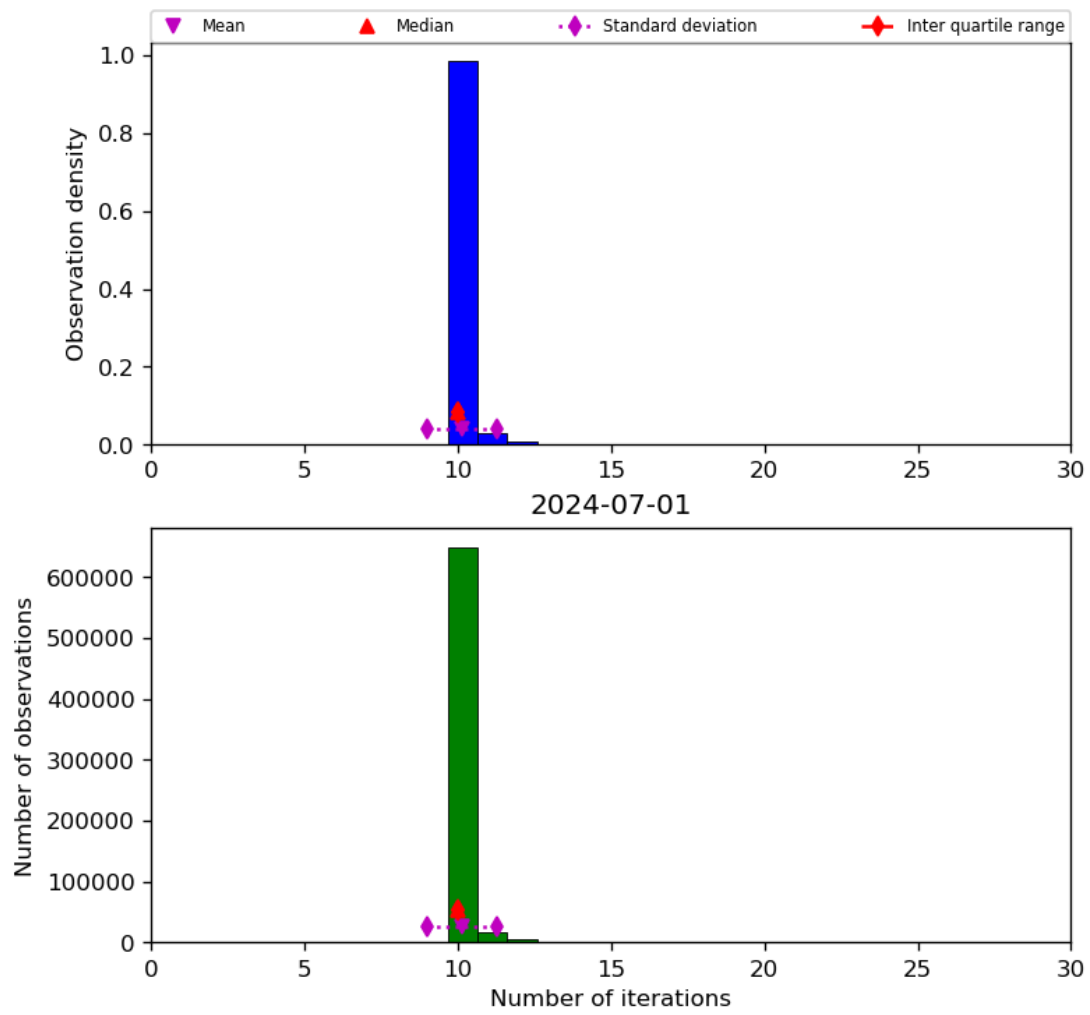
Figure 31: Histogram of “Number of iterations” for 2024-06-30 to 2024-07-02
