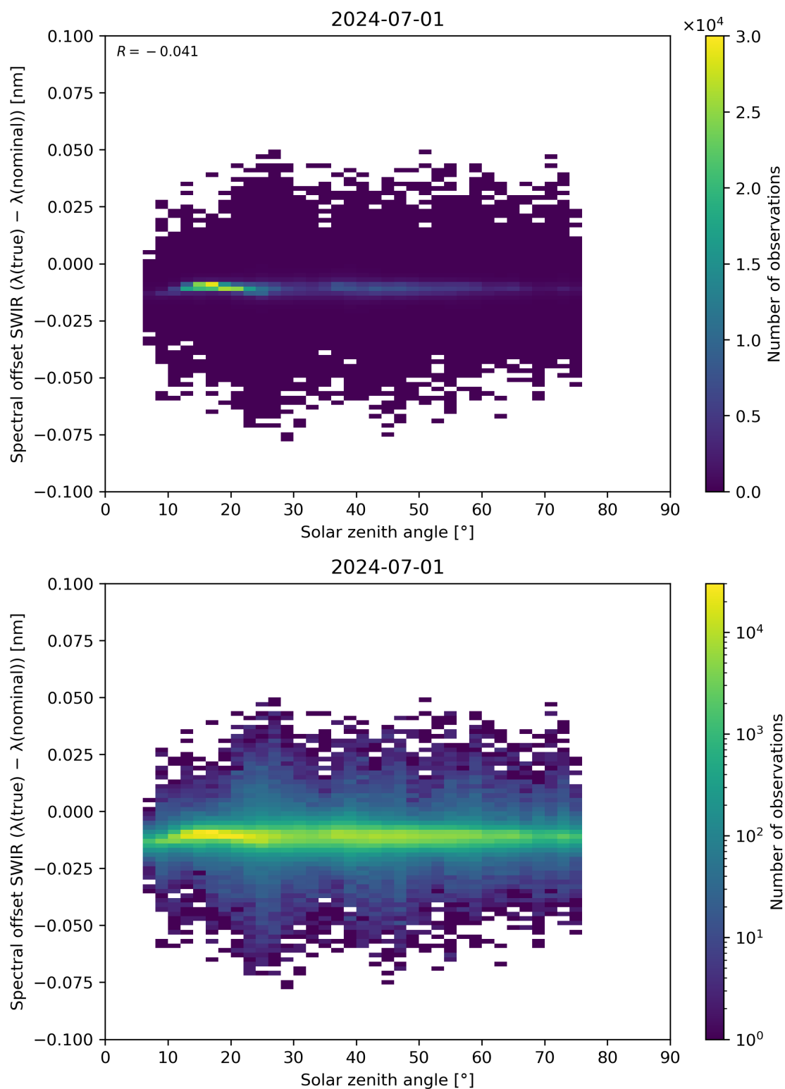
Figure 104: Scatter density plot of “Solar zenith angle” against “Spectral offset SWIR ( \lambda(\text{true}) - \lambda(\text{nominal}) )” for 2024-06-30 to 2024-07-02.
