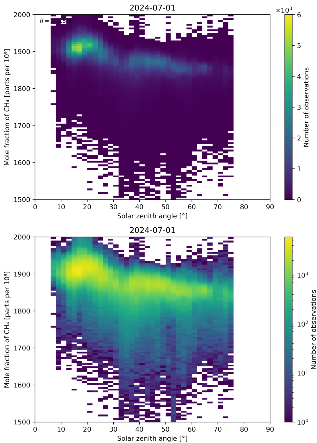
Figure 99: Scatter density plot of “Solar zenith angle” against “Mole fraction of CH 4 ” for 2024-06-30 to 2024-07-02.
