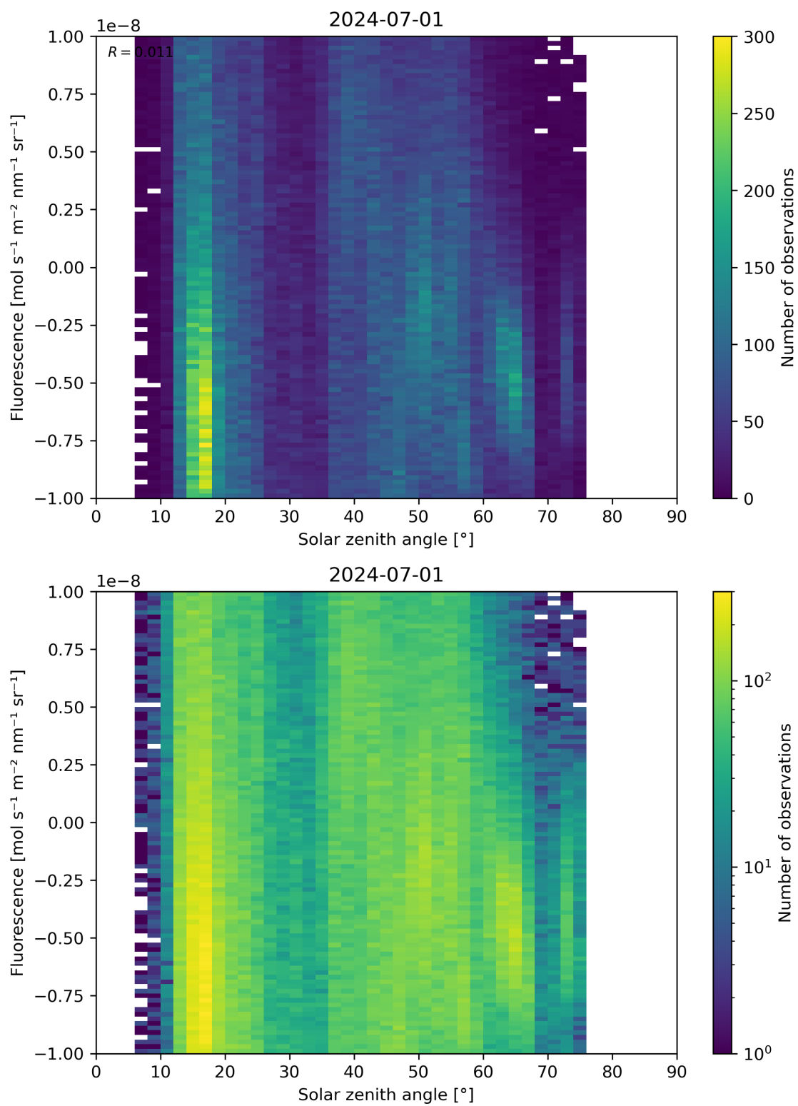
Figure 97: Scatter density plot of “Solar zenith angle” against “Fluorescence” for 2024-06-30 to 2024-07-02.
