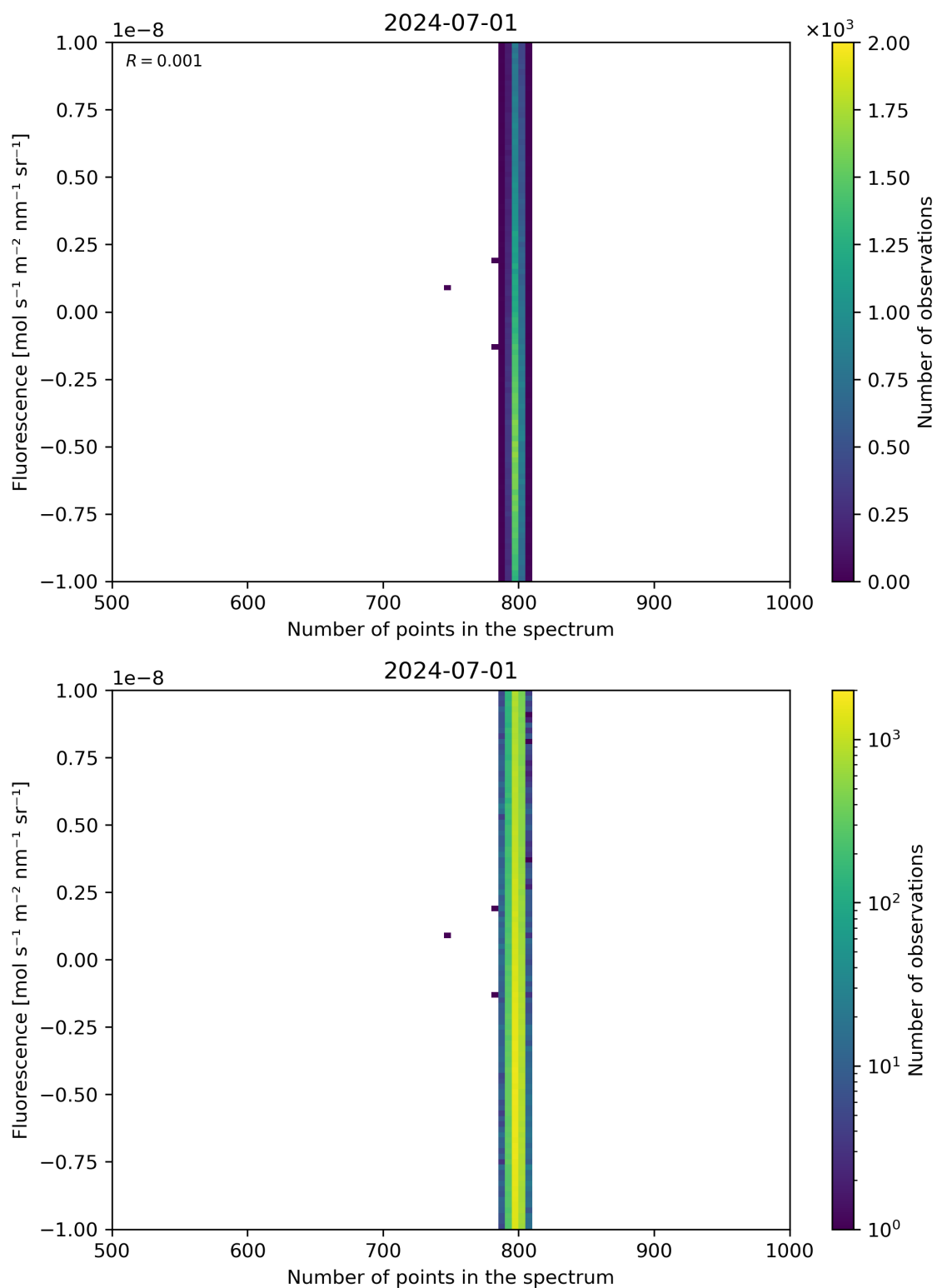
Figure 91: Scatter density plot of “Number of points in the spectrum” against “Fluorescence” for 2024-06-30 to 2024-07-02.
