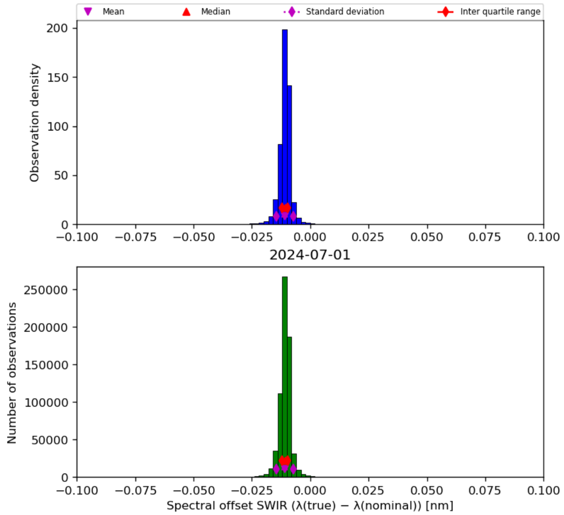
Figure 27: Histogram of “Spectral offset SWIR ( \lambda(\text{true}) - \lambda(\text{nominal}) )” for 2024-06-30 to 2024-07-02
