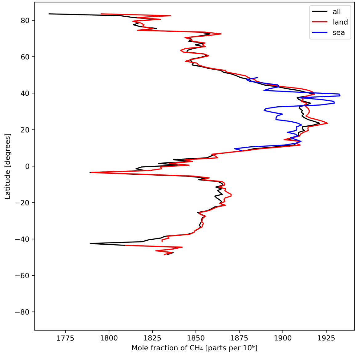
Figure 12: Zonal average of “Mole fraction of \text{CH}_4 ” for 2024-06-30 to 2024-07-02.
