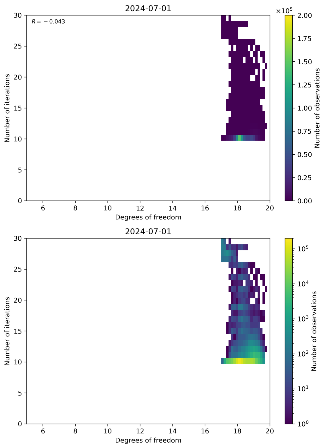
Figure 52: Scatter density plot of “Degrees of freedom” against “Number of iterations” for 2024-06-30 to 2024-07-02.
