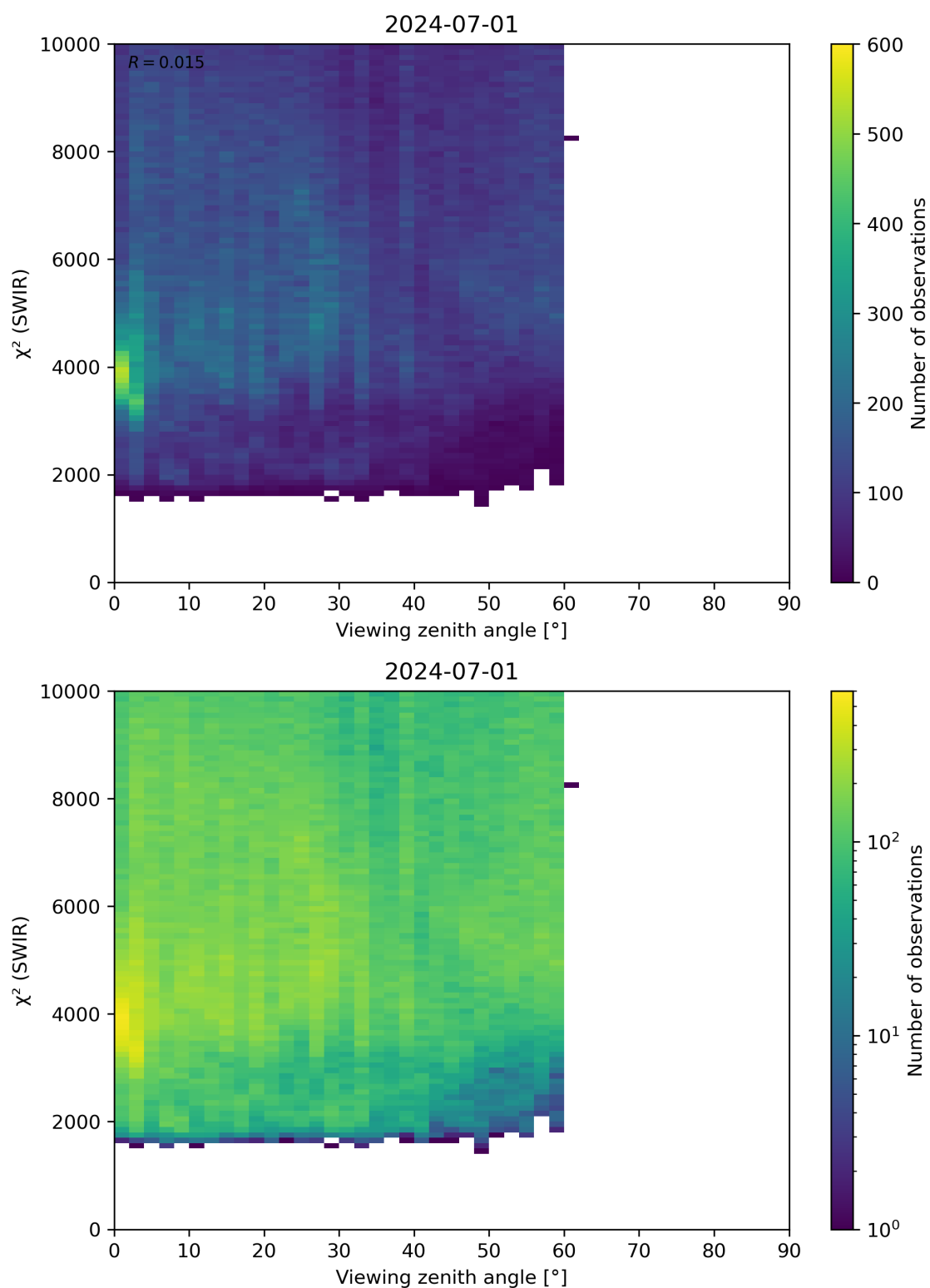
Figure 106: Scatter density plot of “Viewing zenith angle” against “ \chi^2 (SWIR)” for 2024-06-30 to 2024-07-02.
