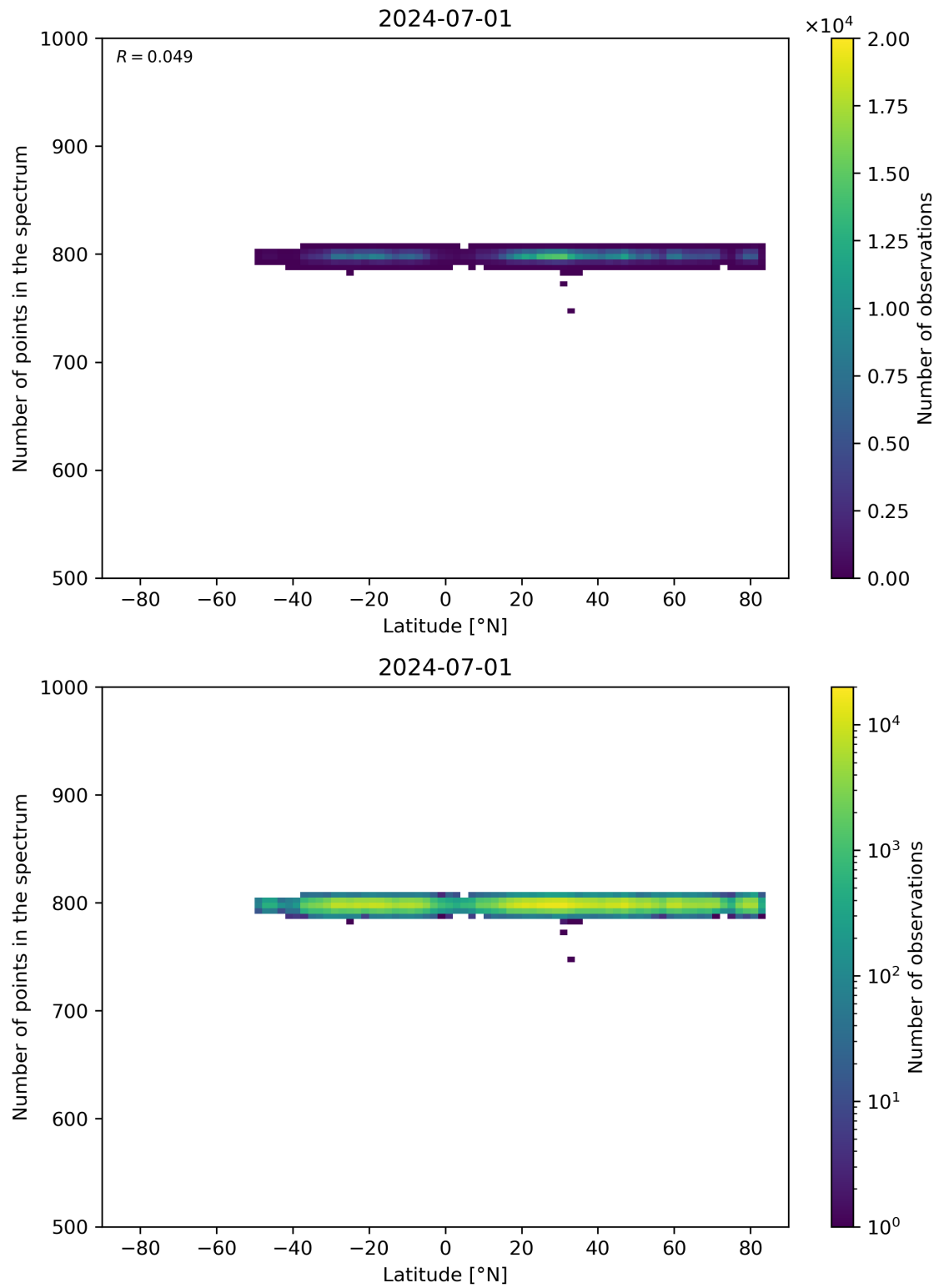
Figure 61: Scatter density plot of “Latitude” against “Number of points in the spectrum” for 2024-06-30 to 2024-07-02.
