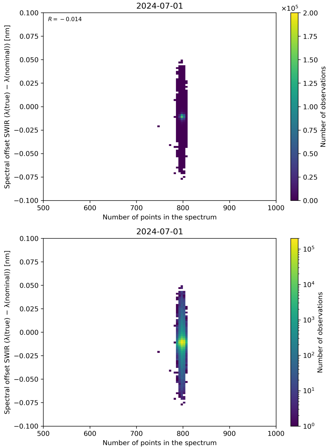
Figure 93: Scatter density plot of “Number of points in the spectrum” against “Spectral offset SWIR ( \lambda(\text{true}) - \lambda(\text{nominal}) )” for 2024-06-30 to 2024-07-02.
