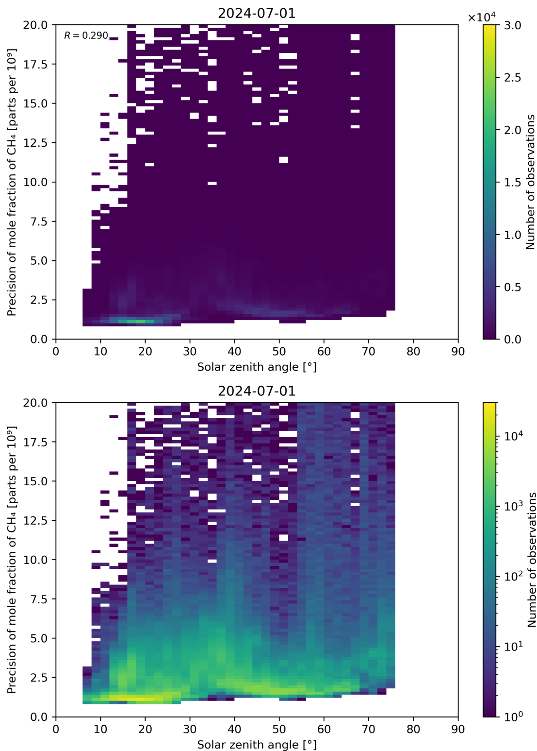
Figure 101: Scatter density plot of “Solar zenith angle” against “Precision of mole fraction of CH 4 ” for 2024-06-30 to 2024-07-02.
