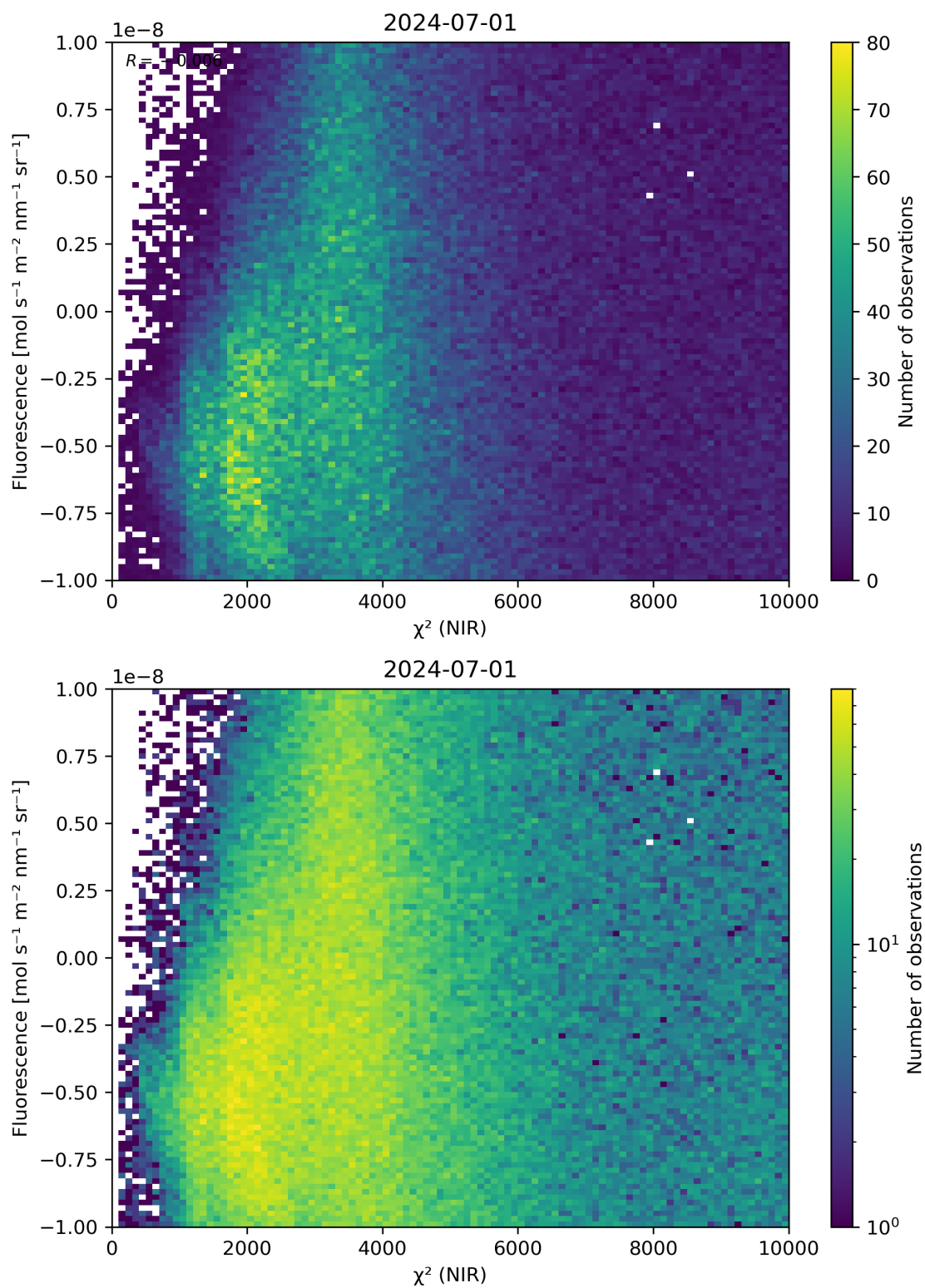
Figure 45: Scatter density plot of “ \chi^2 (NIR)” against “Fluorescence” for 2024-06-30 to 2024-07-02.
