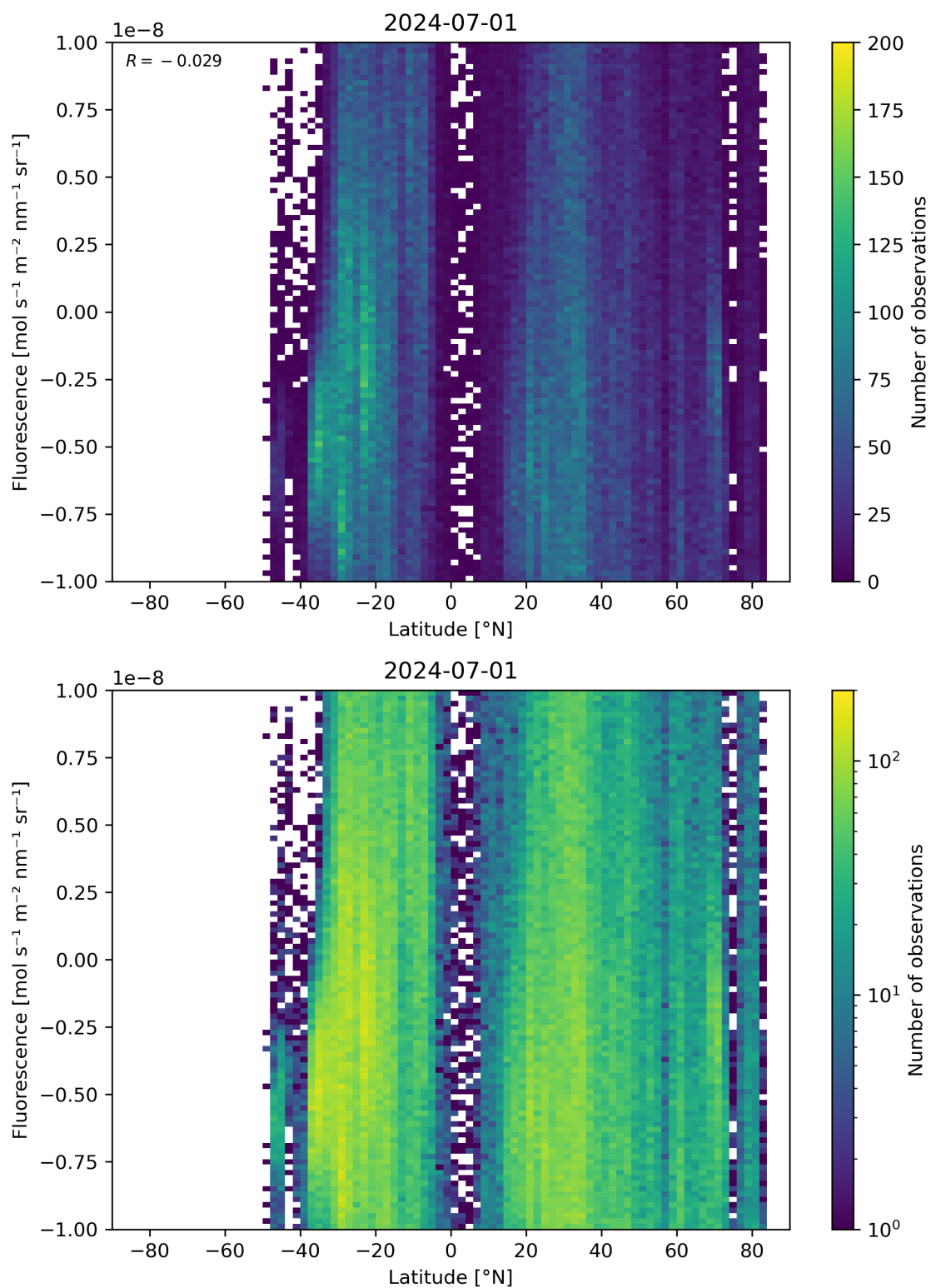
Figure 56: Scatter density plot of “Latitude” against “Fluorescence” for 2024-06-30 to 2024-07-02.
