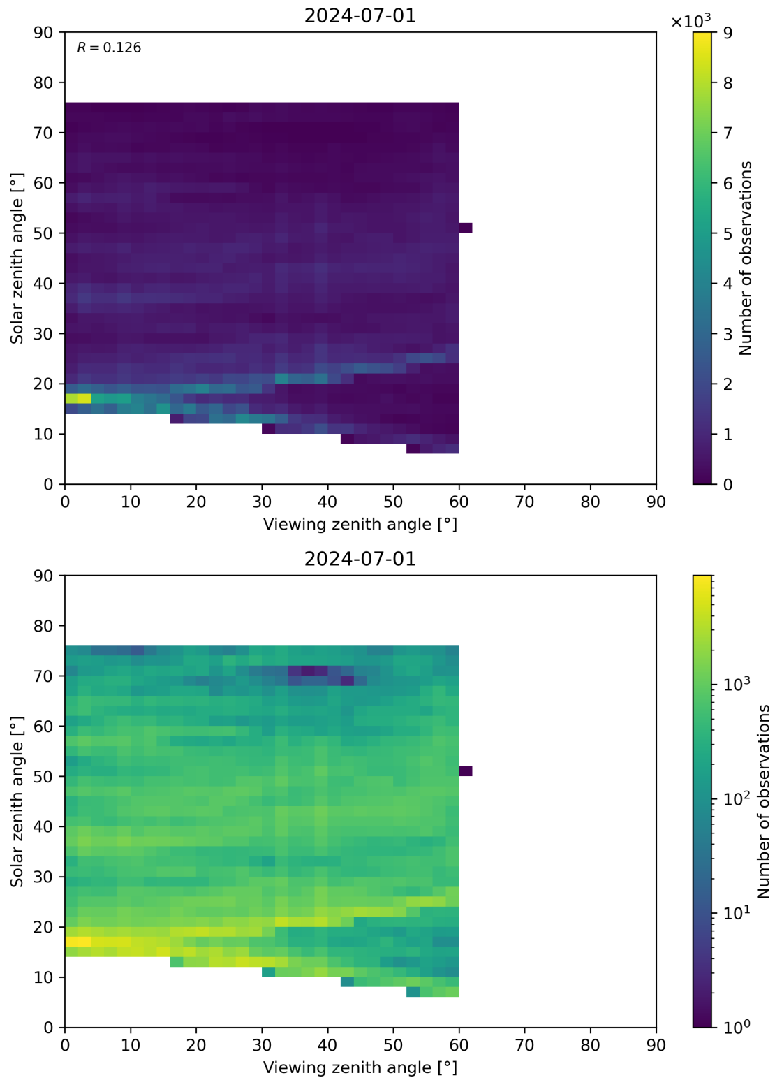
Figure 115: Scatter density plot of “Viewing zenith angle” against “Solar zenith angle” for 2024-06-30 to 2024-07-02.
