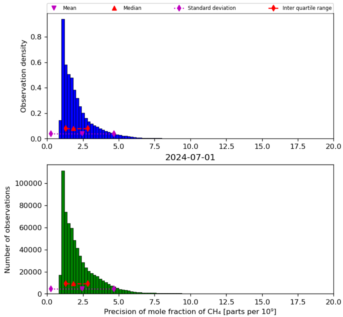
Figure 24: Histogram of “Precision of mole fraction of CH 4 ” for 2024-06-30 to 2024-07-02
