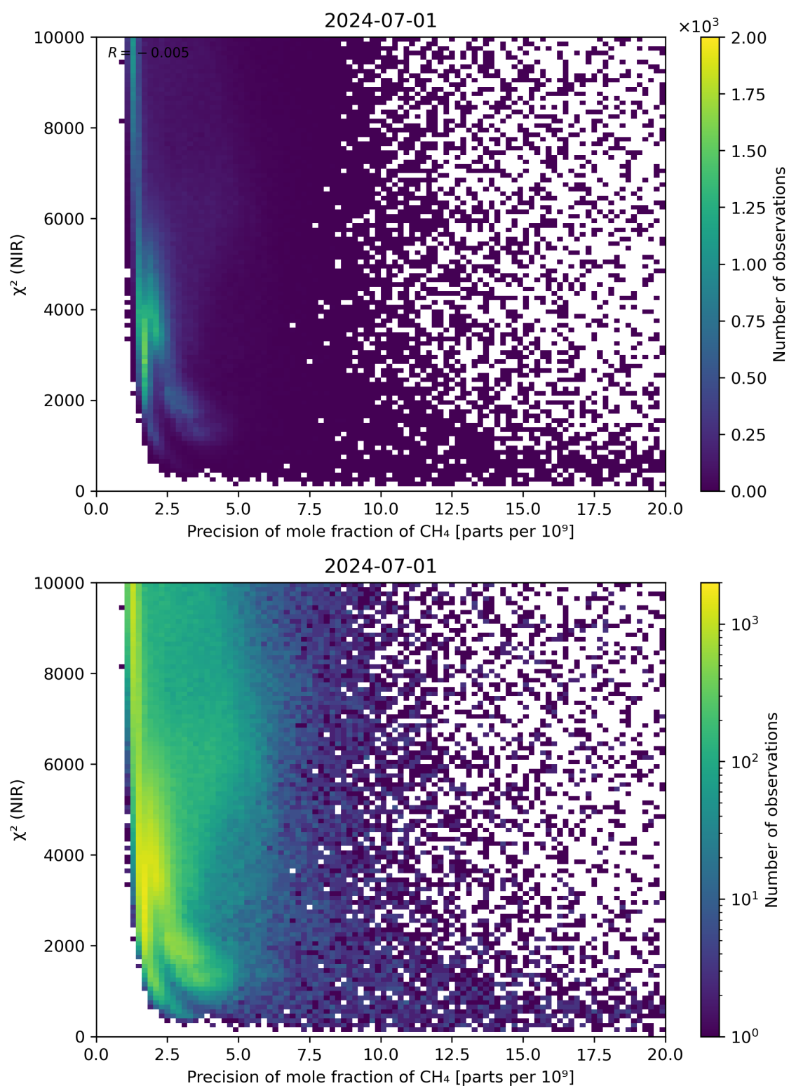
Figure 78: Scatter density plot of “Precision of mole fraction of CH 4 ” against “ \chi^2 (NIR)” for 2024-06-30 to 2024-07-02.
