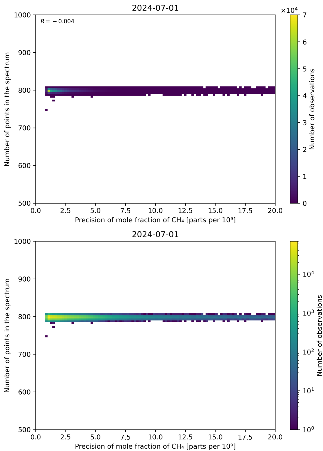
Figure 84: Scatter density plot of “Precision of mole fraction of CH 4 ” against “Number of points in the spectrum” for 2024-06-30 to 2024-07-02.
