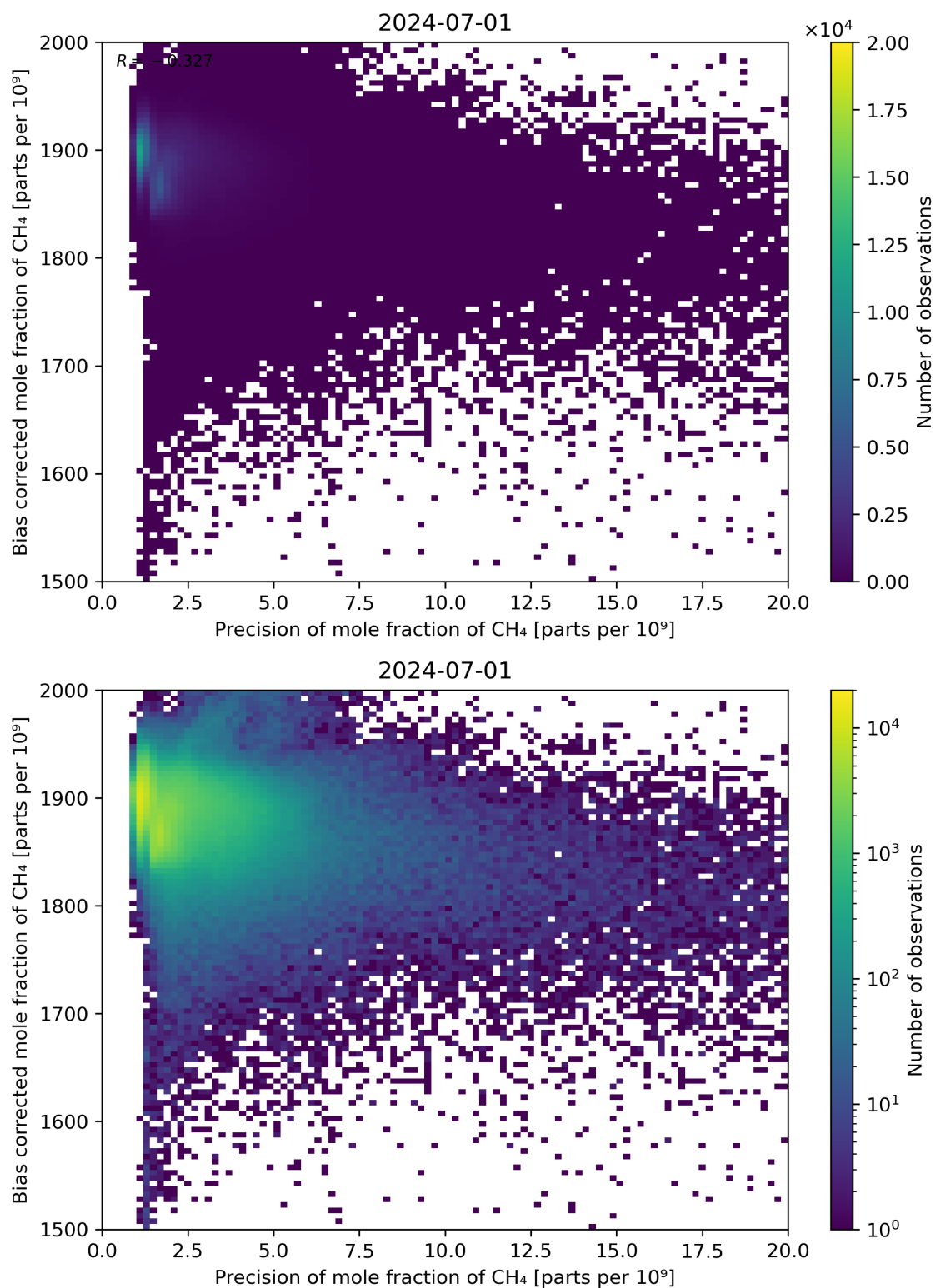
Figure 82: Scatter density plot of “Precision of mole fraction of CH 4 ” against “Bias corrected mole fraction of CH 4 ” for 2024-06-30 to 2024-07-02.
