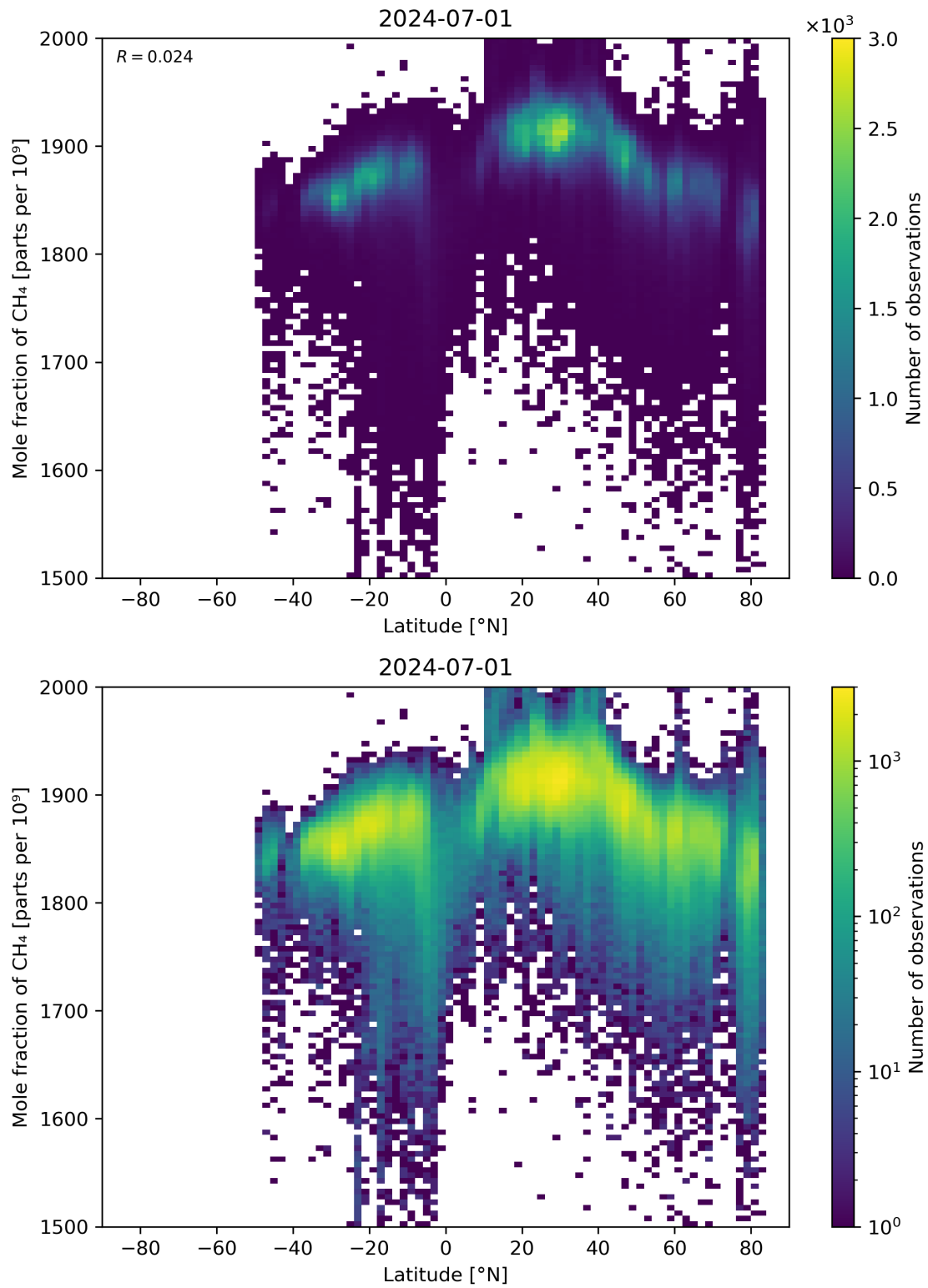
Figure 57: Scatter density plot of “Latitude” against “Mole fraction of \text{CH}_4 ” for 2024-06-30 to 2024-07-02.
