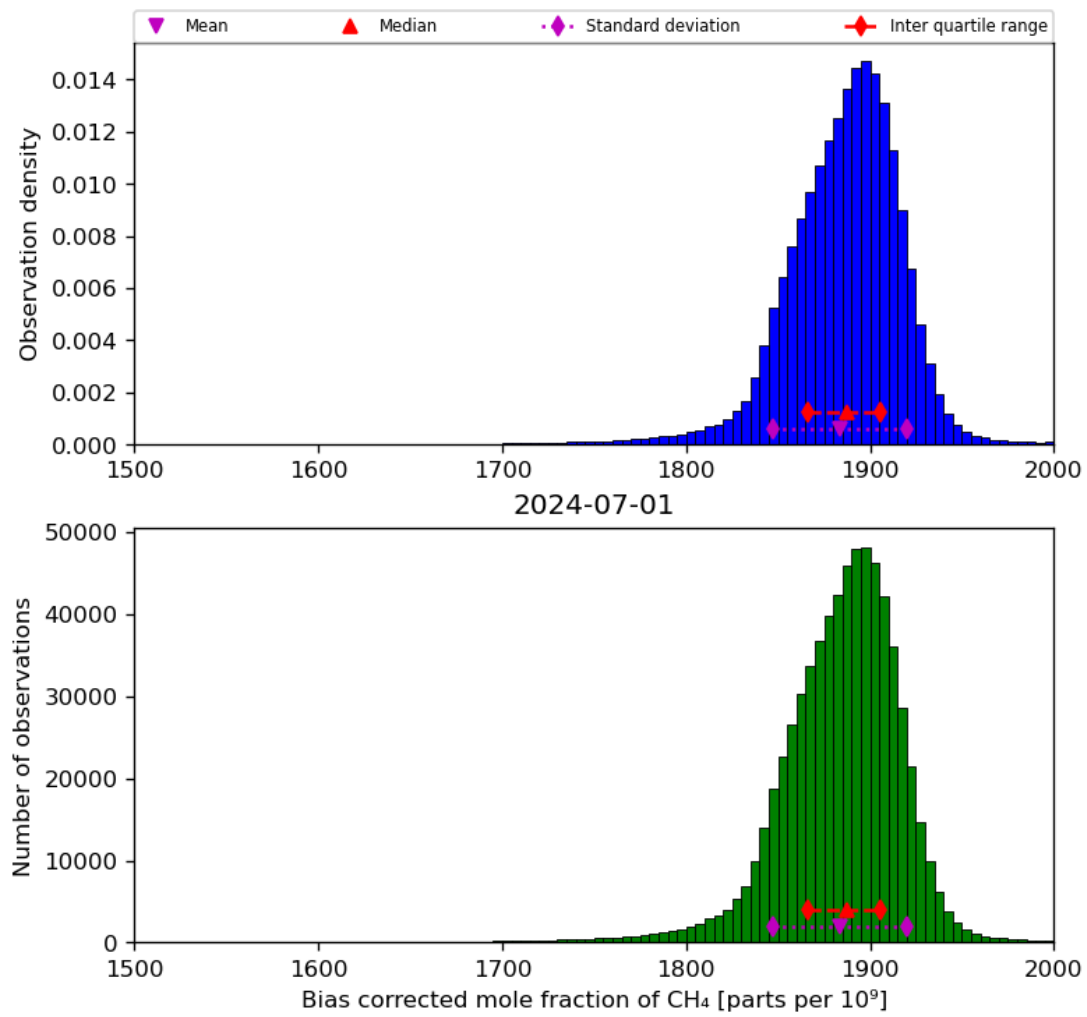
Figure 25: Histogram of “Bias corrected mole fraction of CH 4 ” for 2024-06-30 to 2024-07-02
