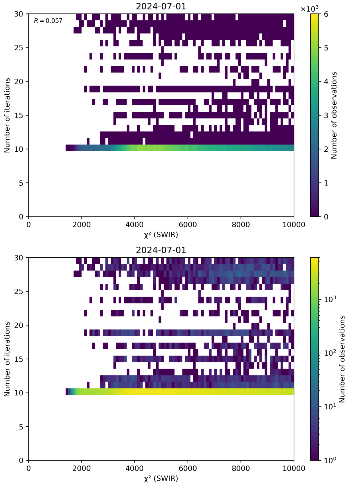
Figure 50: Scatter density plot of “ \chi^2 (SWIR)” against “Number of iterations” for 2024-06-30 to 2024-07-02.
