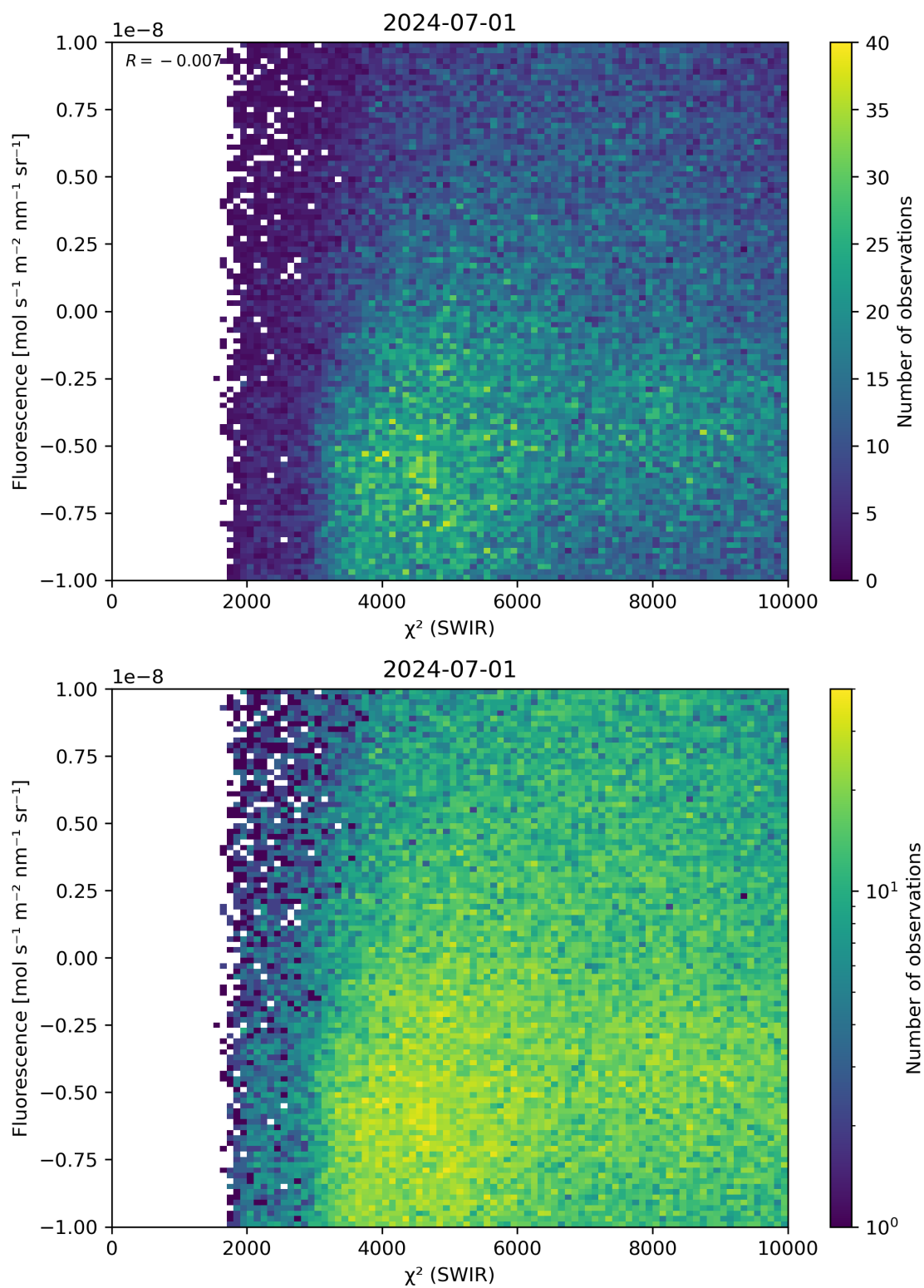
Figure 49: Scatter density plot of “ \chi^2 (SWIR)” against “Fluorescence” for 2024-06-30 to 2024-07-02.
