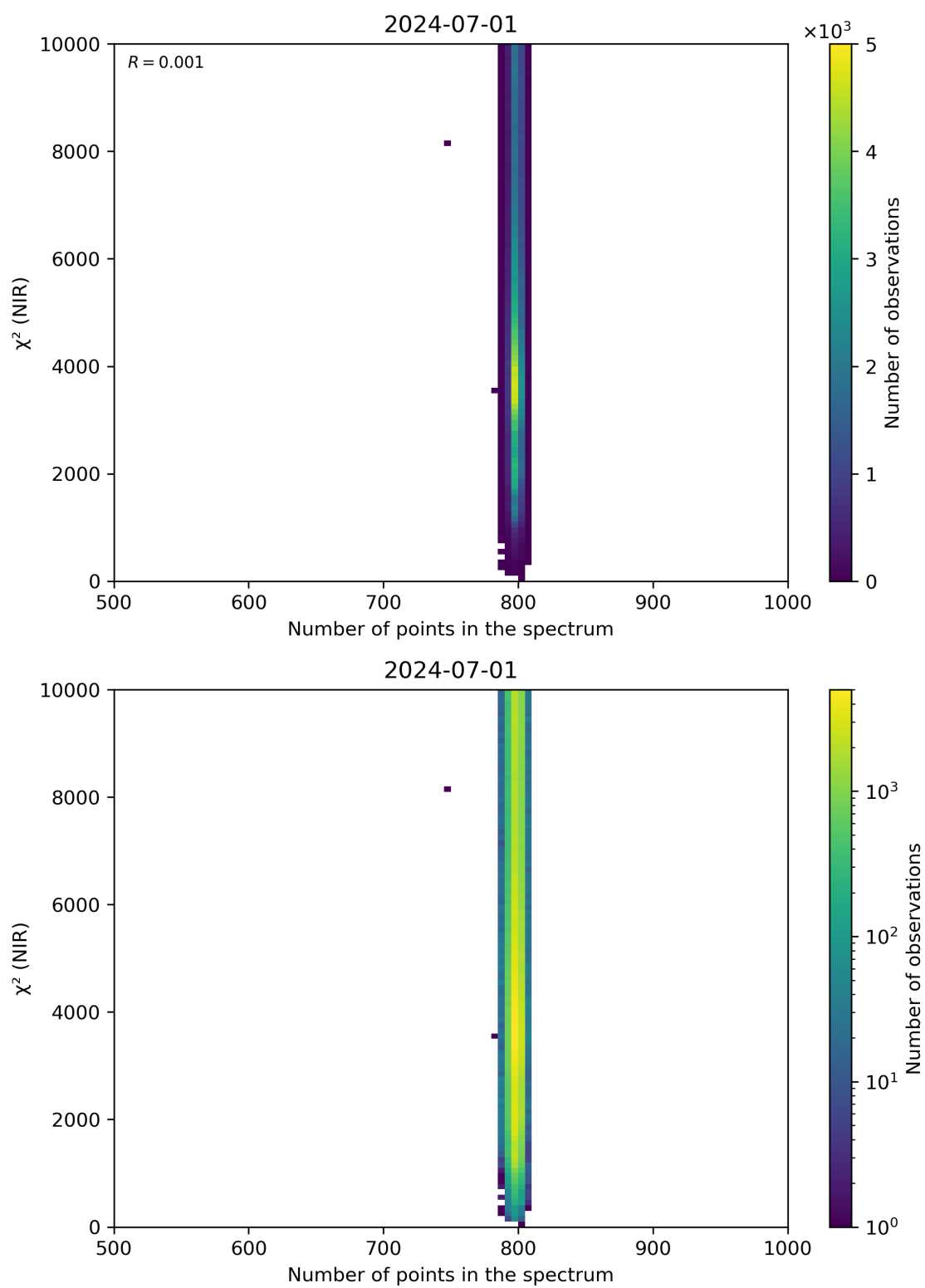
Figure 88: Scatter density plot of “Number of points in the spectrum” against “ \chi^2 (NIR)” for 2024-06-30 to 2024-07-02.
