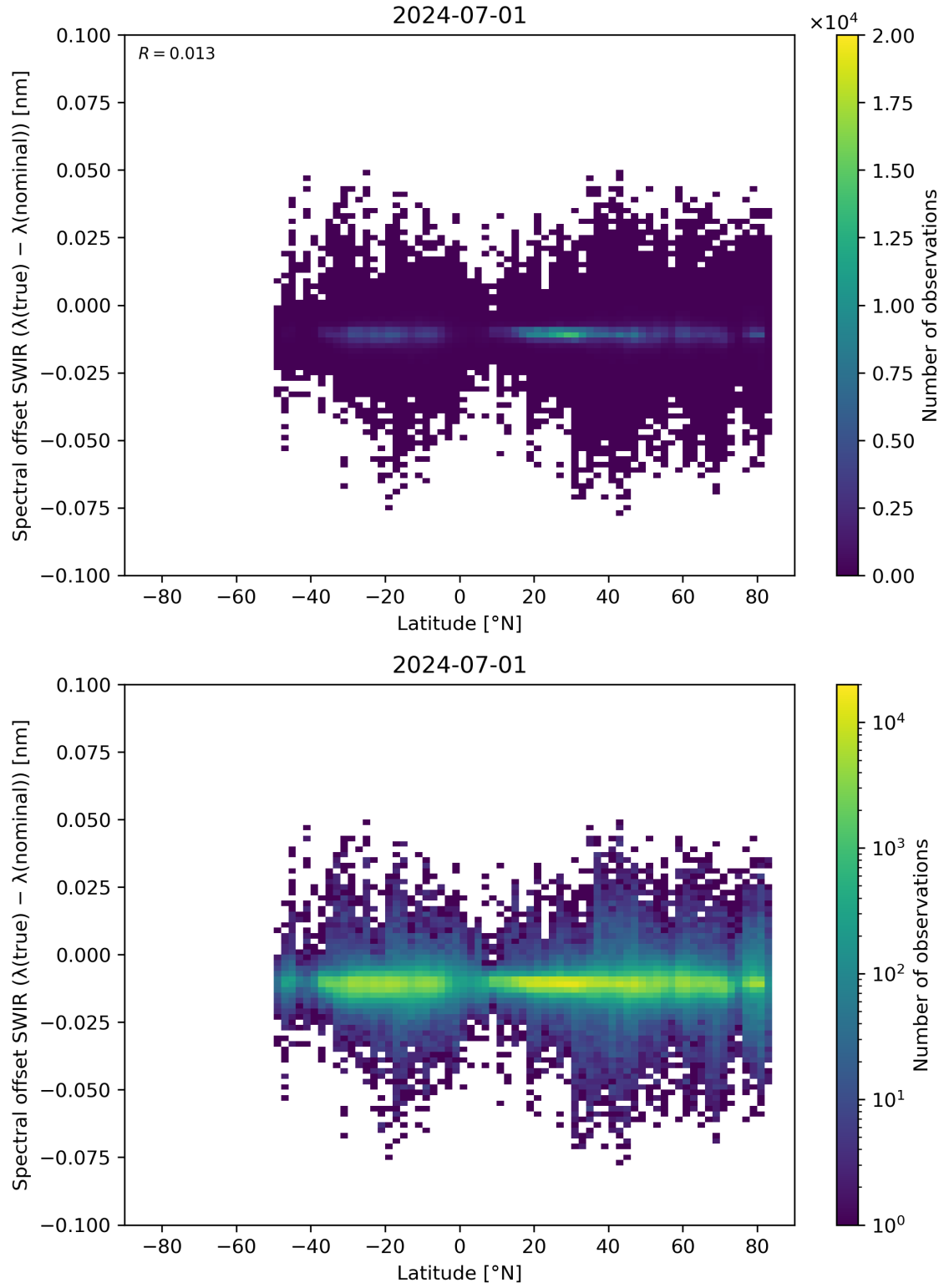
Figure 62: Scatter density plot of “Latitude” against “Spectral offset SWIR ( \lambda(\text{true}) - \lambda(\text{nominal}) )” for 2024-06-30 to 2024-07-02.
