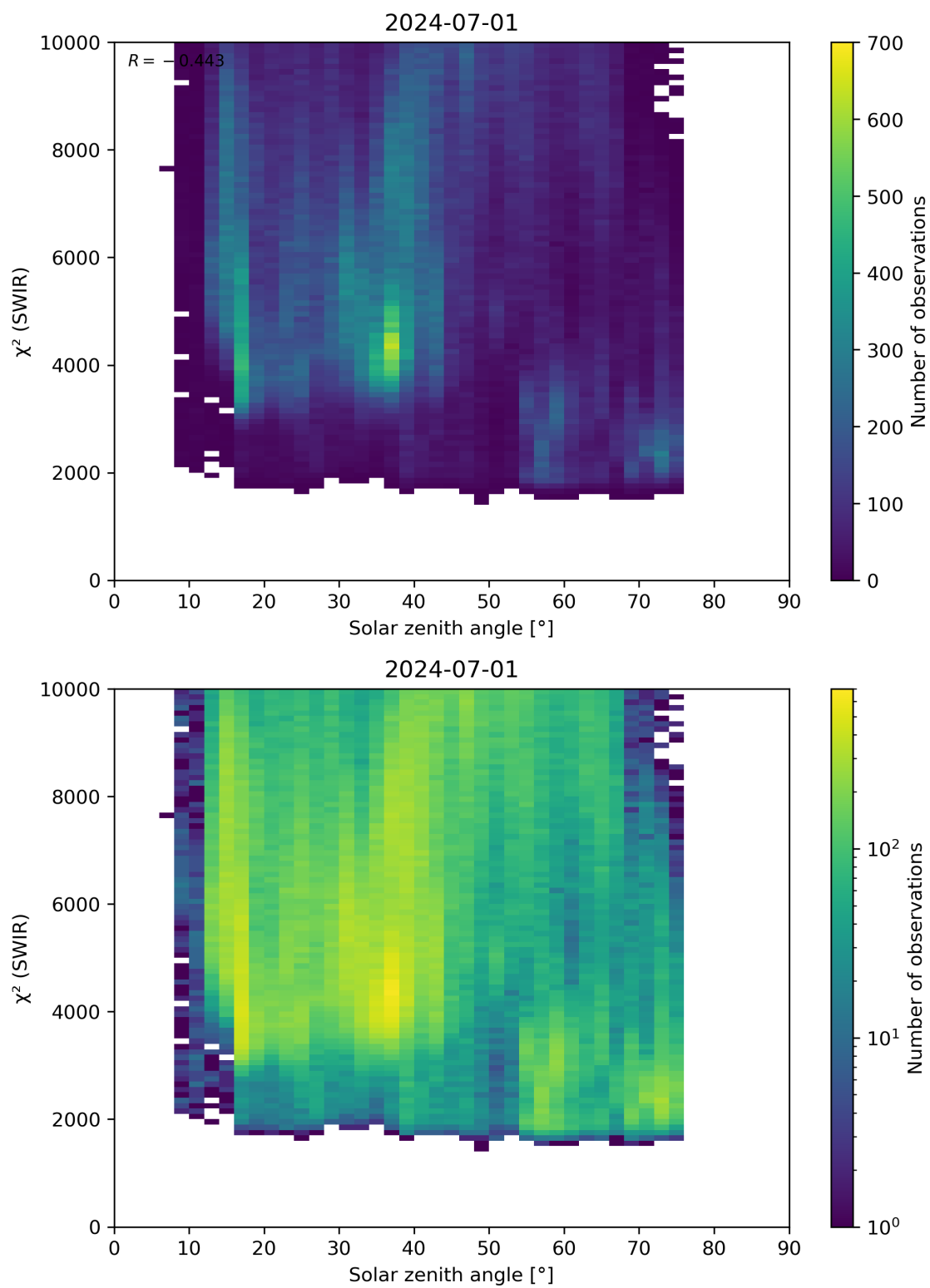
Figure 95: Scatter density plot of “Solar zenith angle” against “ \chi^2 (SWIR)” for 2024-06-30 to 2024-07-02.
