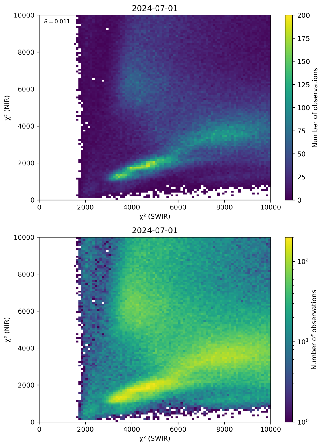
Figure 47: Scatter density plot of “ \chi^2 (SWIR)” against “ \chi^2 (NIR)” for 2024-06-30 to 2024-07-02.
