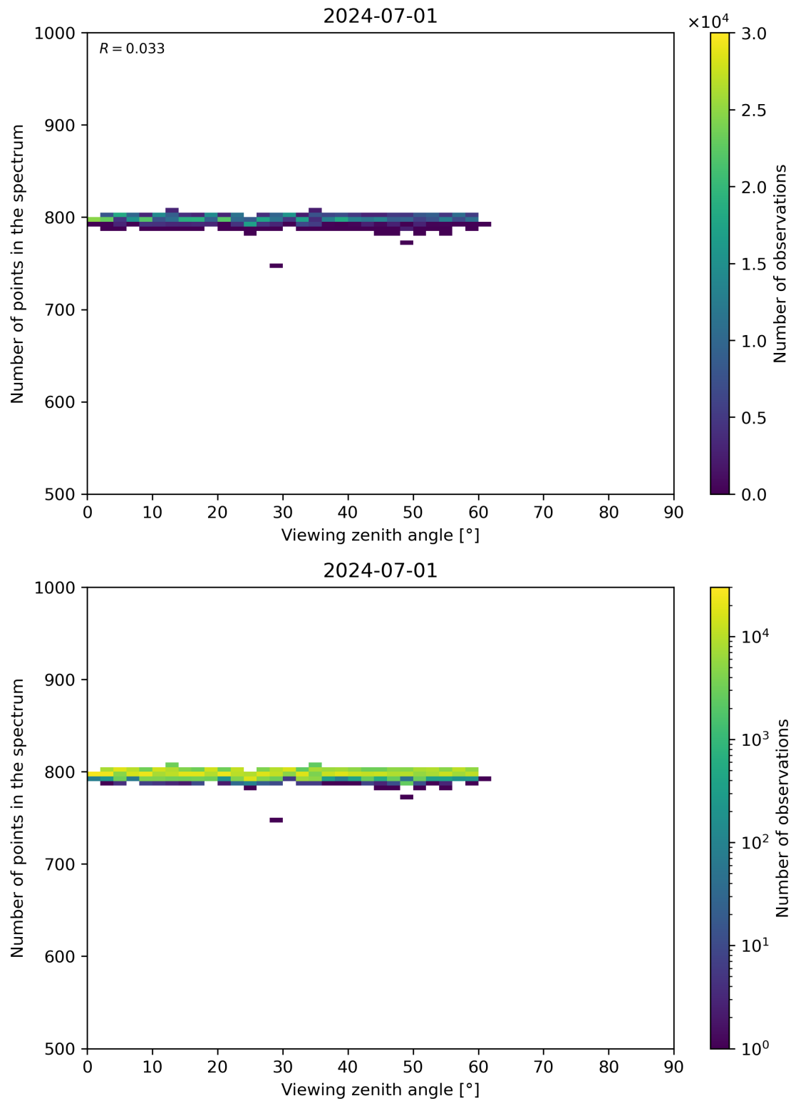
Figure 114: Scatter density plot of “Viewing zenith angle” against “Number of points in the spectrum” for 2024-06-30 to 2024-07-02.
