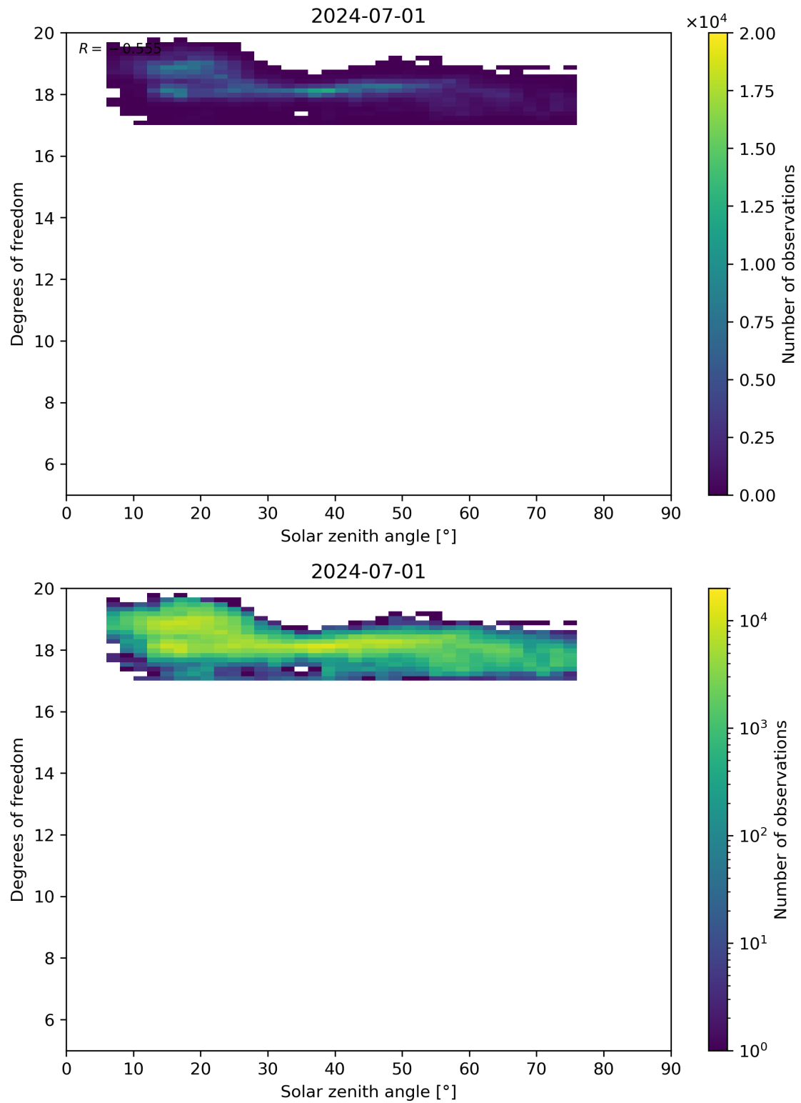
Figure 96: Scatter density plot of “Solar zenith angle” against “Degrees of freedom” for 2024-06-30 to 2024-07-02.
