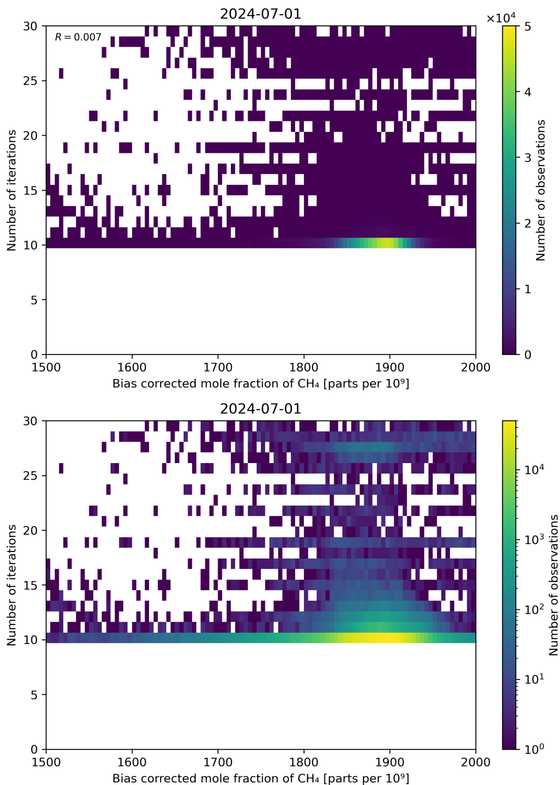
Figure 67: Scatter density plot of “Bias corrected mole fraction of \text{CH}_4 ” against “Number of iterations” for 2024-06-30 to 2024-07-02.
