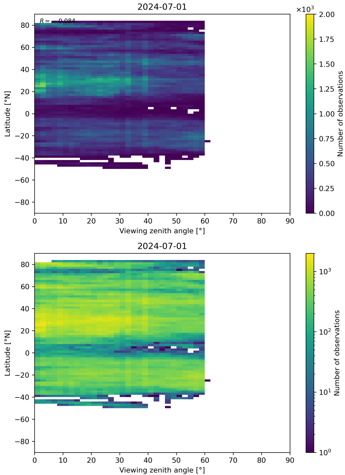
Figure 109: Scatter density plot of “Viewing zenith angle” against “Latitude” for 2024-06-30 to 2024-07-02.
