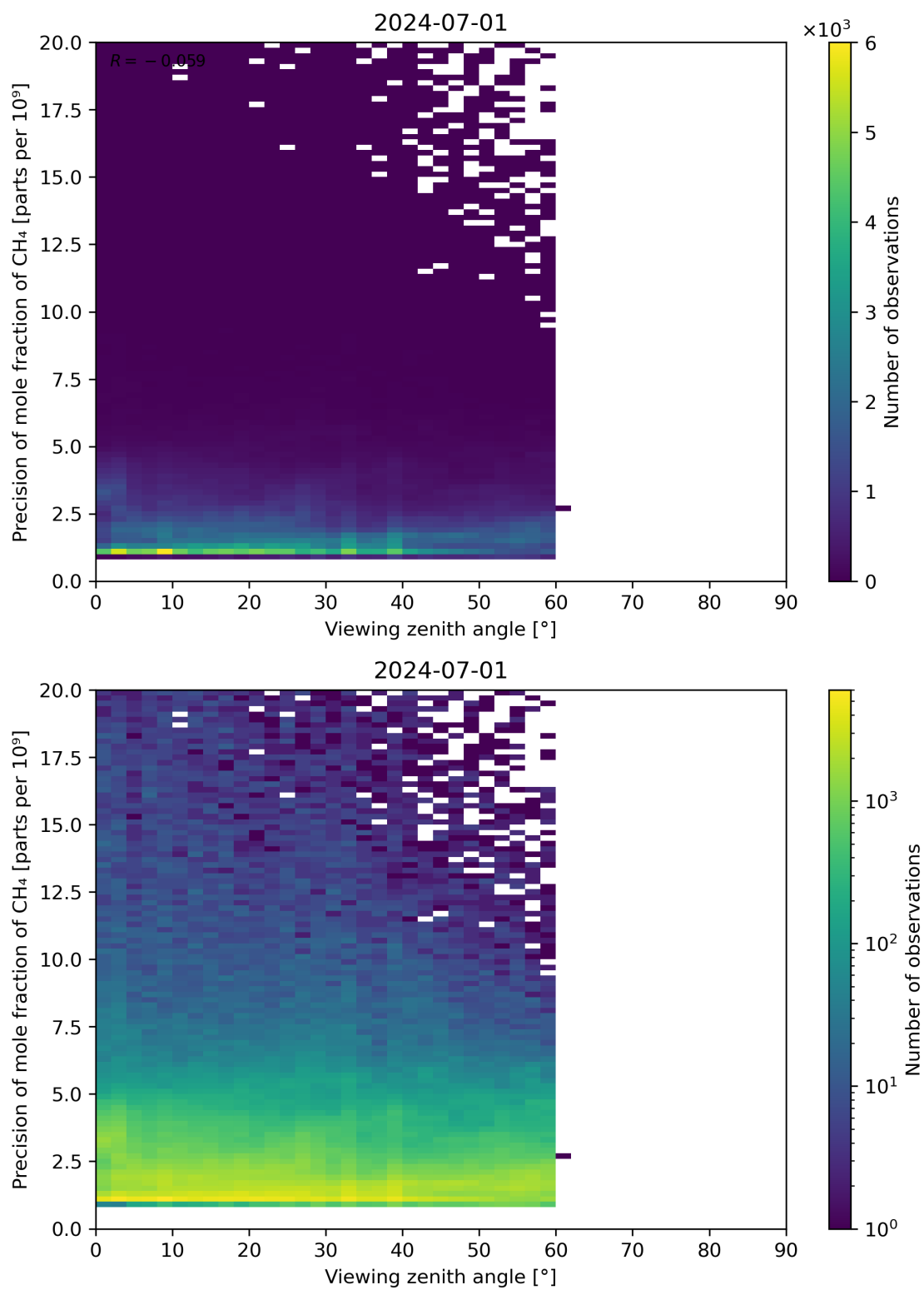
Figure 112: Scatter density plot of “Viewing zenith angle” against “Precision of mole fraction of CH 4 ” for 2024-06-30 to 2024-07-02.
