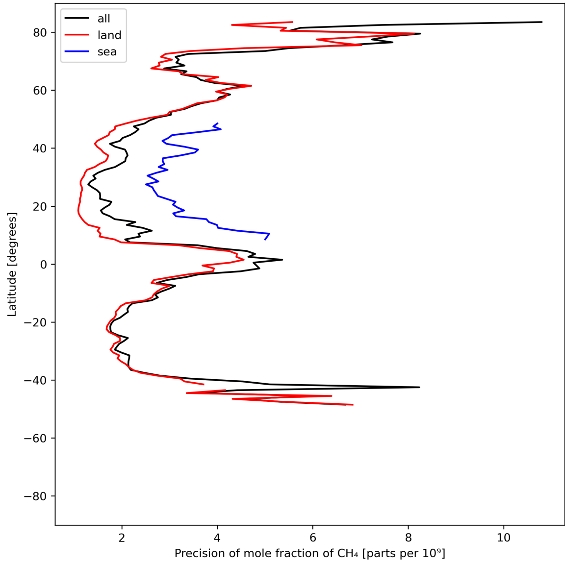
Figure 13: Zonal average of “Precision of mole fraction of CH 4 ” for 2024-06-30 to 2024-07-02.
