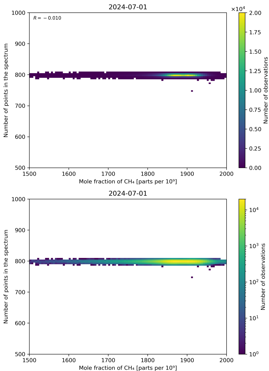
Figure 77: Scatter density plot of “Mole fraction of CH 4 ” against “Number of points in the spectrum” for 2024-06-30 to 2024-07-02.
