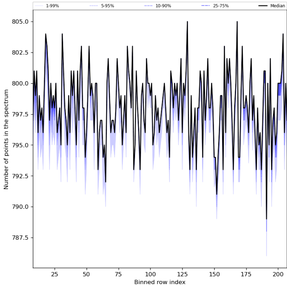
Figure 37: Along track statistics of “Number of points in the spectrum” for 2024-06-30 to 2024-07-02
