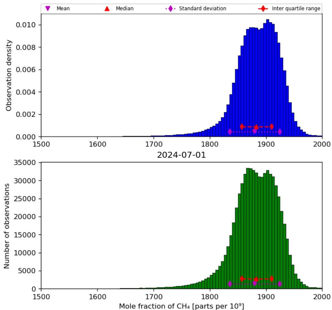
Figure 23: Histogram of “Mole fraction of CH 4 ” for 2024-06-30 to 2024-07-02
