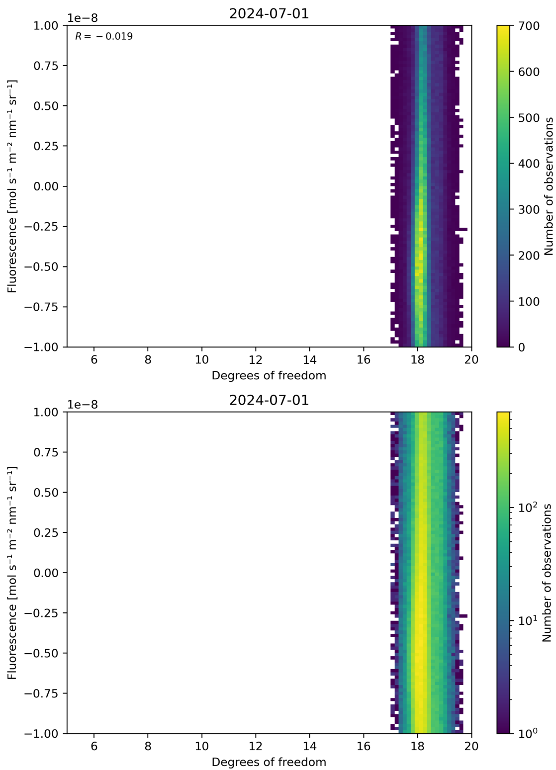
Figure 51: Scatter density plot of “Degrees of freedom” against “Fluorescence” for 2024-06-30 to 2024-07-02.
