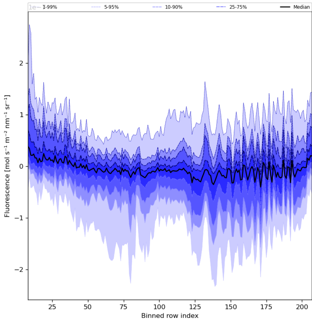
Figure 43: Along track statistics of “Fluorescence” for 2024-06-30 to 2024-07-02
