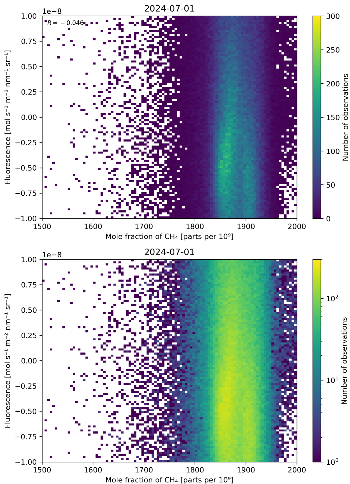
Figure 73: Scatter density plot of “Mole fraction of \text{CH}_4 ” against “Fluorescence” for 2024-06-30 to 2024-07-02.
