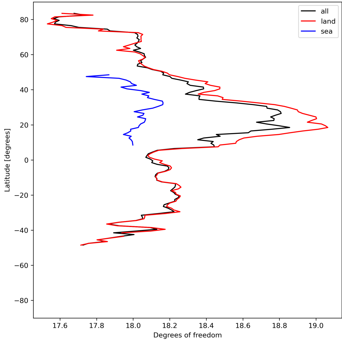
Figure 19: Zonal average of “Degrees of freedom” for 2024-06-30 to 2024-07-02.
