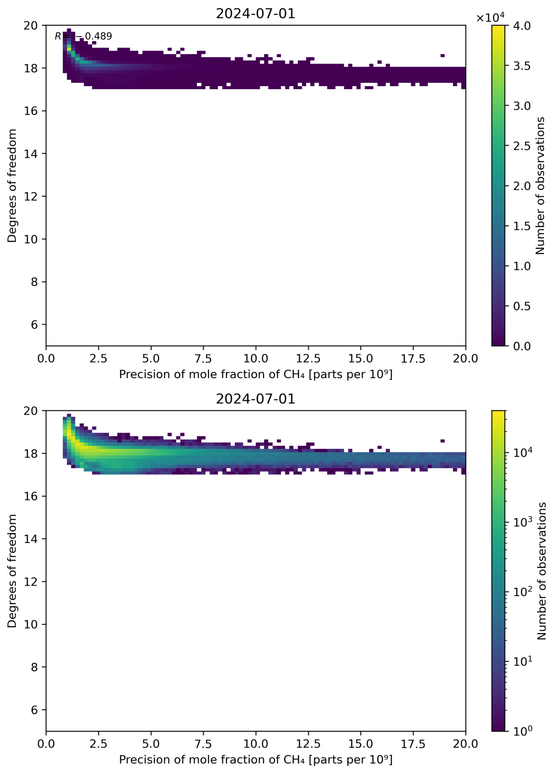
Figure 80: Scatter density plot of “Precision of mole fraction of CH 4 ” against “Degrees of freedom” for 2024-06-30 to 2024-07-02.
