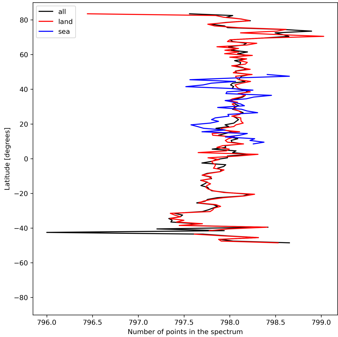
Figure 15: Zonal average of “Number of points in the spectrum” for 2024-06-30 to 2024-07-02.
