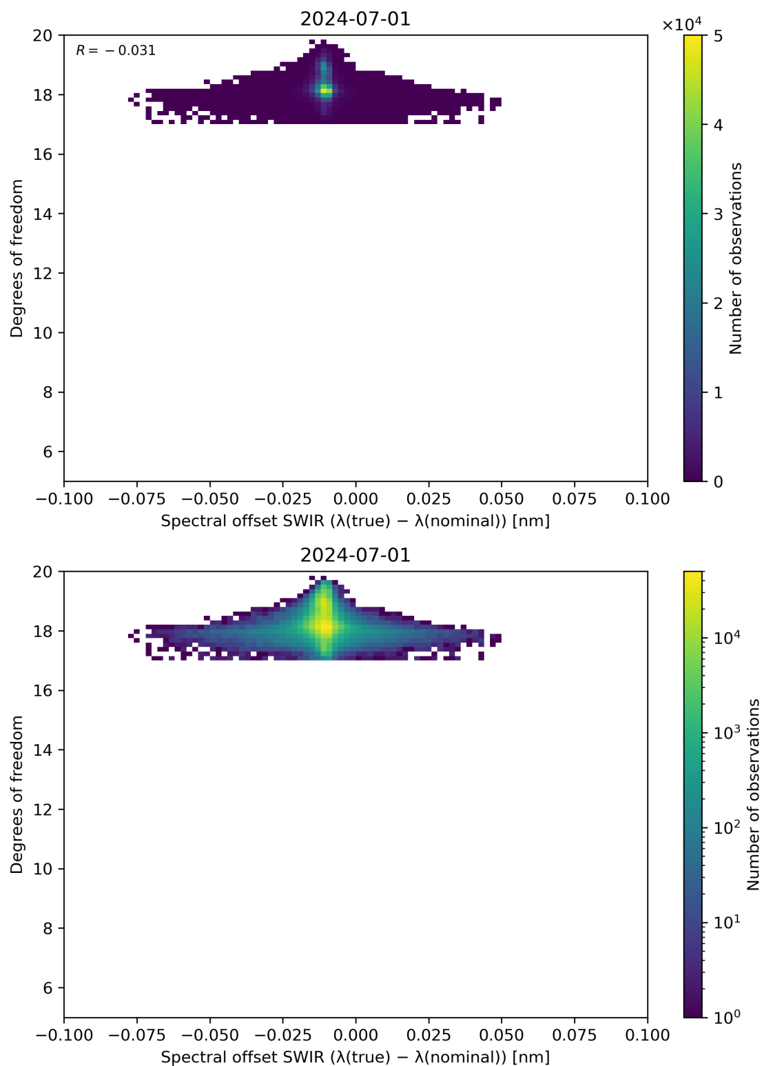
Figure 119: Scatter density plot of “Spectral offset SWIR ( \lambda(\text{true}) - \lambda(\text{nominal}) )” against “Degrees of freedom” for 2024-06-30 to 2024-07-02.
