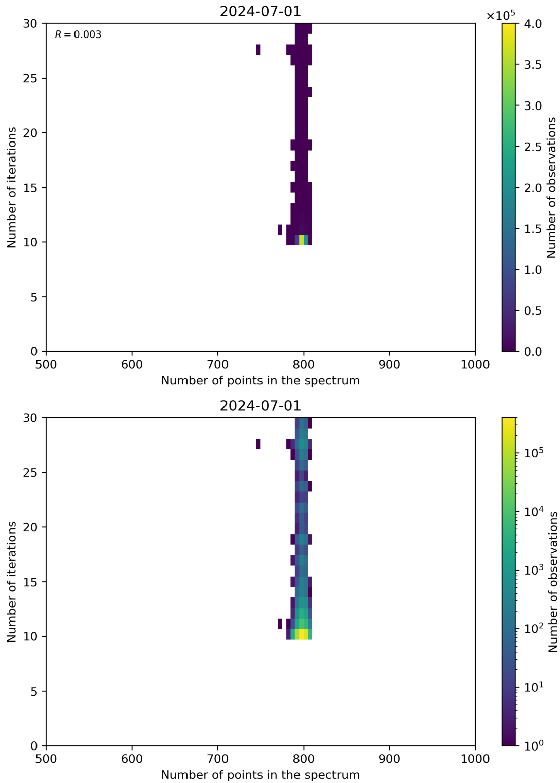
Figure 92: Scatter density plot of “Number of points in the spectrum” against “Number of iterations” for 2024-06-30 to 2024-07-02.
