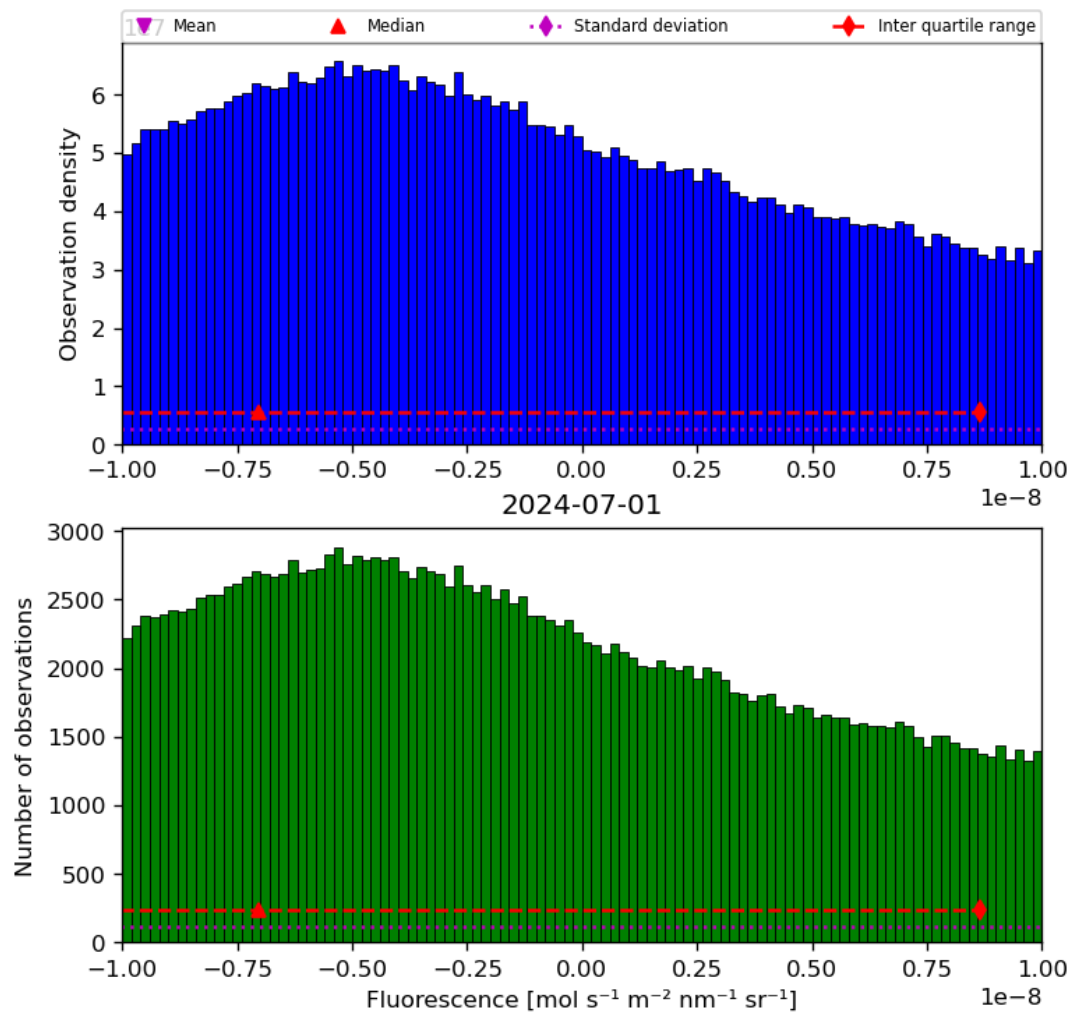
Figure 32: Histogram of “Fluorescence” for 2024-06-30 to 2024-07-02
