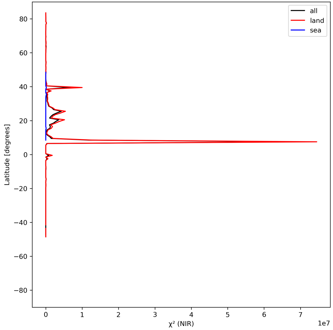
Figure 18: Zonal average of “ \chi^2 (NIR)” for 2024-06-30 to 2024-07-02.
