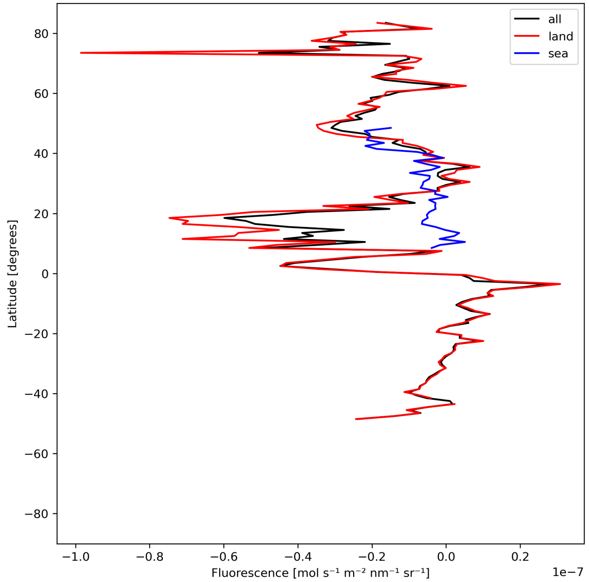
Figure 21: Zonal average of “Fluorescence” for 2024-06-30 to 2024-07-02.
