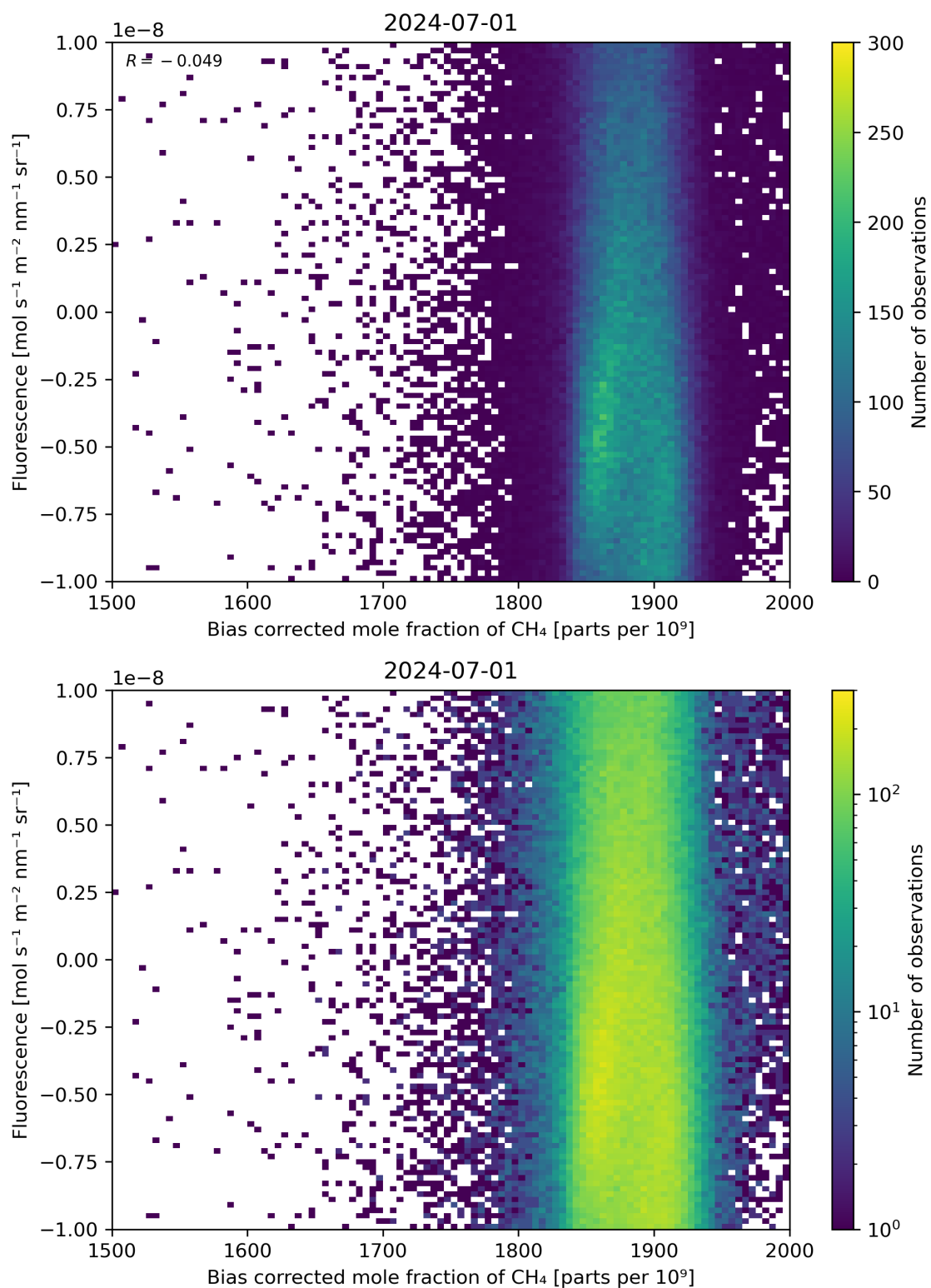
Figure 66: Scatter density plot of “Bias corrected mole fraction of \text{CH}_4 ” against “Fluorescence” for 2024-06-30 to 2024-07-02.
