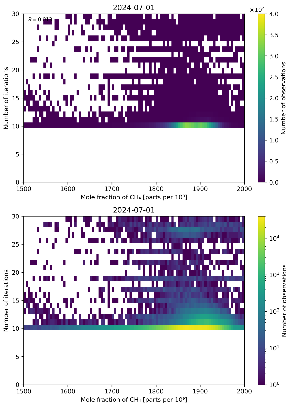
Figure 76: Scatter density plot of “Mole fraction of CH 4 ” against “Number of iterations” for 2024-06-30 to 2024-07-02.
