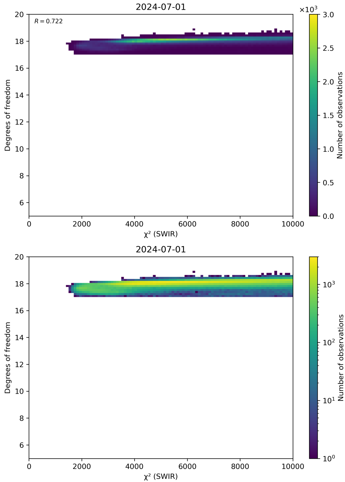
Figure 48: Scatter density plot of “ \chi^2 (SWIR)” against “Degrees of freedom” for 2024-06-30 to 2024-07-02.
