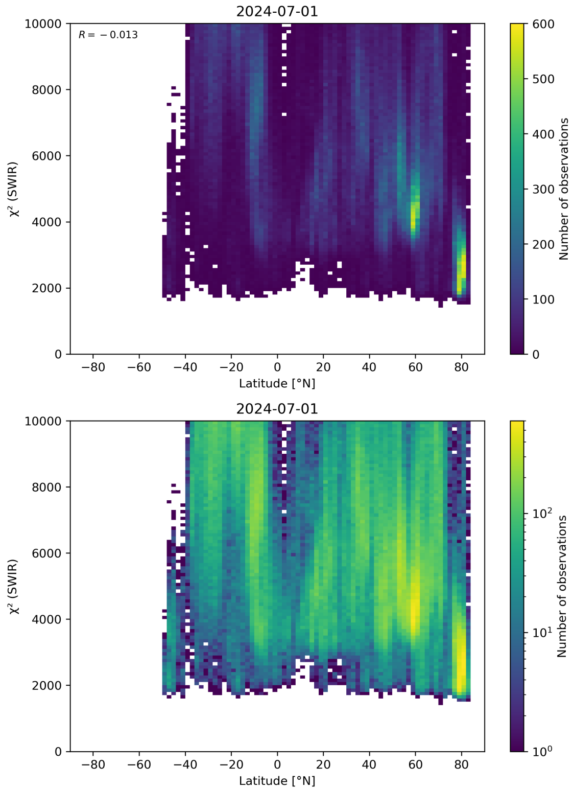
Figure 54: Scatter density plot of “Latitude” against “ \chi^2 (SWIR)” for 2024-06-30 to 2024-07-02.
