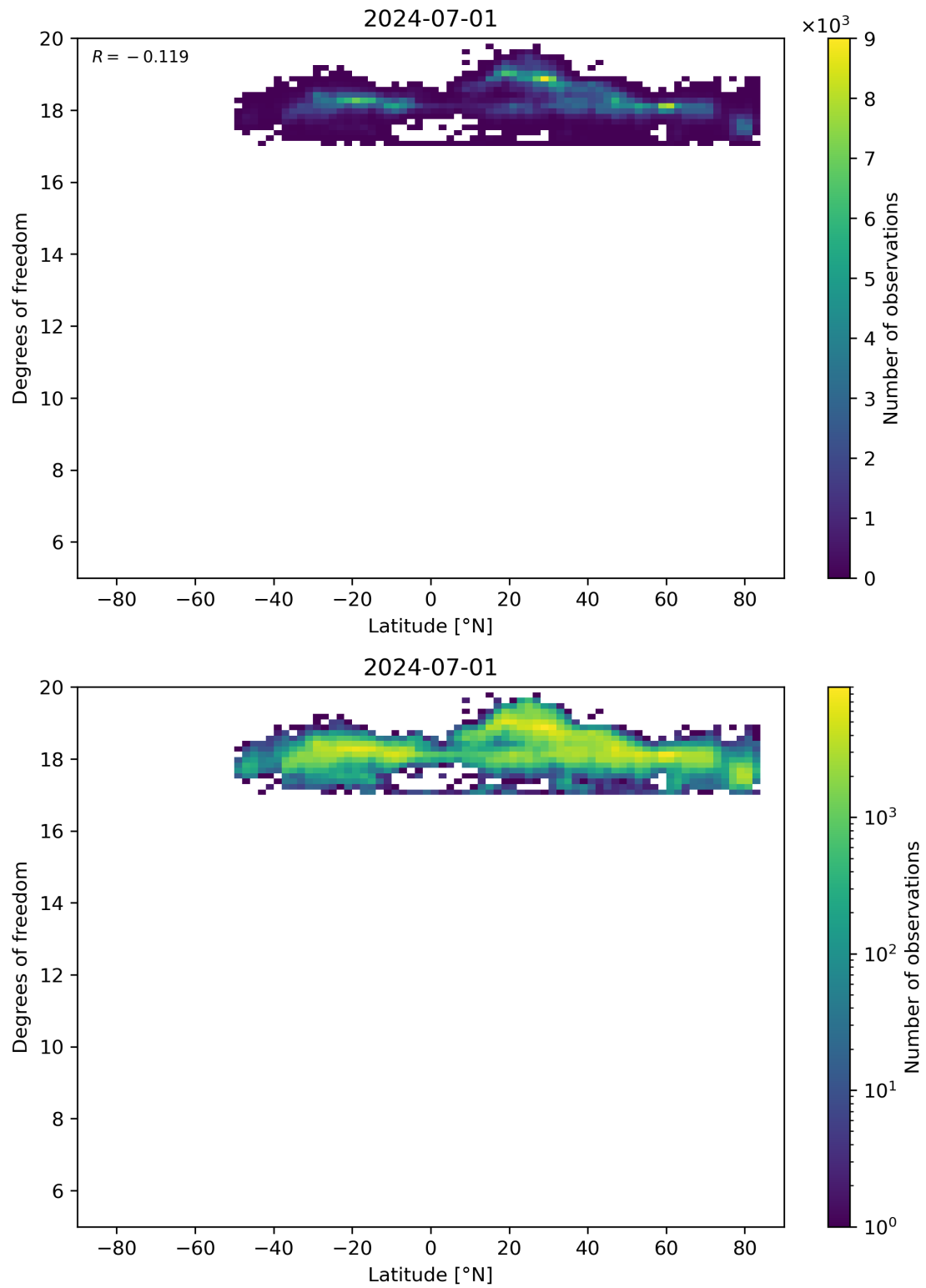
Figure 55: Scatter density plot of “Latitude” against “Degrees of freedom” for 2024-06-30 to 2024-07-02.
