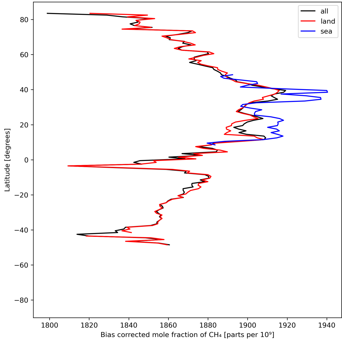
Figure 14: Zonal average of “Bias corrected mole fraction of CH 4 ” for 2024-06-30 to 2024-07-02.
