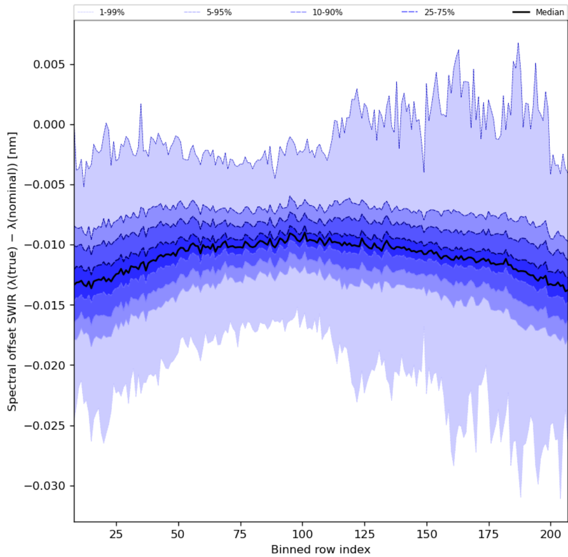
Figure 38: Along track statistics of “Spectral offset SWIR ( \lambda(\text{true}) - \lambda(\text{nominal}) )” for 2024-06-30 to 2024-07-02
