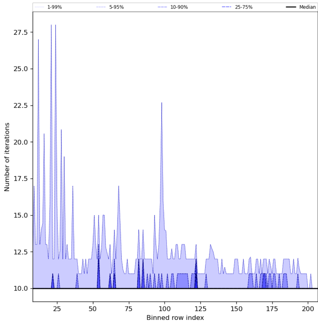
Figure 42: Along track statistics of “Number of iterations” for 2024-06-30 to 2024-07-02
