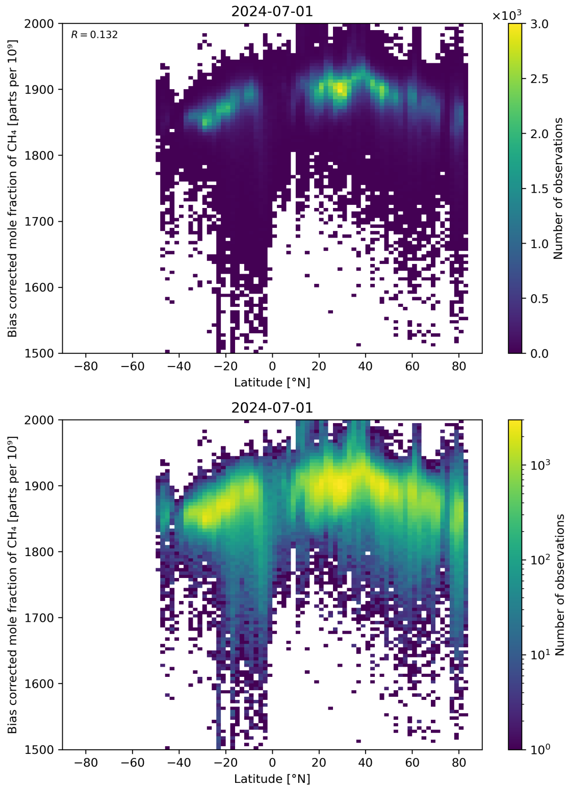
Figure 58: Scatter density plot of “Latitude” against “Bias corrected mole fraction of \text{CH}_4 ” for 2024-06-30 to 2024-07-02.
