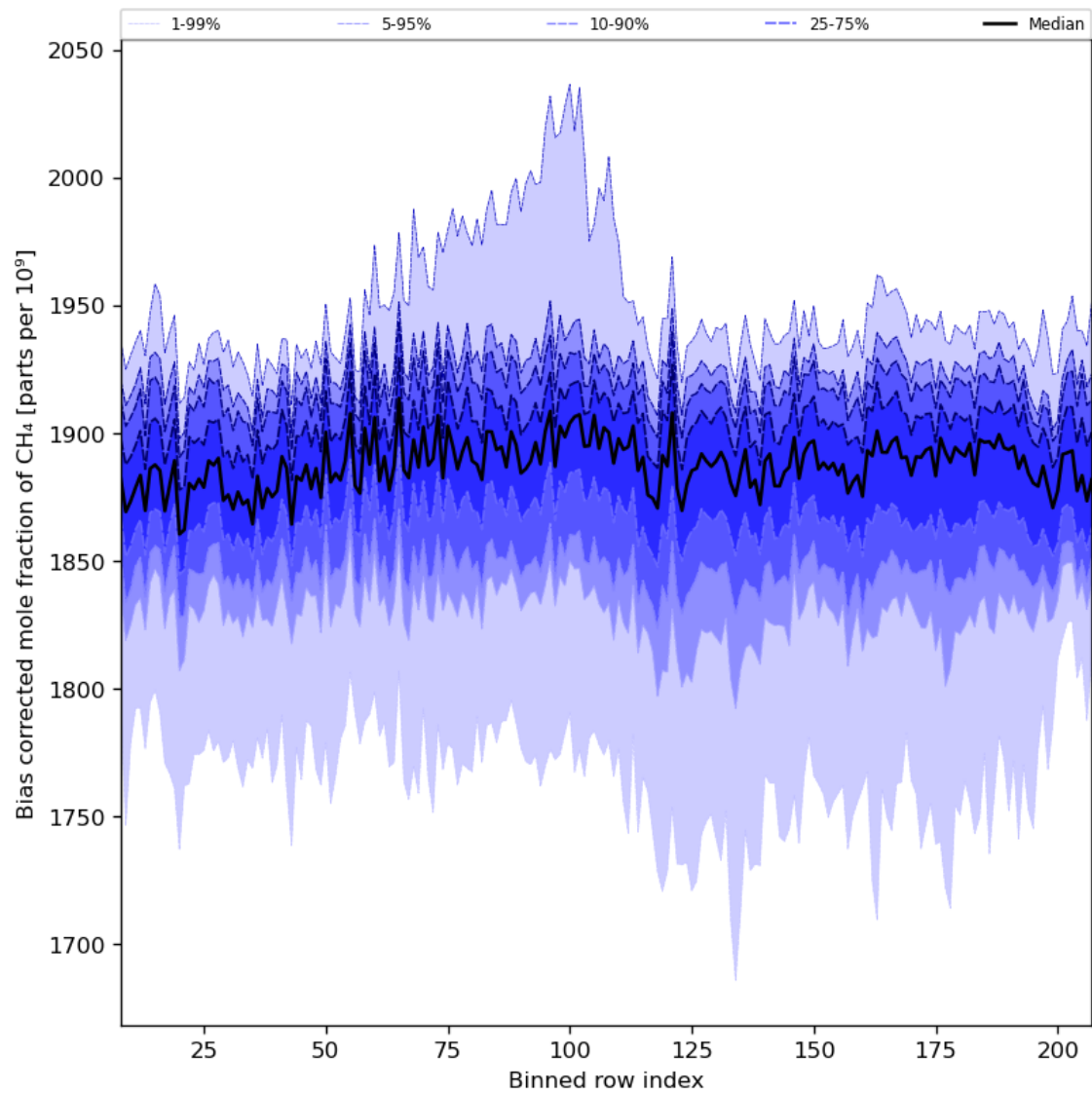
Figure 36: Along track statistics of “Bias corrected mole fraction of CH 4 ” for 2024-06-30 to 2024-07-02
