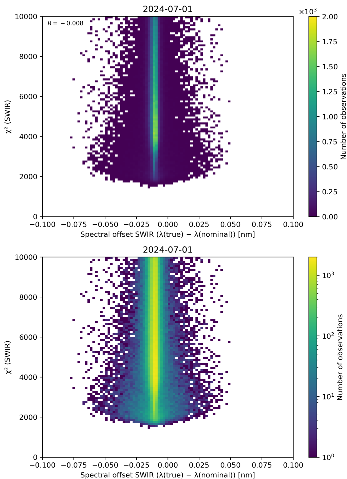
Figure 118: Scatter density plot of “Spectral offset SWIR ( \lambda(\text{true}) - \lambda(\text{nominal}) )” against “ \chi^2 (SWIR)” for 2024-06-30 to 2024-07-02.
