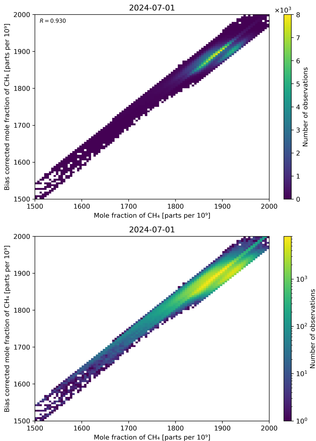
Figure 74: Scatter density plot of “Mole fraction of CH 4 ” against “Bias corrected mole fraction of CH 4 ” for 2024-06-30 to 2024-07-02.
