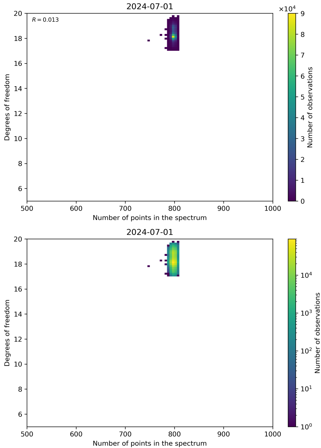
Figure 90: Scatter density plot of “Number of points in the spectrum” against “Degrees of freedom” for 2024-06-30 to 2024-07-02.
