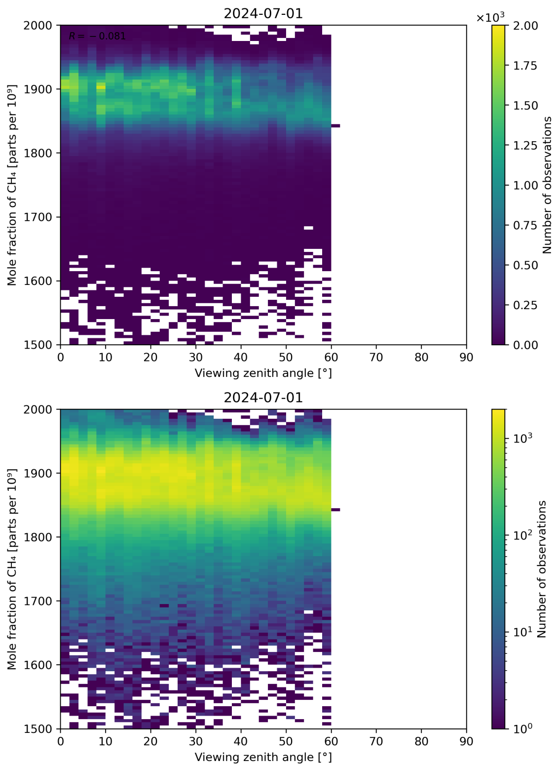
Figure 110: Scatter density plot of “Viewing zenith angle” against “Mole fraction of CH 4 ” for 2024-06-30 to 2024-07-02.
