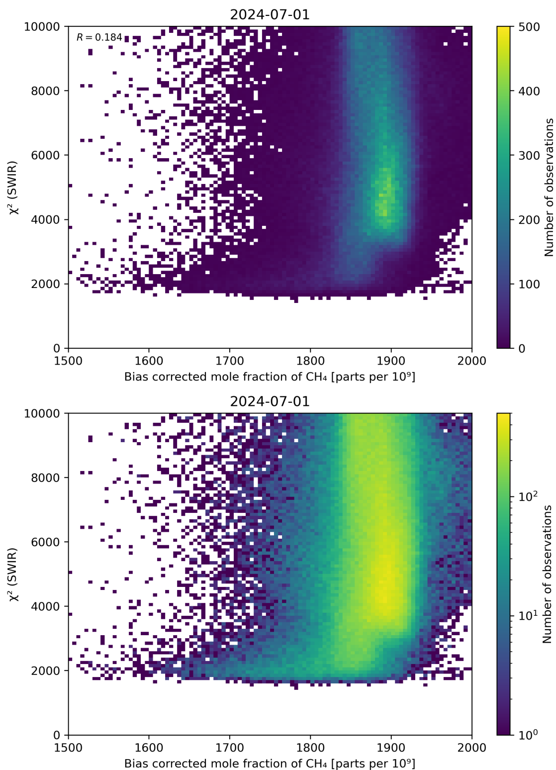
Figure 64: Scatter density plot of “Bias corrected mole fraction of CH 4 ” against “ \chi^2 (SWIR)” for 2024-06-30 to 2024-07-02.
