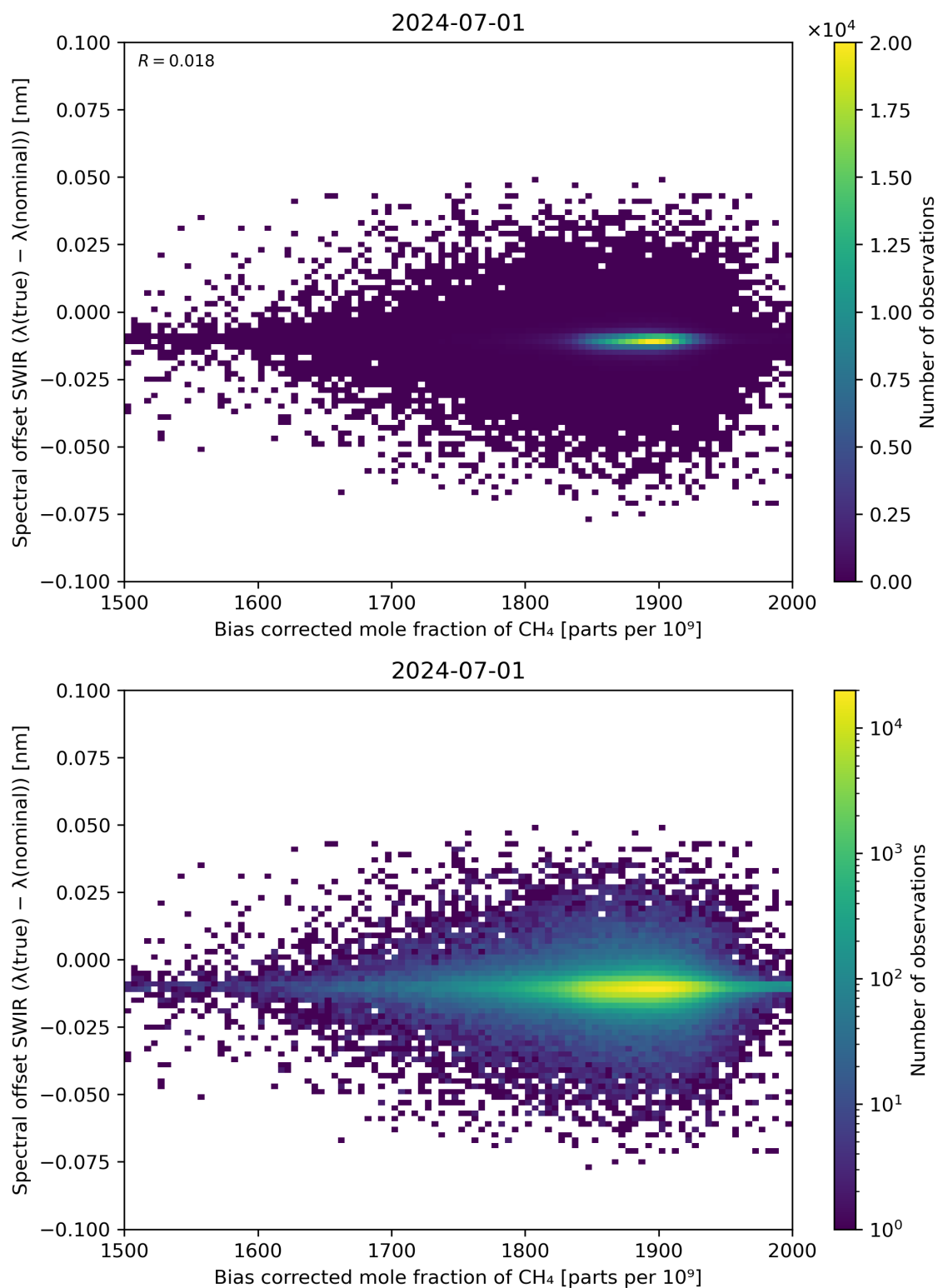
Figure 69: Scatter density plot of “Bias corrected mole fraction of \text{CH}_4 ” against “Spectral offset SWIR ( \lambda(\text{true}) - \lambda(\text{nominal}) )” for 2024-06-30 to 2024-07-02.
