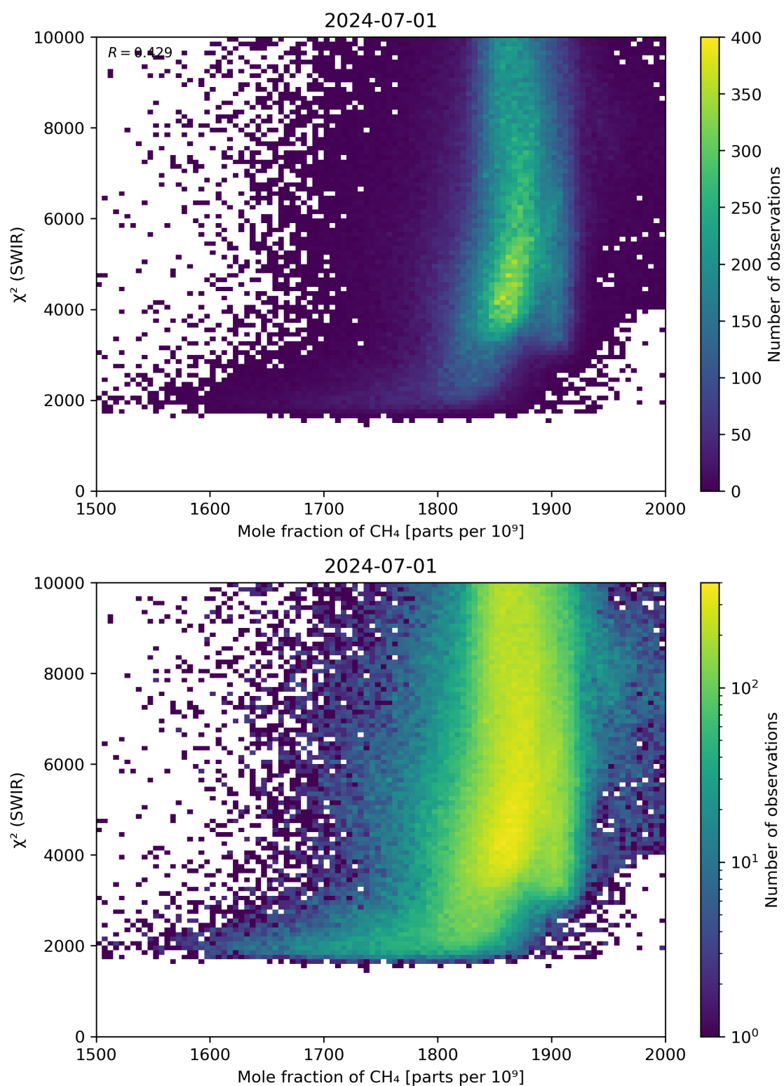
Figure 71: Scatter density plot of “Mole fraction of \text{CH}_4 ” against “ \chi^2 (SWIR)” for 2024-06-30 to 2024-07-02.
