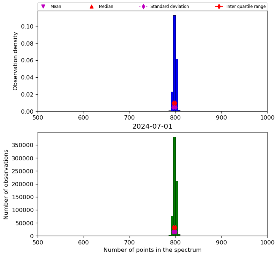
Figure 26: Histogram of “Number of points in the spectrum” for 2024-06-30 to 2024-07-02
