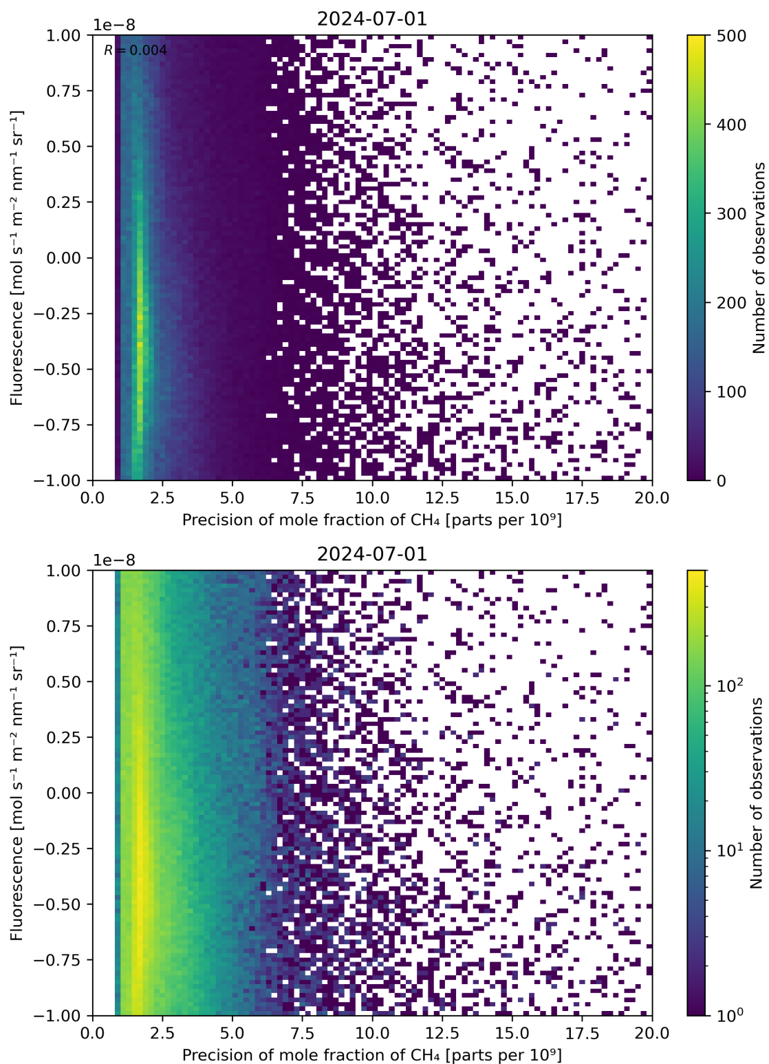
Figure 81: Scatter density plot of “Precision of mole fraction of \text{CH}_4 ” against “Fluorescence” for 2024-06-30 to 2024-07-02.
