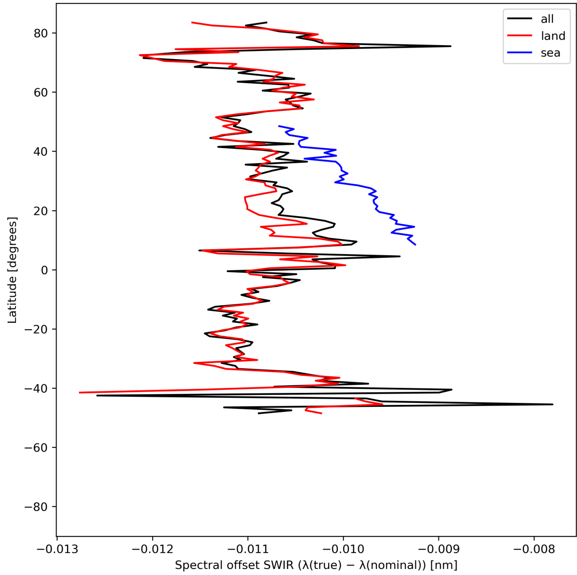
Figure 16: Zonal average of “Spectral offset SWIR ( \lambda(\text{true}) - \lambda(\text{nominal}) )” for 2024-06-30 to 2024-07-02.
