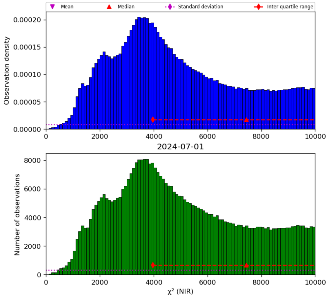
Figure 29: Histogram of " \chi^2 (NIR)" for 2024-06-30 to 2024-07-02
