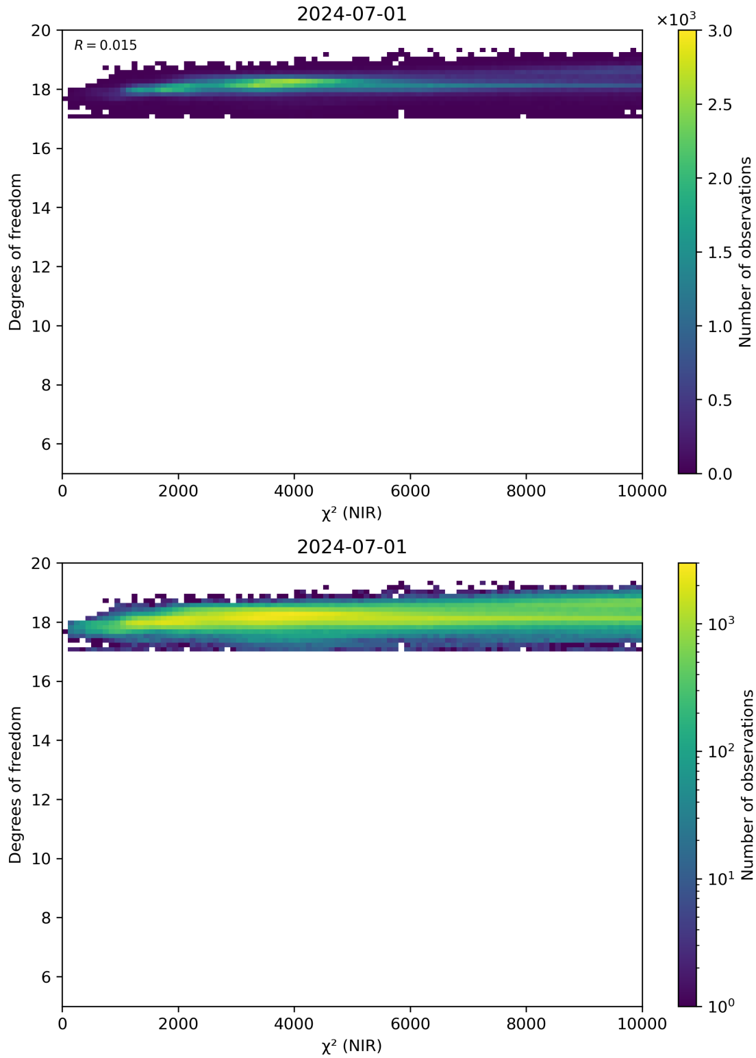
Figure 44: Scatter density plot of “ \chi^2 (NIR)” against “Degrees of freedom” for 2024-06-30 to 2024-07-02.
