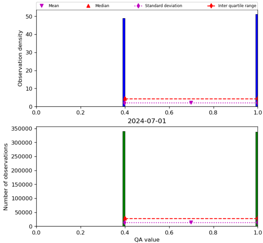
Figure 22: Histogram of “QA value” for 2024-06-30 to 2024-07-02
