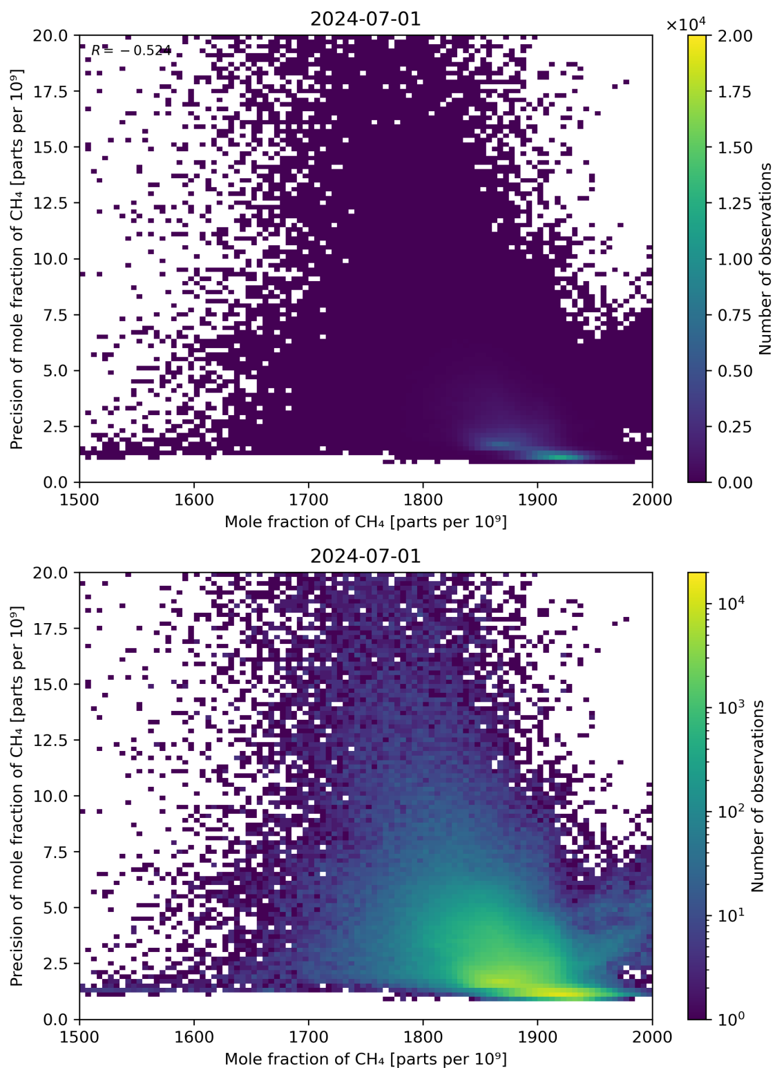
Figure 75: Scatter density plot of “Mole fraction of CH 4 ” against “Precision of mole fraction of CH 4 ” for 2024-06-30 to 2024-07-02.
