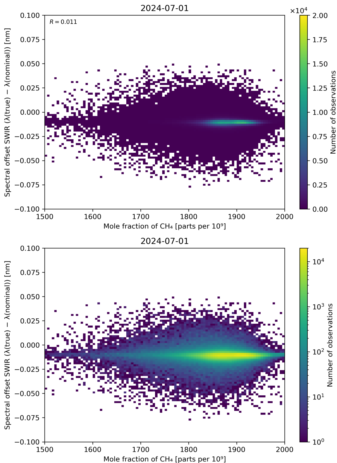
Figure 86: Scatter density plot of “Mole fraction of CH 4 ” against “Spectral offset SWIR ( \lambda(\text{true}) - \lambda(\text{nominal}) )” for 2024-06-30 to 2024-07-02.
