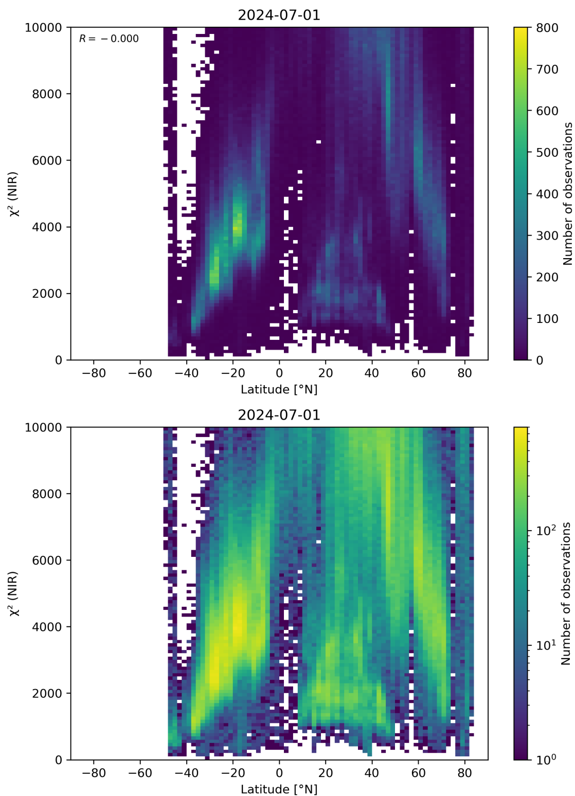
Figure 53: Scatter density plot of “Latitude” against “ \chi^2 (NIR)” for 2024-06-30 to 2024-07-02.
