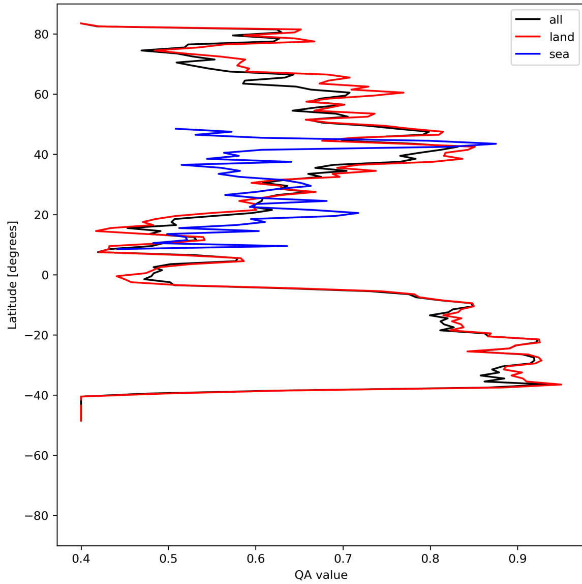
Figure 11: Zonal average of “QA value” for 2024-06-30 to 2024-07-02.
