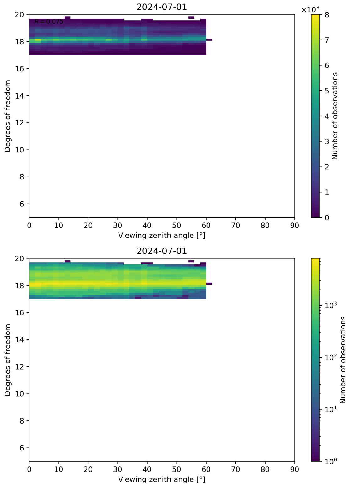
Figure 107: Scatter density plot of “Viewing zenith angle” against “Degrees of freedom” for 2024-06-30 to 2024-07-02.
