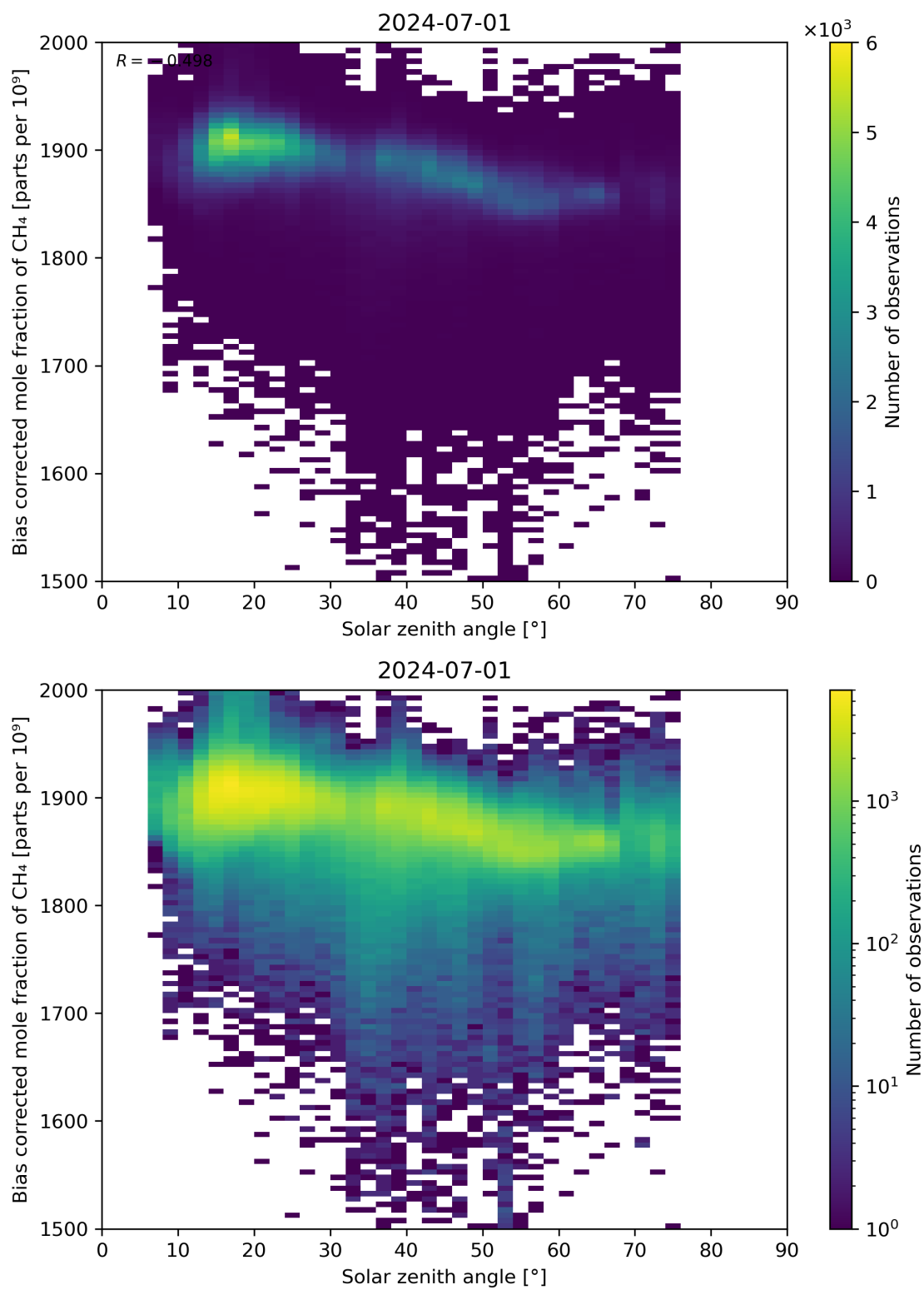
Figure 100: Scatter density plot of “Solar zenith angle” against “Bias corrected mole fraction of CH 4 ” for 2024-06-30 to 2024-07-02.
