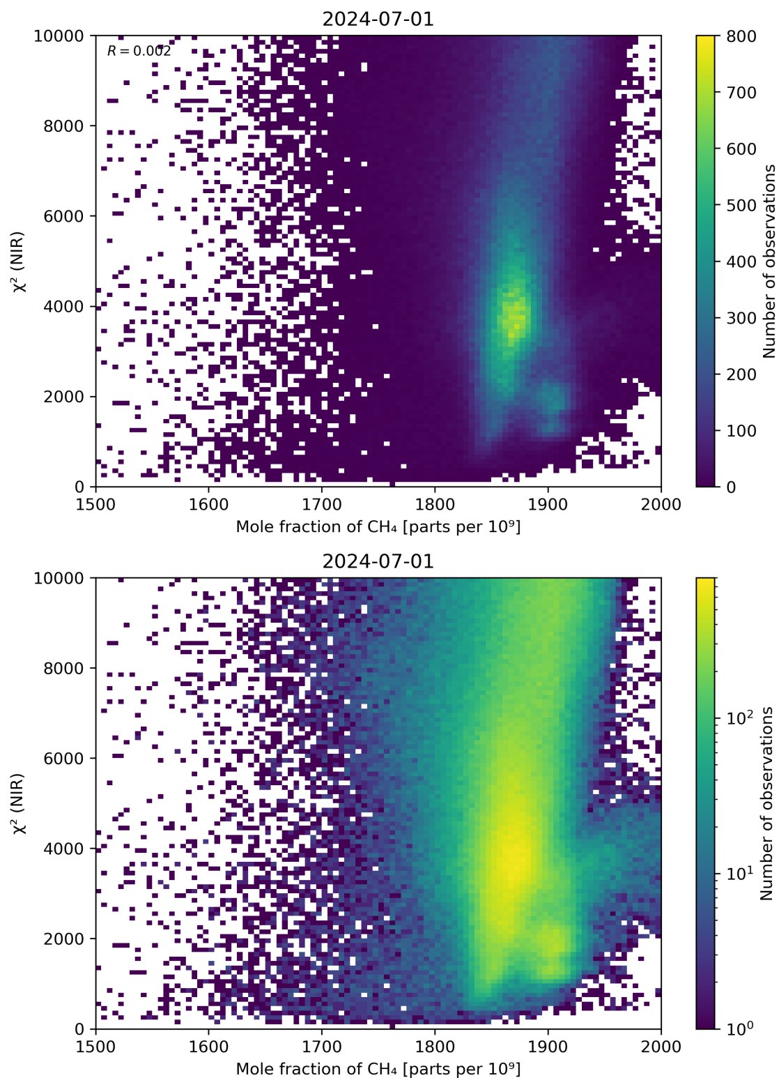
Figure 70: Scatter density plot of “Mole fraction of CH 4 ” against “ \chi^2 (NIR)” for 2024-06-30 to 2024-07-02.
