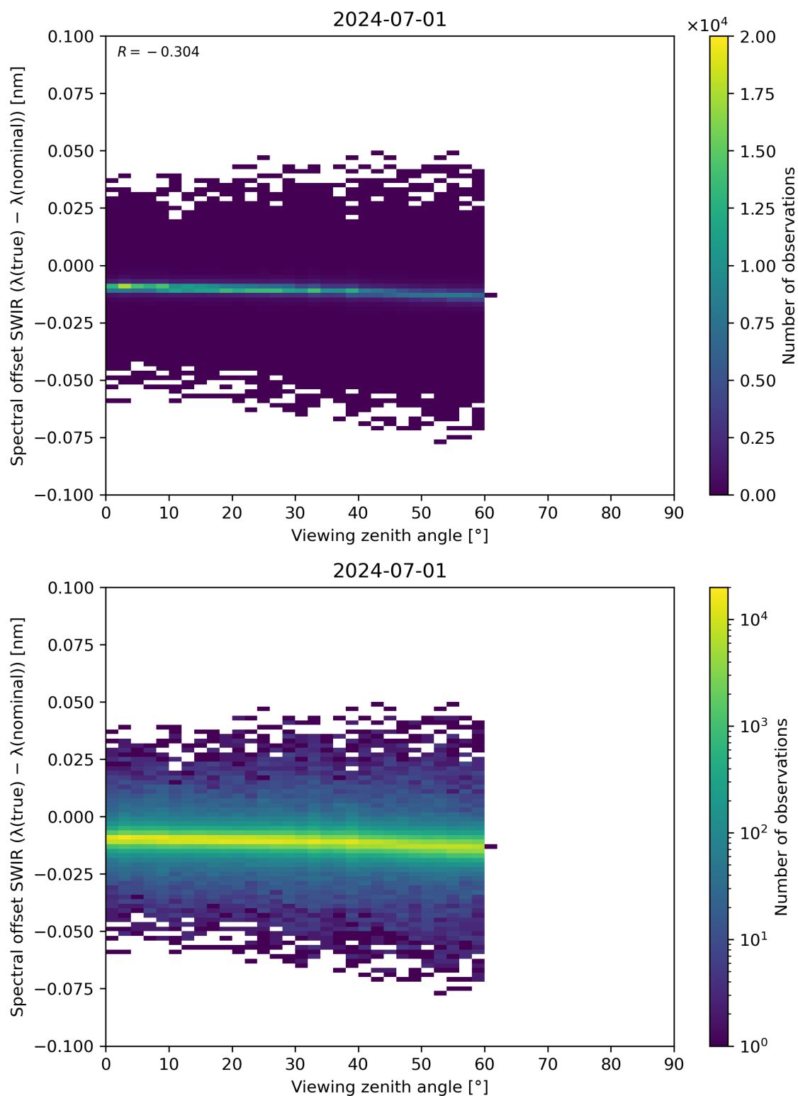
Figure 116: Scatter density plot of “Viewing zenith angle” against “Spectral offset SWIR ( \lambda(\text{true}) - \lambda(\text{nominal}) )” for 2024-06-30 to 2024-07-02.
