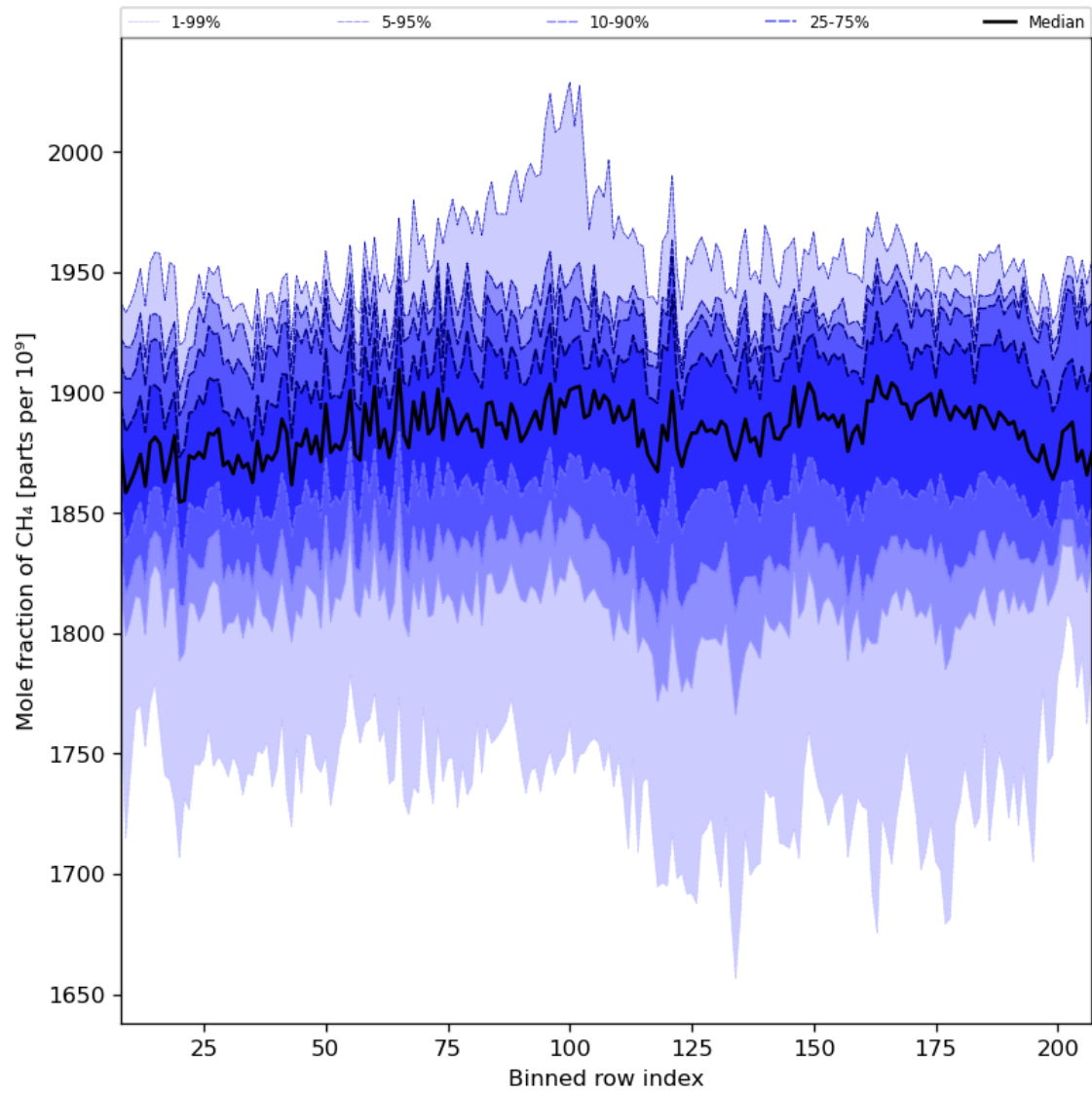
Figure 34: Along track statistics of “Mole fraction of CH 4 ” for 2024-06-30 to 2024-07-02
