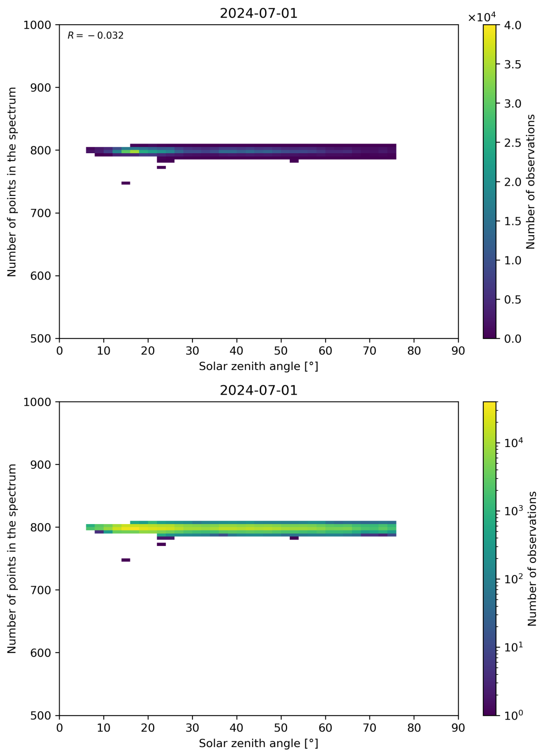
Figure 103: Scatter density plot of “Solar zenith angle” against “Number of points in the spectrum” for 2024-06-30 to 2024-07-02.
