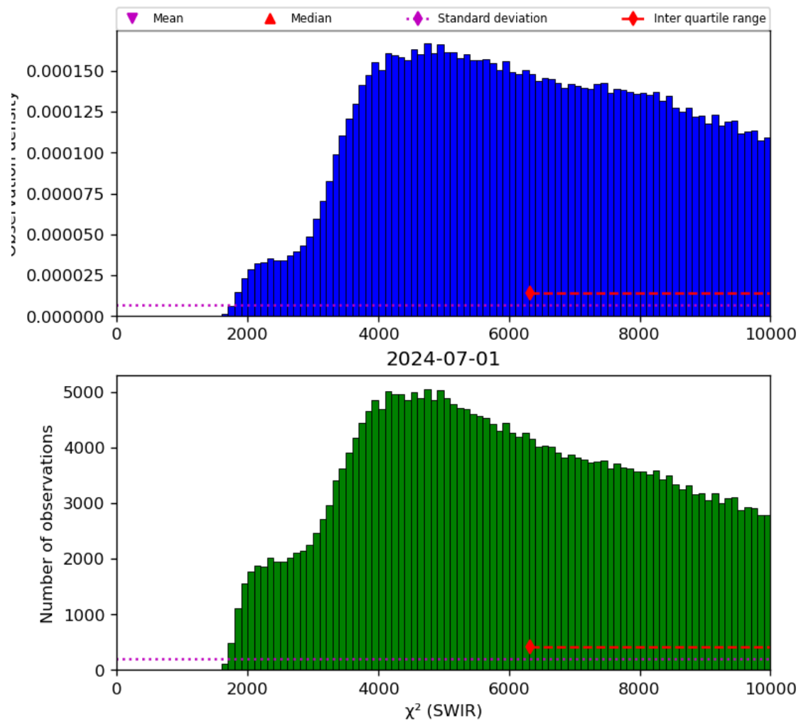
Figure 28: Histogram of “ \chi^2 (SWIR)” for 2024-06-30 to 2024-07-02
