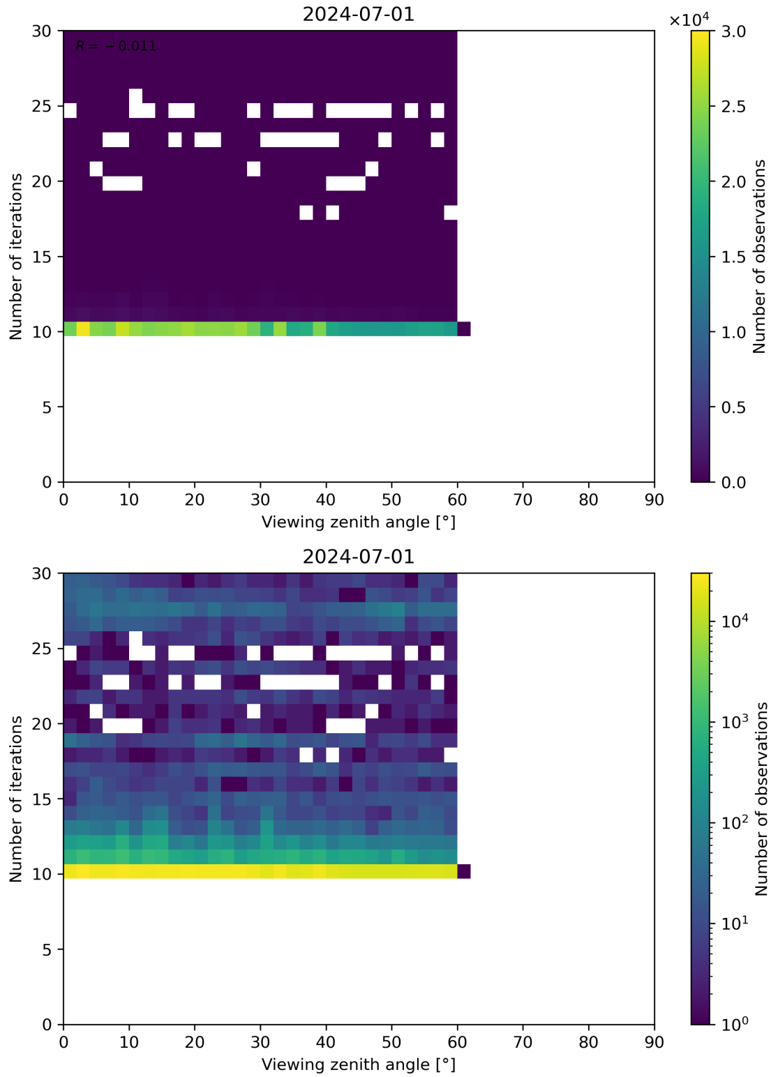
Figure 113: Scatter density plot of “Viewing zenith angle” against “Number of iterations” for 2024-06-30 to 2024-07-02.
