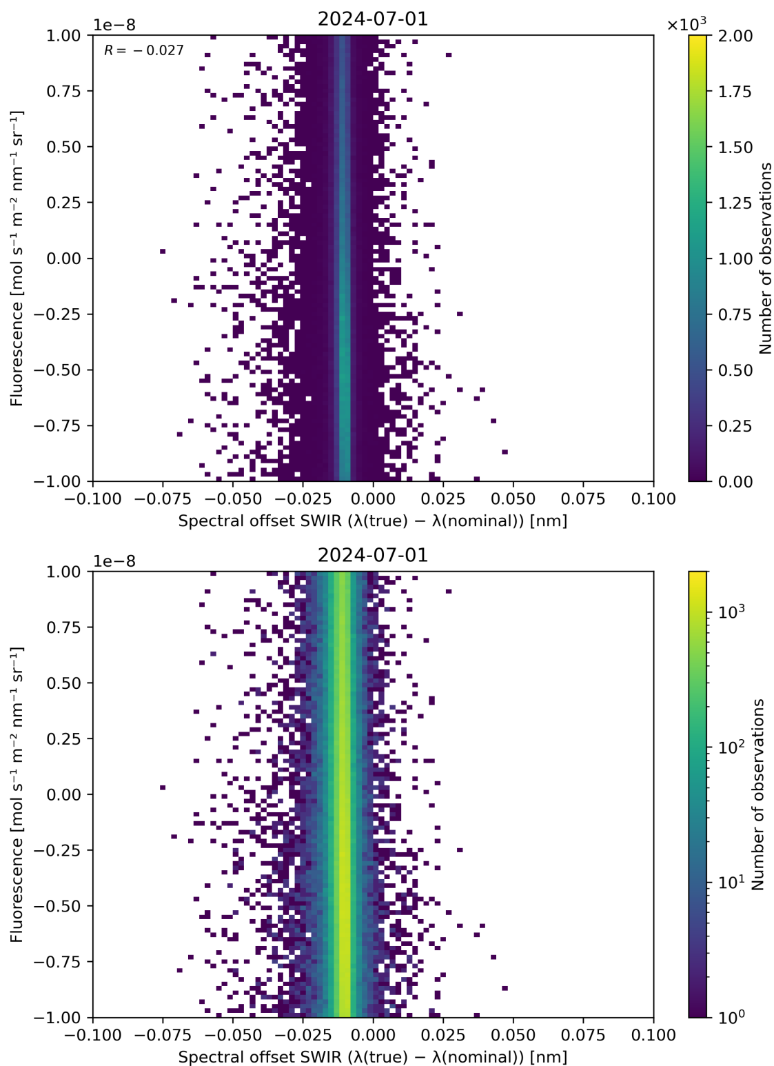
Figure 120: Scatter density plot of “Spectral offset SWIR ( \lambda(\text{true}) - \lambda(\text{nominal}) )” against “Fluorescence” for 2024-06-30 to 2024-07-02.
