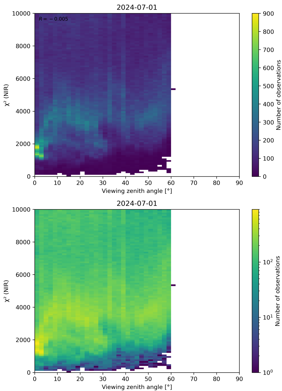
Figure 105: Scatter density plot of “Viewing zenith angle” against “ \chi^2 (NIR)” for 2024-06-30 to 2024-07-02.
