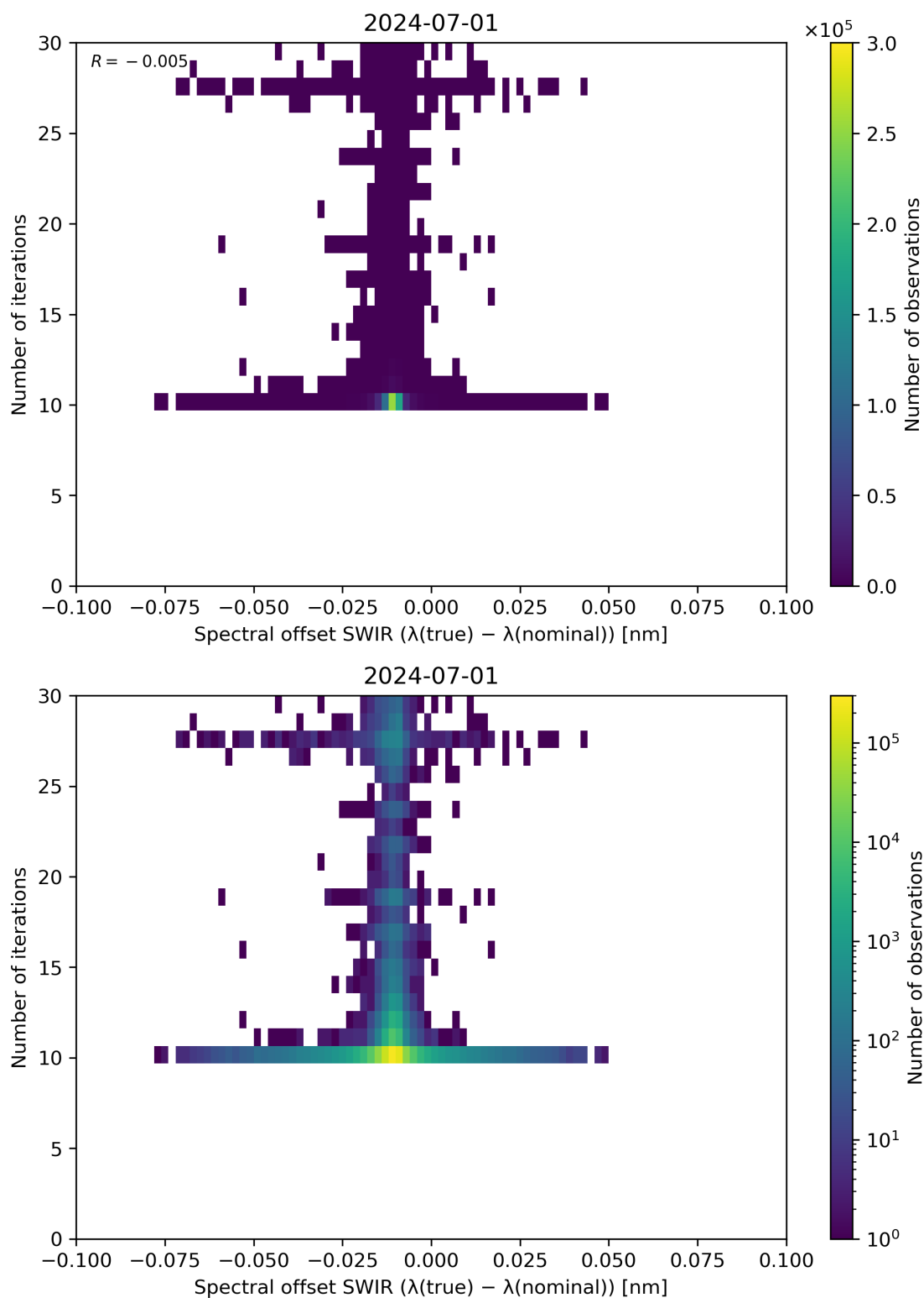
Figure 121: Scatter density plot of “Spectral offset SWIR ( \lambda(\text{true}) - \lambda(\text{nominal}) )” against “Number of iterations” for 2024-06-30 to 2024-07-02.
