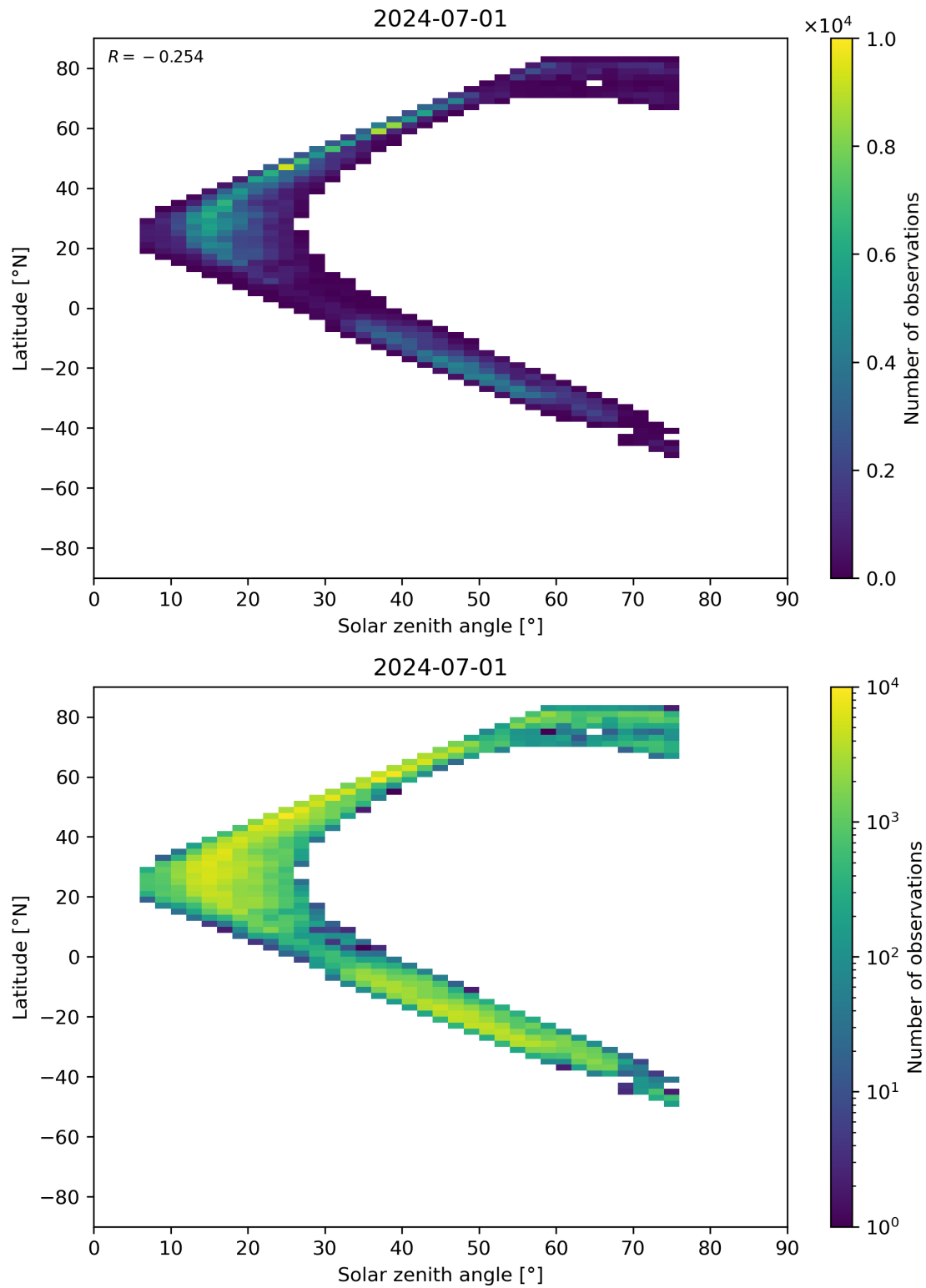
Figure 98: Scatter density plot of “Solar zenith angle” against “Latitude” for 2024-06-30 to 2024-07-02.
