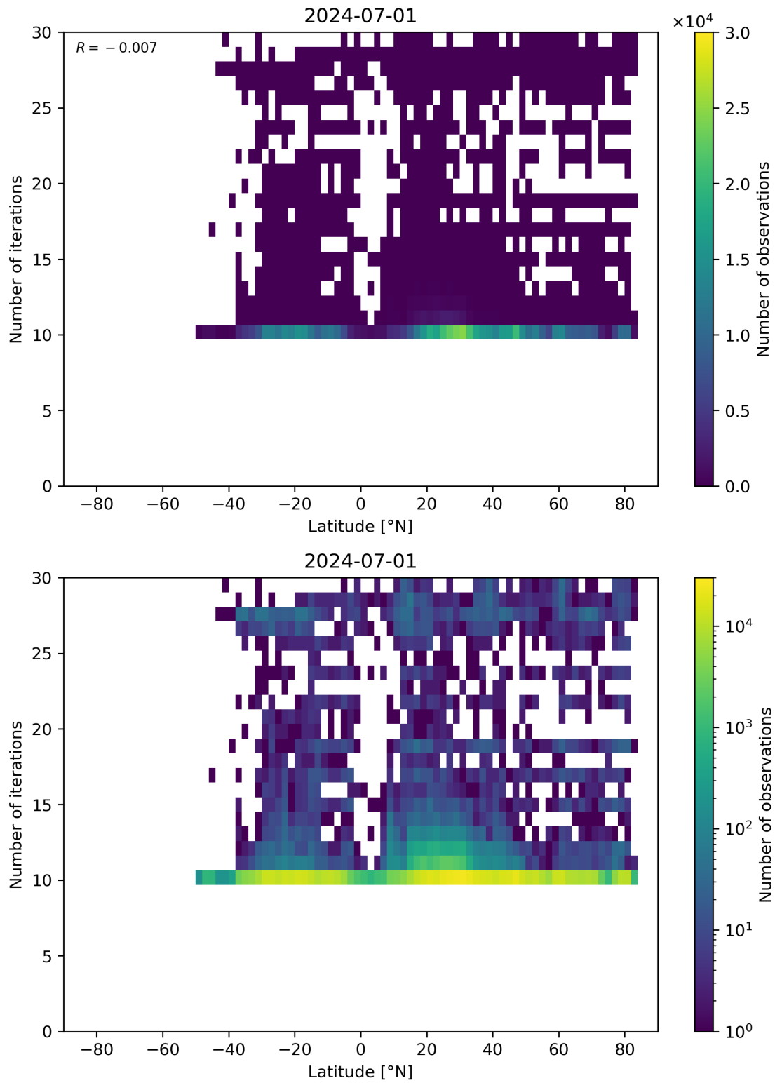
Figure 60: Scatter density plot of “Latitude” against “Number of iterations” for 2024-06-30 to 2024-07-02.
