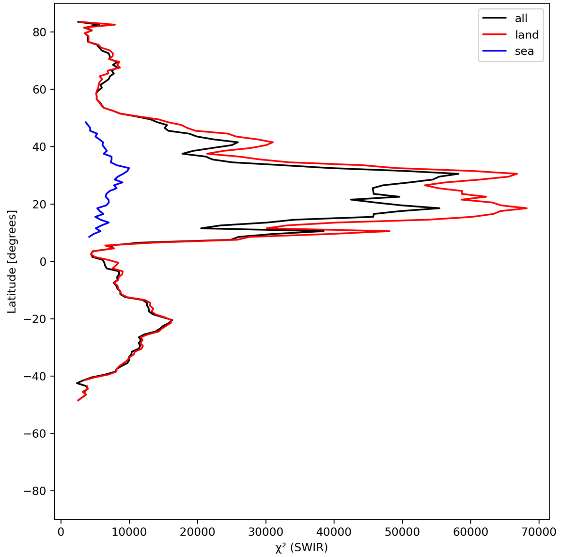
Figure 17: Zonal average of “ \chi^2 (SWIR)” for 2024-06-30 to 2024-07-02.
