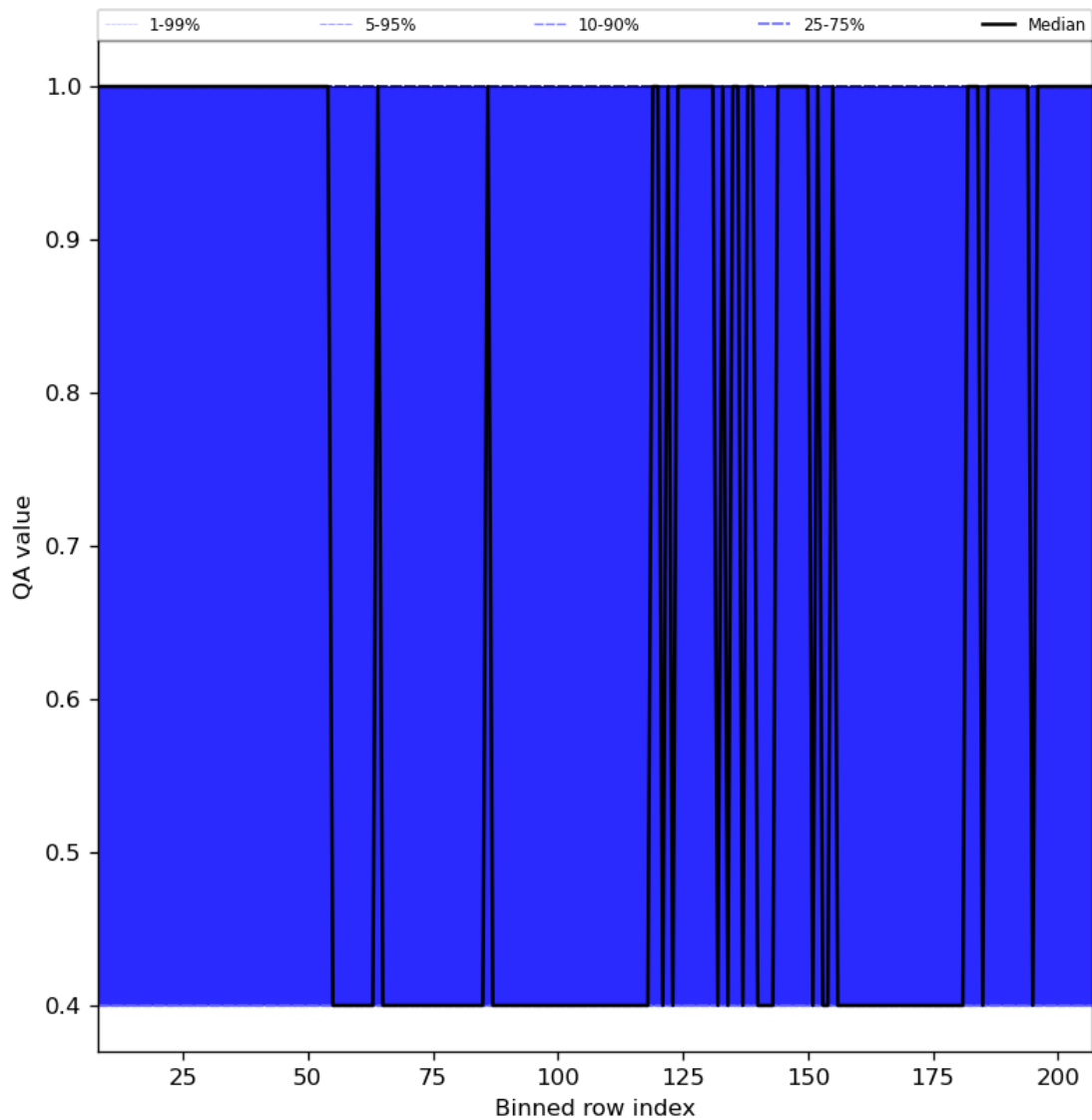
Figure 33: Along track statistics of “QA value” for 2024-06-30 to 2024-07-02
