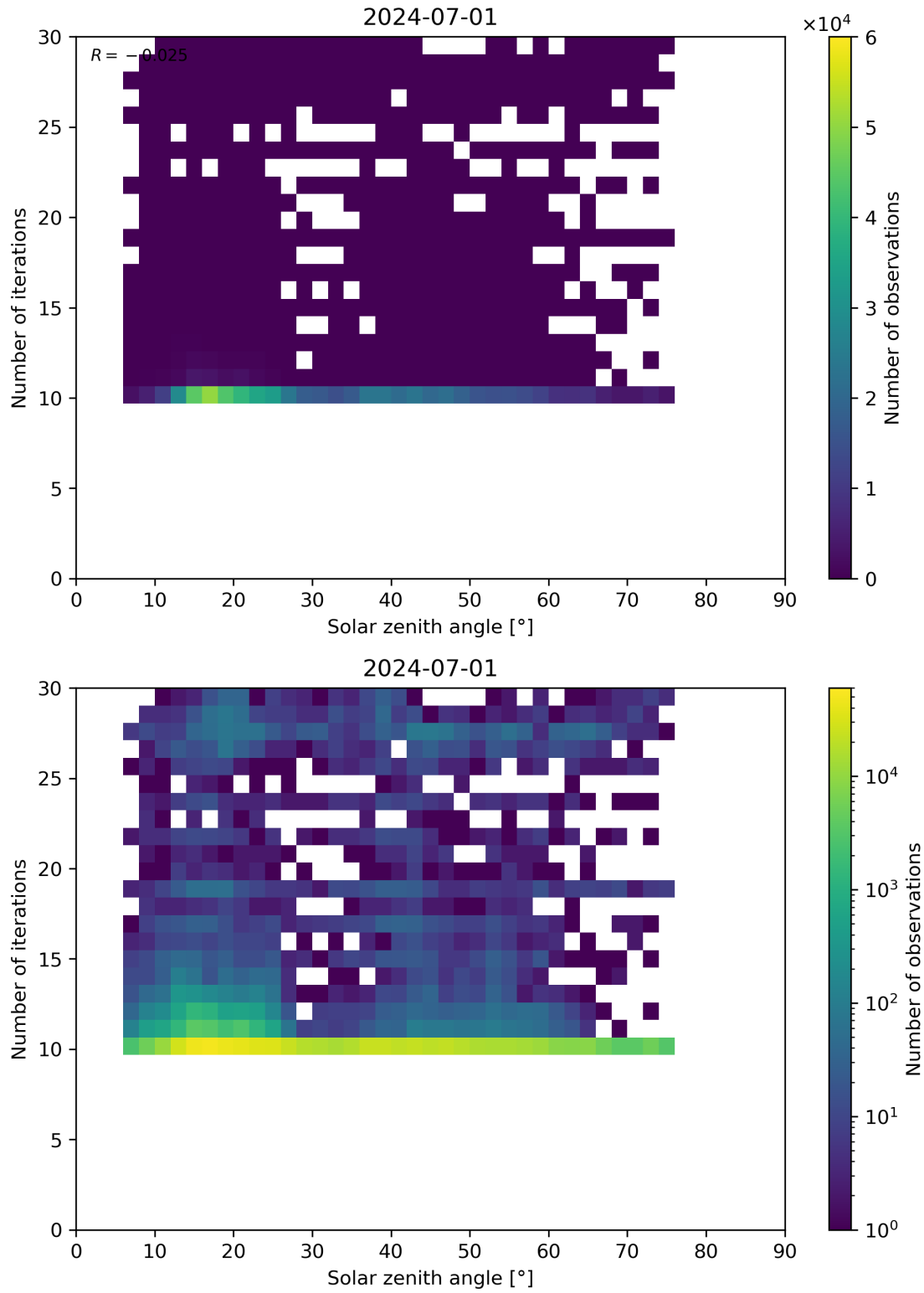
Figure 102: Scatter density plot of “Solar zenith angle” against “Number of iterations” for 2024-06-30 to 2024-07-02.
