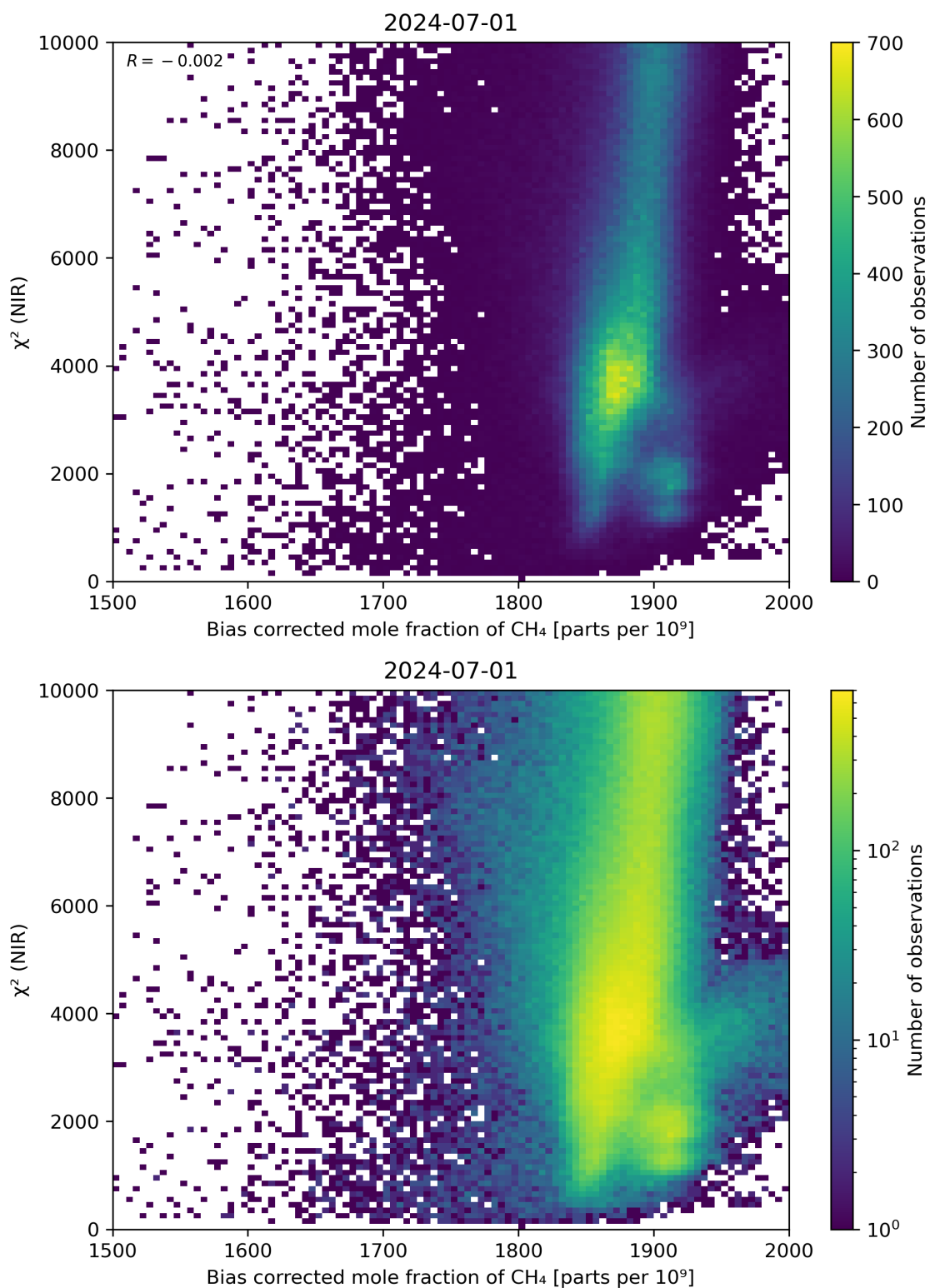
Figure 63: Scatter density plot of “Bias corrected mole fraction of CH 4 ” against “ \chi^2 (NIR)” for 2024-06-30 to 2024-07-02.
