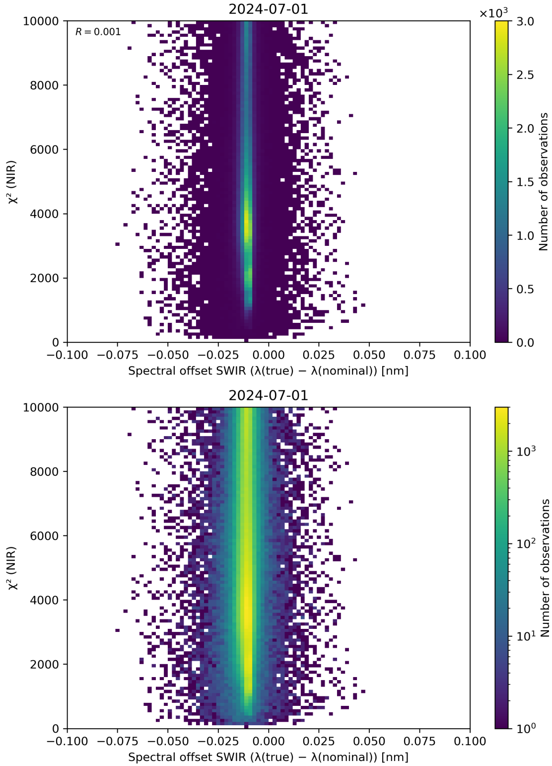
Figure 117: Scatter density plot of “Spectral offset SWIR ( \lambda(\text{true}) - \lambda(\text{nominal}) )” against “ \chi^2 (NIR)” for 2024-06-30 to 2024-07-02.
