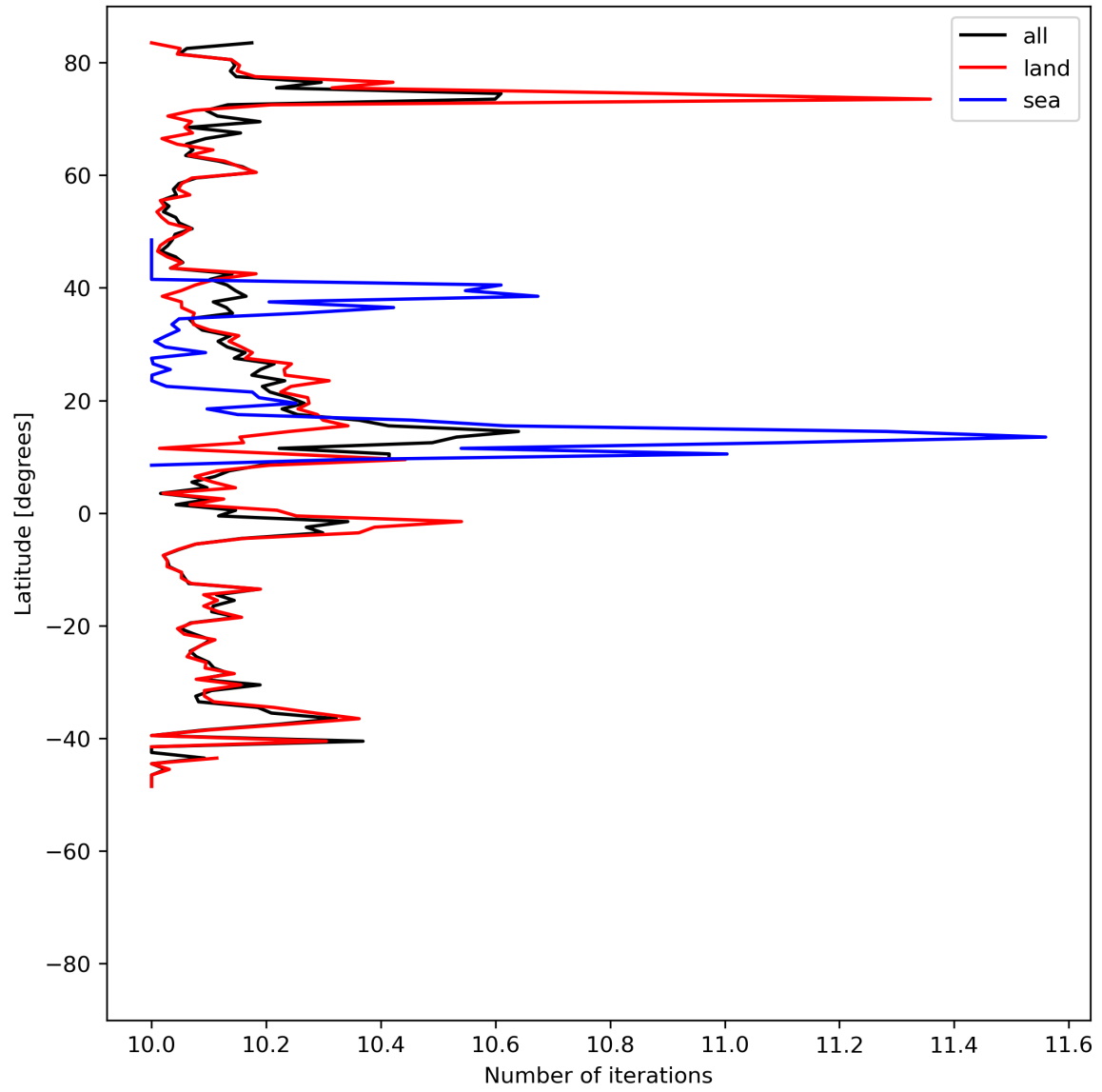
Figure 20: Zonal average of “Number of iterations” for 2024-06-30 to 2024-07-02.
