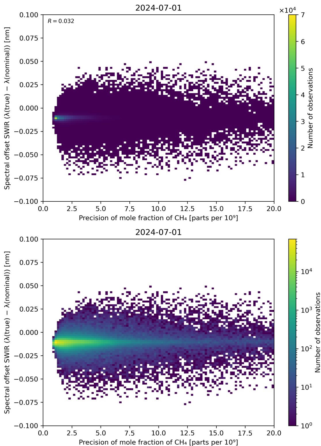
Figure 85: Scatter density plot of “Precision of mole fraction of \text{CH}_4 ” against “Spectral offset SWIR ( \lambda(\text{true}) - \lambda(\text{nominal}) )” for 2024-06-30 to 2024-07-02.
