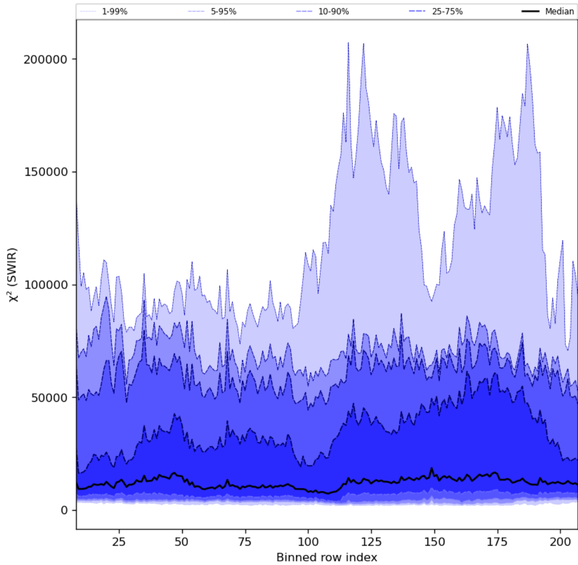
Figure 39: Along track statistics of “ \chi^2 (SWIR)” for 2024-06-30 to 2024-07-02
