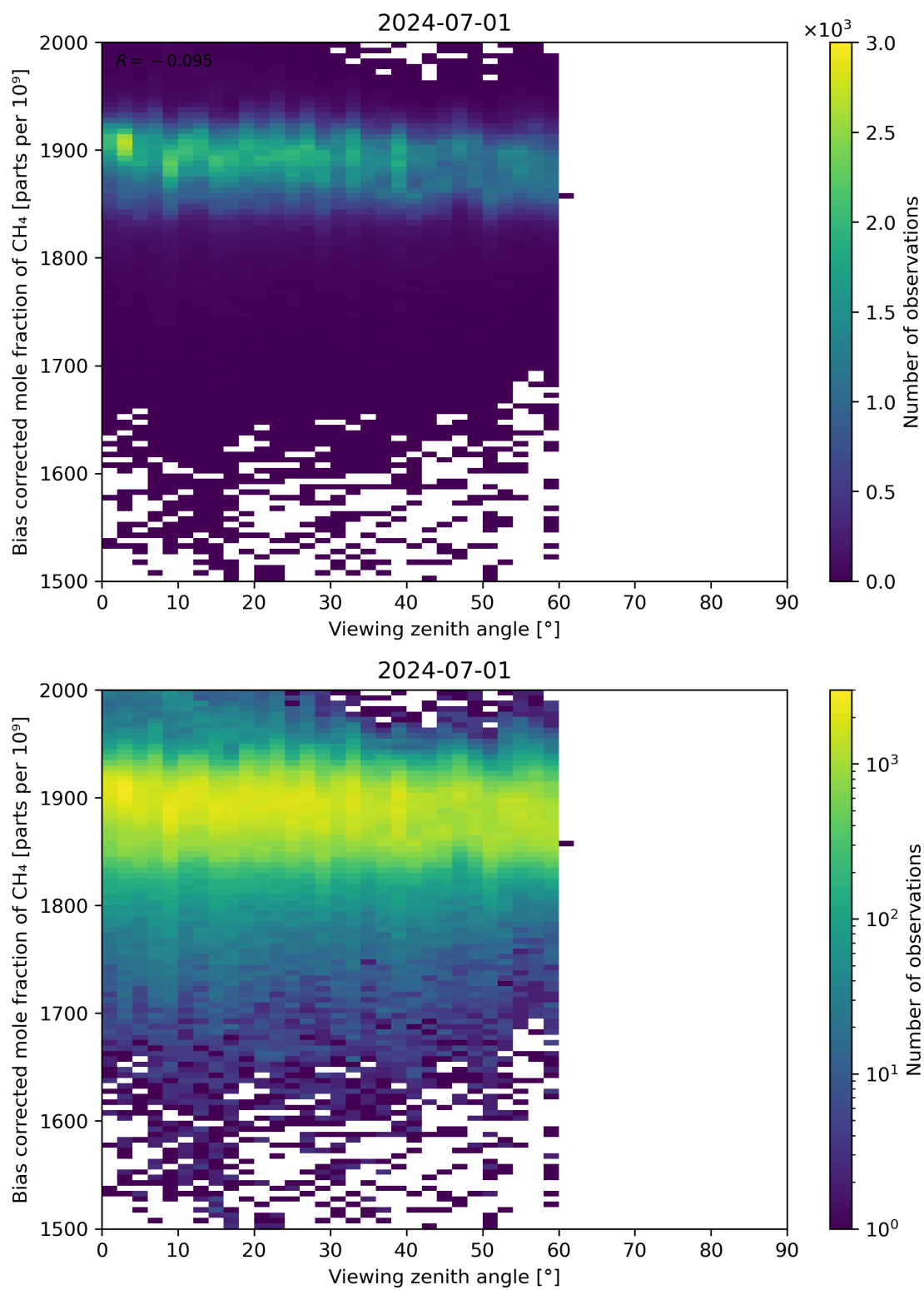
Figure 111: Scatter density plot of “Viewing zenith angle” against “Bias corrected mole fraction of CH 4 ” for 2024-06-30 to 2024-07-02.
