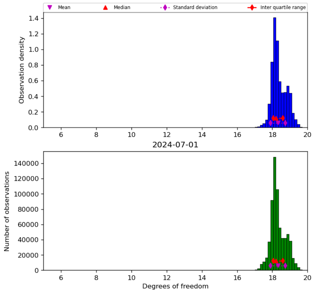
Figure 30: Histogram of “Degrees of freedom” for 2024-06-30 to 2024-07-02
