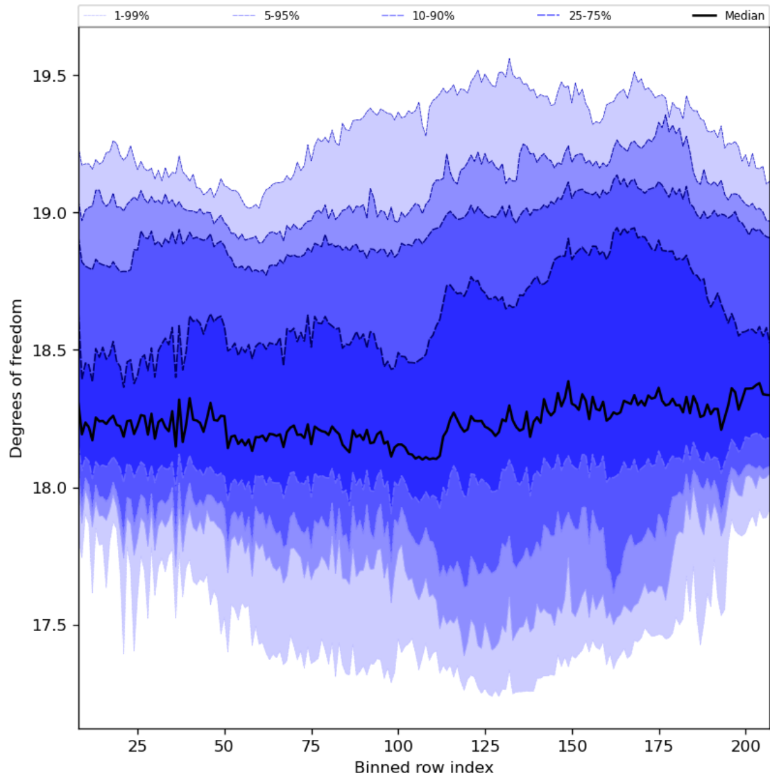
Figure 41: Along track statistics of “Degrees of freedom” for 2024-06-30 to 2024-07-02
