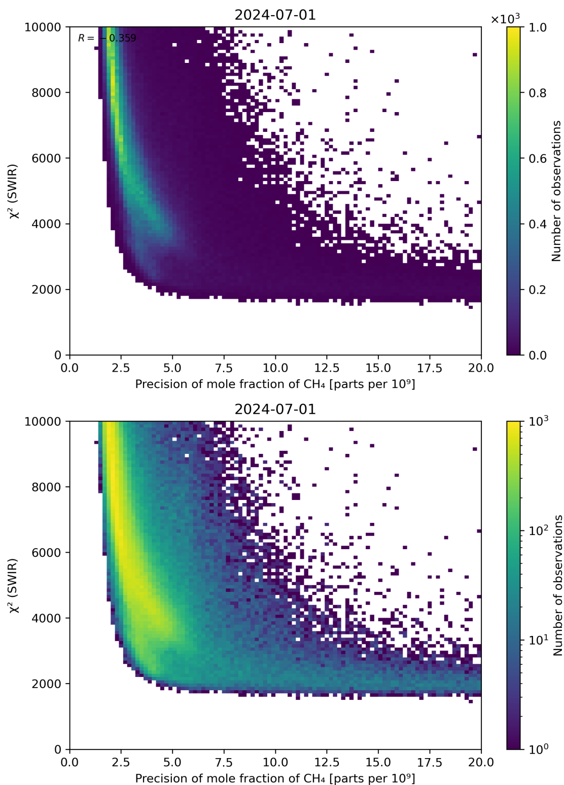
Figure 79: Scatter density plot of “Precision of mole fraction of \text{CH}_4 ” against “ \chi^2 (SWIR)” for 2024-06-30 to 2024-07-02.
