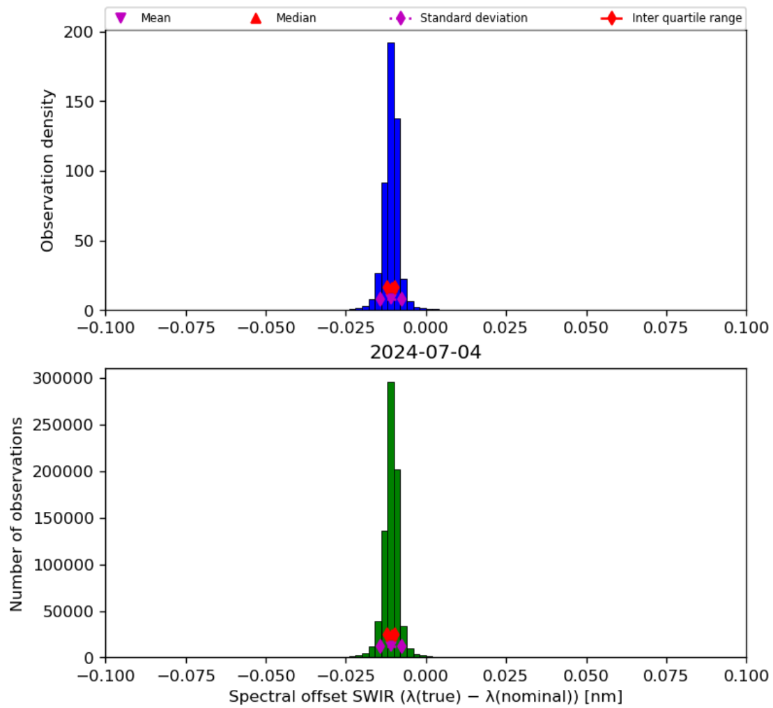
Figure 27: Histogram of “Spectral offset SWIR ( \lambda(\text{true}) - \lambda(\text{nominal}) )” for 2024-07-03 to 2024-07-05
