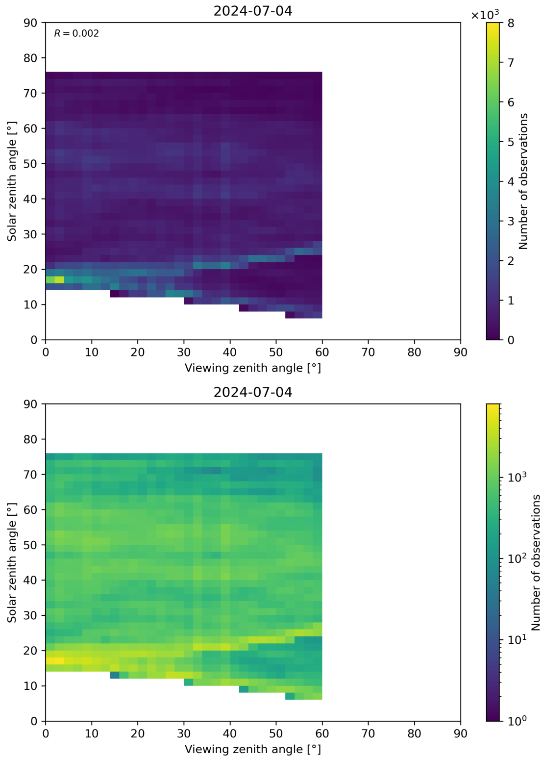
Figure 115: Scatter density plot of “Viewing zenith angle” against “Solar zenith angle” for 2024-07-03 to 2024-07-05.
