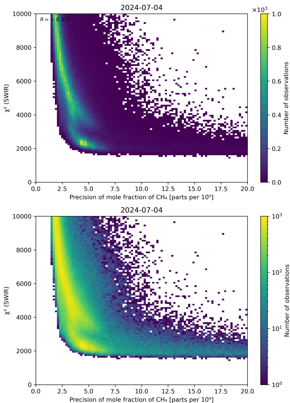
Figure 79: Scatter density plot of “Precision of mole fraction of \text{CH}_4 ” against “ \chi^2 (SWIR)” for 2024-07-03 to 2024-07-05.
