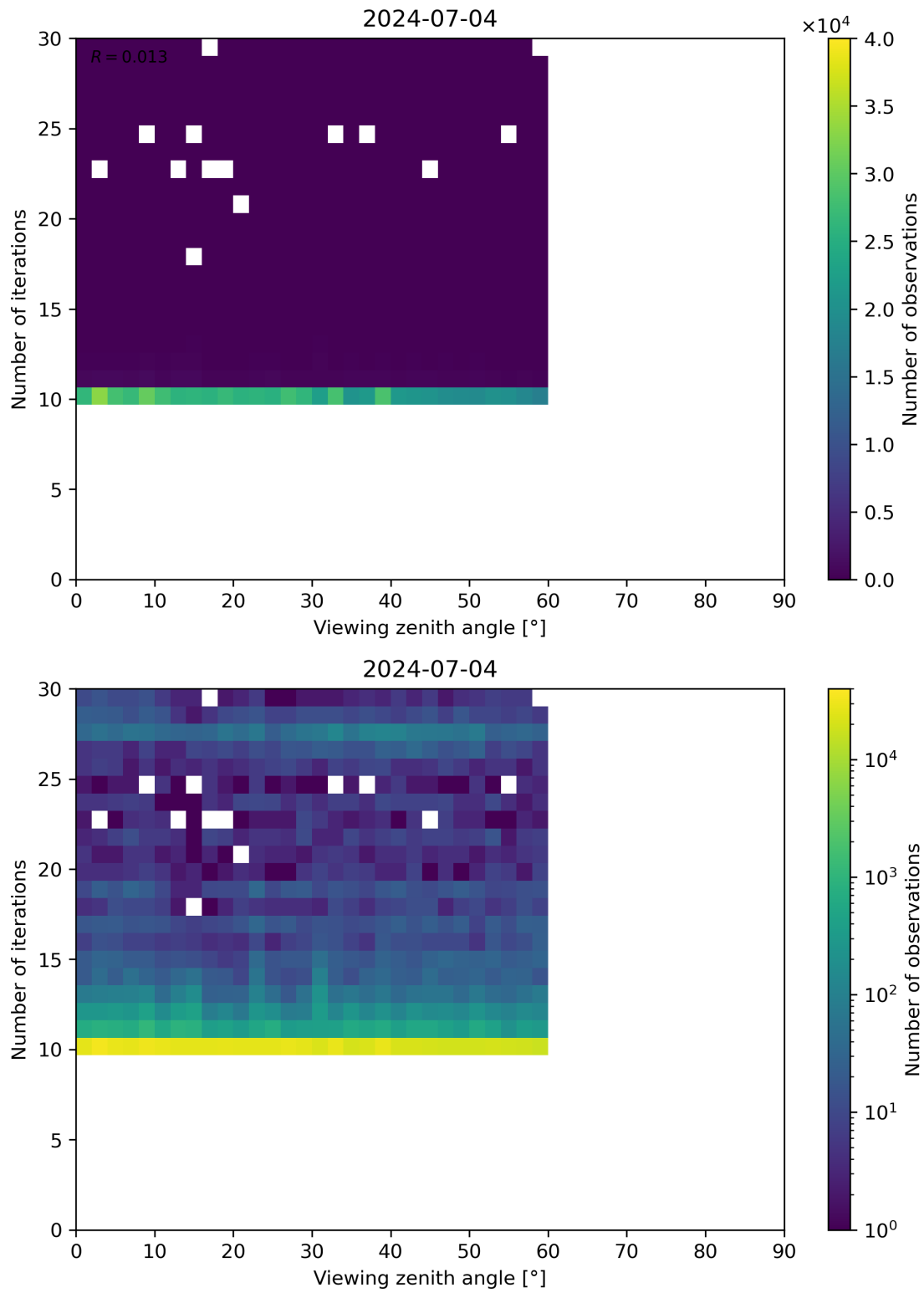
Figure 113: Scatter density plot of “Viewing zenith angle” against “Number of iterations” for 2024-07-03 to 2024-07-05.
