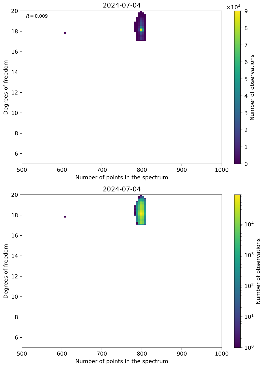
Figure 90: Scatter density plot of “Number of points in the spectrum” against “Degrees of freedom” for 2024-07-03 to 2024-07-05.
