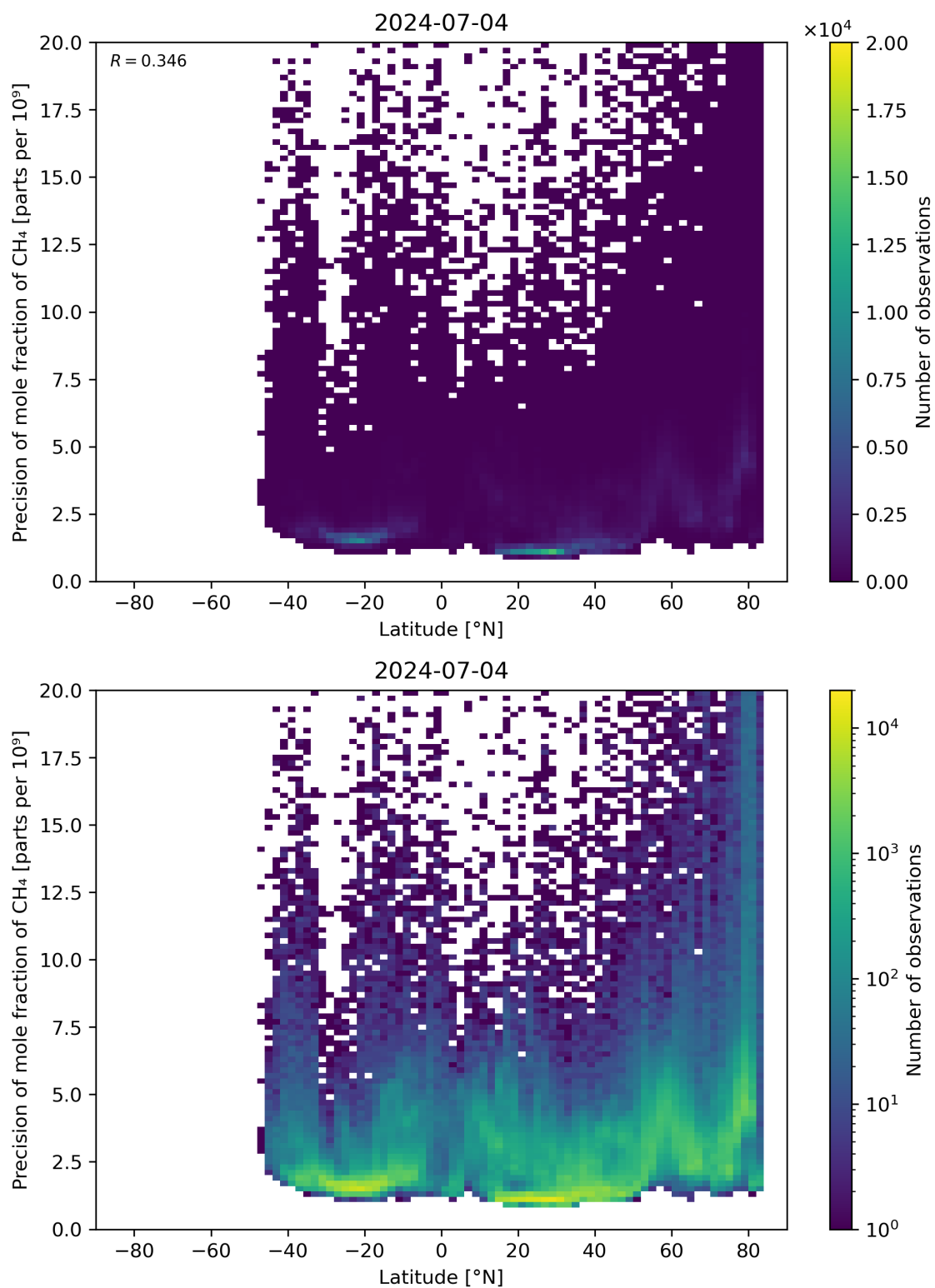
Figure 59: Scatter density plot of “Latitude” against “Precision of mole fraction of \text{CH}_4 ” for 2024-07-03 to 2024-07-05.
