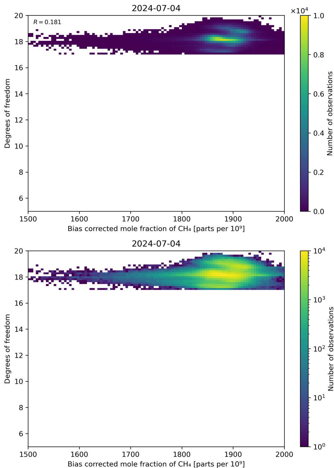
Figure 65: Scatter density plot of “Bias corrected mole fraction of \text{CH}_4 ” against “Degrees of freedom” for 2024-07-03 to 2024-07-05.
