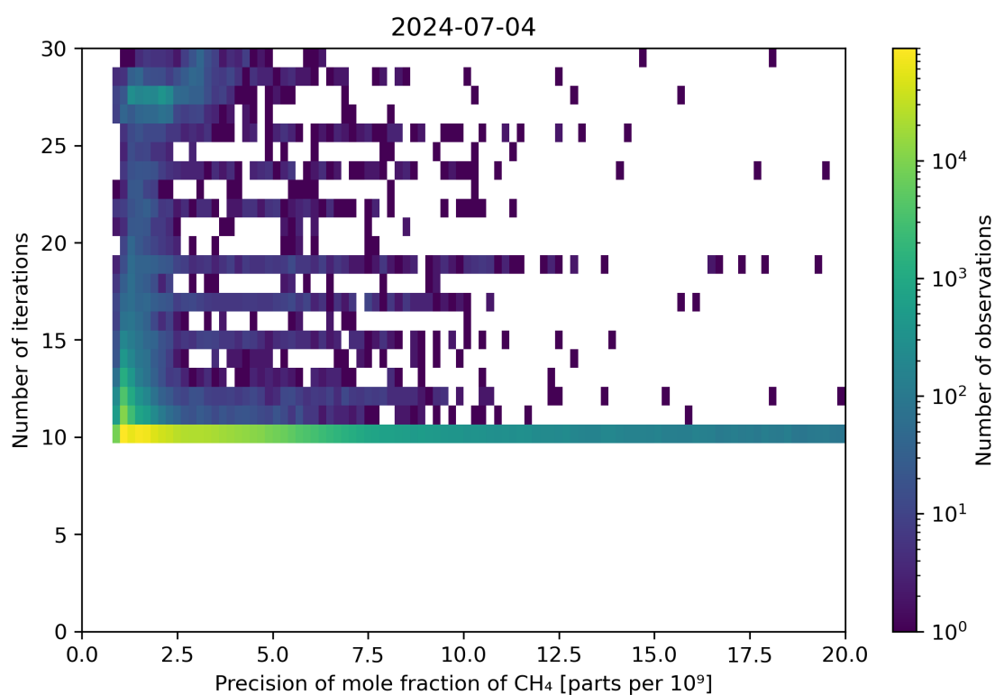
Figure 83: Scatter density plot of “Precision of mole fraction of \text{CH}_4 ” against “Number of iterations” for 2024-07-03 to 2024-07-05.
