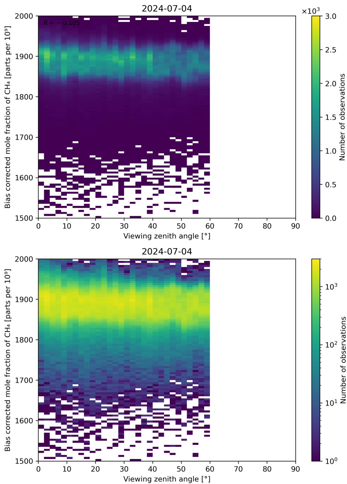
Figure 111: Scatter density plot of “Viewing zenith angle” against “Bias corrected mole fraction of CH 4 ” for 2024-07-03 to 2024-07-05.
