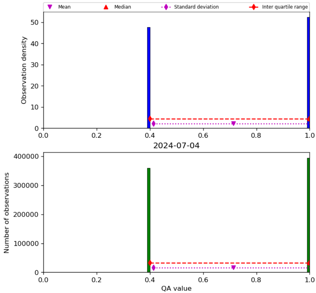
Figure 22: Histogram of “QA value” for 2024-07-03 to 2024-07-05
