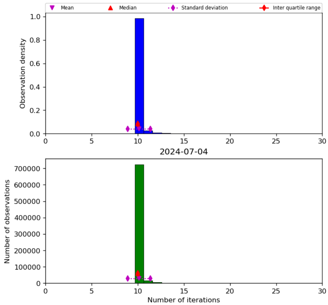
Figure 31: Histogram of “Number of iterations” for 2024-07-03 to 2024-07-05
