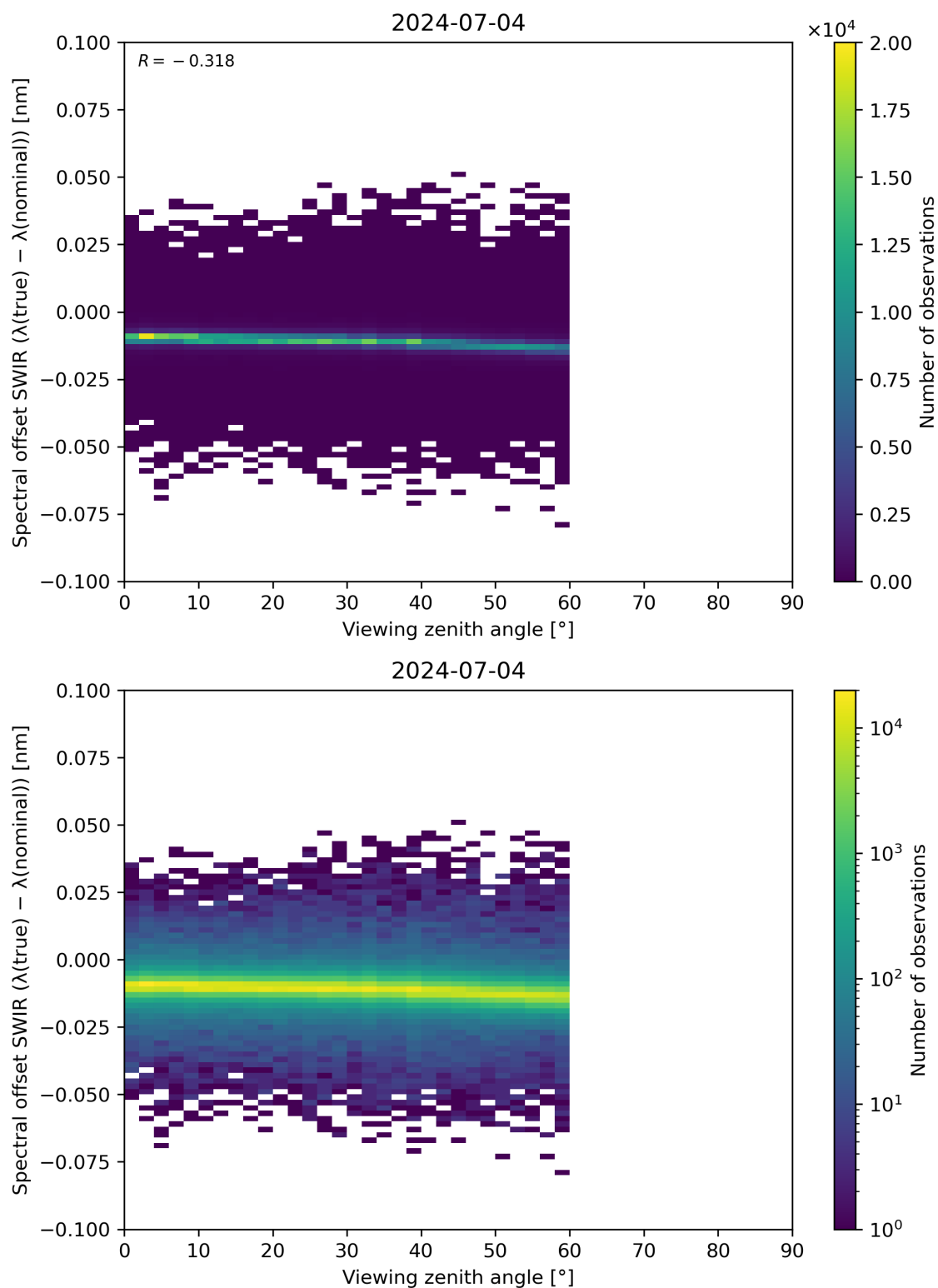
Figure 116: Scatter density plot of “Viewing zenith angle” against “Spectral offset SWIR ( \lambda(\text{true}) - \lambda(\text{nominal}) )” for 2024-07-03 to 2024-07-05.
