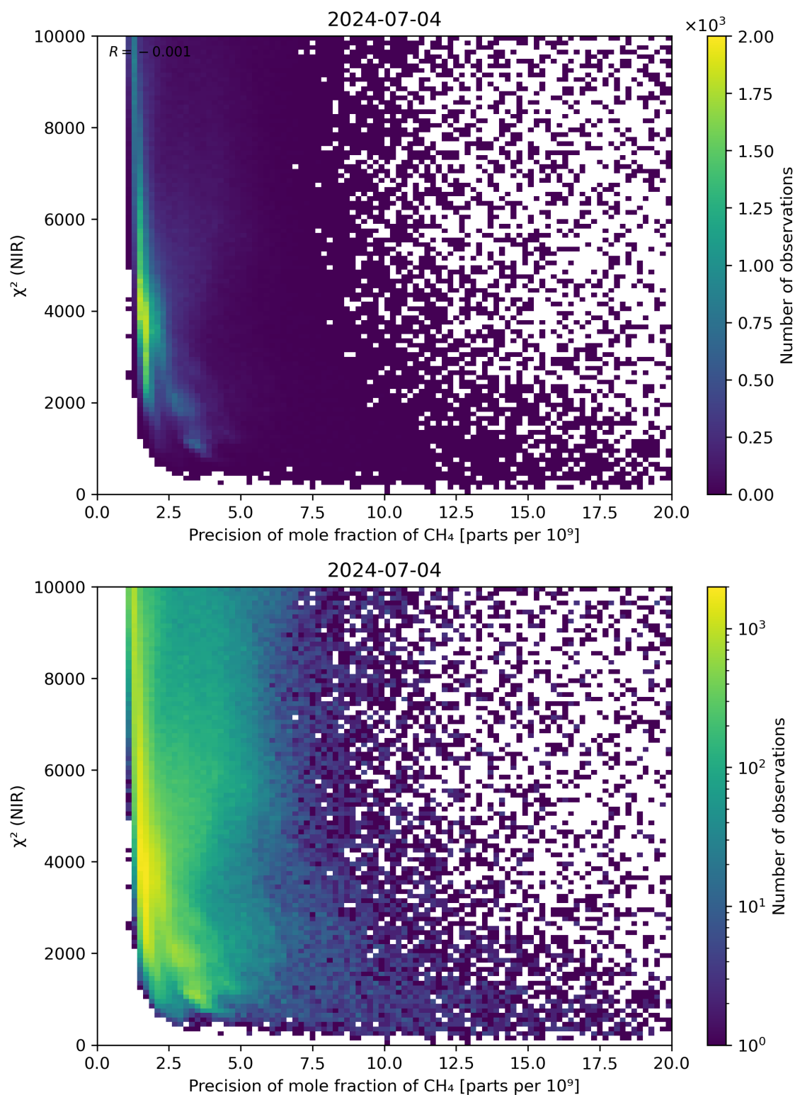
Figure 78: Scatter density plot of “Precision of mole fraction of CH 4 ” against “ \chi^2 (NIR)” for 2024-07-03 to 2024-07-05.
