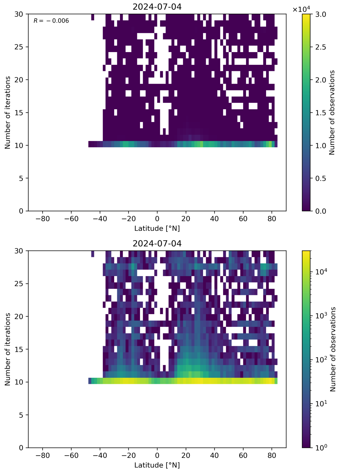
Figure 60: Scatter density plot of “Latitude” against “Number of iterations” for 2024-07-03 to 2024-07-05.
