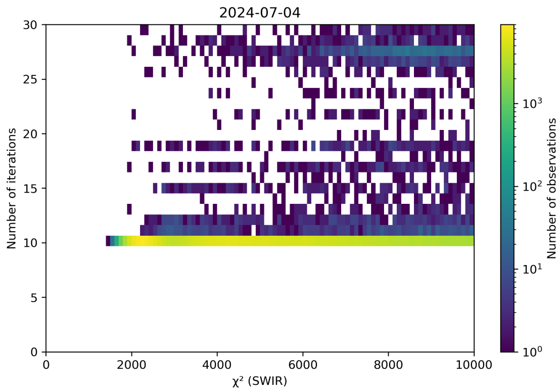
Figure 50: Scatter density plot of “ \chi^2 (SWIR)” against “Number of iterations” for 2024-07-03 to 2024-07-05.
