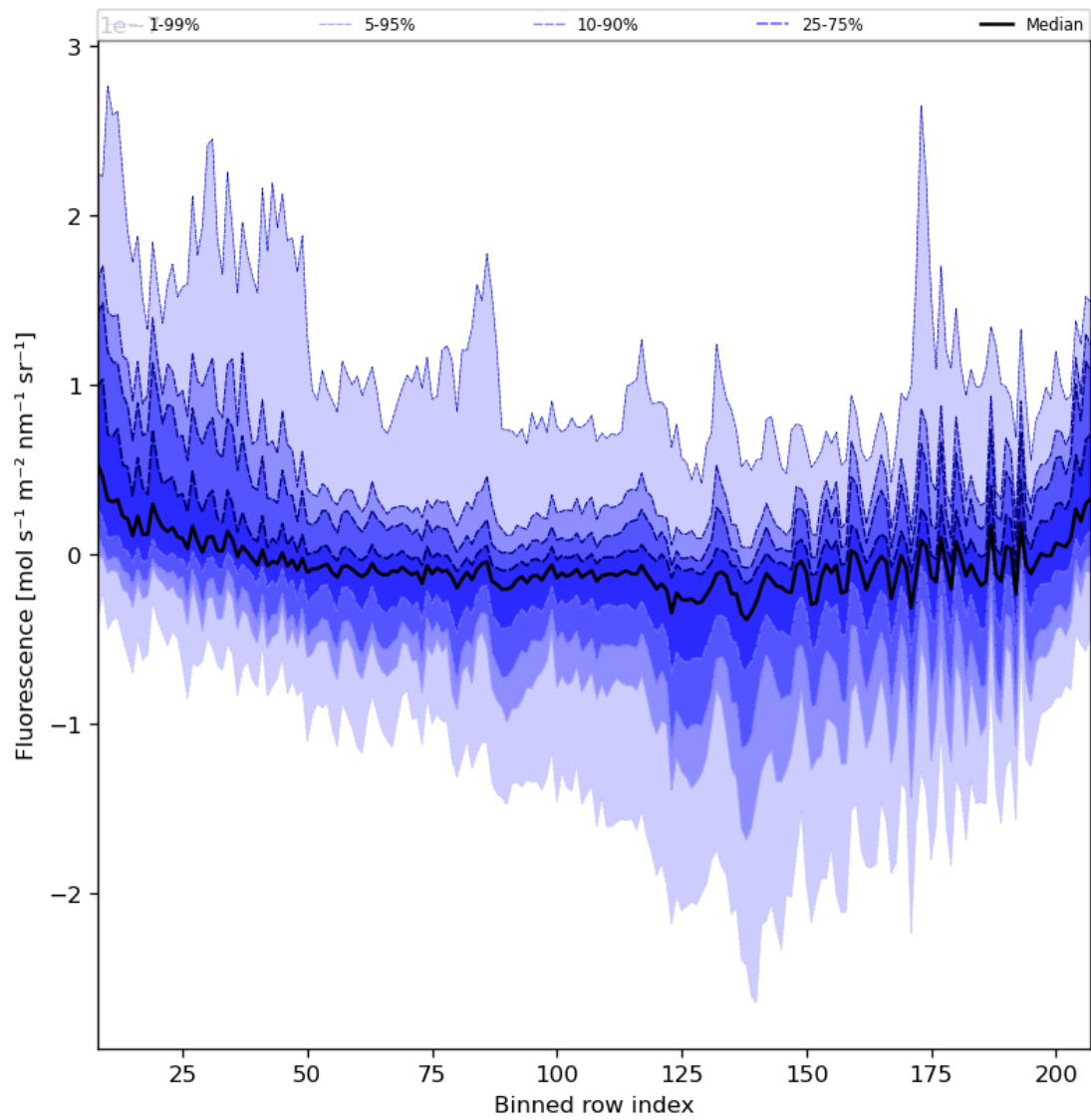
Figure 43: Along track statistics of “Fluorescence” for 2024-07-03 to 2024-07-05
