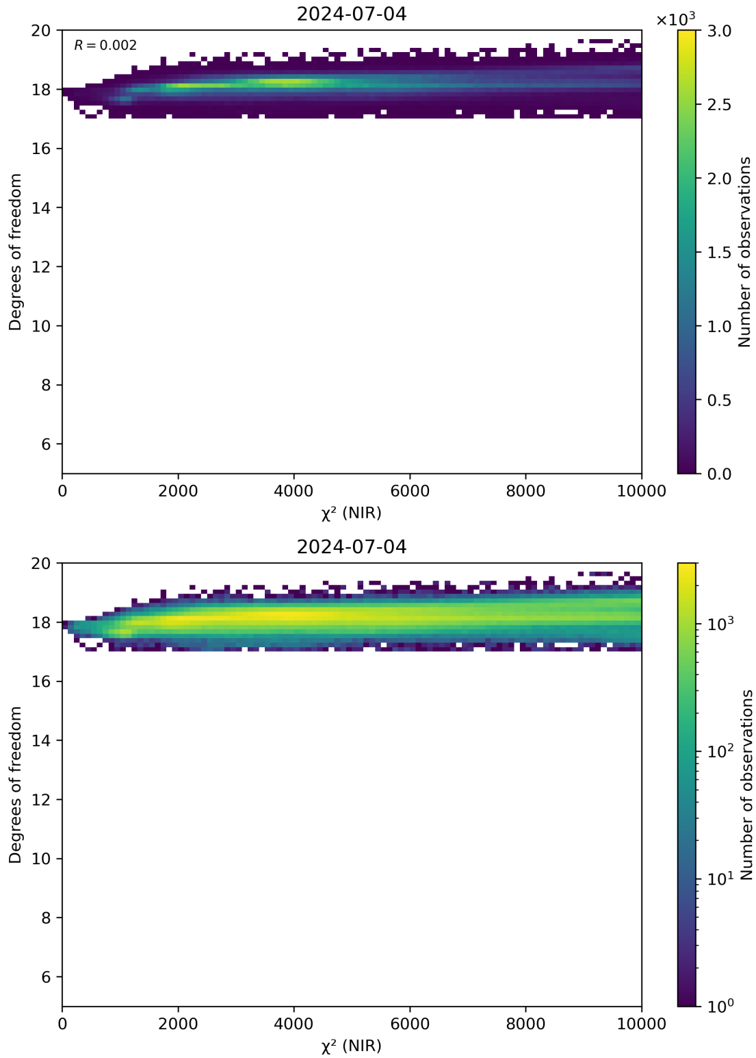
Figure 44: Scatter density plot of “ \chi^2 (NIR)” against “Degrees of freedom” for 2024-07-03 to 2024-07-05.
