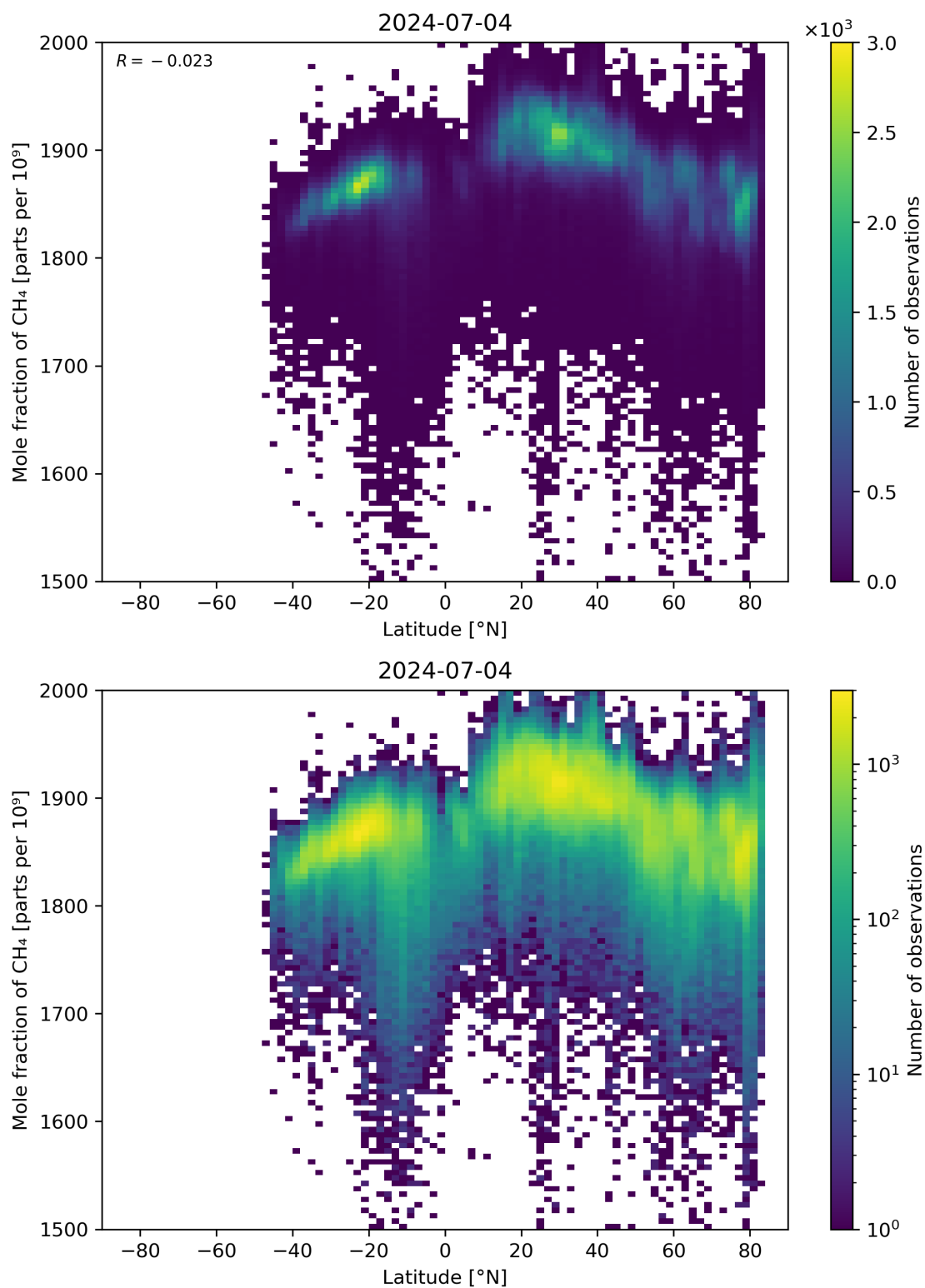
Figure 57: Scatter density plot of “Latitude” against “Mole fraction of \text{CH}_4 ” for 2024-07-03 to 2024-07-05.
