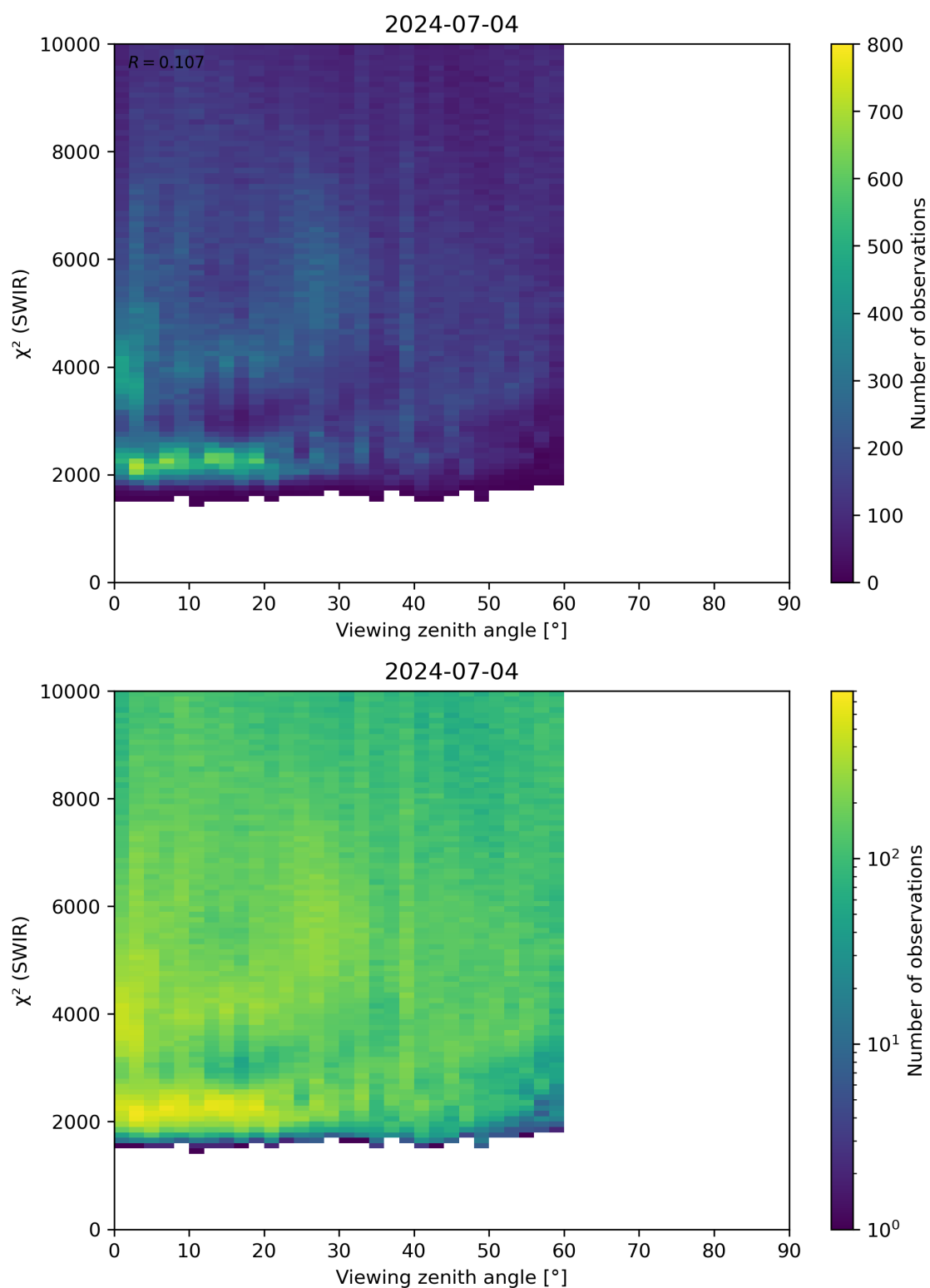
Figure 106: Scatter density plot of “Viewing zenith angle” against “ \chi^2 (SWIR)” for 2024-07-03 to 2024-07-05.
