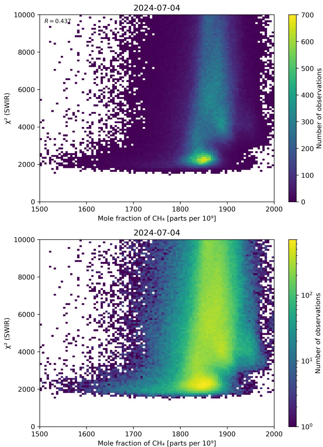
Figure 71: Scatter density plot of “Mole fraction of \text{CH}_4 ” against “ \chi^2 (SWIR)” for 2024-07-03 to 2024-07-05.
