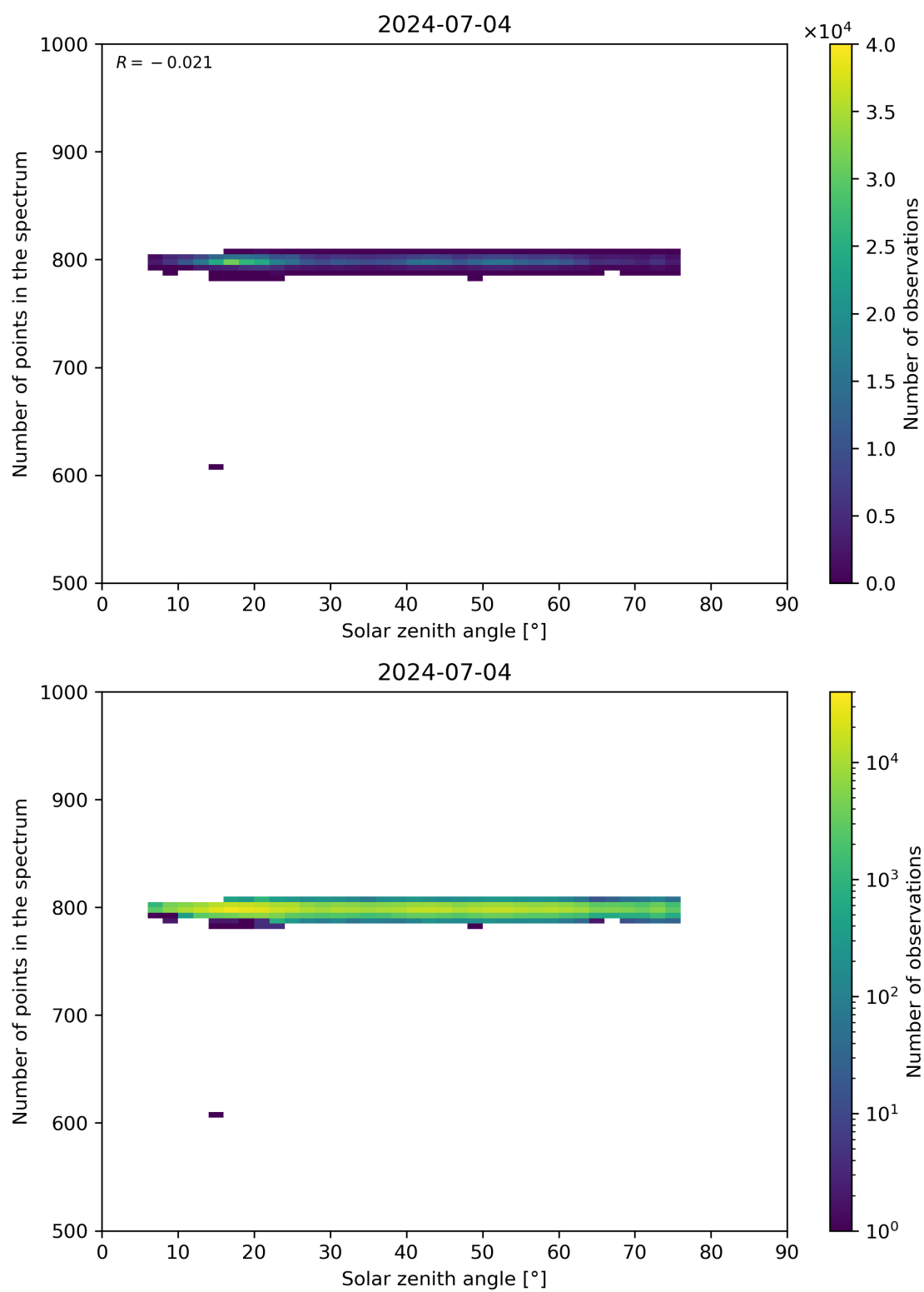
Figure 103: Scatter density plot of “Solar zenith angle” against “Number of points in the spectrum” for 2024-07-03 to 2024-07-05.
