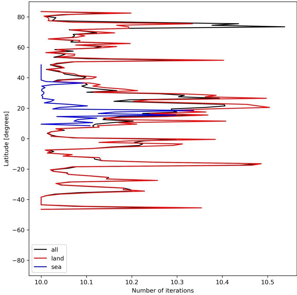
Figure 20: Zonal average of “Number of iterations” for 2024-07-03 to 2024-07-05.
