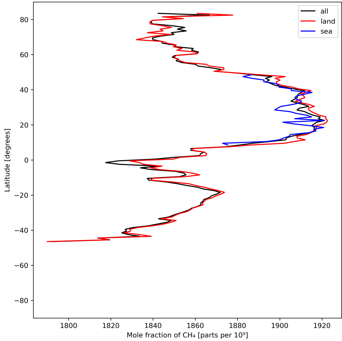
Figure 12: Zonal average of “Mole fraction of \text{CH}_4 ” for 2024-07-03 to 2024-07-05.
