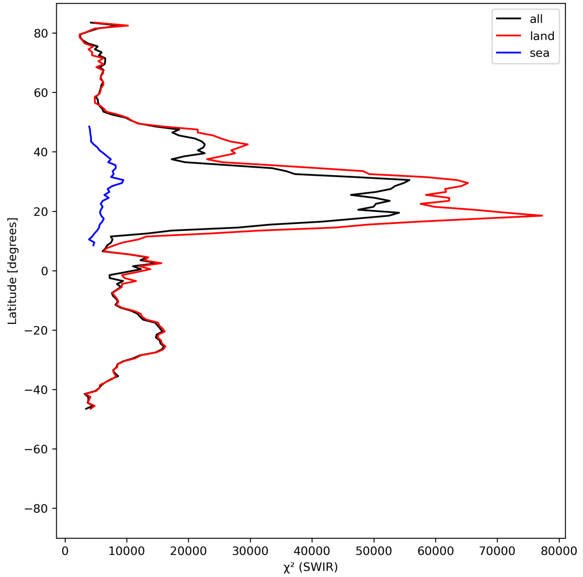
Figure 17: Zonal average of “ \chi^2 (SWIR)” for 2024-07-03 to 2024-07-05.
