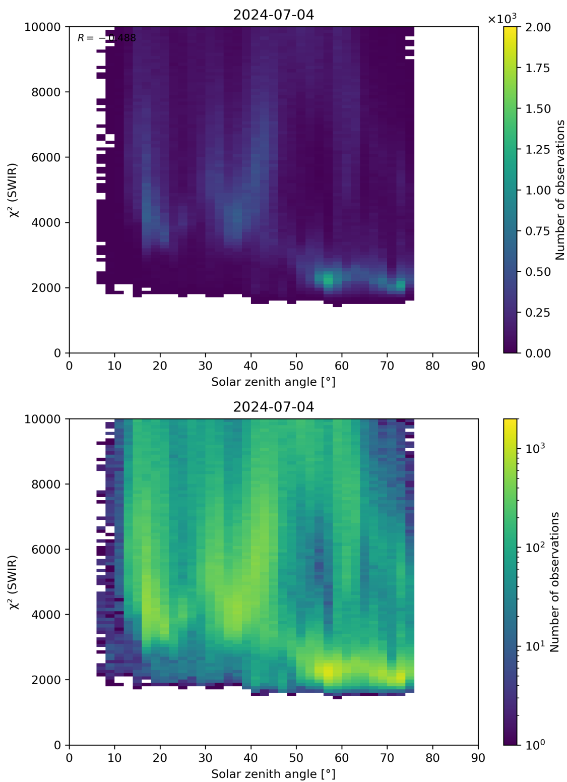
Figure 95: Scatter density plot of “Solar zenith angle” against “ \chi^2 (SWIR)” for 2024-07-03 to 2024-07-05.
