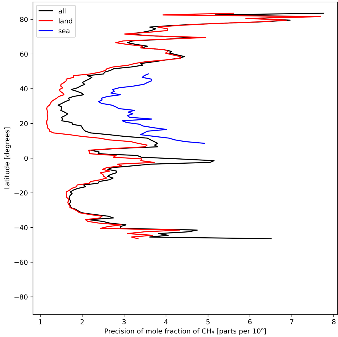
Figure 13: Zonal average of “Precision of mole fraction of CH 4 ” for 2024-07-03 to 2024-07-05.
