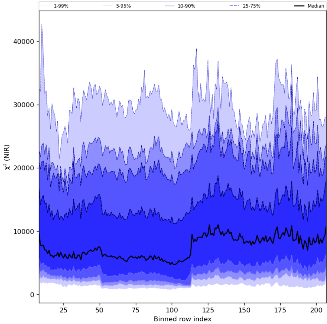
Figure 40: Along track statistics of “ \chi^2 (NIR)” for 2024-07-03 to 2024-07-05
