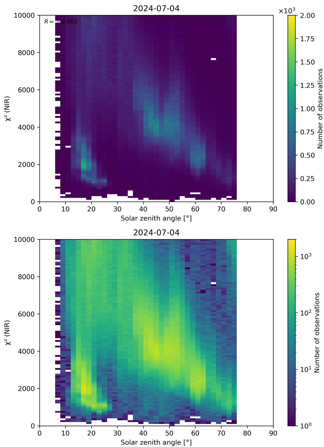
Figure 94: Scatter density plot of “Solar zenith angle” against “ \chi^2 (NIR)” for 2024-07-03 to 2024-07-05.
