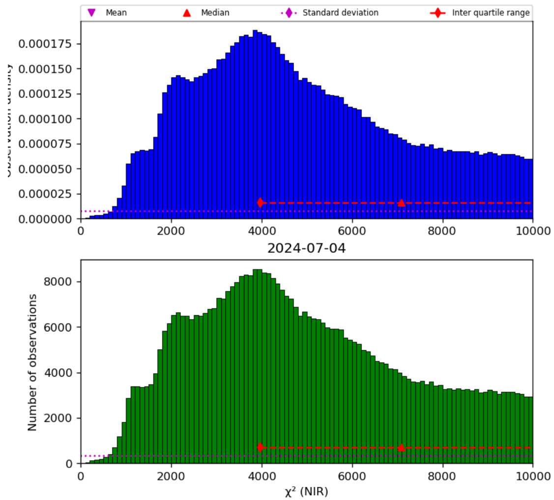
Figure 29: Histogram of “ \chi^2 (NIR)” for 2024-07-03 to 2024-07-05
