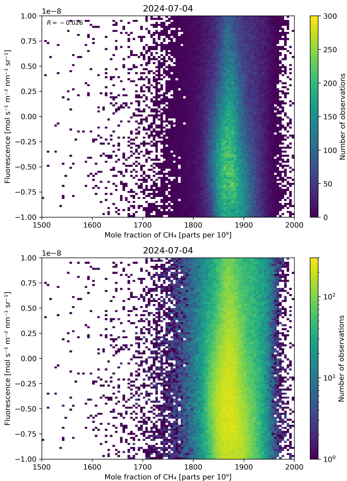
Figure 73: Scatter density plot of “Mole fraction of \text{CH}_4 ” against “Fluorescence” for 2024-07-03 to 2024-07-05.
