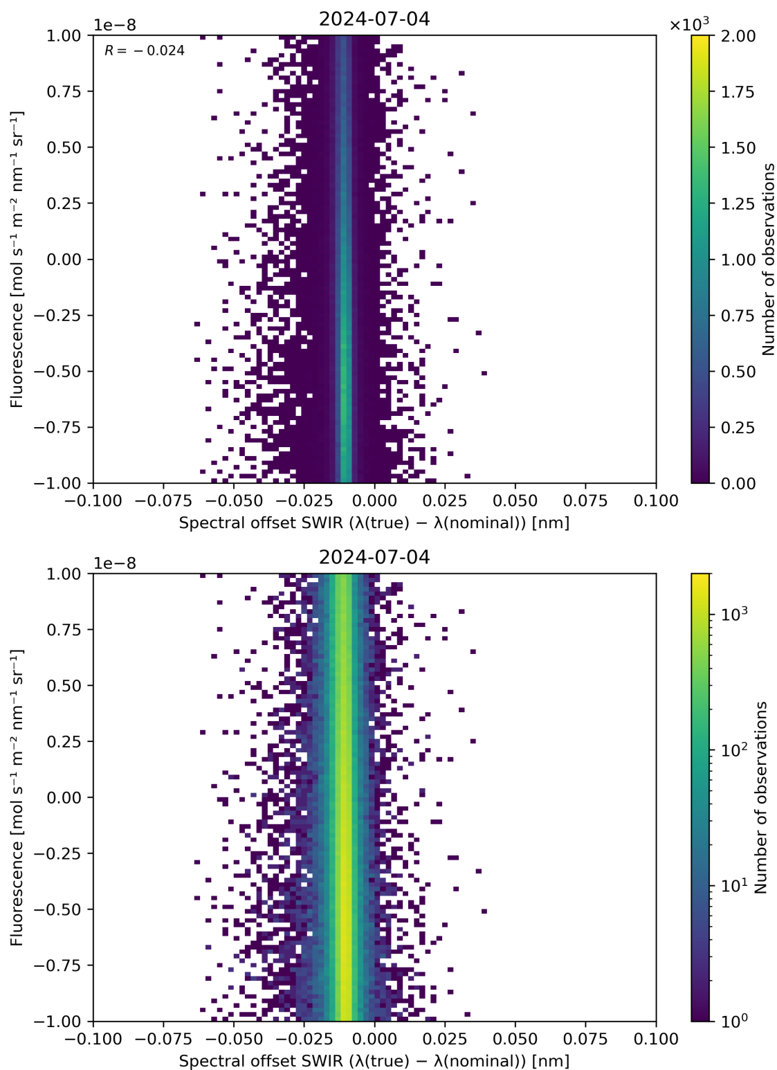
Figure 120: Scatter density plot of “Spectral offset SWIR ( \lambda(\text{true}) - \lambda(\text{nominal}) )” against “Fluorescence” for 2024-07-03 to 2024-07-05.
