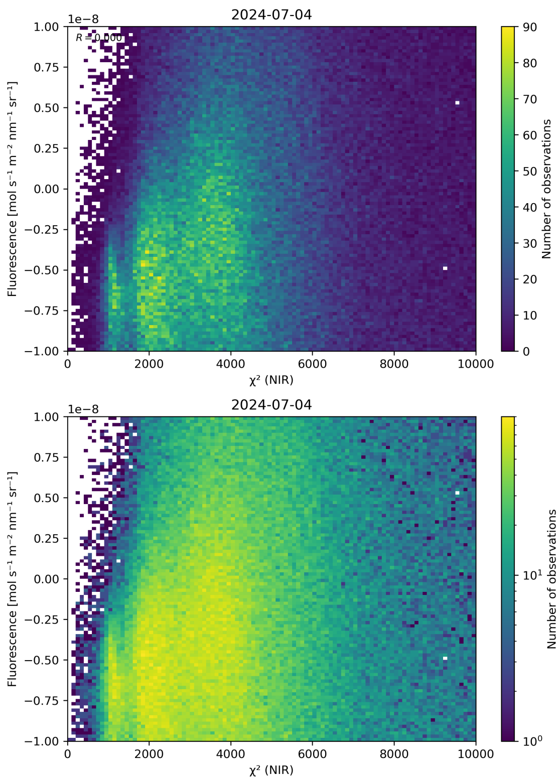
Figure 45: Scatter density plot of “ \chi^2 (NIR)” against “Fluorescence” for 2024-07-03 to 2024-07-05.
