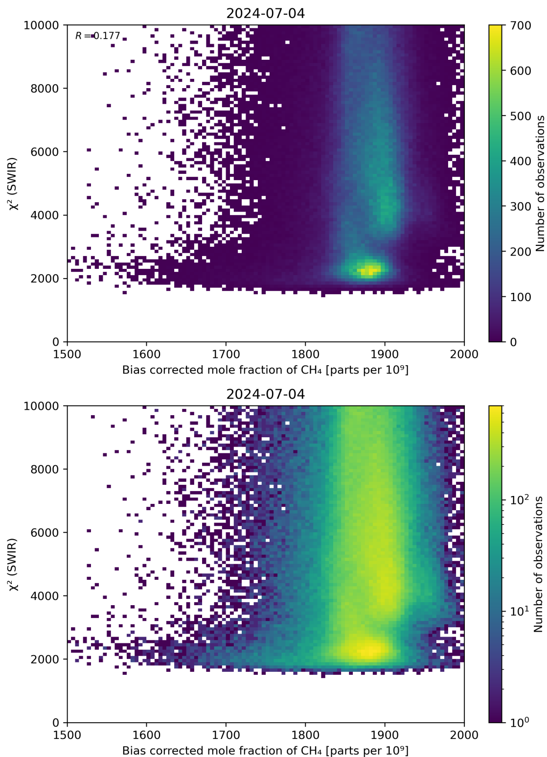
Figure 64: Scatter density plot of “Bias corrected mole fraction of CH 4 ” against “ \chi^2 (SWIR)” for 2024-07-03 to 2024-07-05.
