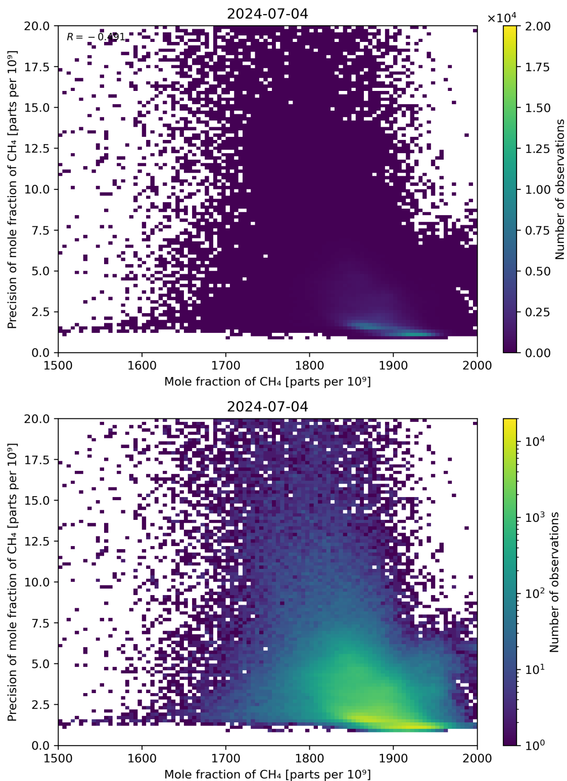
Figure 75: Scatter density plot of “Mole fraction of CH 4 ” against “Precision of mole fraction of CH 4 ” for 2024-07-03 to 2024-07-05.
