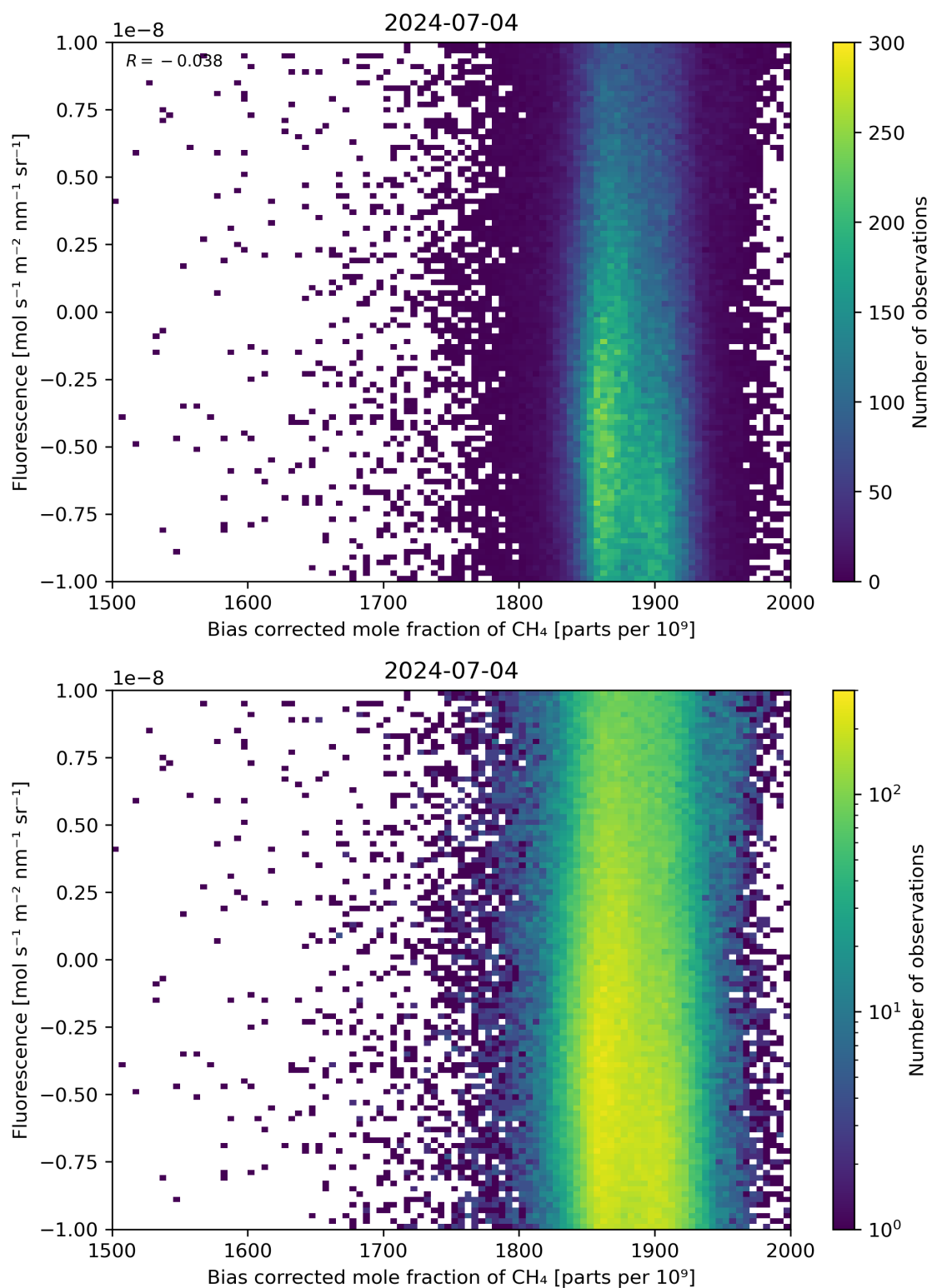
Figure 66: Scatter density plot of “Bias corrected mole fraction of \text{CH}_4 ” against “Fluorescence” for 2024-07-03 to 2024-07-05.
