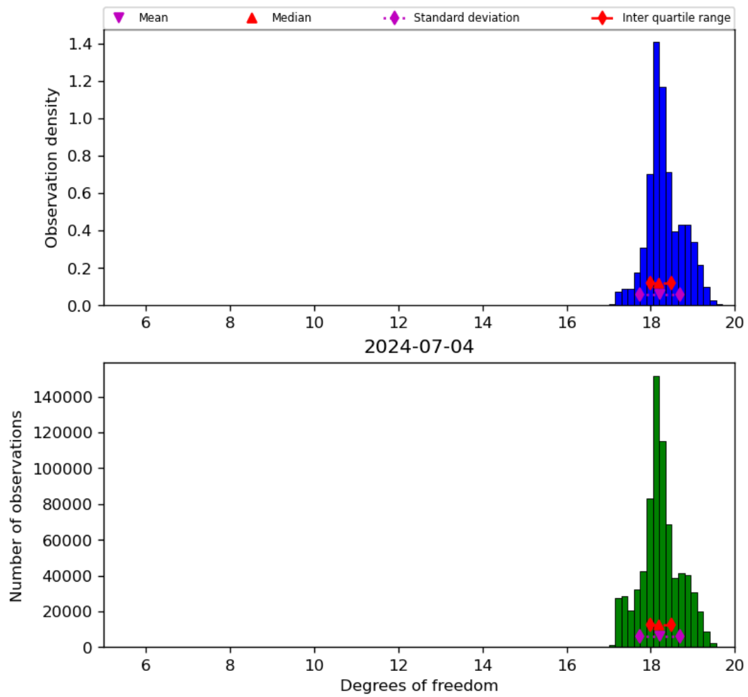
Figure 30: Histogram of “Degrees of freedom” for 2024-07-03 to 2024-07-05
