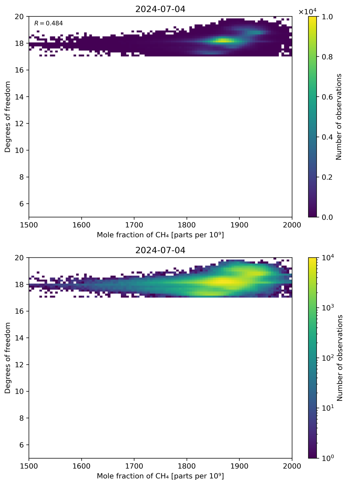
Figure 72: Scatter density plot of “Mole fraction of CH 4 ” against “Degrees of freedom” for 2024-07-03 to 2024-07-05.
