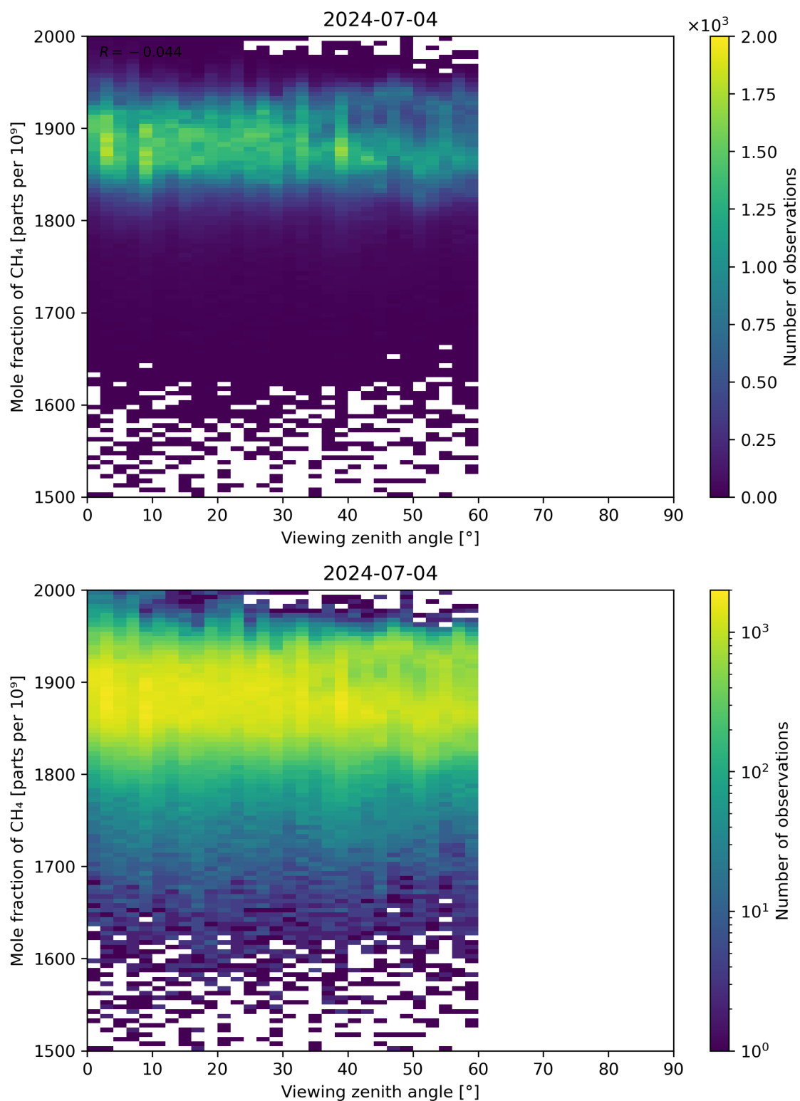
Figure 110: Scatter density plot of “Viewing zenith angle” against “Mole fraction of CH 4 ” for 2024-07-03 to 2024-07-05.
