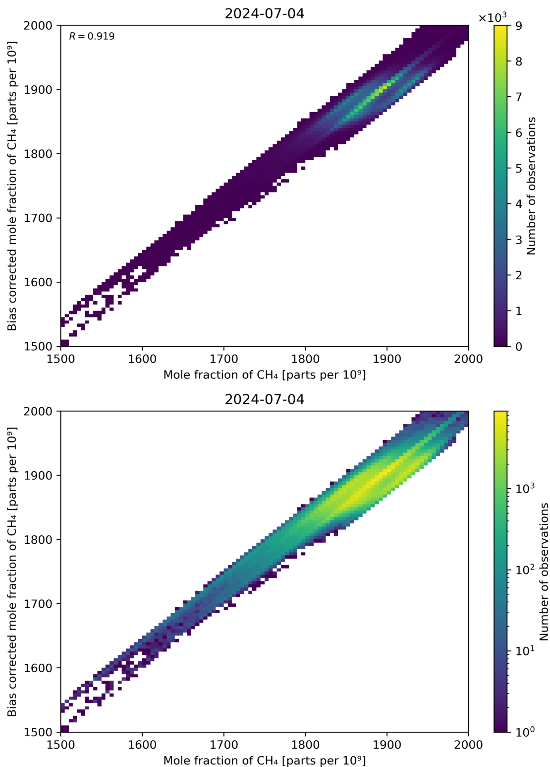
Figure 74: Scatter density plot of “Mole fraction of CH 4 ” against “Bias corrected mole fraction of CH 4 ” for 2024-07-03 to 2024-07-05.
