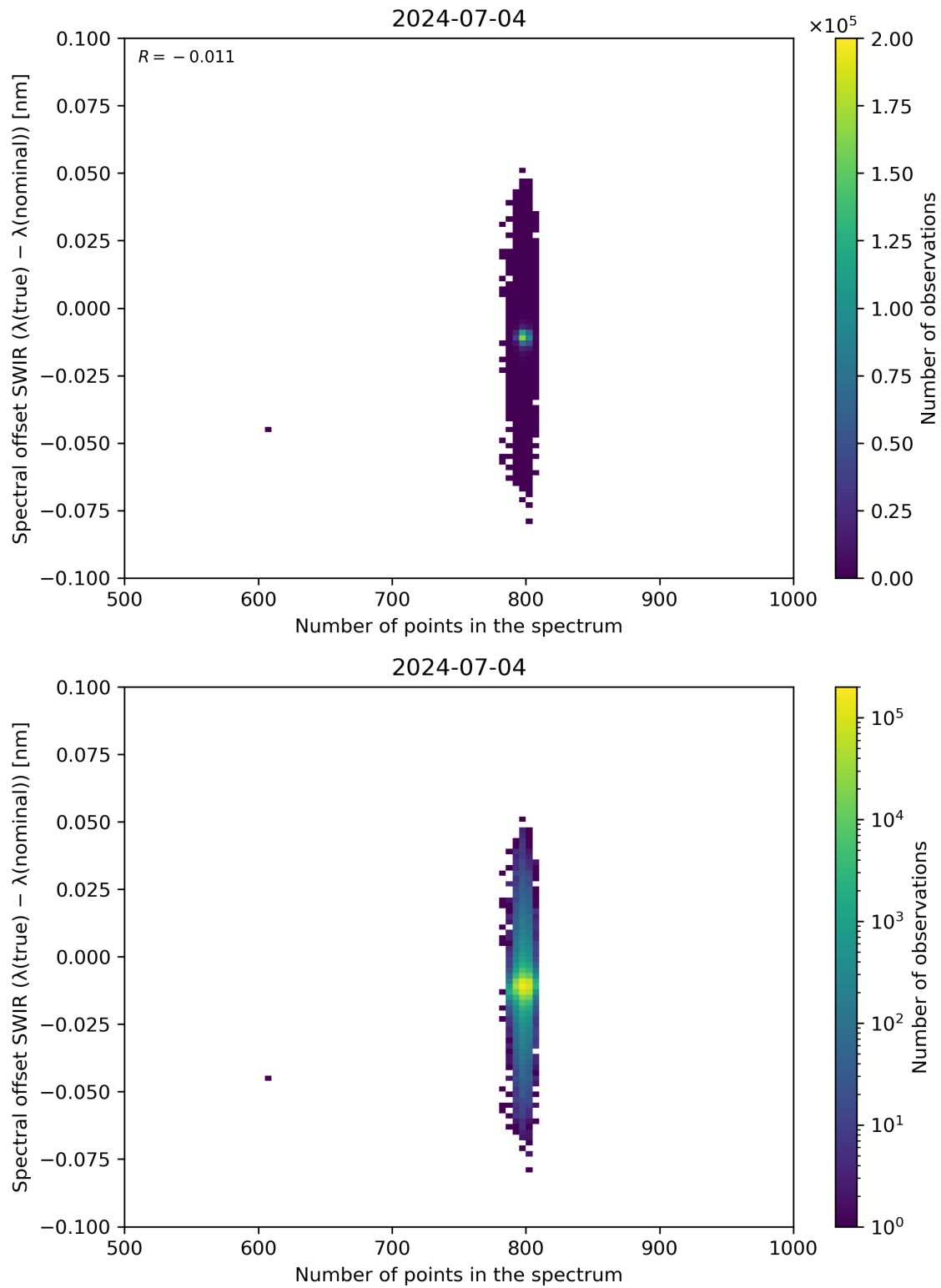
Figure 93: Scatter density plot of “Number of points in the spectrum” against “Spectral offset SWIR ( \lambda(\text{true}) - \lambda(\text{nominal}) )” for 2024-07-03 to 2024-07-05.
