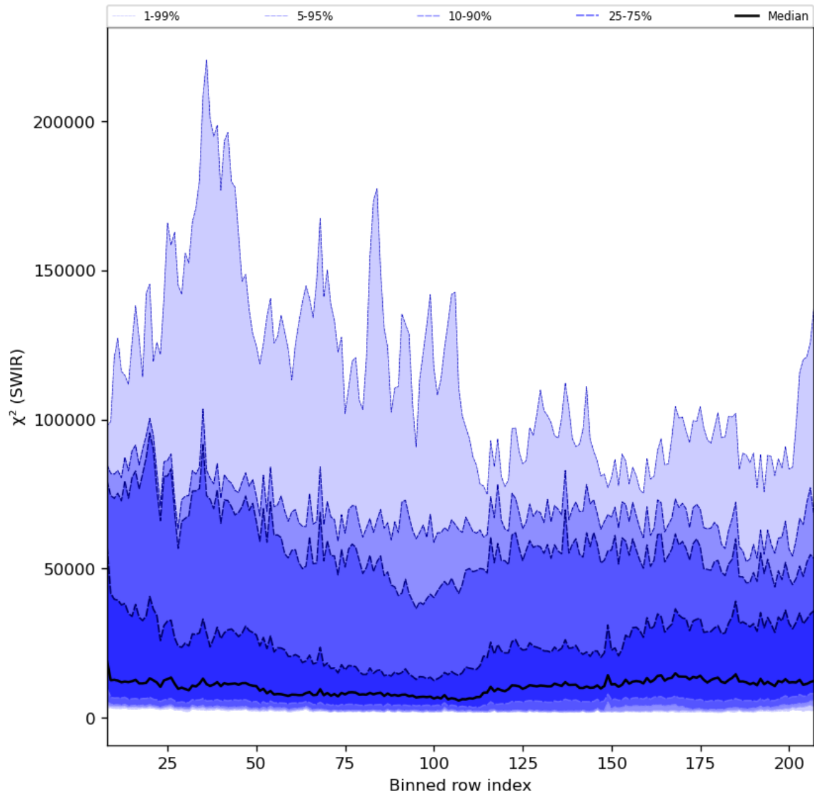
Figure 39: Along track statistics of “ \chi^2 (SWIR)” for 2024-07-03 to 2024-07-05
