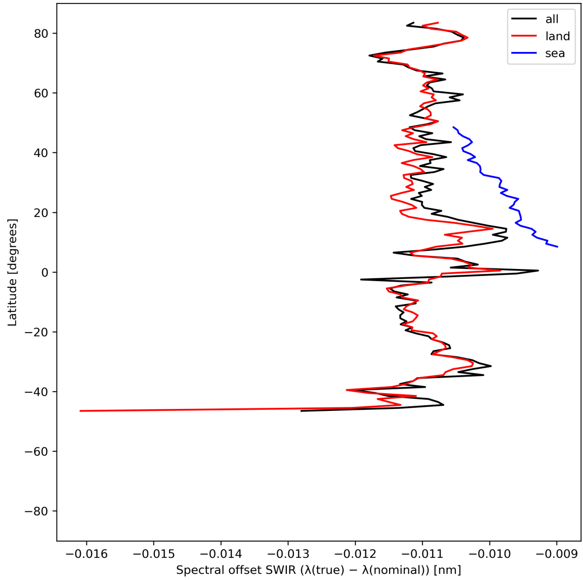
Figure 16: Zonal average of “Spectral offset SWIR ( \lambda(\text{true}) - \lambda(\text{nominal}) )” for 2024-07-03 to 2024-07-05.
