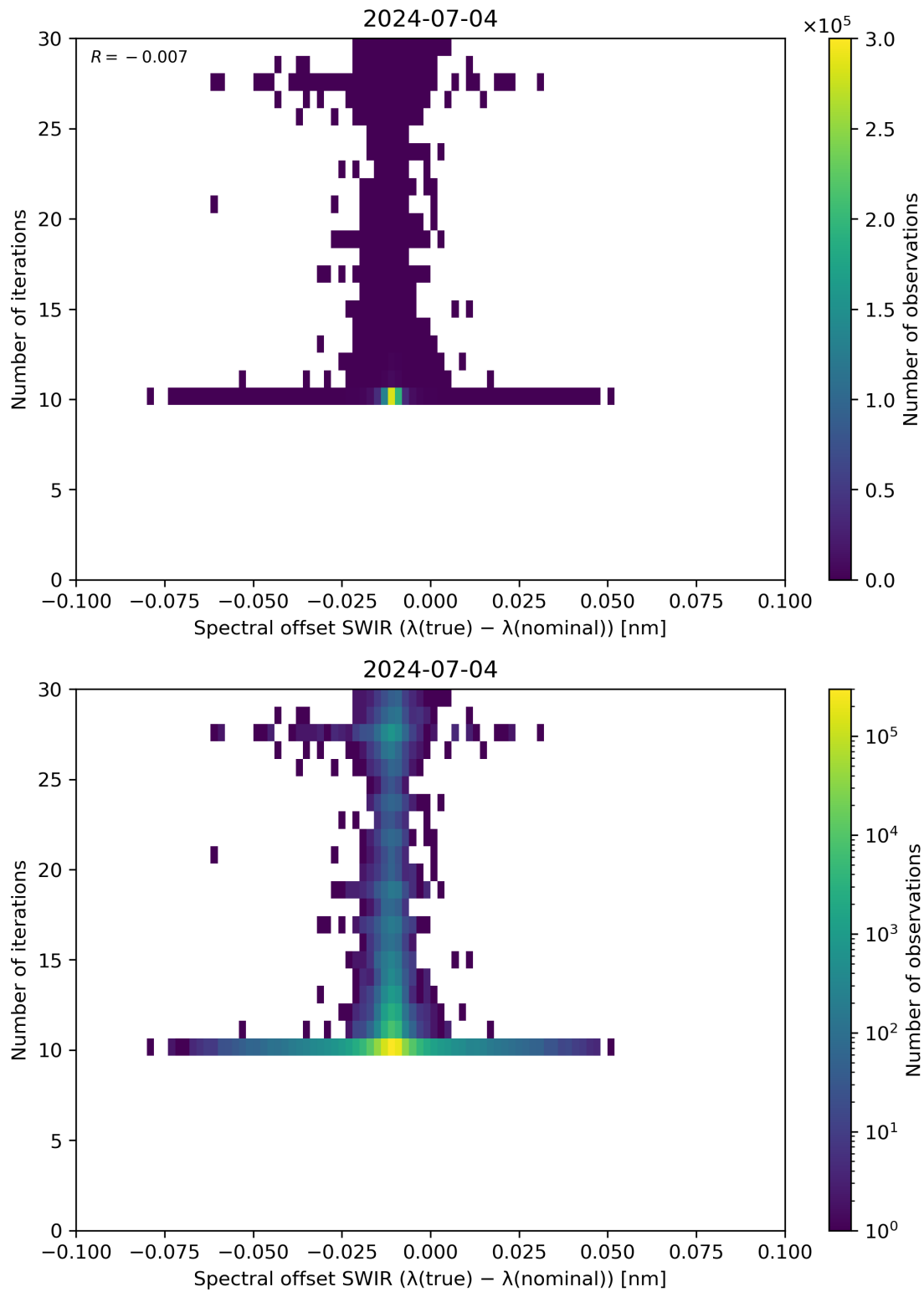
Figure 121: Scatter density plot of “Spectral offset SWIR ( \lambda(\text{true}) - \lambda(\text{nominal}) )” against “Number of iterations” for 2024-07-03 to 2024-07-05.
