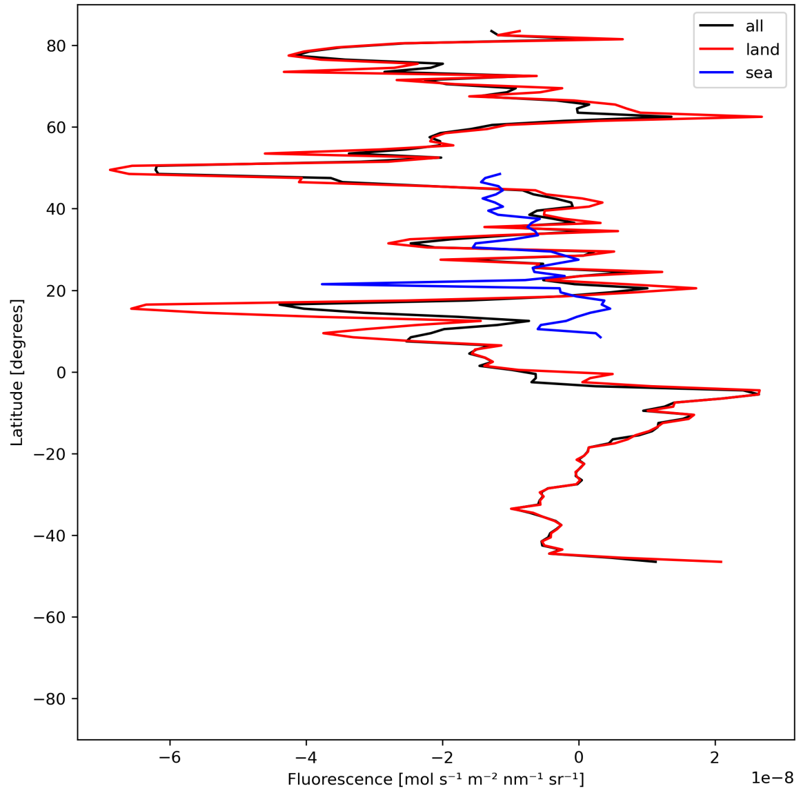
Figure 21: Zonal average of “Fluorescence” for 2024-07-03 to 2024-07-05.
