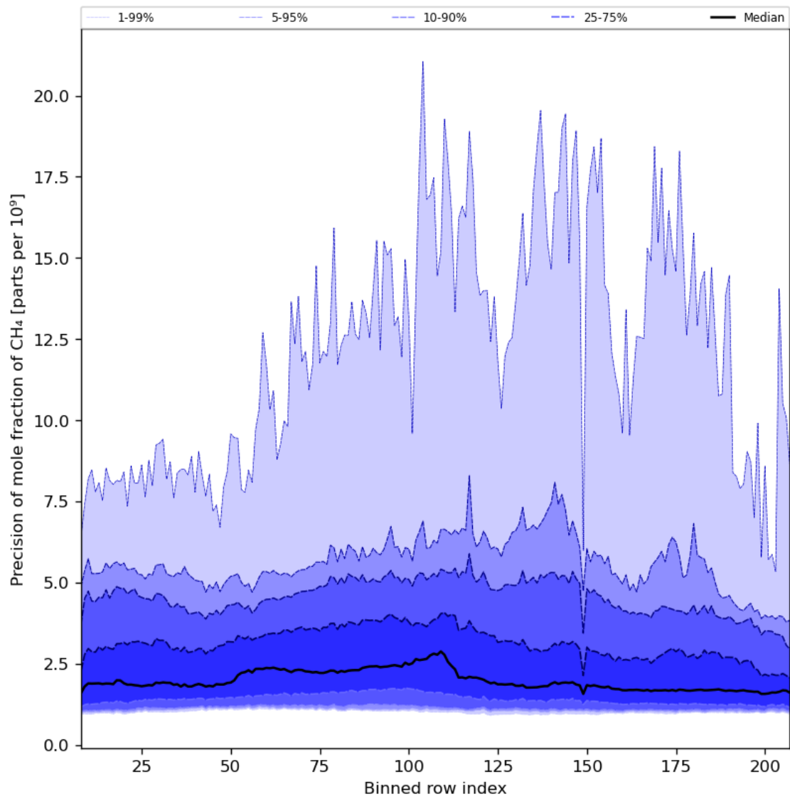
Figure 35: Along track statistics of “Precision of mole fraction of CH 4 ” for 2024-07-03 to 2024-07-05
