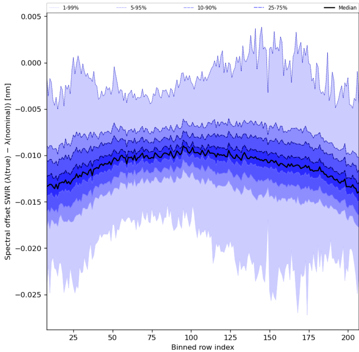
Figure 38: Along track statistics of “Spectral offset SWIR ( \lambda(\text{true}) - \lambda(\text{nominal}) )” for 2024-07-03 to 2024-07-05
