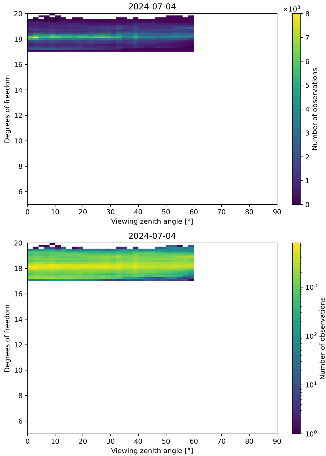
Figure 107: Scatter density plot of “Viewing zenith angle” against “Degrees of freedom” for 2024-07-03 to 2024-07-05.
