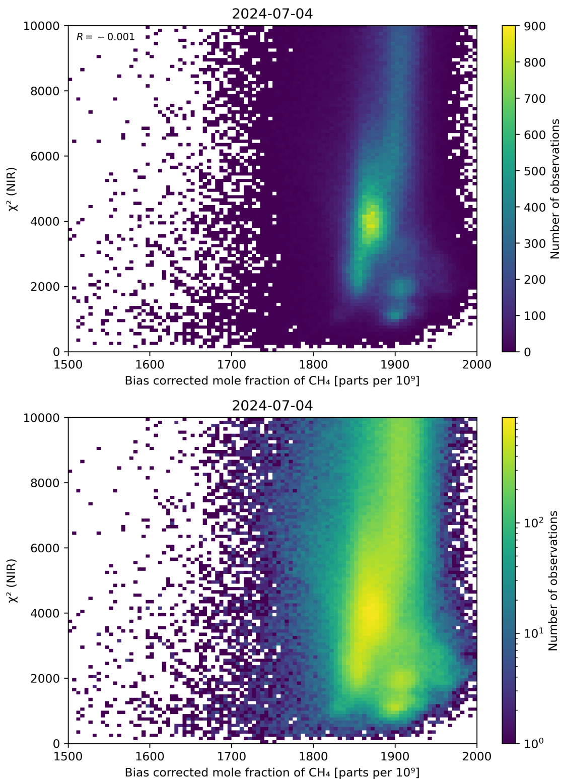
Figure 63: Scatter density plot of “Bias corrected mole fraction of CH 4 ” against “ \chi^2 (NIR)” for 2024-07-03 to 2024-07-05.
