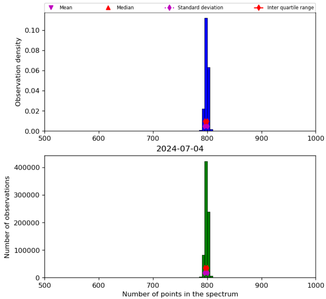
Figure 26: Histogram of “Number of points in the spectrum” for 2024-07-03 to 2024-07-05
