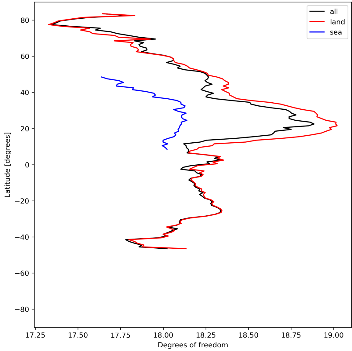
Figure 19: Zonal average of “Degrees of freedom” for 2024-07-03 to 2024-07-05.
