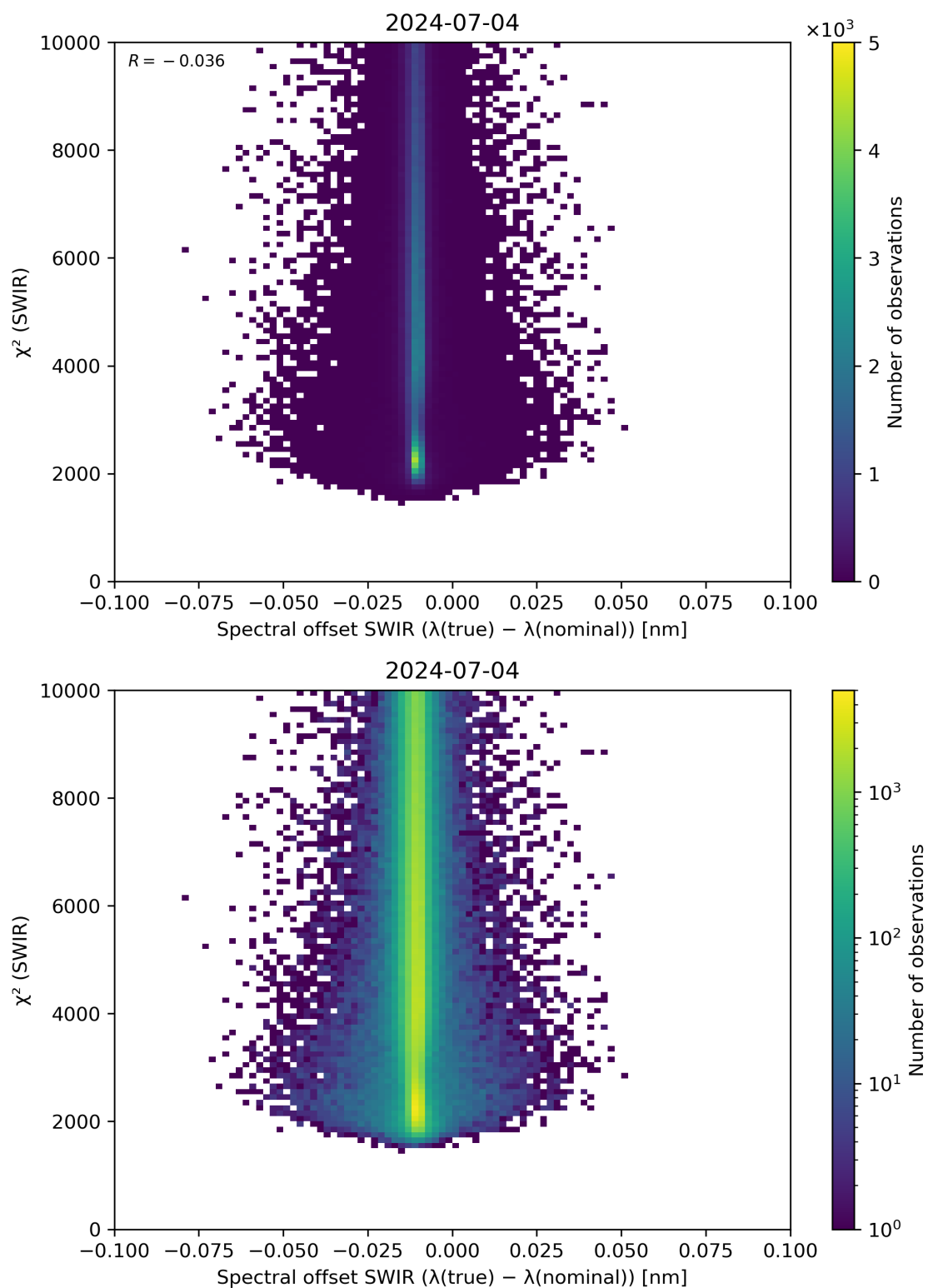
Figure 118: Scatter density plot of “Spectral offset SWIR ( \lambda(\text{true}) - \lambda(\text{nominal}) )” against “ \chi^2 (SWIR)” for 2024-07-03 to 2024-07-05.
