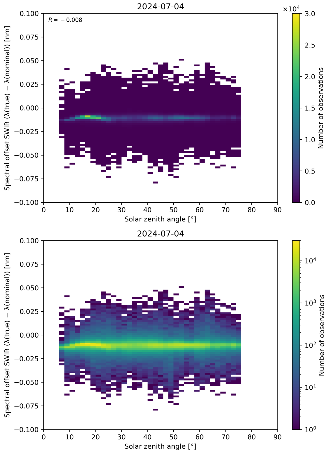
Figure 104: Scatter density plot of “Solar zenith angle” against “Spectral offset SWIR ( \lambda(\text{true}) - \lambda(\text{nominal}) )” for 2024-07-03 to 2024-07-05.
