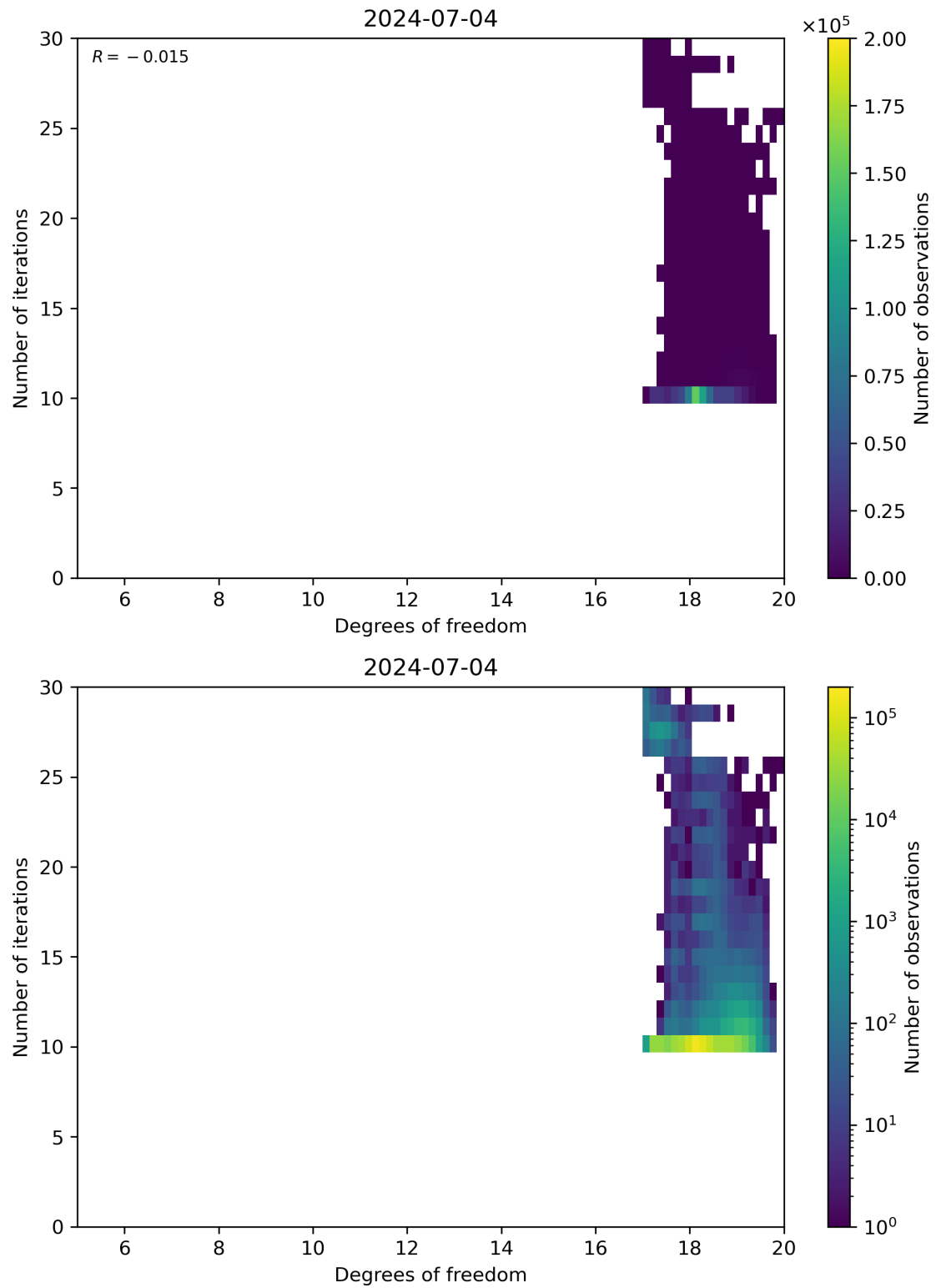
Figure 52: Scatter density plot of “Degrees of freedom” against “Number of iterations” for 2024-07-03 to 2024-07-05.
