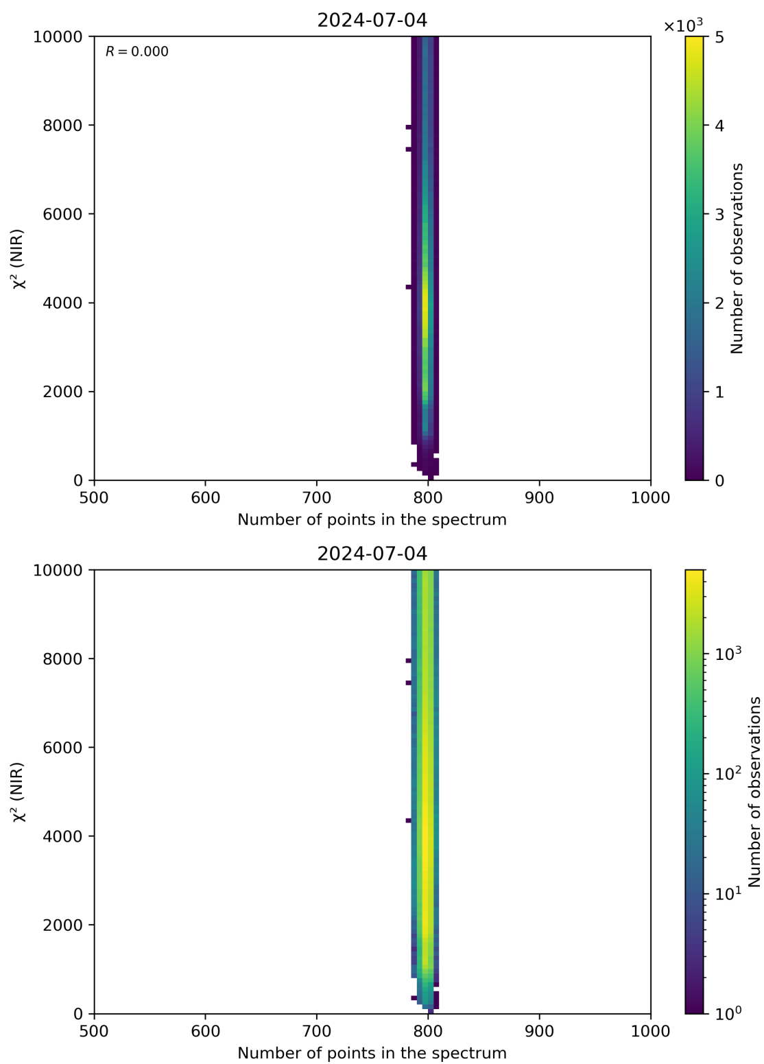
Figure 88: Scatter density plot of “Number of points in the spectrum” against “ \chi^2 (NIR)” for 2024-07-03 to 2024-07-05.
