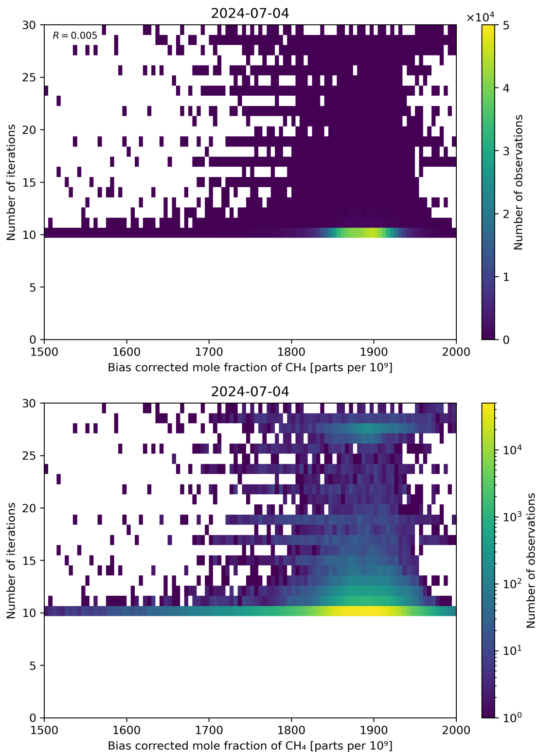
Figure 67: Scatter density plot of “Bias corrected mole fraction of \text{CH}_4 ” against “Number of iterations” for 2024-07-03 to 2024-07-05.
