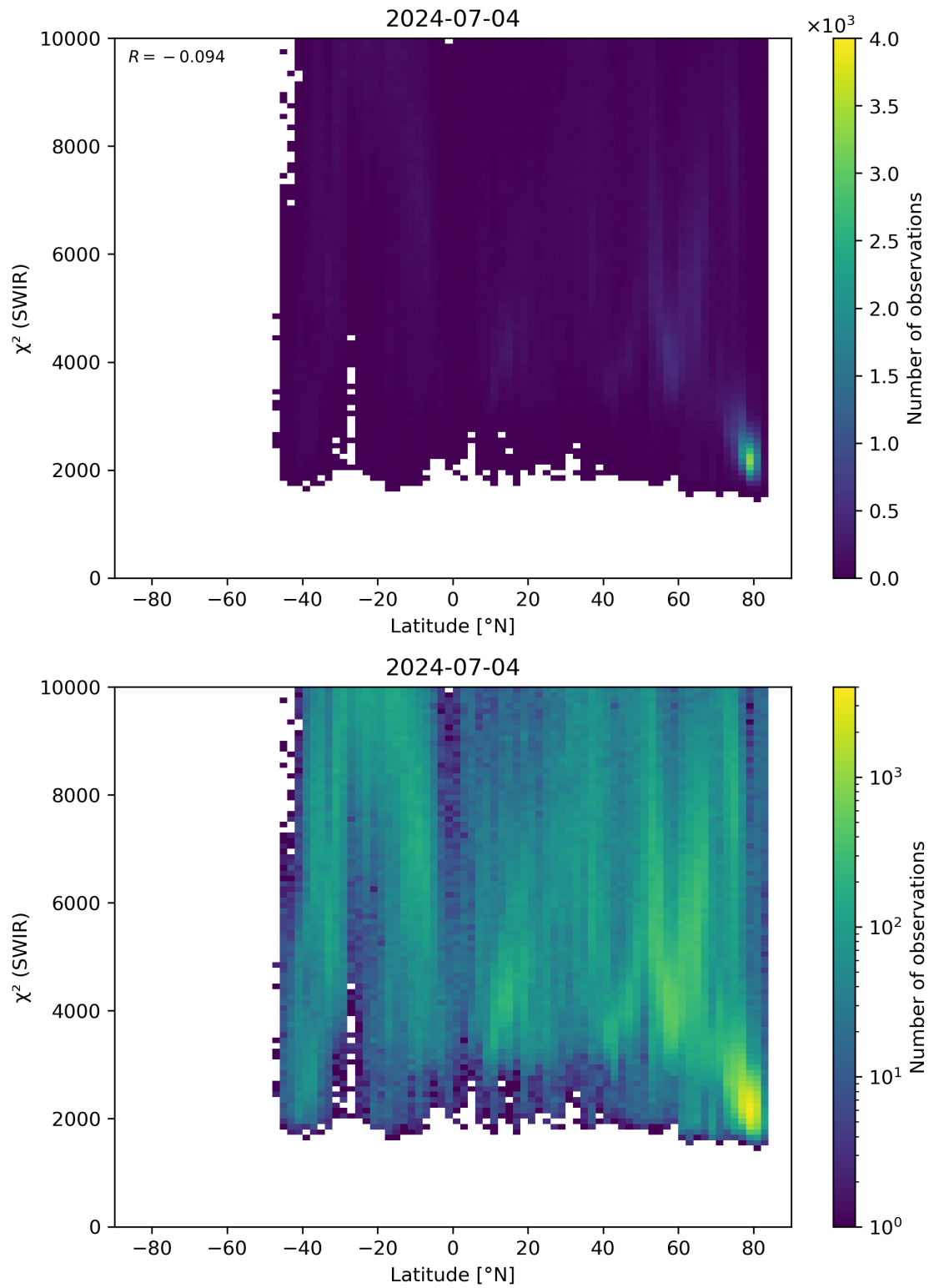
Figure 54: Scatter density plot of “Latitude” against “ \chi^2 (SWIR)” for 2024-07-03 to 2024-07-05.
