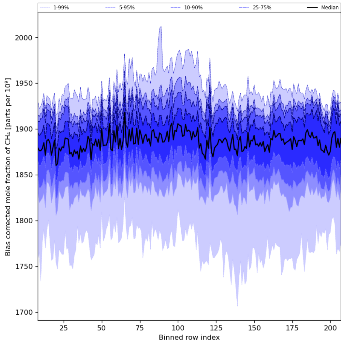
Figure 36: Along track statistics of “Bias corrected mole fraction of CH 4 ” for 2024-07-03 to 2024-07-05
