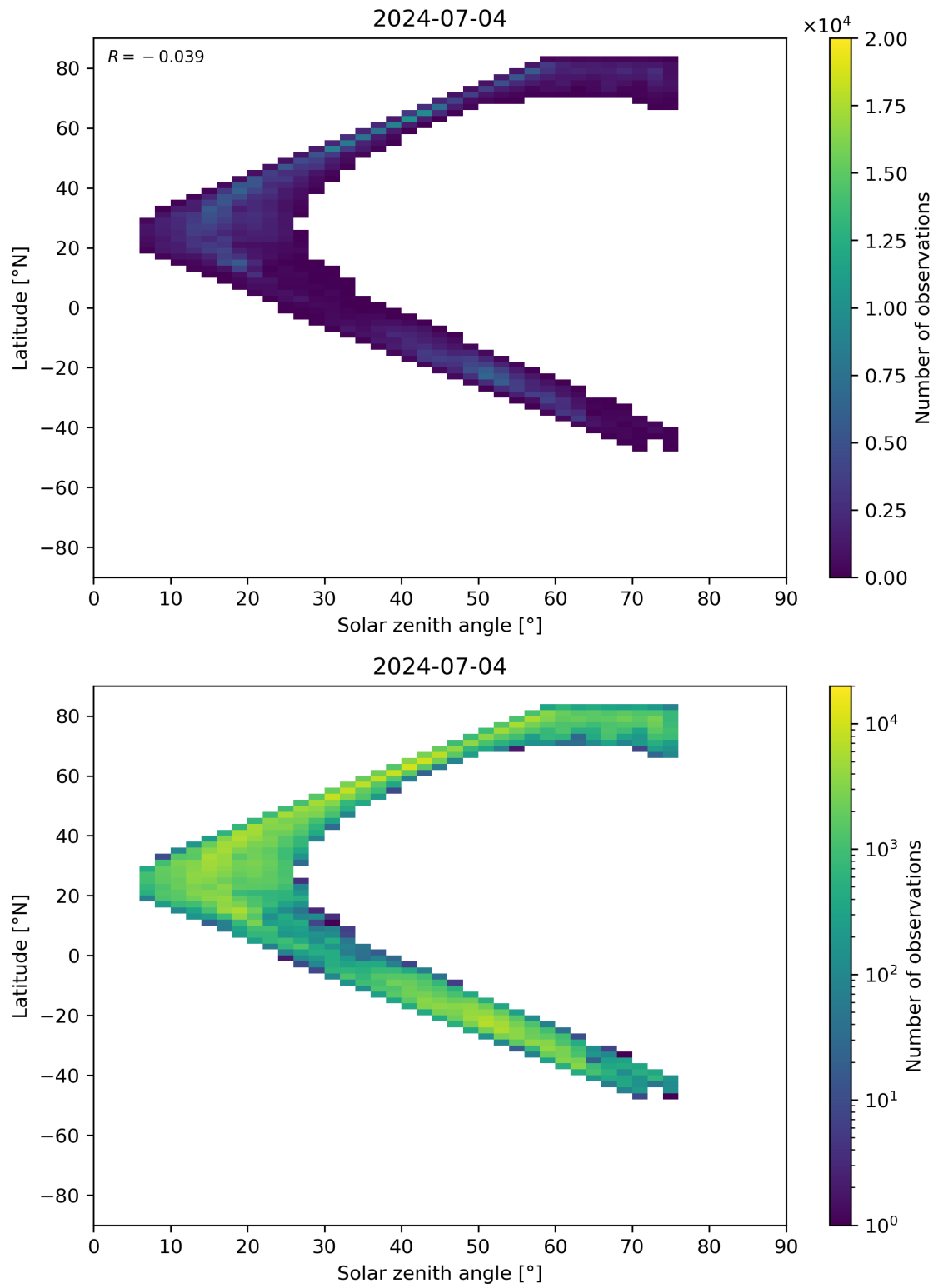
Figure 98: Scatter density plot of “Solar zenith angle” against “Latitude” for 2024-07-03 to 2024-07-05.
