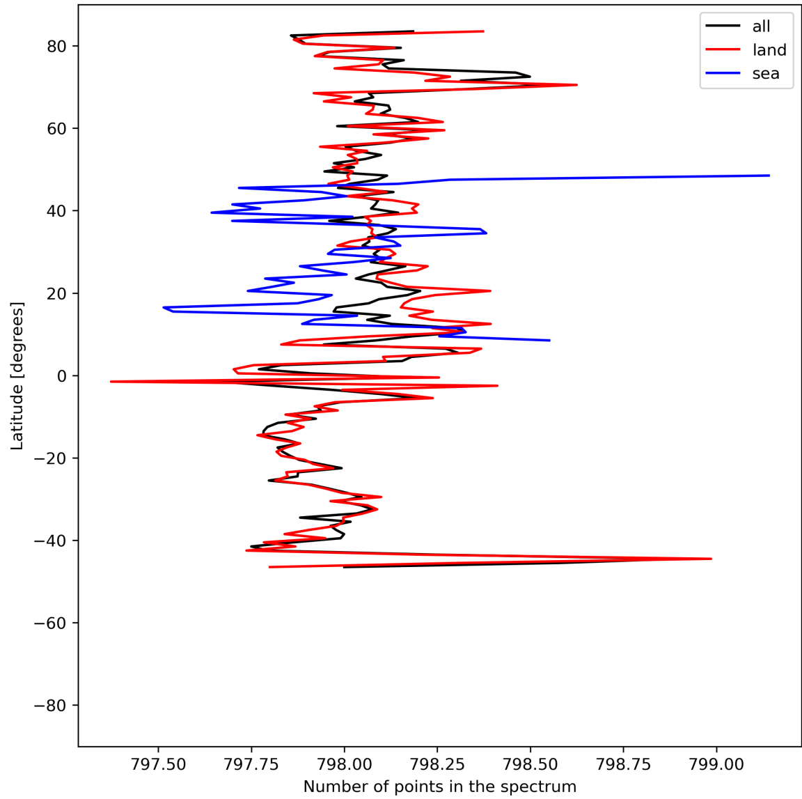
Figure 15: Zonal average of “Number of points in the spectrum” for 2024-07-03 to 2024-07-05.
