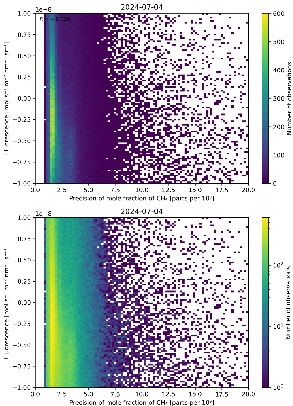
Figure 81: Scatter density plot of “Precision of mole fraction of \text{CH}_4 ” against “Fluorescence” for 2024-07-03 to 2024-07-05.
