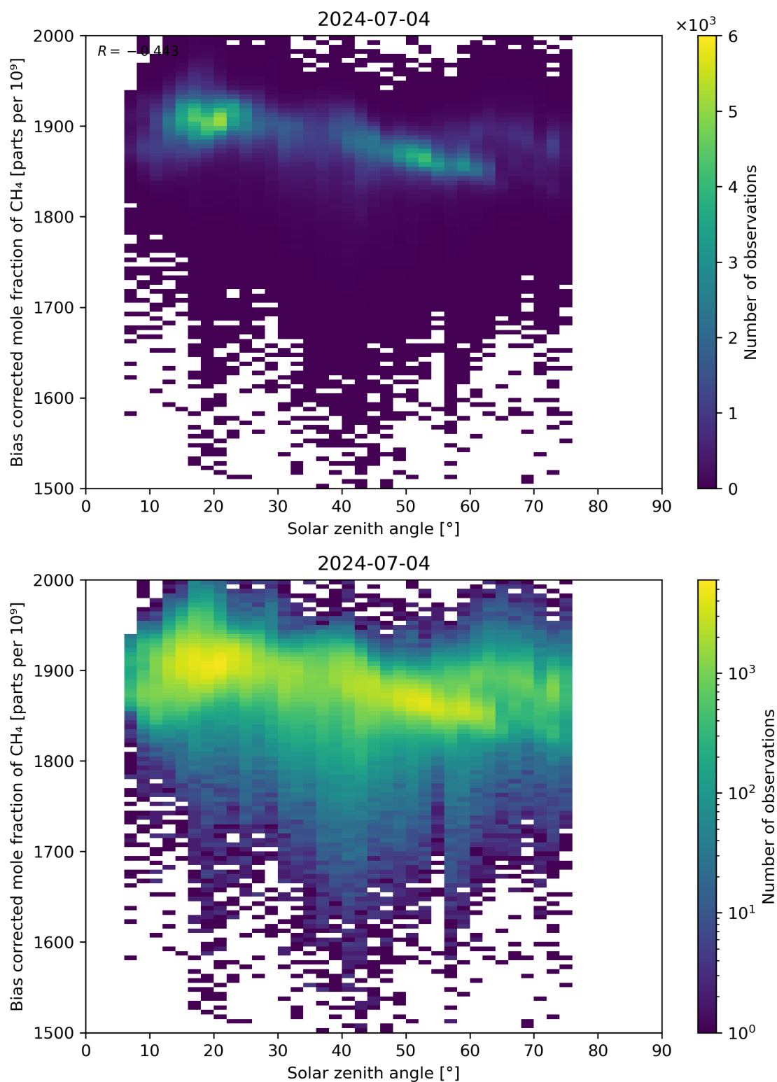
Figure 100: Scatter density plot of “Solar zenith angle” against “Bias corrected mole fraction of \text{CH}_4 ” for 2024-07-03 to 2024-07-05.
