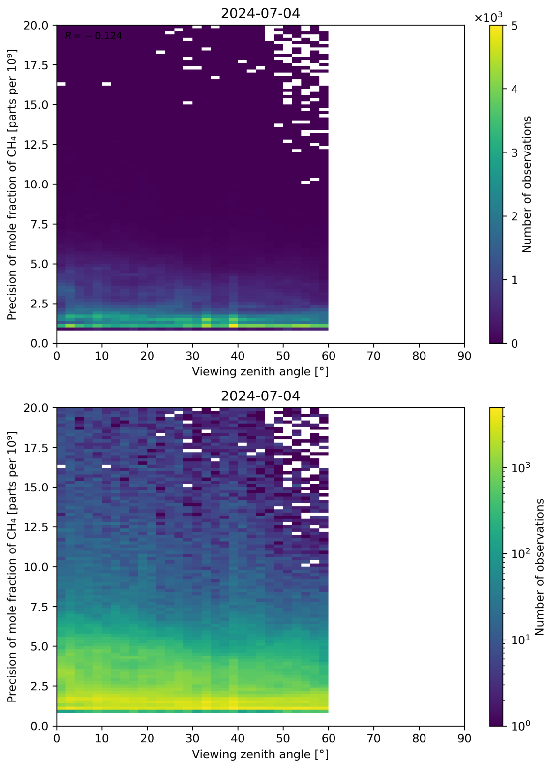
Figure 112: Scatter density plot of “Viewing zenith angle” against “Precision of mole fraction of CH 4 ” for 2024-07-03 to 2024-07-05.
