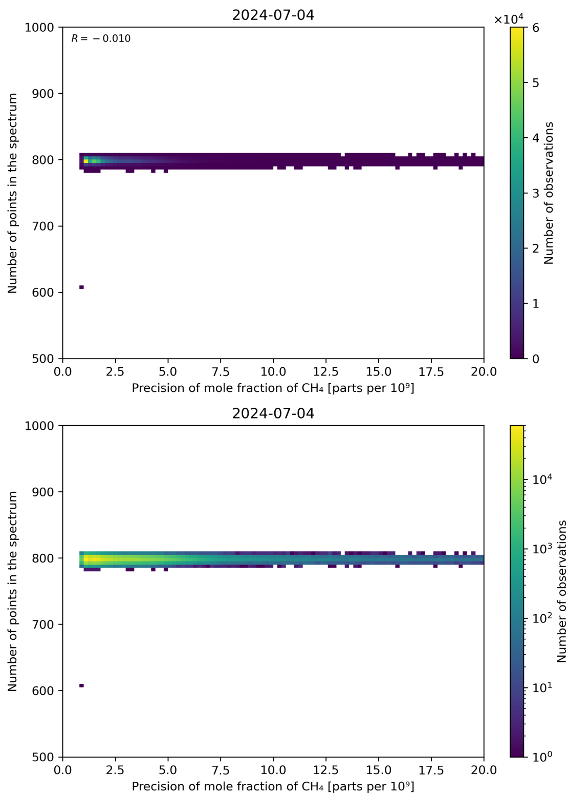
Figure 84: Scatter density plot of “Precision of mole fraction of CH 4 ” against “Number of points in the spectrum” for 2024-07-03 to 2024-07-05.
