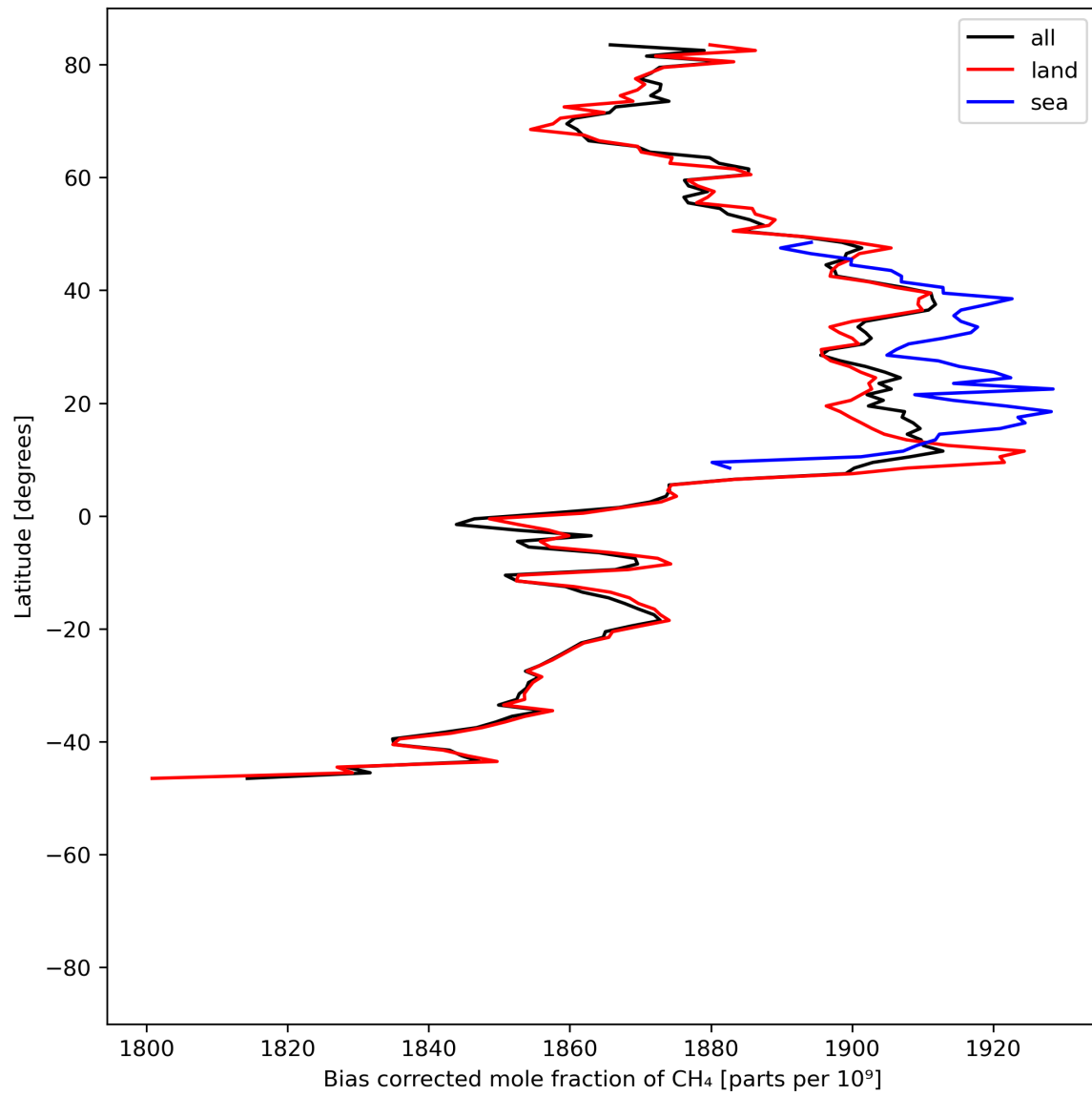
Figure 14: Zonal average of “Bias corrected mole fraction of CH 4 ” for 2024-07-03 to 2024-07-05.
