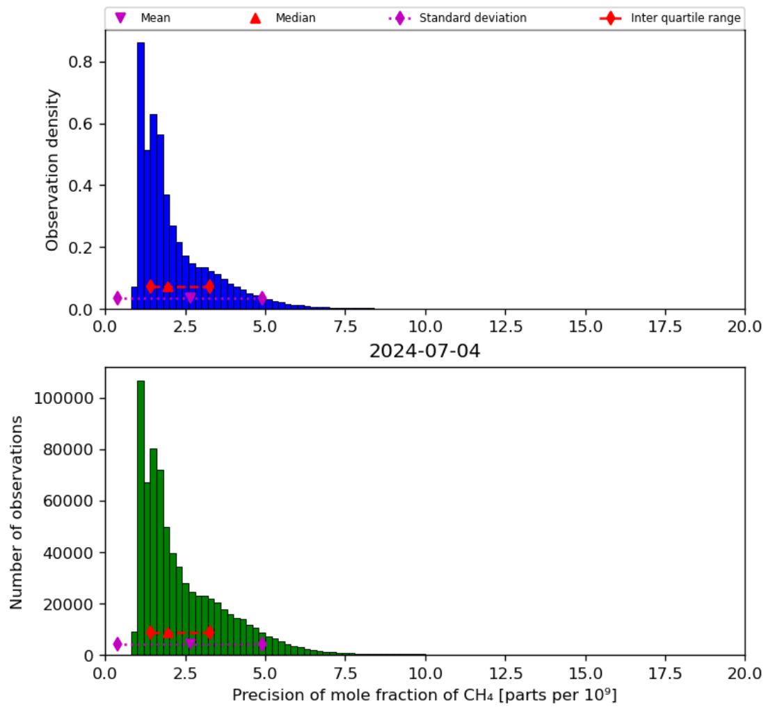
Figure 24: Histogram of “Precision of mole fraction of CH 4 ” for 2024-07-03 to 2024-07-05
