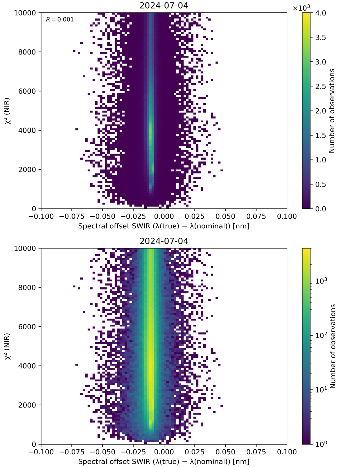
Figure 117: Scatter density plot of “Spectral offset SWIR ( \lambda(\text{true}) - \lambda(\text{nominal}) )” against “ \chi^2 (NIR)” for 2024-07-03 to 2024-07-05.
