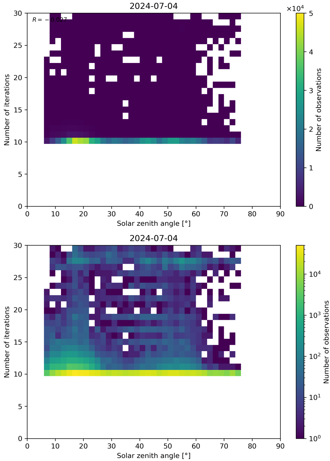
Figure 102: Scatter density plot of “Solar zenith angle” against “Number of iterations” for 2024-07-03 to 2024-07-05.
