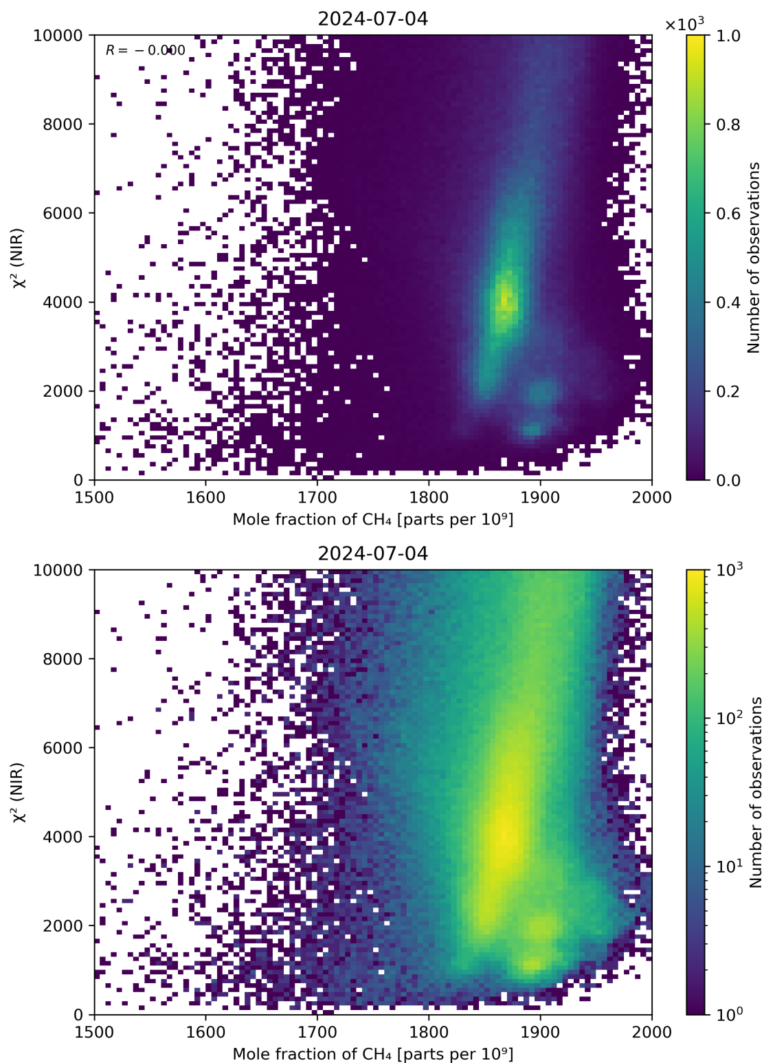
Figure 70: Scatter density plot of “Mole fraction of \text{CH}_4 ” against “ \chi^2 (NIR)” for 2024-07-03 to 2024-07-05.
