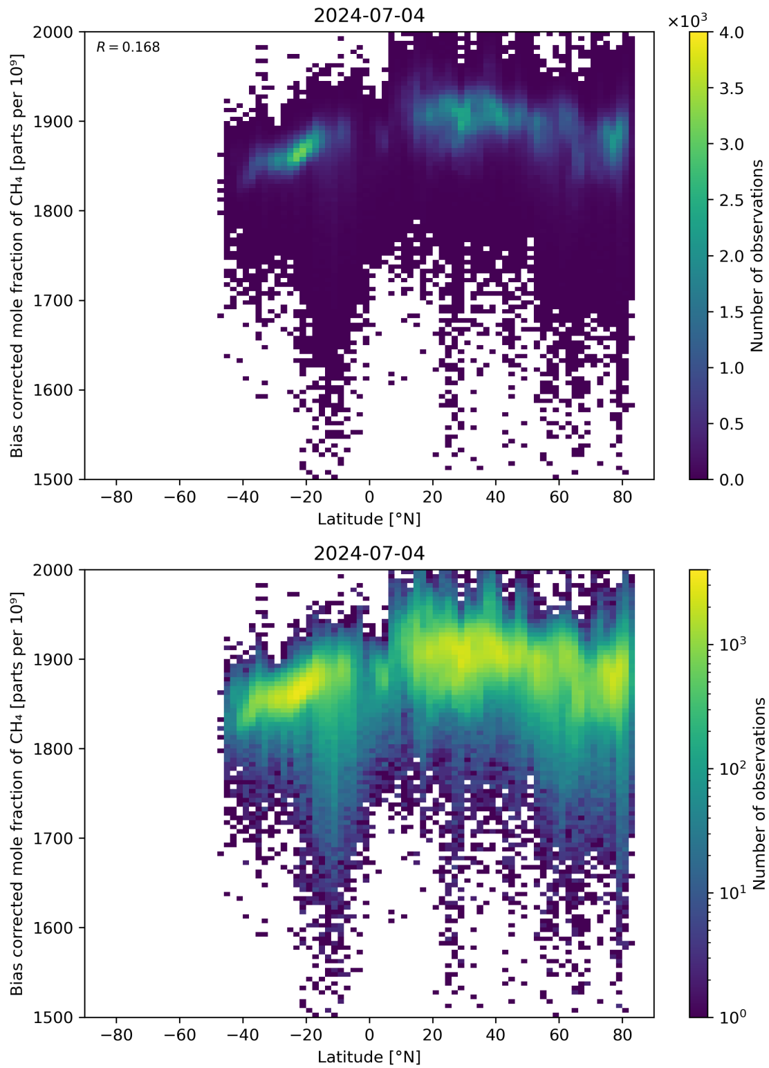
Figure 58: Scatter density plot of “Latitude” against “Bias corrected mole fraction of \text{CH}_4 ” for 2024-07-03 to 2024-07-05.
