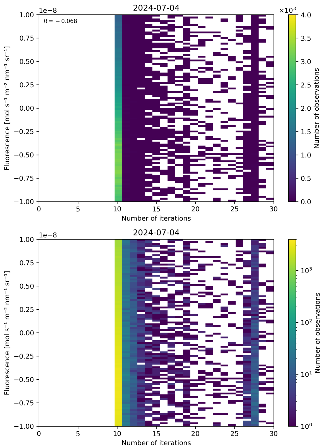
Figure 87: Scatter density plot of “Number of iterations” against “Fluorescence” for 2024-07-03 to 2024-07-05.
