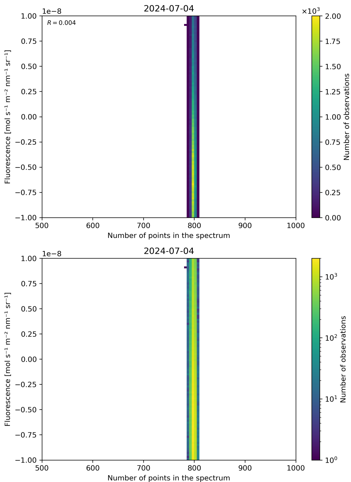
Figure 91: Scatter density plot of “Number of points in the spectrum” against “Fluorescence” for 2024-07-03 to 2024-07-05.
