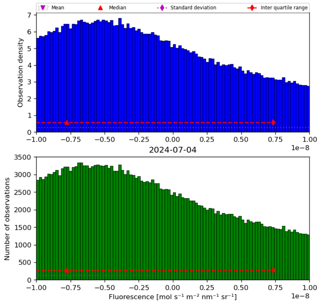
Figure 32: Histogram of “Fluorescence” for 2024-07-03 to 2024-07-05
