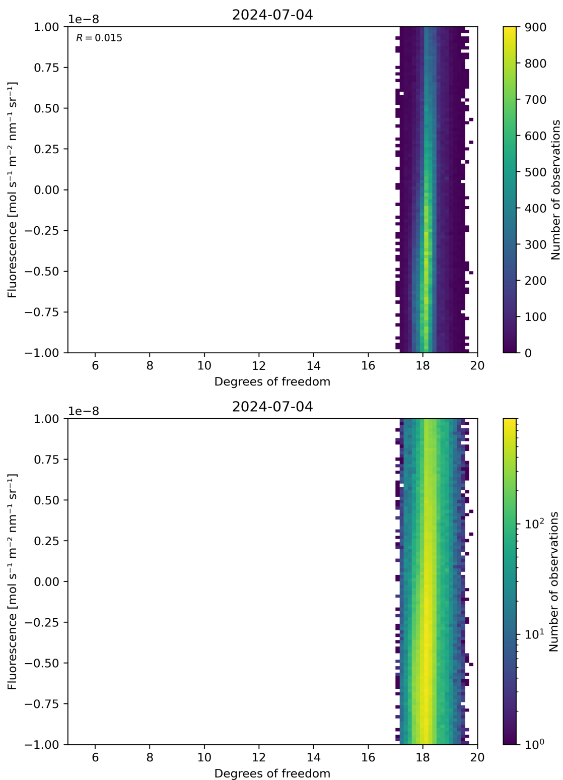
Figure 51: Scatter density plot of “Degrees of freedom” against “Fluorescence” for 2024-07-03 to 2024-07-05.
