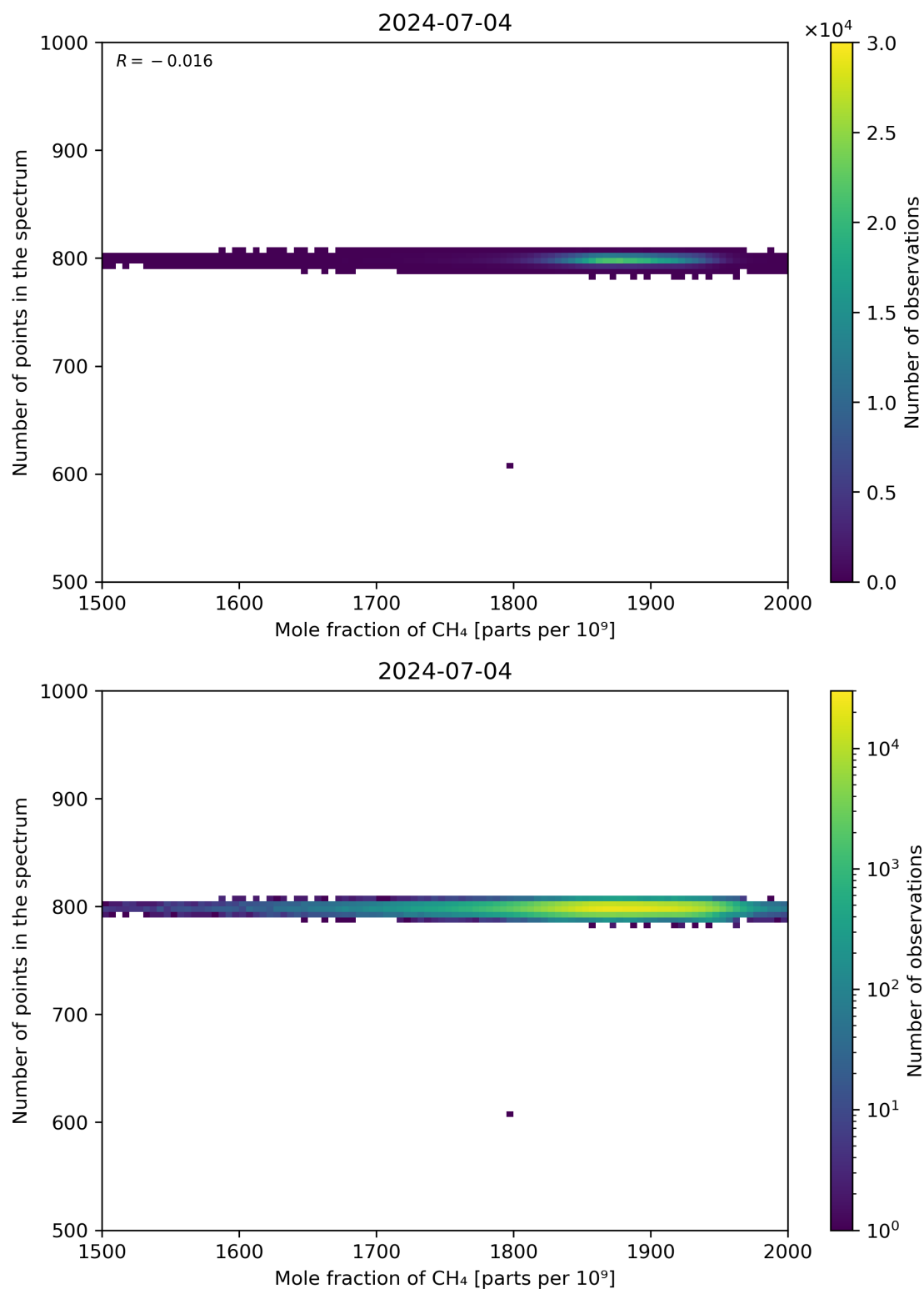
Figure 77: Scatter density plot of “Mole fraction of CH 4 ” against “Number of points in the spectrum” for 2024-07-03 to 2024-07-05.
