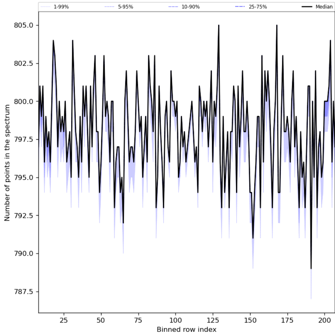
Figure 37: Along track statistics of “Number of points in the spectrum” for 2024-07-03 to 2024-07-05
