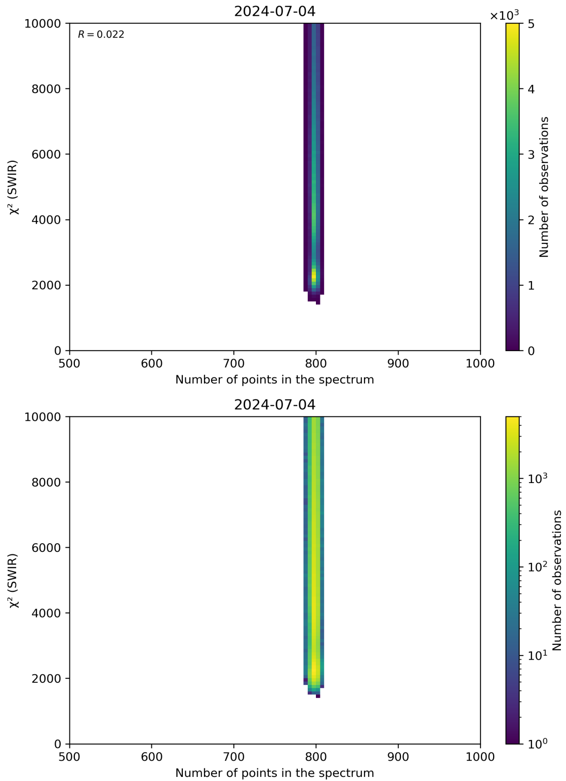
Figure 89: Scatter density plot of “Number of points in the spectrum” against “ \chi^2 (SWIR)” for 2024-07-03 to 2024-07-05.
