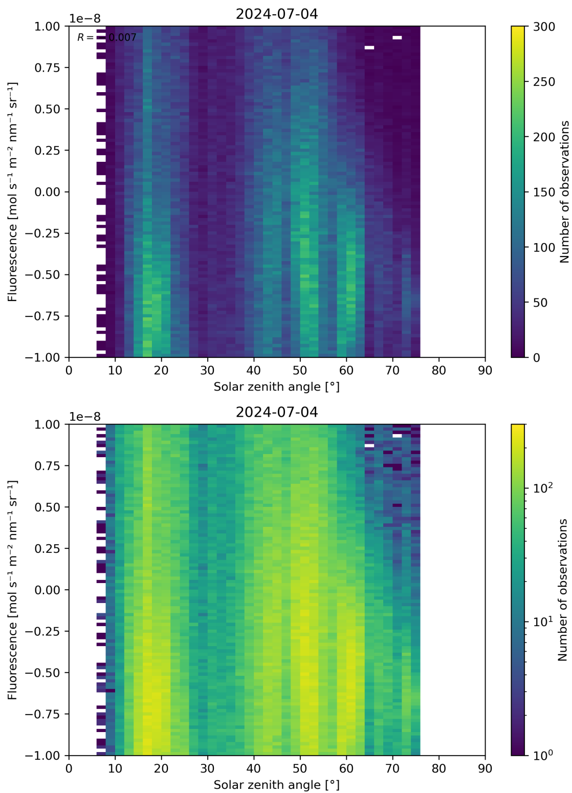
Figure 97: Scatter density plot of “Solar zenith angle” against “Fluorescence” for 2024-07-03 to 2024-07-05.
