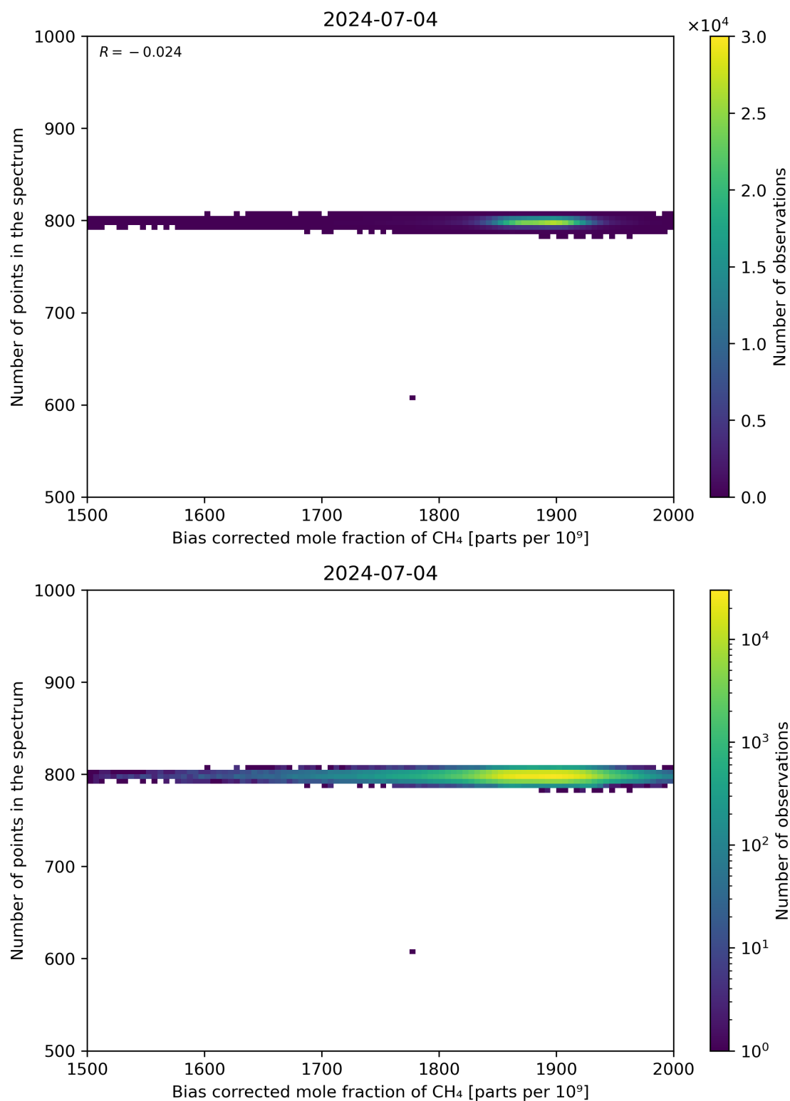
Figure 68: Scatter density plot of “Bias corrected mole fraction of CH 4 ” against “Number of points in the spectrum” for 2024-07-03 to 2024-07-05.
