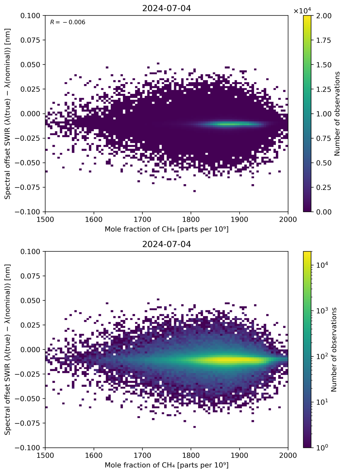
Figure 86: Scatter density plot of “Mole fraction of CH 4 ” against “Spectral offset SWIR ( \lambda(\text{true}) - \lambda(\text{nominal}) )” for 2024-07-03 to 2024-07-05.
