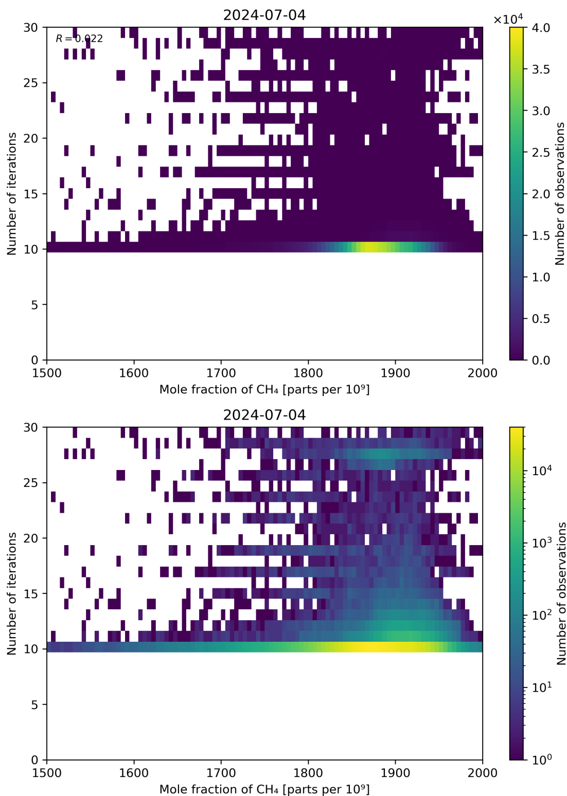
Figure 76: Scatter density plot of “Mole fraction of CH 4 ” against “Number of iterations” for 2024-07-03 to 2024-07-05.
