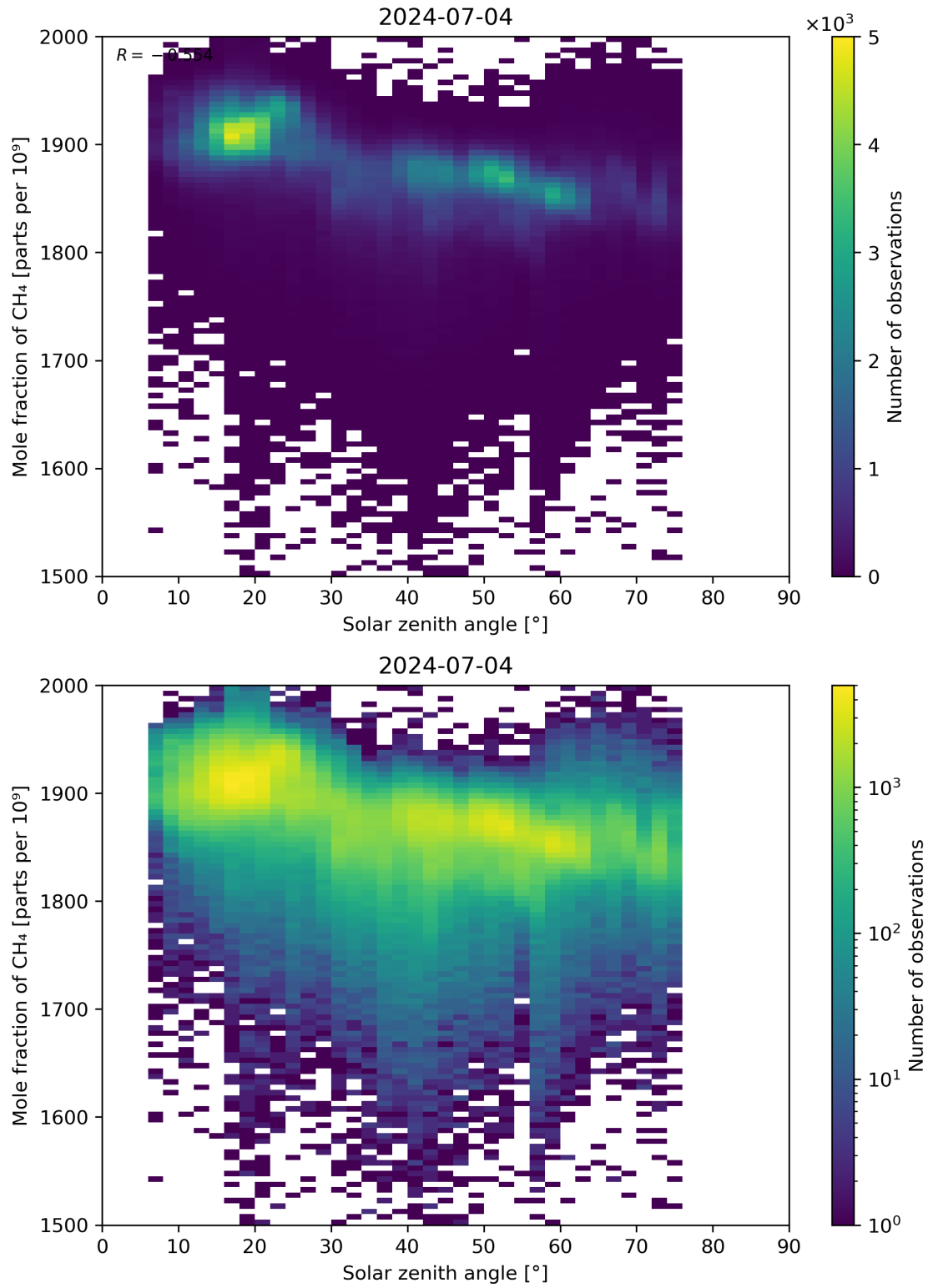
Figure 99: Scatter density plot of “Solar zenith angle” against “Mole fraction of CH 4 ” for 2024-07-03 to 2024-07-05.
