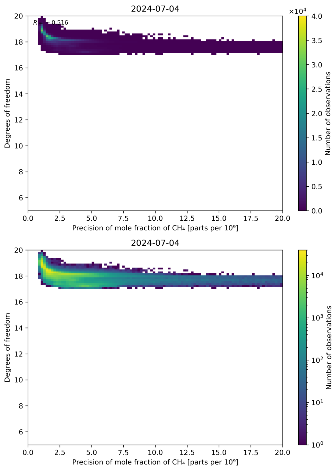
Figure 80: Scatter density plot of “Precision of mole fraction of CH 4 ” against “Degrees of freedom” for 2024-07-03 to 2024-07-05.
