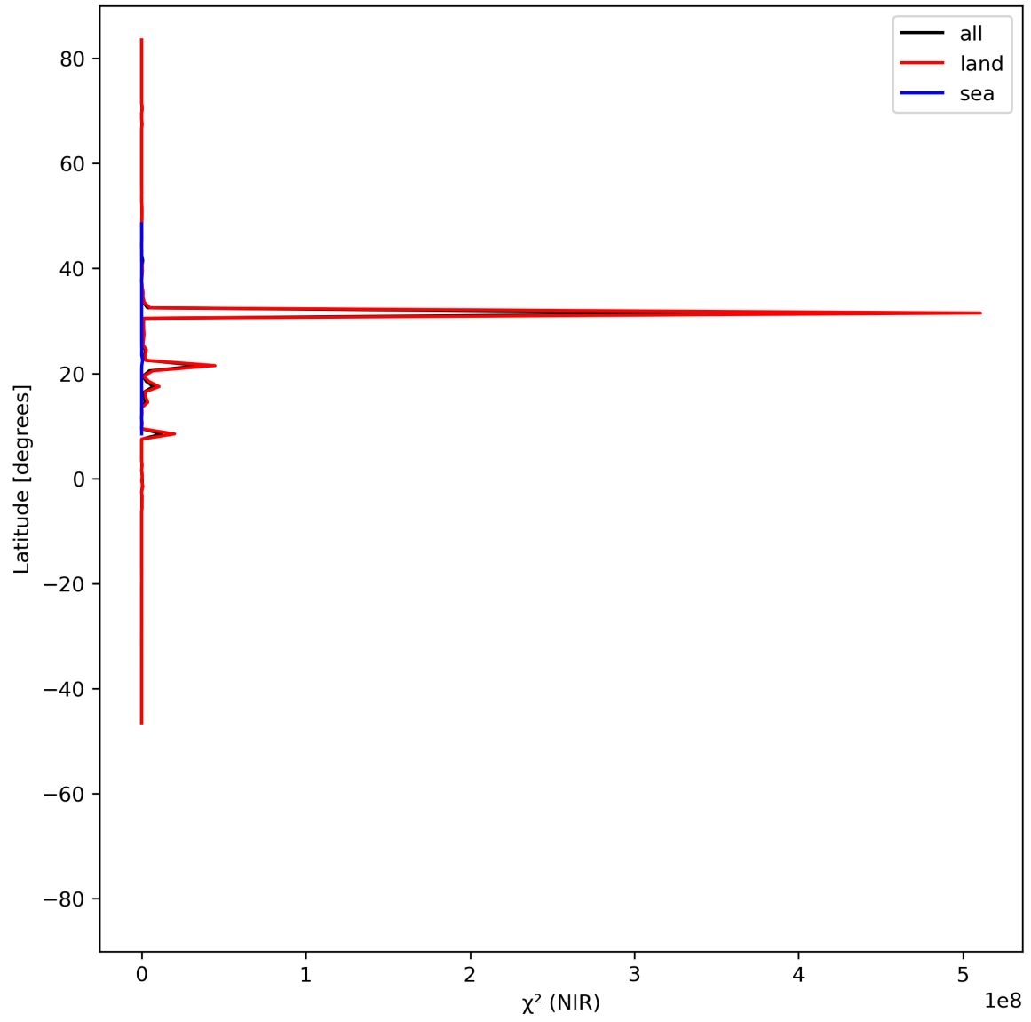
Figure 18: Zonal average of “ \chi^2 (NIR)” for 2024-07-03 to 2024-07-05.
