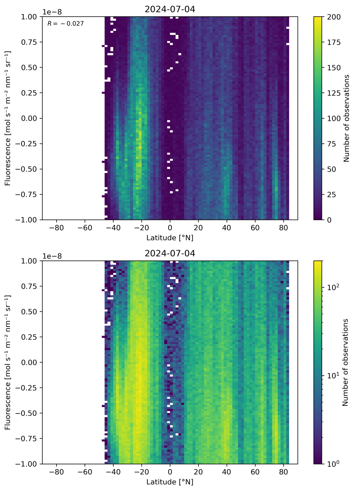
Figure 56: Scatter density plot of “Latitude” against “Fluorescence” for 2024-07-03 to 2024-07-05.
