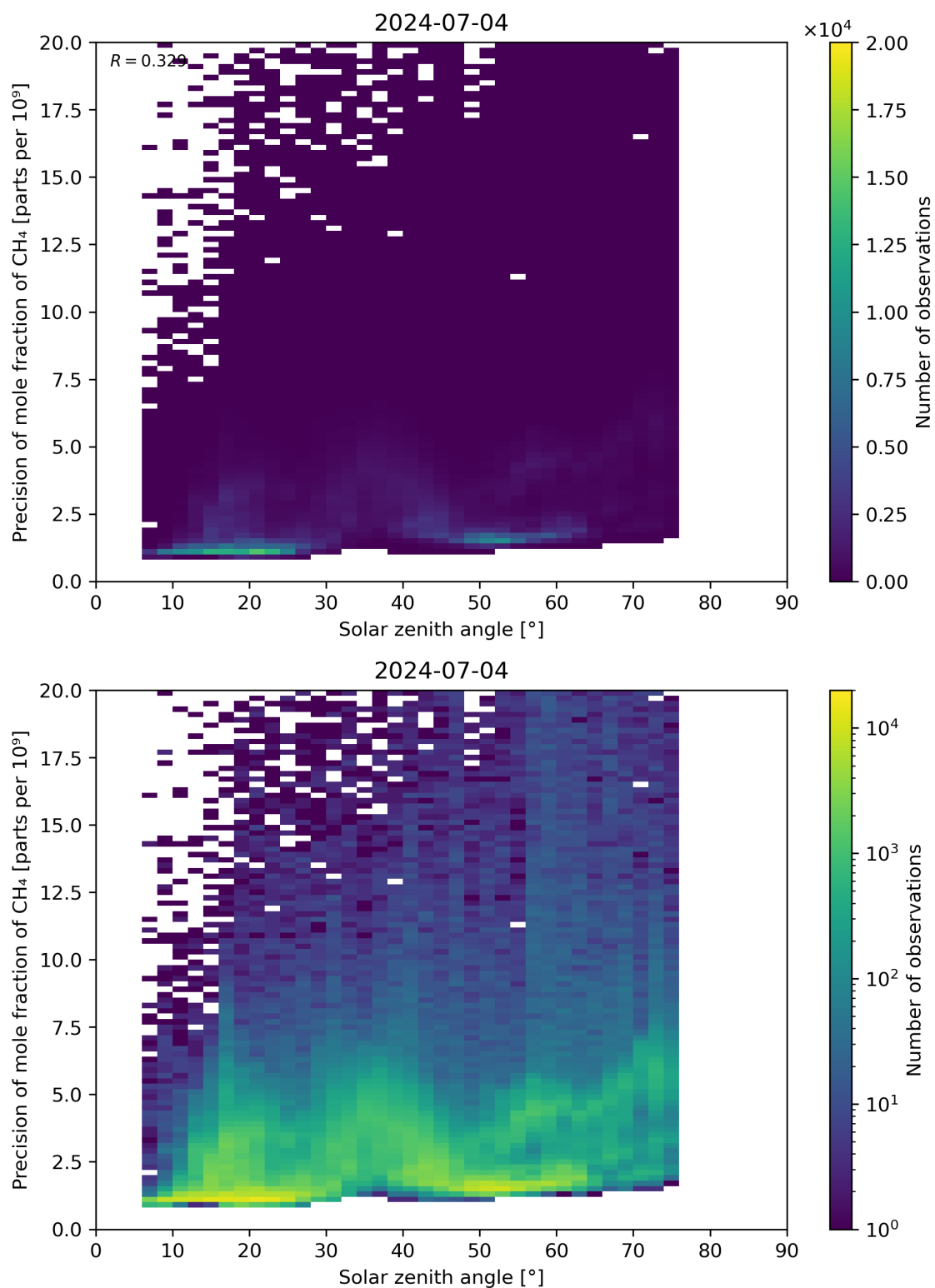
Figure 101: Scatter density plot of “Solar zenith angle” against “Precision of mole fraction of CH 4 ” for 2024-07-03 to 2024-07-05.
