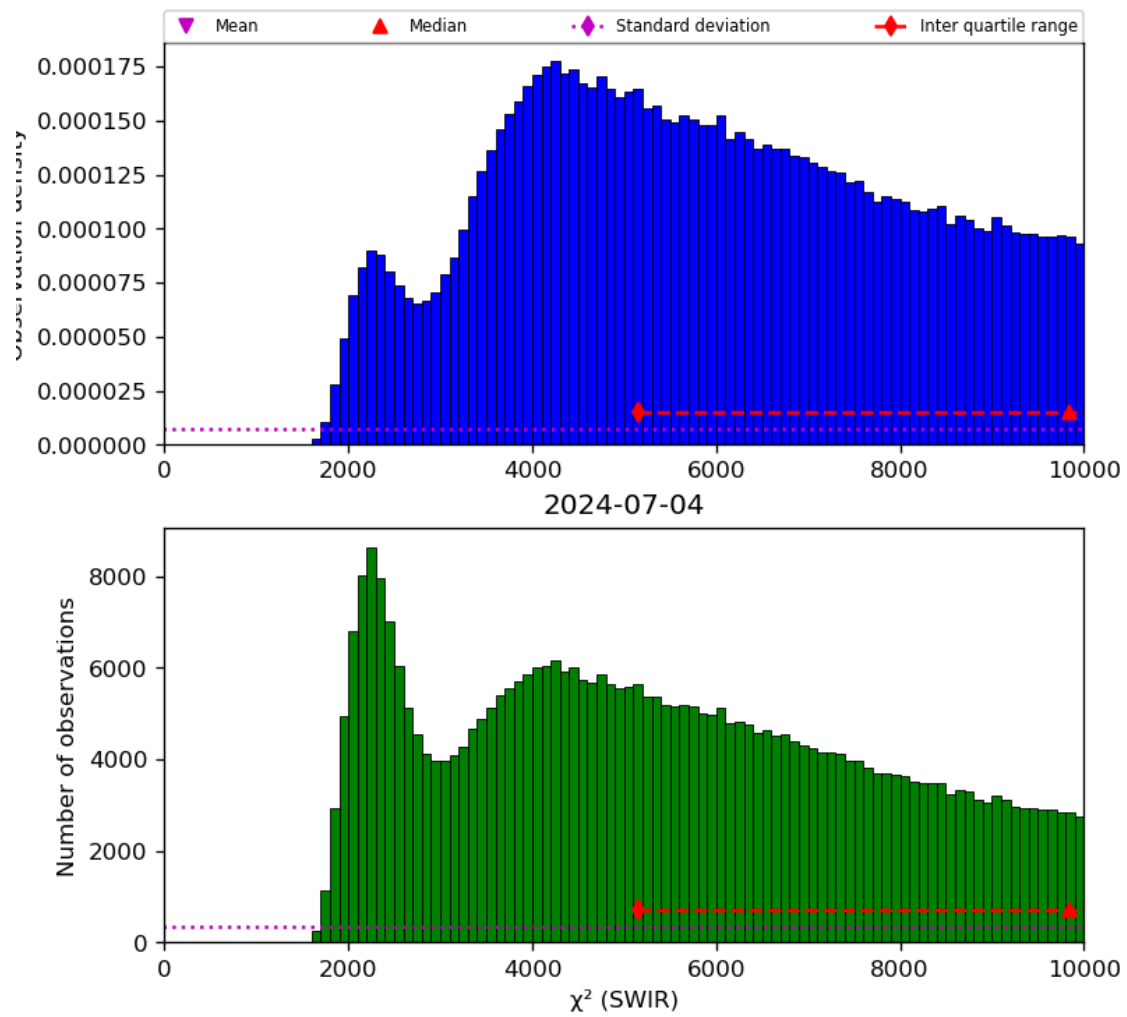
Figure 28: Histogram of “ \chi^2 (SWIR)” for 2024-07-03 to 2024-07-05
