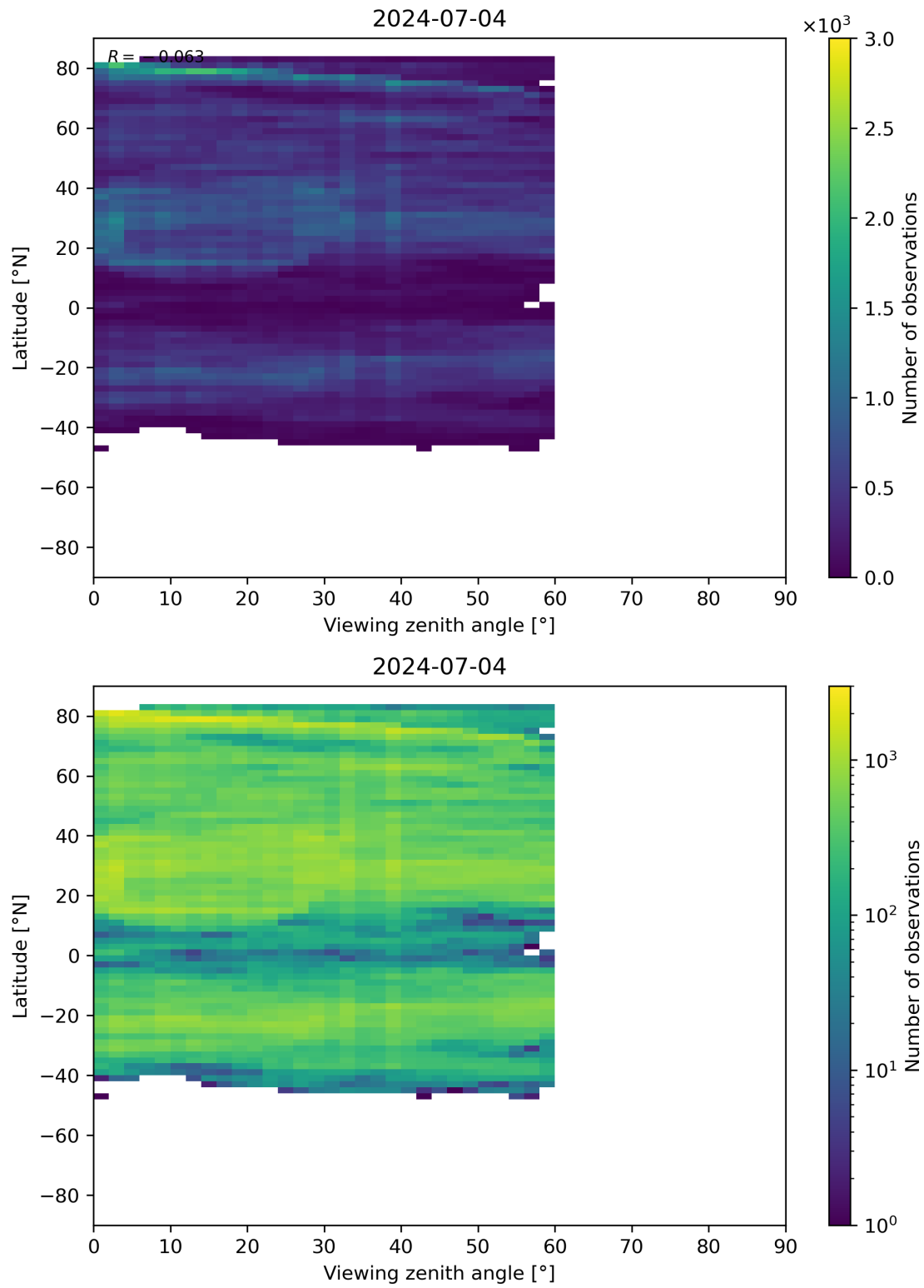
Figure 109: Scatter density plot of “Viewing zenith angle” against “Latitude” for 2024-07-03 to 2024-07-05.
