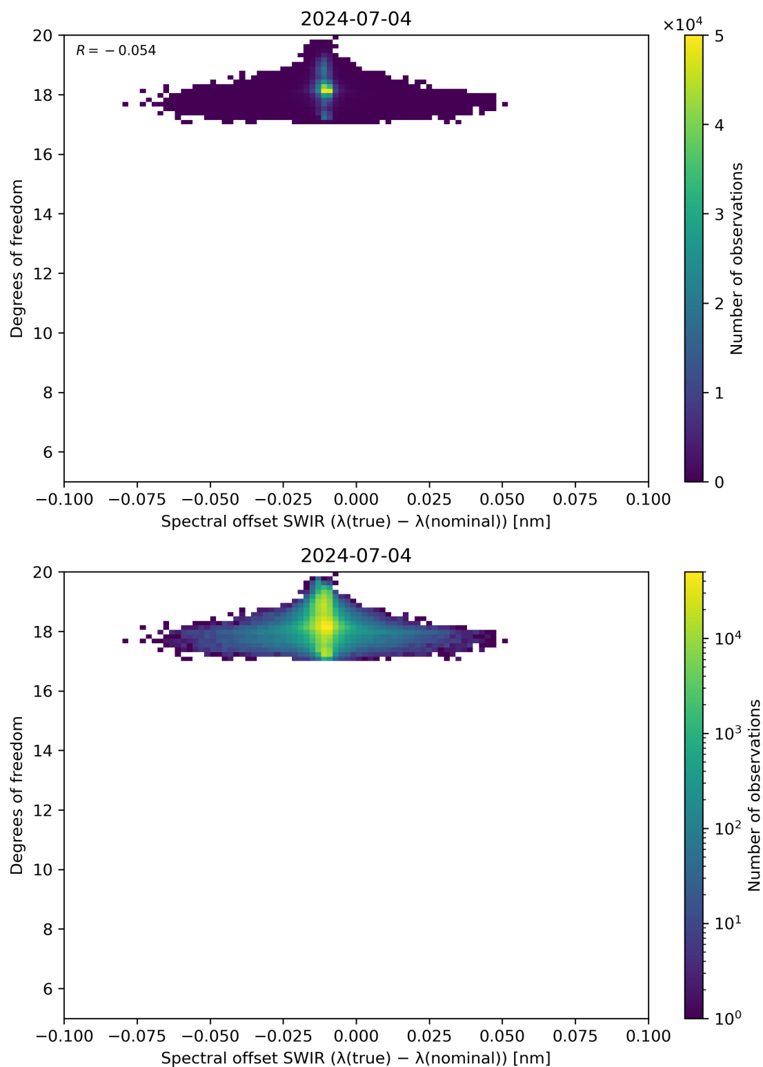
Figure 119: Scatter density plot of “Spectral offset SWIR ( \lambda(\text{true}) - \lambda(\text{nominal}) )” against “Degrees of freedom” for 2024-07-03 to 2024-07-05.
