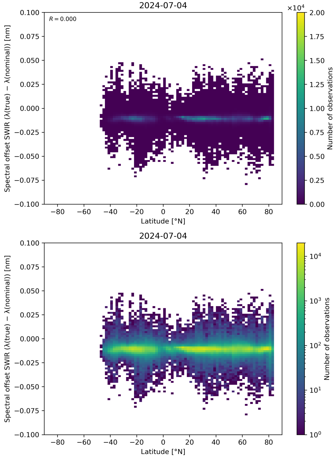
Figure 62: Scatter density plot of “Latitude” against “Spectral offset SWIR ( \lambda(\text{true}) - \lambda(\text{nominal}) )” for 2024-07-03 to 2024-07-05.
