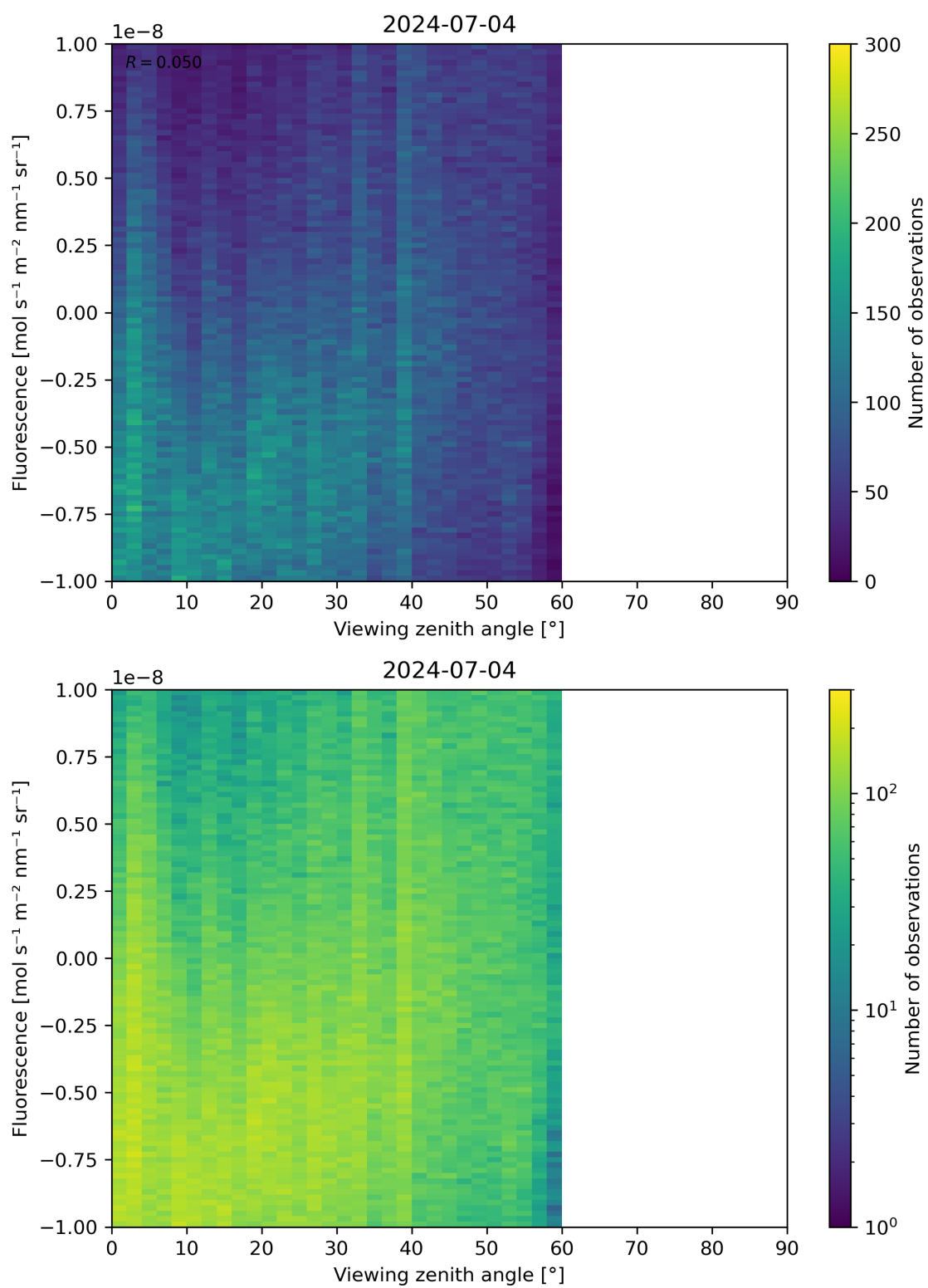
Figure 108: Scatter density plot of “Viewing zenith angle” against “Fluorescence” for 2024-07-03 to 2024-07-05.
