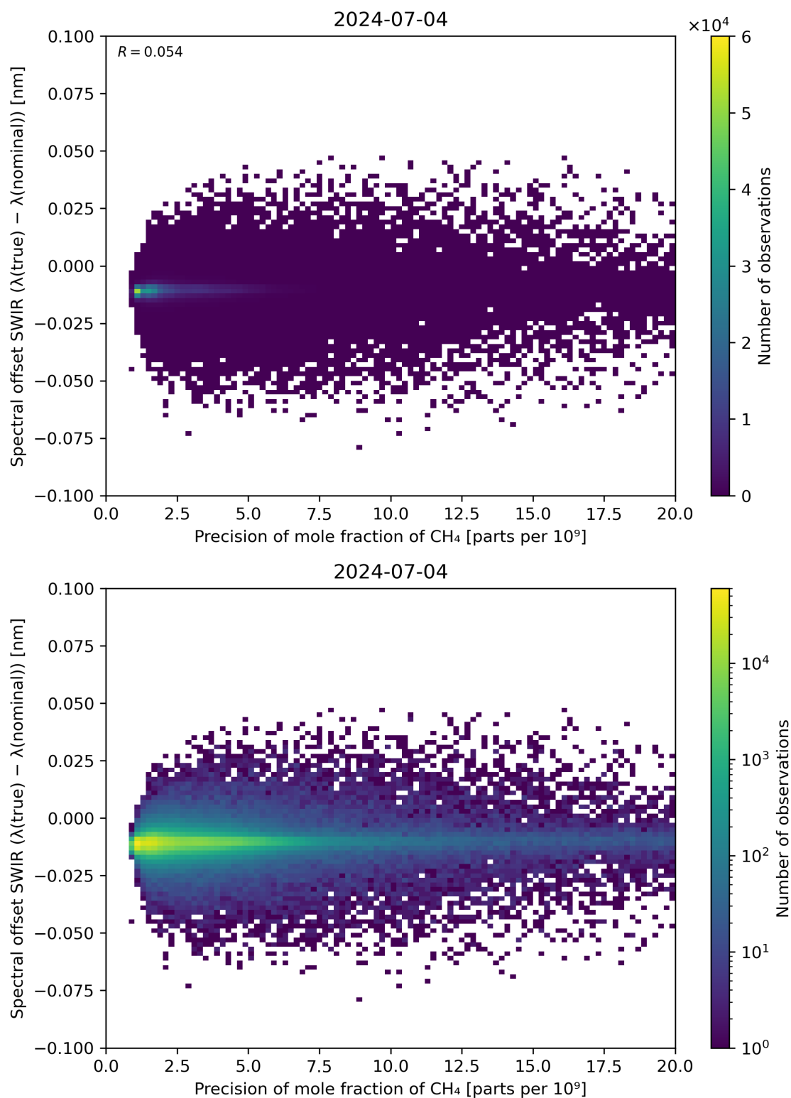
Figure 85: Scatter density plot of “Precision of mole fraction of \text{CH}_4 ” against “Spectral offset SWIR ( \lambda(\text{true}) - \lambda(\text{nominal}) )” for 2024-07-03 to 2024-07-05.
