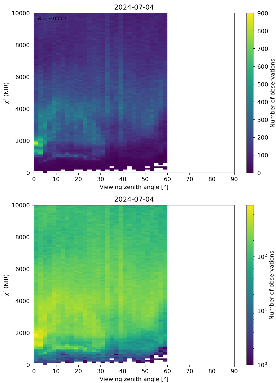
Figure 105: Scatter density plot of “Viewing zenith angle” against “ \chi^2 (NIR)” for 2024-07-03 to 2024-07-05.
