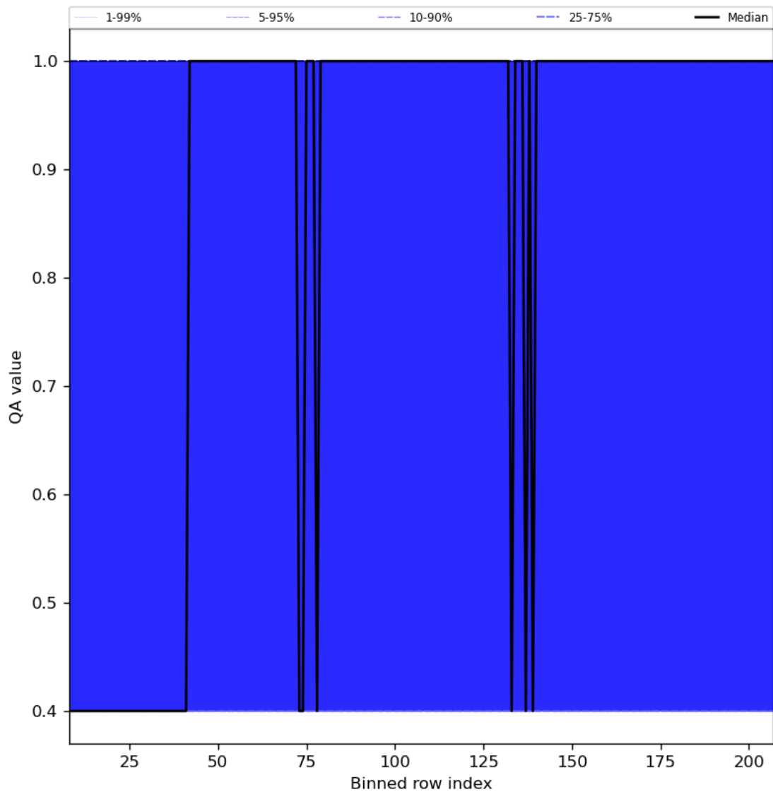
Figure 33: Along track statistics of “QA value” for 2024-07-03 to 2024-07-05
