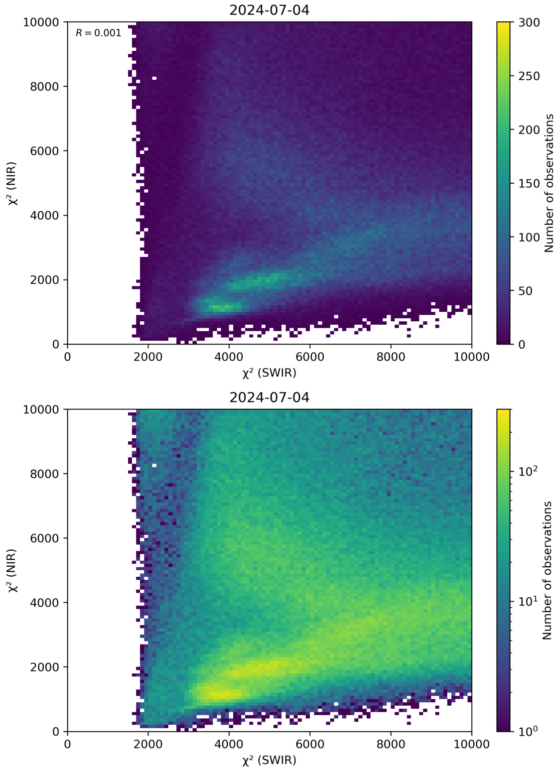
Figure 47: Scatter density plot of “ \chi^2 (SWIR)” against “ \chi^2 (NIR)” for 2024-07-03 to 2024-07-05.
