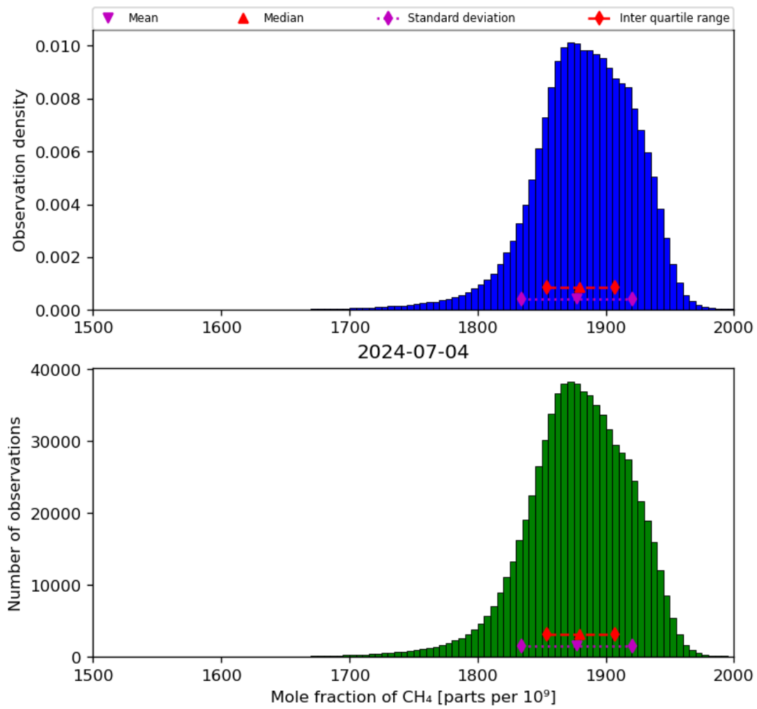
Figure 23: Histogram of “Mole fraction of CH 4 ” for 2024-07-03 to 2024-07-05
