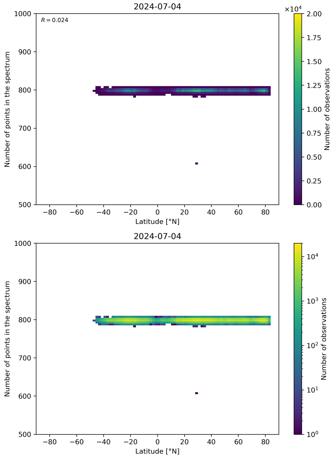
Figure 61: Scatter density plot of “Latitude” against “Number of points in the spectrum” for 2024-07-03 to 2024-07-05.
