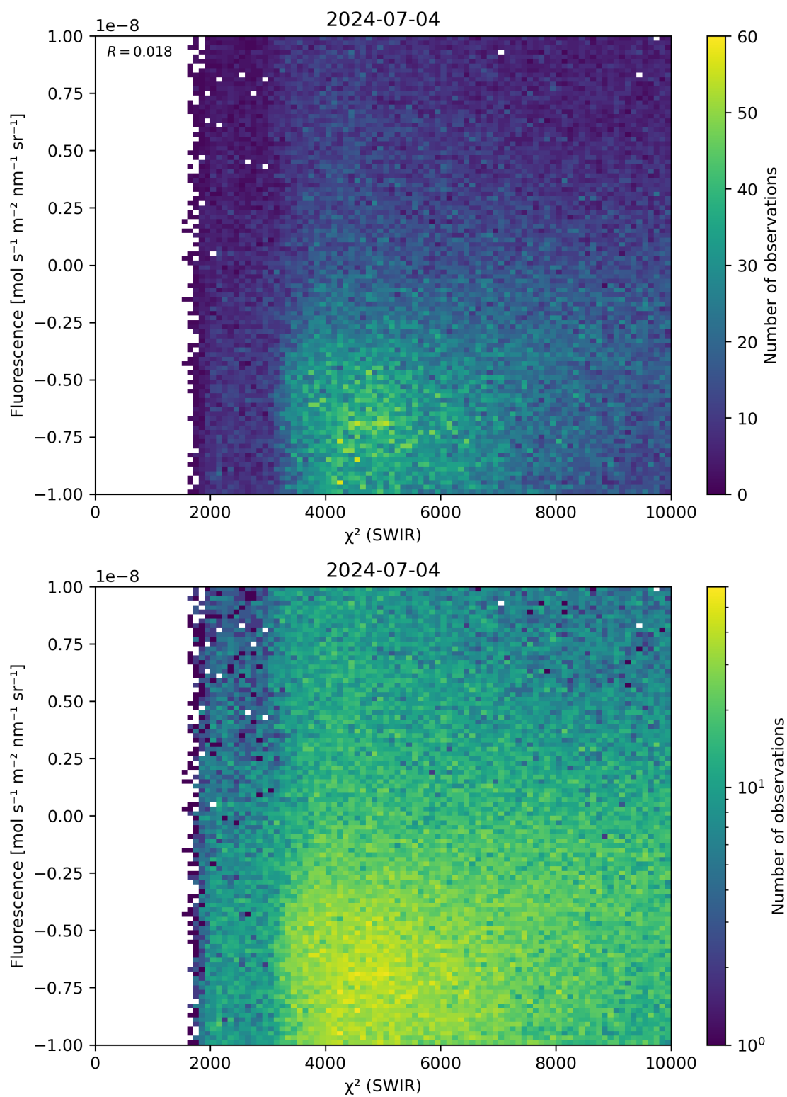
Figure 49: Scatter density plot of “ \chi^2 (SWIR)” against “Fluorescence” for 2024-07-03 to 2024-07-05.
