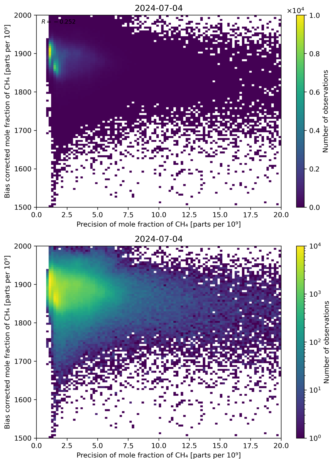
Figure 82: Scatter density plot of “Precision of mole fraction of \text{CH}_4 ” against “Bias corrected mole fraction of \text{CH}_4 ” for 2024-07-03 to 2024-07-05.
