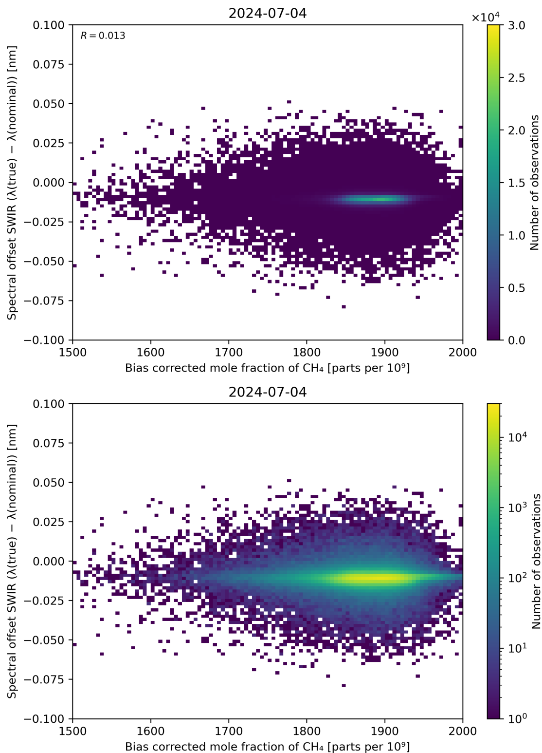
Figure 69: Scatter density plot of “Bias corrected mole fraction of \text{CH}_4 ” against “Spectral offset SWIR ( \lambda(\text{true}) - \lambda(\text{nominal}) )” for 2024-07-03 to 2024-07-05.
