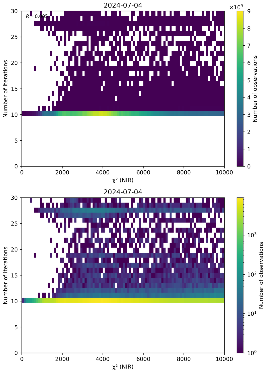
Figure 46: Scatter density plot of “ \chi^2 (NIR)” against “Number of iterations” for 2024-07-03 to 2024-07-05.
