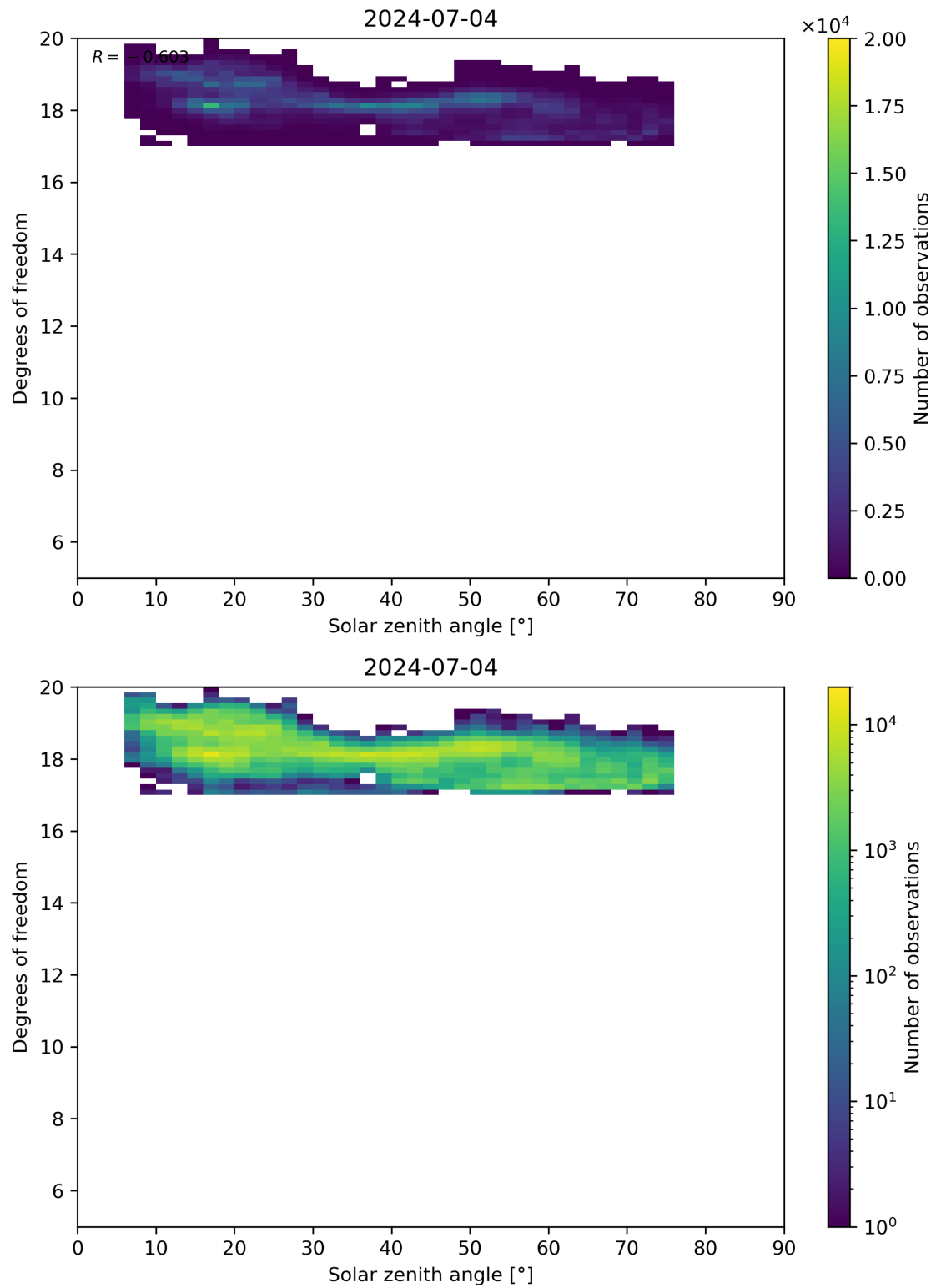
Figure 96: Scatter density plot of “Solar zenith angle” against “Degrees of freedom” for 2024-07-03 to 2024-07-05.
