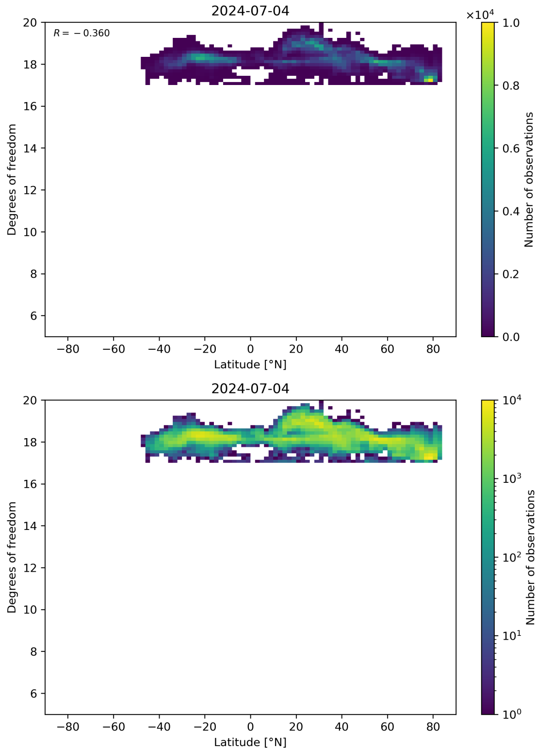
Figure 55: Scatter density plot of “Latitude” against “Degrees of freedom” for 2024-07-03 to 2024-07-05.
