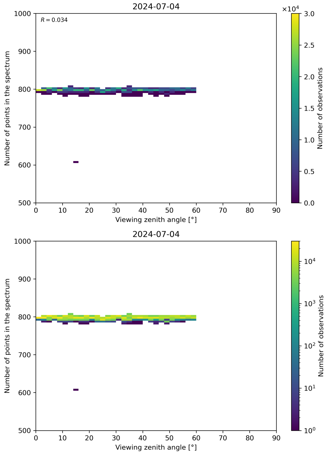
Figure 114: Scatter density plot of “Viewing zenith angle” against “Number of points in the spectrum” for 2024-07-03 to 2024-07-05.
