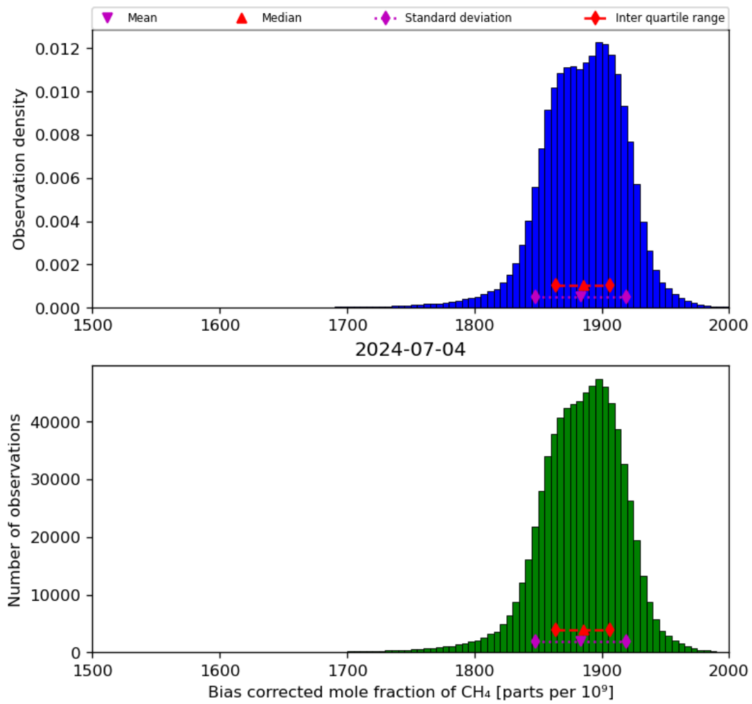
Figure 25: Histogram of “Bias corrected mole fraction of CH 4 ” for 2024-07-03 to 2024-07-05
