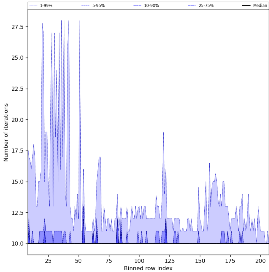
Figure 42: Along track statistics of “Number of iterations” for 2024-07-03 to 2024-07-05
