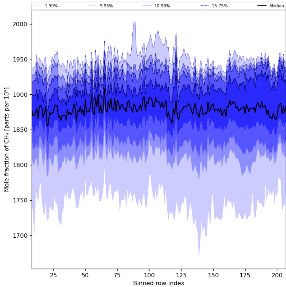
Figure 34: Along track statistics of “Mole fraction of CH 4 ” for 2024-07-03 to 2024-07-05
