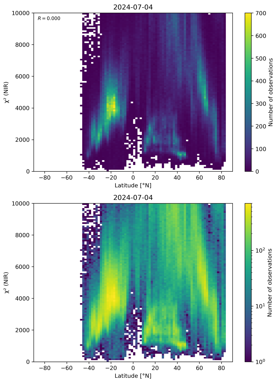
Figure 53: Scatter density plot of “Latitude” against “ \chi^2 (NIR)” for 2024-07-03 to 2024-07-05.
