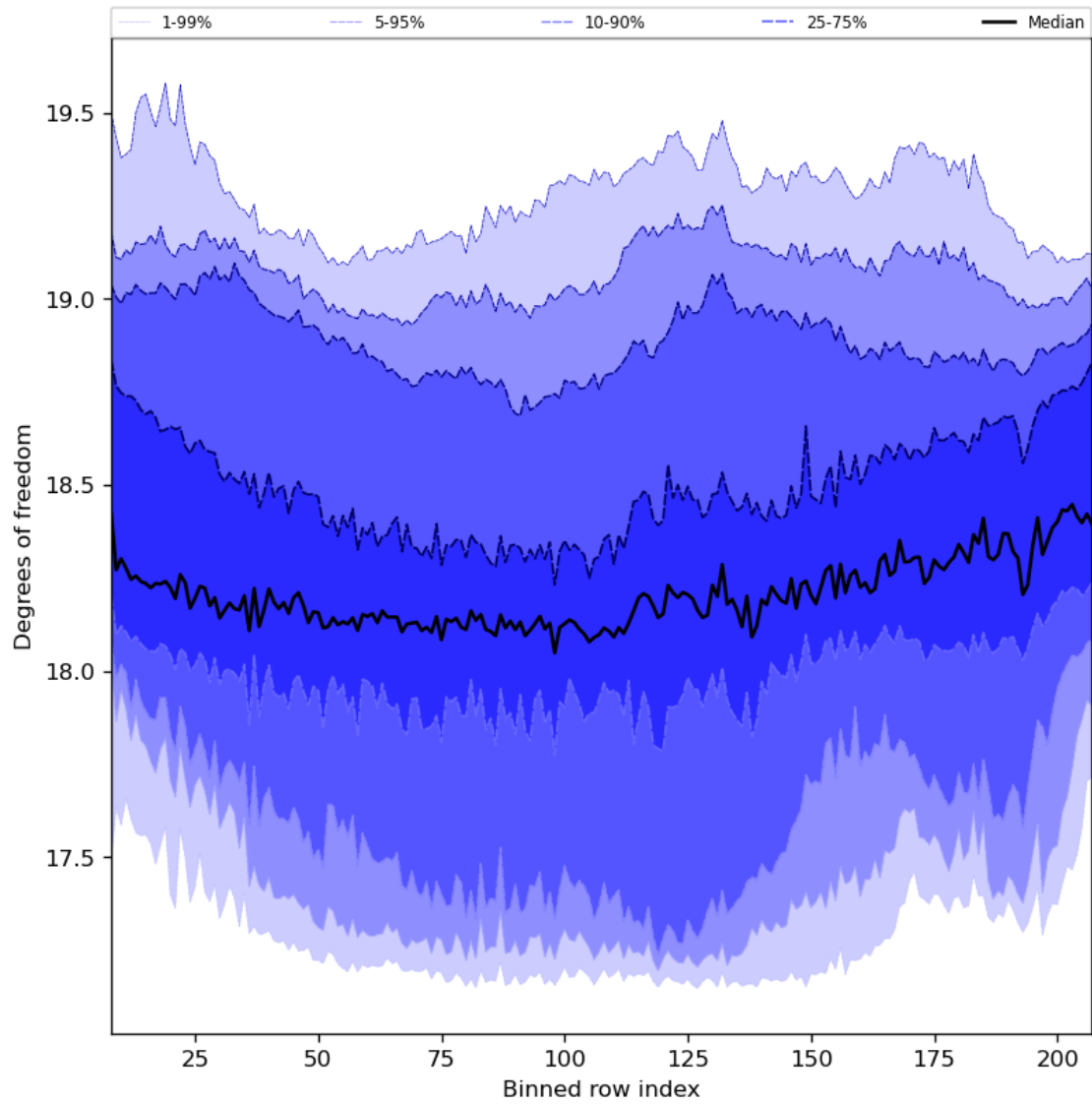
Figure 41: Along track statistics of “Degrees of freedom” for 2024-07-03 to 2024-07-05
