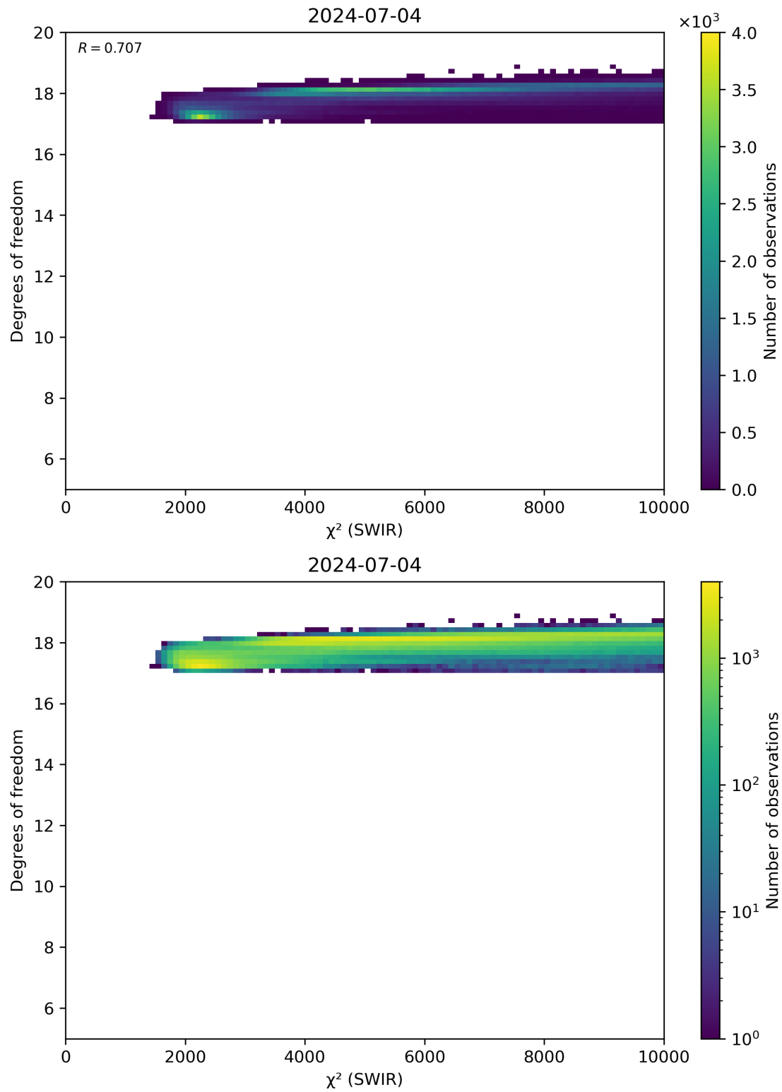
Figure 48: Scatter density plot of “ \chi^2 (SWIR)” against “Degrees of freedom” for 2024-07-03 to 2024-07-05.
