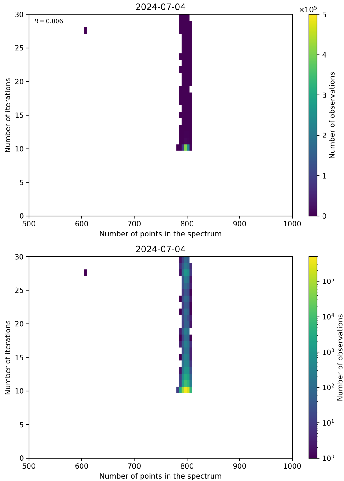
Figure 92: Scatter density plot of “Number of points in the spectrum” against “Number of iterations” for 2024-07-03 to 2024-07-05.
