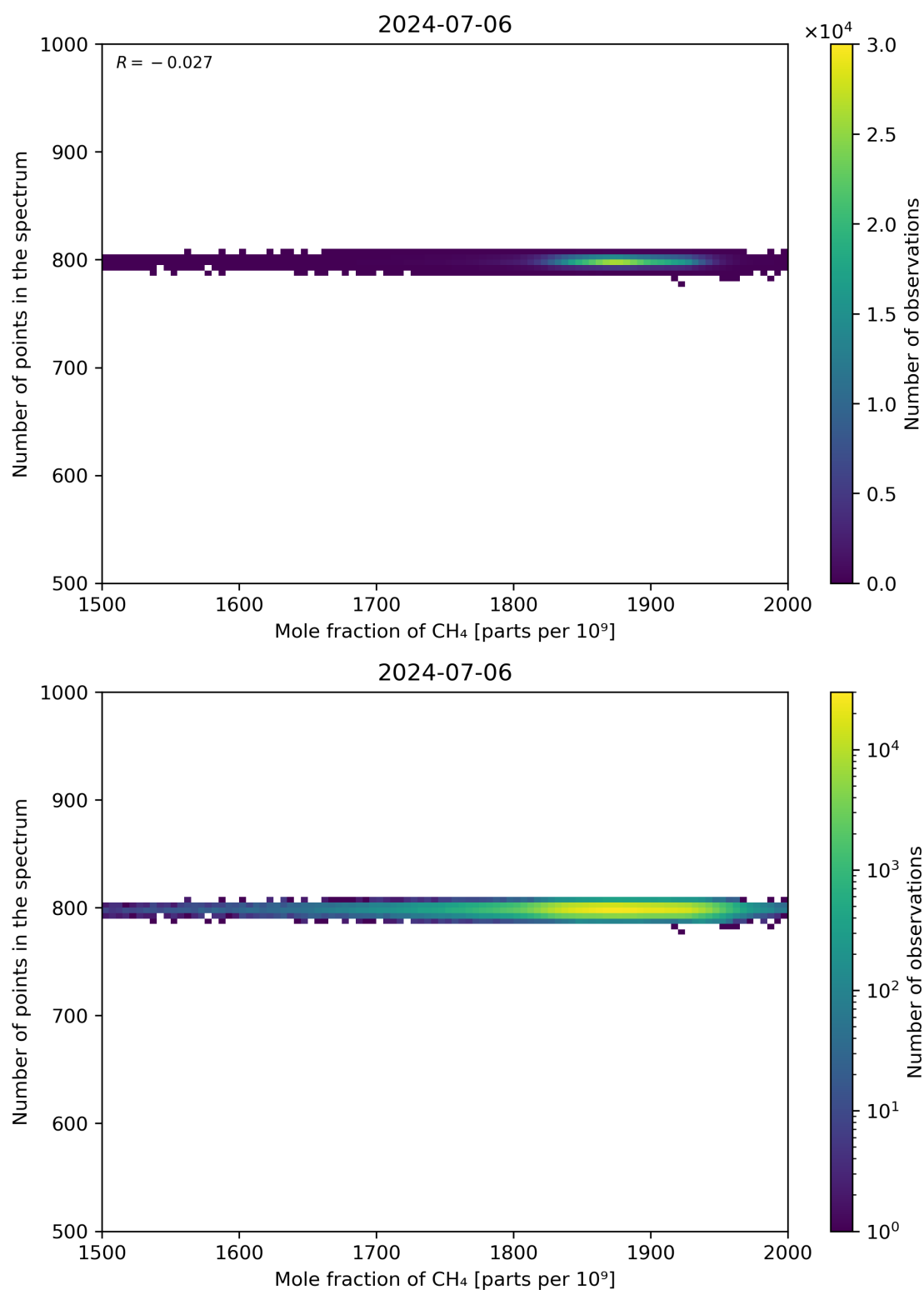
Figure 77: Scatter density plot of “Mole fraction of CH 4 ” against “Number of points in the spectrum” for 2024-07-05 to 2024-07-07.
