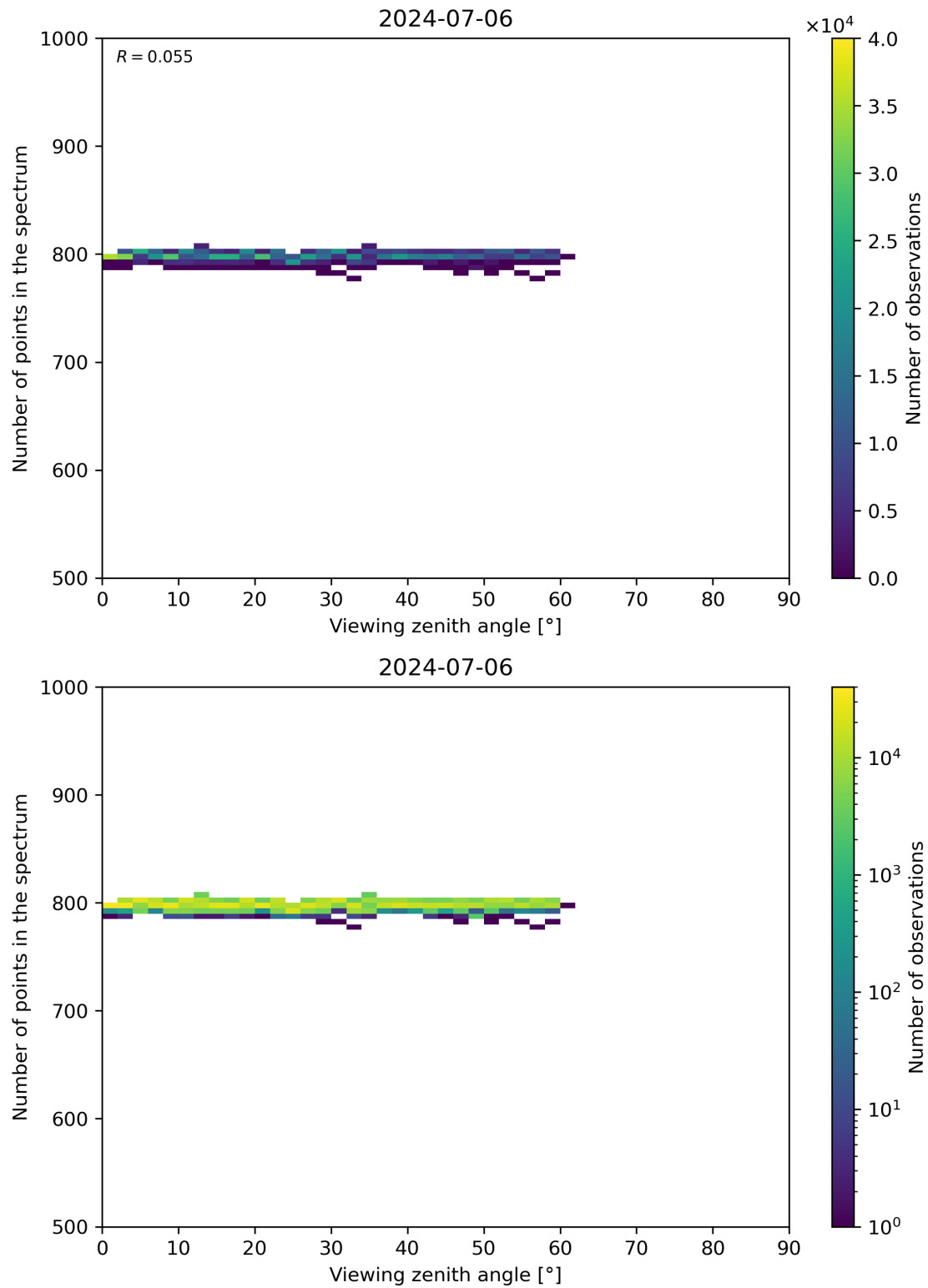
Figure 114: Scatter density plot of “Viewing zenith angle” against “Number of points in the spectrum” for 2024-07-05 to 2024-07-07.
