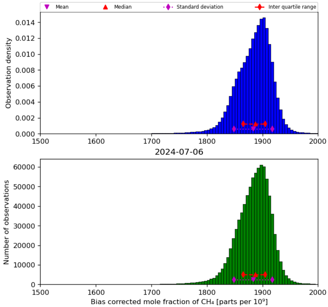
Figure 25: Histogram of “Bias corrected mole fraction of CH 4 ” for 2024-07-05 to 2024-07-07
