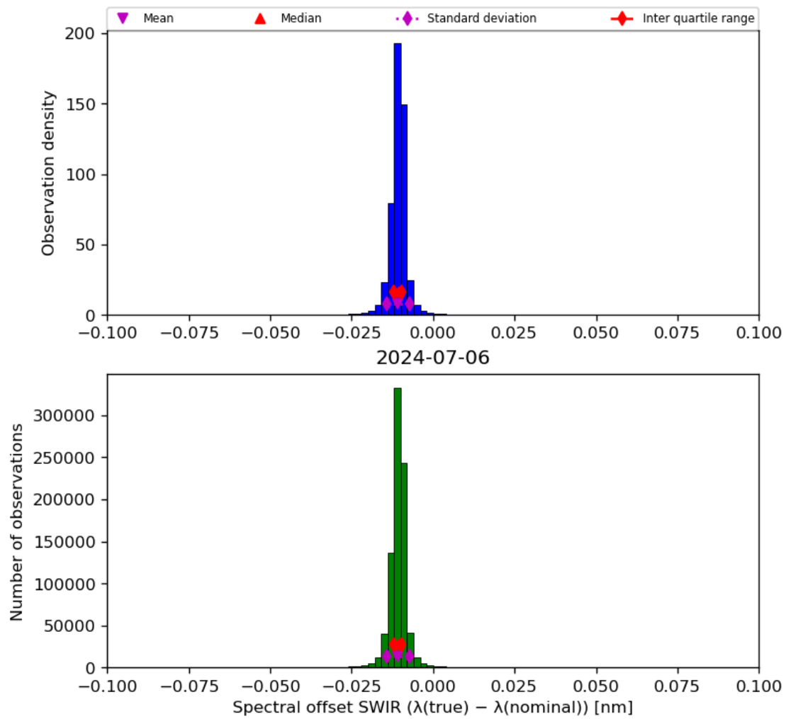
Figure 27: Histogram of “Spectral offset SWIR ( \lambda(\text{true}) - \lambda(\text{nominal}) )” for 2024-07-05 to 2024-07-07
