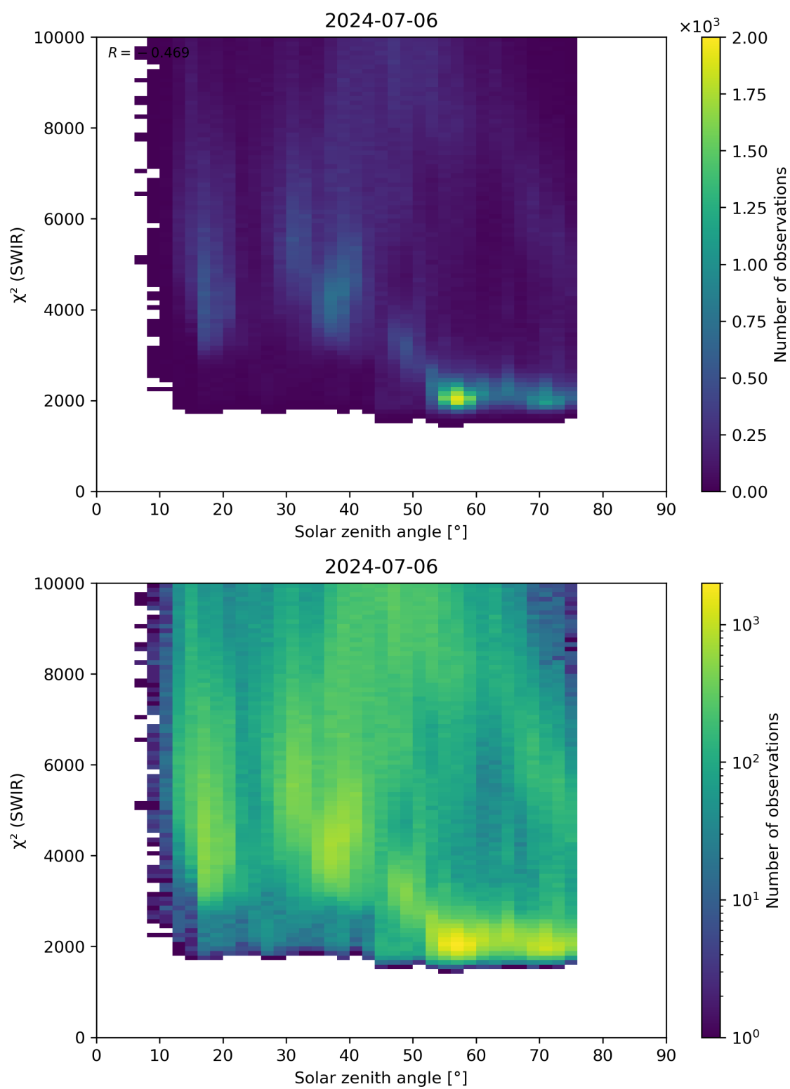
Figure 95: Scatter density plot of “Solar zenith angle” against “ \chi^2 (SWIR)” for 2024-07-05 to 2024-07-07.
