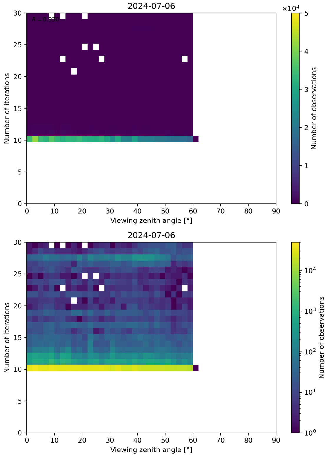
Figure 113: Scatter density plot of “Viewing zenith angle” against “Number of iterations” for 2024-07-05 to 2024-07-07.
