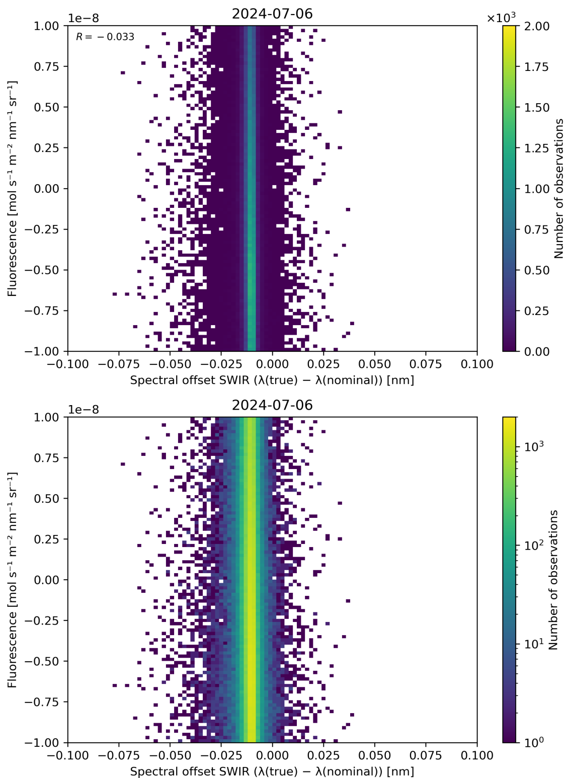
Figure 120: Scatter density plot of “Spectral offset SWIR ( \lambda(\text{true}) - \lambda(\text{nominal}) )” against “Fluorescence” for 2024-07-05 to 2024-07-07.
