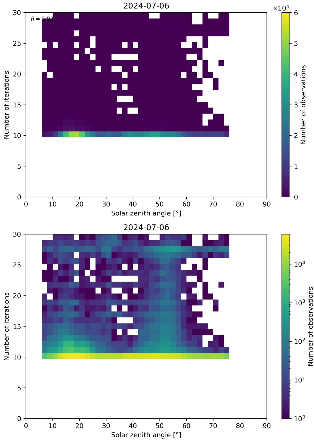
Figure 102: Scatter density plot of “Solar zenith angle” against “Number of iterations” for 2024-07-05 to 2024-07-07.
