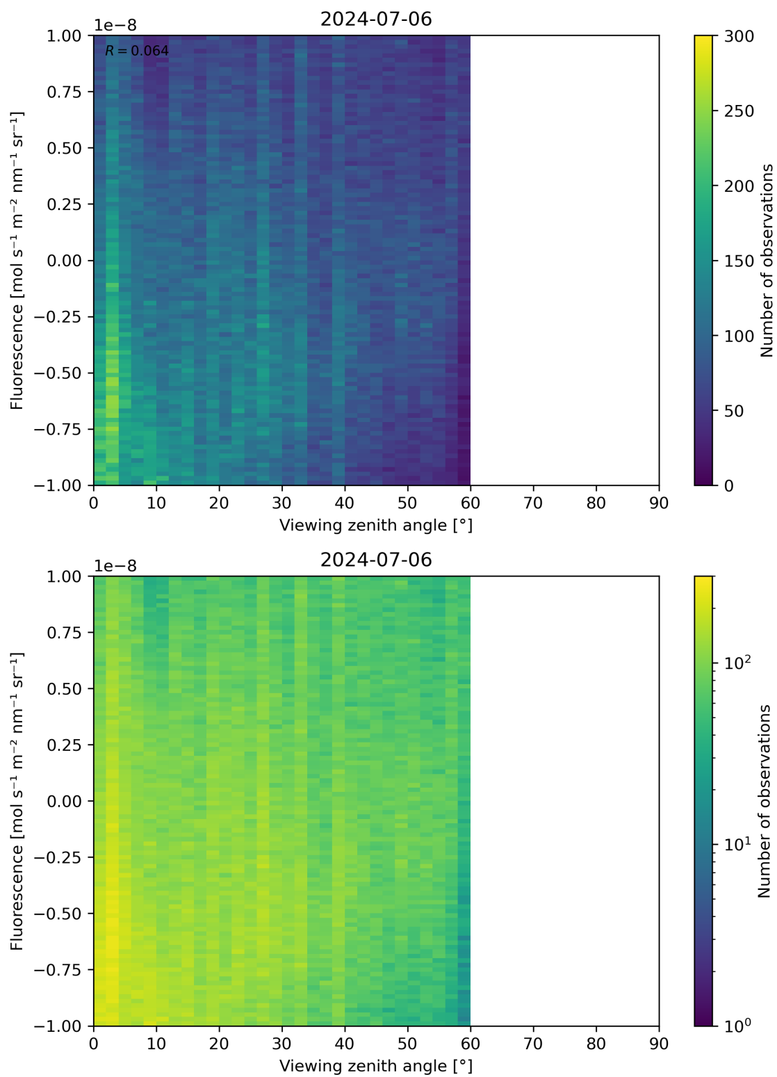
Figure 108: Scatter density plot of “Viewing zenith angle” against “Fluorescence” for 2024-07-05 to 2024-07-07.
