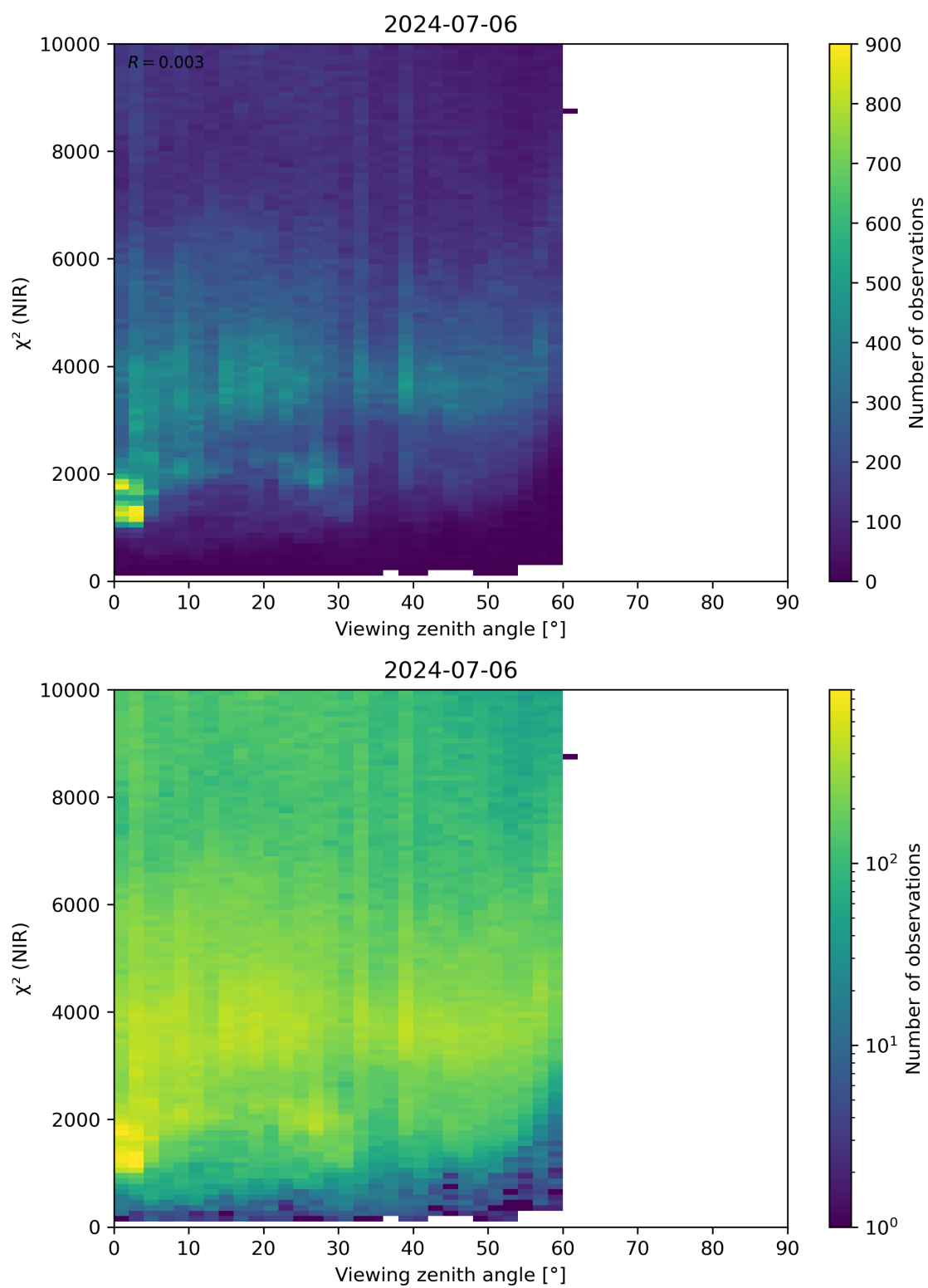
Figure 105: Scatter density plot of “Viewing zenith angle” against “ \chi^2 (NIR)” for 2024-07-05 to 2024-07-07.
