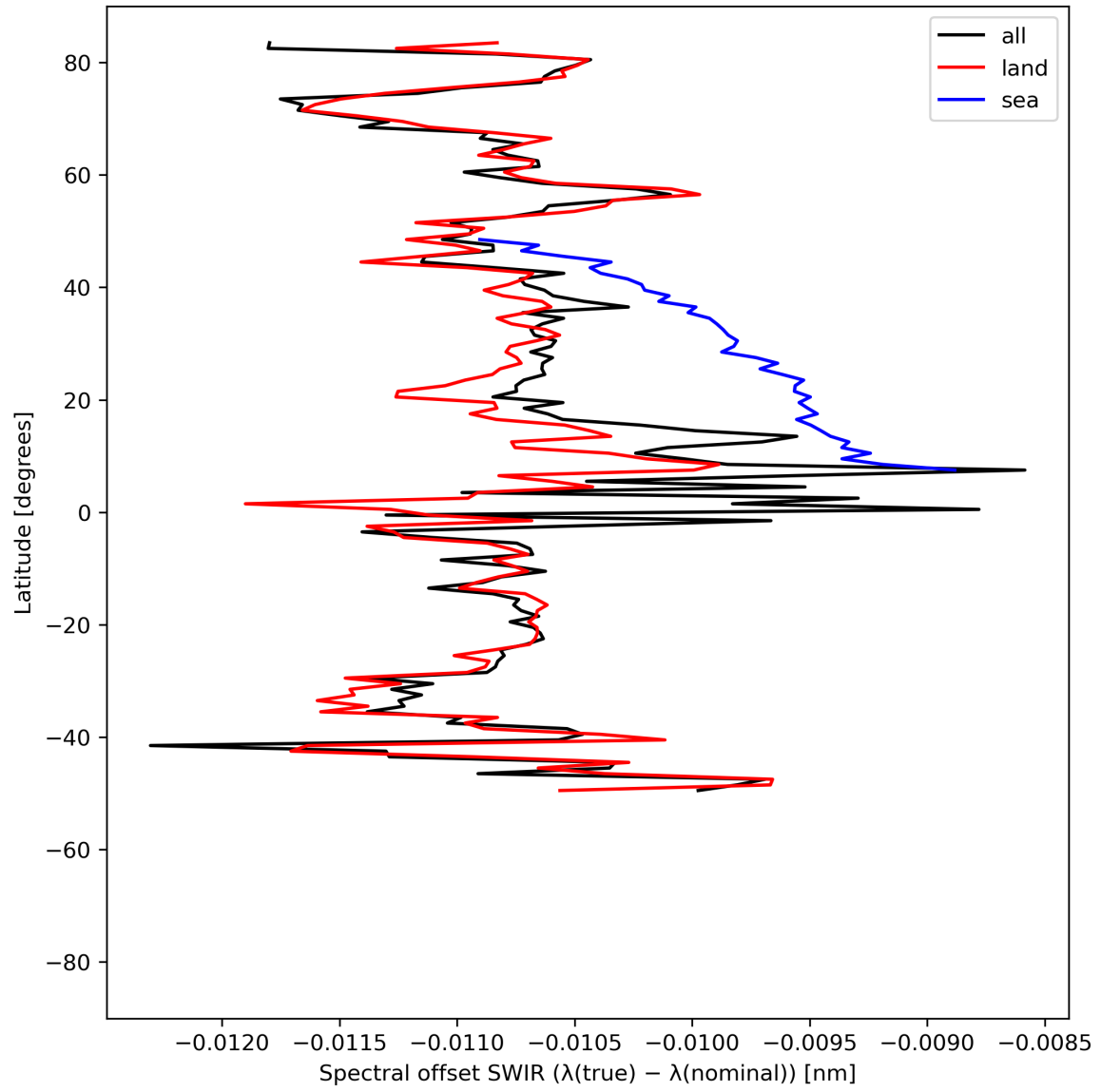
Figure 16: Zonal average of “Spectral offset SWIR ( \lambda(\text{true}) - \lambda(\text{nominal}) )” for 2024-07-05 to 2024-07-07.
