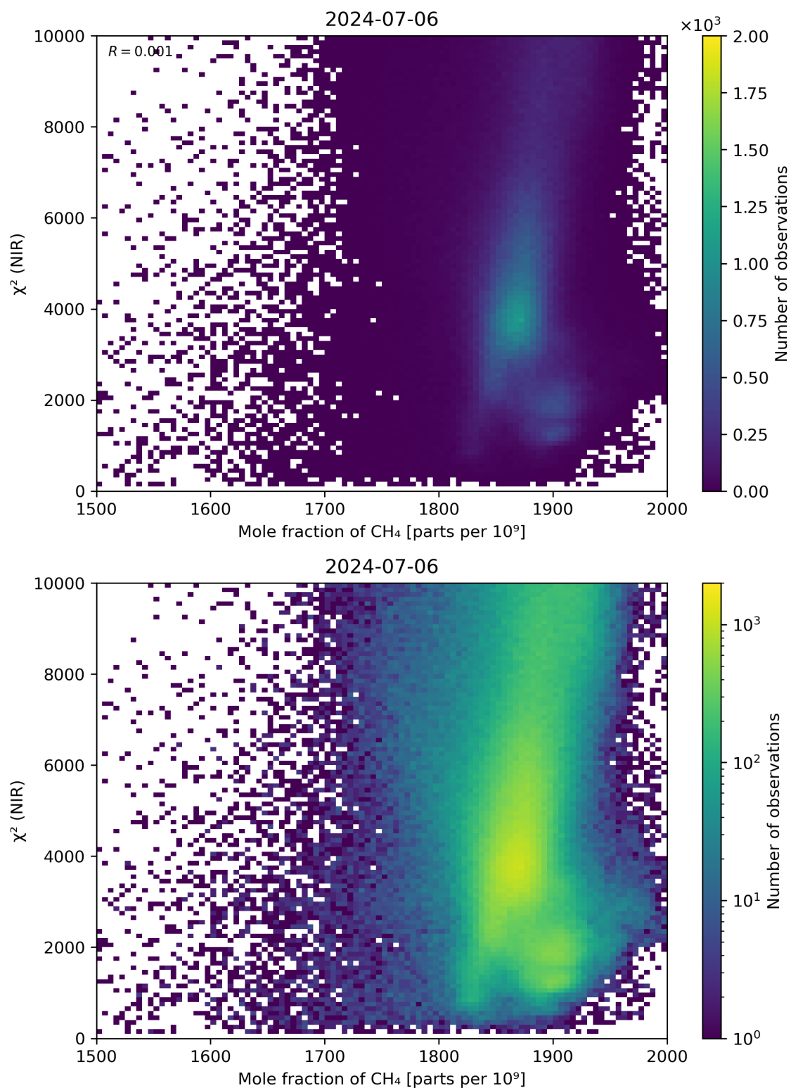
Figure 70: Scatter density plot of “Mole fraction of CH 4 ” against “ \chi^2 (NIR)” for 2024-07-05 to 2024-07-07.
