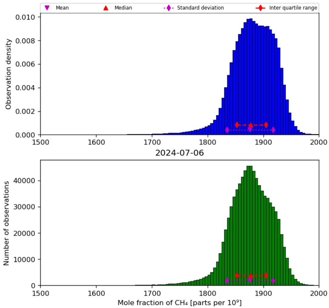
Figure 23: Histogram of “Mole fraction of CH 4 ” for 2024-07-05 to 2024-07-07
