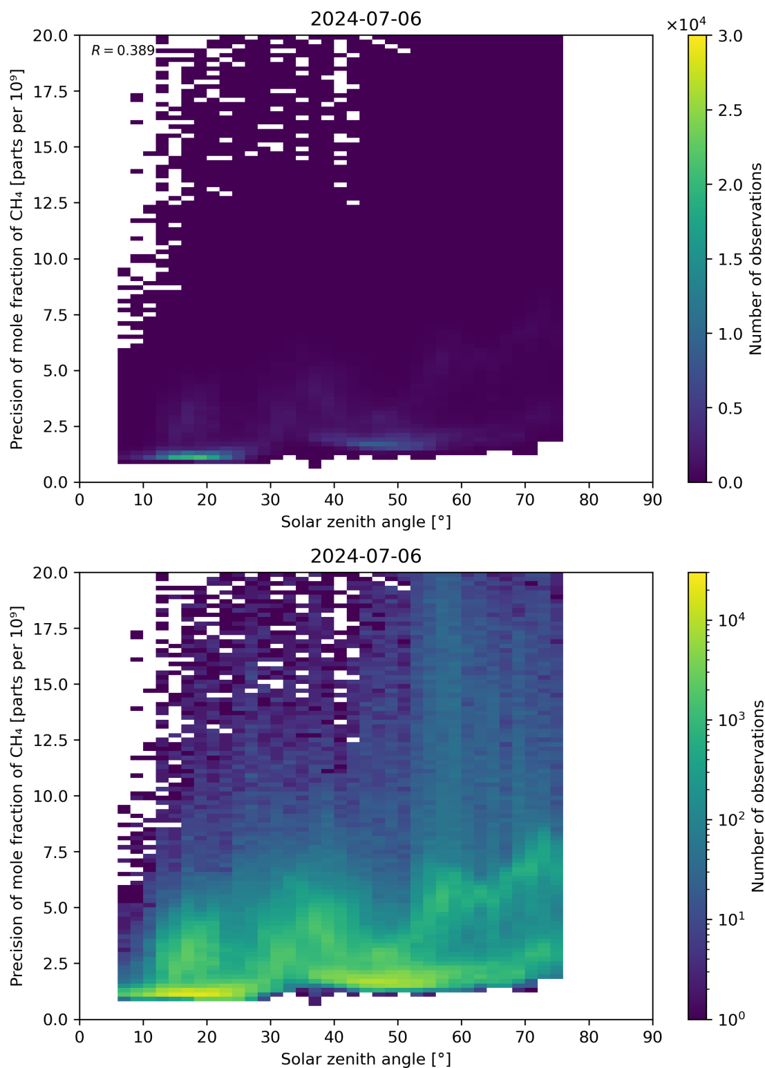
Figure 101: Scatter density plot of “Solar zenith angle” against “Precision of mole fraction of CH 4 ” for 2024-07-05 to 2024-07-07.
