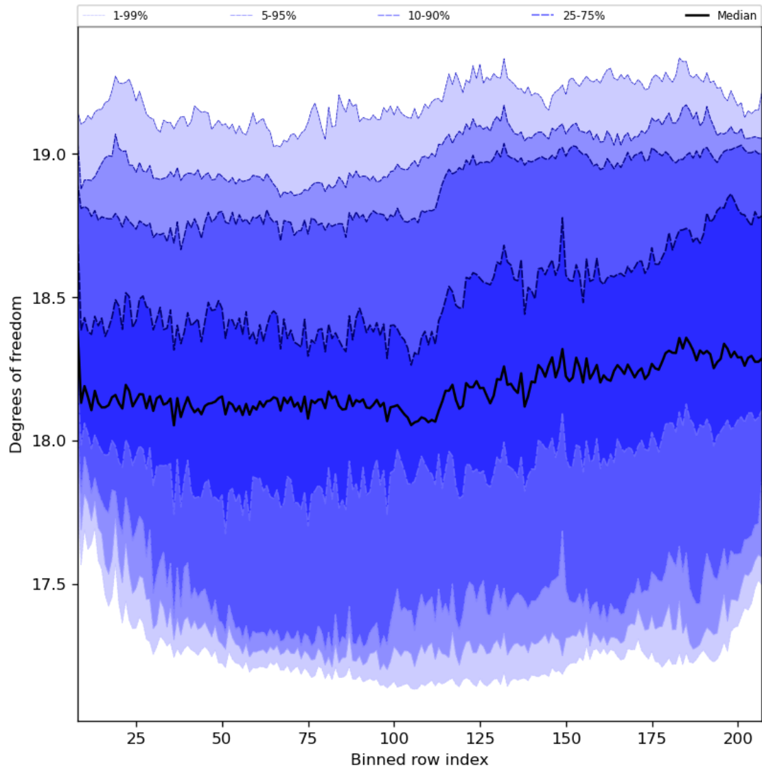
Figure 41: Along track statistics of “Degrees of freedom” for 2024-07-05 to 2024-07-07
