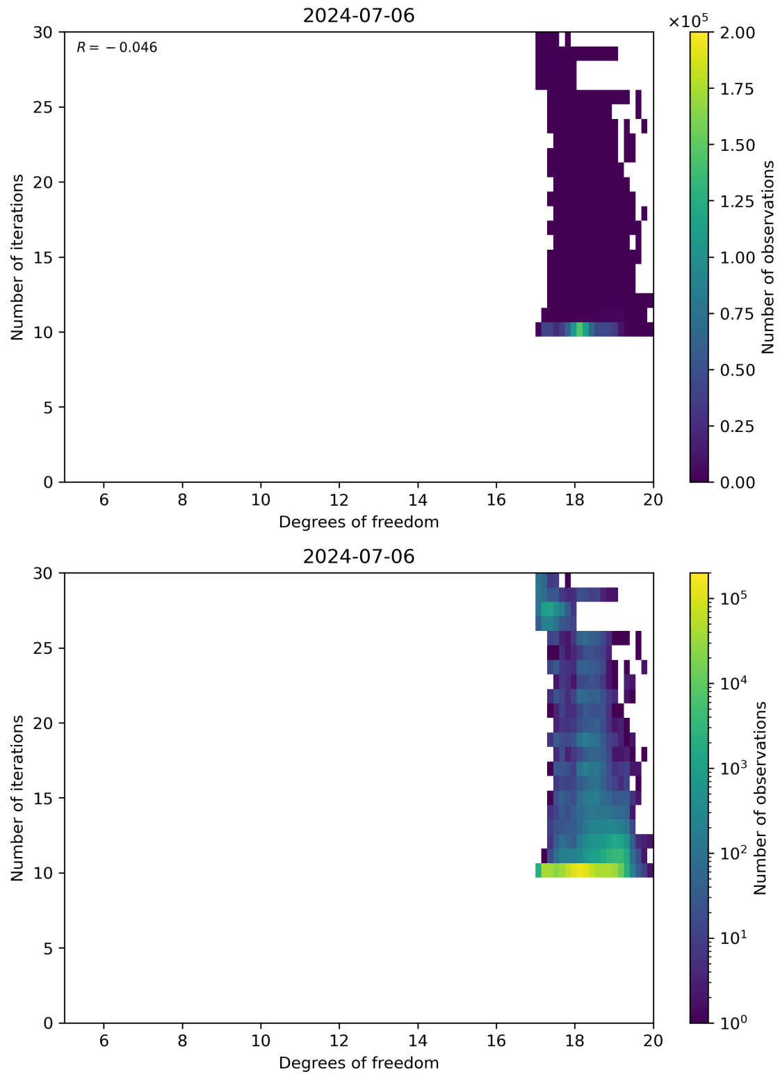
Figure 52: Scatter density plot of “Degrees of freedom” against “Number of iterations” for 2024-07-05 to 2024-07-07.
