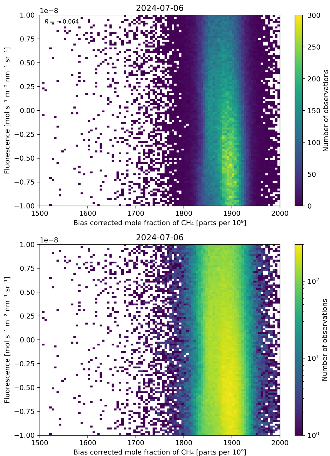
Figure 66: Scatter density plot of “Bias corrected mole fraction of \text{CH}_4 ” against “Fluorescence” for 2024-07-05 to 2024-07-07.
