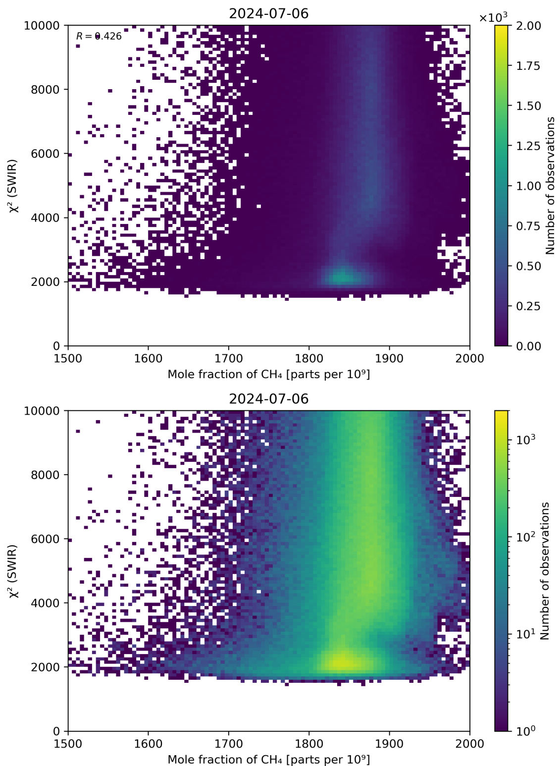
Figure 71: Scatter density plot of “Mole fraction of \text{CH}_4 ” against “ \chi^2 (SWIR)” for 2024-07-05 to 2024-07-07.
