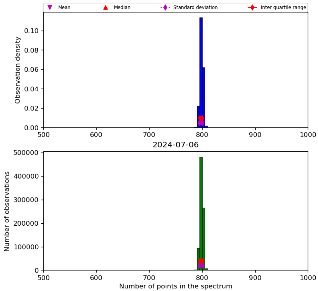
Figure 26: Histogram of “Number of points in the spectrum” for 2024-07-05 to 2024-07-07
