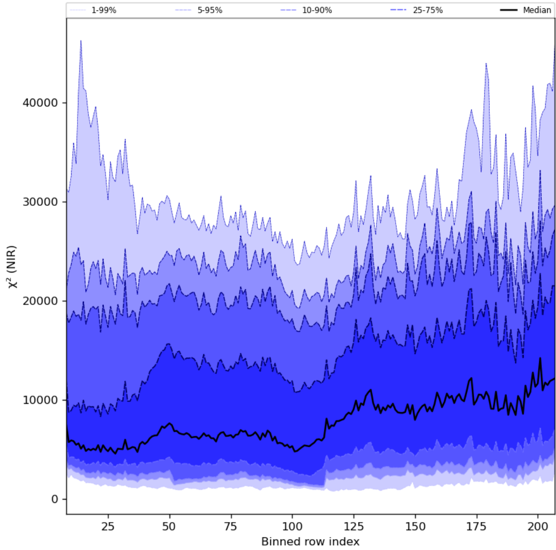
Figure 40: Along track statistics of " \chi^2 (NIR)" for 2024-07-05 to 2024-07-07
