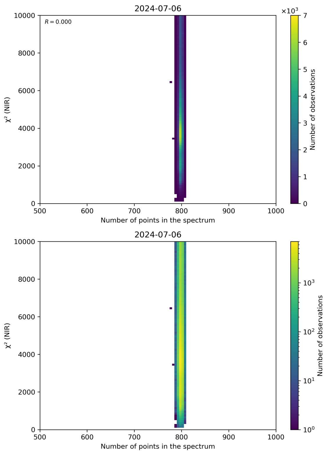
Figure 88: Scatter density plot of “Number of points in the spectrum” against “ \chi^2 (NIR)” for 2024-07-05 to 2024-07-07.
