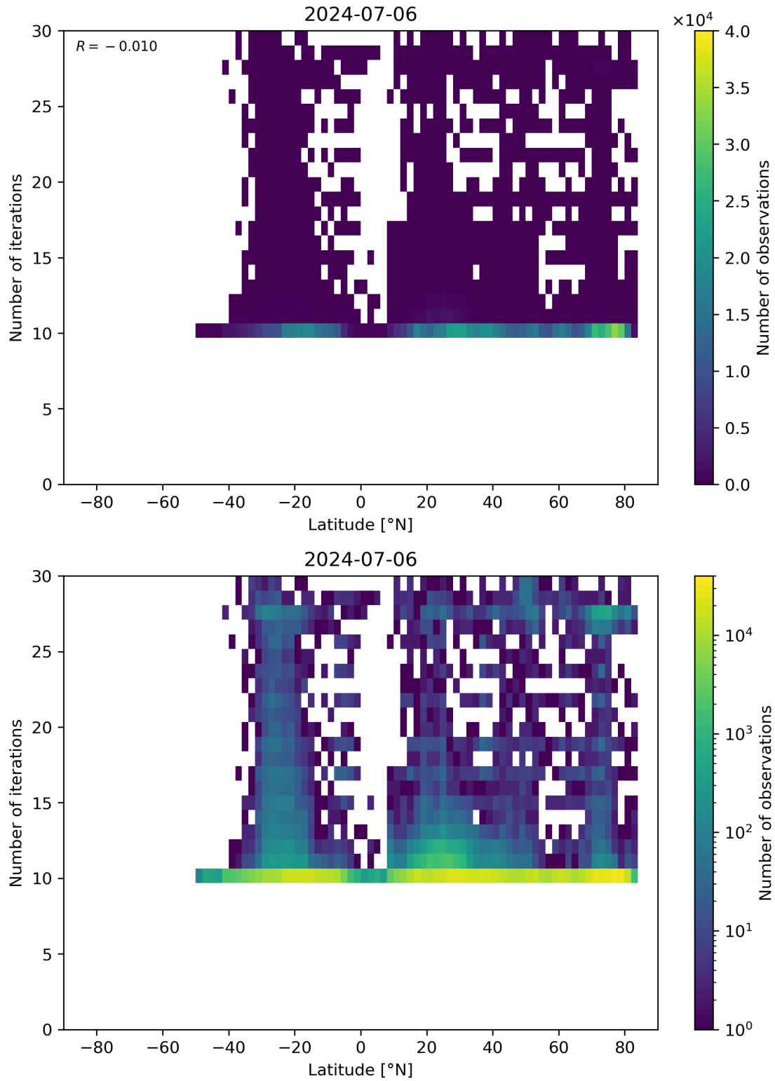
Figure 60: Scatter density plot of “Latitude” against “Number of iterations” for 2024-07-05 to 2024-07-07.
