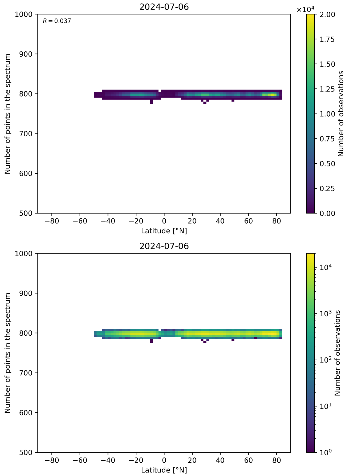
Figure 61: Scatter density plot of “Latitude” against “Number of points in the spectrum” for 2024-07-05 to 2024-07-07.
