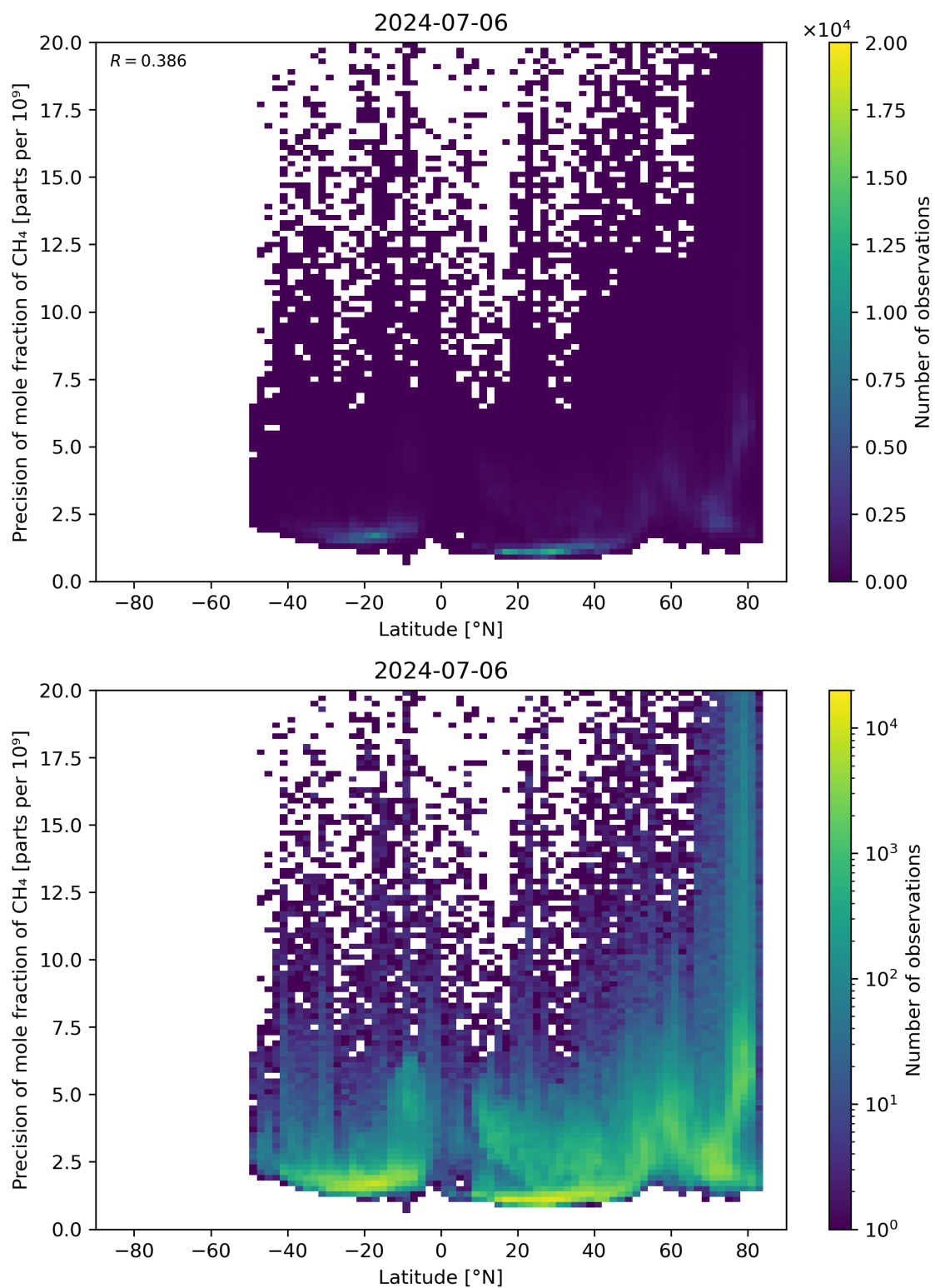
Figure 59: Scatter density plot of “Latitude” against “Precision of mole fraction of CH 4 ” for 2024-07-05 to 2024-07-07.
