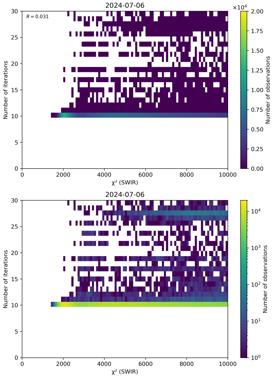
Figure 50: Scatter density plot of “ \chi^2 (SWIR)” against “Number of iterations” for 2024-07-05 to 2024-07-07.
