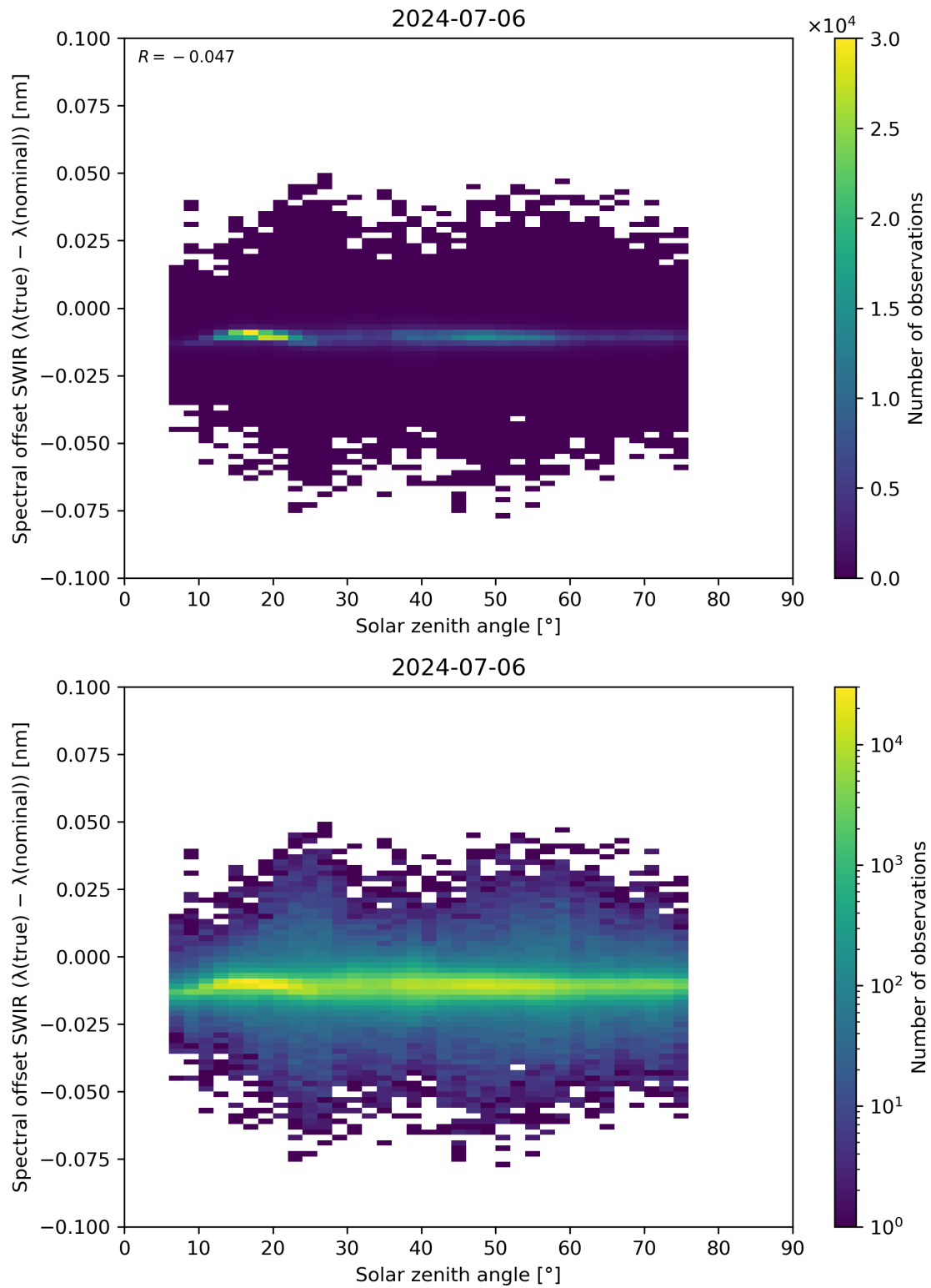
Figure 104: Scatter density plot of “Solar zenith angle” against “Spectral offset SWIR ( \lambda(\text{true}) - \lambda(\text{nominal}) )” for 2024-07-05 to 2024-07-07.
