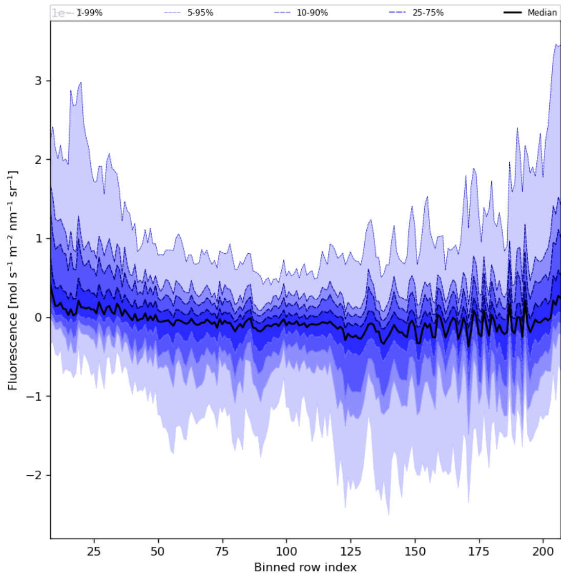
Figure 43: Along track statistics of “Fluorescence” for 2024-07-05 to 2024-07-07
