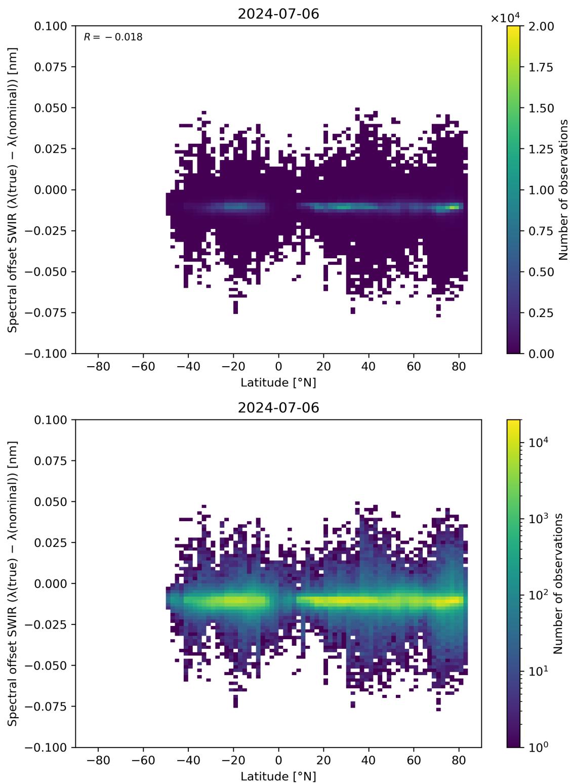
Figure 62: Scatter density plot of “Latitude” against “Spectral offset SWIR ( \lambda(\text{true}) - \lambda(\text{nominal}) )” for 2024-07-05 to 2024-07-07.
