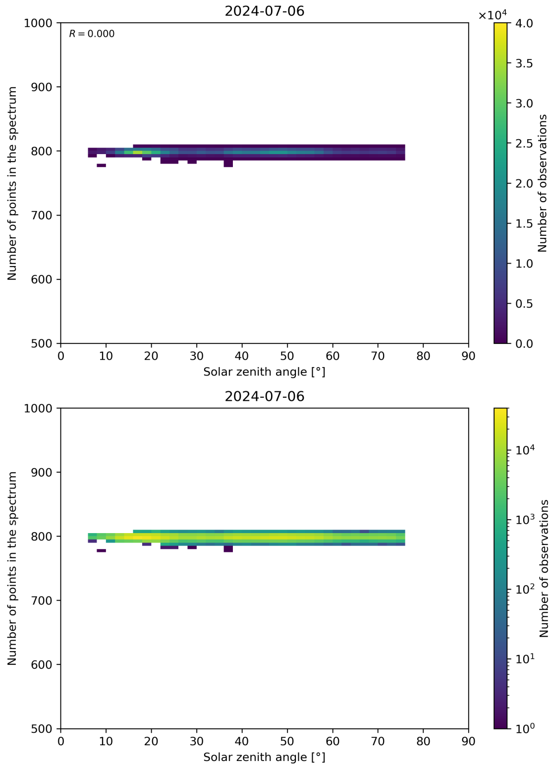
Figure 103: Scatter density plot of “Solar zenith angle” against “Number of points in the spectrum” for 2024-07-05 to 2024-07-07.
