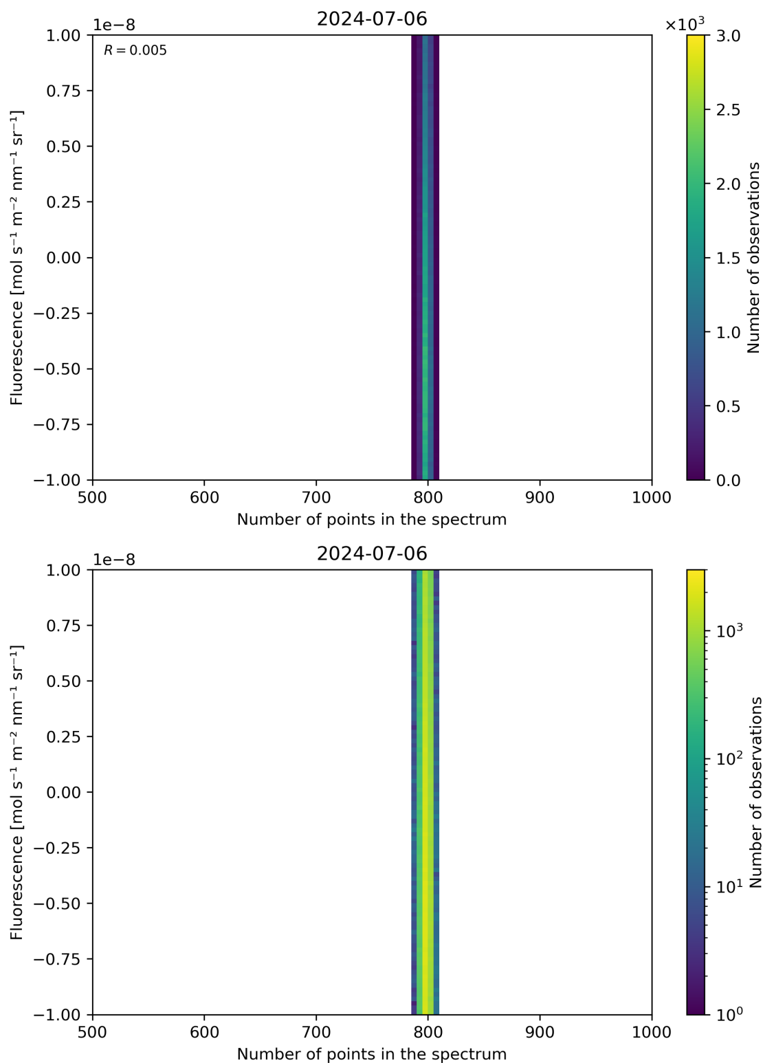
Figure 91: Scatter density plot of “Number of points in the spectrum” against “Fluorescence” for 2024-07-05 to 2024-07-07.
