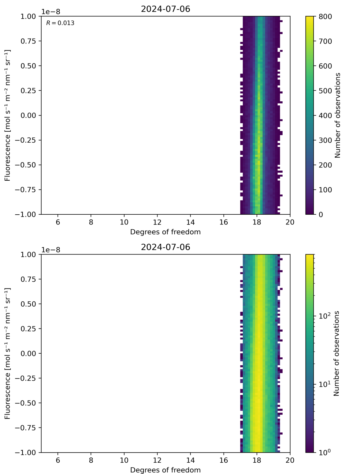
Figure 51: Scatter density plot of “Degrees of freedom” against “Fluorescence” for 2024-07-05 to 2024-07-07.
