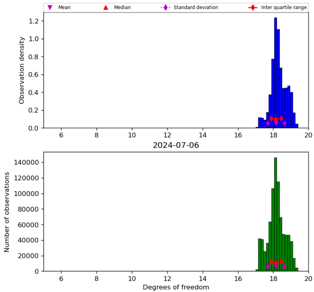
Figure 30: Histogram of “Degrees of freedom” for 2024-07-05 to 2024-07-07
