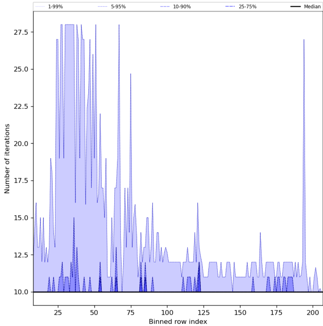
Figure 42: Along track statistics of “Number of iterations” for 2024-07-05 to 2024-07-07
