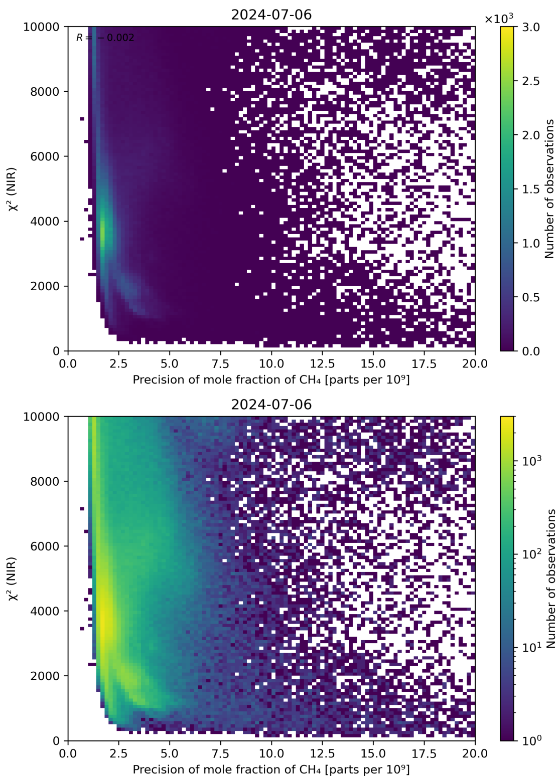
Figure 78: Scatter density plot of “Precision of mole fraction of CH 4 ” against “ \chi^2 (NIR)” for 2024-07-05 to 2024-07-07.
