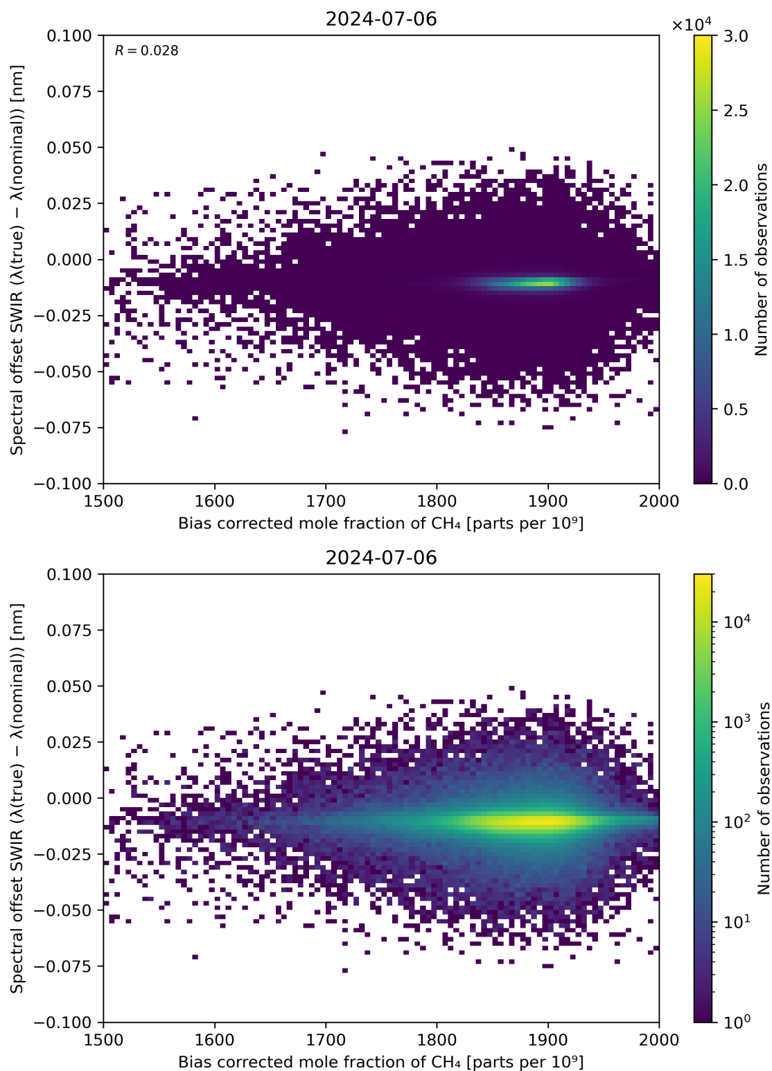
Figure 69: Scatter density plot of “Bias corrected mole fraction of \text{CH}_4 ” against “Spectral offset SWIR ( \lambda(\text{true}) - \lambda(\text{nominal}) )” for 2024-07-05 to 2024-07-07.
