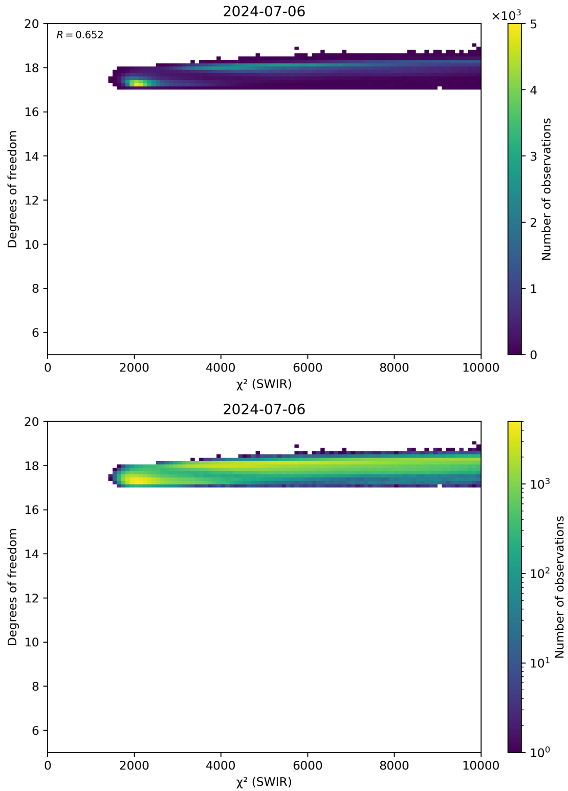
Figure 48: Scatter density plot of “ \chi^2 (SWIR)” against “Degrees of freedom” for 2024-07-05 to 2024-07-07.
