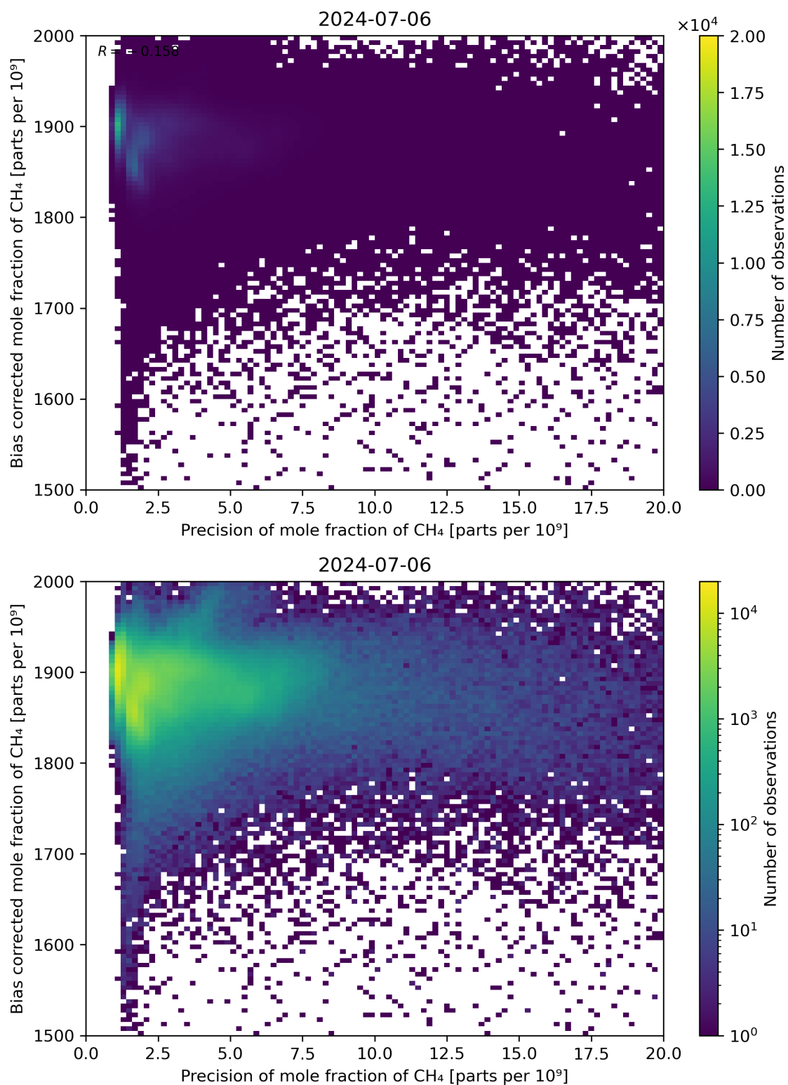
Figure 82: Scatter density plot of “Precision of mole fraction of CH 4 ” against “Bias corrected mole fraction of CH 4 ” for 2024-07-05 to 2024-07-07.
