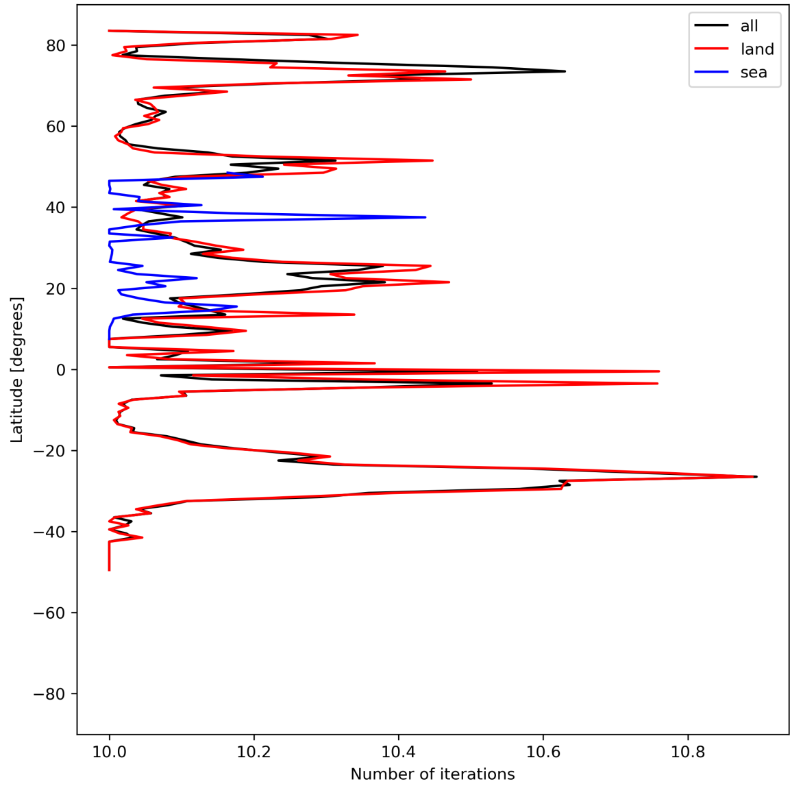
Figure 20: Zonal average of “Number of iterations” for 2024-07-05 to 2024-07-07.
