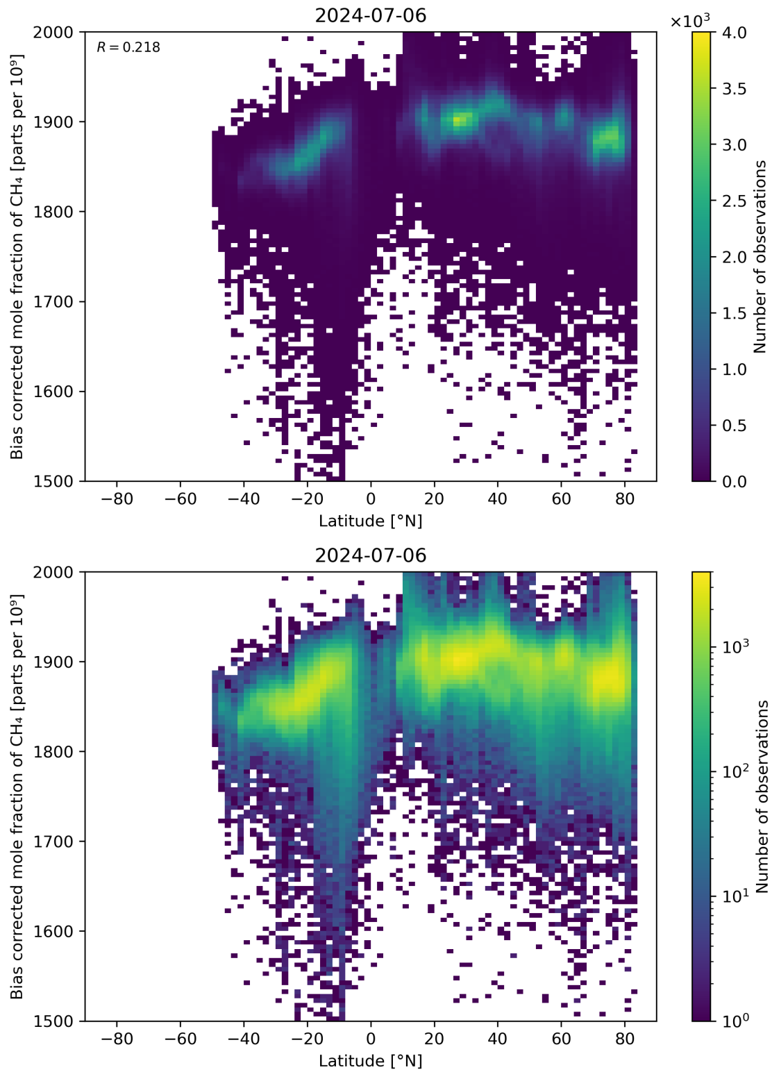
Figure 58: Scatter density plot of “Latitude” against “Bias corrected mole fraction of \text{CH}_4 ” for 2024-07-05 to 2024-07-07.
