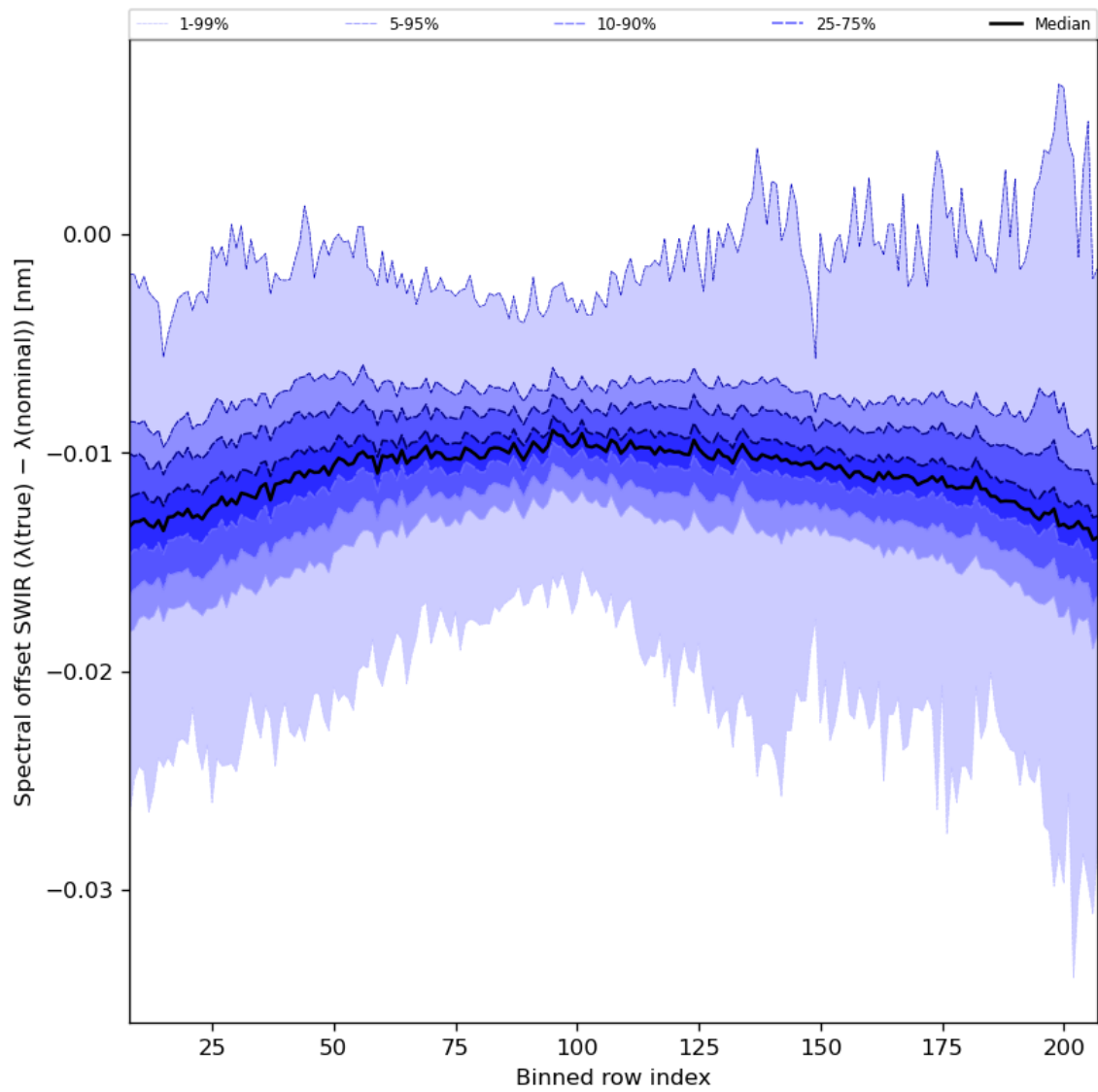
Figure 38: Along track statistics of “Spectral offset SWIR ( \lambda(\text{true}) - \lambda(\text{nominal}) )” for 2024-07-05 to 2024-07-07
