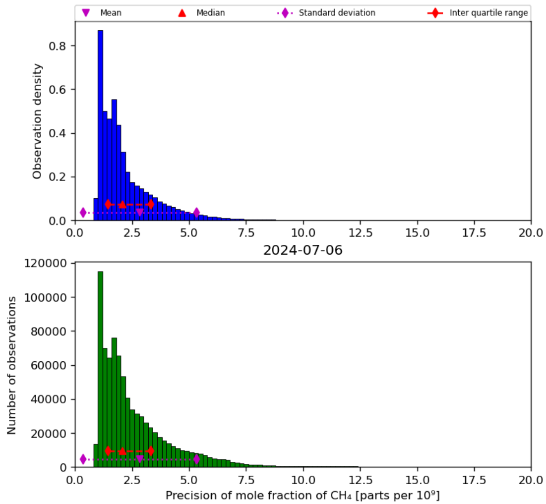
Figure 24: Histogram of “Precision of mole fraction of CH 4 ” for 2024-07-05 to 2024-07-07
