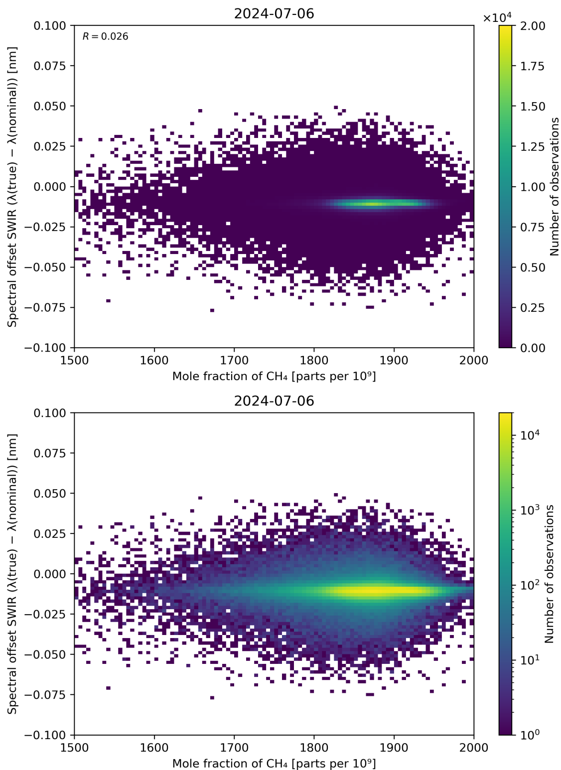
Figure 86: Scatter density plot of “Mole fraction of CH 4 ” against “Spectral offset SWIR ( \lambda(\text{true}) - \lambda(\text{nominal}) )” for 2024-07-05 to 2024-07-07.
