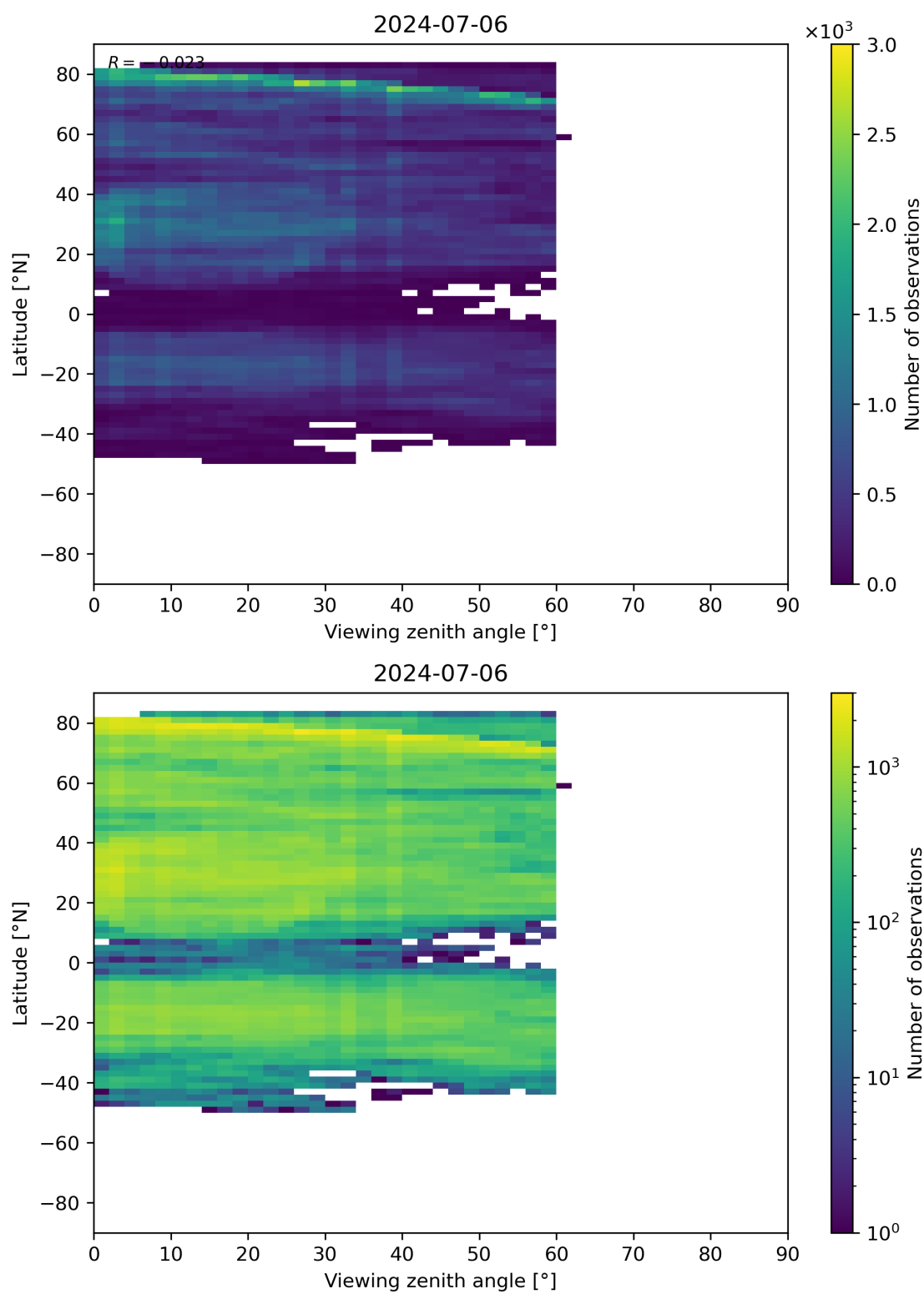
Figure 109: Scatter density plot of “Viewing zenith angle” against “Latitude” for 2024-07-05 to 2024-07-07.
