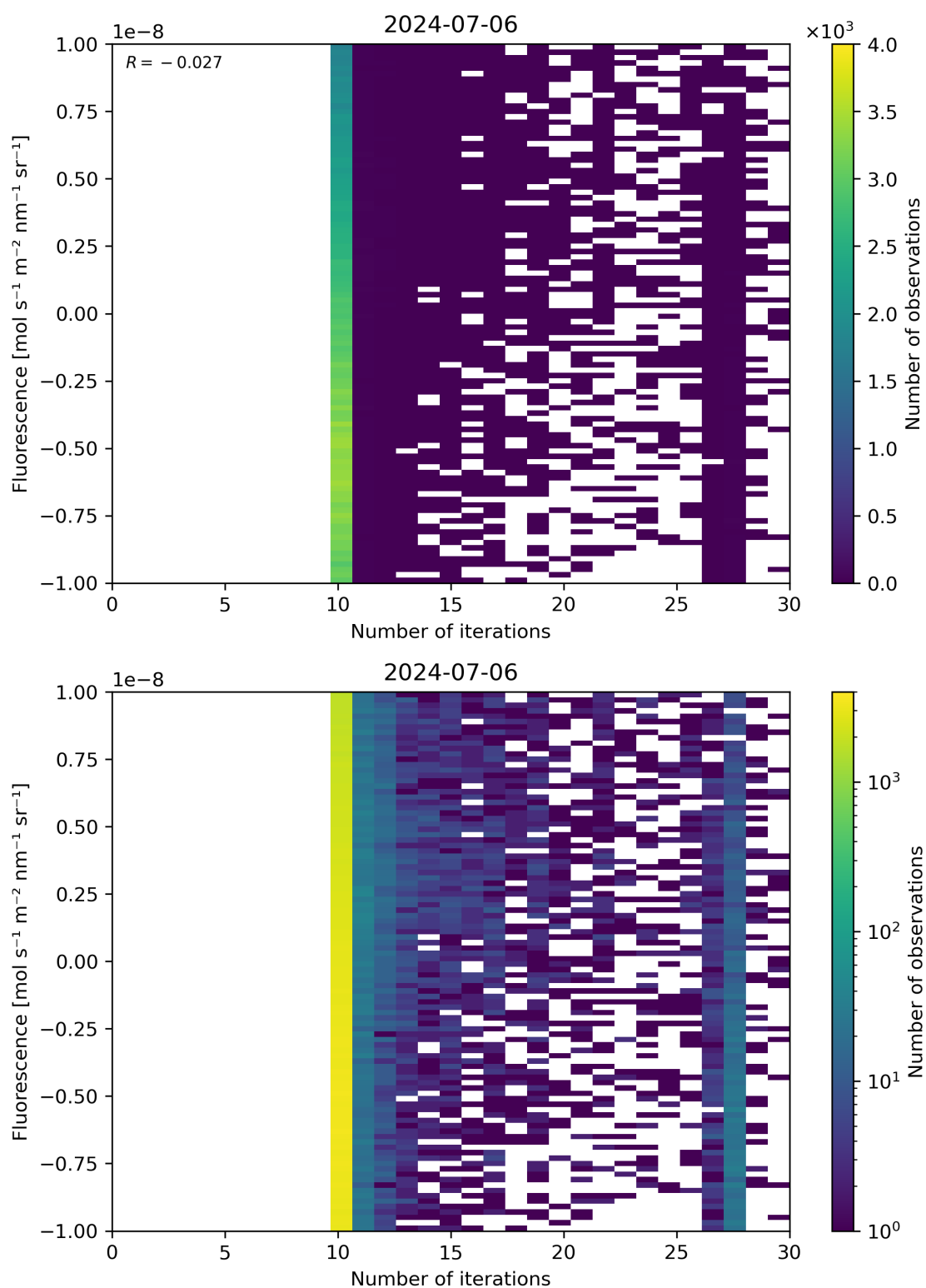
Figure 87: Scatter density plot of “Number of iterations” against “Fluorescence” for 2024-07-05 to 2024-07-07.
