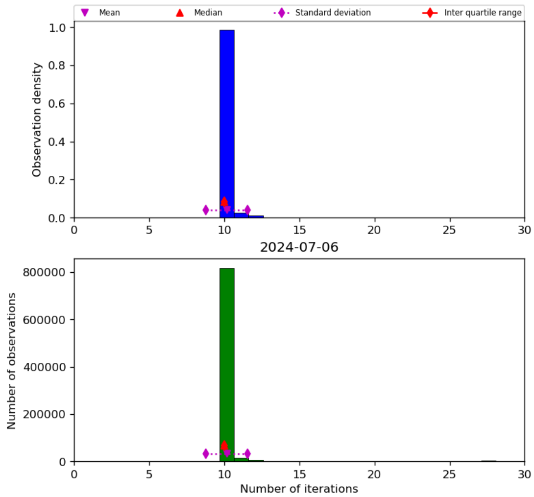
Figure 31: Histogram of “Number of iterations” for 2024-07-05 to 2024-07-07
