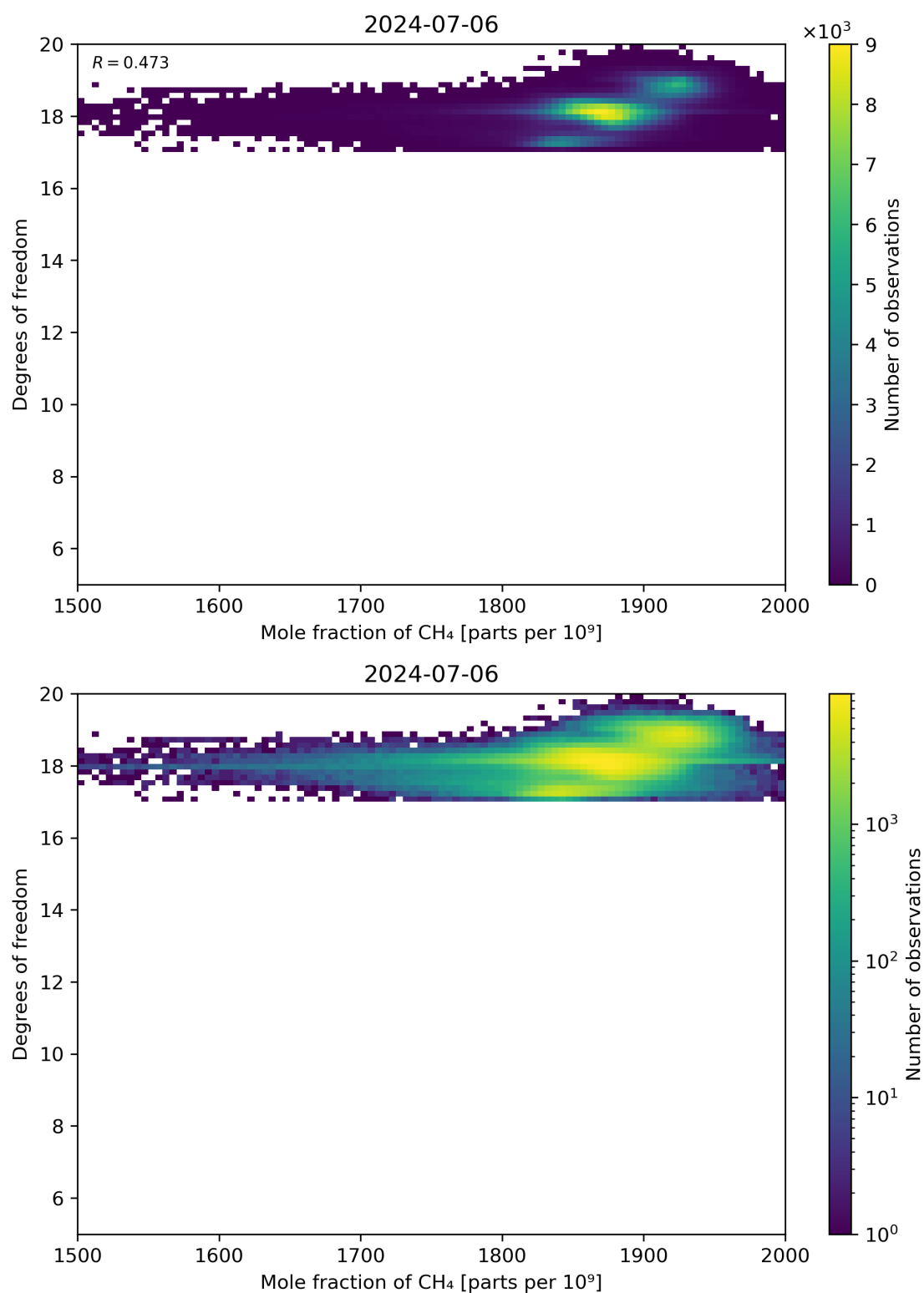
Figure 72: Scatter density plot of “Mole fraction of CH 4 ” against “Degrees of freedom” for 2024-07-05 to 2024-07-07.
