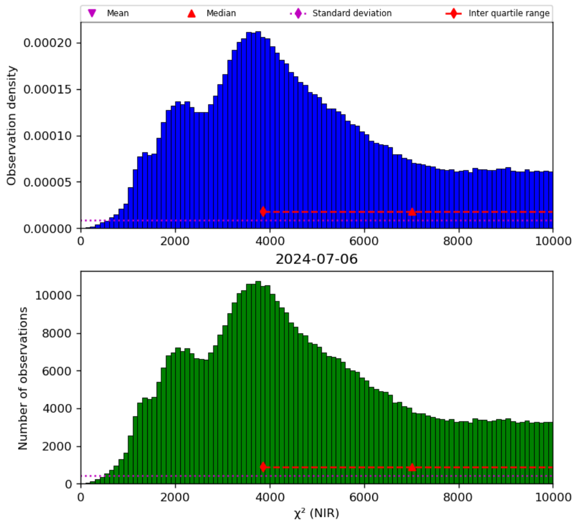
Figure 29: Histogram of “ \chi^2 (NIR)” for 2024-07-05 to 2024-07-07
