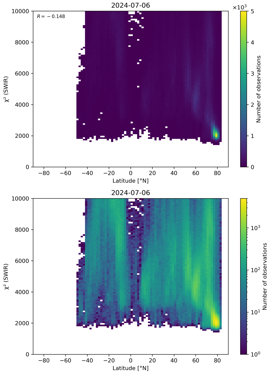
Figure 54: Scatter density plot of “Latitude” against “ \chi^2 (SWIR)” for 2024-07-05 to 2024-07-07.
