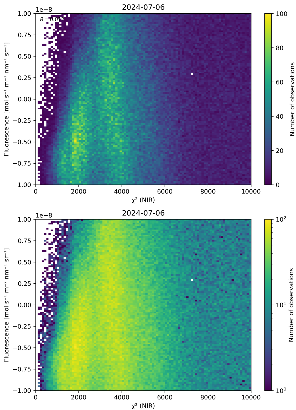
Figure 45: Scatter density plot of “ \chi^2 (NIR)” against “Fluorescence” for 2024-07-05 to 2024-07-07.
