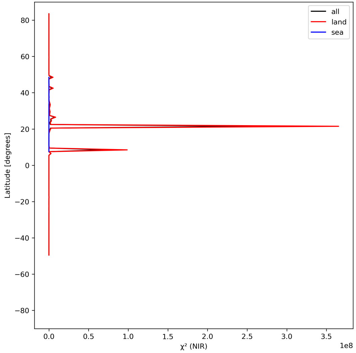
Figure 18: Zonal average of “ \chi^2 (NIR)” for 2024-07-05 to 2024-07-07.
