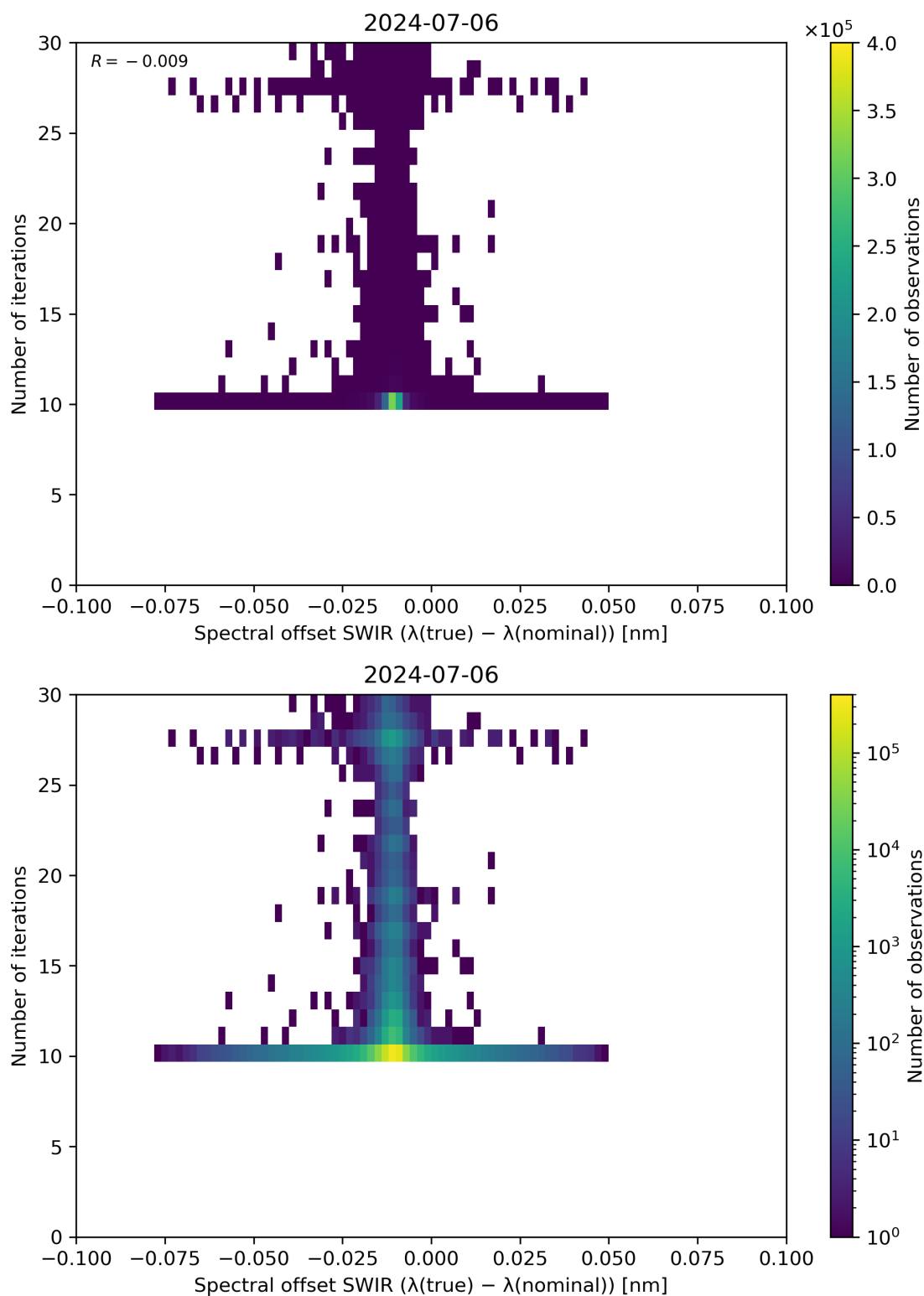
Figure 121: Scatter density plot of “Spectral offset SWIR ( \lambda(\text{true}) - \lambda(\text{nominal}) )” against “Number of iterations” for 2024-07-05 to 2024-07-07.
