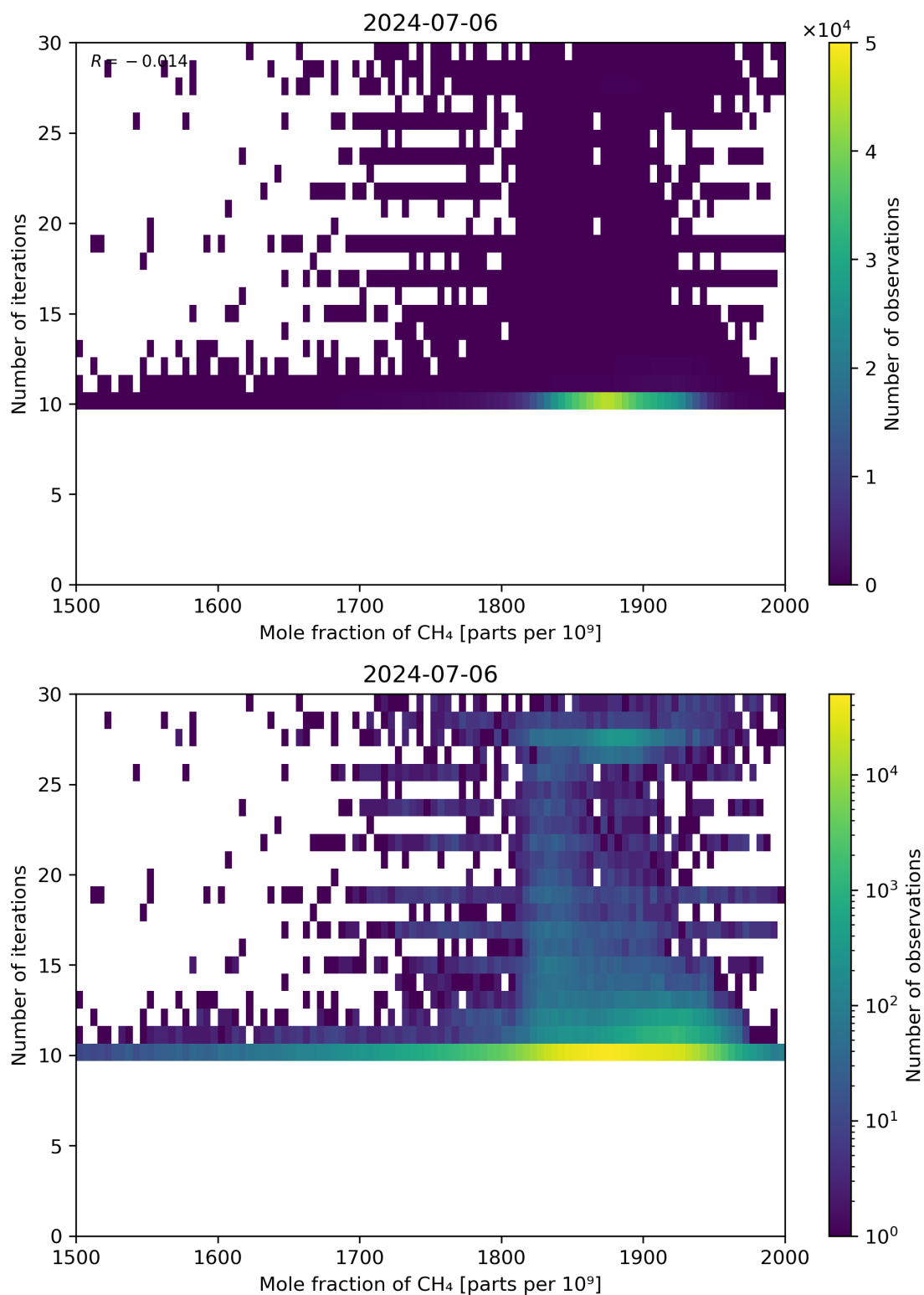
Figure 76: Scatter density plot of “Mole fraction of CH 4 ” against “Number of iterations” for 2024-07-05 to 2024-07-07.
