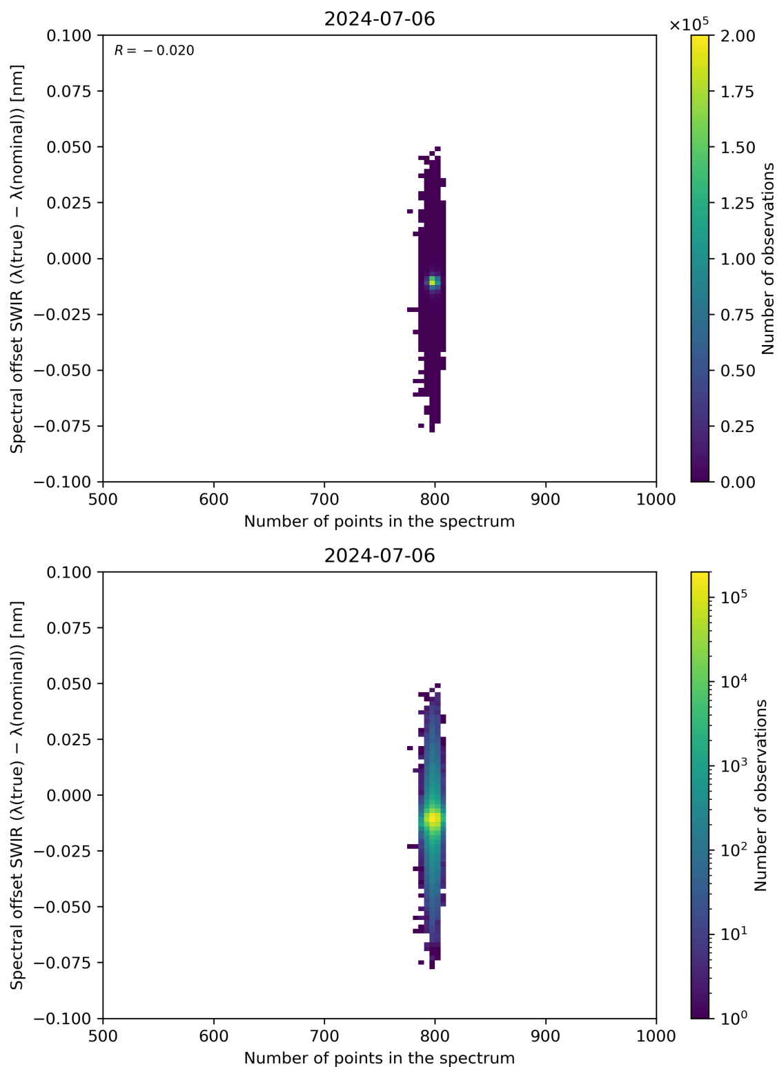
Figure 93: Scatter density plot of “Number of points in the spectrum” against “Spectral offset SWIR ( \lambda(\text{true}) - \lambda(\text{nominal}) )” for 2024-07-05 to 2024-07-07.
