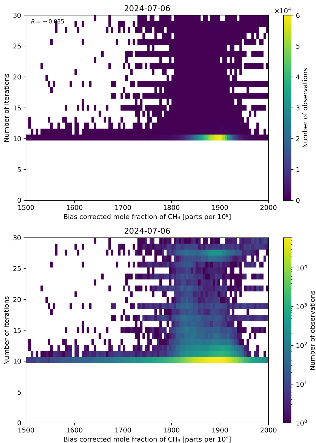
Figure 67: Scatter density plot of “Bias corrected mole fraction of CH 4 ” against “Number of iterations” for 2024-07-05 to 2024-07-07.
