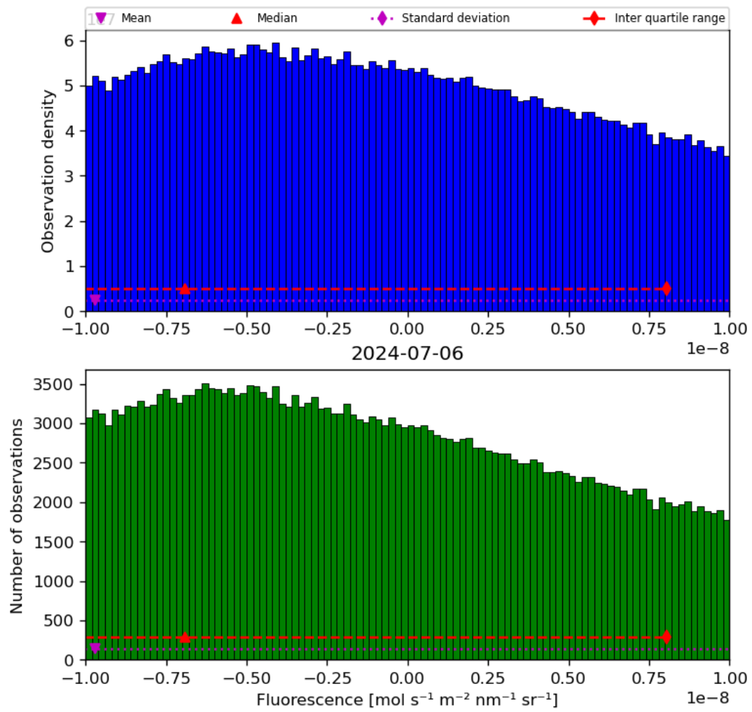
Figure 32: Histogram of “Fluorescence” for 2024-07-05 to 2024-07-07
