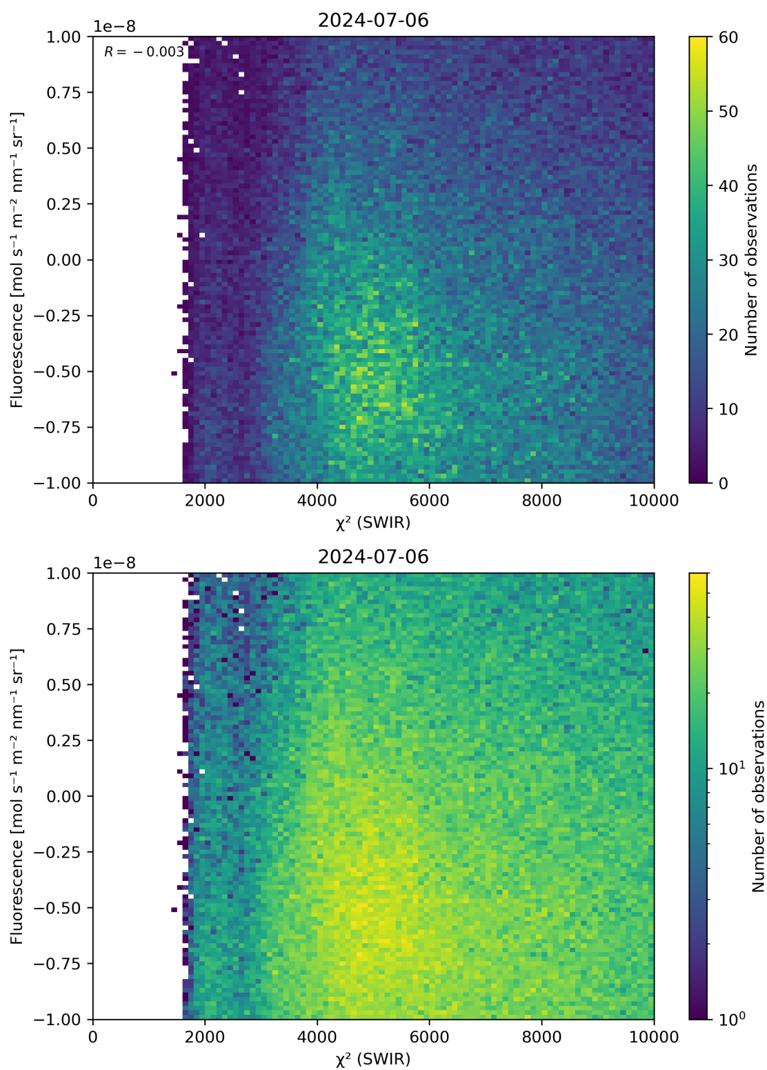
Figure 49: Scatter density plot of “ \chi^2 (SWIR)” against “Fluorescence” for 2024-07-05 to 2024-07-07.
