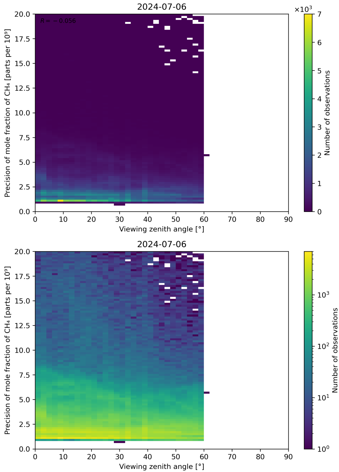
Figure 112: Scatter density plot of “Viewing zenith angle” against “Precision of mole fraction of CH 4 ” for 2024-07-05 to 2024-07-07.
