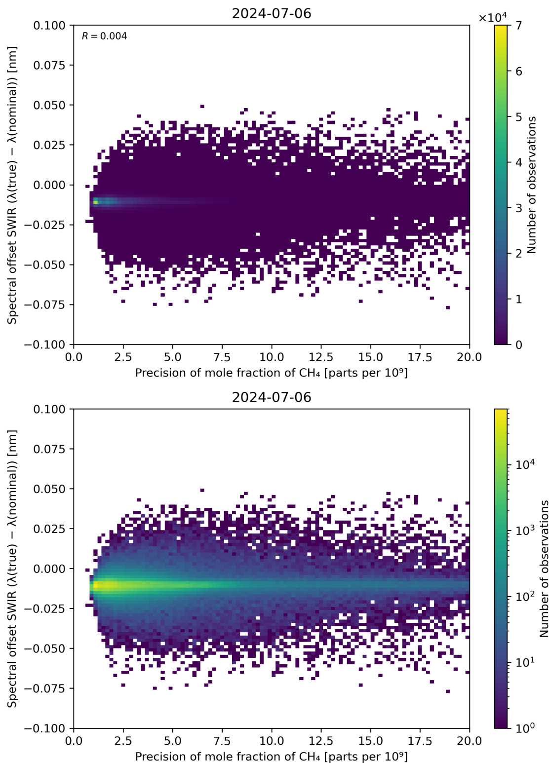
Figure 85: Scatter density plot of “Precision of mole fraction of \text{CH}_4 ” against “Spectral offset SWIR ( \lambda(\text{true}) - \lambda(\text{nominal}) )” for 2024-07-05 to 2024-07-07.
