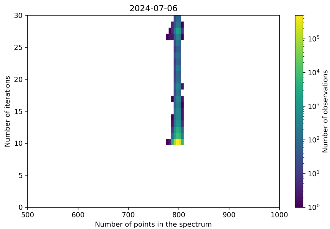
Figure 92: Scatter density plot of “Number of points in the spectrum” against “Number of iterations” for 2024-07-05 to 2024-07-07.
