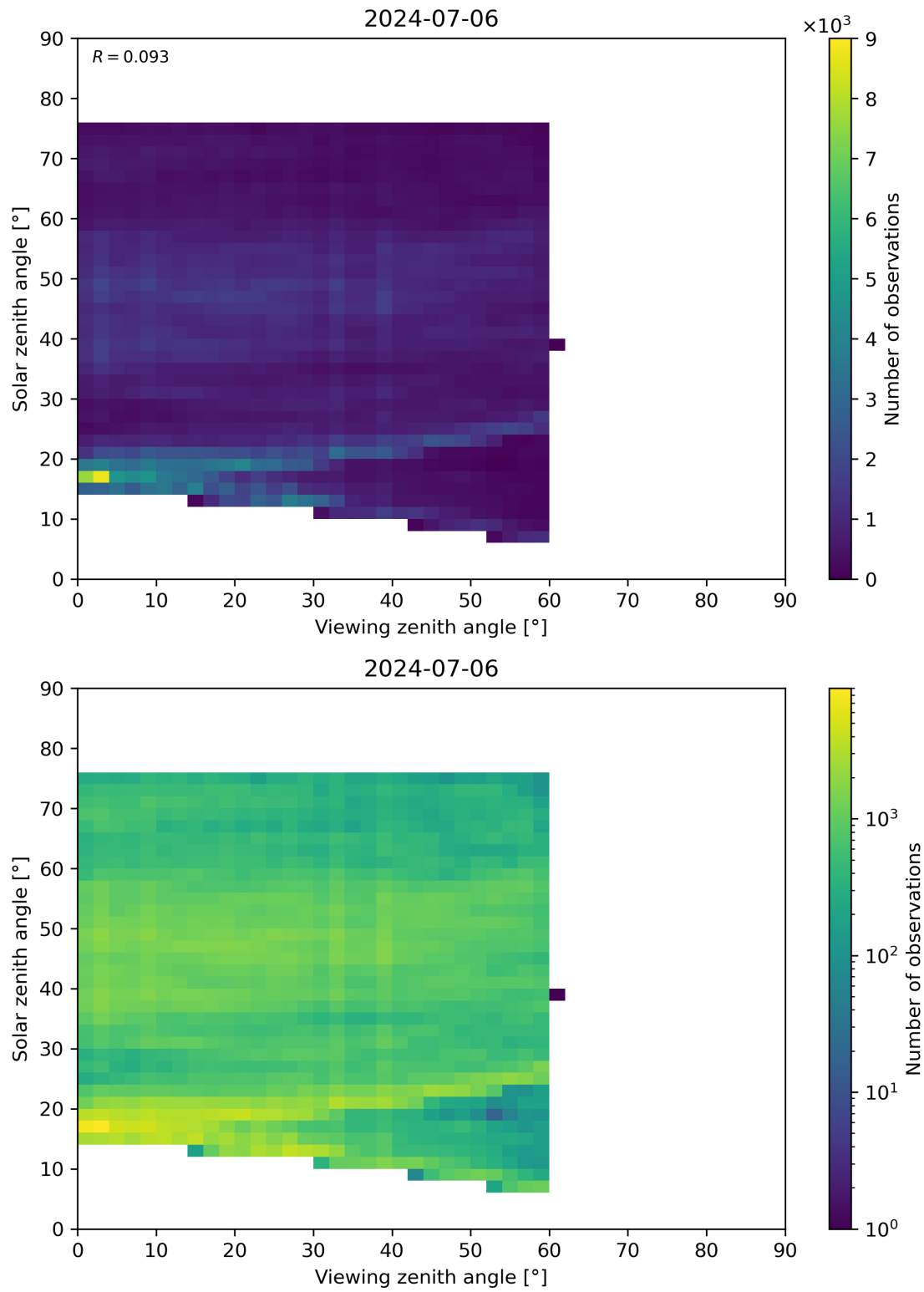
Figure 115: Scatter density plot of “Viewing zenith angle” against “Solar zenith angle” for 2024-07-05 to 2024-07-07.
