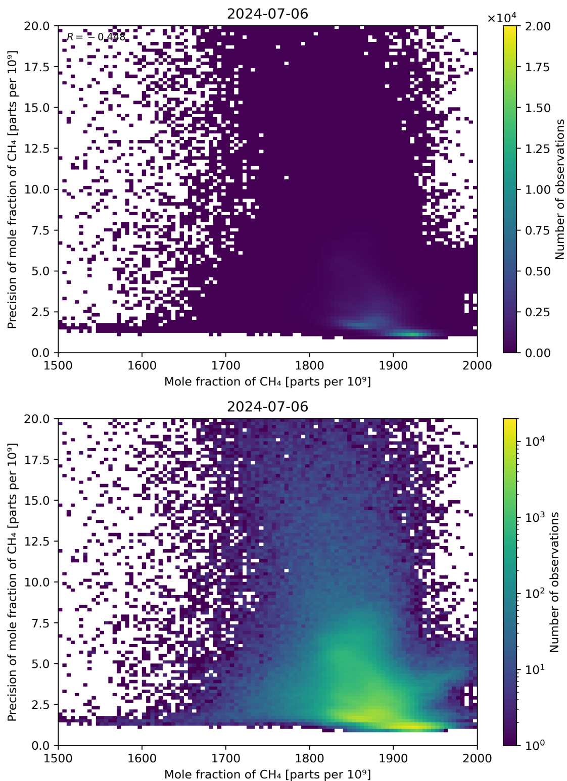
Figure 75: Scatter density plot of “Mole fraction of CH 4 ” against “Precision of mole fraction of CH 4 ” for 2024-07-05 to 2024-07-07.
