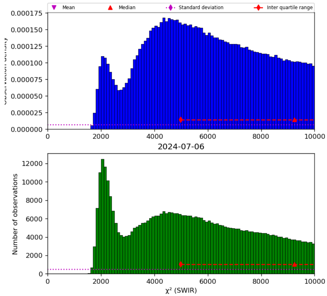
Figure 28: Histogram of “ \chi^2 (SWIR)” for 2024-07-05 to 2024-07-07
