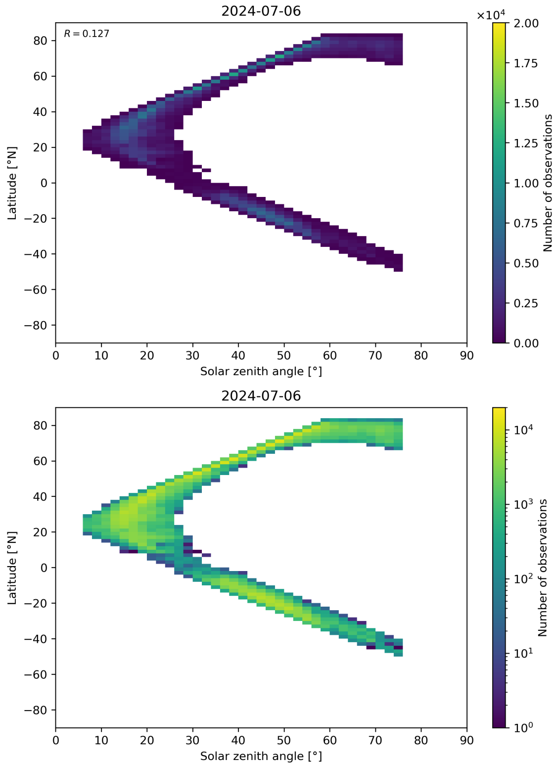
Figure 98: Scatter density plot of “Solar zenith angle” against “Latitude” for 2024-07-05 to 2024-07-07.
