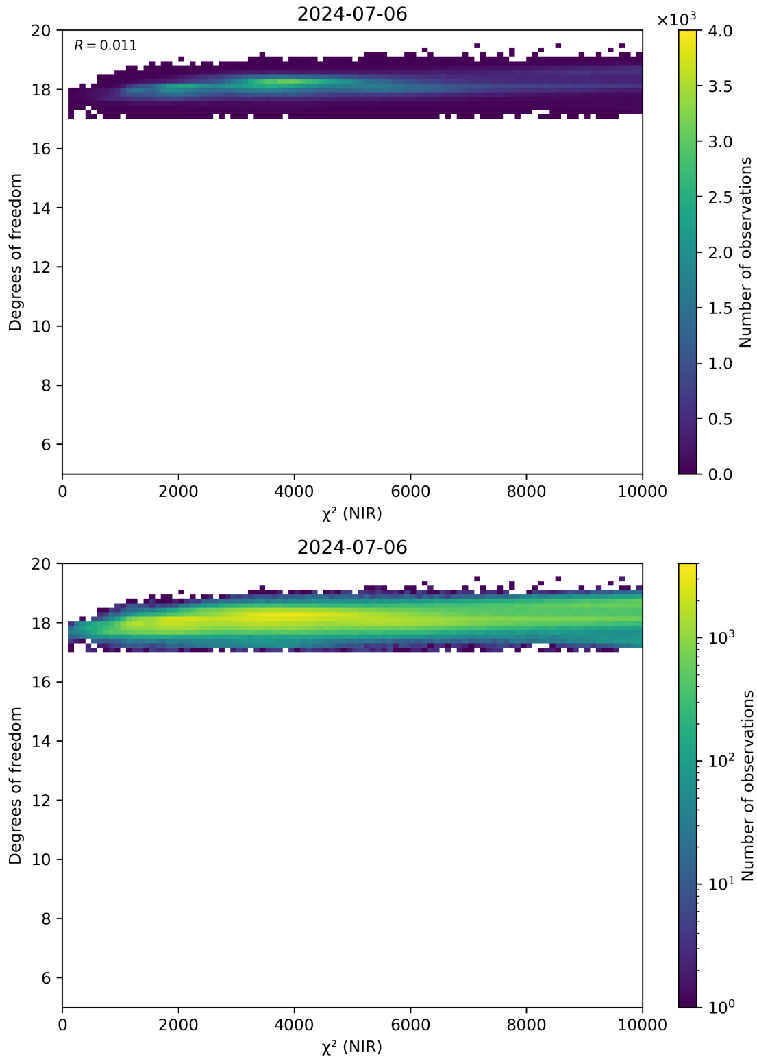
Figure 44: Scatter density plot of “ \chi^2 (NIR)” against “Degrees of freedom” for 2024-07-05 to 2024-07-07.
