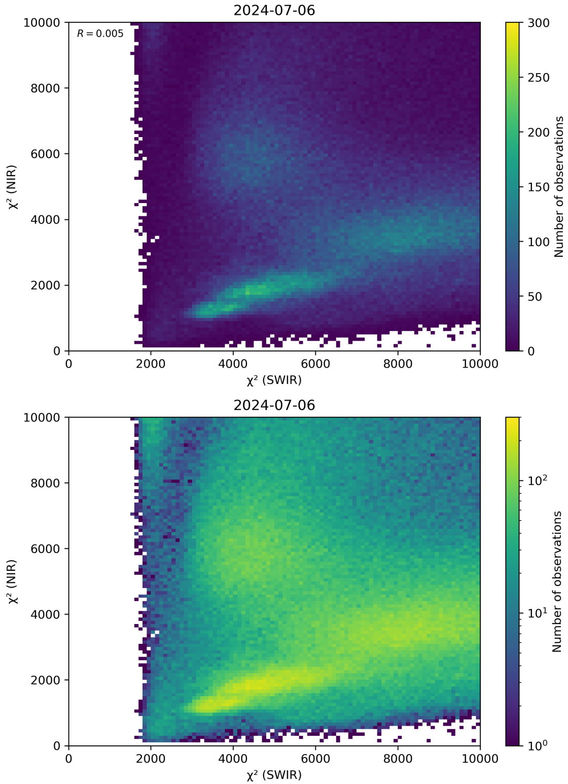
Figure 47: Scatter density plot of “ \chi^2 (SWIR)” against “ \chi^2 (NIR)” for 2024-07-05 to 2024-07-07.
