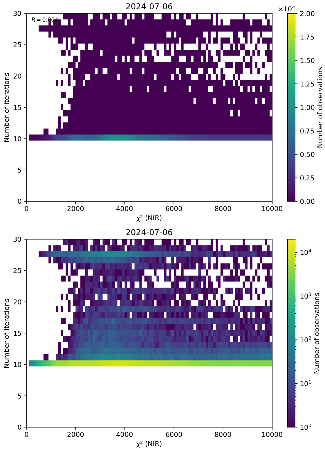
Figure 46: Scatter density plot of “ \chi^2 (NIR)” against “Number of iterations” for 2024-07-05 to 2024-07-07.
