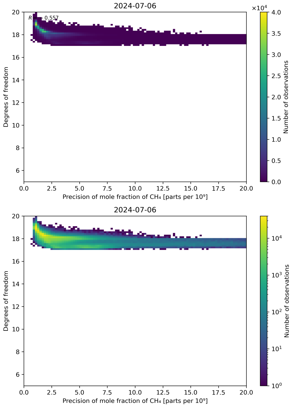
Figure 80: Scatter density plot of “Precision of mole fraction of CH 4 ” against “Degrees of freedom” for 2024-07-05 to 2024-07-07.
