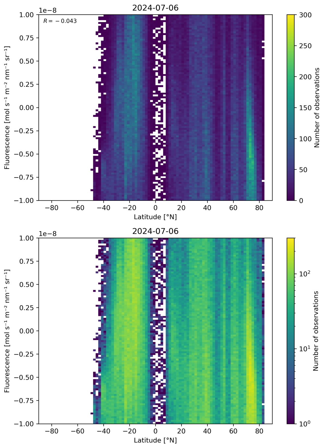
Figure 56: Scatter density plot of “Latitude” against “Fluorescence” for 2024-07-05 to 2024-07-07.
