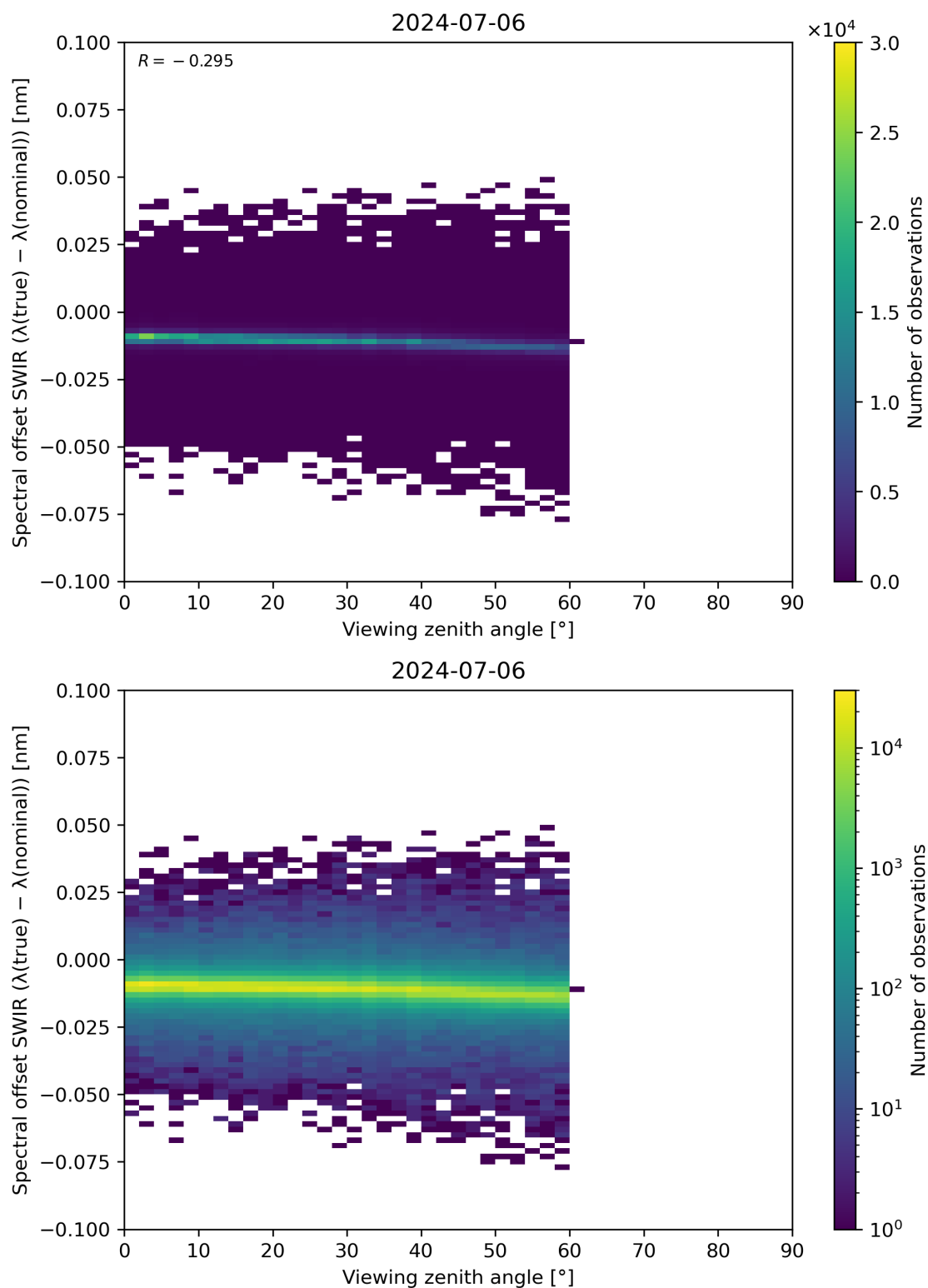
Figure 116: Scatter density plot of “Viewing zenith angle” against “Spectral offset SWIR ( \lambda(\text{true}) - \lambda(\text{nominal}) )” for 2024-07-05 to 2024-07-07.
