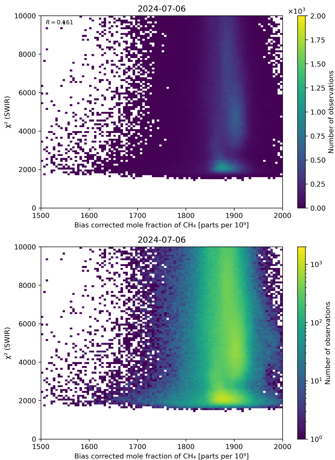
Figure 64: Scatter density plot of “Bias corrected mole fraction of CH 4 ” against “ \chi^2 (SWIR)” for 2024-07-05 to 2024-07-07.
