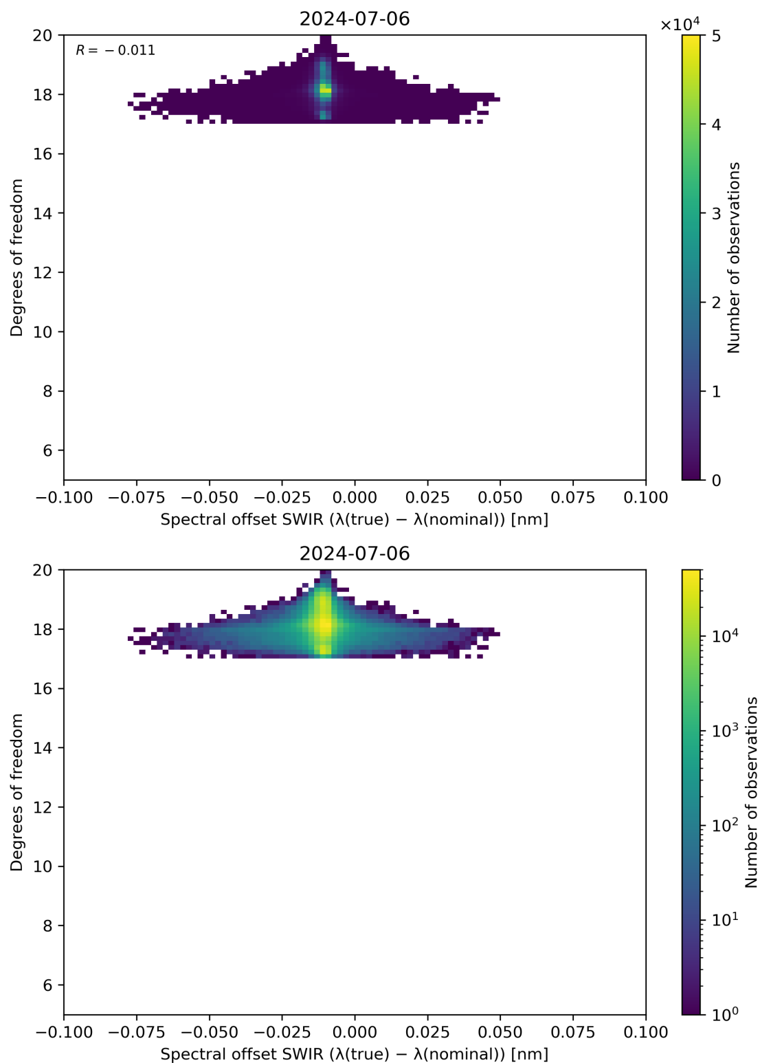
Figure 119: Scatter density plot of “Spectral offset SWIR ( \lambda(\text{true}) - \lambda(\text{nominal}) )” against “Degrees of freedom” for 2024-07-05 to 2024-07-07.
