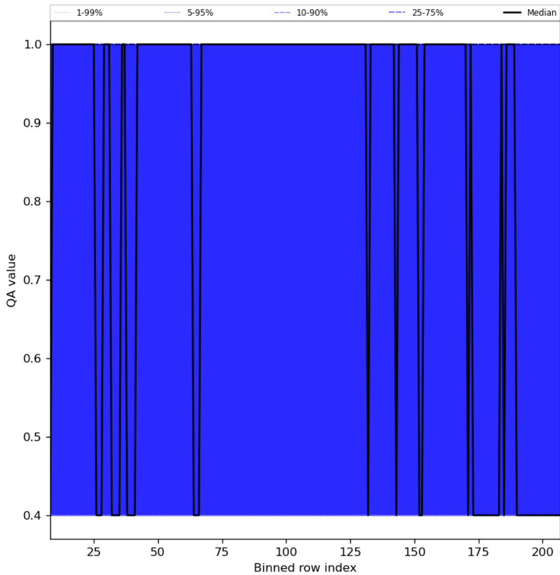
Figure 33: Along track statistics of “QA value” for 2024-07-05 to 2024-07-07
