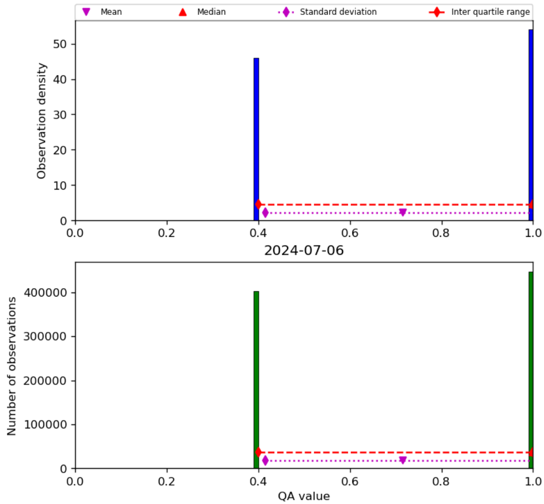
Figure 22: Histogram of “QA value” for 2024-07-05 to 2024-07-07
