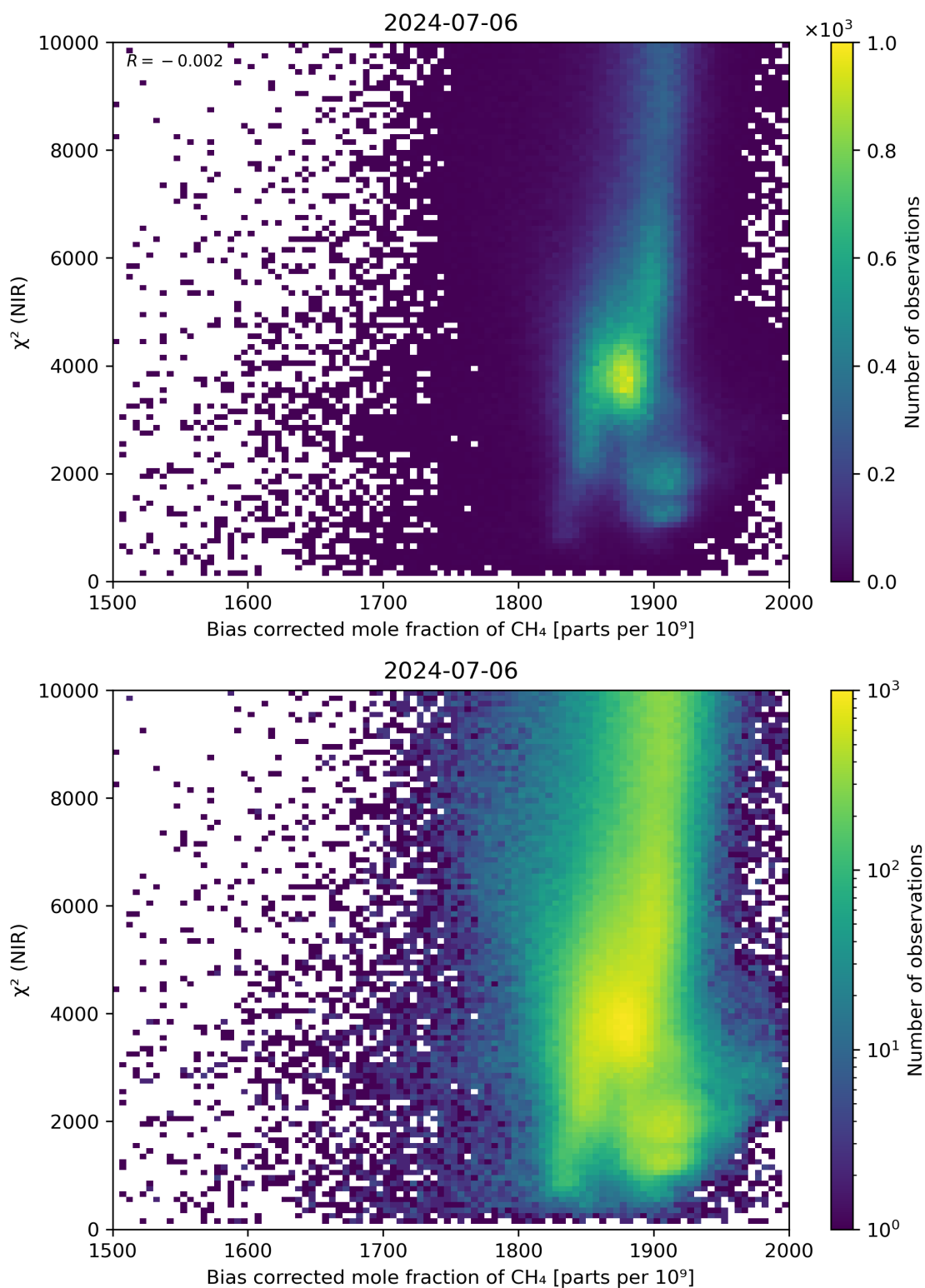
Figure 63: Scatter density plot of “Bias corrected mole fraction of CH 4 ” against “ \chi^2 (NIR)” for 2024-07-05 to 2024-07-07.
