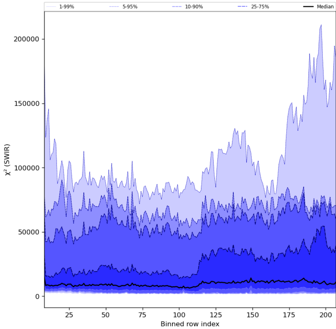
Figure 39: Along track statistics of " \chi^2 (SWIR)" for 2024-07-05 to 2024-07-07
