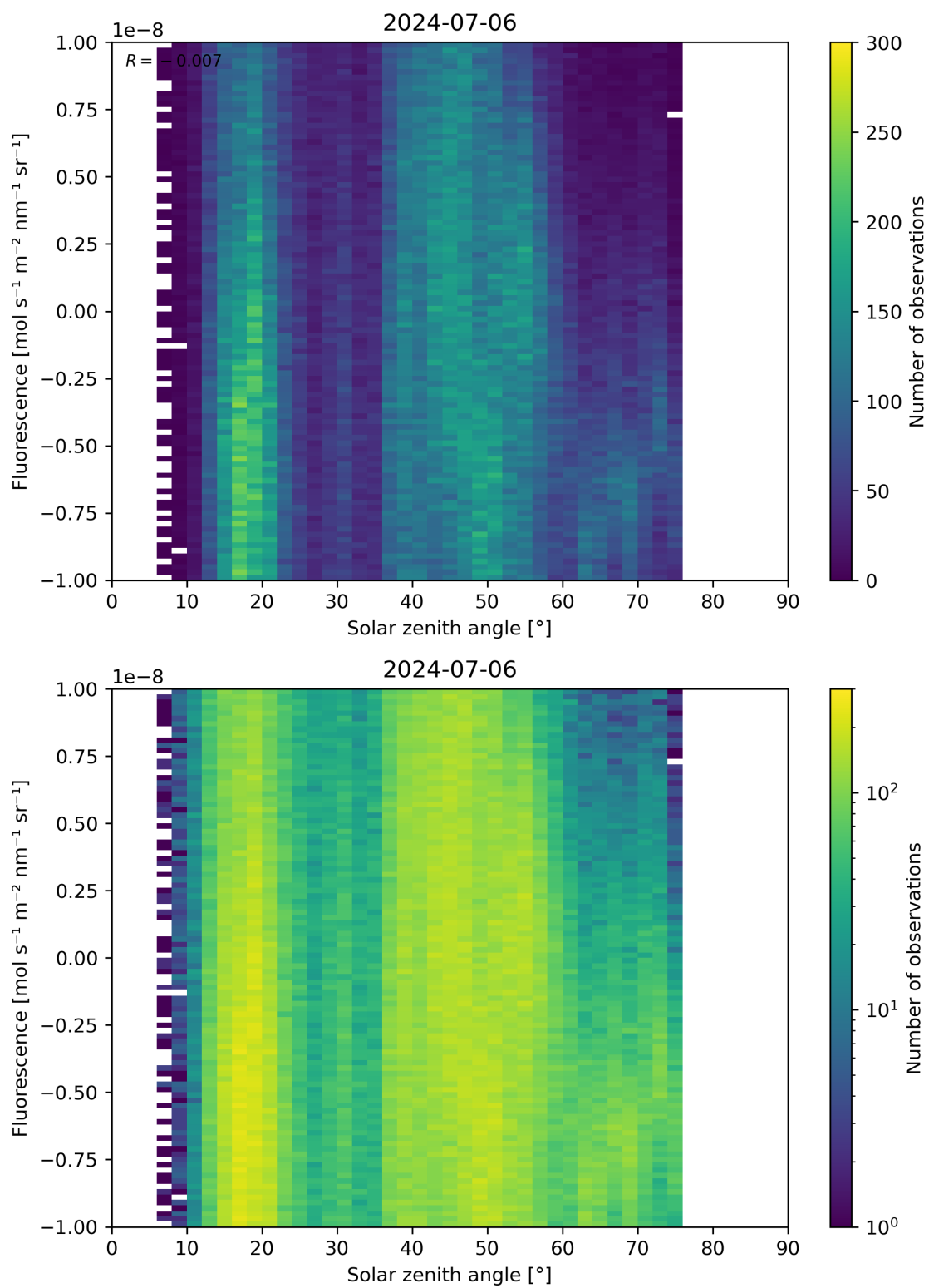
Figure 97: Scatter density plot of “Solar zenith angle” against “Fluorescence” for 2024-07-05 to 2024-07-07.
