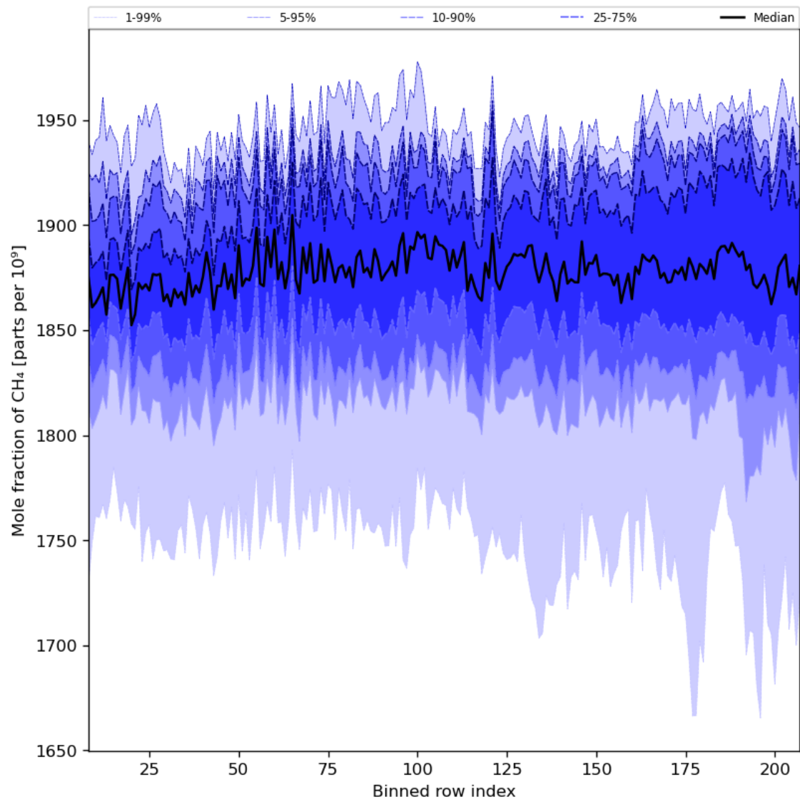
Figure 34: Along track statistics of “Mole fraction of CH 4 ” for 2024-07-05 to 2024-07-07
