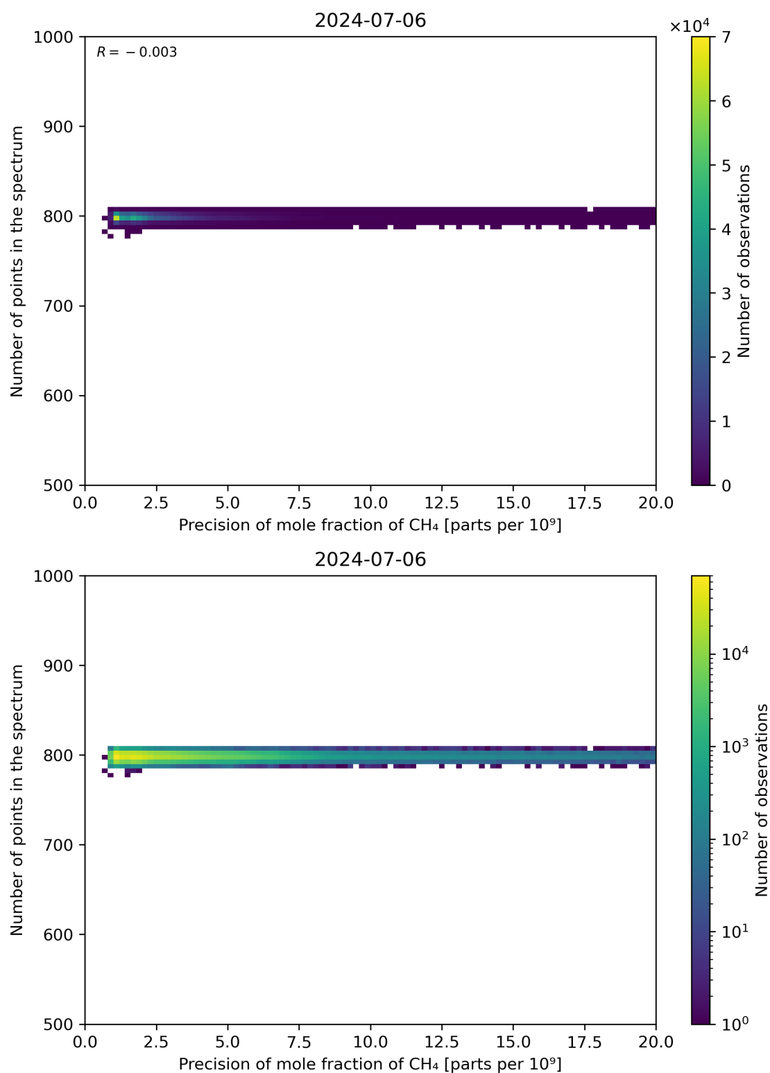
Figure 84: Scatter density plot of “Precision of mole fraction of CH 4 ” against “Number of points in the spectrum” for 2024-07-05 to 2024-07-07.
