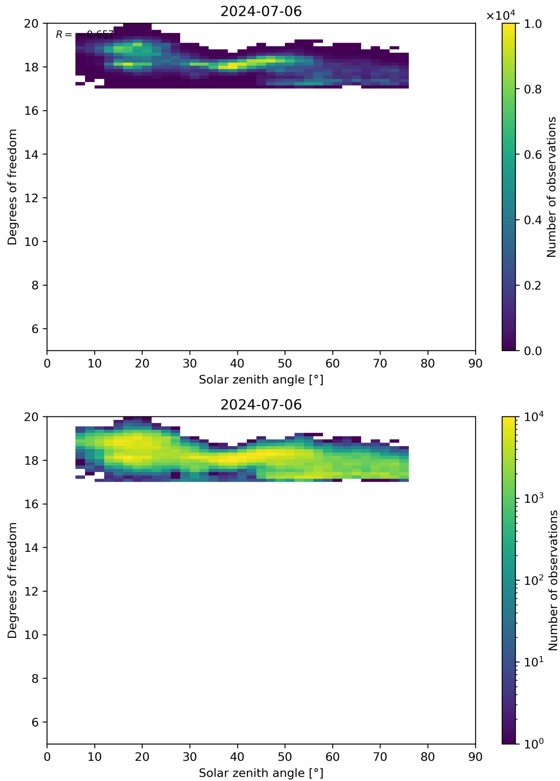
Figure 96: Scatter density plot of “Solar zenith angle” against “Degrees of freedom” for 2024-07-05 to 2024-07-07.
