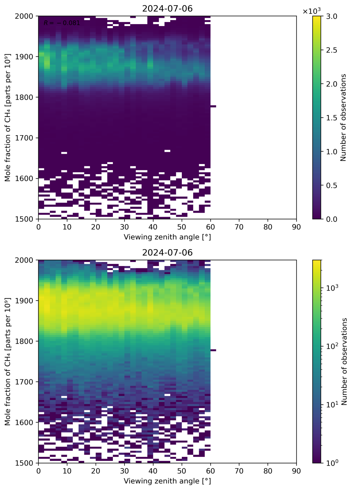
Figure 110: Scatter density plot of “Viewing zenith angle” against “Mole fraction of CH 4 ” for 2024-07-05 to 2024-07-07.
