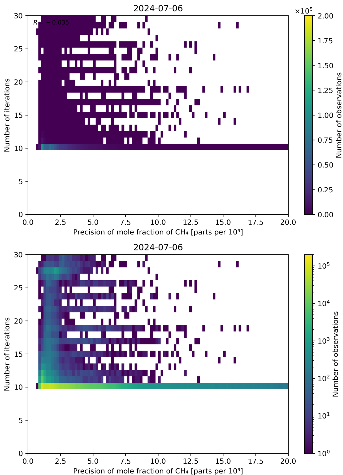
Figure 83: Scatter density plot of “Precision of mole fraction of CH 4 ” against “Number of iterations” for 2024-07-05 to 2024-07-07.
