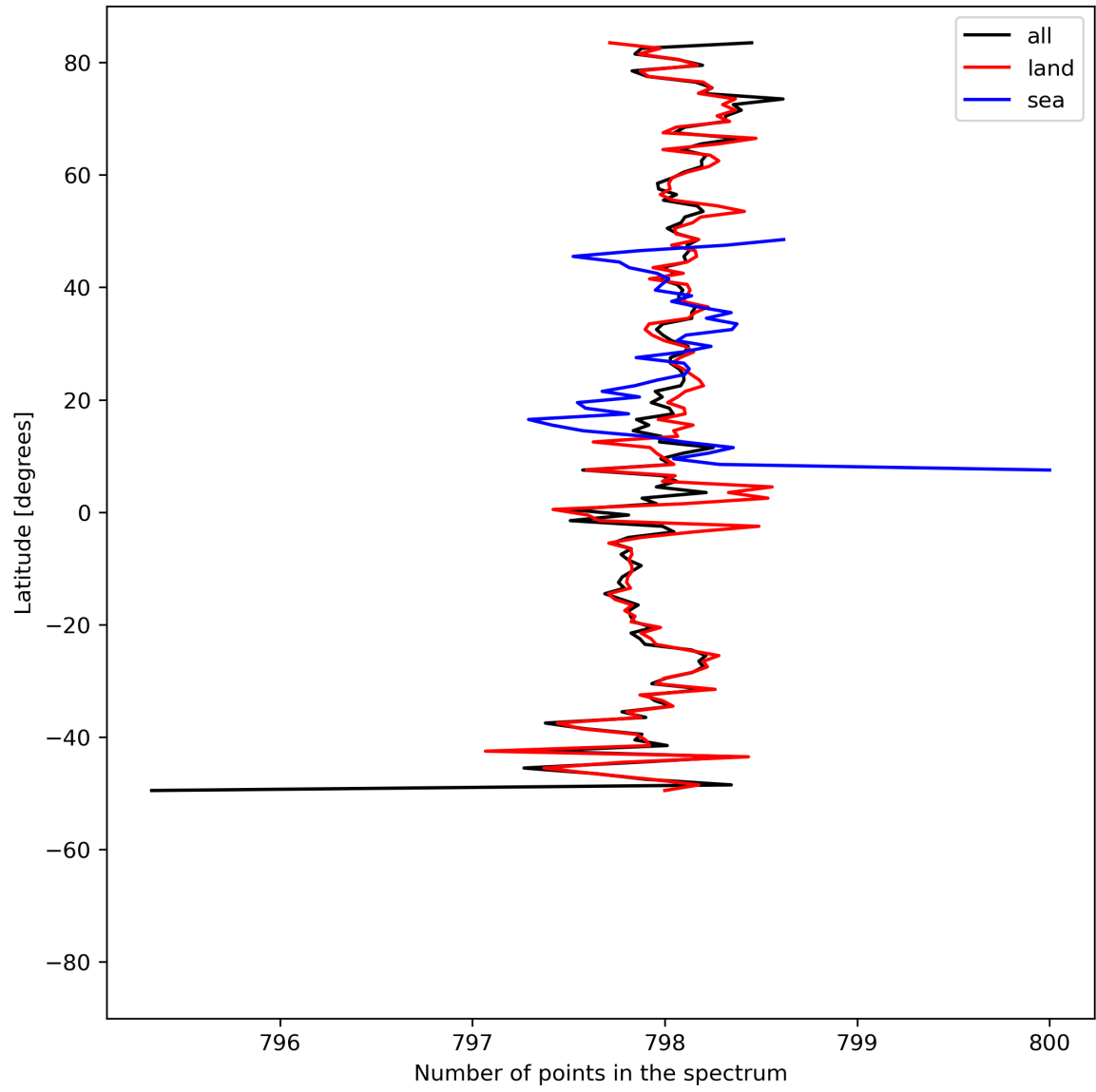
Figure 15: Zonal average of “Number of points in the spectrum” for 2024-07-05 to 2024-07-07.
