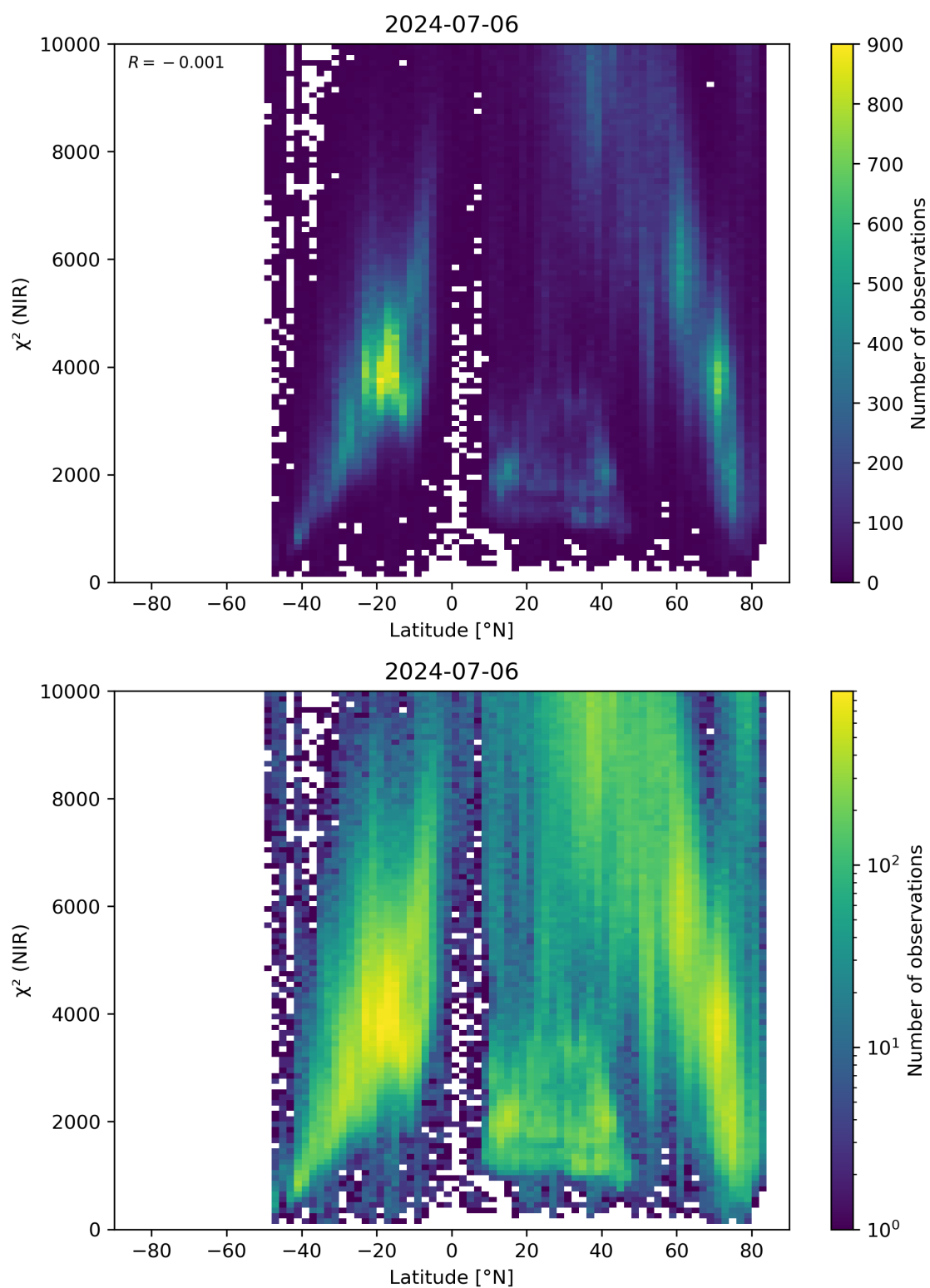
Figure 53: Scatter density plot of “Latitude” against “ \chi^2 (NIR)” for 2024-07-05 to 2024-07-07.
