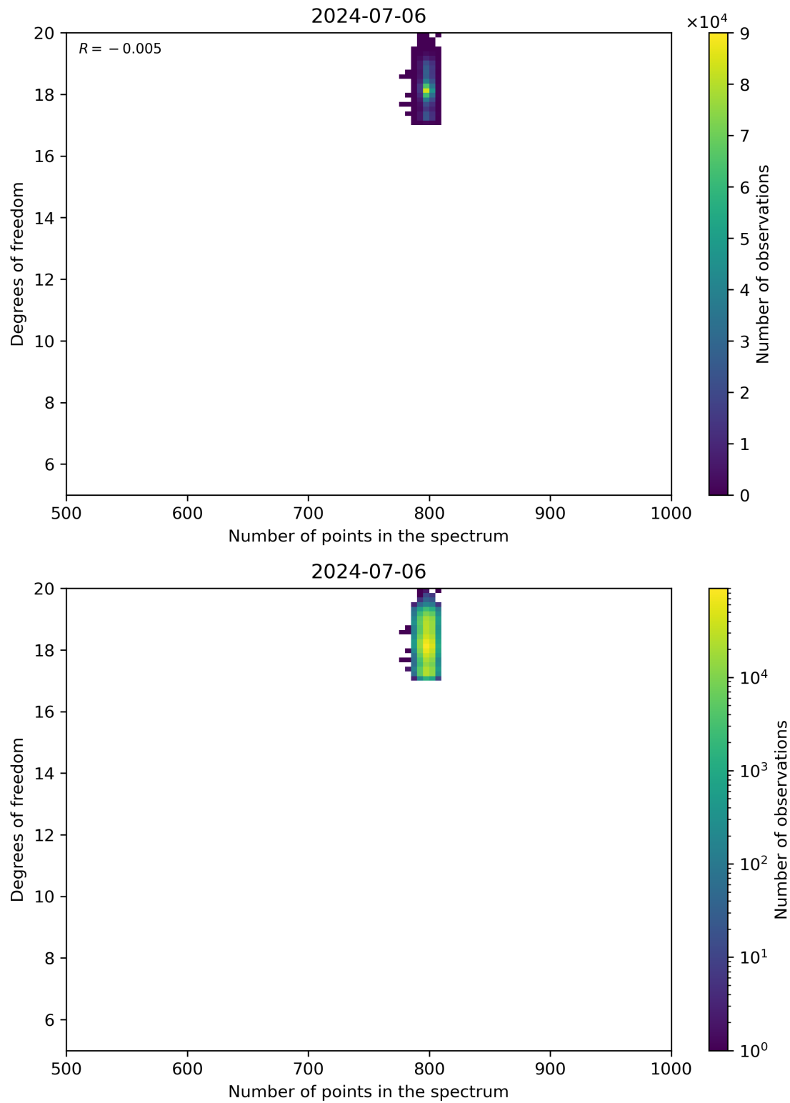
Figure 90: Scatter density plot of “Number of points in the spectrum” against “Degrees of freedom” for 2024-07-05 to 2024-07-07.
