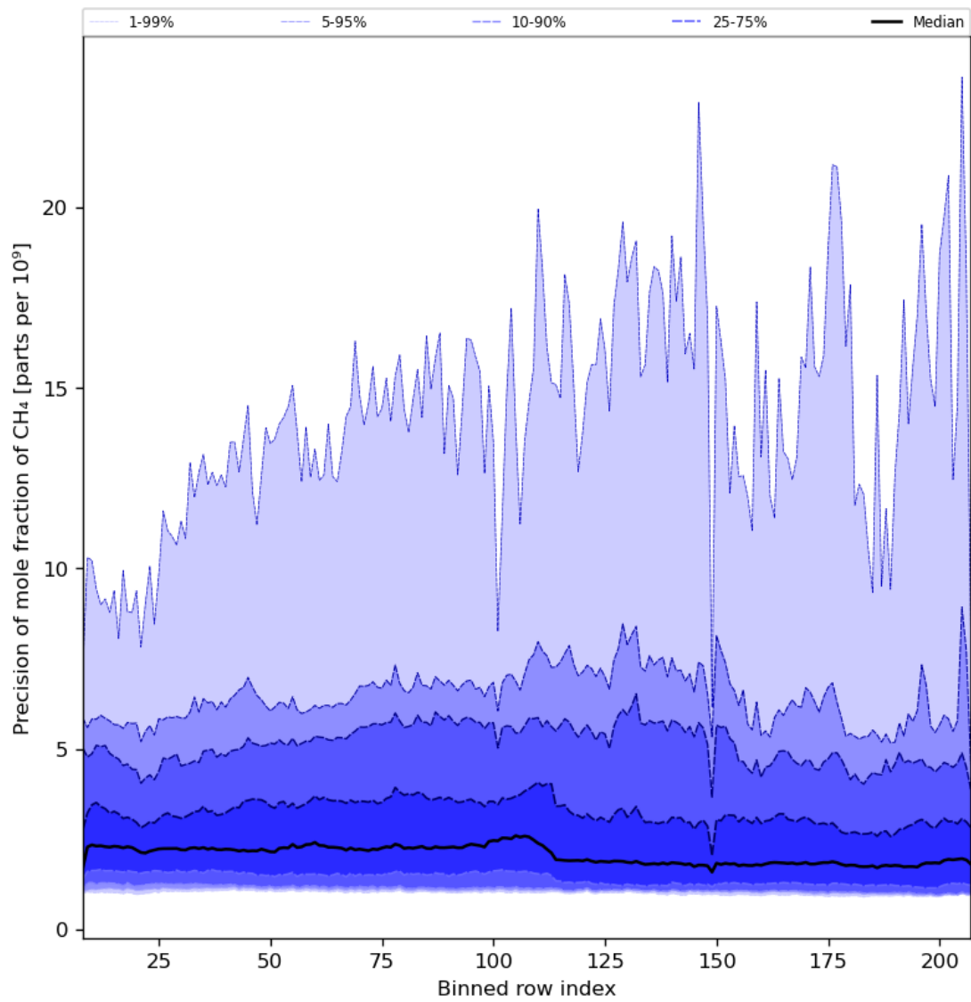
Figure 35: Along track statistics of “Precision of mole fraction of CH 4 ” for 2024-07-05 to 2024-07-07
