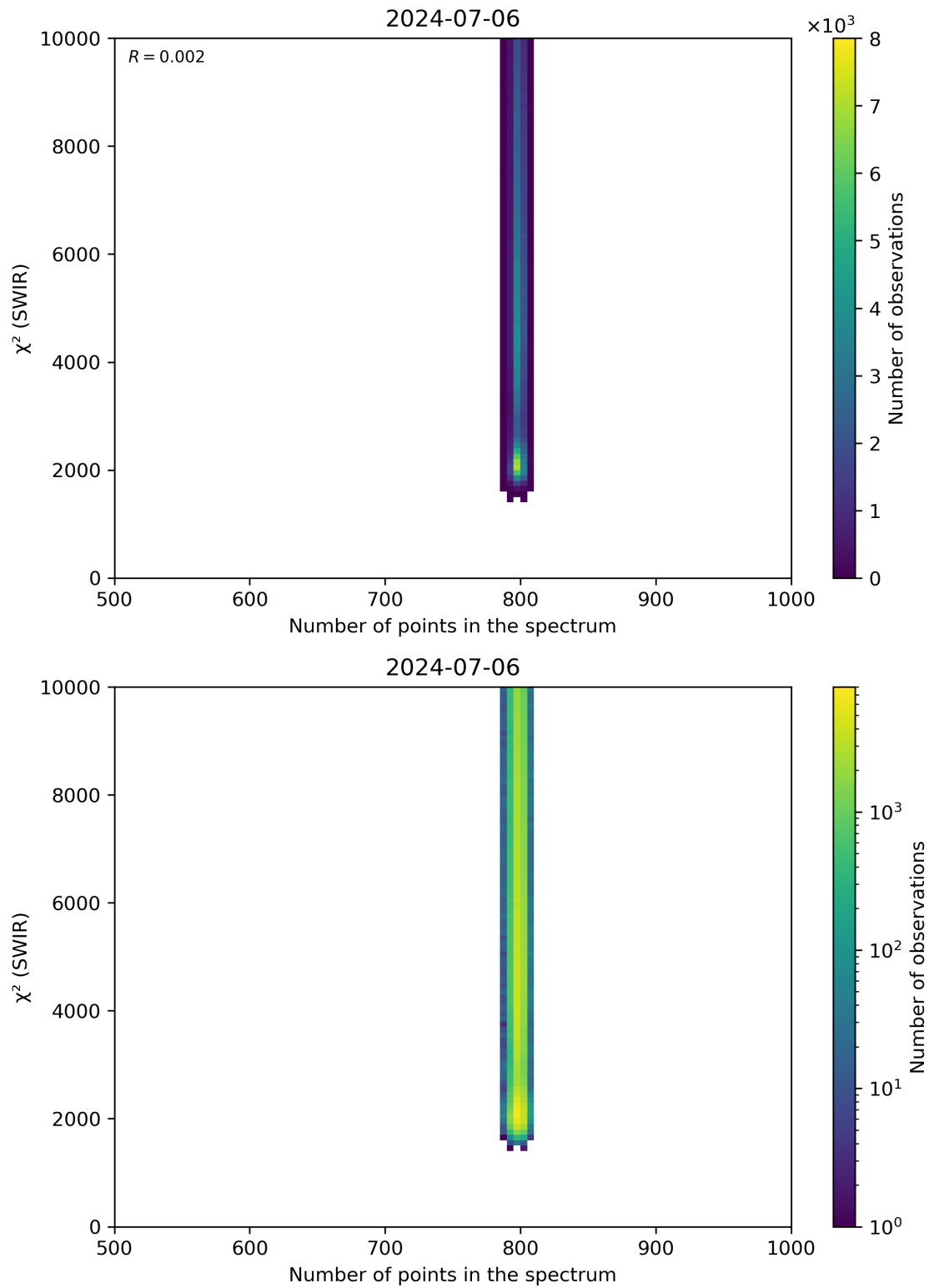
Figure 89: Scatter density plot of “Number of points in the spectrum” against “ \chi^2 (SWIR)” for 2024-07-05 to 2024-07-07.
