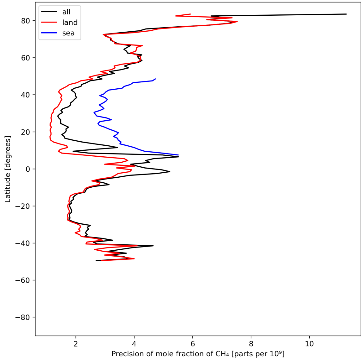
Figure 13: Zonal average of “Precision of mole fraction of CH 4 ” for 2024-07-05 to 2024-07-07.
