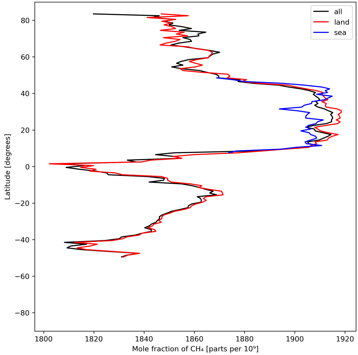
Figure 12: Zonal average of “Mole fraction of \text{CH}_4 ” for 2024-07-05 to 2024-07-07.
