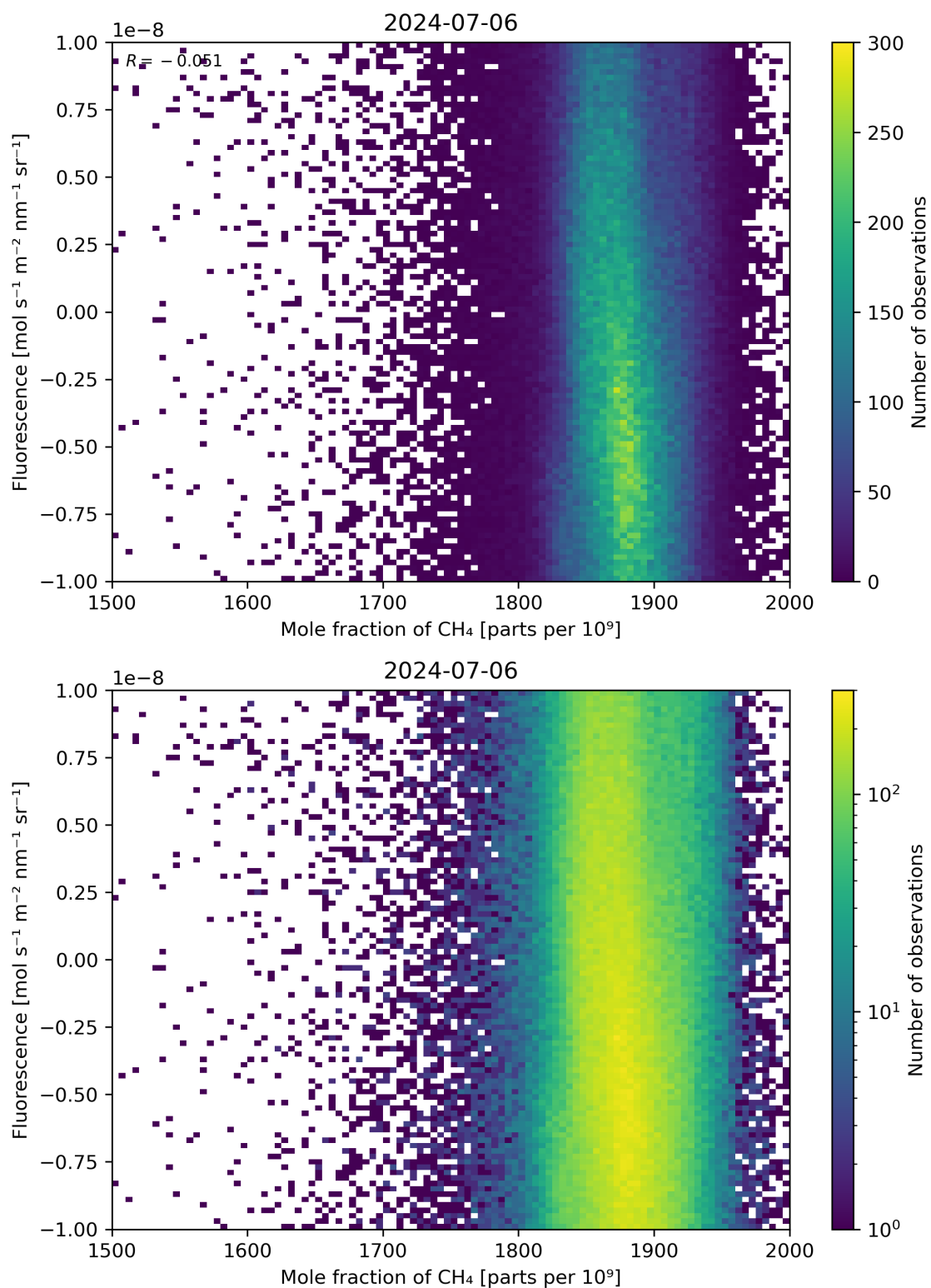
Figure 73: Scatter density plot of “Mole fraction of \text{CH}_4 ” against “Fluorescence” for 2024-07-05 to 2024-07-07.
