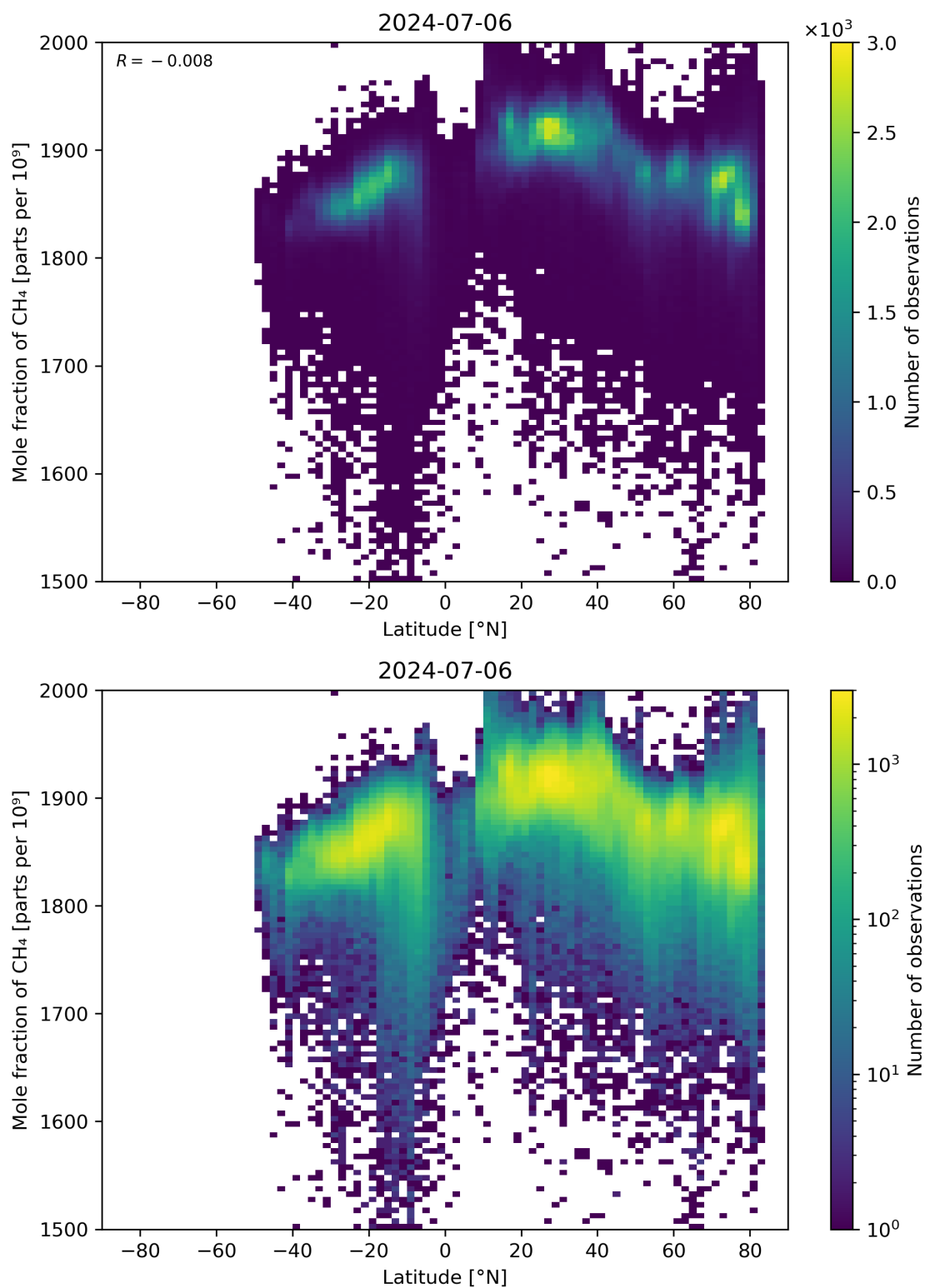
Figure 57: Scatter density plot of “Latitude” against “Mole fraction of CH 4 ” for 2024-07-05 to 2024-07-07.
