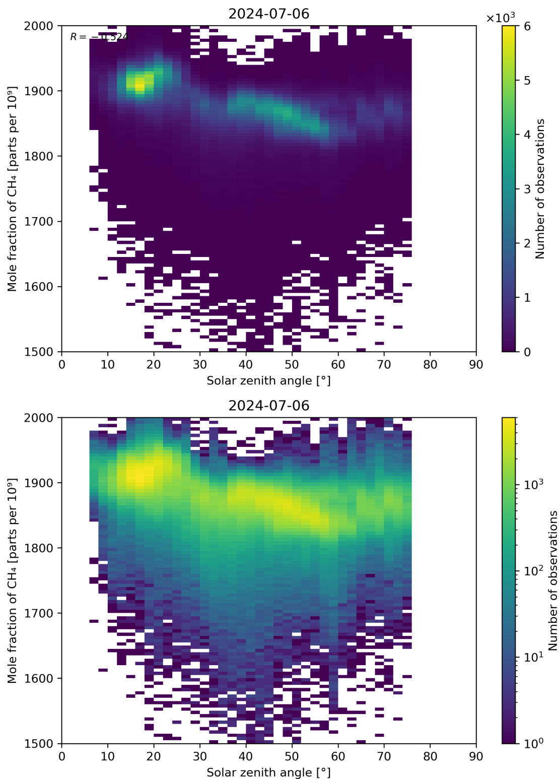
Figure 99: Scatter density plot of “Solar zenith angle” against “Mole fraction of CH 4 ” for 2024-07-05 to 2024-07-07.
