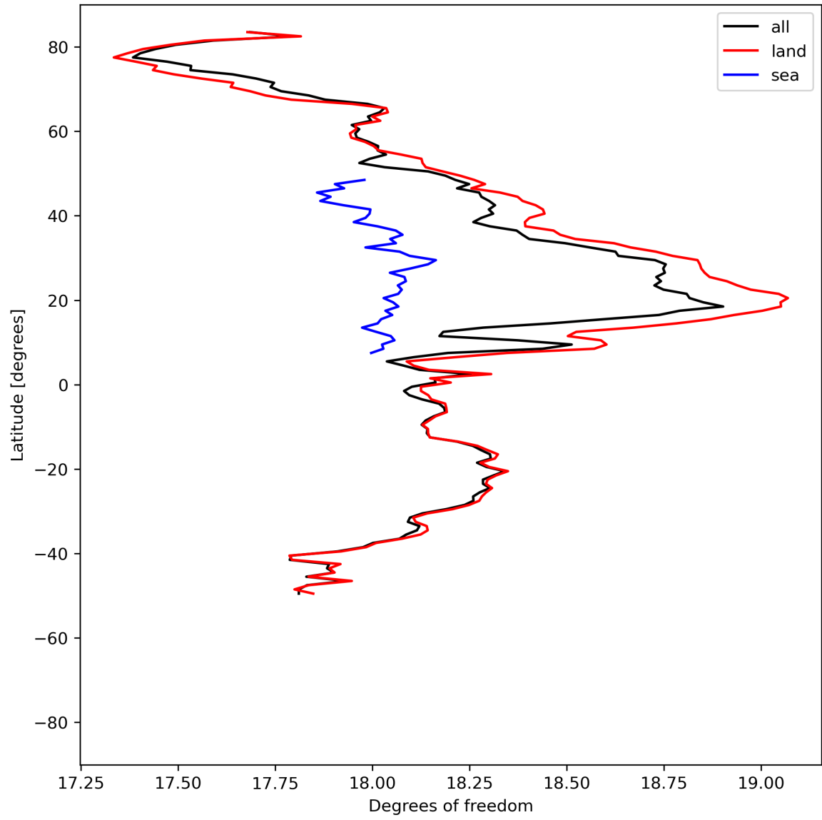
Figure 19: Zonal average of “Degrees of freedom” for 2024-07-05 to 2024-07-07.
