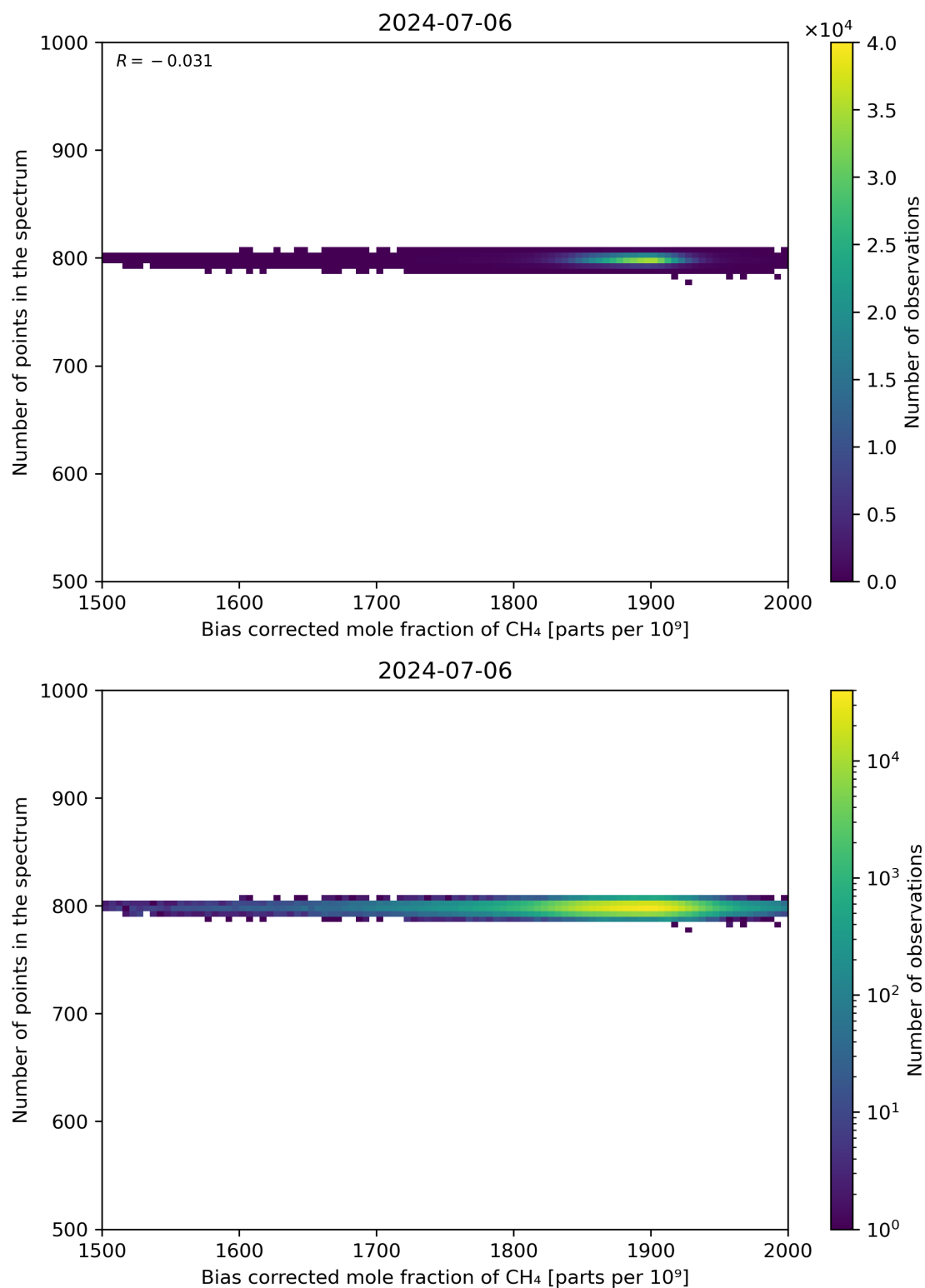
Figure 68: Scatter density plot of “Bias corrected mole fraction of CH 4 ” against “Number of points in the spectrum” for 2024-07-05 to 2024-07-07.
