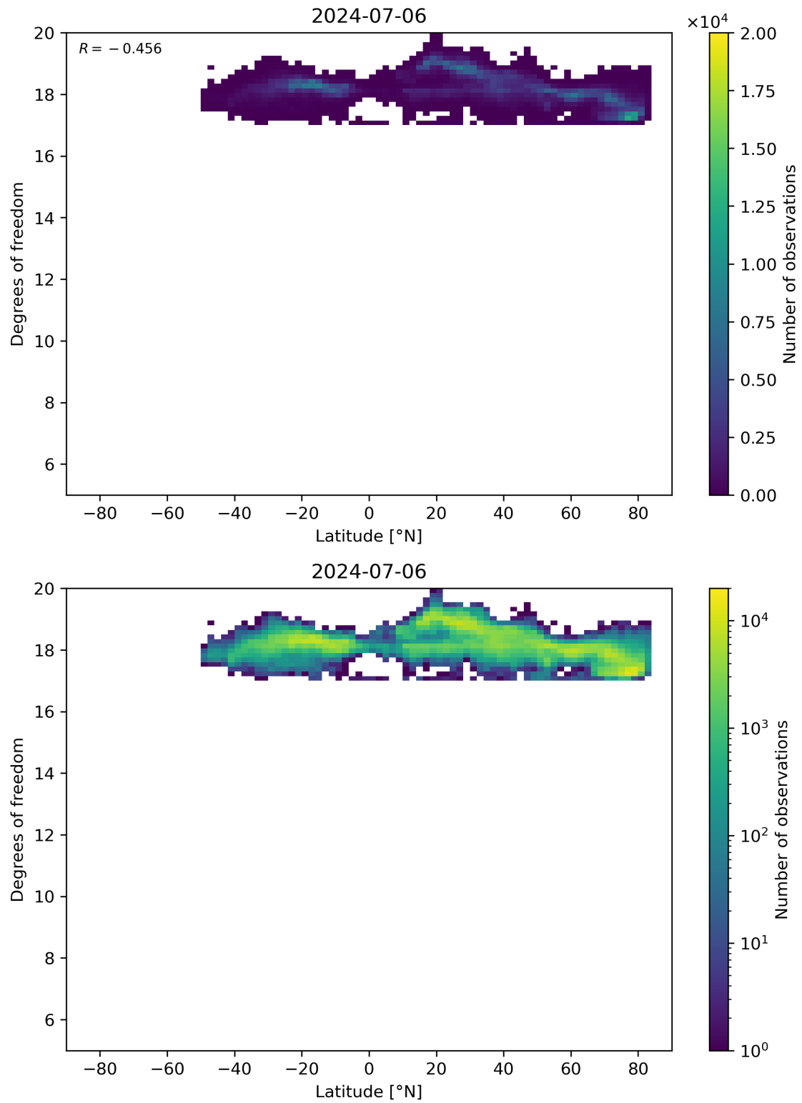
Figure 55: Scatter density plot of “Latitude” against “Degrees of freedom” for 2024-07-05 to 2024-07-07.
