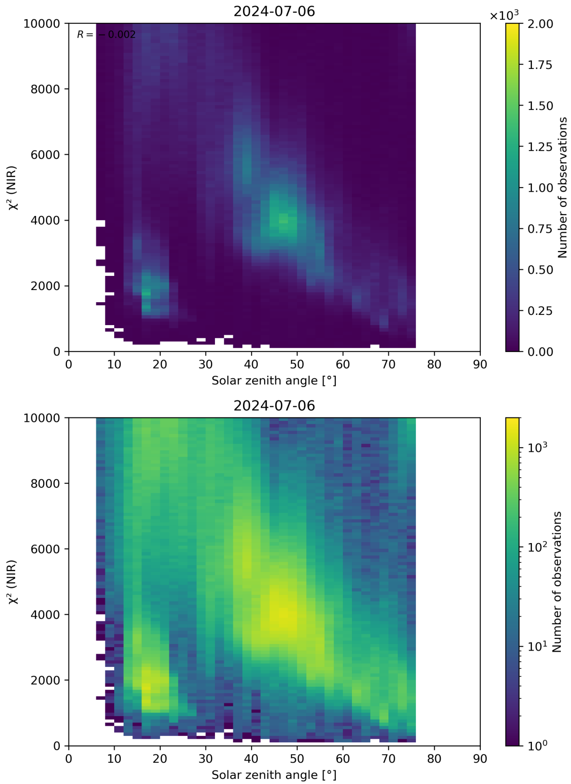
Figure 94: Scatter density plot of “Solar zenith angle” against “ \chi^2 (NIR)” for 2024-07-05 to 2024-07-07.
