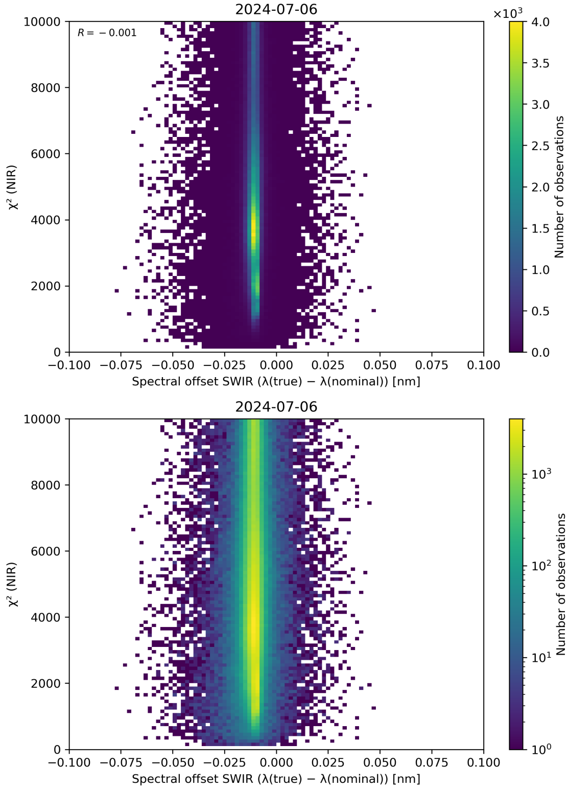
Figure 117: Scatter density plot of “Spectral offset SWIR ( \lambda(\text{true}) - \lambda(\text{nominal}) )” against “ \chi^2 (NIR)” for 2024-07-05 to 2024-07-07.
