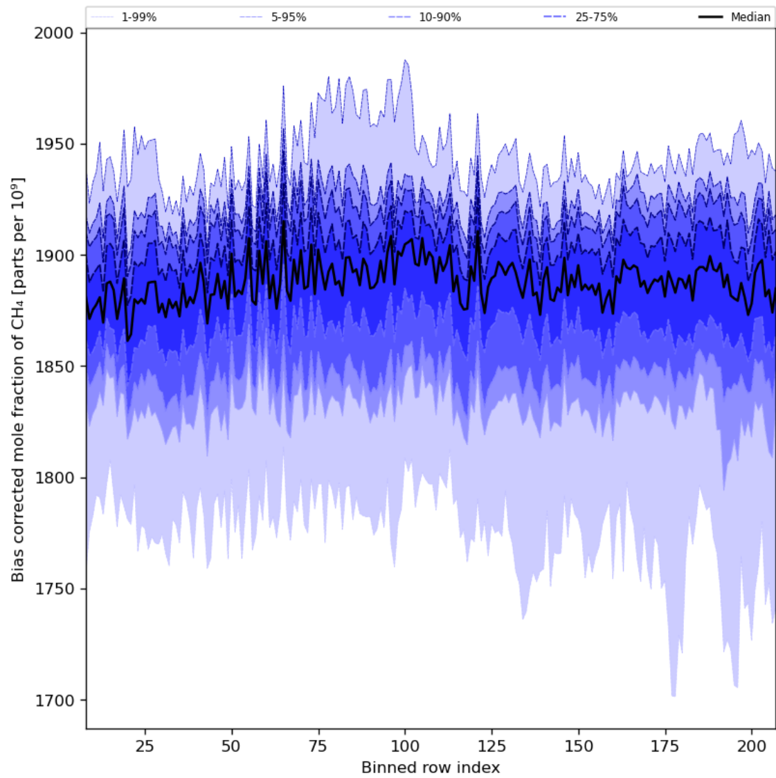
Figure 36: Along track statistics of “Bias corrected mole fraction of CH 4 ” for 2024-07-05 to 2024-07-07
