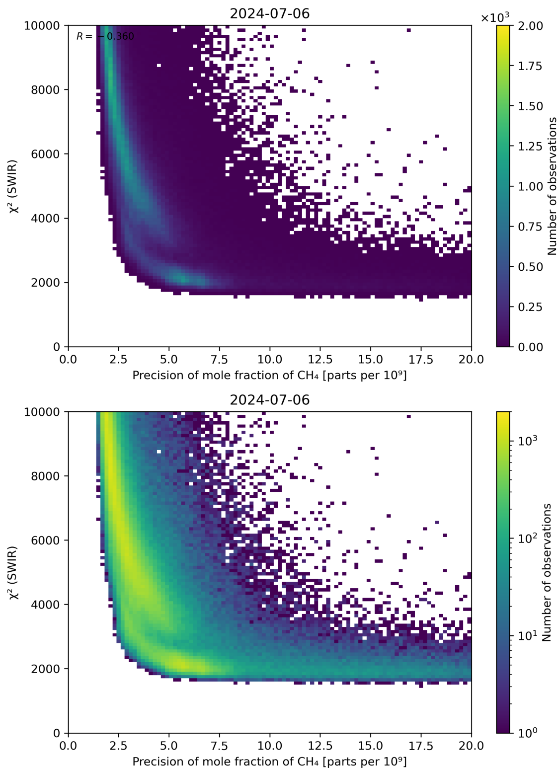
Figure 79: Scatter density plot of “Precision of mole fraction of \text{CH}_4 ” against “ \chi^2 (SWIR)” for 2024-07-05 to 2024-07-07.
