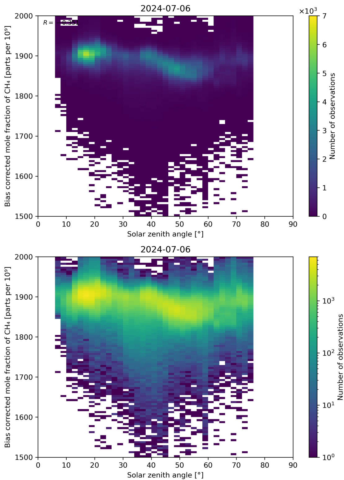
Figure 100: Scatter density plot of “Solar zenith angle” against “Bias corrected mole fraction of CH 4 ” for 2024-07-05 to 2024-07-07.
