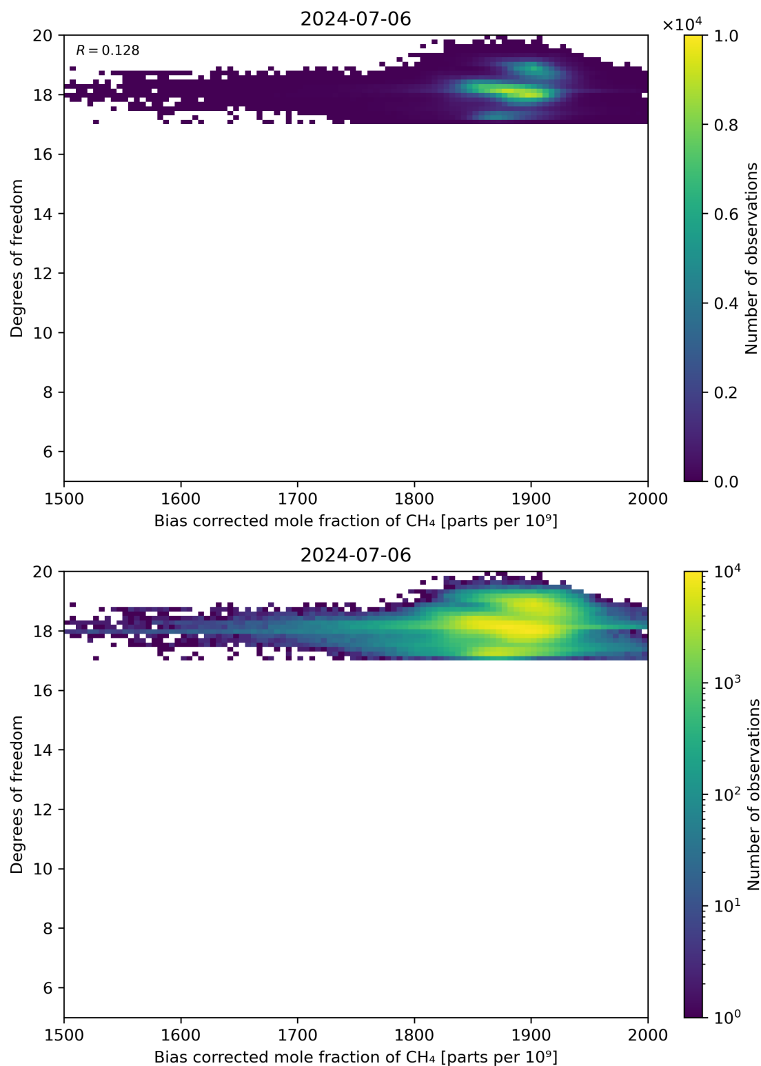
Figure 65: Scatter density plot of “Bias corrected mole fraction of \text{CH}_4 ” against “Degrees of freedom” for 2024-07-05 to 2024-07-07.
