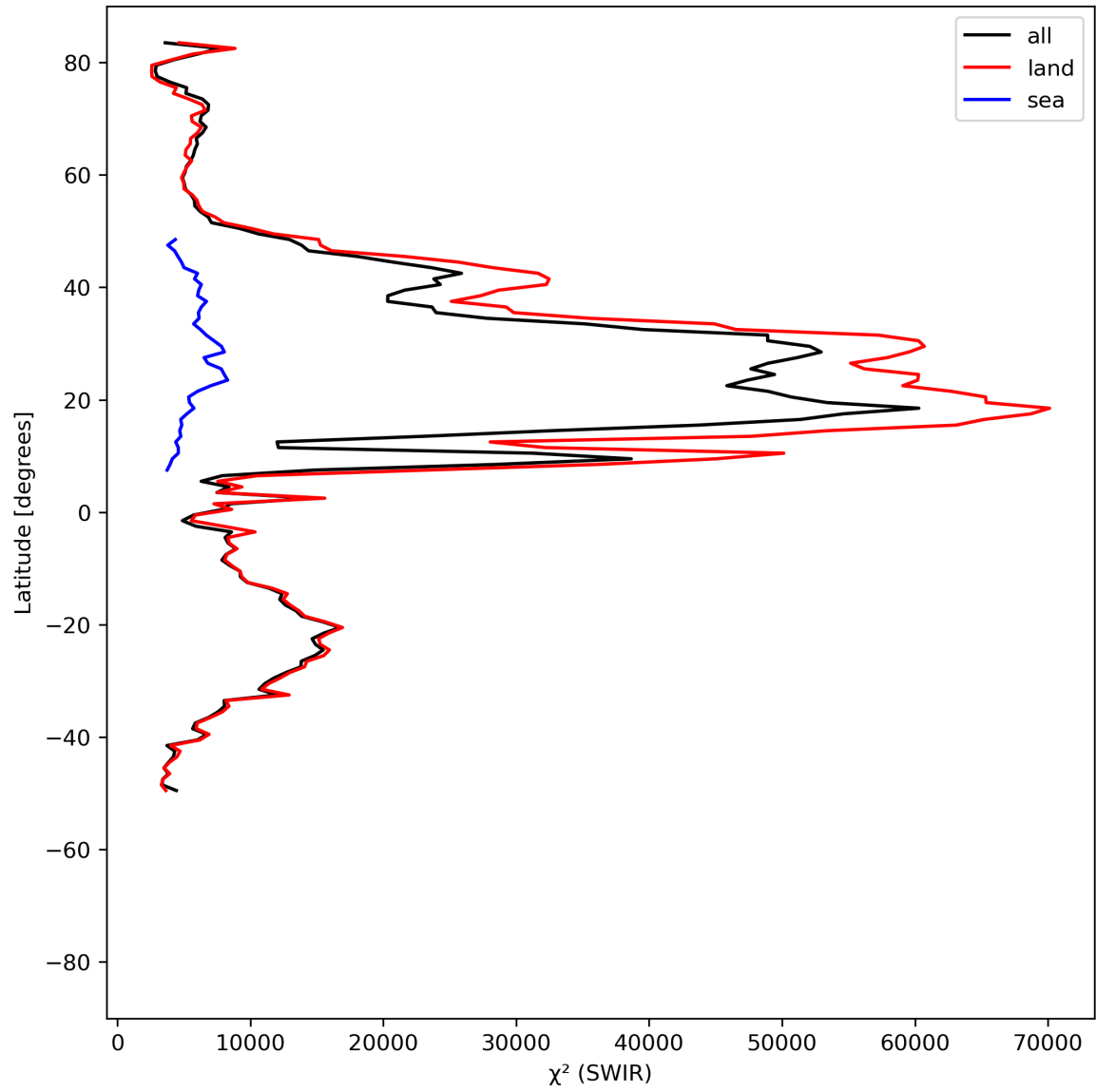
Figure 17: Zonal average of “ \chi^2 (SWIR)” for 2024-07-05 to 2024-07-07.
