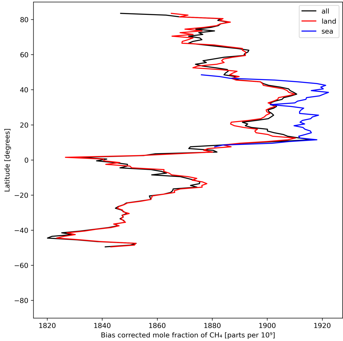
Figure 14: Zonal average of “Bias corrected mole fraction of CH 4 ” for 2024-07-05 to 2024-07-07.
