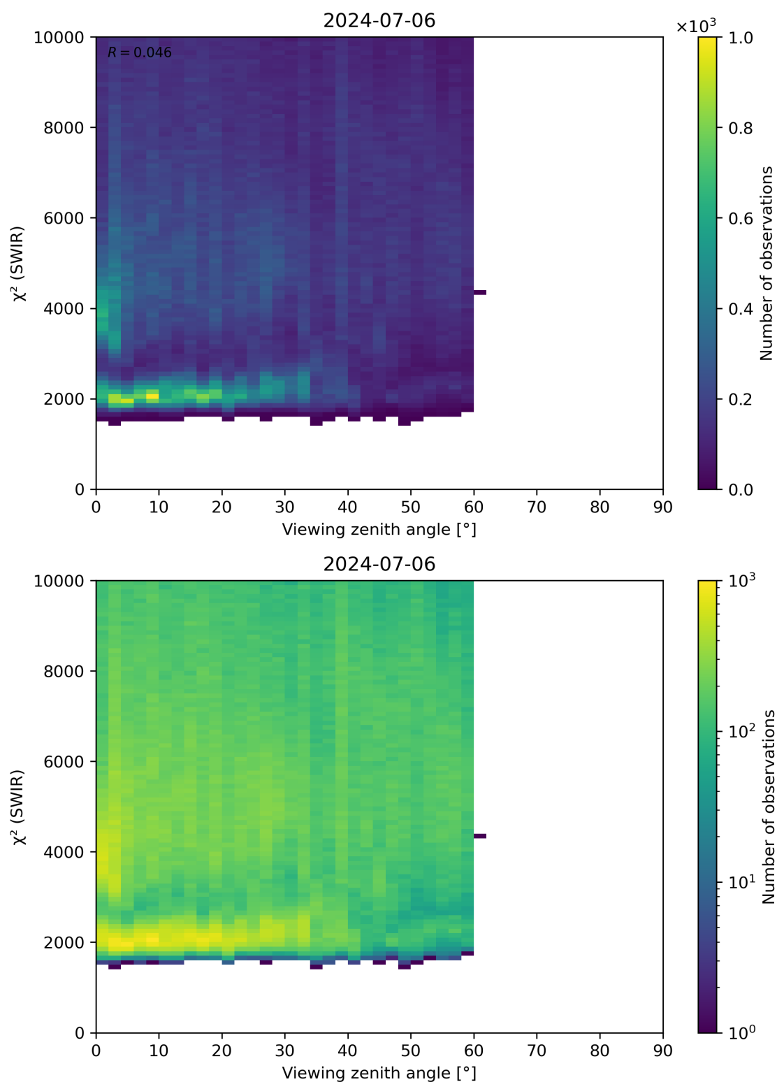
Figure 106: Scatter density plot of “Viewing zenith angle” against “ \chi^2 (SWIR)” for 2024-07-05 to 2024-07-07.
