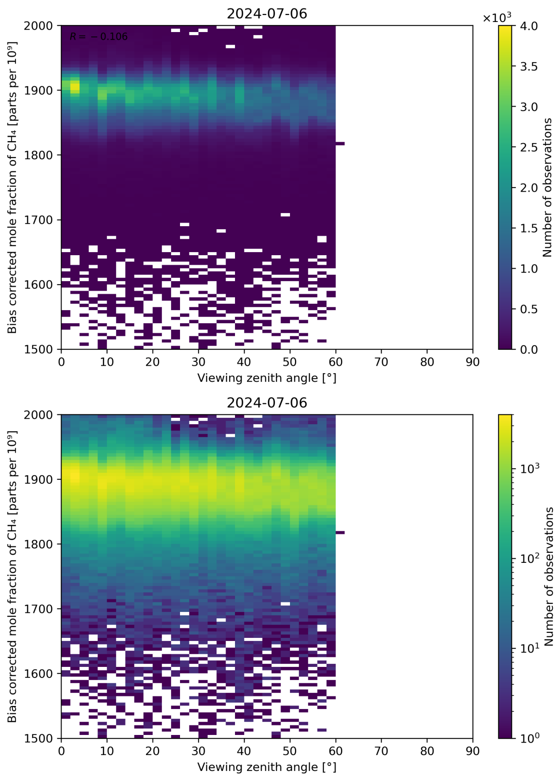
Figure 111: Scatter density plot of “Viewing zenith angle” against “Bias corrected mole fraction of CH 4 ” for 2024-07-05 to 2024-07-07.
