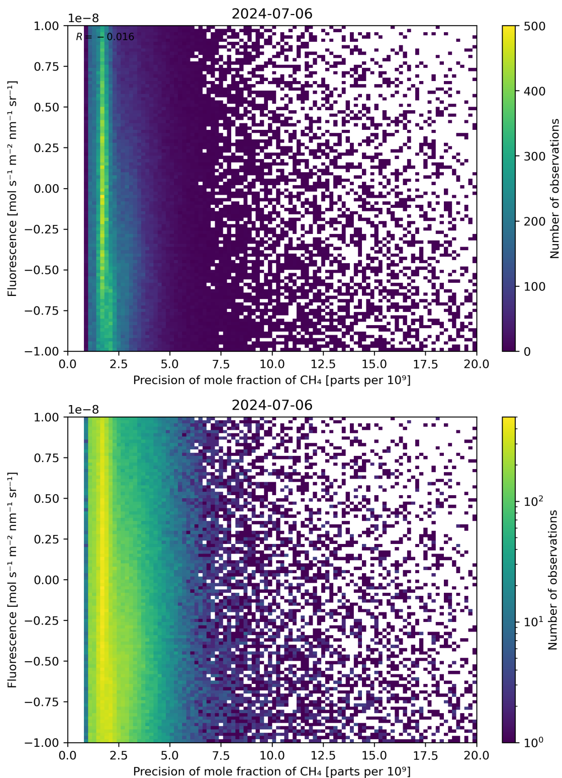
Figure 81: Scatter density plot of “Precision of mole fraction of \text{CH}_4 ” against “Fluorescence” for 2024-07-05 to 2024-07-07.
