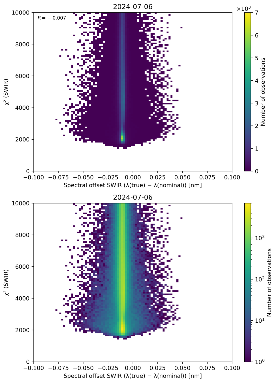
Figure 118: Scatter density plot of “Spectral offset SWIR ( \lambda(\text{true}) - \lambda(\text{nominal}) )” against “ \chi^2 (SWIR)” for 2024-07-05 to 2024-07-07.
