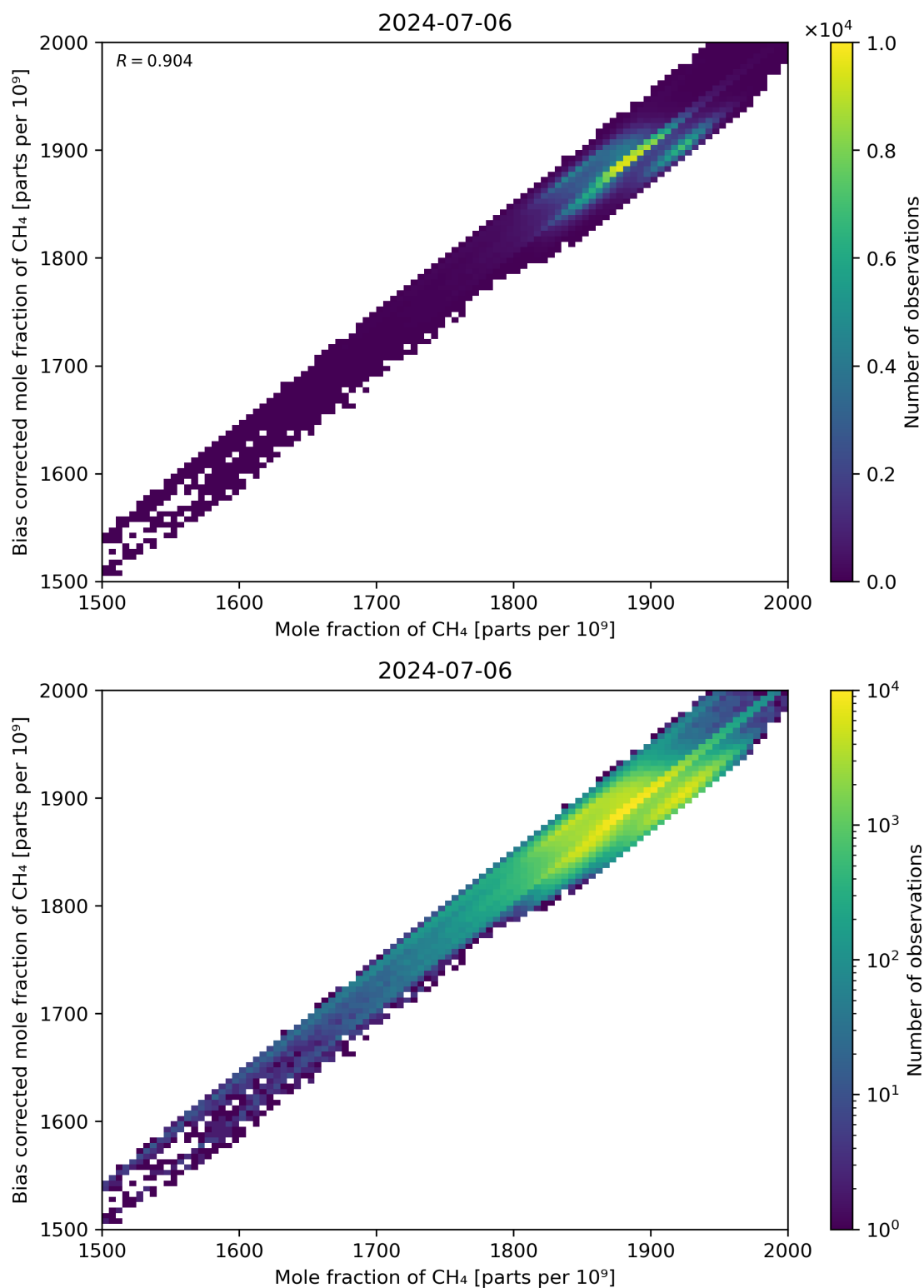
Figure 74: Scatter density plot of “Mole fraction of CH 4 ” against “Bias corrected mole fraction of CH 4 ” for 2024-07-05 to 2024-07-07.
