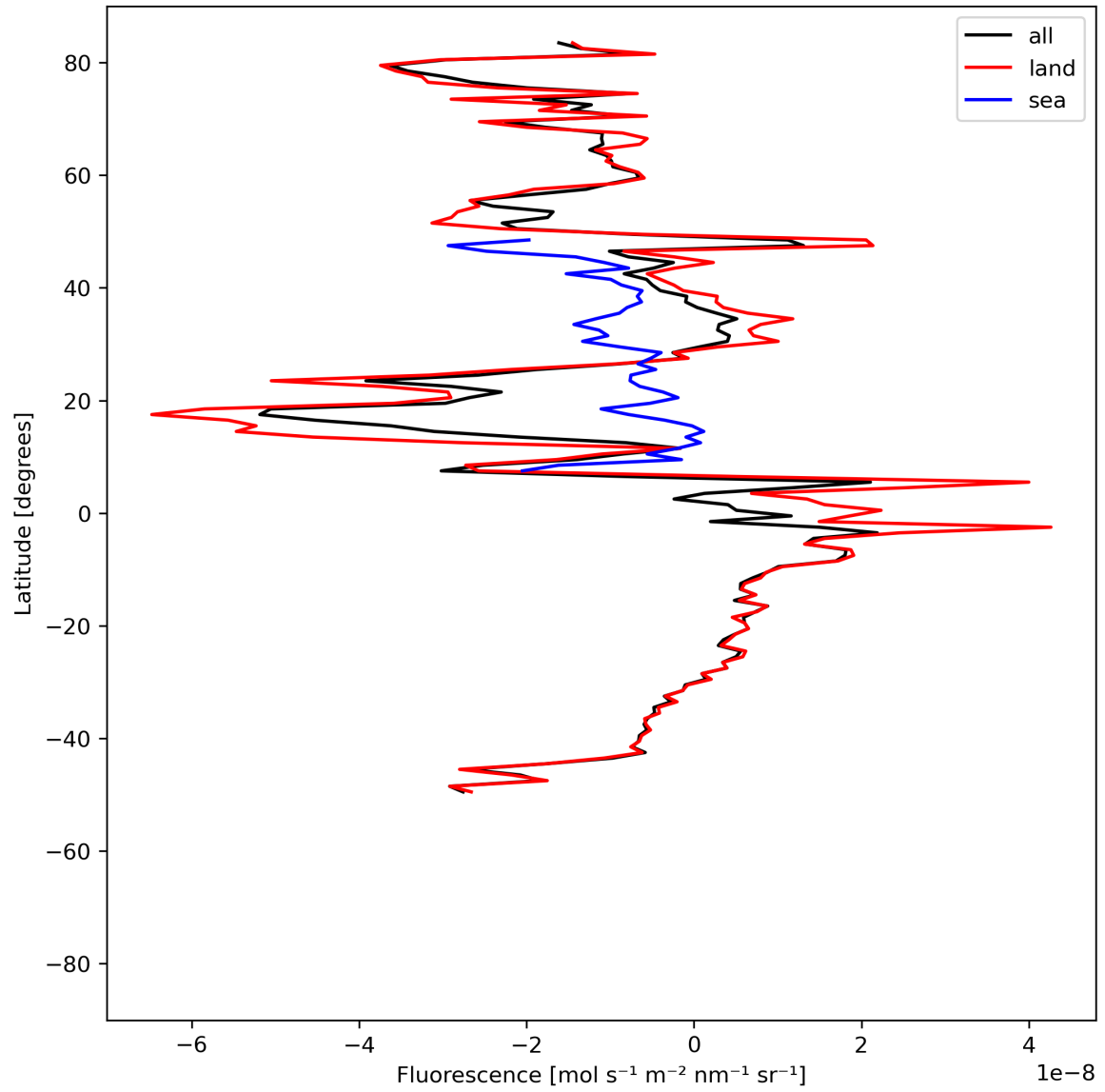
Figure 21: Zonal average of “Fluorescence” for 2024-07-05 to 2024-07-07.
