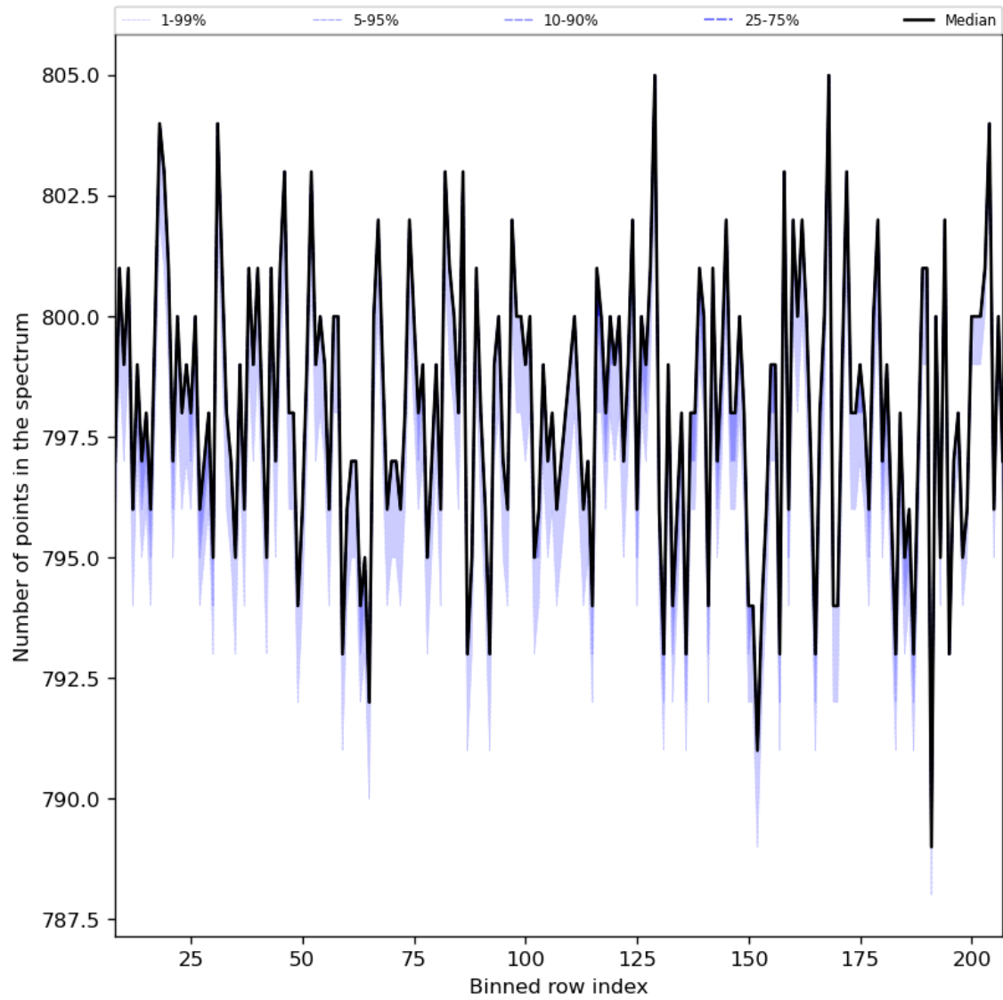
Figure 37: Along track statistics of “Number of points in the spectrum” for 2024-07-05 to 2024-07-07
