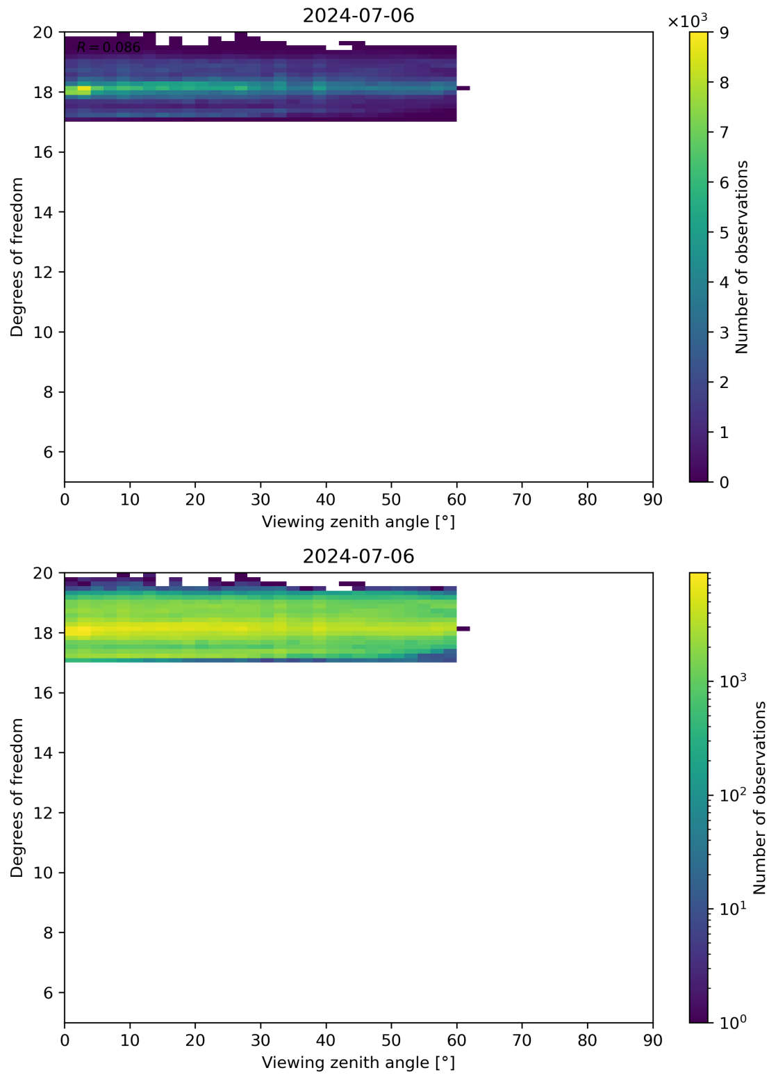
Figure 107: Scatter density plot of “Viewing zenith angle” against “Degrees of freedom” for 2024-07-05 to 2024-07-07.
