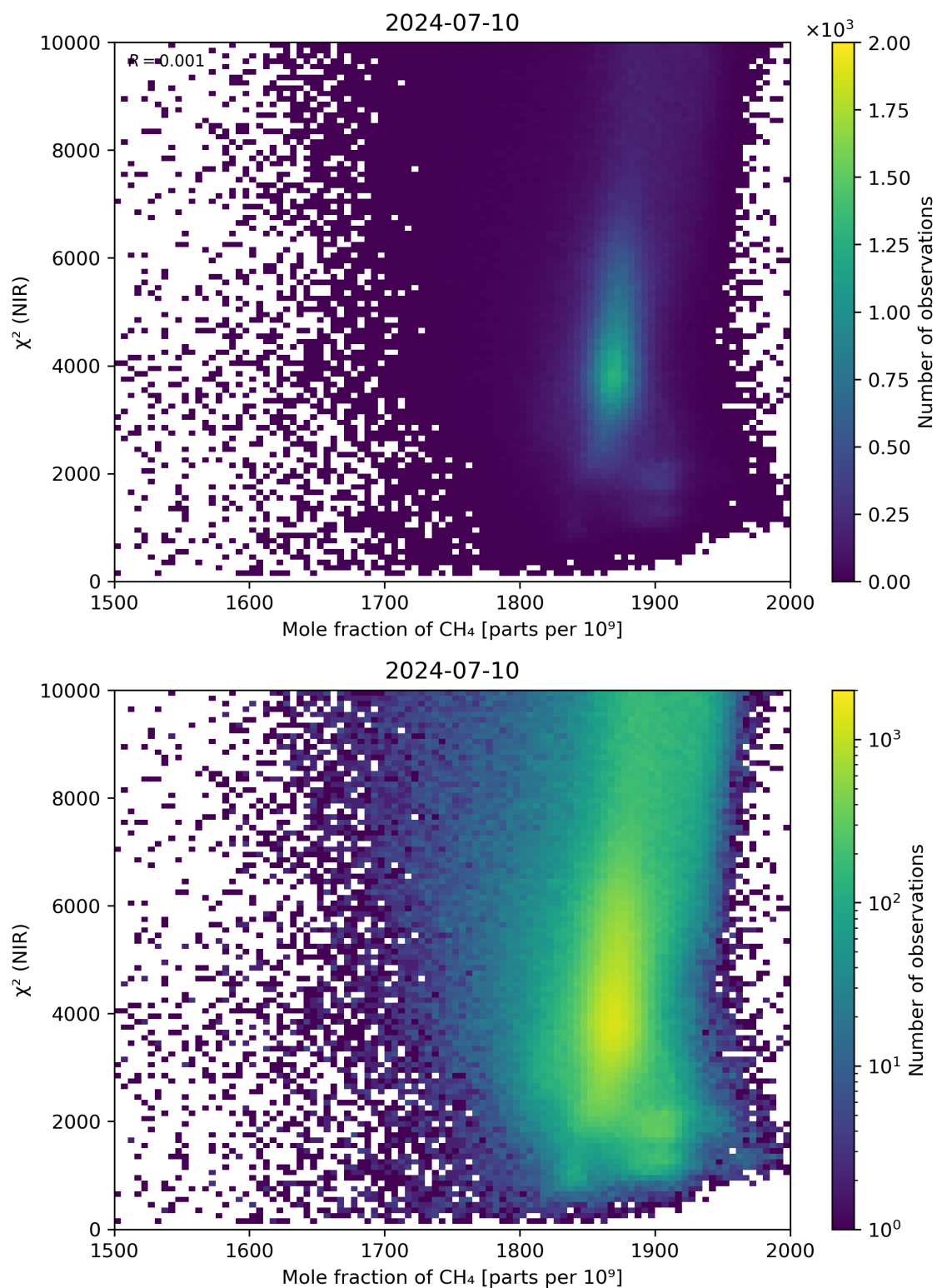
Figure 70: Scatter density plot of “Mole fraction of \text{CH}_4 ” against “ \chi^2 (NIR)” for 2024-07-10 to 2024-07-11.
