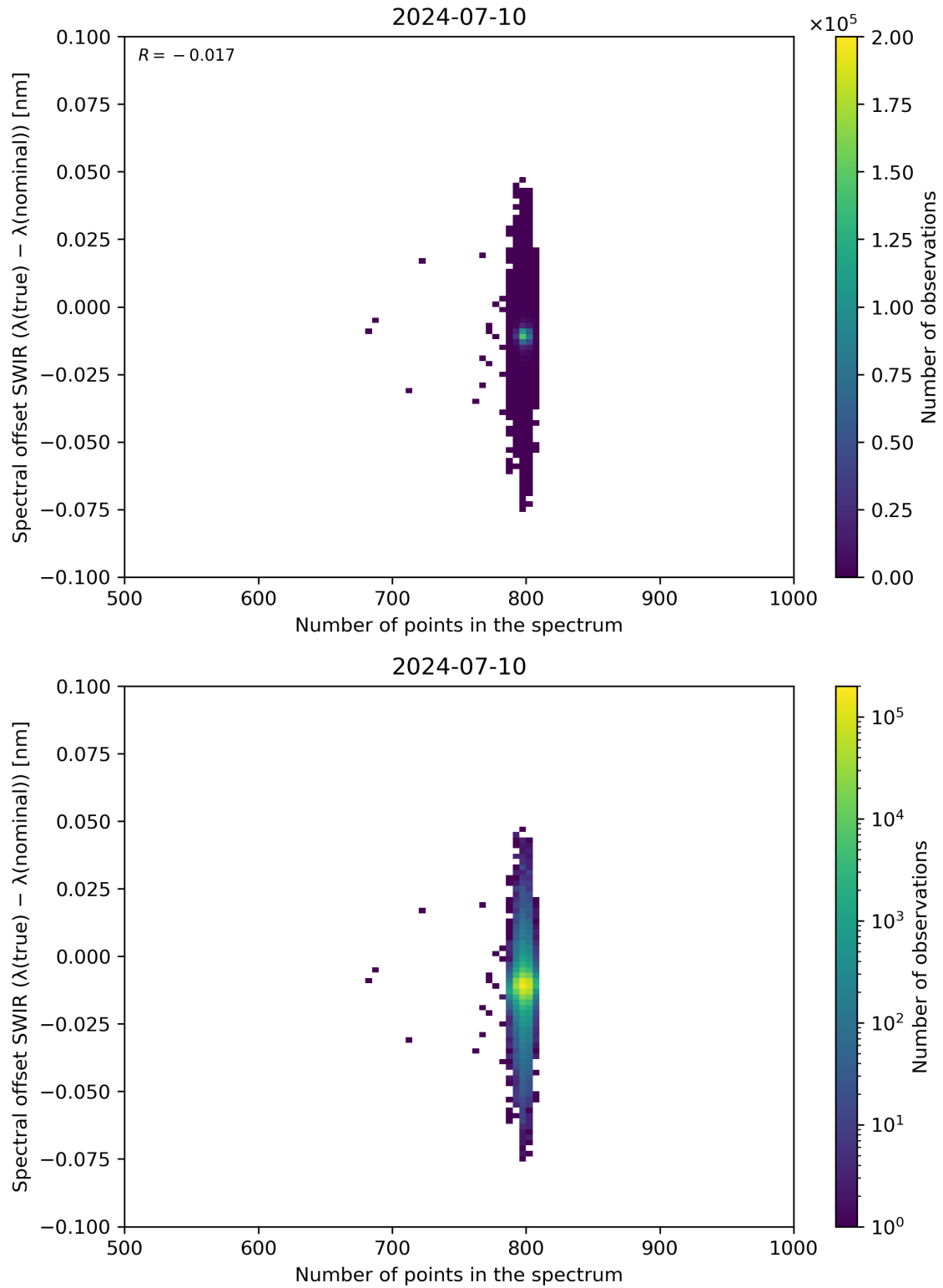
Figure 93: Scatter density plot of “Number of points in the spectrum” against “Spectral offset SWIR ( \lambda(\text{true}) - \lambda(\text{nominal}) )” for 2024-07-10 to 2024-07-11.
