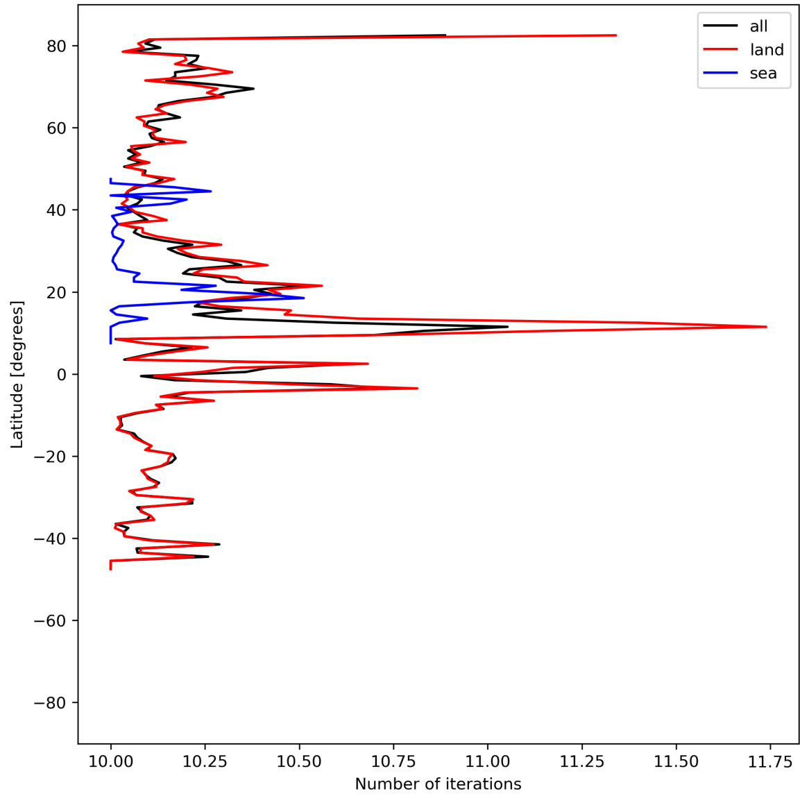
Figure 20: Zonal average of “Number of iterations” for 2024-07-10 to 2024-07-11.
