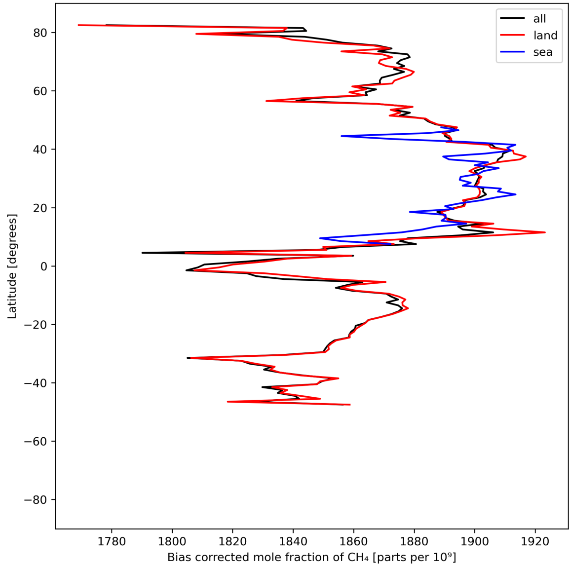
Figure 14: Zonal average of “Bias corrected mole fraction of CH 4 ” for 2024-07-10 to 2024-07-11.
