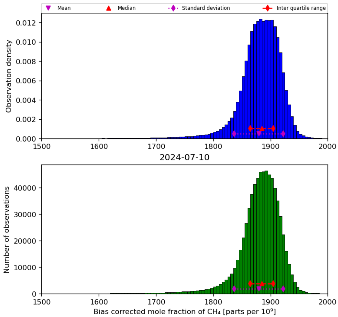
Figure 25: Histogram of “Bias corrected mole fraction of CH 4 ” for 2024-07-10 to 2024-07-11
