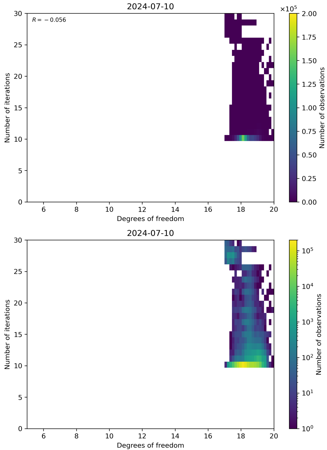
Figure 52: Scatter density plot of “Degrees of freedom” against “Number of iterations” for 2024-07-10 to 2024-07-11.
