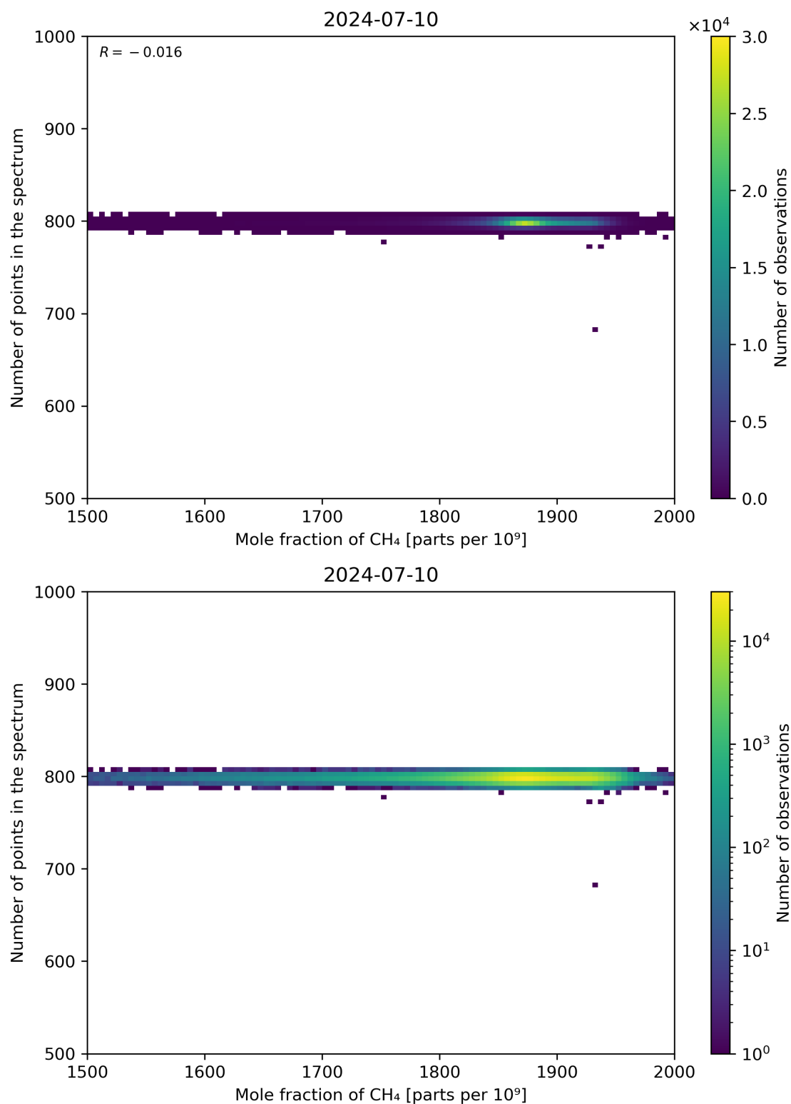
Figure 77: Scatter density plot of “Mole fraction of CH 4 ” against “Number of points in the spectrum” for 2024-07-10 to 2024-07-11.
