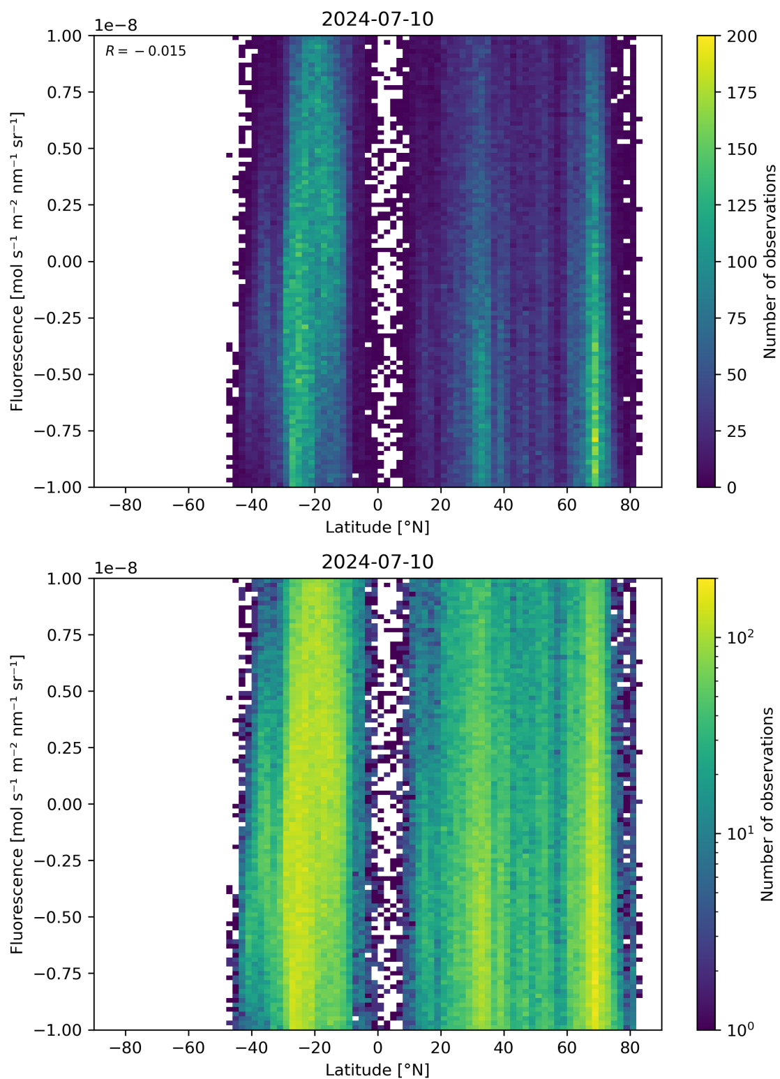
Figure 56: Scatter density plot of “Latitude” against “Fluorescence” for 2024-07-10 to 2024-07-11.
