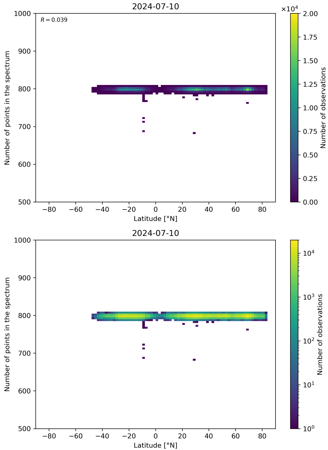
Figure 61: Scatter density plot of “Latitude” against “Number of points in the spectrum” for 2024-07-10 to 2024-07-11.
