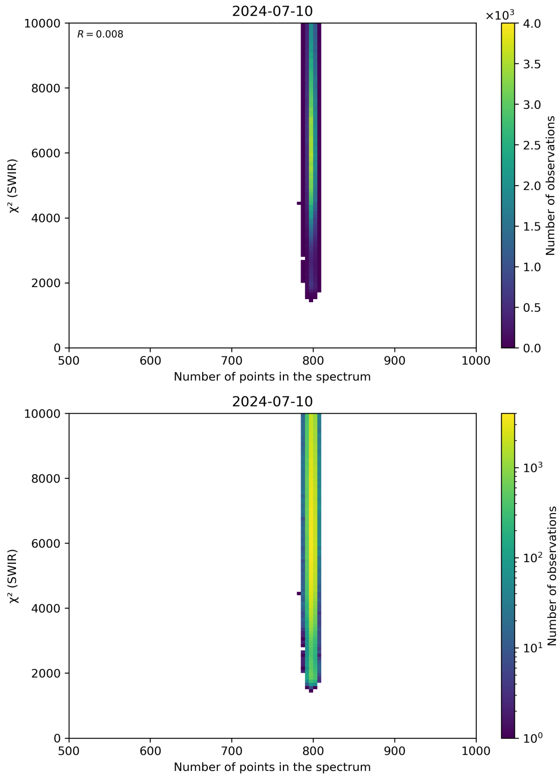
Figure 89: Scatter density plot of “Number of points in the spectrum” against “ \chi^2 (SWIR)” for 2024-07-10 to 2024-07-11.
