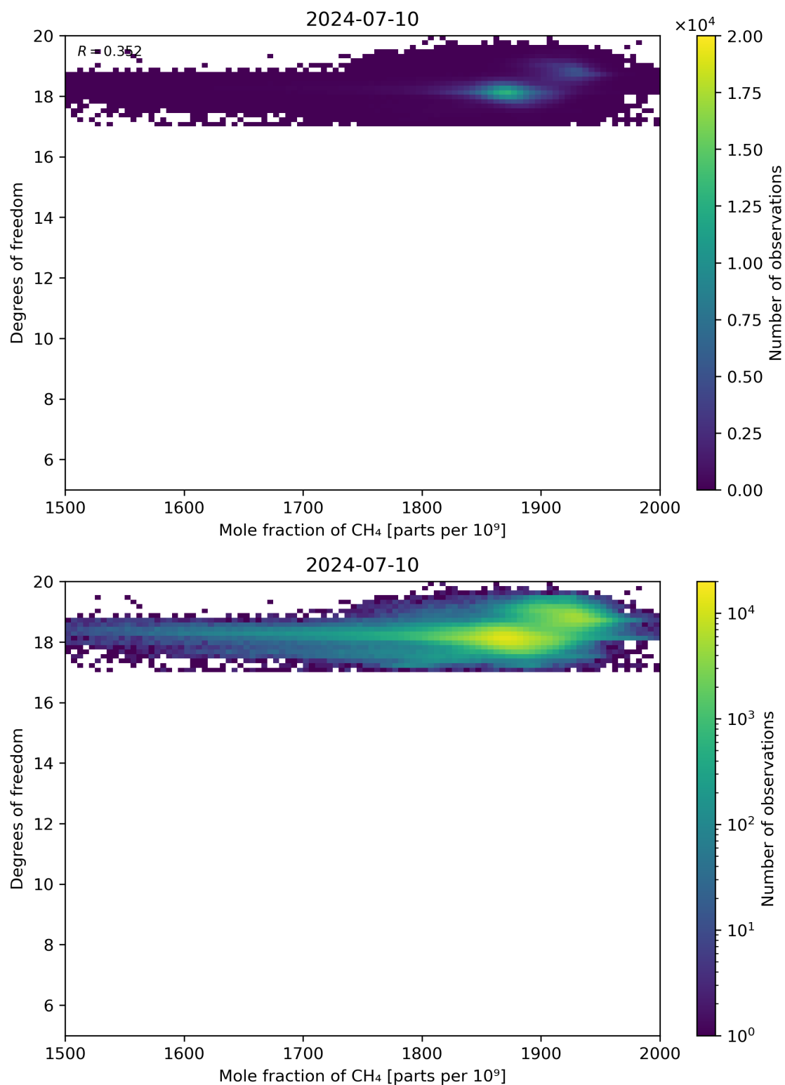
Figure 72: Scatter density plot of “Mole fraction of CH 4 ” against “Degrees of freedom” for 2024-07-10 to 2024-07-11.
