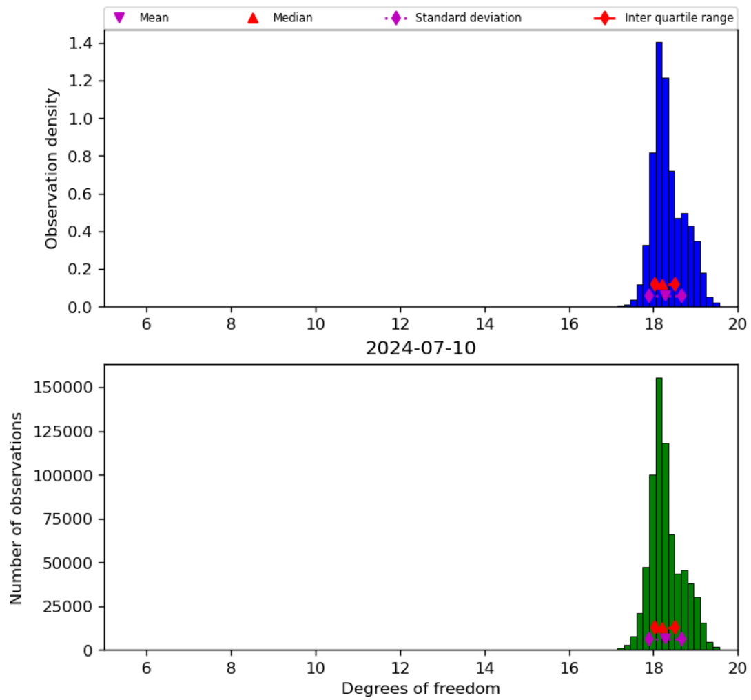
Figure 30: Histogram of “Degrees of freedom” for 2024-07-10 to 2024-07-11
