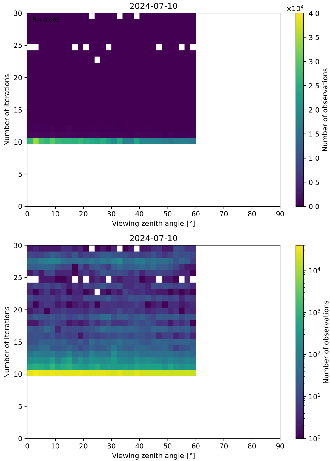
Figure 113: Scatter density plot of “Viewing zenith angle” against “Number of iterations” for 2024-07-10 to 2024-07-11.
