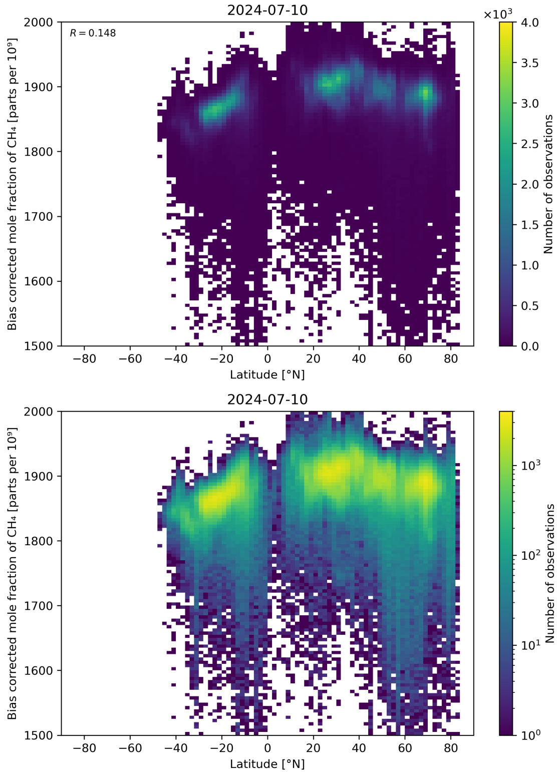
Figure 58: Scatter density plot of “Latitude” against “Bias corrected mole fraction of \text{CH}_4 ” for 2024-07-10 to 2024-07-11.
