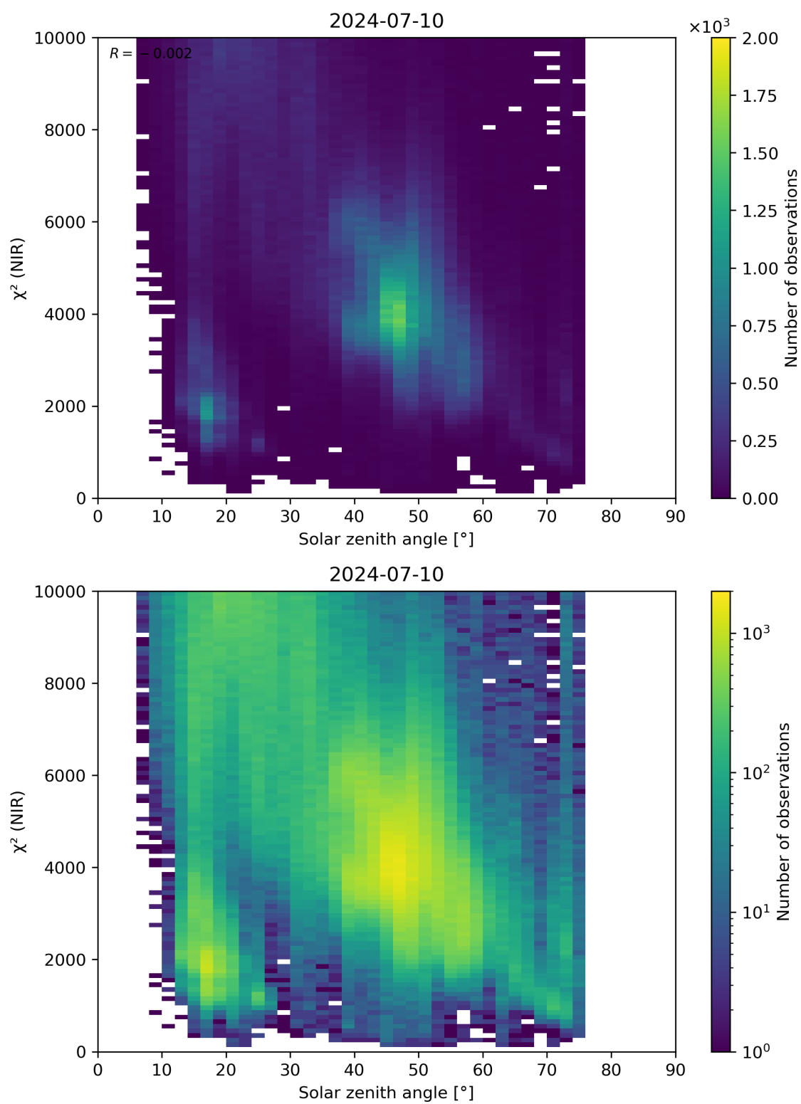
Figure 94: Scatter density plot of “Solar zenith angle” against “ \chi^2 (NIR)” for 2024-07-10 to 2024-07-11.
