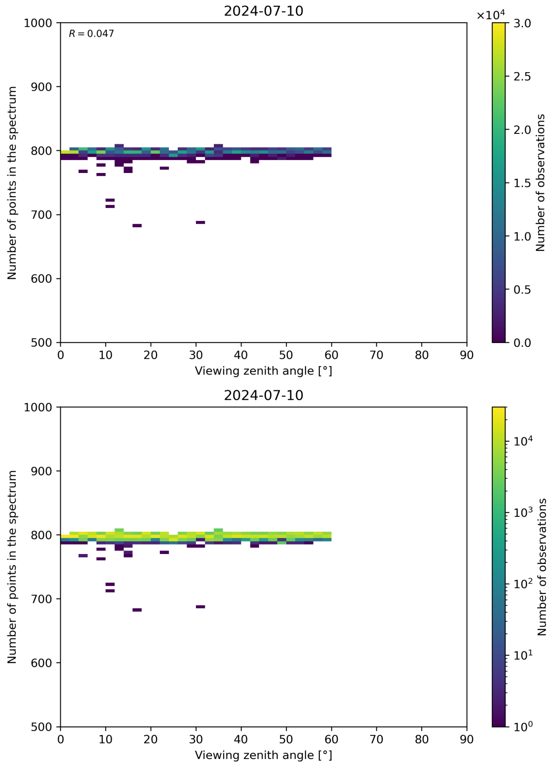
Figure 114: Scatter density plot of “Viewing zenith angle” against “Number of points in the spectrum” for 2024-07-10 to 2024-07-11.
