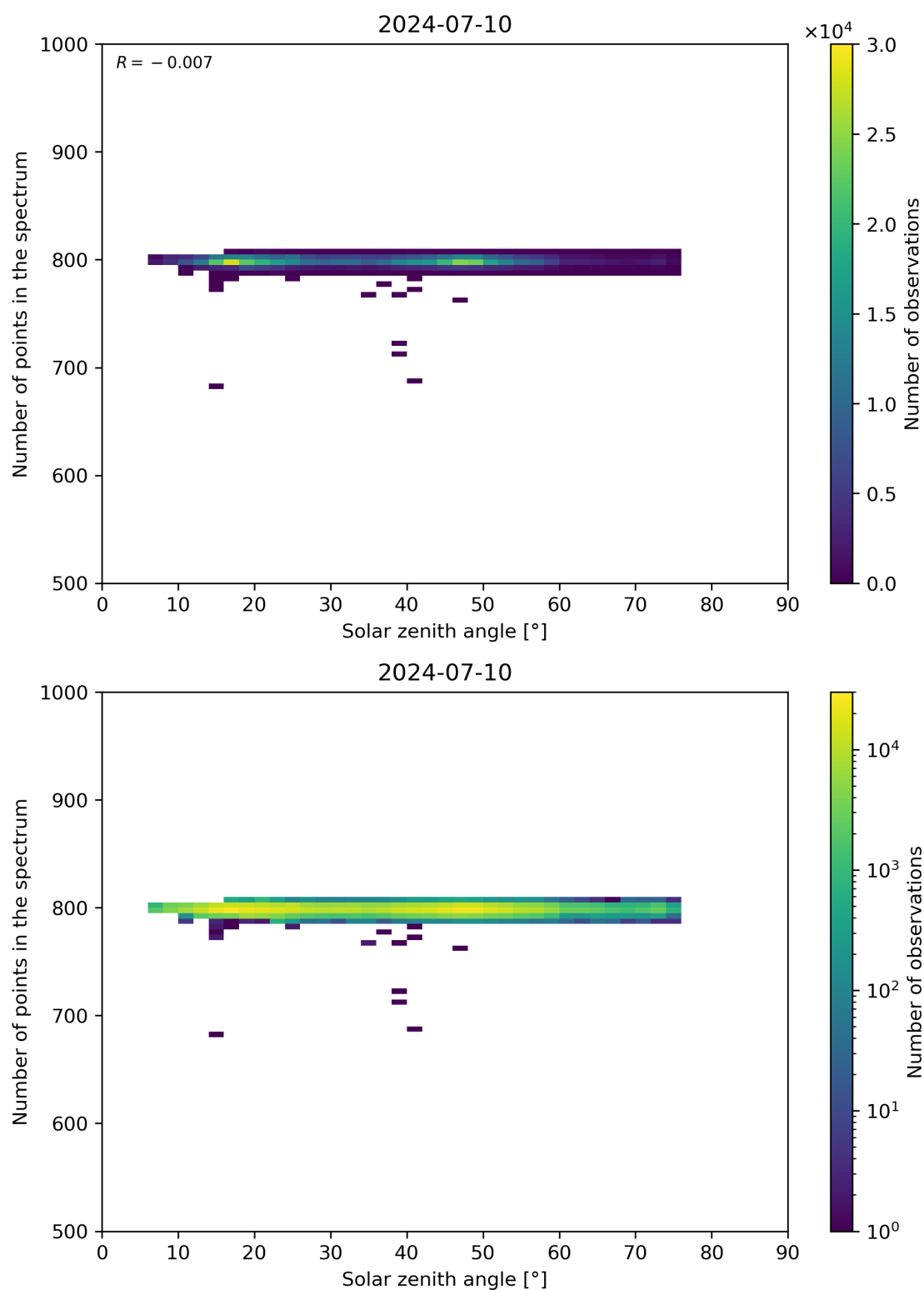
Figure 103: Scatter density plot of “Solar zenith angle” against “Number of points in the spectrum” for 2024-07-10 to 2024-07-11.
