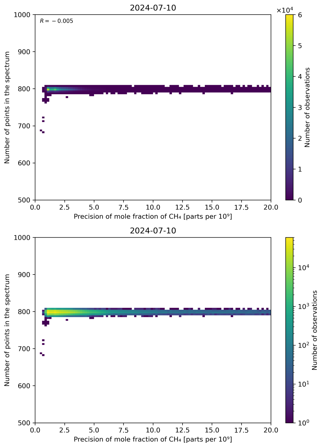
Figure 84: Scatter density plot of “Precision of mole fraction of CH 4 ” against “Number of points in the spectrum” for 2024-07-10 to 2024-07-11.
