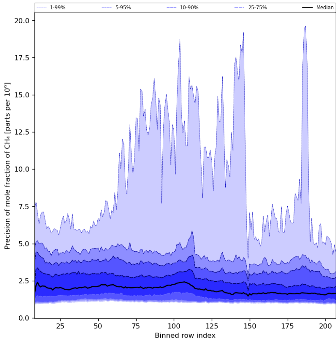
Figure 35: Along track statistics of “Precision of mole fraction of CH 4 ” for 2024-07-10 to 2024-07-11
