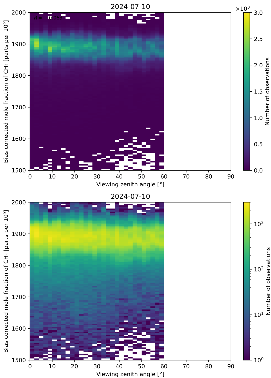
Figure 111: Scatter density plot of “Viewing zenith angle” against “Bias corrected mole fraction of CH 4 ” for 2024-07-10 to 2024-07-11.
