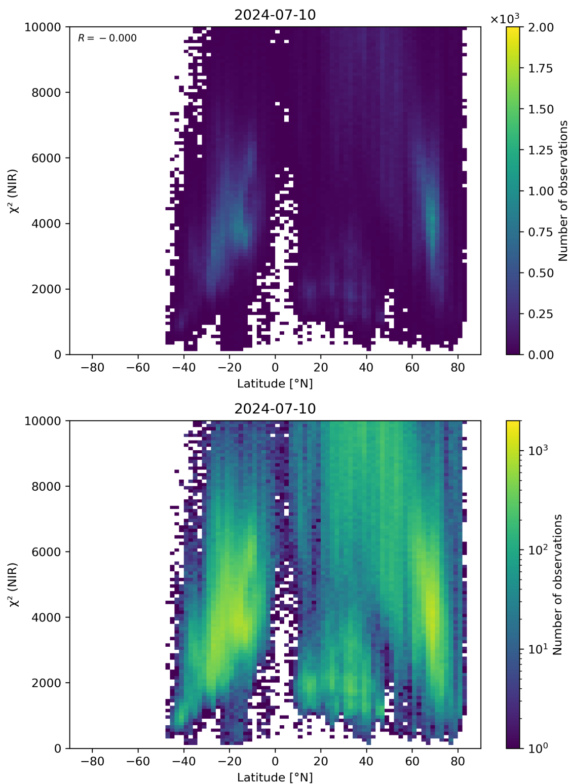
Figure 53: Scatter density plot of “Latitude” against “ \chi^2 (NIR)” for 2024-07-10 to 2024-07-11.
