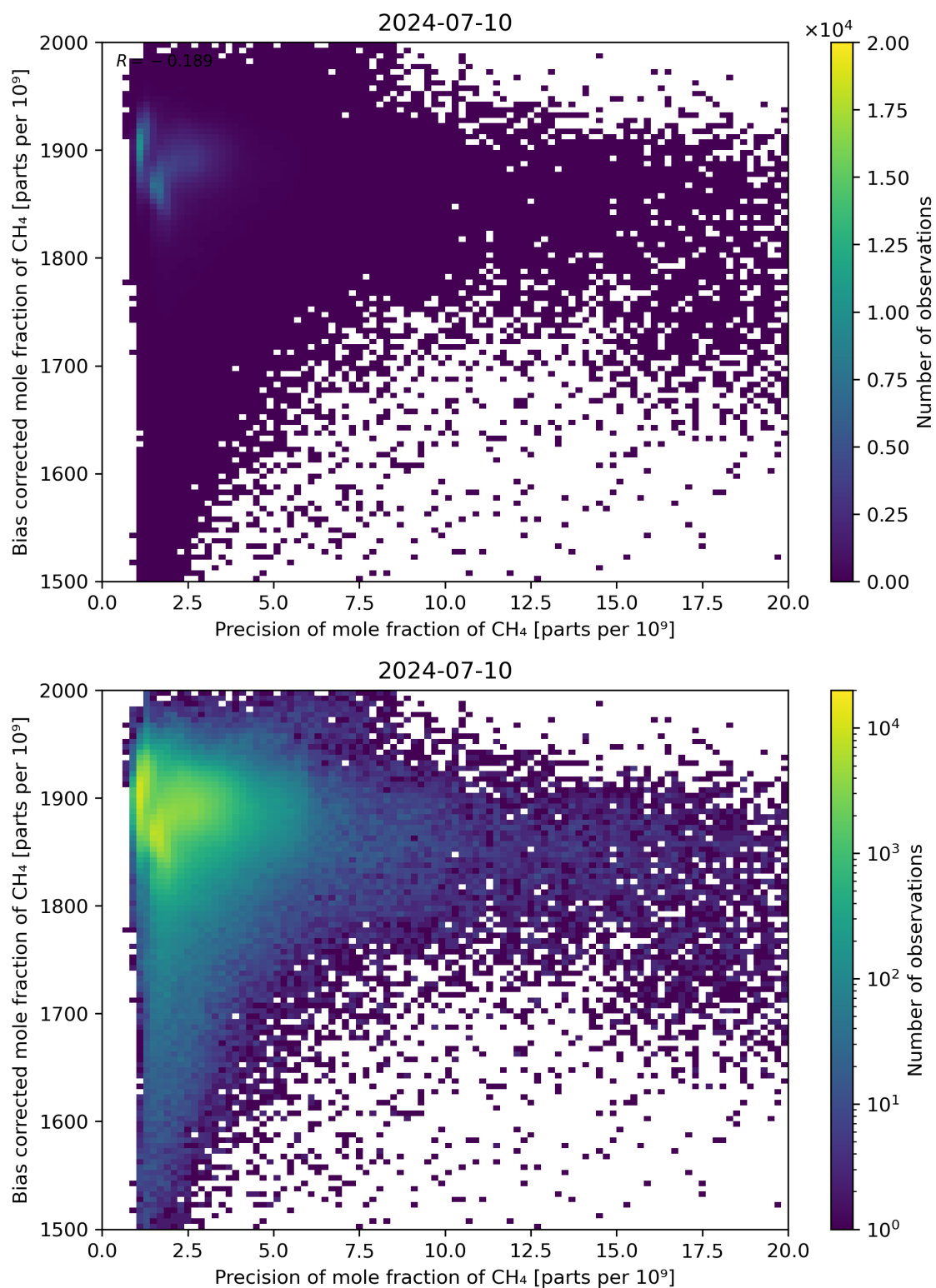
Figure 82: Scatter density plot of “Precision of mole fraction of CH 4 ” against “Bias corrected mole fraction of CH 4 ” for 2024-07-10 to 2024-07-11.
