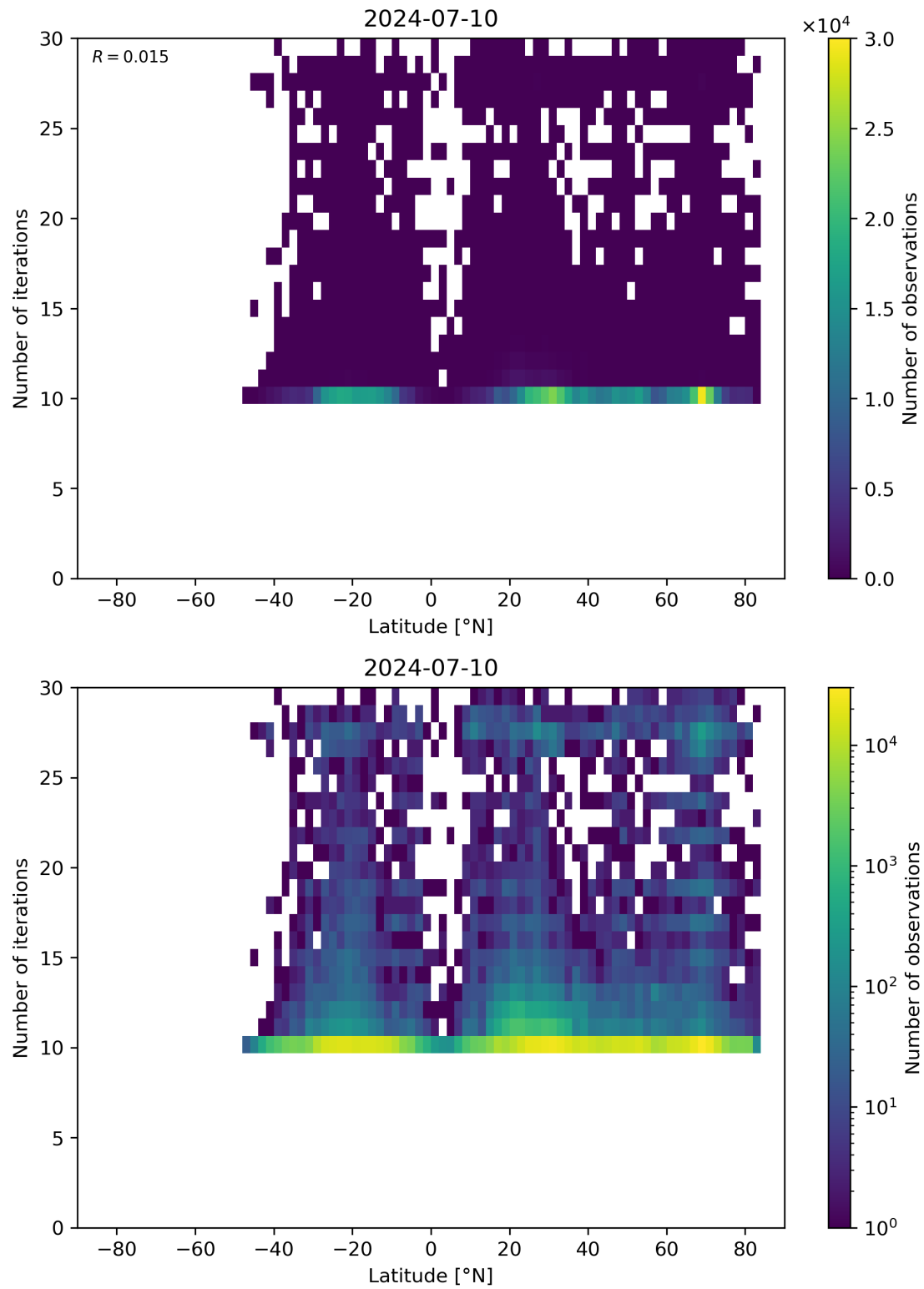
Figure 60: Scatter density plot of “Latitude” against “Number of iterations” for 2024-07-10 to 2024-07-11.
