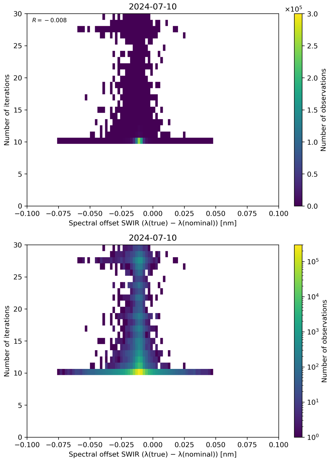
Figure 121: Scatter density plot of “Spectral offset SWIR ( \lambda(\text{true}) - \lambda(\text{nominal}) )” against “Number of iterations” for 2024-07-10 to 2024-07-11.
