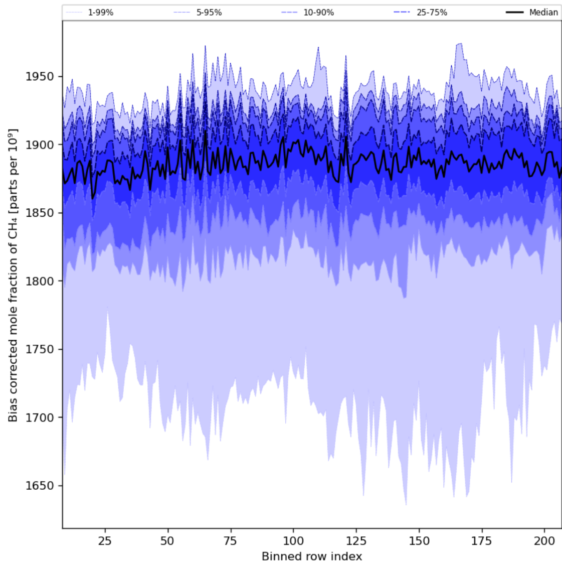
Figure 36: Along track statistics of “Bias corrected mole fraction of \text{CH}_4 ” for 2024-07-10 to 2024-07-11
