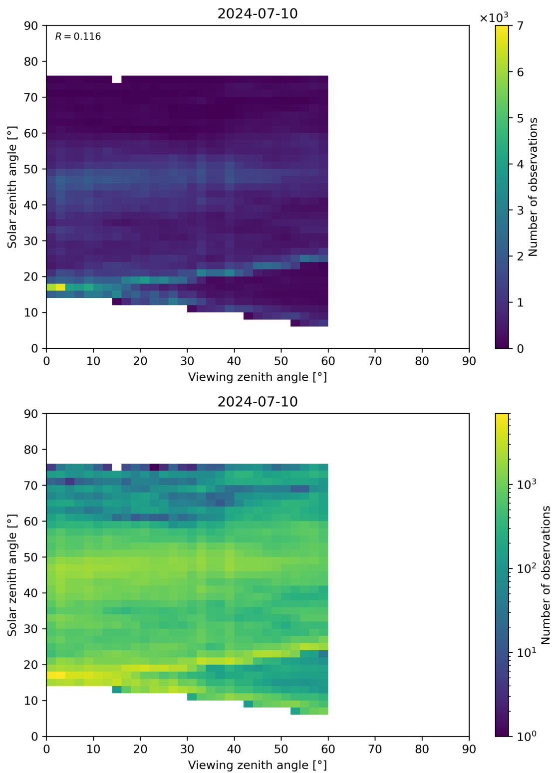
Figure 115: Scatter density plot of “Viewing zenith angle” against “Solar zenith angle” for 2024-07-10 to 2024-07-11.
