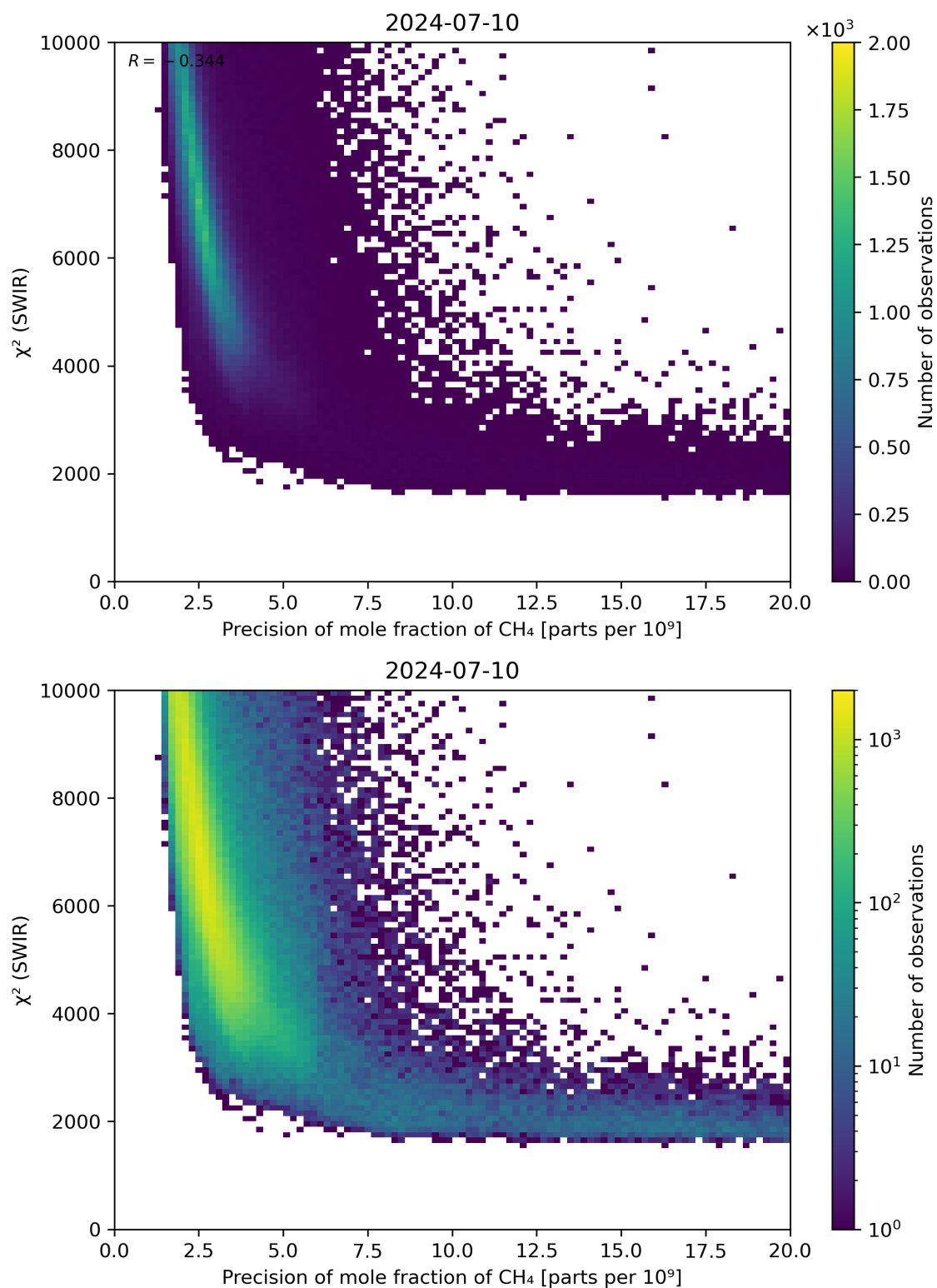
Figure 79: Scatter density plot of “Precision of mole fraction of \text{CH}_4 ” against “ \chi^2 (SWIR)” for 2024-07-10 to 2024-07-11.
