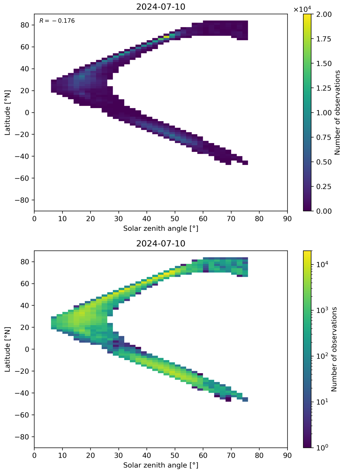
Figure 98: Scatter density plot of “Solar zenith angle” against “Latitude” for 2024-07-10 to 2024-07-11.
