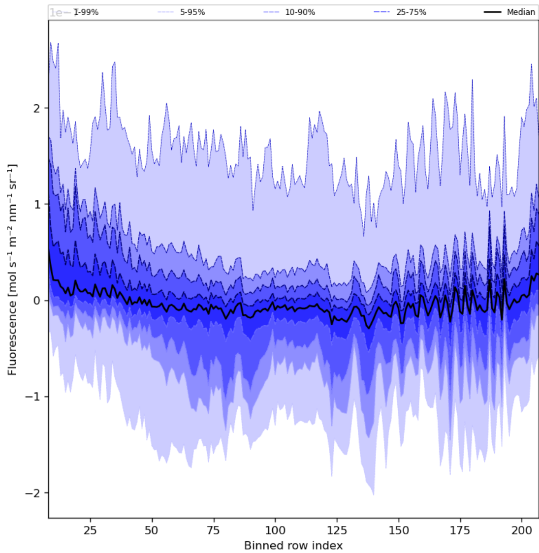
Figure 43: Along track statistics of “Fluorescence” for 2024-07-10 to 2024-07-11
