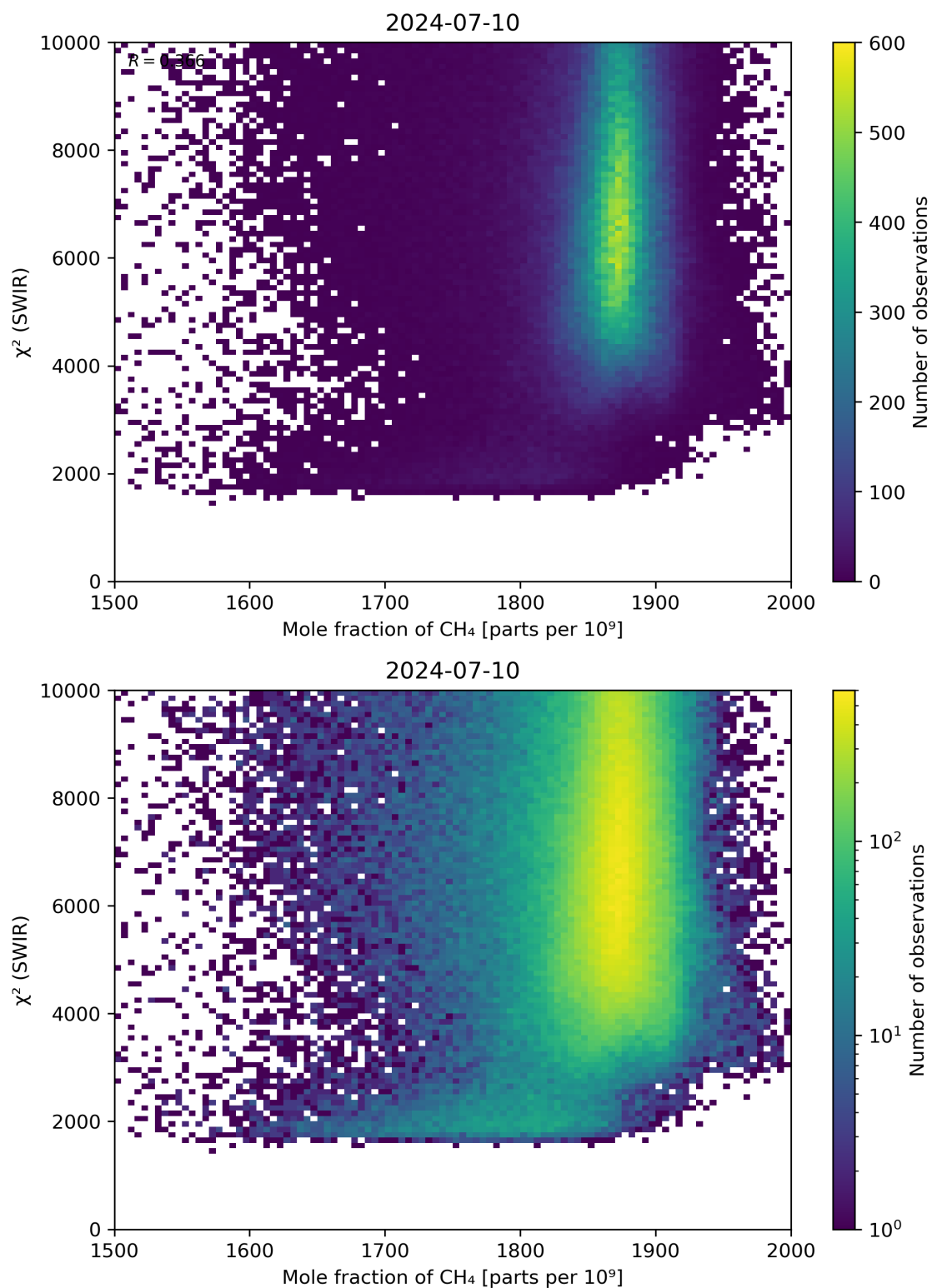
Figure 71: Scatter density plot of “Mole fraction of \text{CH}_4 ” against “ \chi^2 (SWIR)” for 2024-07-10 to 2024-07-11.
