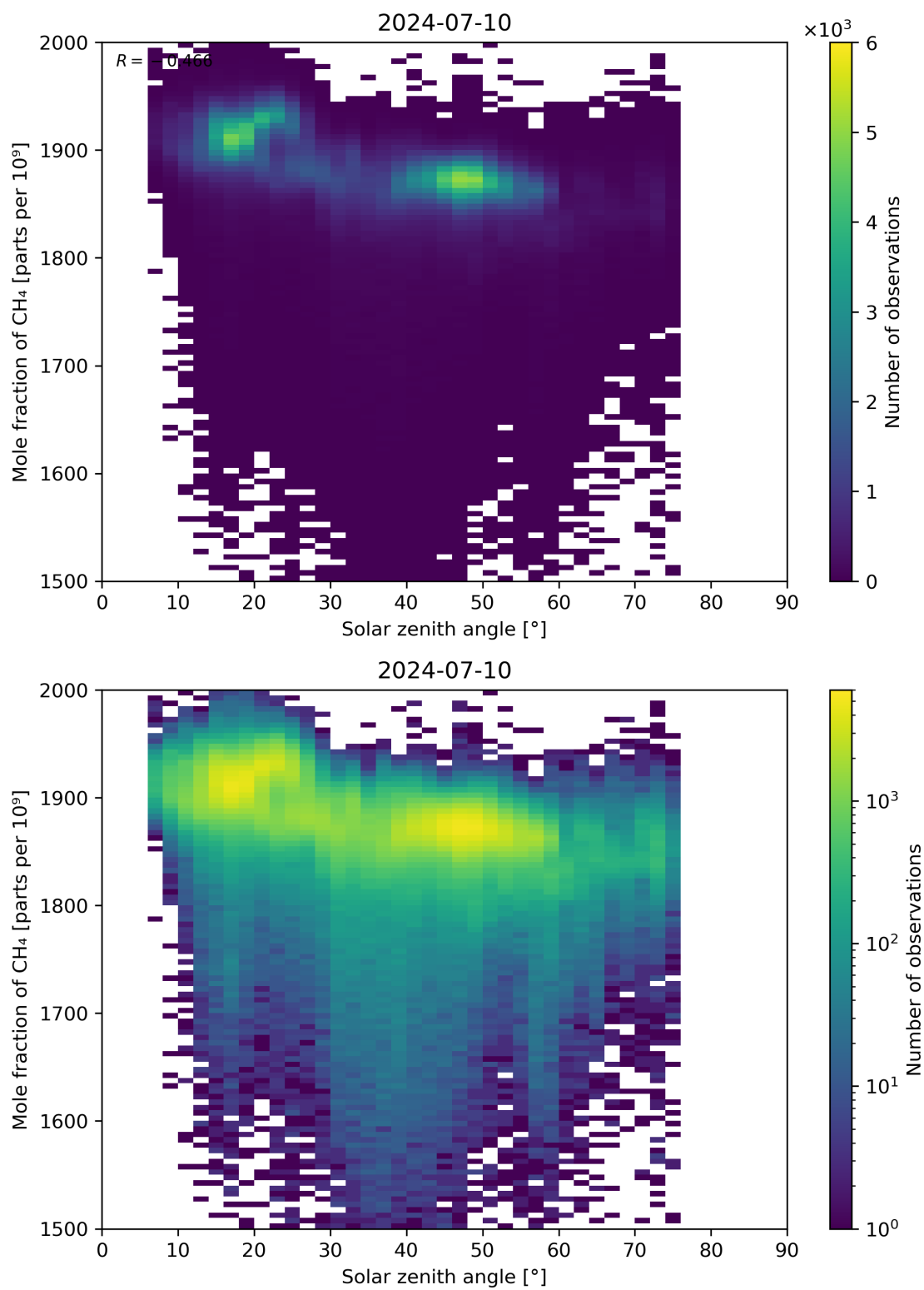
Figure 99: Scatter density plot of “Solar zenith angle” against “Mole fraction of CH 4 ” for 2024-07-10 to 2024-07-11.
