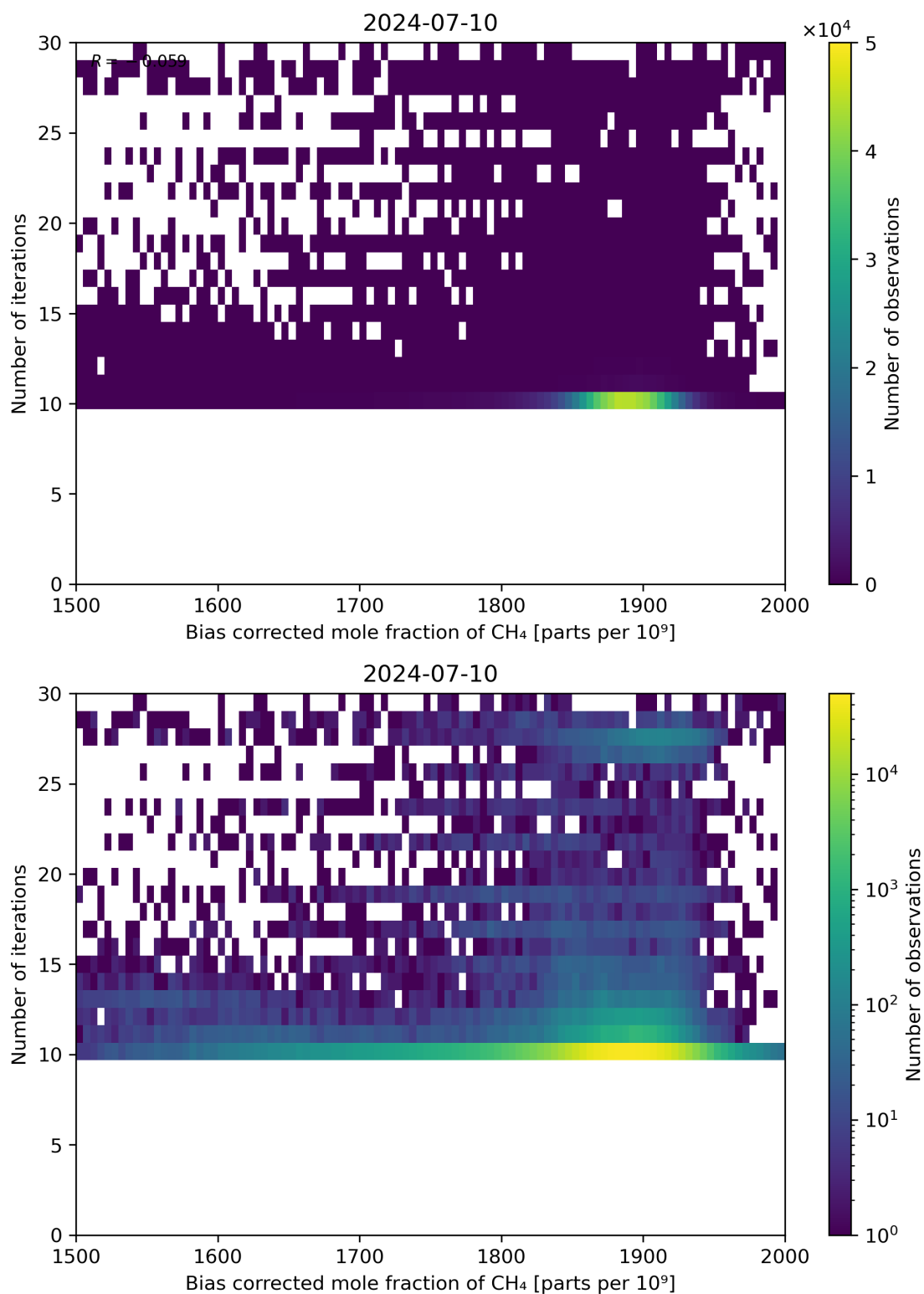
Figure 67: Scatter density plot of “Bias corrected mole fraction of \text{CH}_4 ” against “Number of iterations” for 2024-07-10 to 2024-07-11.
