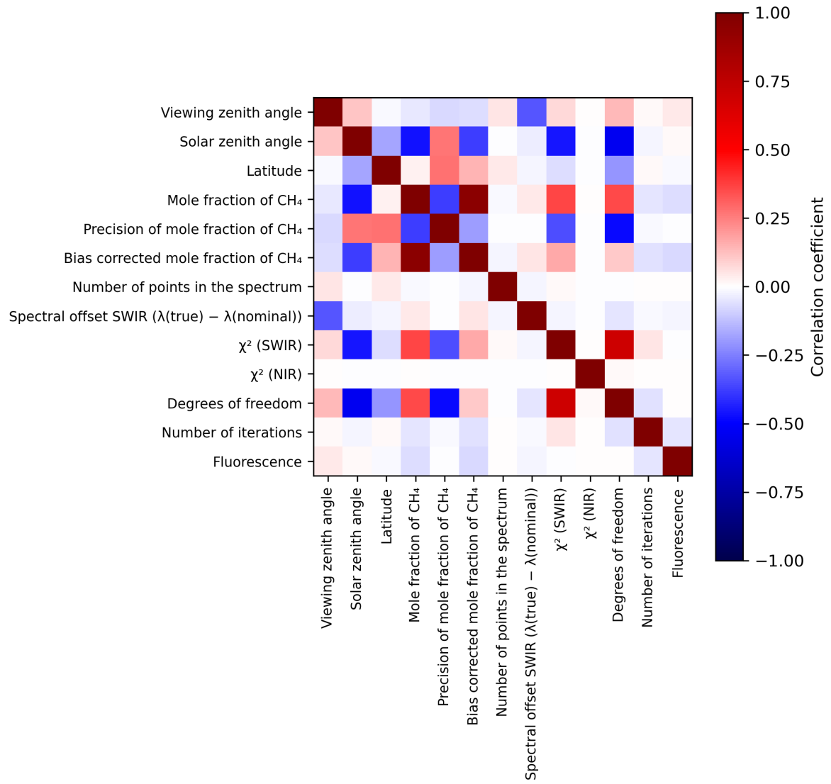
Figure 2: Map of correlation matrix for 2024-07-10 to 2024-07-11.
