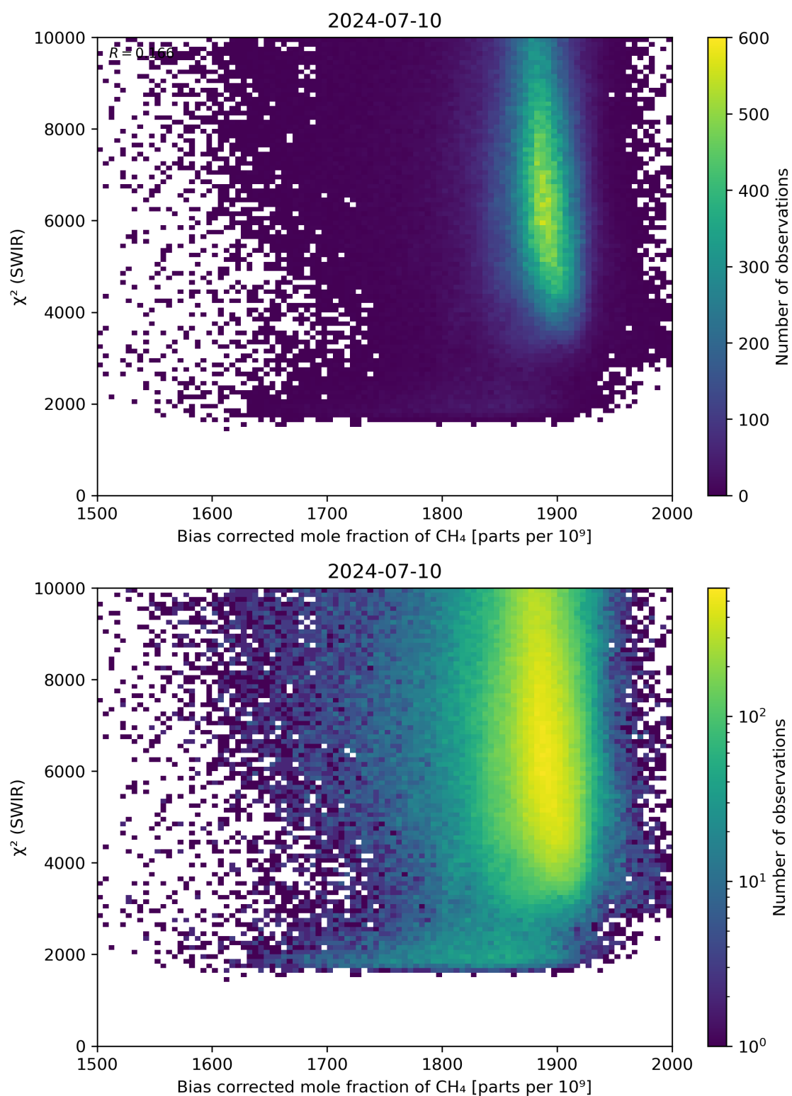
Figure 64: Scatter density plot of “Bias corrected mole fraction of CH 4 ” against “ \chi^2 (SWIR)” for 2024-07-10 to 2024-07-11.
