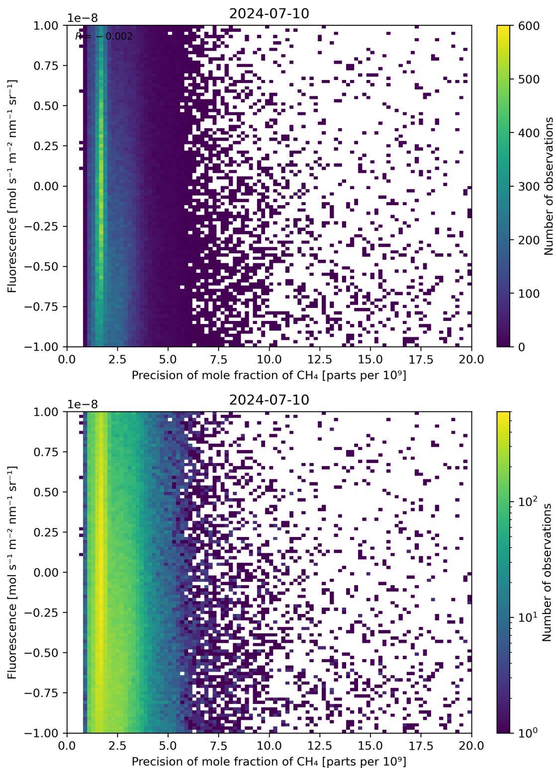
Figure 81: Scatter density plot of “Precision of mole fraction of \text{CH}_4 ” against “Fluorescence” for 2024-07-10 to 2024-07-11.
