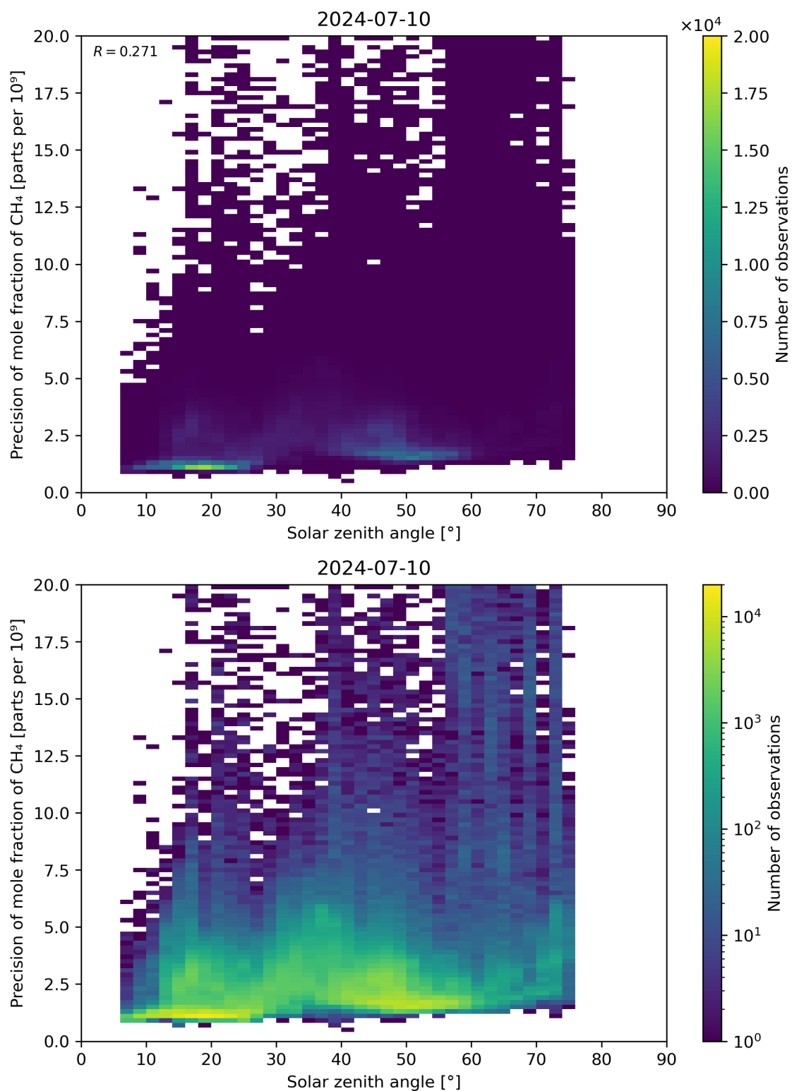
Figure 101: Scatter density plot of “Solar zenith angle” against “Precision of mole fraction of CH 4 ” for 2024-07-10 to 2024-07-11.
