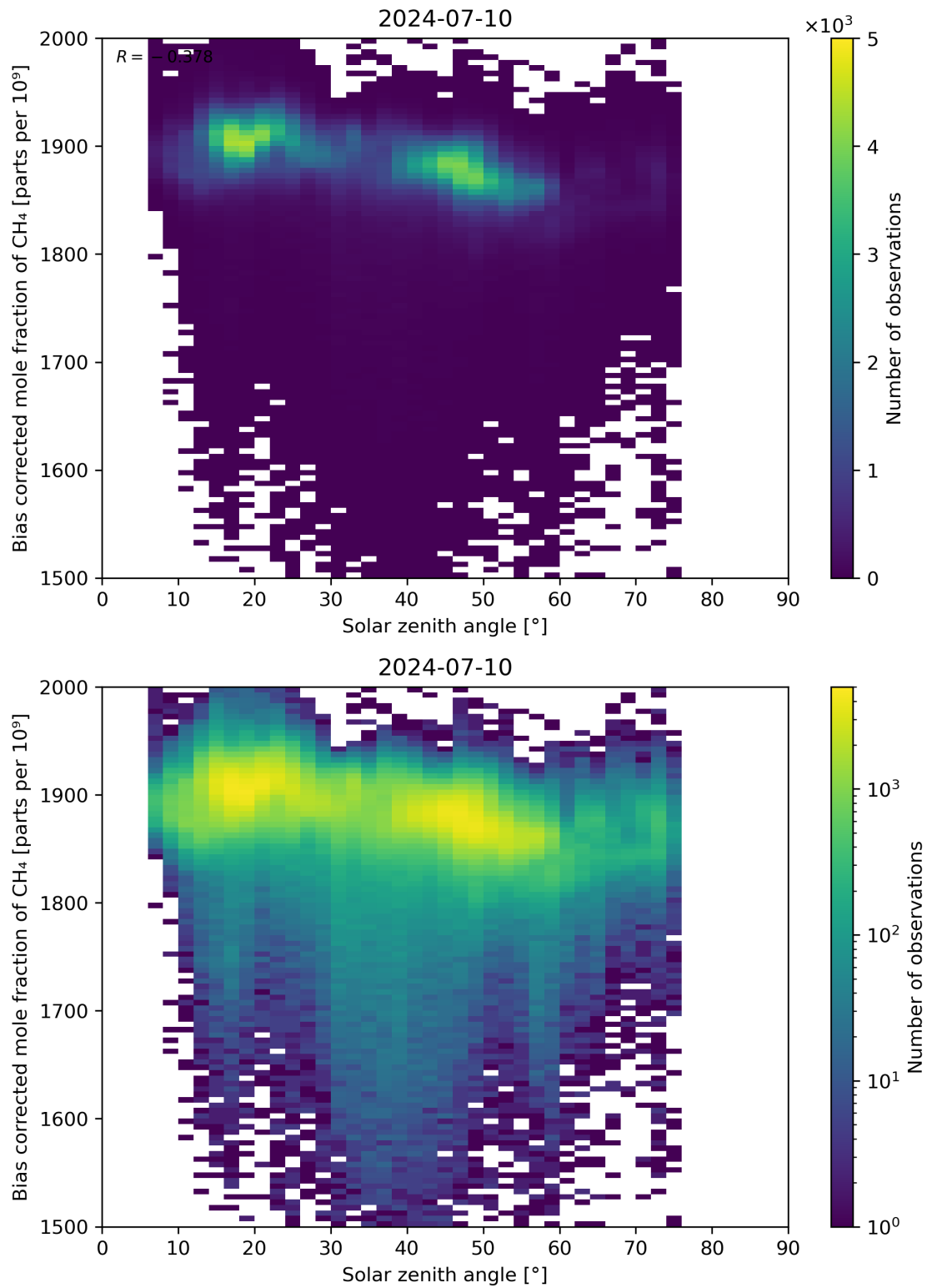
Figure 100: Scatter density plot of “Solar zenith angle” against “Bias corrected mole fraction of CH 4 ” for 2024-07-10 to 2024-07-11.
