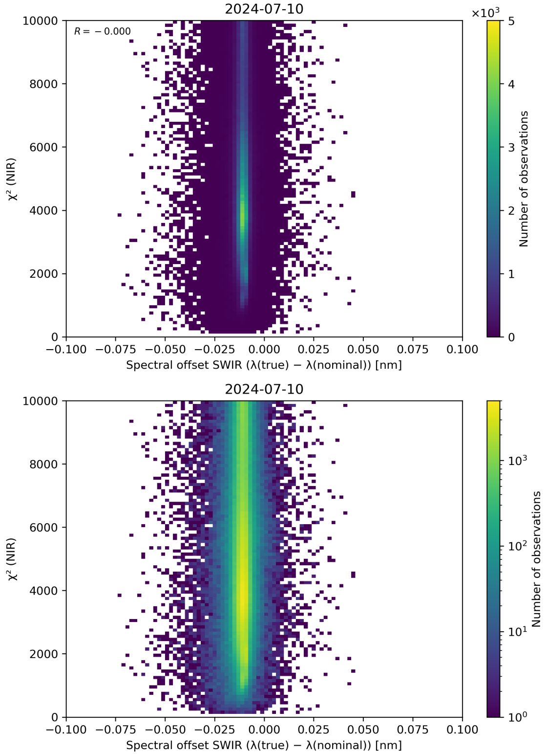
Figure 117: Scatter density plot of “Spectral offset SWIR ( \lambda(\text{true}) - \lambda(\text{nominal}) )” against “ \chi^2 (NIR)” for 2024-07-10 to 2024-07-11.
