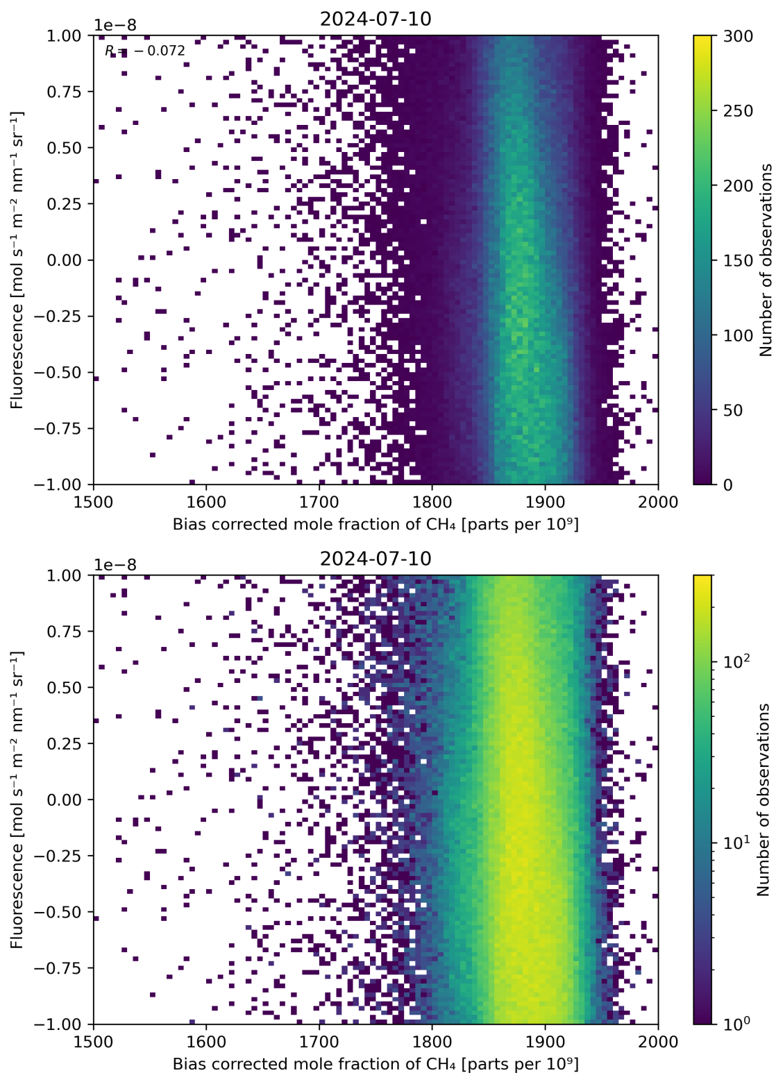
Figure 66: Scatter density plot of “Bias corrected mole fraction of \text{CH}_4 ” against “Fluorescence” for 2024-07-10 to 2024-07-11.
