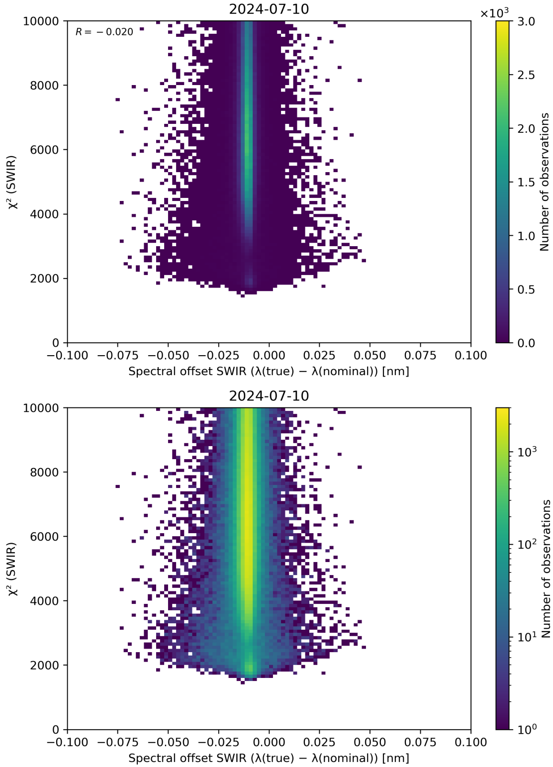
Figure 118: Scatter density plot of “Spectral offset SWIR ( \lambda(\text{true}) - \lambda(\text{nominal}) )” against “ \chi^2 (SWIR)” for 2024-07-10 to 2024-07-11.
