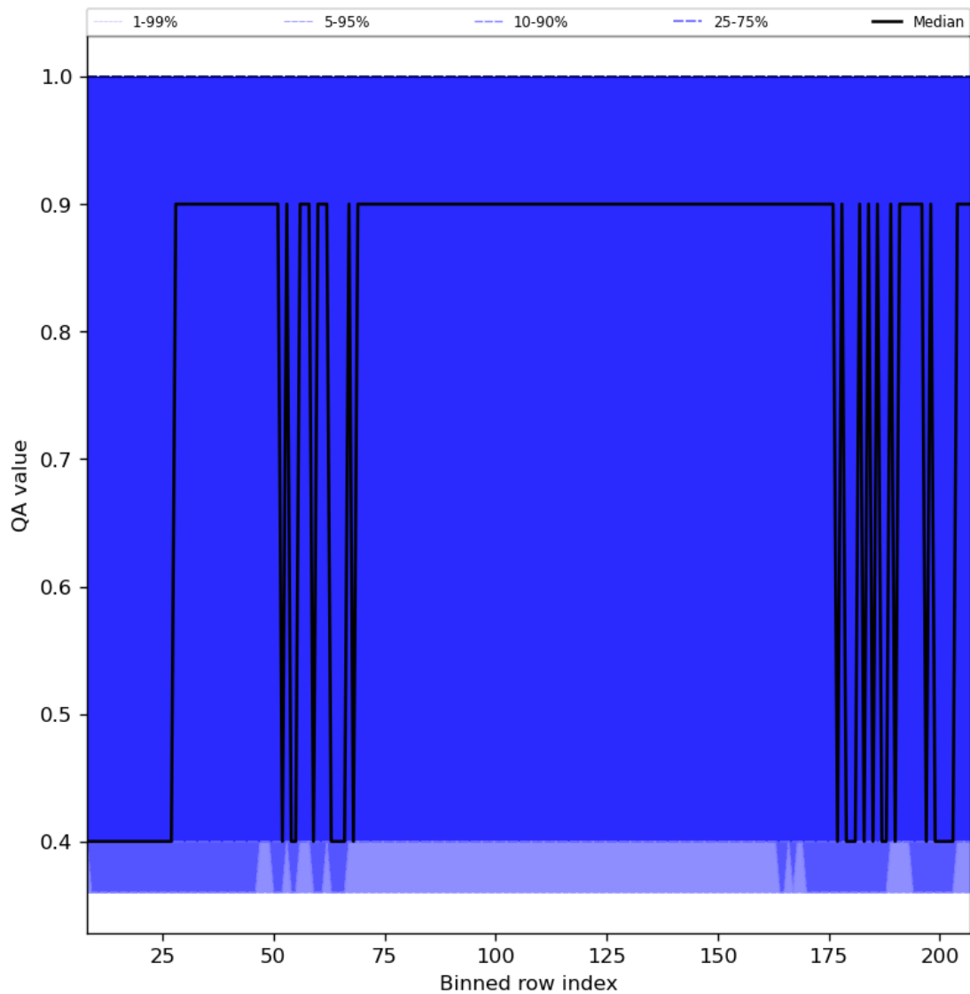
Figure 33: Along track statistics of “QA value” for 2024-07-10 to 2024-07-11
