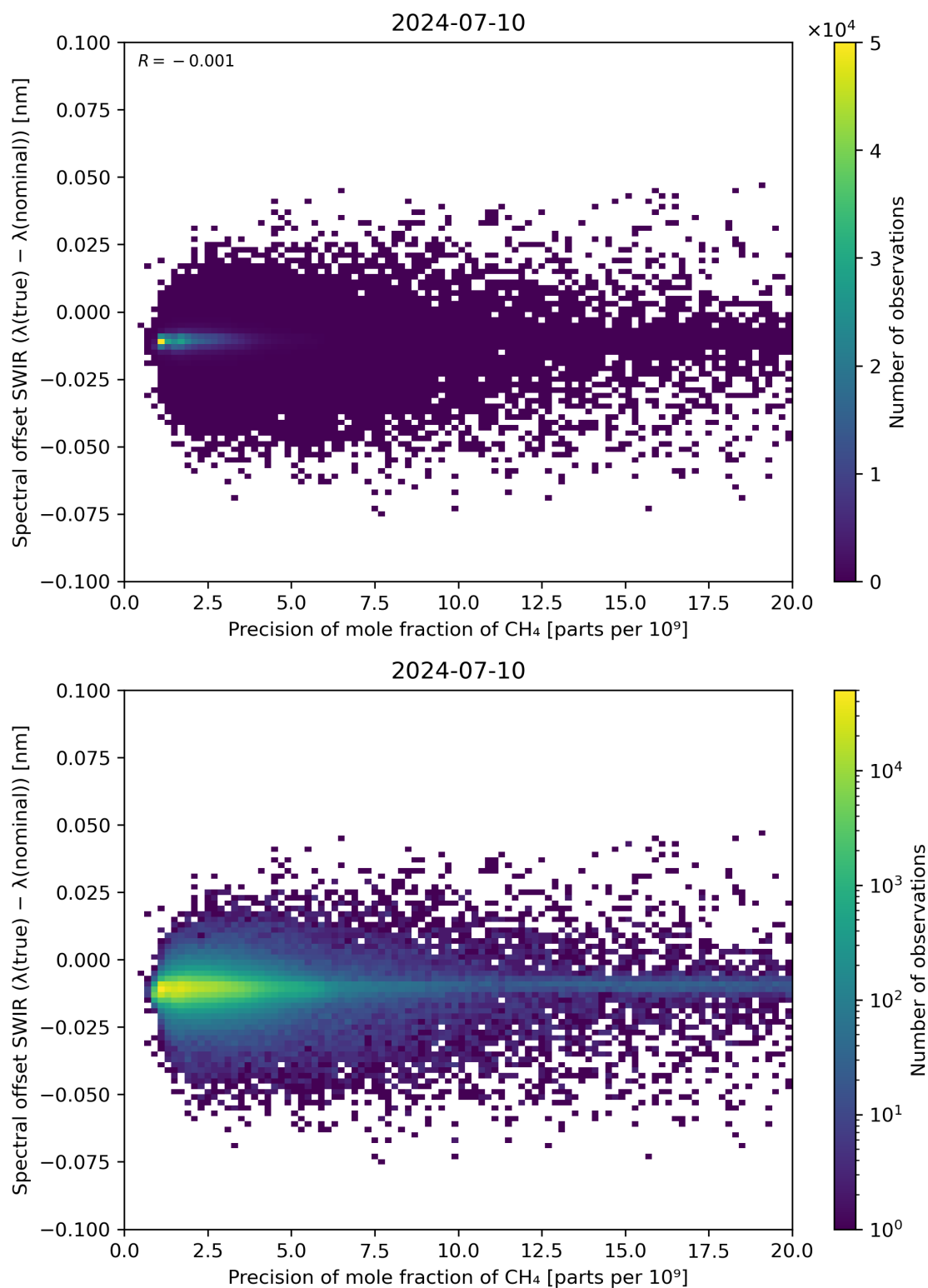
Figure 85: Scatter density plot of “Precision of mole fraction of CH 4 ” against “Spectral offset SWIR ( \lambda(\text{true}) - \lambda(\text{nominal}) )” for 2024-07-10 to 2024-07-11.
