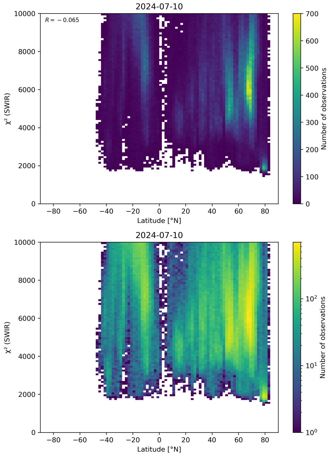
Figure 54: Scatter density plot of “Latitude” against “ \chi^2 (SWIR)” for 2024-07-10 to 2024-07-11.
