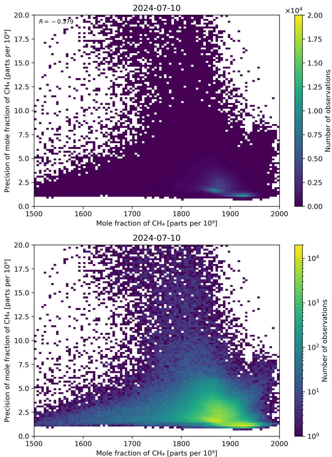
Figure 75: Scatter density plot of “Mole fraction of CH 4 ” against “Precision of mole fraction of CH 4 ” for 2024-07-10 to 2024-07-11.
