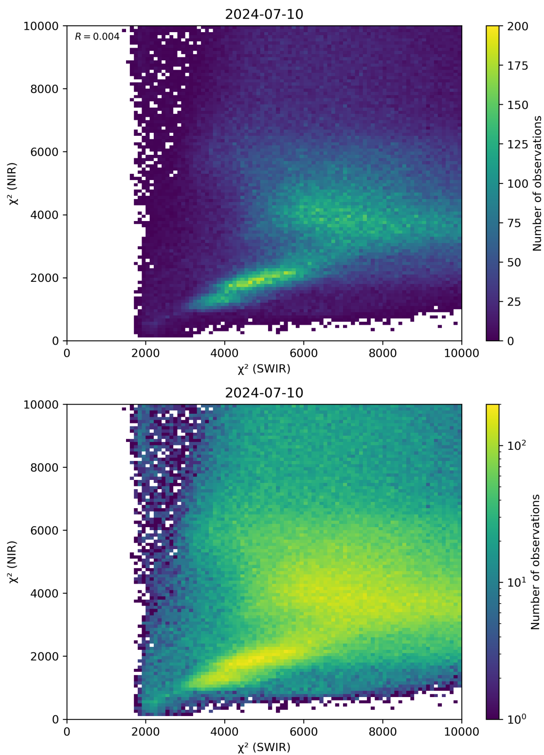
Figure 47: Scatter density plot of “ \chi^2 (SWIR)” against “ \chi^2 (NIR)” for 2024-07-10 to 2024-07-11.
