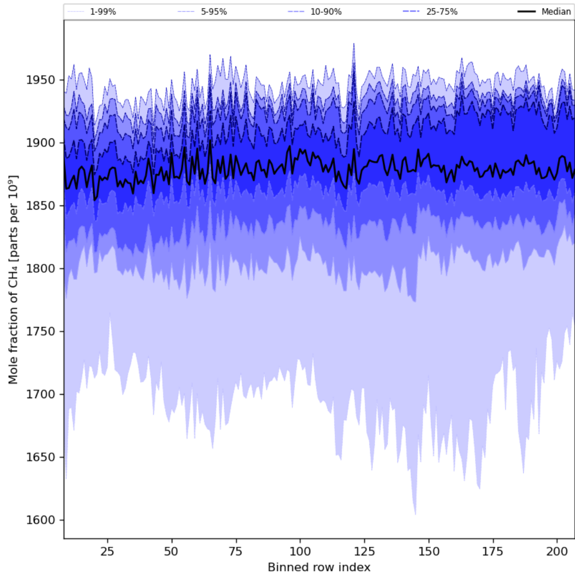
Figure 34: Along track statistics of “Mole fraction of CH 4 ” for 2024-07-10 to 2024-07-11
