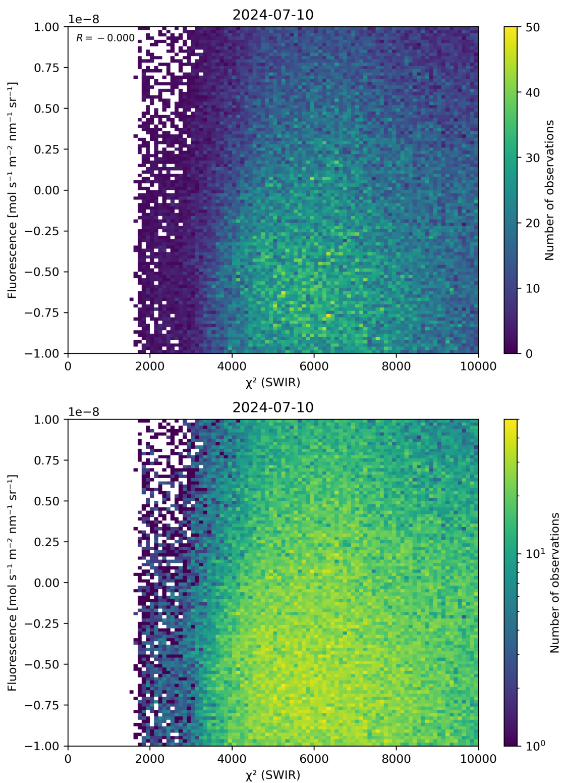
Figure 49: Scatter density plot of “ \chi^2 (SWIR)” against “Fluorescence” for 2024-07-10 to 2024-07-11.
