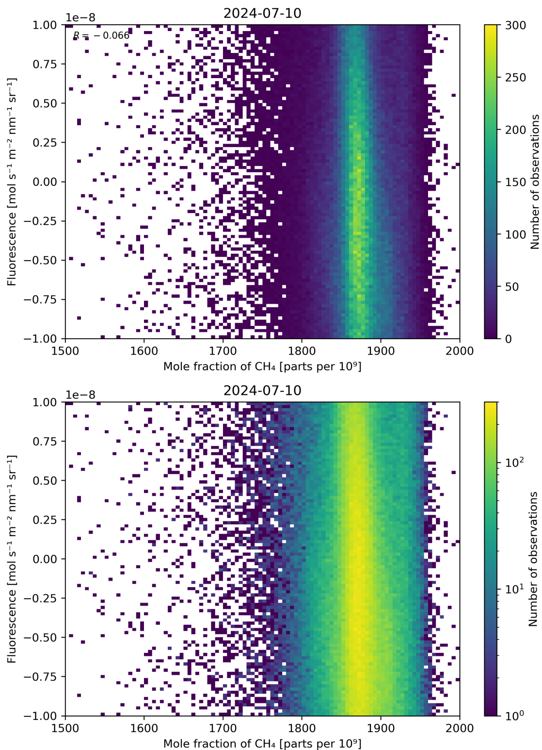
Figure 73: Scatter density plot of “Mole fraction of CH 4 ” against “Fluorescence” for 2024-07-10 to 2024-07-11.
