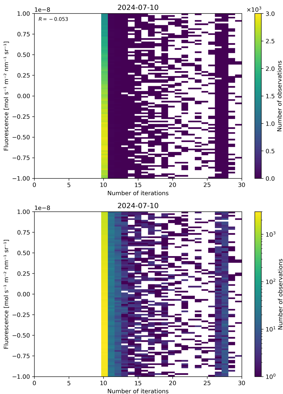
Figure 87: Scatter density plot of “Number of iterations” against “Fluorescence” for 2024-07-10 to 2024-07-11.
