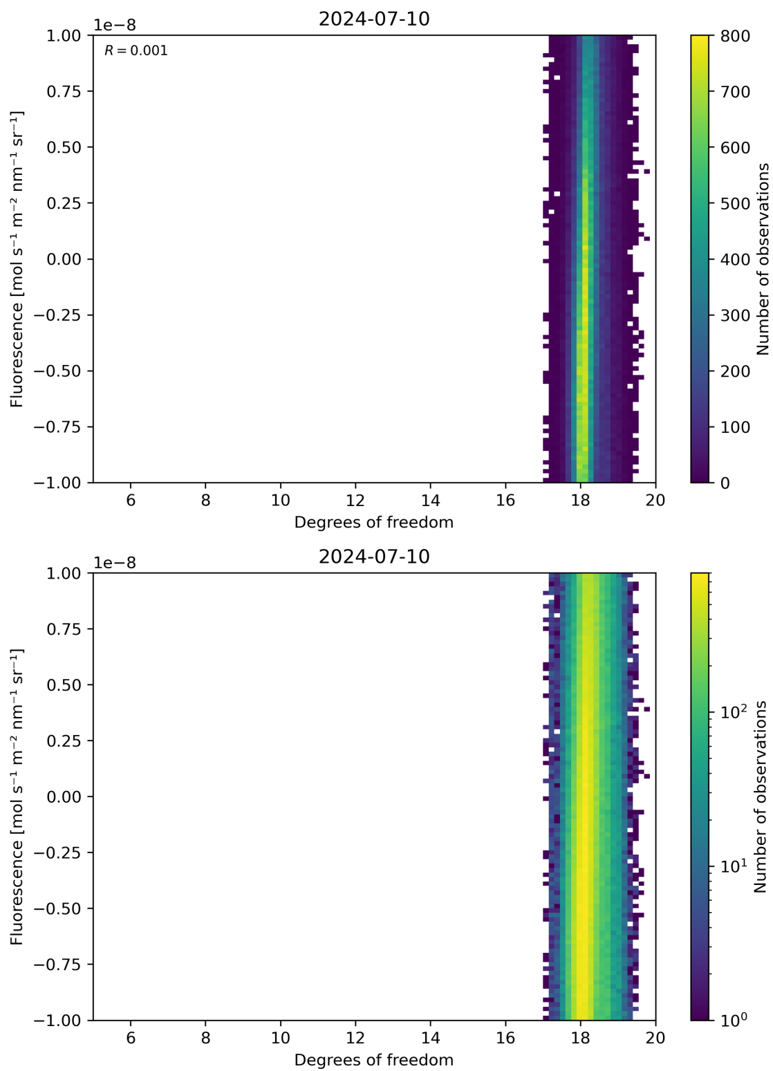
Figure 51: Scatter density plot of “Degrees of freedom” against “Fluorescence” for 2024-07-10 to 2024-07-11.
