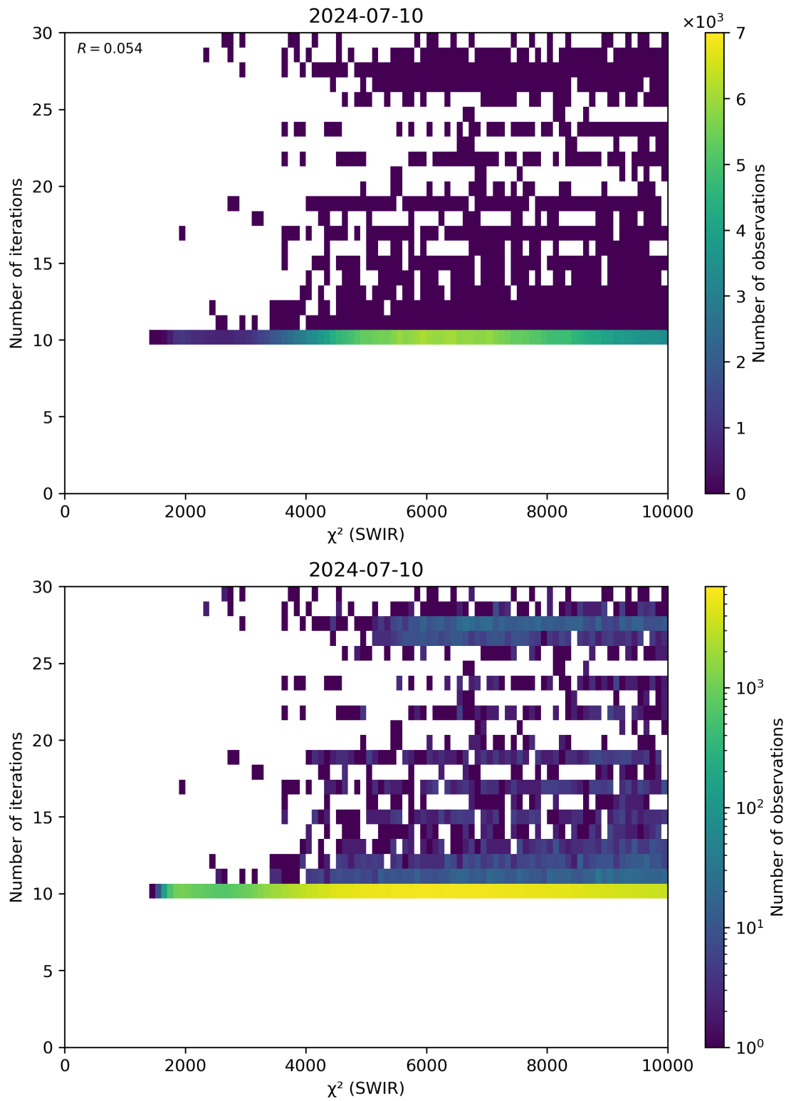
Figure 50: Scatter density plot of “ \chi^2 (SWIR)” against “Number of iterations” for 2024-07-10 to 2024-07-11.
