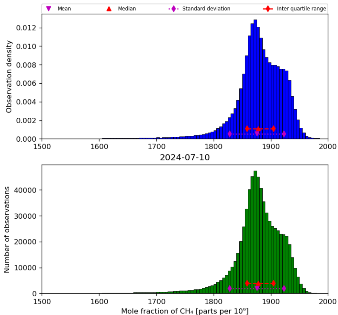
Figure 23: Histogram of “Mole fraction of CH 4 ” for 2024-07-10 to 2024-07-11
