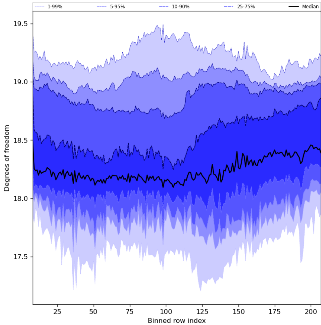
Figure 41: Along track statistics of “Degrees of freedom” for 2024-07-10 to 2024-07-11
