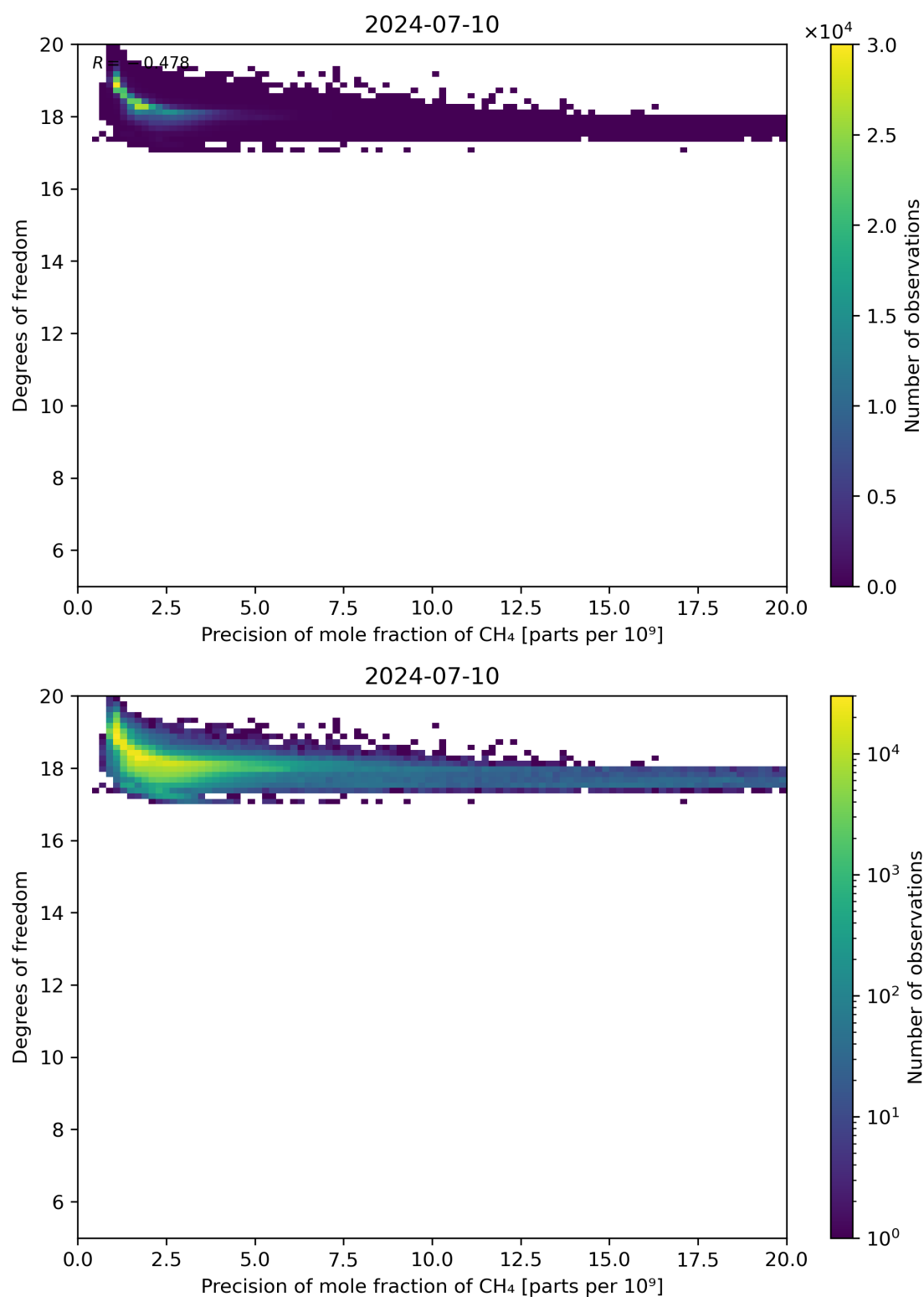
Figure 80: Scatter density plot of “Precision of mole fraction of CH 4 ” against “Degrees of freedom” for 2024-07-10 to 2024-07-11.
