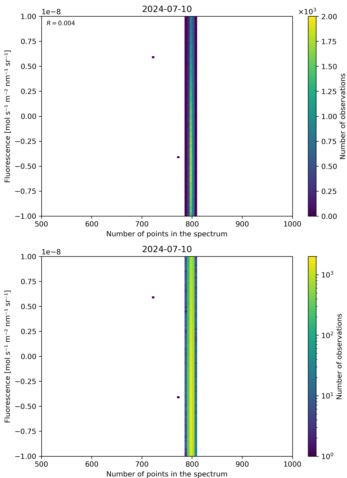
Figure 91: Scatter density plot of “Number of points in the spectrum” against “Fluorescence” for 2024-07-10 to 2024-07-11.
