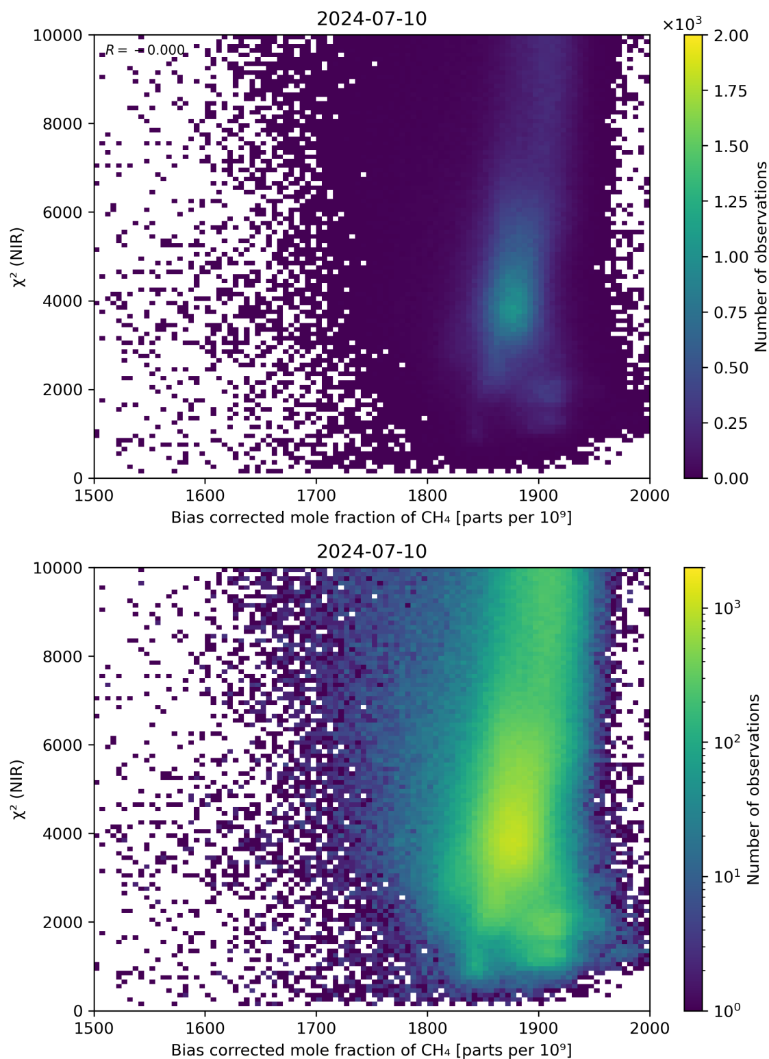
Figure 63: Scatter density plot of “Bias corrected mole fraction of \text{CH}_4 ” against “ \chi^2 (NIR)” for 2024-07-10 to 2024-07-11.
