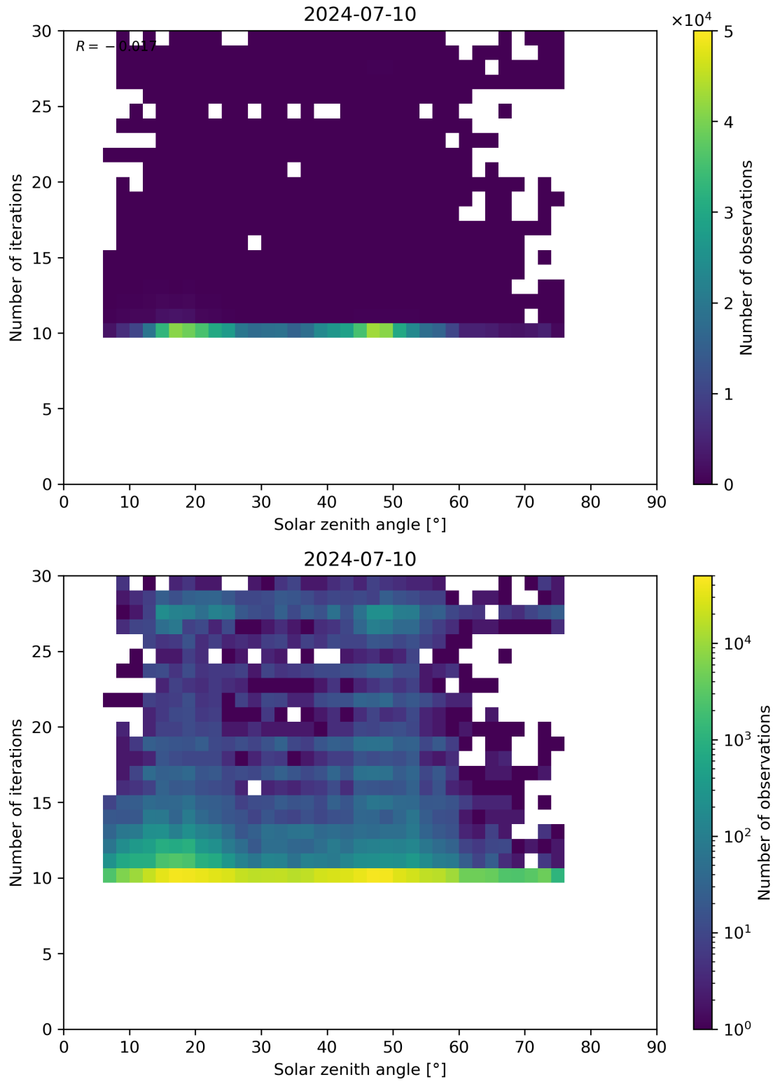
Figure 102: Scatter density plot of “Solar zenith angle” against “Number of iterations” for 2024-07-10 to 2024-07-11.
