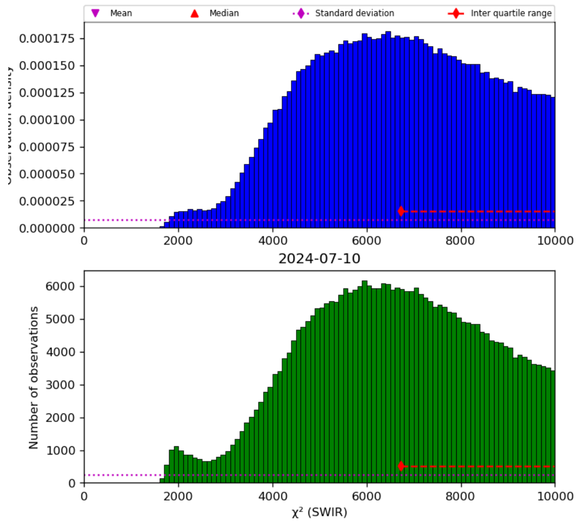
Figure 28: Histogram of “ \chi^2 (SWIR)” for 2024-07-10 to 2024-07-11
