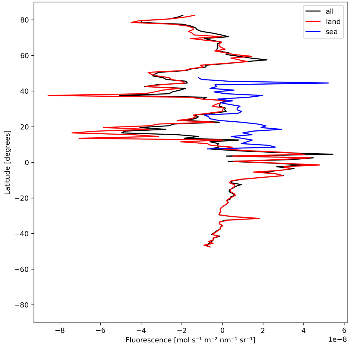
Figure 21: Zonal average of “Fluorescence” for 2024-07-10 to 2024-07-11.
