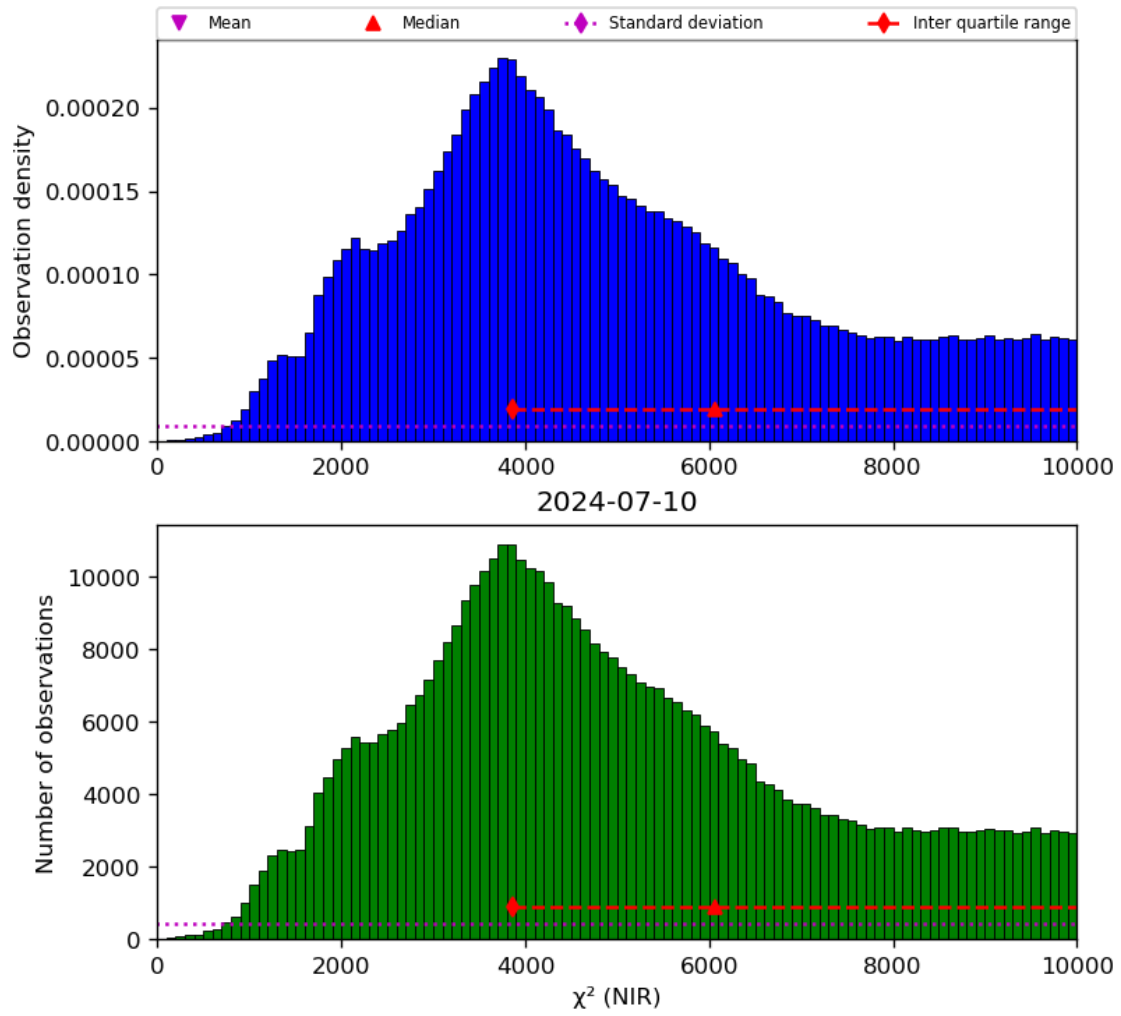
Figure 29: Histogram of “ \chi^2 (NIR)” for 2024-07-10 to 2024-07-11
