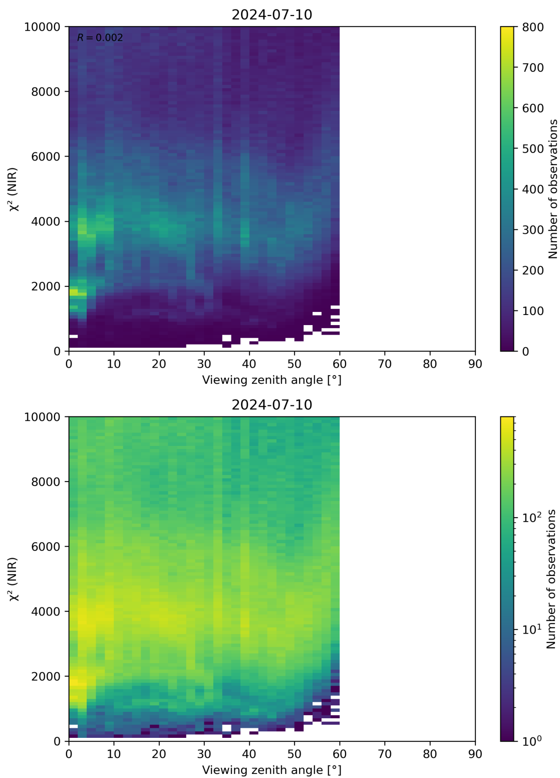
Figure 105: Scatter density plot of “Viewing zenith angle” against “ \chi^2 (NIR)” for 2024-07-10 to 2024-07-11.
