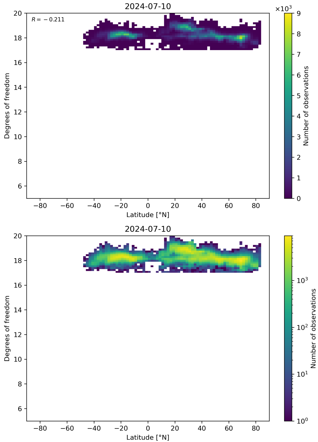
Figure 55: Scatter density plot of “Latitude” against “Degrees of freedom” for 2024-07-10 to 2024-07-11.
