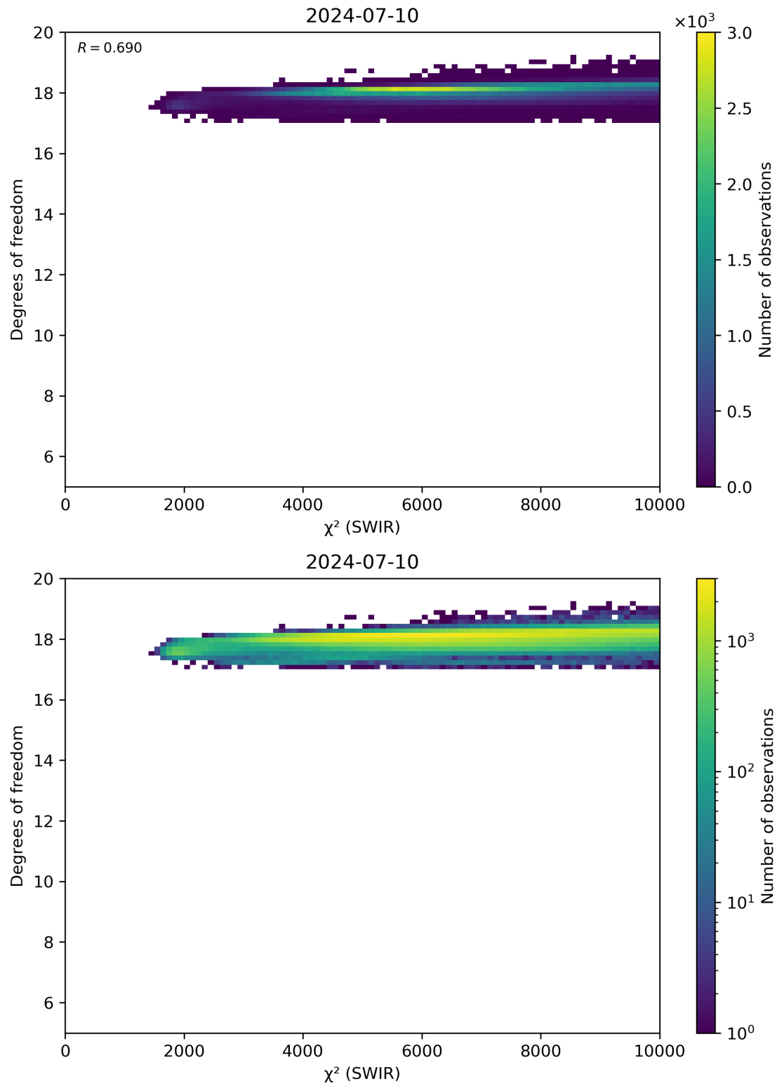
Figure 48: Scatter density plot of " \chi^2 (SWIR)" against "Degrees of freedom" for 2024-07-10 to 2024-07-11.
