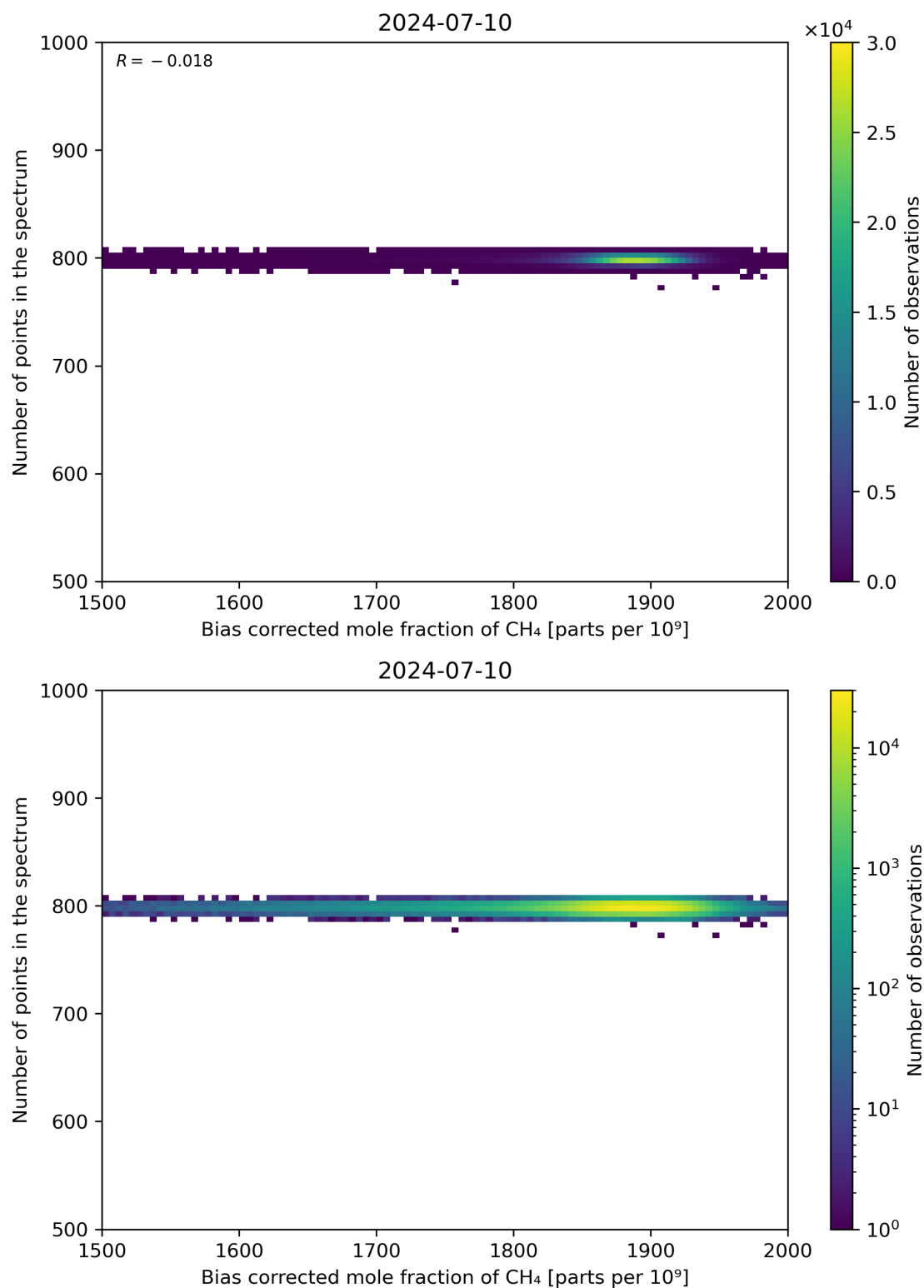
Figure 68: Scatter density plot of “Bias corrected mole fraction of CH 4 ” against “Number of points in the spectrum” for 2024-07-10 to 2024-07-11.
