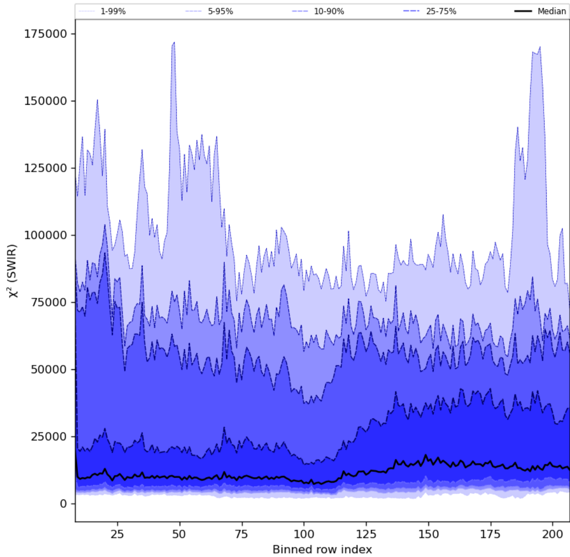
Figure 39: Along track statistics of " \chi^2 (SWIR)" for 2024-07-10 to 2024-07-11
