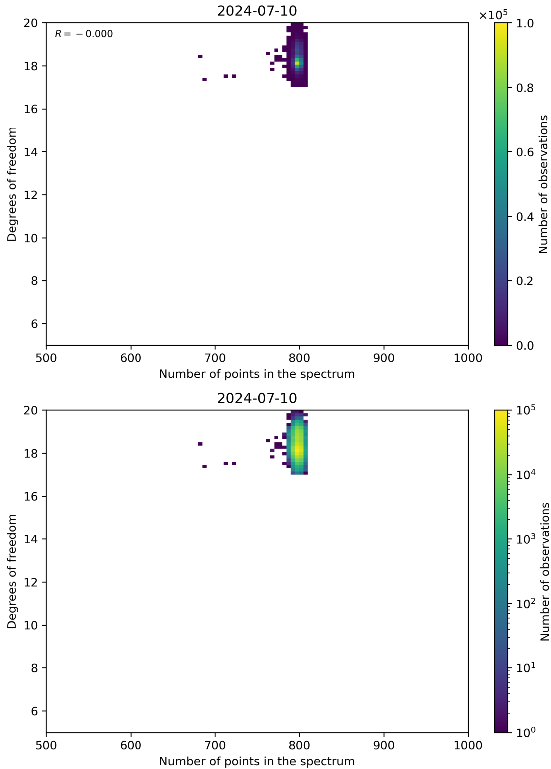
Figure 90: Scatter density plot of “Number of points in the spectrum” against “Degrees of freedom” for 2024-07-10 to 2024-07-11.
