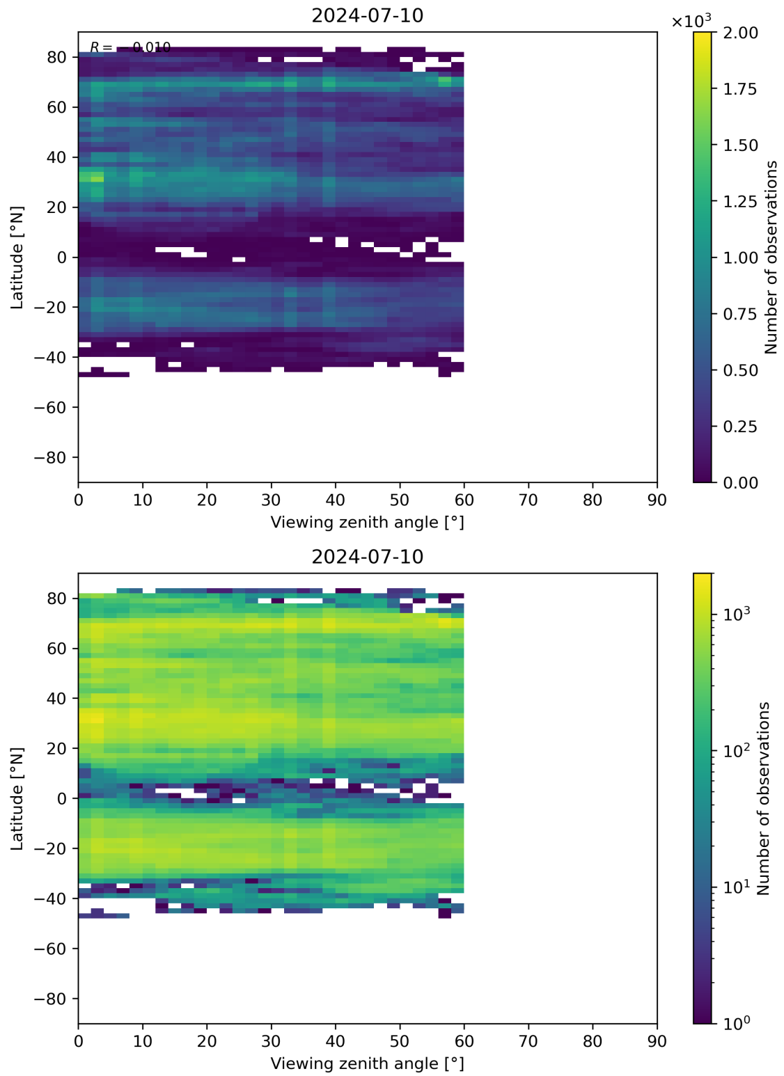
Figure 109: Scatter density plot of “Viewing zenith angle” against “Latitude” for 2024-07-10 to 2024-07-11.
