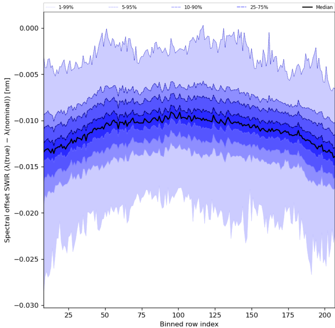
Figure 38: Along track statistics of “Spectral offset SWIR ( \lambda(\text{true}) - \lambda(\text{nominal}) )” for 2024-07-10 to 2024-07-11
