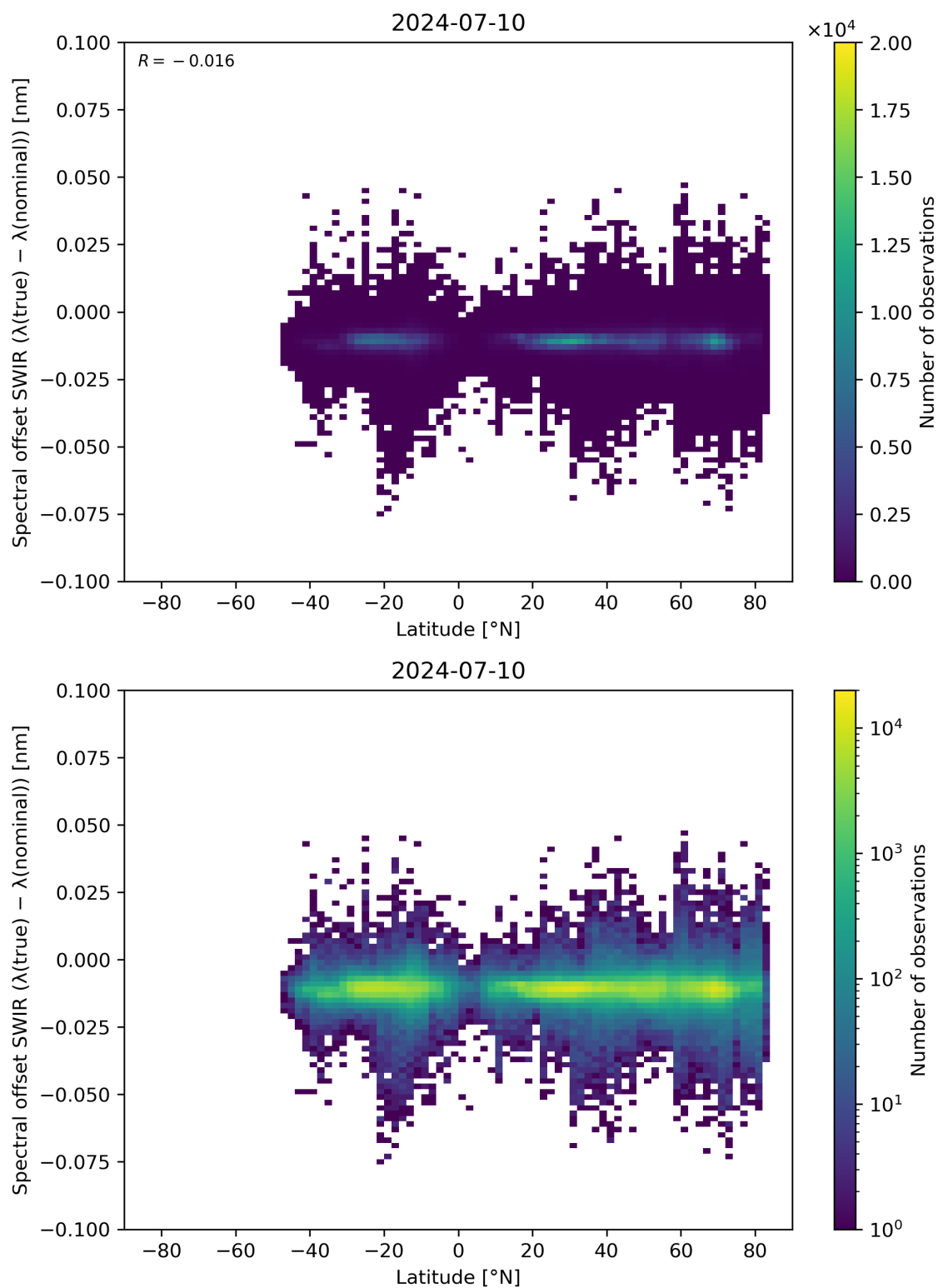
Figure 62: Scatter density plot of “Latitude” against “Spectral offset SWIR ( \lambda(\text{true}) - \lambda(\text{nominal}) )” for 2024-07-10 to 2024-07-11.
