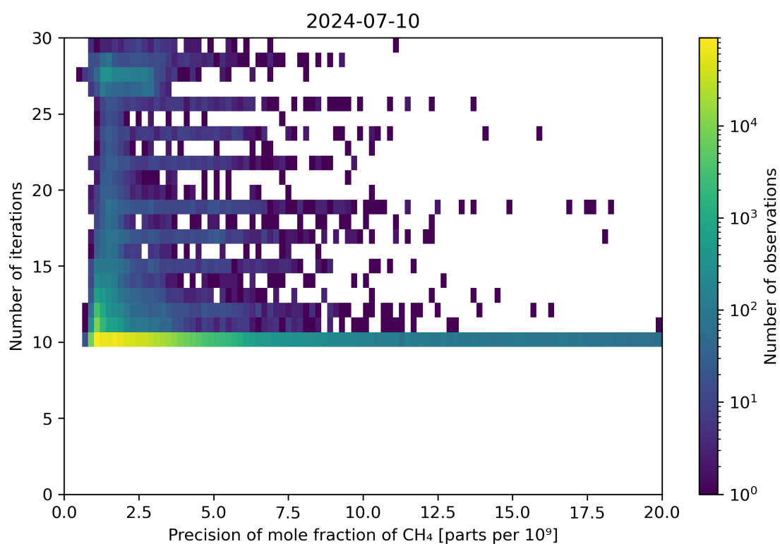
Figure 83: Scatter density plot of “Precision of mole fraction of CH 4 ” against “Number of iterations” for 2024-07-10 to 2024-07-11.
