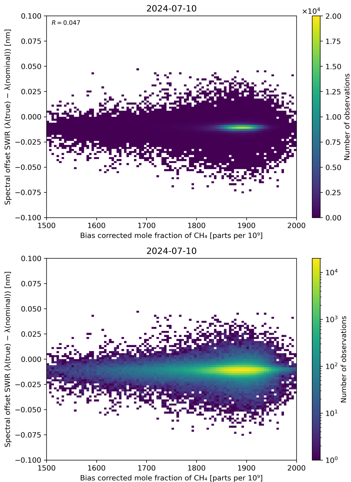
Figure 69: Scatter density plot of “Bias corrected mole fraction of \text{CH}_4 ” against “Spectral offset SWIR ( \lambda(\text{true}) - \lambda(\text{nominal}) )” for 2024-07-10 to 2024-07-11.
