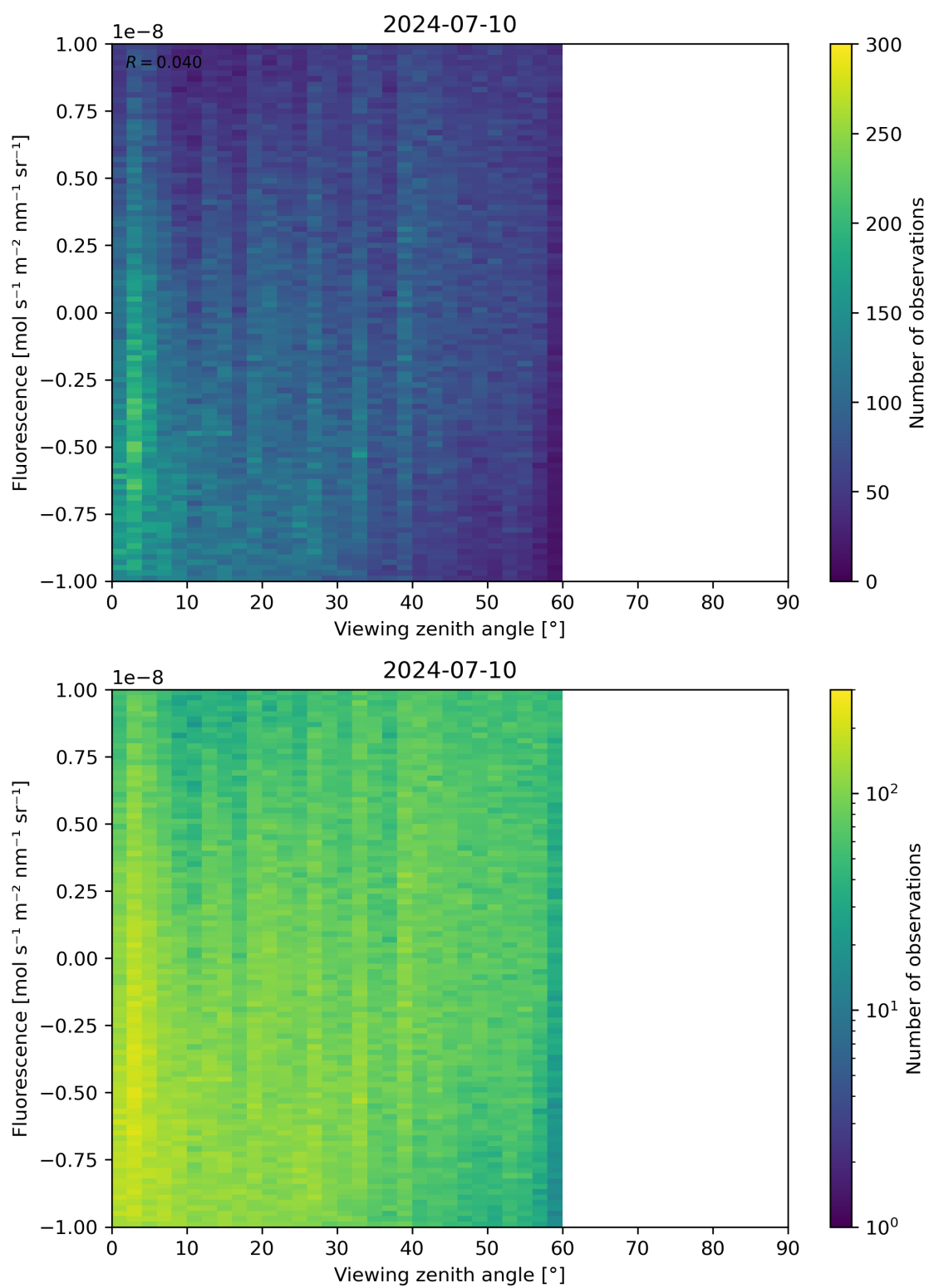
Figure 108: Scatter density plot of “Viewing zenith angle” against “Fluorescence” for 2024-07-10 to 2024-07-11.
