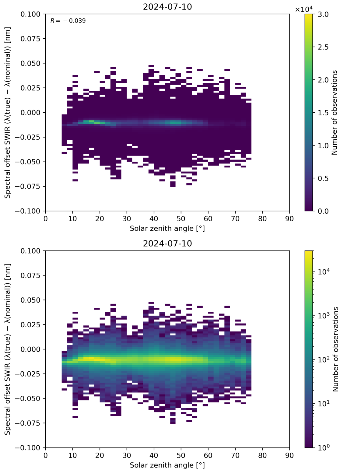
Figure 104: Scatter density plot of “Solar zenith angle” against “Spectral offset SWIR ( \lambda(\text{true}) - \lambda(\text{nominal}) )” for 2024-07-10 to 2024-07-11.
