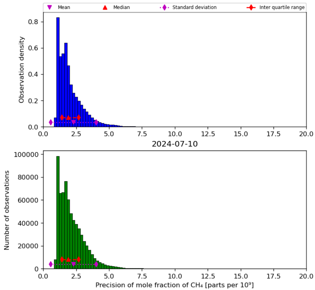
Figure 24: Histogram of “Precision of mole fraction of CH 4 ” for 2024-07-10 to 2024-07-11
