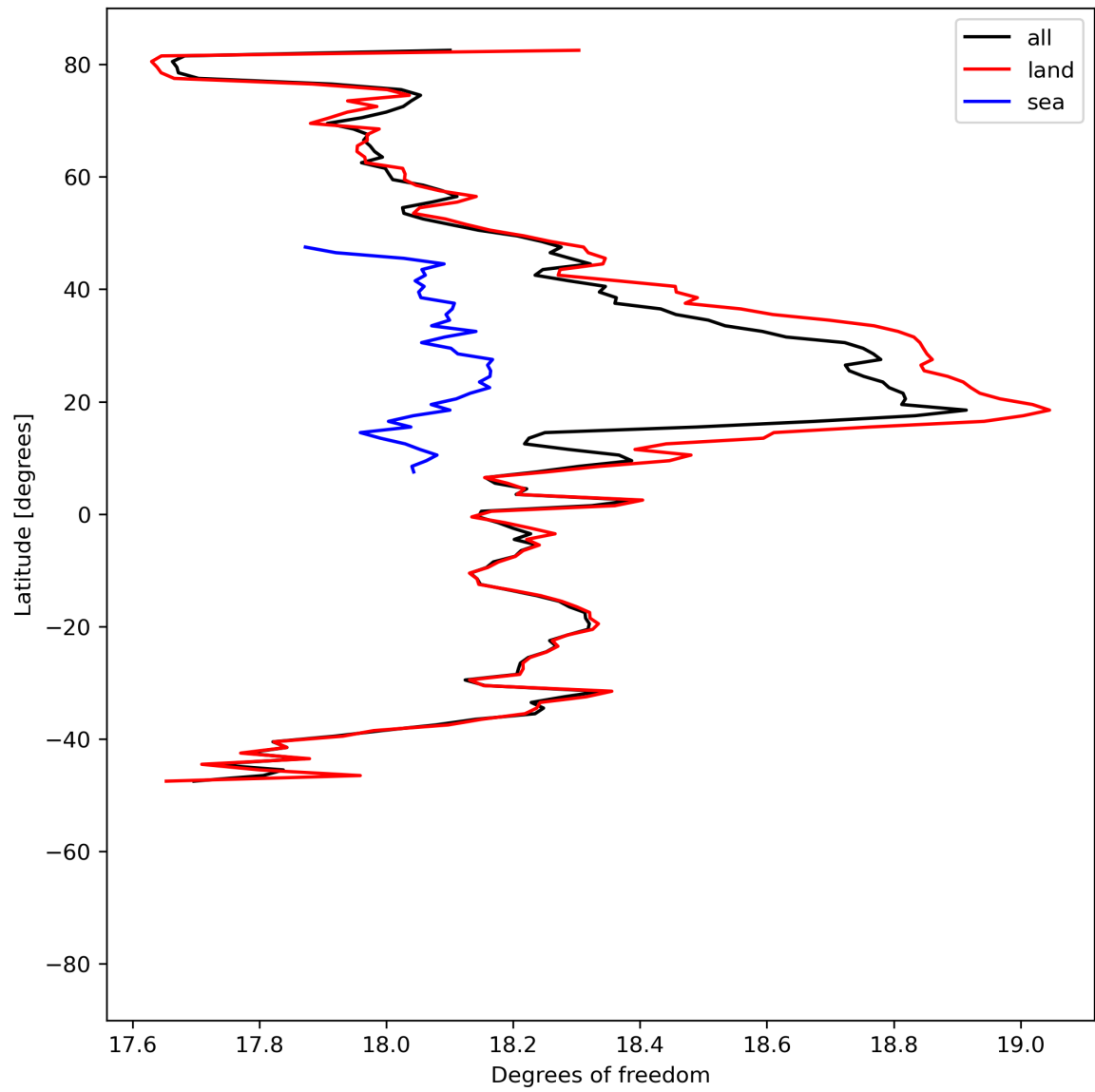
Figure 19: Zonal average of “Degrees of freedom” for 2024-07-10 to 2024-07-11.
