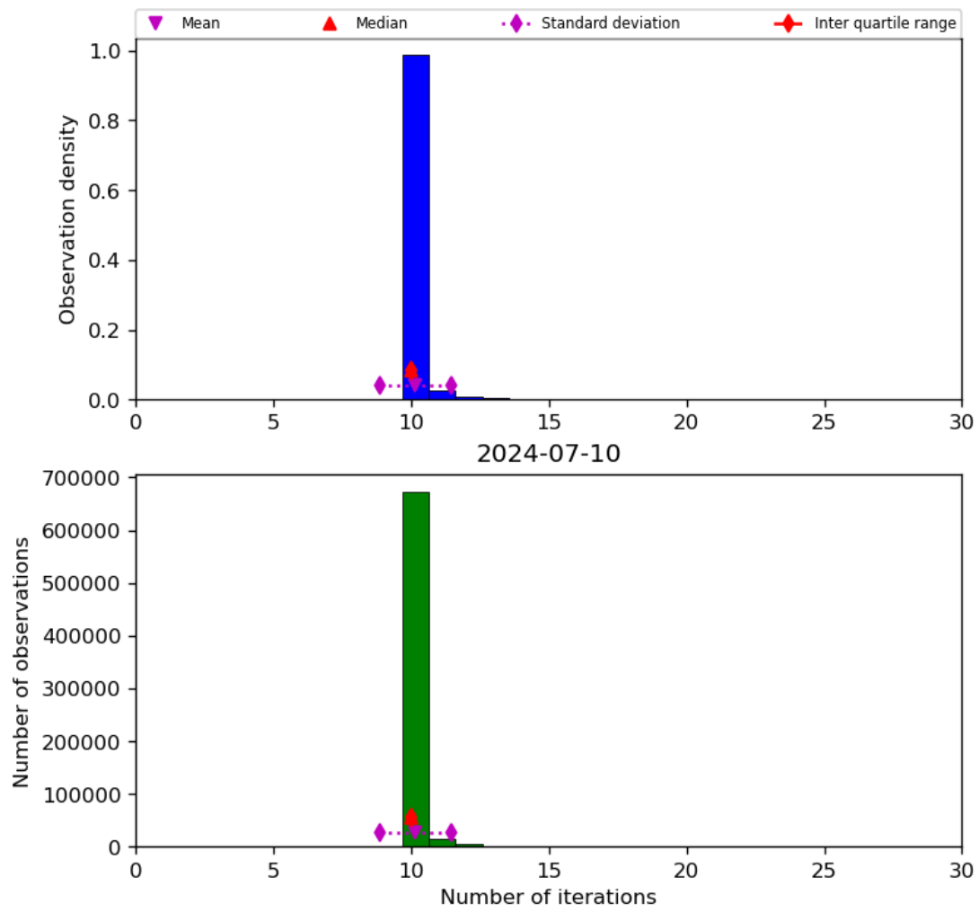
Figure 31: Histogram of “Number of iterations” for 2024-07-10 to 2024-07-11
