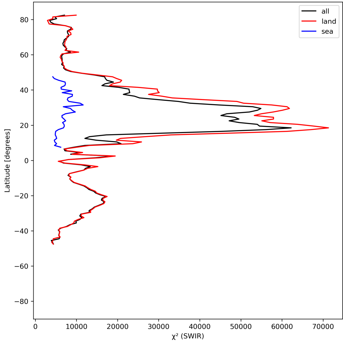
Figure 17: Zonal average of “ \chi^2 (SWIR)” for 2024-07-10 to 2024-07-11.
