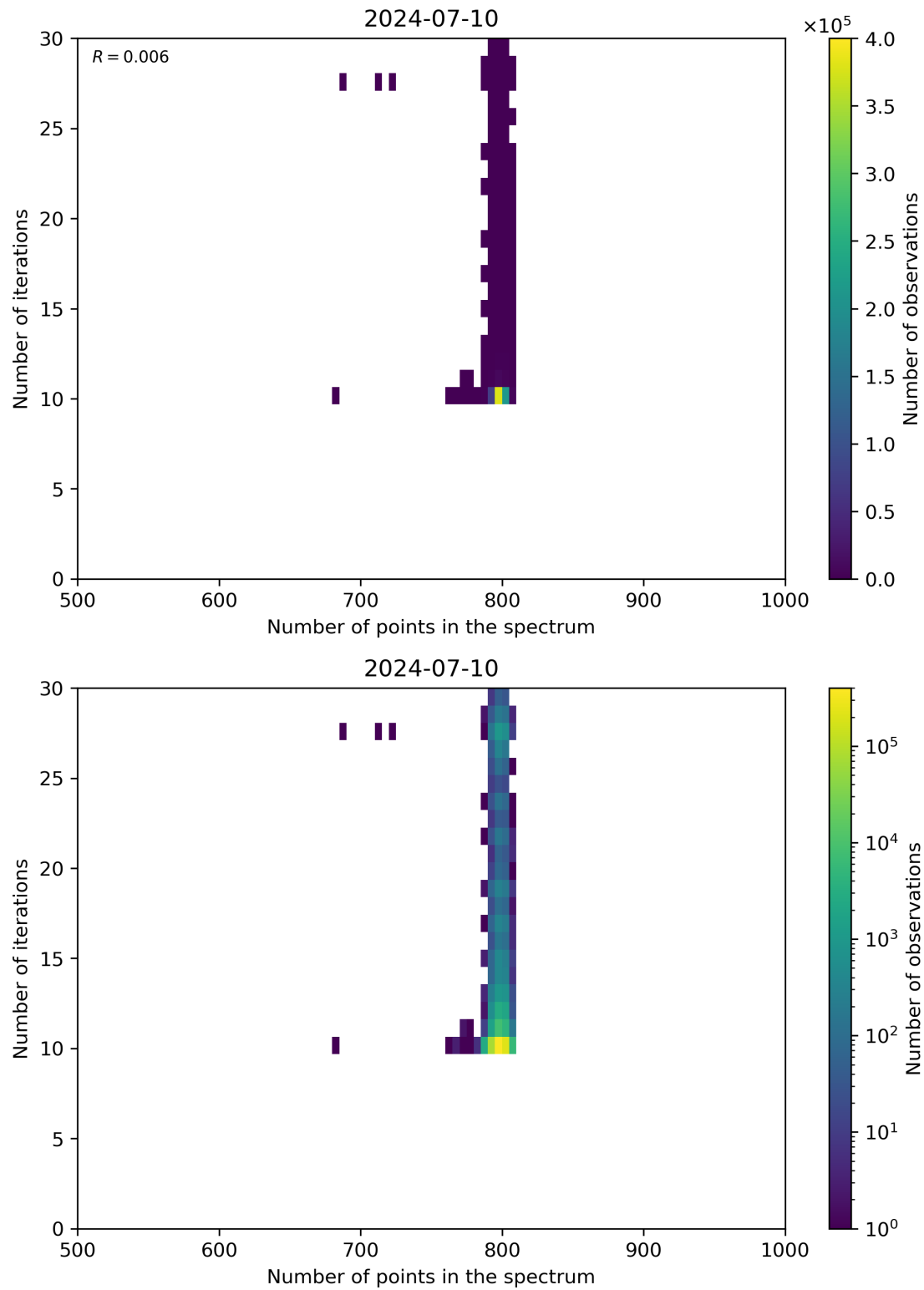
Figure 92: Scatter density plot of “Number of points in the spectrum” against “Number of iterations” for 2024-07-10 to 2024-07-11.
