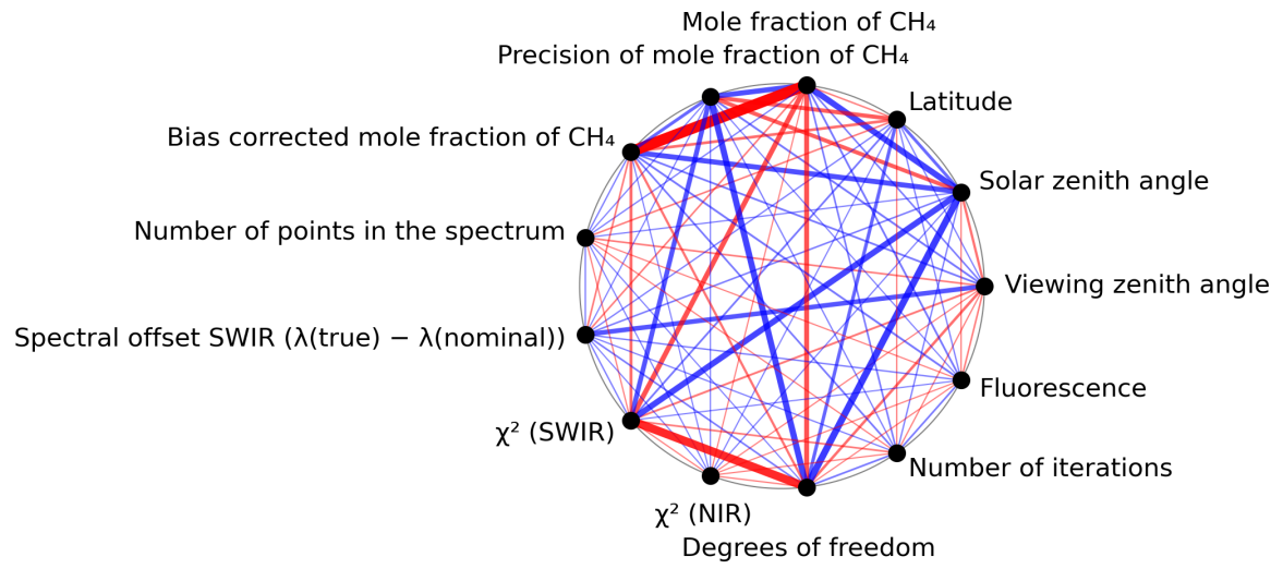
Figure 1: Map of correlation graph for 2024-07-10 to 2024-07-11.
