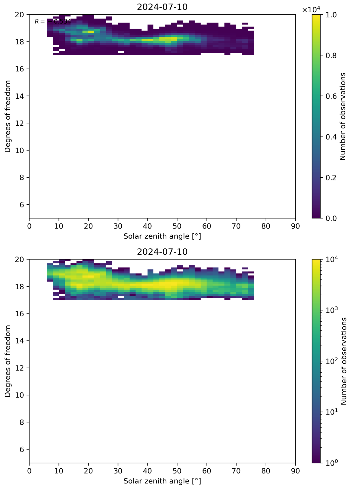
Figure 96: Scatter density plot of “Solar zenith angle” against “Degrees of freedom” for 2024-07-10 to 2024-07-11.
