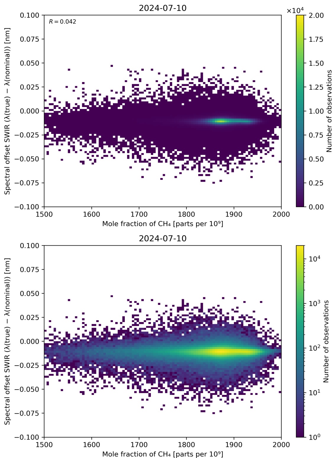
Figure 86: Scatter density plot of “Mole fraction of CH 4 ” against “Spectral offset SWIR ( \lambda(\text{true}) - \lambda(\text{nominal}) )” for 2024-07-10 to 2024-07-11.
