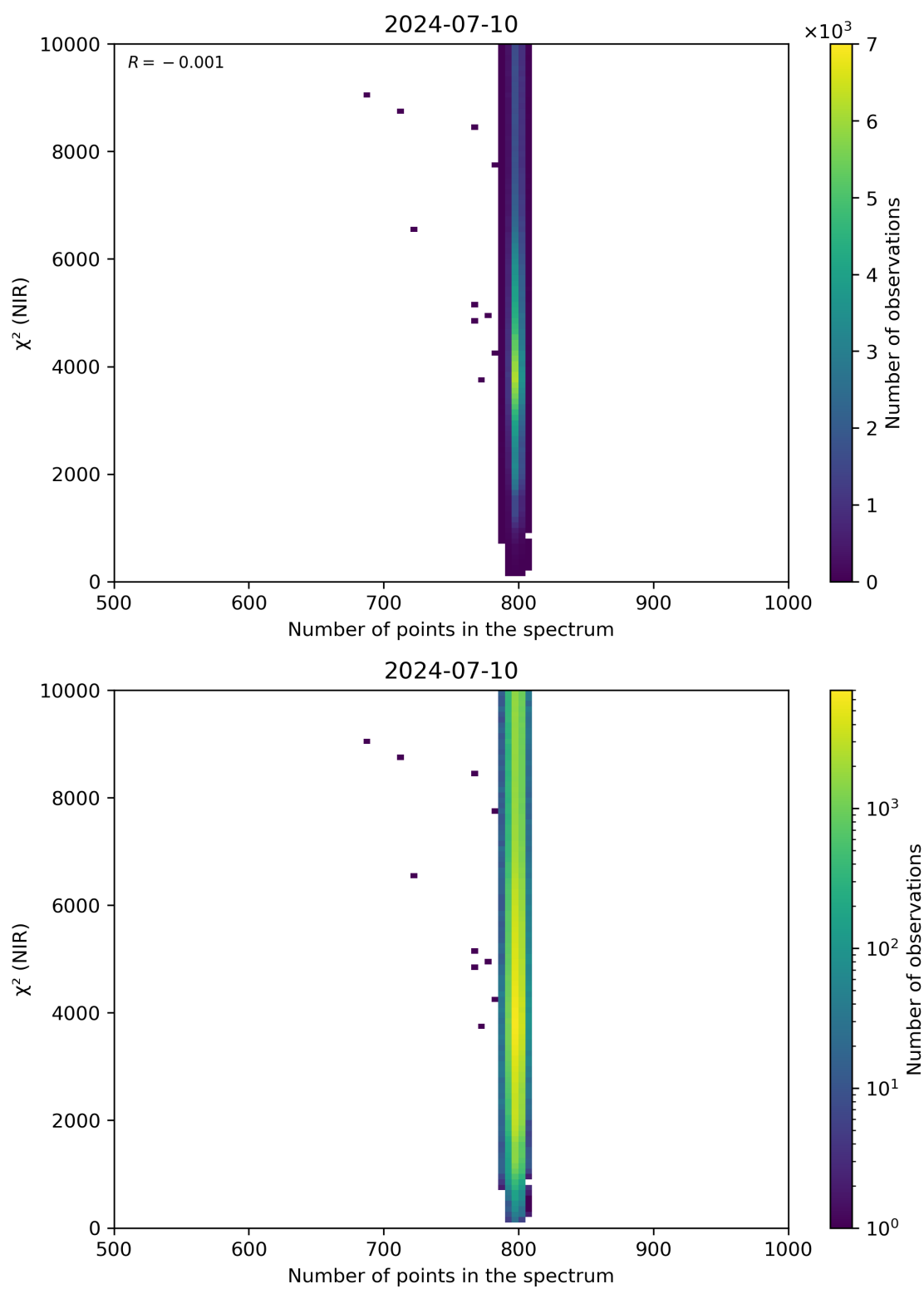
Figure 88: Scatter density plot of “Number of points in the spectrum” against “ \chi^2 (NIR)” for 2024-07-10 to 2024-07-11.
