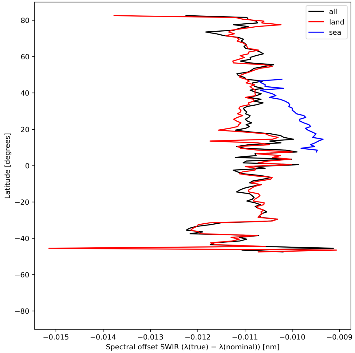
Figure 16: Zonal average of “Spectral offset SWIR ( \lambda(\text{true}) - \lambda(\text{nominal}) )” for 2024-07-10 to 2024-07-11.
