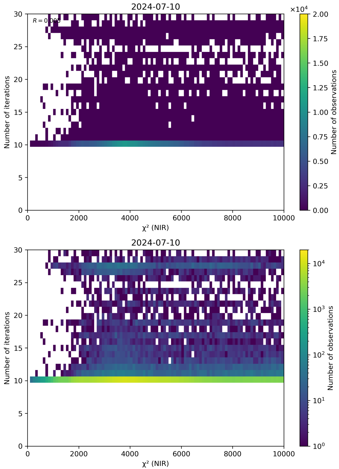
Figure 46: Scatter density plot of “ \chi^2 (NIR)” against “Number of iterations” for 2024-07-10 to 2024-07-11.
