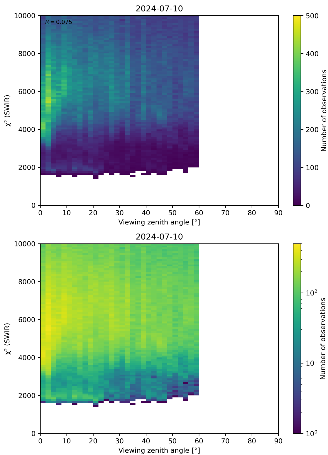
Figure 106: Scatter density plot of “Viewing zenith angle” against “ \chi^2 (SWIR)” for 2024-07-10 to 2024-07-11.
