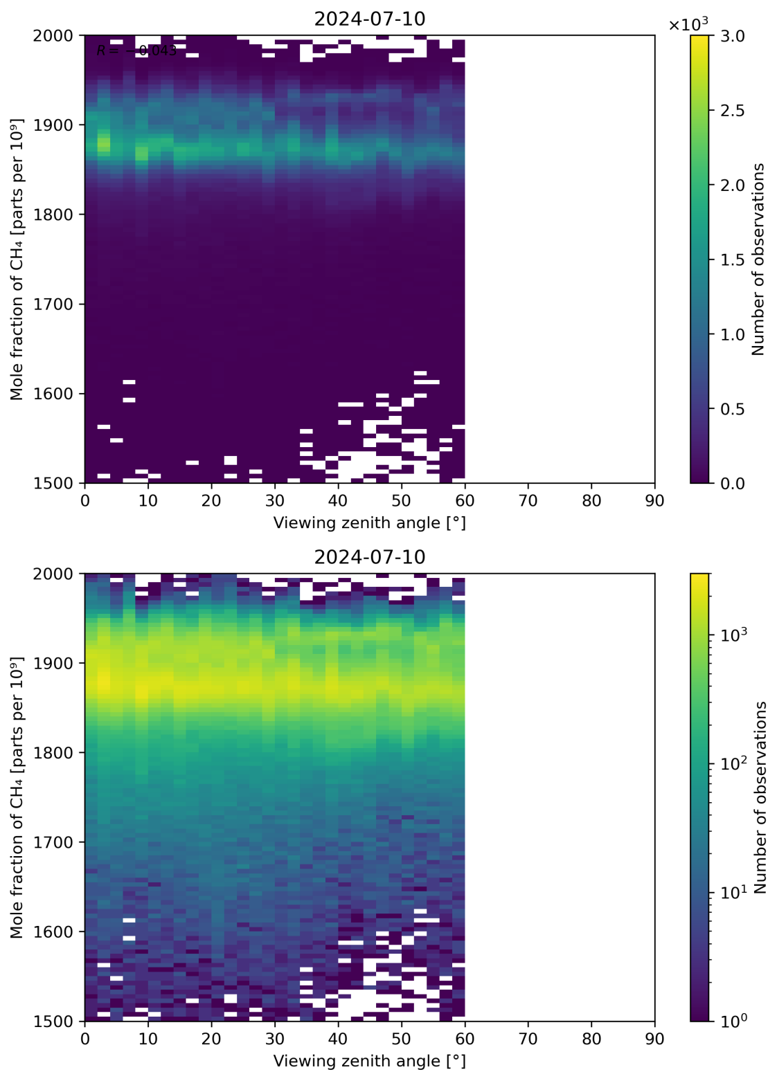
Figure 110: Scatter density plot of “Viewing zenith angle” against “Mole fraction of CH 4 ” for 2024-07-10 to 2024-07-11.
