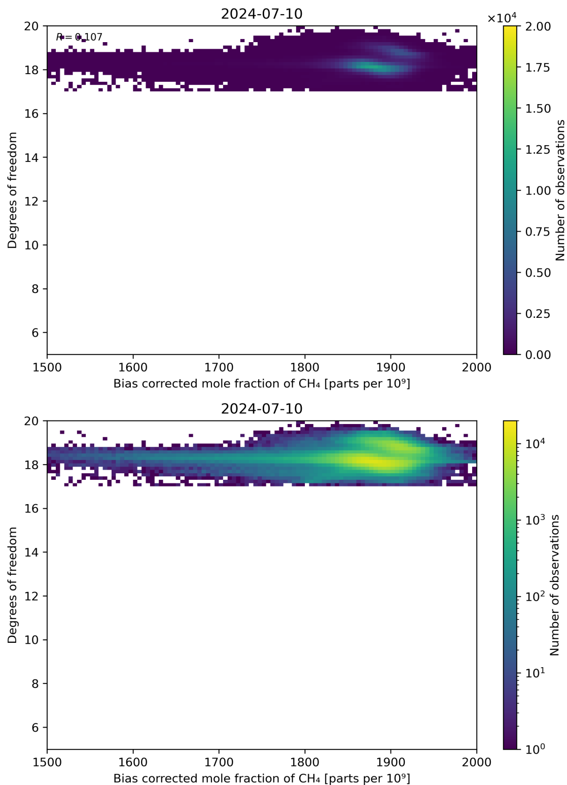
Figure 65: Scatter density plot of “Bias corrected mole fraction of CH 4 ” against “Degrees of freedom” for 2024-07-10 to 2024-07-11.
