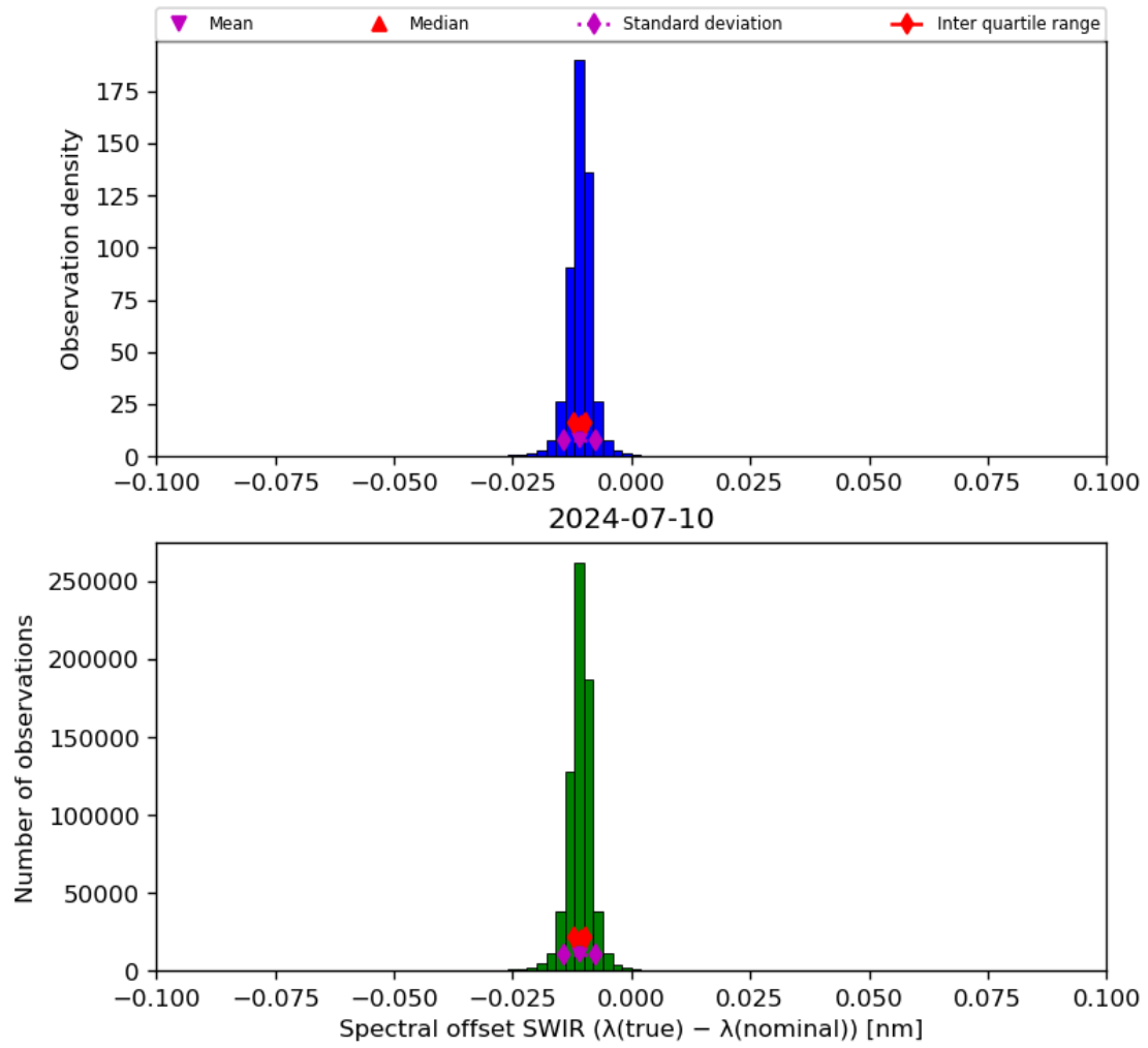
Figure 27: Histogram of “Spectral offset SWIR ( \lambda(\text{true}) - \lambda(\text{nominal}) )” for 2024-07-10 to 2024-07-11
