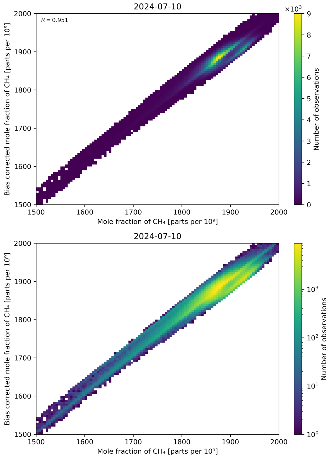
Figure 74: Scatter density plot of “Mole fraction of CH 4 ” against “Bias corrected mole fraction of CH 4 ” for 2024-07-10 to 2024-07-11.
