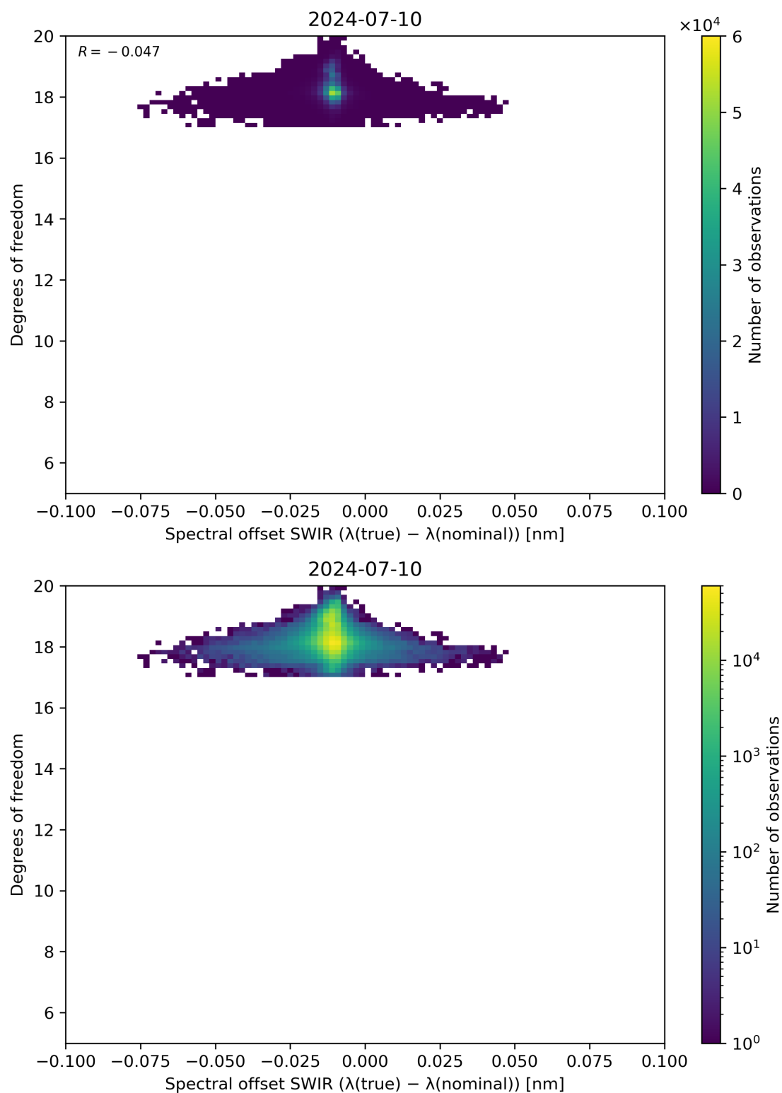
Figure 119: Scatter density plot of “Spectral offset SWIR ( \lambda(\text{true}) - \lambda(\text{nominal}) )” against “Degrees of freedom” for 2024-07-10 to 2024-07-11.
