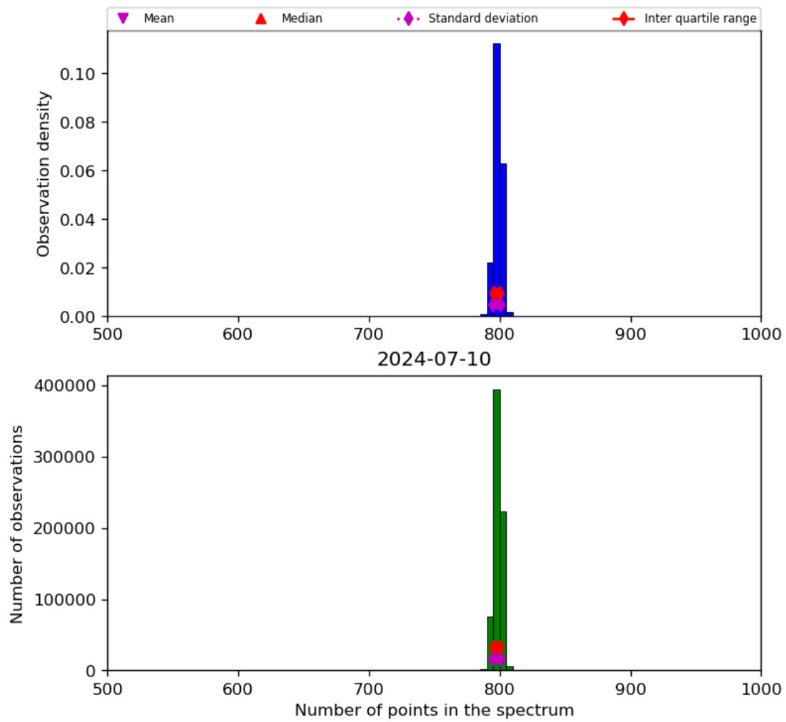
Figure 26: Histogram of “Number of points in the spectrum” for 2024-07-10 to 2024-07-11
