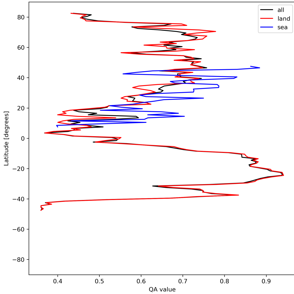
Figure 11: Zonal average of “QA value” for 2024-07-10 to 2024-07-11.
