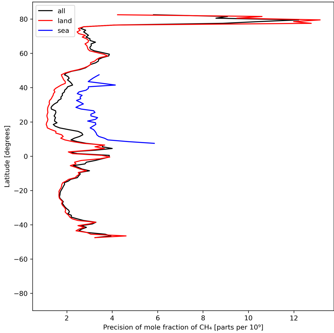
Figure 13: Zonal average of “Precision of mole fraction of CH 4 ” for 2024-07-10 to 2024-07-11.
