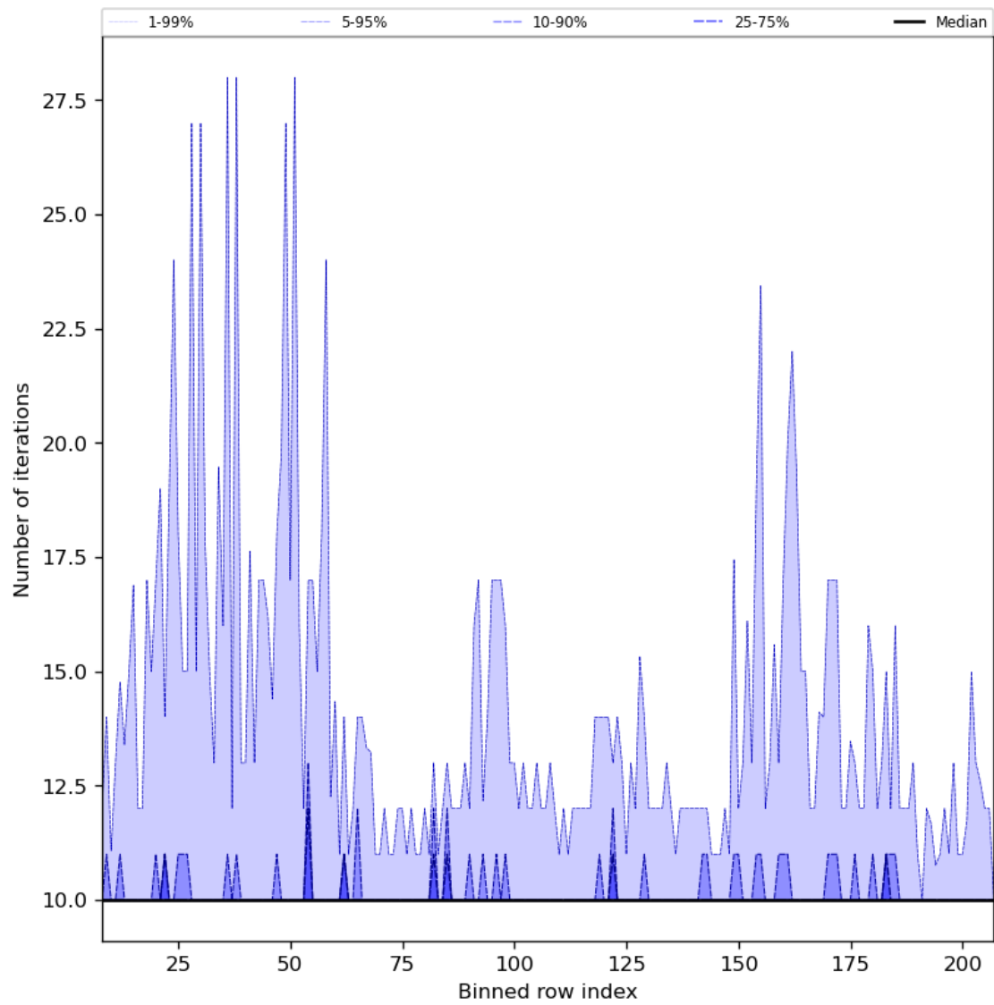
Figure 42: Along track statistics of “Number of iterations” for 2024-07-10 to 2024-07-11
