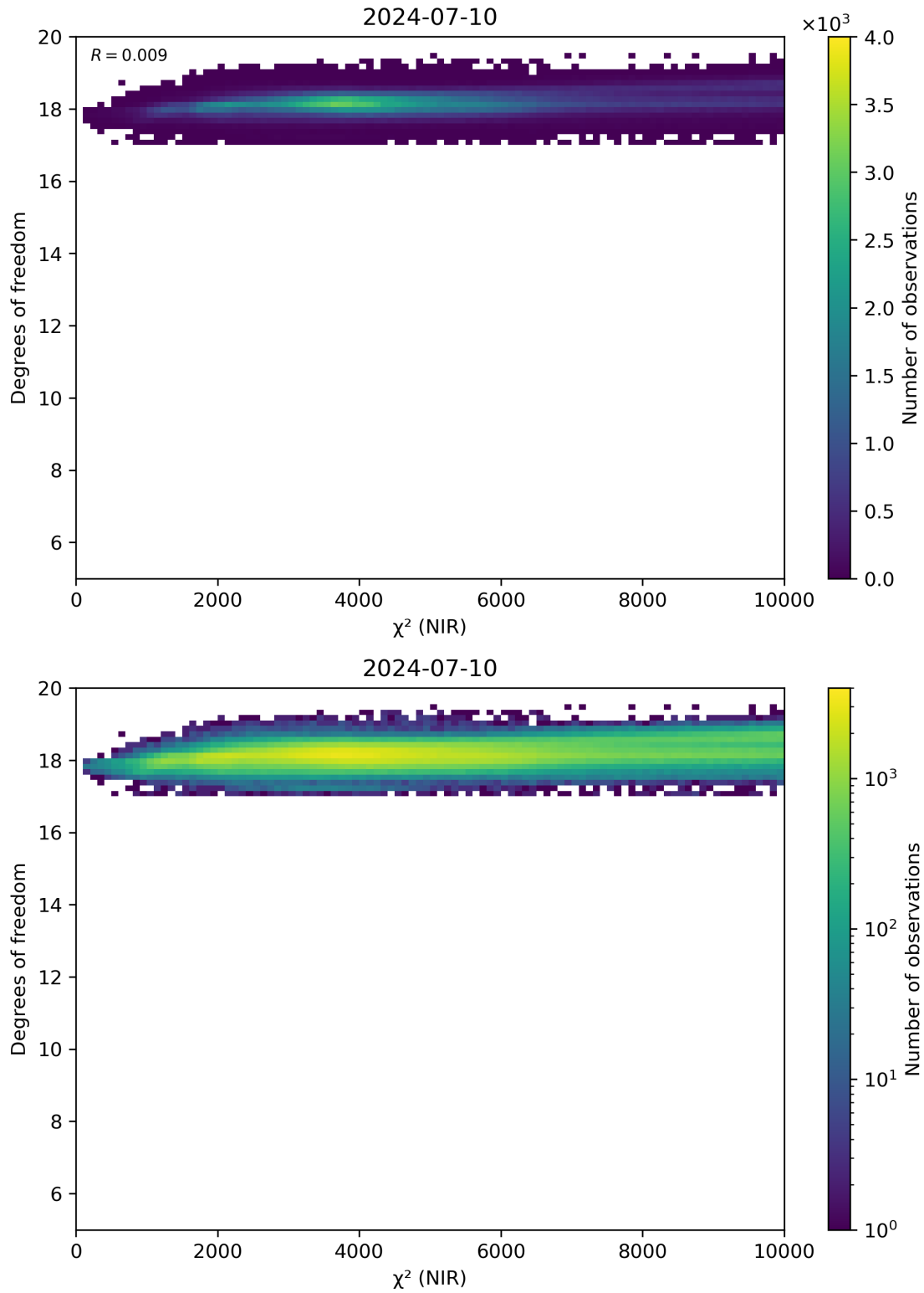
Figure 44: Scatter density plot of “ \chi^2 (NIR)” against “Degrees of freedom” for 2024-07-10 to 2024-07-11.
