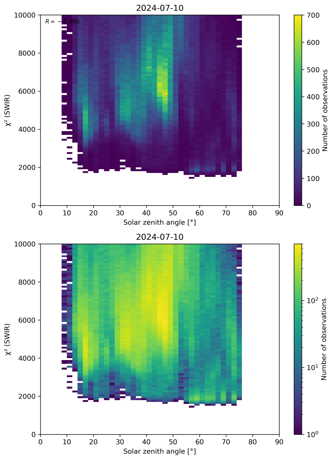
Figure 95: Scatter density plot of “Solar zenith angle” against “ \chi^2 (SWIR)” for 2024-07-10 to 2024-07-11.
