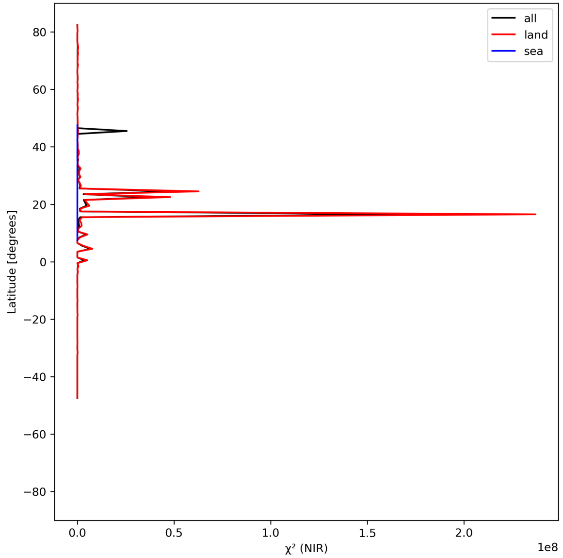
Figure 18: Zonal average of “ \chi^2 (NIR)” for 2024-07-10 to 2024-07-11.
