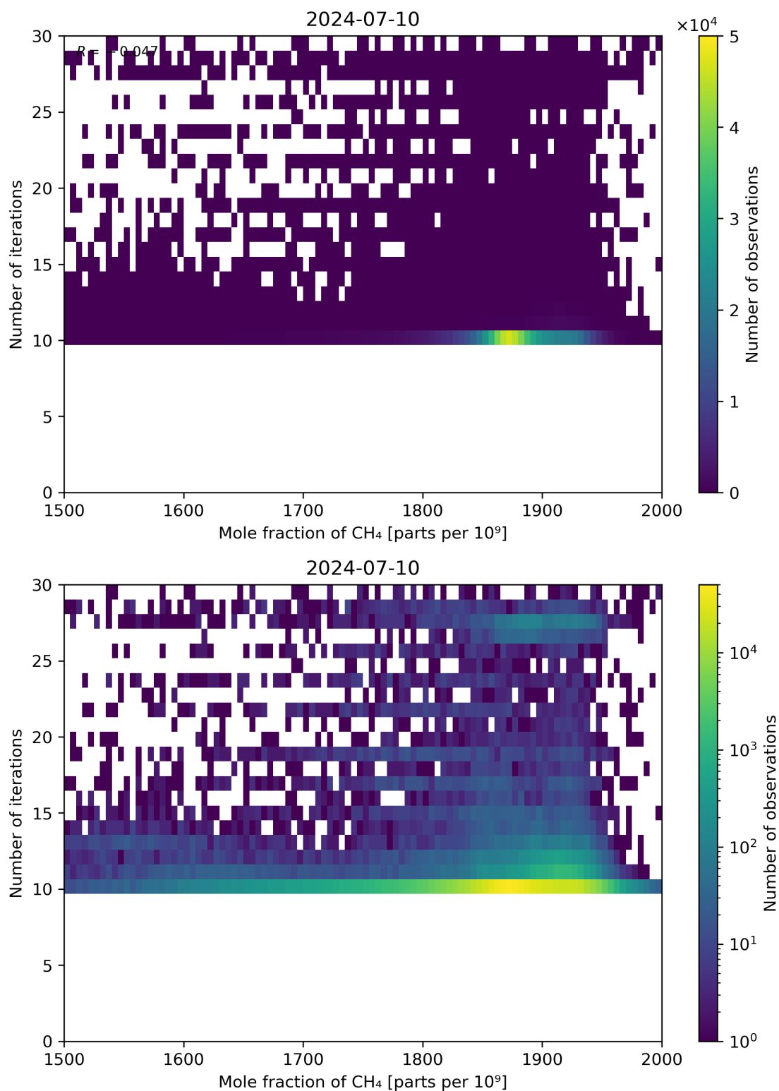
Figure 76: Scatter density plot of “Mole fraction of CH 4 ” against “Number of iterations” for 2024-07-10 to 2024-07-11.
