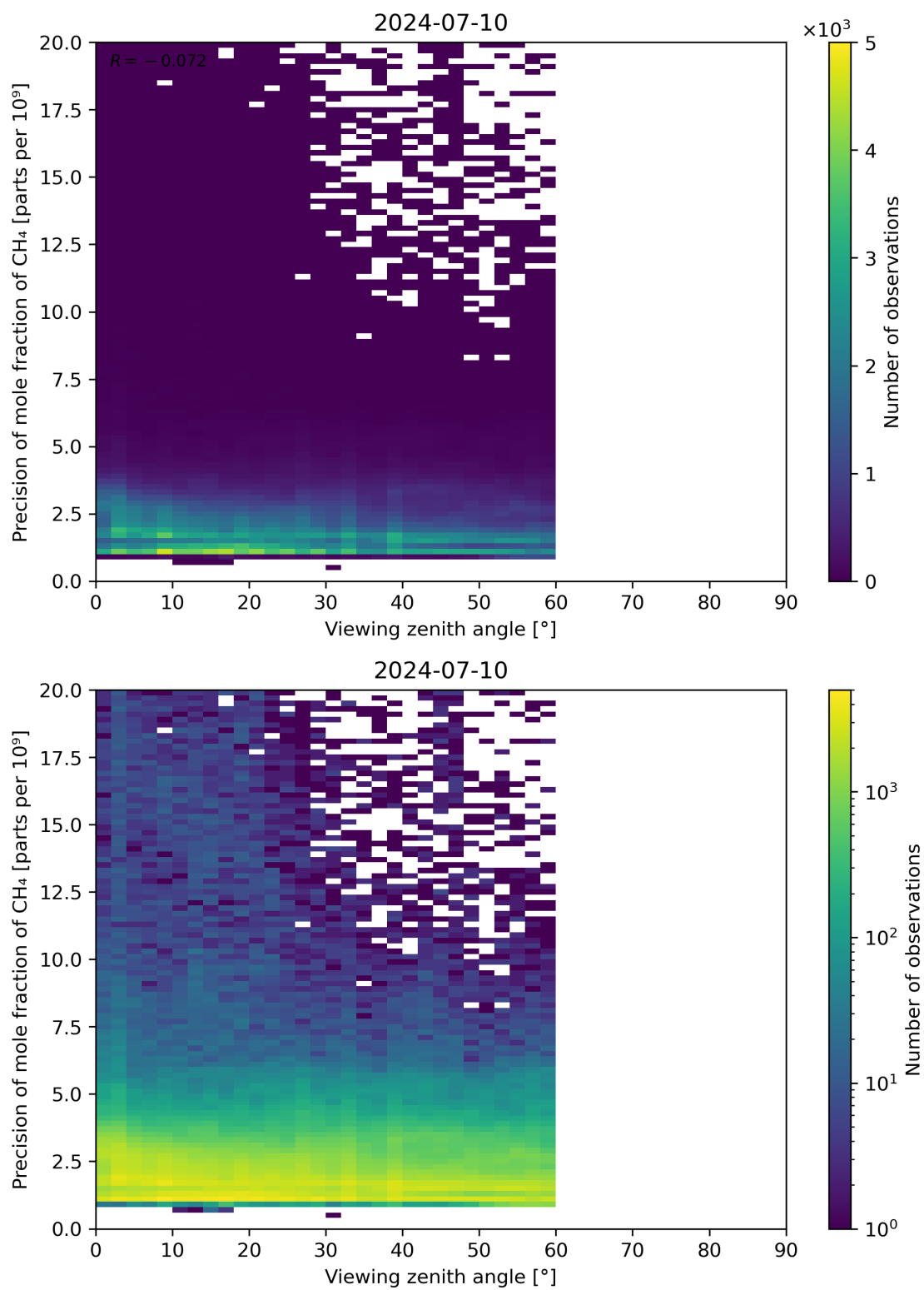
Figure 112: Scatter density plot of “Viewing zenith angle” against “Precision of mole fraction of CH 4 ” for 2024-07-10 to 2024-07-11.
