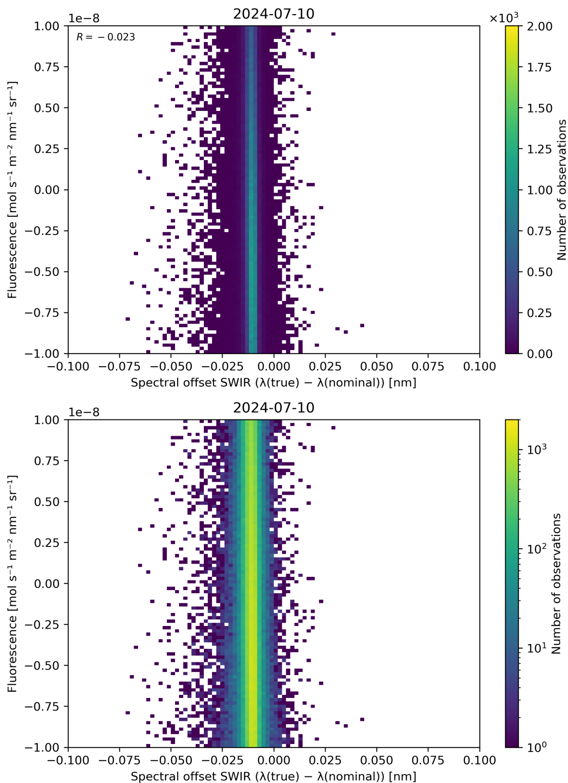
Figure 120: Scatter density plot of “Spectral offset SWIR ( \lambda(\text{true}) - \lambda(\text{nominal}) )” against “Fluorescence” for 2024-07-10 to 2024-07-11.
