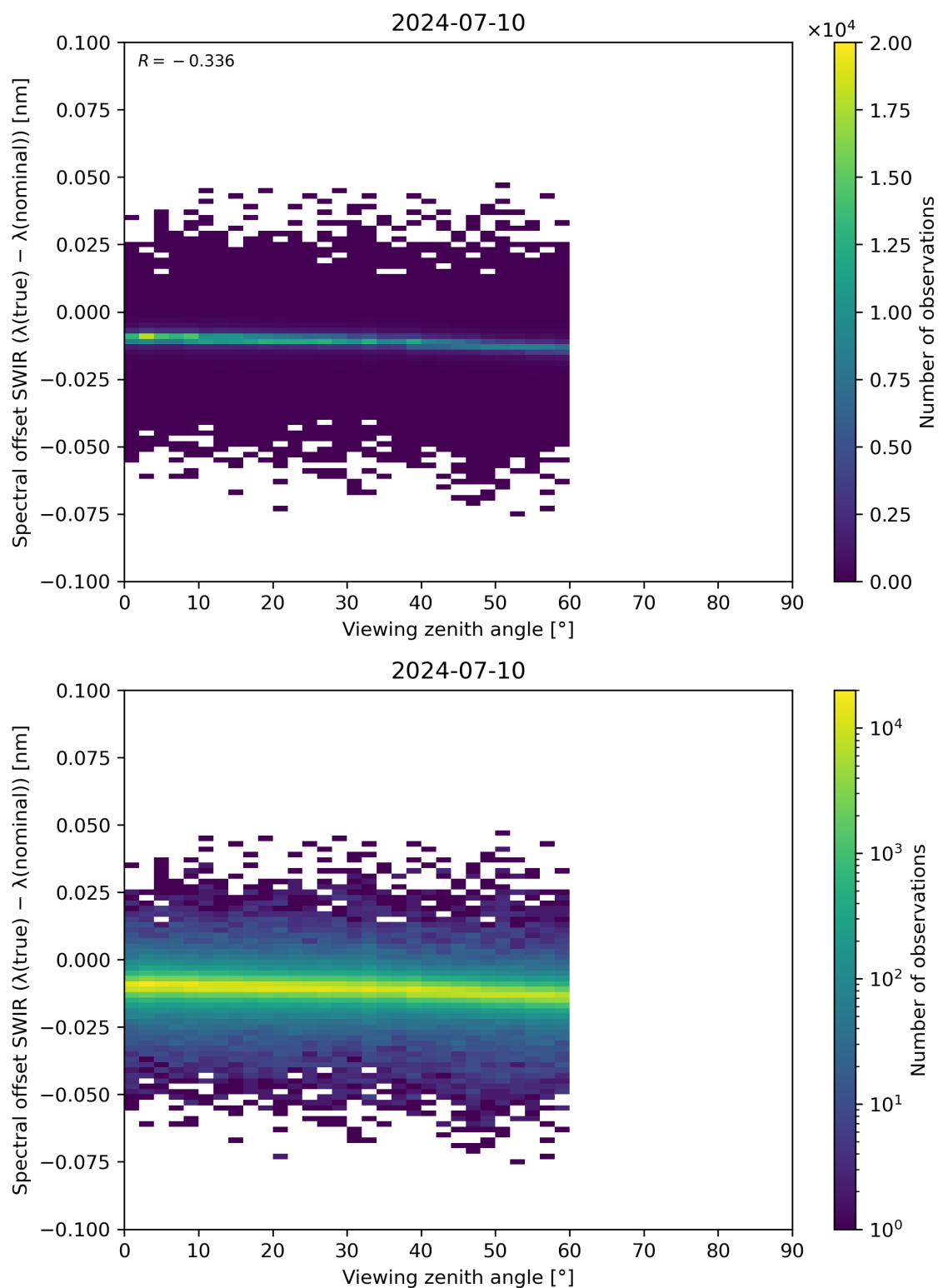
Figure 116: Scatter density plot of “Viewing zenith angle” against “Spectral offset SWIR ( \lambda(\text{true}) - \lambda(\text{nominal}) )” for 2024-07-10 to 2024-07-11.
