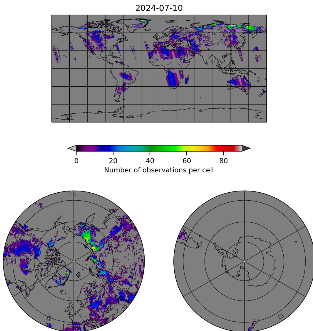
Figure 10: Map of the number of observations for 2024-07-10 to 2024-07-11
