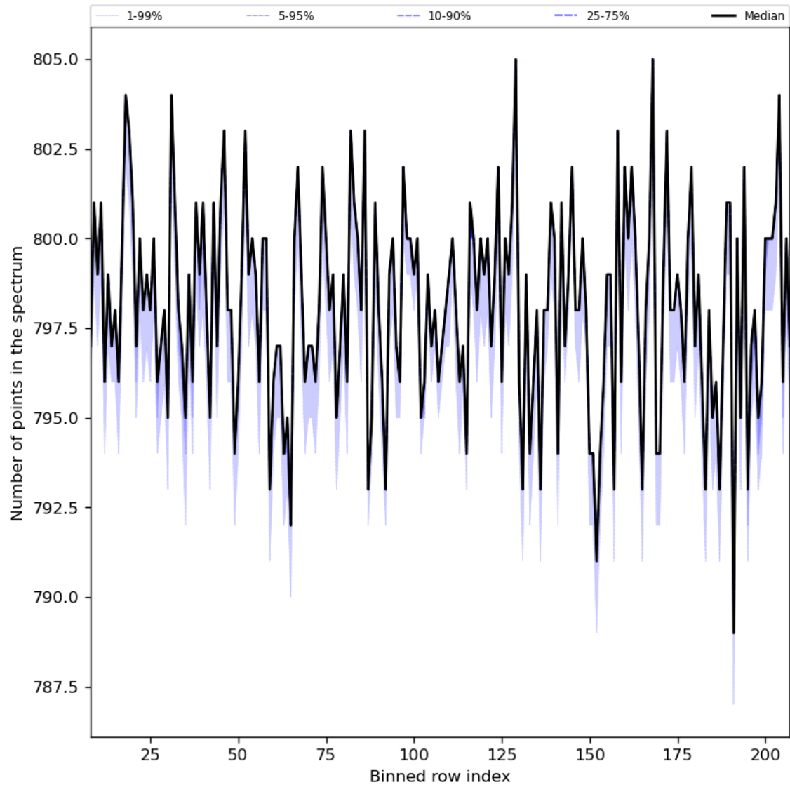
Figure 37: Along track statistics of “Number of points in the spectrum” for 2024-07-10 to 2024-07-11
