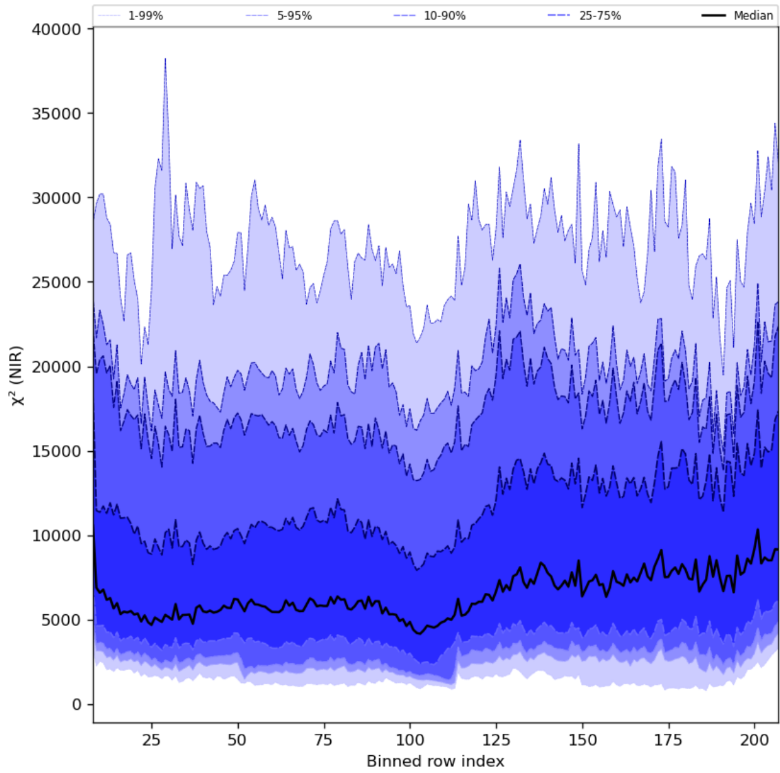
Figure 40: Along track statistics of “ \chi^2 (NIR)” for 2024-07-10 to 2024-07-11
