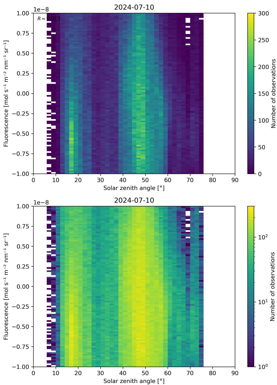
Figure 97: Scatter density plot of “Solar zenith angle” against “Fluorescence” for 2024-07-10 to 2024-07-11.
