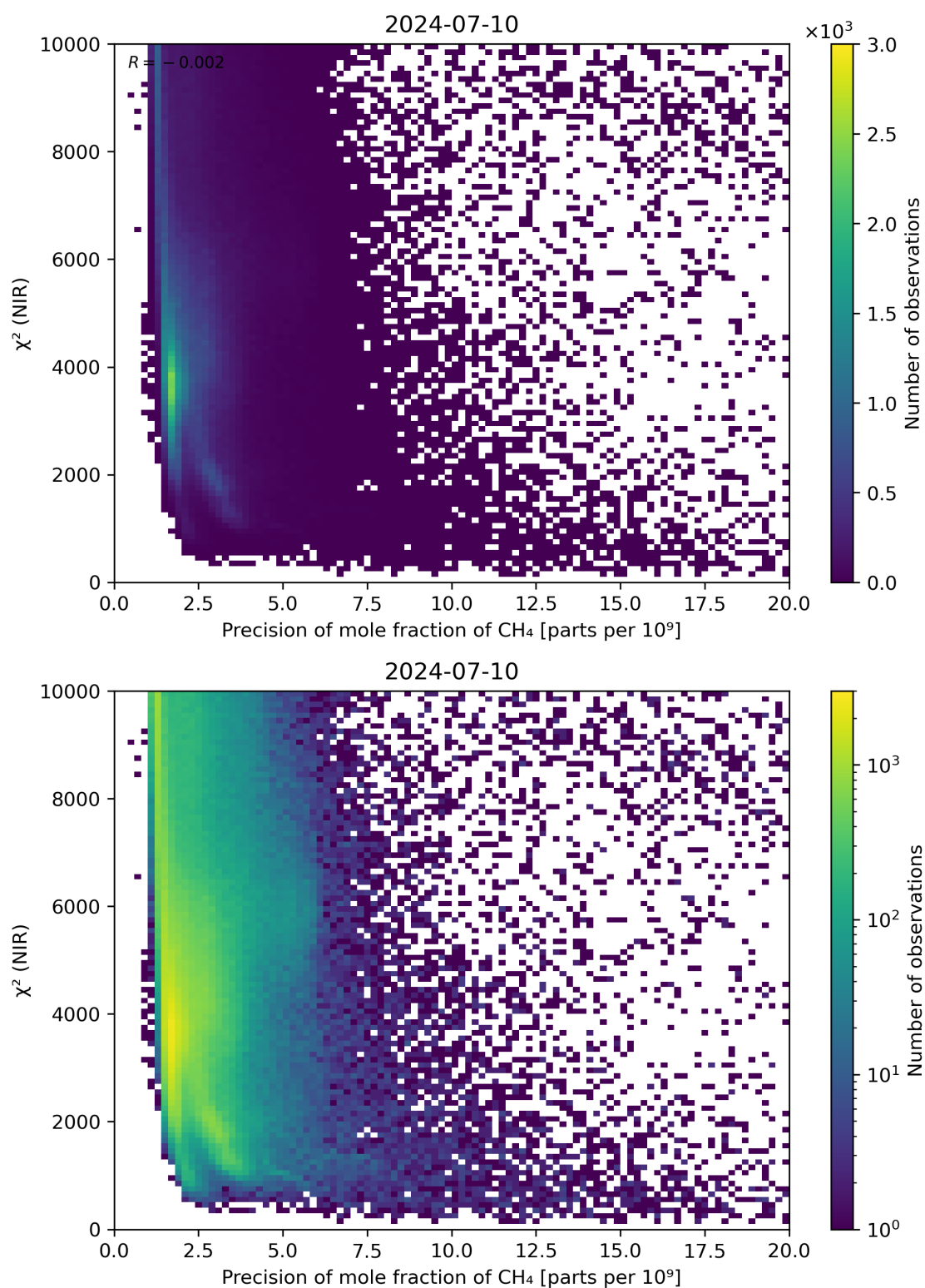
Figure 78: Scatter density plot of “Precision of mole fraction of CH 4 ” against “ \chi^2 (NIR)” for 2024-07-10 to 2024-07-11.
