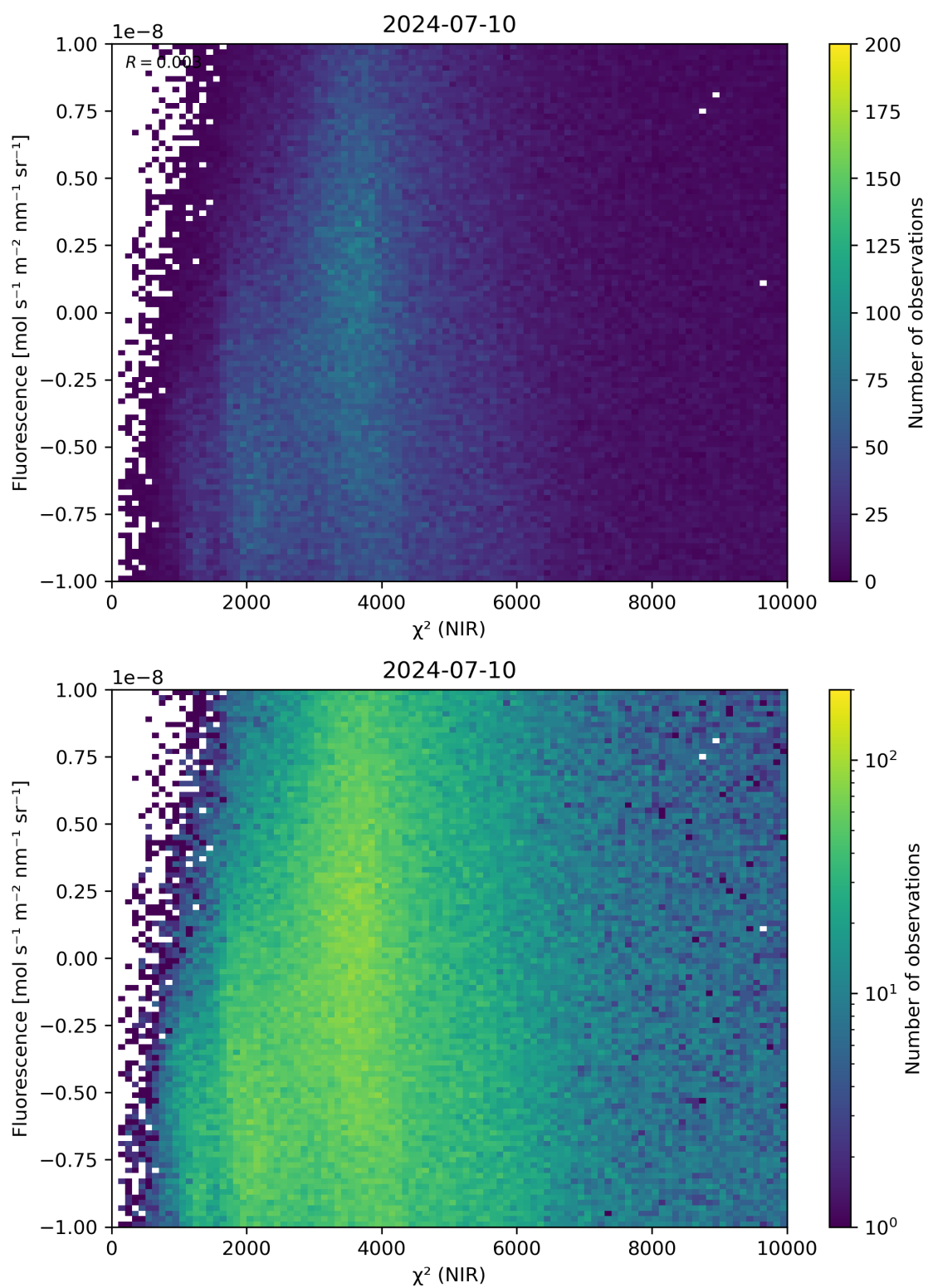
Figure 45: Scatter density plot of “ \chi^2 (NIR)” against “Fluorescence” for 2024-07-10 to 2024-07-11.
