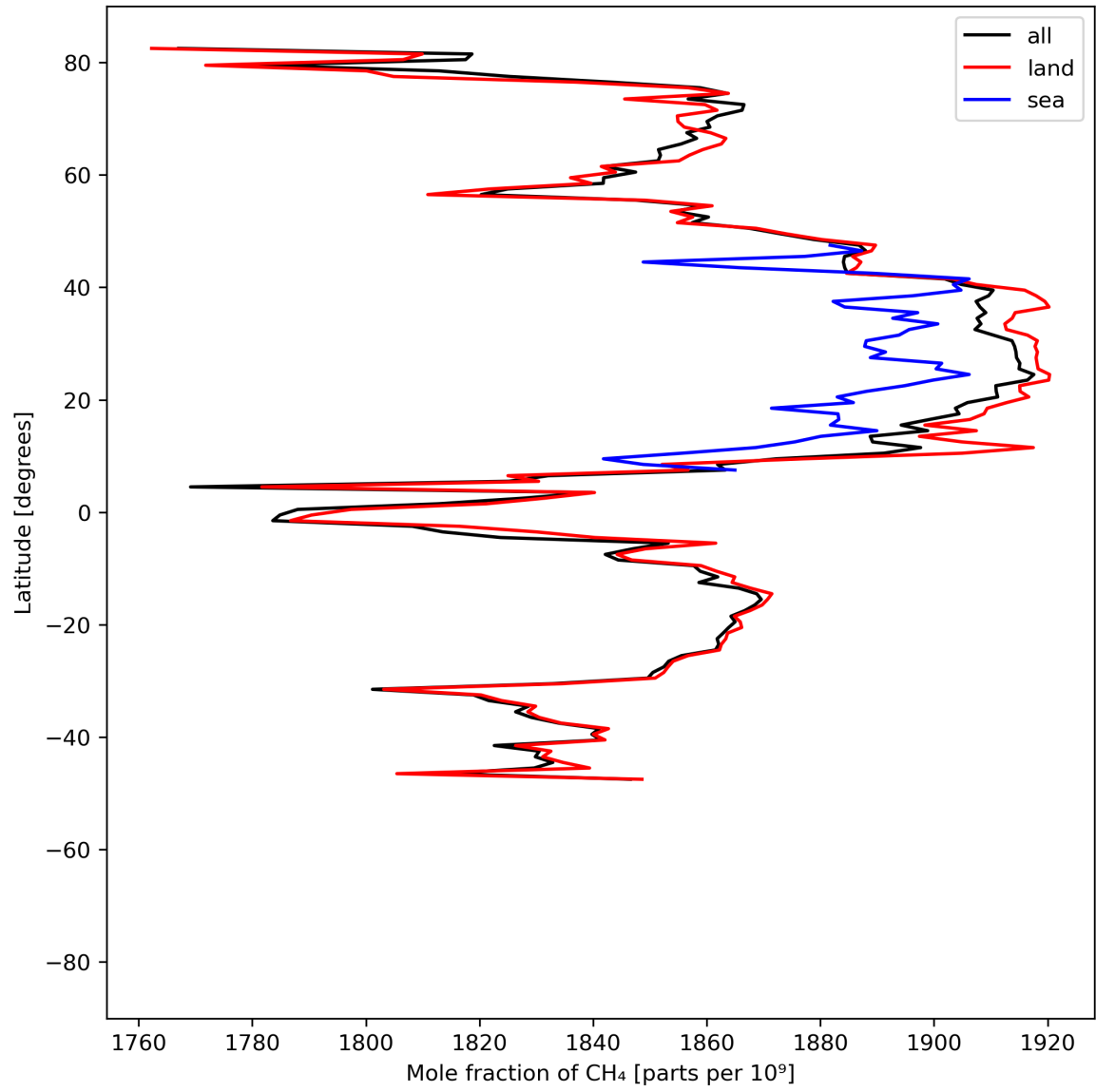
Figure 12: Zonal average of “Mole fraction of \text{CH}_4 ” for 2024-07-10 to 2024-07-11.
