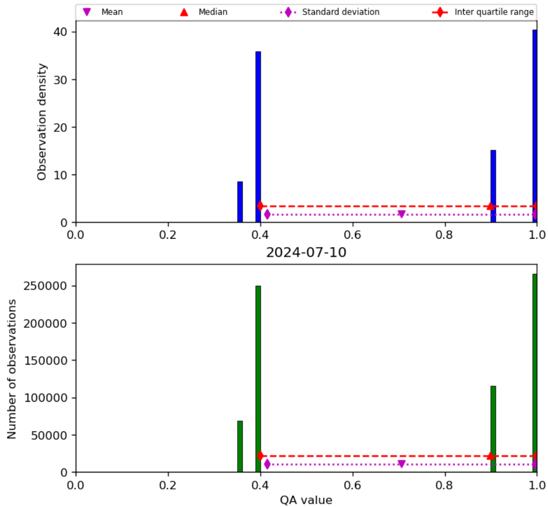
Figure 22: Histogram of “QA value” for 2024-07-10 to 2024-07-11
