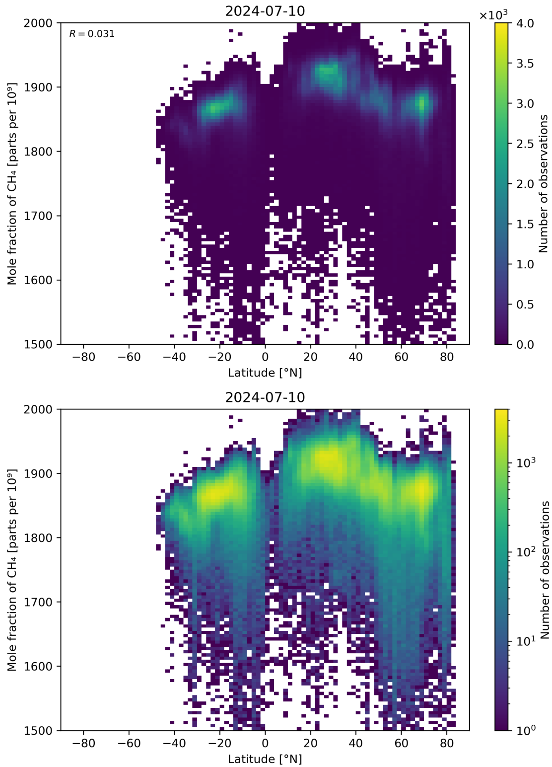
Figure 57: Scatter density plot of “Latitude” against “Mole fraction of \text{CH}_4 ” for 2024-07-10 to 2024-07-11.
