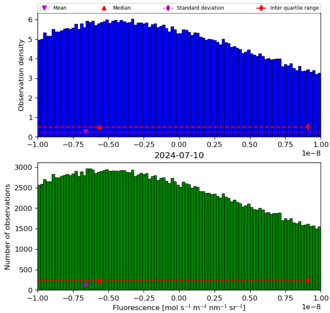
Figure 32: Histogram of “Fluorescence” for 2024-07-10 to 2024-07-11
