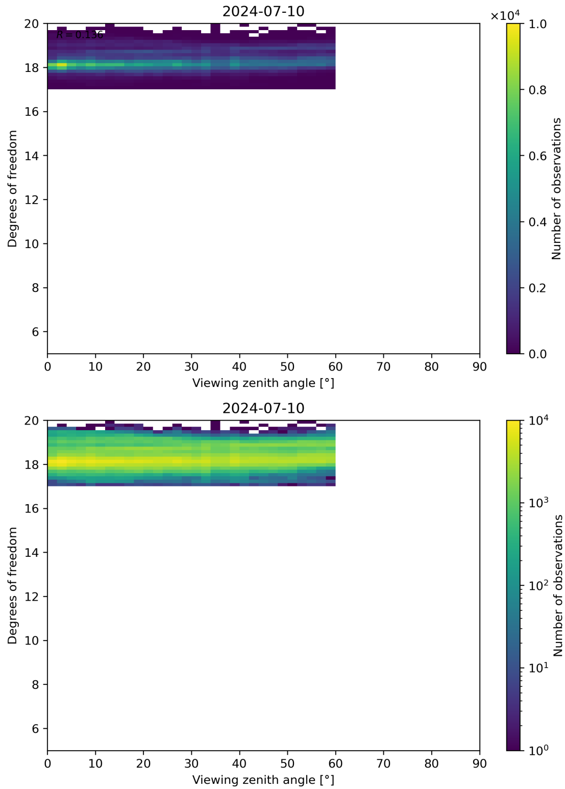
Figure 107: Scatter density plot of “Viewing zenith angle” against “Degrees of freedom” for 2024-07-10 to 2024-07-11.
