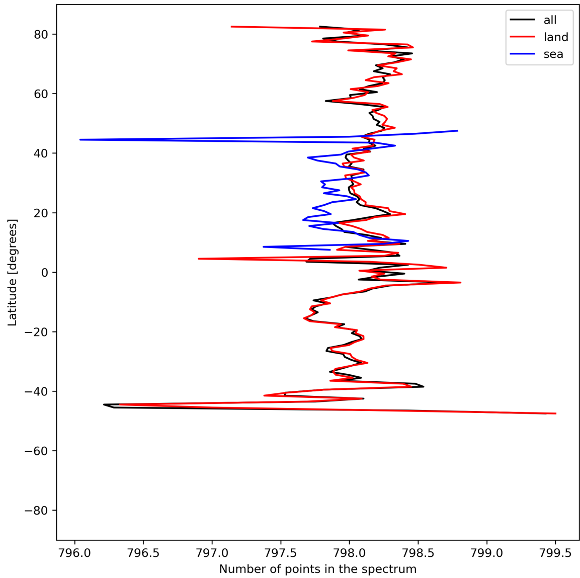
Figure 15: Zonal average of “Number of points in the spectrum” for 2024-07-10 to 2024-07-11.
