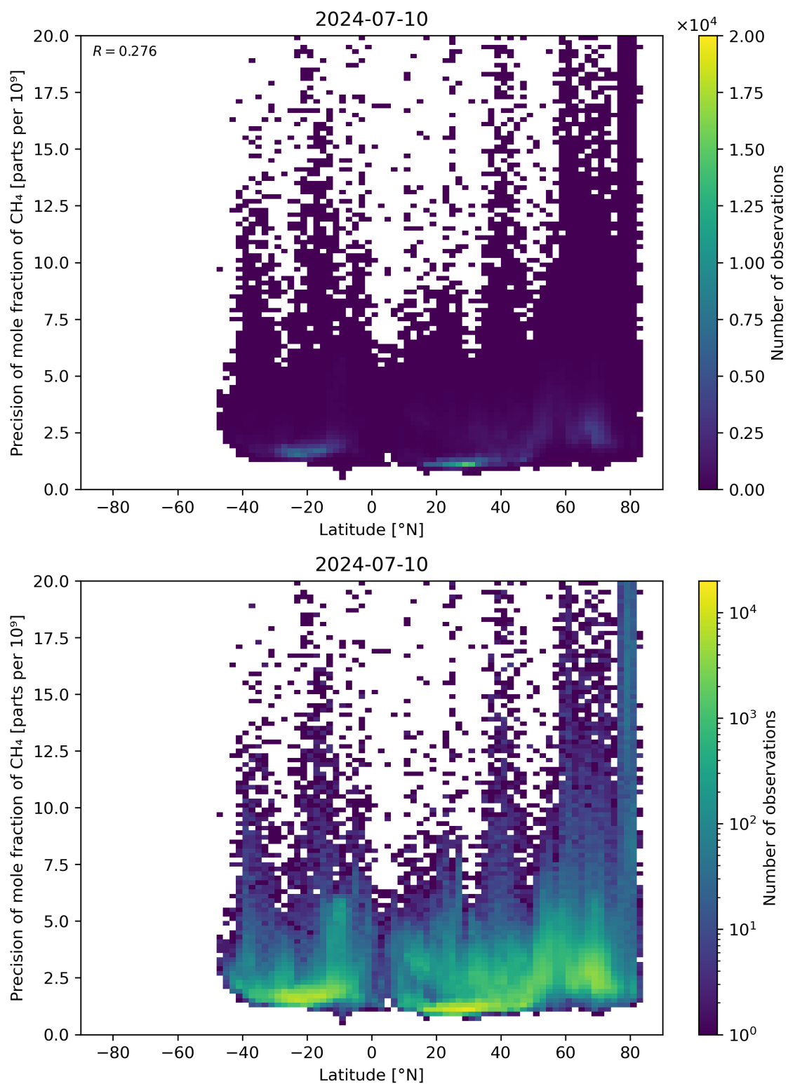
Figure 59: Scatter density plot of “Latitude” against “Precision of mole fraction of \text{CH}_4 ” for 2024-07-10 to 2024-07-11.
