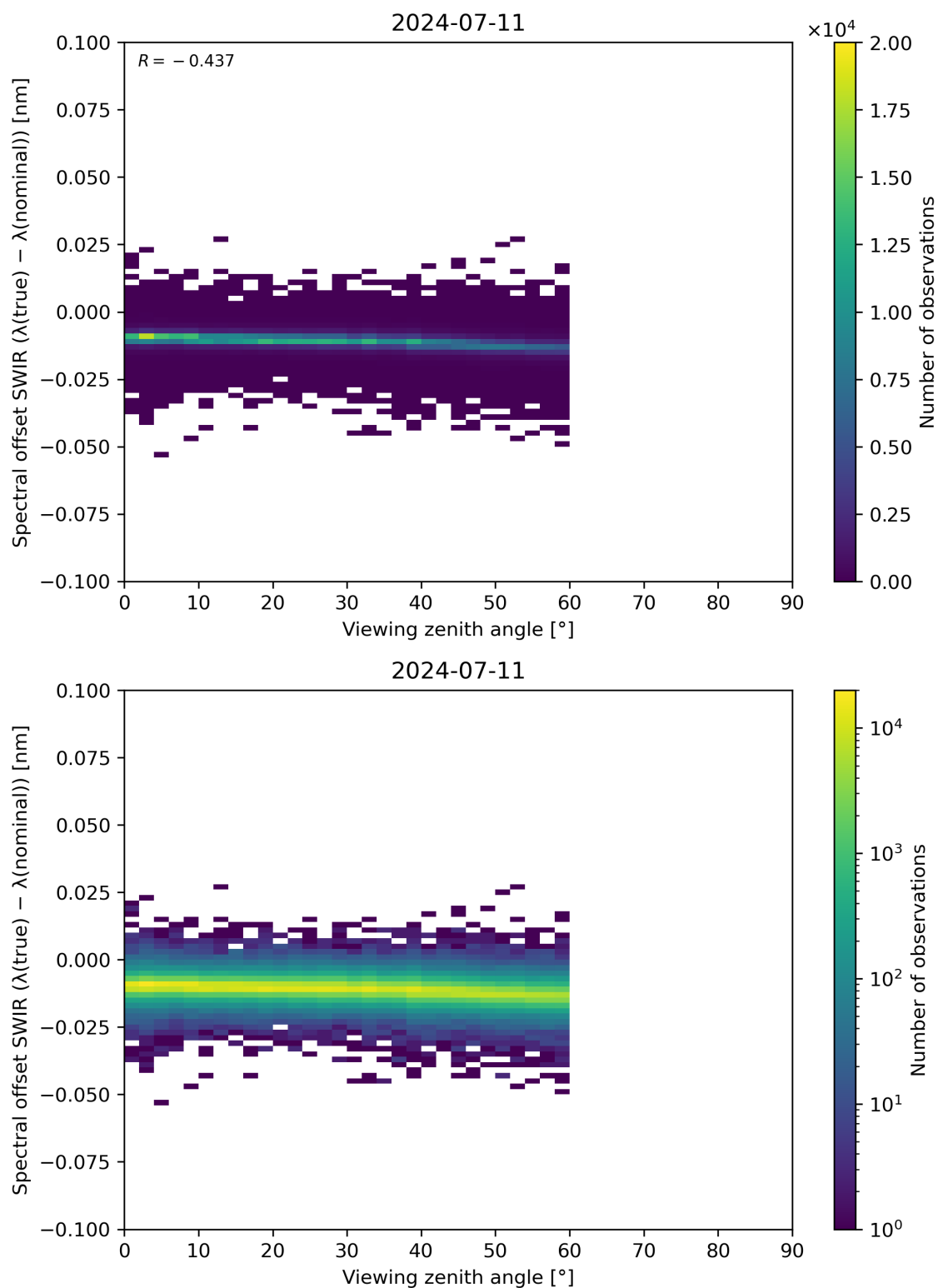
Figure 116: Scatter density plot of “Viewing zenith angle” against “Spectral offset SWIR ( \lambda(\text{true}) - \lambda(\text{nominal}) )” for 2024-07-10 to 2024-07-12.
