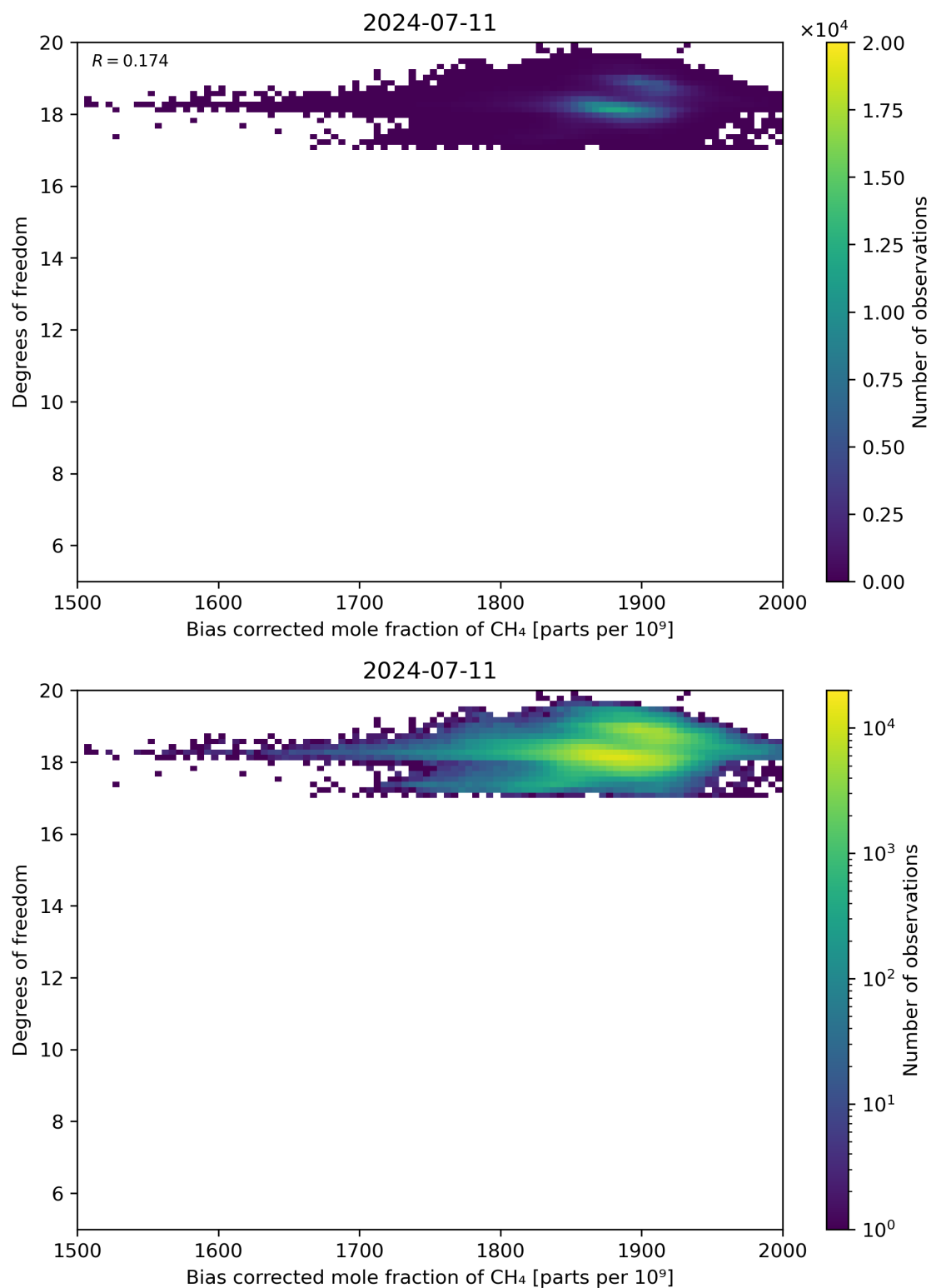
Figure 65: Scatter density plot of “Bias corrected mole fraction of CH 4 ” against “Degrees of freedom” for 2024-07-10 to 2024-07-12.
