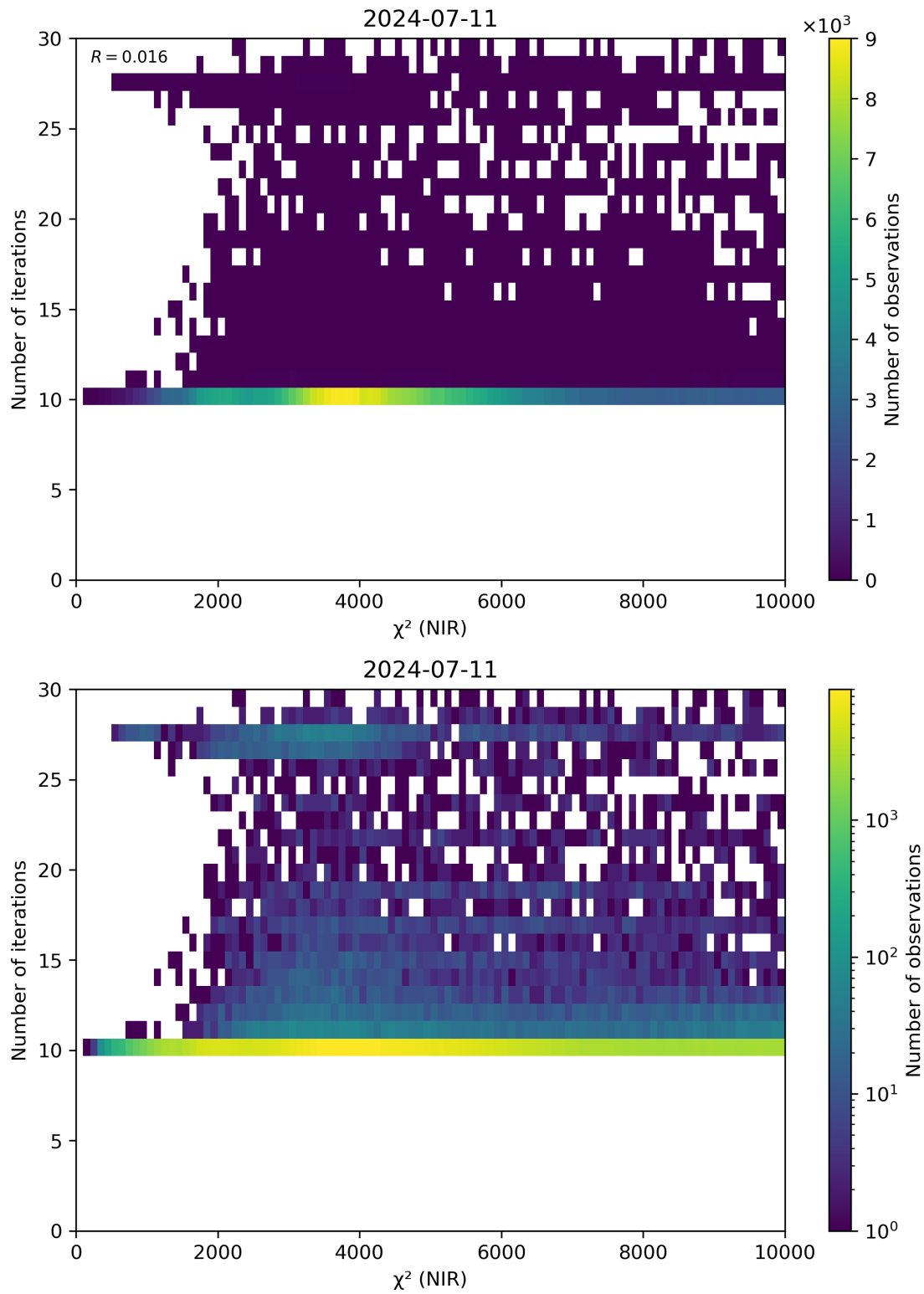
Figure 46: Scatter density plot of “ \chi^2 (NIR)” against “Number of iterations” for 2024-07-10 to 2024-07-12.
