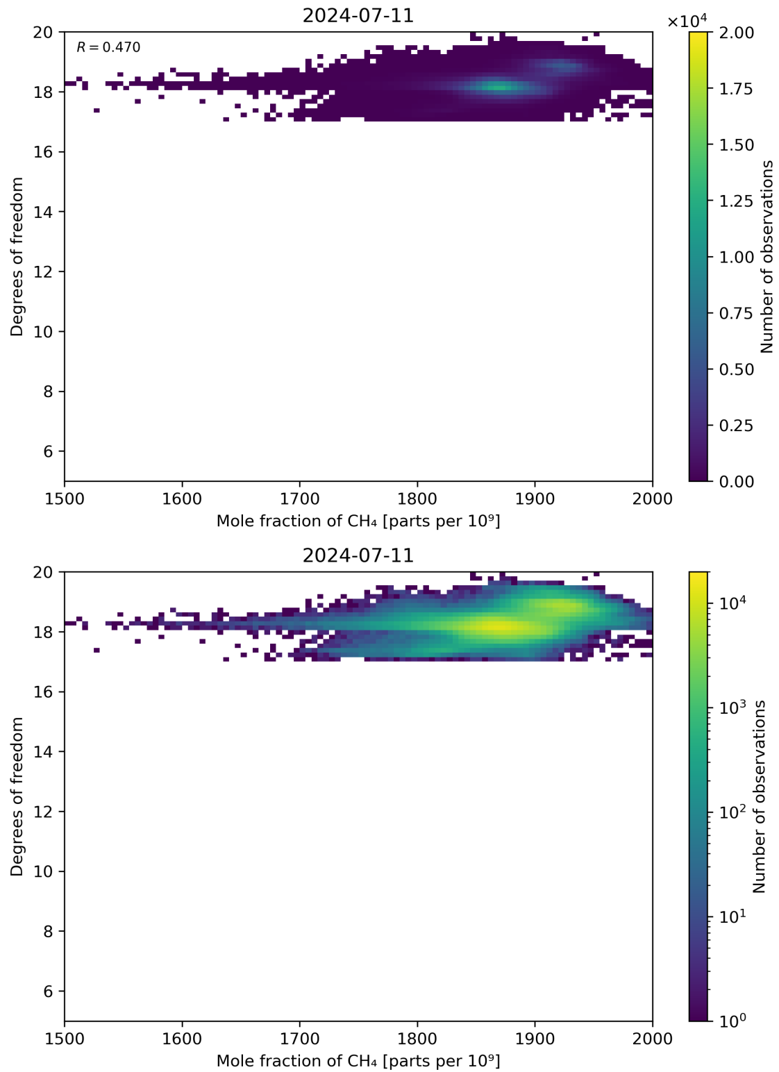
Figure 72: Scatter density plot of “Mole fraction of CH 4 ” against “Degrees of freedom” for 2024-07-10 to 2024-07-12.
