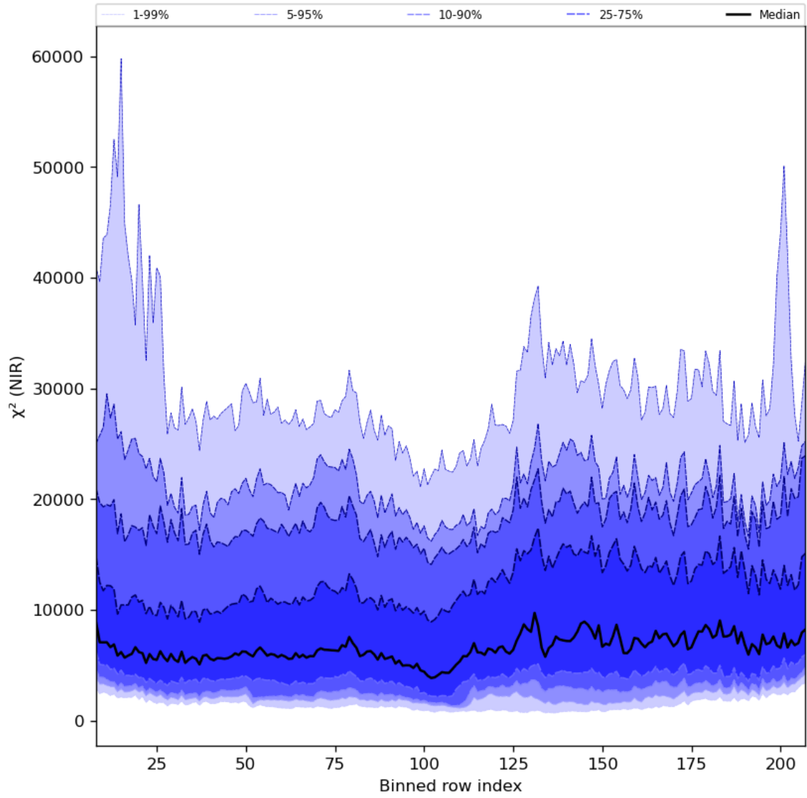
Figure 40: Along track statistics of “ \chi^2 (NIR)” for 2024-07-10 to 2024-07-12
