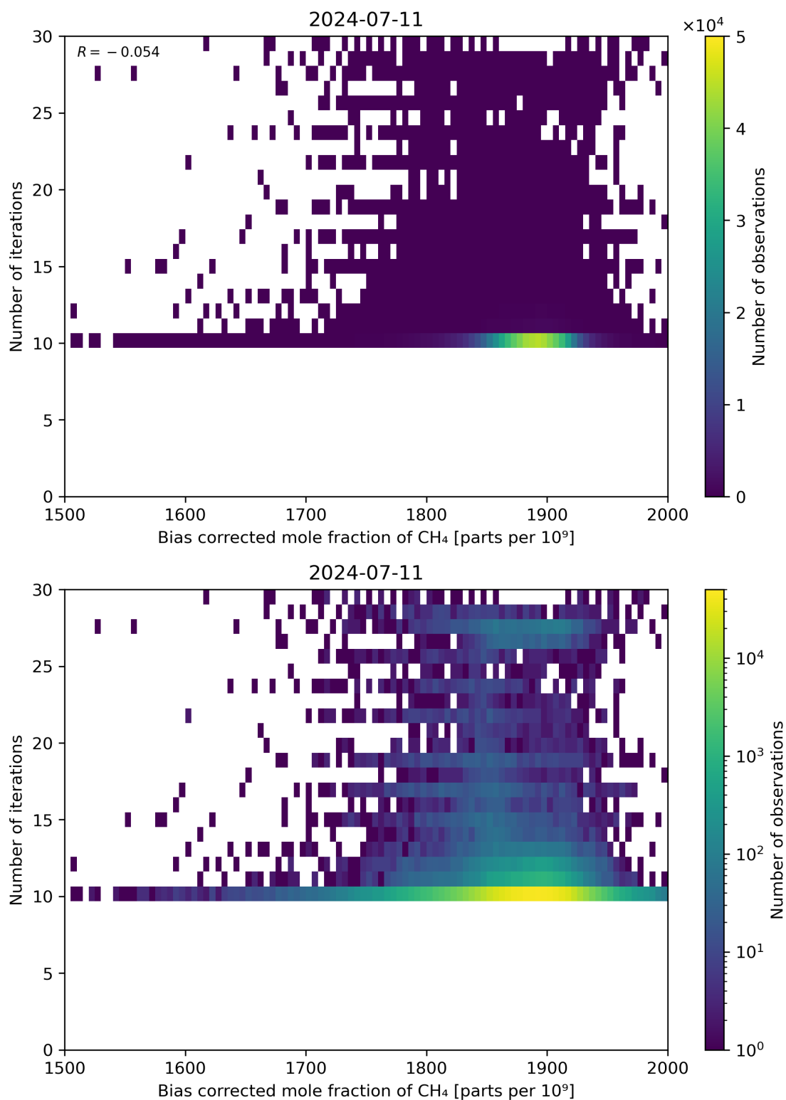
Figure 67: Scatter density plot of “Bias corrected mole fraction of CH 4 ” against “Number of iterations” for 2024-07-10 to 2024-07-12.
