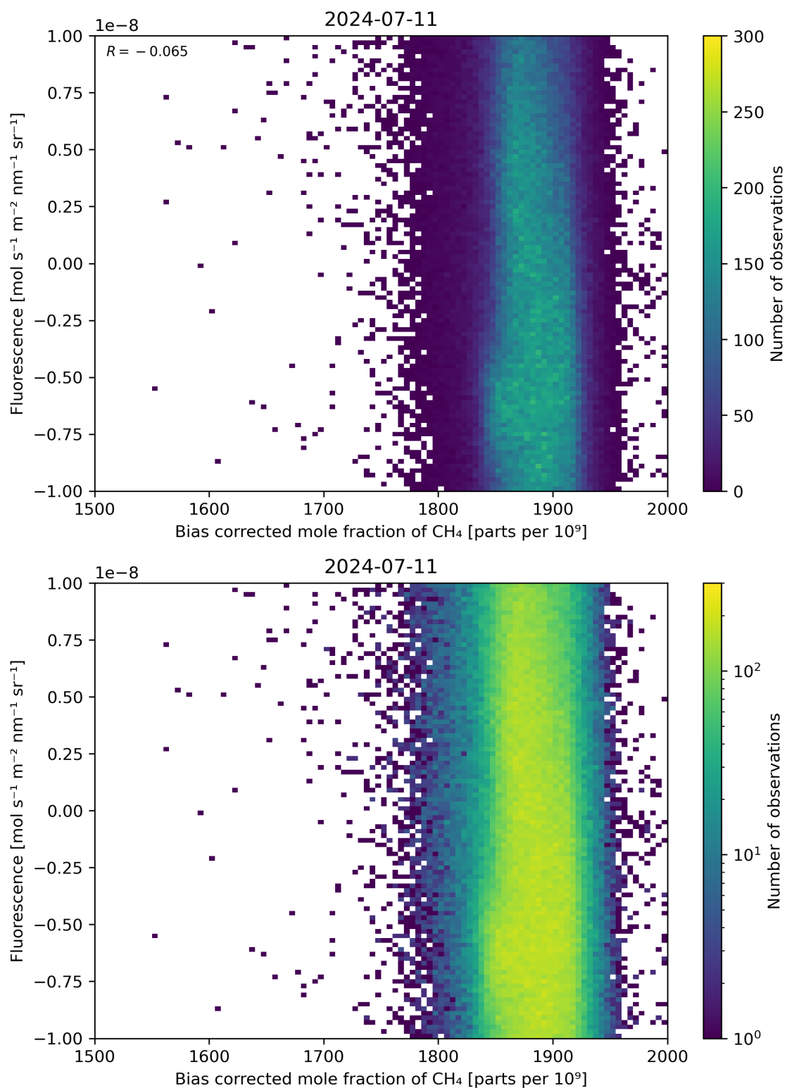
Figure 66: Scatter density plot of “Bias corrected mole fraction of \text{CH}_4 ” against “Fluorescence” for 2024-07-10 to 2024-07-12.
