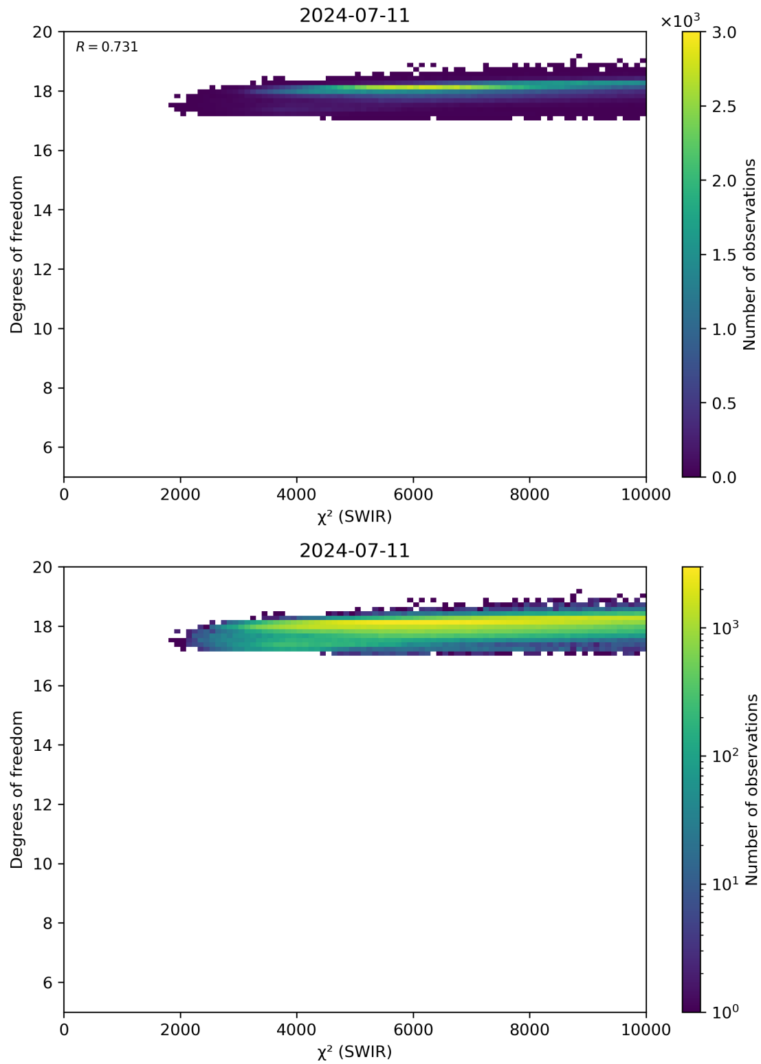
Figure 48: Scatter density plot of “ \chi^2 (SWIR)” against “Degrees of freedom” for 2024-07-10 to 2024-07-12.
