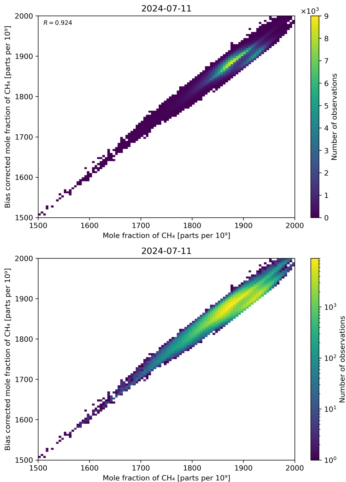
Figure 74: Scatter density plot of “Mole fraction of CH 4 ” against “Bias corrected mole fraction of CH 4 ” for 2024-07-10 to 2024-07-12.
