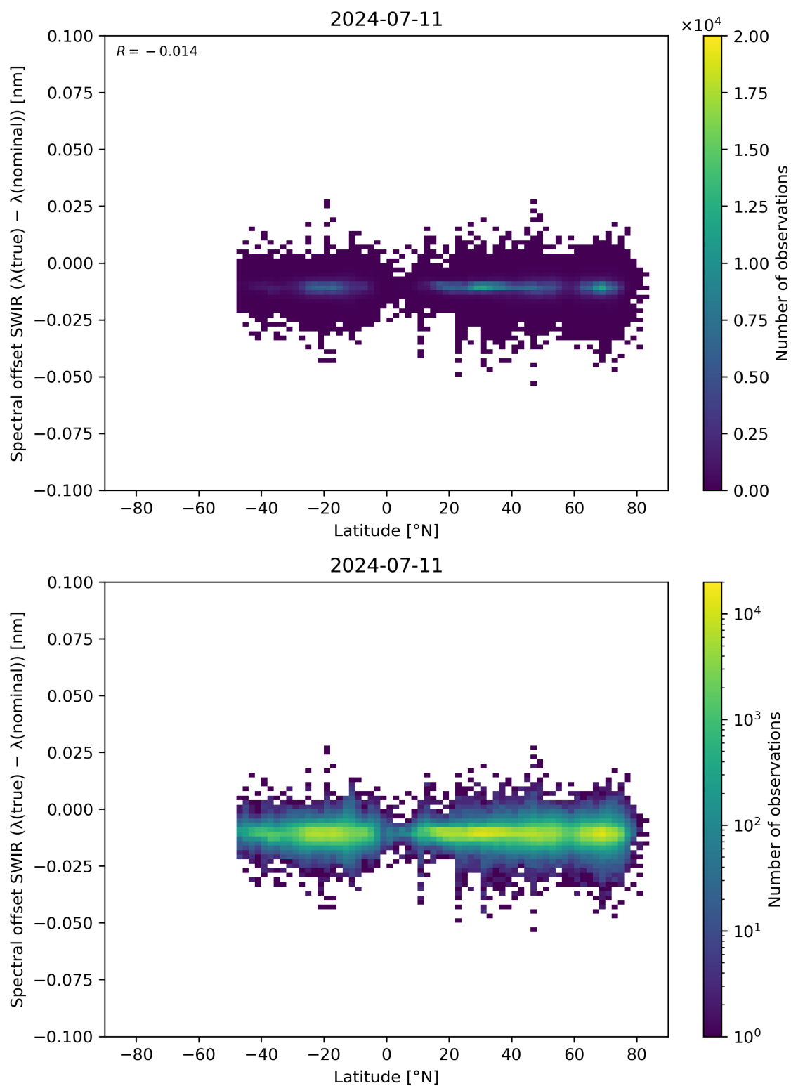
Figure 62: Scatter density plot of “Latitude” against “Spectral offset SWIR ( \lambda(\text{true}) - \lambda(\text{nominal}) )” for 2024-07-10 to 2024-07-12.
