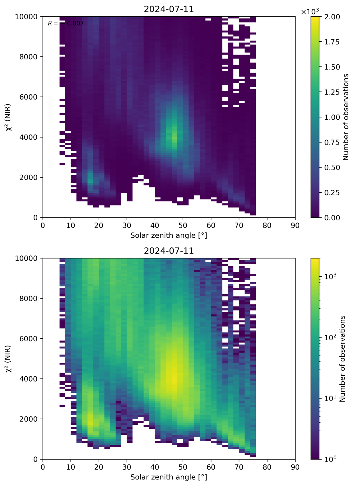
Figure 94: Scatter density plot of “Solar zenith angle” against “ \chi^2 (NIR)” for 2024-07-10 to 2024-07-12.
