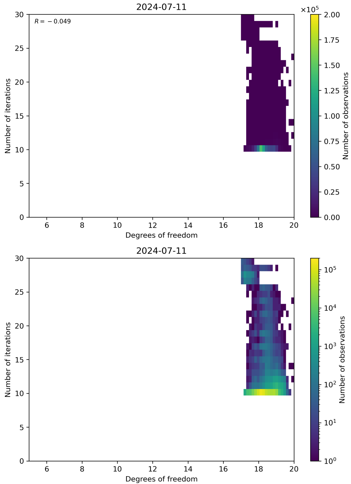
Figure 52: Scatter density plot of “Degrees of freedom” against “Number of iterations” for 2024-07-10 to 2024-07-12.
