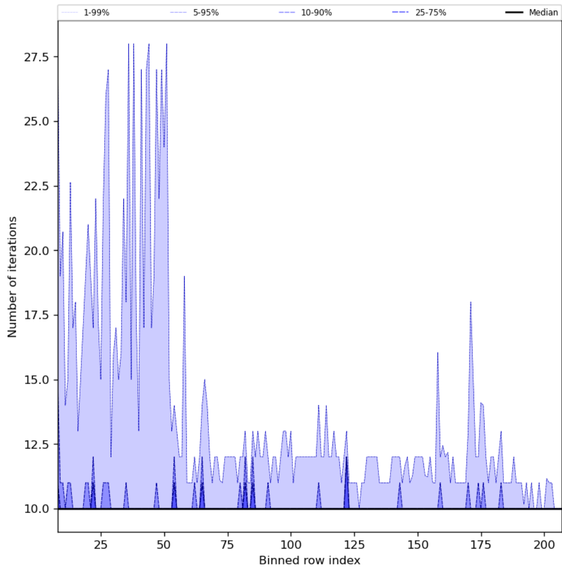
Figure 42: Along track statistics of “Number of iterations” for 2024-07-10 to 2024-07-12
