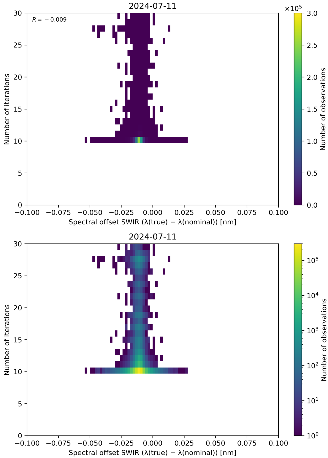
Figure 121: Scatter density plot of “Spectral offset SWIR ( \lambda(\text{true}) - \lambda(\text{nominal}) )” against “Number of iterations” for 2024-07-10 to 2024-07-12.
