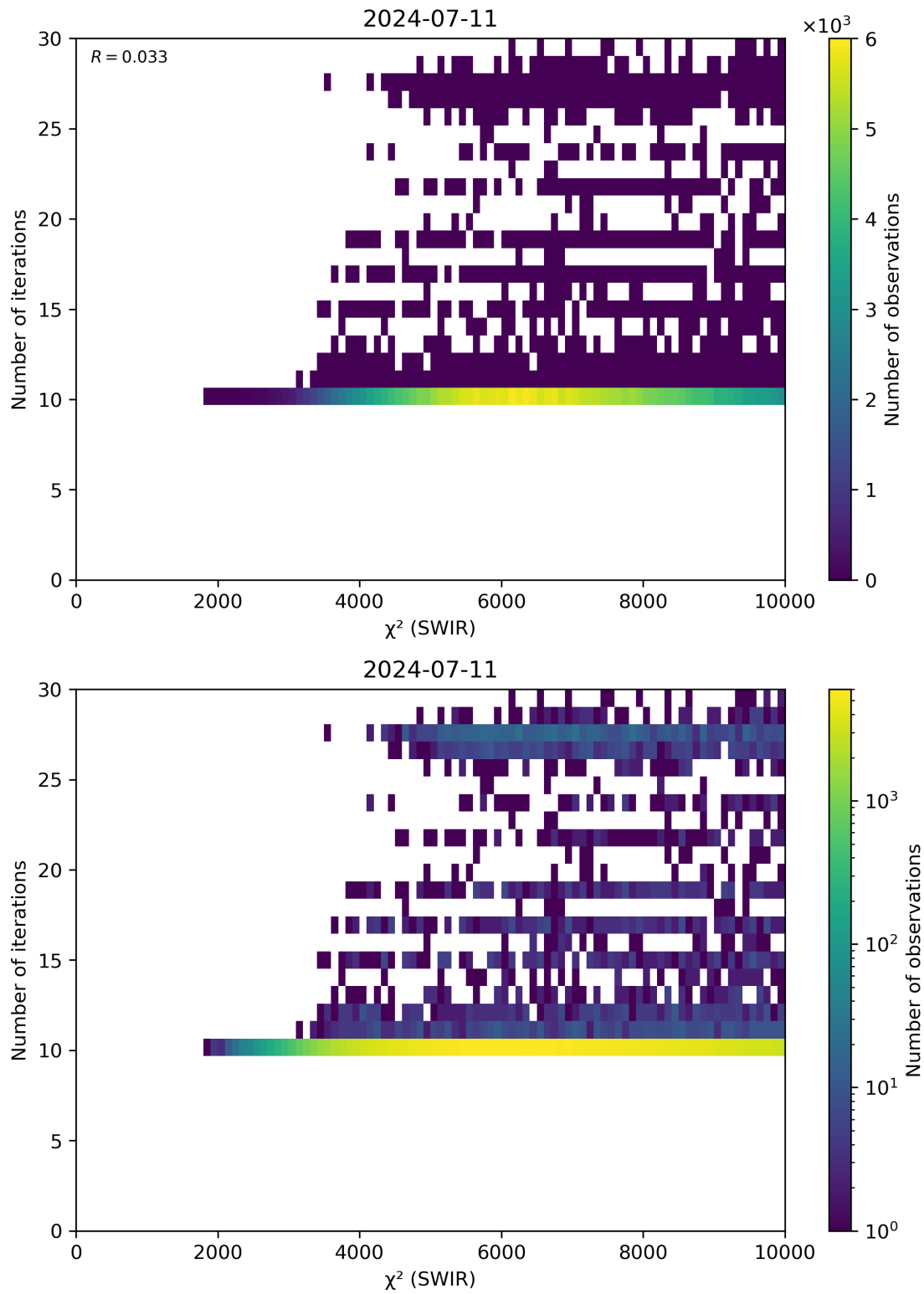
Figure 50: Scatter density plot of “ \chi^2 (SWIR)” against “Number of iterations” for 2024-07-10 to 2024-07-12.
