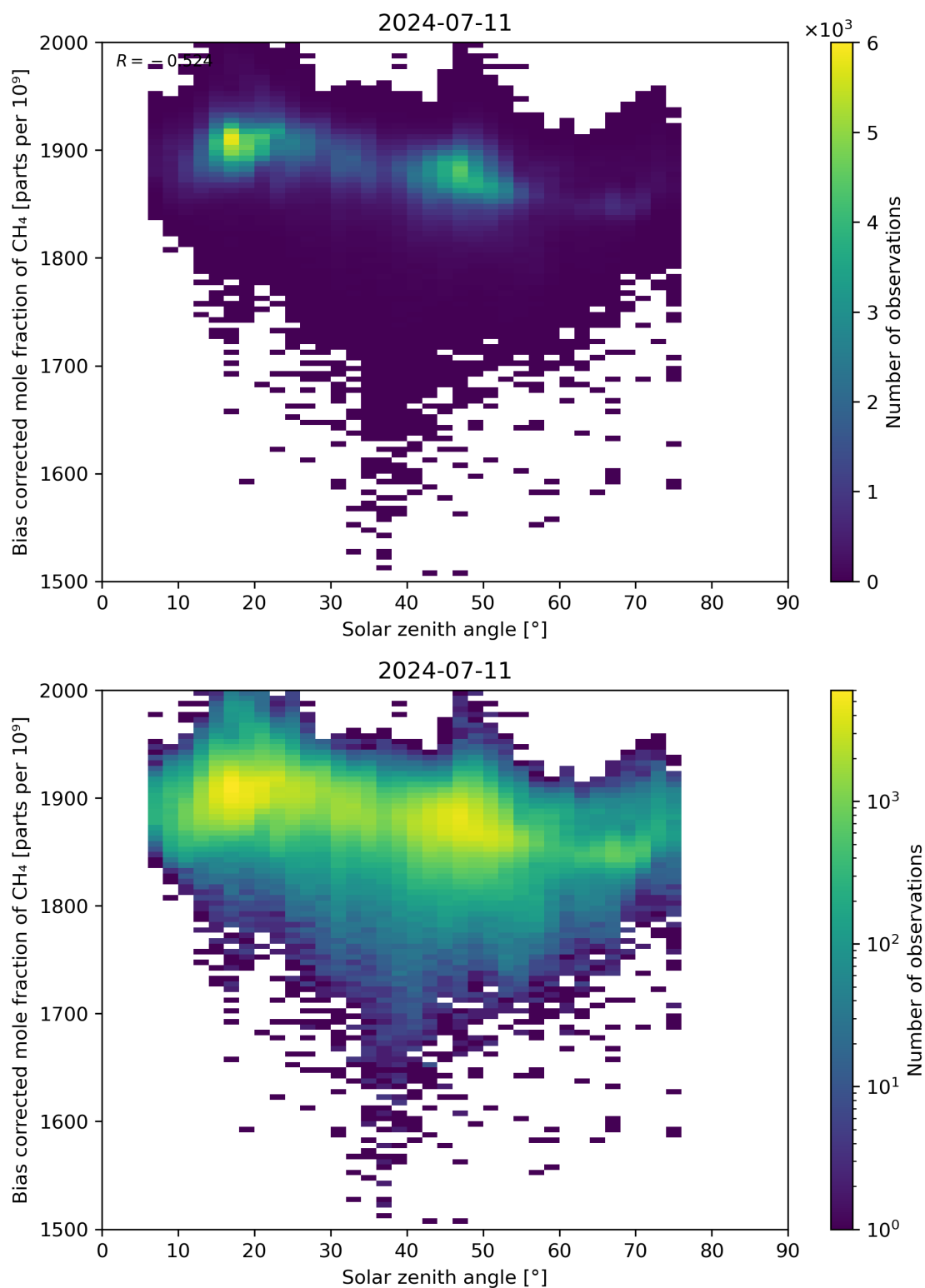
Figure 100: Scatter density plot of “Solar zenith angle” against “Bias corrected mole fraction of CH 4 ” for 2024-07-10 to 2024-07-12.
