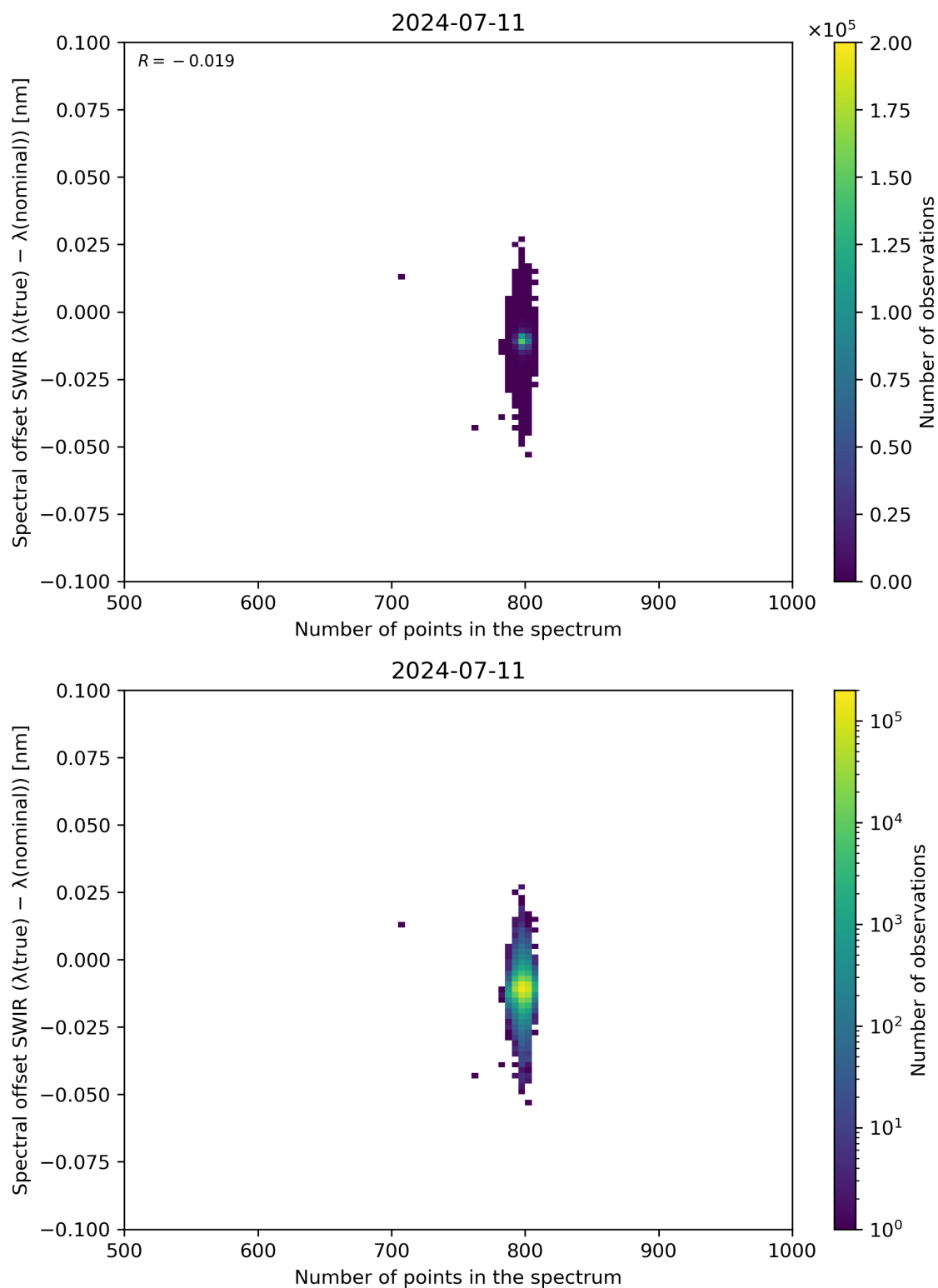
Figure 93: Scatter density plot of “Number of points in the spectrum” against “Spectral offset SWIR ( \lambda(\text{true}) - \lambda(\text{nominal}) )” for 2024-07-10 to 2024-07-12.
