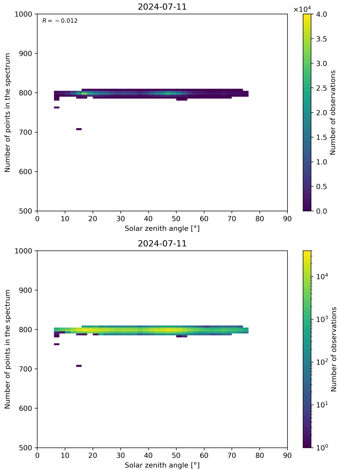
Figure 103: Scatter density plot of “Solar zenith angle” against “Number of points in the spectrum” for 2024-07-10 to 2024-07-12.
