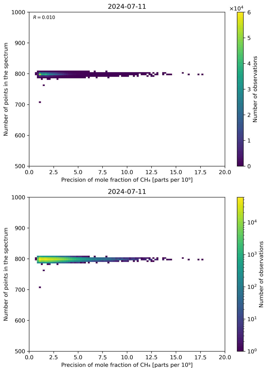
Figure 84: Scatter density plot of “Precision of mole fraction of CH 4 ” against “Number of points in the spectrum” for 2024-07-10 to 2024-07-12.
