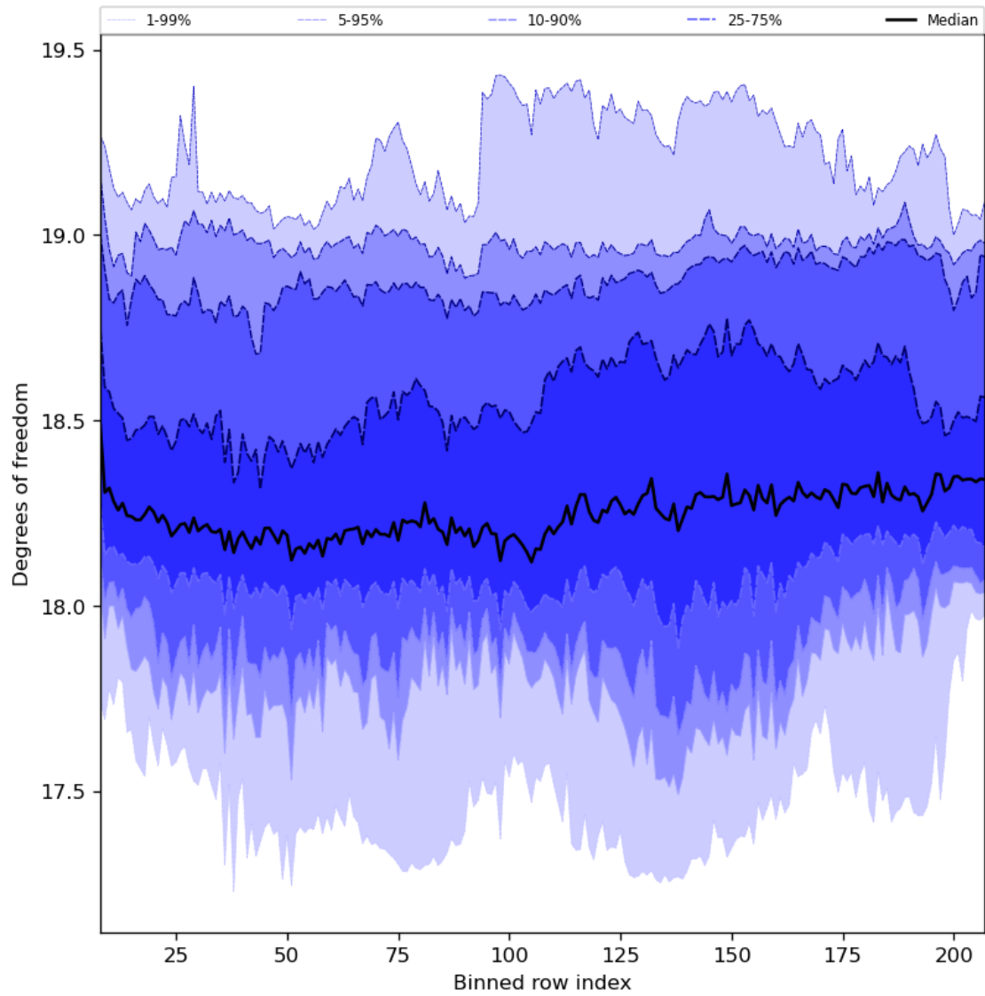
Figure 41: Along track statistics of “Degrees of freedom” for 2024-07-10 to 2024-07-12
