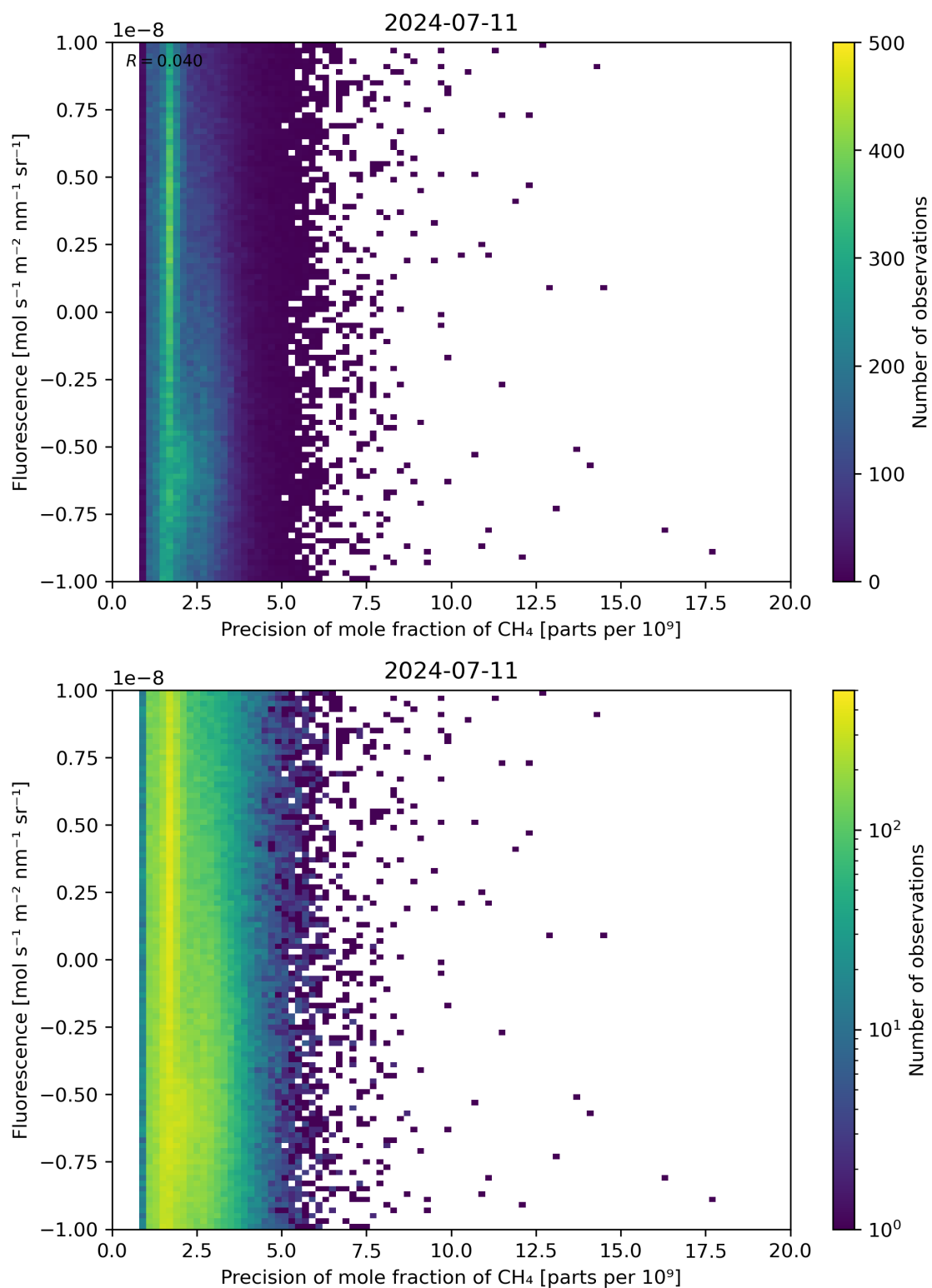
Figure 81: Scatter density plot of “Precision of mole fraction of \text{CH}_4 ” against “Fluorescence” for 2024-07-10 to 2024-07-12.
