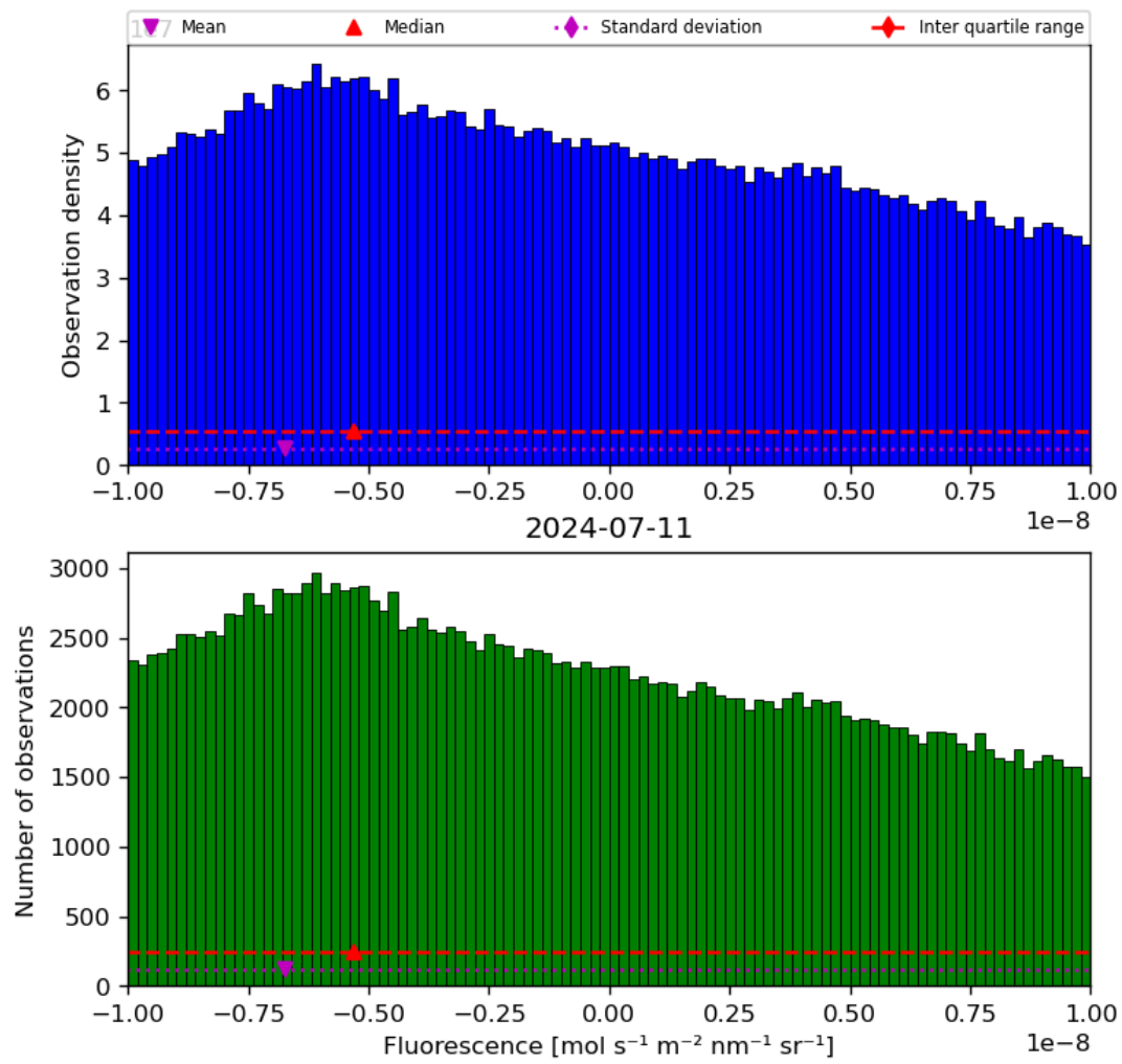
Figure 32: Histogram of “Fluorescence” for 2024-07-10 to 2024-07-12
