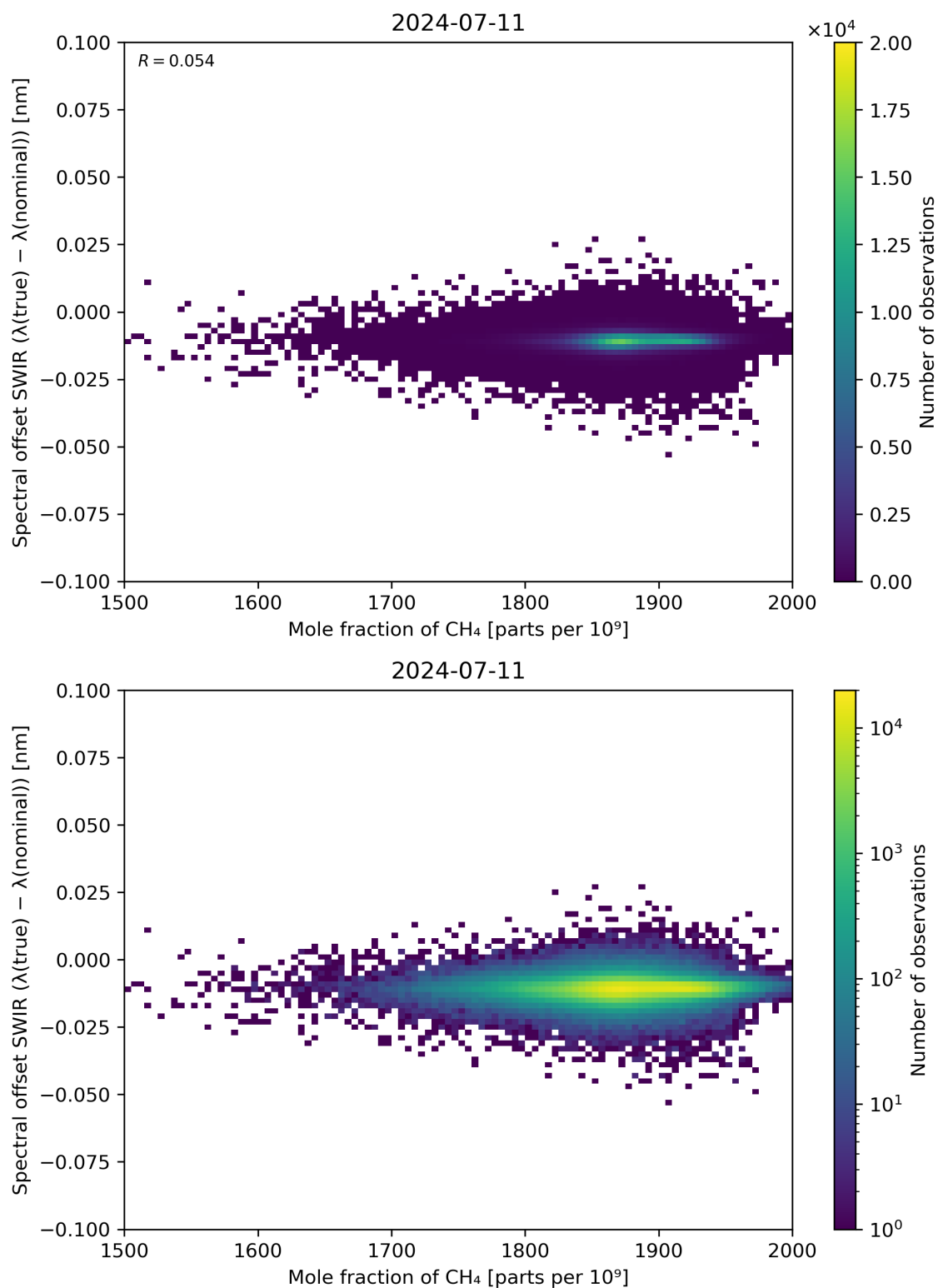
Figure 86: Scatter density plot of “Mole fraction of CH 4 ” against “Spectral offset SWIR ( \lambda(\text{true}) - \lambda(\text{nominal}) )” for 2024-07-10 to 2024-07-12.
