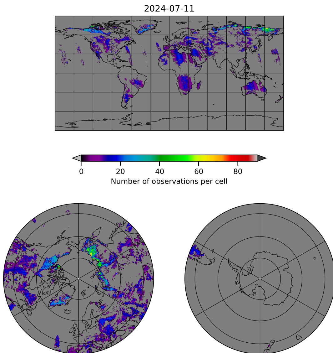
Figure 10: Map of the number of observations for 2024-07-10 to 2024-07-12
