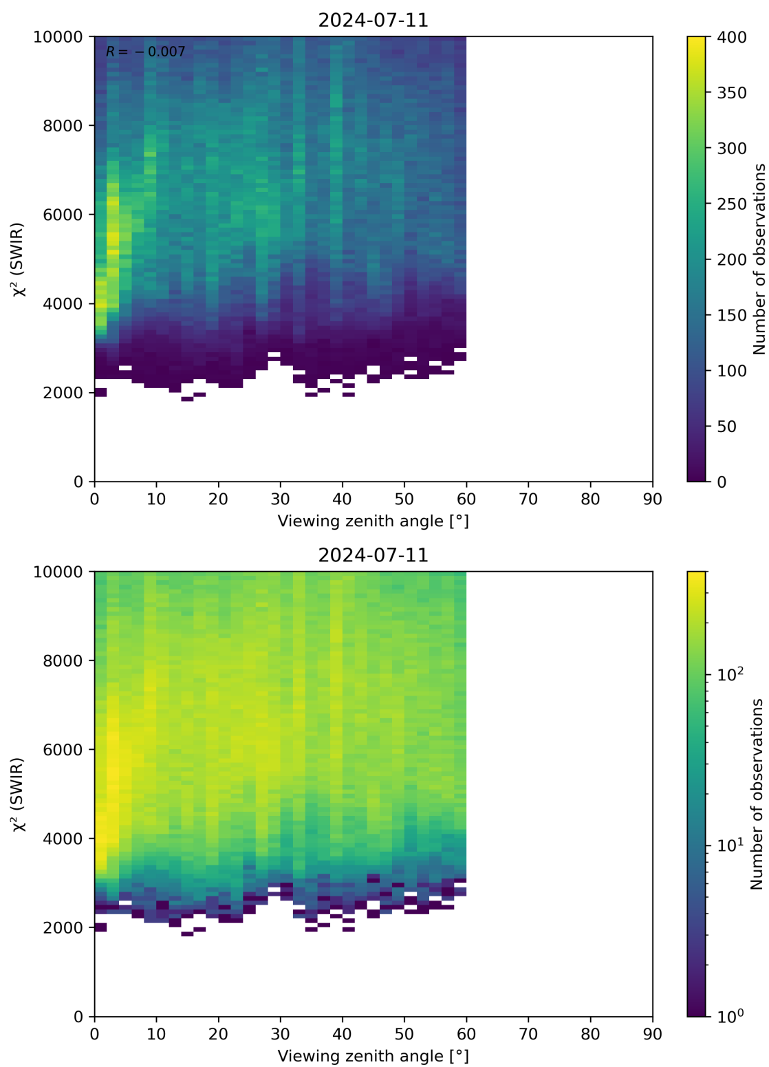
Figure 106: Scatter density plot of “Viewing zenith angle” against “ \chi^2 (SWIR)” for 2024-07-10 to 2024-07-12.
