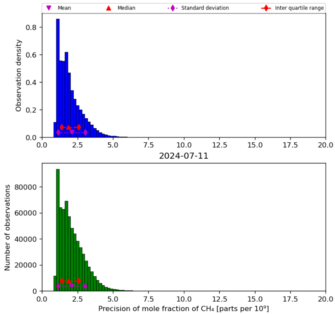
Figure 24: Histogram of “Precision of mole fraction of CH 4 ” for 2024-07-10 to 2024-07-12
