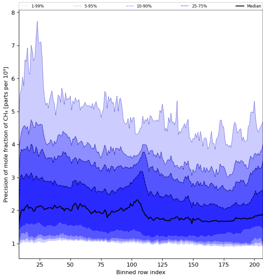
Figure 35: Along track statistics of “Precision of mole fraction of CH 4 ” for 2024-07-10 to 2024-07-12
