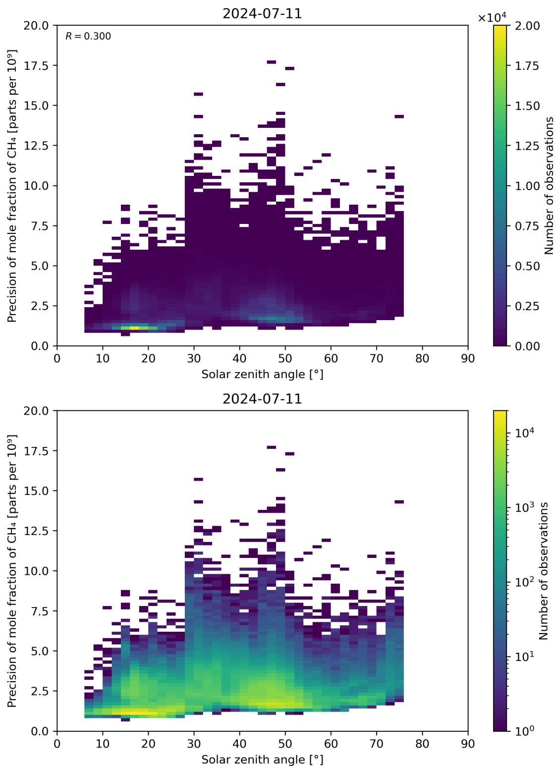
Figure 101: Scatter density plot of “Solar zenith angle” against “Precision of mole fraction of CH 4 ” for 2024-07-10 to 2024-07-12.
