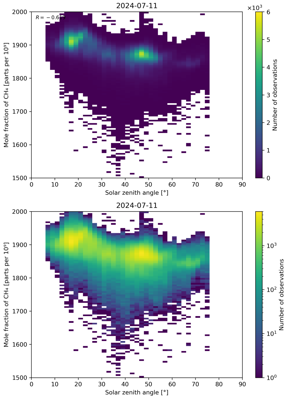
Figure 99: Scatter density plot of “Solar zenith angle” against “Mole fraction of CH 4 ” for 2024-07-10 to 2024-07-12.
