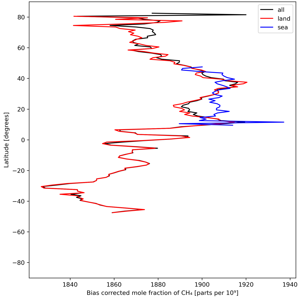
Figure 14: Zonal average of “Bias corrected mole fraction of CH 4 ” for 2024-07-10 to 2024-07-12.
