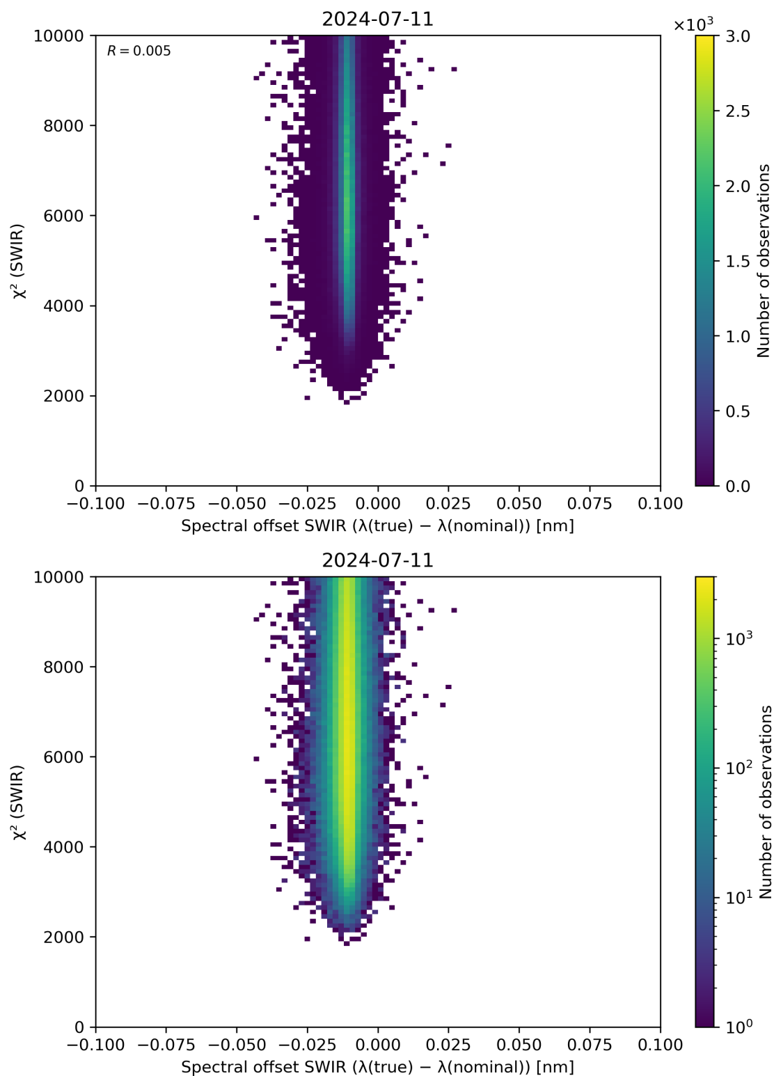
Figure 118: Scatter density plot of “Spectral offset SWIR ( \lambda(\text{true}) - \lambda(\text{nominal}) )” against “ \chi^2 (SWIR)” for 2024-07-10 to 2024-07-12.
