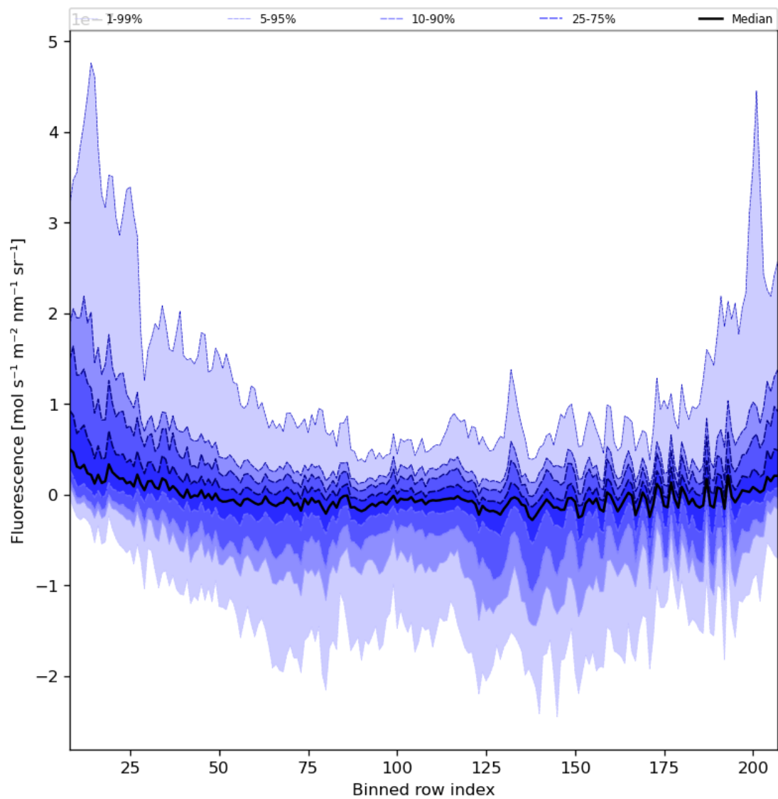
Figure 43: Along track statistics of “Fluorescence” for 2024-07-10 to 2024-07-12
