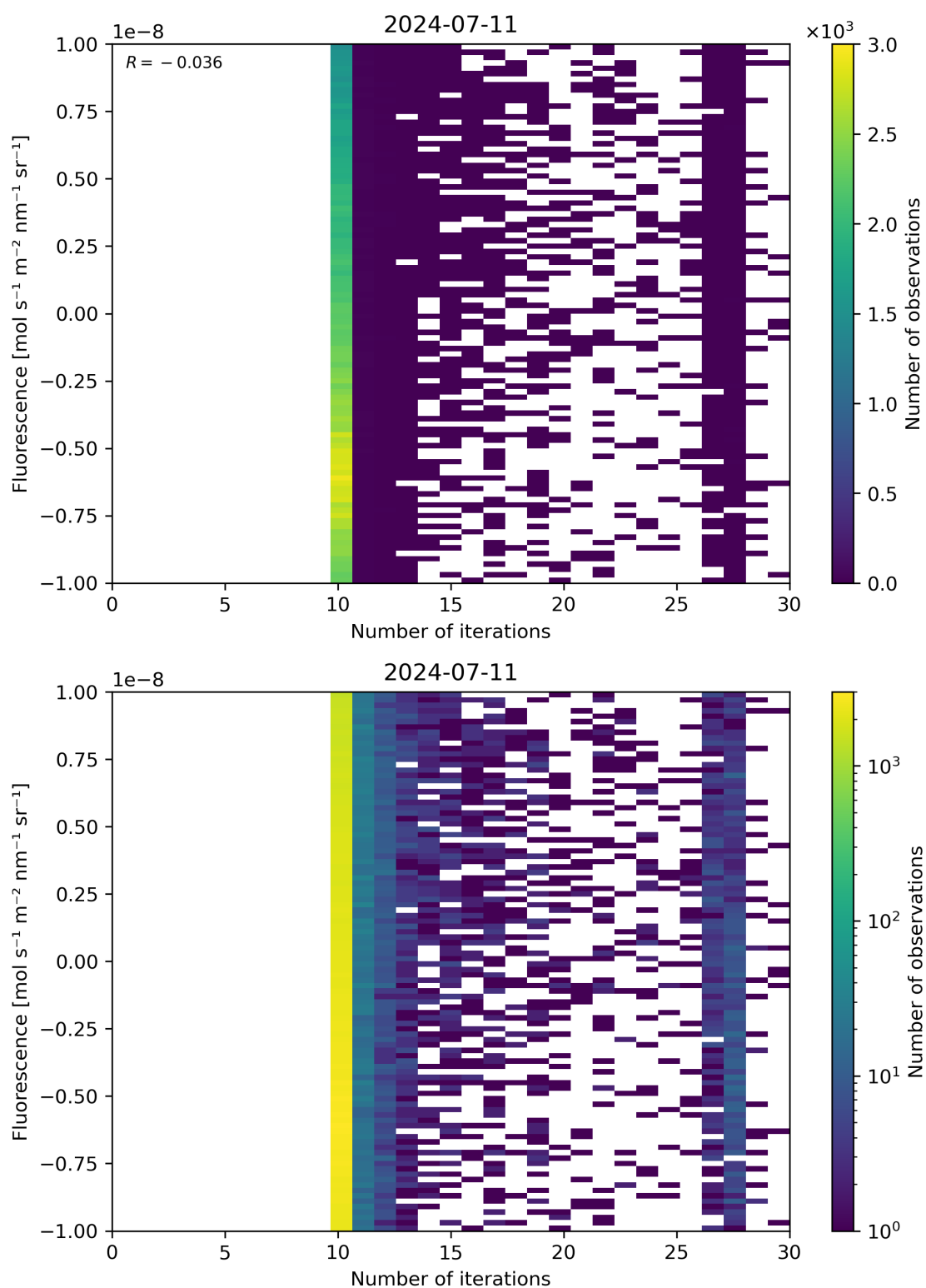
Figure 87: Scatter density plot of “Number of iterations” against “Fluorescence” for 2024-07-10 to 2024-07-12.
