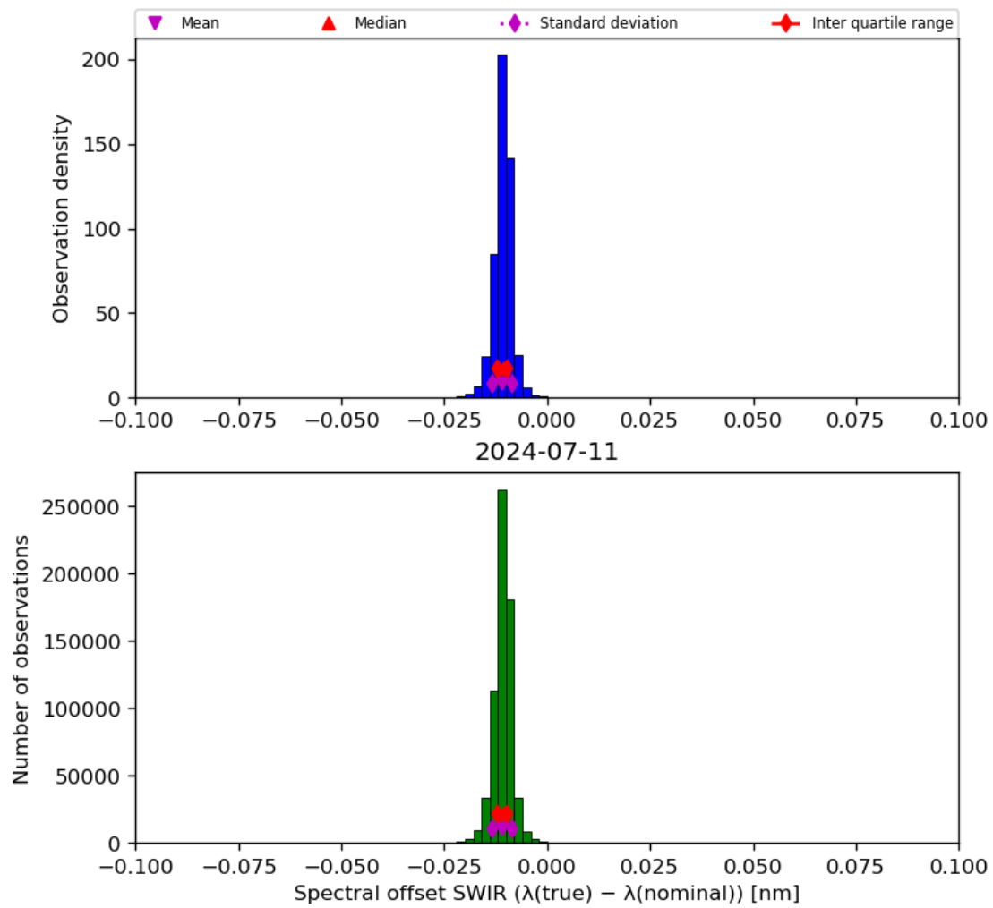
Figure 27: Histogram of “Spectral offset SWIR ( \lambda(\text{true}) - \lambda(\text{nominal}) )” for 2024-07-10 to 2024-07-12
