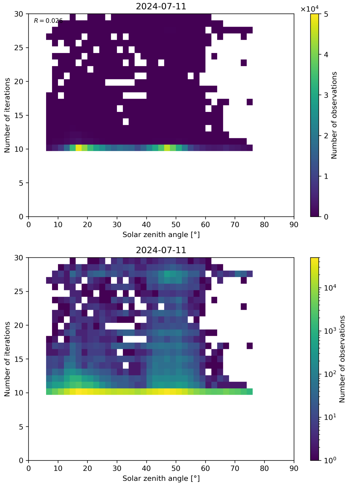
Figure 102: Scatter density plot of “Solar zenith angle” against “Number of iterations” for 2024-07-10 to 2024-07-12.
