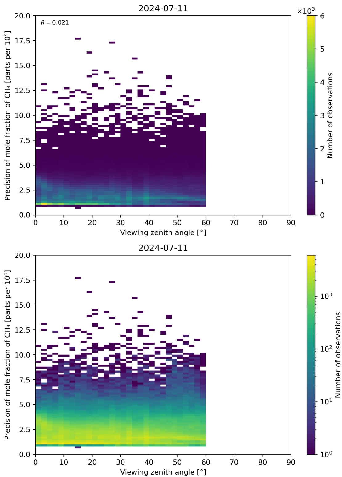
Figure 112: Scatter density plot of “Viewing zenith angle” against “Precision of mole fraction of CH 4 ” for 2024-07-10 to 2024-07-12.
