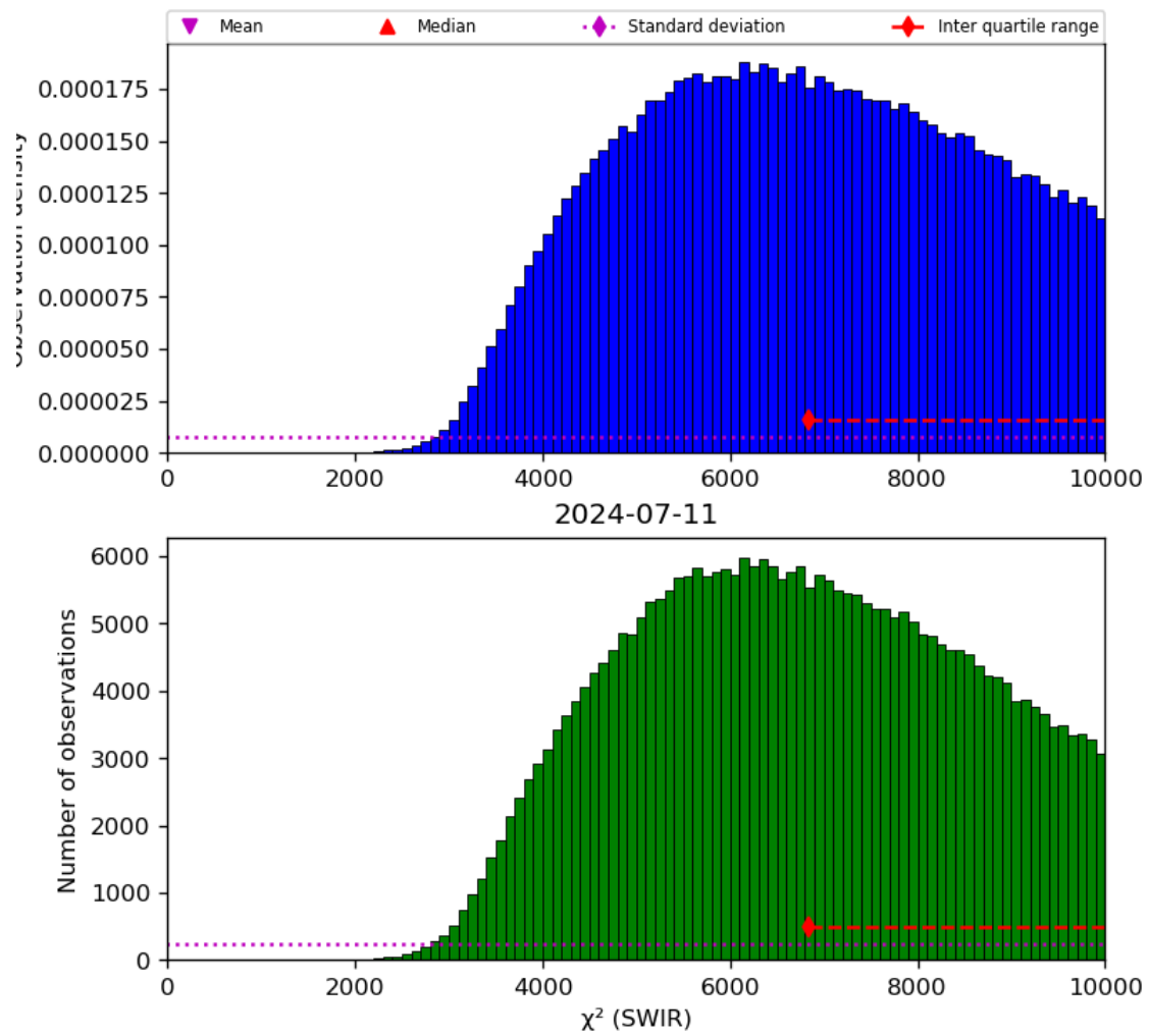
Figure 28: Histogram of “ \chi^2 (SWIR)” for 2024-07-10 to 2024-07-12
