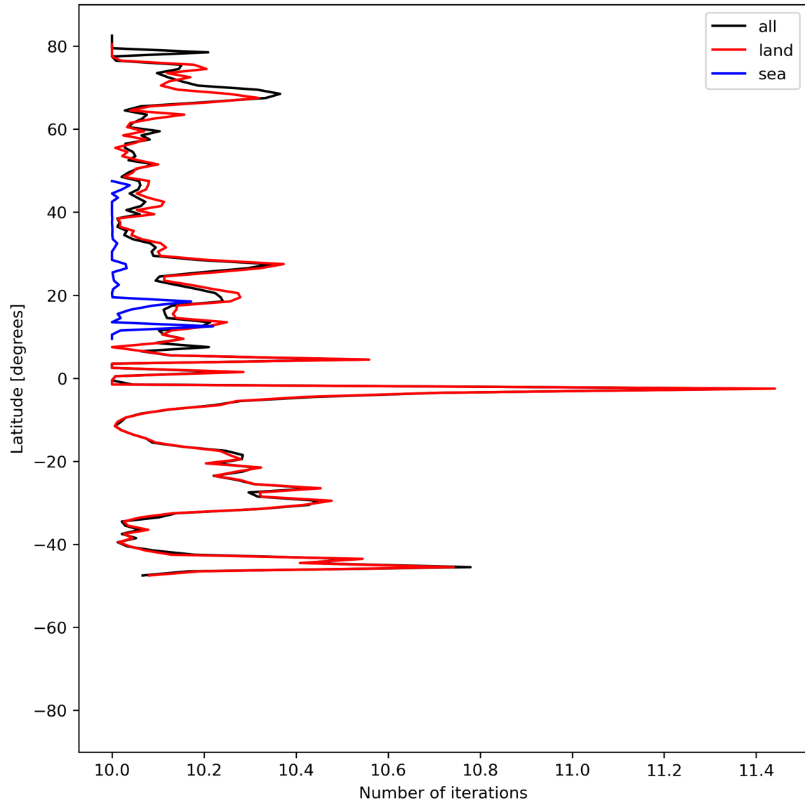
Figure 20: Zonal average of “Number of iterations” for 2024-07-10 to 2024-07-12.
