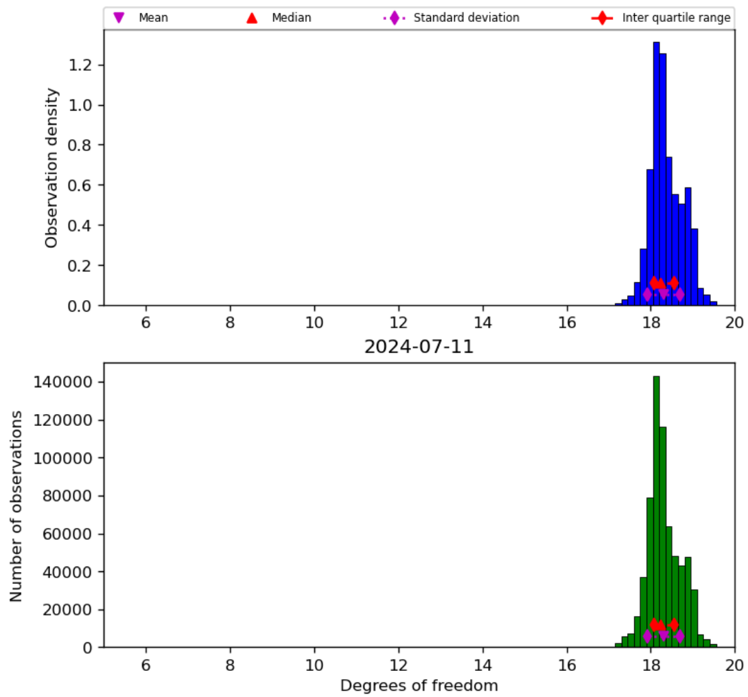
Figure 30: Histogram of “Degrees of freedom” for 2024-07-10 to 2024-07-12
