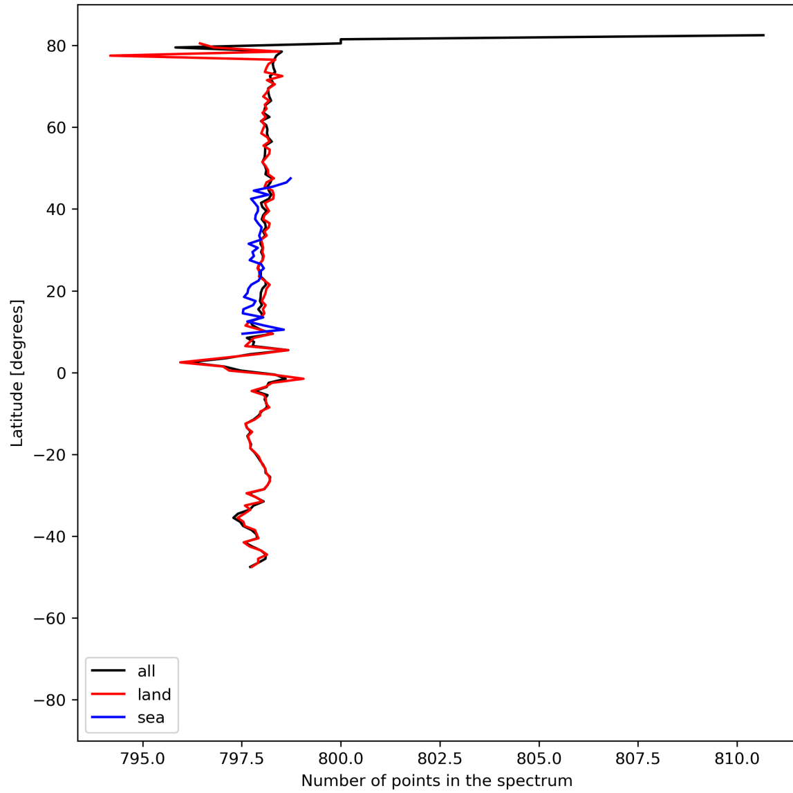
Figure 15: Zonal average of “Number of points in the spectrum” for 2024-07-10 to 2024-07-12.
