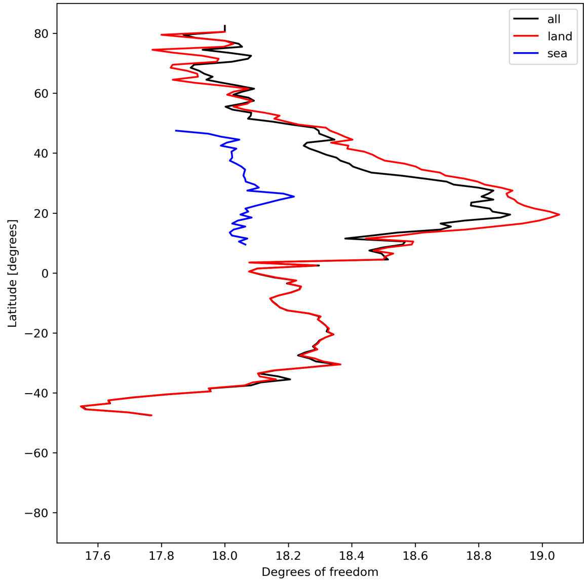
Figure 19: Zonal average of “Degrees of freedom” for 2024-07-10 to 2024-07-12.
