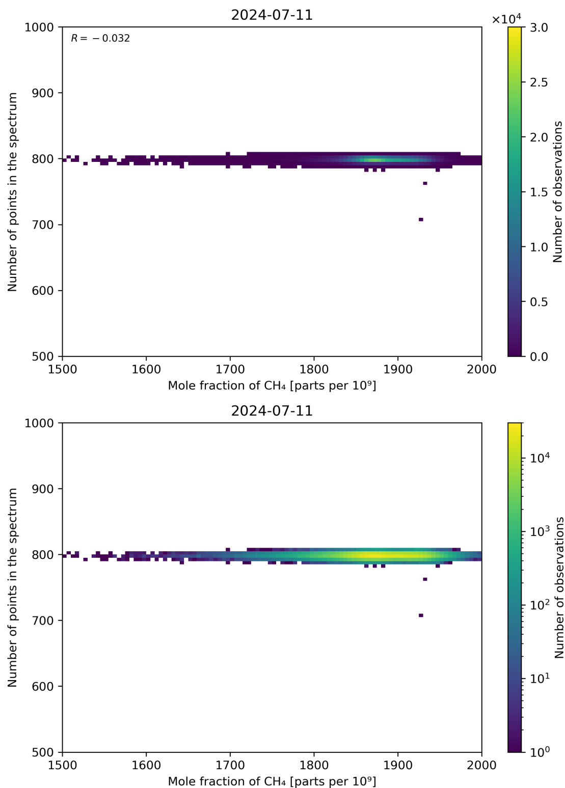
Figure 77: Scatter density plot of “Mole fraction of CH 4 ” against “Number of points in the spectrum” for 2024-07-10 to 2024-07-12.
