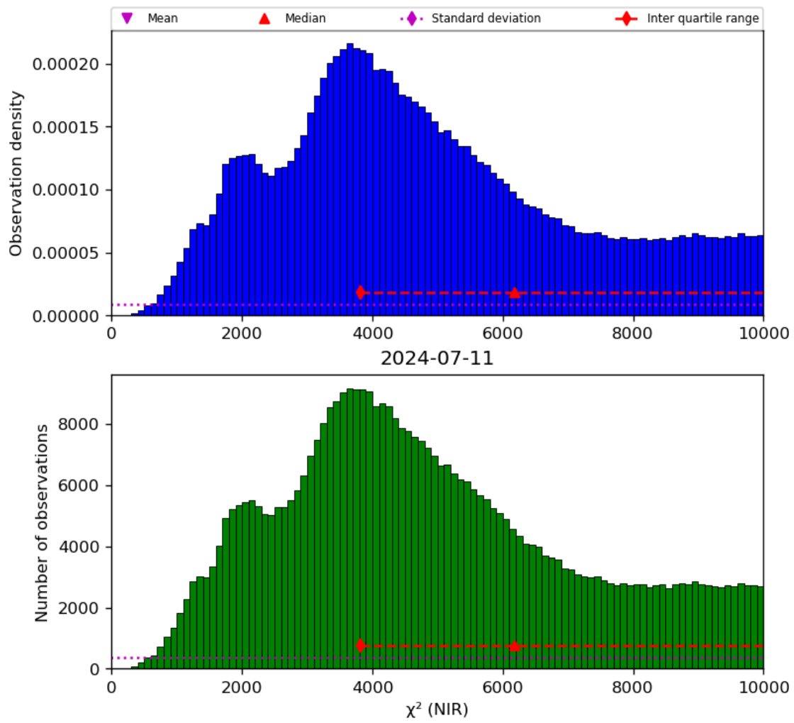
Figure 29: Histogram of “ \chi^2 (NIR)” for 2024-07-10 to 2024-07-12
