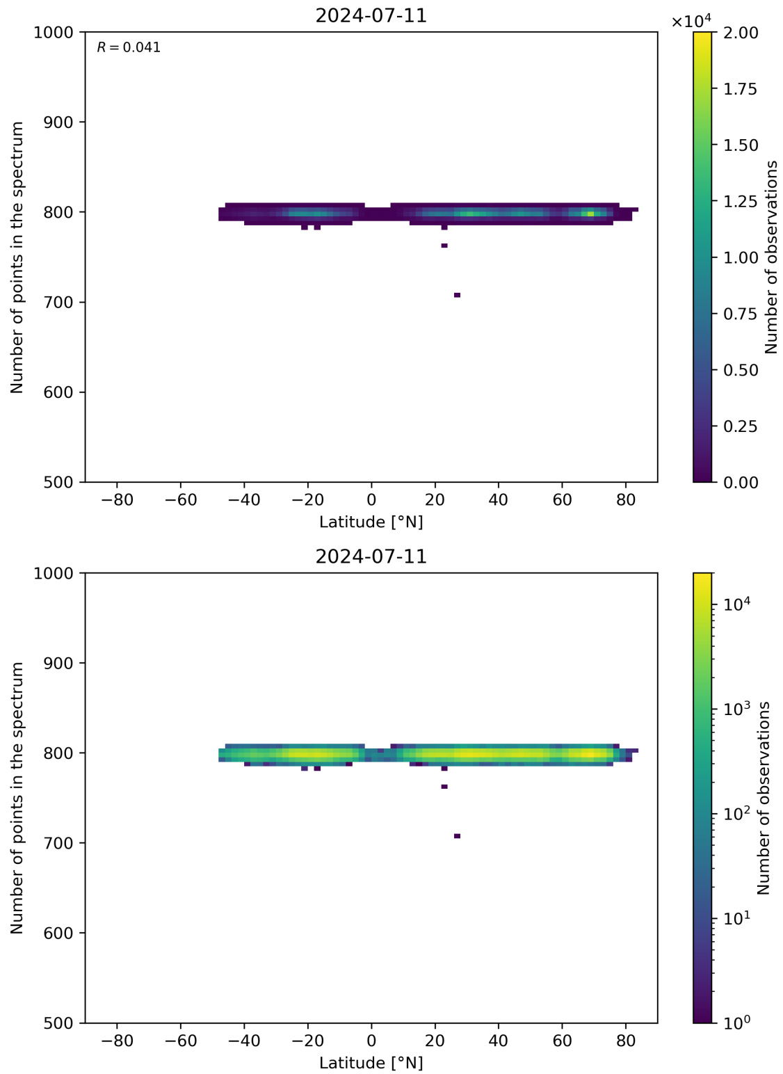
Figure 61: Scatter density plot of “Latitude” against “Number of points in the spectrum” for 2024-07-10 to 2024-07-12.
