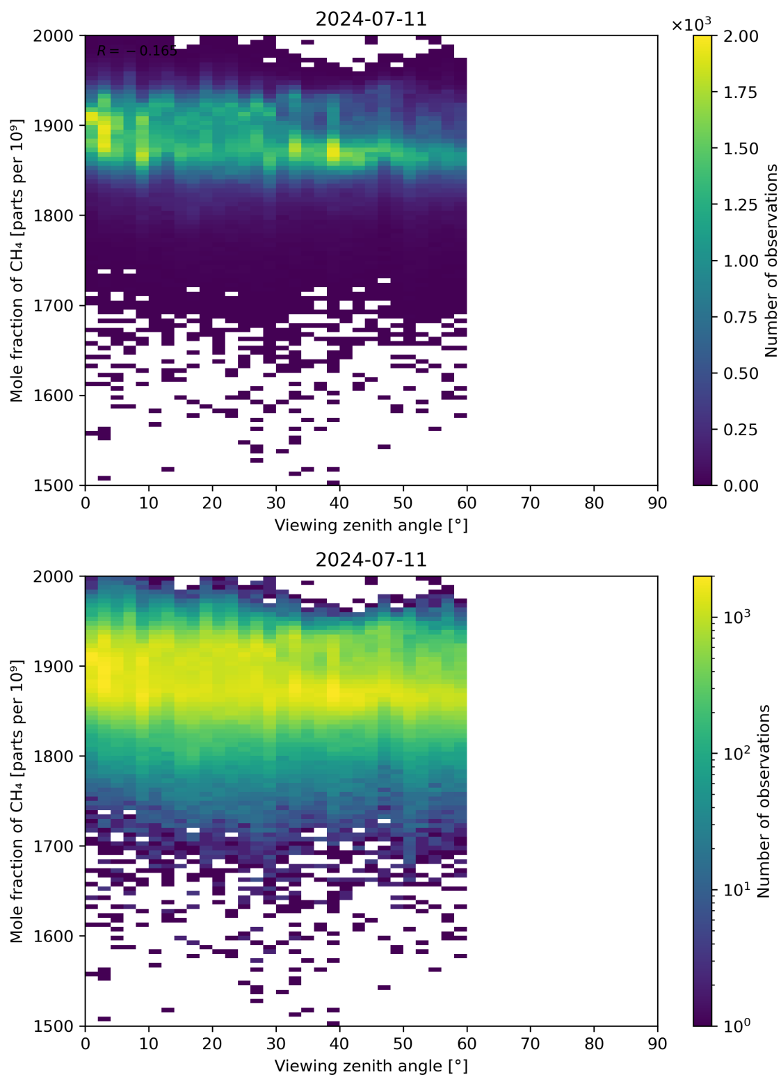
Figure 110: Scatter density plot of “Viewing zenith angle” against “Mole fraction of CH 4 ” for 2024-07-10 to 2024-07-12.
