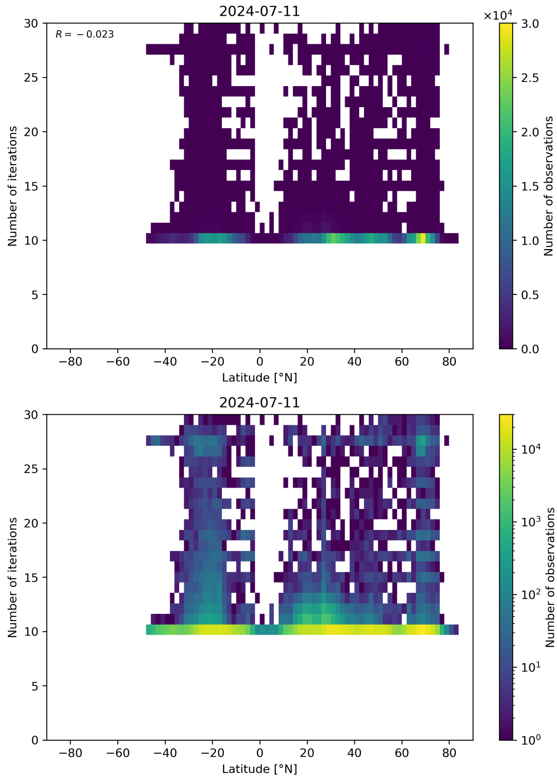
Figure 60: Scatter density plot of “Latitude” against “Number of iterations” for 2024-07-10 to 2024-07-12.
