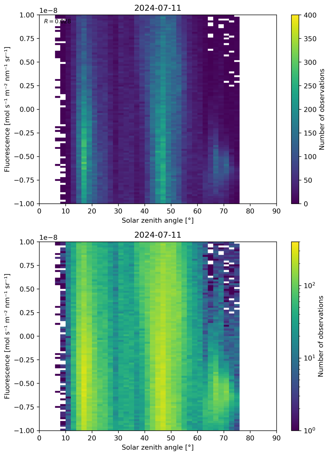
Figure 97: Scatter density plot of “Solar zenith angle” against “Fluorescence” for 2024-07-10 to 2024-07-12.
