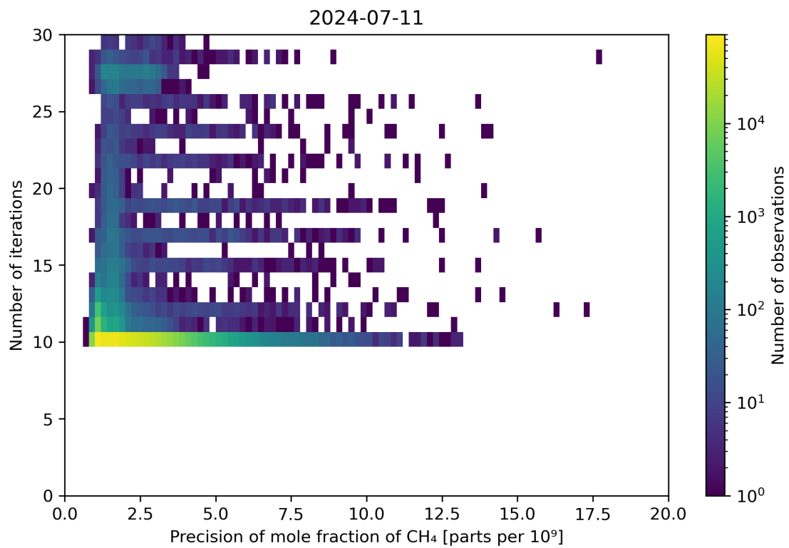
Figure 83: Scatter density plot of “Precision of mole fraction of CH 4 ” against “Number of iterations” for 2024-07-10 to 2024-07-12.
