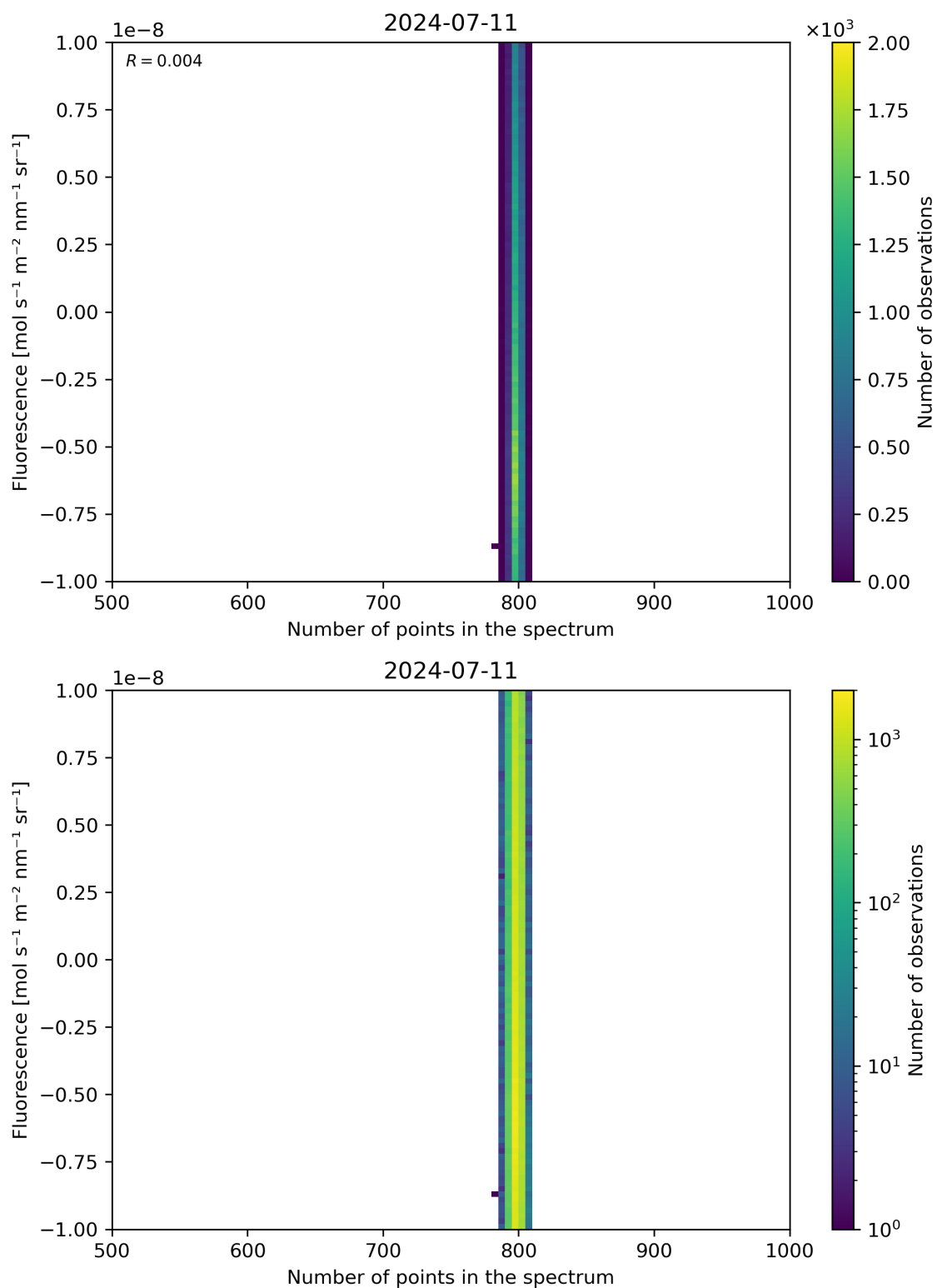
Figure 91: Scatter density plot of “Number of points in the spectrum” against “Fluorescence” for 2024-07-10 to 2024-07-12.
