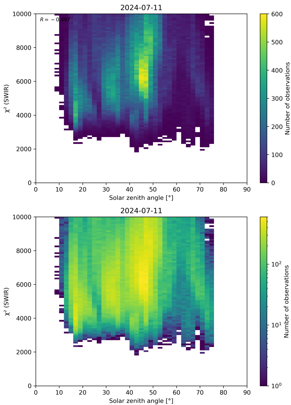
Figure 95: Scatter density plot of “Solar zenith angle” against “ \chi^2 (SWIR)” for 2024-07-10 to 2024-07-12.
