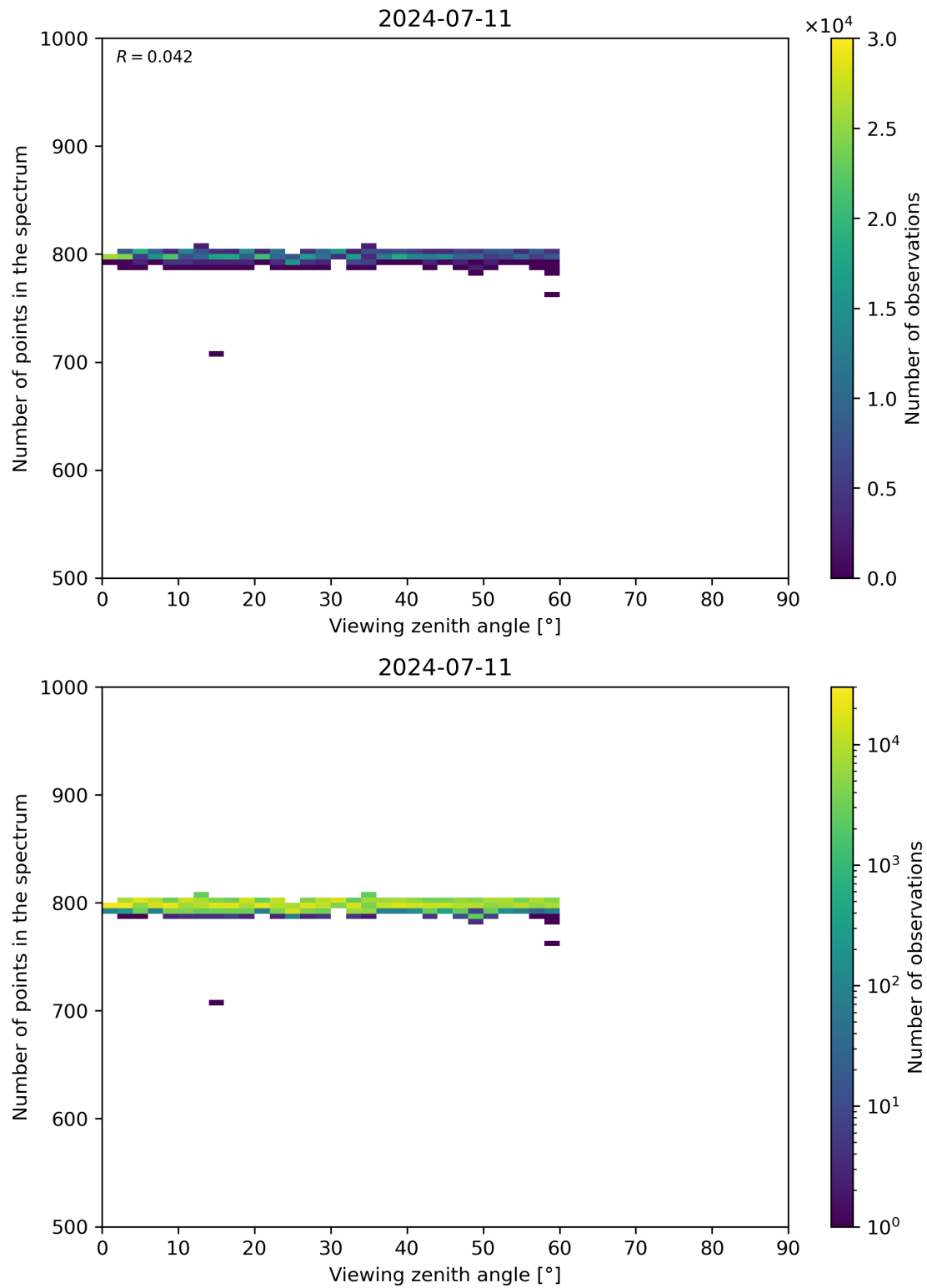
Figure 114: Scatter density plot of “Viewing zenith angle” against “Number of points in the spectrum” for 2024-07-10 to 2024-07-12.
