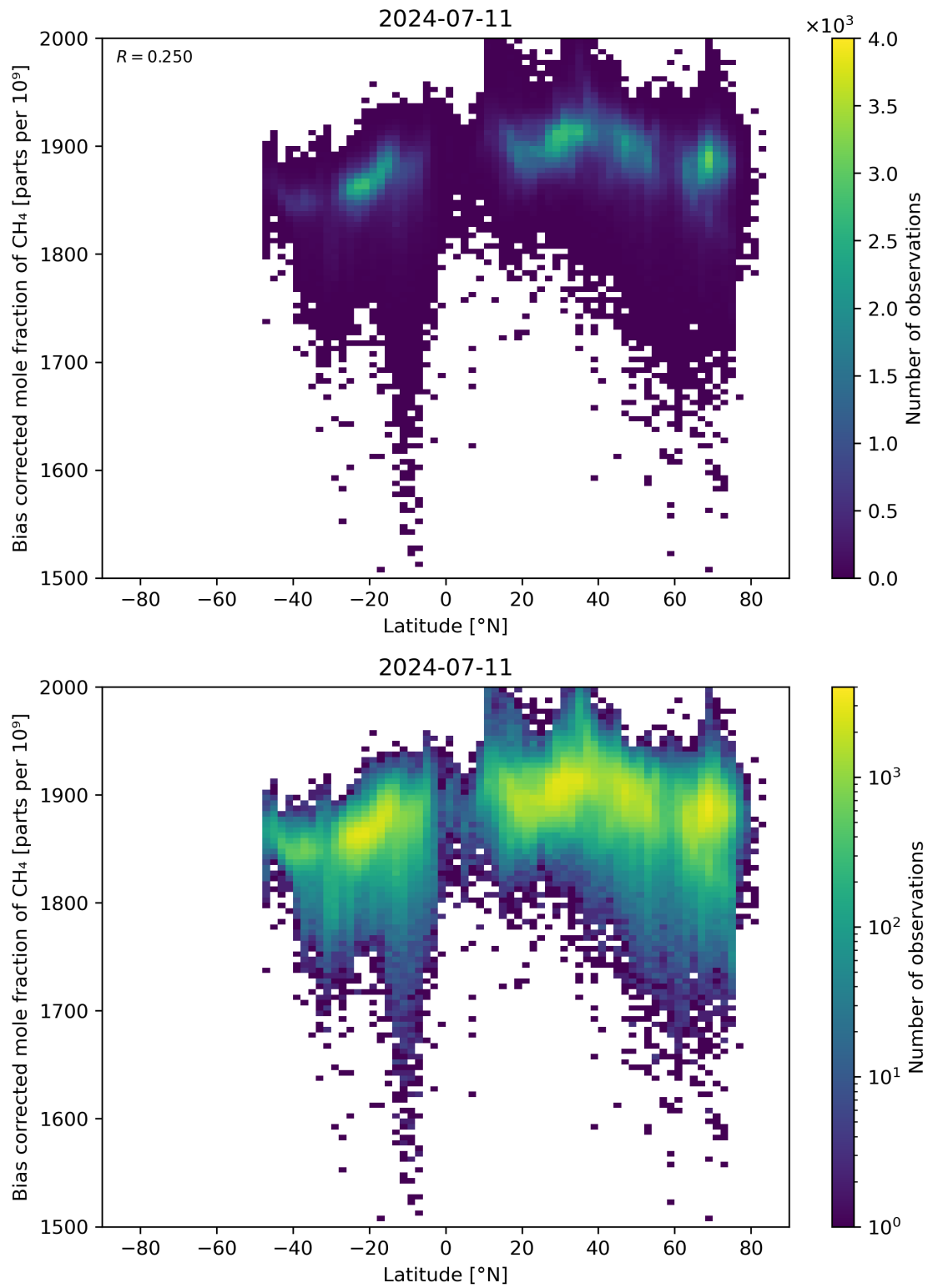
Figure 58: Scatter density plot of “Latitude” against “Bias corrected mole fraction of CH 4 ” for 2024-07-10 to 2024-07-12.
