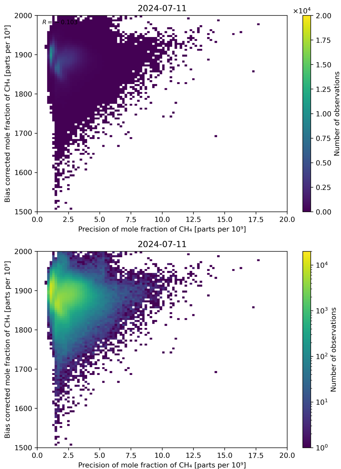
Figure 82: Scatter density plot of “Precision of mole fraction of \text{CH}_4 ” against “Bias corrected mole fraction of \text{CH}_4 ” for 2024-07-10 to 2024-07-12.
