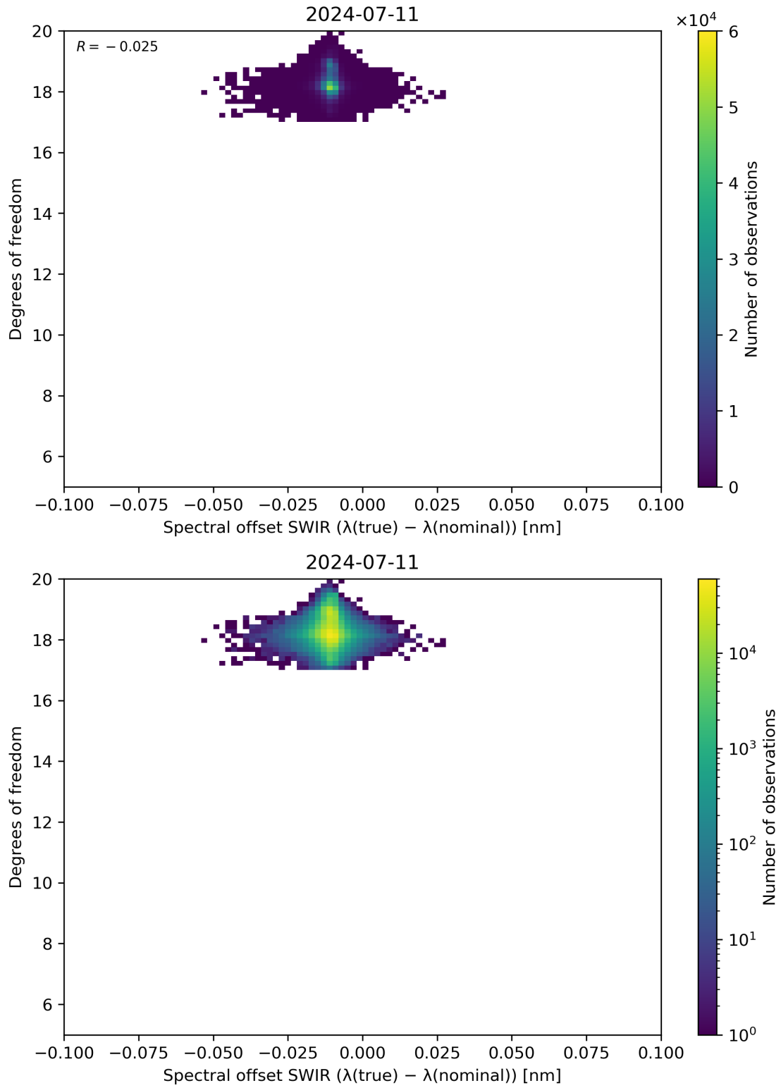
Figure 119: Scatter density plot of “Spectral offset SWIR ( \lambda(\text{true}) - \lambda(\text{nominal}) )” against “Degrees of freedom” for 2024-07-10 to 2024-07-12.
