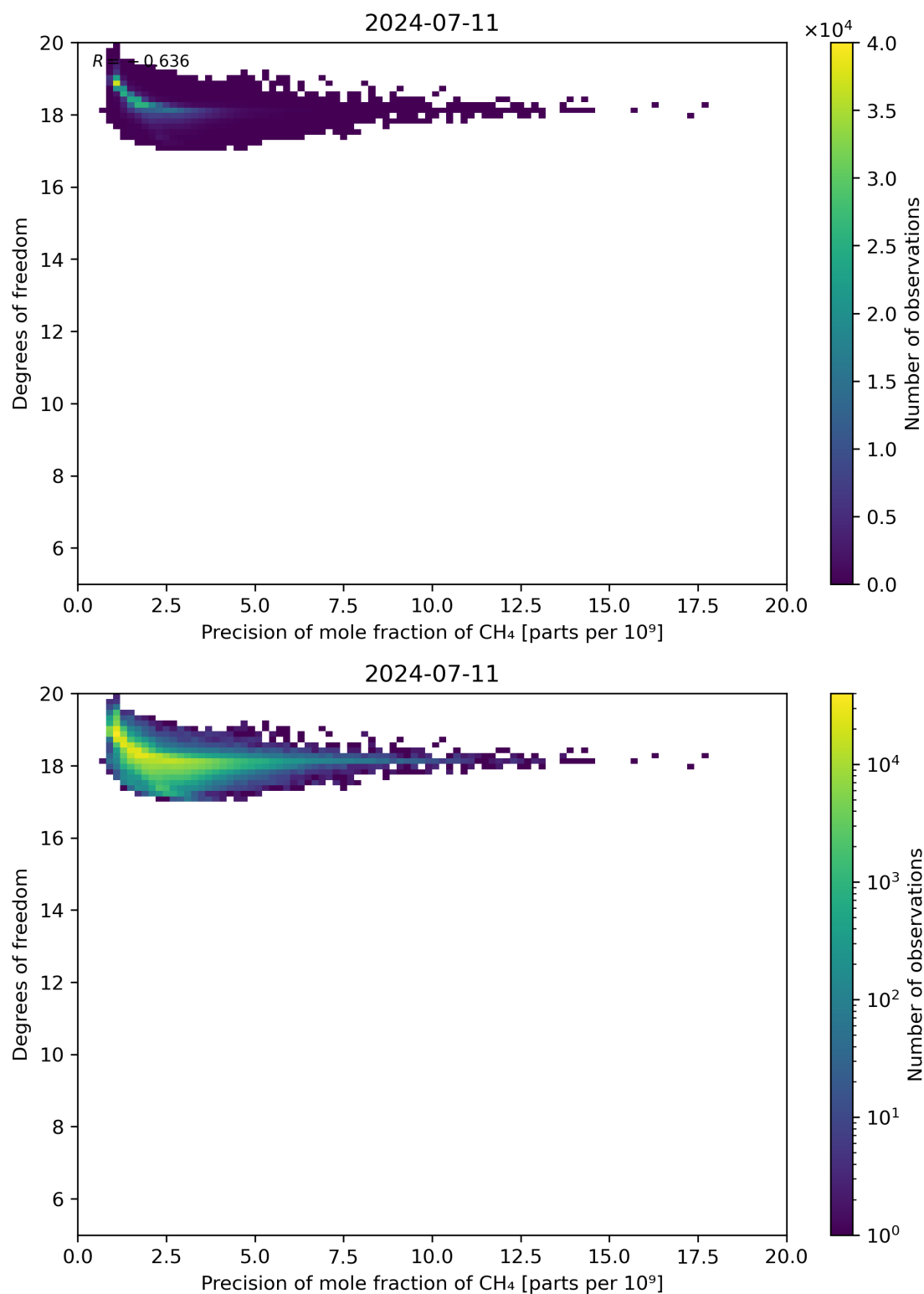
Figure 80: Scatter density plot of “Precision of mole fraction of CH 4 ” against “Degrees of freedom” for 2024-07-10 to 2024-07-12.
