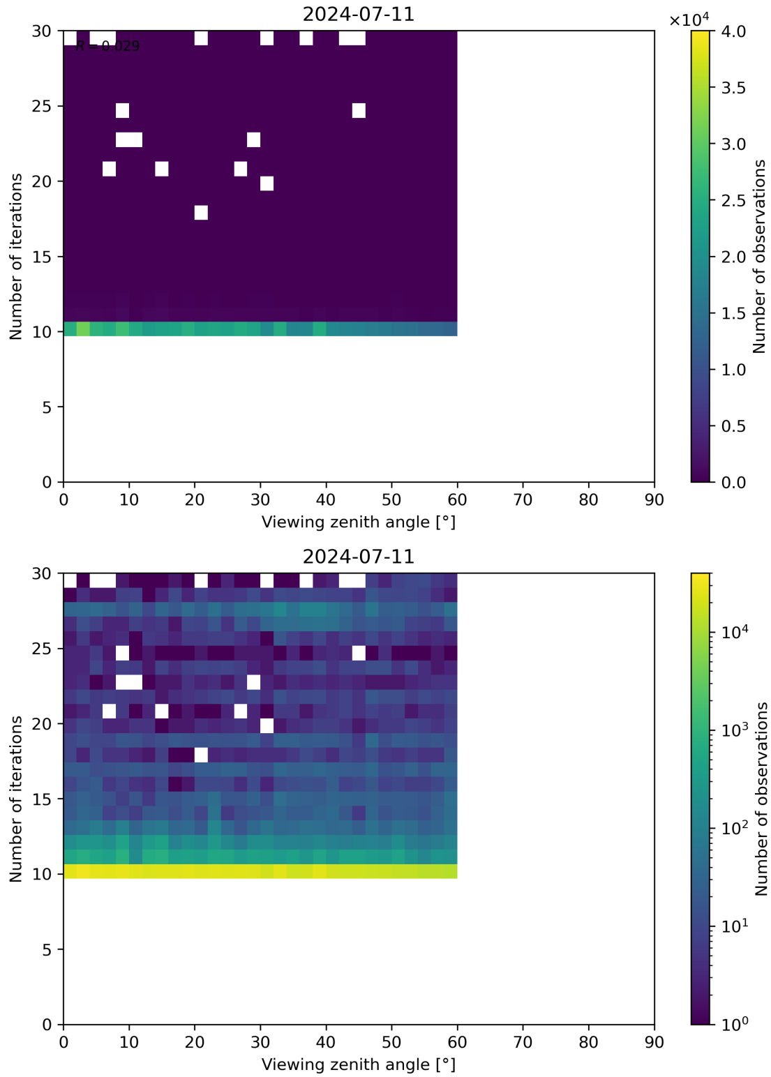
Figure 113: Scatter density plot of “Viewing zenith angle” against “Number of iterations” for 2024-07-10 to 2024-07-12.
