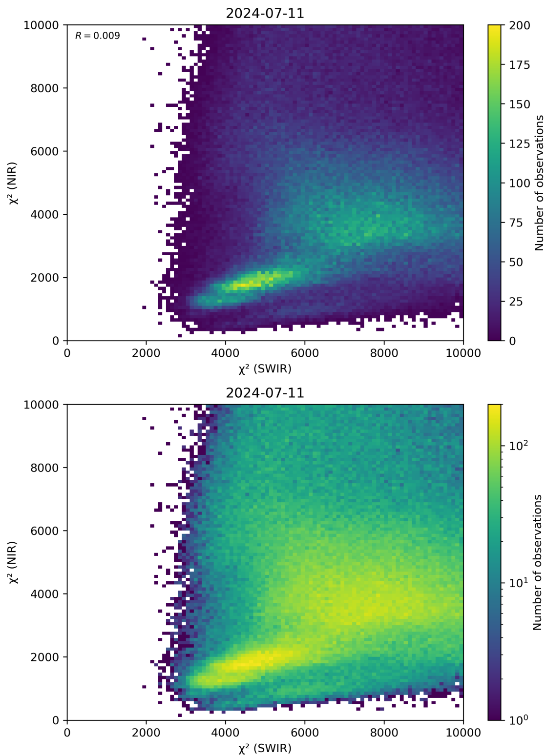
Figure 47: Scatter density plot of “ \chi^2 (SWIR)” against “ \chi^2 (NIR)” for 2024-07-10 to 2024-07-12.
