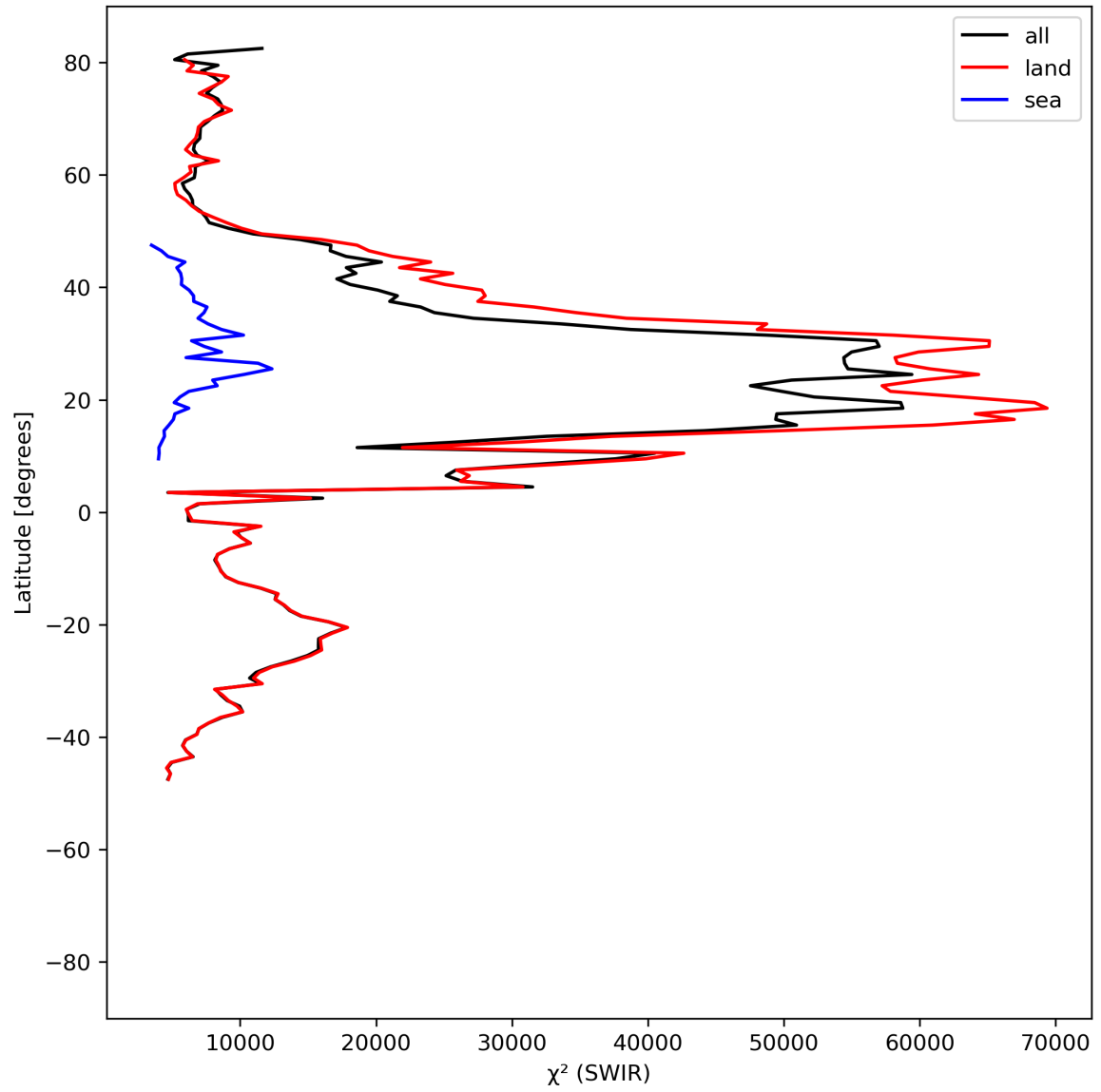
Figure 17: Zonal average of “ \chi^2 (SWIR)” for 2024-07-10 to 2024-07-12.
