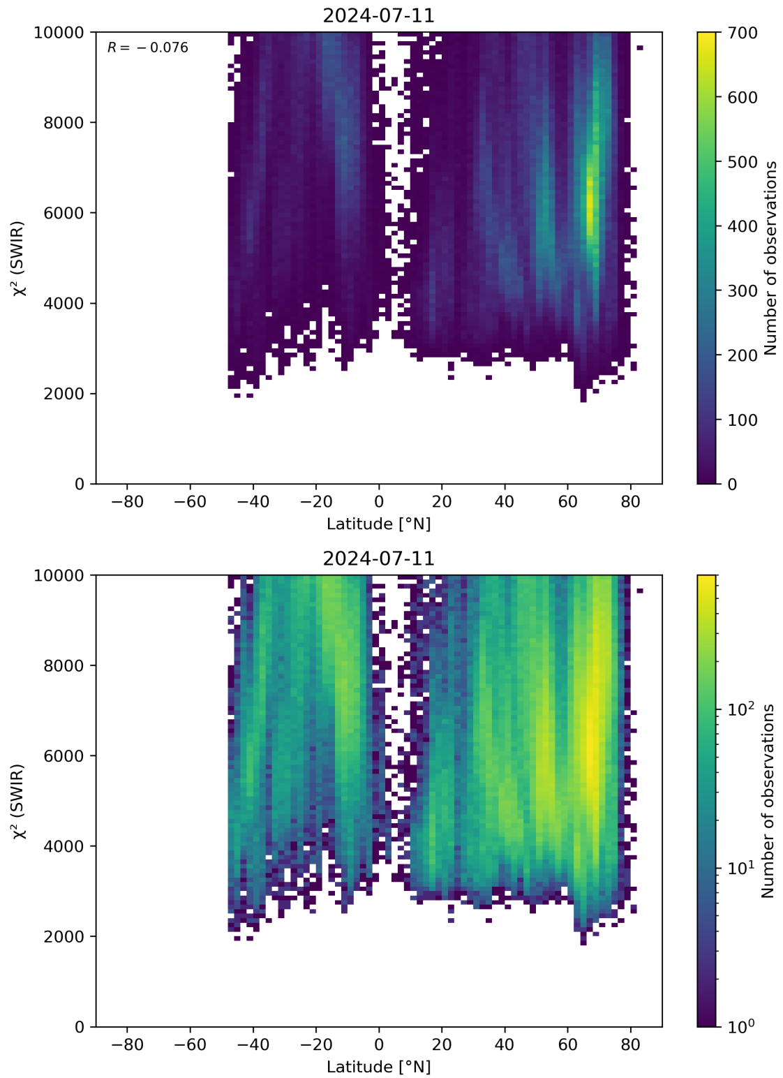
Figure 54: Scatter density plot of “Latitude” against “ \chi^2 (SWIR)” for 2024-07-10 to 2024-07-12.
