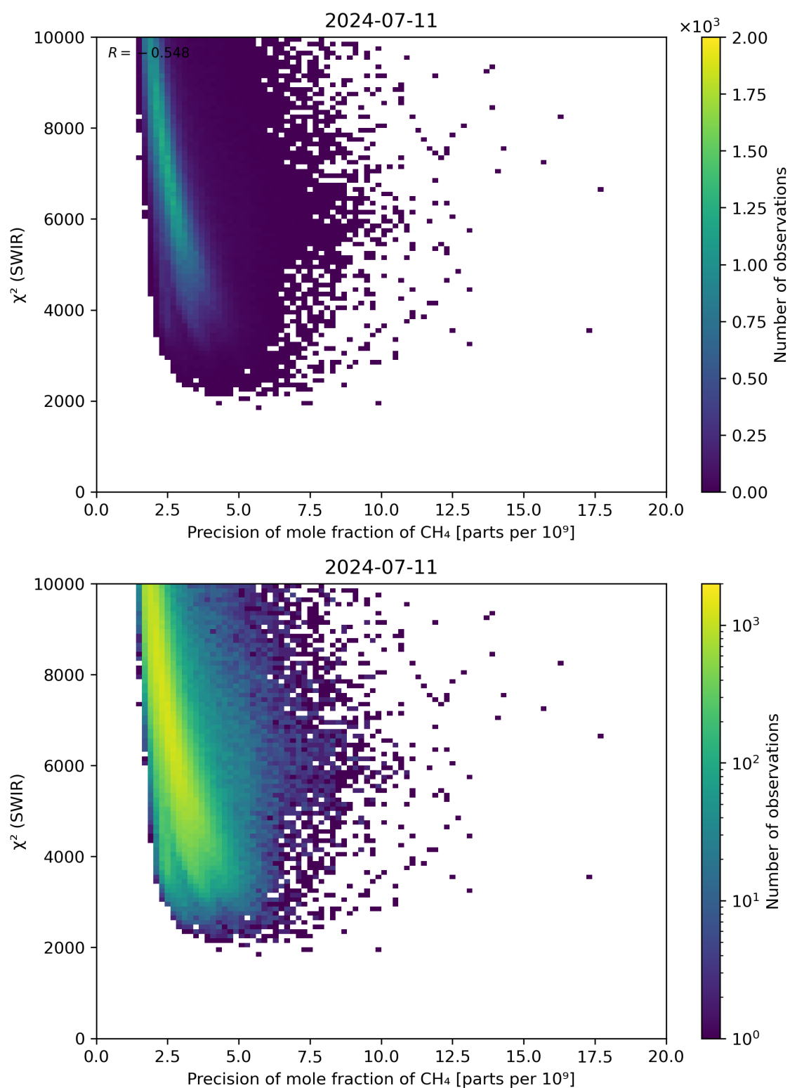
Figure 79: Scatter density plot of “Precision of mole fraction of CH 4 ” against “ \chi^2 (SWIR)” for 2024-07-10 to 2024-07-12.
