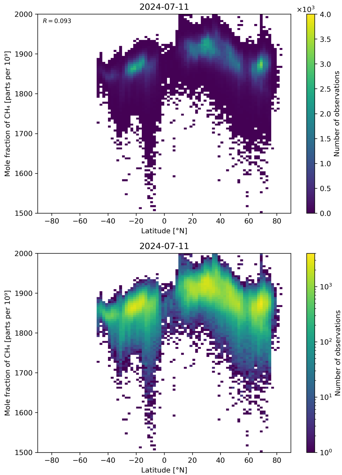
Figure 57: Scatter density plot of “Latitude” against “Mole fraction of CH 4 ” for 2024-07-10 to 2024-07-12.
