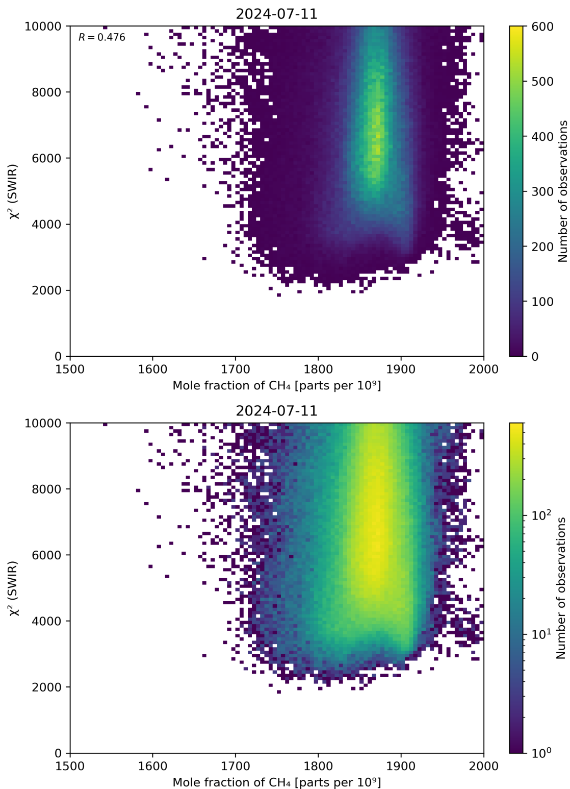
Figure 71: Scatter density plot of “Mole fraction of \text{CH}_4 ” against “ \chi^2 (SWIR)” for 2024-07-10 to 2024-07-12.
