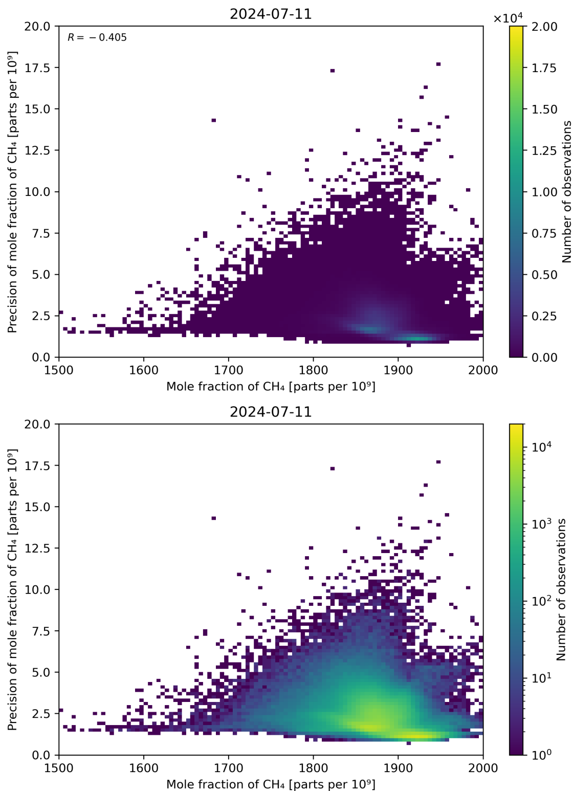
Figure 75: Scatter density plot of “Mole fraction of CH 4 ” against “Precision of mole fraction of CH 4 ” for 2024-07-10 to 2024-07-12.
