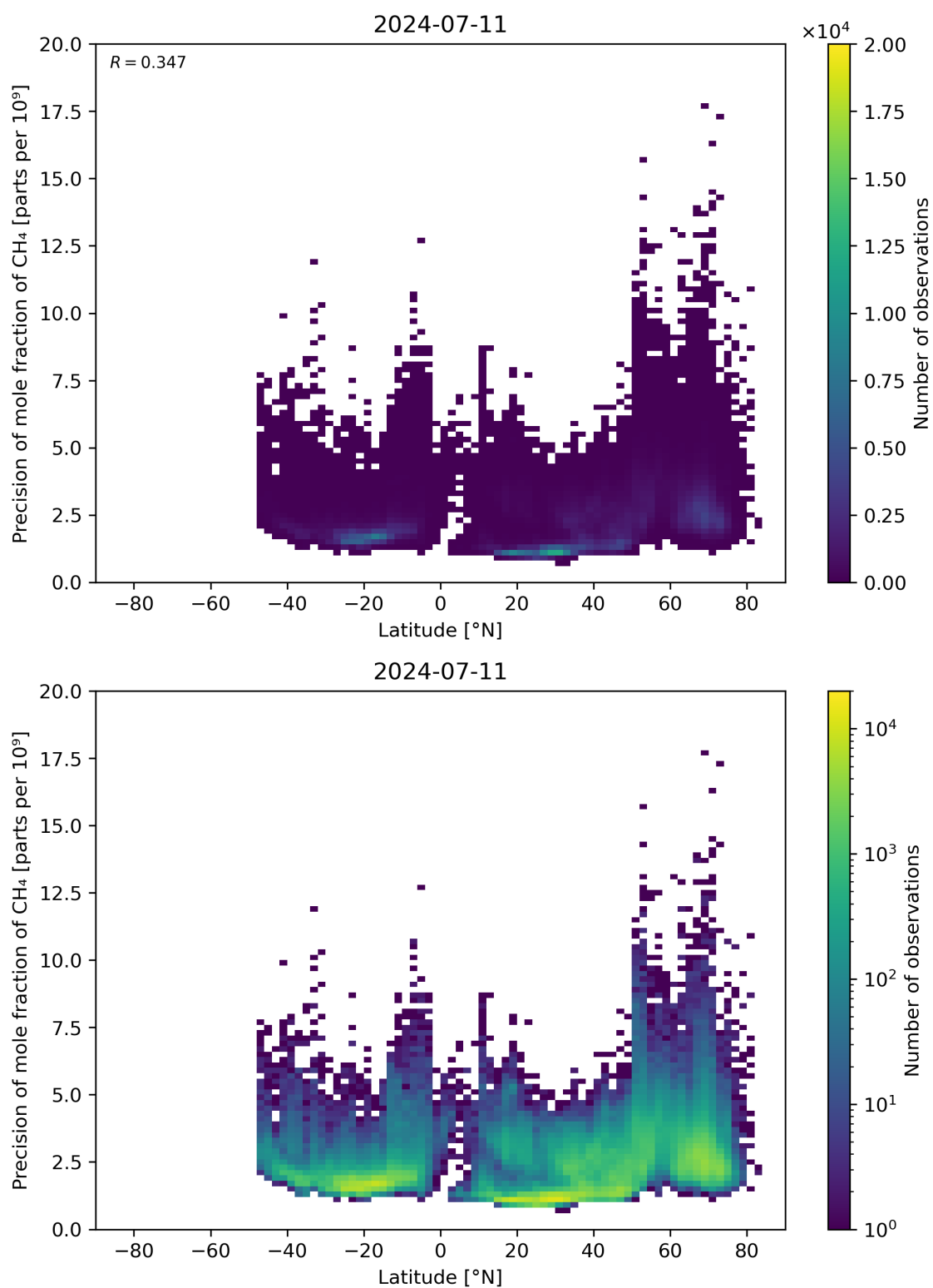
Figure 59: Scatter density plot of “Latitude” against “Precision of mole fraction of \text{CH}_4 ” for 2024-07-10 to 2024-07-12.
