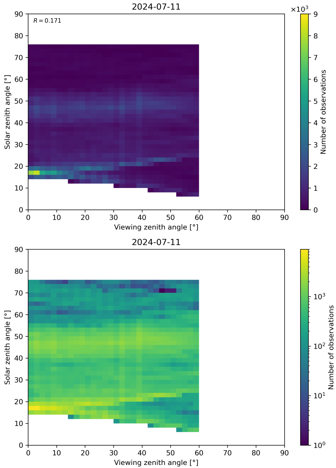
Figure 115: Scatter density plot of “Viewing zenith angle” against “Solar zenith angle” for 2024-07-10 to 2024-07-12.
