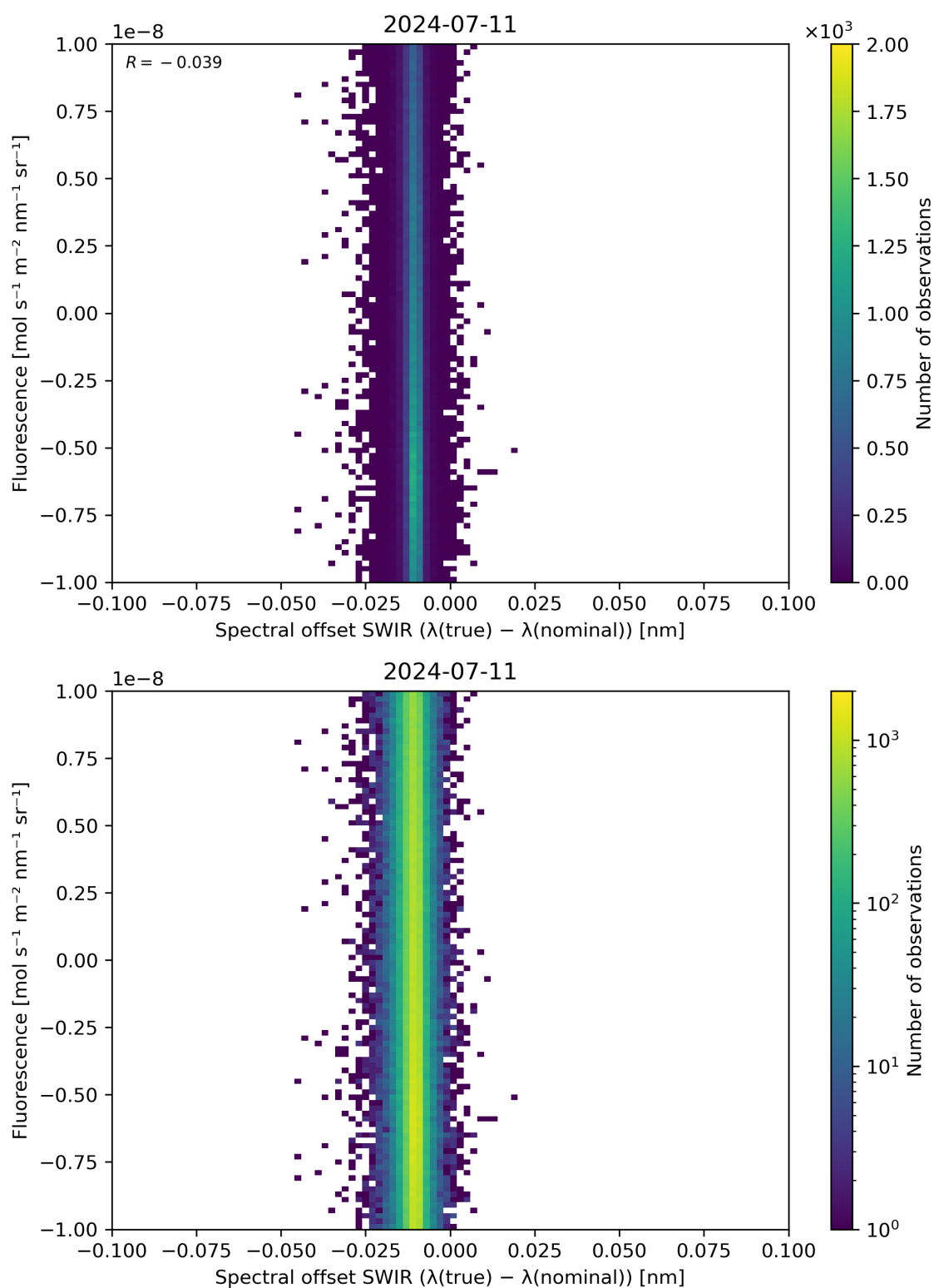
Figure 120: Scatter density plot of “Spectral offset SWIR ( \lambda(\text{true}) - \lambda(\text{nominal}) )” against “Fluorescence” for 2024-07-10 to 2024-07-12.
