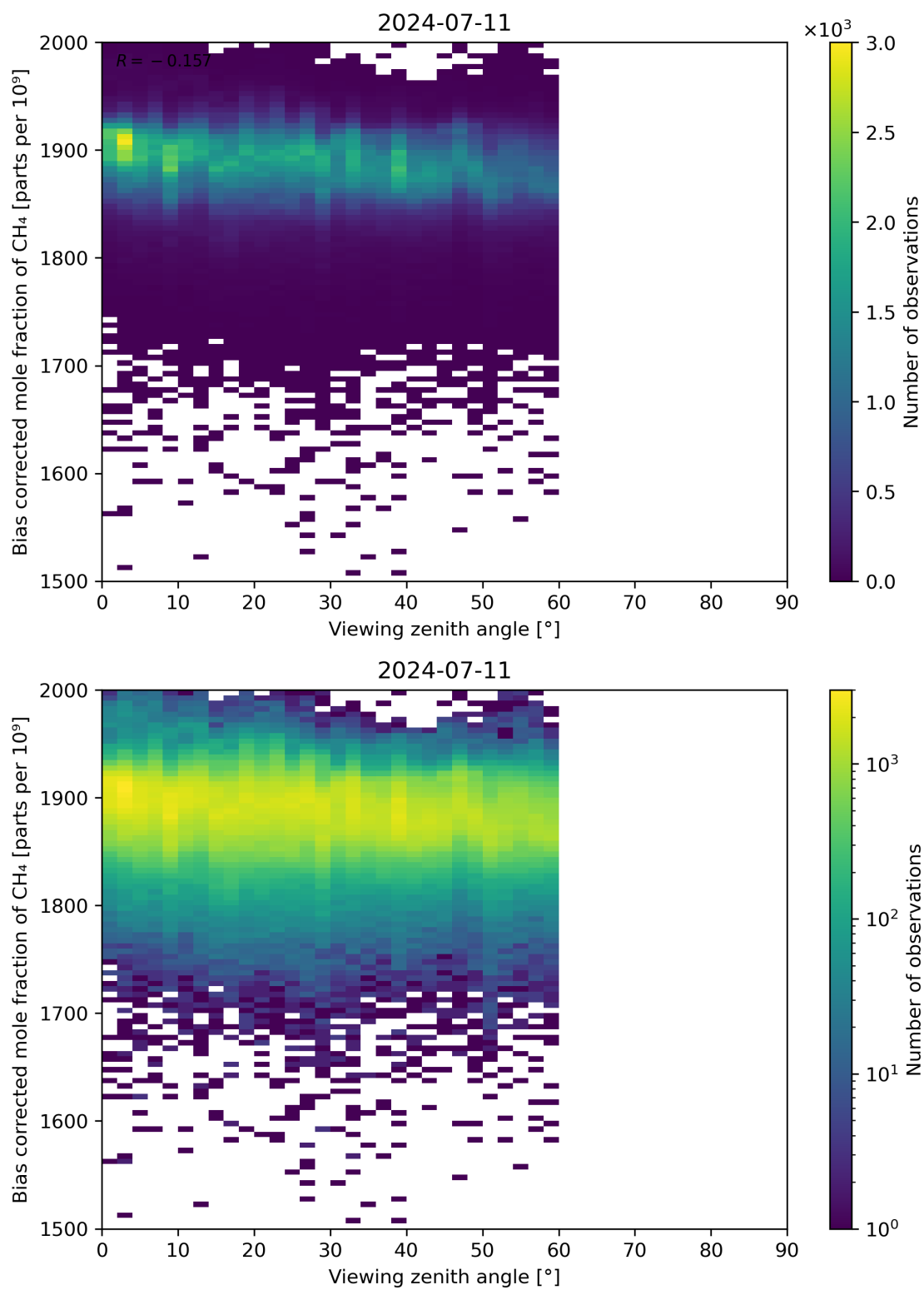
Figure 111: Scatter density plot of “Viewing zenith angle” against “Bias corrected mole fraction of CH 4 ” for 2024-07-10 to 2024-07-12.
