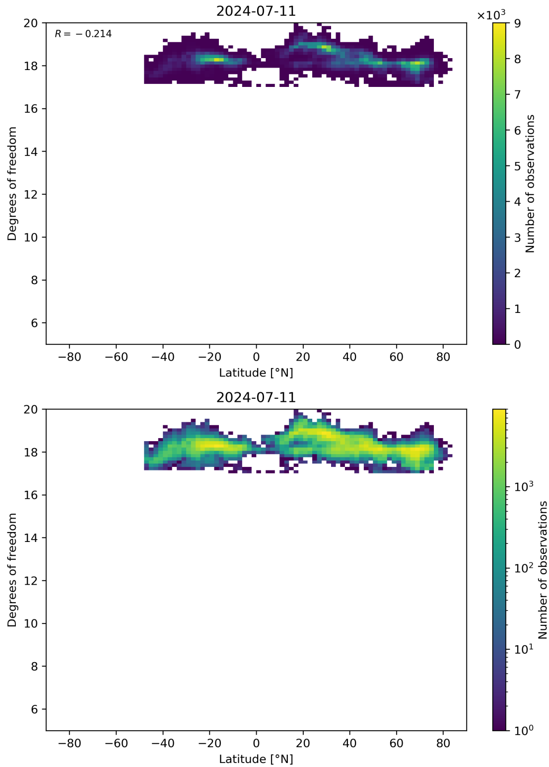
Figure 55: Scatter density plot of “Latitude” against “Degrees of freedom” for 2024-07-10 to 2024-07-12.
