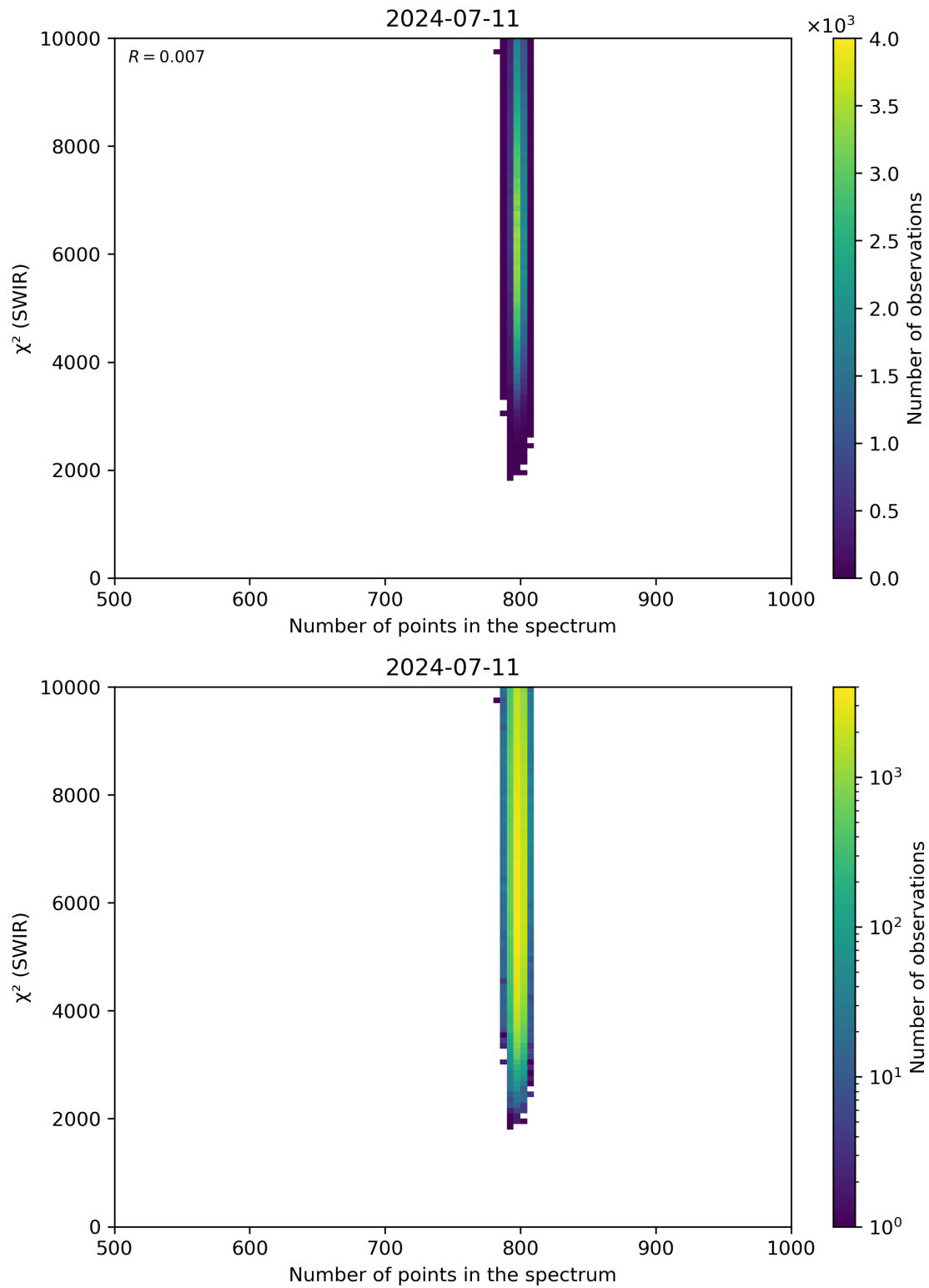
Figure 89: Scatter density plot of “Number of points in the spectrum” against “ \chi^2 (SWIR)” for 2024-07-10 to 2024-07-12.
