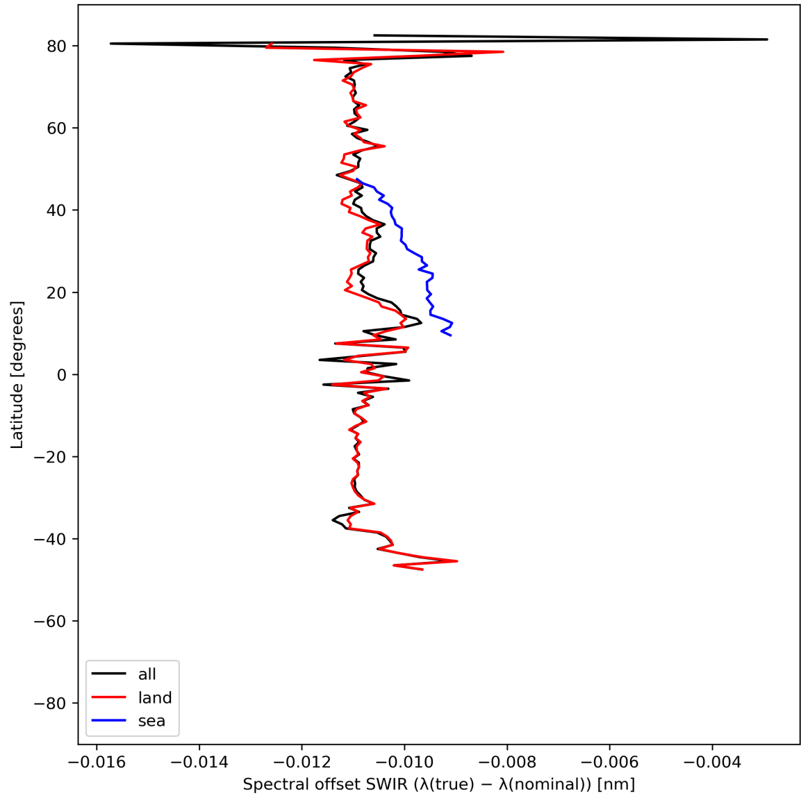
Figure 16: Zonal average of “Spectral offset SWIR ( \lambda(\text{true}) - \lambda(\text{nominal}) )” for 2024-07-10 to 2024-07-12.
