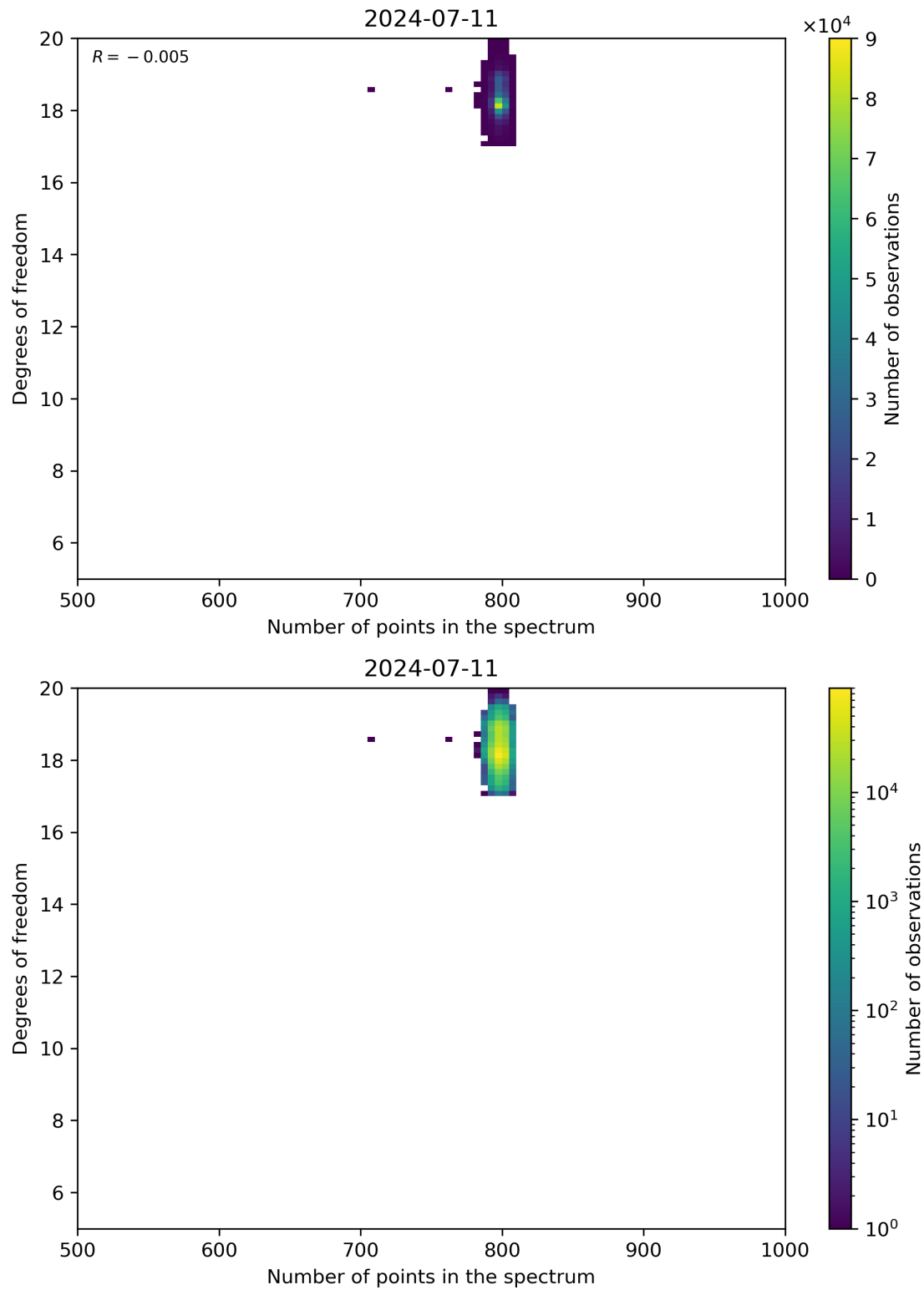
Figure 90: Scatter density plot of “Number of points in the spectrum” against “Degrees of freedom” for 2024-07-10 to 2024-07-12.
