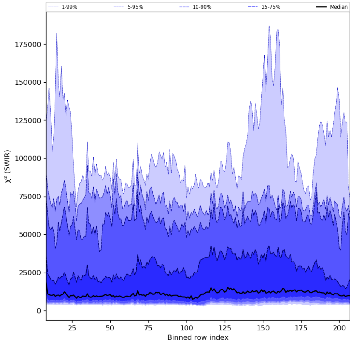
Figure 39: Along track statistics of “ \chi^2 (SWIR)” for 2024-07-10 to 2024-07-12
