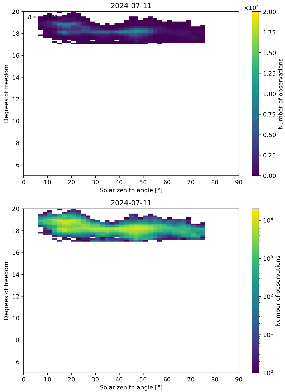
Figure 96: Scatter density plot of “Solar zenith angle” against “Degrees of freedom” for 2024-07-10 to 2024-07-12.
