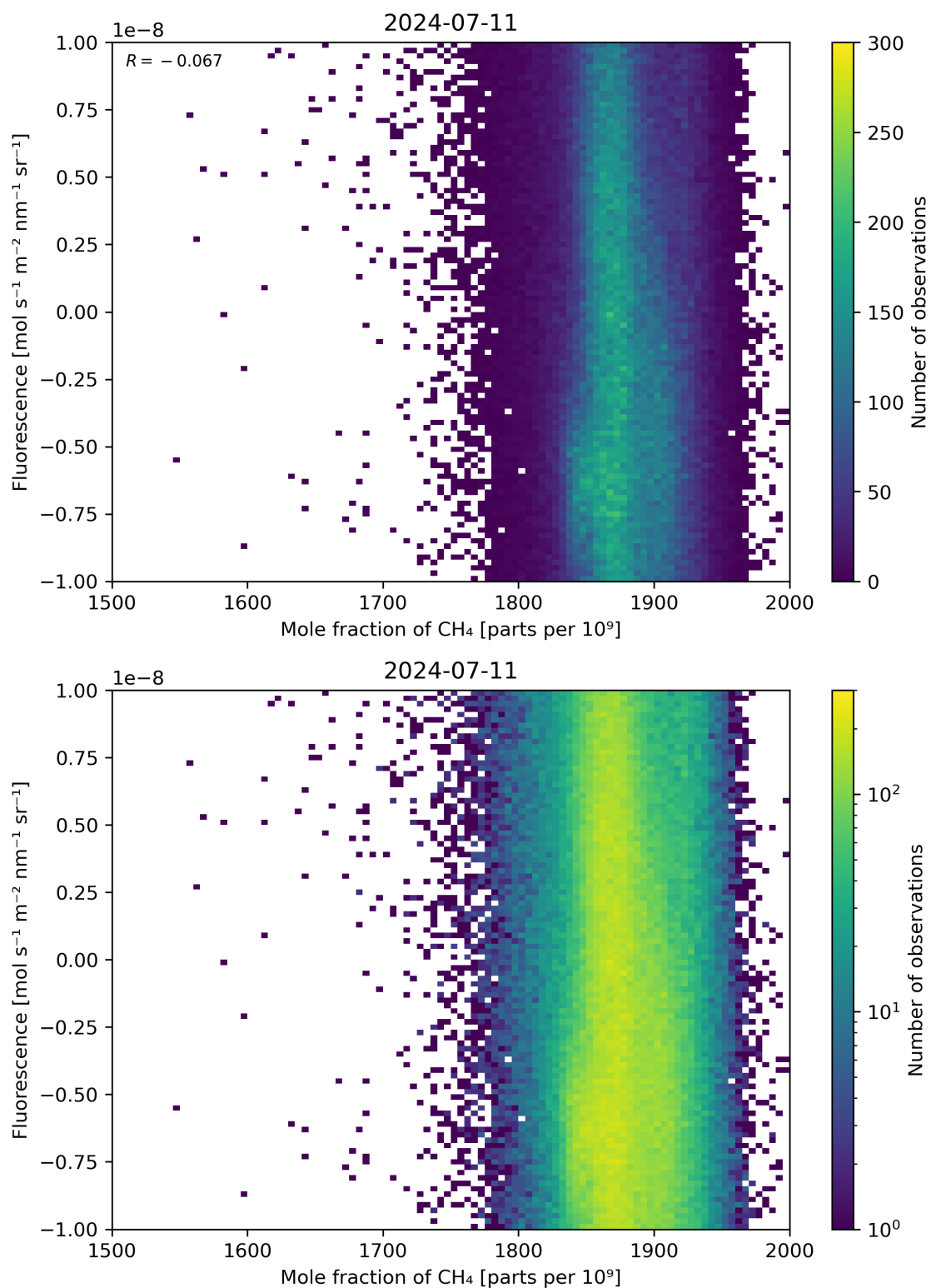
Figure 73: Scatter density plot of “Mole fraction of \text{CH}_4 ” against “Fluorescence” for 2024-07-10 to 2024-07-12.
