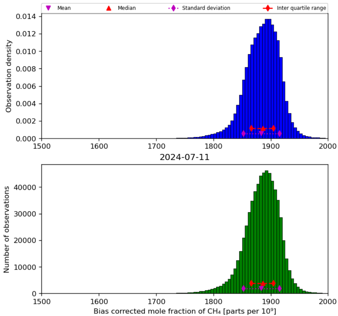
Figure 25: Histogram of “Bias corrected mole fraction of CH 4 ” for 2024-07-10 to 2024-07-12
