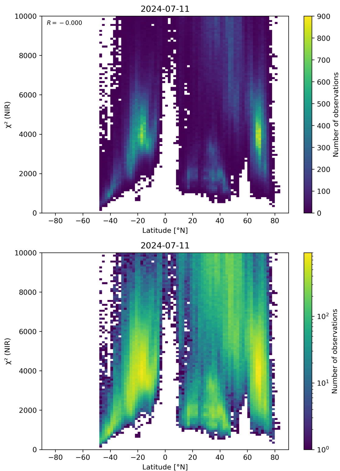
Figure 53: Scatter density plot of “Latitude” against “ \chi^2 (NIR)” for 2024-07-10 to 2024-07-12.
