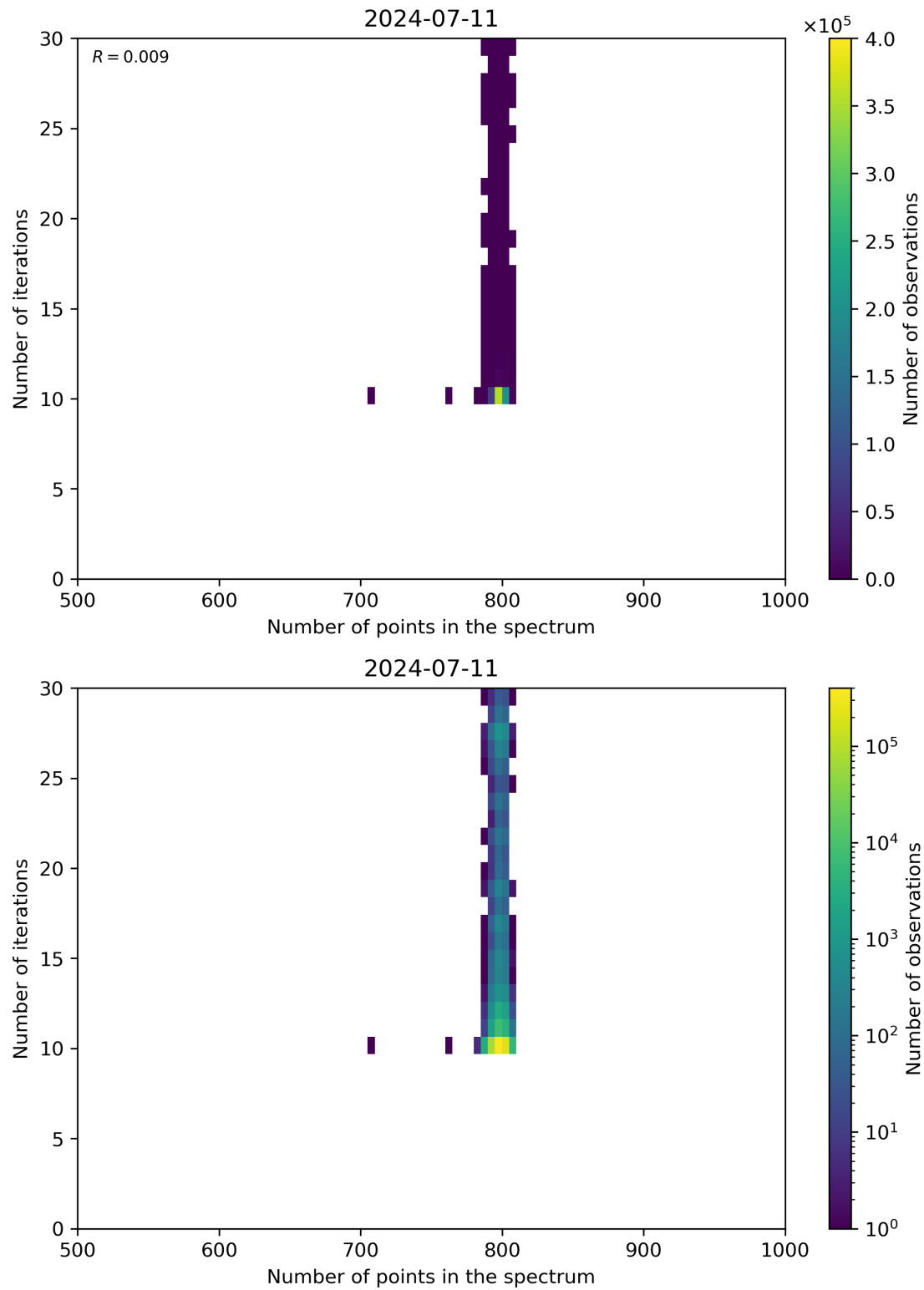
Figure 92: Scatter density plot of “Number of points in the spectrum” against “Number of iterations” for 2024-07-10 to 2024-07-12.
