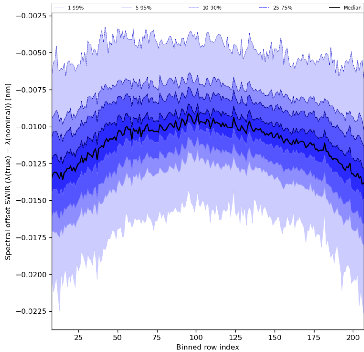
Figure 38: Along track statistics of “Spectral offset SWIR ( \lambda(\text{true}) - \lambda(\text{nominal}) )” for 2024-07-10 to 2024-07-12
