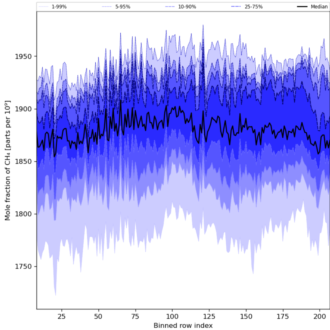
Figure 34: Along track statistics of “Mole fraction of CH 4 ” for 2024-07-10 to 2024-07-12
