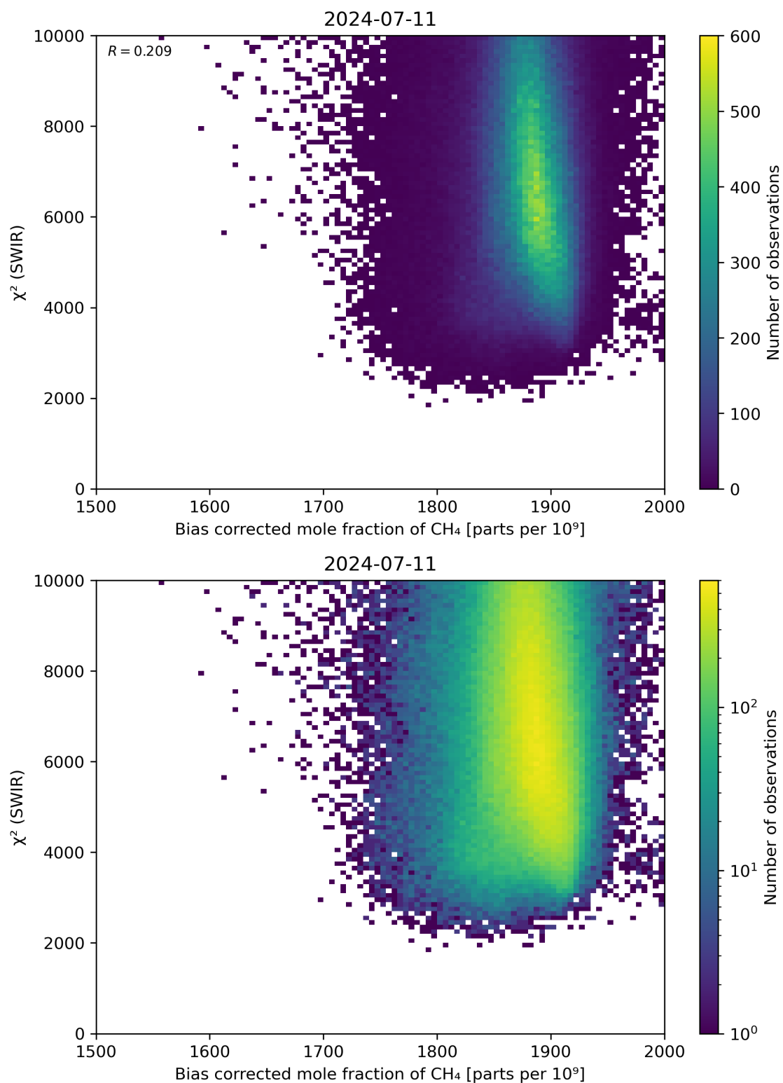
Figure 64: Scatter density plot of “Bias corrected mole fraction of CH 4 ” against “ \chi^2 (SWIR)” for 2024-07-10 to 2024-07-12.
