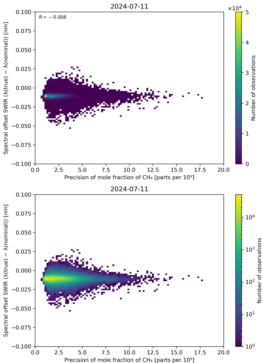
Figure 85: Scatter density plot of “Precision of mole fraction of CH 4 ” against “Spectral offset SWIR ( \lambda(\text{true}) - \lambda(\text{nominal}) )” for 2024-07-10 to 2024-07-12.
