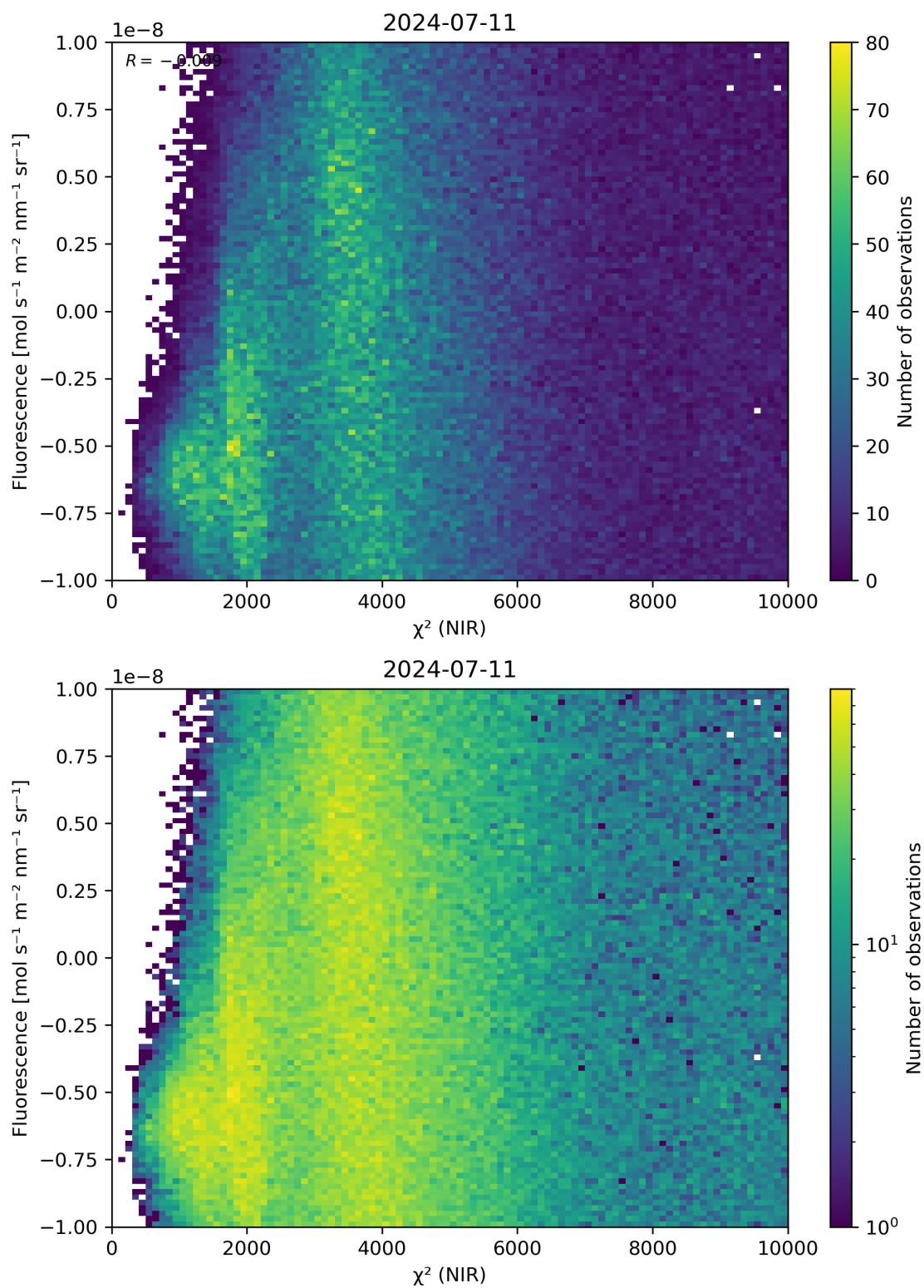
Figure 45: Scatter density plot of “ \chi^2 (NIR)” against “Fluorescence” for 2024-07-10 to 2024-07-12.
