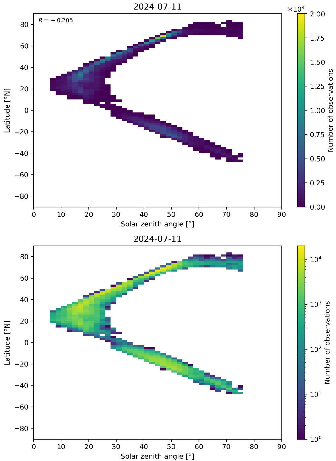
Figure 98: Scatter density plot of “Solar zenith angle” against “Latitude” for 2024-07-10 to 2024-07-12.
