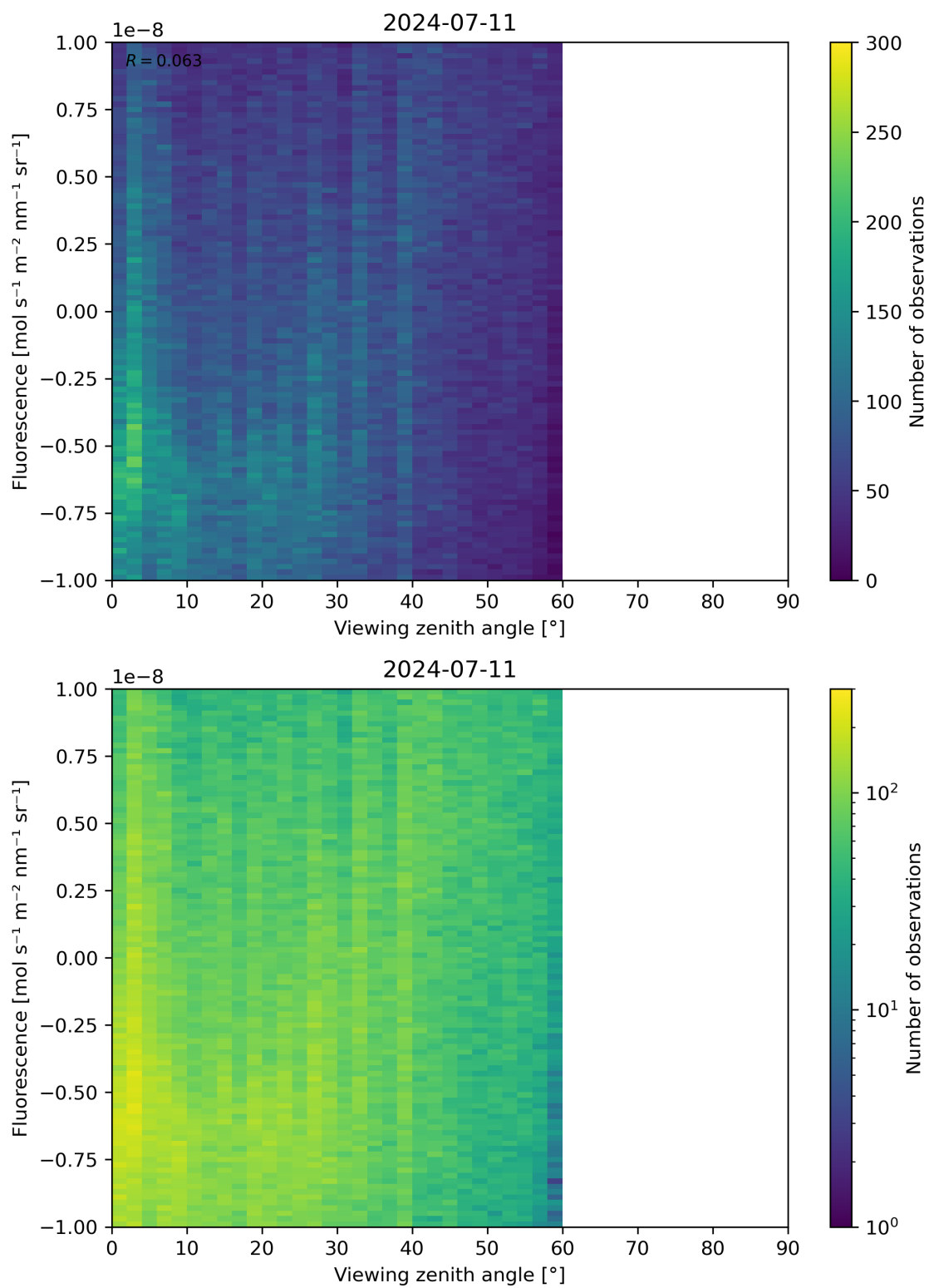
Figure 108: Scatter density plot of “Viewing zenith angle” against “Fluorescence” for 2024-07-10 to 2024-07-12.
