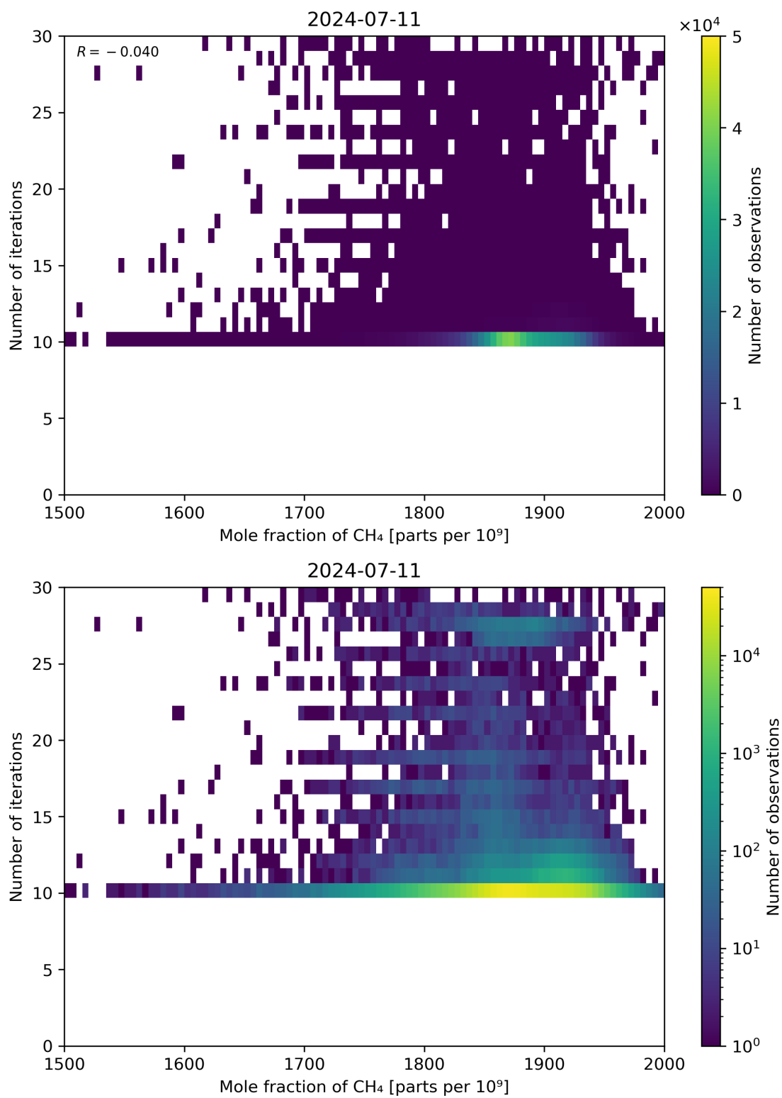
Figure 76: Scatter density plot of “Mole fraction of CH 4 ” against “Number of iterations” for 2024-07-10 to 2024-07-12.
