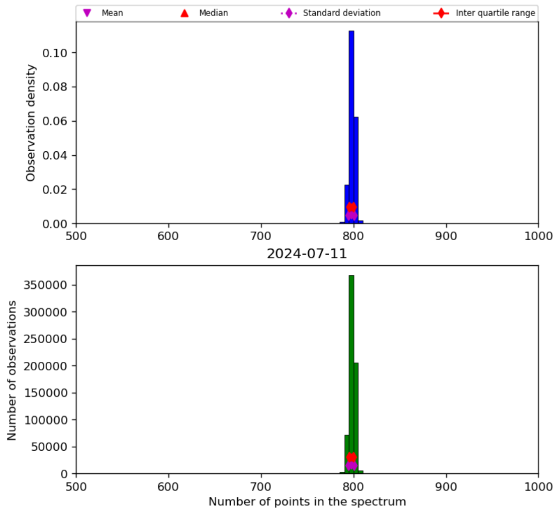
Figure 26: Histogram of “Number of points in the spectrum” for 2024-07-10 to 2024-07-12
