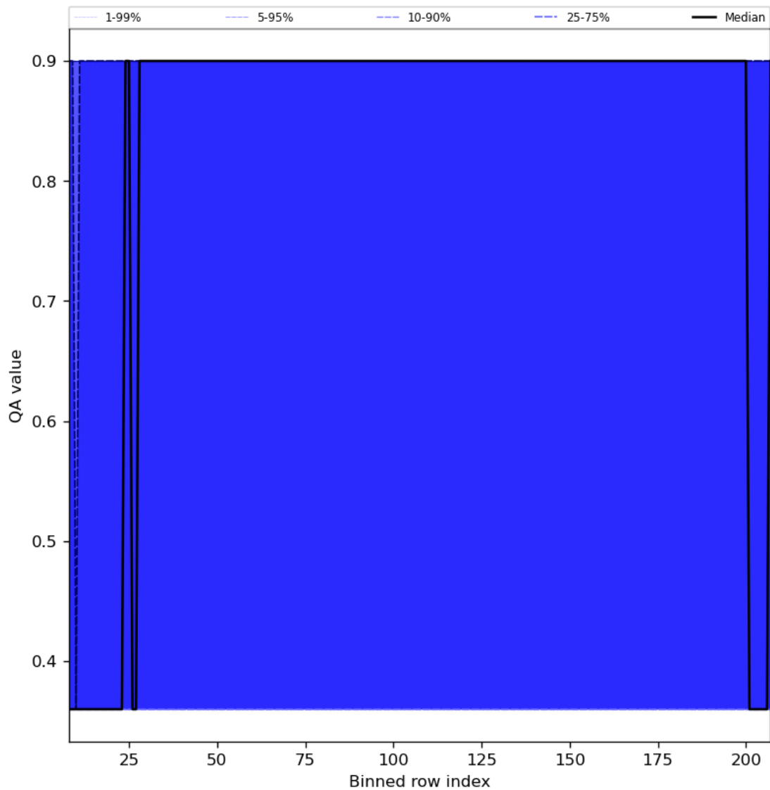
Figure 33: Along track statistics of “QA value” for 2024-07-10 to 2024-07-12
