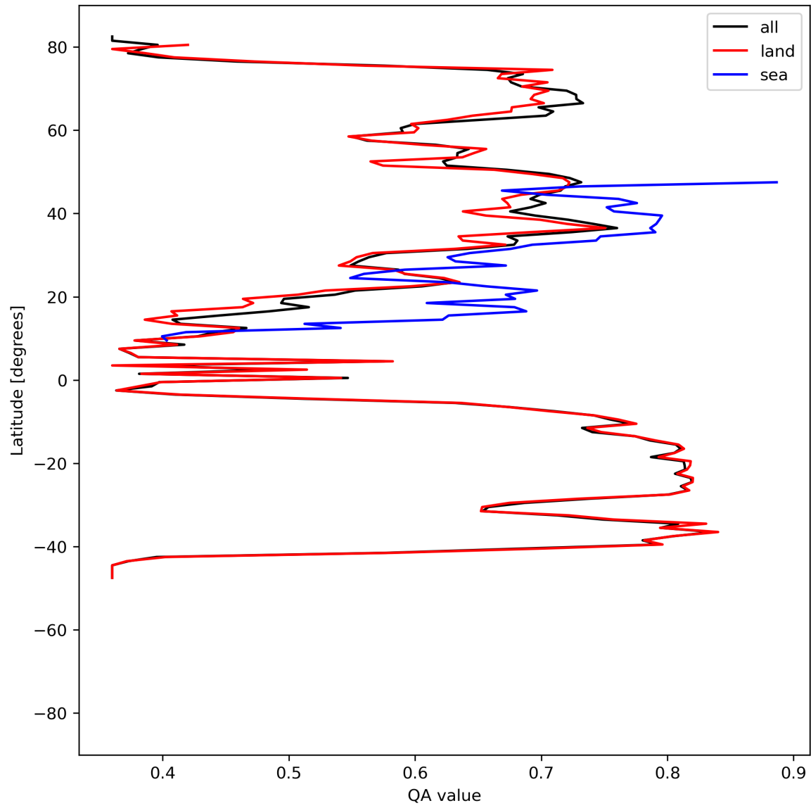
Figure 11: Zonal average of “QA value” for 2024-07-10 to 2024-07-12.
