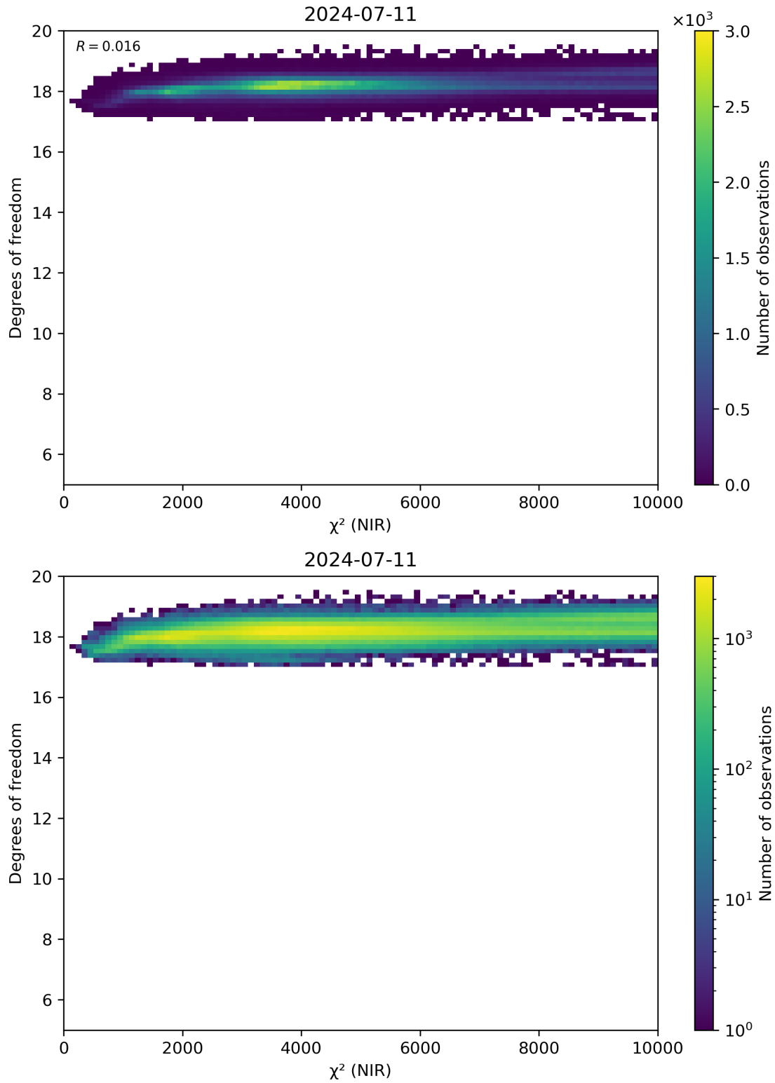
Figure 44: Scatter density plot of “ \chi^2 (NIR)” against “Degrees of freedom” for 2024-07-10 to 2024-07-12.
