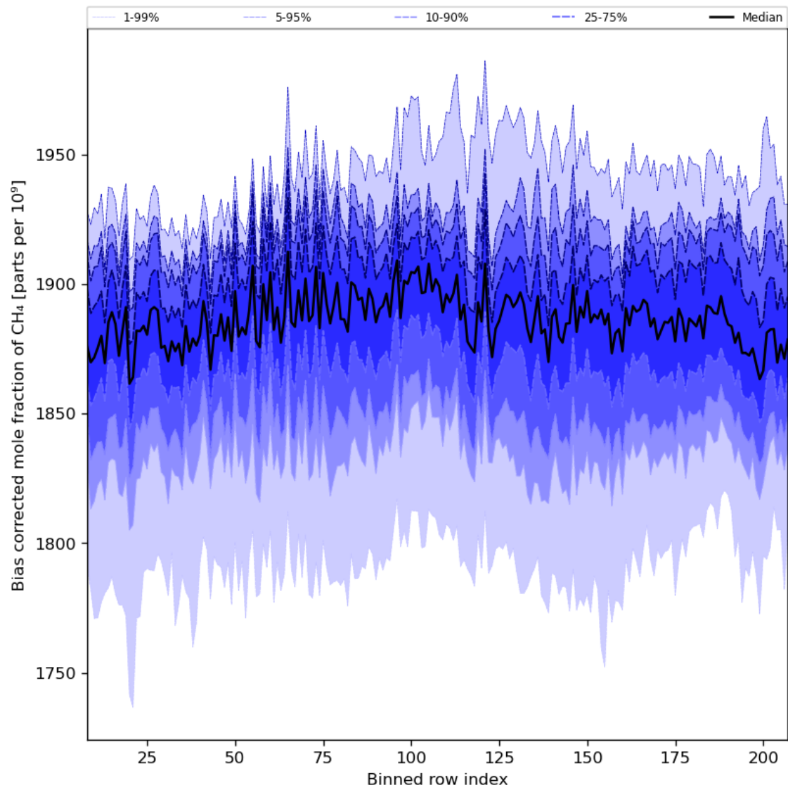
Figure 36: Along track statistics of “Bias corrected mole fraction of CH 4 ” for 2024-07-10 to 2024-07-12
