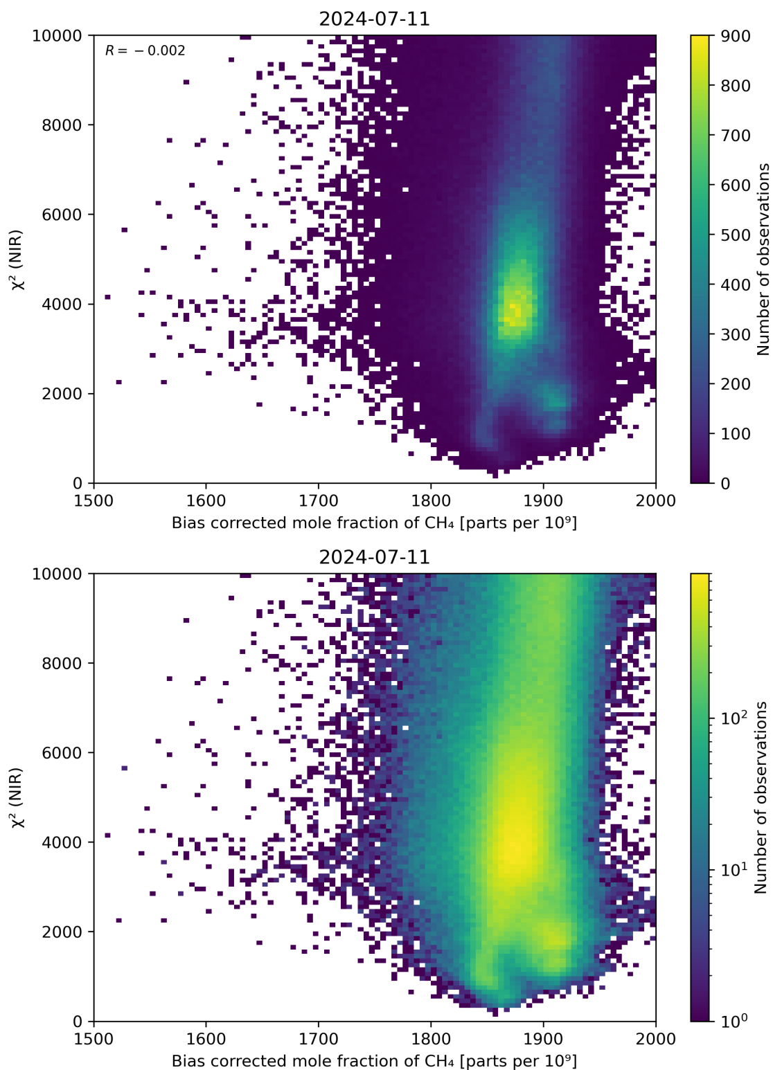
Figure 63: Scatter density plot of “Bias corrected mole fraction of CH 4 ” against “ \chi^2 (NIR)” for 2024-07-10 to 2024-07-12.
