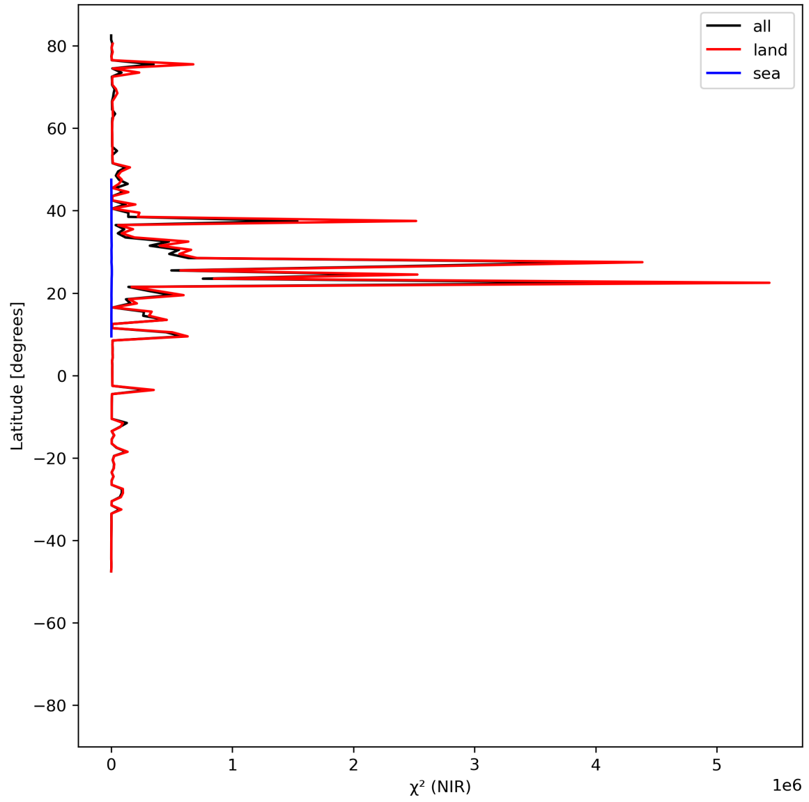
Figure 18: Zonal average of “ \chi^2 (NIR)” for 2024-07-10 to 2024-07-12.
