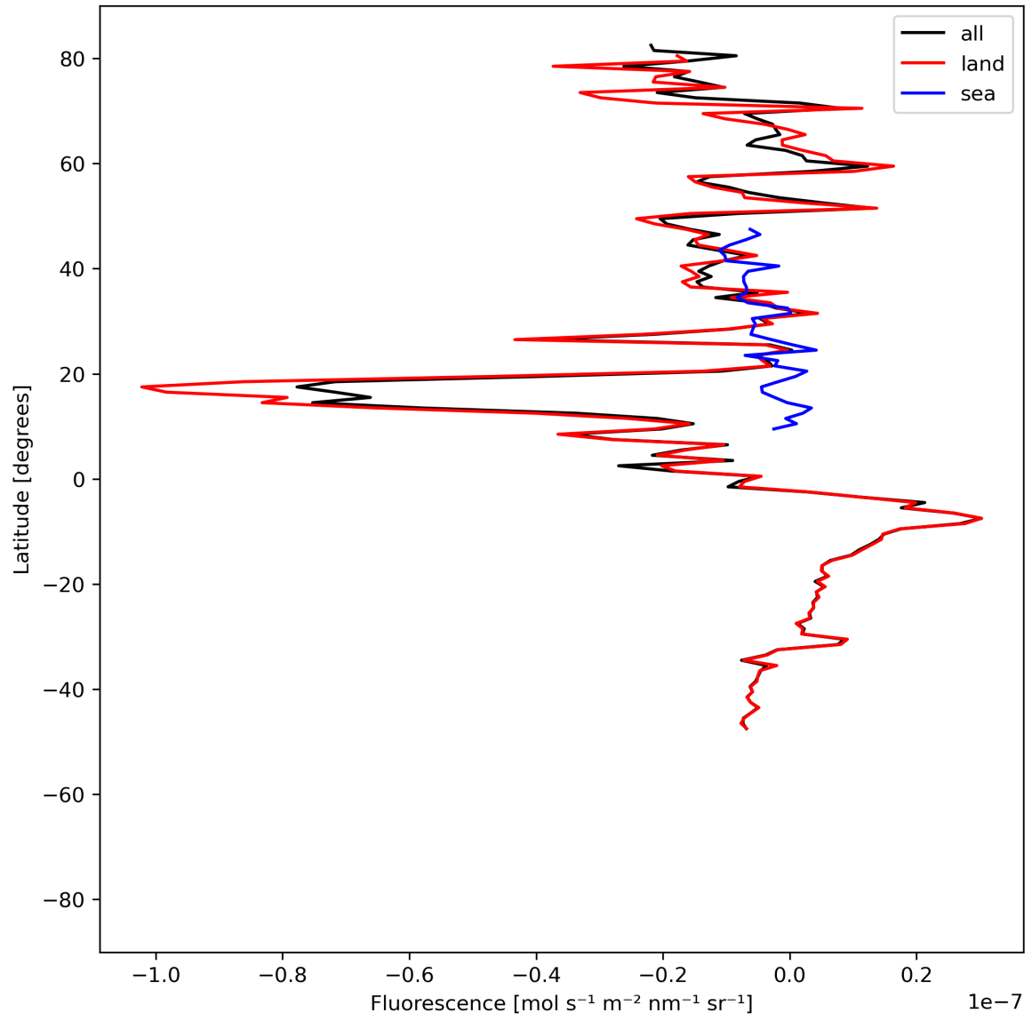
Figure 21: Zonal average of “Fluorescence” for 2024-07-10 to 2024-07-12.
