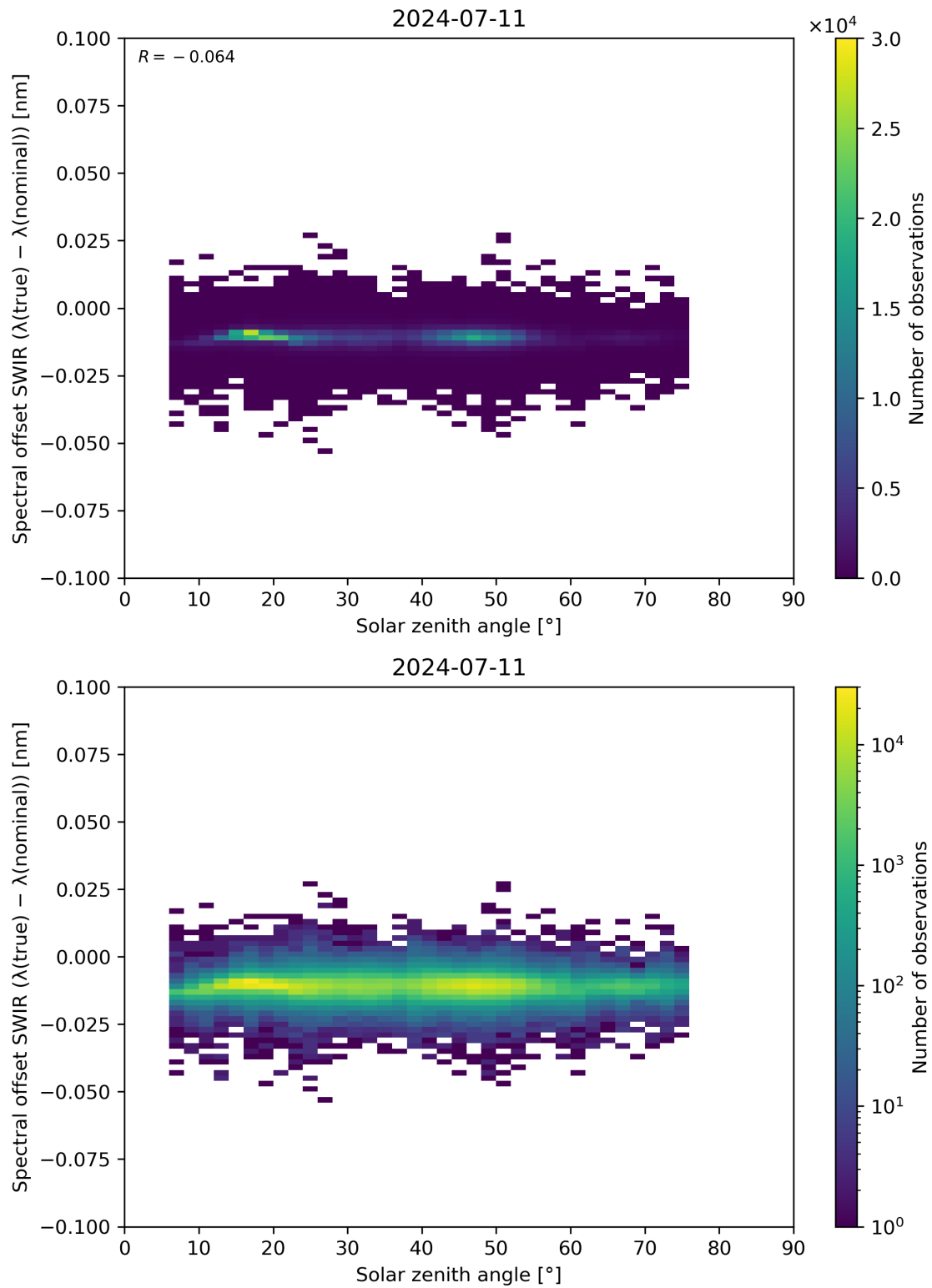
Figure 104: Scatter density plot of “Solar zenith angle” against “Spectral offset SWIR ( \lambda(\text{true}) - \lambda(\text{nominal}) )” for 2024-07-10 to 2024-07-12.
