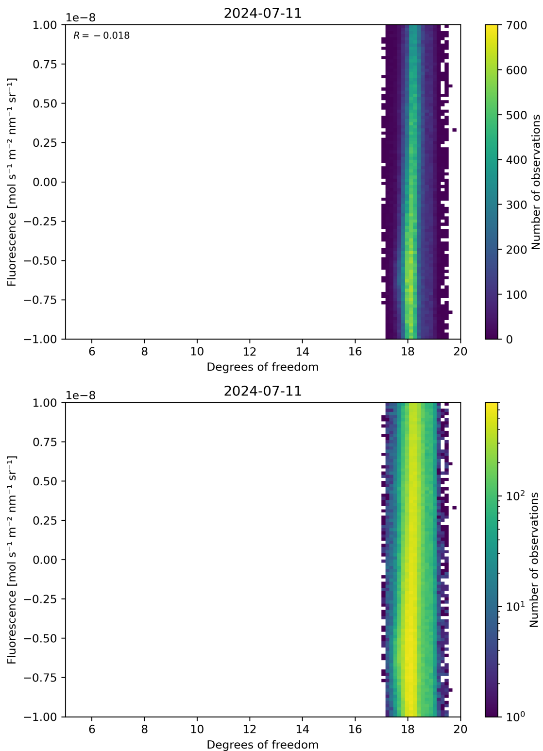
Figure 51: Scatter density plot of “Degrees of freedom” against “Fluorescence” for 2024-07-10 to 2024-07-12.
