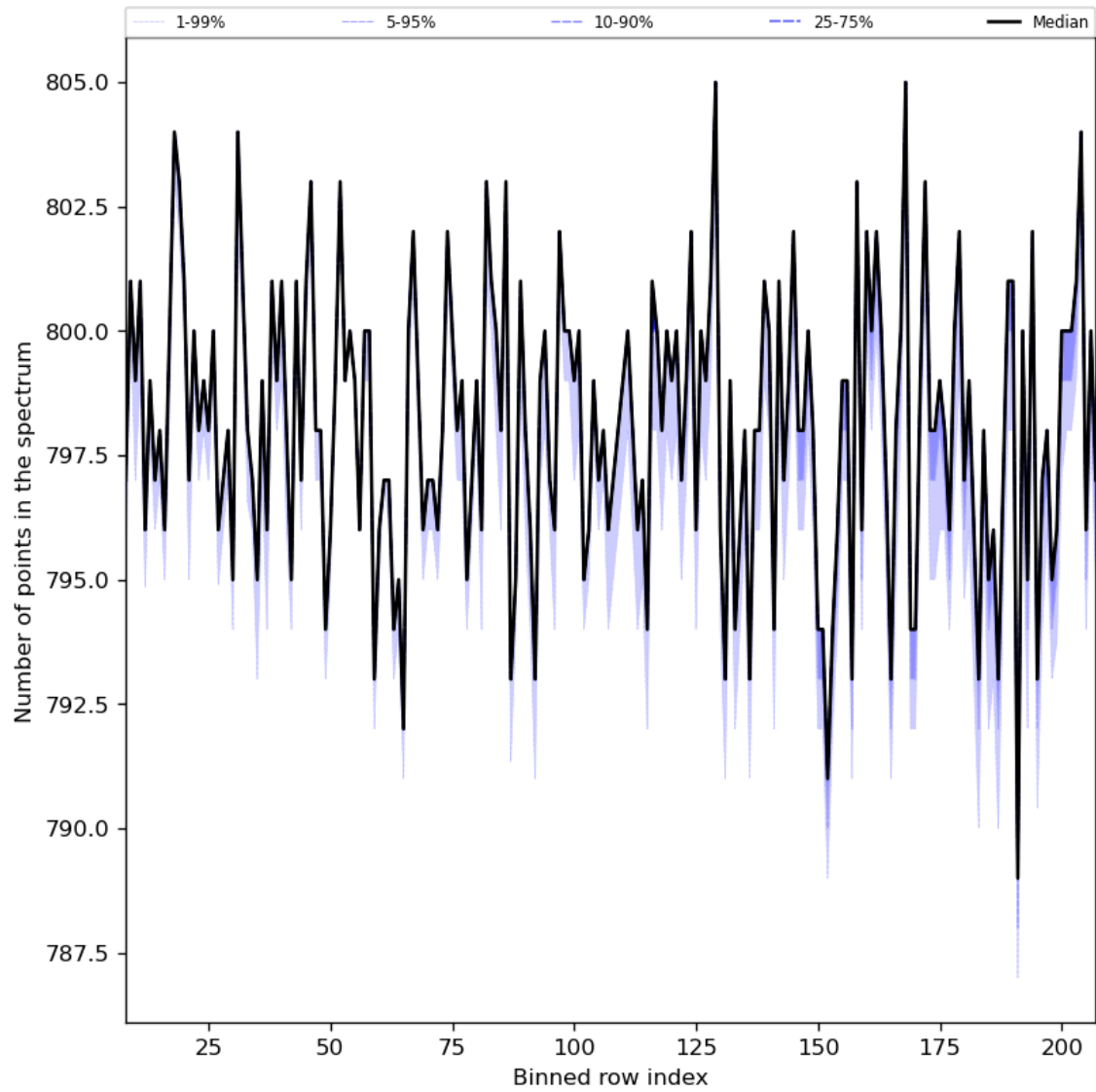
Figure 37: Along track statistics of “Number of points in the spectrum” for 2024-07-10 to 2024-07-12
