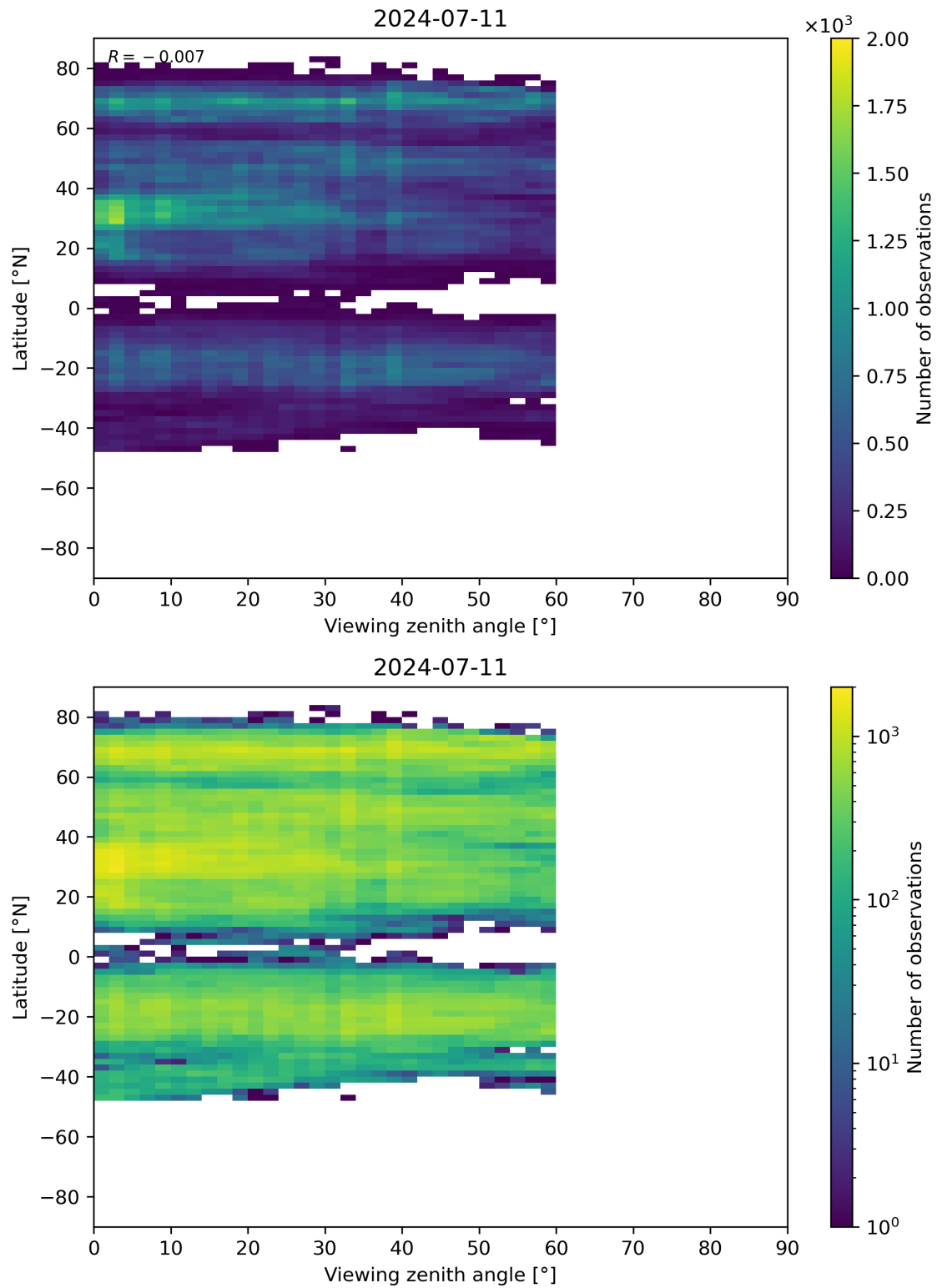
Figure 109: Scatter density plot of “Viewing zenith angle” against “Latitude” for 2024-07-10 to 2024-07-12.
