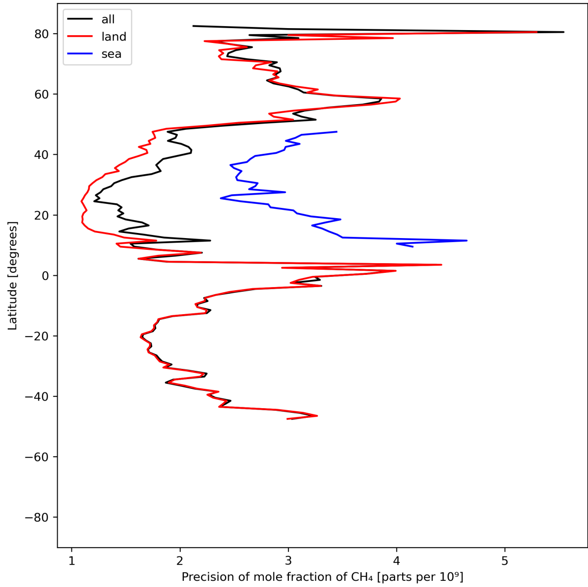
Figure 13: Zonal average of “Precision of mole fraction of \text{CH}_4 ” for 2024-07-10 to 2024-07-12.
