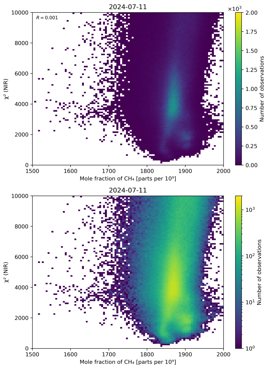
Figure 70: Scatter density plot of “Mole fraction of \text{CH}_4 ” against “ \chi^2 (NIR)” for 2024-07-10 to 2024-07-12.
