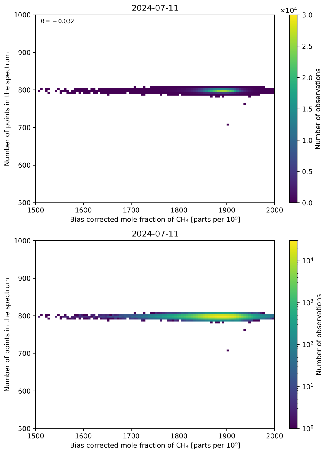
Figure 68: Scatter density plot of “Bias corrected mole fraction of CH 4 ” against “Number of points in the spectrum” for 2024-07-10 to 2024-07-12.
