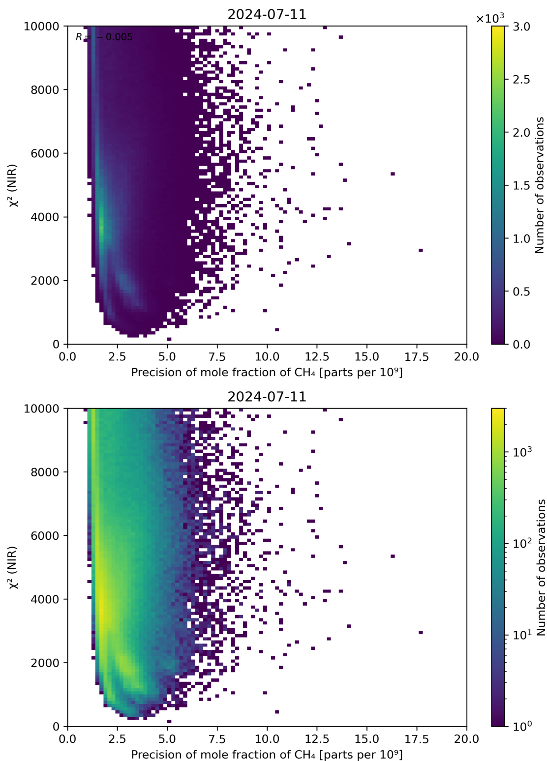
Figure 78: Scatter density plot of “Precision of mole fraction of CH 4 ” against “ \chi^2 (NIR)” for 2024-07-10 to 2024-07-12.
