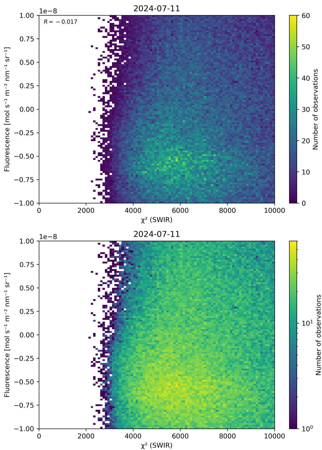
Figure 49: Scatter density plot of “ \chi^2 (SWIR)” against “Fluorescence” for 2024-07-10 to 2024-07-12.
