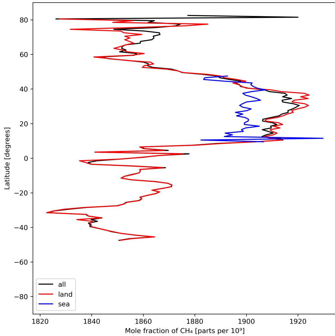
Figure 12: Zonal average of “Mole fraction of CH 4 ” for 2024-07-10 to 2024-07-12.
