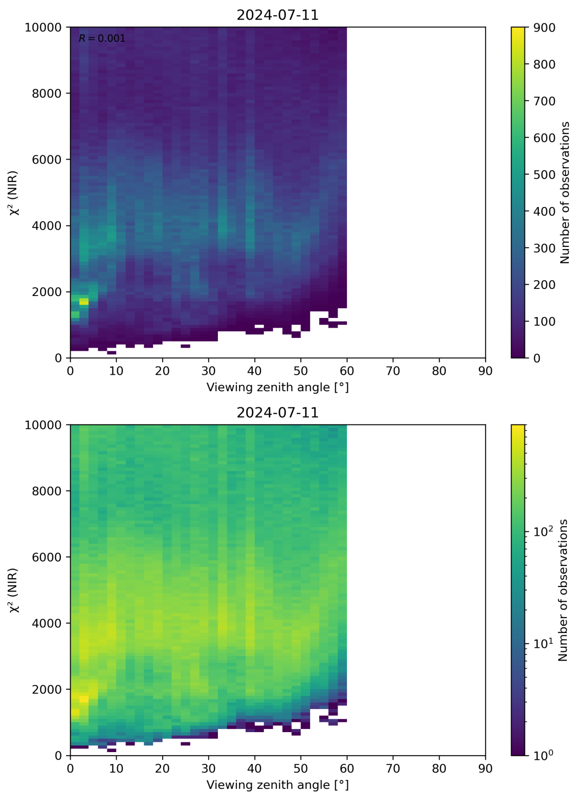
Figure 105: Scatter density plot of “Viewing zenith angle” against “ \chi^2 (NIR)” for 2024-07-10 to 2024-07-12.
