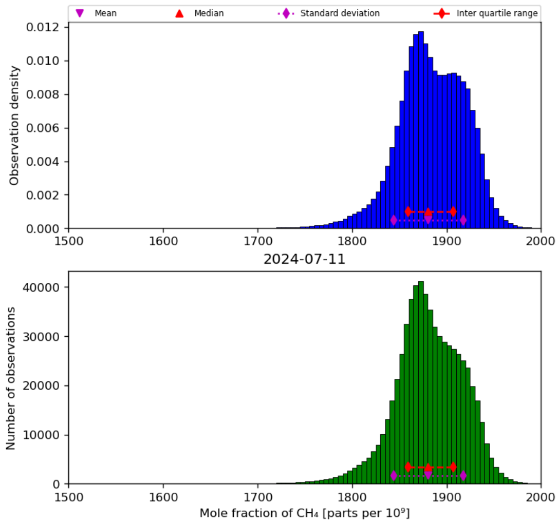
Figure 23: Histogram of “Mole fraction of CH 4 ” for 2024-07-10 to 2024-07-12
