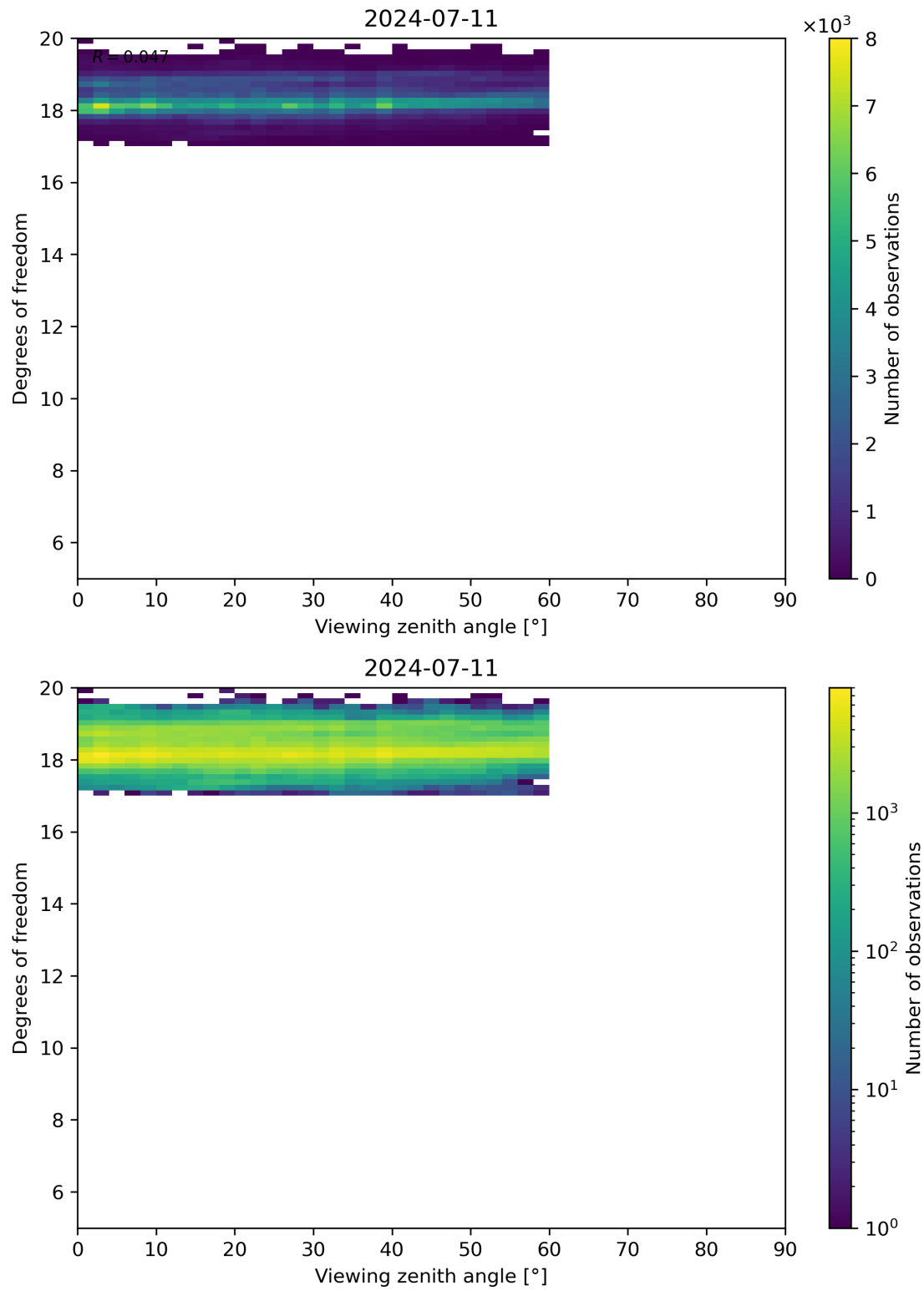
Figure 107: Scatter density plot of “Viewing zenith angle” against “Degrees of freedom” for 2024-07-10 to 2024-07-12.
