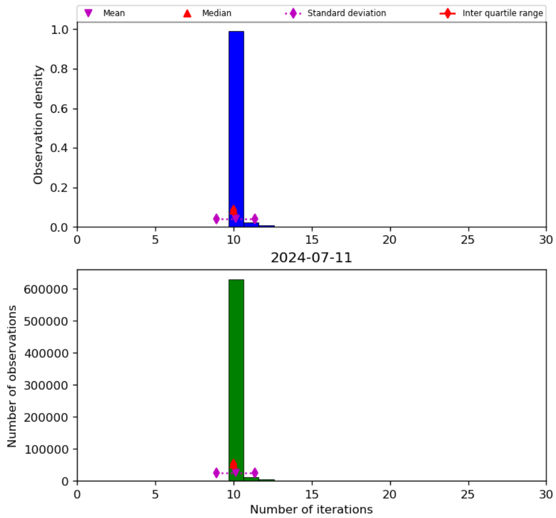
Figure 31: Histogram of “Number of iterations” for 2024-07-10 to 2024-07-12
