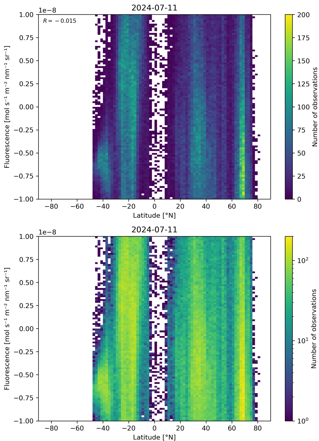
Figure 56: Scatter density plot of “Latitude” against “Fluorescence” for 2024-07-10 to 2024-07-12.
