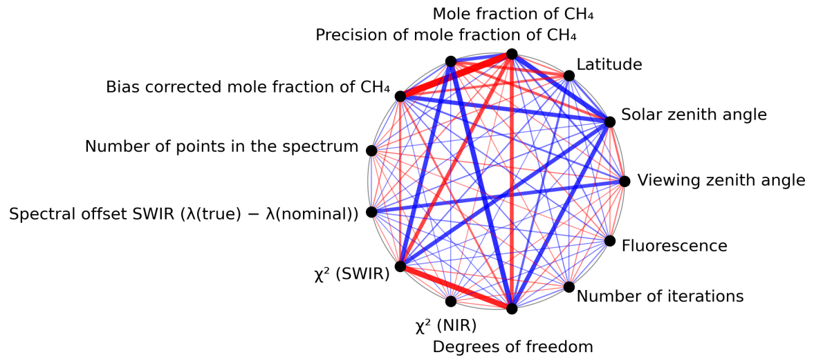
Figure 1: Map of correlation graph for 2024-07-10 to 2024-07-12.
