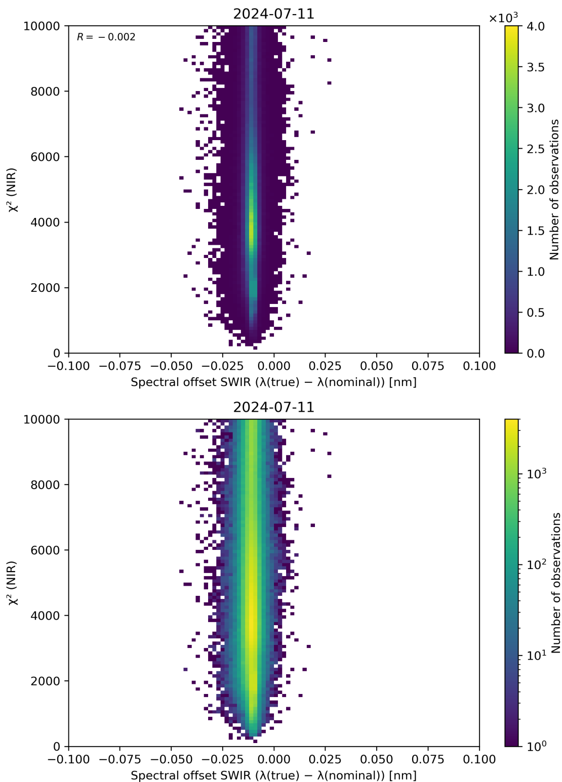
Figure 117: Scatter density plot of “Spectral offset SWIR ( \lambda(\text{true}) - \lambda(\text{nominal}) )” against “ \chi^2 (NIR)” for 2024-07-10 to 2024-07-12.
