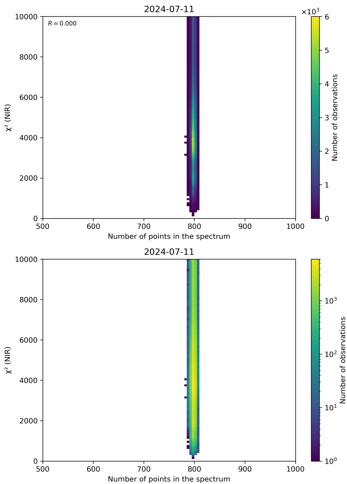
Figure 88: Scatter density plot of “Number of points in the spectrum” against “ \chi^2 (NIR)” for 2024-07-10 to 2024-07-12.
