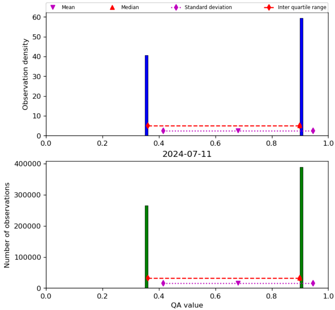
Figure 22: Histogram of “QA value” for 2024-07-10 to 2024-07-12
