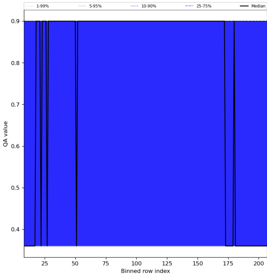
Figure 33: Along track statistics of “QA value” for 2024-07-11 to 2024-07-13
