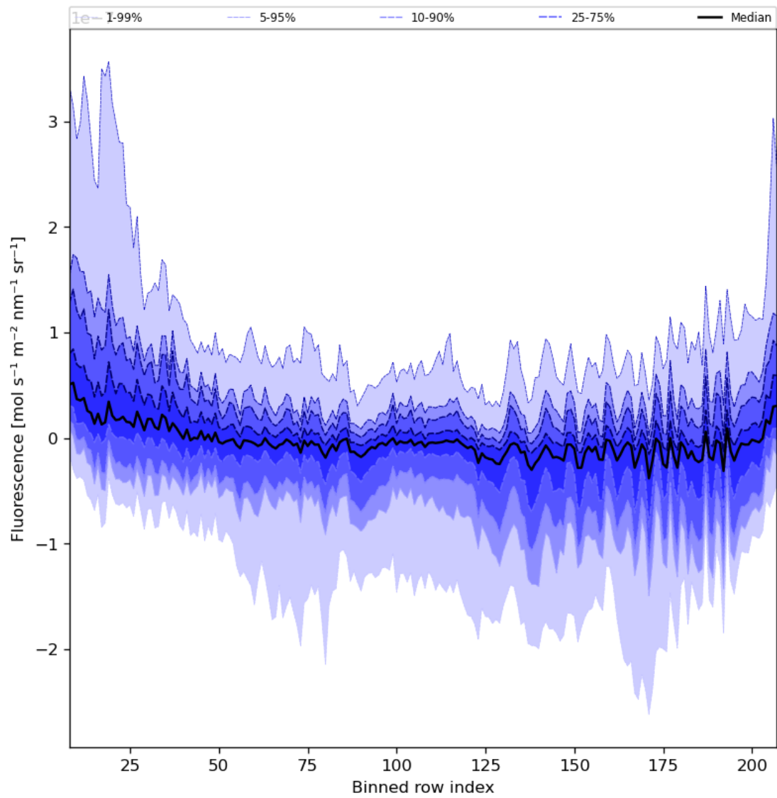
Figure 43: Along track statistics of “Fluorescence” for 2024-07-11 to 2024-07-13
