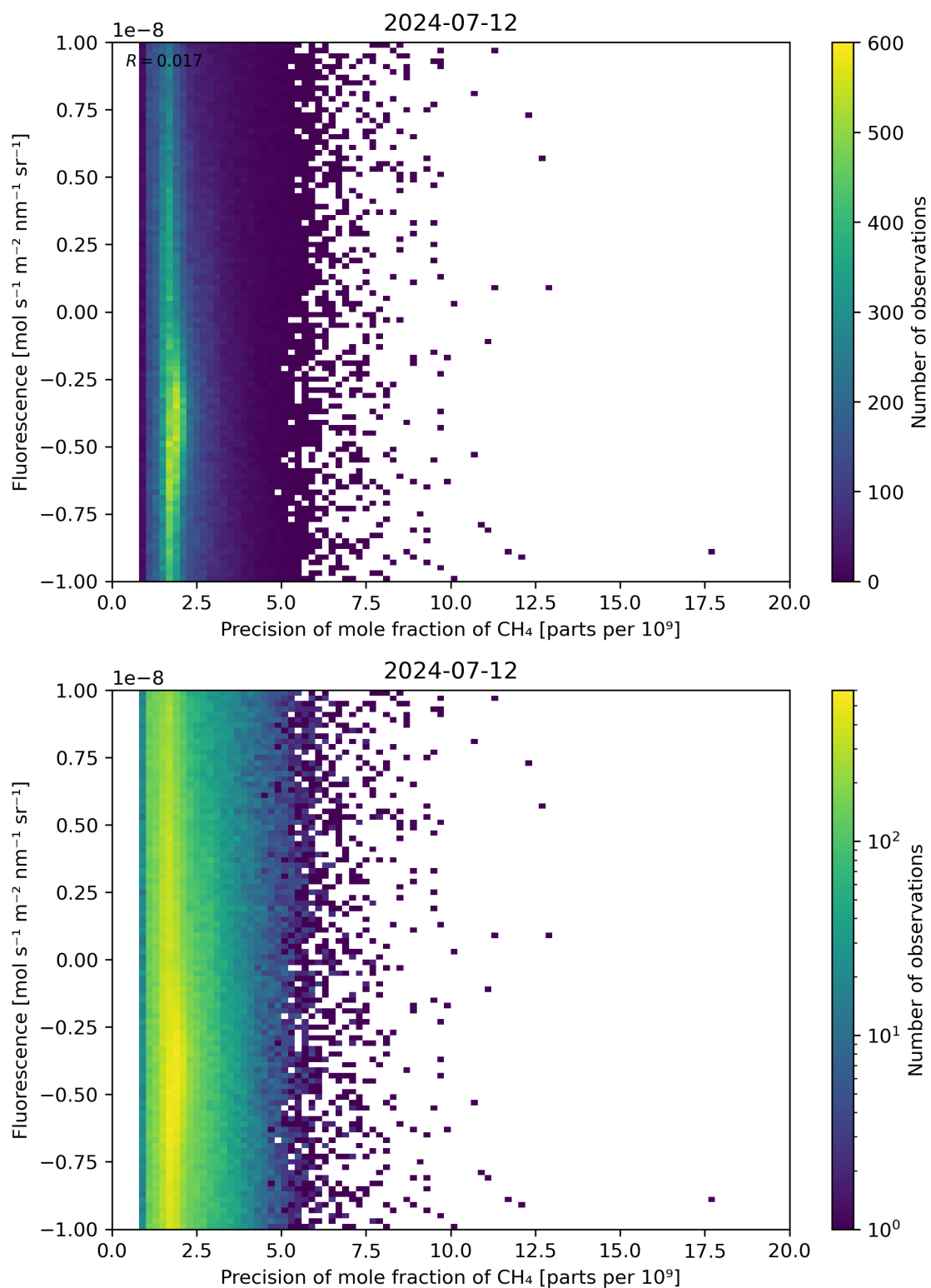
Figure 81: Scatter density plot of “Precision of mole fraction of \text{CH}_4 ” against “Fluorescence” for 2024-07-11 to 2024-07-13.
