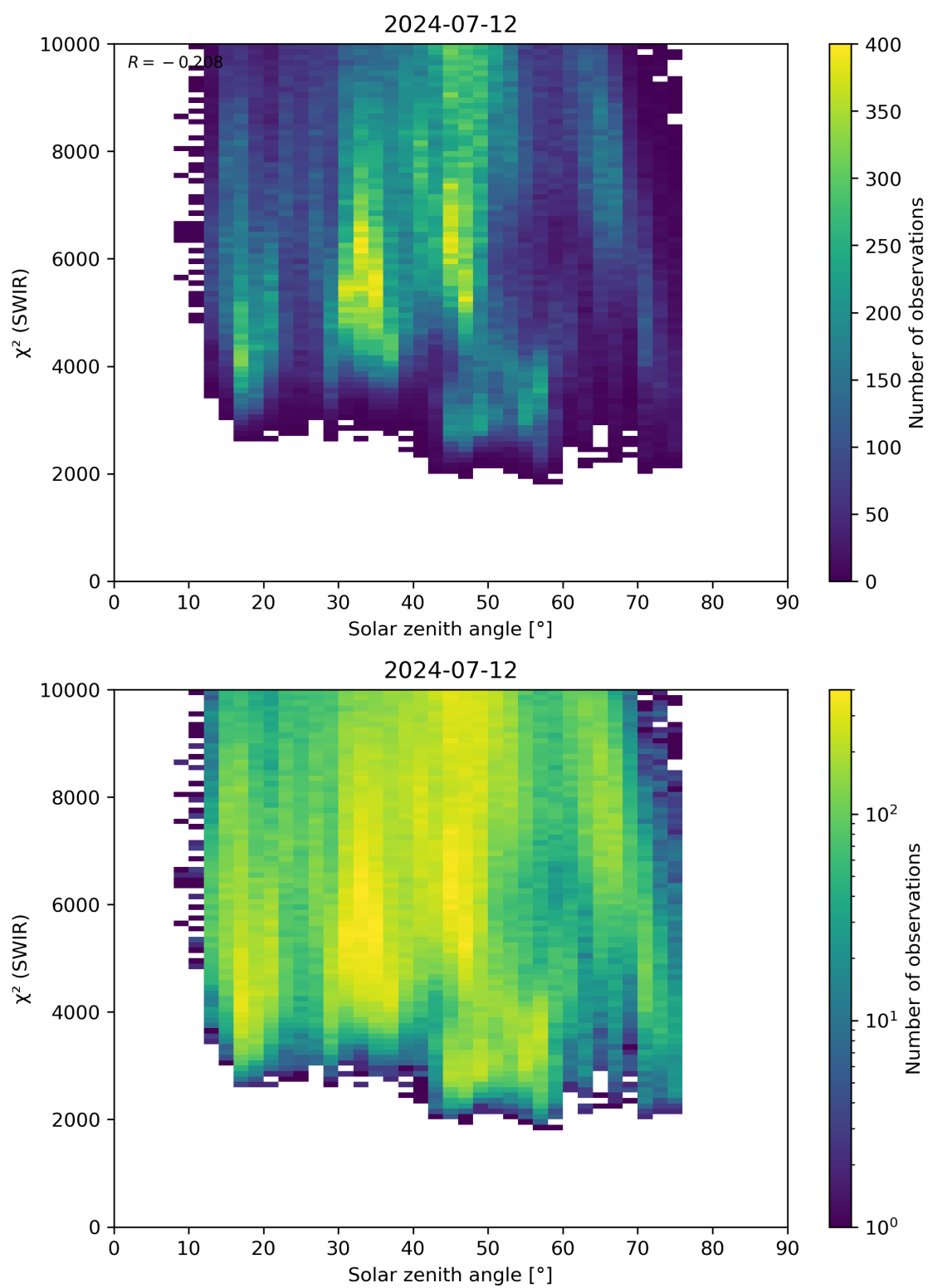
Figure 95: Scatter density plot of “Solar zenith angle” against “ \chi^2 (SWIR)” for 2024-07-11 to 2024-07-13.
