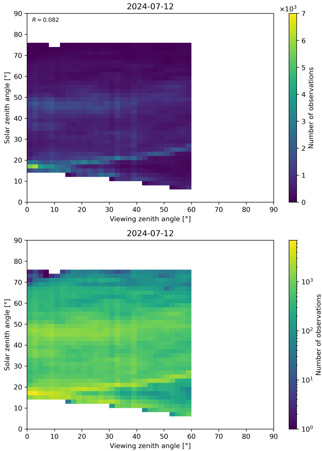
Figure 115: Scatter density plot of “Viewing zenith angle” against “Solar zenith angle” for 2024-07-11 to 2024-07-13.
