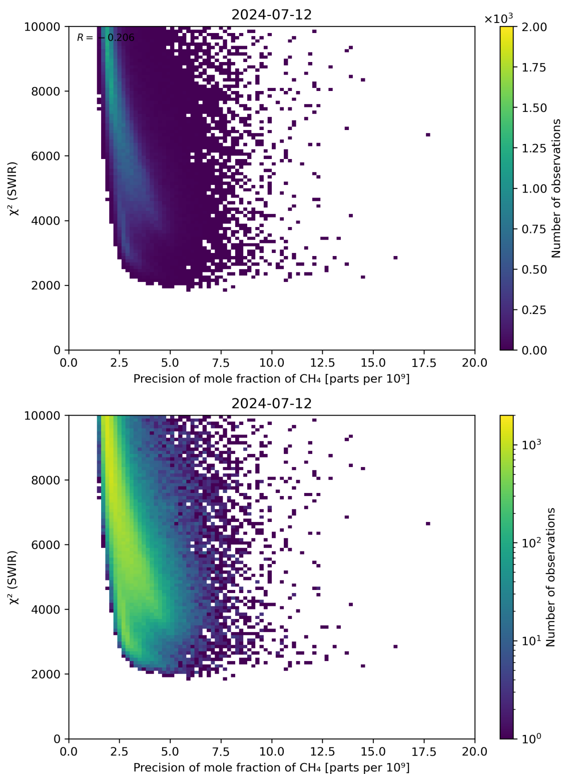
Figure 79: Scatter density plot of “Precision of mole fraction of \text{CH}_4 ” against “ \chi^2 (SWIR)” for 2024-07-11 to 2024-07-13.
