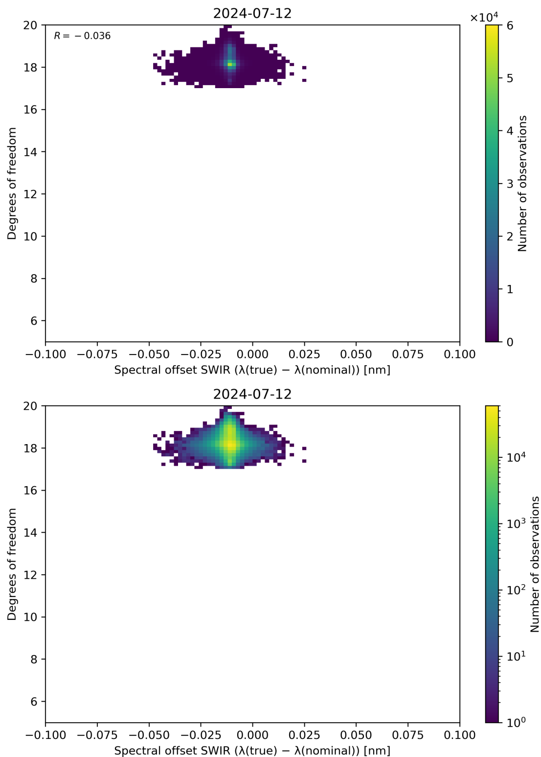
Figure 119: Scatter density plot of “Spectral offset SWIR ( \lambda(\text{true}) - \lambda(\text{nominal}) )” against “Degrees of freedom” for 2024-07-11 to 2024-07-13.
