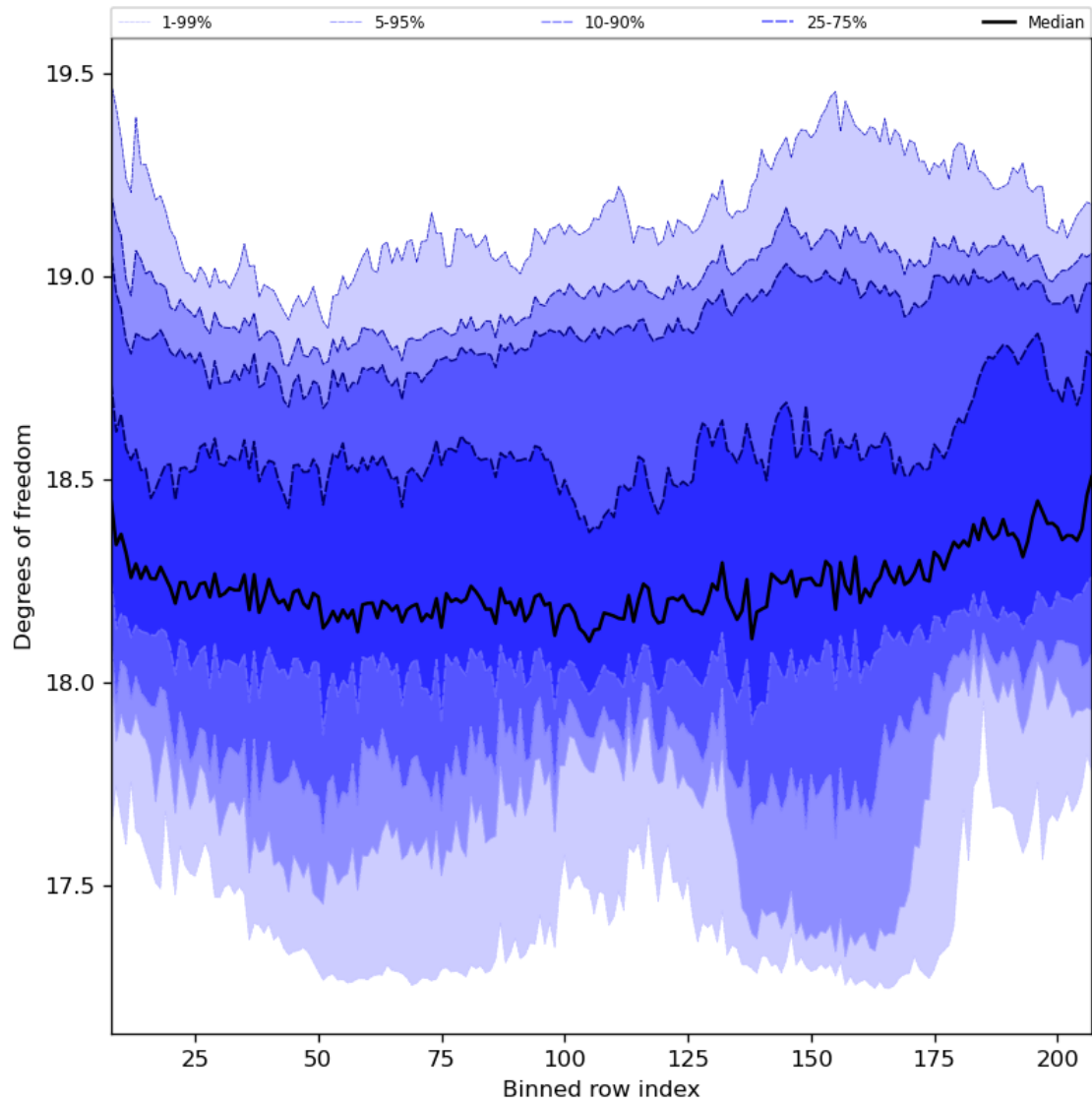
Figure 41: Along track statistics of “Degrees of freedom” for 2024-07-11 to 2024-07-13
