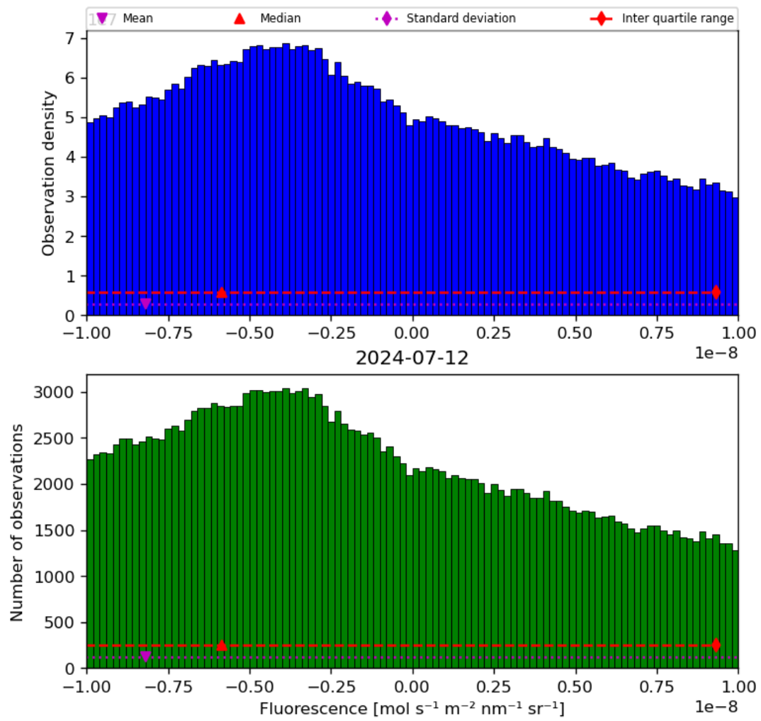
Figure 32: Histogram of “Fluorescence” for 2024-07-11 to 2024-07-13
