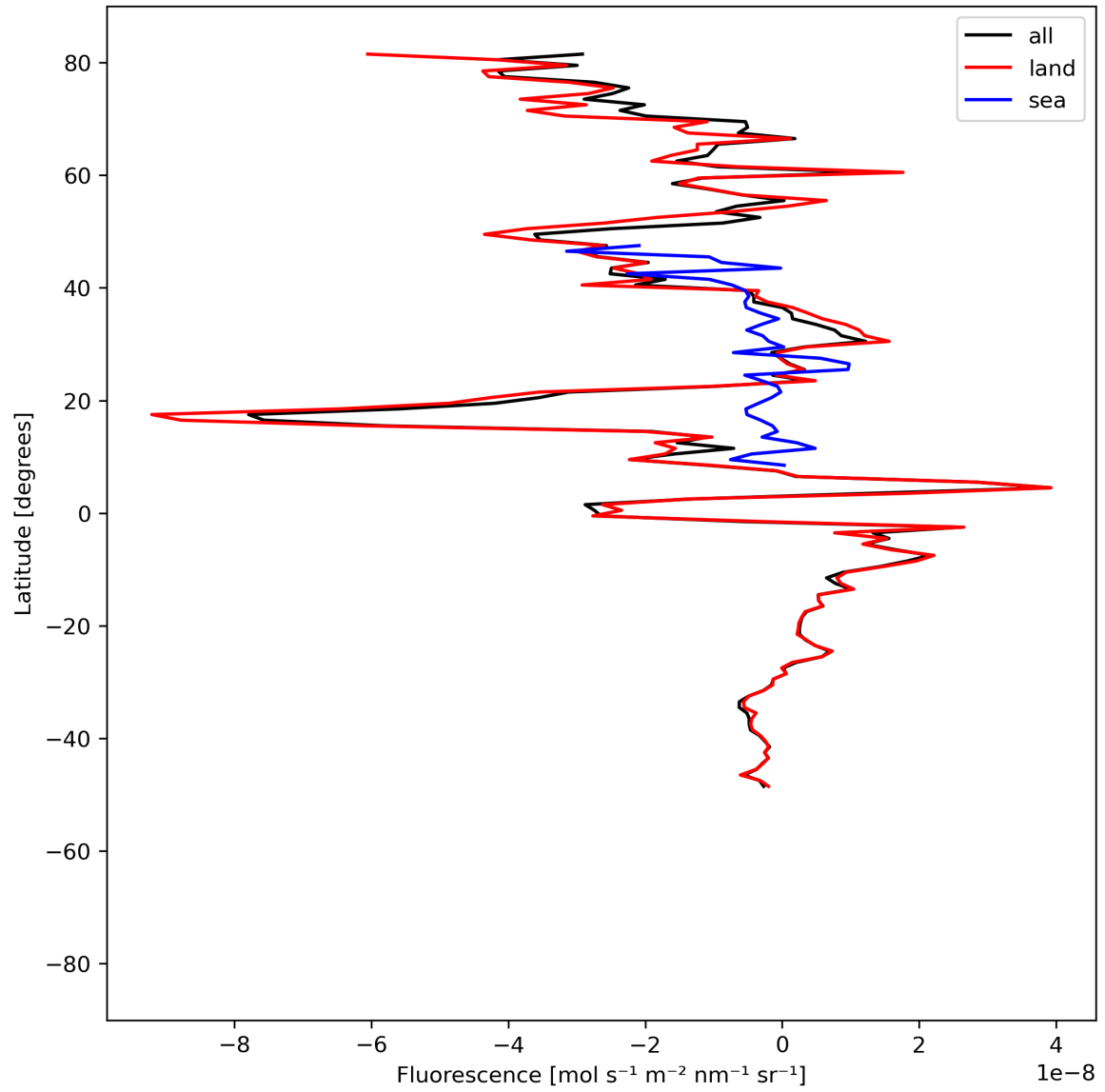
Figure 21: Zonal average of “Fluorescence” for 2024-07-11 to 2024-07-13.
