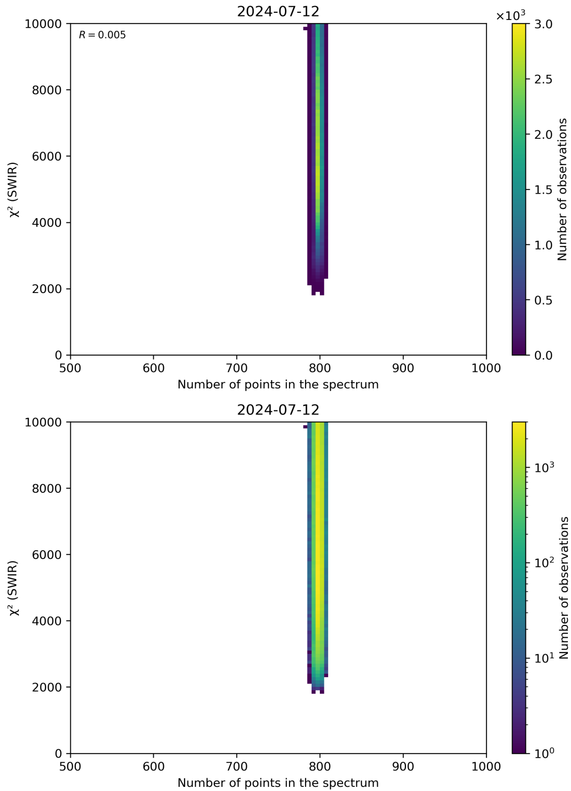
Figure 89: Scatter density plot of “Number of points in the spectrum” against “ \chi^2 (SWIR)” for 2024-07-11 to 2024-07-13.
