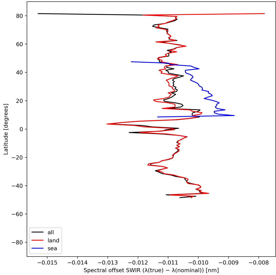
Figure 16: Zonal average of “Spectral offset SWIR ( \lambda(\text{true}) - \lambda(\text{nominal}) )” for 2024-07-11 to 2024-07-13.
