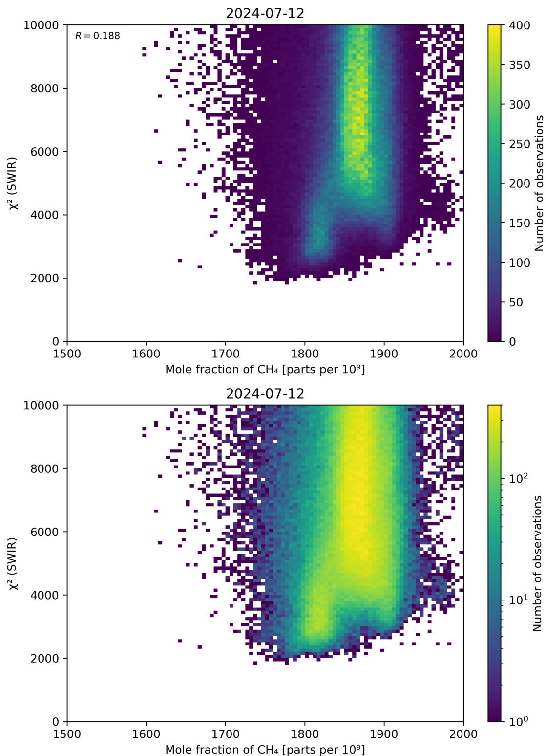
Figure 71: Scatter density plot of “Mole fraction of \text{CH}_4 ” against “ \chi^2 (SWIR)” for 2024-07-11 to 2024-07-13.
