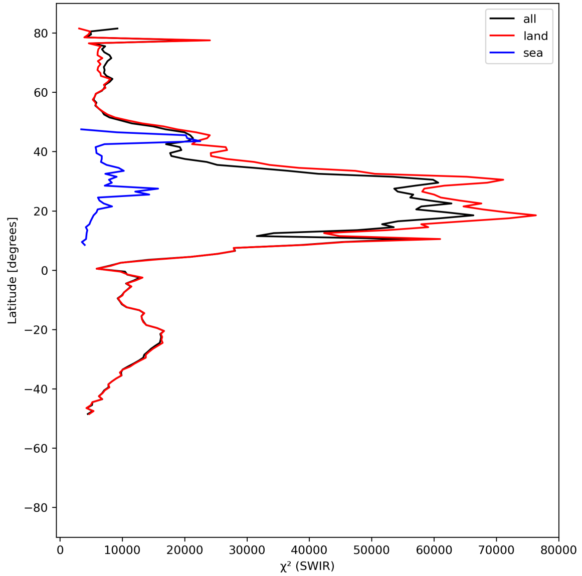
Figure 17: Zonal average of “ \chi^2 (SWIR)” for 2024-07-11 to 2024-07-13.
