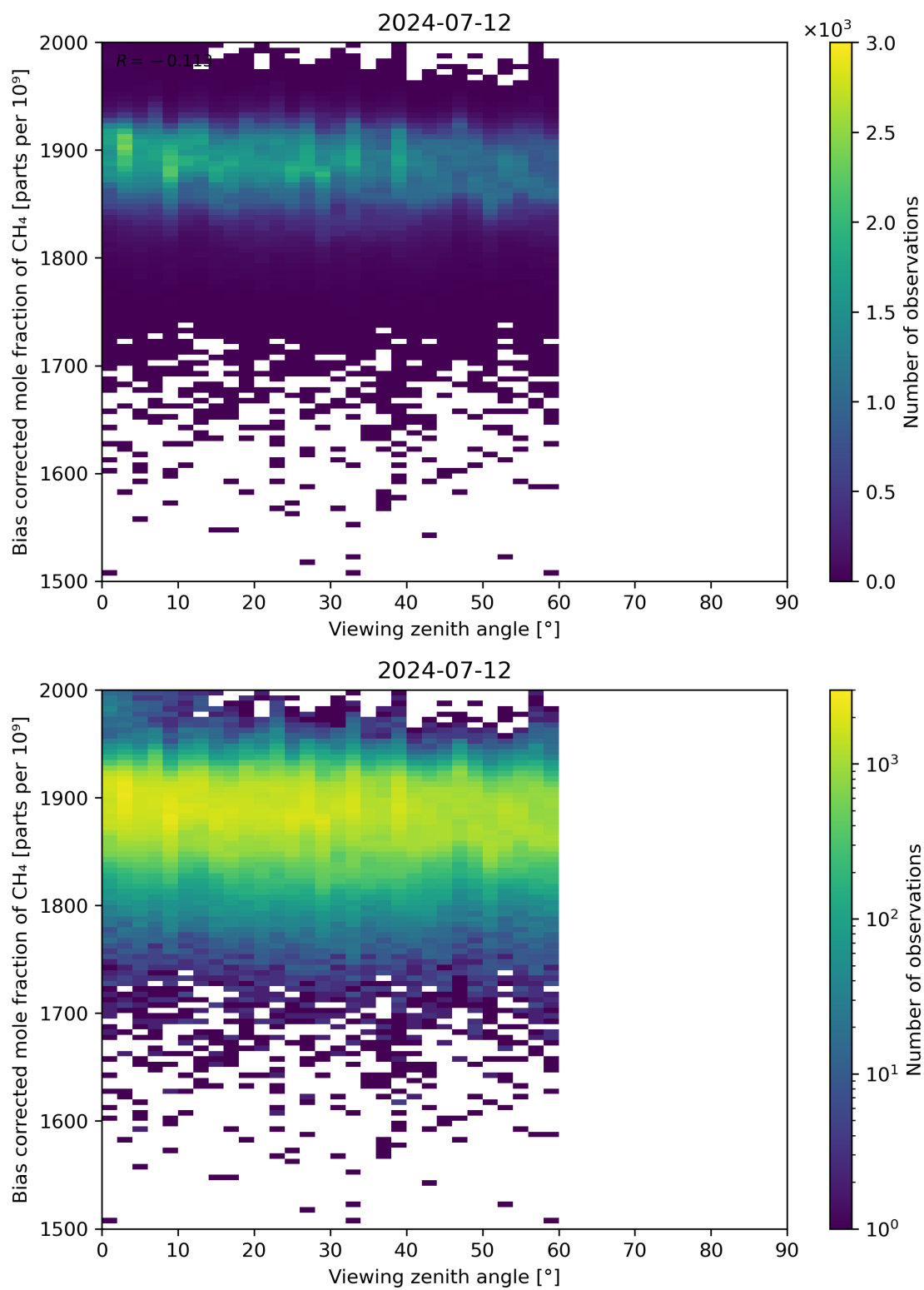
Figure 111: Scatter density plot of “Viewing zenith angle” against “Bias corrected mole fraction of CH 4 ” for 2024-07-11 to 2024-07-13.
