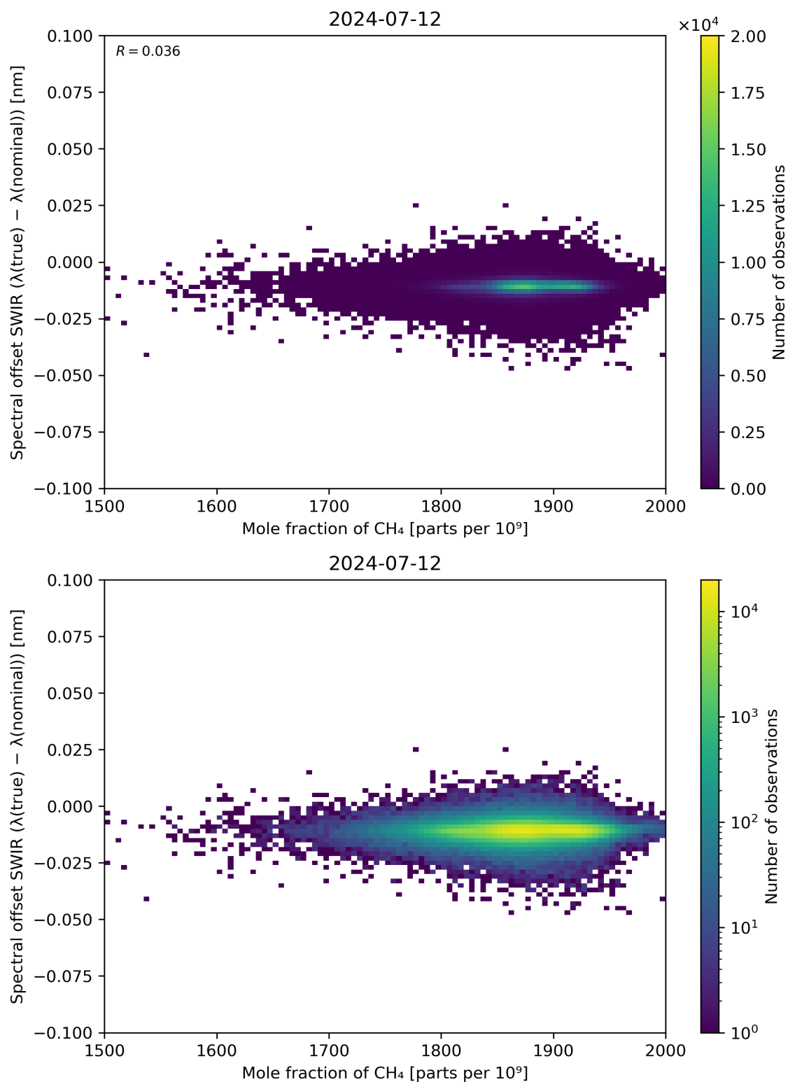
Figure 86: Scatter density plot of “Mole fraction of CH 4 ” against “Spectral offset SWIR ( \lambda(\text{true}) - \lambda(\text{nominal}) )” for 2024-07-11 to 2024-07-13.
