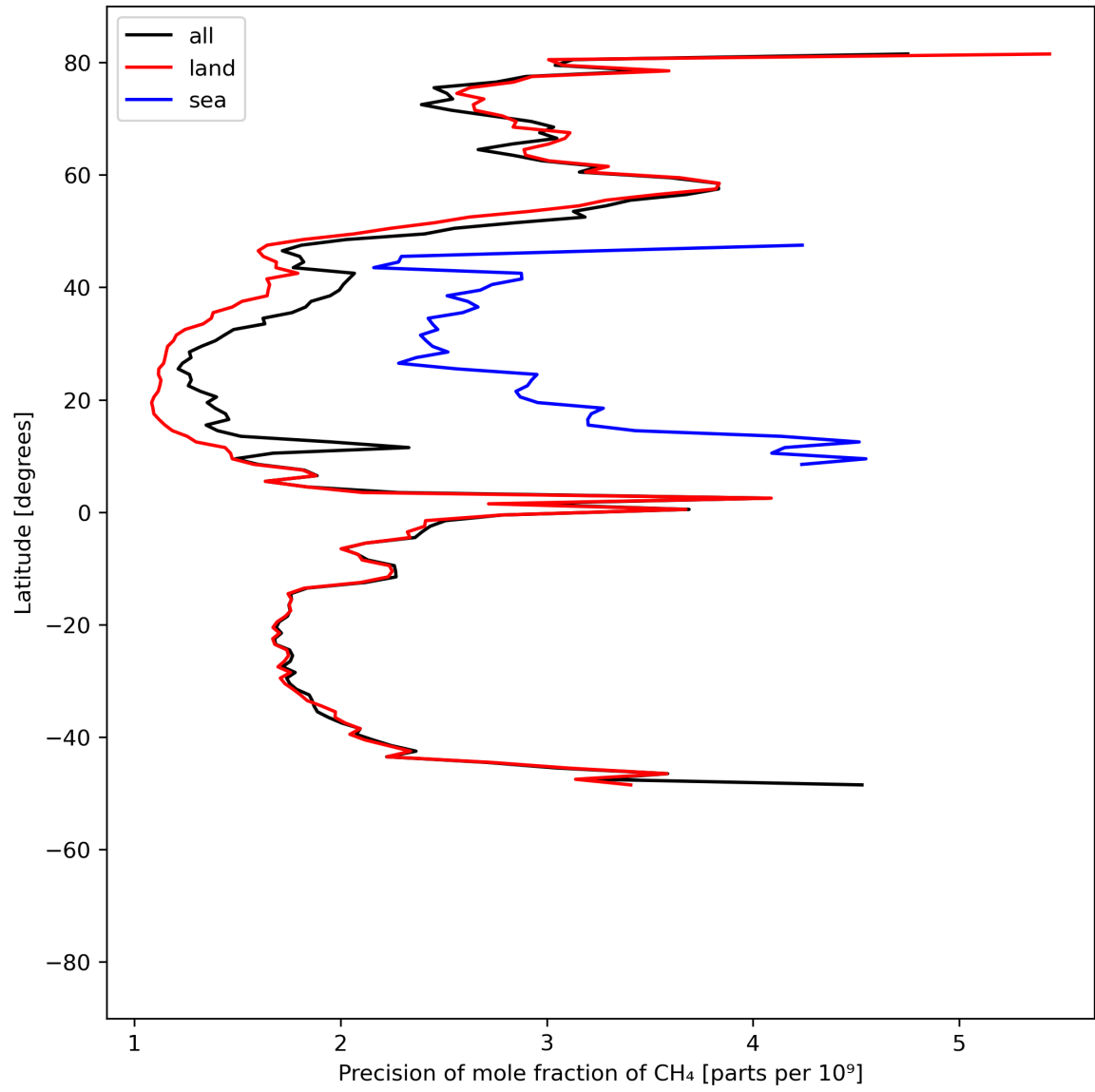
Figure 13: Zonal average of “Precision of mole fraction of CH 4 ” for 2024-07-11 to 2024-07-13.
