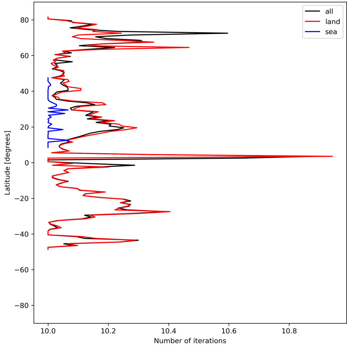
Figure 20: Zonal average of “Number of iterations” for 2024-07-11 to 2024-07-13.
