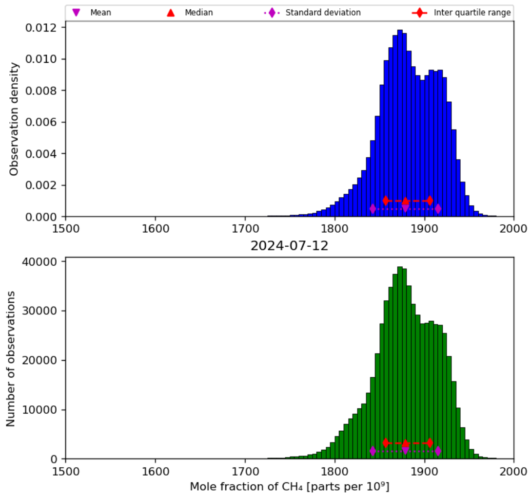
Figure 23: Histogram of “Mole fraction of CH 4 ” for 2024-07-11 to 2024-07-13
