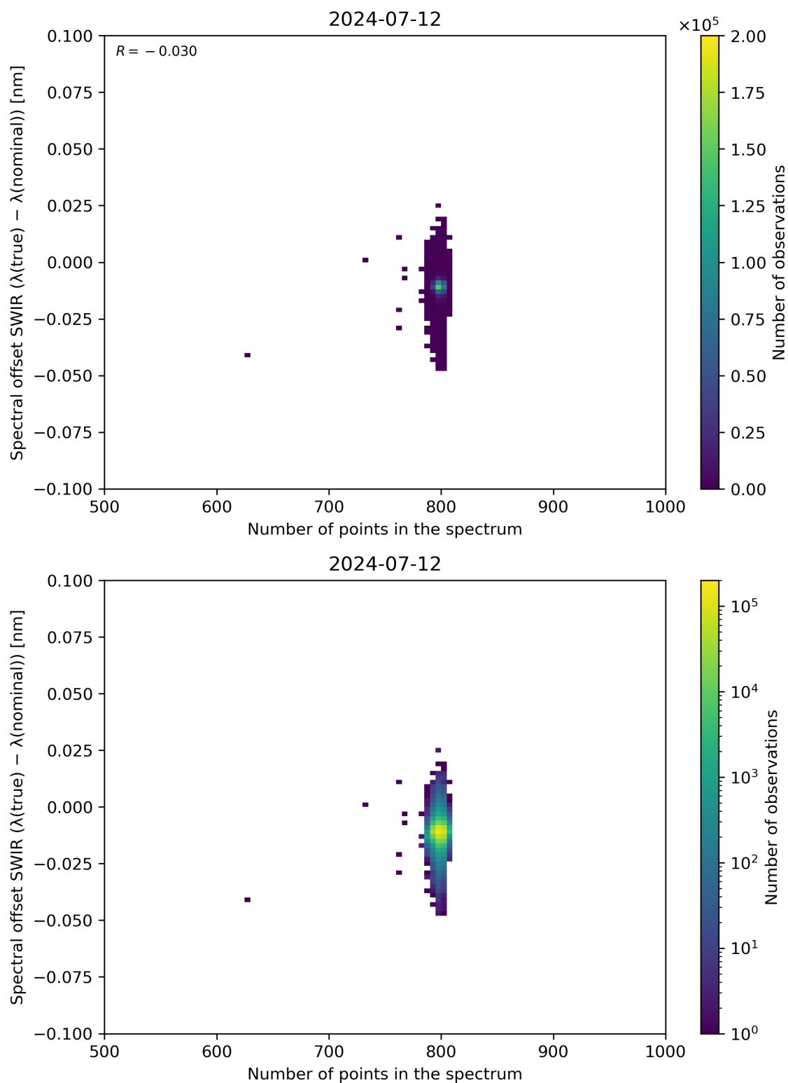
Figure 93: Scatter density plot of “Number of points in the spectrum” against “Spectral offset SWIR ( \lambda(\text{true}) - \lambda(\text{nominal}) )” for 2024-07-11 to 2024-07-13.
