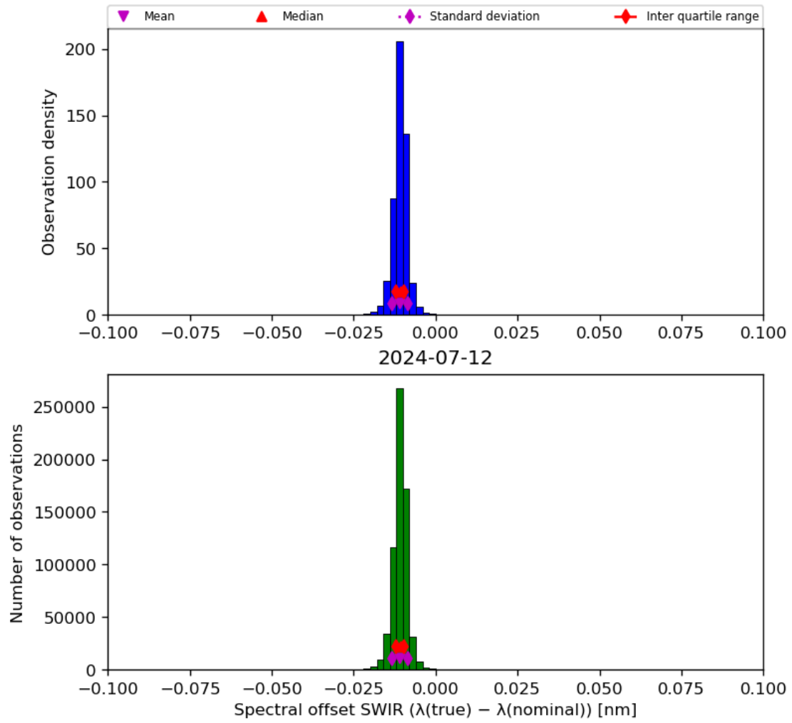
Figure 27: Histogram of “Spectral offset SWIR ( \lambda(\text{true}) - \lambda(\text{nominal}) )” for 2024-07-11 to 2024-07-13
