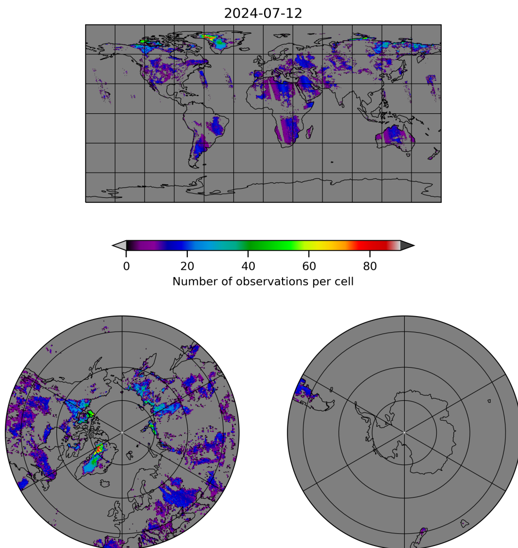
Figure 10: Map of the number of observations for 2024-07-11 to 2024-07-13
