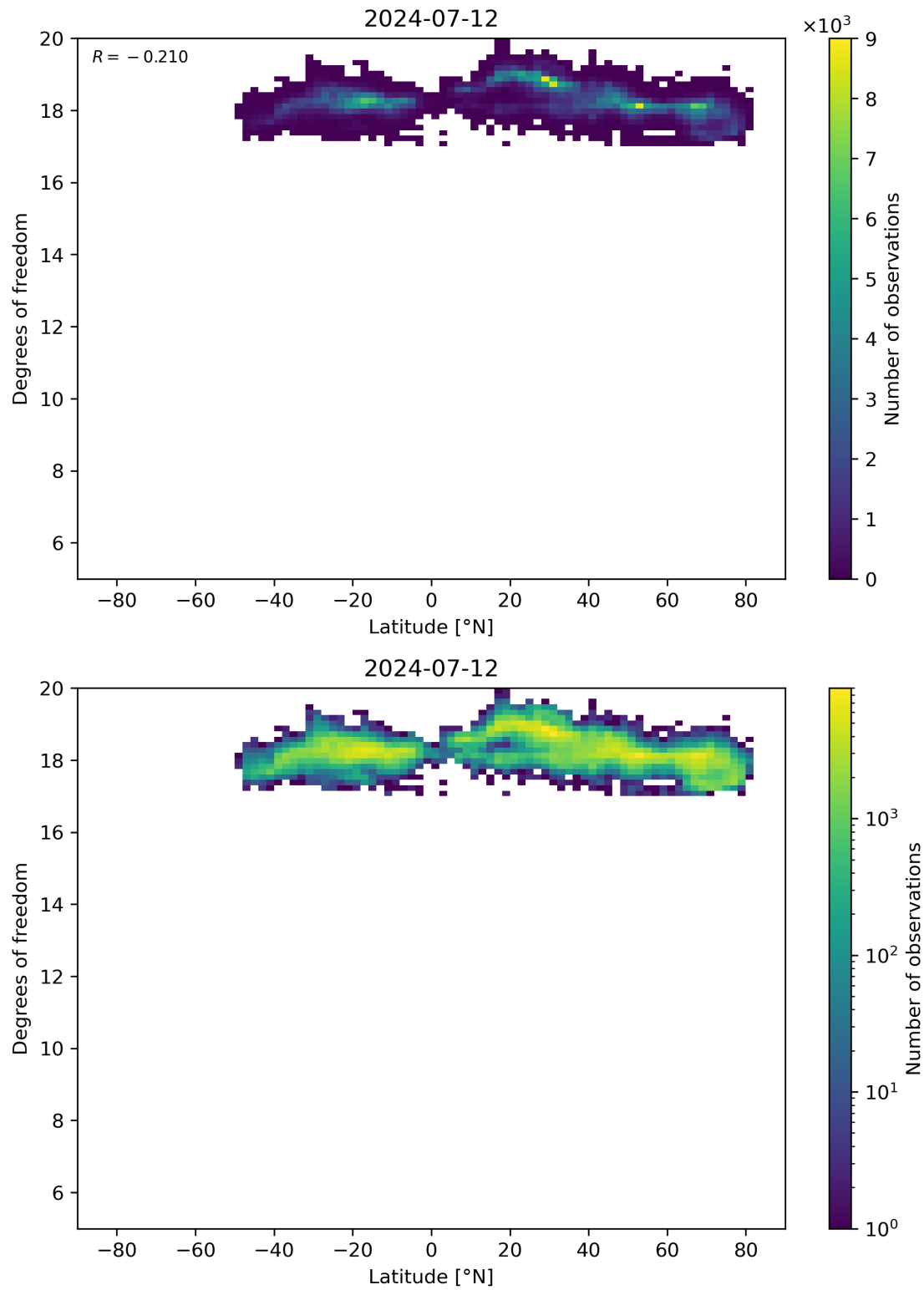
Figure 55: Scatter density plot of “Latitude” against “Degrees of freedom” for 2024-07-11 to 2024-07-13.
