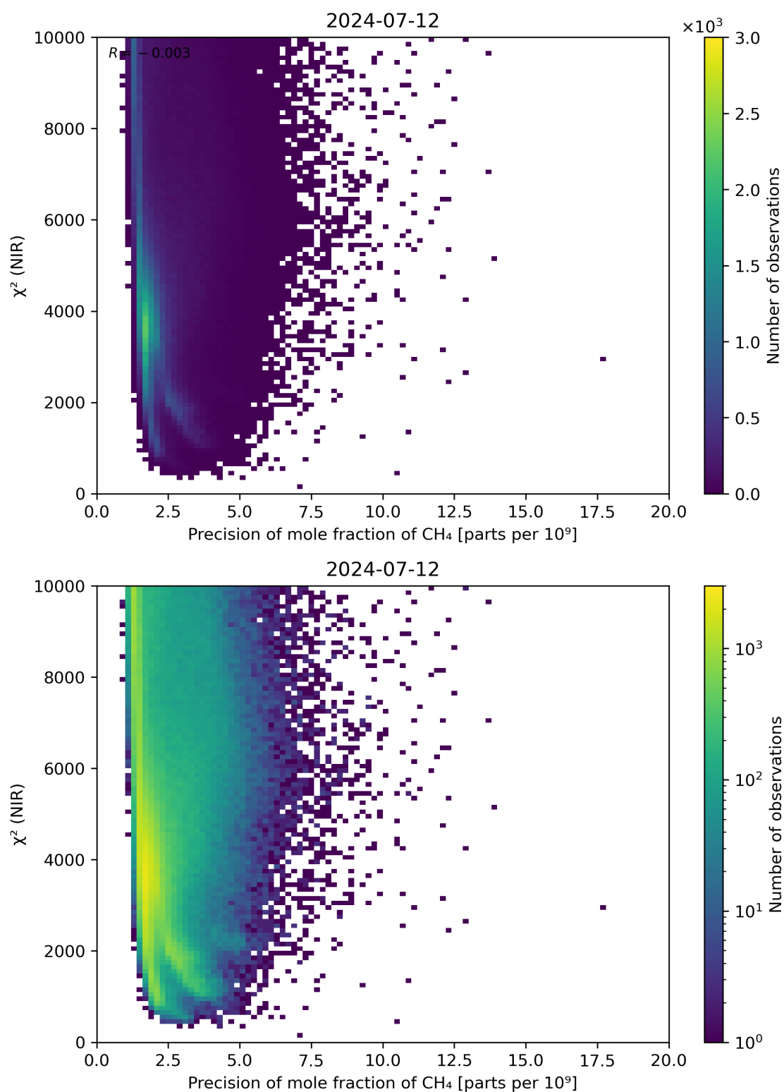
Figure 78: Scatter density plot of “Precision of mole fraction of \text{CH}_4 ” against “ \chi^2 (NIR)” for 2024-07-11 to 2024-07-13.
