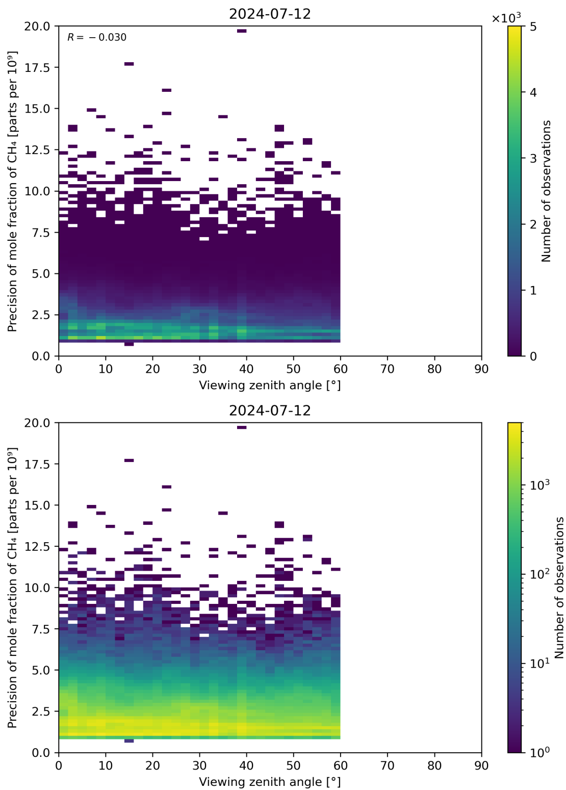
Figure 112: Scatter density plot of “Viewing zenith angle” against “Precision of mole fraction of \text{CH}_4 ” for 2024-07-11 to 2024-07-13.
