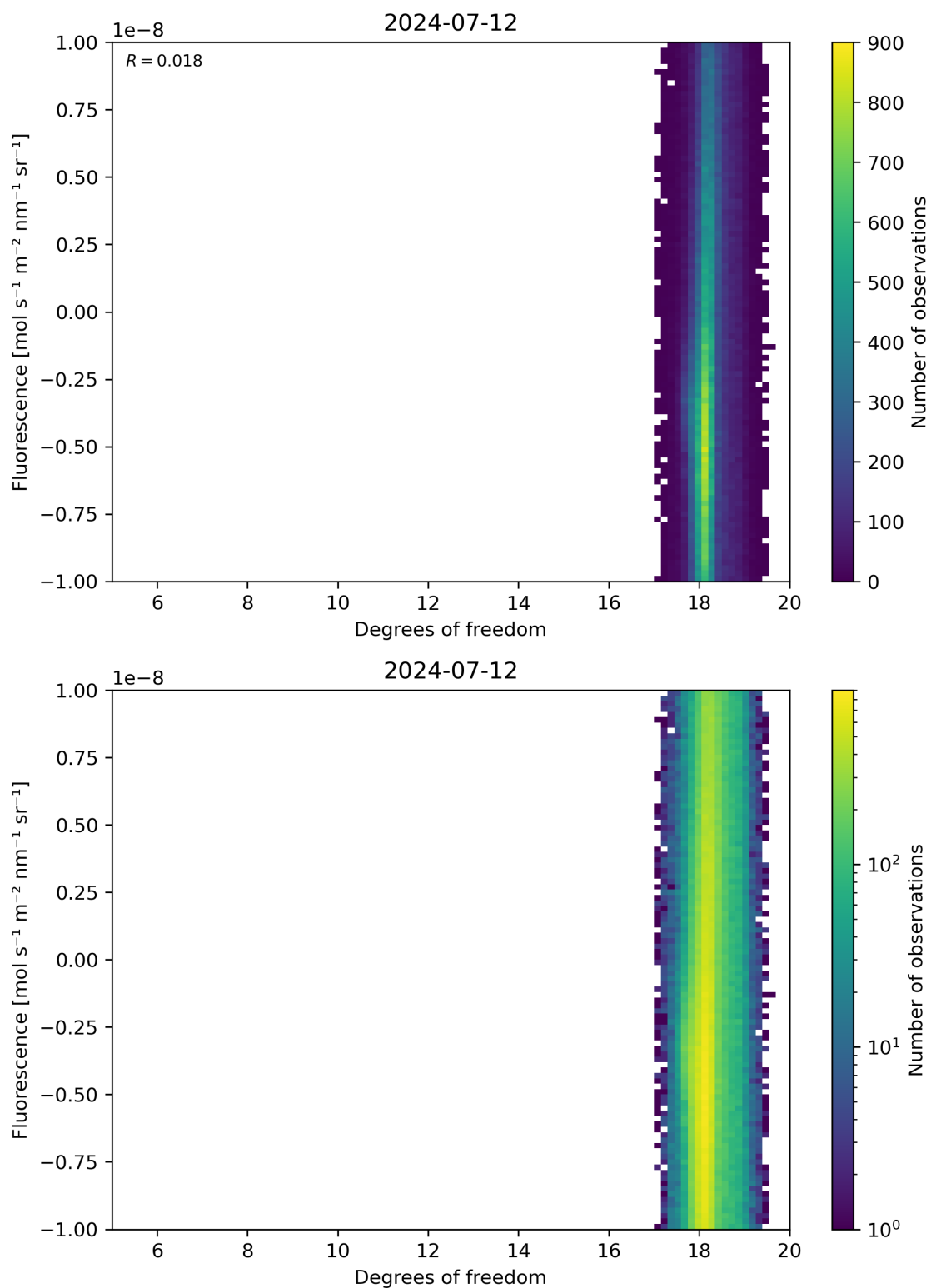
Figure 51: Scatter density plot of “Degrees of freedom” against “Fluorescence” for 2024-07-11 to 2024-07-13.
