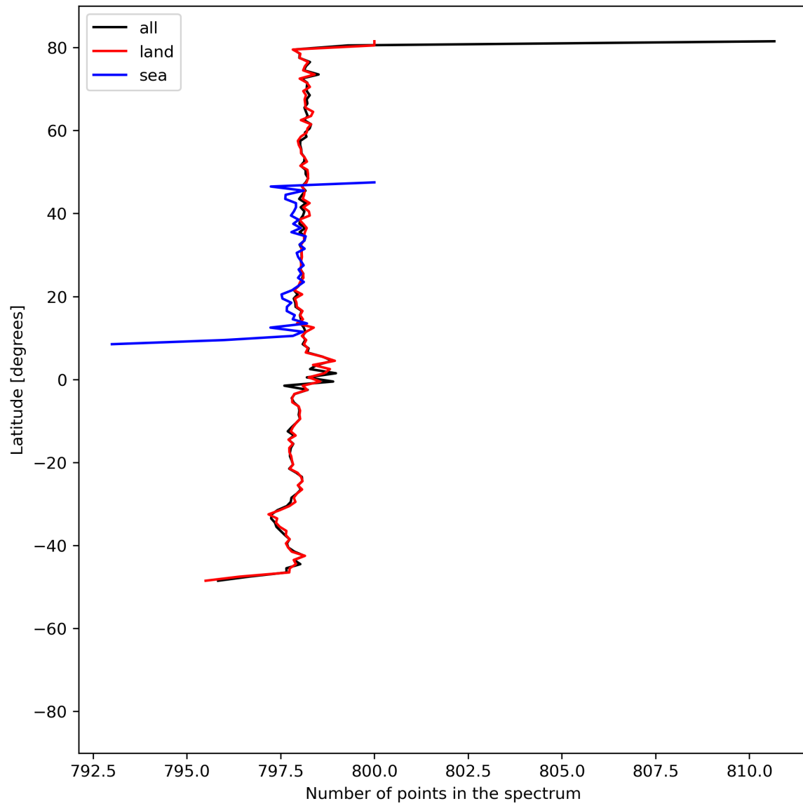
Figure 15: Zonal average of “Number of points in the spectrum” for 2024-07-11 to 2024-07-13.
