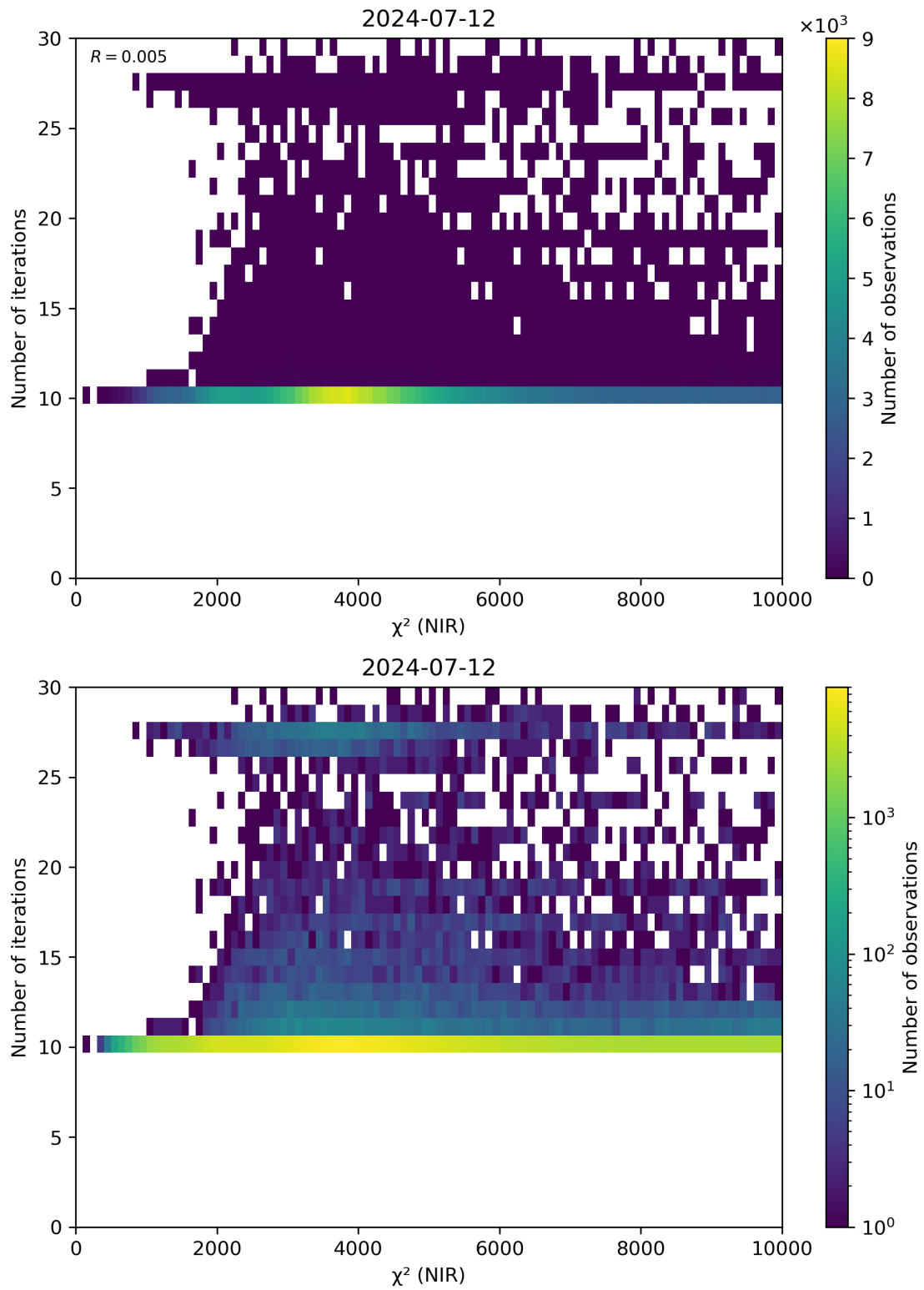
Figure 46: Scatter density plot of “ \chi^2 (NIR)” against “Number of iterations” for 2024-07-11 to 2024-07-13.
