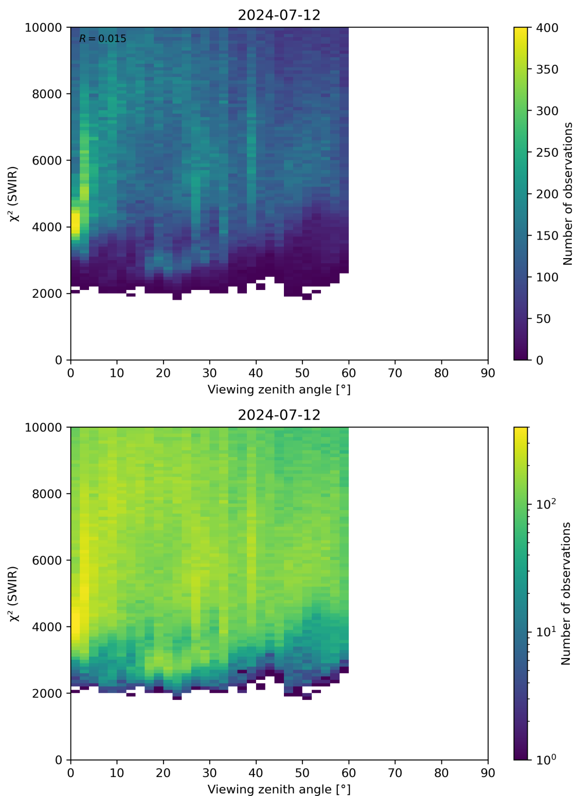
Figure 106: Scatter density plot of “Viewing zenith angle” against “ \chi^2 (SWIR)” for 2024-07-11 to 2024-07-13.
