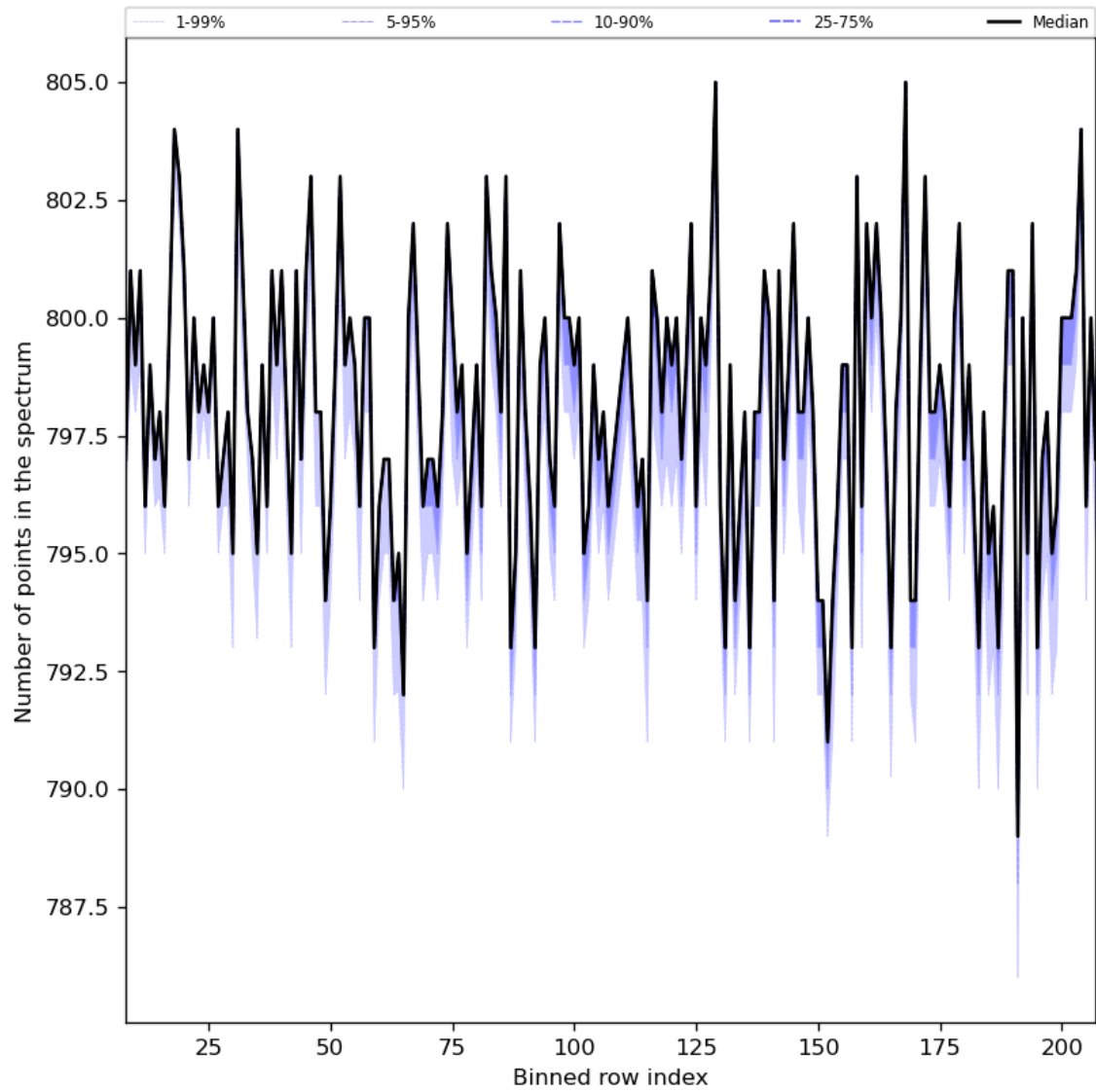
Figure 37: Along track statistics of “Number of points in the spectrum” for 2024-07-11 to 2024-07-13
