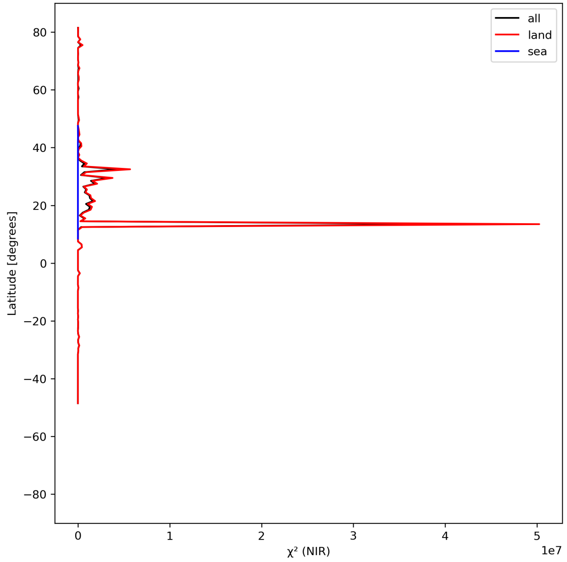
Figure 18: Zonal average of “ \chi^2 (NIR)” for 2024-07-11 to 2024-07-13.
