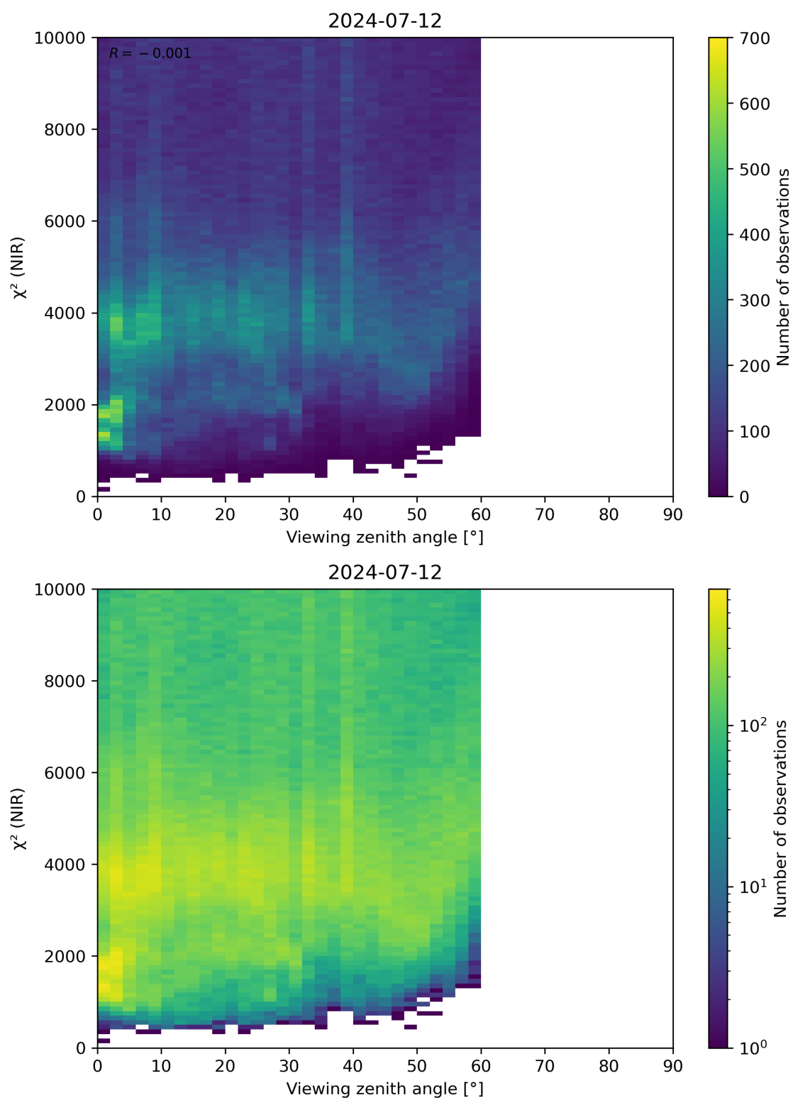
Figure 105: Scatter density plot of “Viewing zenith angle” against “ \chi^2 (NIR)” for 2024-07-11 to 2024-07-13.
