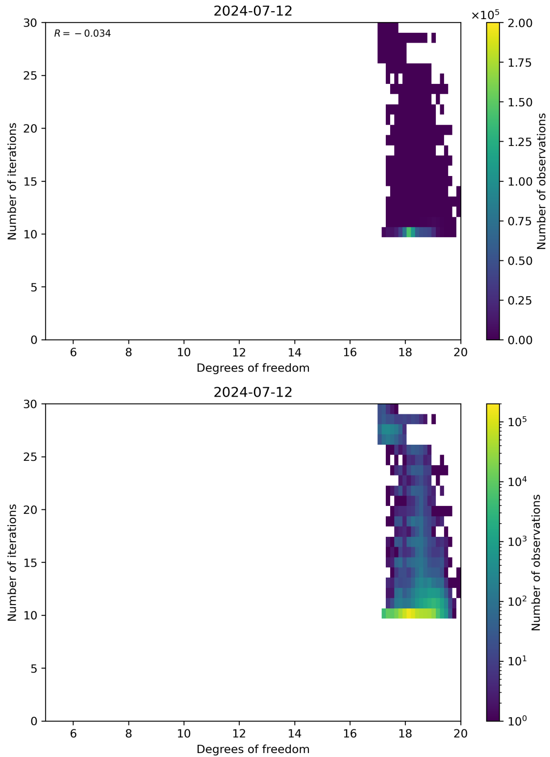
Figure 52: Scatter density plot of “Degrees of freedom” against “Number of iterations” for 2024-07-11 to 2024-07-13.
