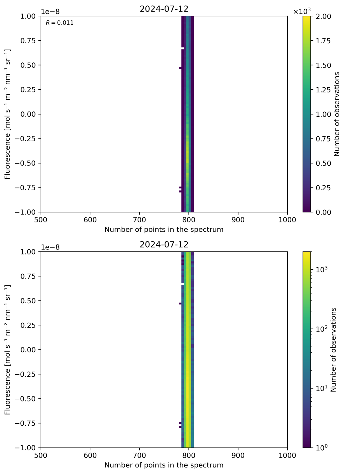
Figure 91: Scatter density plot of “Number of points in the spectrum” against “Fluorescence” for 2024-07-11 to 2024-07-13.
