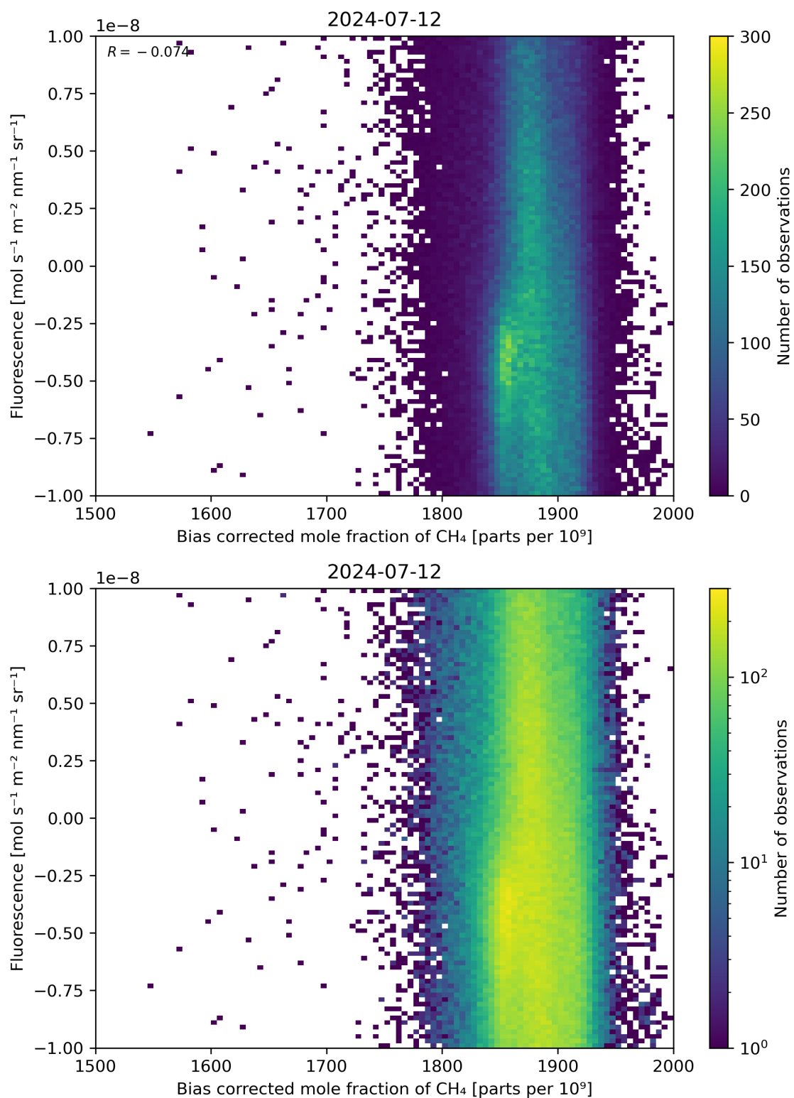
Figure 66: Scatter density plot of “Bias corrected mole fraction of \text{CH}_4 ” against “Fluorescence” for 2024-07-11 to 2024-07-13.
