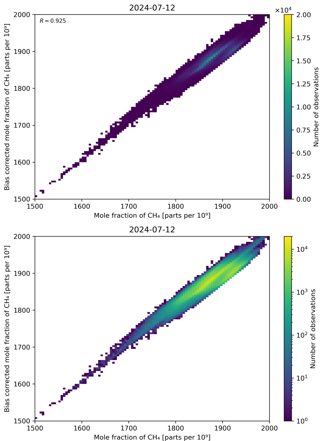
Figure 74: Scatter density plot of “Mole fraction of CH 4 ” against “Bias corrected mole fraction of CH 4 ” for 2024-07-11 to 2024-07-13.
