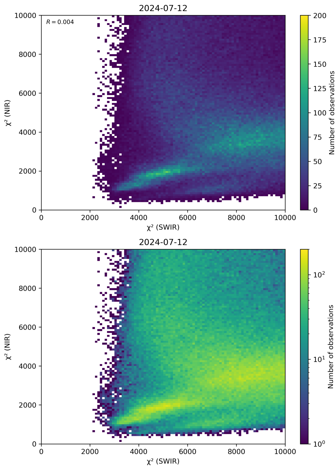
Figure 47: Scatter density plot of “ \chi^2 (SWIR)” against “ \chi^2 (NIR)” for 2024-07-11 to 2024-07-13.
