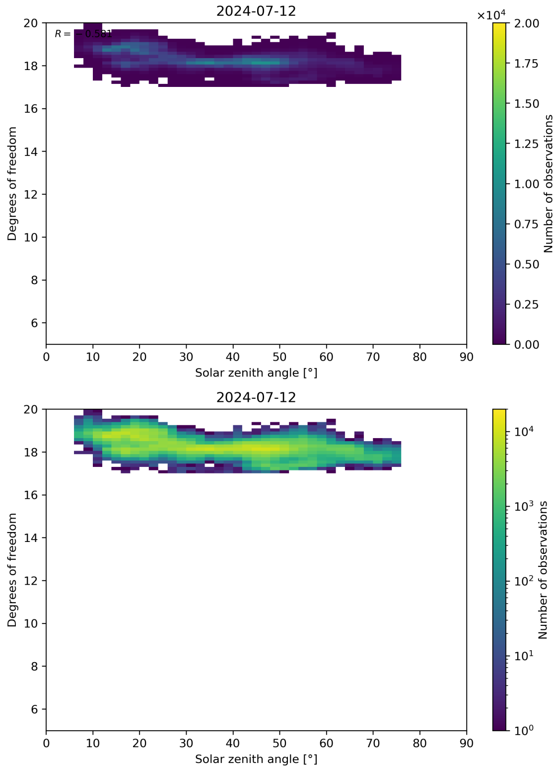
Figure 96: Scatter density plot of “Solar zenith angle” against “Degrees of freedom” for 2024-07-11 to 2024-07-13.
