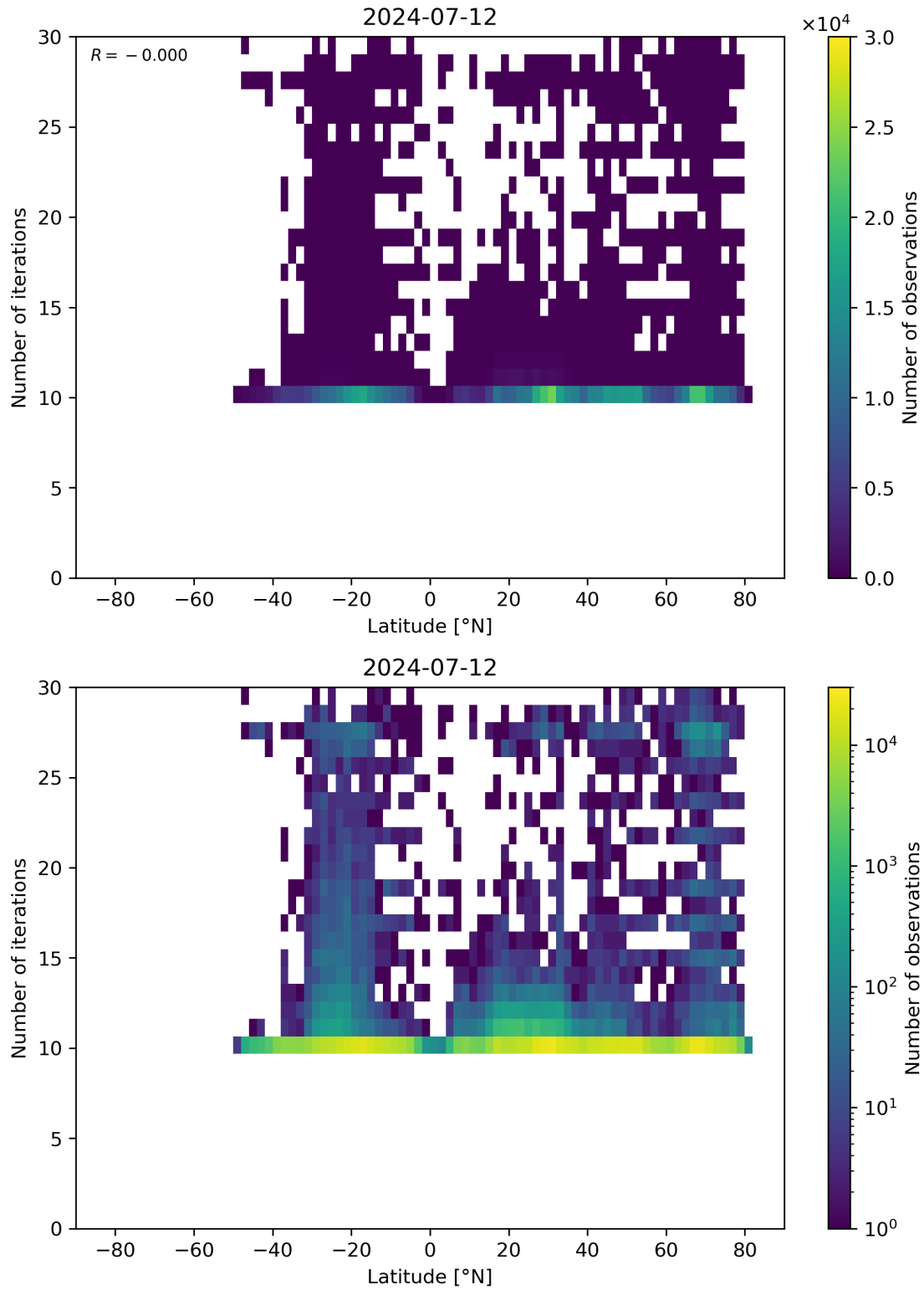
Figure 60: Scatter density plot of “Latitude” against “Number of iterations” for 2024-07-11 to 2024-07-13.
