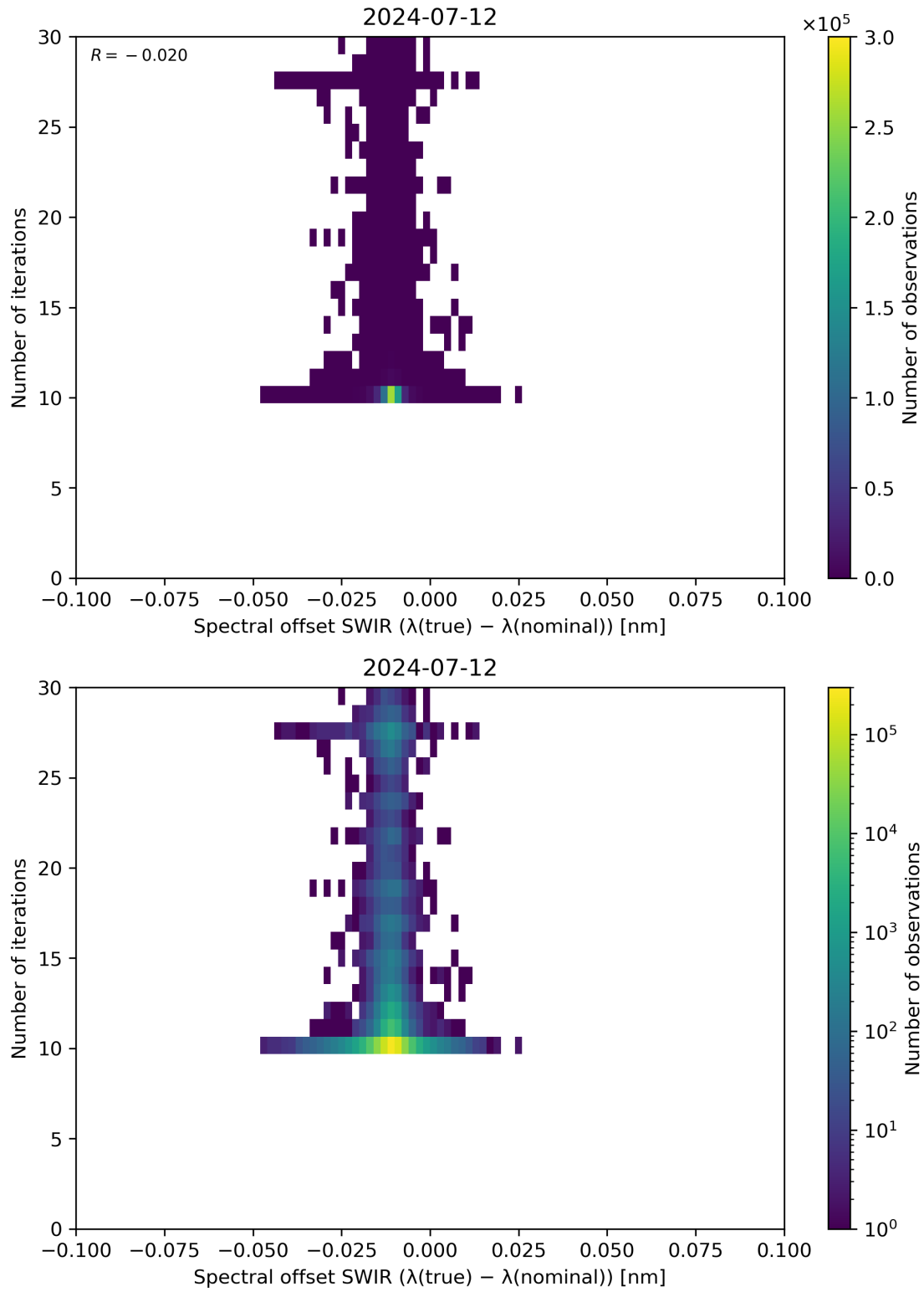
Figure 121: Scatter density plot of “Spectral offset SWIR ( \lambda(\text{true}) - \lambda(\text{nominal}) )” against “Number of iterations” for 2024-07-11 to 2024-07-13.
