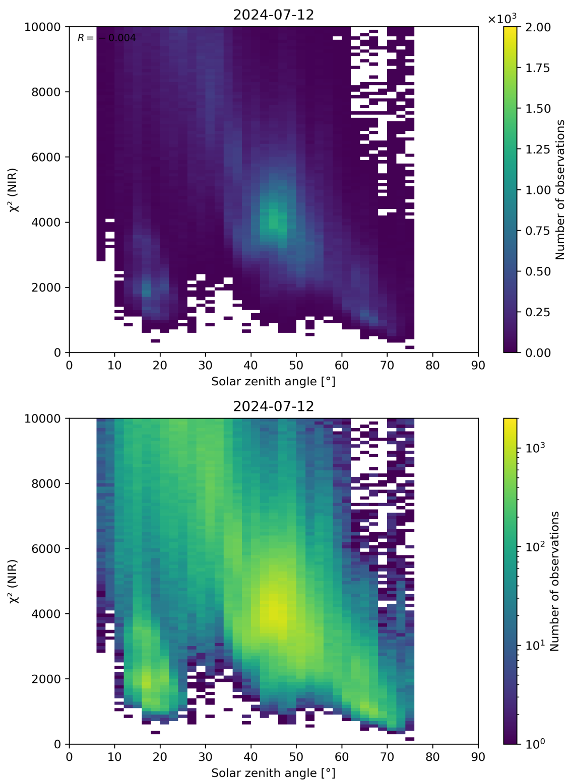
Figure 94: Scatter density plot of “Solar zenith angle” against “ \chi^2 (NIR)” for 2024-07-11 to 2024-07-13.
