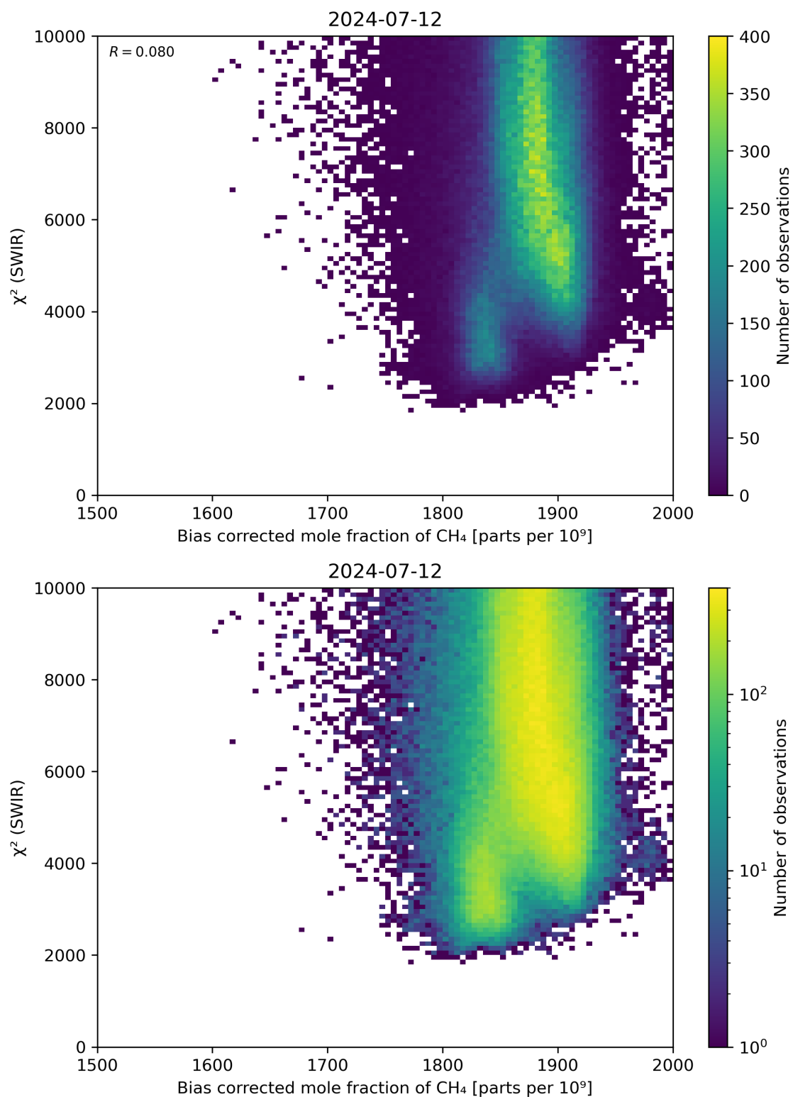
Figure 64: Scatter density plot of “Bias corrected mole fraction of CH 4 ” against “ \chi^2 (SWIR)” for 2024-07-11 to 2024-07-13.
