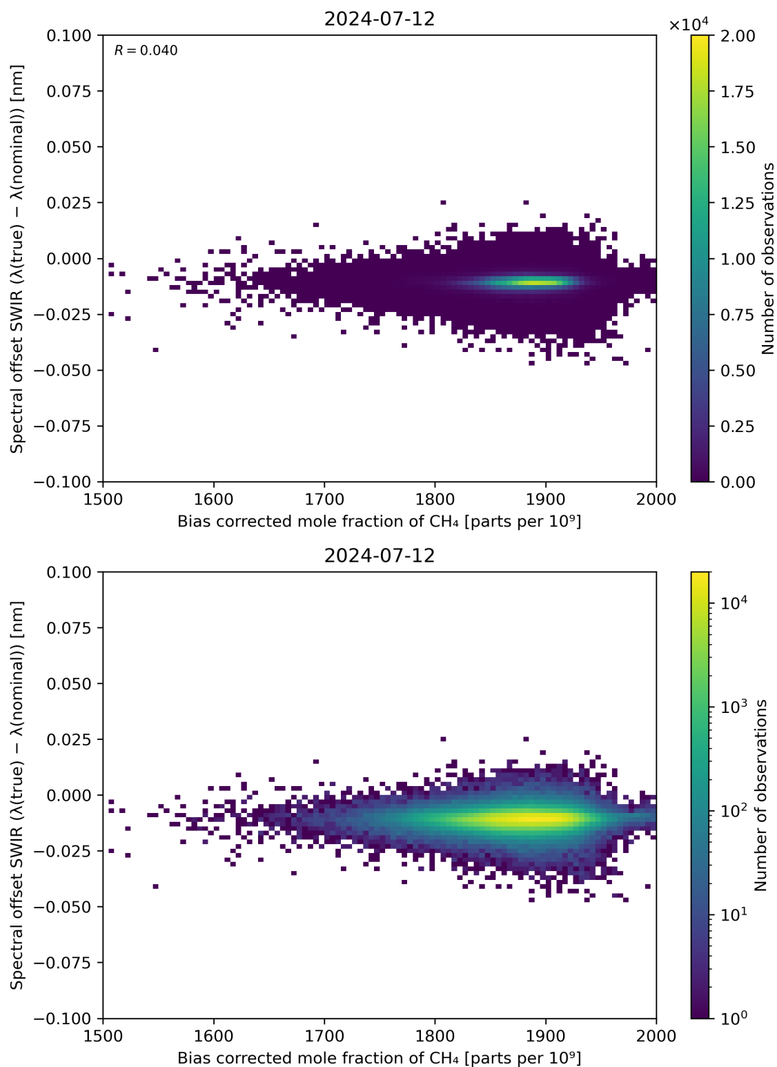
Figure 69: Scatter density plot of “Bias corrected mole fraction of \text{CH}_4 ” against “Spectral offset SWIR ( \lambda(\text{true}) - \lambda(\text{nominal}) )” for 2024-07-11 to 2024-07-13.
