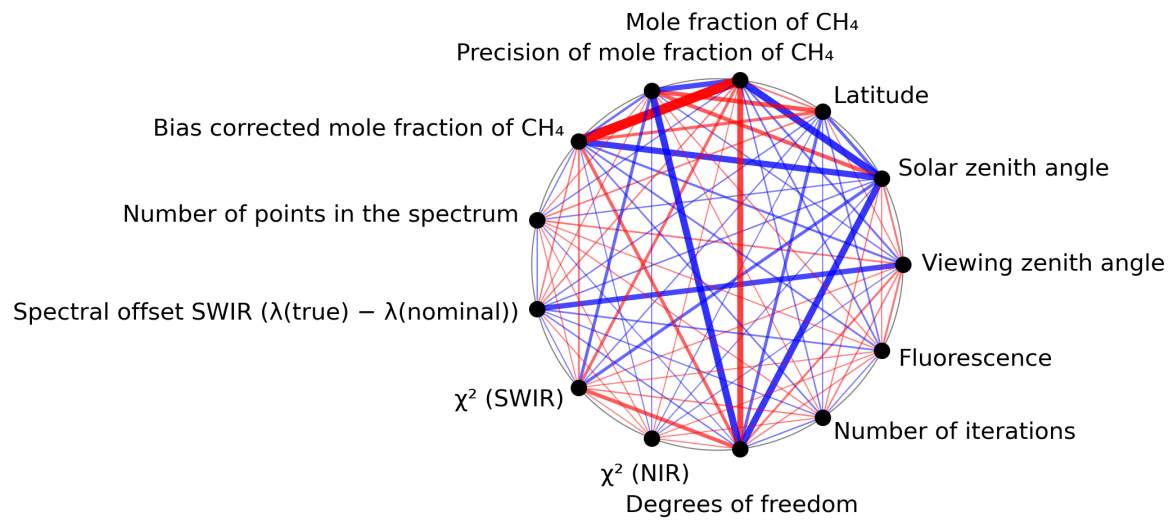
Figure 1: Map of correlation graph for 2024-07-11 to 2024-07-13.
