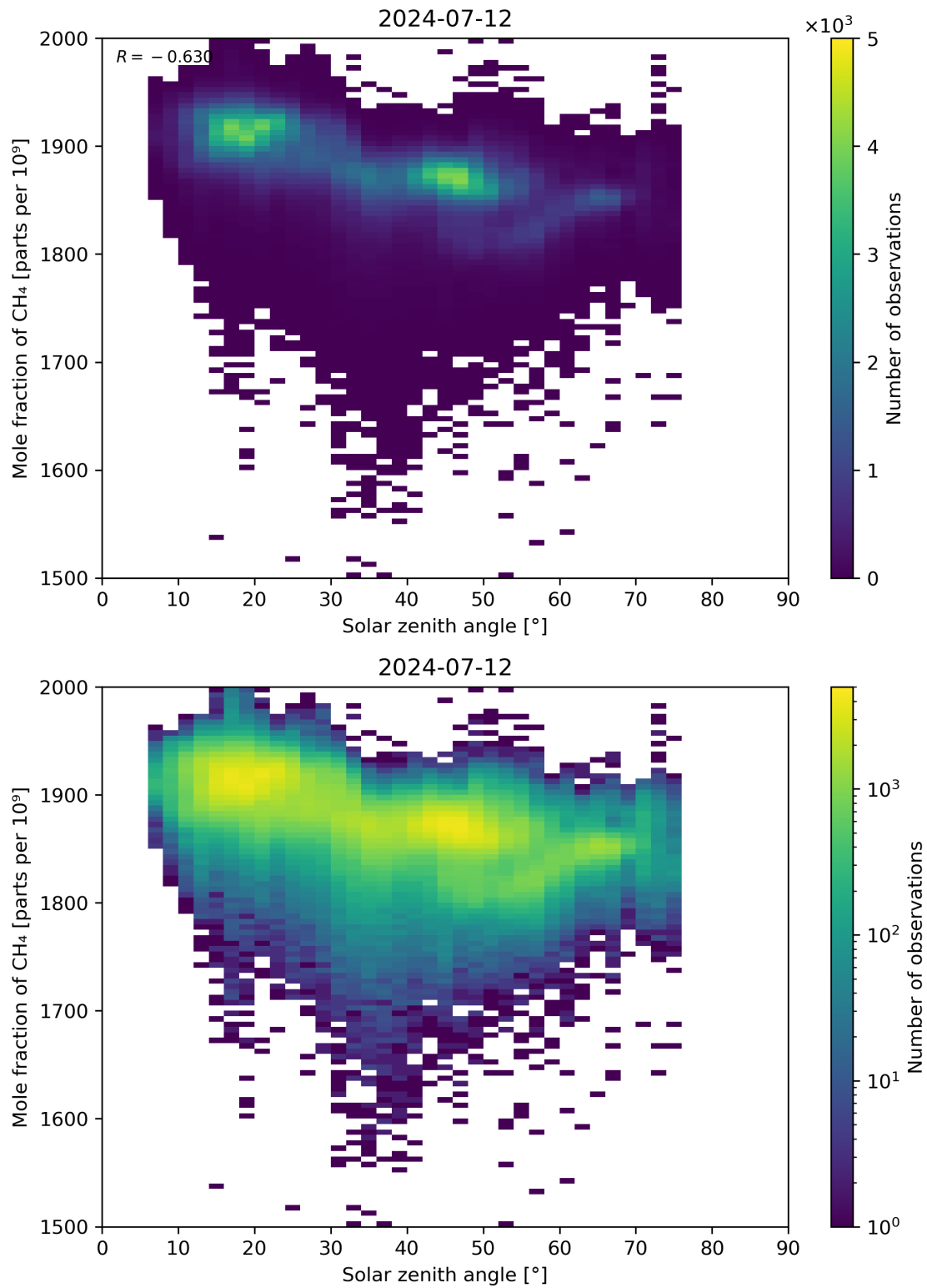
Figure 99: Scatter density plot of “Solar zenith angle” against “Mole fraction of CH 4 ” for 2024-07-11 to 2024-07-13.
