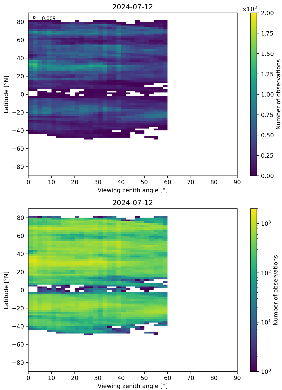
Figure 109: Scatter density plot of “Viewing zenith angle” against “Latitude” for 2024-07-11 to 2024-07-13.
