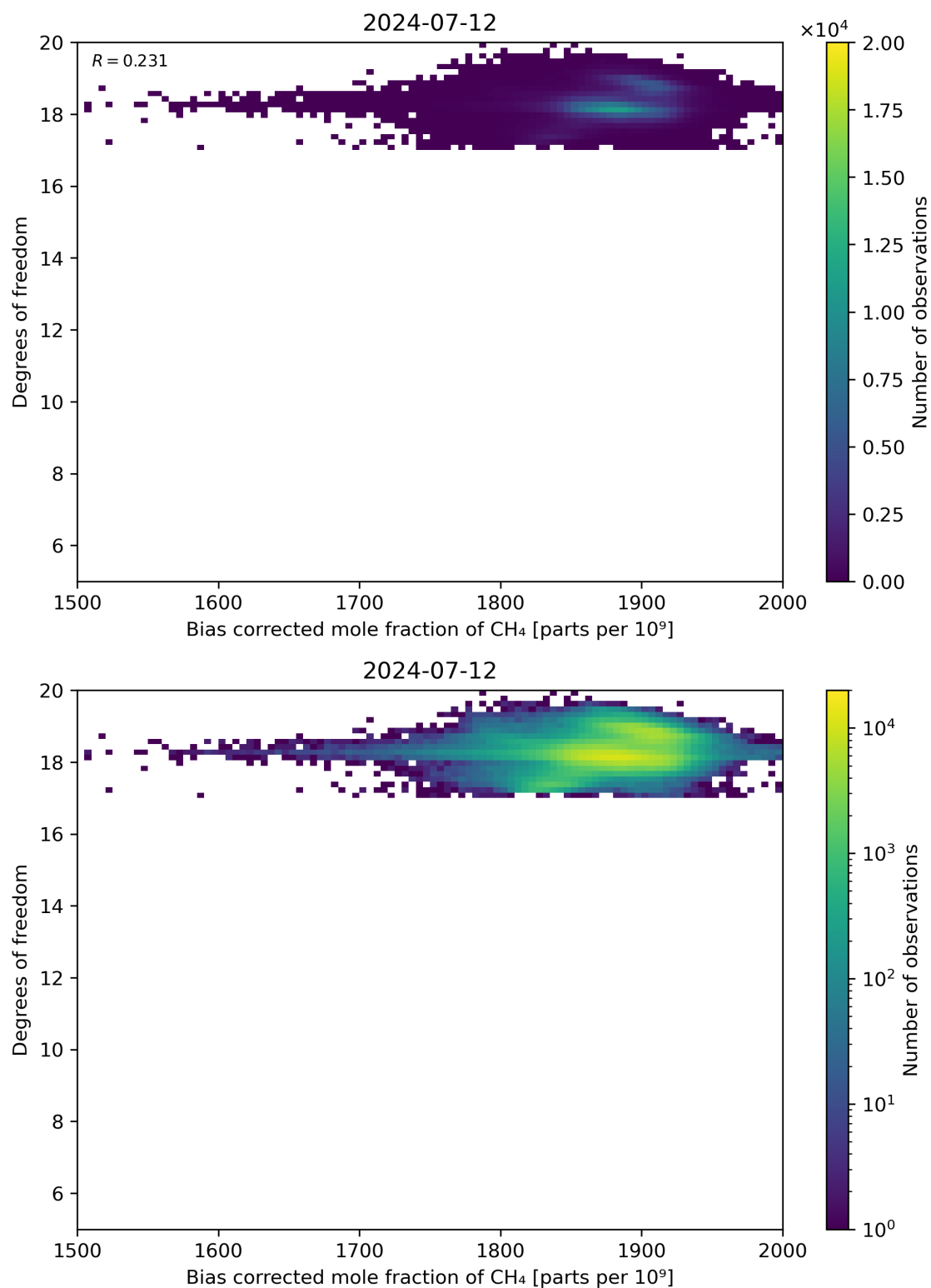
Figure 65: Scatter density plot of “Bias corrected mole fraction of CH 4 ” against “Degrees of freedom” for 2024-07-11 to 2024-07-13.
