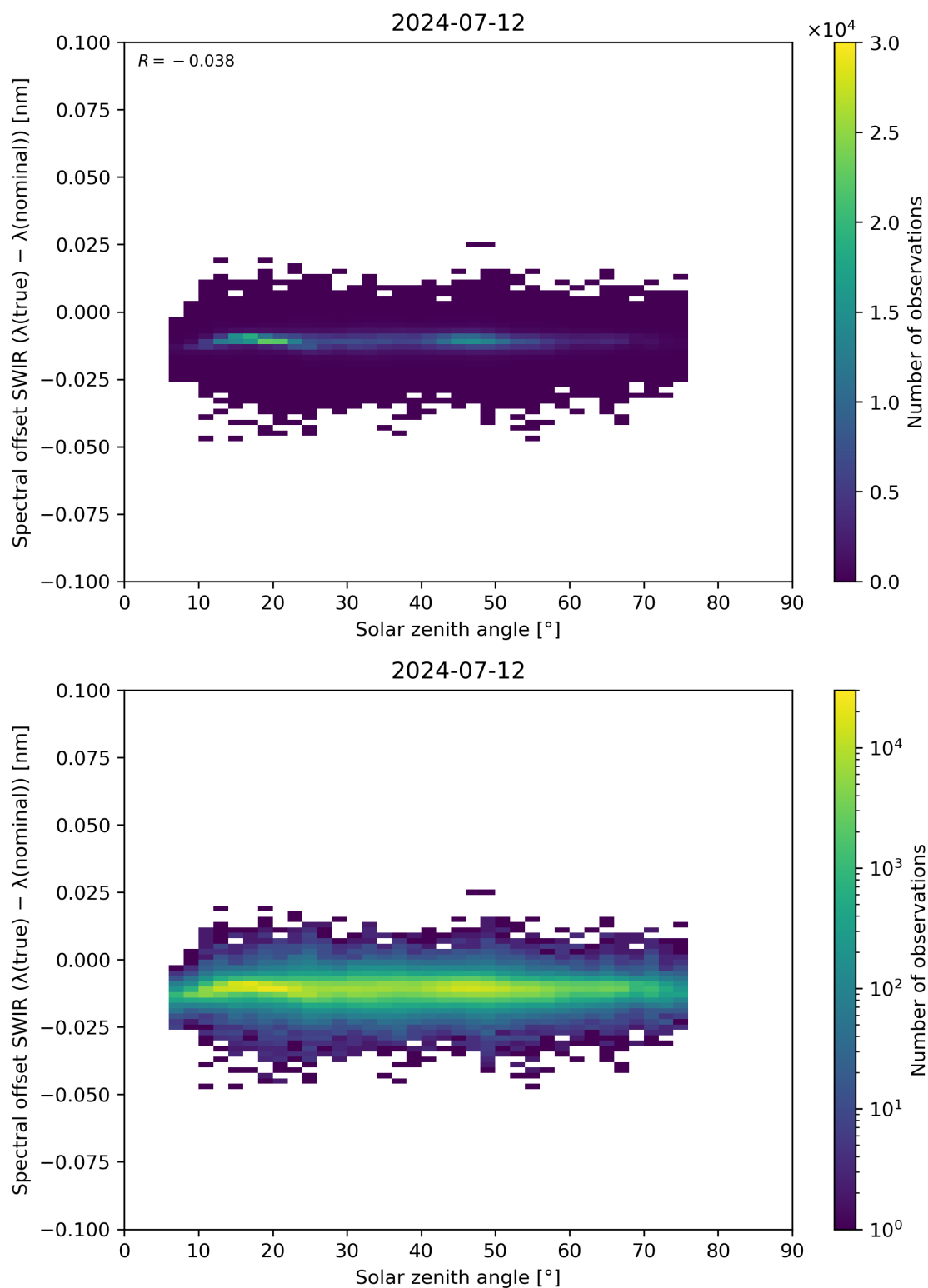
Figure 104: Scatter density plot of “Solar zenith angle” against “Spectral offset SWIR ( \lambda(\text{true}) - \lambda(\text{nominal}) )” for 2024-07-11 to 2024-07-13.
