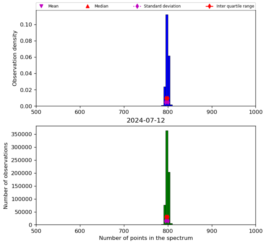
Figure 26: Histogram of “Number of points in the spectrum” for 2024-07-11 to 2024-07-13
