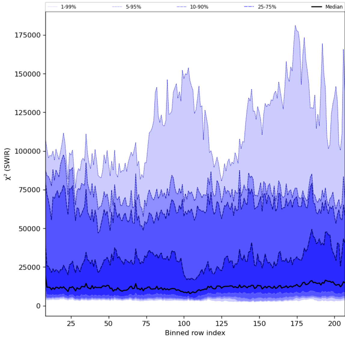
Figure 39: Along track statistics of “ \chi^2 (SWIR)” for 2024-07-11 to 2024-07-13
