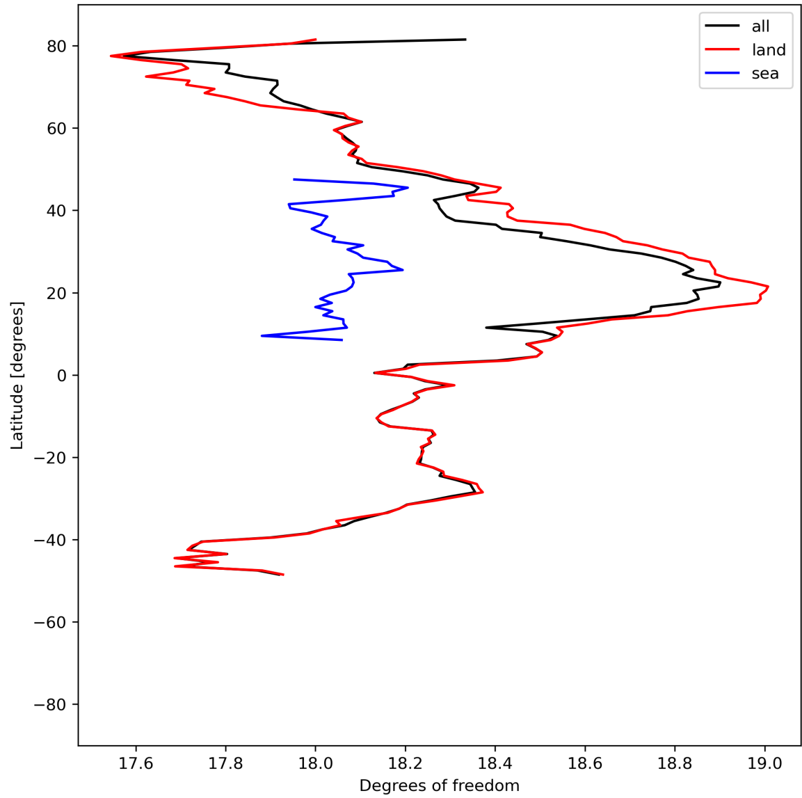
Figure 19: Zonal average of “Degrees of freedom” for 2024-07-11 to 2024-07-13.
