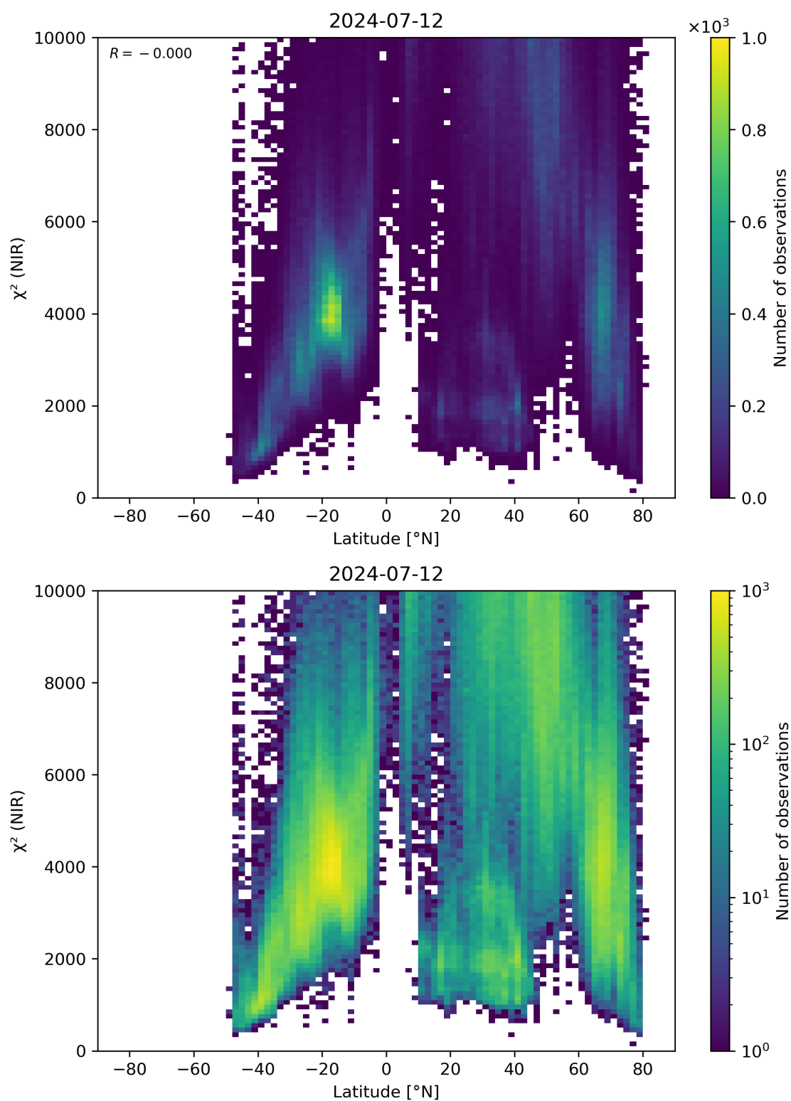
Figure 53: Scatter density plot of “Latitude” against “ \chi^2 (NIR)” for 2024-07-11 to 2024-07-13.
