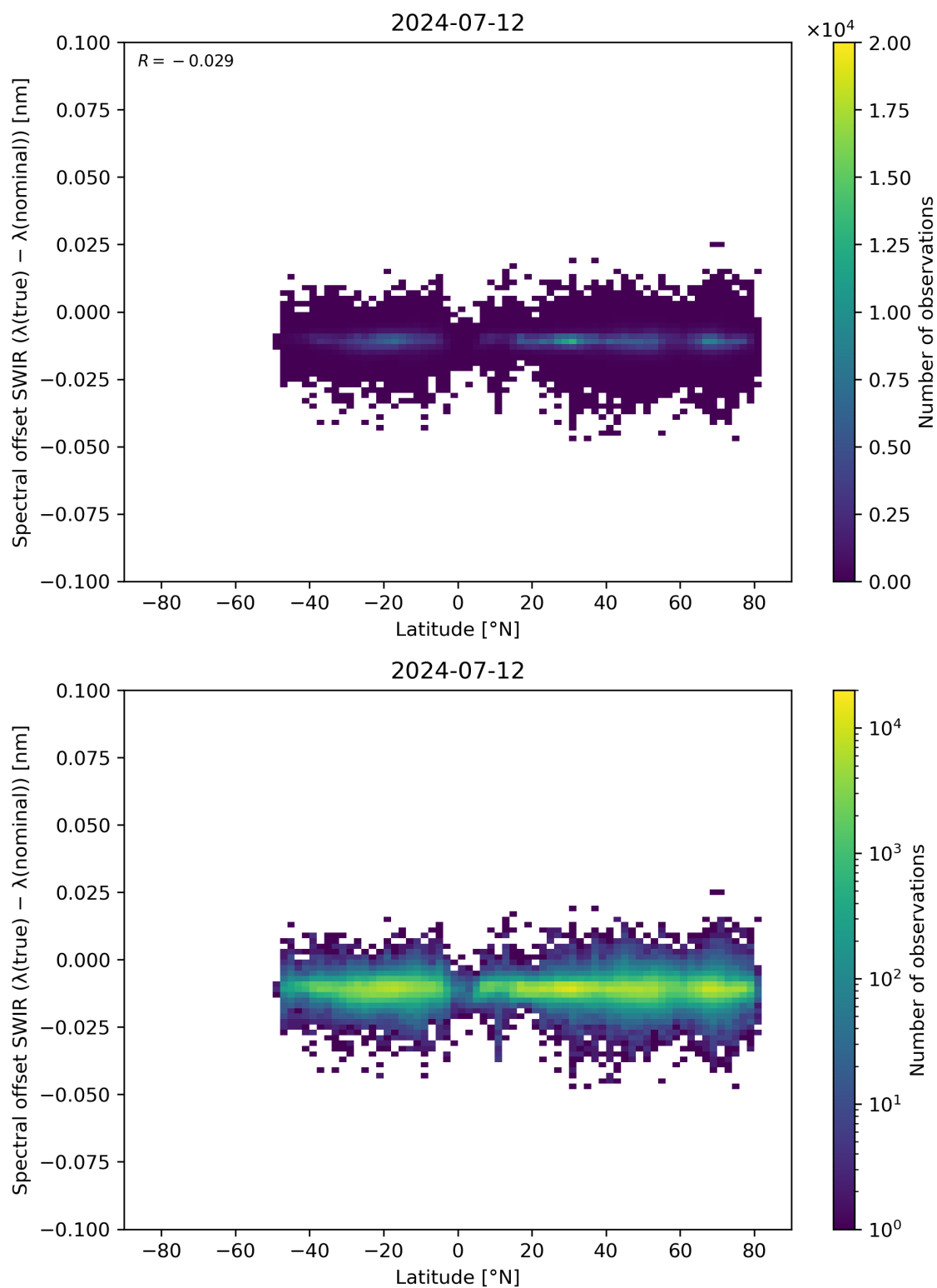
Figure 62: Scatter density plot of “Latitude” against “Spectral offset SWIR ( \lambda(\text{true}) - \lambda(\text{nominal}) )” for 2024-07-11 to 2024-07-13.
