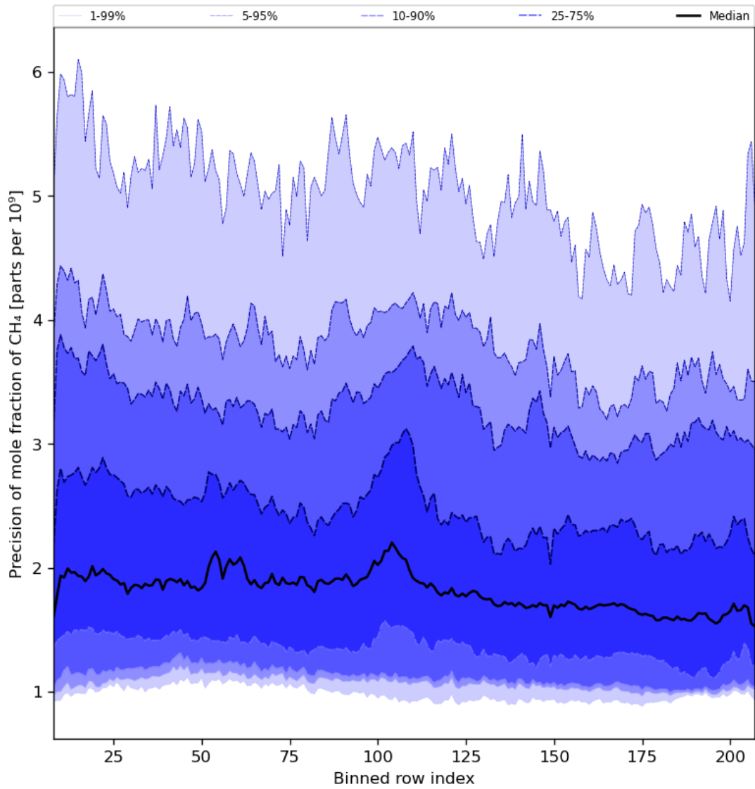
Figure 35: Along track statistics of “Precision of mole fraction of CH 4 ” for 2024-07-11 to 2024-07-13
