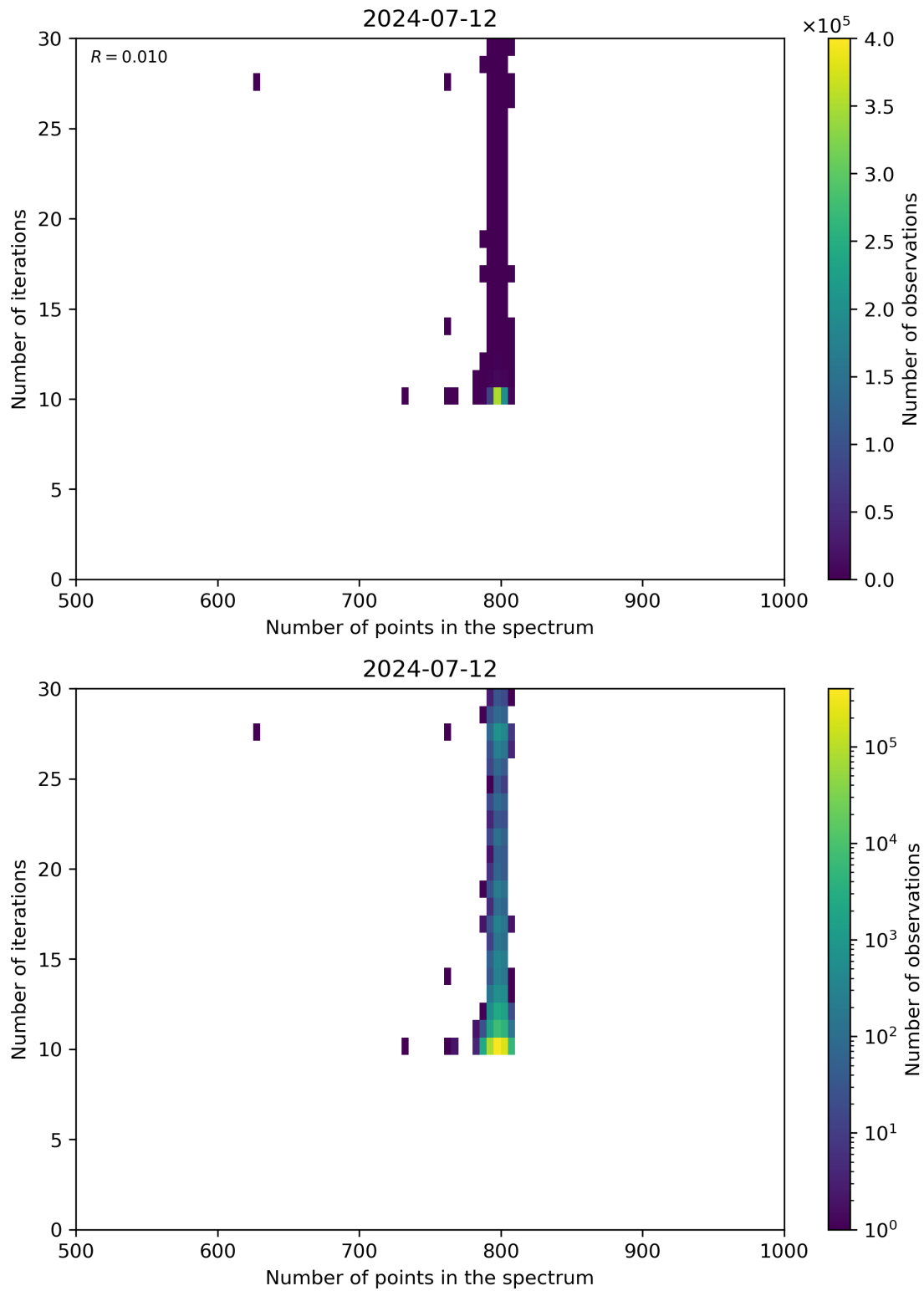
Figure 92: Scatter density plot of “Number of points in the spectrum” against “Number of iterations” for 2024-07-11 to 2024-07-13.
