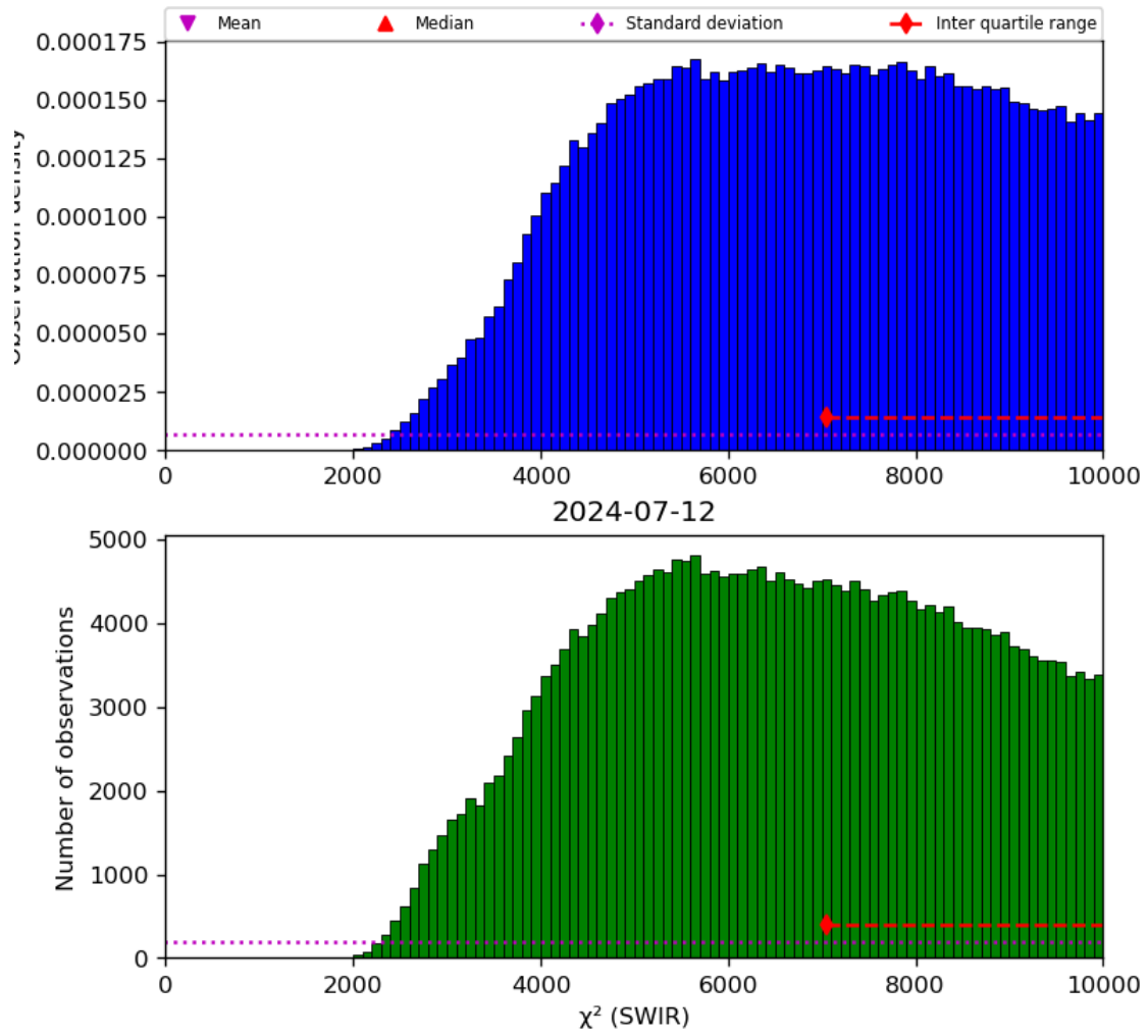
Figure 28: Histogram of “ \chi^2 (SWIR)” for 2024-07-11 to 2024-07-13
