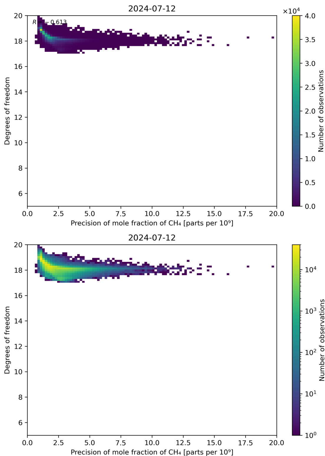
Figure 80: Scatter density plot of “Precision of mole fraction of CH 4 ” against “Degrees of freedom” for 2024-07-11 to 2024-07-13.
