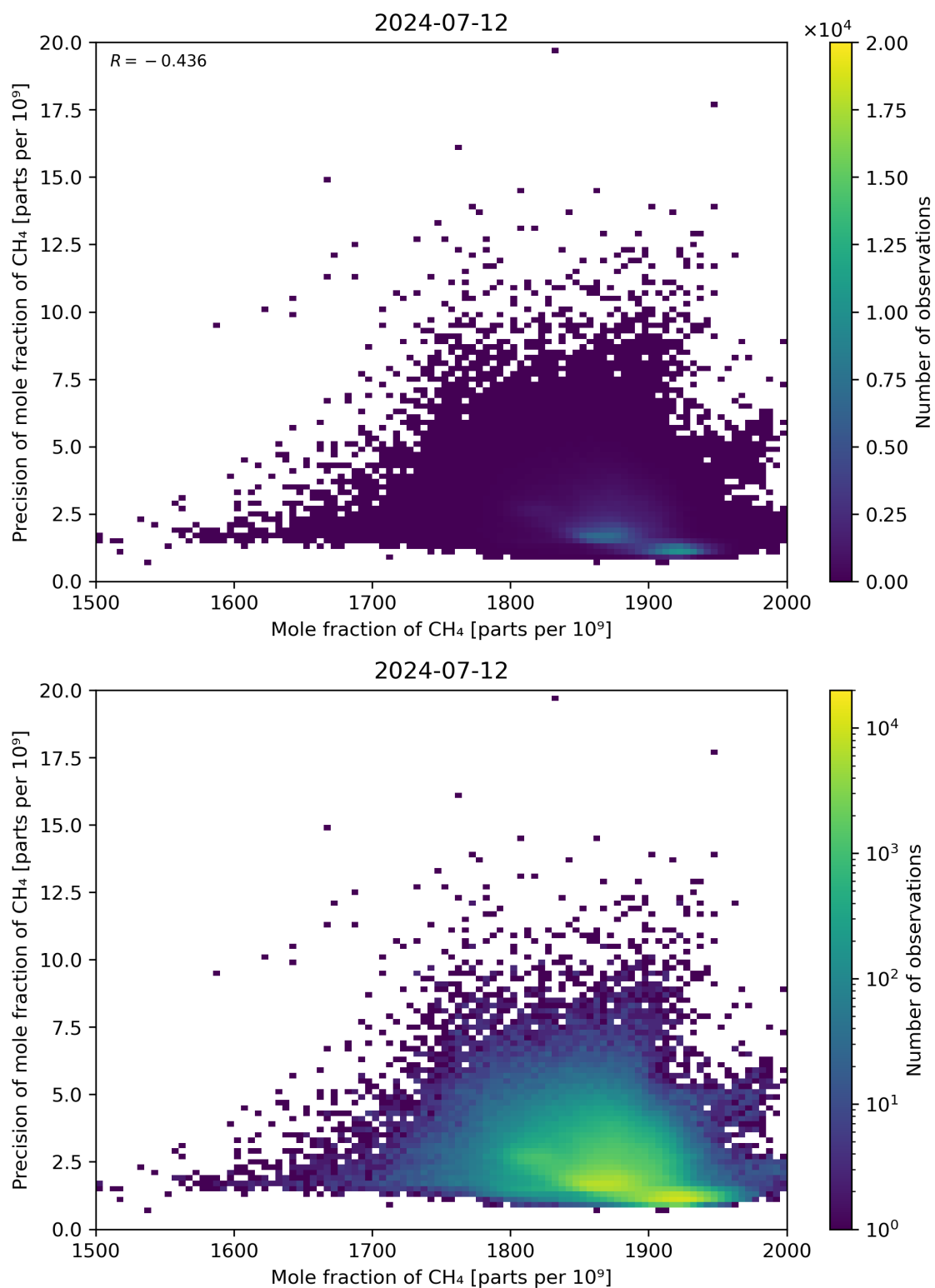
Figure 75: Scatter density plot of “Mole fraction of CH 4 ” against “Precision of mole fraction of CH 4 ” for 2024-07-11 to 2024-07-13.
