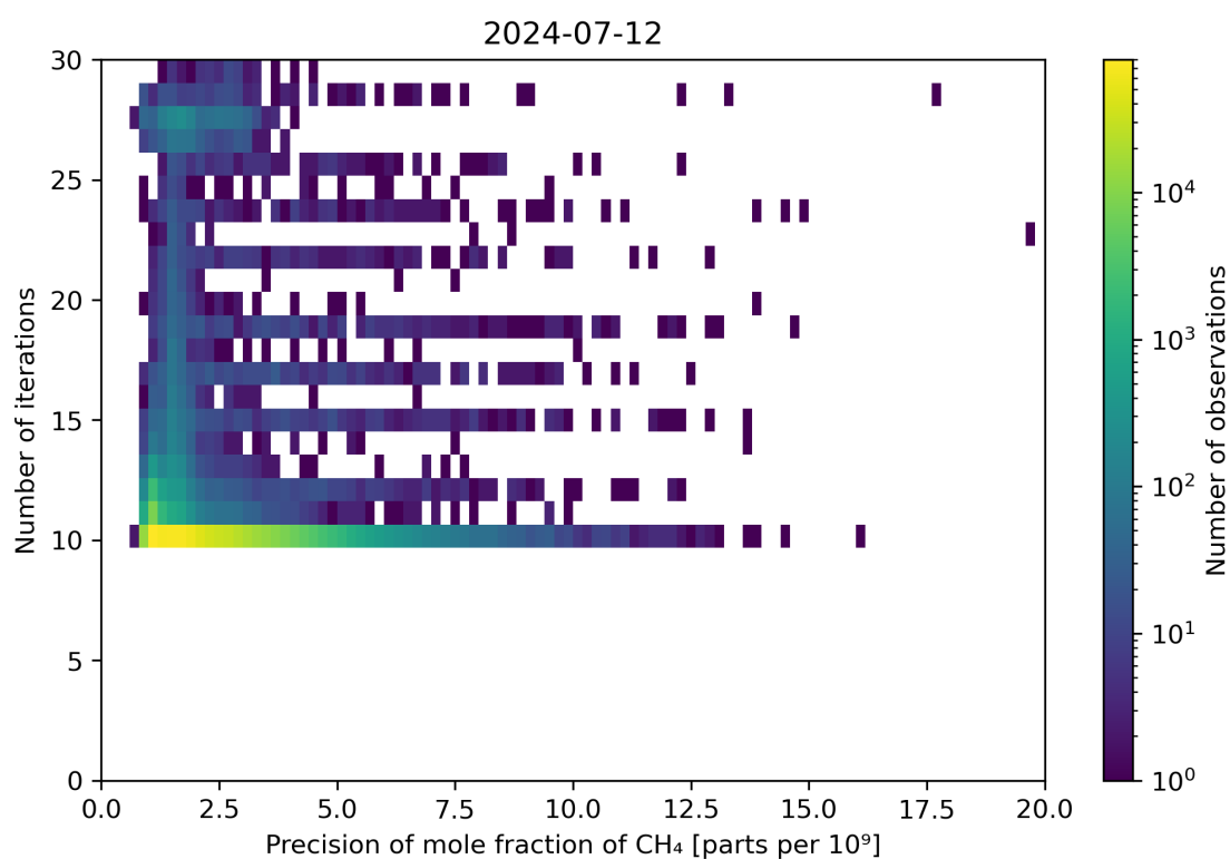
Figure 83: Scatter density plot of “Precision of mole fraction of CH 4 ” against “Number of iterations” for 2024-07-11 to 2024-07-13.
