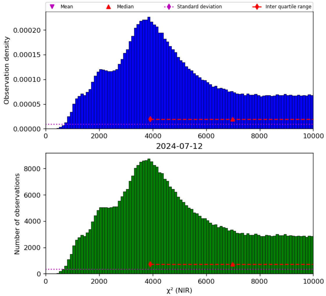
Figure 29: Histogram of " \chi^2 (NIR)" for 2024-07-11 to 2024-07-13
