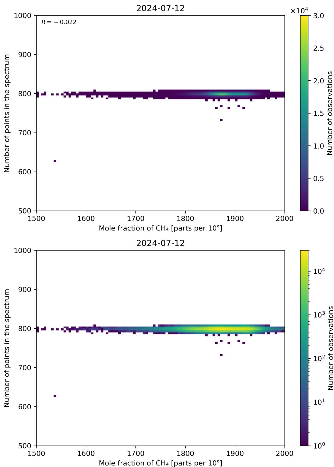
Figure 77: Scatter density plot of “Mole fraction of CH 4 ” against “Number of points in the spectrum” for 2024-07-11 to 2024-07-13.
