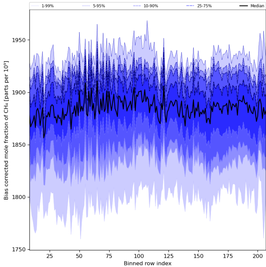
Figure 36: Along track statistics of “Bias corrected mole fraction of CH 4 ” for 2024-07-11 to 2024-07-13
