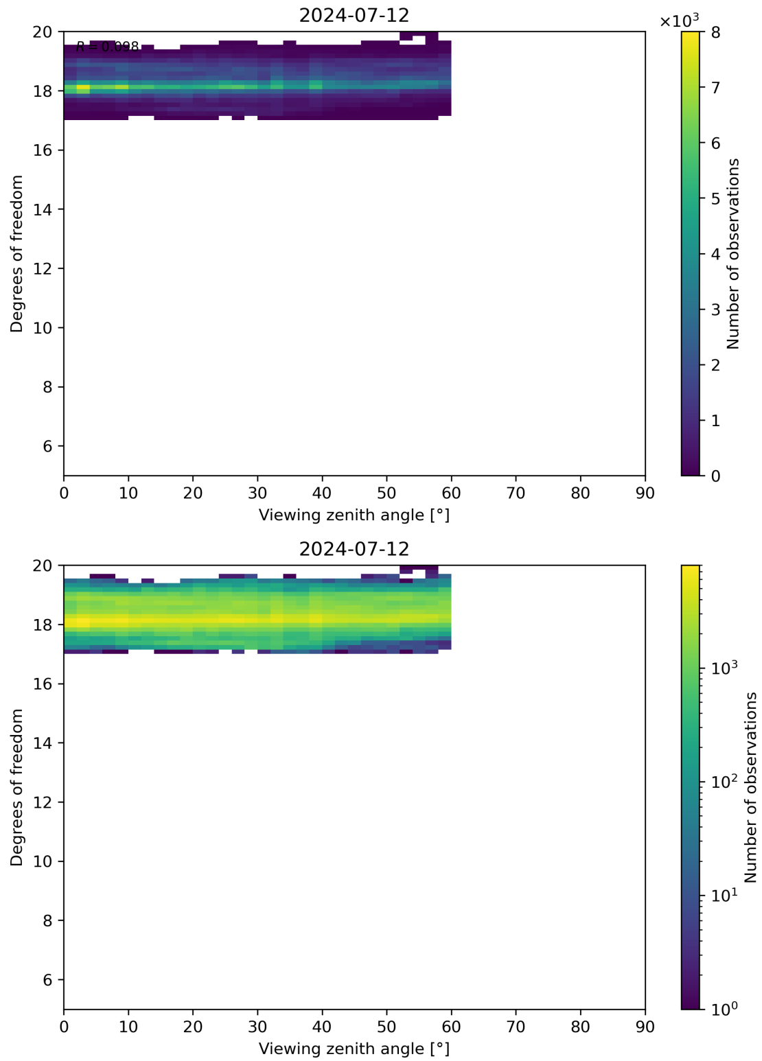
Figure 107: Scatter density plot of “Viewing zenith angle” against “Degrees of freedom” for 2024-07-11 to 2024-07-13.
