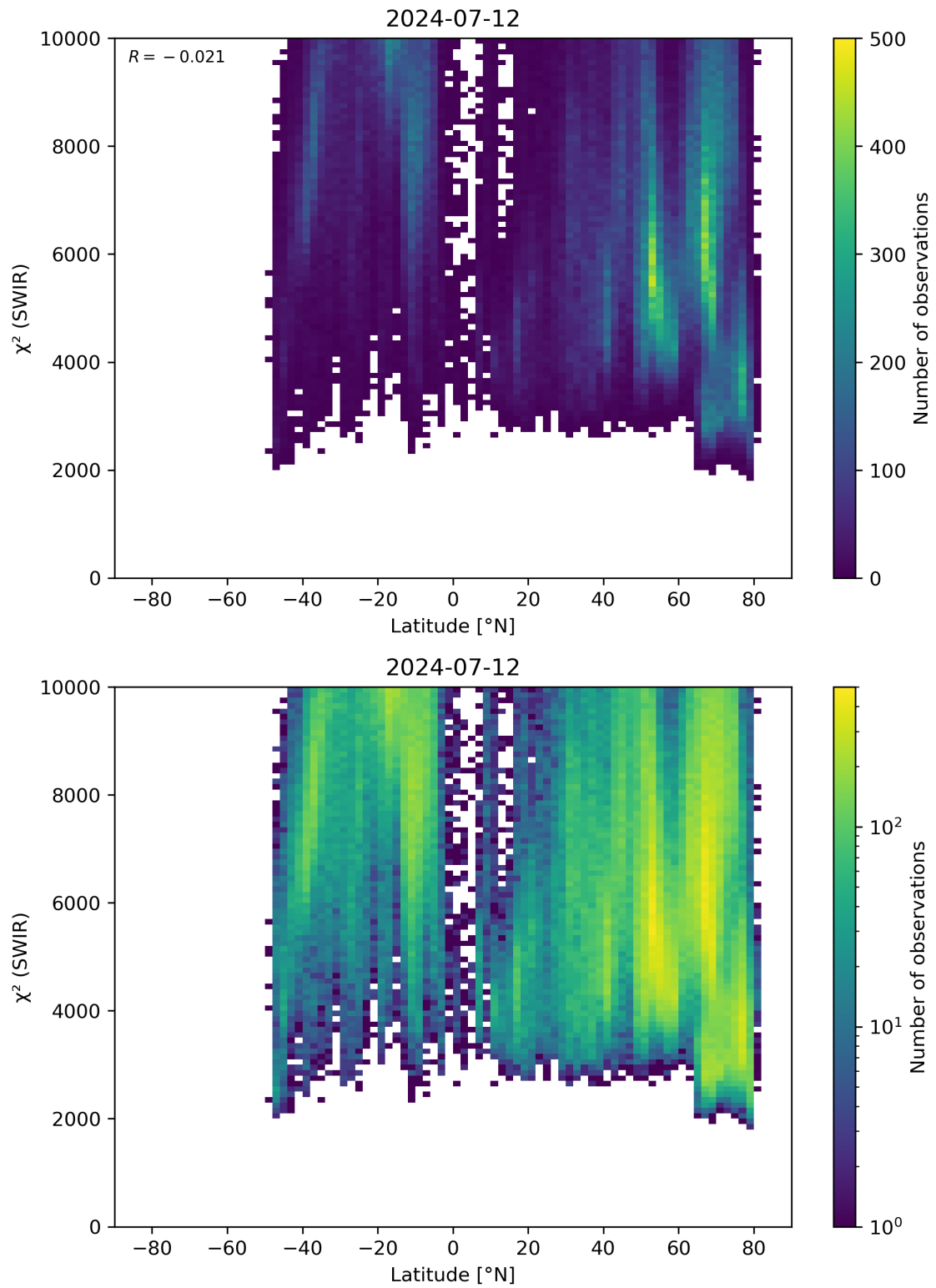
Figure 54: Scatter density plot of “Latitude” against “ \chi^2 (SWIR)” for 2024-07-11 to 2024-07-13.
