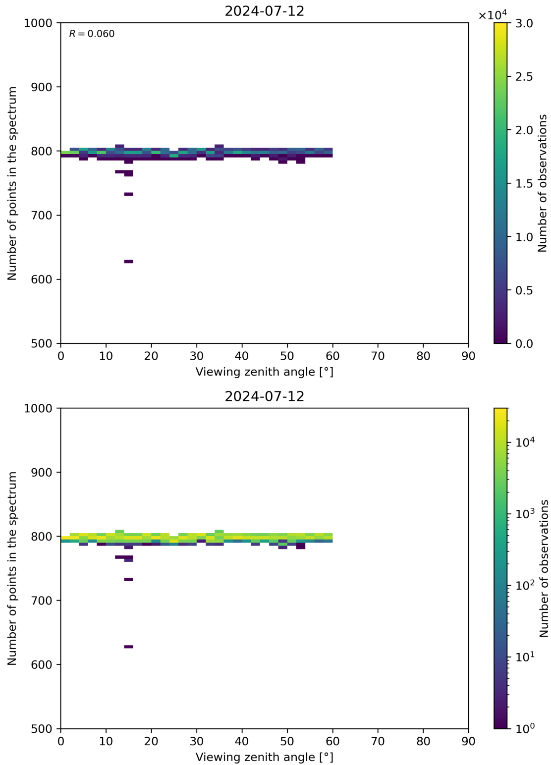
Figure 114: Scatter density plot of “Viewing zenith angle” against “Number of points in the spectrum” for 2024-07-11 to 2024-07-13.
