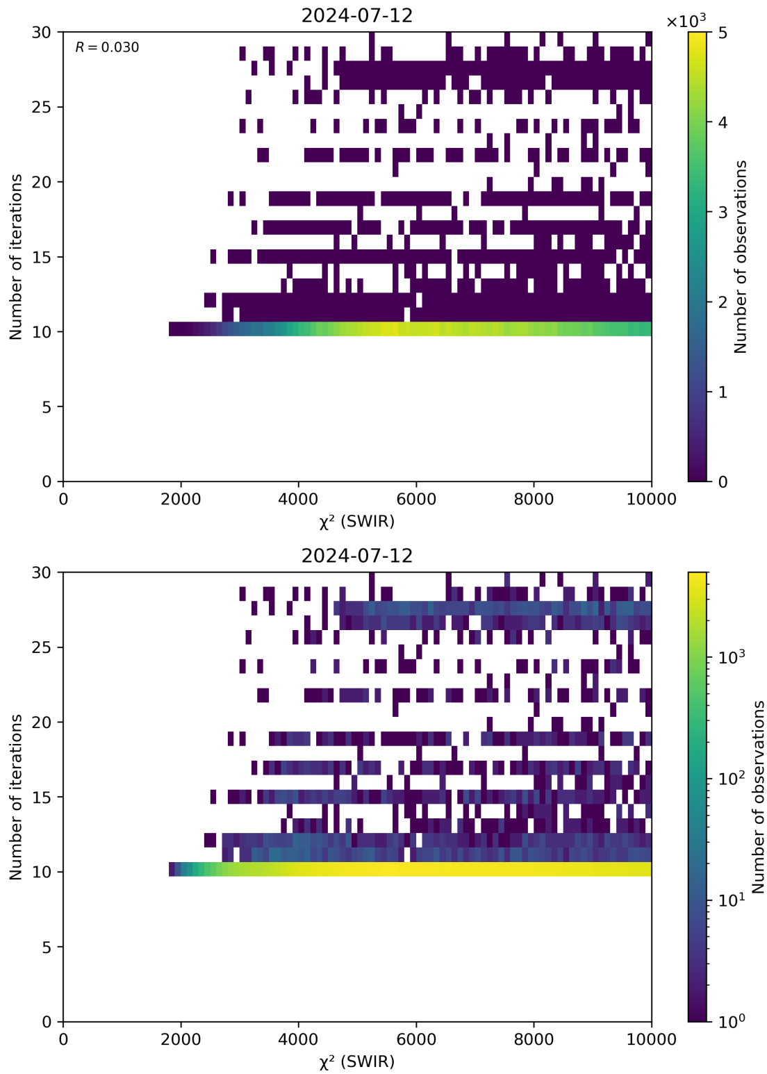
Figure 50: Scatter density plot of “ \chi^2 (SWIR)” against “Number of iterations” for 2024-07-11 to 2024-07-13.
