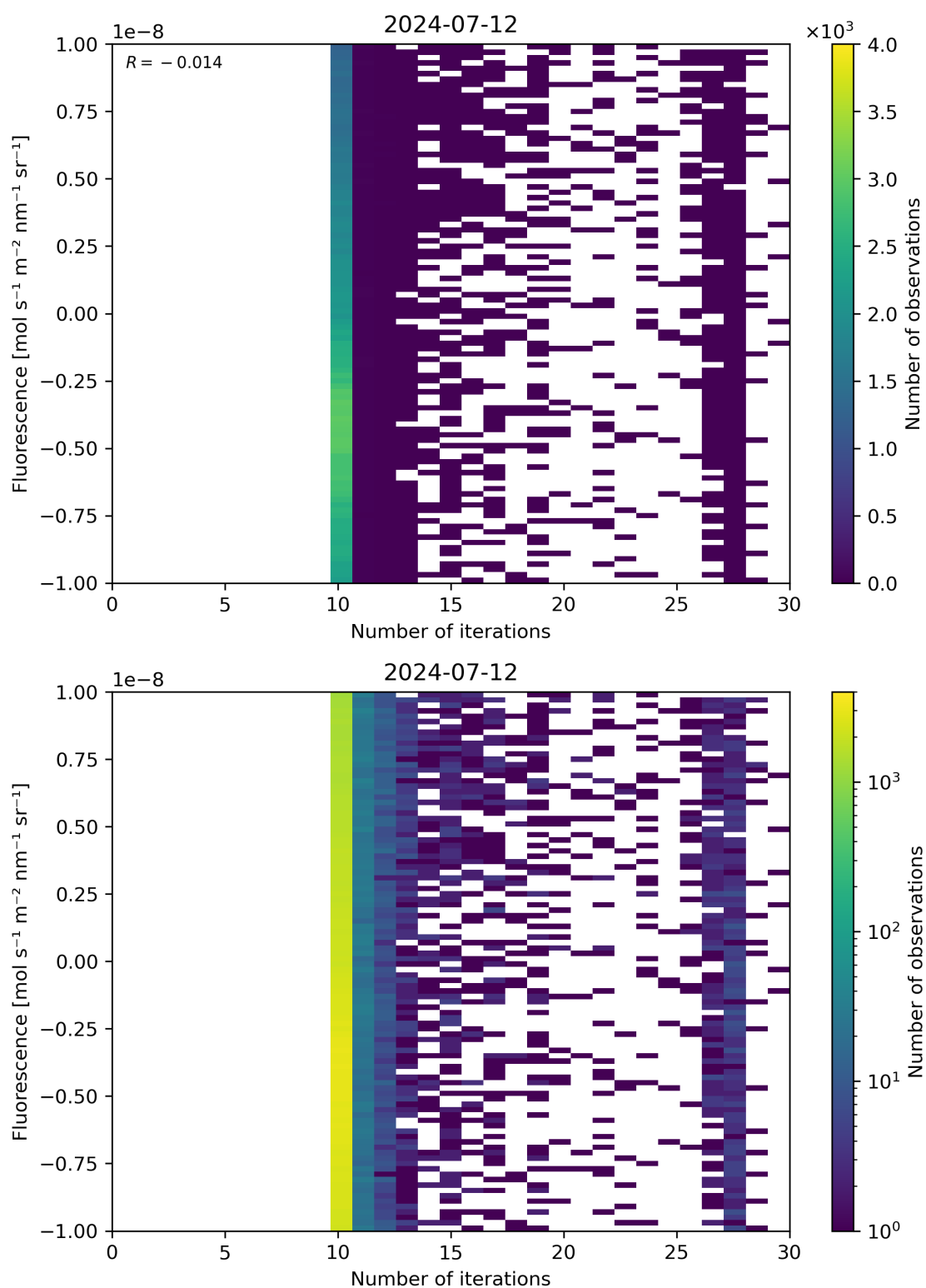
Figure 87: Scatter density plot of “Number of iterations” against “Fluorescence” for 2024-07-11 to 2024-07-13.
