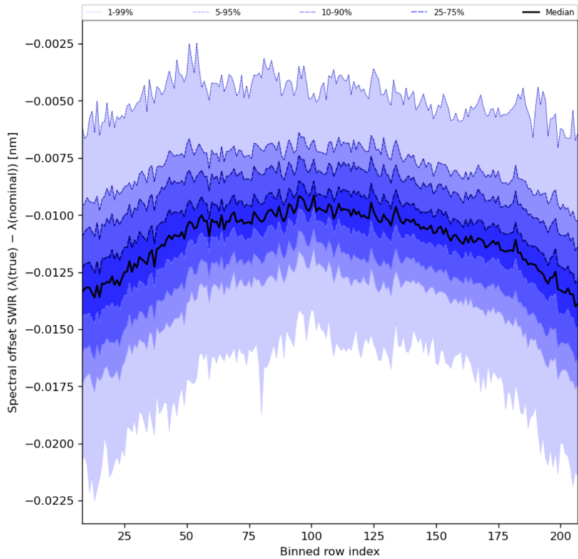
Figure 38: Along track statistics of “Spectral offset SWIR ( \lambda(\text{true}) - \lambda(\text{nominal}) )” for 2024-07-11 to 2024-07-13
