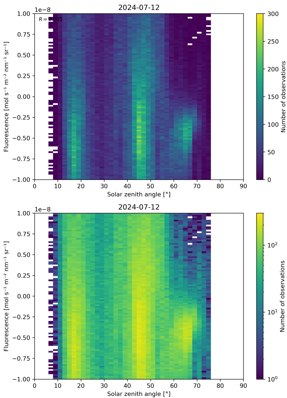
Figure 97: Scatter density plot of “Solar zenith angle” against “Fluorescence” for 2024-07-11 to 2024-07-13.
