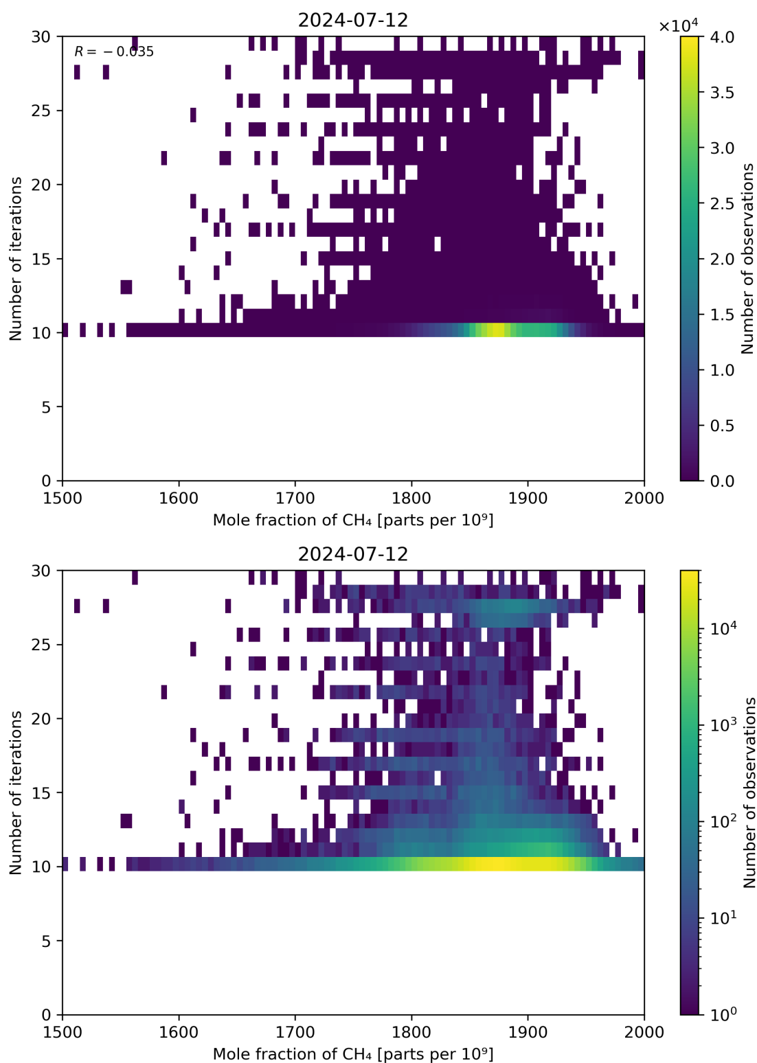
Figure 76: Scatter density plot of “Mole fraction of CH 4 ” against “Number of iterations” for 2024-07-11 to 2024-07-13.
