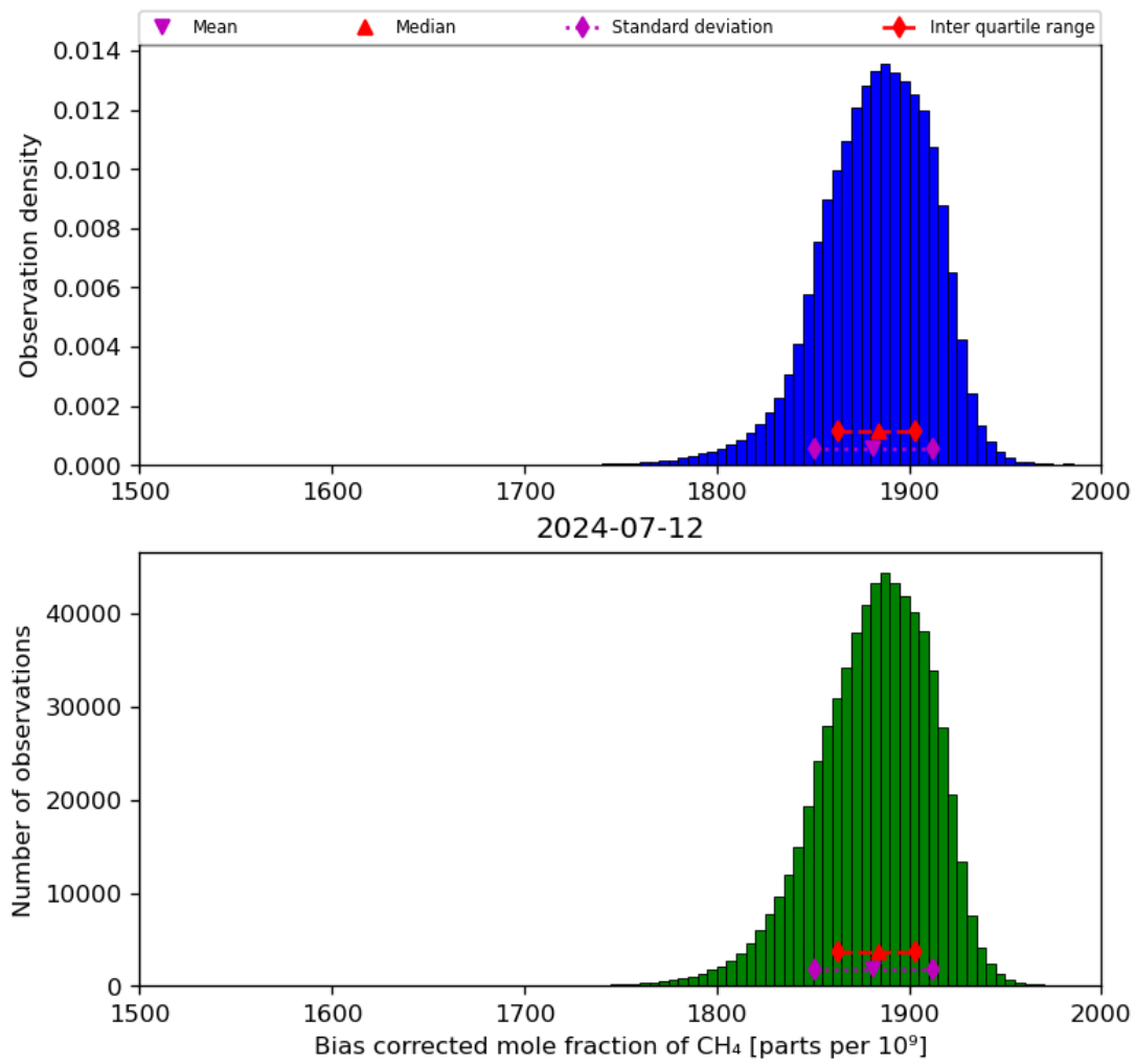
Figure 25: Histogram of “Bias corrected mole fraction of CH 4 ” for 2024-07-11 to 2024-07-13
