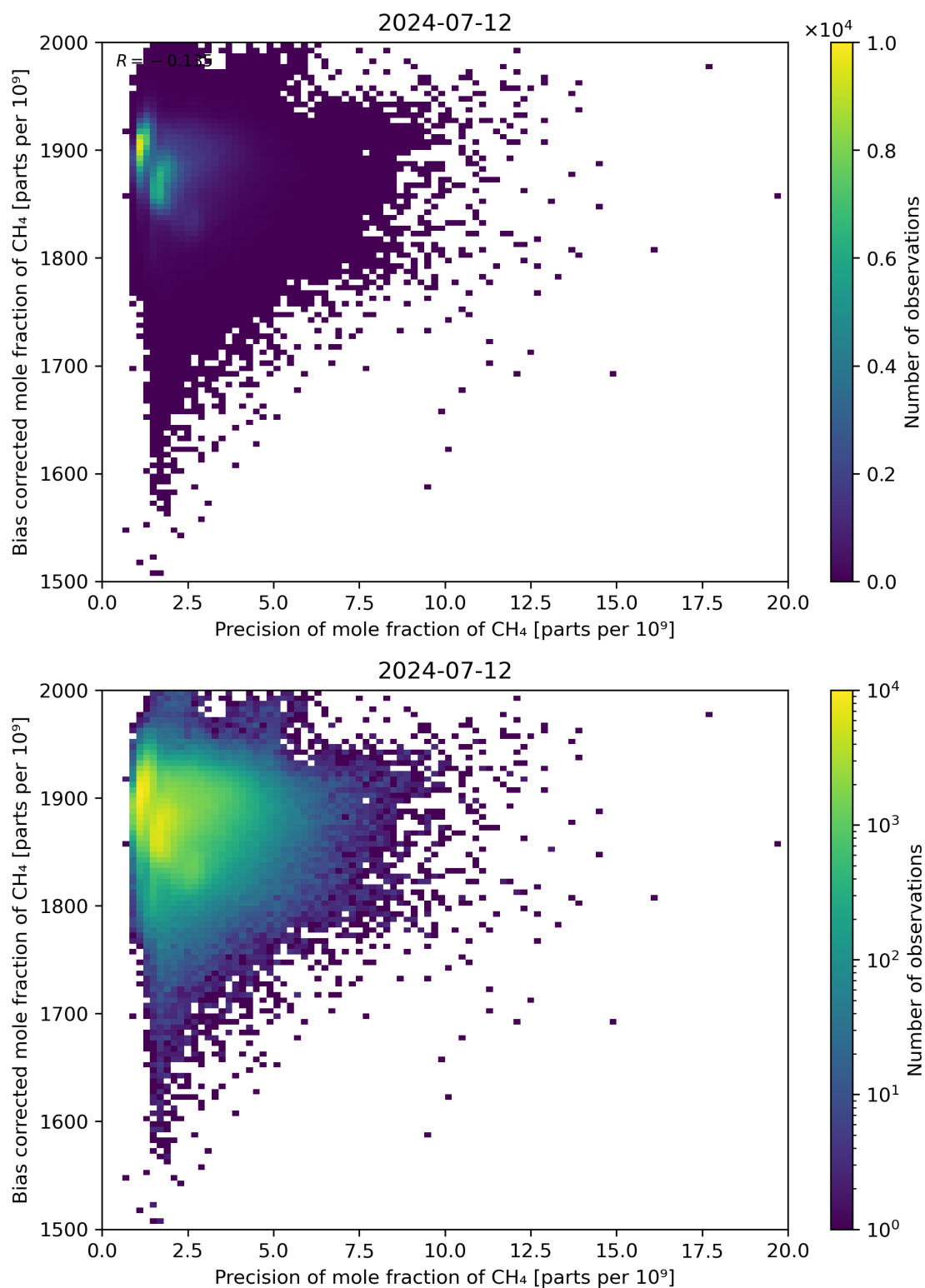
Figure 82: Scatter density plot of “Precision of mole fraction of \text{CH}_4 ” against “Bias corrected mole fraction of \text{CH}_4 ” for 2024-07-11 to 2024-07-13.
