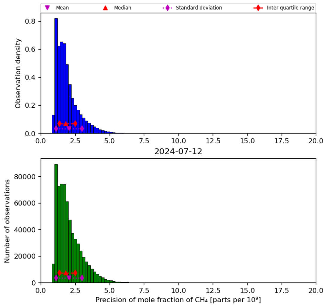
Figure 24: Histogram of “Precision of mole fraction of CH 4 ” for 2024-07-11 to 2024-07-13
