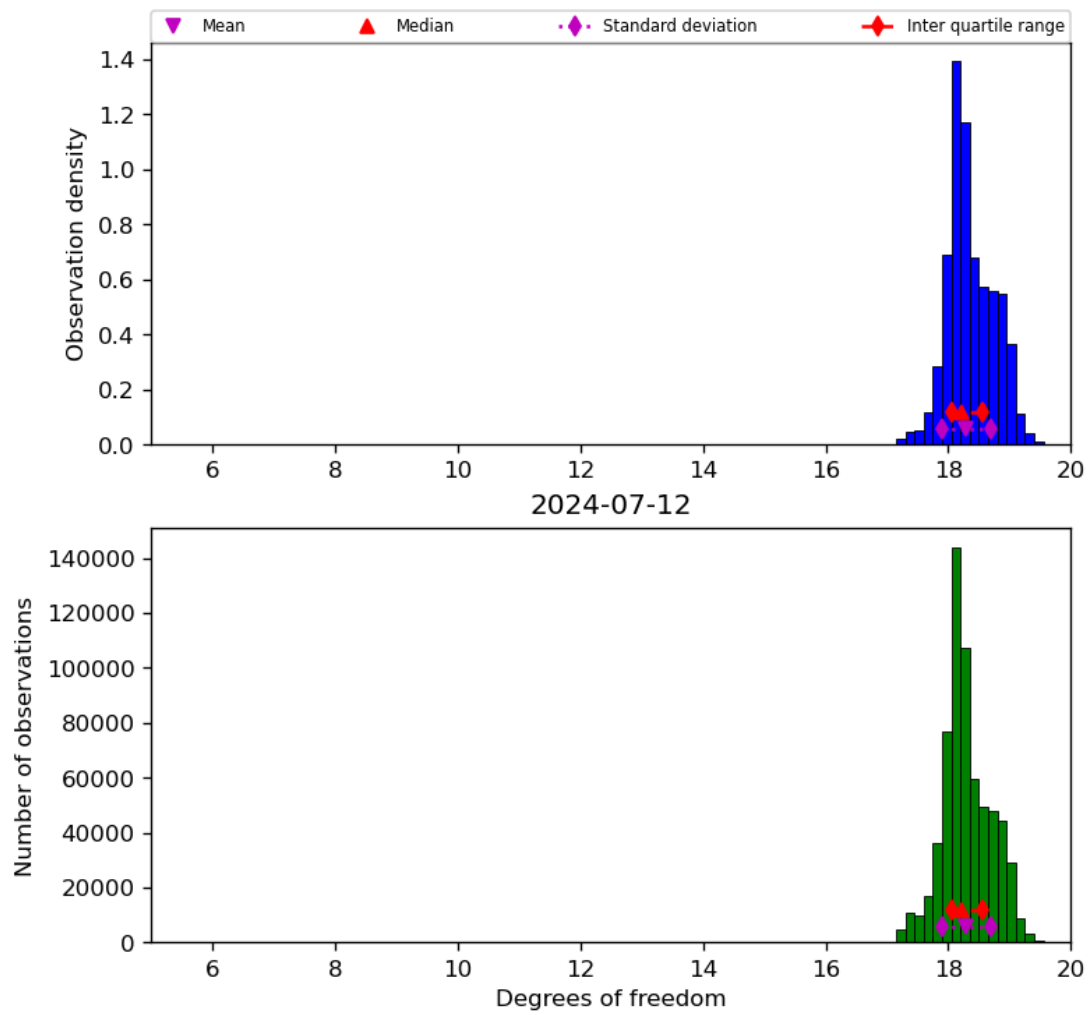
Figure 30: Histogram of “Degrees of freedom” for 2024-07-11 to 2024-07-13
