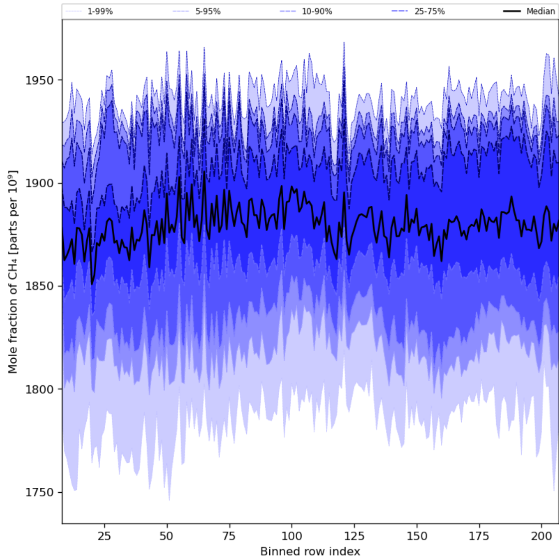
Figure 34: Along track statistics of “Mole fraction of CH 4 ” for 2024-07-11 to 2024-07-13
