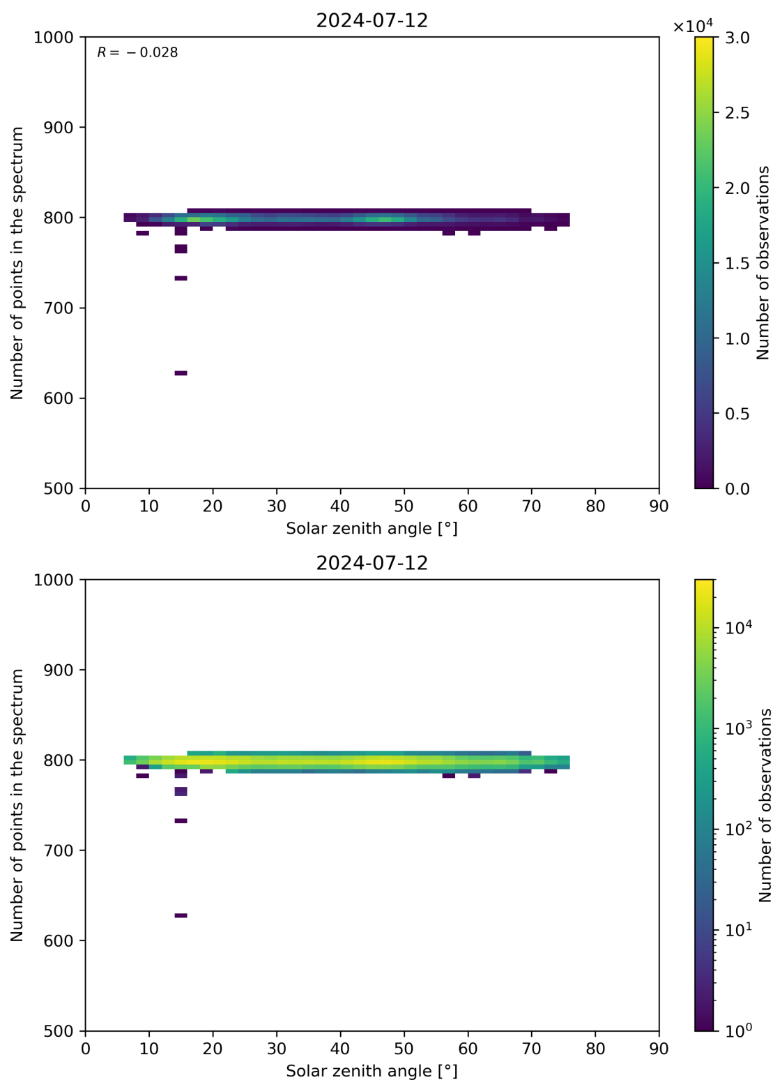
Figure 103: Scatter density plot of “Solar zenith angle” against “Number of points in the spectrum” for 2024-07-11 to 2024-07-13.
