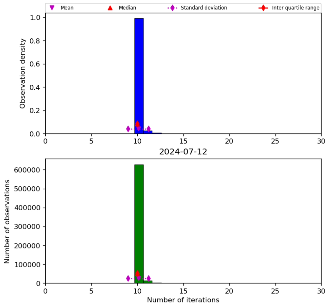
Figure 31: Histogram of “Number of iterations” for 2024-07-11 to 2024-07-13
