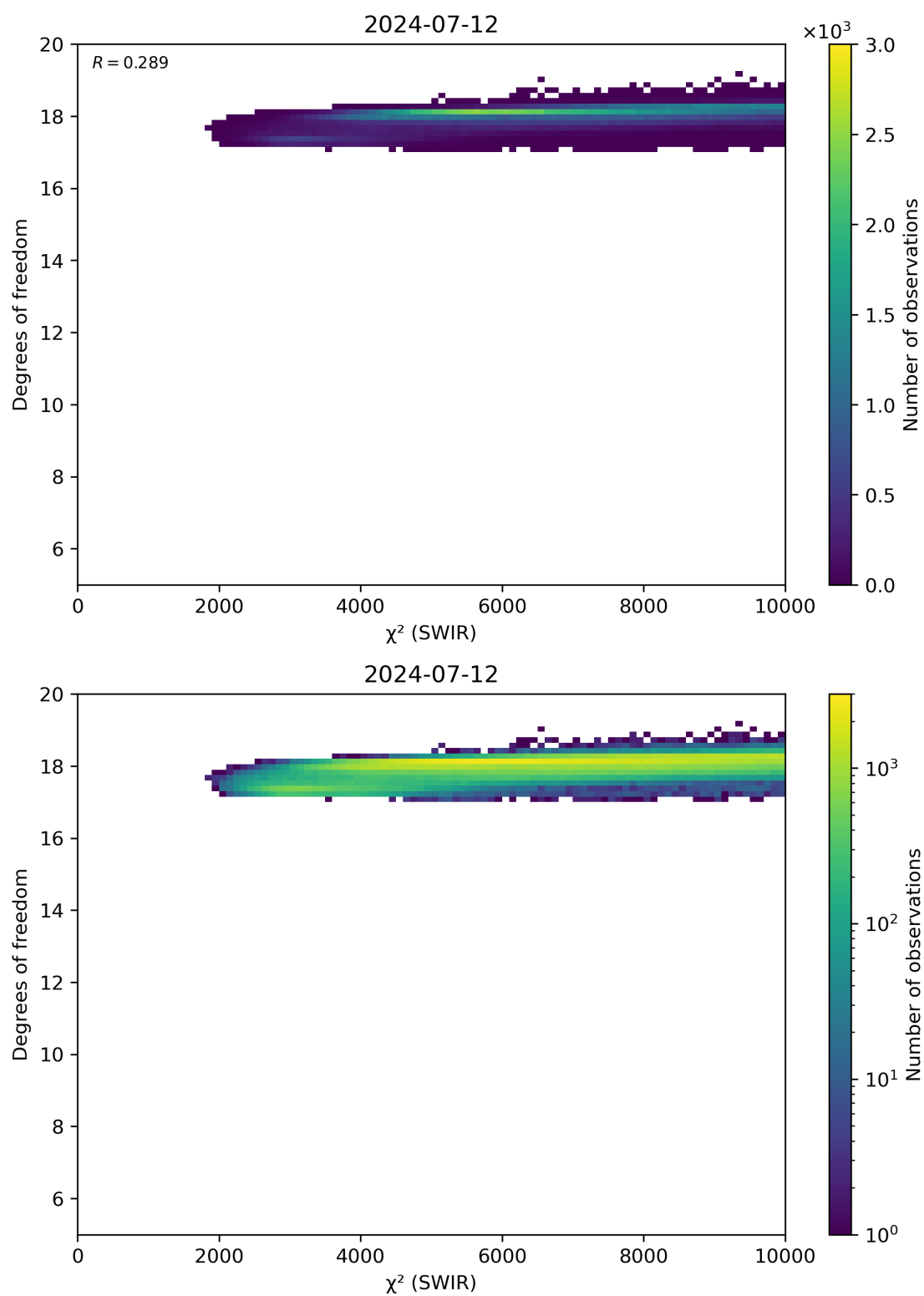
Figure 48: Scatter density plot of “ \chi^2 (SWIR)” against “Degrees of freedom” for 2024-07-11 to 2024-07-13.
