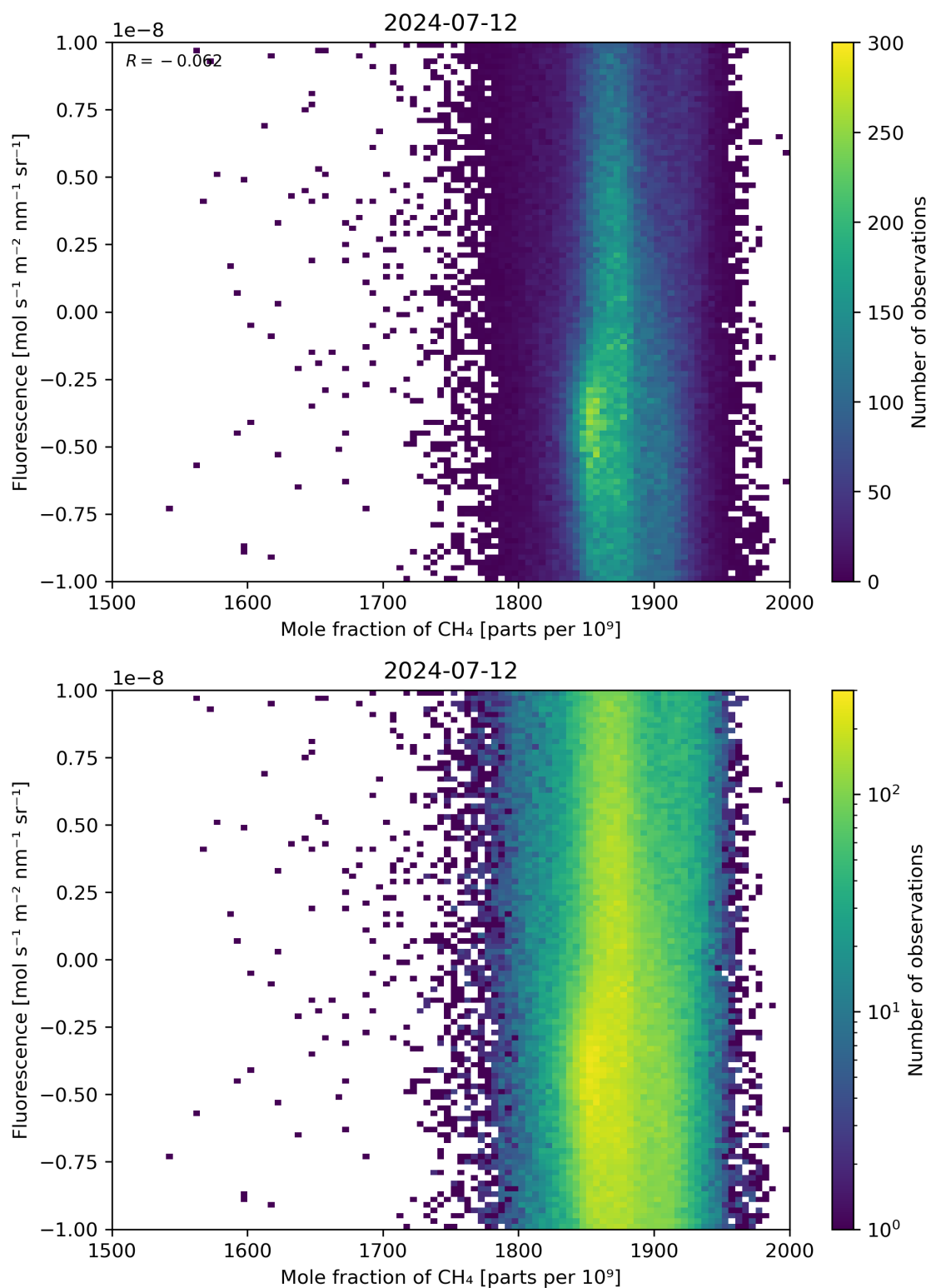
Figure 73: Scatter density plot of “Mole fraction of \text{CH}_4 ” against “Fluorescence” for 2024-07-11 to 2024-07-13.
