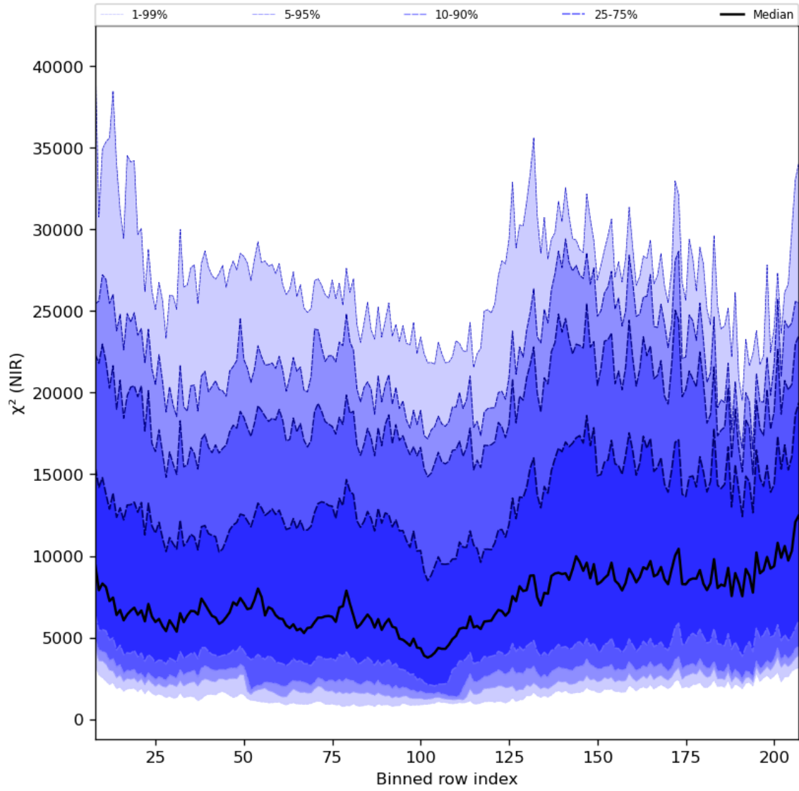
Figure 40: Along track statistics of “ \chi^2 (NIR)” for 2024-07-11 to 2024-07-13
