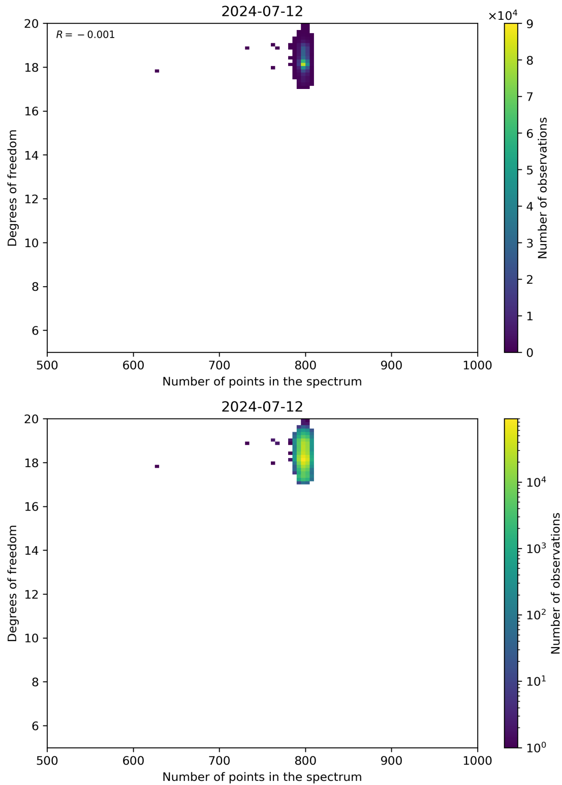
Figure 90: Scatter density plot of “Number of points in the spectrum” against “Degrees of freedom” for 2024-07-11 to 2024-07-13.
