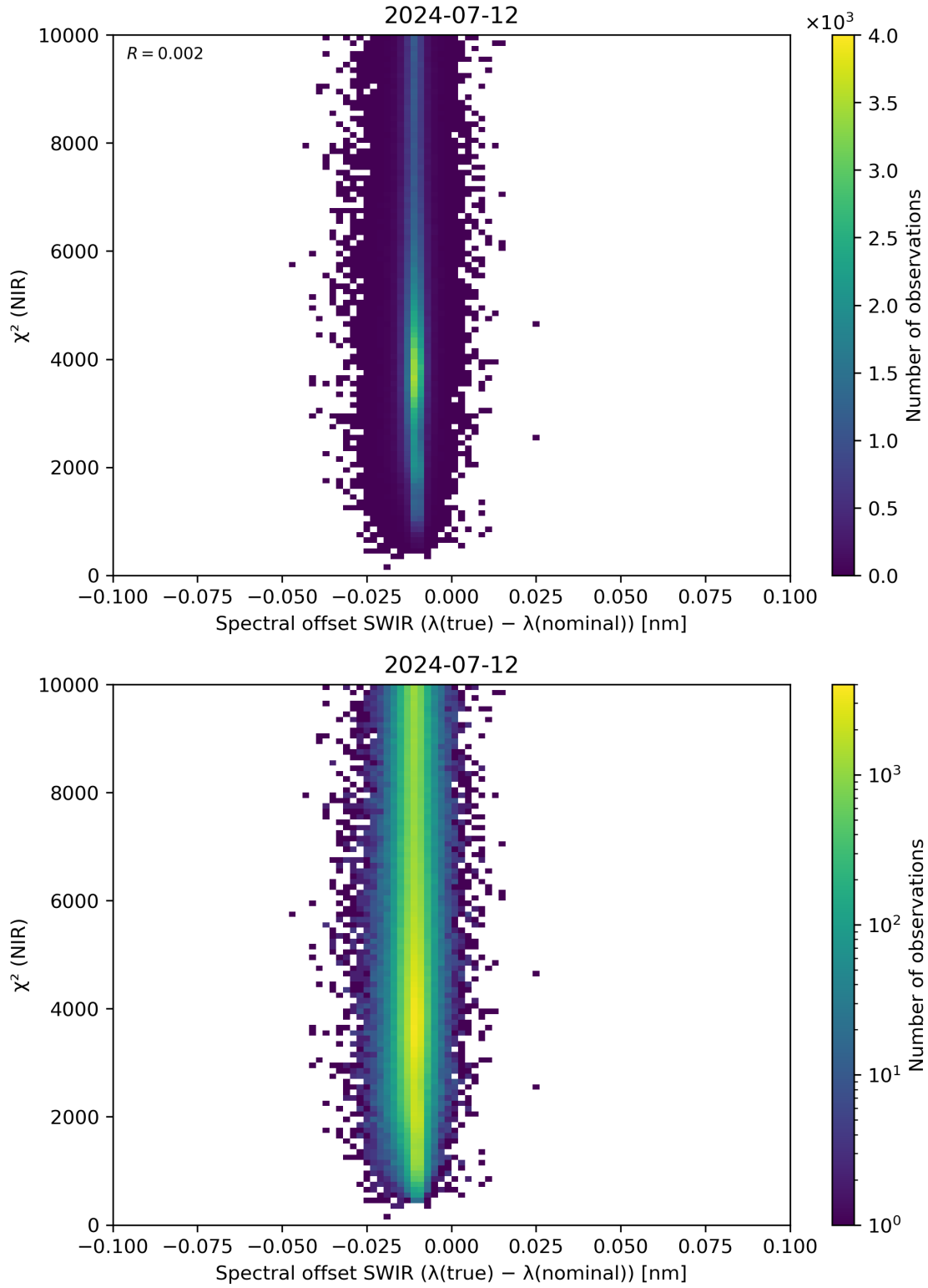
Figure 117: Scatter density plot of “Spectral offset SWIR ( \lambda(\text{true}) - \lambda(\text{nominal}) )” against “ \chi^2 (NIR)” for 2024-07-11 to 2024-07-13.
