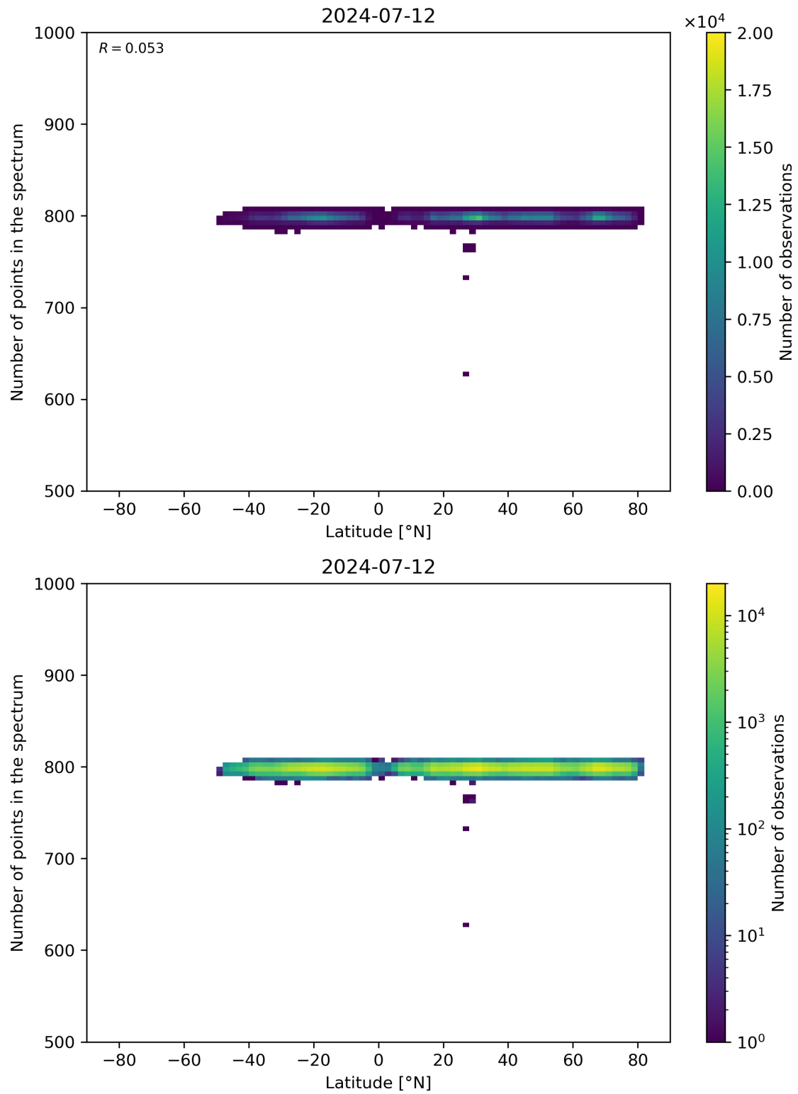
Figure 61: Scatter density plot of “Latitude” against “Number of points in the spectrum” for 2024-07-11 to 2024-07-13.
