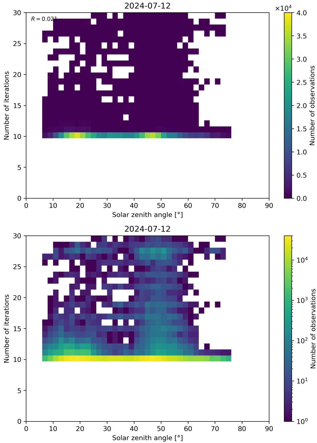
Figure 102: Scatter density plot of “Solar zenith angle” against “Number of iterations” for 2024-07-11 to 2024-07-13.
