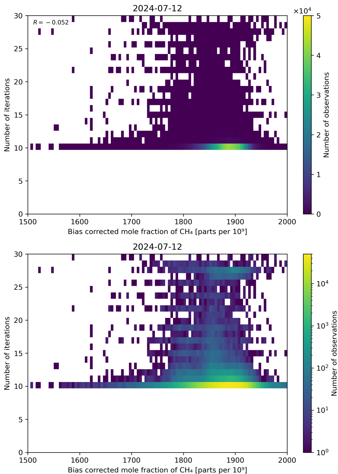
Figure 67: Scatter density plot of “Bias corrected mole fraction of CH 4 ” against “Number of iterations” for 2024-07-11 to 2024-07-13.
