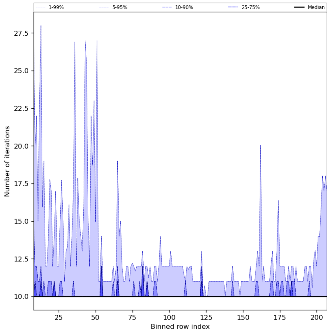
Figure 42: Along track statistics of “Number of iterations” for 2024-07-11 to 2024-07-13
