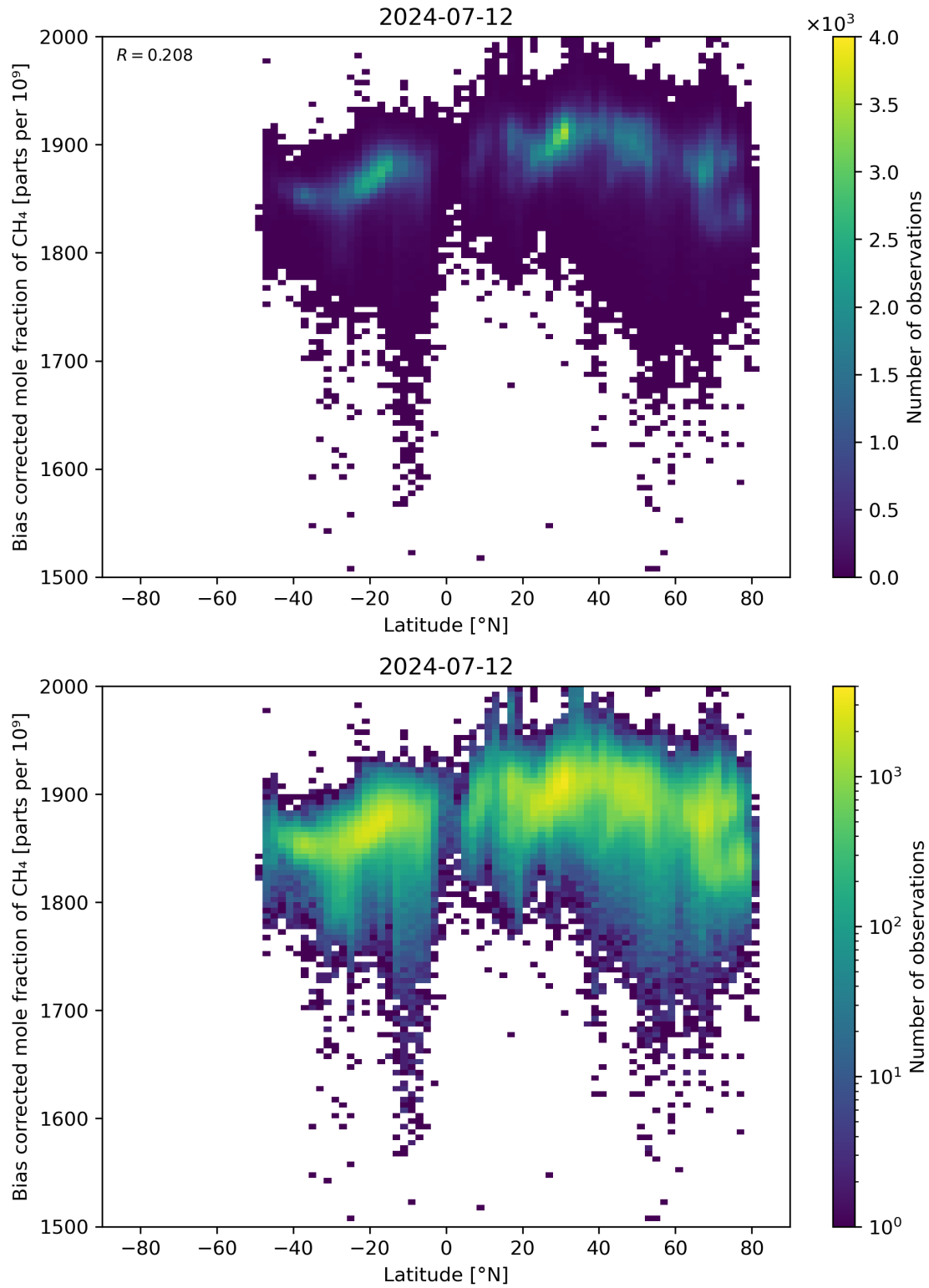
Figure 58: Scatter density plot of “Latitude” against “Bias corrected mole fraction of \text{CH}_4 ” for 2024-07-11 to 2024-07-13.
