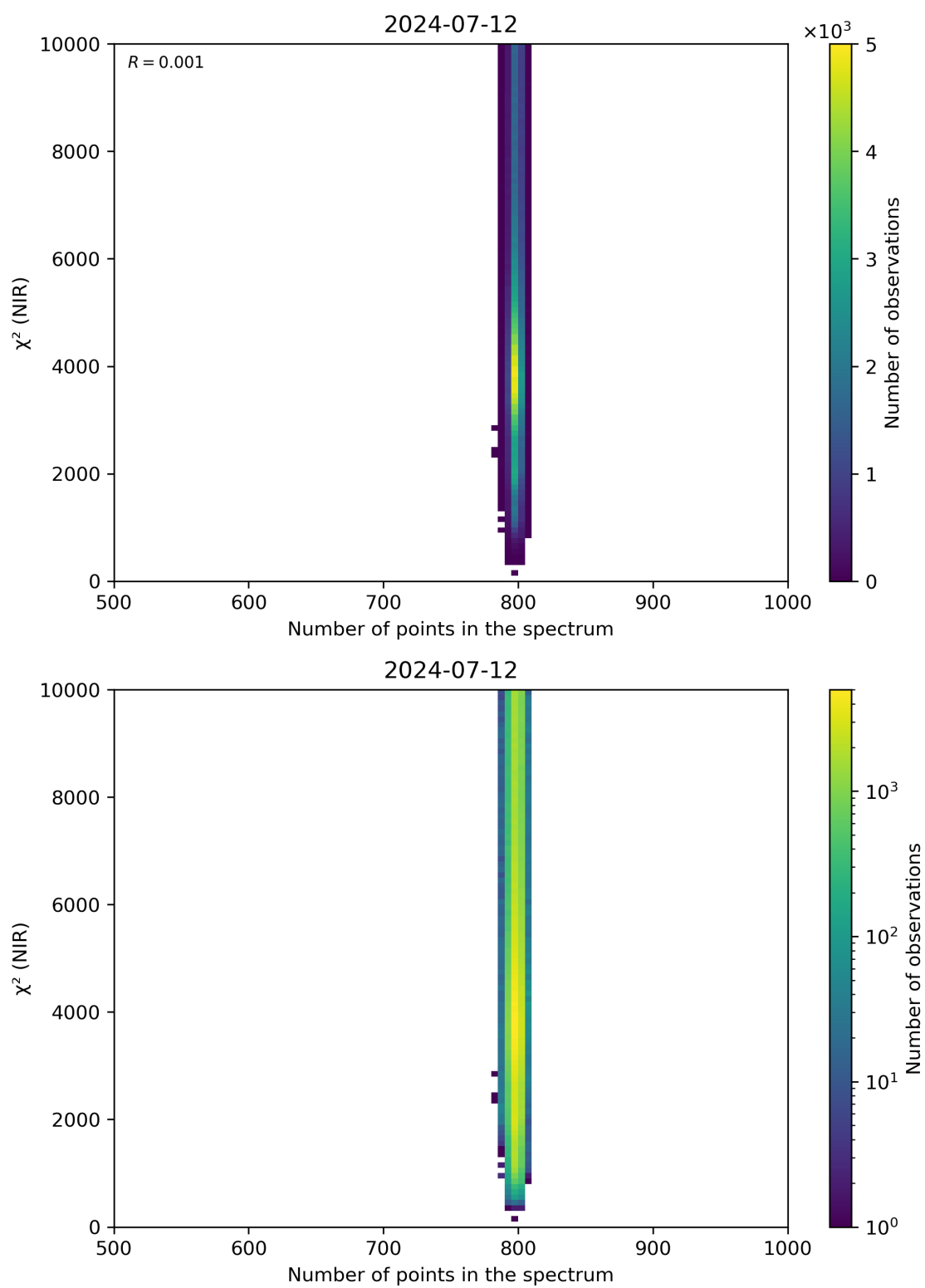
Figure 88: Scatter density plot of “Number of points in the spectrum” against “ \chi^2 (NIR)” for 2024-07-11 to 2024-07-13.
