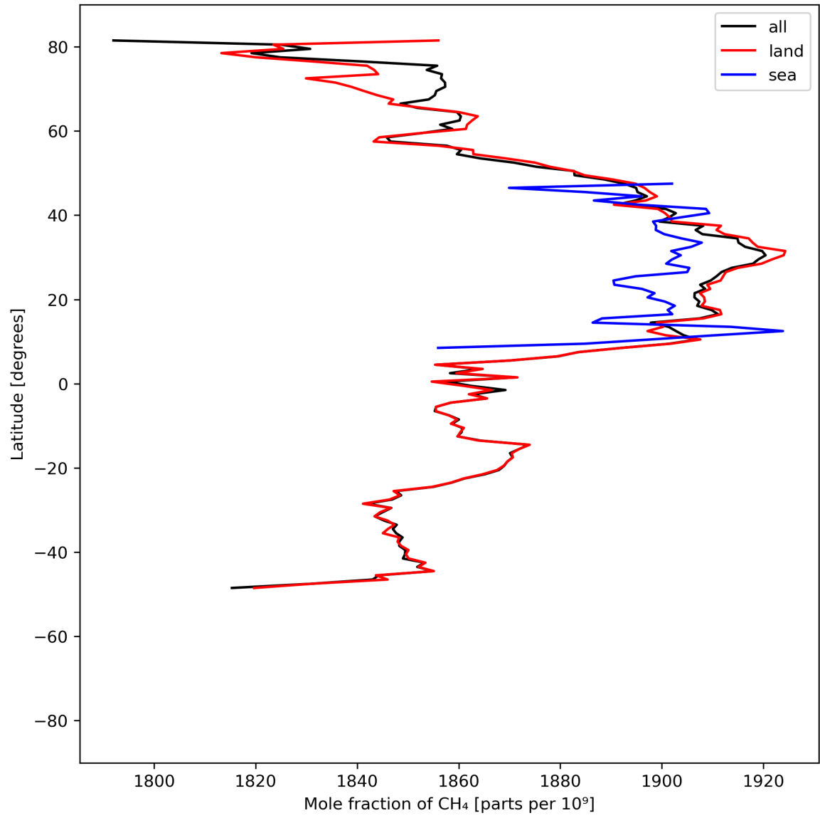
Figure 12: Zonal average of “Mole fraction of \text{CH}_4 ” for 2024-07-11 to 2024-07-13.
