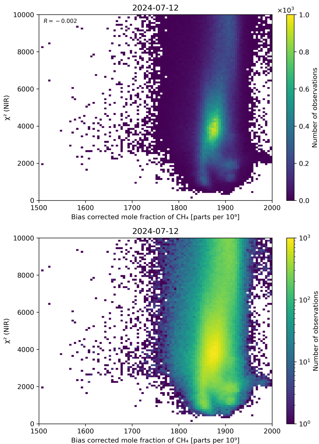
Figure 63: Scatter density plot of “Bias corrected mole fraction of CH 4 ” against “ \chi^2 (NIR)” for 2024-07-11 to 2024-07-13.
