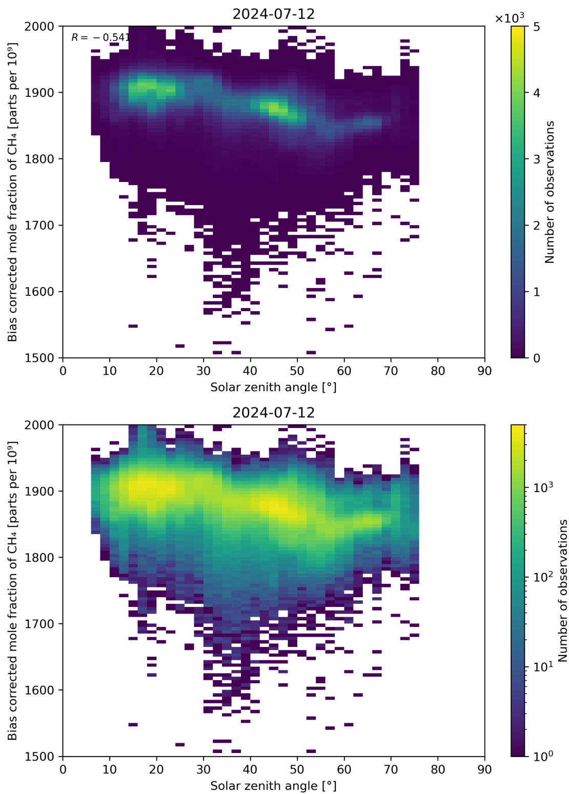
Figure 100: Scatter density plot of “Solar zenith angle” against “Bias corrected mole fraction of CH 4 ” for 2024-07-11 to 2024-07-13.
