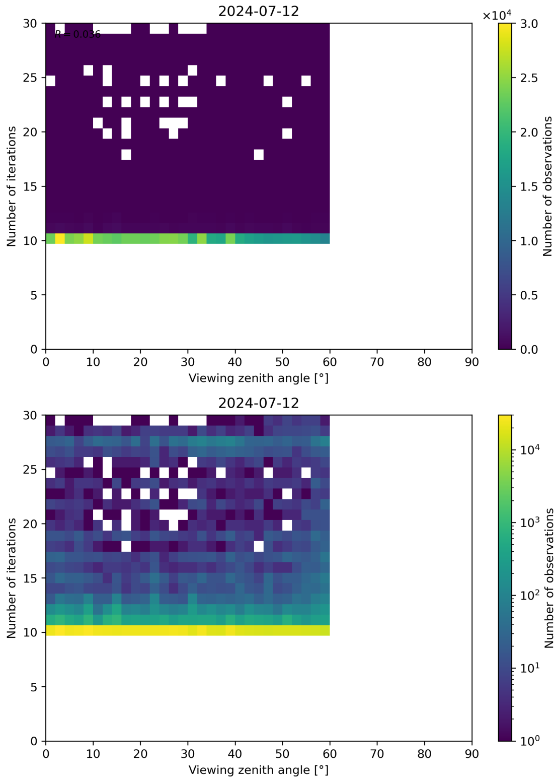
Figure 113: Scatter density plot of “Viewing zenith angle” against “Number of iterations” for 2024-07-11 to 2024-07-13.
