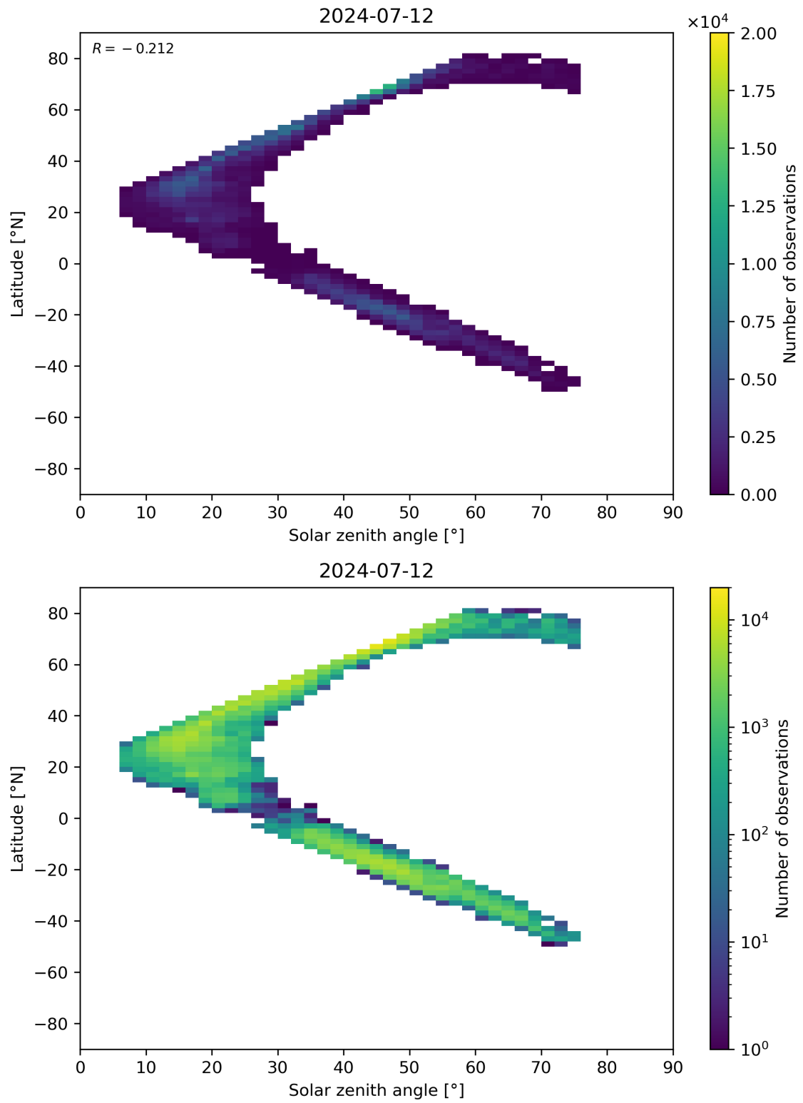
Figure 98: Scatter density plot of “Solar zenith angle” against “Latitude” for 2024-07-11 to 2024-07-13.
