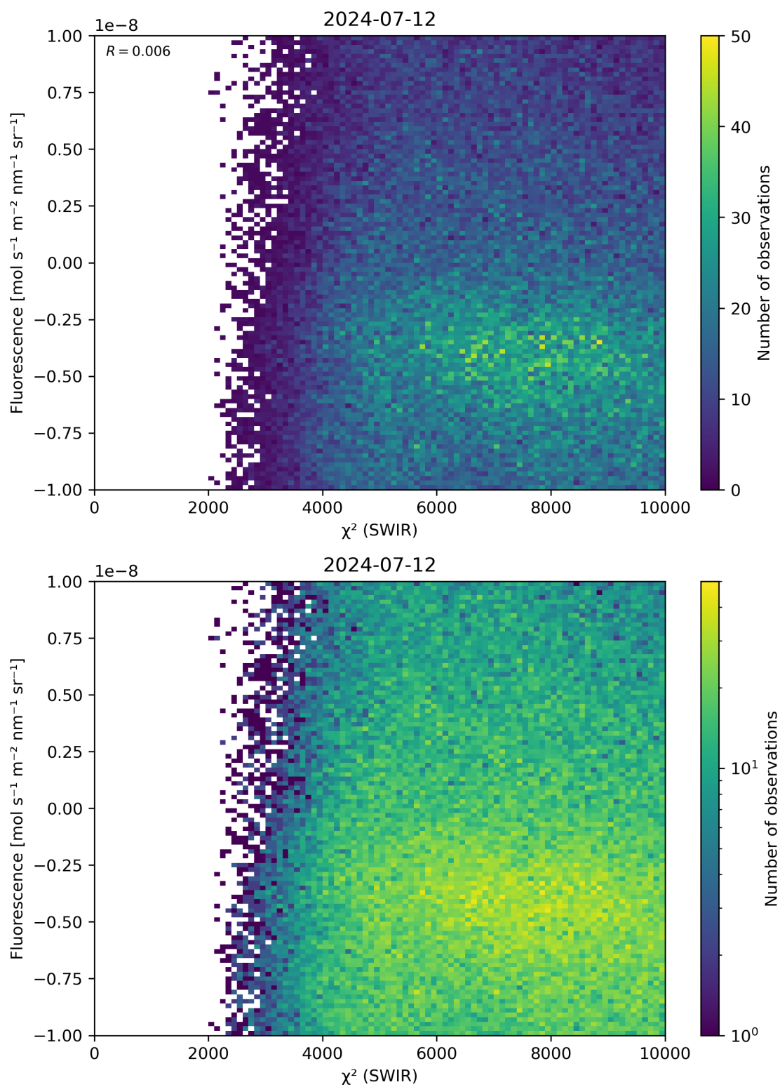
Figure 49: Scatter density plot of “ \chi^2 (SWIR)” against “Fluorescence” for 2024-07-11 to 2024-07-13.
