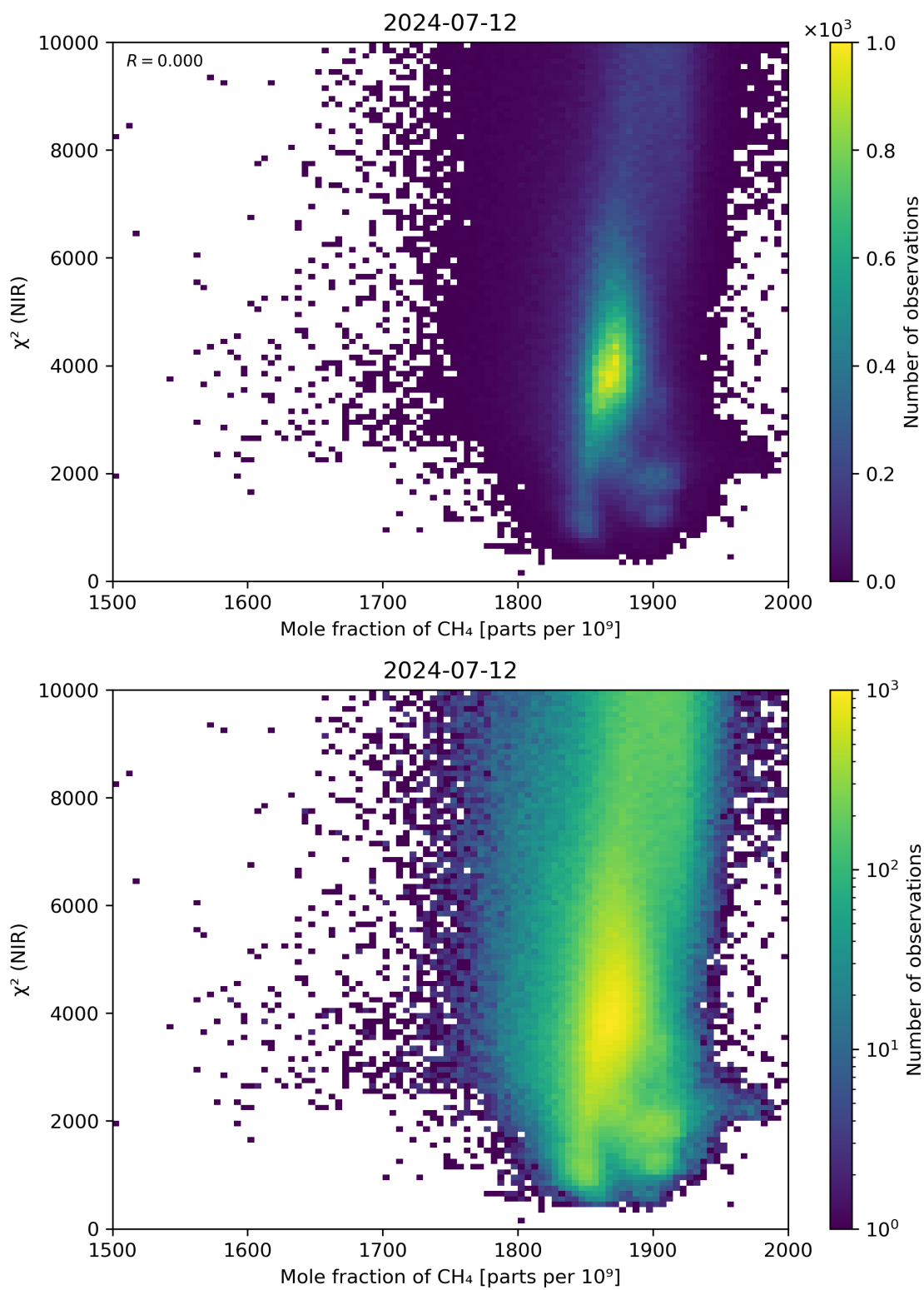
Figure 70: Scatter density plot of “Mole fraction of \text{CH}_4 ” against “ \chi^2 (NIR)” for 2024-07-11 to 2024-07-13.
