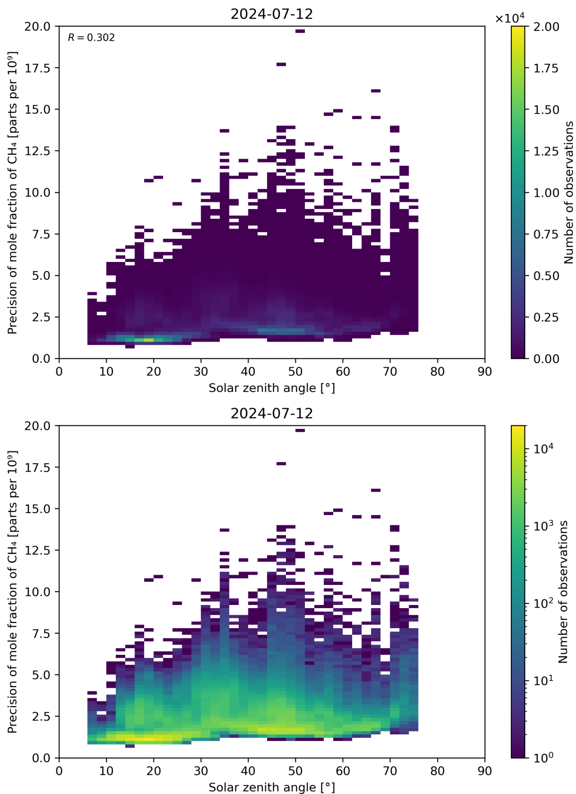
Figure 101: Scatter density plot of “Solar zenith angle” against “Precision of mole fraction of CH 4 ” for 2024-07-11 to 2024-07-13.
