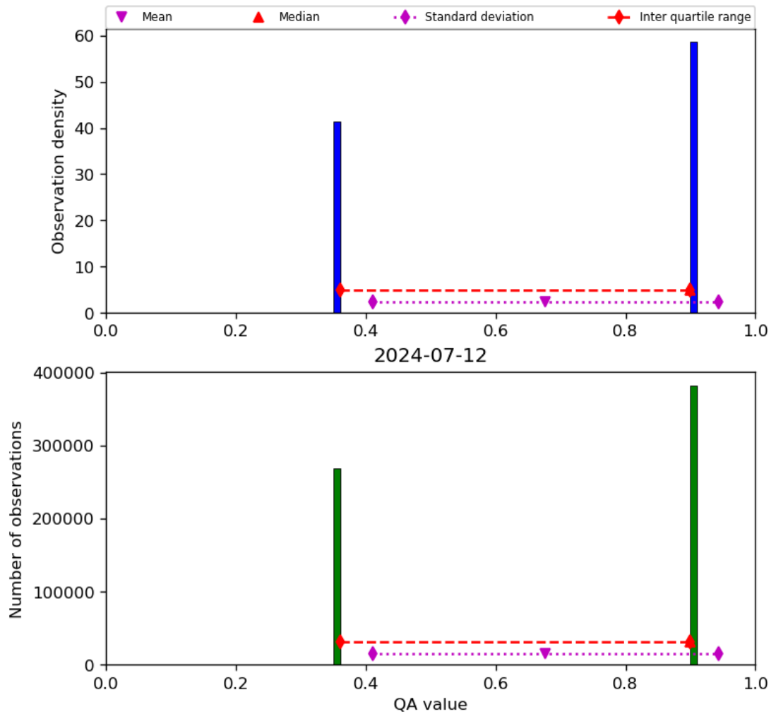
Figure 22: Histogram of “QA value” for 2024-07-11 to 2024-07-13
