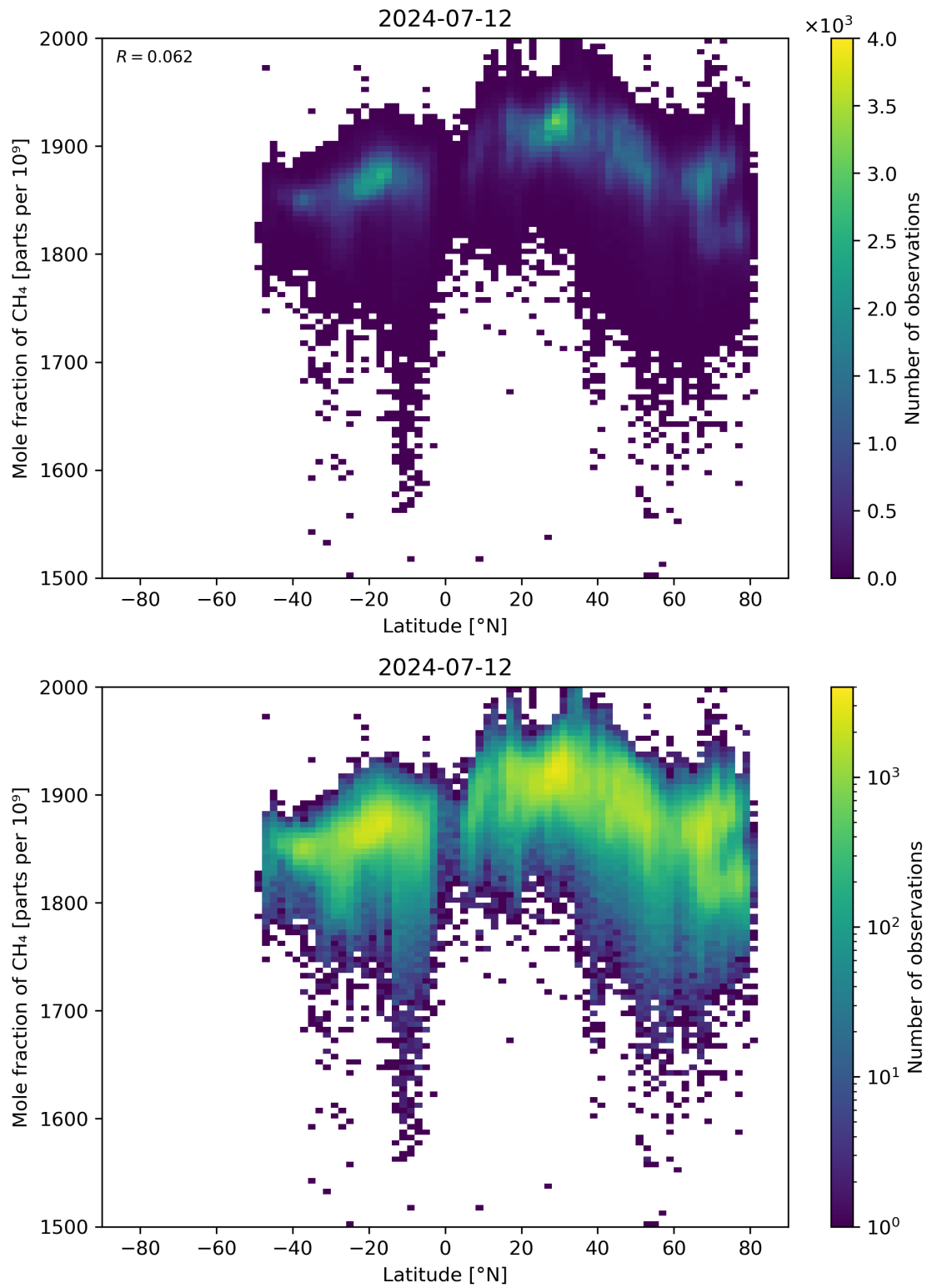
Figure 57: Scatter density plot of “Latitude” against “Mole fraction of \text{CH}_4 ” for 2024-07-11 to 2024-07-13.
