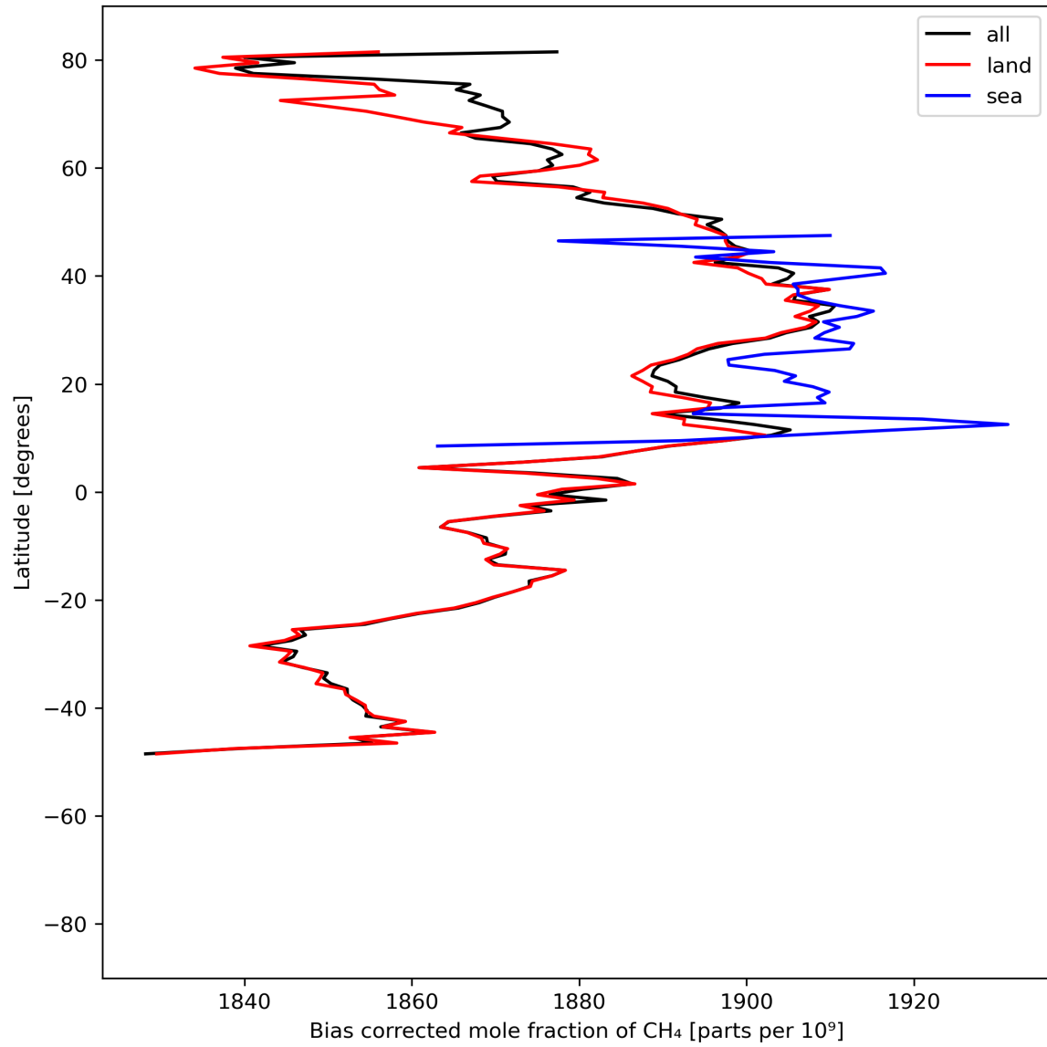
Figure 14: Zonal average of “Bias corrected mole fraction of CH 4 ” for 2024-07-11 to 2024-07-13.
