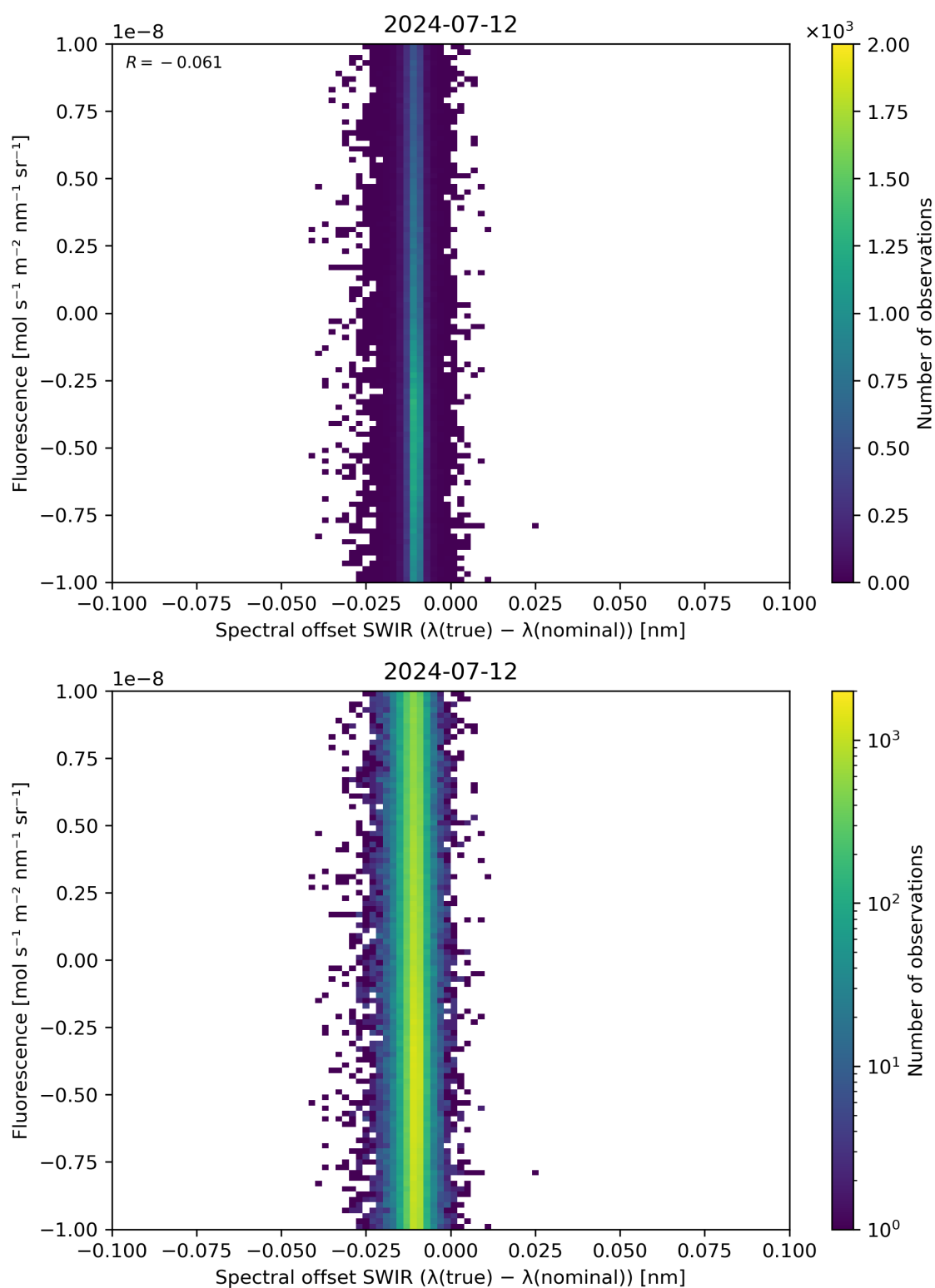
Figure 120: Scatter density plot of “Spectral offset SWIR ( \lambda(\text{true}) - \lambda(\text{nominal}) )” against “Fluorescence” for 2024-07-11 to 2024-07-13.
