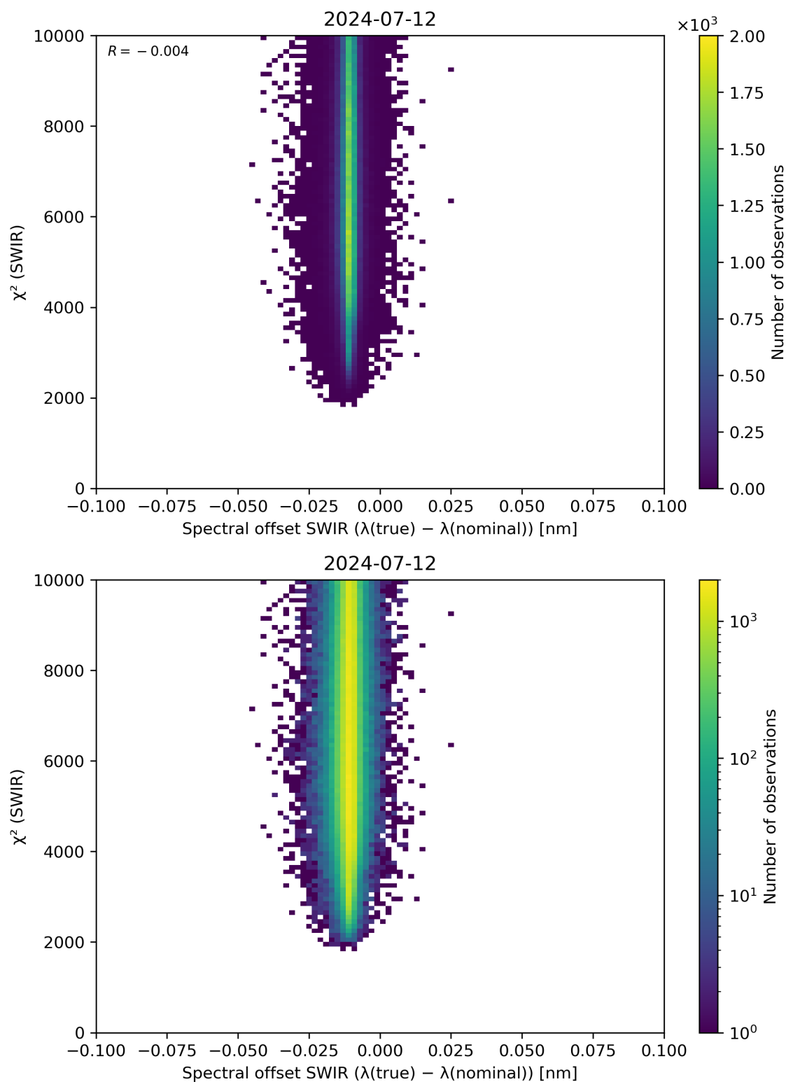
Figure 118: Scatter density plot of “Spectral offset SWIR ( \lambda(\text{true}) - \lambda(\text{nominal}) )” against “ \chi^2 (SWIR)” for 2024-07-11 to 2024-07-13.
