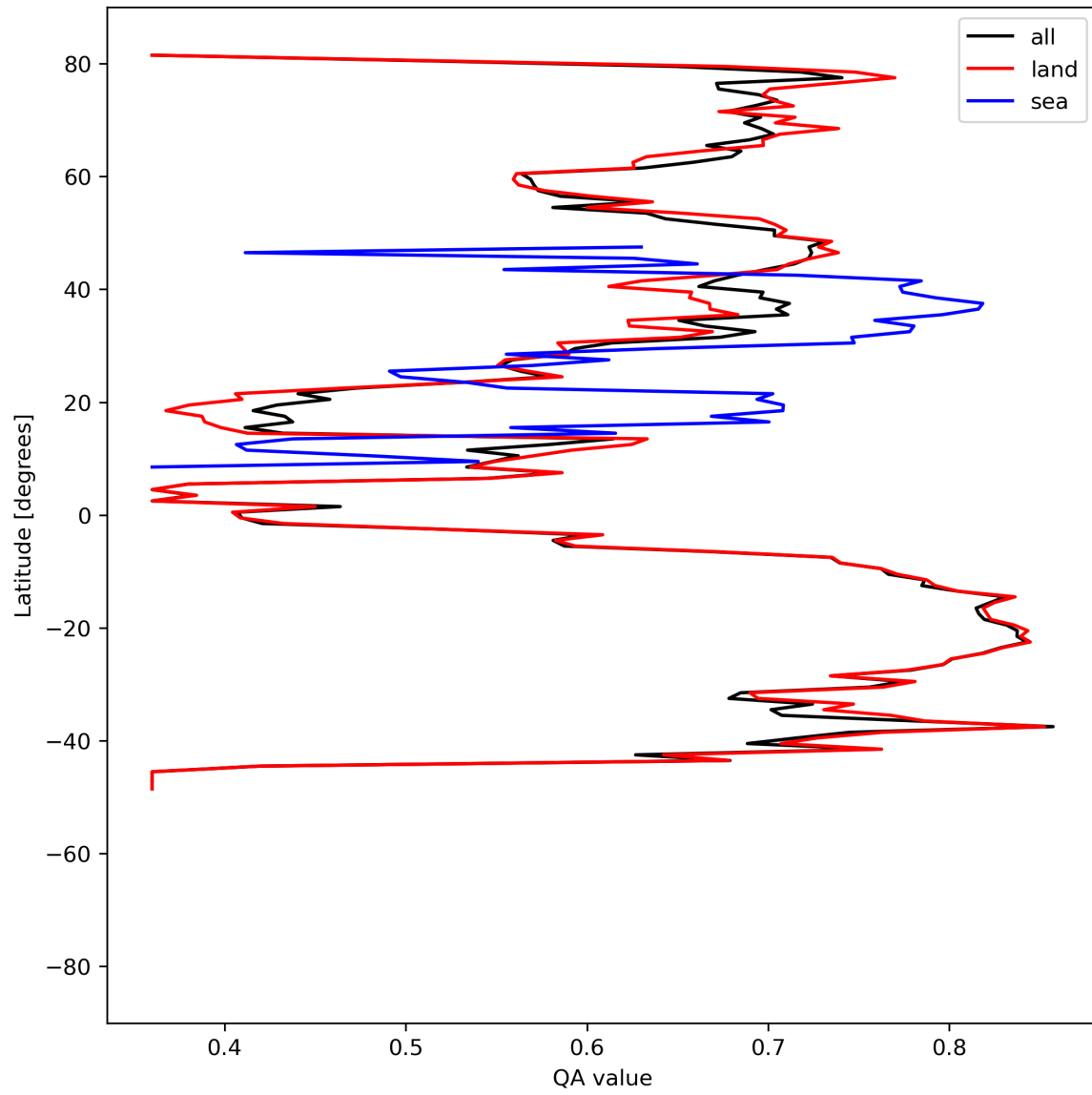
Figure 11: Zonal average of “QA value” for 2024-07-11 to 2024-07-13.
