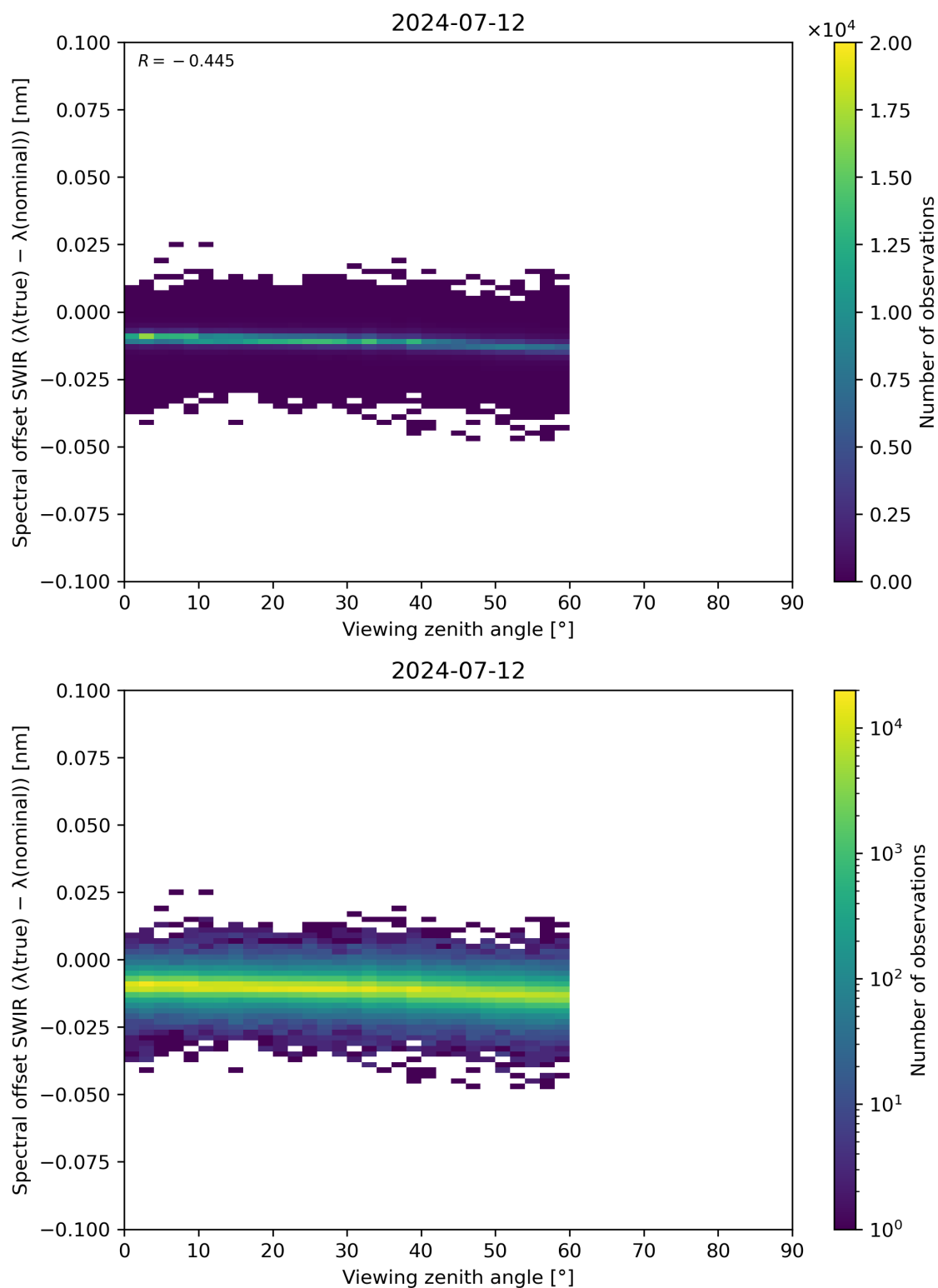
Figure 116: Scatter density plot of “Viewing zenith angle” against “Spectral offset SWIR ( \lambda(\text{true}) - \lambda(\text{nominal}) )” for 2024-07-11 to 2024-07-13.
