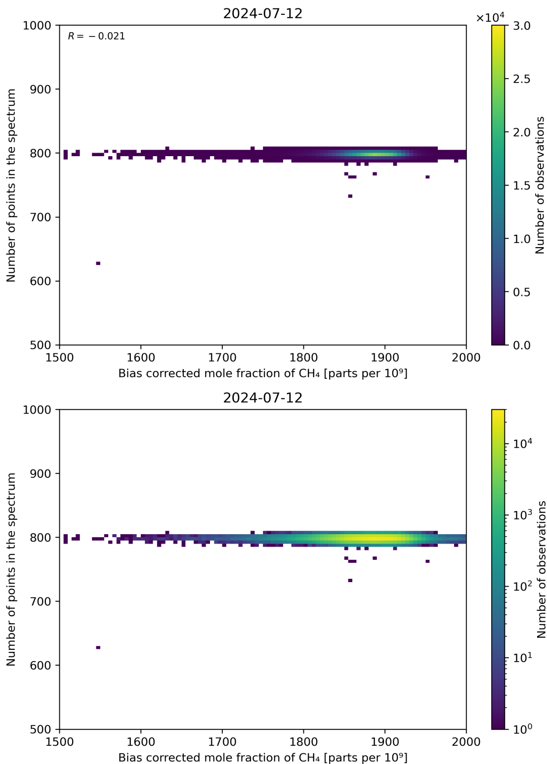
Figure 68: Scatter density plot of “Bias corrected mole fraction of CH 4 ” against “Number of points in the spectrum” for 2024-07-11 to 2024-07-13.
