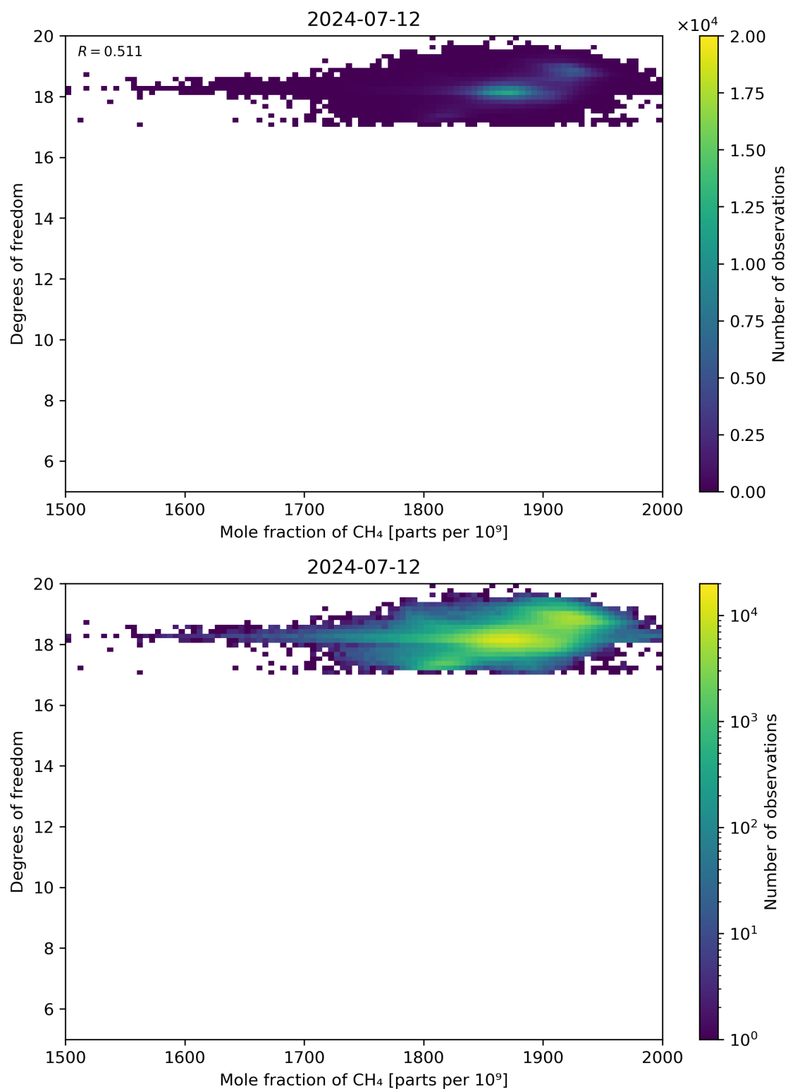
Figure 72: Scatter density plot of “Mole fraction of CH 4 ” against “Degrees of freedom” for 2024-07-11 to 2024-07-13.
