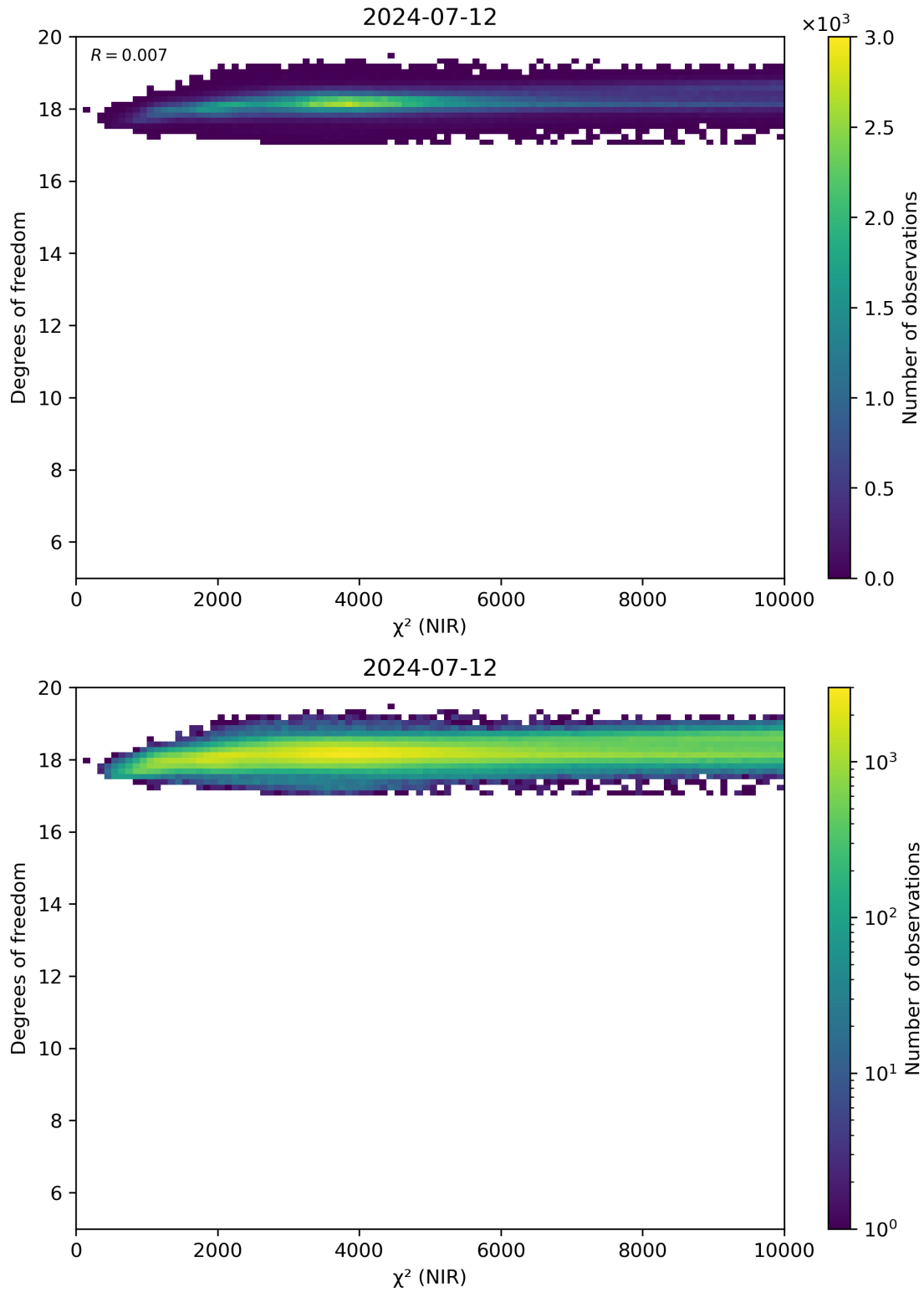
Figure 44: Scatter density plot of “ \chi^2 (NIR)” against “Degrees of freedom” for 2024-07-11 to 2024-07-13.
