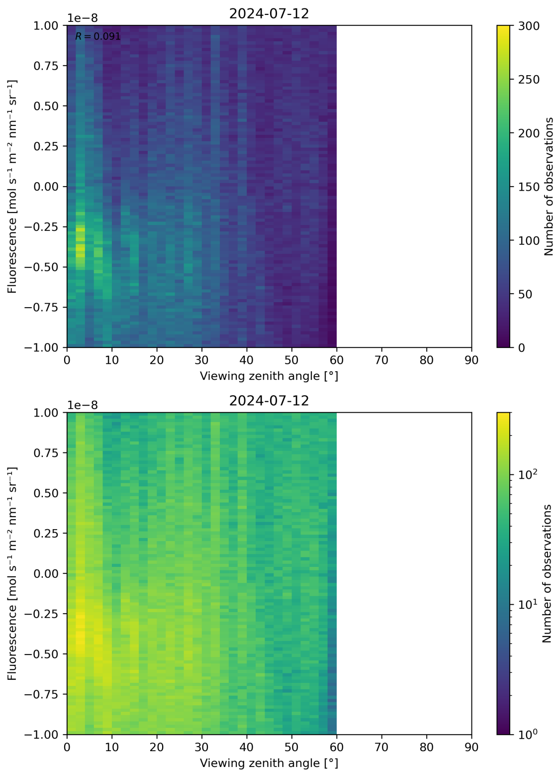
Figure 108: Scatter density plot of “Viewing zenith angle” against “Fluorescence” for 2024-07-11 to 2024-07-13.
