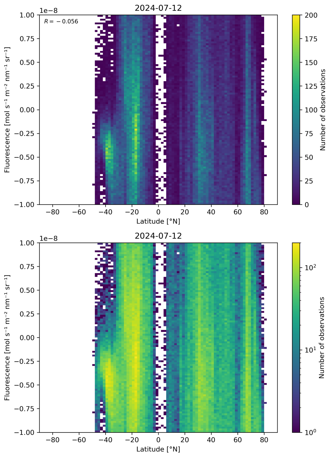
Figure 56: Scatter density plot of “Latitude” against “Fluorescence” for 2024-07-11 to 2024-07-13.
