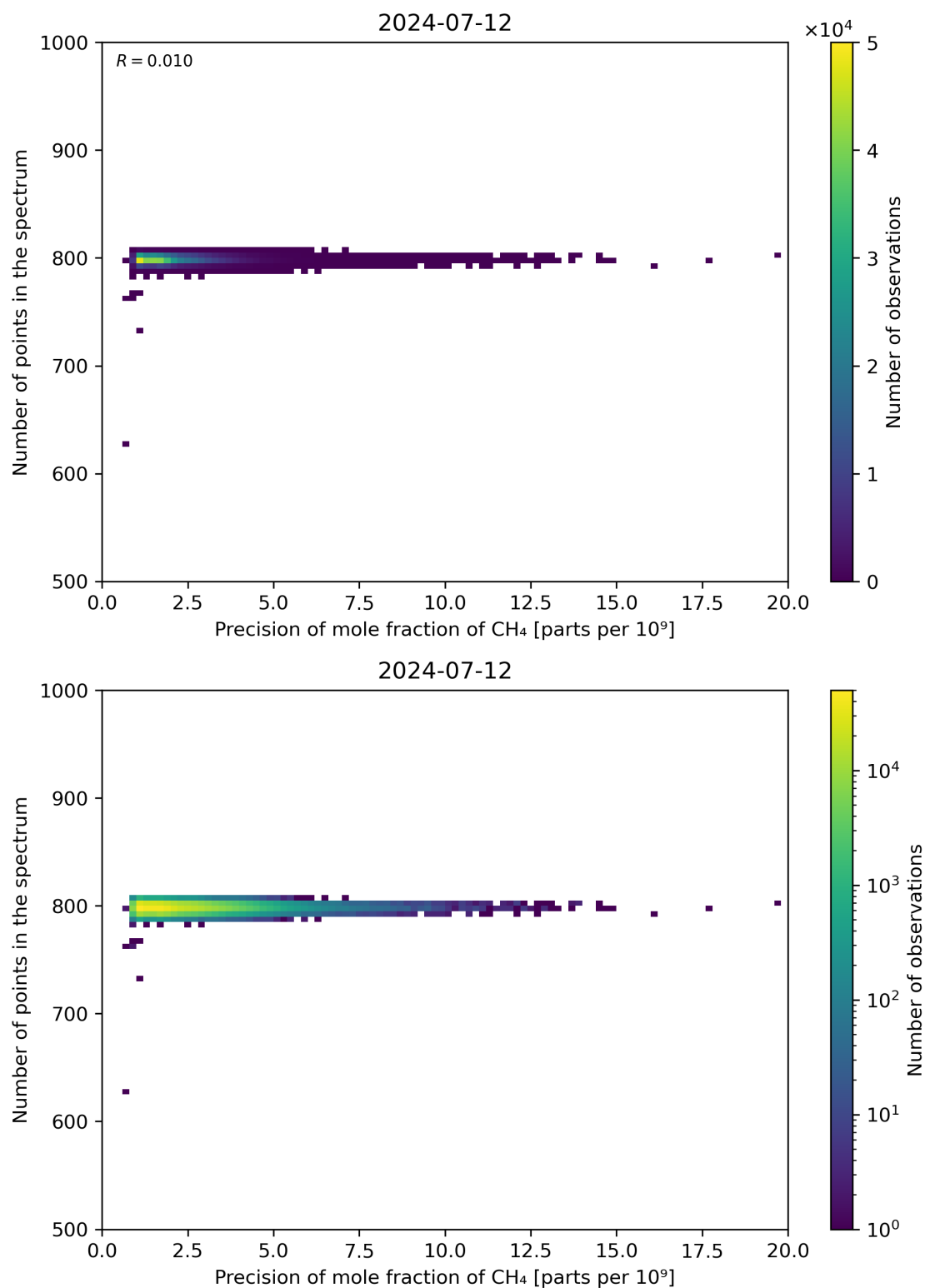
Figure 84: Scatter density plot of “Precision of mole fraction of \text{CH}_4 ” against “Number of points in the spectrum” for 2024-07-11 to 2024-07-13.
