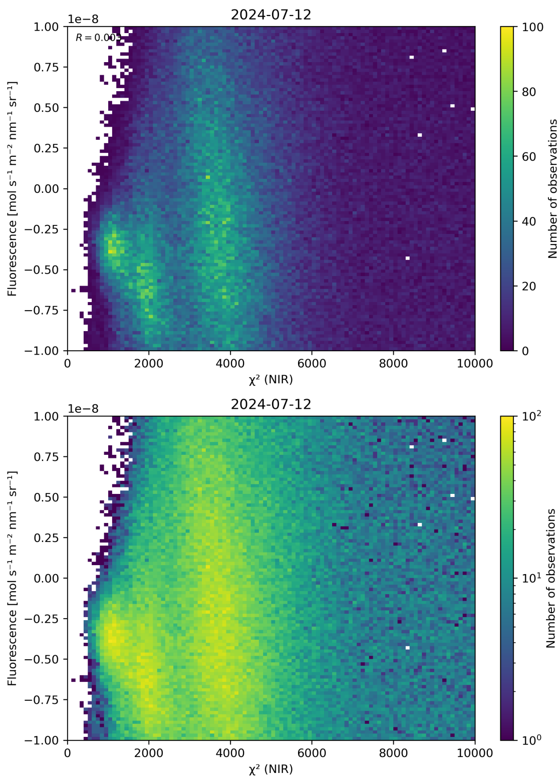
Figure 45: Scatter density plot of “ \chi^2 (NIR)” against “Fluorescence” for 2024-07-11 to 2024-07-13.
