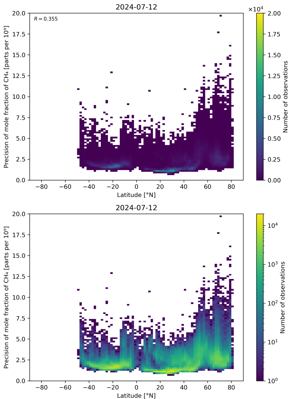
Figure 59: Scatter density plot of “Latitude” against “Precision of mole fraction of \text{CH}_4 ” for 2024-07-11 to 2024-07-13.
