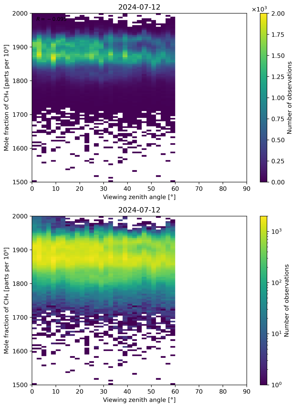
Figure 110: Scatter density plot of “Viewing zenith angle” against “Mole fraction of CH 4 ” for 2024-07-11 to 2024-07-13.
