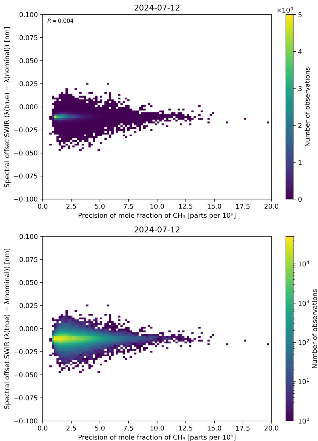
Figure 85: Scatter density plot of “Precision of mole fraction of CH 4 ” against “Spectral offset SWIR ( \lambda(\text{true}) - \lambda(\text{nominal}) )” for 2024-07-11 to 2024-07-13.
