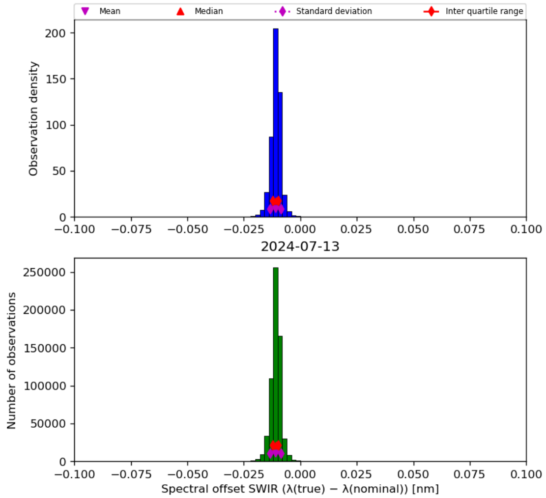
Figure 27: Histogram of “Spectral offset SWIR ( \lambda(\text{true}) - \lambda(\text{nominal}) )” for 2024-07-12 to 2024-07-14
