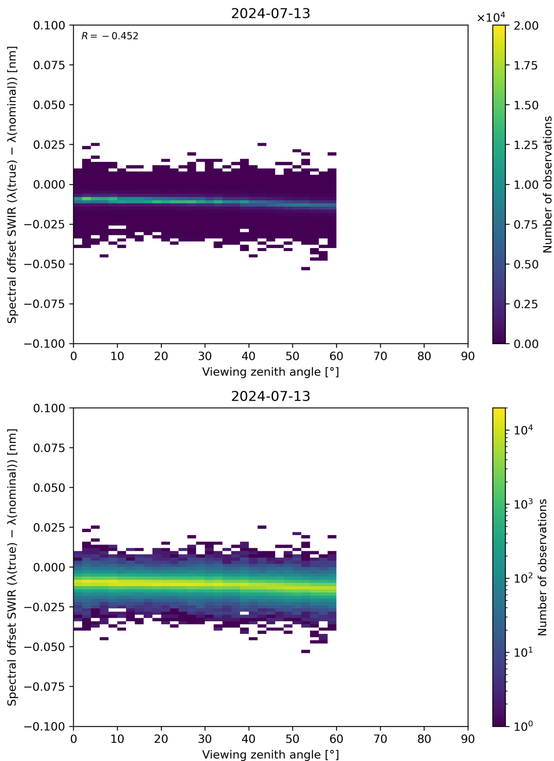
Figure 116: Scatter density plot of “Viewing zenith angle” against “Spectral offset SWIR ( \lambda(\text{true}) - \lambda(\text{nominal}) )” for 2024-07-12 to 2024-07-14.
