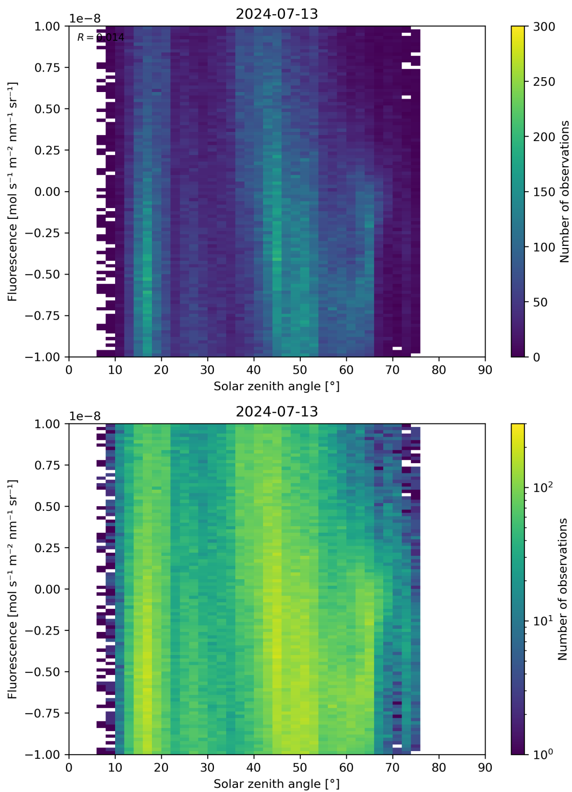
Figure 97: Scatter density plot of “Solar zenith angle” against “Fluorescence” for 2024-07-12 to 2024-07-14.
