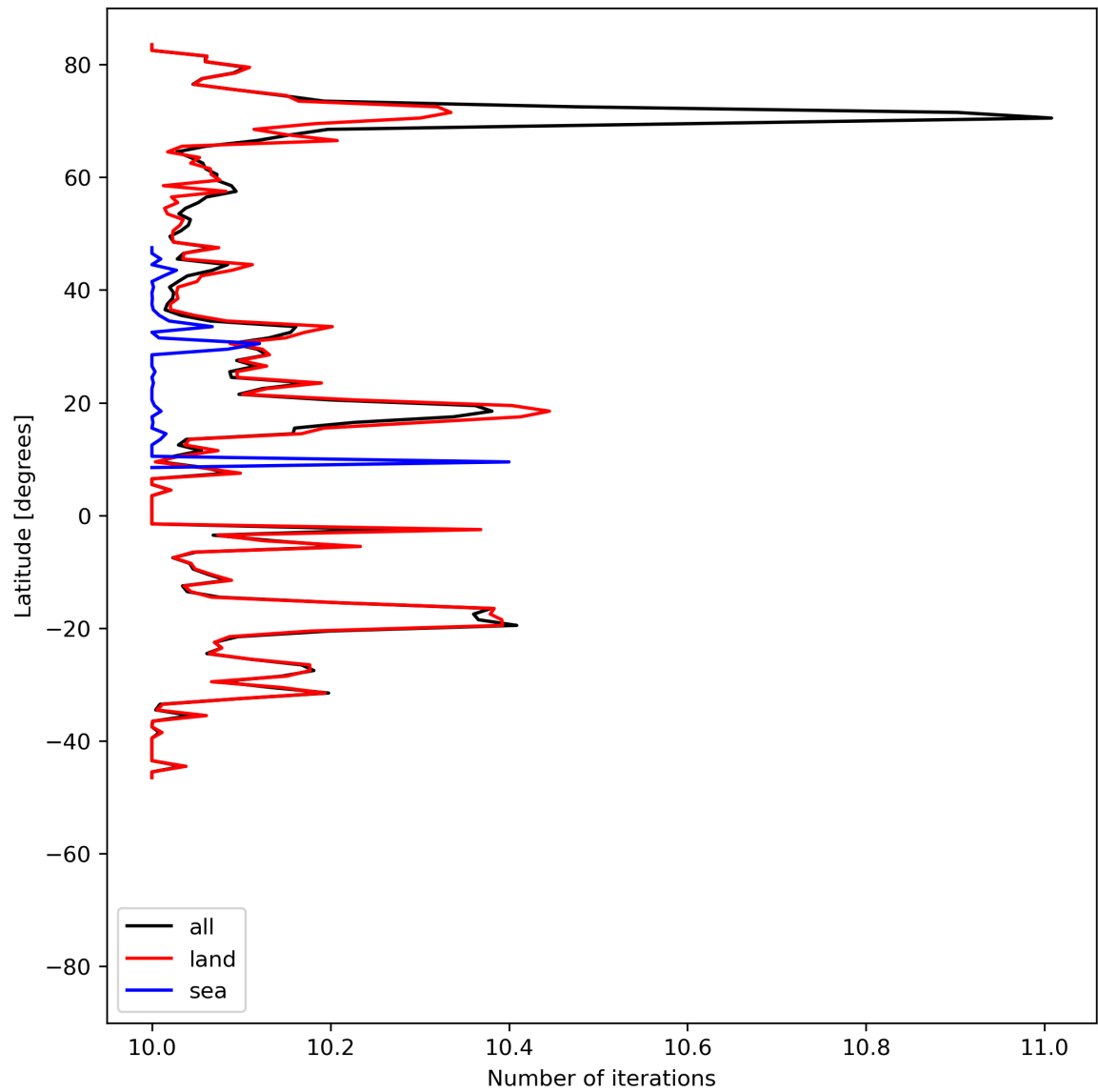
Figure 20: Zonal average of “Number of iterations” for 2024-07-12 to 2024-07-14.
