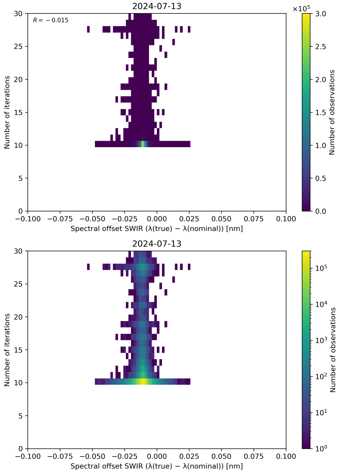
Figure 121: Scatter density plot of “Spectral offset SWIR ( \lambda(\text{true}) - \lambda(\text{nominal}) )” against “Number of iterations” for 2024-07-12 to 2024-07-14.
