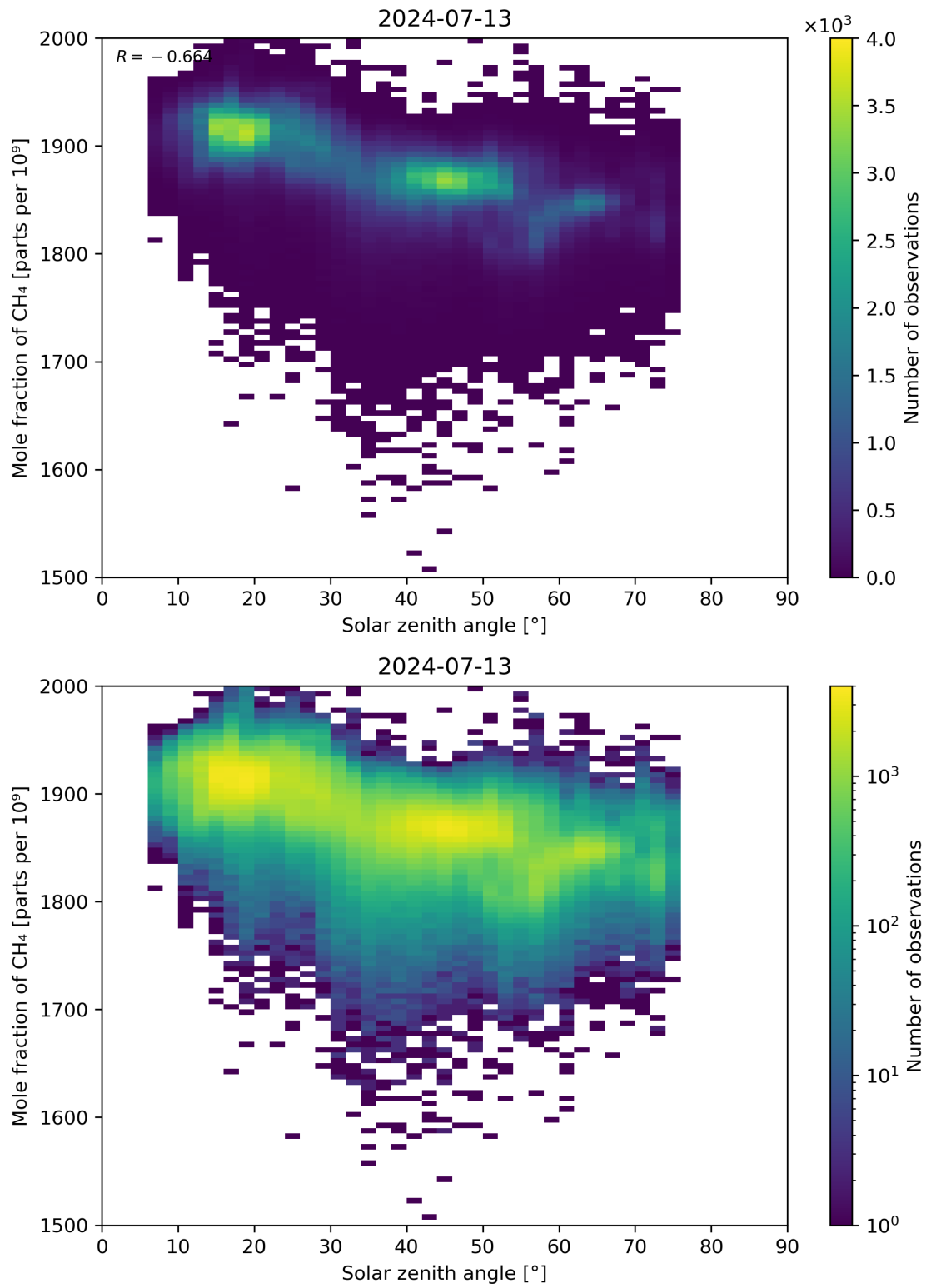
Figure 99: Scatter density plot of “Solar zenith angle” against “Mole fraction of CH 4 ” for 2024-07-12 to 2024-07-14.
