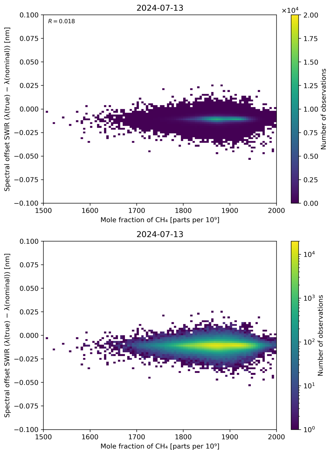
Figure 86: Scatter density plot of “Mole fraction of CH 4 ” against “Spectral offset SWIR ( \lambda(\text{true}) - \lambda(\text{nominal}) )” for 2024-07-12 to 2024-07-14.
