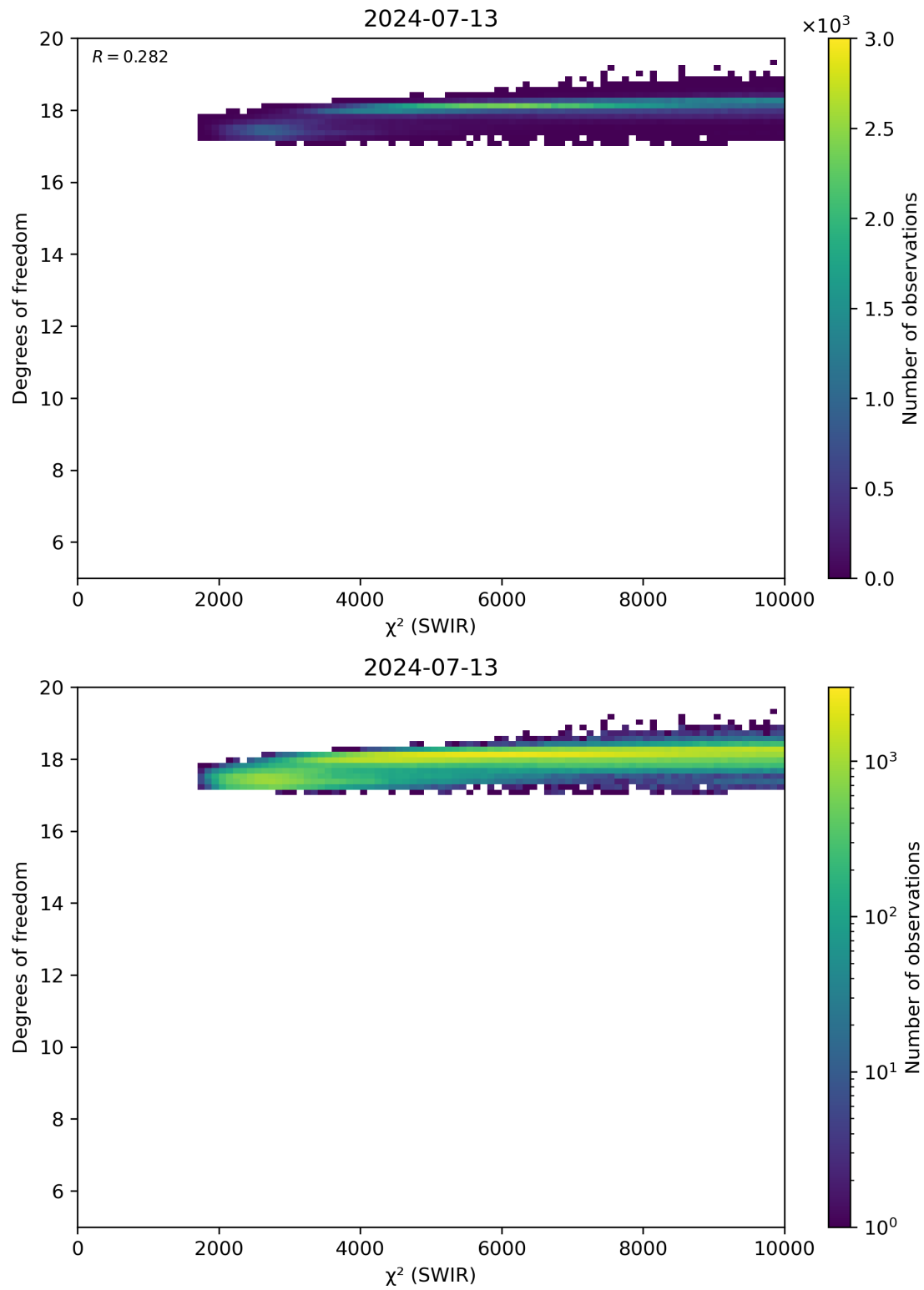
Figure 48: Scatter density plot of “ \chi^2 (SWIR)” against “Degrees of freedom” for 2024-07-12 to 2024-07-14.
