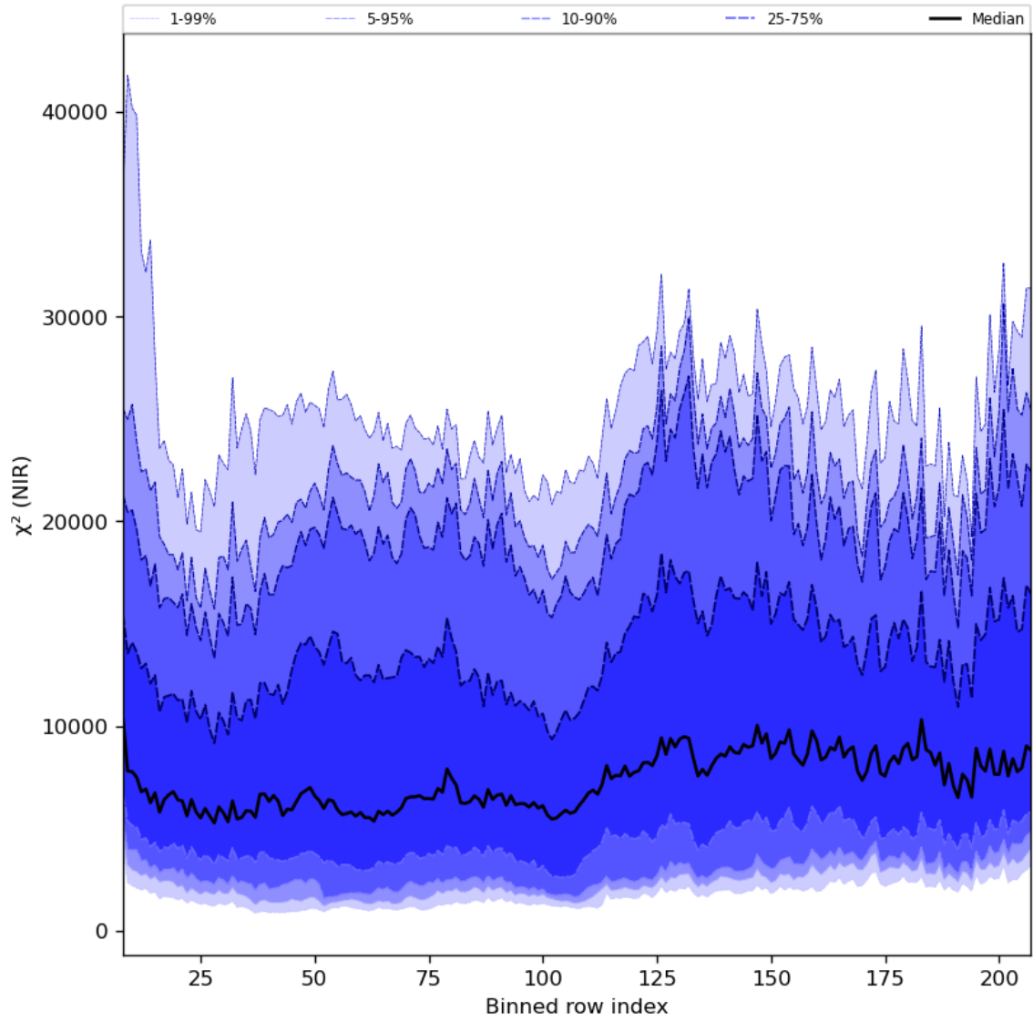
Figure 40: Along track statistics of “ \chi^2 (NIR)” for 2024-07-12 to 2024-07-14
