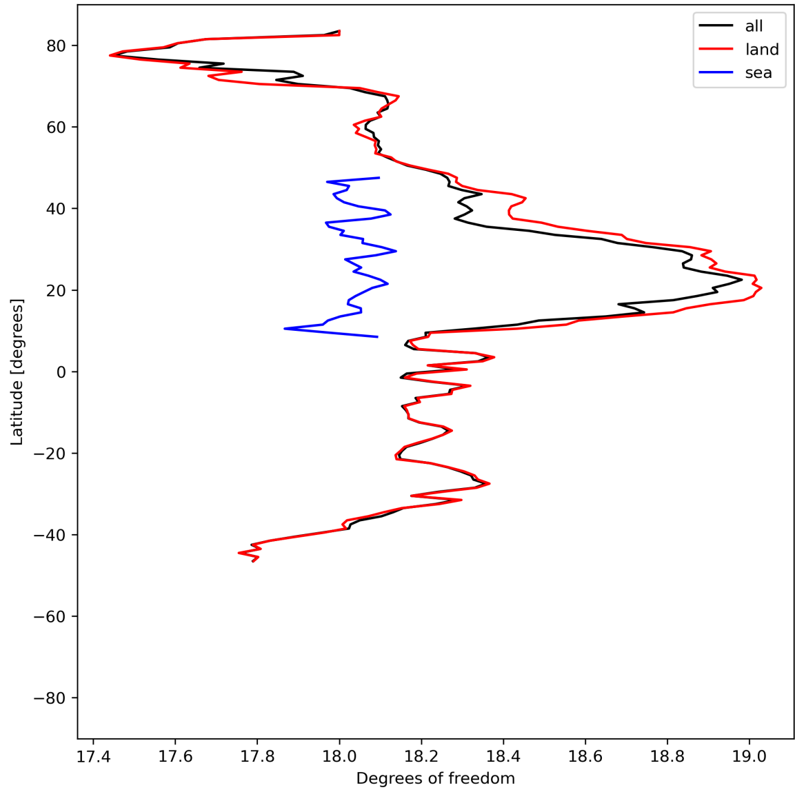
Figure 19: Zonal average of “Degrees of freedom” for 2024-07-12 to 2024-07-14.
