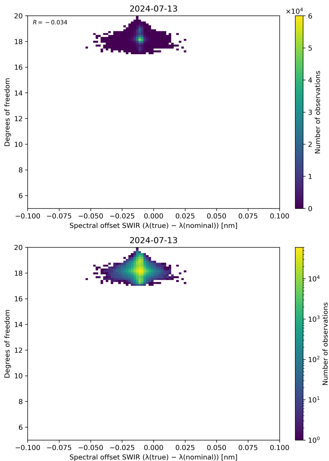
Figure 119: Scatter density plot of “Spectral offset SWIR ( \lambda(\text{true}) - \lambda(\text{nominal}) )” against “Degrees of freedom” for 2024-07-12 to 2024-07-14.
