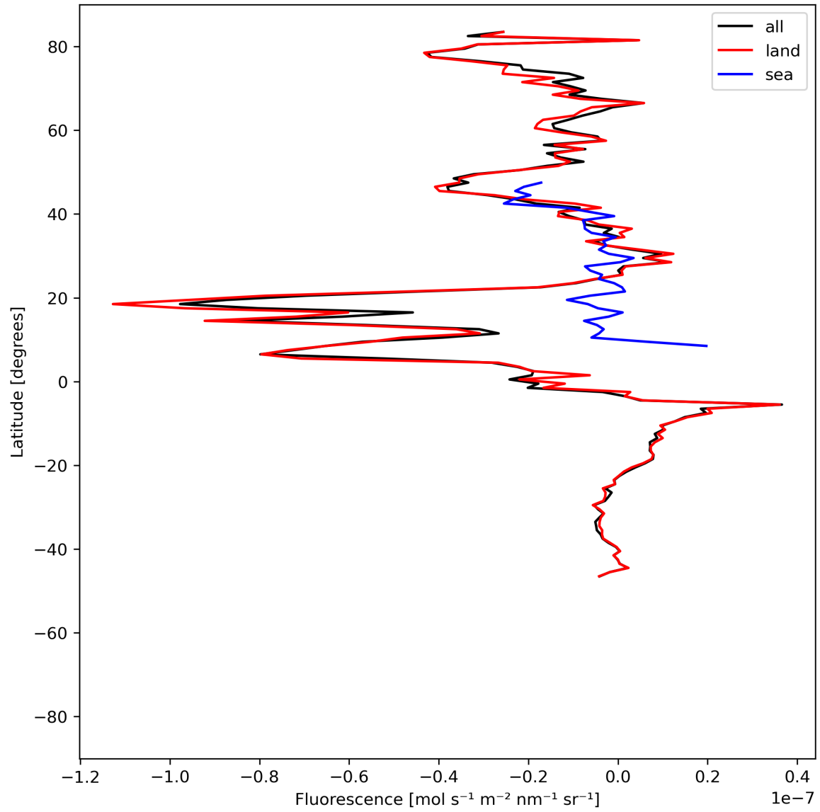
Figure 21: Zonal average of “Fluorescence” for 2024-07-12 to 2024-07-14.
