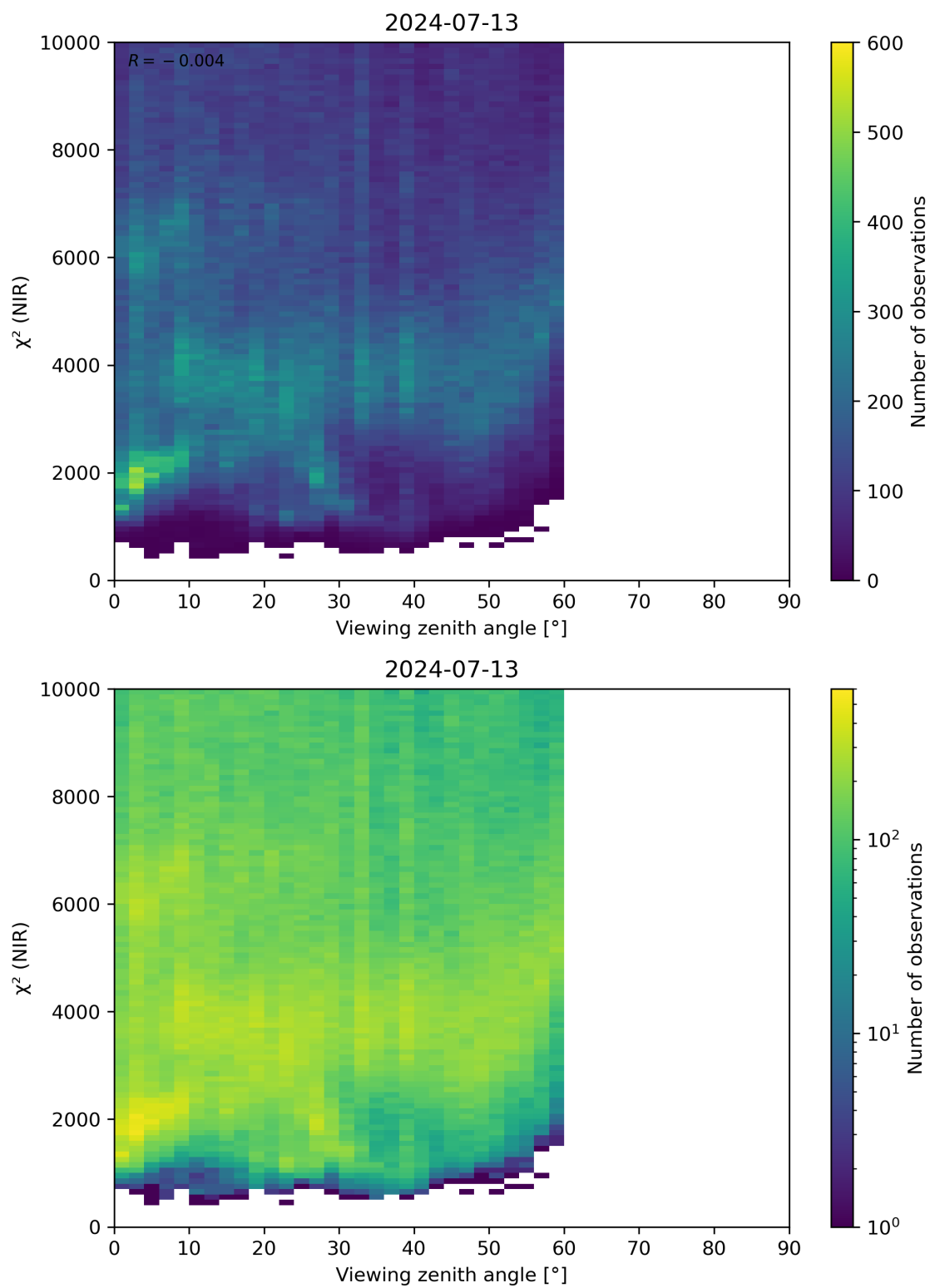
Figure 105: Scatter density plot of “Viewing zenith angle” against “ \chi^2 (NIR)” for 2024-07-12 to 2024-07-14.
