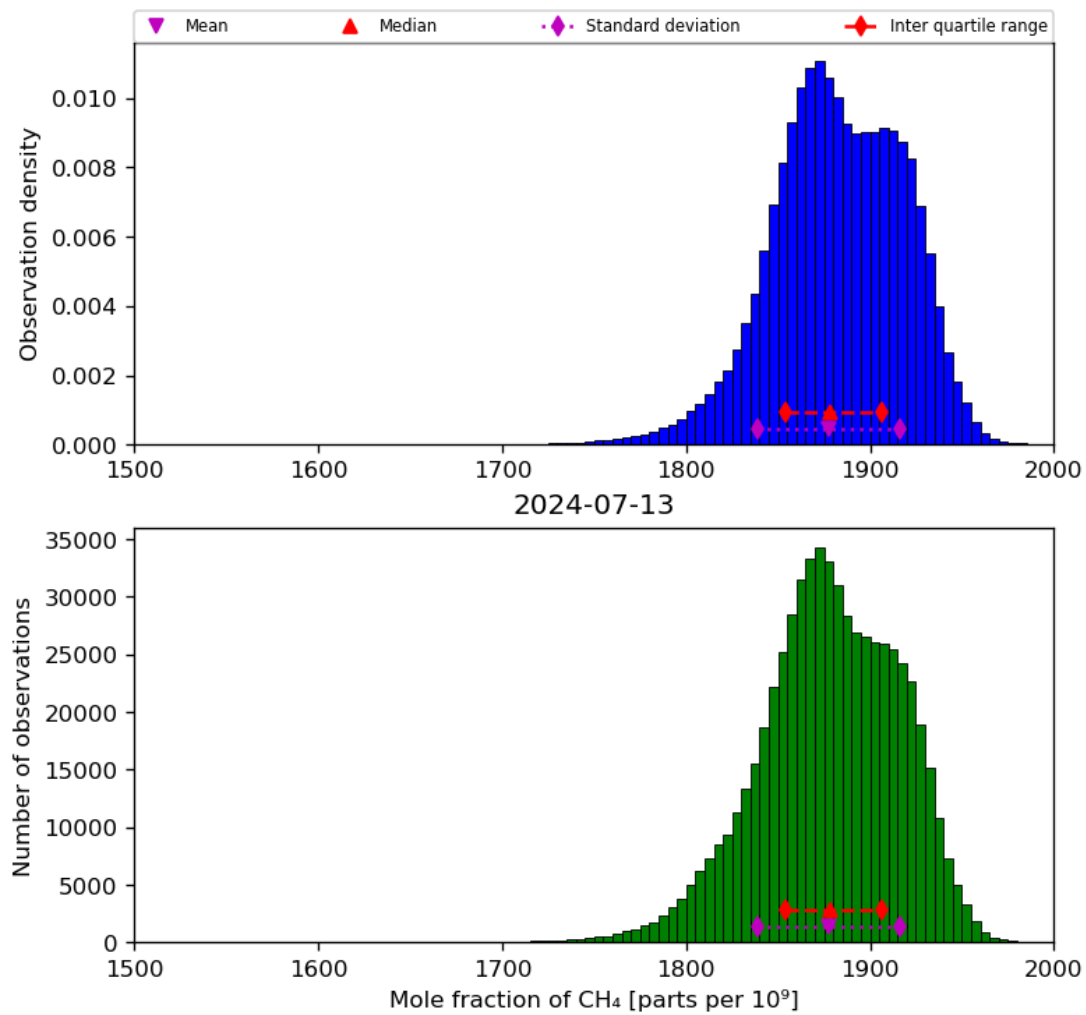
Figure 23: Histogram of “Mole fraction of CH 4 ” for 2024-07-12 to 2024-07-14
