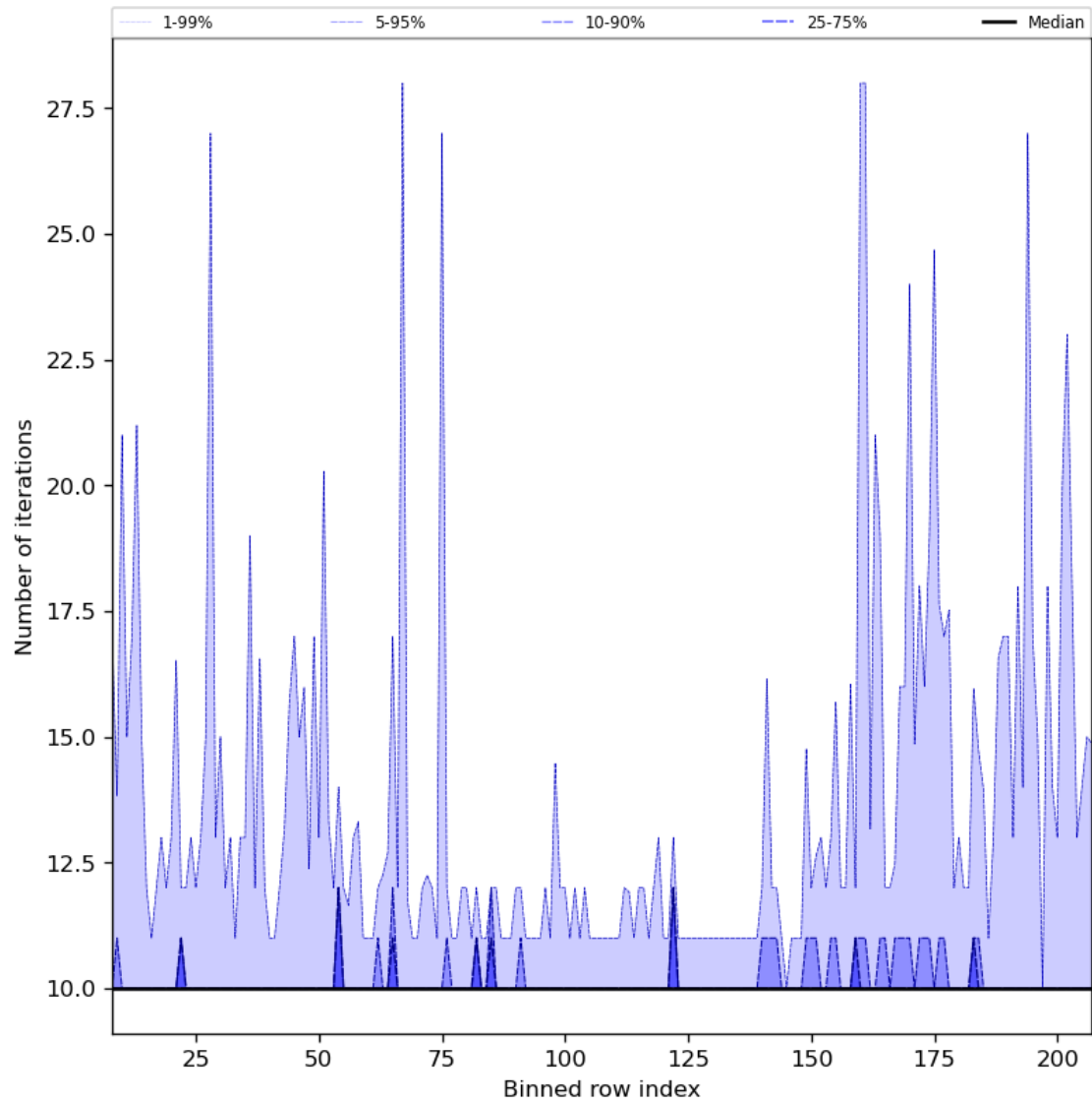
Figure 42: Along track statistics of “Number of iterations” for 2024-07-12 to 2024-07-14
