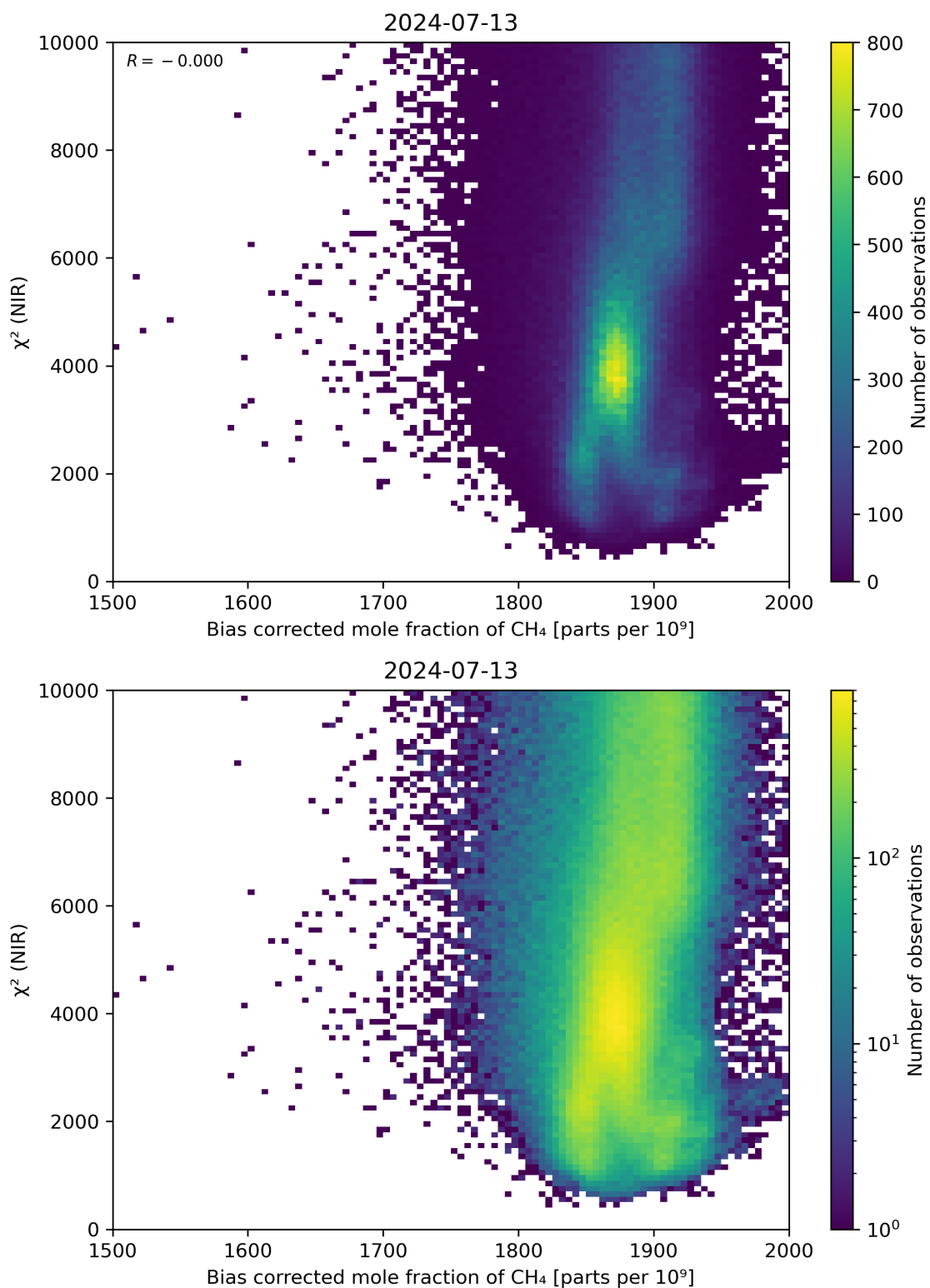
Figure 63: Scatter density plot of “Bias corrected mole fraction of CH 4 ” against “ \chi^2 (NIR)” for 2024-07-12 to 2024-07-14.
