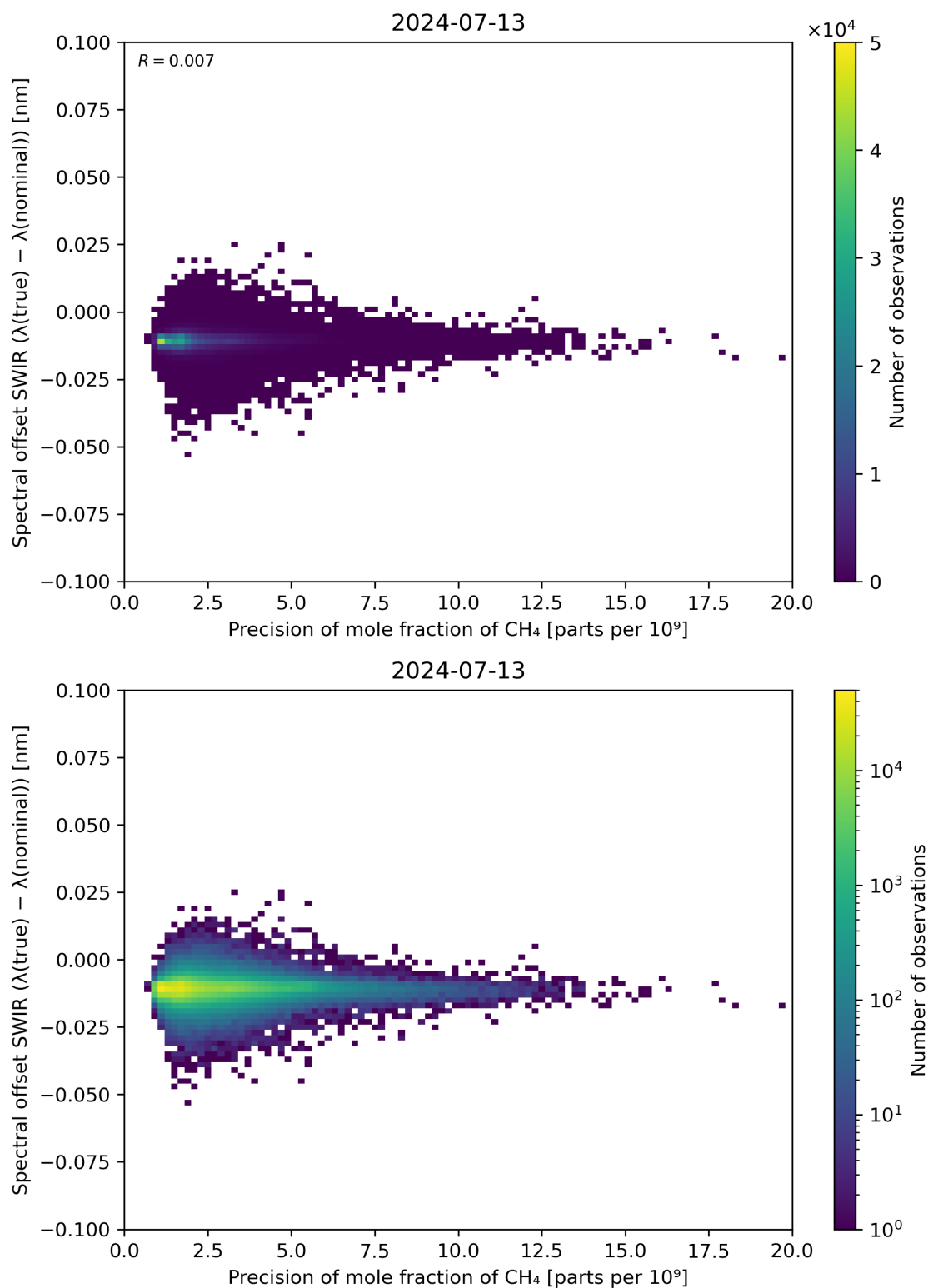
Figure 85: Scatter density plot of “Precision of mole fraction of CH 4 ” against “Spectral offset SWIR ( \lambda(\text{true}) - \lambda(\text{nominal}) )” for 2024-07-12 to 2024-07-14.
