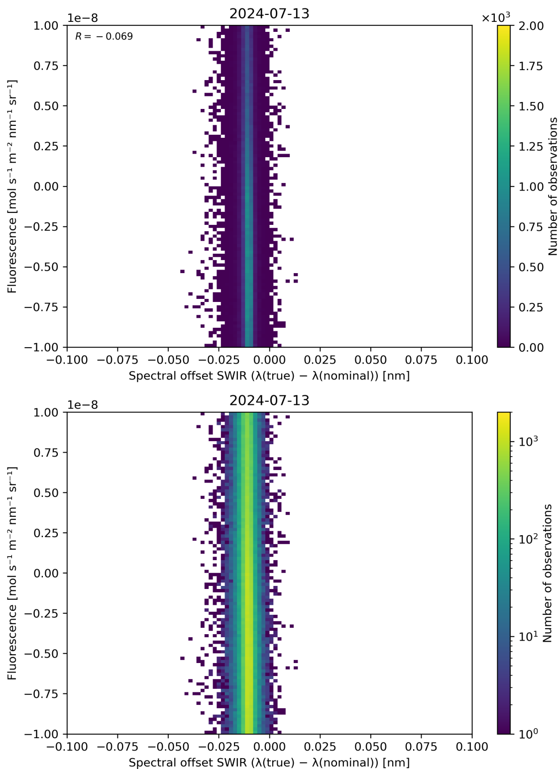
Figure 120: Scatter density plot of “Spectral offset SWIR ( \lambda(\text{true}) - \lambda(\text{nominal}) )” against “Fluorescence” for 2024-07-12 to 2024-07-14.
