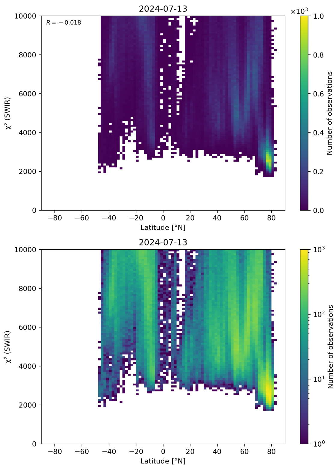
Figure 54: Scatter density plot of “Latitude” against “ \chi^2 (SWIR)” for 2024-07-12 to 2024-07-14.
