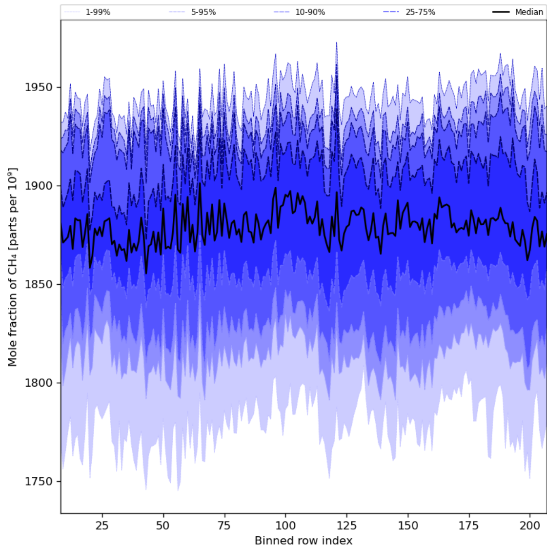
Figure 34: Along track statistics of “Mole fraction of CH 4 ” for 2024-07-12 to 2024-07-14
