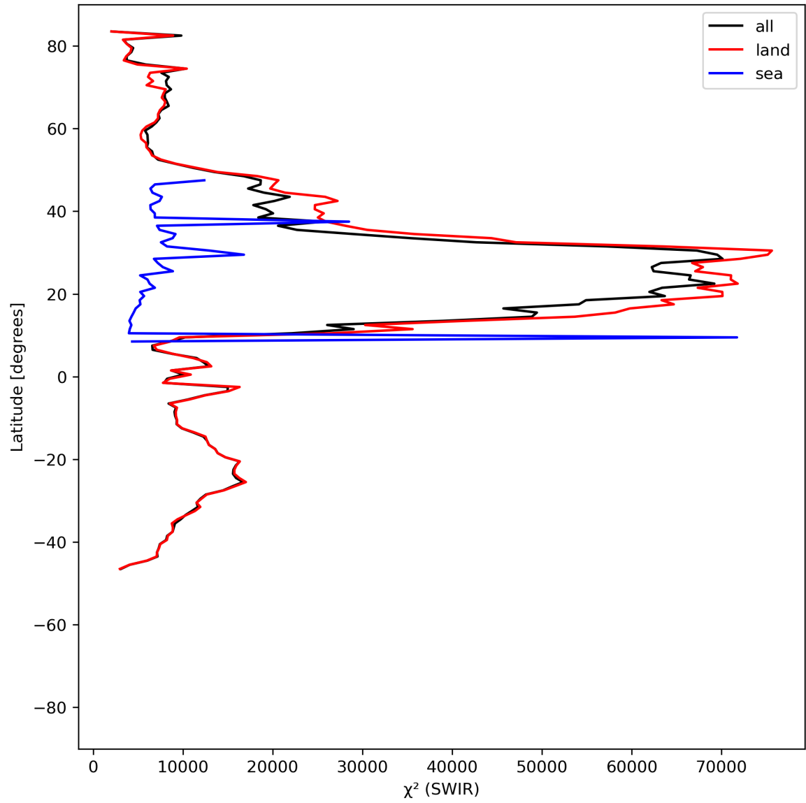
Figure 17: Zonal average of “ \chi^2 (SWIR)” for 2024-07-12 to 2024-07-14.
