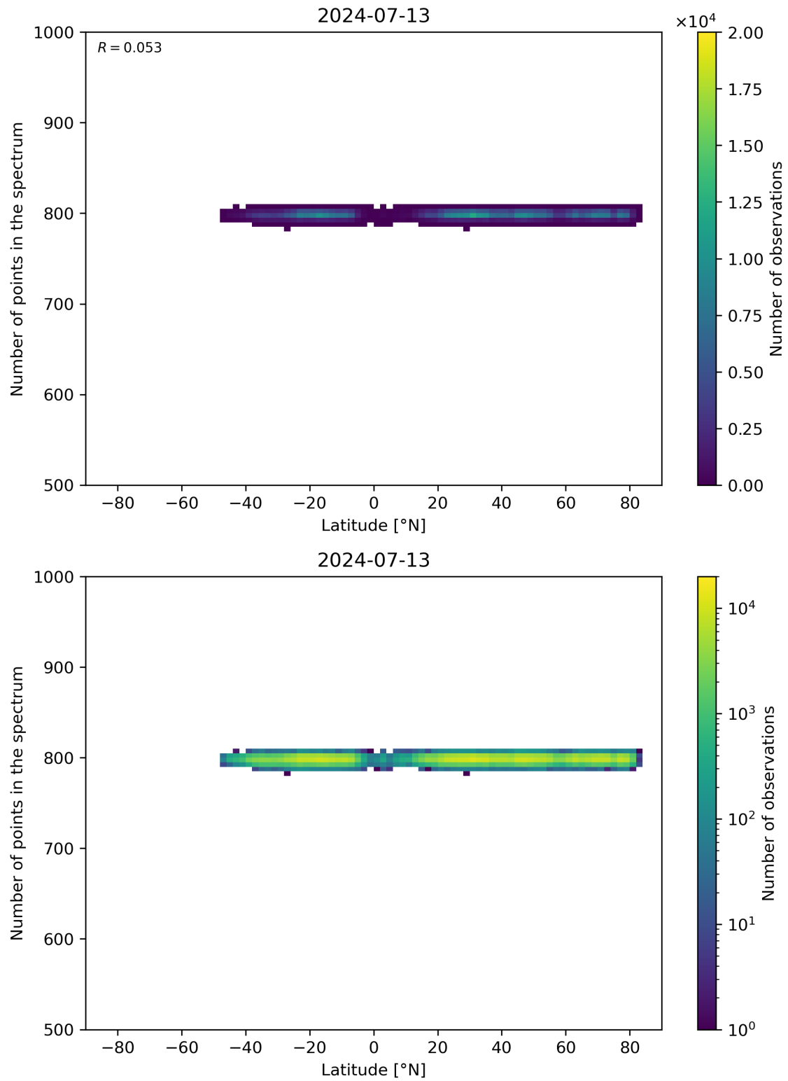
Figure 61: Scatter density plot of “Latitude” against “Number of points in the spectrum” for 2024-07-12 to 2024-07-14.
