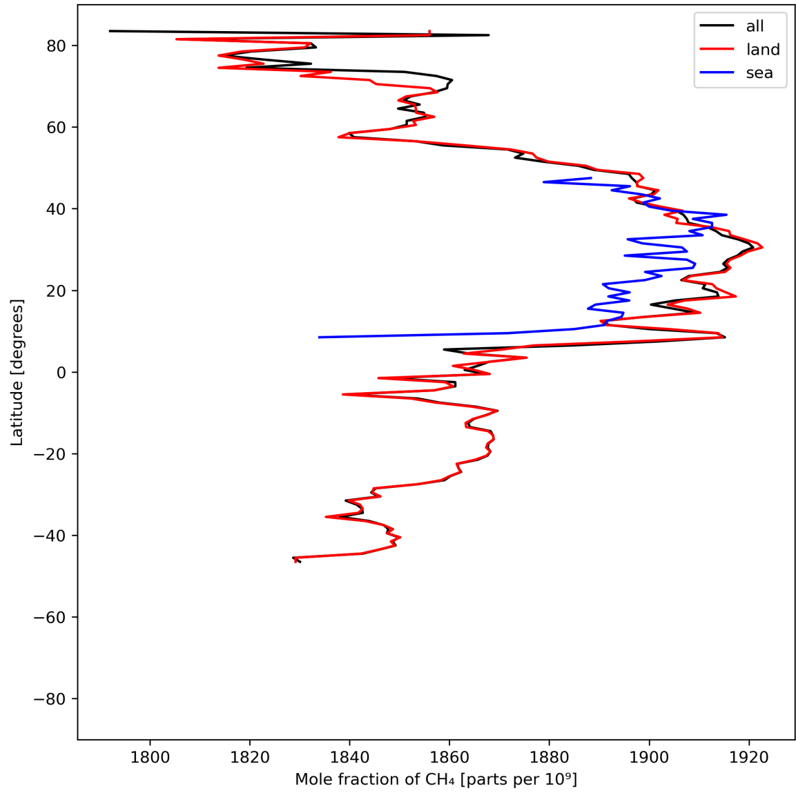
Figure 12: Zonal average of “Mole fraction of \text{CH}_4 ” for 2024-07-12 to 2024-07-14.
