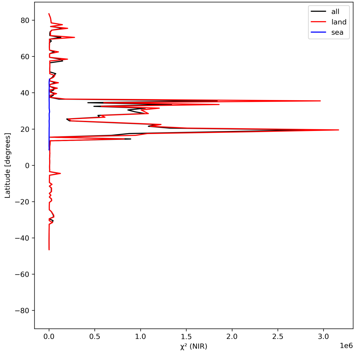
Figure 18: Zonal average of “ \chi^2 (NIR)” for 2024-07-12 to 2024-07-14.
