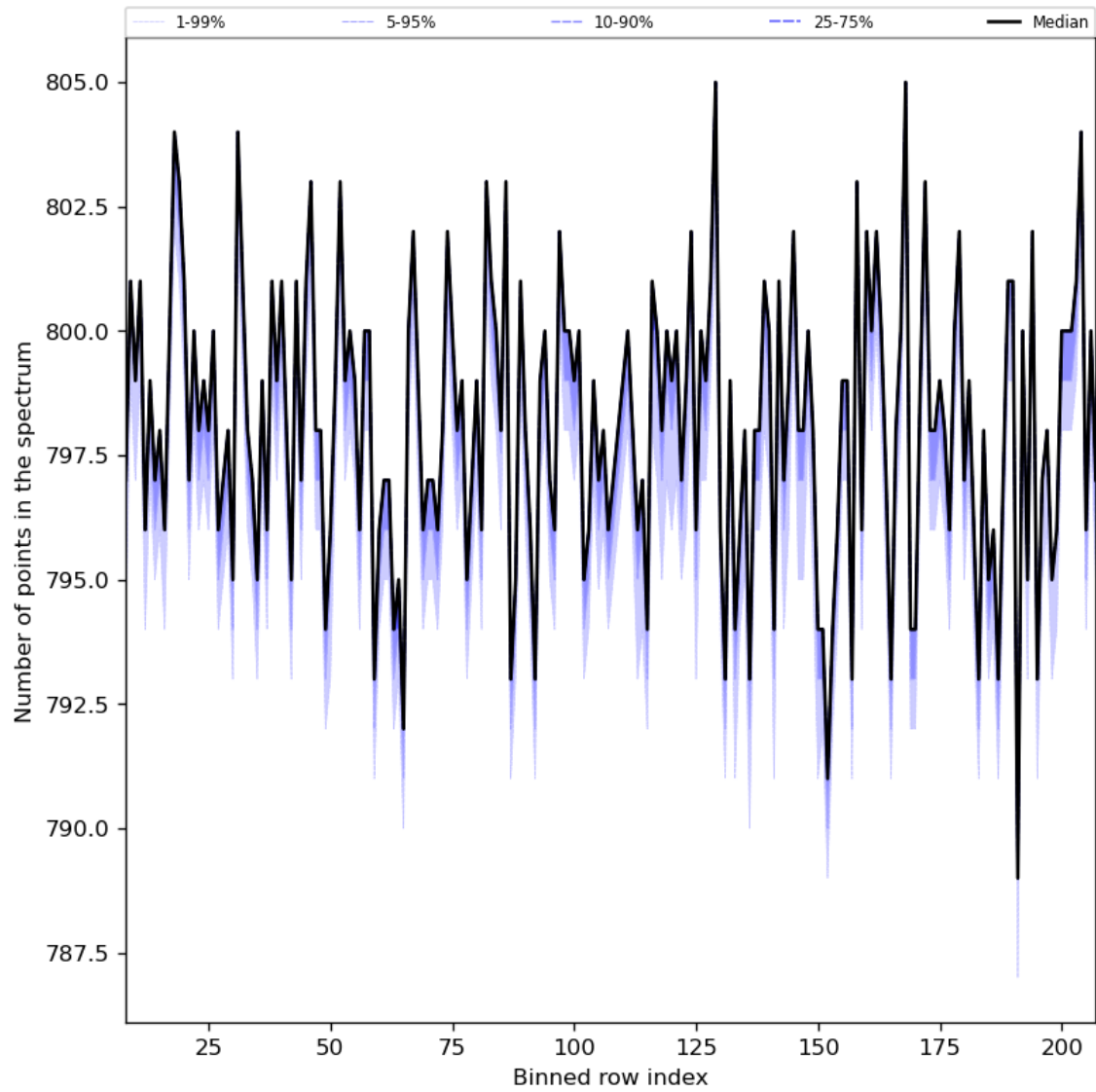
Figure 37: Along track statistics of “Number of points in the spectrum” for 2024-07-12 to 2024-07-14
