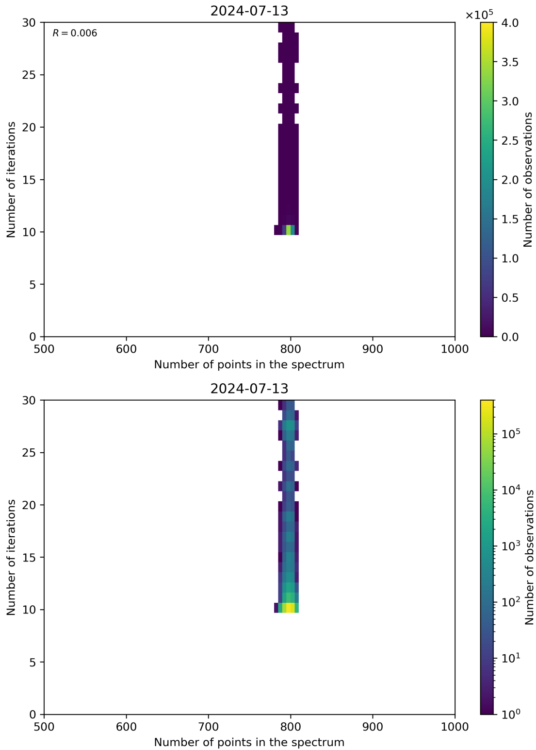
Figure 92: Scatter density plot of “Number of points in the spectrum” against “Number of iterations” for 2024-07-12 to 2024-07-14.
