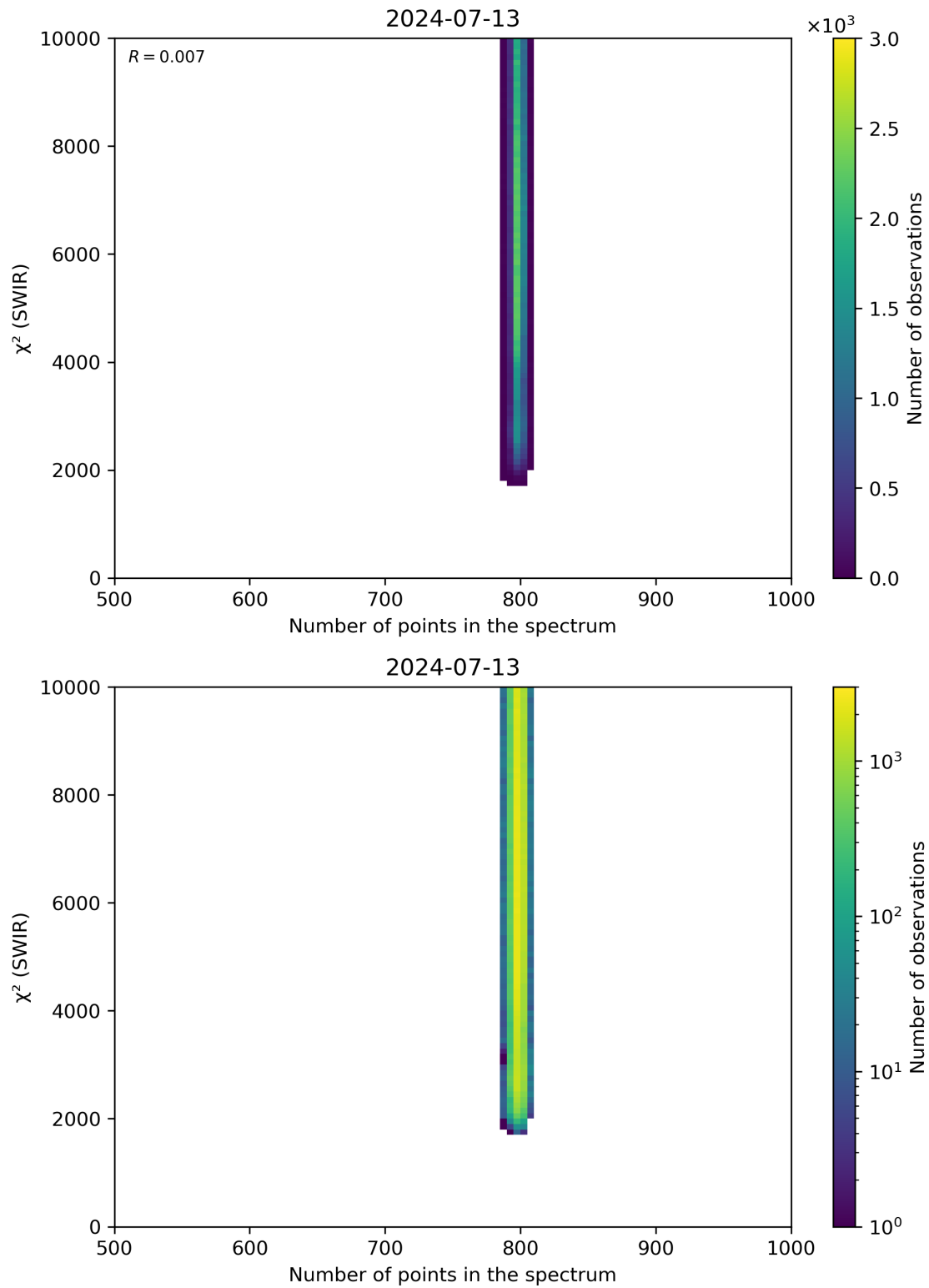
Figure 89: Scatter density plot of “Number of points in the spectrum” against “ \chi^2 (SWIR)” for 2024-07-12 to 2024-07-14.
