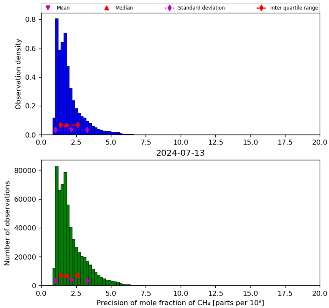
Figure 24: Histogram of “Precision of mole fraction of CH 4 ” for 2024-07-12 to 2024-07-14
