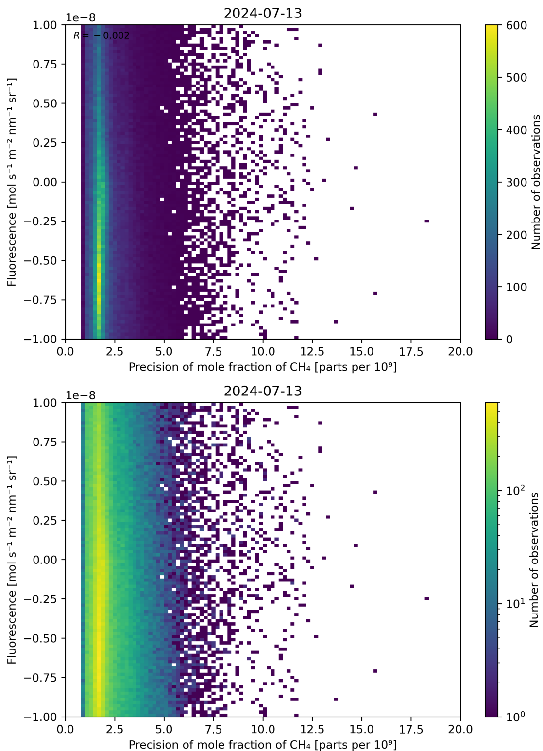
Figure 81: Scatter density plot of “Precision of mole fraction of \text{CH}_4 ” against “Fluorescence” for 2024-07-12 to 2024-07-14.
