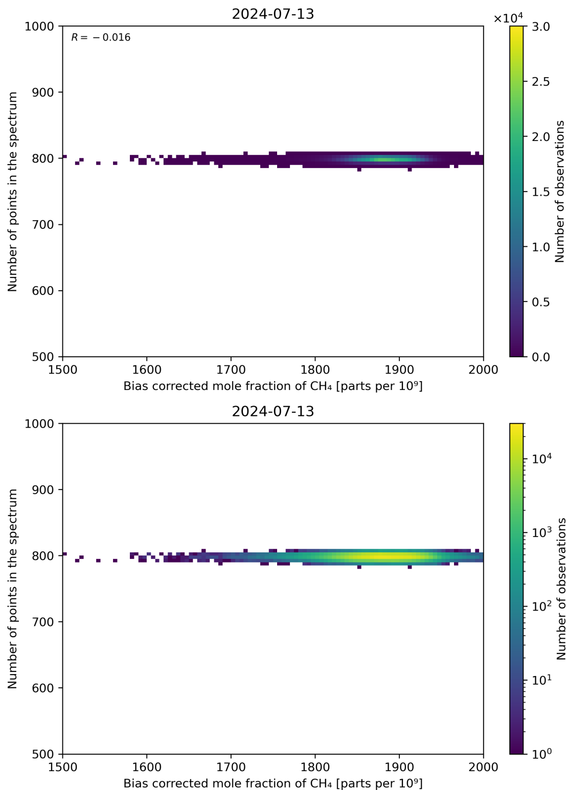
Figure 68: Scatter density plot of “Bias corrected mole fraction of CH 4 ” against “Number of points in the spectrum” for 2024-07-12 to 2024-07-14.
