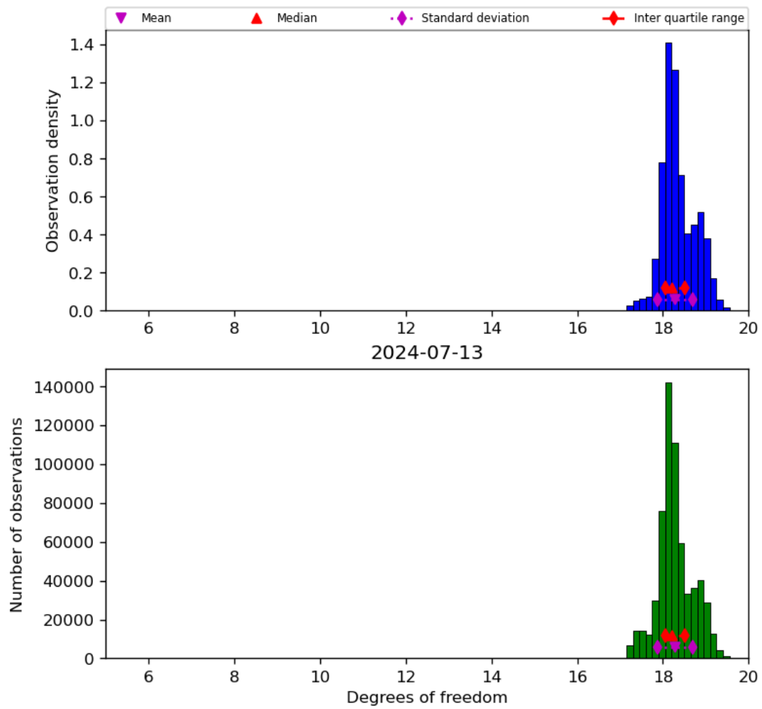
Figure 30: Histogram of “Degrees of freedom” for 2024-07-12 to 2024-07-14
