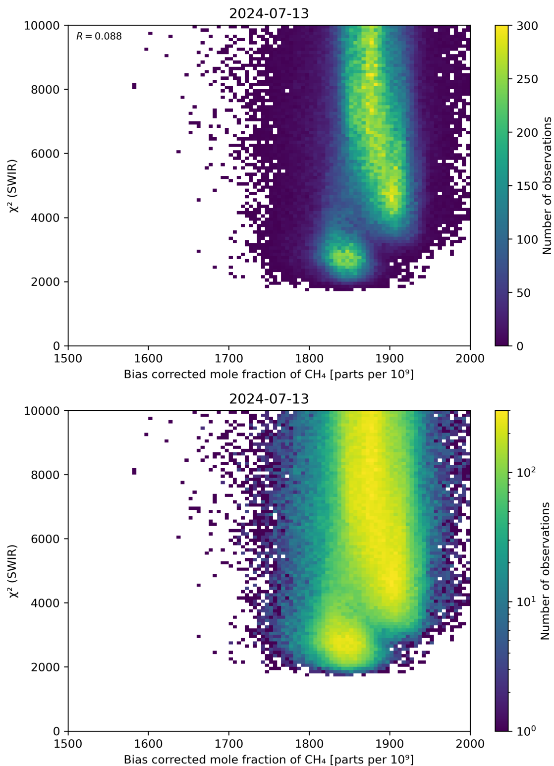
Figure 64: Scatter density plot of “Bias corrected mole fraction of CH 4 ” against “ \chi^2 (SWIR)” for 2024-07-12 to 2024-07-14.
