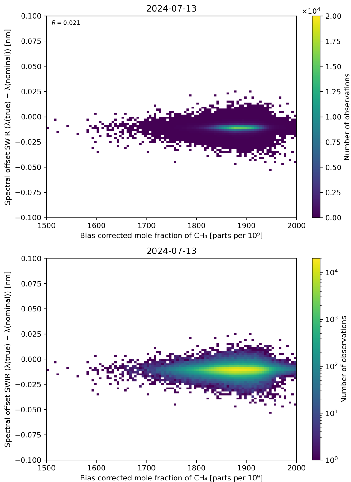
Figure 69: Scatter density plot of “Bias corrected mole fraction of \text{CH}_4 ” against “Spectral offset SWIR ( \lambda(\text{true}) - \lambda(\text{nominal}) )” for 2024-07-12 to 2024-07-14.
