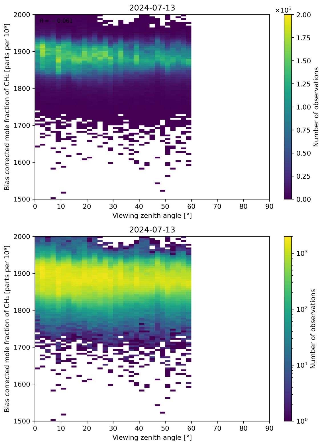
Figure 111: Scatter density plot of “Viewing zenith angle” against “Bias corrected mole fraction of CH 4 ” for 2024-07-12 to 2024-07-14.
