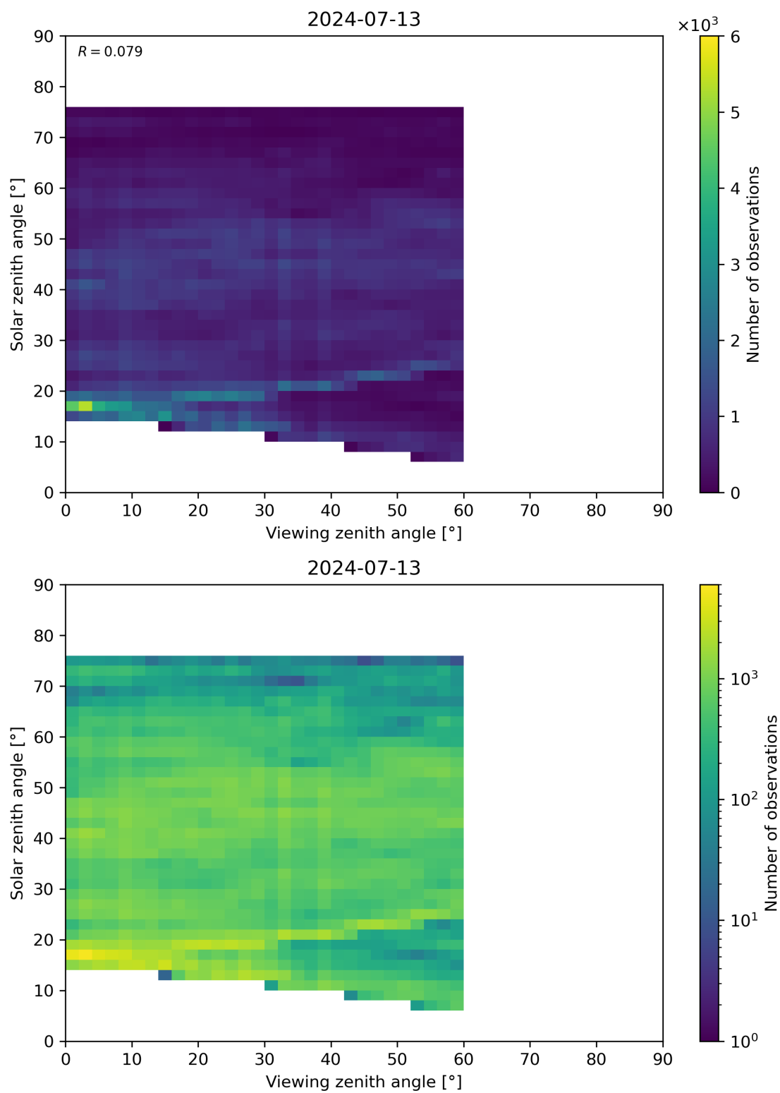
Figure 115: Scatter density plot of “Viewing zenith angle” against “Solar zenith angle” for 2024-07-12 to 2024-07-14.
