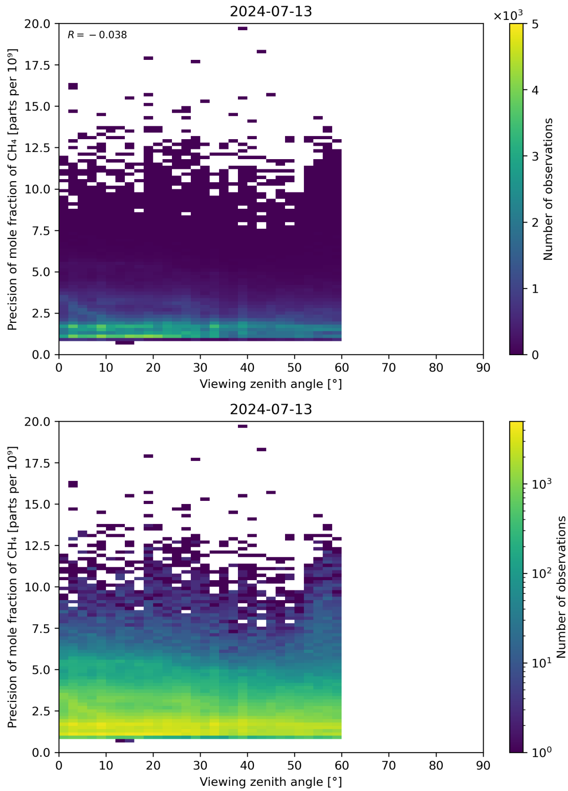
Figure 112: Scatter density plot of “Viewing zenith angle” against “Precision of mole fraction of \text{CH}_4 ” for 2024-07-12 to 2024-07-14.
