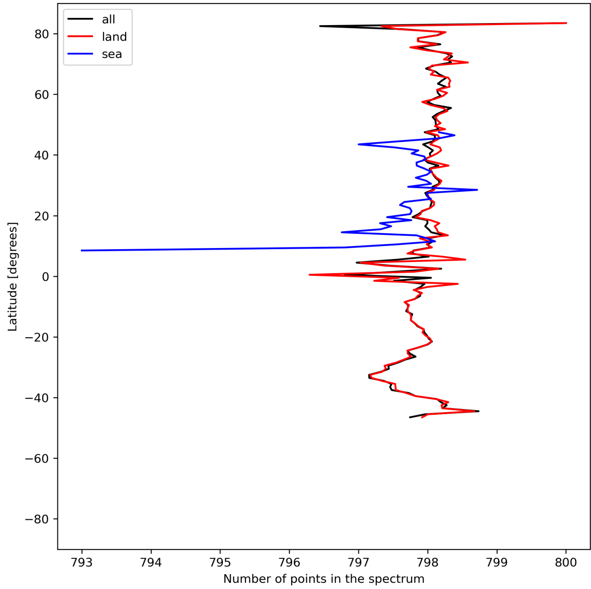
Figure 15: Zonal average of “Number of points in the spectrum” for 2024-07-12 to 2024-07-14.
