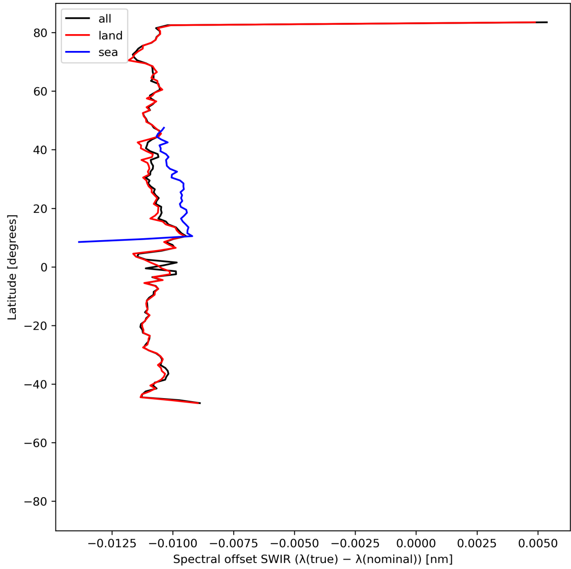
Figure 16: Zonal average of “Spectral offset SWIR ( \lambda(\text{true}) - \lambda(\text{nominal}) )” for 2024-07-12 to 2024-07-14.
