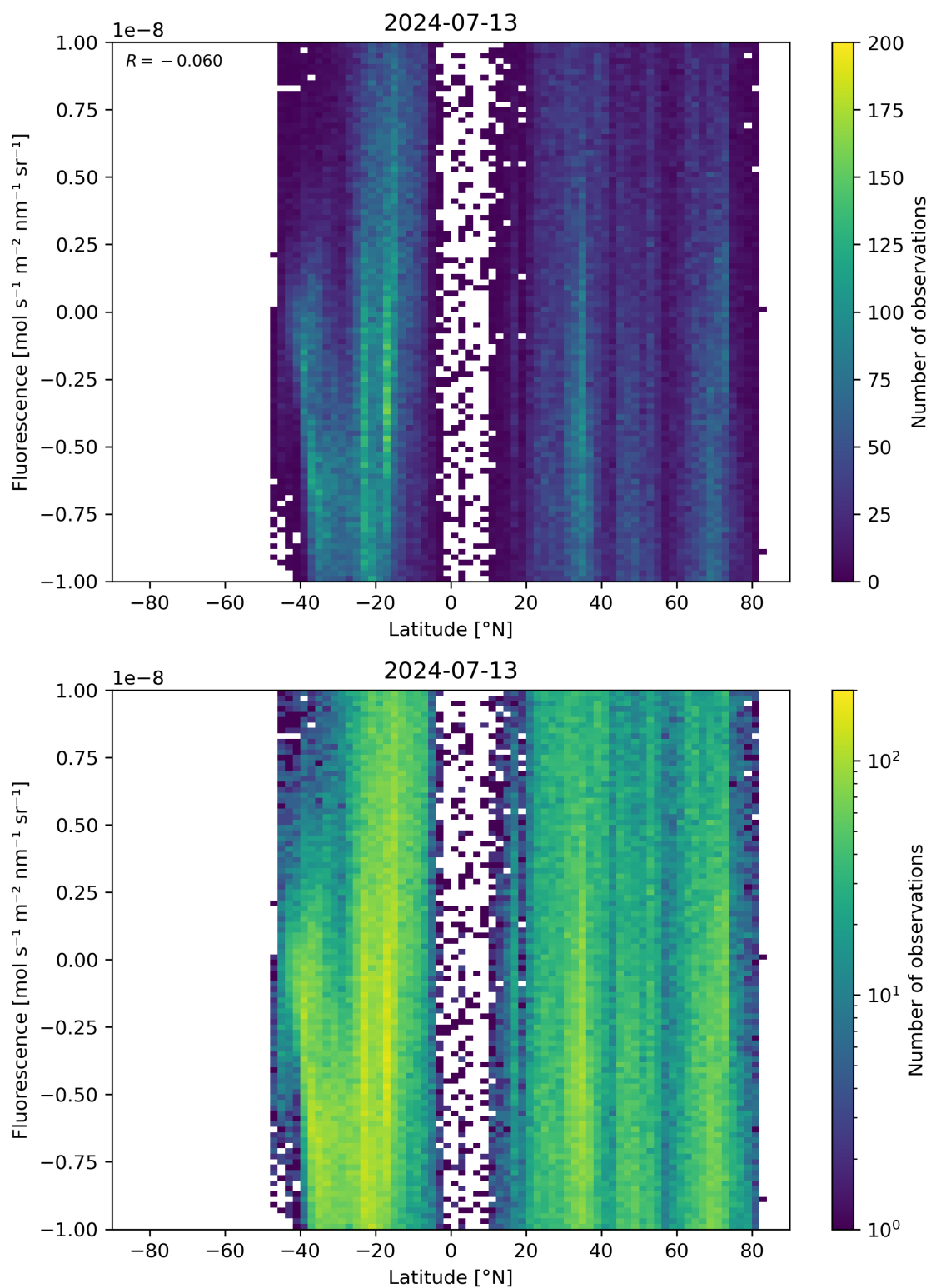
Figure 56: Scatter density plot of “Latitude” against “Fluorescence” for 2024-07-12 to 2024-07-14.
