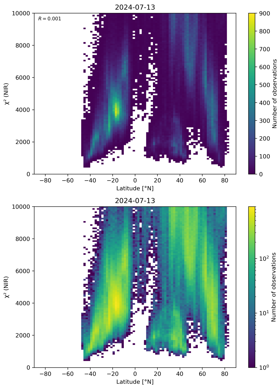
Figure 53: Scatter density plot of “Latitude” against “ \chi^2 (NIR)” for 2024-07-12 to 2024-07-14.
