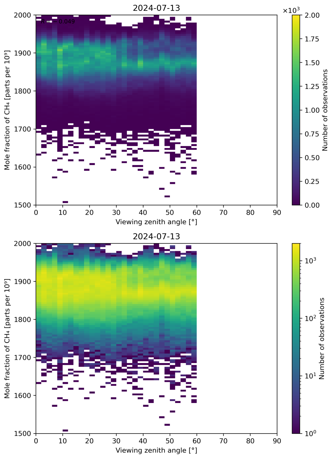
Figure 110: Scatter density plot of “Viewing zenith angle” against “Mole fraction of CH 4 ” for 2024-07-12 to 2024-07-14.
