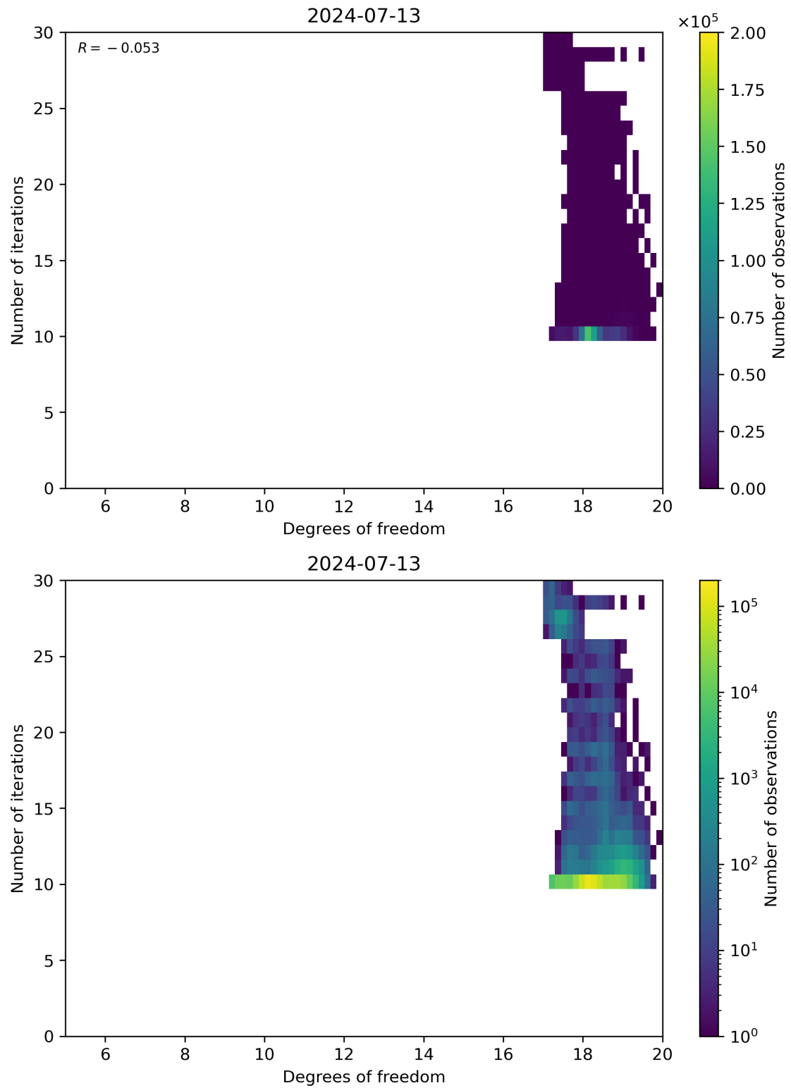
Figure 52: Scatter density plot of “Degrees of freedom” against “Number of iterations” for 2024-07-12 to 2024-07-14.
