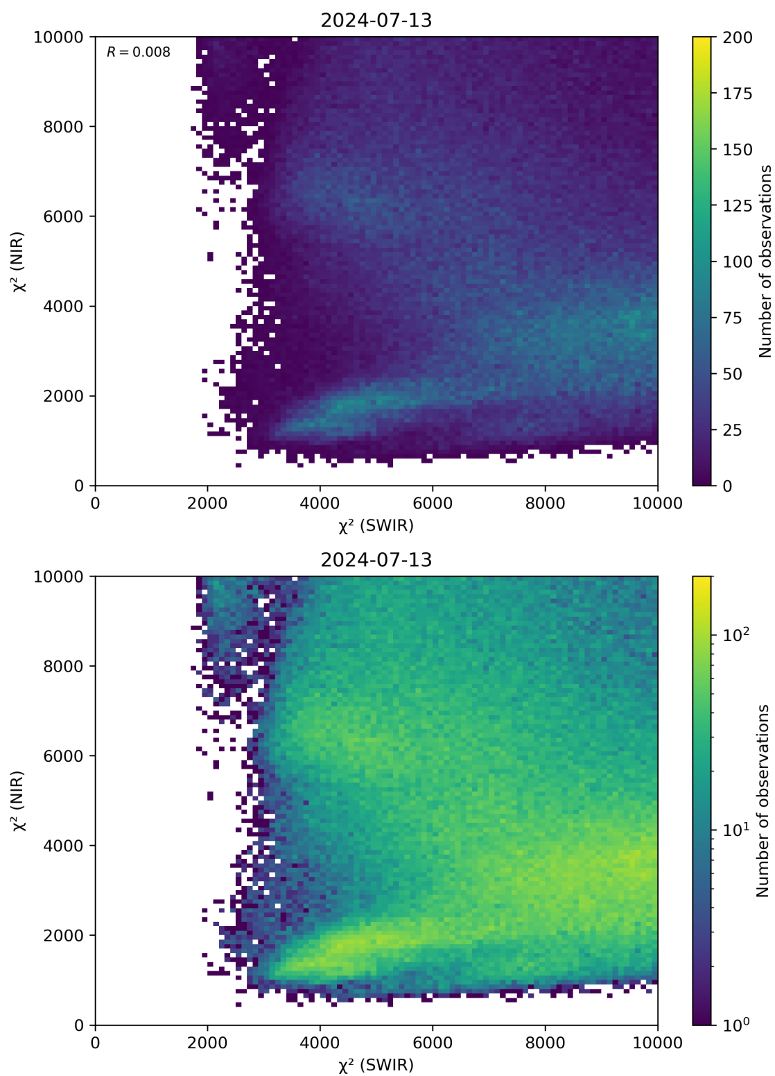
Figure 47: Scatter density plot of “ \chi^2 (SWIR)” against “ \chi^2 (NIR)” for 2024-07-12 to 2024-07-14.
