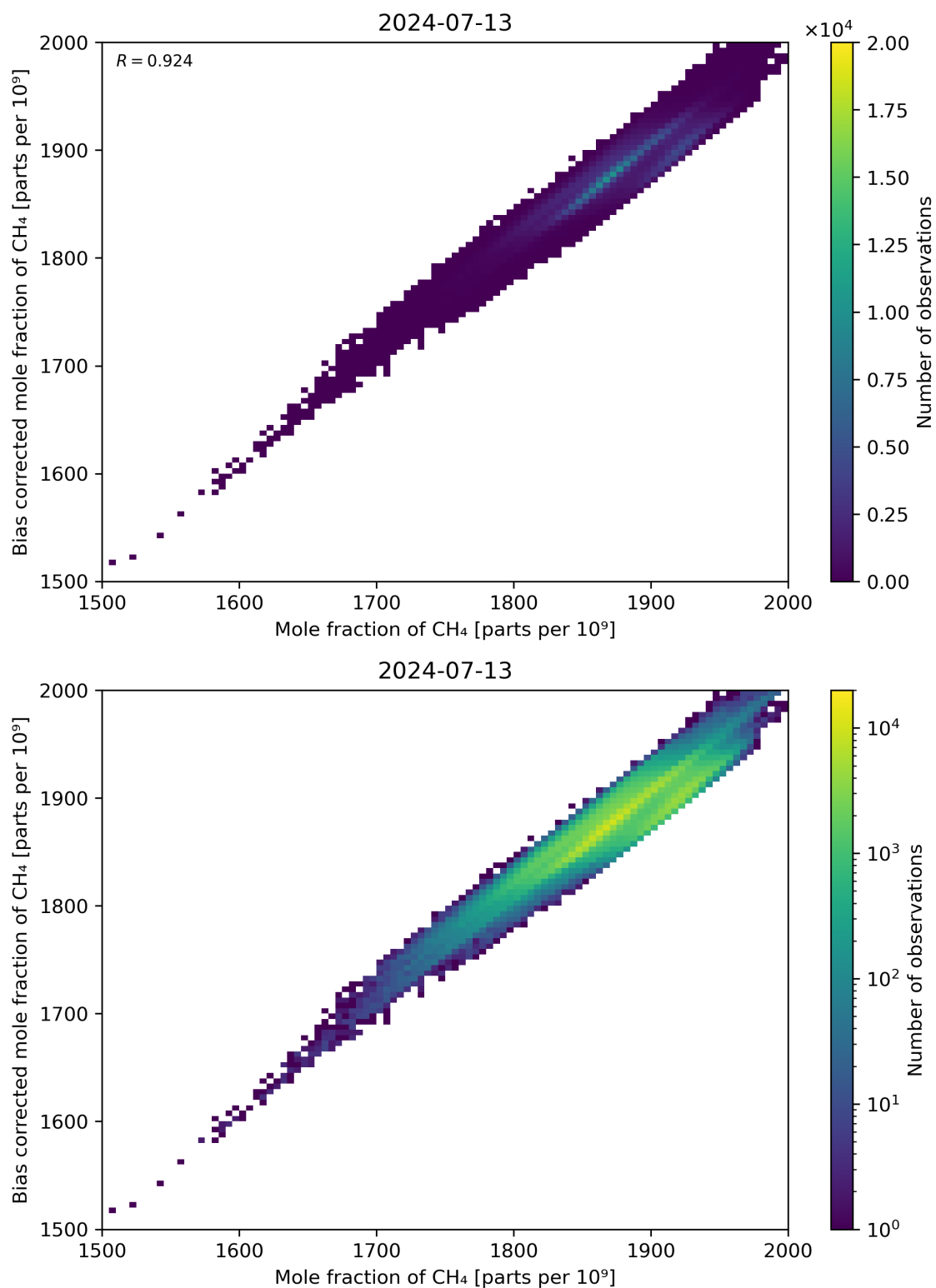
Figure 74: Scatter density plot of “Mole fraction of CH 4 ” against “Bias corrected mole fraction of CH 4 ” for 2024-07-12 to 2024-07-14.
