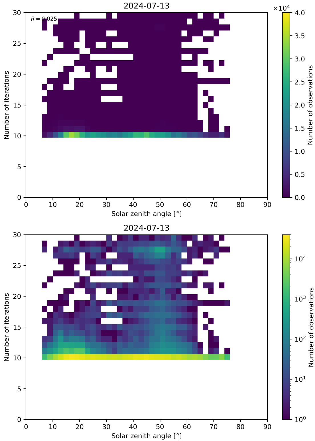
Figure 102: Scatter density plot of “Solar zenith angle” against “Number of iterations” for 2024-07-12 to 2024-07-14.
