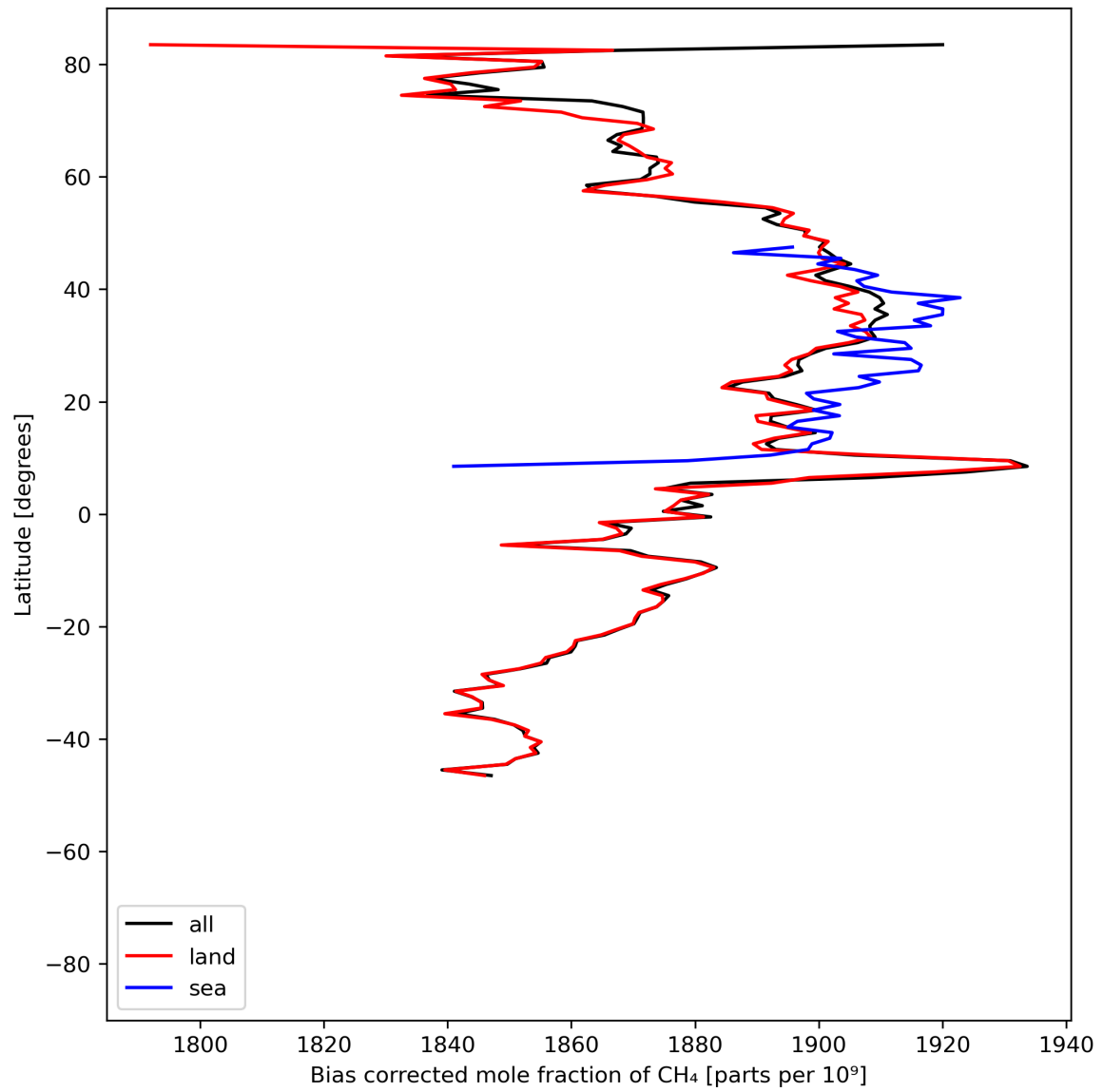
Figure 14: Zonal average of “Bias corrected mole fraction of CH 4 ” for 2024-07-12 to 2024-07-14.
