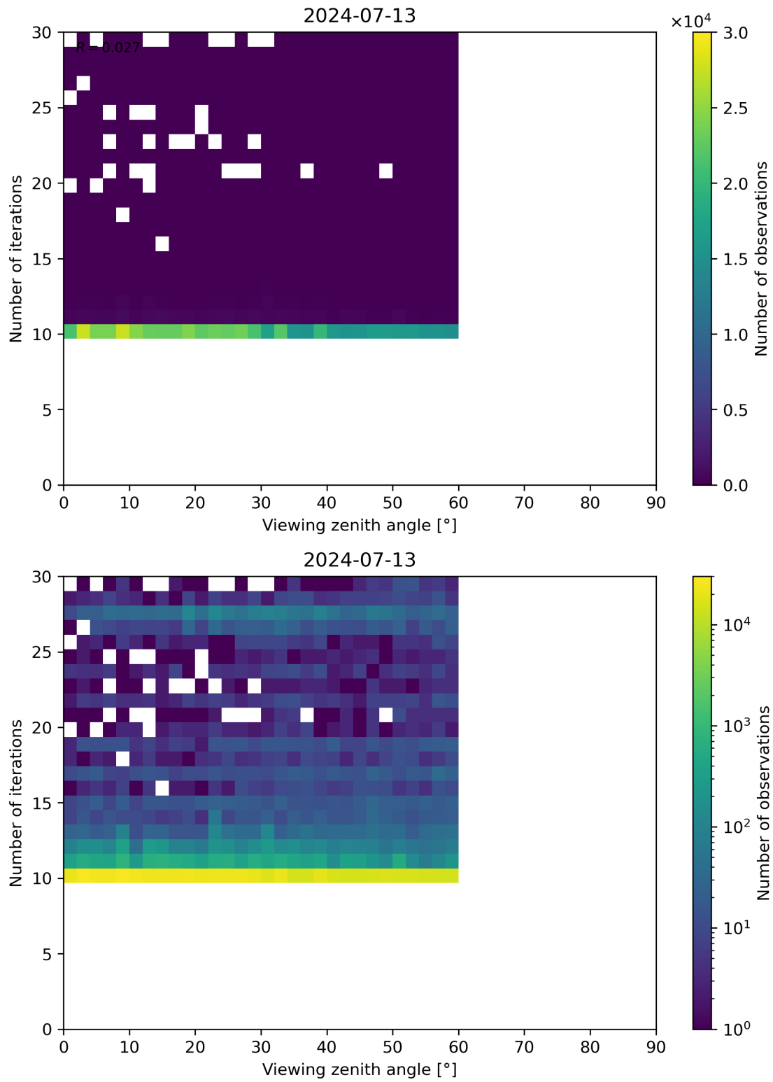
Figure 113: Scatter density plot of “Viewing zenith angle” against “Number of iterations” for 2024-07-12 to 2024-07-14.
