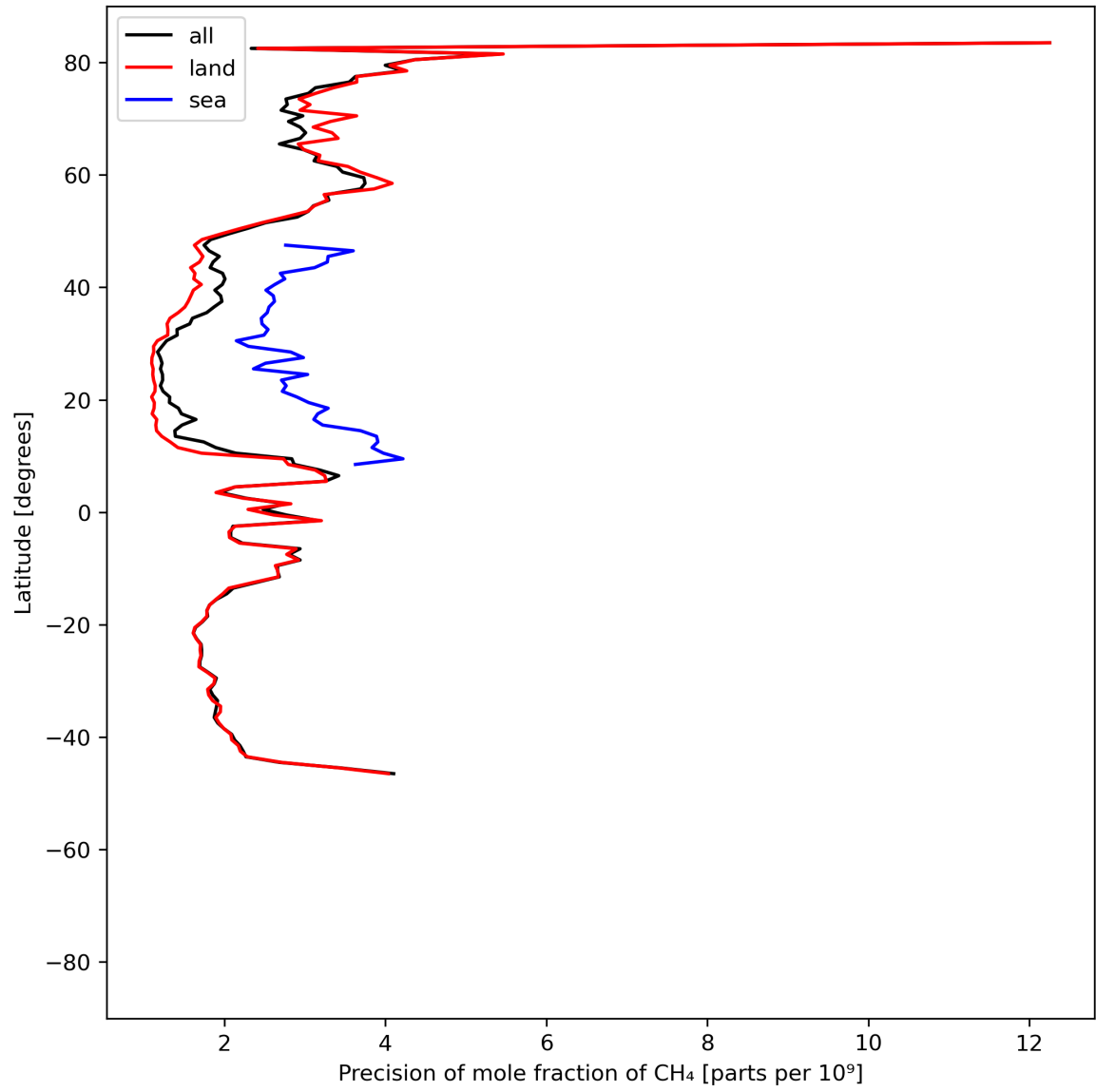
Figure 13: Zonal average of “Precision of mole fraction of CH 4 ” for 2024-07-12 to 2024-07-14.
