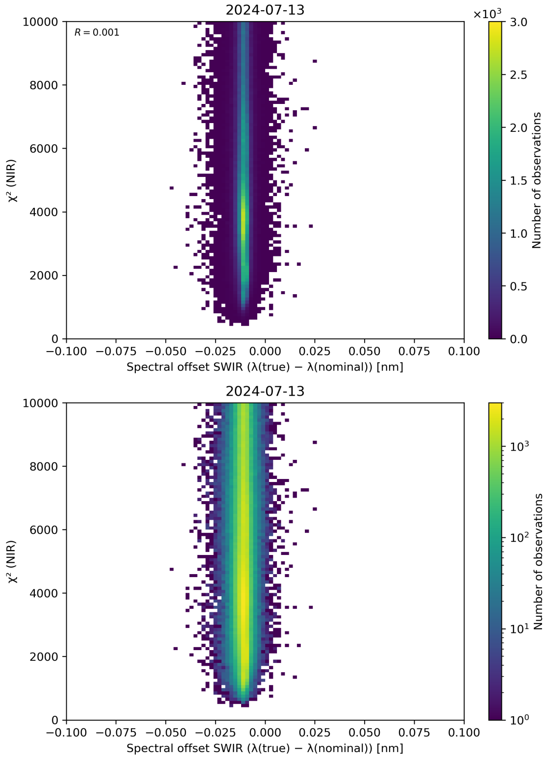
Figure 117: Scatter density plot of “Spectral offset SWIR ( \lambda(\text{true}) - \lambda(\text{nominal}) )” against “ \chi^2 (NIR)” for 2024-07-12 to 2024-07-14.
