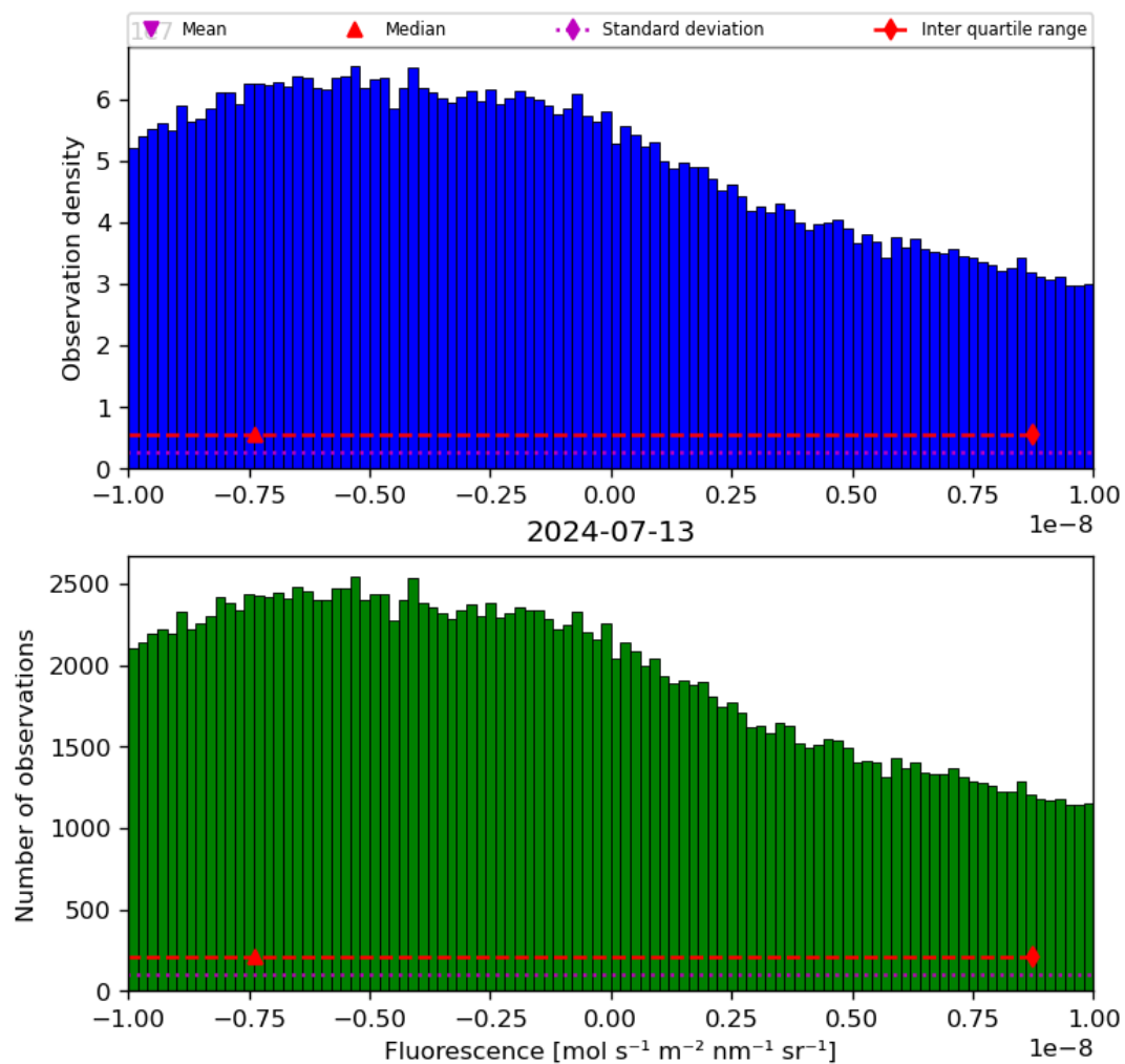
Figure 32: Histogram of “Fluorescence” for 2024-07-12 to 2024-07-14
