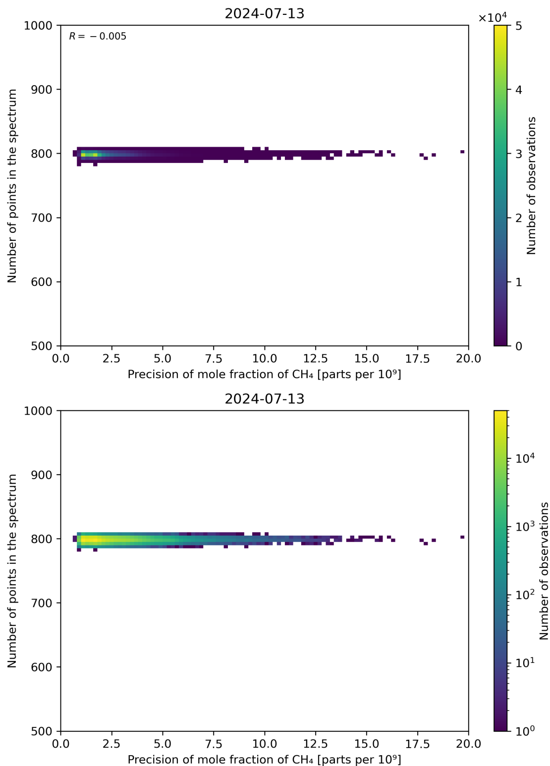
Figure 84: Scatter density plot of “Precision of mole fraction of CH 4 ” against “Number of points in the spectrum” for 2024-07-12 to 2024-07-14.
