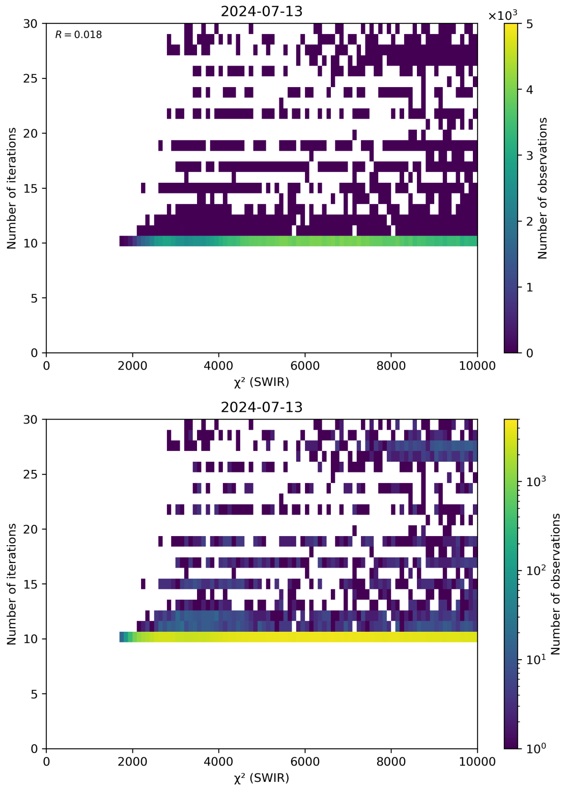
Figure 50: Scatter density plot of “ \chi^2 (SWIR)” against “Number of iterations” for 2024-07-12 to 2024-07-14.
