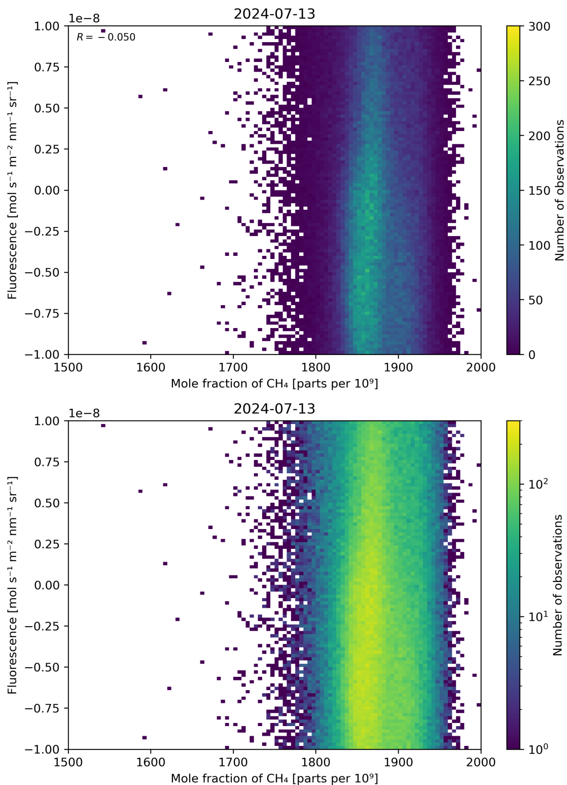
Figure 73: Scatter density plot of “Mole fraction of \text{CH}_4 ” against “Fluorescence” for 2024-07-12 to 2024-07-14.
