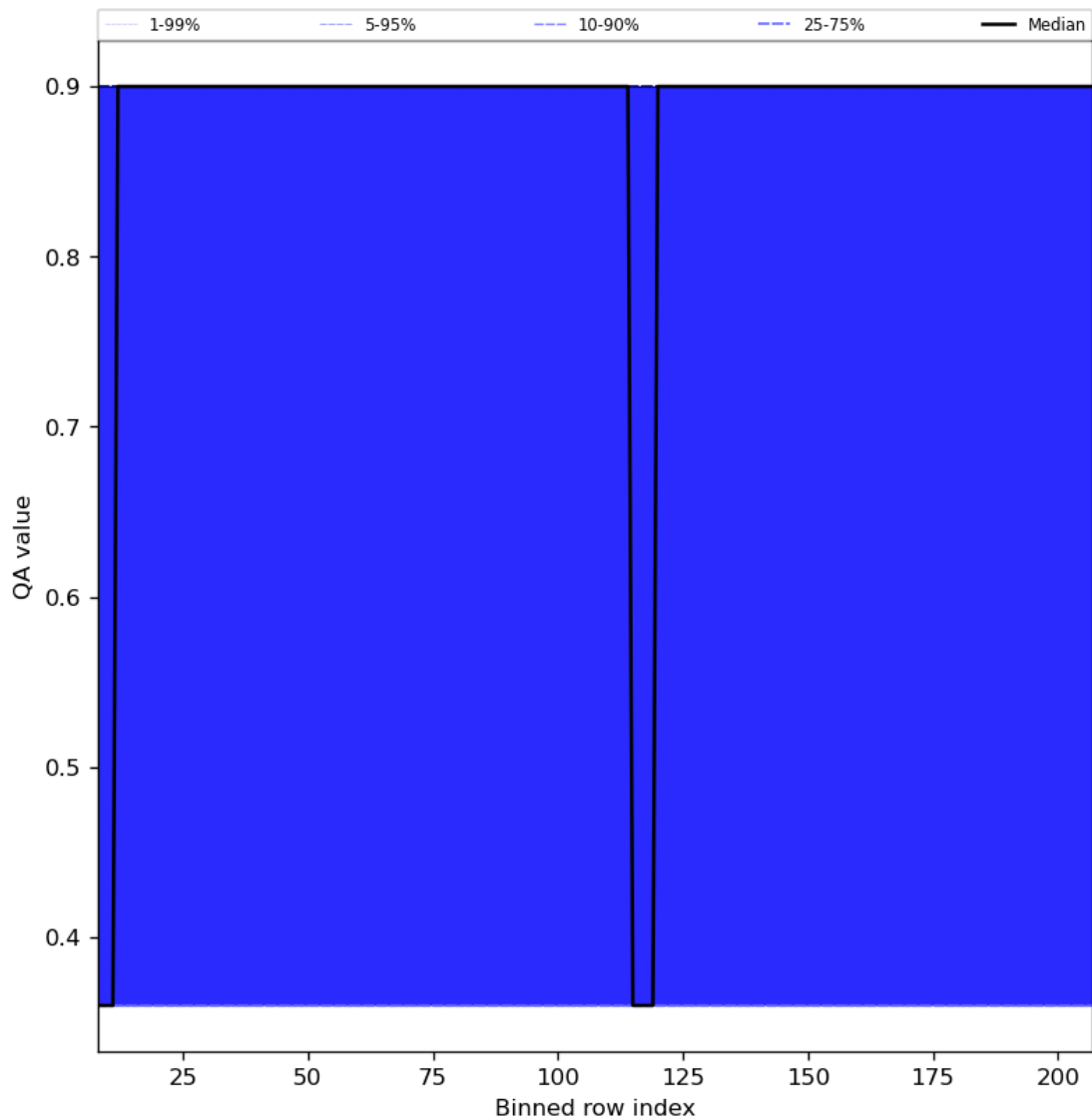
Figure 33: Along track statistics of “QA value” for 2024-07-12 to 2024-07-14
