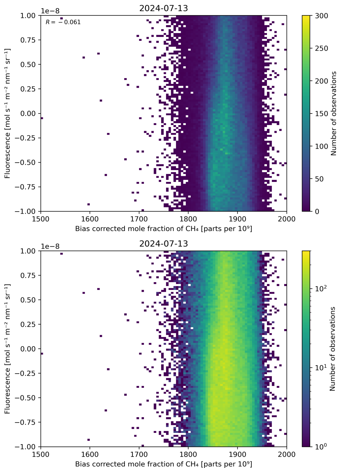
Figure 66: Scatter density plot of “Bias corrected mole fraction of \text{CH}_4 ” against “Fluorescence” for 2024-07-12 to 2024-07-14.
