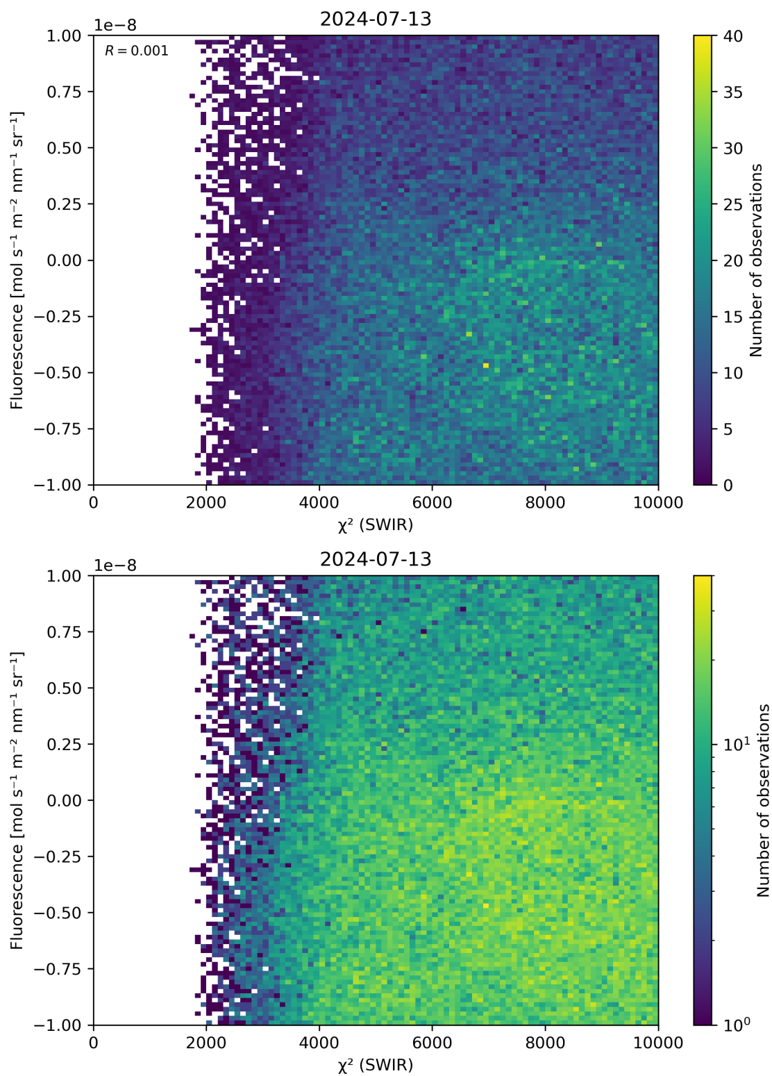
Figure 49: Scatter density plot of “ \chi^2 (SWIR)” against “Fluorescence” for 2024-07-12 to 2024-07-14.
