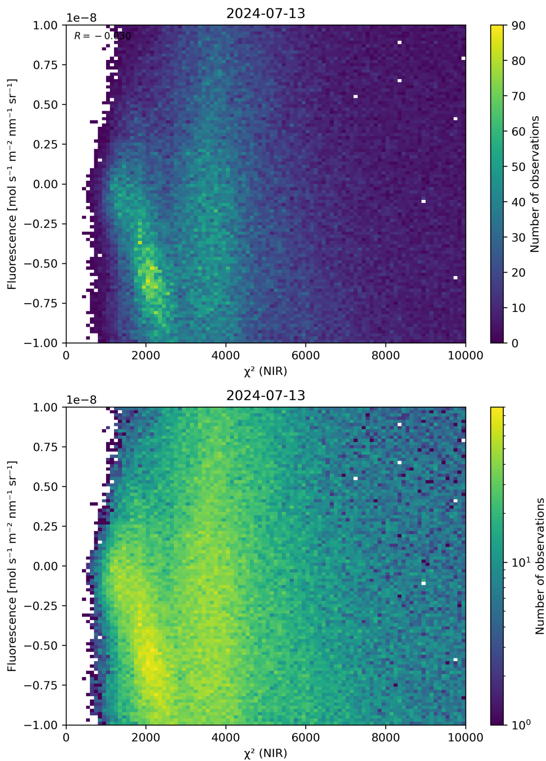
Figure 45: Scatter density plot of “ \chi^2 (NIR)” against “Fluorescence” for 2024-07-12 to 2024-07-14.
