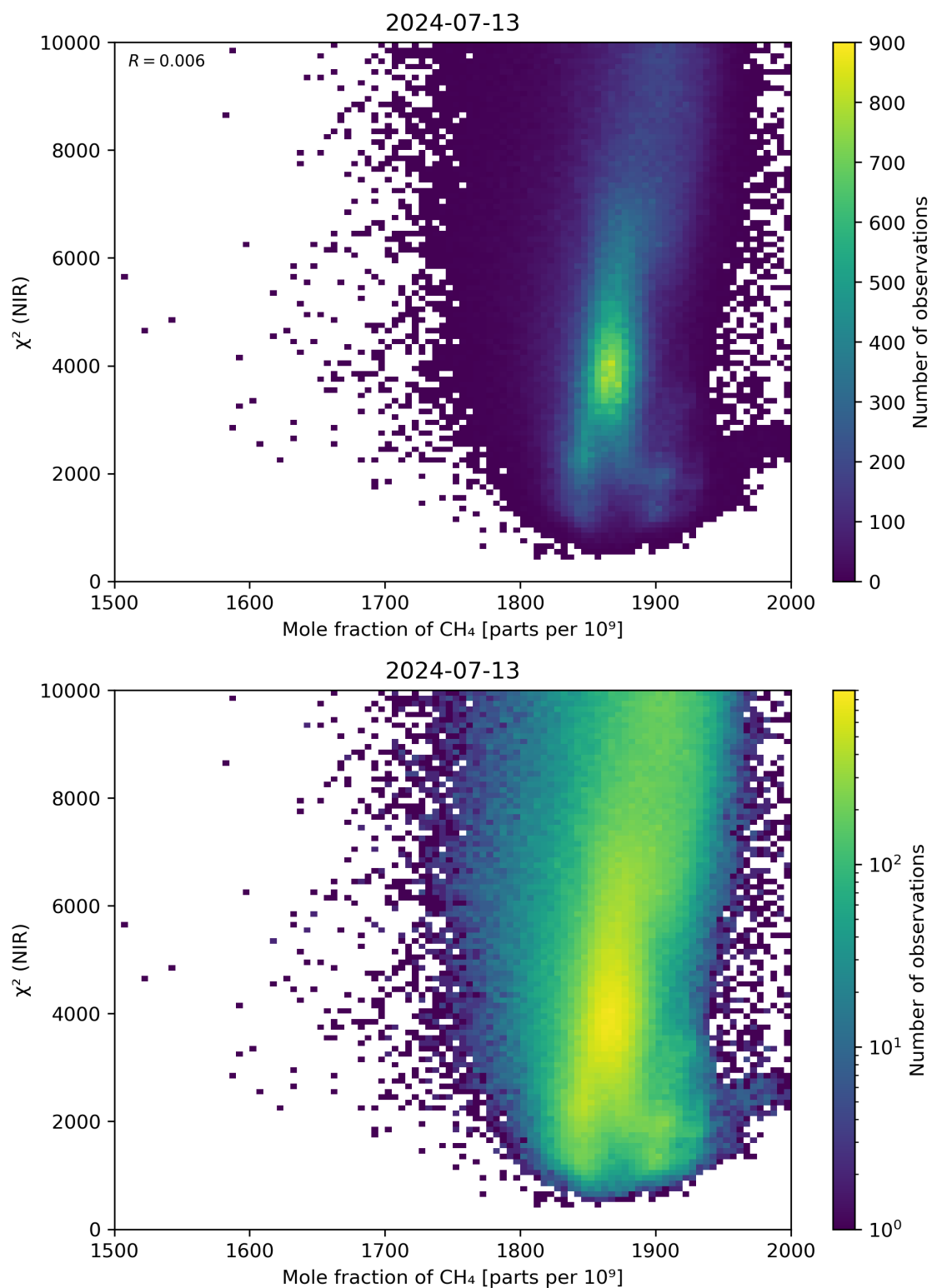
Figure 70: Scatter density plot of “Mole fraction of CH 4 ” against “ \chi^2 (NIR)” for 2024-07-12 to 2024-07-14.
