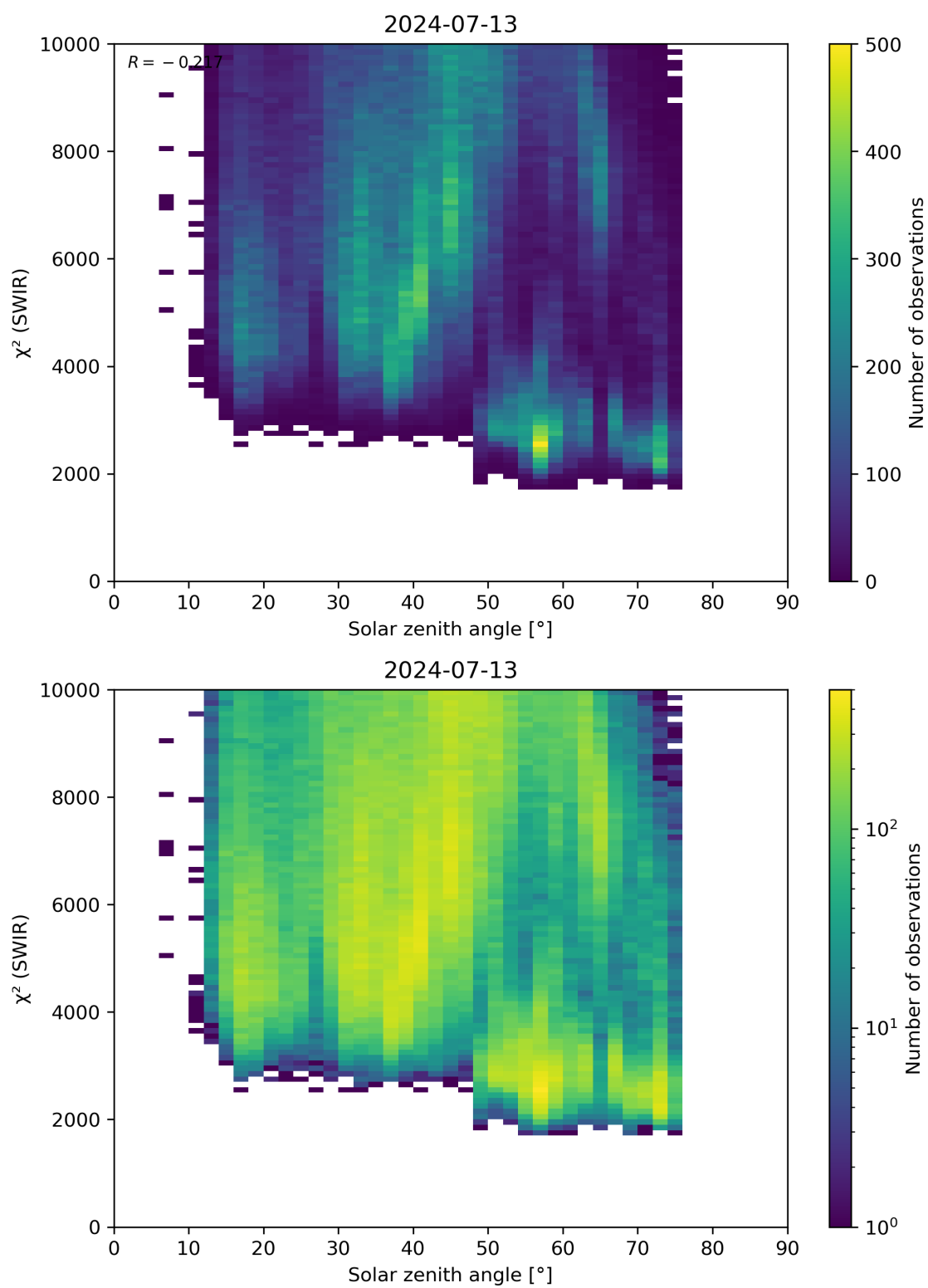
Figure 95: Scatter density plot of “Solar zenith angle” against “ \chi^2 (SWIR)” for 2024-07-12 to 2024-07-14.
