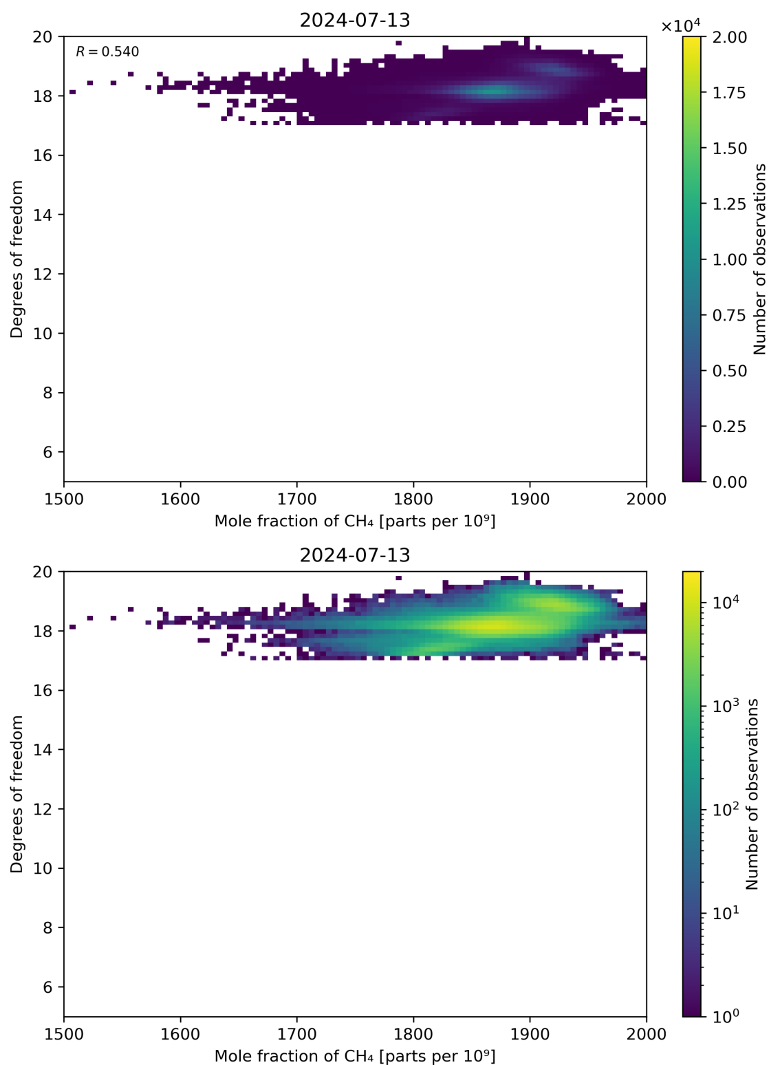
Figure 72: Scatter density plot of “Mole fraction of CH 4 ” against “Degrees of freedom” for 2024-07-12 to 2024-07-14.
