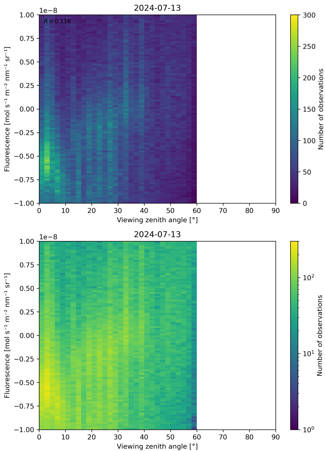
Figure 108: Scatter density plot of “Viewing zenith angle” against “Fluorescence” for 2024-07-12 to 2024-07-14.
