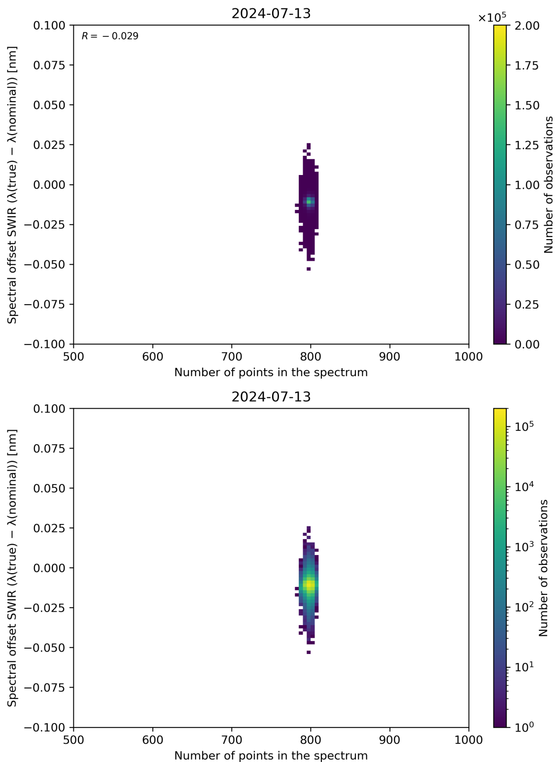
Figure 93: Scatter density plot of “Number of points in the spectrum” against “Spectral offset SWIR ( \lambda(\text{true}) - \lambda(\text{nominal}) )” for 2024-07-12 to 2024-07-14.
