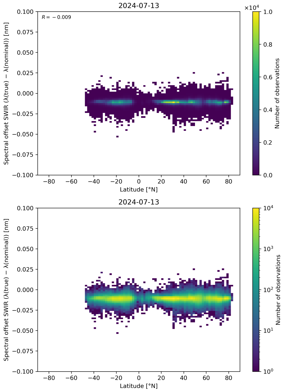
Figure 62: Scatter density plot of “Latitude” against “Spectral offset SWIR ( \lambda(\text{true}) - \lambda(\text{nominal}) )” for 2024-07-12 to 2024-07-14.
