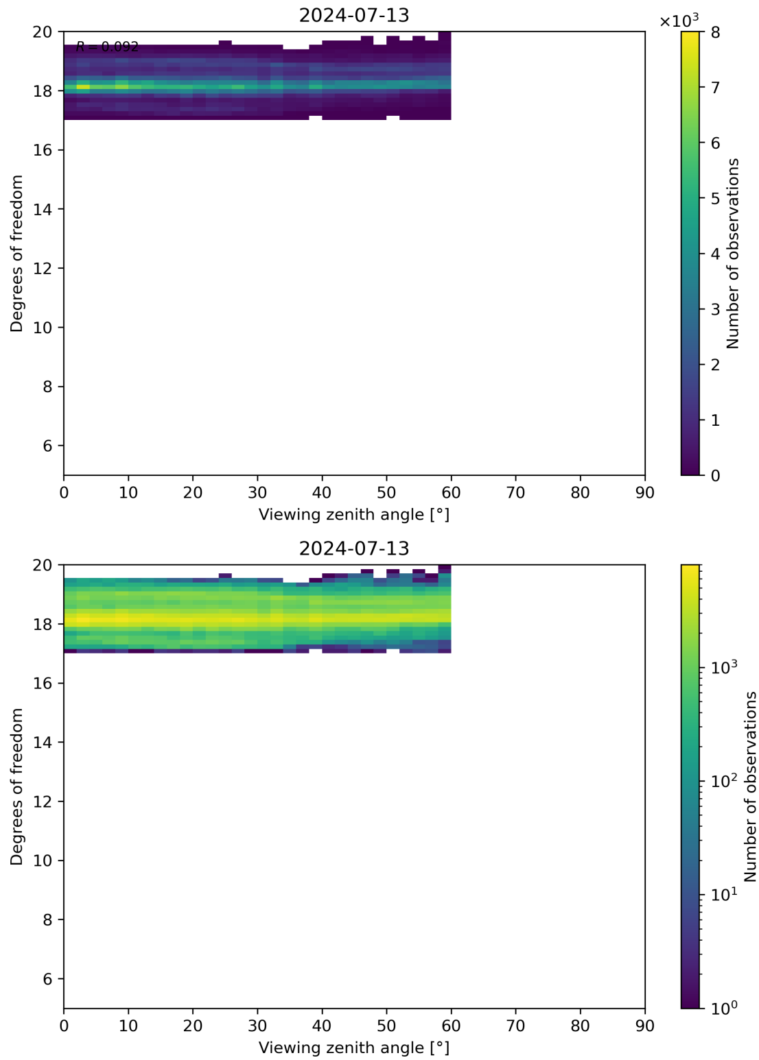
Figure 107: Scatter density plot of “Viewing zenith angle” against “Degrees of freedom” for 2024-07-12 to 2024-07-14.
