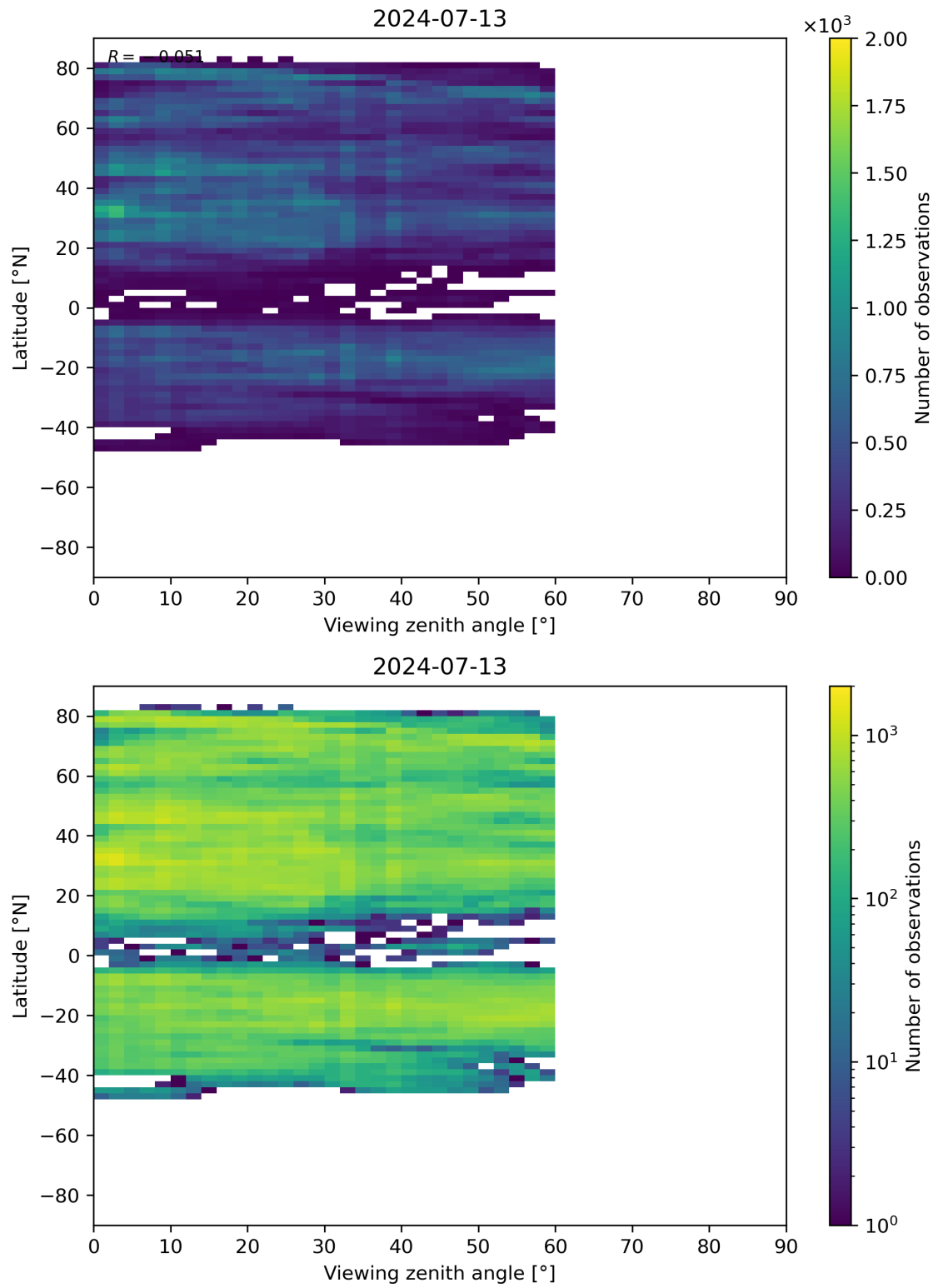
Figure 109: Scatter density plot of “Viewing zenith angle” against “Latitude” for 2024-07-12 to 2024-07-14.
