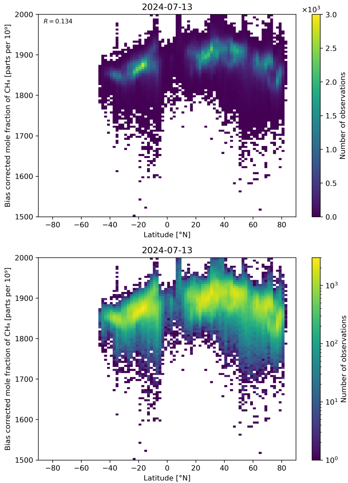
Figure 58: Scatter density plot of “Latitude” against “Bias corrected mole fraction of \text{CH}_4 ” for 2024-07-12 to 2024-07-14.
