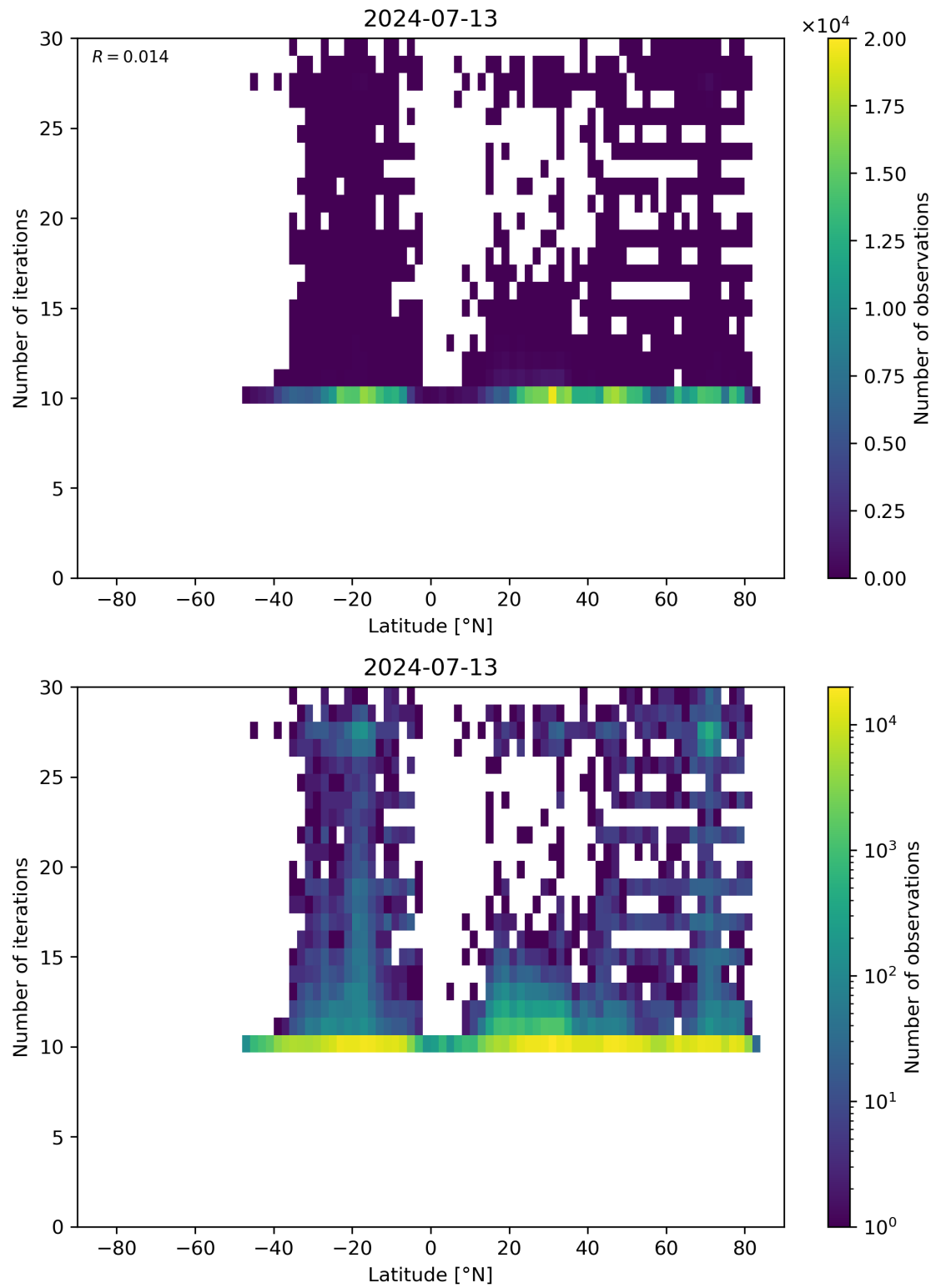
Figure 60: Scatter density plot of “Latitude” against “Number of iterations” for 2024-07-12 to 2024-07-14.
