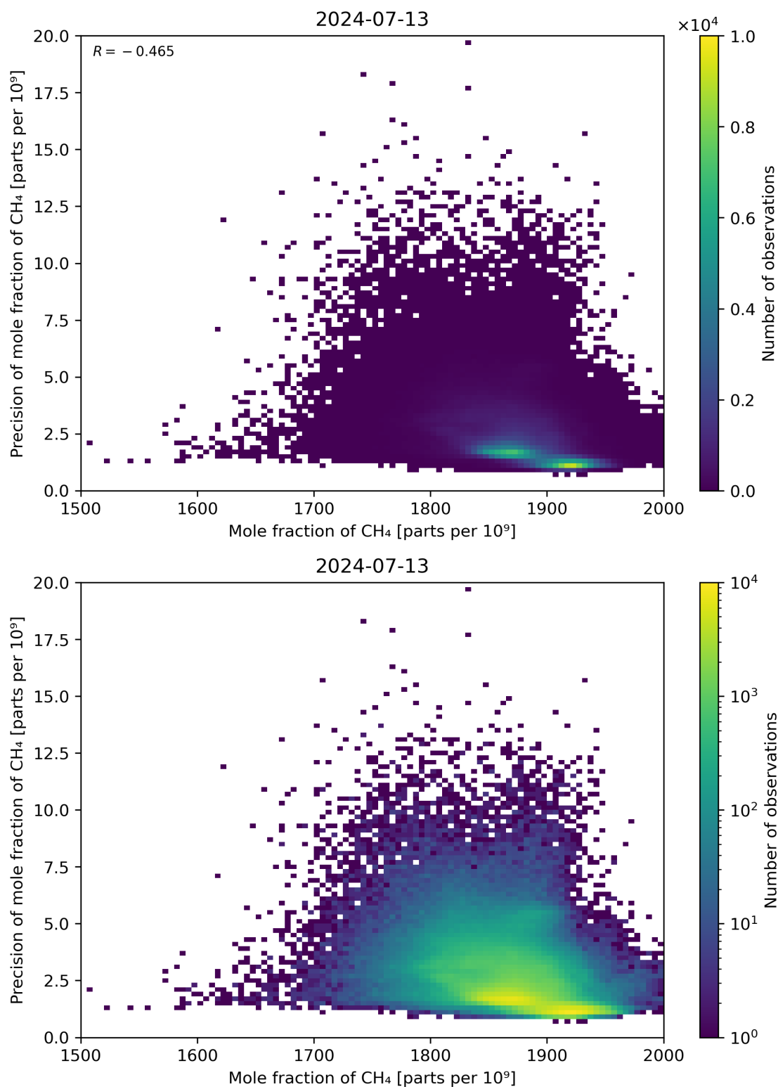
Figure 75: Scatter density plot of “Mole fraction of CH 4 ” against “Precision of mole fraction of CH 4 ” for 2024-07-12 to 2024-07-14.
