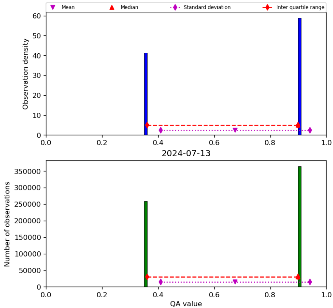
Figure 22: Histogram of “QA value” for 2024-07-12 to 2024-07-14
