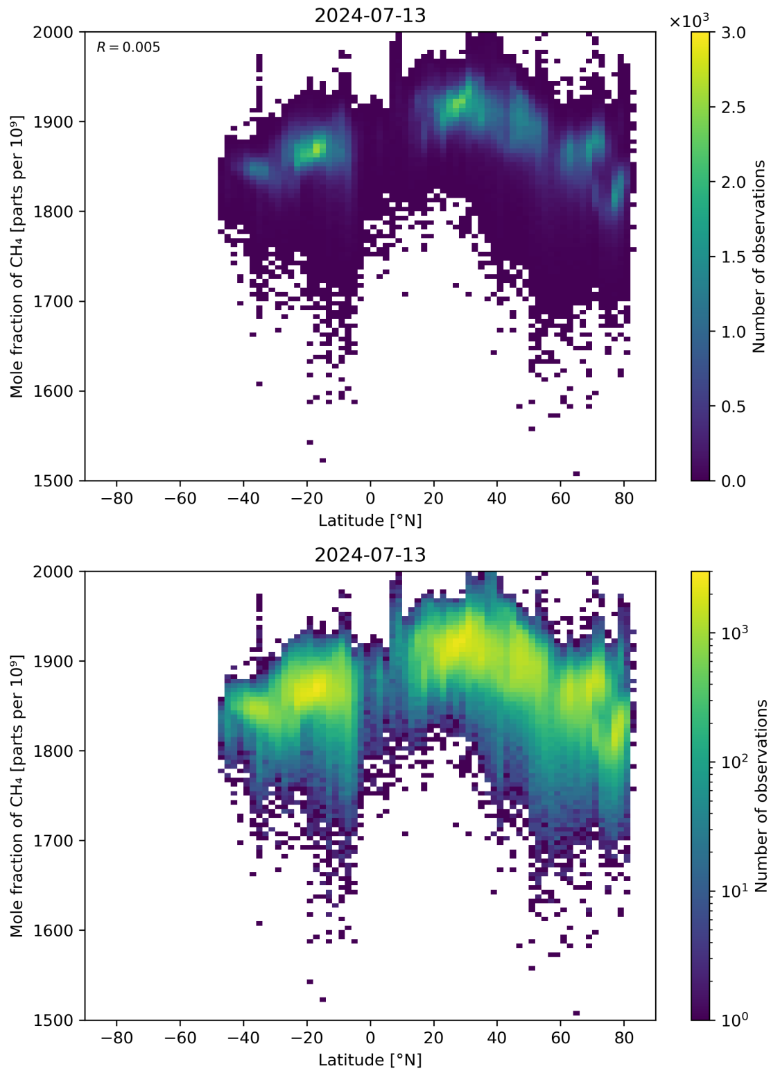
Figure 57: Scatter density plot of “Latitude” against “Mole fraction of \text{CH}_4 ” for 2024-07-12 to 2024-07-14.
