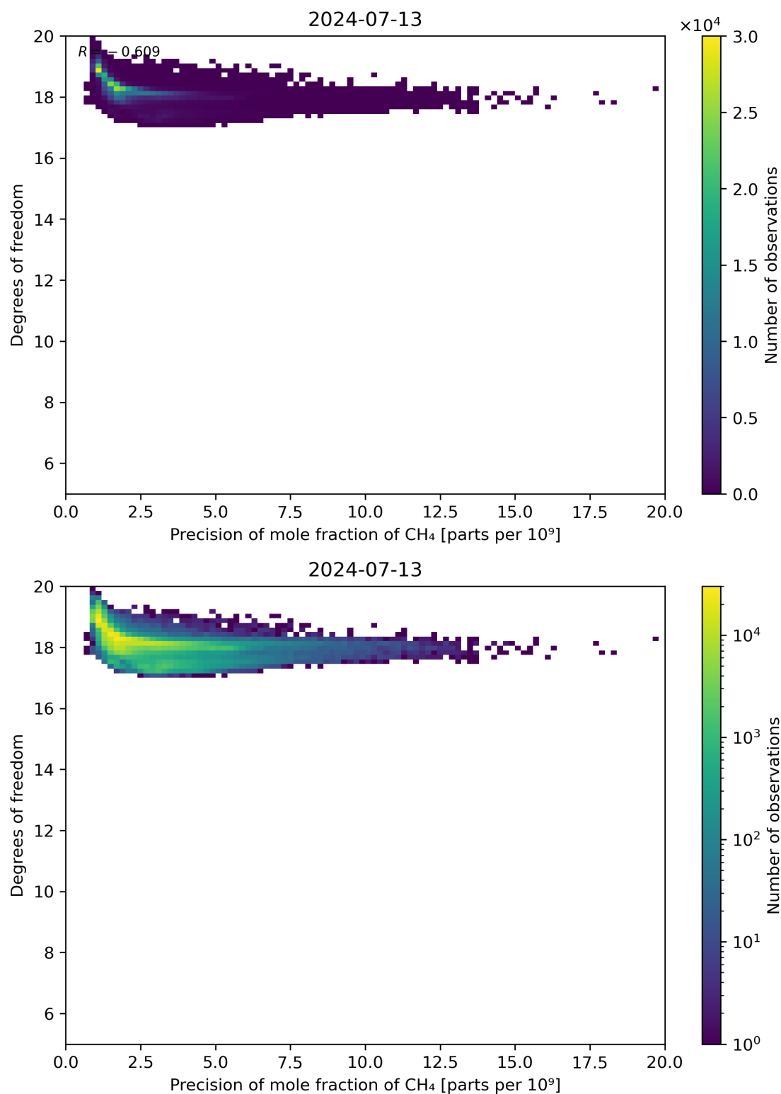
Figure 80: Scatter density plot of “Precision of mole fraction of CH 4 ” against “Degrees of freedom” for 2024-07-12 to 2024-07-14.
