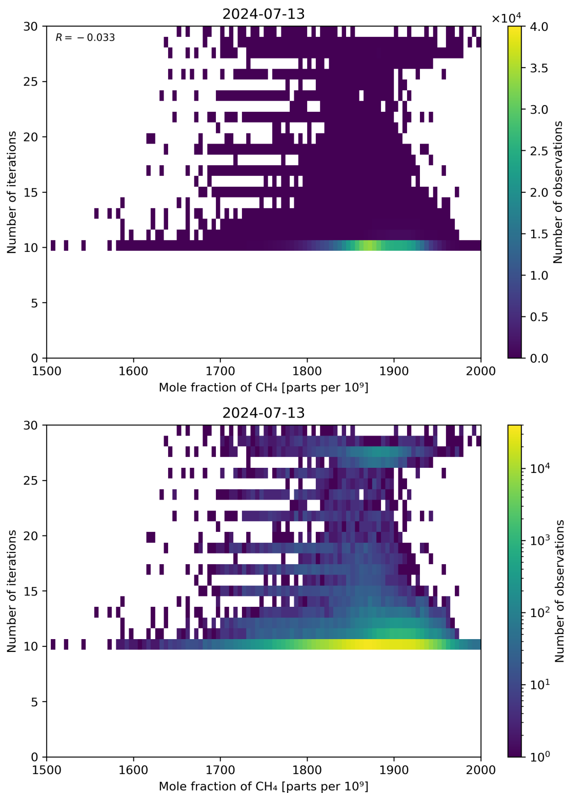
Figure 76: Scatter density plot of “Mole fraction of CH 4 ” against “Number of iterations” for 2024-07-12 to 2024-07-14.
