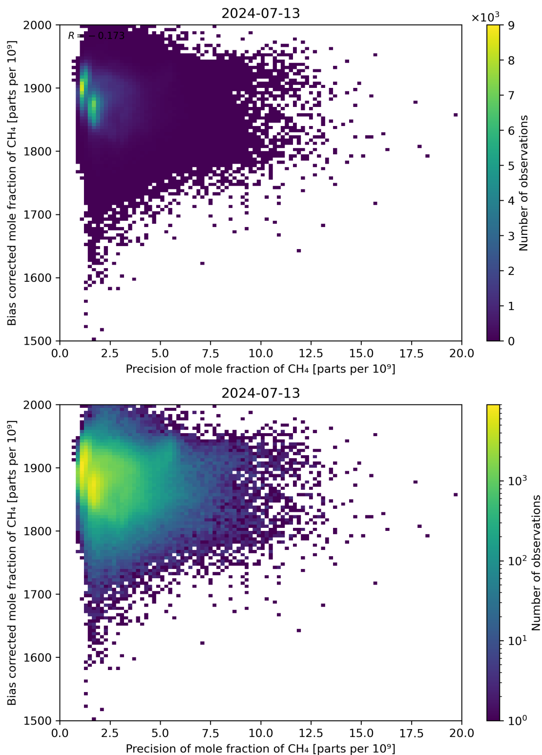
Figure 82: Scatter density plot of “Precision of mole fraction of CH 4 ” against “Bias corrected mole fraction of CH 4 ” for 2024-07-12 to 2024-07-14.
