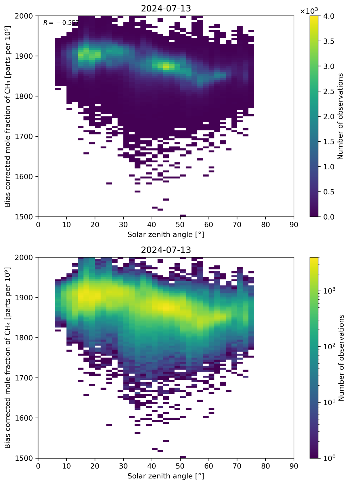
Figure 100: Scatter density plot of “Solar zenith angle” against “Bias corrected mole fraction of \text{CH}_4 ” for 2024-07-12 to 2024-07-14.
