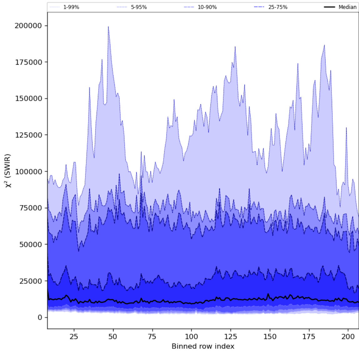
Figure 39: Along track statistics of " \chi^2 (SWIR)" for 2024-07-12 to 2024-07-14
