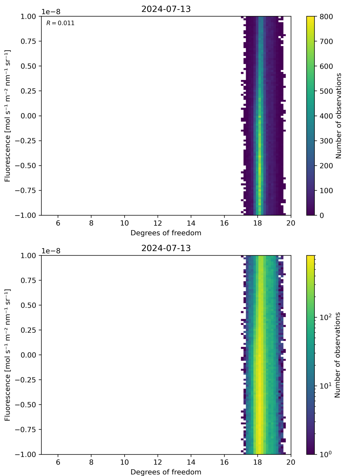
Figure 51: Scatter density plot of “Degrees of freedom” against “Fluorescence” for 2024-07-12 to 2024-07-14.
