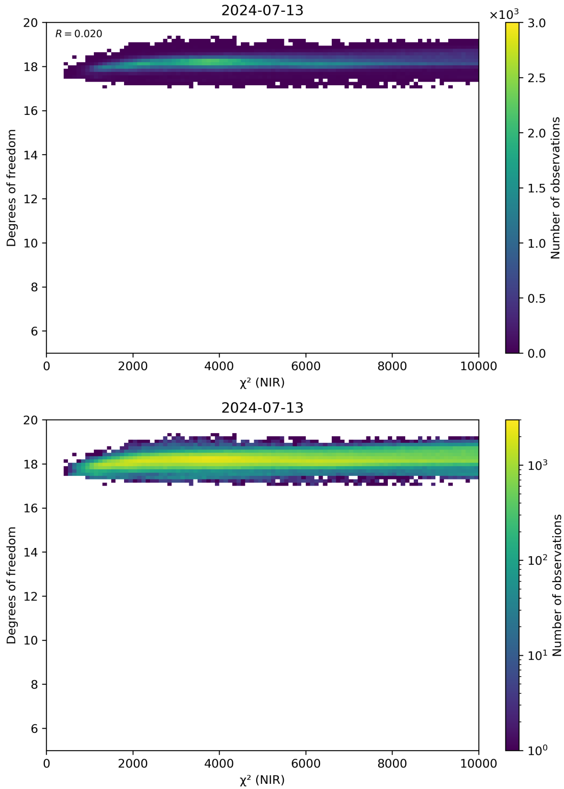
Figure 44: Scatter density plot of “ \chi^2 (NIR)” against “Degrees of freedom” for 2024-07-12 to 2024-07-14.
