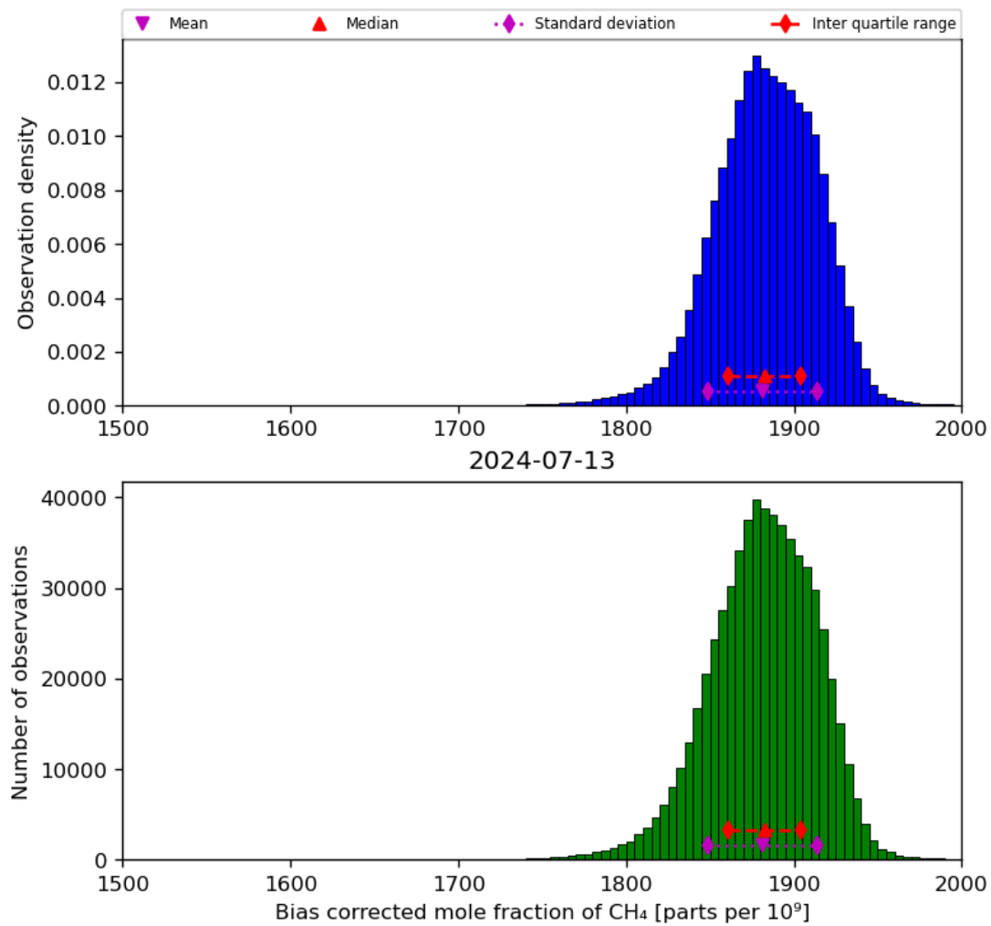
Figure 25: Histogram of “Bias corrected mole fraction of CH 4 ” for 2024-07-12 to 2024-07-14
