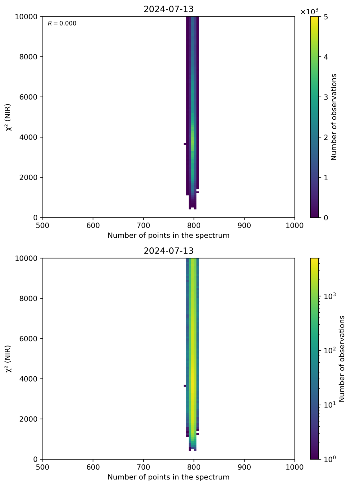
Figure 88: Scatter density plot of “Number of points in the spectrum” against “ \chi^2 (NIR)” for 2024-07-12 to 2024-07-14.
