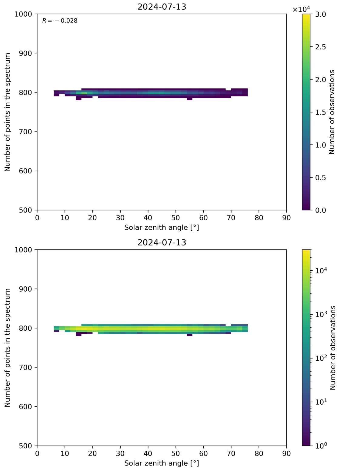
Figure 103: Scatter density plot of “Solar zenith angle” against “Number of points in the spectrum” for 2024-07-12 to 2024-07-14.
