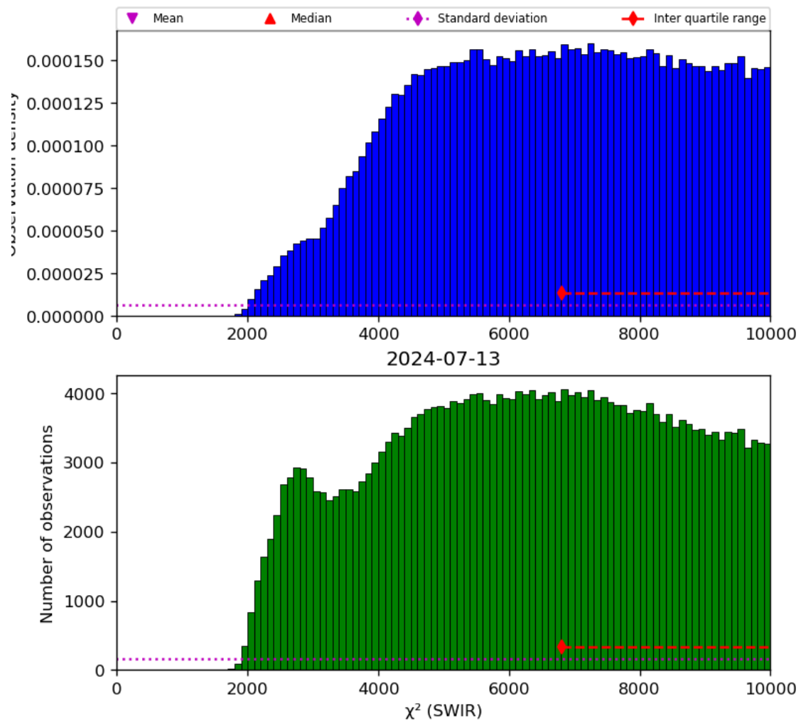
Figure 28: Histogram of “ \chi^2 (SWIR)” for 2024-07-12 to 2024-07-14
