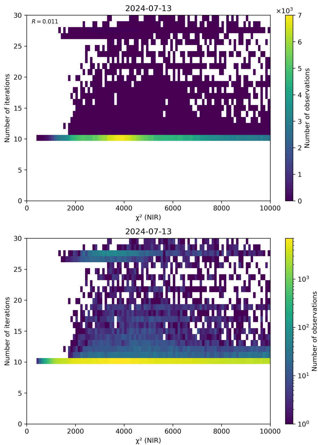
Figure 46: Scatter density plot of “ \chi^2 (NIR)” against “Number of iterations” for 2024-07-12 to 2024-07-14.
