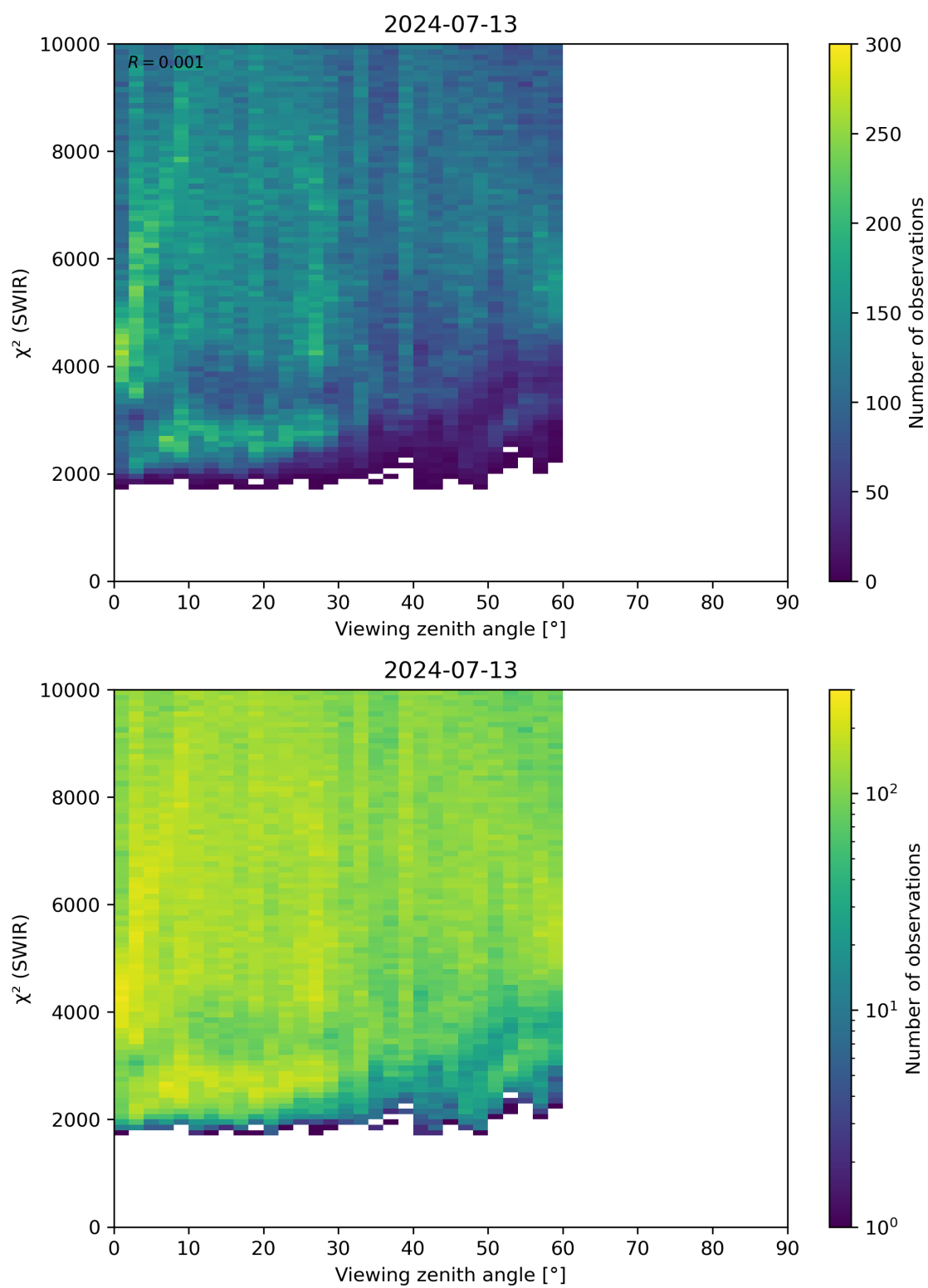
Figure 106: Scatter density plot of “Viewing zenith angle” against “ \chi^2 (SWIR)” for 2024-07-12 to 2024-07-14.
