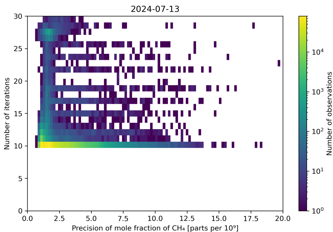
Figure 83: Scatter density plot of “Precision of mole fraction of CH 4 ” against “Number of iterations” for 2024-07-12 to 2024-07-14.
