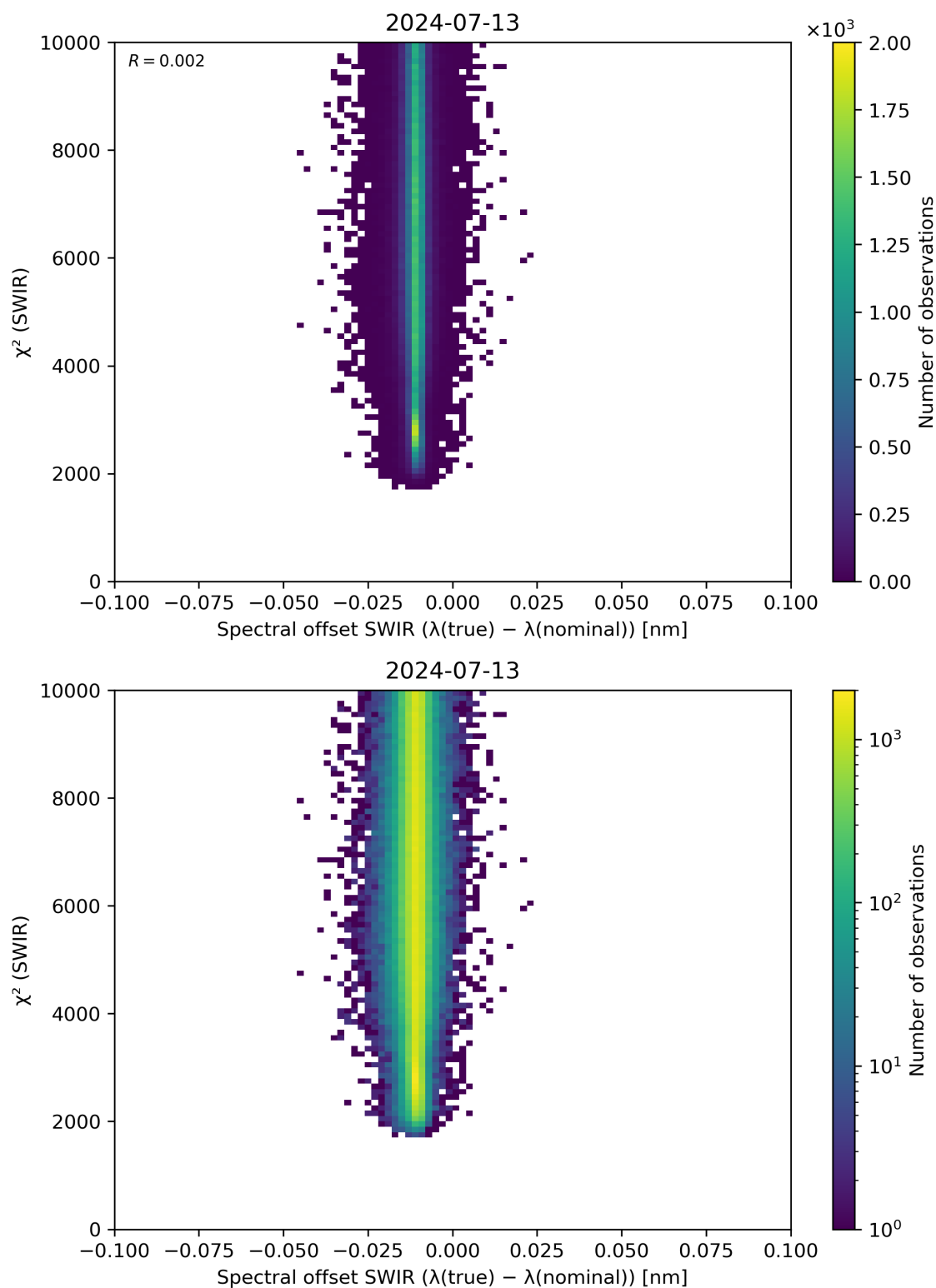
Figure 118: Scatter density plot of “Spectral offset SWIR ( \lambda(\text{true}) - \lambda(\text{nominal}) )” against “ \chi^2 (SWIR)” for 2024-07-12 to 2024-07-14.
