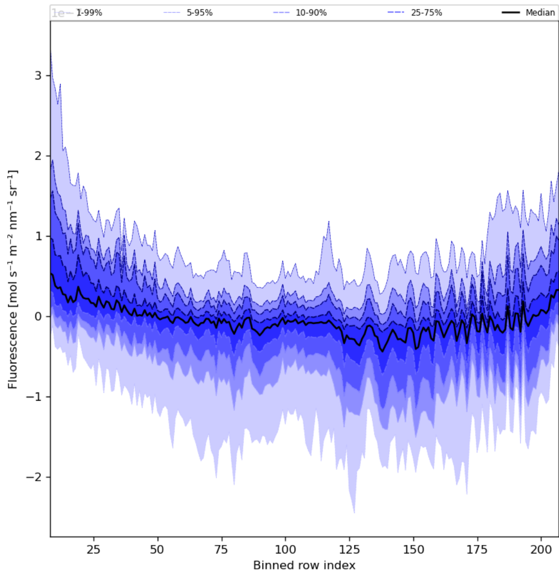
Figure 43: Along track statistics of “Fluorescence” for 2024-07-12 to 2024-07-14
