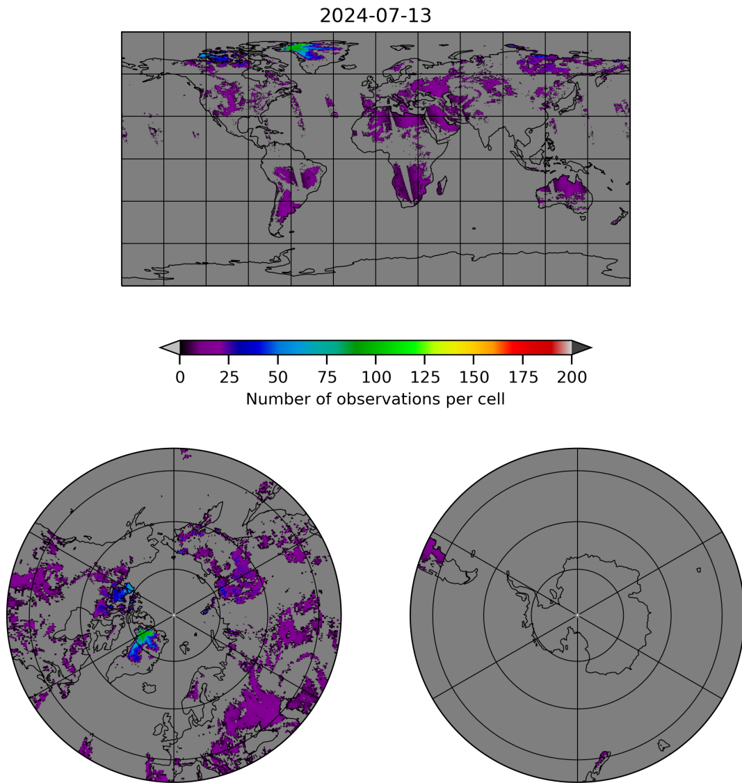
Figure 10: Map of the number of observations for 2024-07-12 to 2024-07-14
