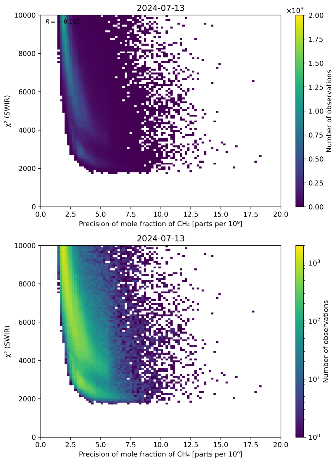
Figure 79: Scatter density plot of “Precision of mole fraction of \text{CH}_4 ” against “ \chi^2 (SWIR)” for 2024-07-12 to 2024-07-14.
