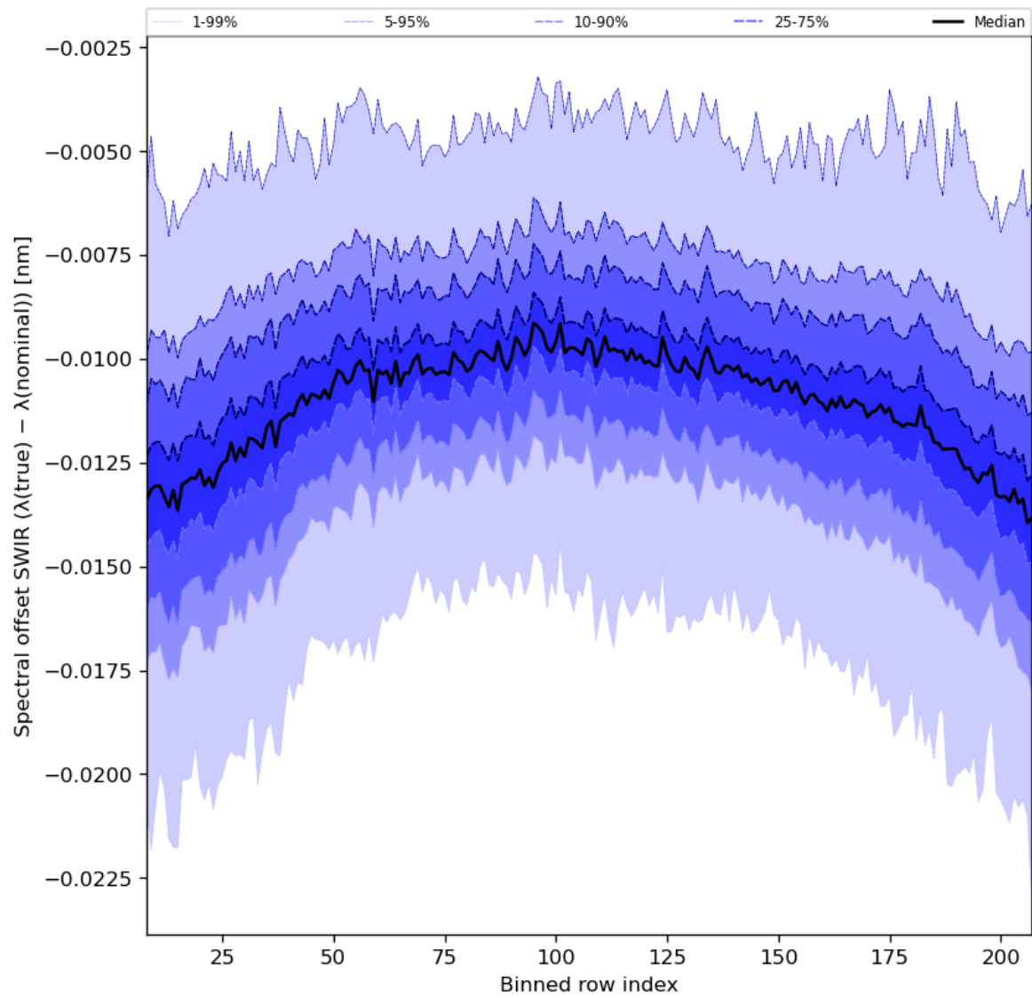
Figure 38: Along track statistics of “Spectral offset SWIR ( \lambda(\text{true}) - \lambda(\text{nominal}) )” for 2024-07-12 to 2024-07-14
