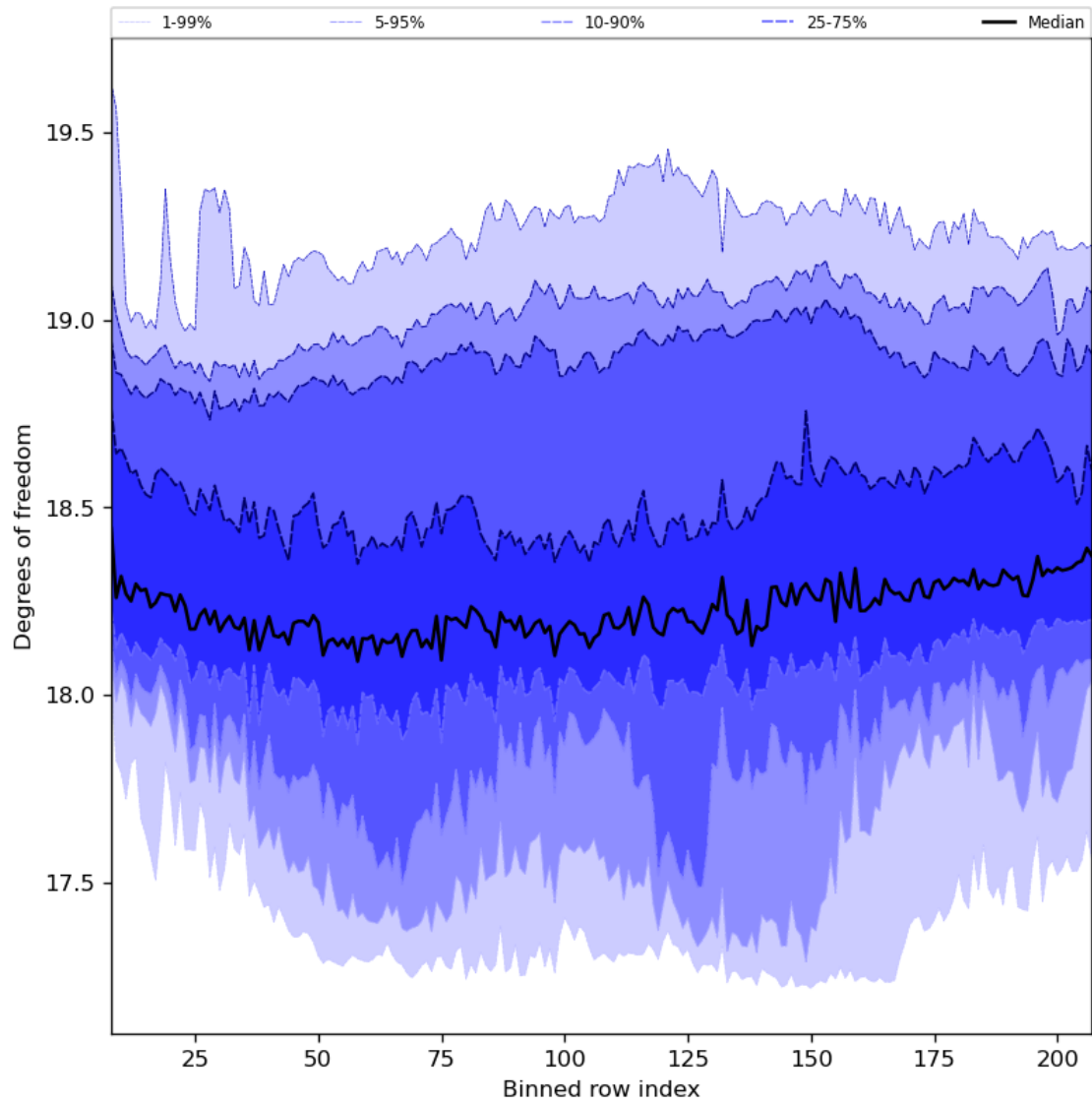
Figure 41: Along track statistics of “Degrees of freedom” for 2024-07-12 to 2024-07-14
