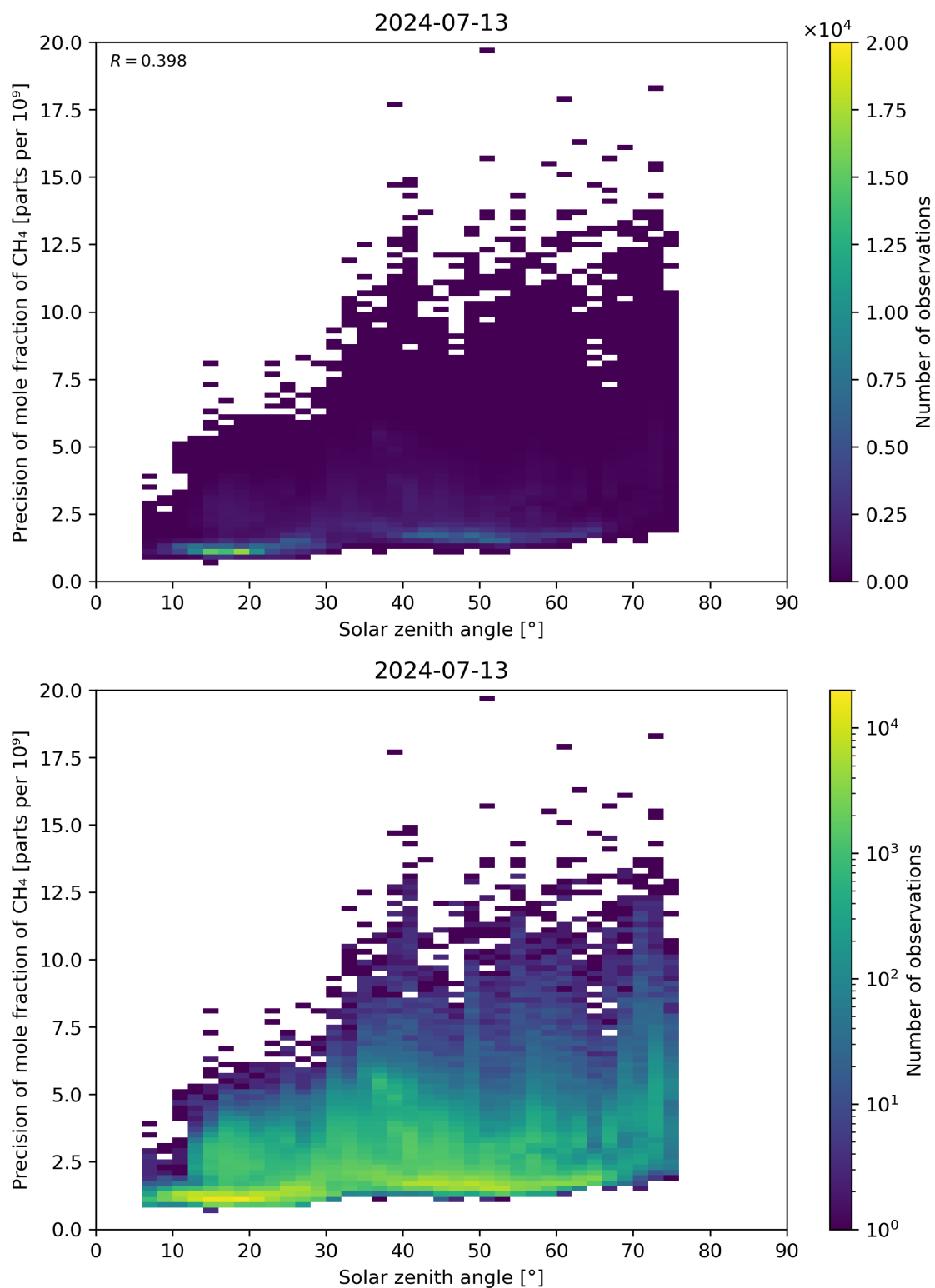
Figure 101: Scatter density plot of “Solar zenith angle” against “Precision of mole fraction of \text{CH}_4 ” for 2024-07-12 to 2024-07-14.
