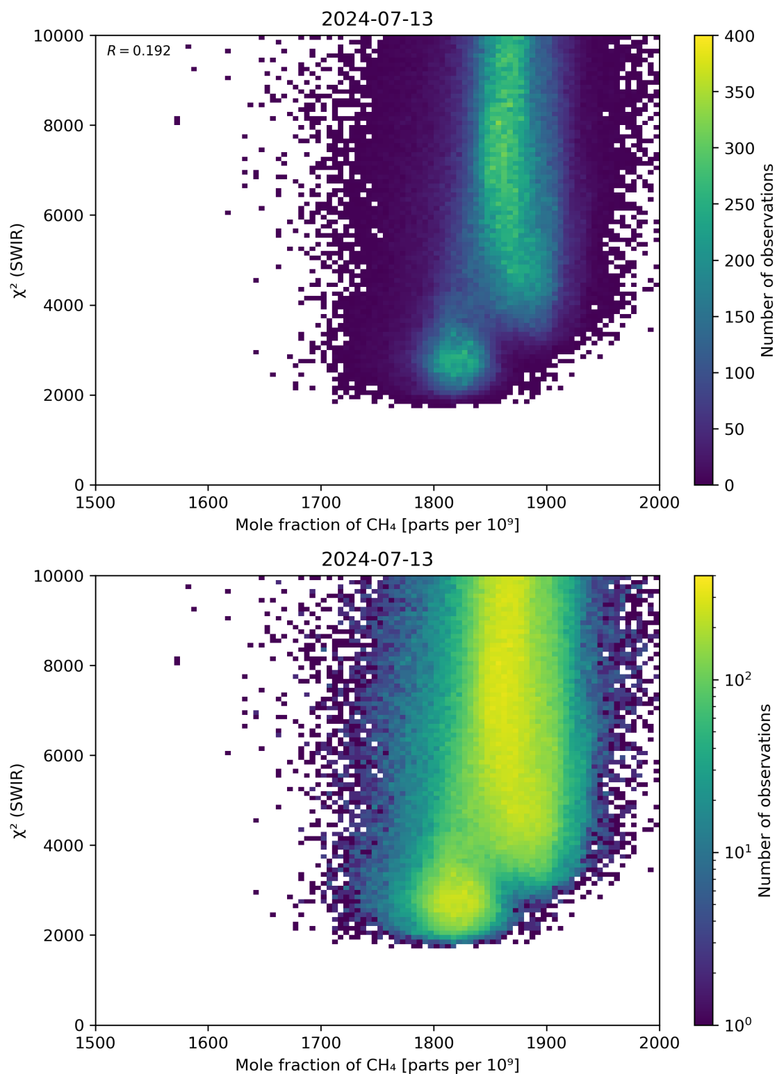
Figure 71: Scatter density plot of “Mole fraction of \text{CH}_4 ” against “ \chi^2 (SWIR)” for 2024-07-12 to 2024-07-14.
