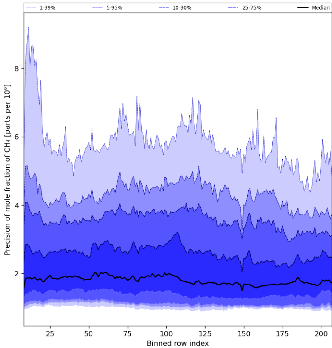
Figure 35: Along track statistics of “Precision of mole fraction of CH 4 ” for 2024-07-12 to 2024-07-14
