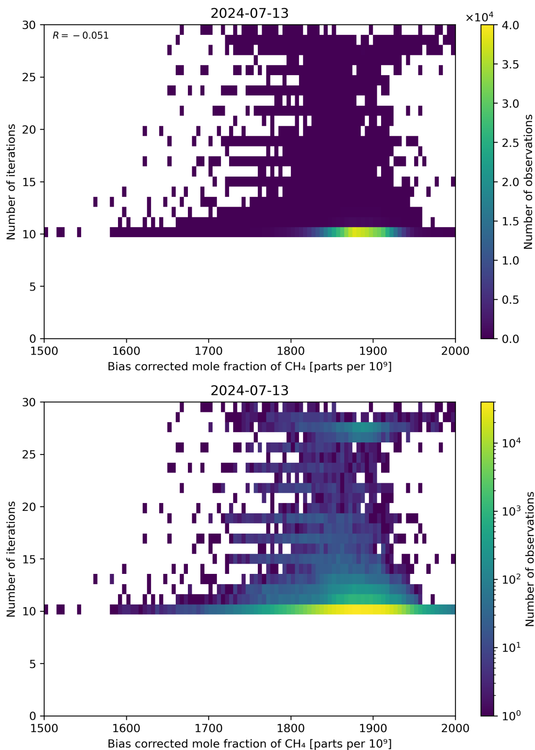
Figure 67: Scatter density plot of “Bias corrected mole fraction of \text{CH}_4 ” against “Number of iterations” for 2024-07-12 to 2024-07-14.
