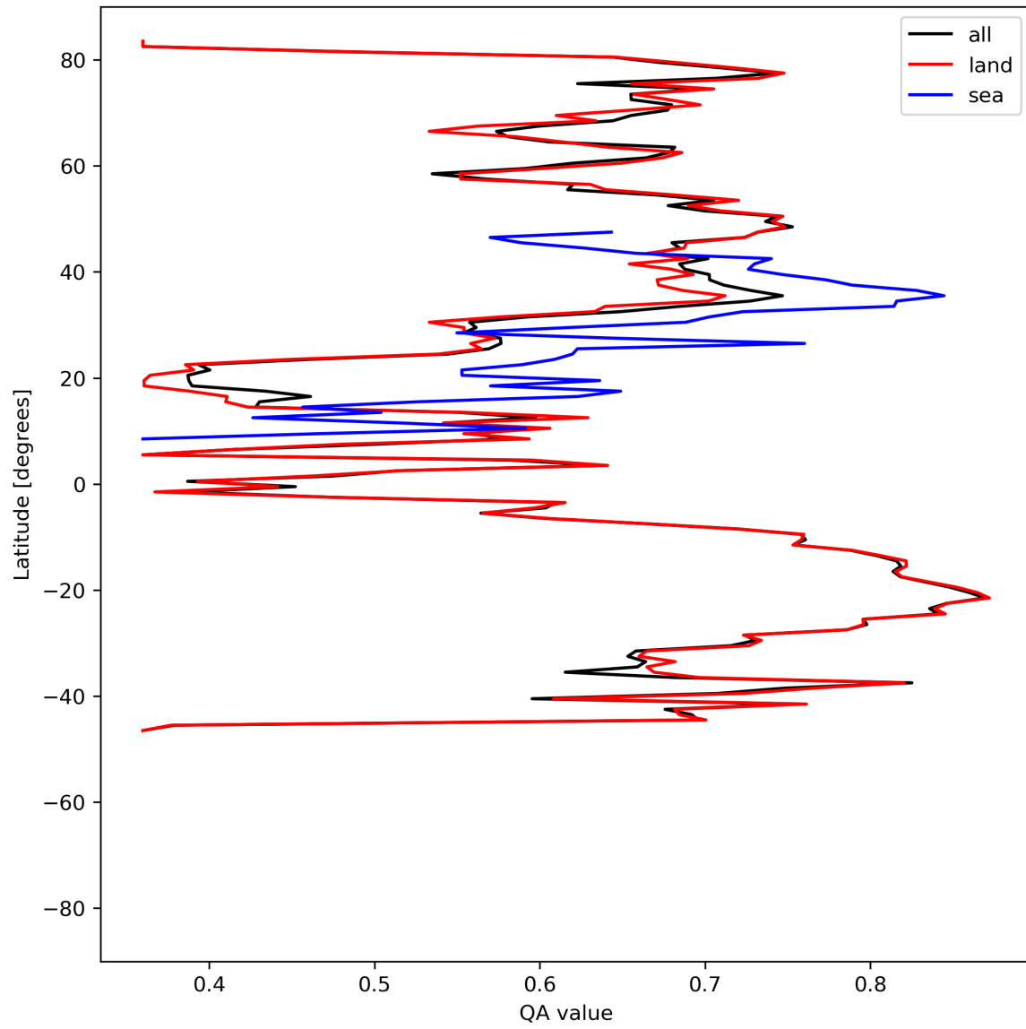
Figure 11: Zonal average of “QA value” for 2024-07-12 to 2024-07-14.
