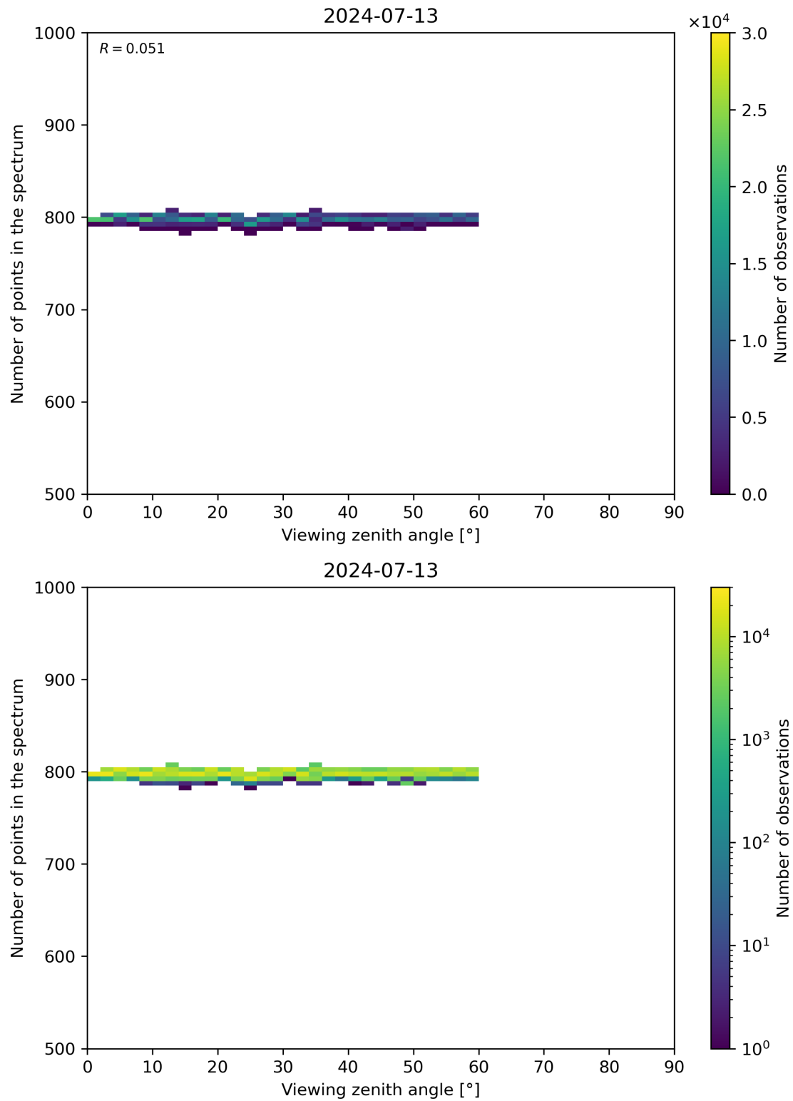
Figure 114: Scatter density plot of “Viewing zenith angle” against “Number of points in the spectrum” for 2024-07-12 to 2024-07-14.
