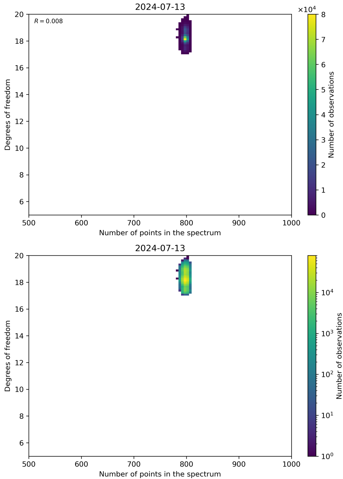
Figure 90: Scatter density plot of “Number of points in the spectrum” against “Degrees of freedom” for 2024-07-12 to 2024-07-14.
