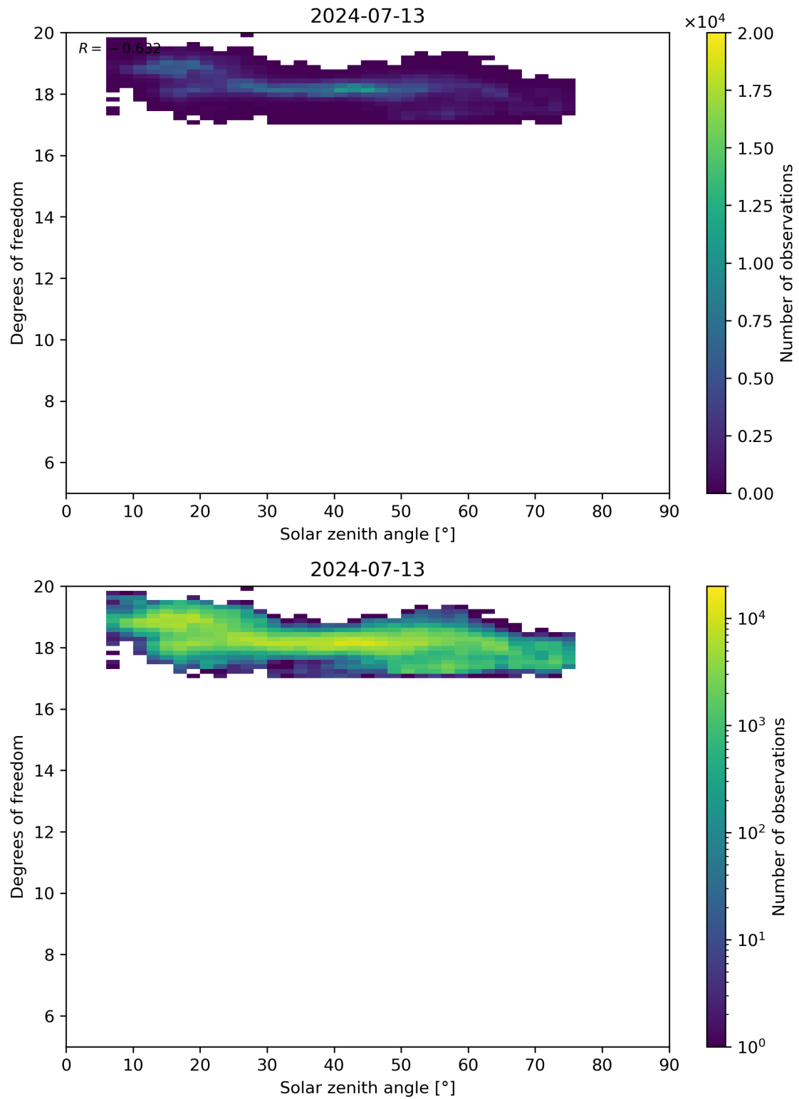
Figure 96: Scatter density plot of “Solar zenith angle” against “Degrees of freedom” for 2024-07-12 to 2024-07-14.
