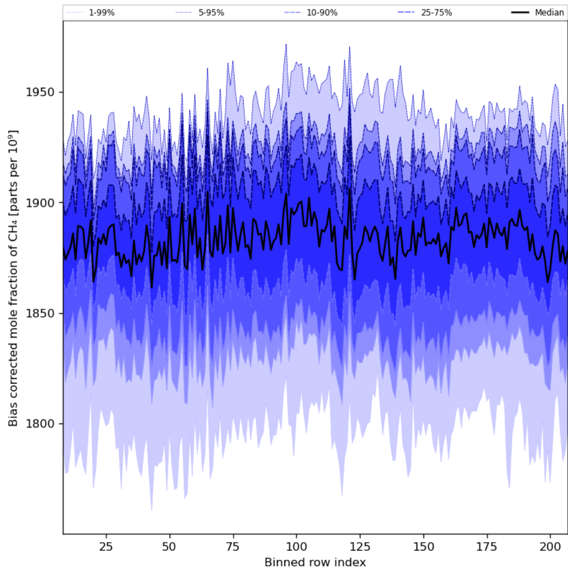
Figure 36: Along track statistics of “Bias corrected mole fraction of CH 4 ” for 2024-07-12 to 2024-07-14
