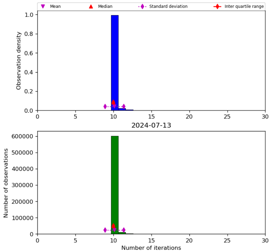
Figure 31: Histogram of “Number of iterations” for 2024-07-12 to 2024-07-14
