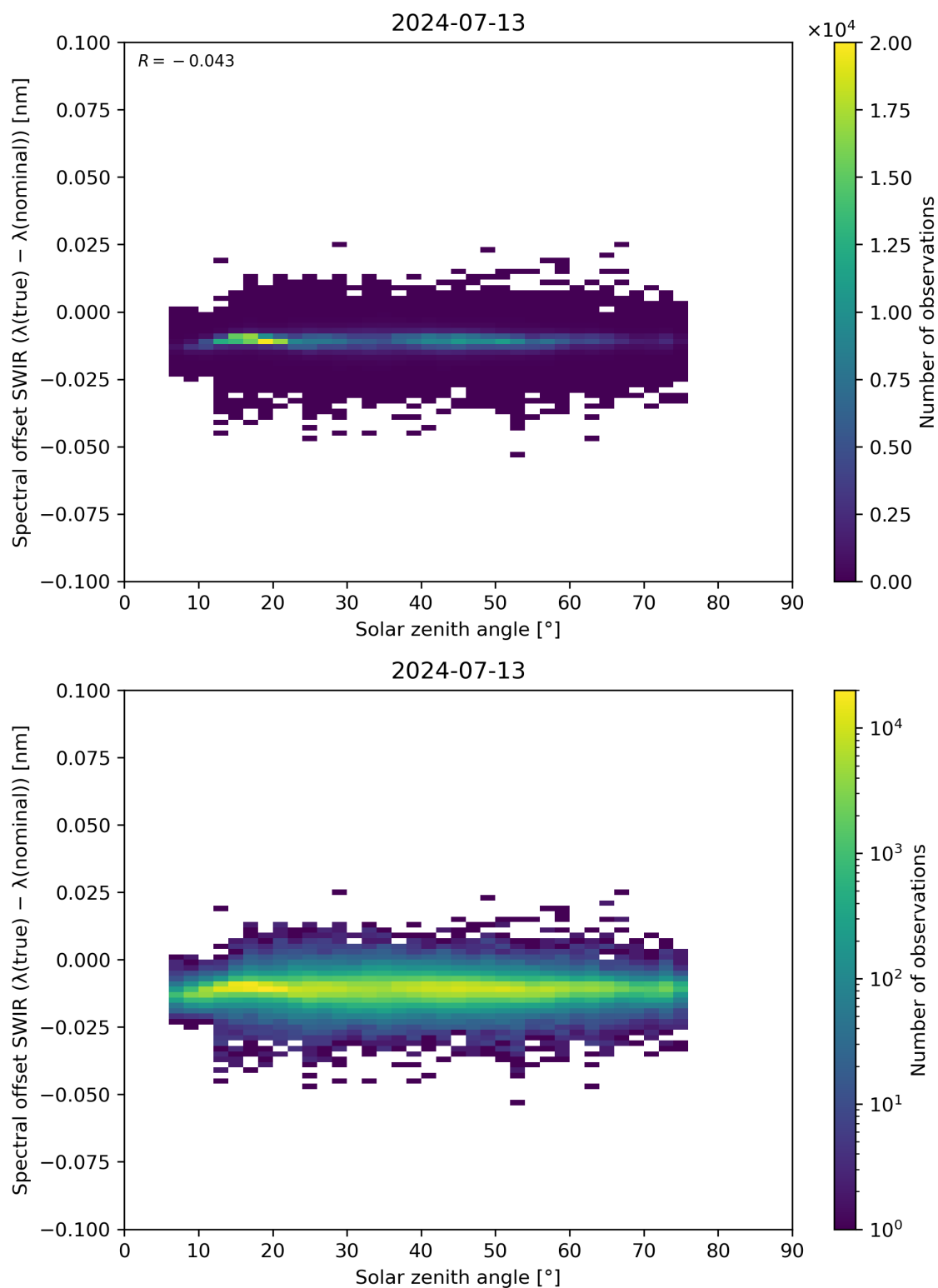
Figure 104: Scatter density plot of “Solar zenith angle” against “Spectral offset SWIR ( \lambda(\text{true}) - \lambda(\text{nominal}) )” for 2024-07-12 to 2024-07-14.
