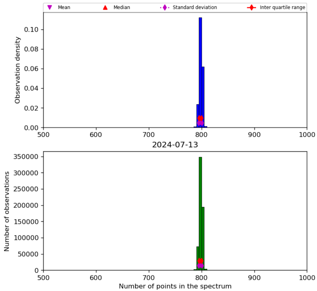
Figure 26: Histogram of “Number of points in the spectrum” for 2024-07-12 to 2024-07-14
