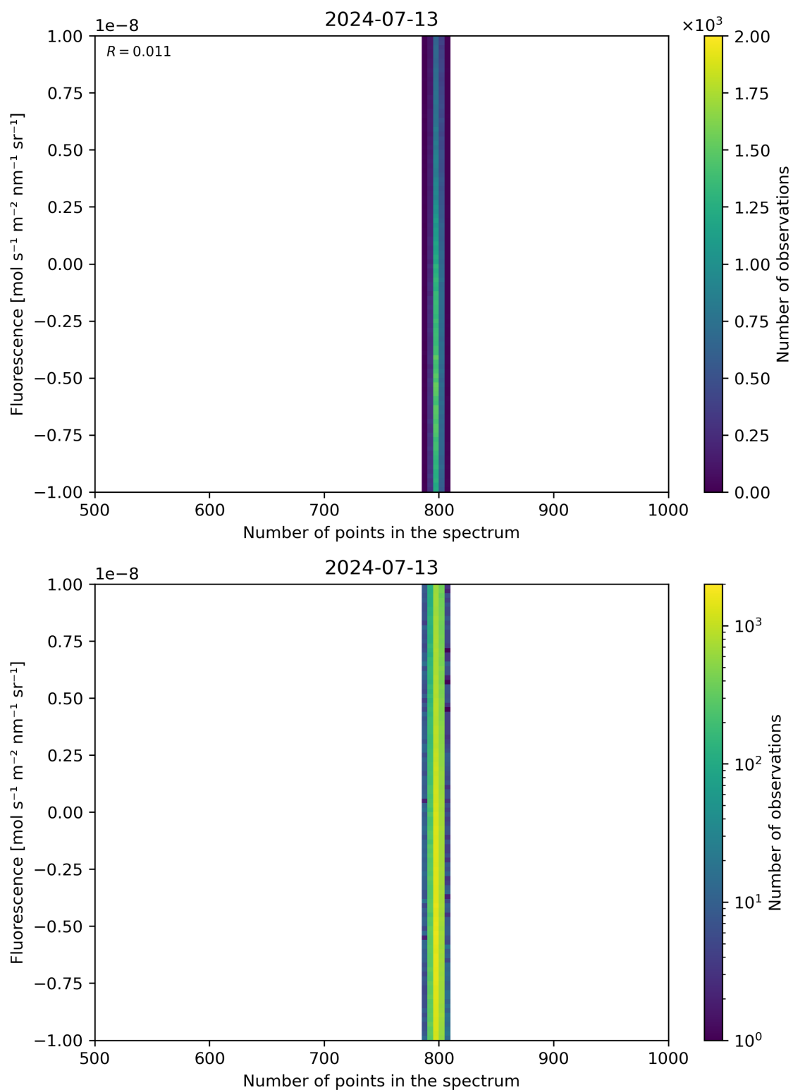
Figure 91: Scatter density plot of “Number of points in the spectrum” against “Fluorescence” for 2024-07-12 to 2024-07-14.
