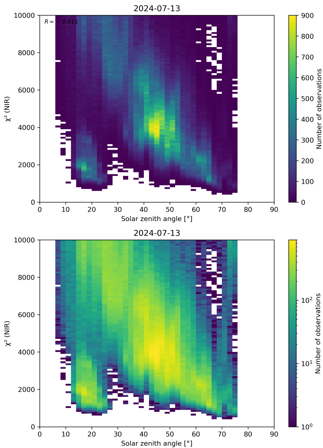
Figure 94: Scatter density plot of “Solar zenith angle” against “ \chi^2 (NIR)” for 2024-07-12 to 2024-07-14.
