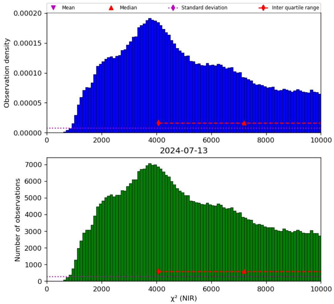
Figure 29: Histogram of “ \chi^2 (NIR)” for 2024-07-12 to 2024-07-14
