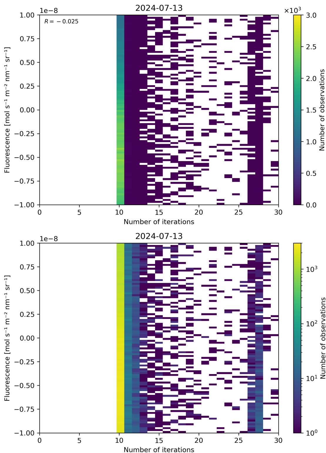
Figure 87: Scatter density plot of “Number of iterations” against “Fluorescence” for 2024-07-12 to 2024-07-14.
