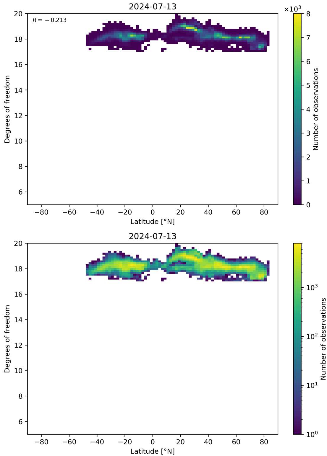
Figure 55: Scatter density plot of “Latitude” against “Degrees of freedom” for 2024-07-12 to 2024-07-14.
