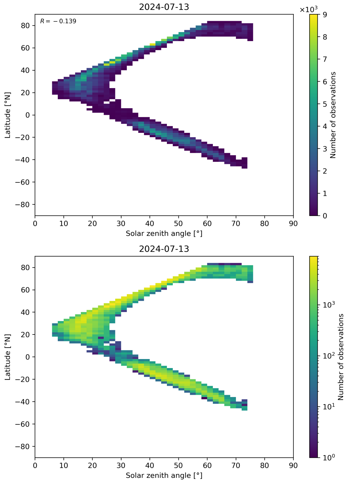
Figure 98: Scatter density plot of “Solar zenith angle” against “Latitude” for 2024-07-12 to 2024-07-14.
