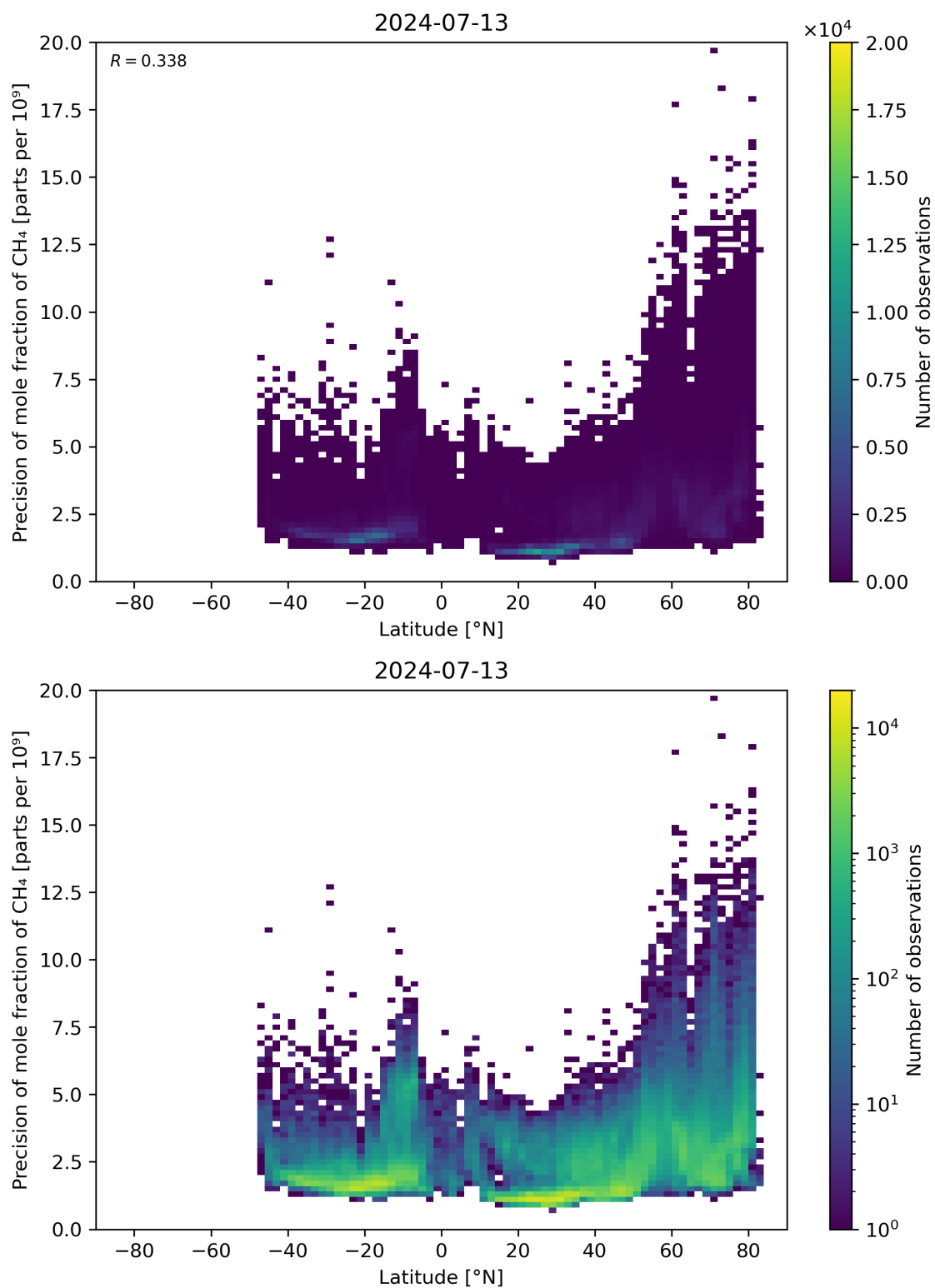
Figure 59: Scatter density plot of “Latitude” against “Precision of mole fraction of \text{CH}_4 ” for 2024-07-12 to 2024-07-14.
