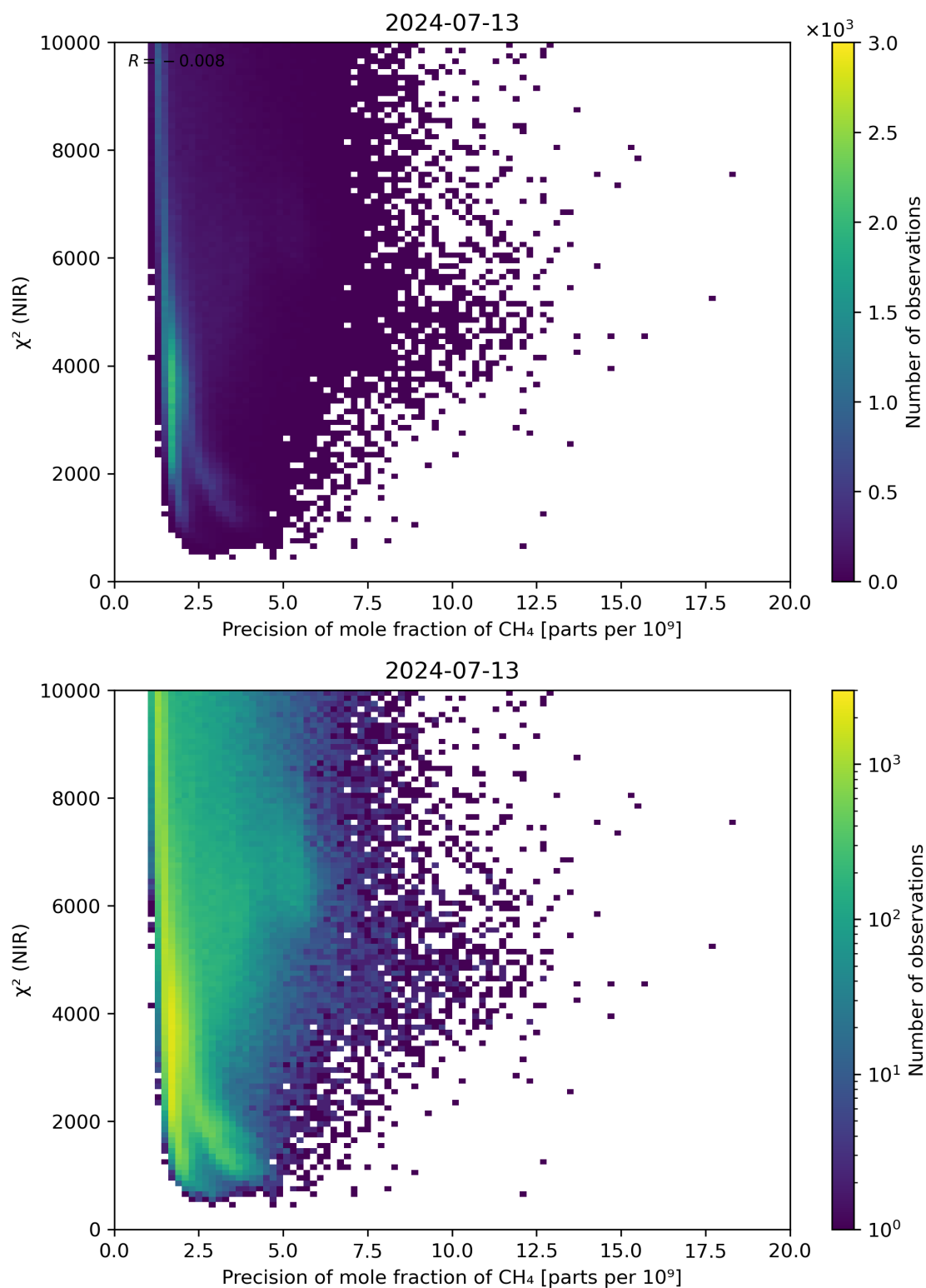
Figure 78: Scatter density plot of “Precision of mole fraction of CH 4 ” against “ \chi^2 (NIR)” for 2024-07-12 to 2024-07-14.
