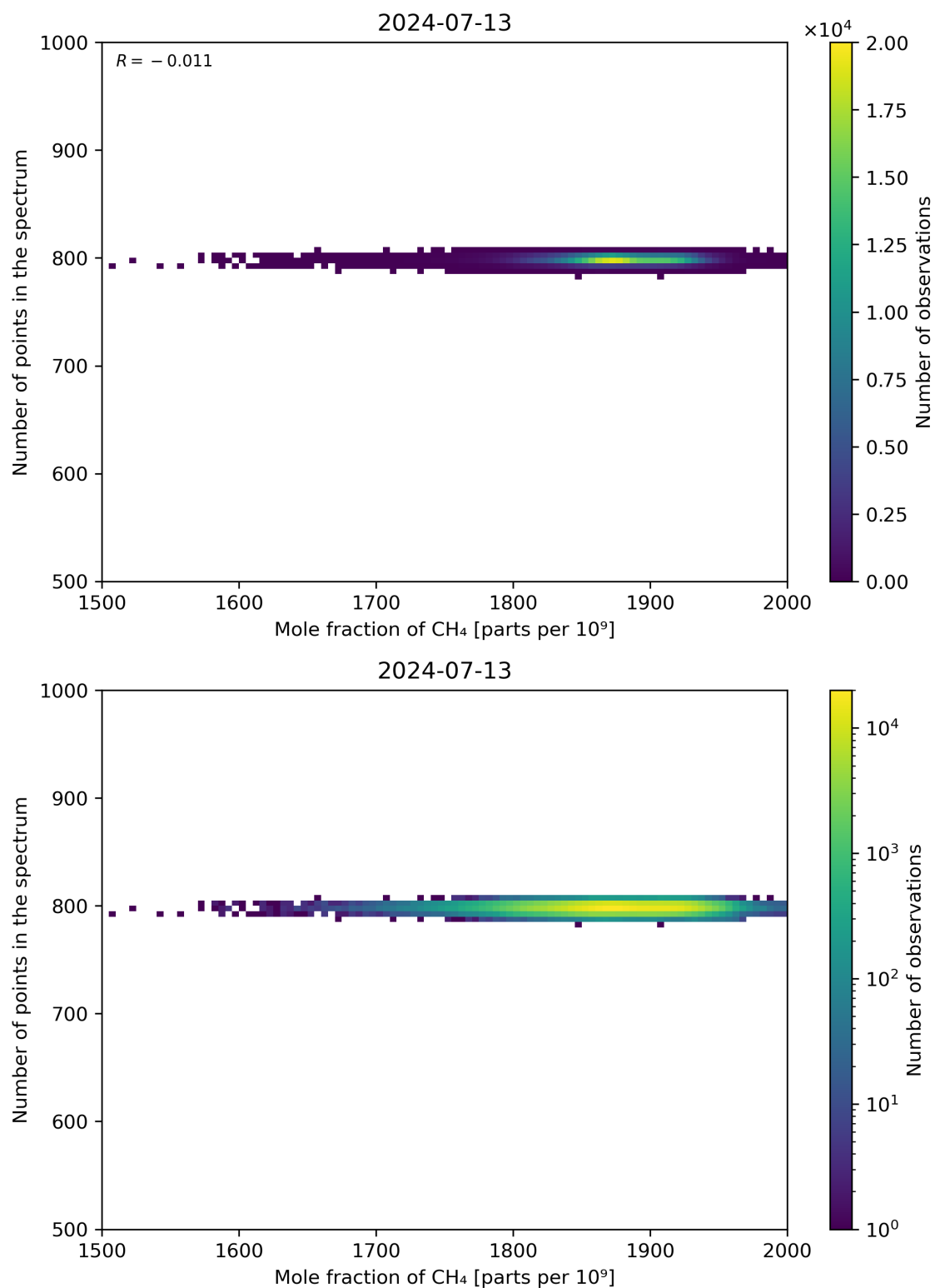
Figure 77: Scatter density plot of “Mole fraction of CH 4 ” against “Number of points in the spectrum” for 2024-07-12 to 2024-07-14.
