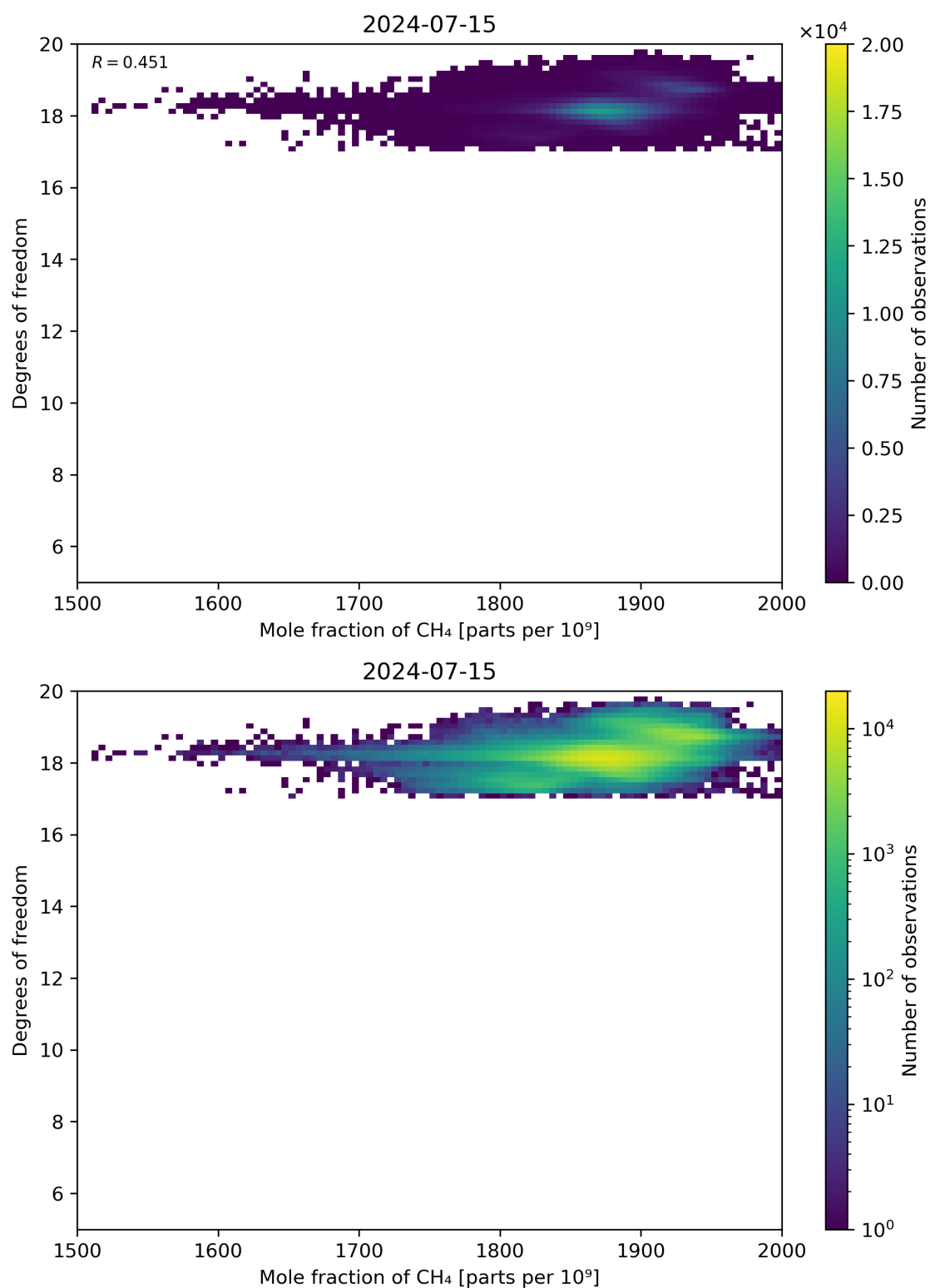
Figure 72: Scatter density plot of “Mole fraction of CH 4 ” against “Degrees of freedom” for 2024-07-15 to 2024-07-16.
