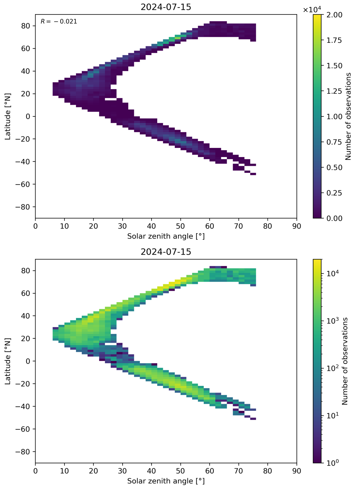
Figure 98: Scatter density plot of “Solar zenith angle” against “Latitude” for 2024-07-15 to 2024-07-16.
