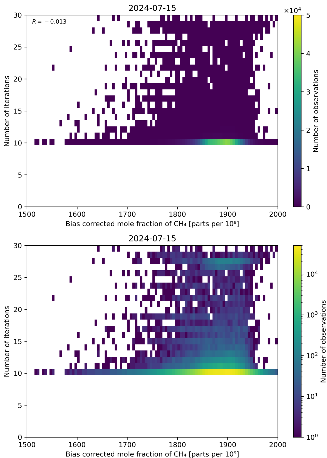
Figure 67: Scatter density plot of “Bias corrected mole fraction of CH 4 ” against “Number of iterations” for 2024-07-15 to 2024-07-16.
