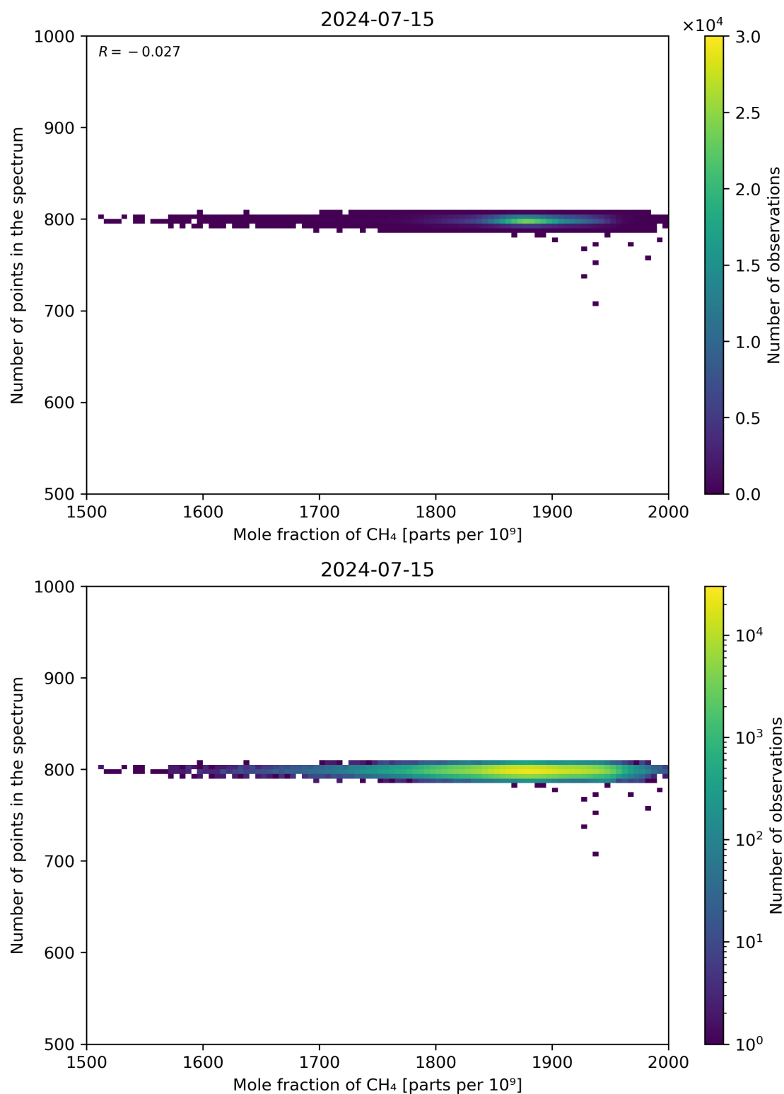
Figure 77: Scatter density plot of “Mole fraction of CH 4 ” against “Number of points in the spectrum” for 2024-07-15 to 2024-07-16.
