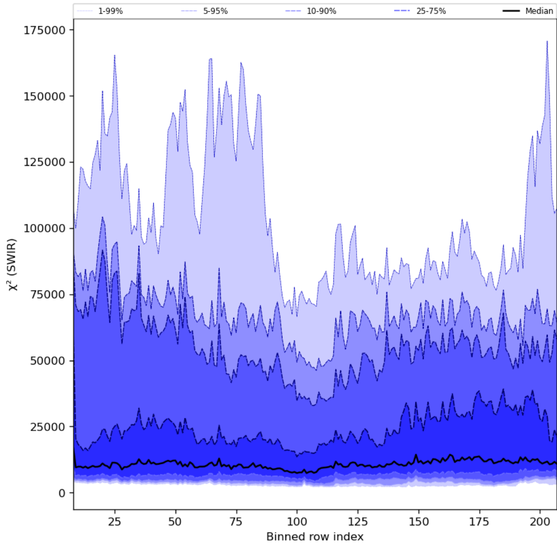
Figure 39: Along track statistics of “ \chi^2 (SWIR)” for 2024-07-15 to 2024-07-16
