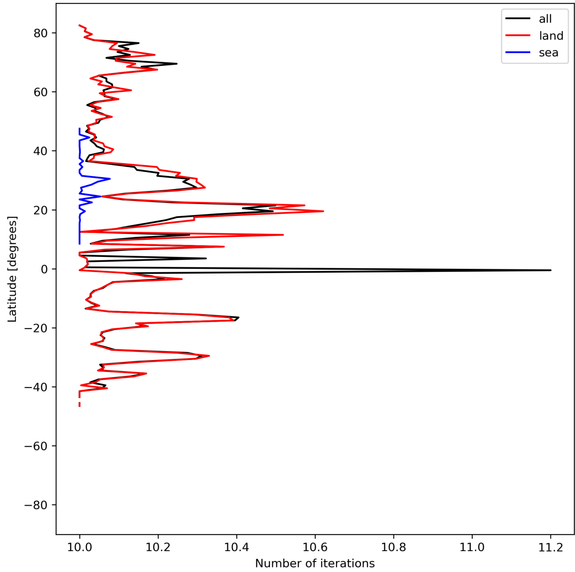
Figure 20: Zonal average of “Number of iterations” for 2024-07-15 to 2024-07-16.
