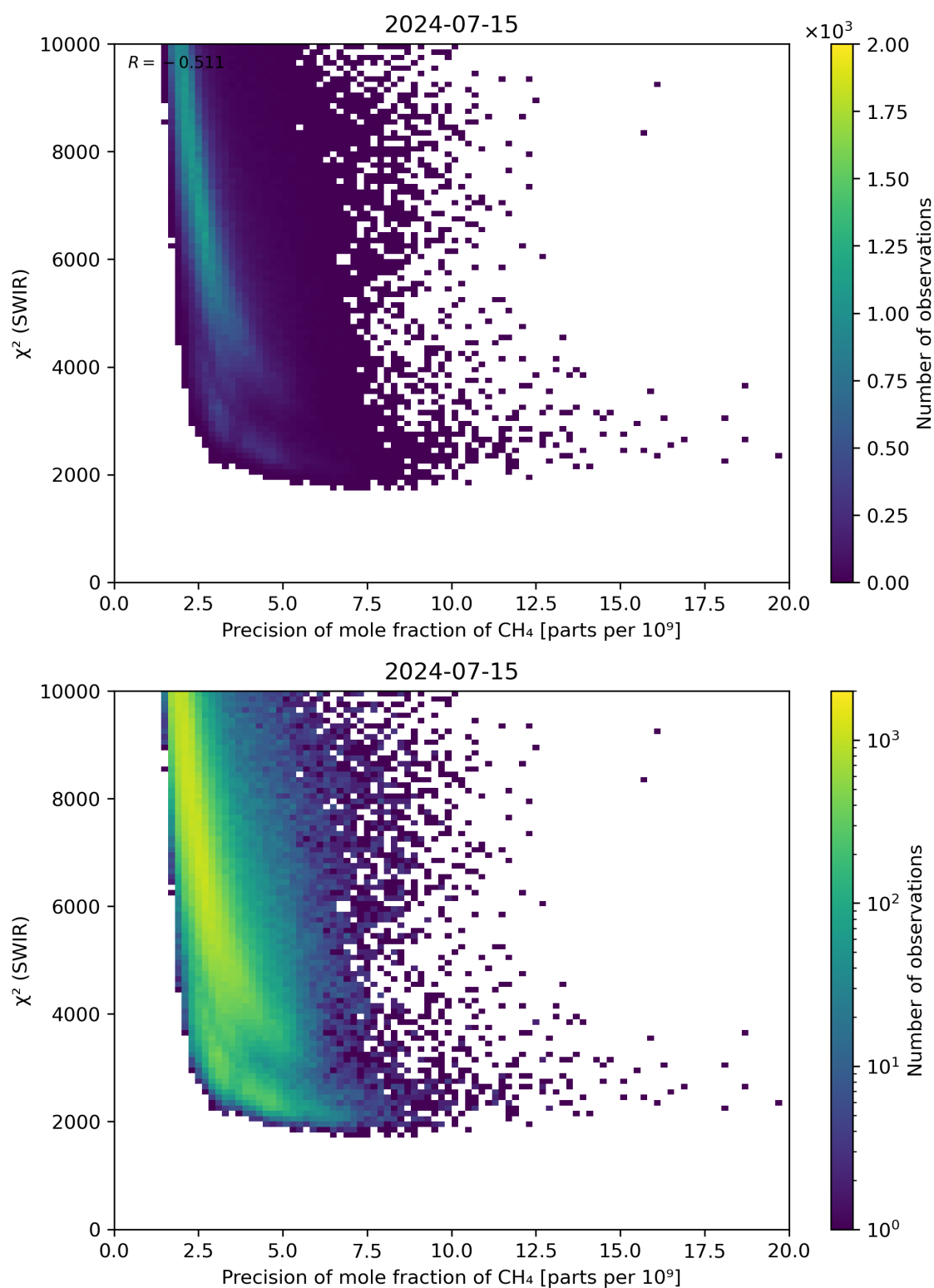
Figure 79: Scatter density plot of “Precision of mole fraction of \text{CH}_4 ” against “ \chi^2 (SWIR)” for 2024-07-15 to 2024-07-16.
