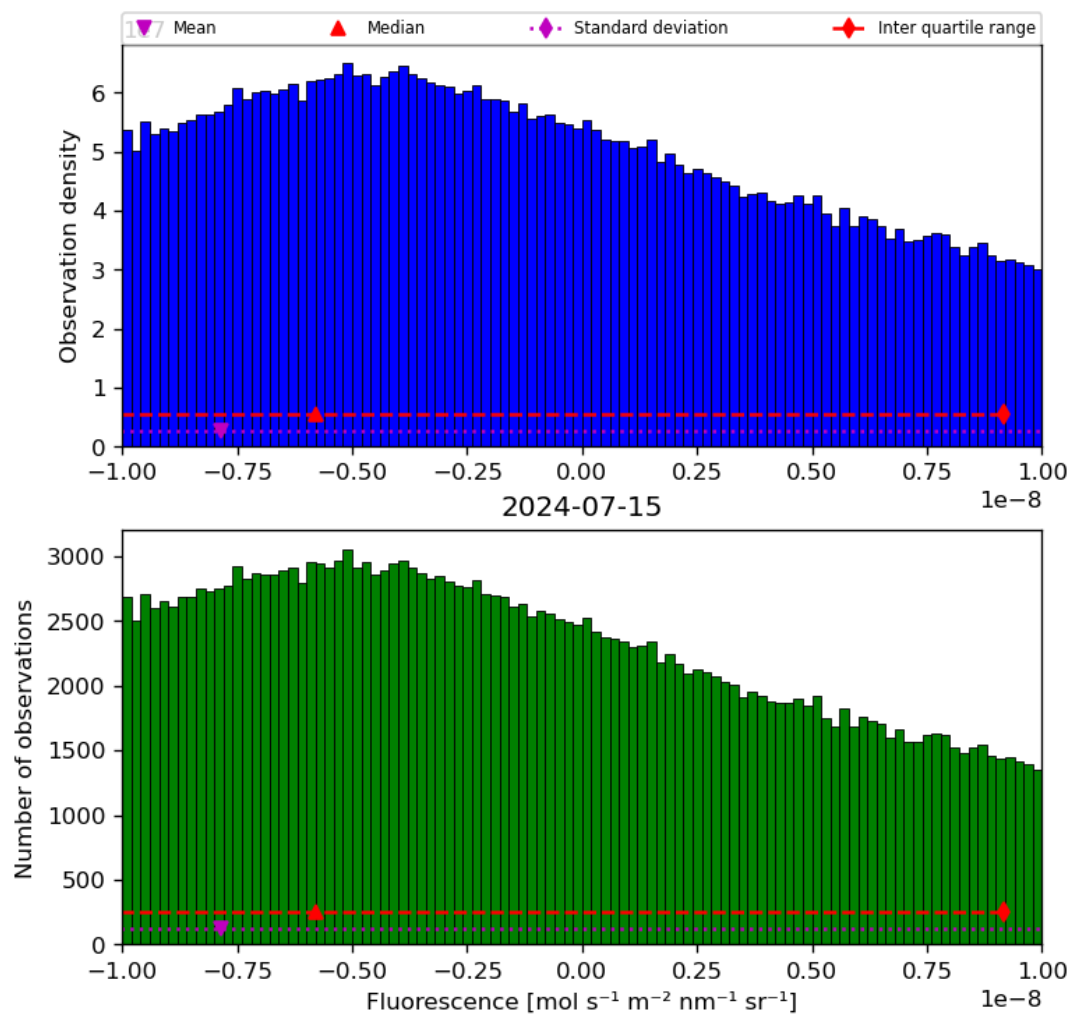
Figure 32: Histogram of “Fluorescence” for 2024-07-15 to 2024-07-16
