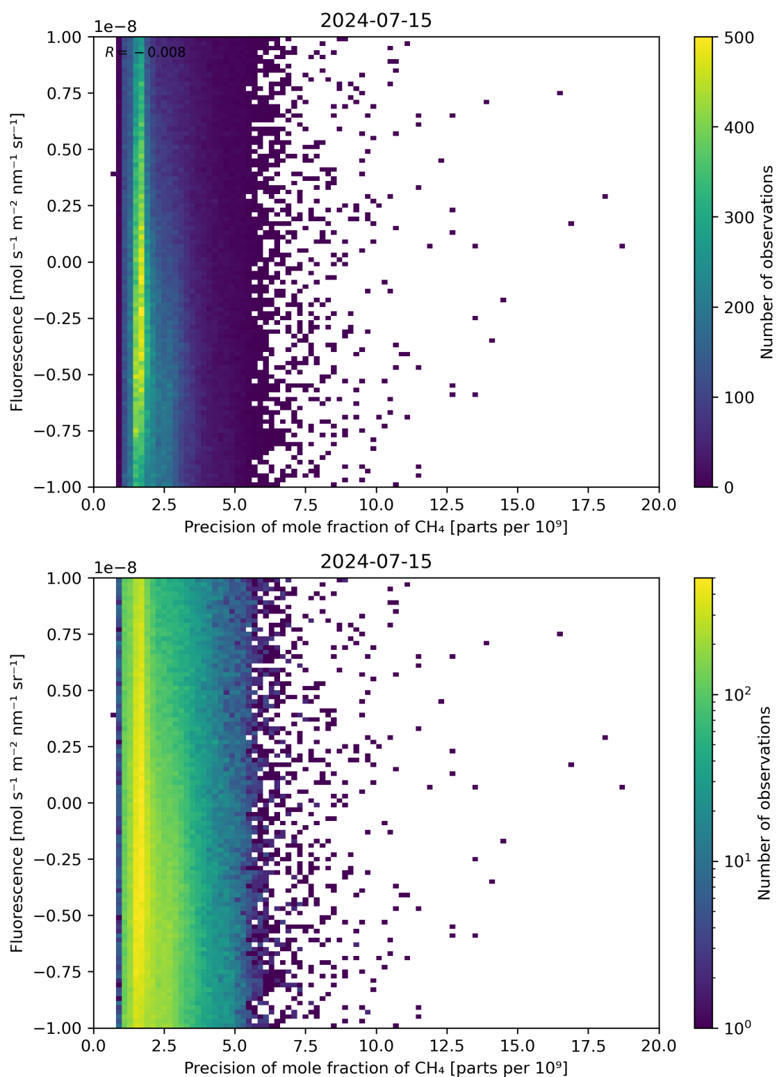
Figure 81: Scatter density plot of “Precision of mole fraction of CH 4 ” against “Fluorescence” for 2024-07-15 to 2024-07-16.
