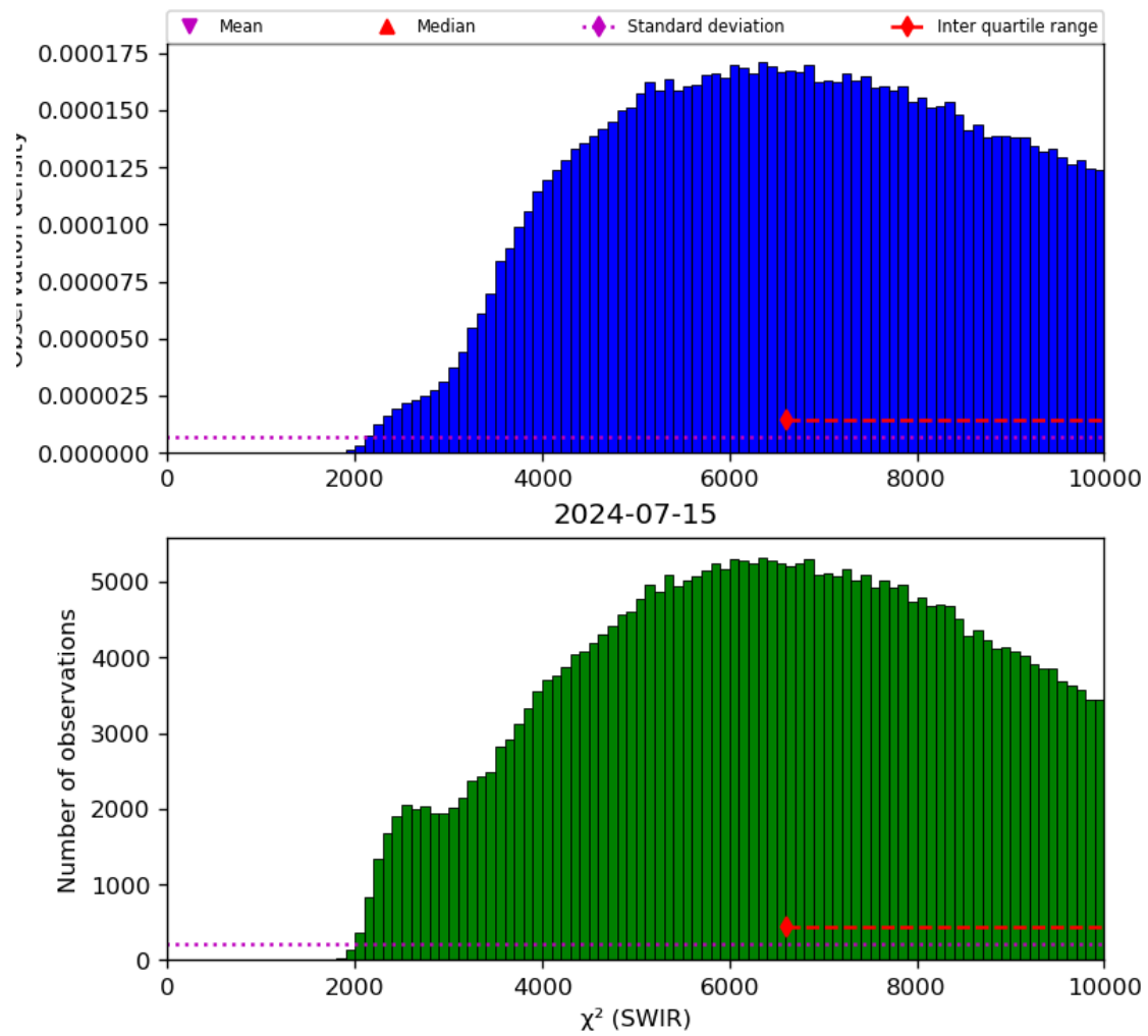
Figure 28: Histogram of “ \chi^2 (SWIR)” for 2024-07-15 to 2024-07-16
