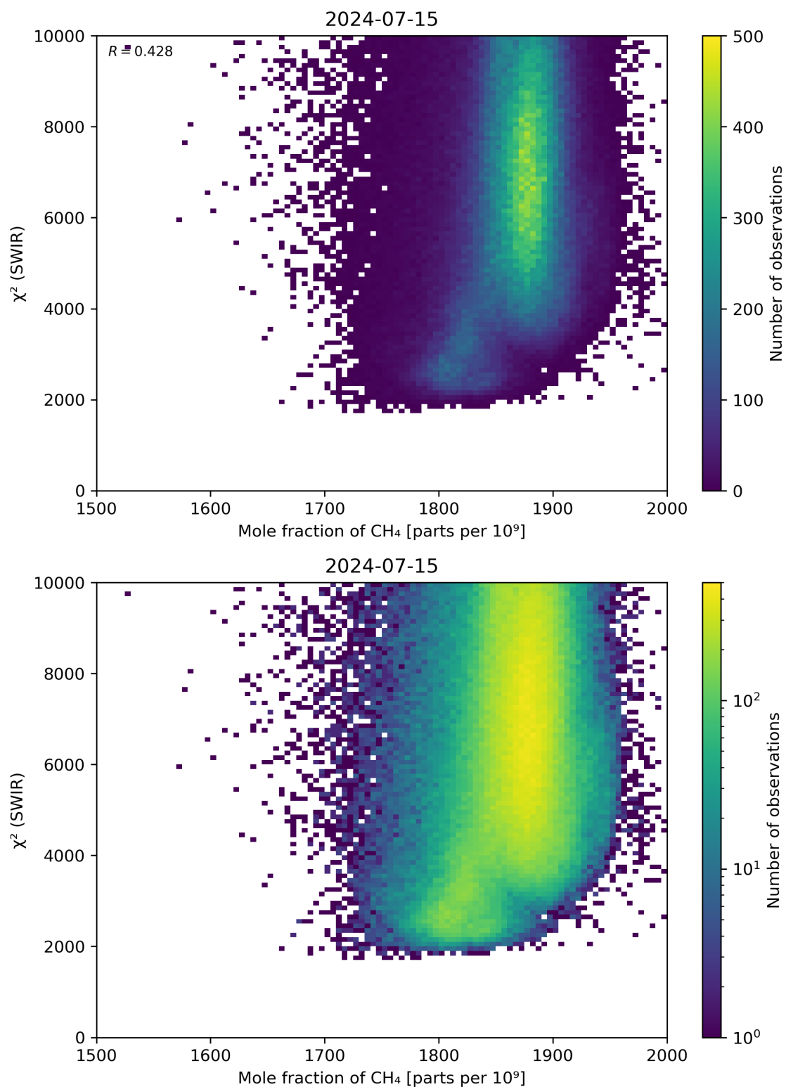
Figure 71: Scatter density plot of “Mole fraction of \text{CH}_4 ” against “ \chi^2 (SWIR)” for 2024-07-15 to 2024-07-16.
