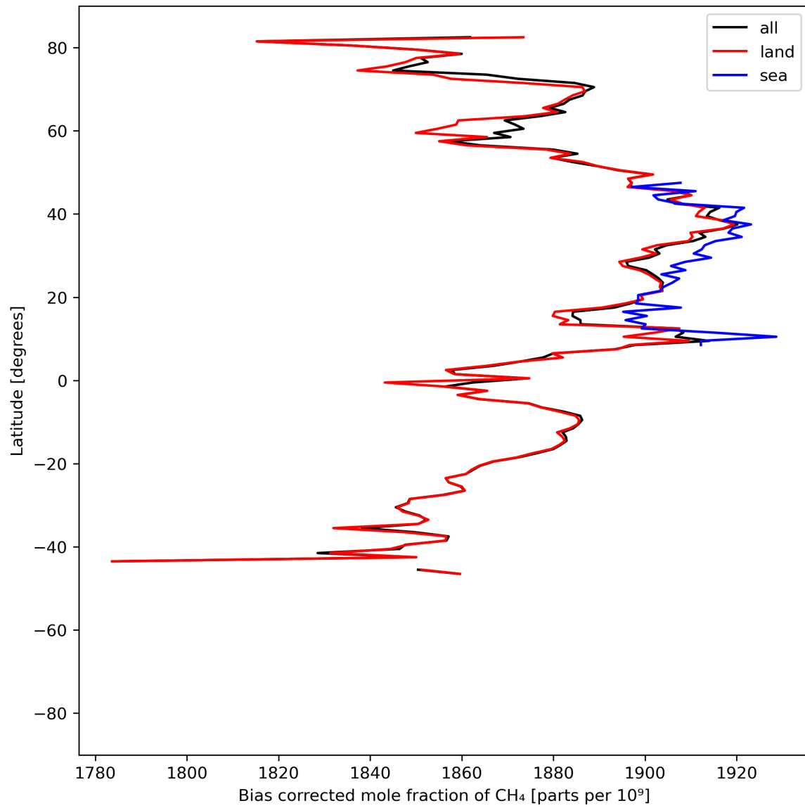
Figure 14: Zonal average of “Bias corrected mole fraction of \text{CH}_4 ” for 2024-07-15 to 2024-07-16.
