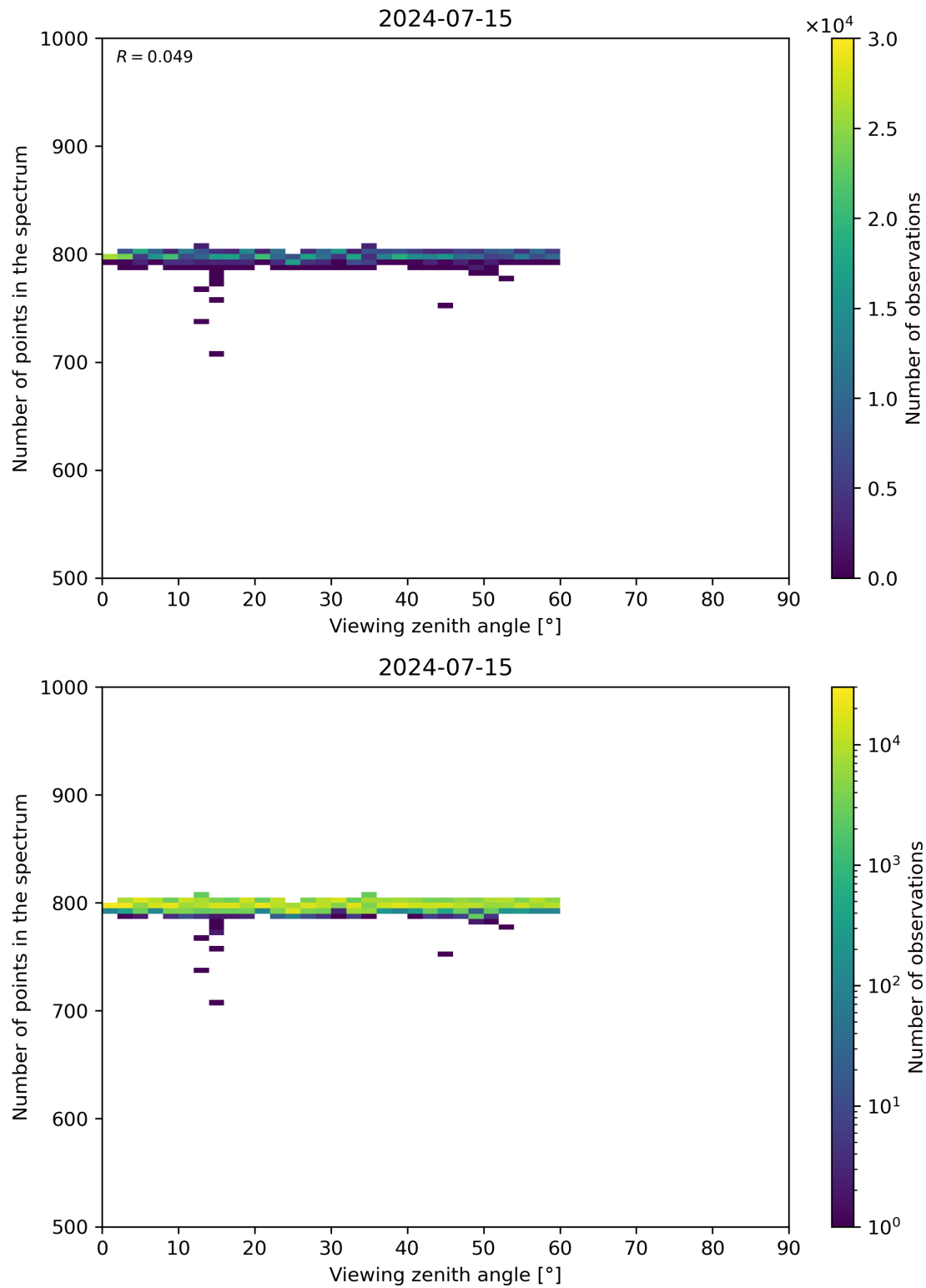
Figure 114: Scatter density plot of “Viewing zenith angle” against “Number of points in the spectrum” for 2024-07-15 to 2024-07-16.
