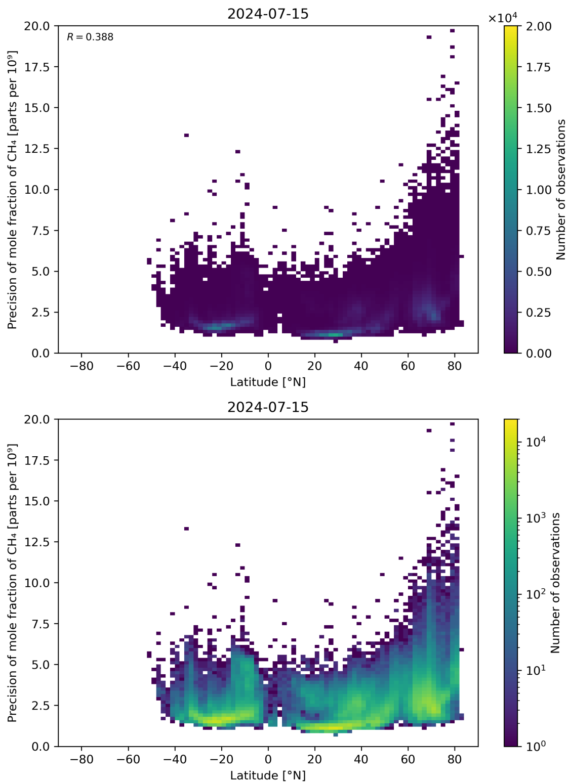
Figure 59: Scatter density plot of “Latitude” against “Precision of mole fraction of CH 4 ” for 2024-07-15 to 2024-07-16.
