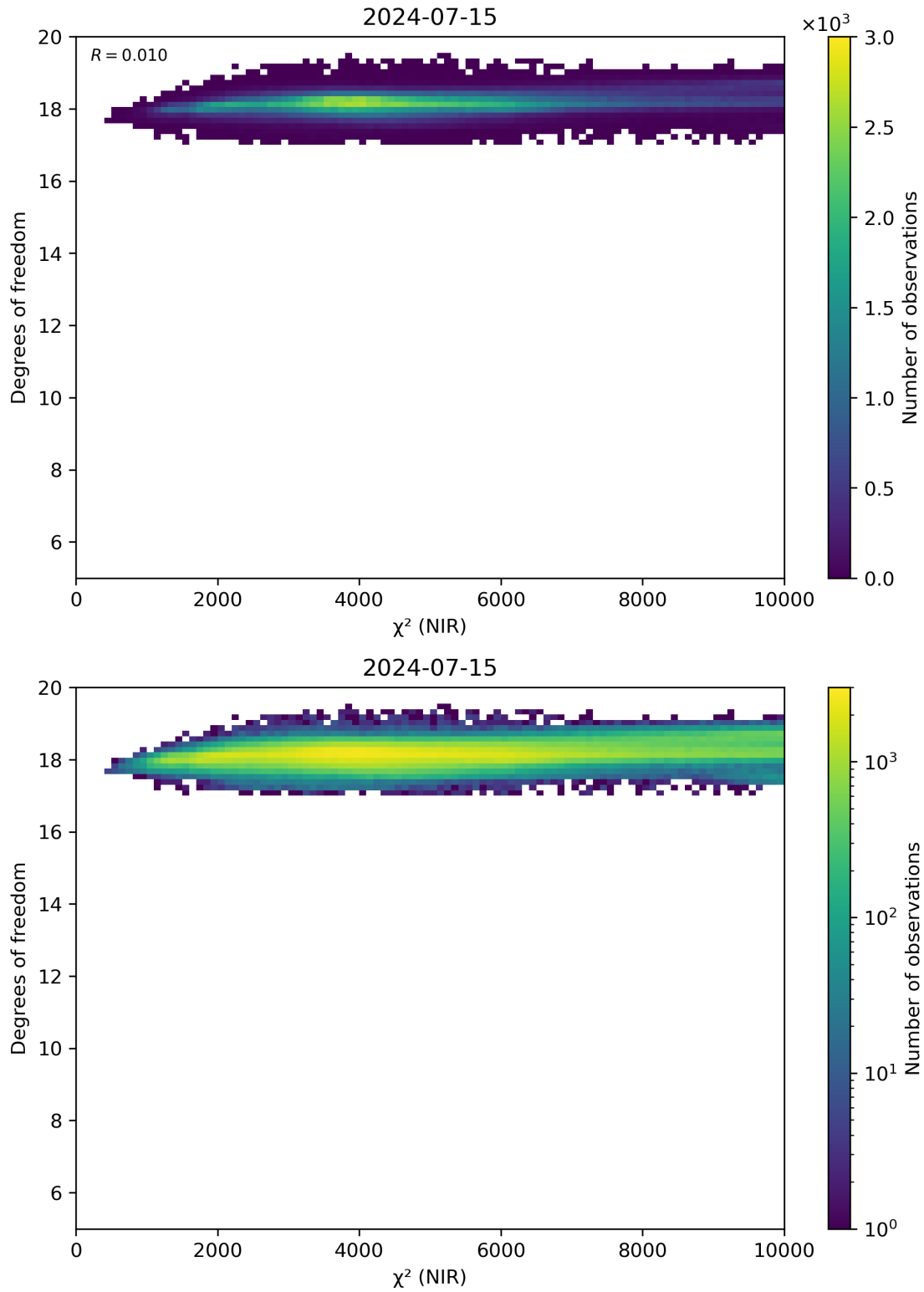
Figure 44: Scatter density plot of “ \chi^2 (NIR)” against “Degrees of freedom” for 2024-07-15 to 2024-07-16.
