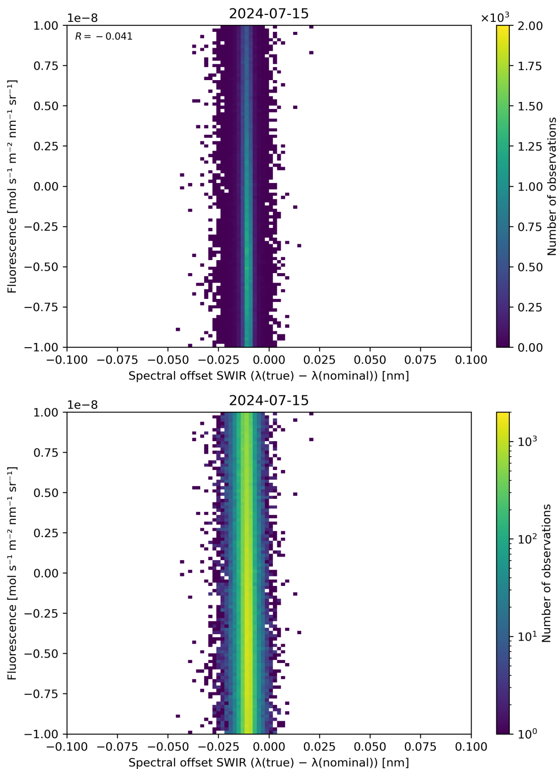
Figure 120: Scatter density plot of “Spectral offset SWIR ( \lambda(\text{true}) - \lambda(\text{nominal}) )” against “Fluorescence” for 2024-07-15 to 2024-07-16.
