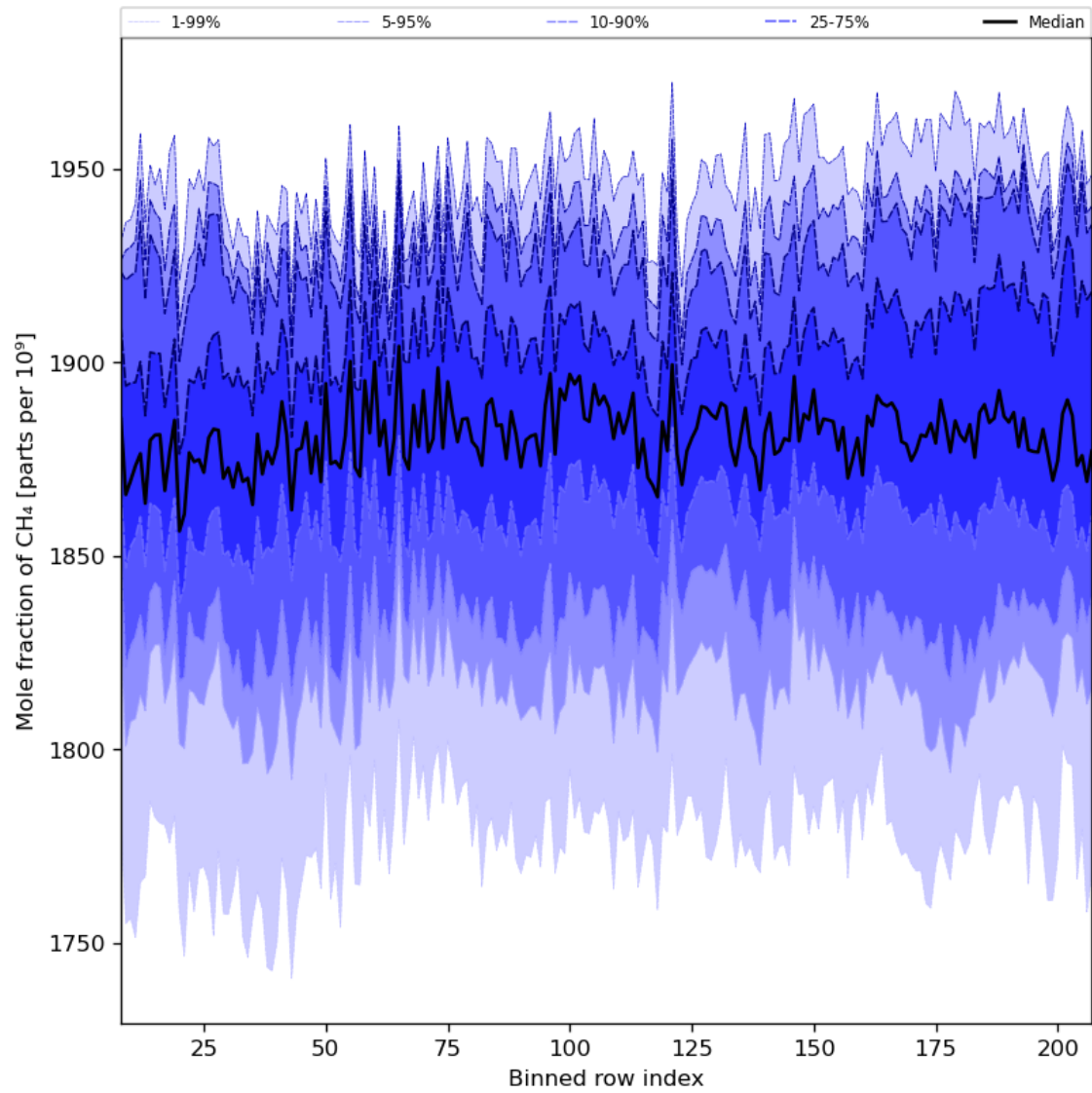
Figure 34: Along track statistics of “Mole fraction of CH 4 ” for 2024-07-15 to 2024-07-16
