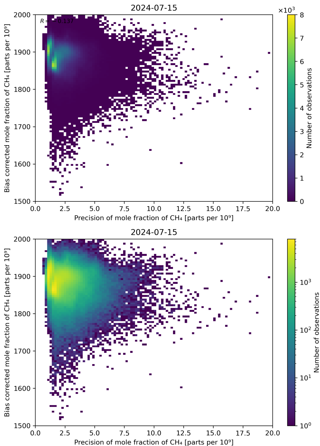
Figure 82: Scatter density plot of “Precision of mole fraction of CH 4 ” against “Bias corrected mole fraction of CH 4 ” for 2024-07-15 to 2024-07-16.
