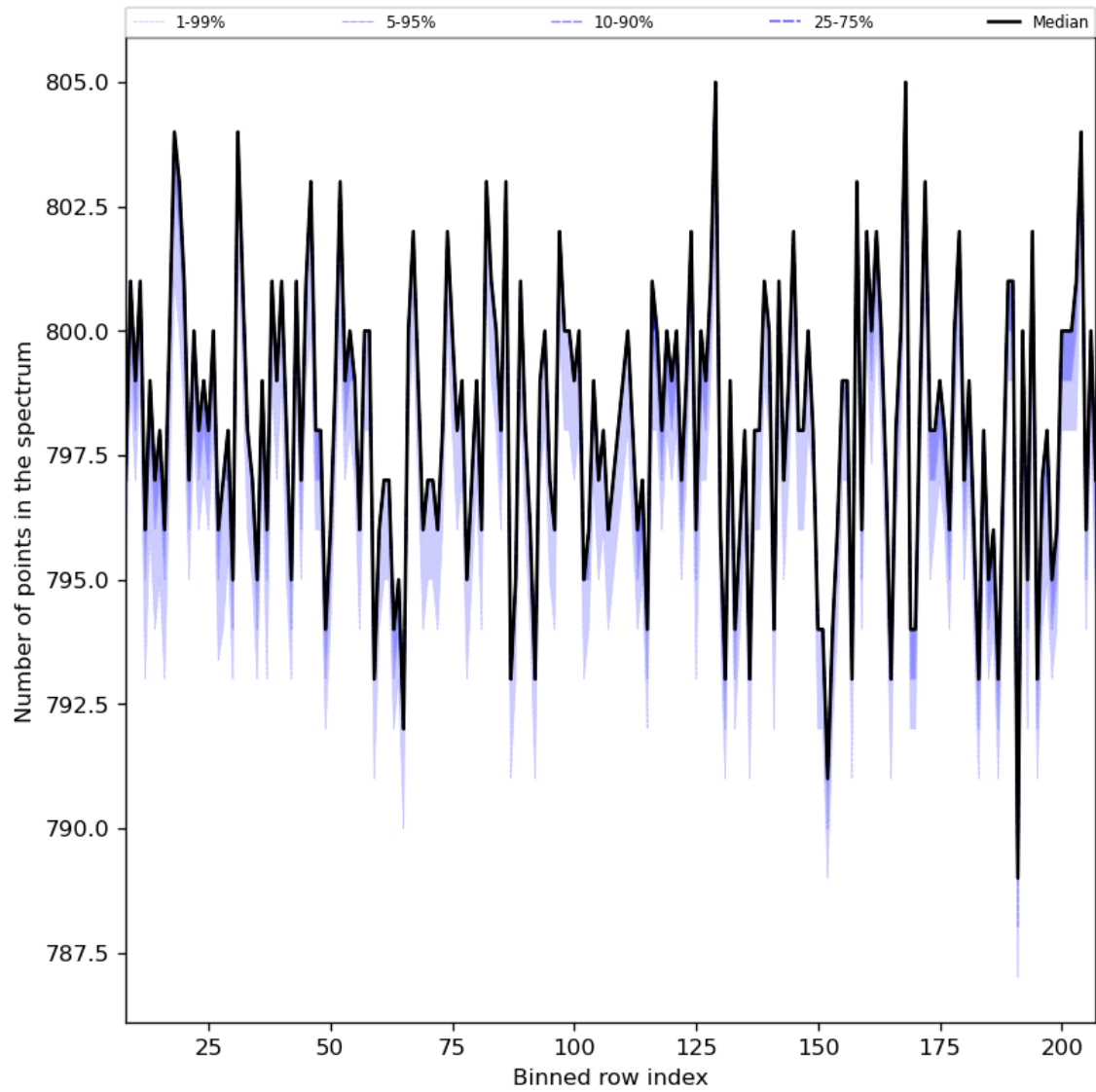
Figure 37: Along track statistics of “Number of points in the spectrum” for 2024-07-15 to 2024-07-16
