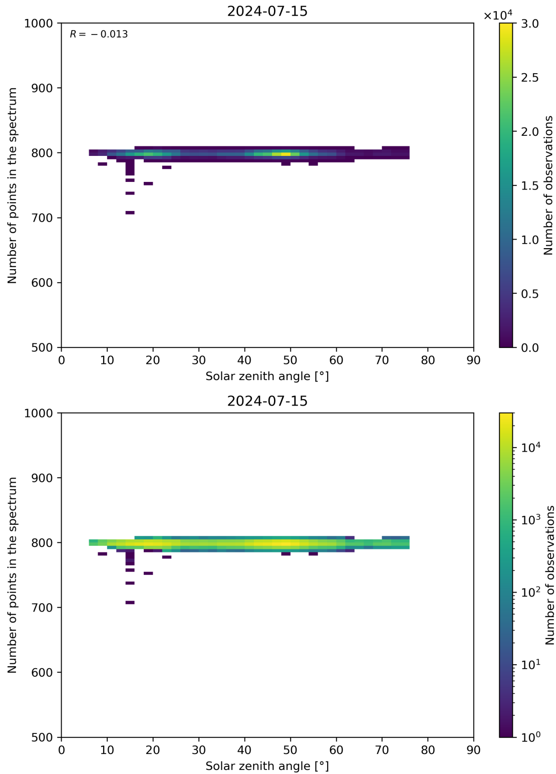
Figure 103: Scatter density plot of “Solar zenith angle” against “Number of points in the spectrum” for 2024-07-15 to 2024-07-16.
