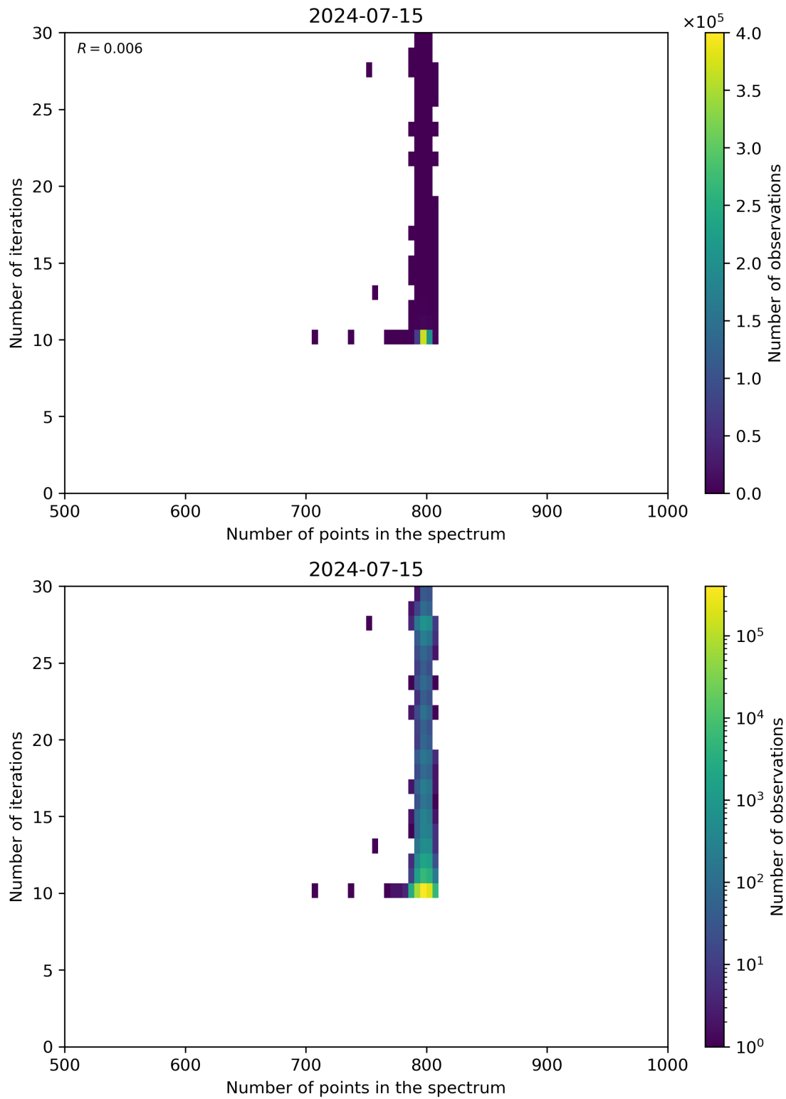
Figure 92: Scatter density plot of “Number of points in the spectrum” against “Number of iterations” for 2024-07-15 to 2024-07-16.
