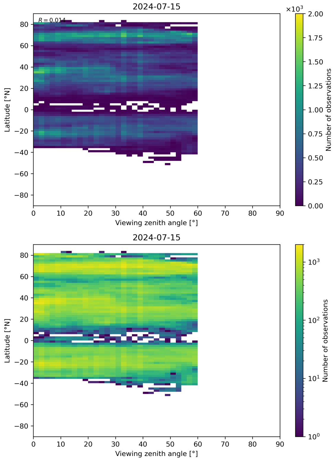
Figure 109: Scatter density plot of “Viewing zenith angle” against “Latitude” for 2024-07-15 to 2024-07-16.
