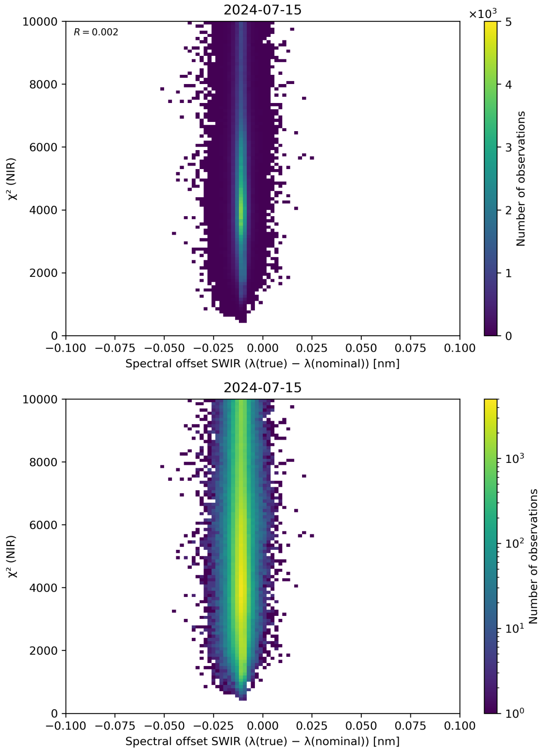
Figure 117: Scatter density plot of “Spectral offset SWIR ( \lambda(\text{true}) - \lambda(\text{nominal}) )” against “ \chi^2 (NIR)” for 2024-07-15 to 2024-07-16.
