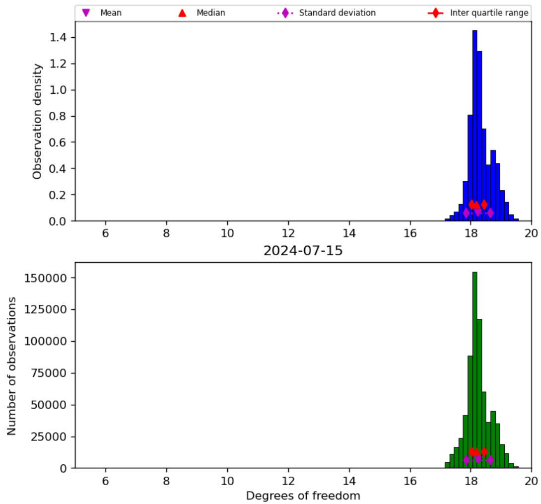
Figure 30: Histogram of “Degrees of freedom” for 2024-07-15 to 2024-07-16
