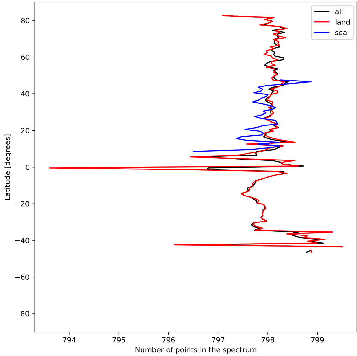
Figure 15: Zonal average of “Number of points in the spectrum” for 2024-07-15 to 2024-07-16.
