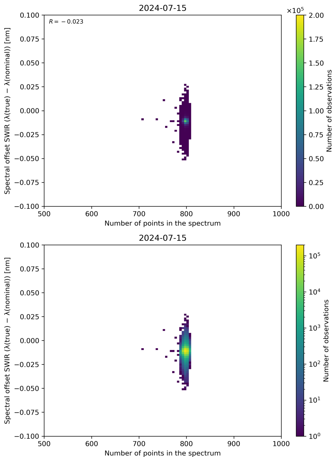
Figure 93: Scatter density plot of “Number of points in the spectrum” against “Spectral offset SWIR ( \lambda(\text{true}) - \lambda(\text{nominal}) )” for 2024-07-15 to 2024-07-16.
