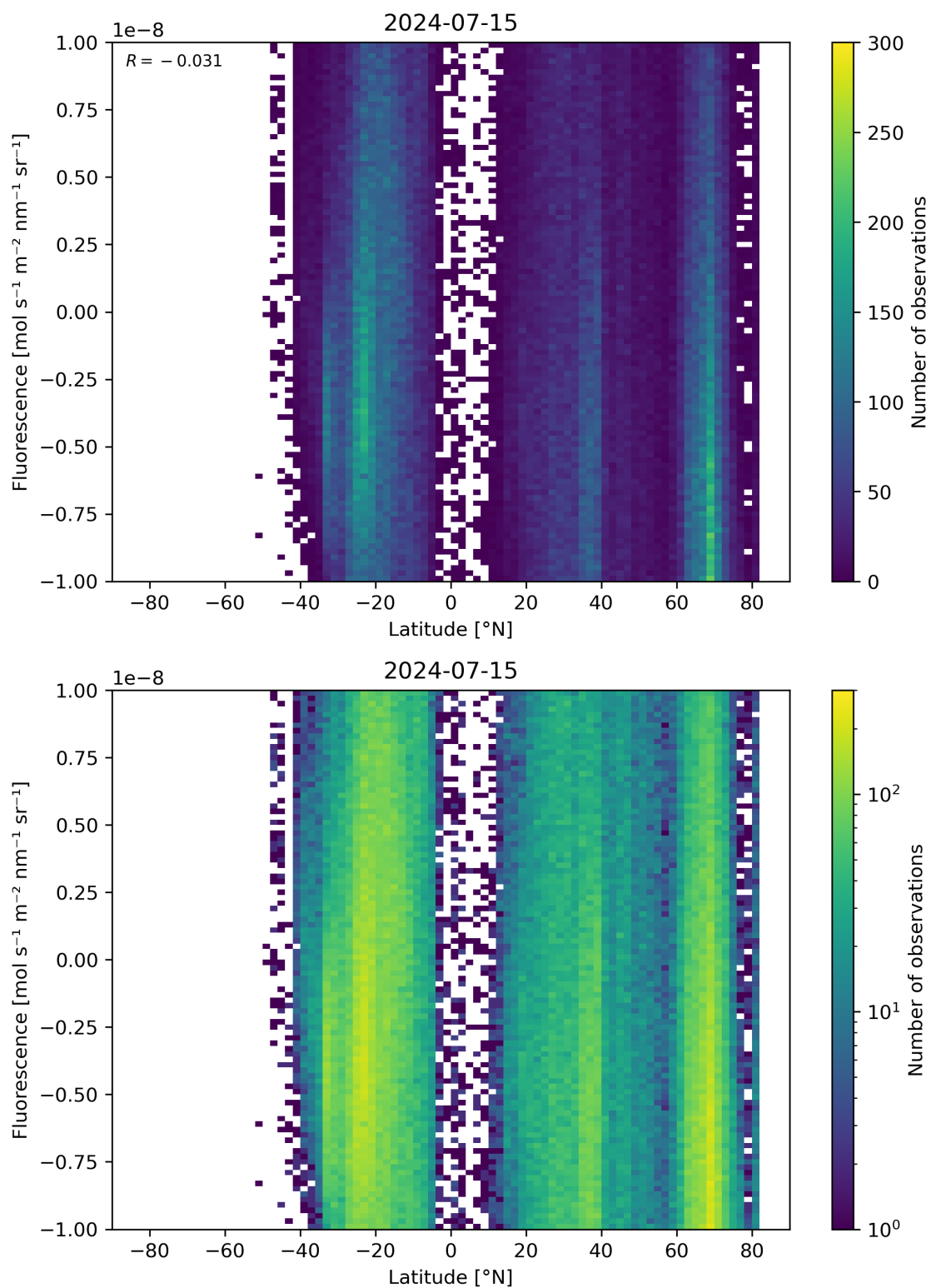
Figure 56: Scatter density plot of “Latitude” against “Fluorescence” for 2024-07-15 to 2024-07-16.
