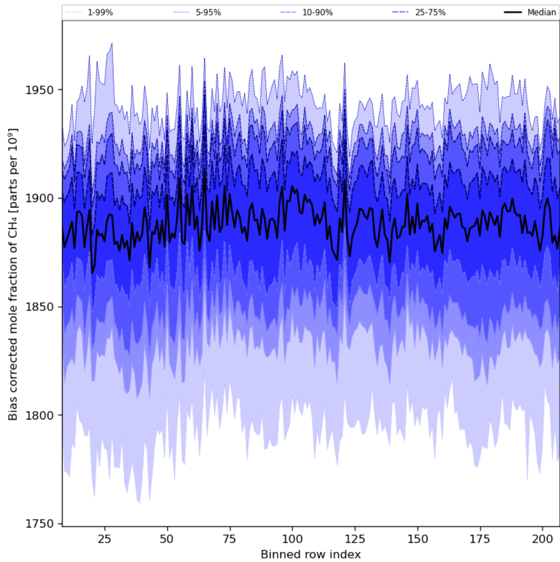
Figure 36: Along track statistics of “Bias corrected mole fraction of CH 4 ” for 2024-07-15 to 2024-07-16
