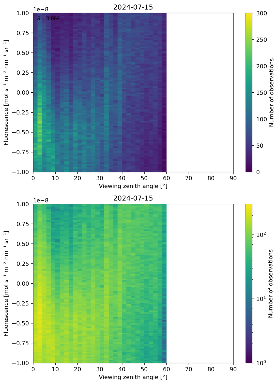
Figure 108: Scatter density plot of “Viewing zenith angle” against “Fluorescence” for 2024-07-15 to 2024-07-16.
