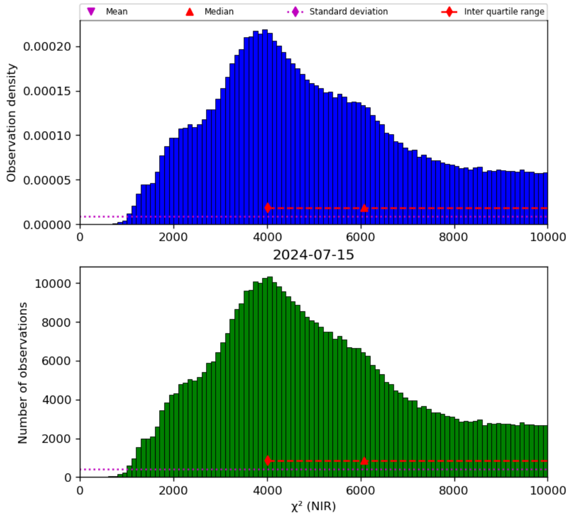
Figure 29: Histogram of “ \chi^2 (NIR)” for 2024-07-15 to 2024-07-16
