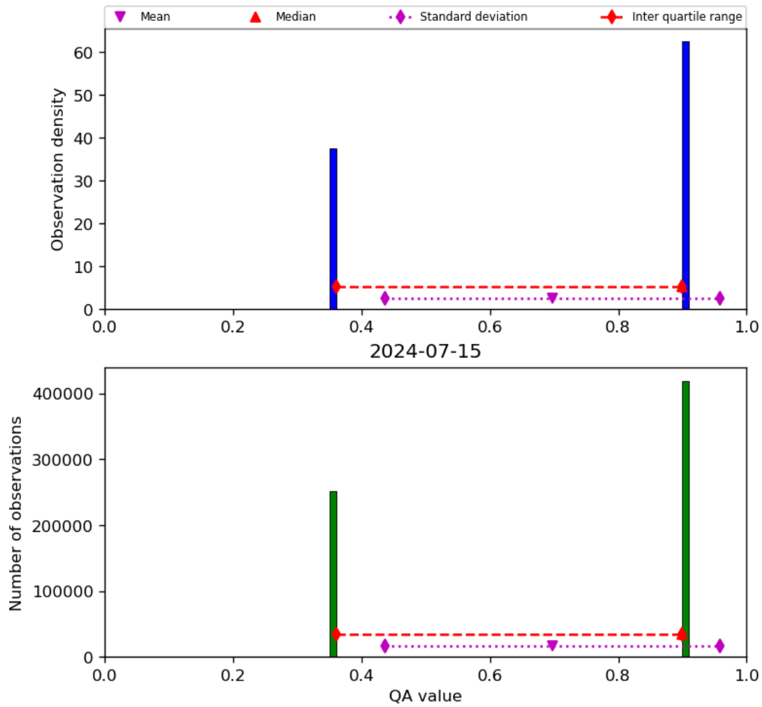
Figure 22: Histogram of “QA value” for 2024-07-15 to 2024-07-16
