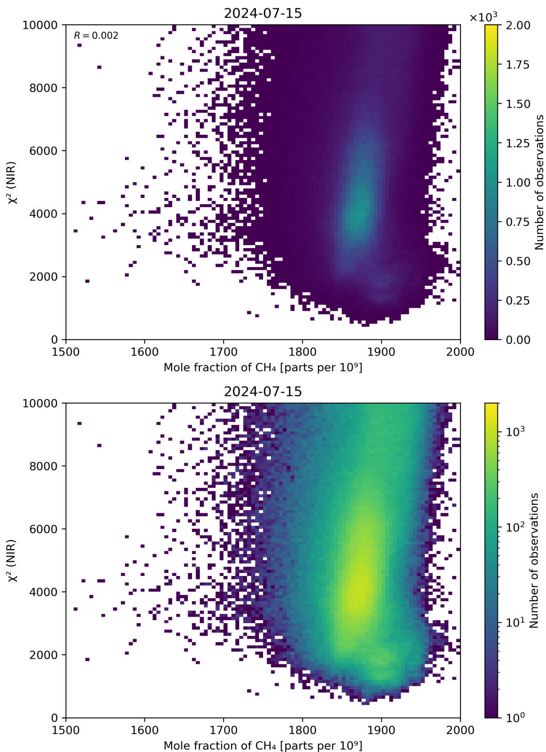
Figure 70: Scatter density plot of “Mole fraction of \text{CH}_4 ” against “ \chi^2 (NIR)” for 2024-07-15 to 2024-07-16.
