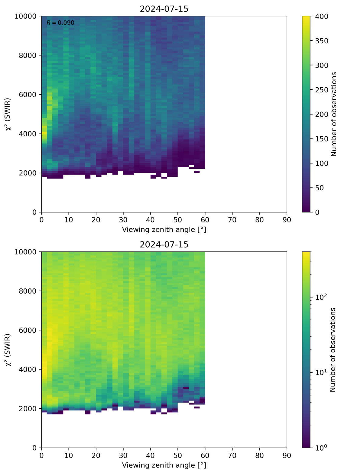
Figure 106: Scatter density plot of “Viewing zenith angle” against “ \chi^2 (SWIR)” for 2024-07-15 to 2024-07-16.
