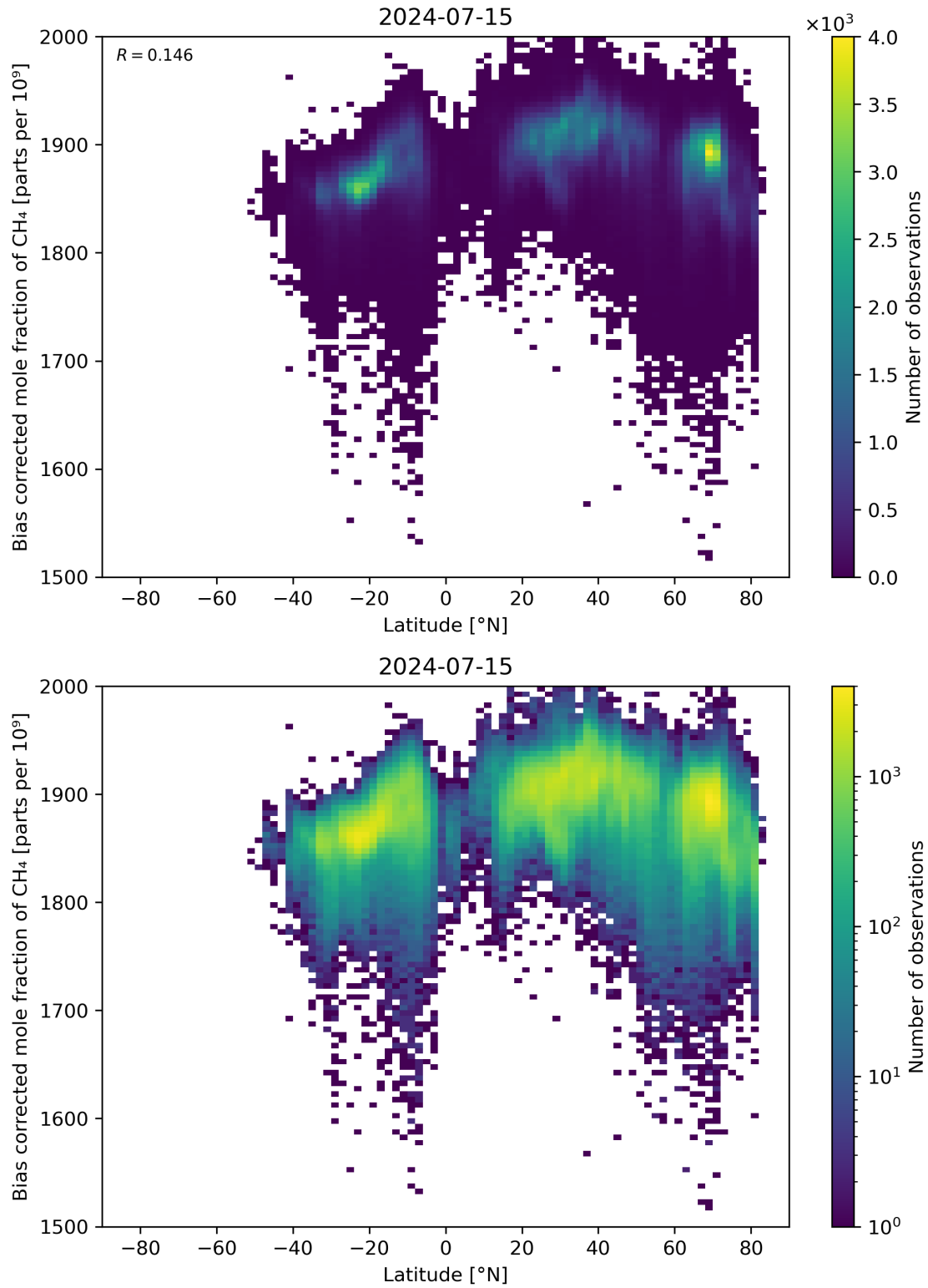
Figure 58: Scatter density plot of “Latitude” against “Bias corrected mole fraction of CH 4 ” for 2024-07-15 to 2024-07-16.
