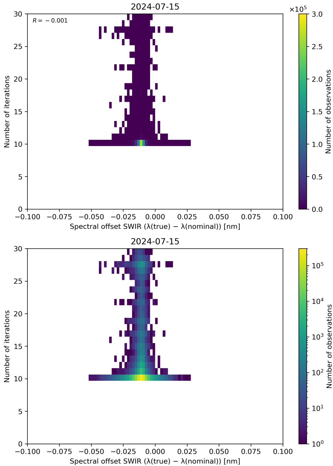
Figure 121: Scatter density plot of “Spectral offset SWIR ( \lambda(\text{true}) - \lambda(\text{nominal}) )” against “Number of iterations” for 2024-07-15 to 2024-07-16.
