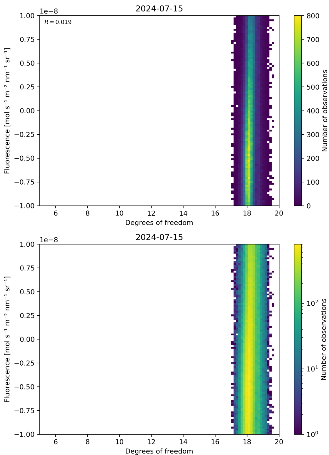
Figure 51: Scatter density plot of “Degrees of freedom” against “Fluorescence” for 2024-07-15 to 2024-07-16.
