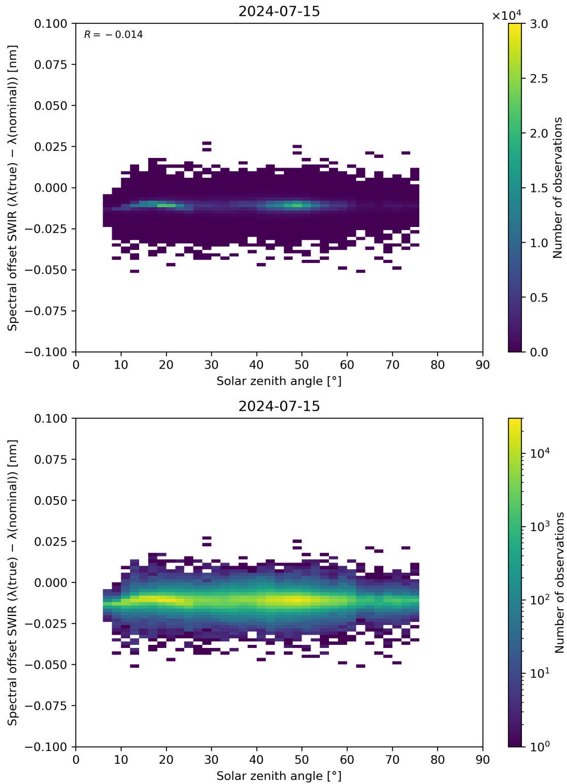
Figure 104: Scatter density plot of “Solar zenith angle” against “Spectral offset SWIR ( \lambda(\text{true}) - \lambda(\text{nominal}) )” for 2024-07-15 to 2024-07-16.
