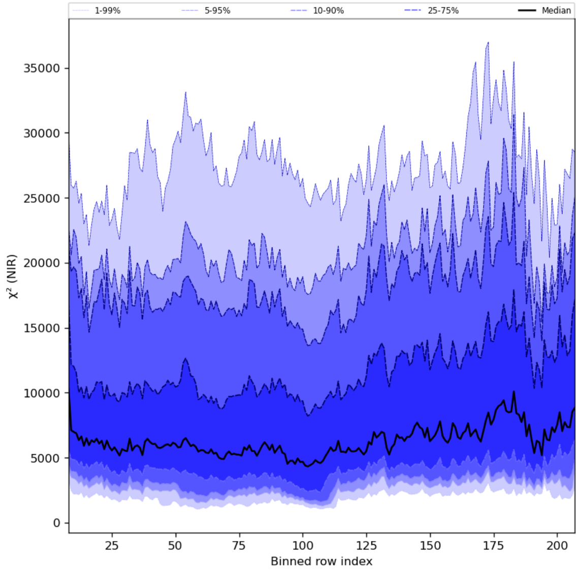
Figure 40: Along track statistics of “ \chi^2 (NIR)” for 2024-07-15 to 2024-07-16
