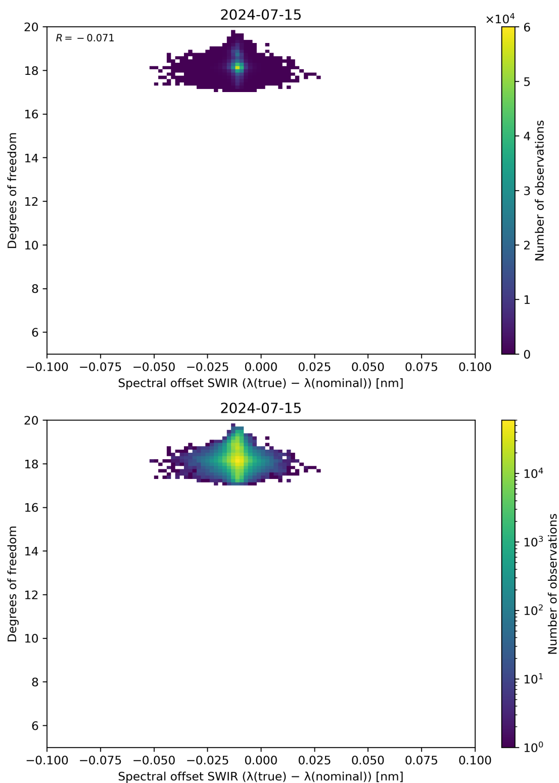
Figure 119: Scatter density plot of “Spectral offset SWIR ( \lambda(\text{true}) - \lambda(\text{nominal}) )” against “Degrees of freedom” for 2024-07-15 to 2024-07-16.
