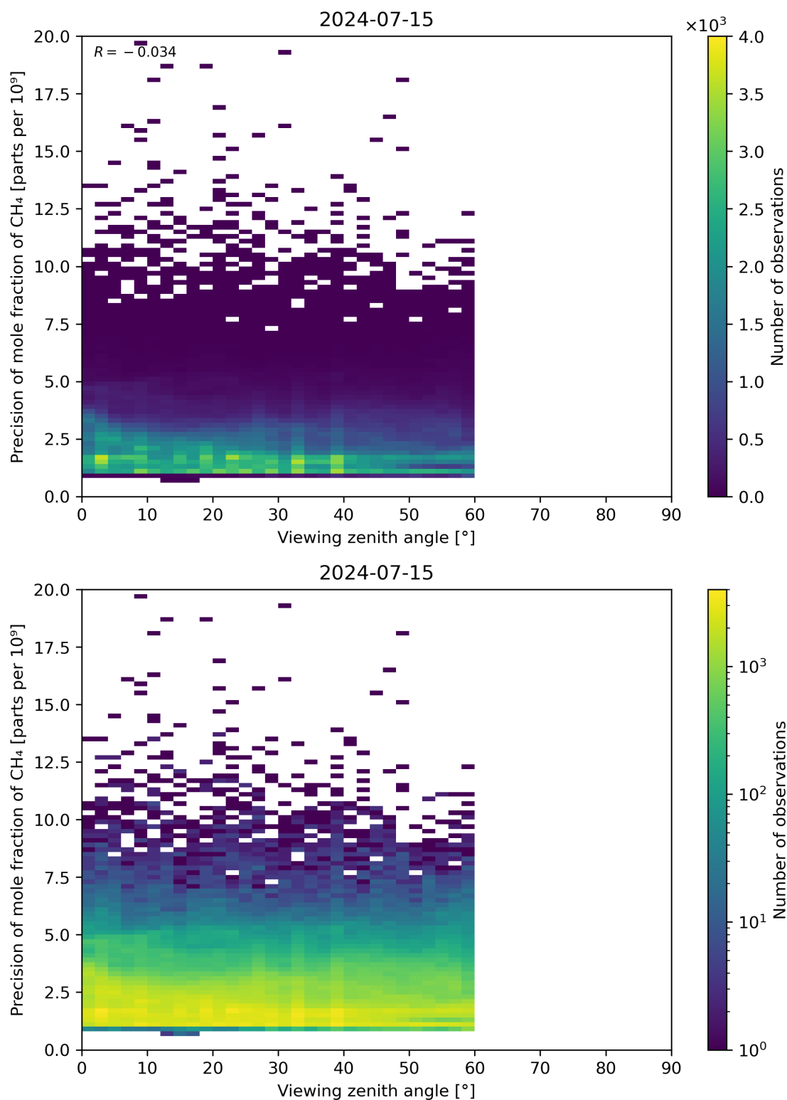
Figure 112: Scatter density plot of “Viewing zenith angle” against “Precision of mole fraction of CH 4 ” for 2024-07-15 to 2024-07-16.
