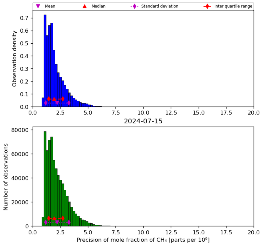
Figure 24: Histogram of “Precision of mole fraction of CH 4 ” for 2024-07-15 to 2024-07-16
