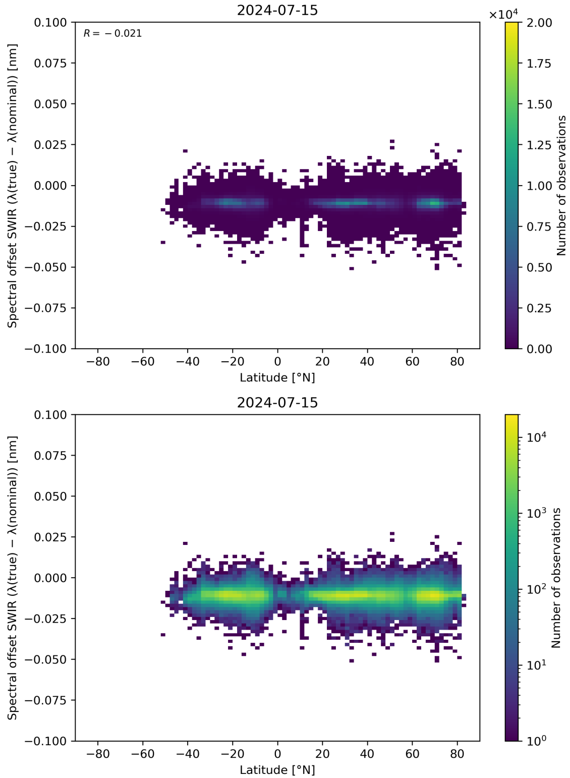
Figure 62: Scatter density plot of “Latitude” against “Spectral offset SWIR ( \lambda(\text{true}) - \lambda(\text{nominal}) )” for 2024-07-15 to 2024-07-16.
