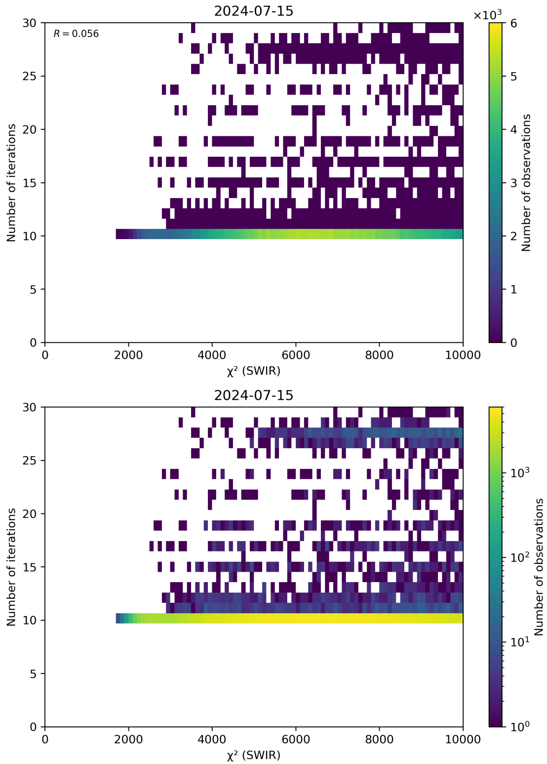
Figure 50: Scatter density plot of “ \chi^2 (SWIR)” against “Number of iterations” for 2024-07-15 to 2024-07-16.
