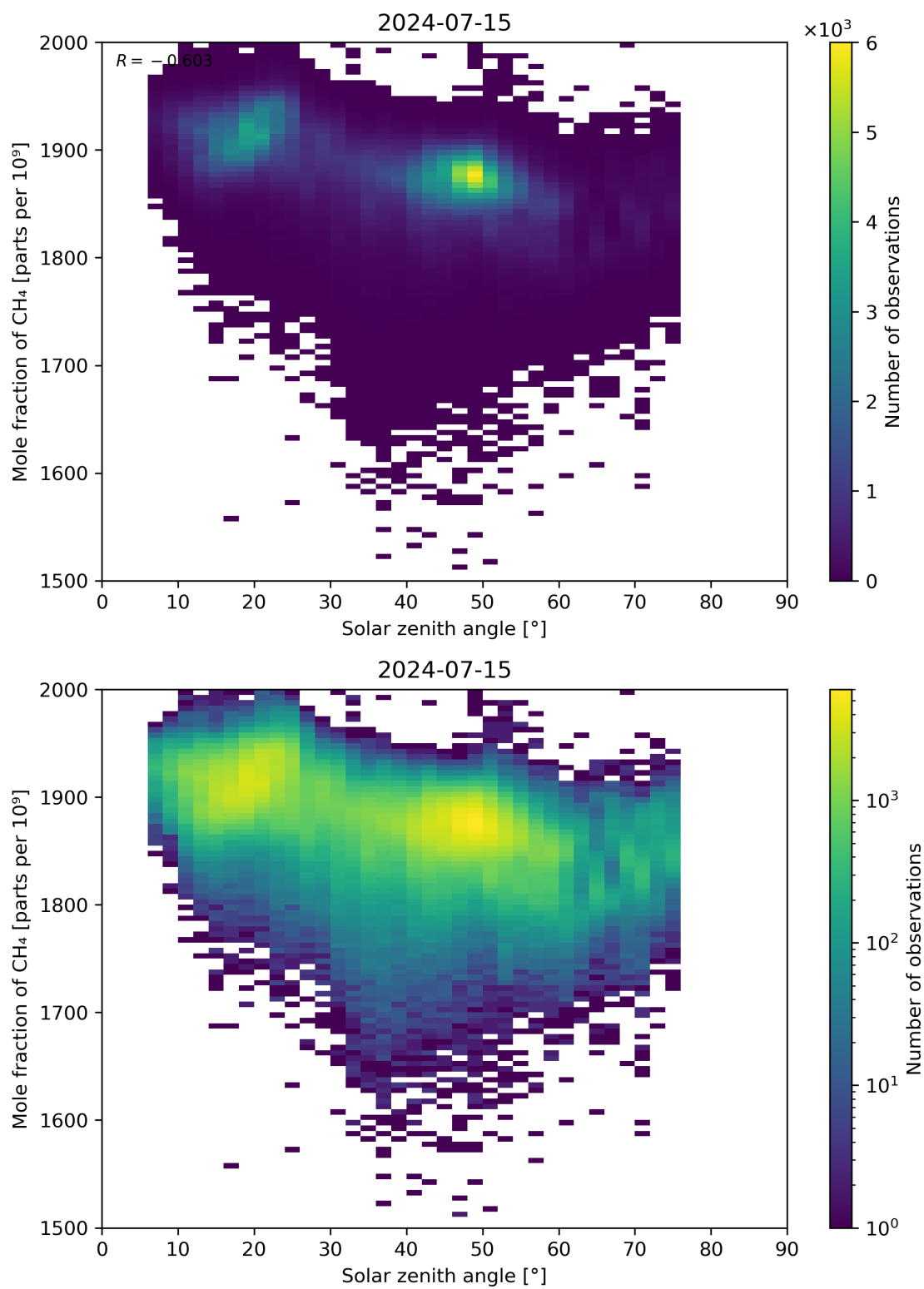
Figure 99: Scatter density plot of “Solar zenith angle” against “Mole fraction of CH 4 ” for 2024-07-15 to 2024-07-16.
