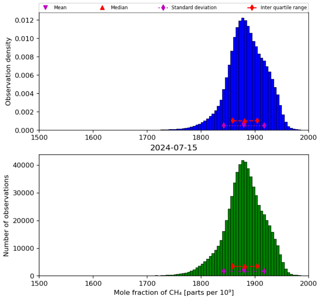
Figure 23: Histogram of "Mole fraction of CH 4 " for 2024-07-15 to 2024-07-16
