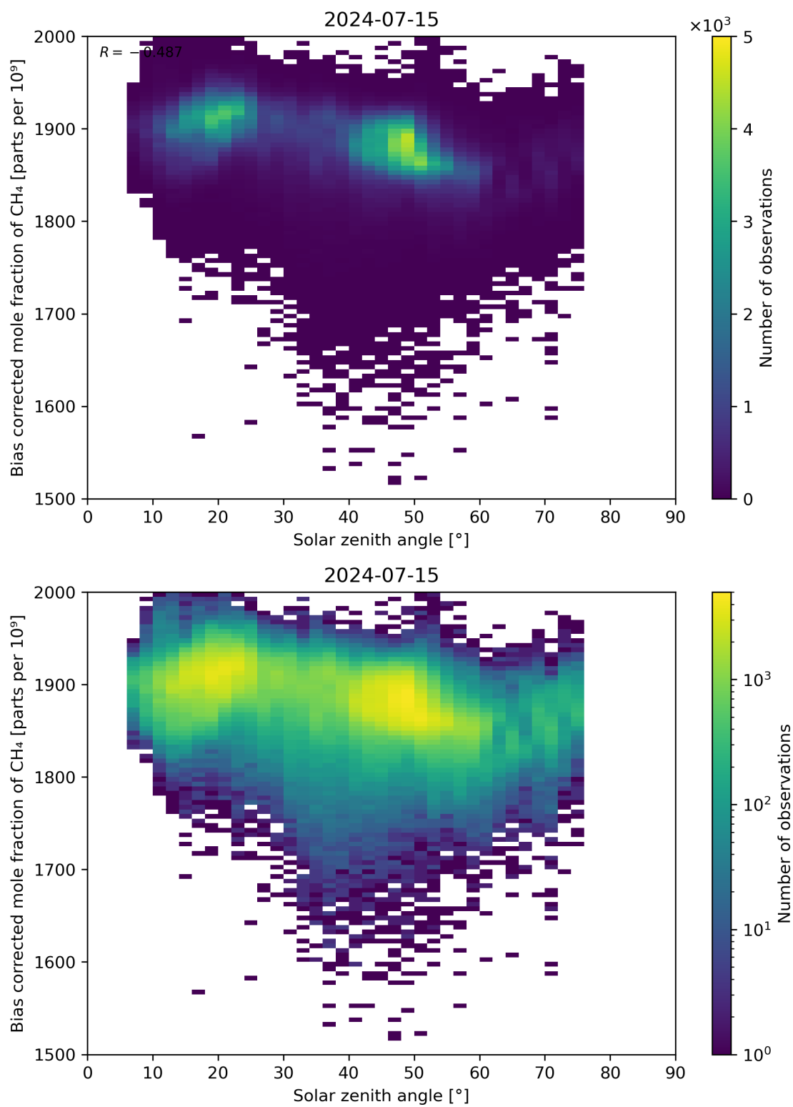
Figure 100: Scatter density plot of “Solar zenith angle” against “Bias corrected mole fraction of CH 4 ” for 2024-07-15 to 2024-07-16.
