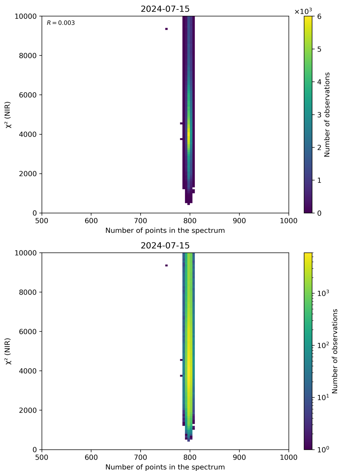
Figure 88: Scatter density plot of “Number of points in the spectrum” against “ \chi^2 (NIR)” for 2024-07-15 to 2024-07-16.
