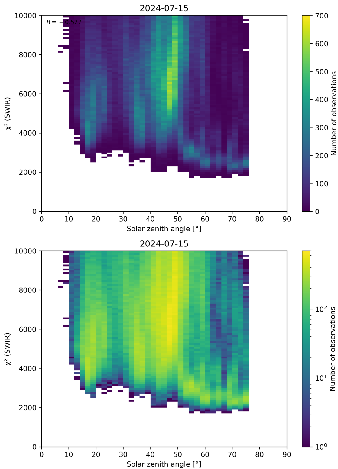
Figure 95: Scatter density plot of “Solar zenith angle” against “ \chi^2 (SWIR)” for 2024-07-15 to 2024-07-16.
