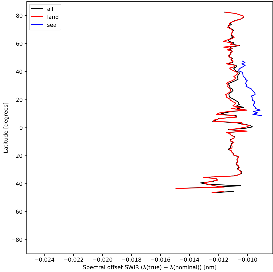
Figure 16: Zonal average of “Spectral offset SWIR ( \lambda(\text{true}) - \lambda(\text{nominal}) )” for 2024-07-15 to 2024-07-16.
