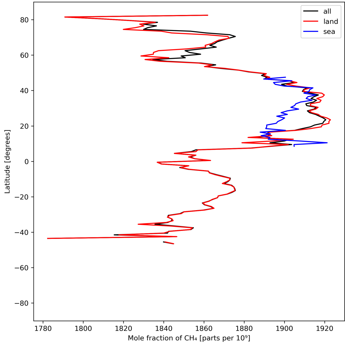
Figure 12: Zonal average of “Mole fraction of \text{CH}_4 ” for 2024-07-15 to 2024-07-16.
