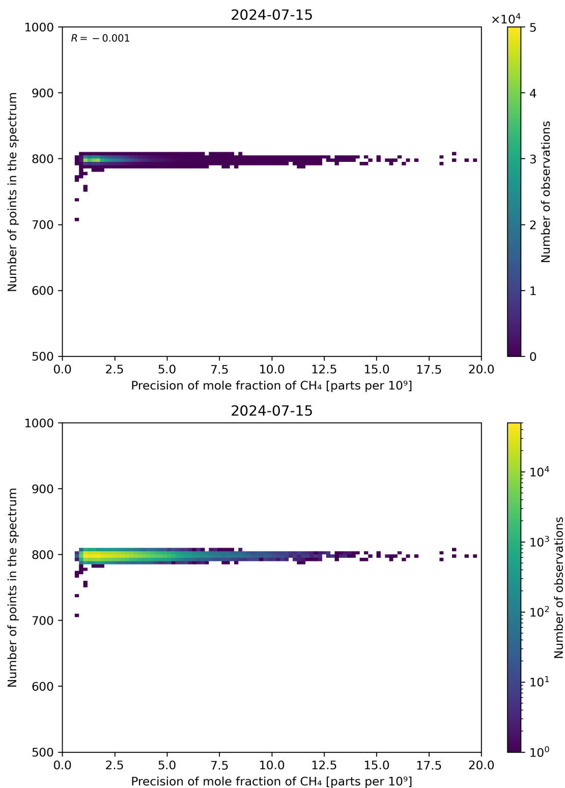
Figure 84: Scatter density plot of “Precision of mole fraction of CH 4 ” against “Number of points in the spectrum” for 2024-07-15 to 2024-07-16.
