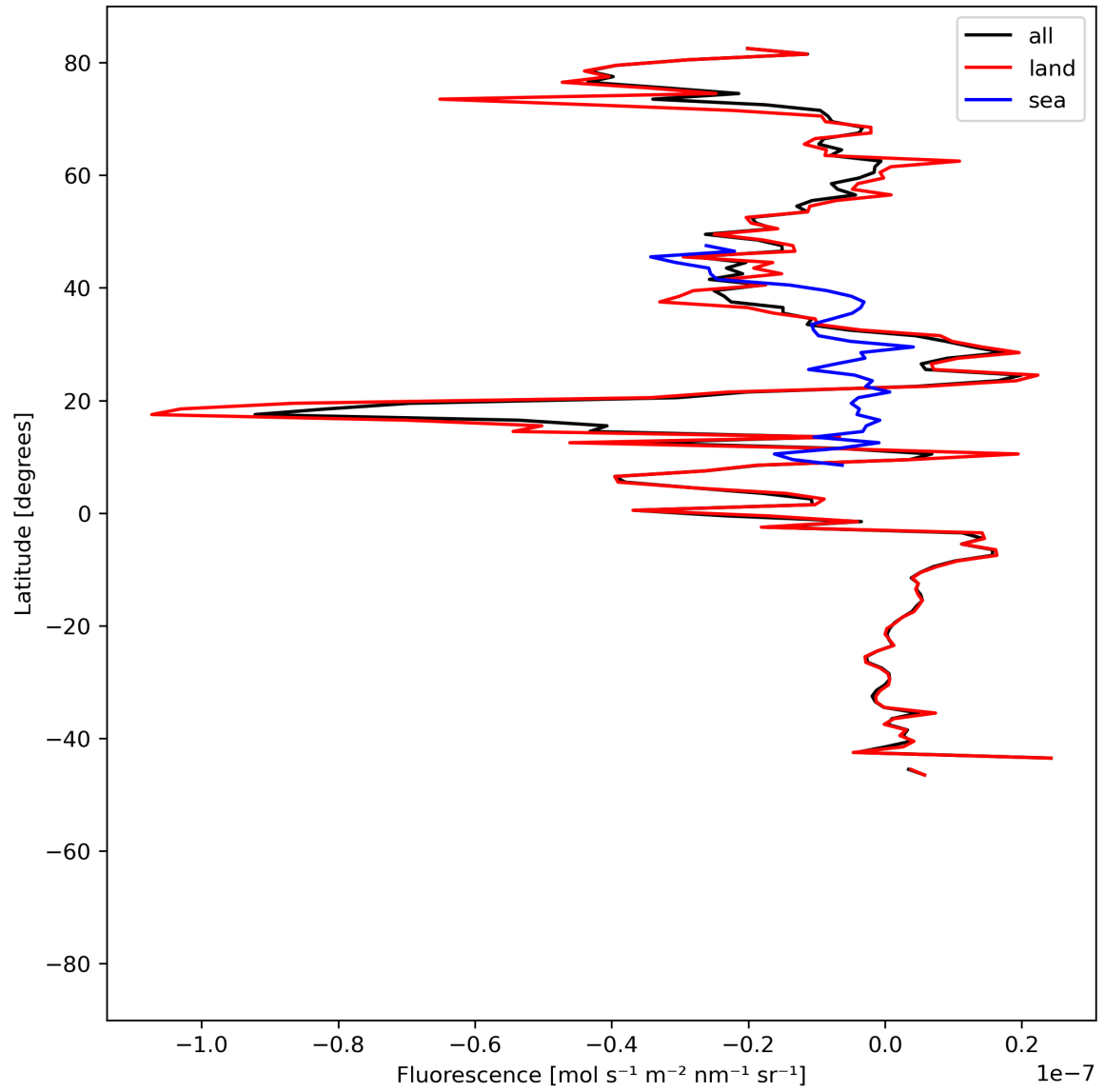
Figure 21: Zonal average of “Fluorescence” for 2024-07-15 to 2024-07-16.
