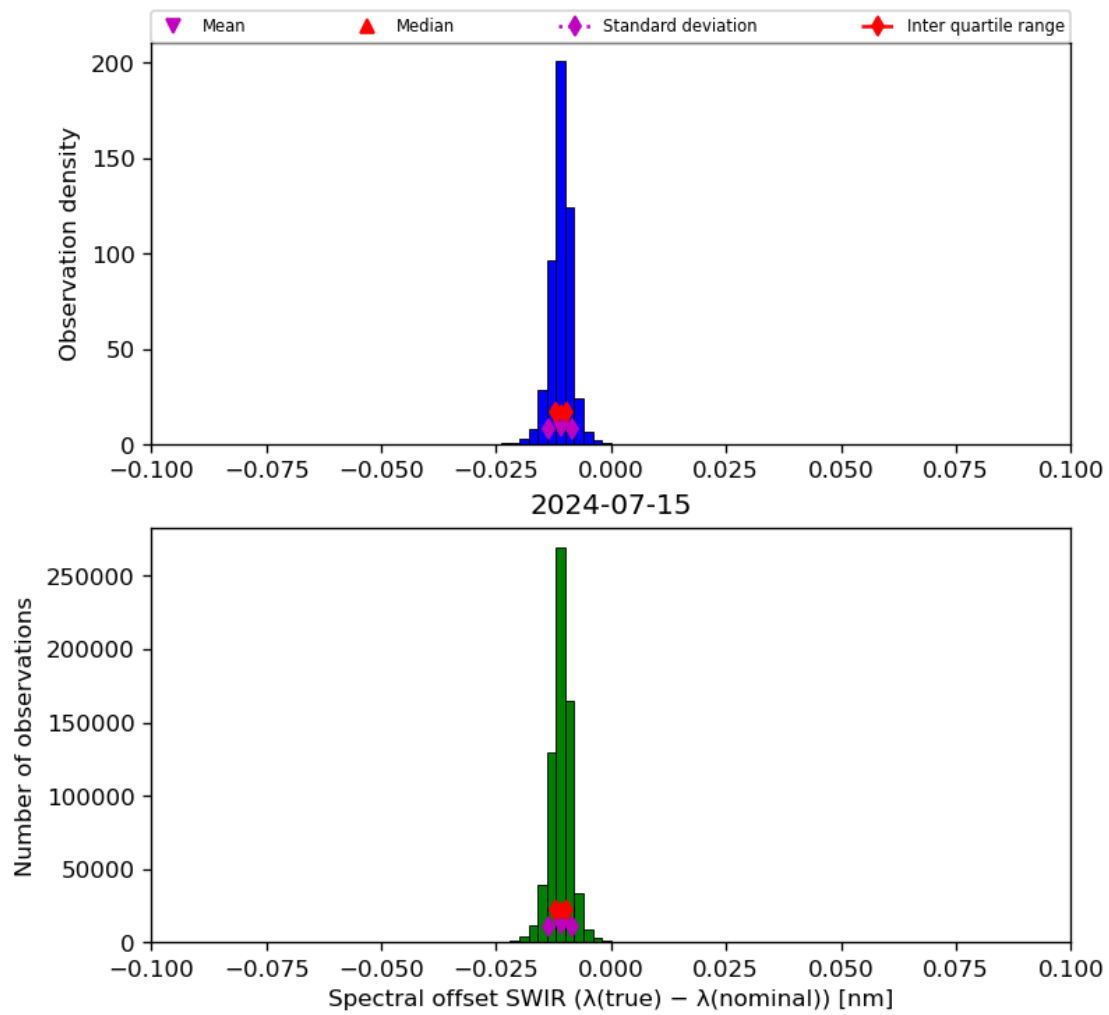
Figure 27: Histogram of “Spectral offset SWIR ( \lambda(\text{true}) - \lambda(\text{nominal}) )” for 2024-07-15 to 2024-07-16
