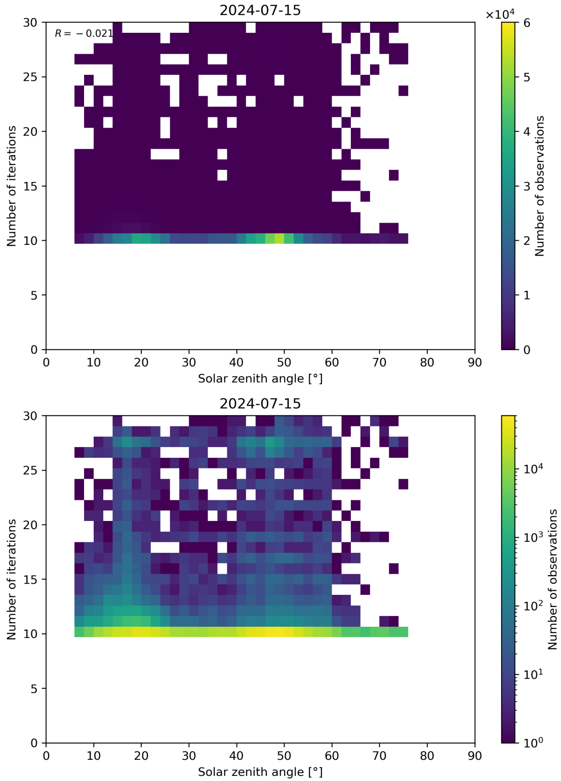
Figure 102: Scatter density plot of “Solar zenith angle” against “Number of iterations” for 2024-07-15 to 2024-07-16.
