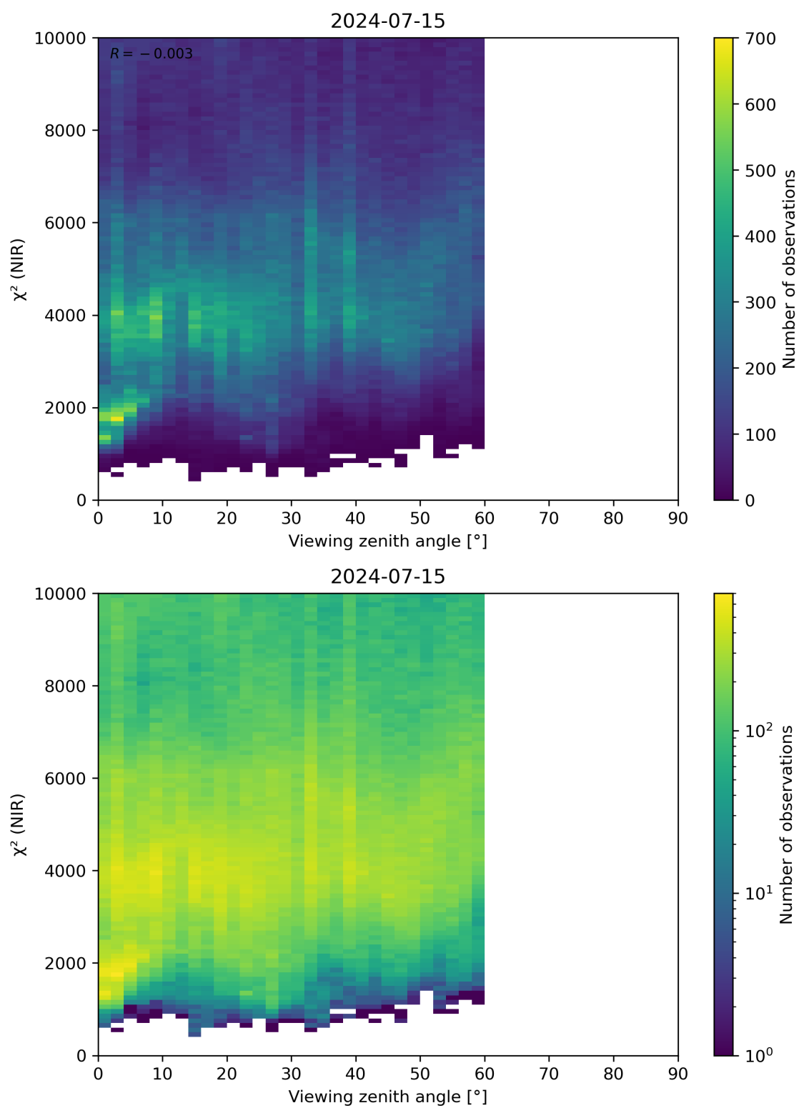
Figure 105: Scatter density plot of “Viewing zenith angle” against “ \chi^2 (NIR)” for 2024-07-15 to 2024-07-16.
