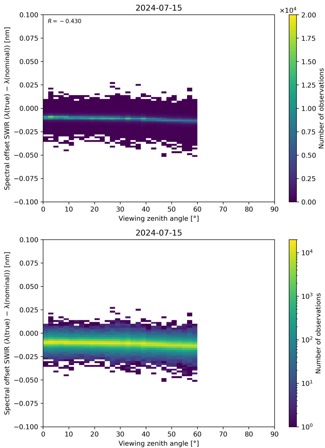
Figure 116: Scatter density plot of “Viewing zenith angle” against “Spectral offset SWIR ( \lambda(\text{true}) - \lambda(\text{nominal}) )” for 2024-07-15 to 2024-07-16.
