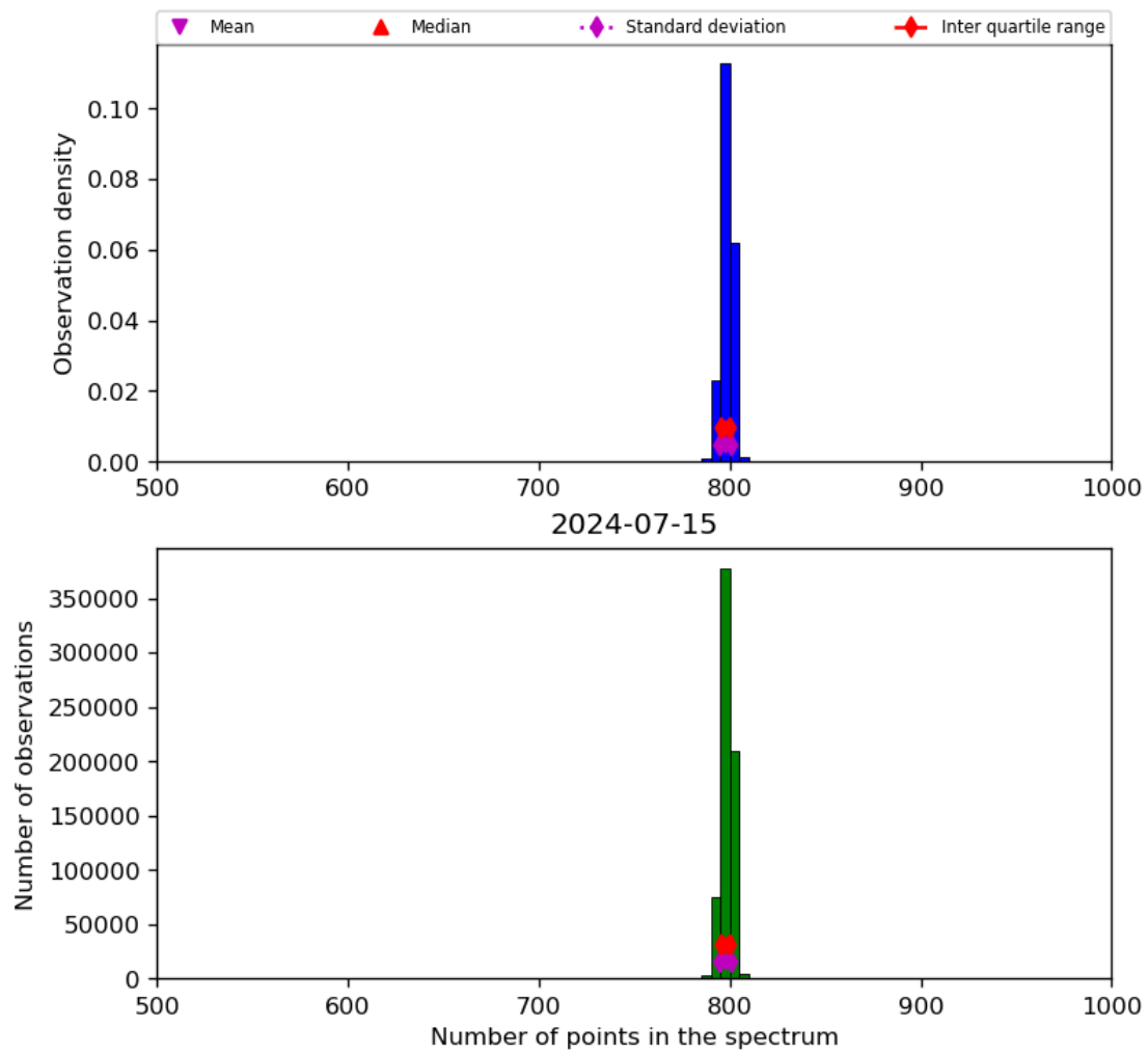
Figure 26: Histogram of “Number of points in the spectrum” for 2024-07-15 to 2024-07-16
