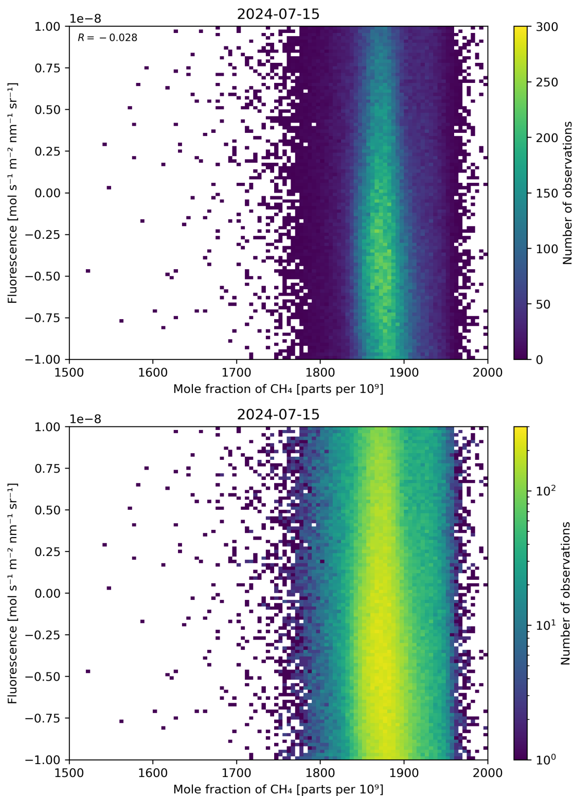
Figure 73: Scatter density plot of “Mole fraction of \text{CH}_4 ” against “Fluorescence” for 2024-07-15 to 2024-07-16.
