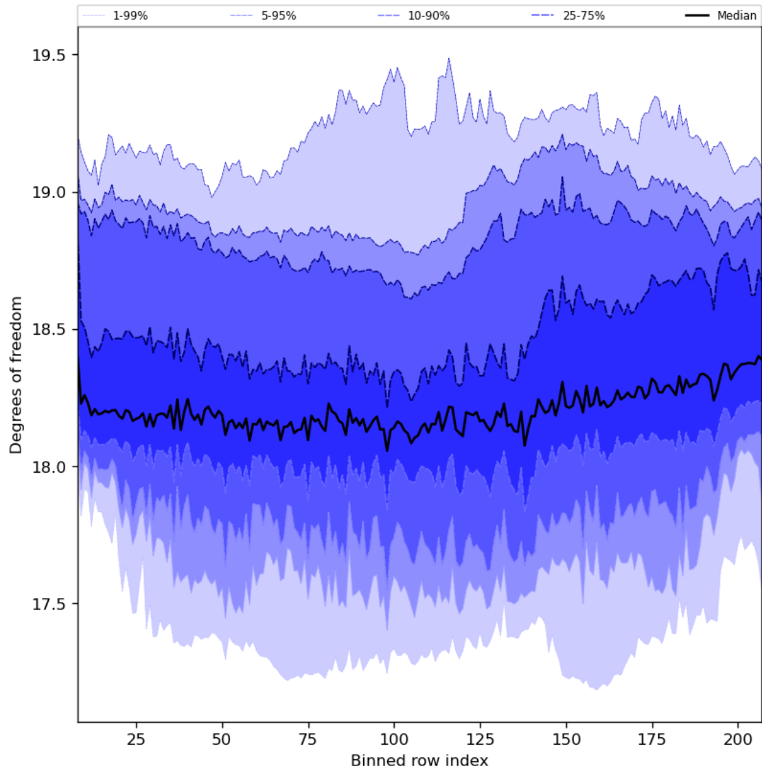
Figure 41: Along track statistics of “Degrees of freedom” for 2024-07-15 to 2024-07-16
