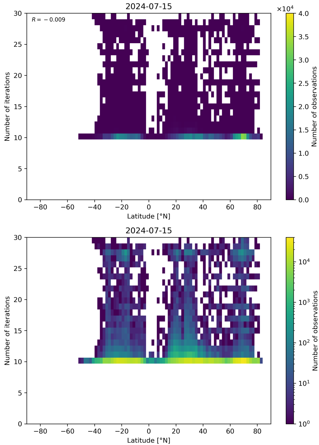
Figure 60: Scatter density plot of “Latitude” against “Number of iterations” for 2024-07-15 to 2024-07-16.
