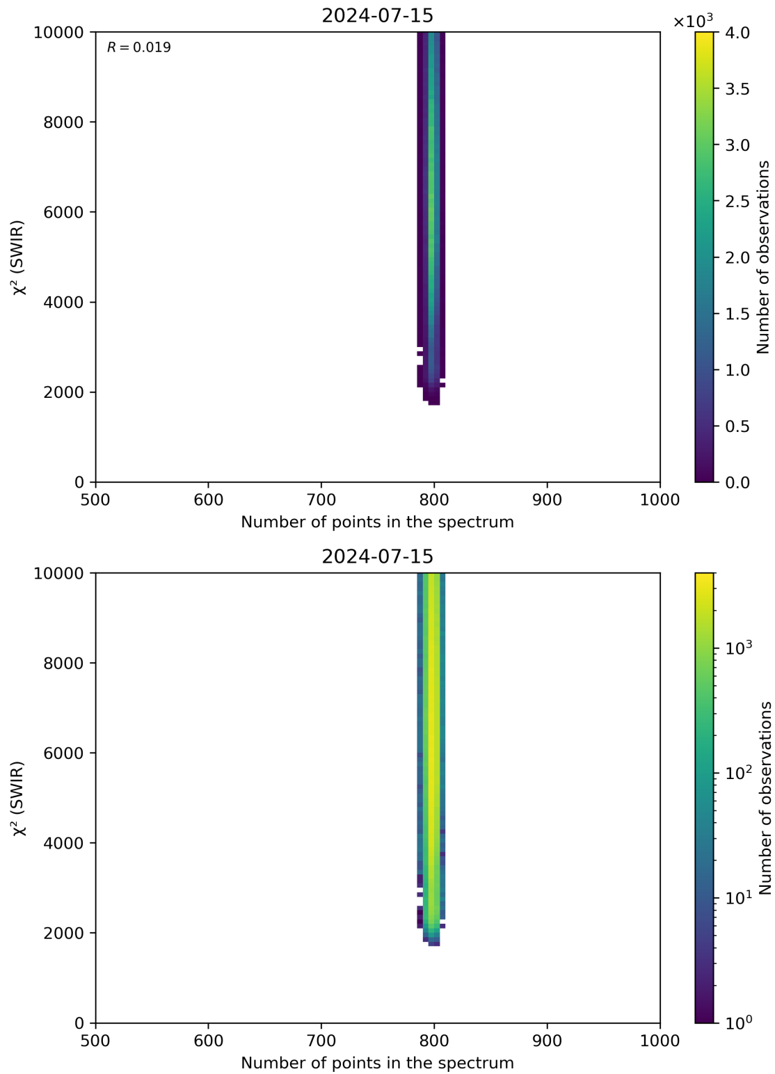
Figure 89: Scatter density plot of “Number of points in the spectrum” against “ \chi^2 (SWIR)” for 2024-07-15 to 2024-07-16.
