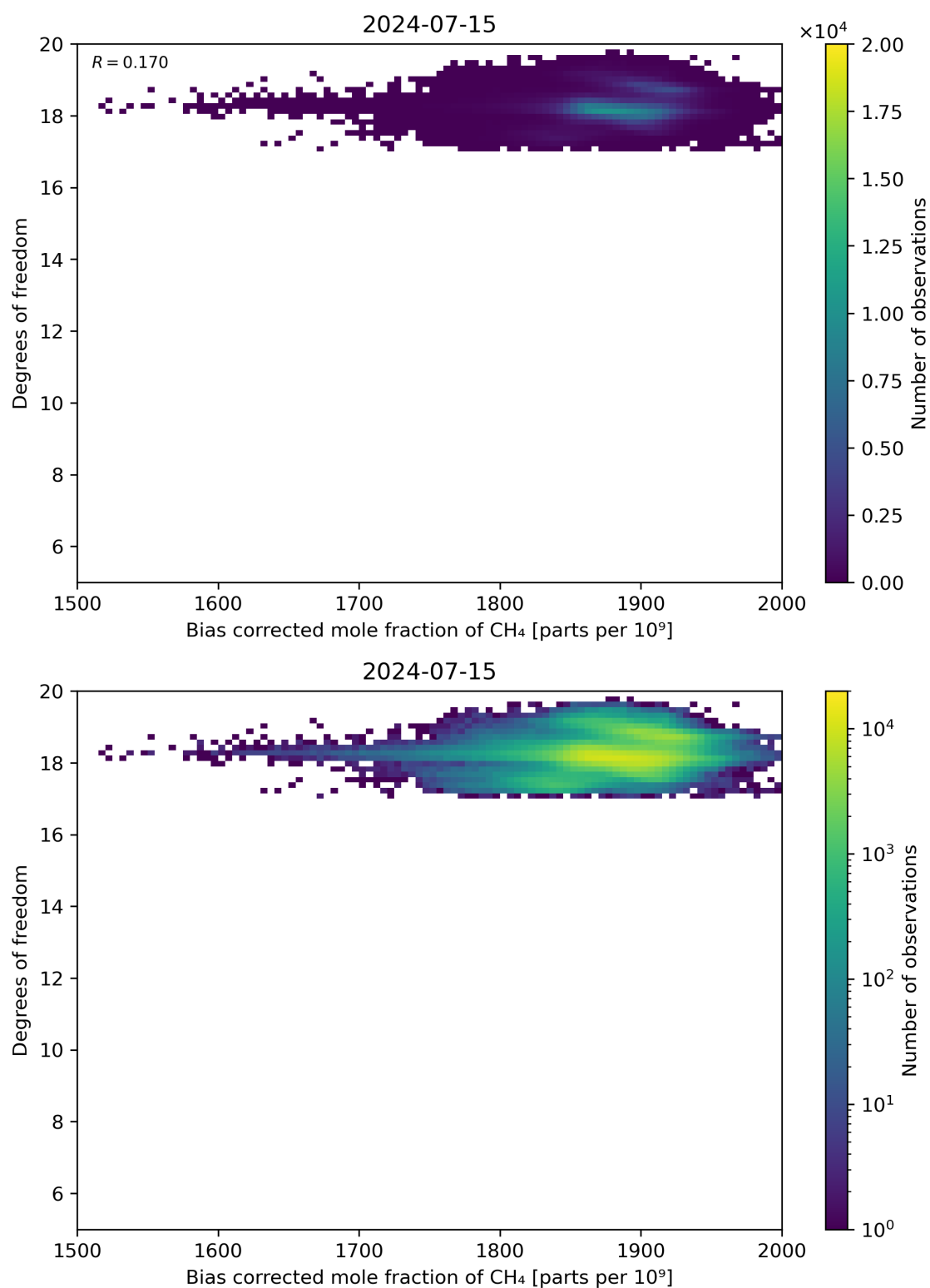
Figure 65: Scatter density plot of “Bias corrected mole fraction of CH 4 ” against “Degrees of freedom” for 2024-07-15 to 2024-07-16.
