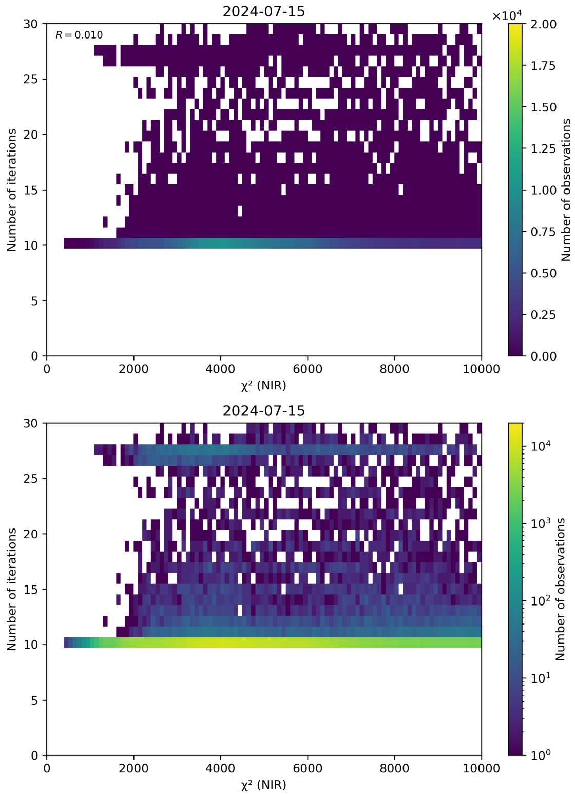
Figure 46: Scatter density plot of “ \chi^2 (NIR)” against “Number of iterations” for 2024-07-15 to 2024-07-16.
