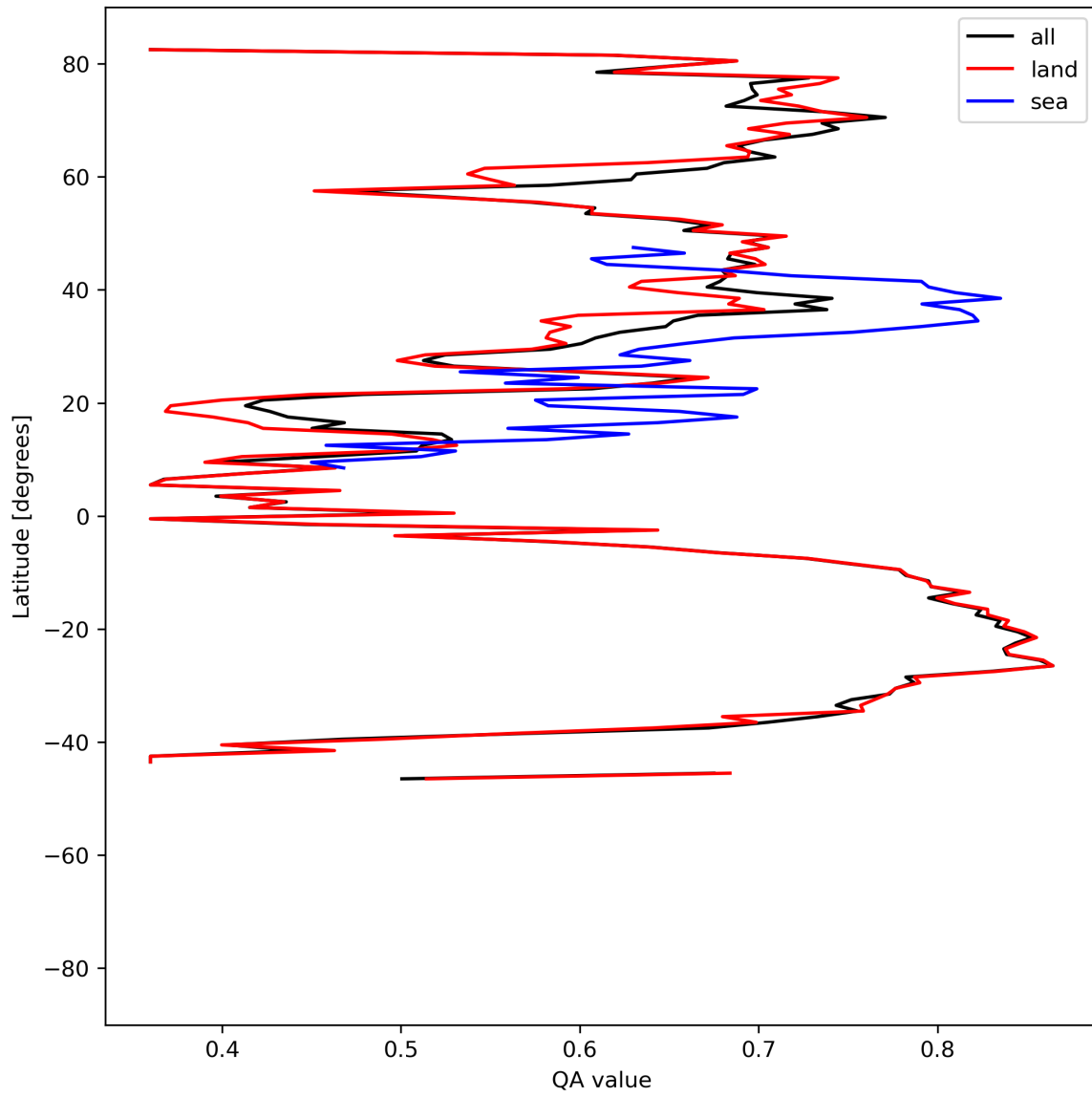
Figure 11: Zonal average of “QA value” for 2024-07-15 to 2024-07-16.
