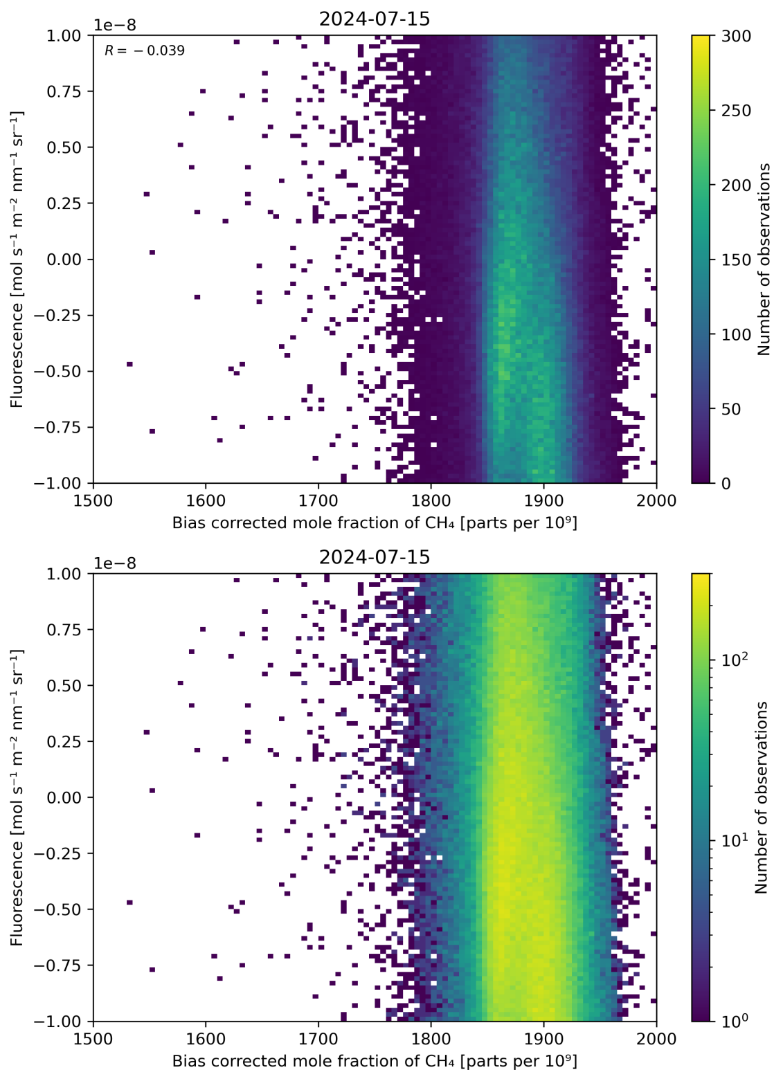
Figure 66: Scatter density plot of “Bias corrected mole fraction of \text{CH}_4 ” against “Fluorescence” for 2024-07-15 to 2024-07-16.
