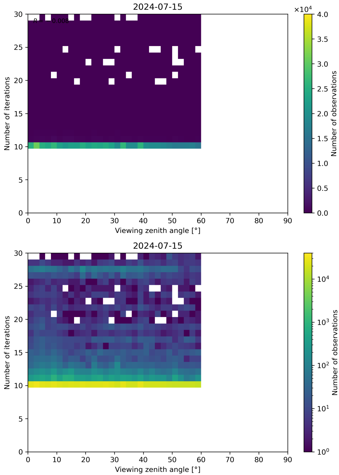
Figure 113: Scatter density plot of “Viewing zenith angle” against “Number of iterations” for 2024-07-15 to 2024-07-16.
