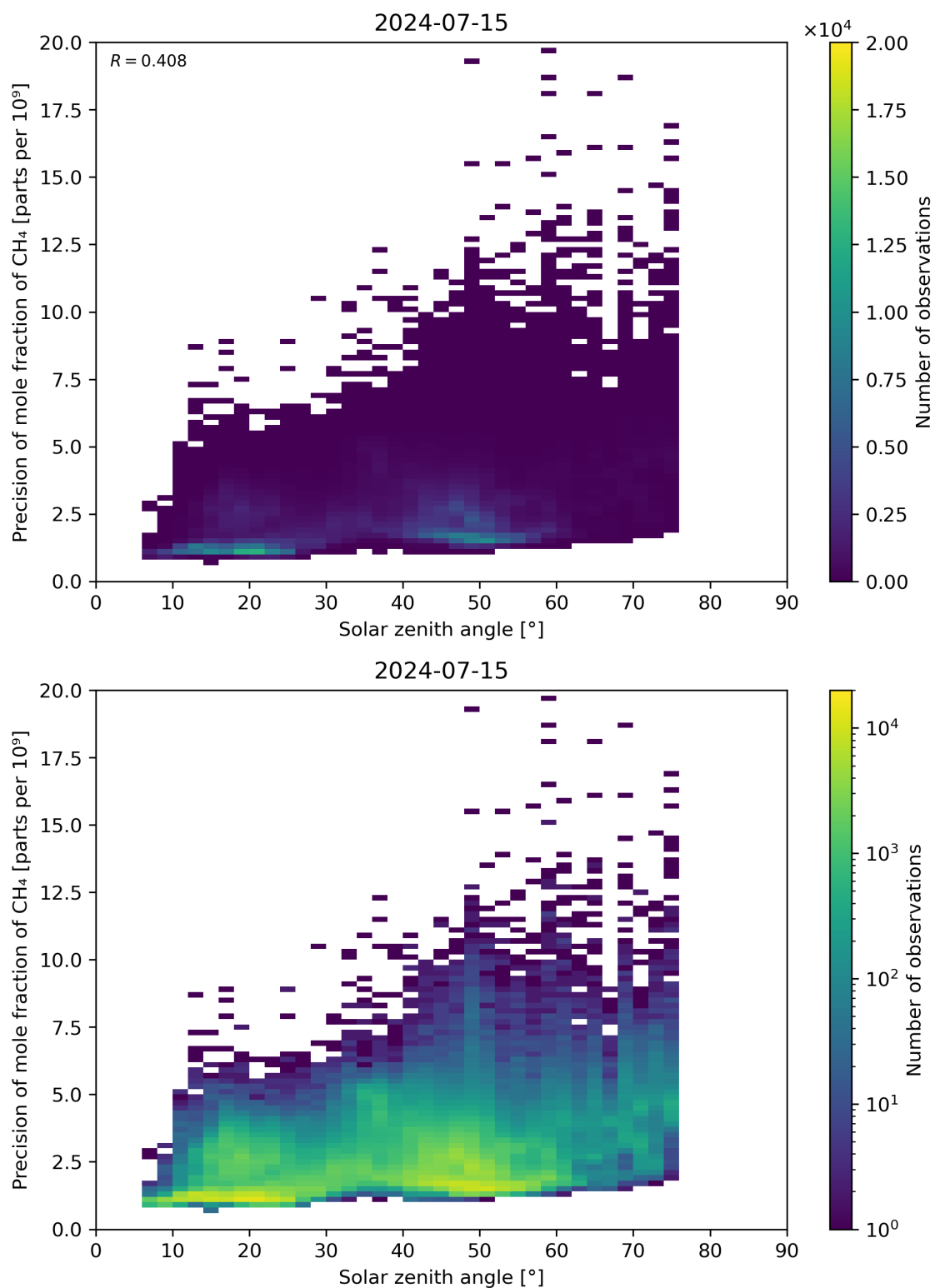
Figure 101: Scatter density plot of “Solar zenith angle” against “Precision of mole fraction of CH 4 ” for 2024-07-15 to 2024-07-16.
