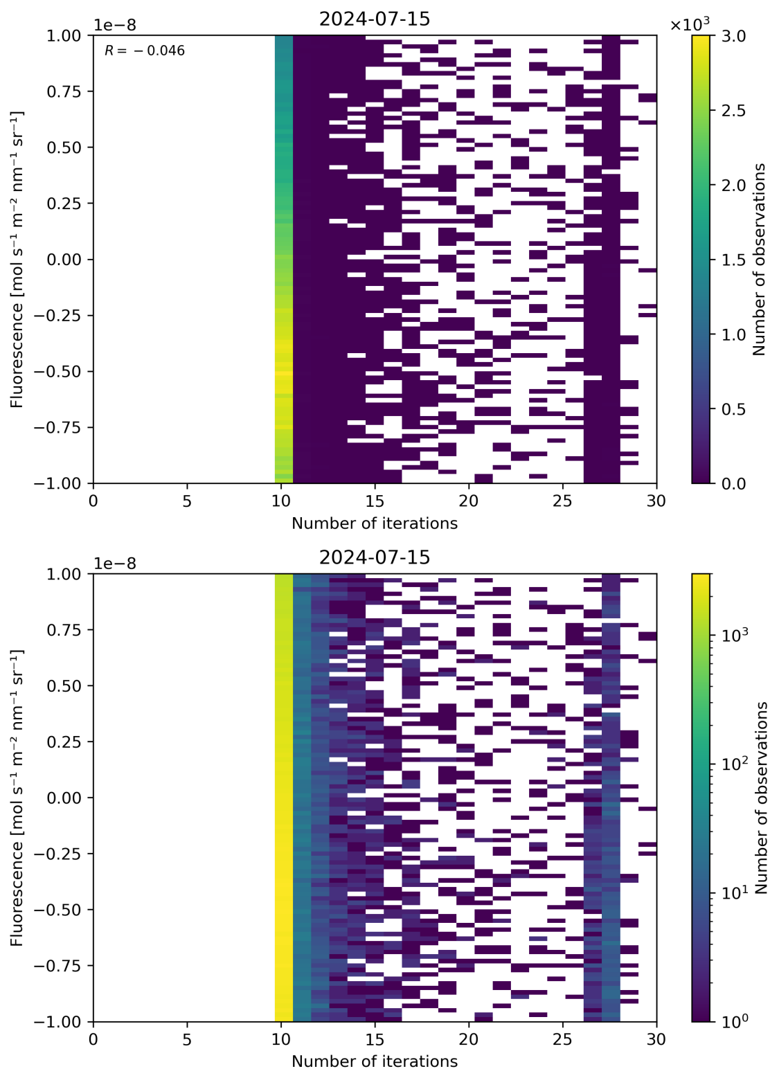
Figure 87: Scatter density plot of “Number of iterations” against “Fluorescence” for 2024-07-15 to 2024-07-16.
