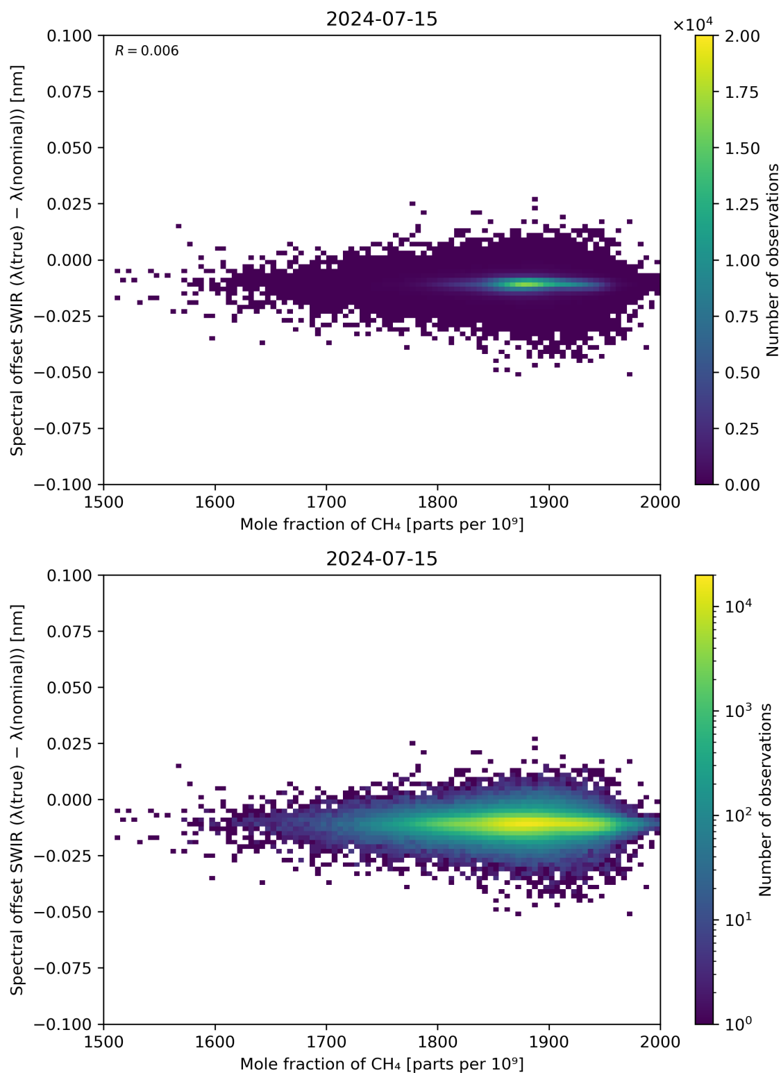
Figure 86: Scatter density plot of “Mole fraction of \text{CH}_4 ” against “Spectral offset SWIR ( \lambda(\text{true}) - \lambda(\text{nominal}) )” for 2024-07-15 to 2024-07-16.
