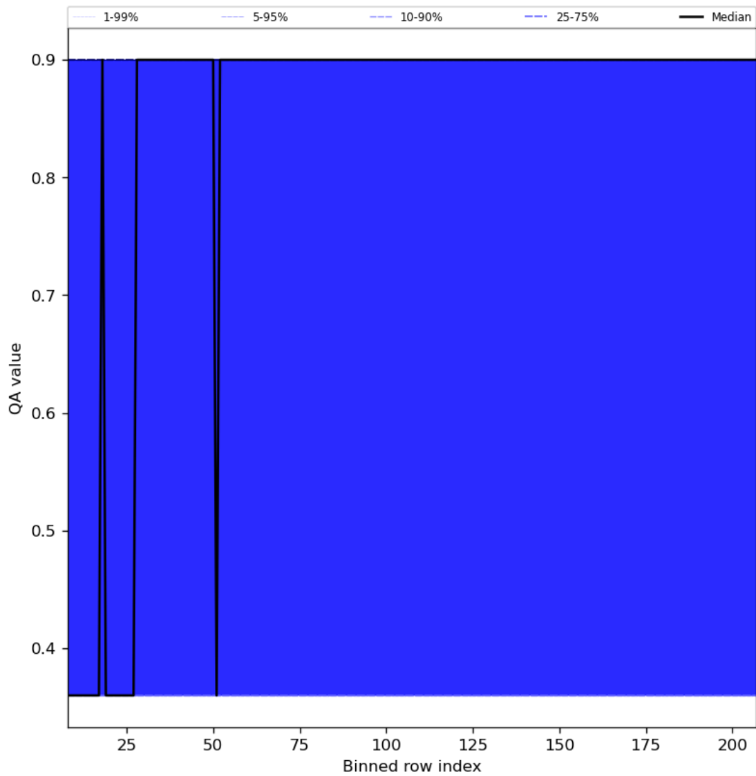
Figure 33: Along track statistics of “QA value” for 2024-07-15 to 2024-07-16
