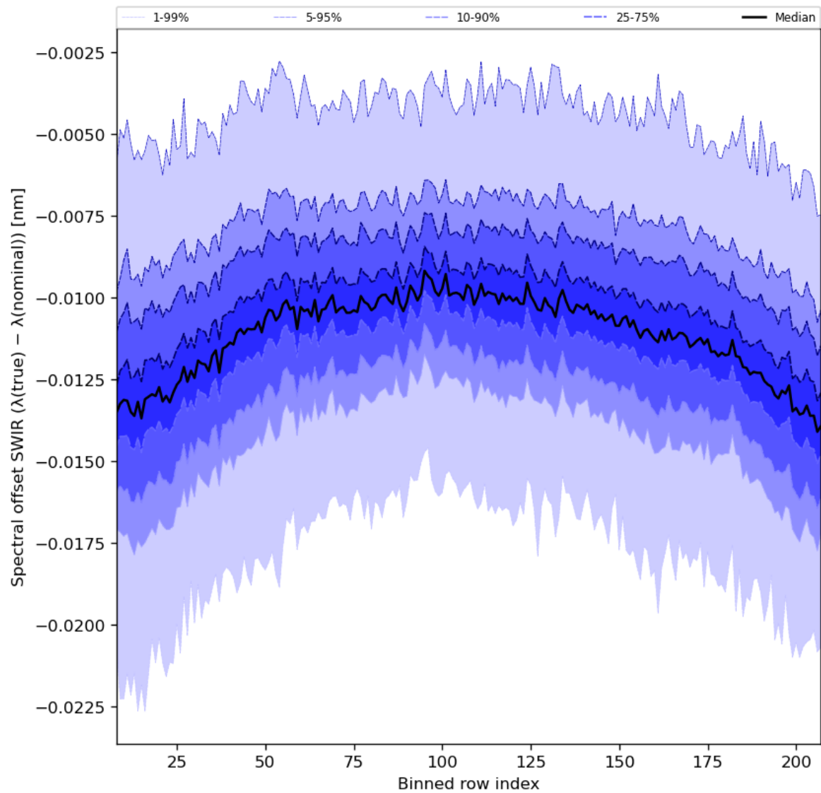
Figure 38: Along track statistics of “Spectral offset SWIR ( \lambda(\text{true}) - \lambda(\text{nominal}) )” for 2024-07-15 to 2024-07-16
