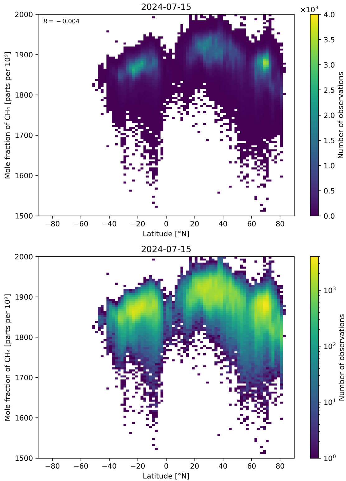
Figure 57: Scatter density plot of “Latitude” against “Mole fraction of CH 4 ” for 2024-07-15 to 2024-07-16.
