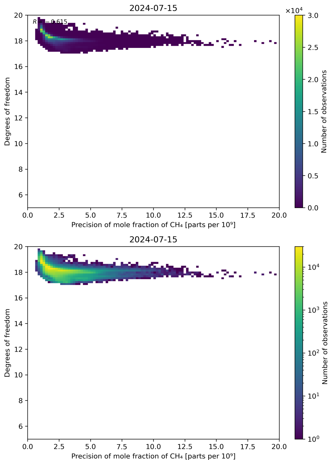
Figure 80: Scatter density plot of “Precision of mole fraction of CH 4 ” against “Degrees of freedom” for 2024-07-15 to 2024-07-16.
