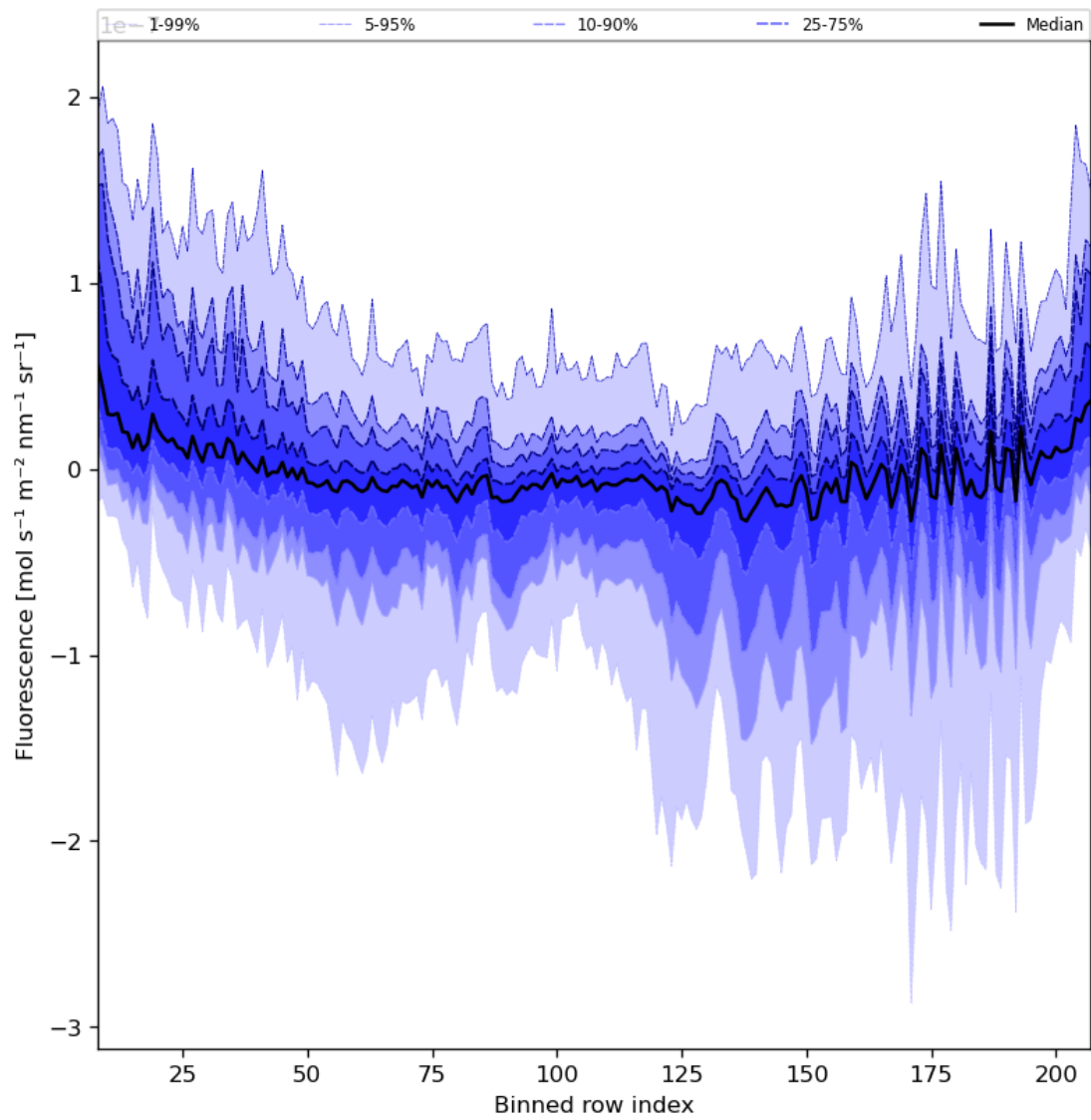
Figure 43: Along track statistics of “Fluorescence” for 2024-07-15 to 2024-07-16
