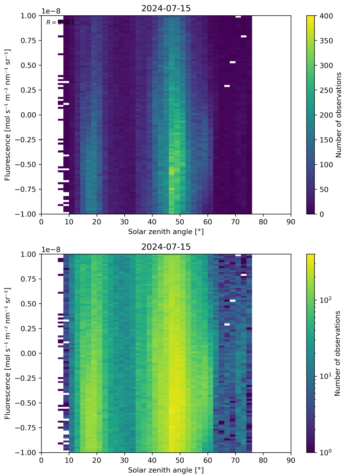
Figure 97: Scatter density plot of “Solar zenith angle” against “Fluorescence” for 2024-07-15 to 2024-07-16.
