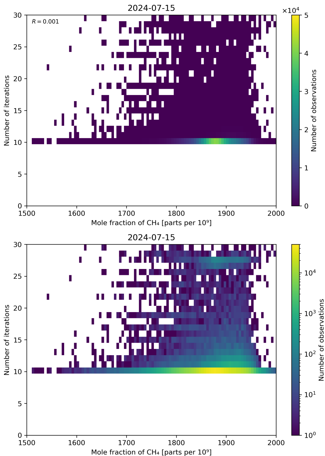
Figure 76: Scatter density plot of “Mole fraction of CH 4 ” against “Number of iterations” for 2024-07-15 to 2024-07-16.
