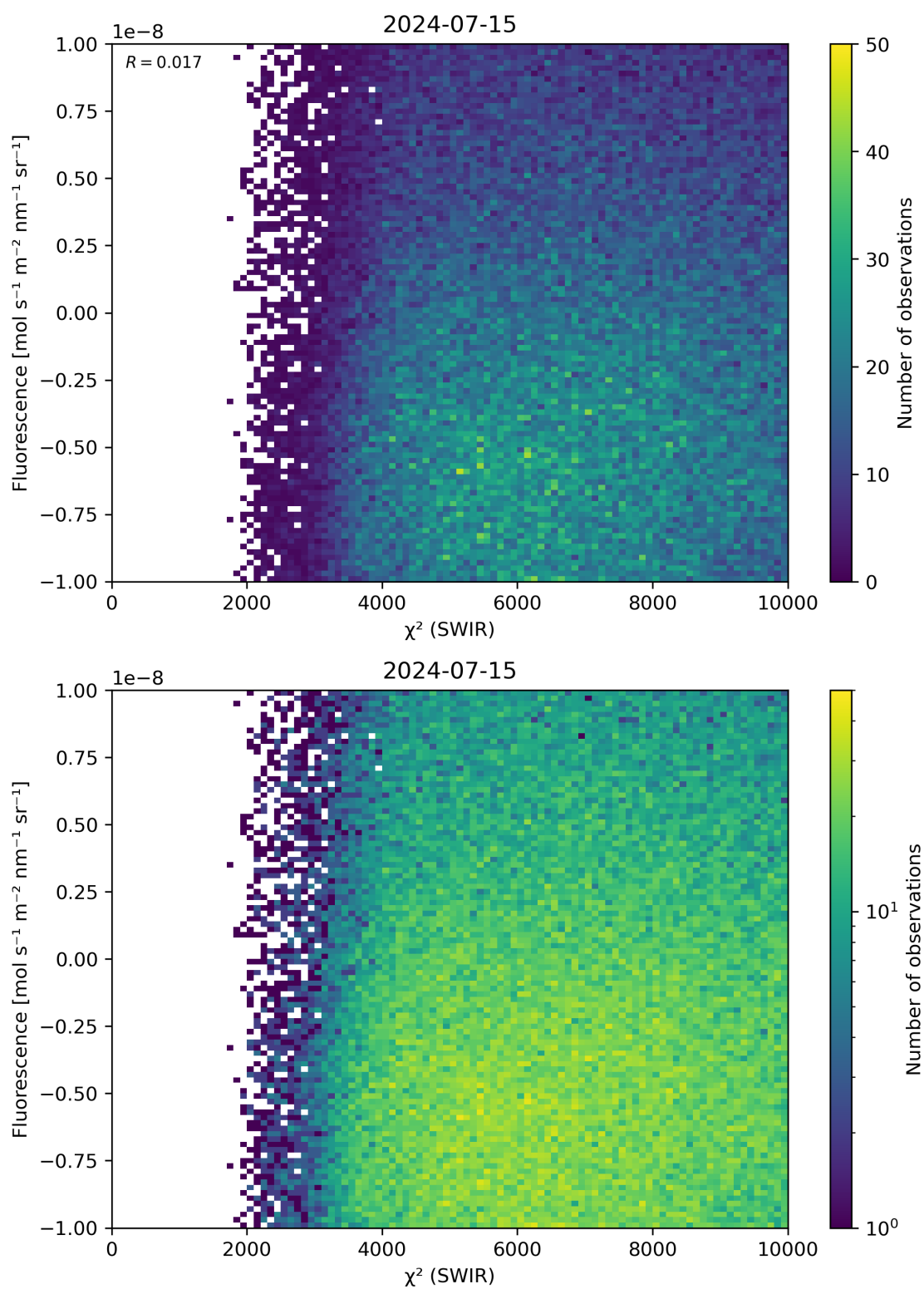
Figure 49: Scatter density plot of “ \chi^2 (SWIR)” against “Fluorescence” for 2024-07-15 to 2024-07-16.
