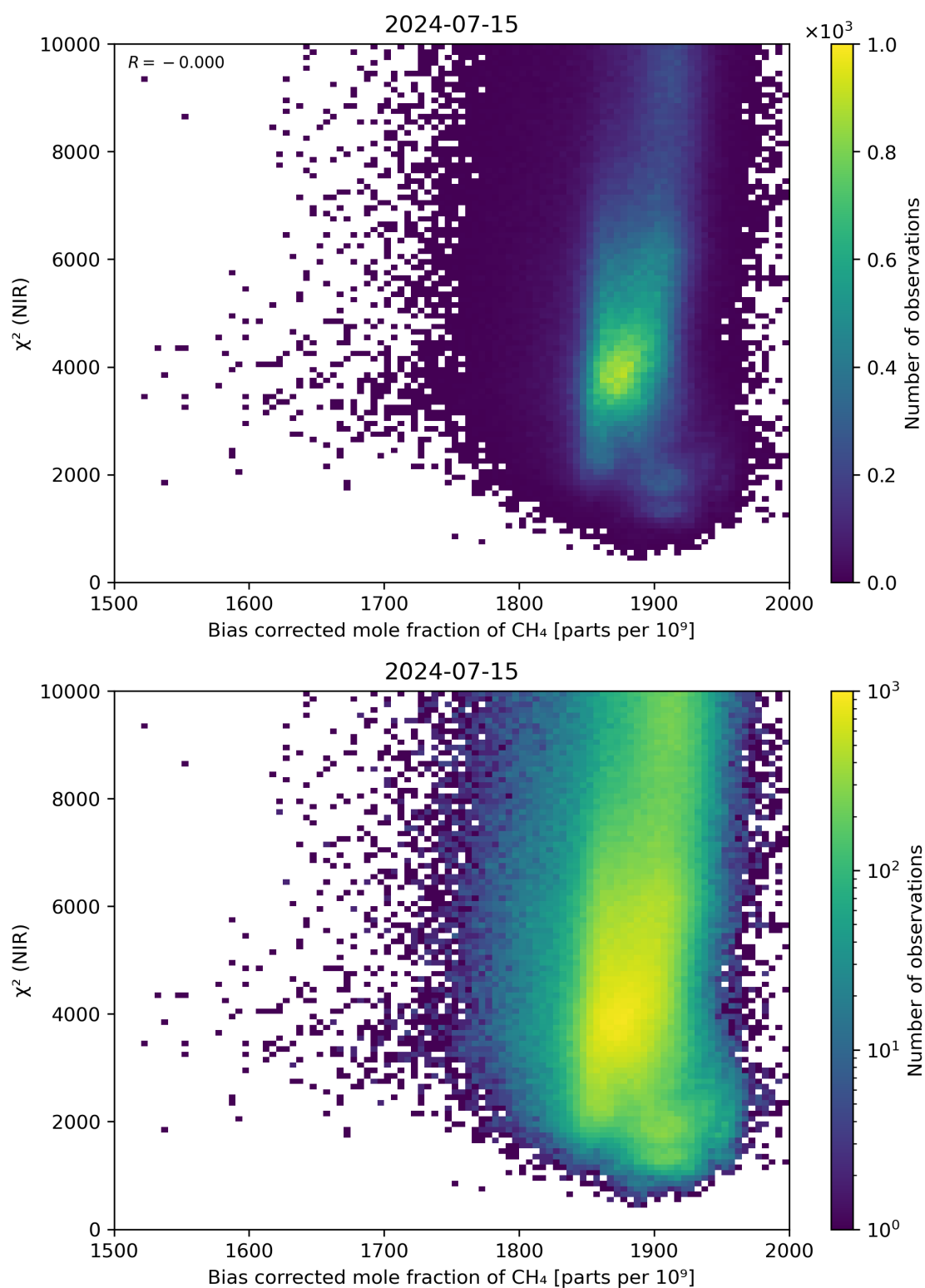
Figure 63: Scatter density plot of “Bias corrected mole fraction of CH 4 ” against “ \chi^2 (NIR)” for 2024-07-15 to 2024-07-16.
