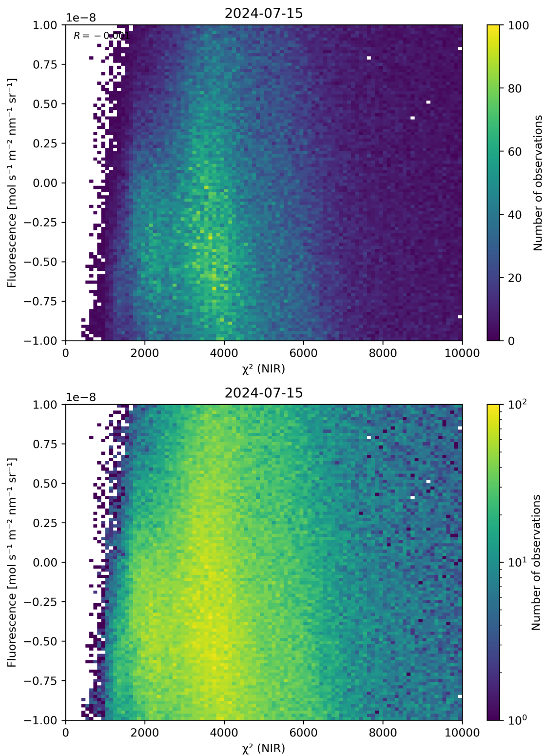
Figure 45: Scatter density plot of “ \chi^2 (NIR)” against “Fluorescence” for 2024-07-15 to 2024-07-16.
