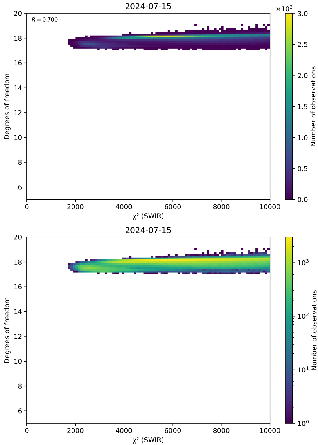
Figure 48: Scatter density plot of “ \chi^2 (SWIR)” against “Degrees of freedom” for 2024-07-15 to 2024-07-16.
