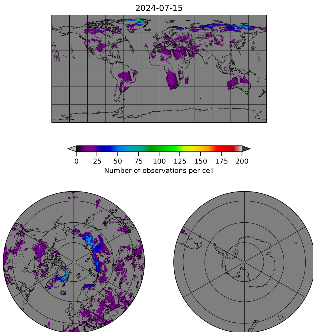
Figure 10: Map of the number of observations for 2024-07-15 to 2024-07-16
