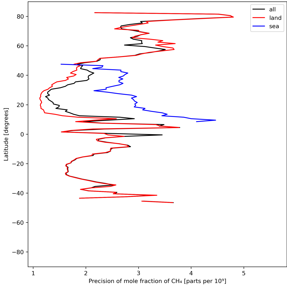
Figure 13: Zonal average of “Precision of mole fraction of \text{CH}_4 ” for 2024-07-15 to 2024-07-16.
