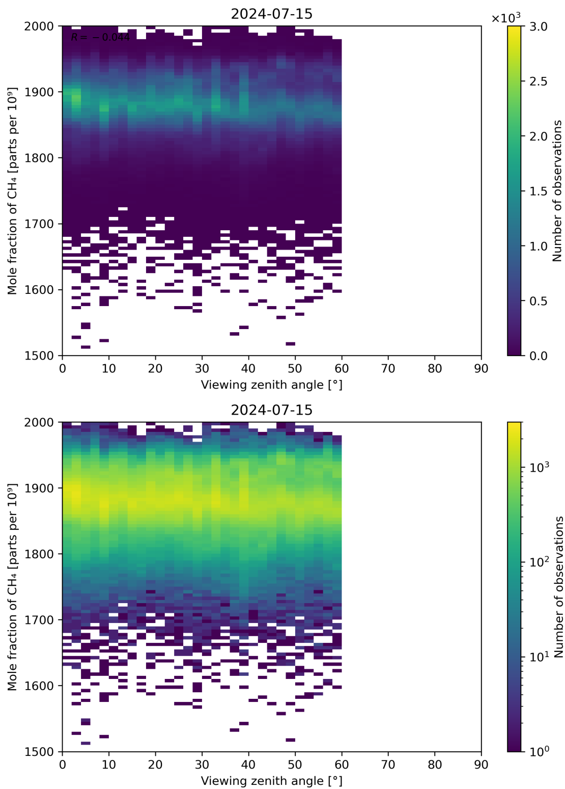
Figure 110: Scatter density plot of “Viewing zenith angle” against “Mole fraction of CH 4 ” for 2024-07-15 to 2024-07-16.
