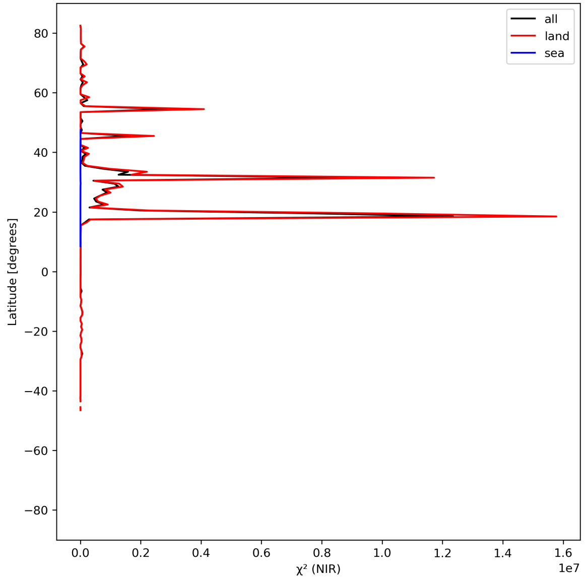
Figure 18: Zonal average of “ \chi^2 (NIR)” for 2024-07-15 to 2024-07-16.
