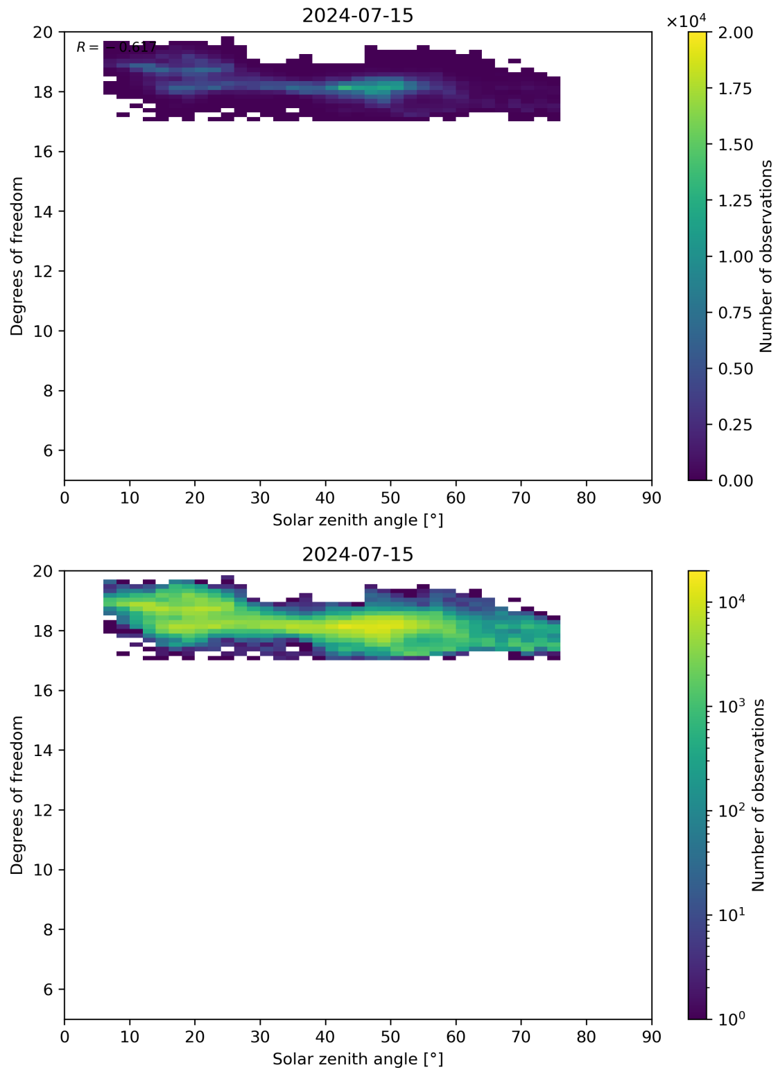
Figure 96: Scatter density plot of “Solar zenith angle” against “Degrees of freedom” for 2024-07-15 to 2024-07-16.
