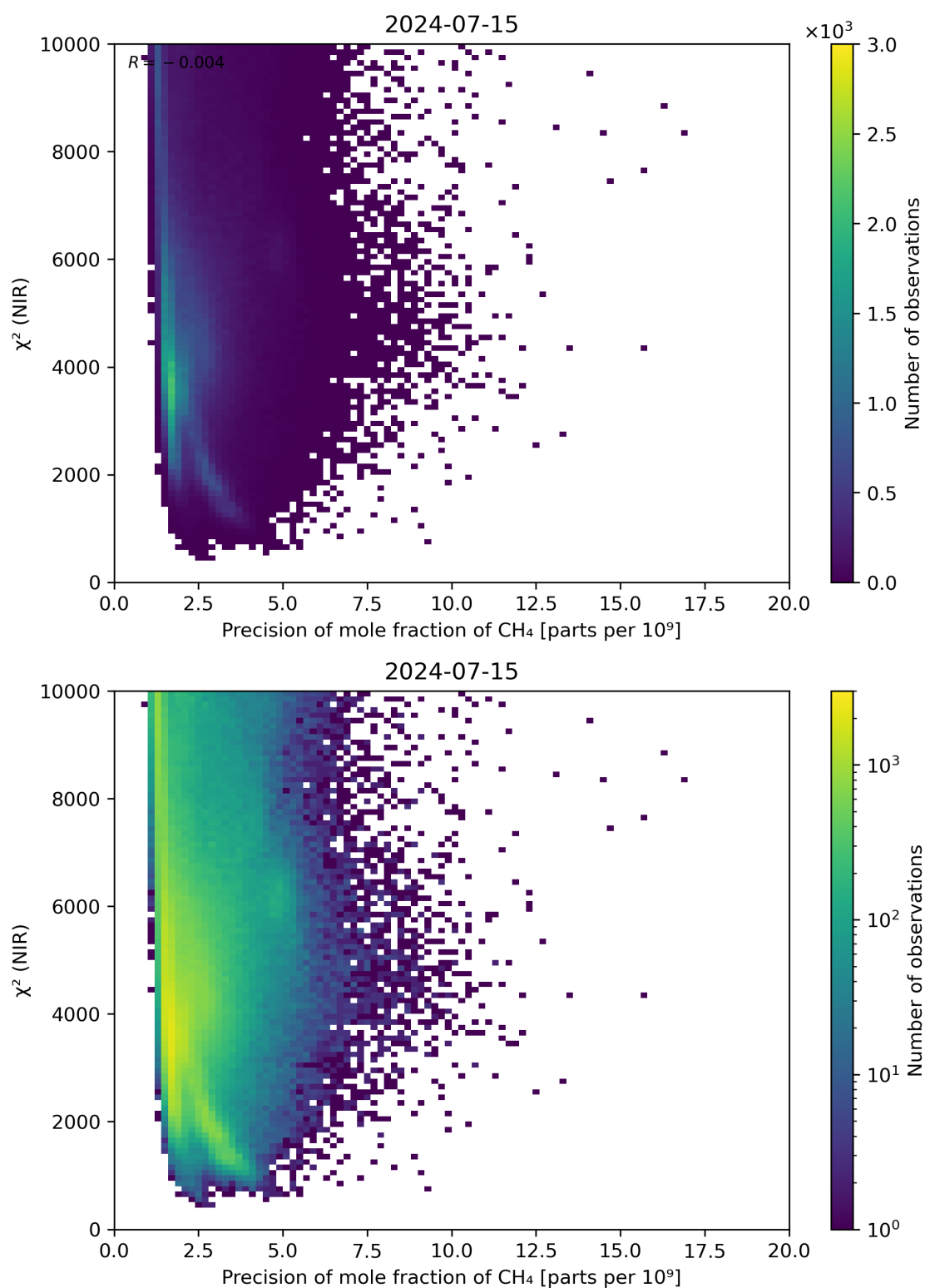
Figure 78: Scatter density plot of “Precision of mole fraction of \text{CH}_4 ” against “ \chi^2 (NIR)” for 2024-07-15 to 2024-07-16.
