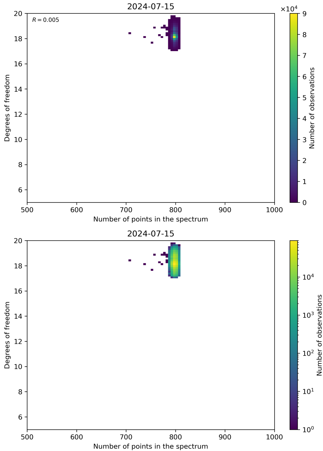
Figure 90: Scatter density plot of “Number of points in the spectrum” against “Degrees of freedom” for 2024-07-15 to 2024-07-16.
