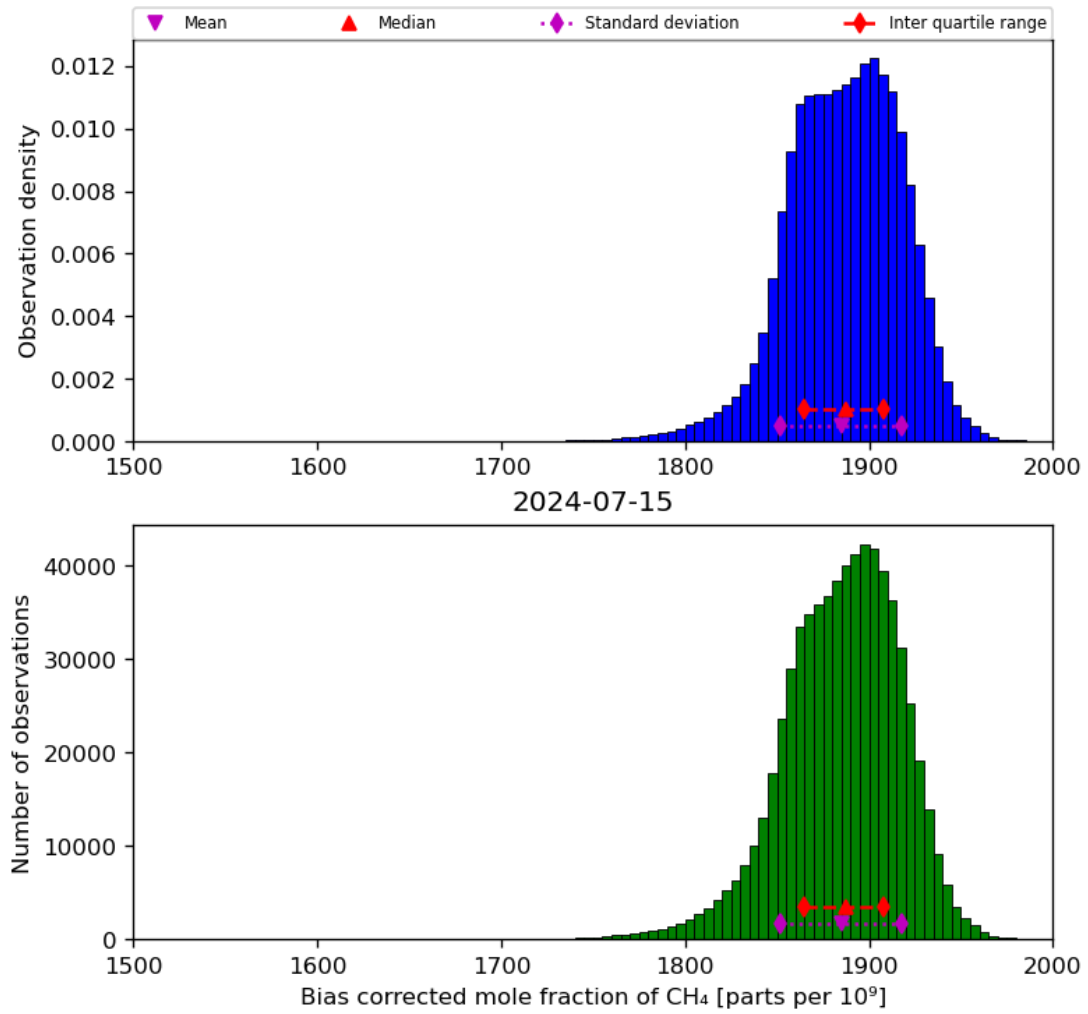
Figure 25: Histogram of “Bias corrected mole fraction of CH 4 ” for 2024-07-15 to 2024-07-16
