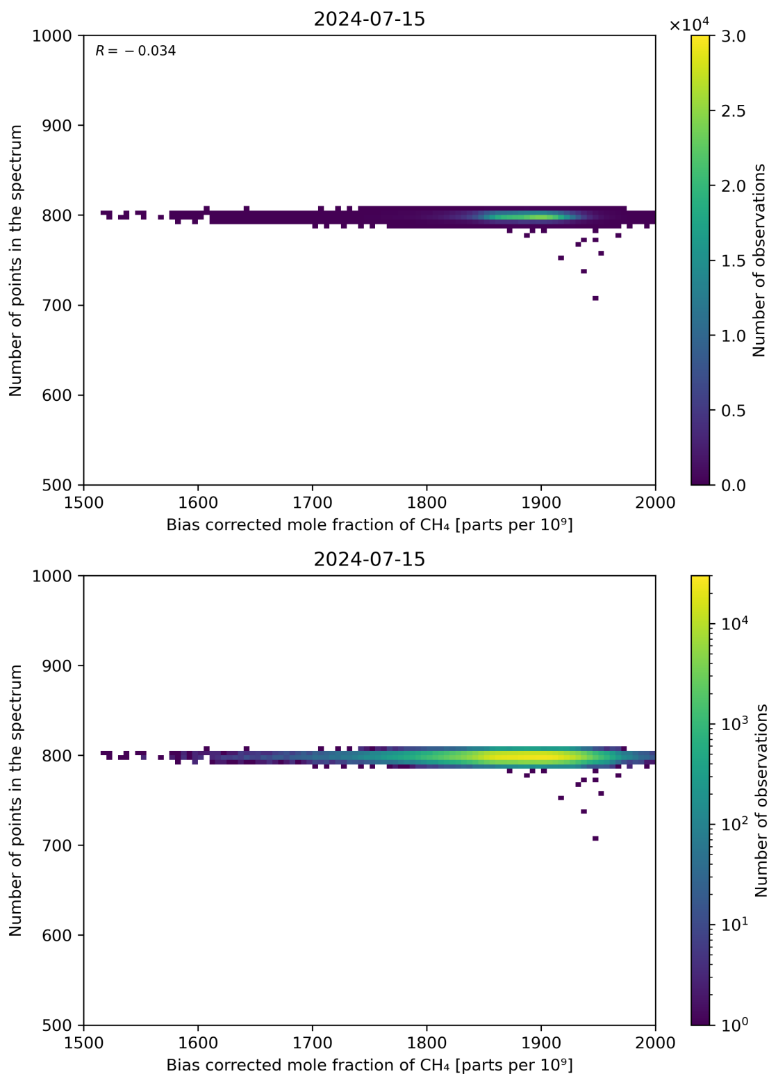
Figure 68: Scatter density plot of “Bias corrected mole fraction of CH 4 ” against “Number of points in the spectrum” for 2024-07-15 to 2024-07-16.
