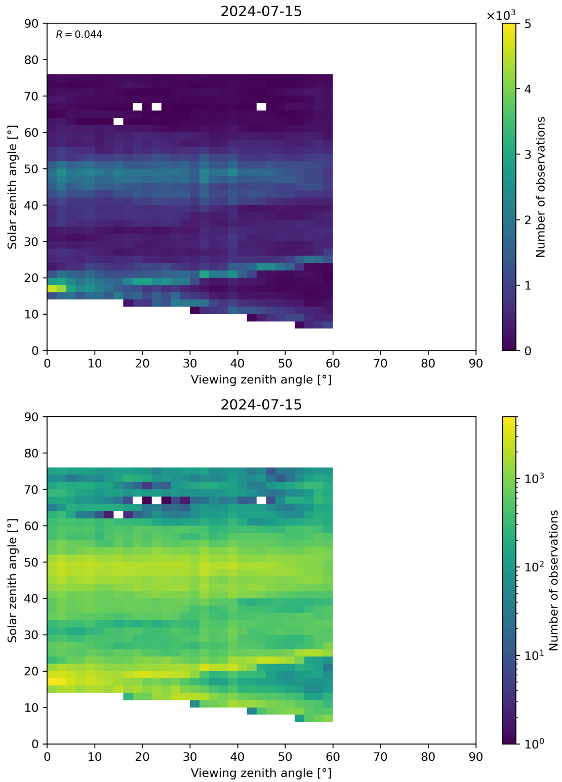
Figure 115: Scatter density plot of “Viewing zenith angle” against “Solar zenith angle” for 2024-07-15 to 2024-07-16.
