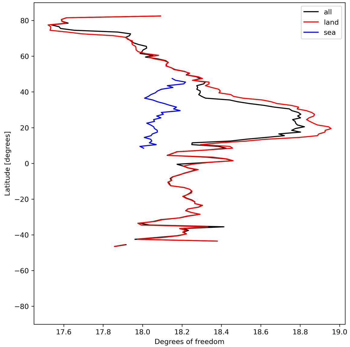
Figure 19: Zonal average of “Degrees of freedom” for 2024-07-15 to 2024-07-16.
