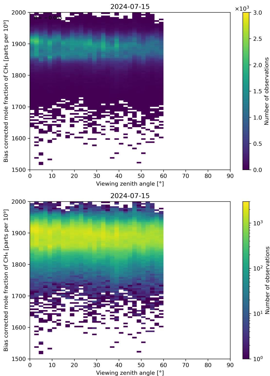
Figure 111: Scatter density plot of “Viewing zenith angle” against “Bias corrected mole fraction of CH 4 ” for 2024-07-15 to 2024-07-16.
