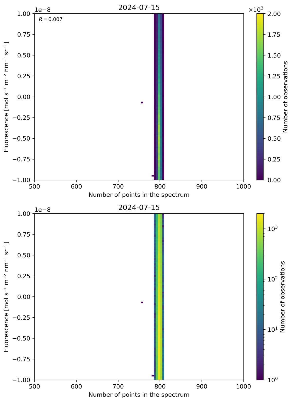
Figure 91: Scatter density plot of “Number of points in the spectrum” against “Fluorescence” for 2024-07-15 to 2024-07-16.
