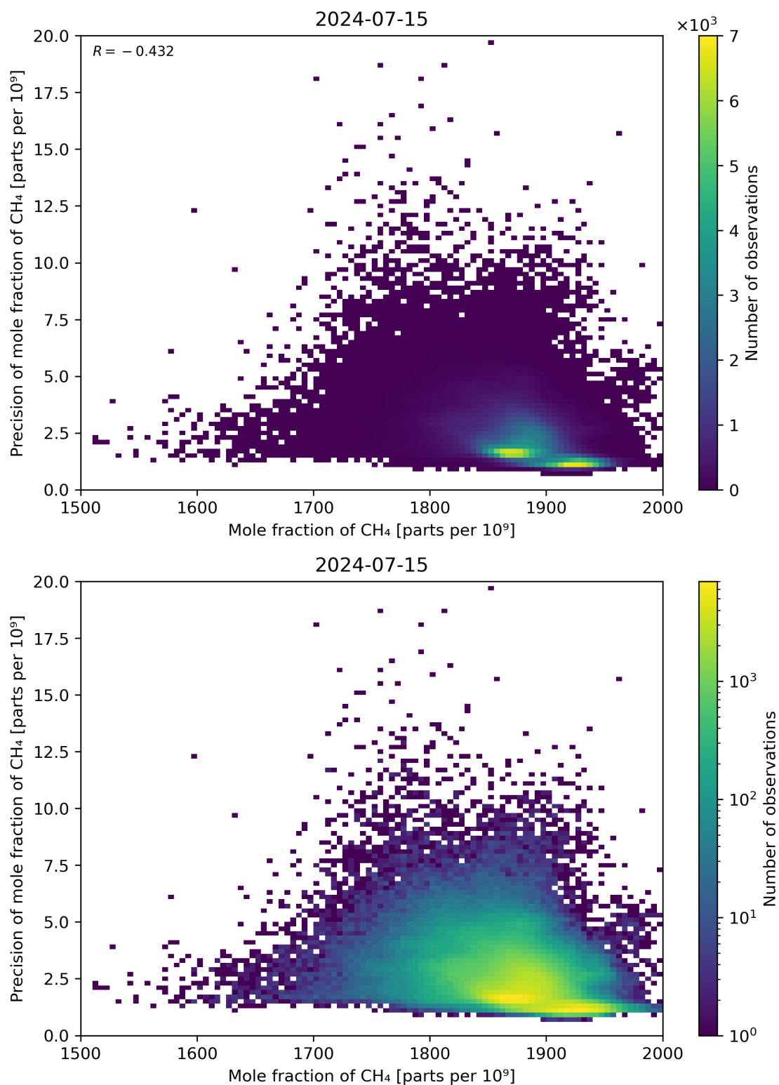
Figure 75: Scatter density plot of “Mole fraction of CH 4 ” against “Precision of mole fraction of CH 4 ” for 2024-07-15 to 2024-07-16.
