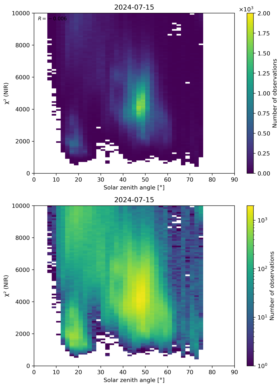
Figure 94: Scatter density plot of “Solar zenith angle” against “ \chi^2 (NIR)” for 2024-07-15 to 2024-07-16.
