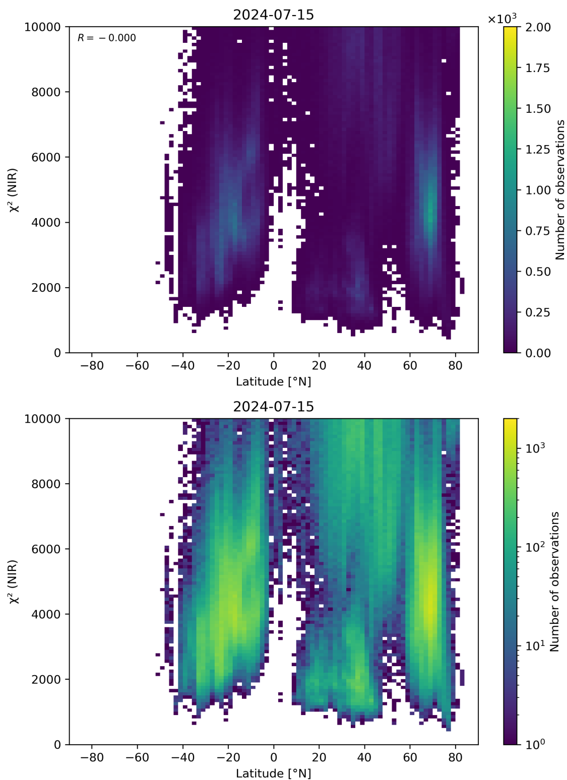
Figure 53: Scatter density plot of “Latitude” against “ \chi^2 (NIR)” for 2024-07-15 to 2024-07-16.
