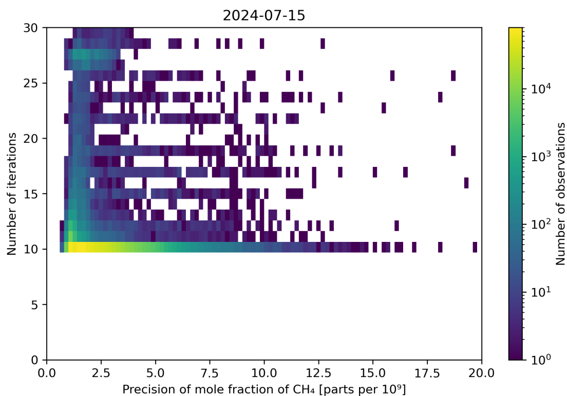
Figure 83: Scatter density plot of “Precision of mole fraction of CH 4 ” against “Number of iterations” for 2024-07-15 to 2024-07-16.
