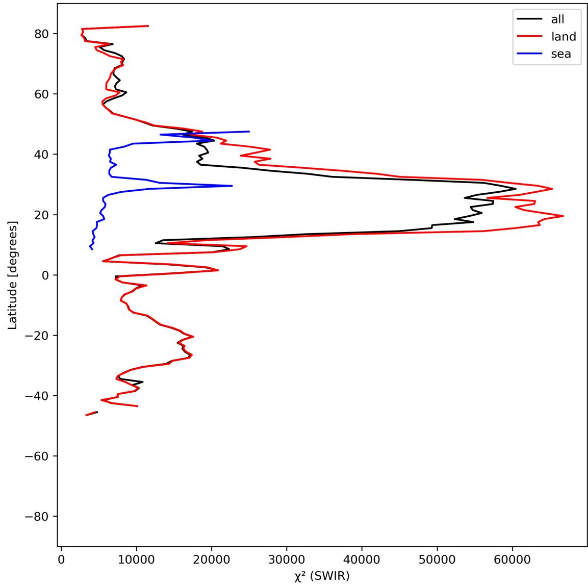
Figure 17: Zonal average of “ \chi^2 (SWIR)” for 2024-07-15 to 2024-07-16.
