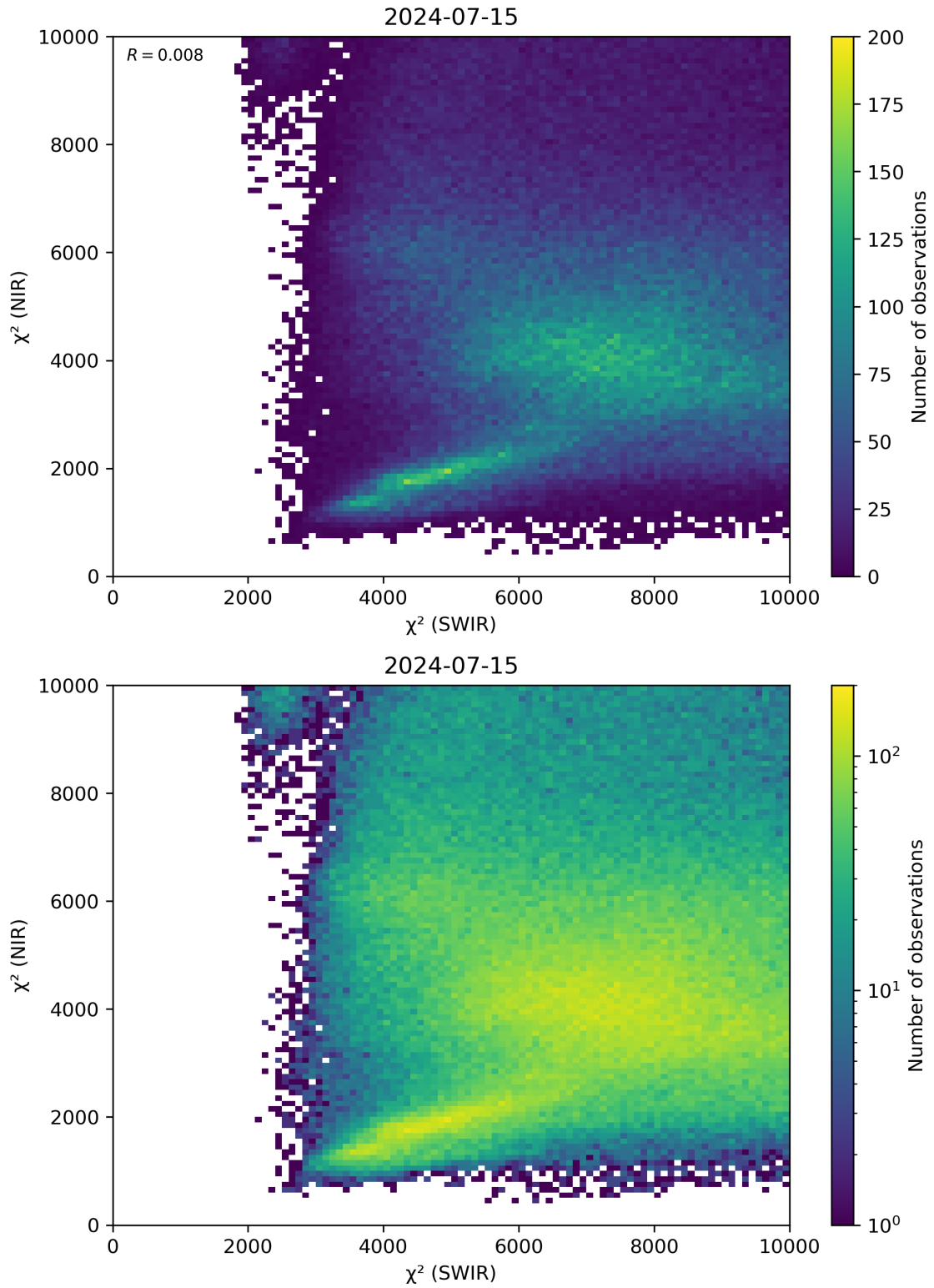
Figure 47: Scatter density plot of “ \chi^2 (SWIR)” against “ \chi^2 (NIR)” for 2024-07-15 to 2024-07-16.
