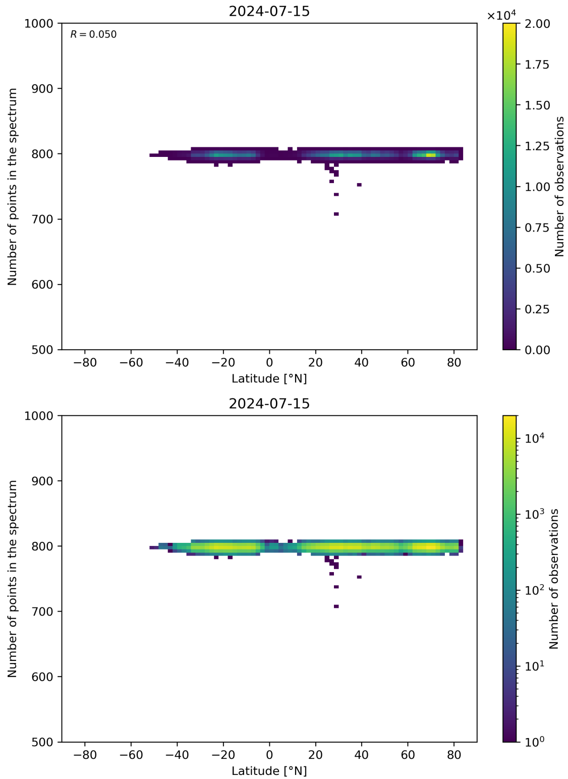
Figure 61: Scatter density plot of “Latitude” against “Number of points in the spectrum” for 2024-07-15 to 2024-07-16.
