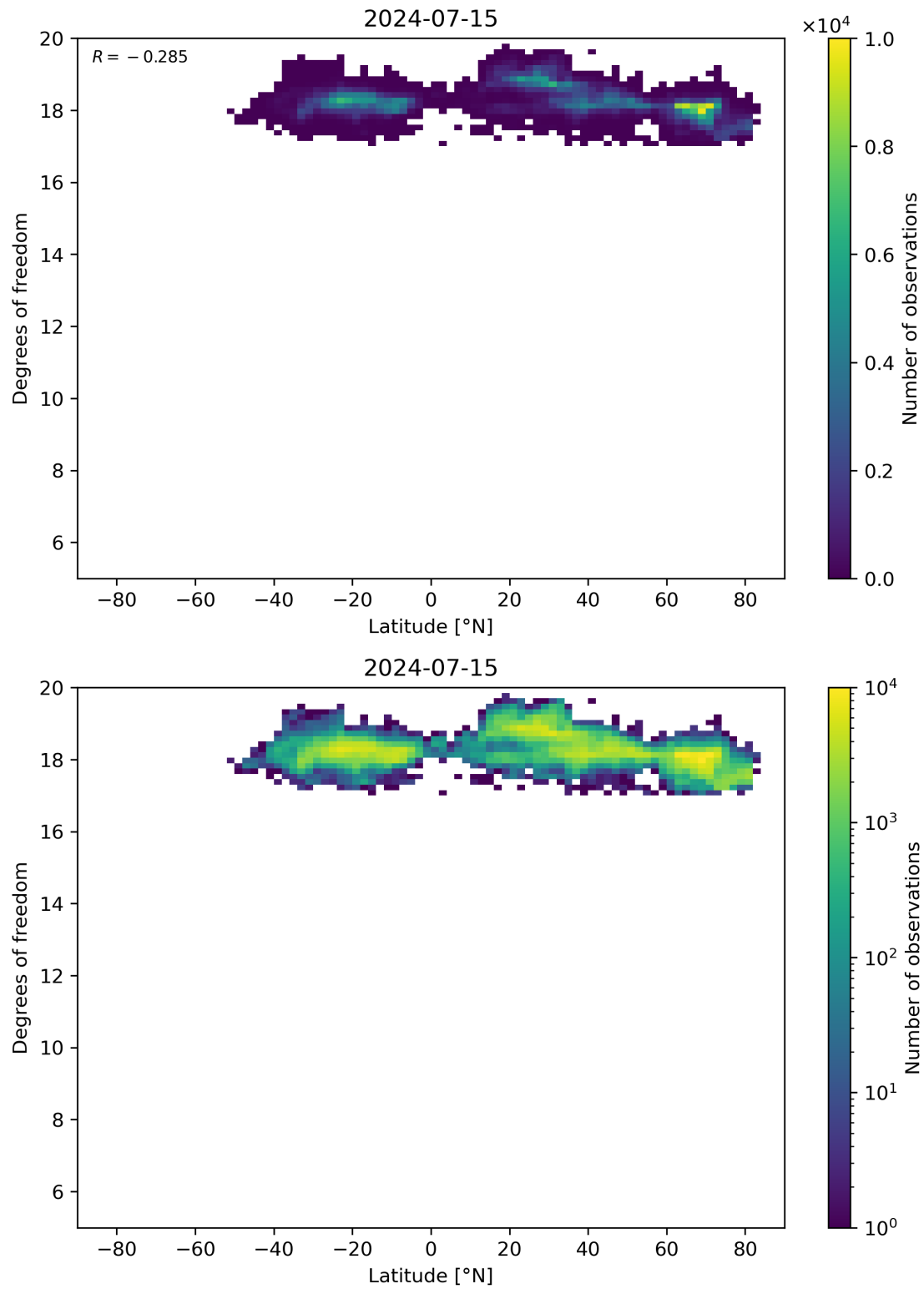
Figure 55: Scatter density plot of “Latitude” against “Degrees of freedom” for 2024-07-15 to 2024-07-16.
