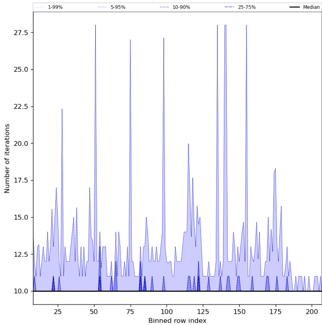
Figure 42: Along track statistics of “Number of iterations” for 2024-07-15 to 2024-07-16
