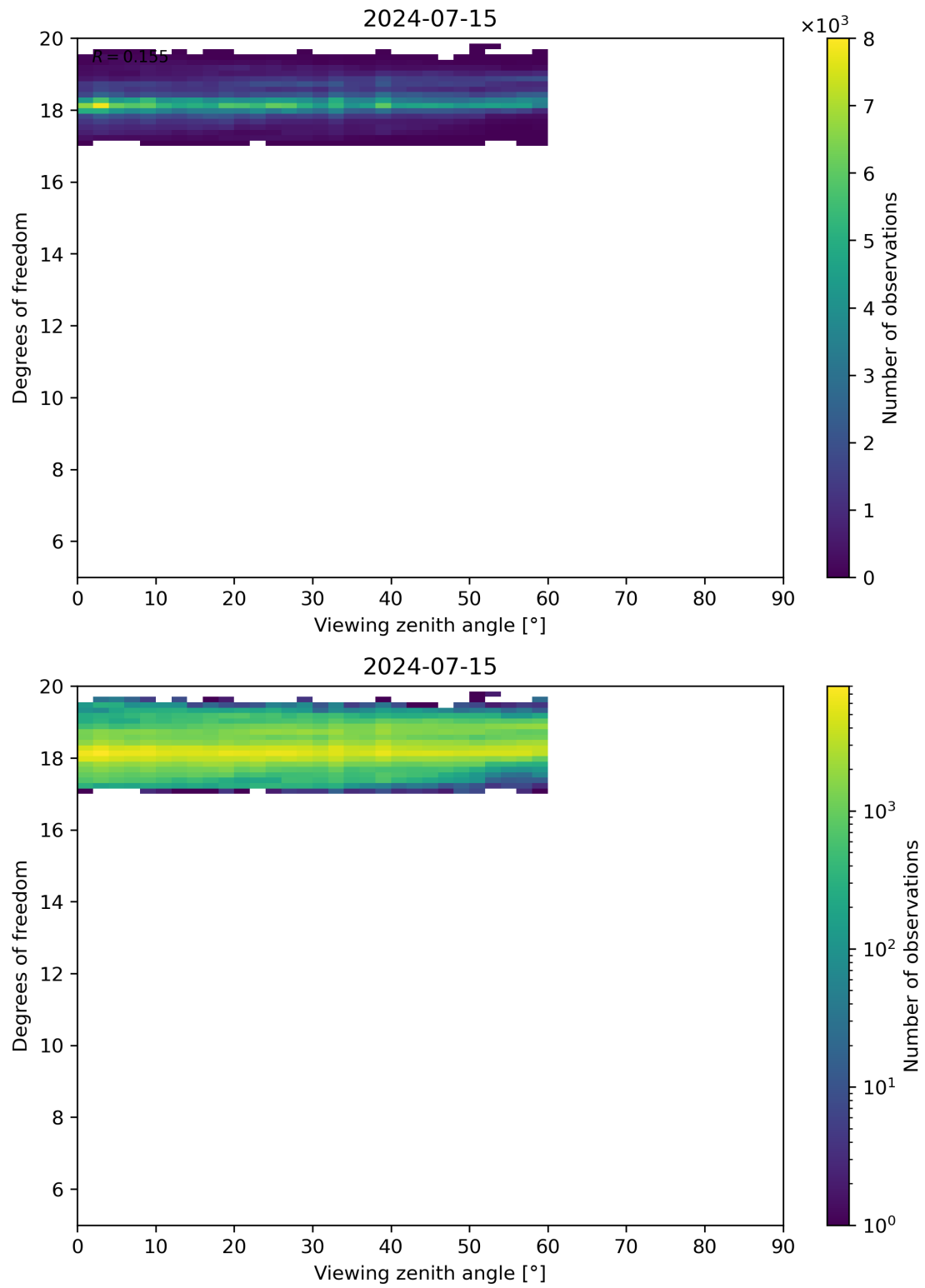
Figure 107: Scatter density plot of “Viewing zenith angle” against “Degrees of freedom” for 2024-07-15 to 2024-07-16.
