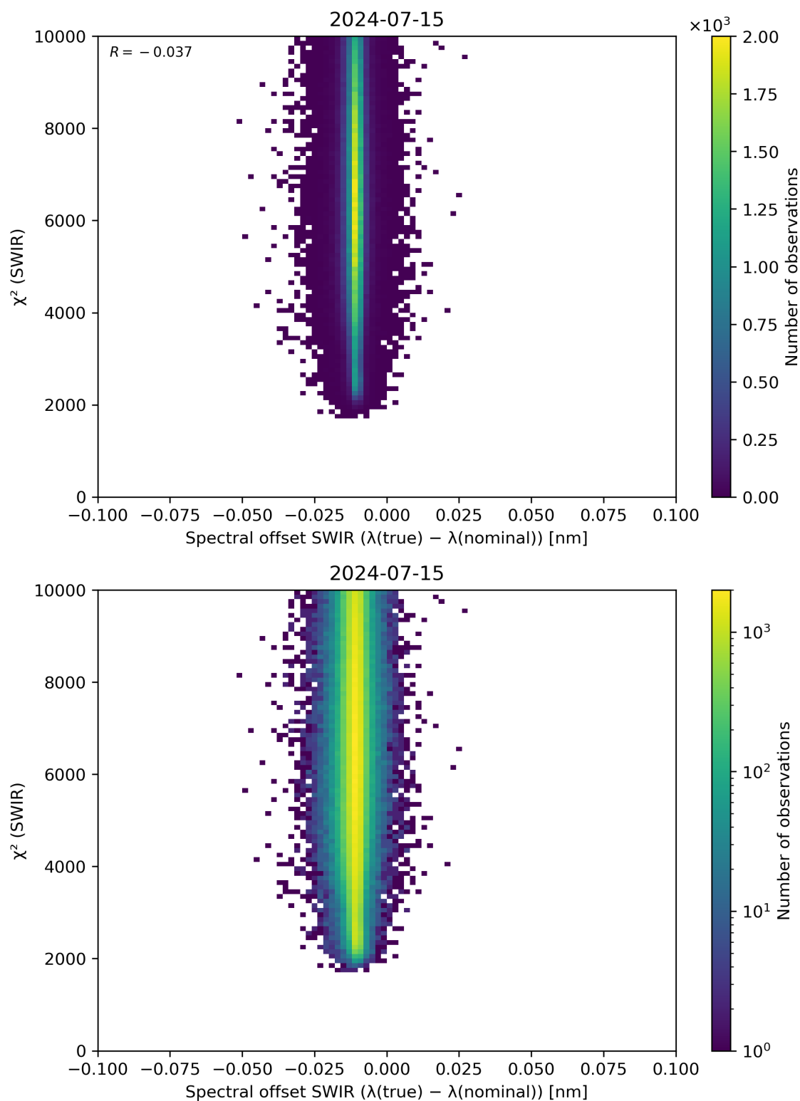
Figure 118: Scatter density plot of “Spectral offset SWIR ( \lambda(\text{true}) - \lambda(\text{nominal}) )” against “ \chi^2 (SWIR)” for 2024-07-15 to 2024-07-16.
