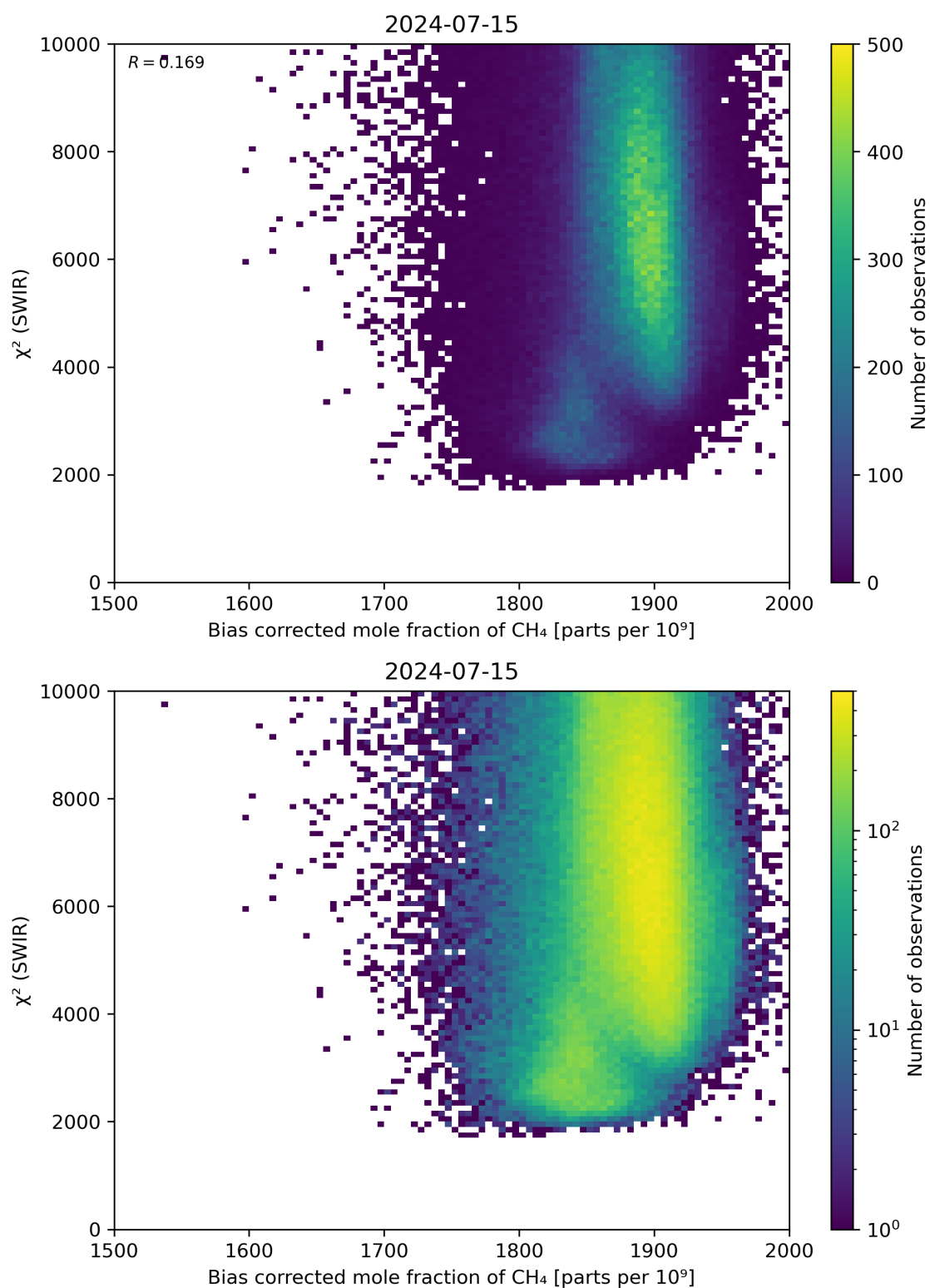
Figure 64: Scatter density plot of “Bias corrected mole fraction of CH 4 ” against “ \chi^2 (SWIR)” for 2024-07-15 to 2024-07-16.
