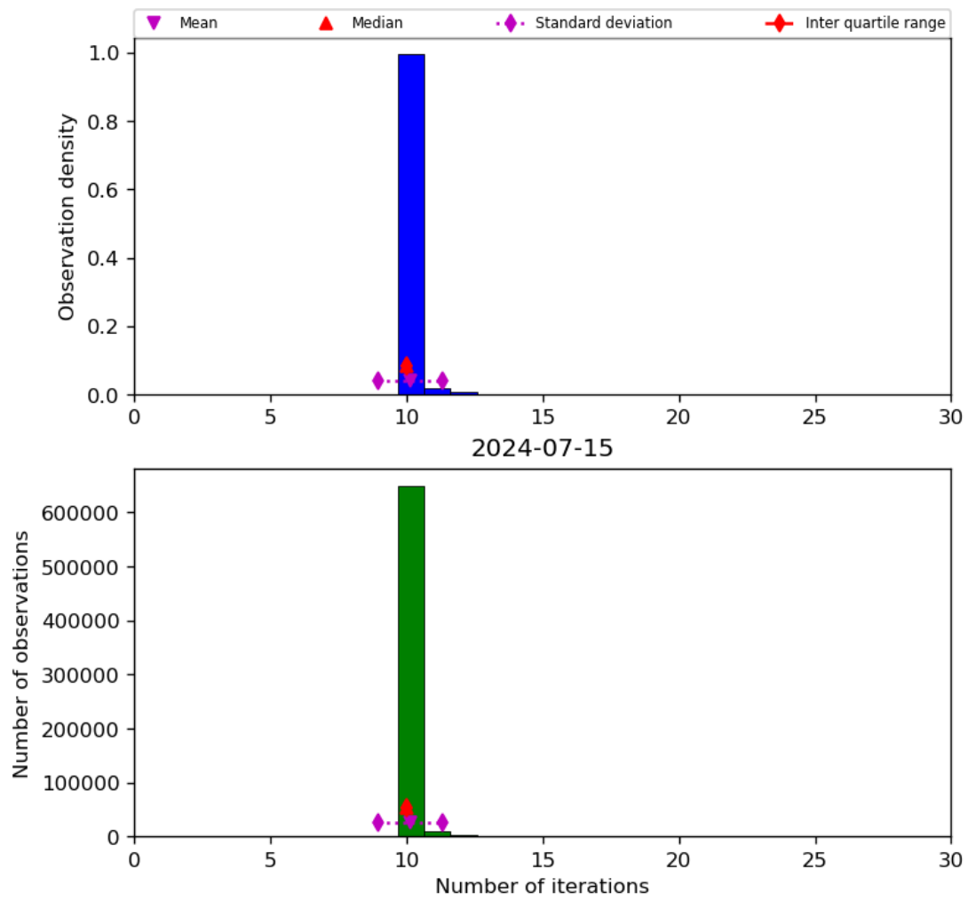
Figure 31: Histogram of “Number of iterations” for 2024-07-15 to 2024-07-16
