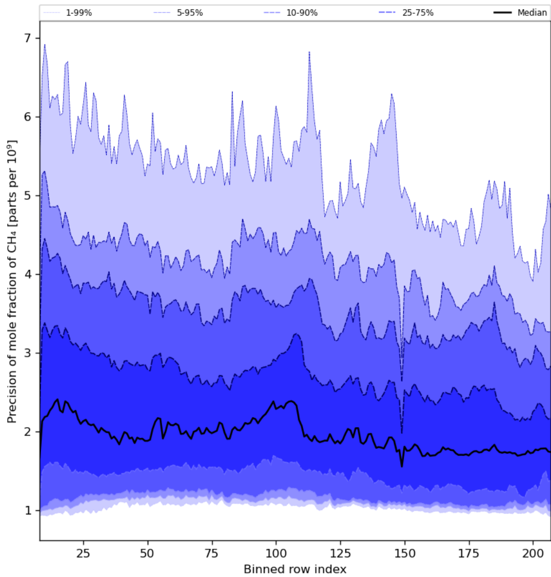
Figure 35: Along track statistics of “Precision of mole fraction of CH 4 ” for 2024-07-15 to 2024-07-16
