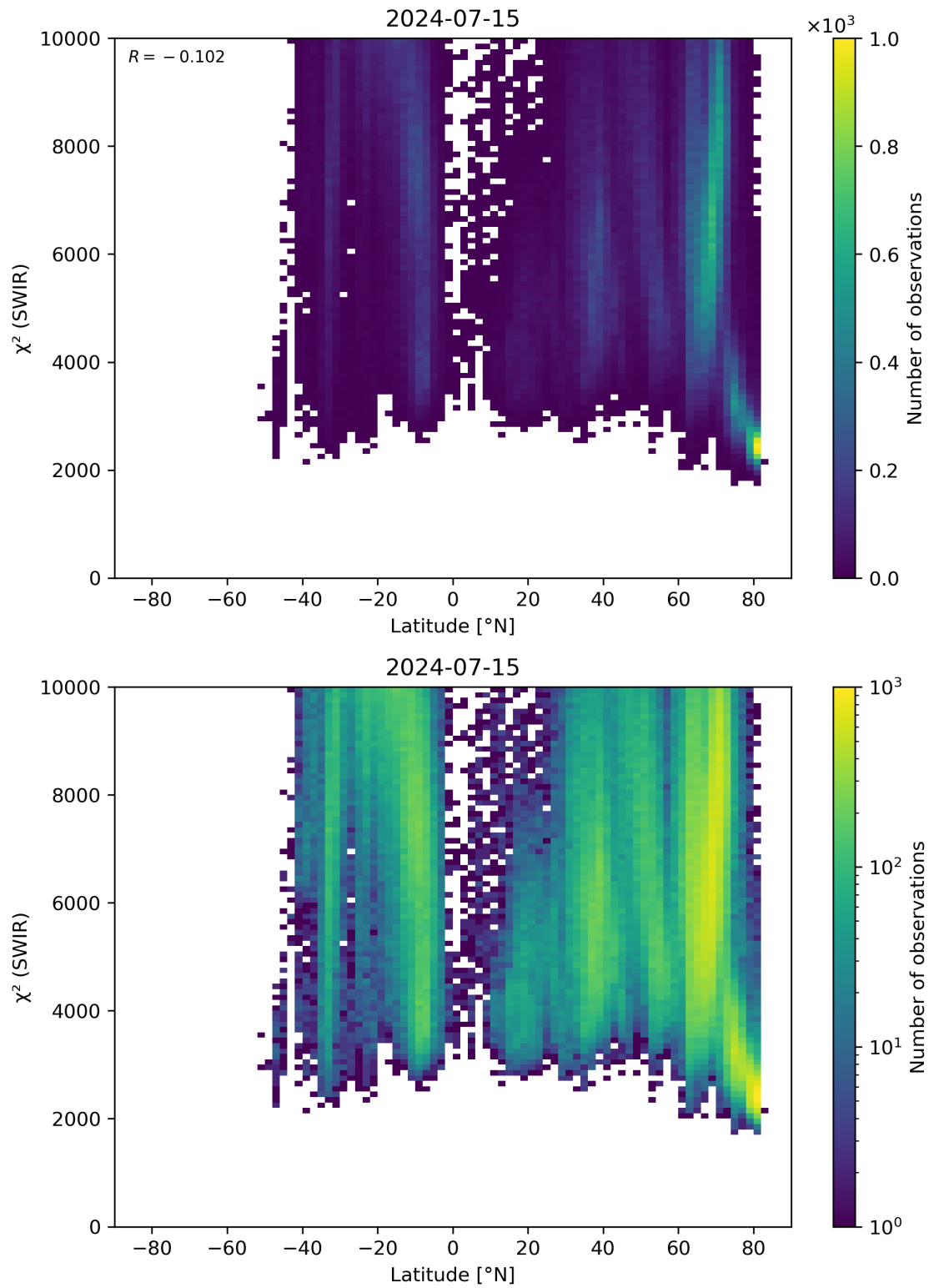
Figure 54: Scatter density plot of “Latitude” against “ \chi^2 (SWIR)” for 2024-07-15 to 2024-07-16.
