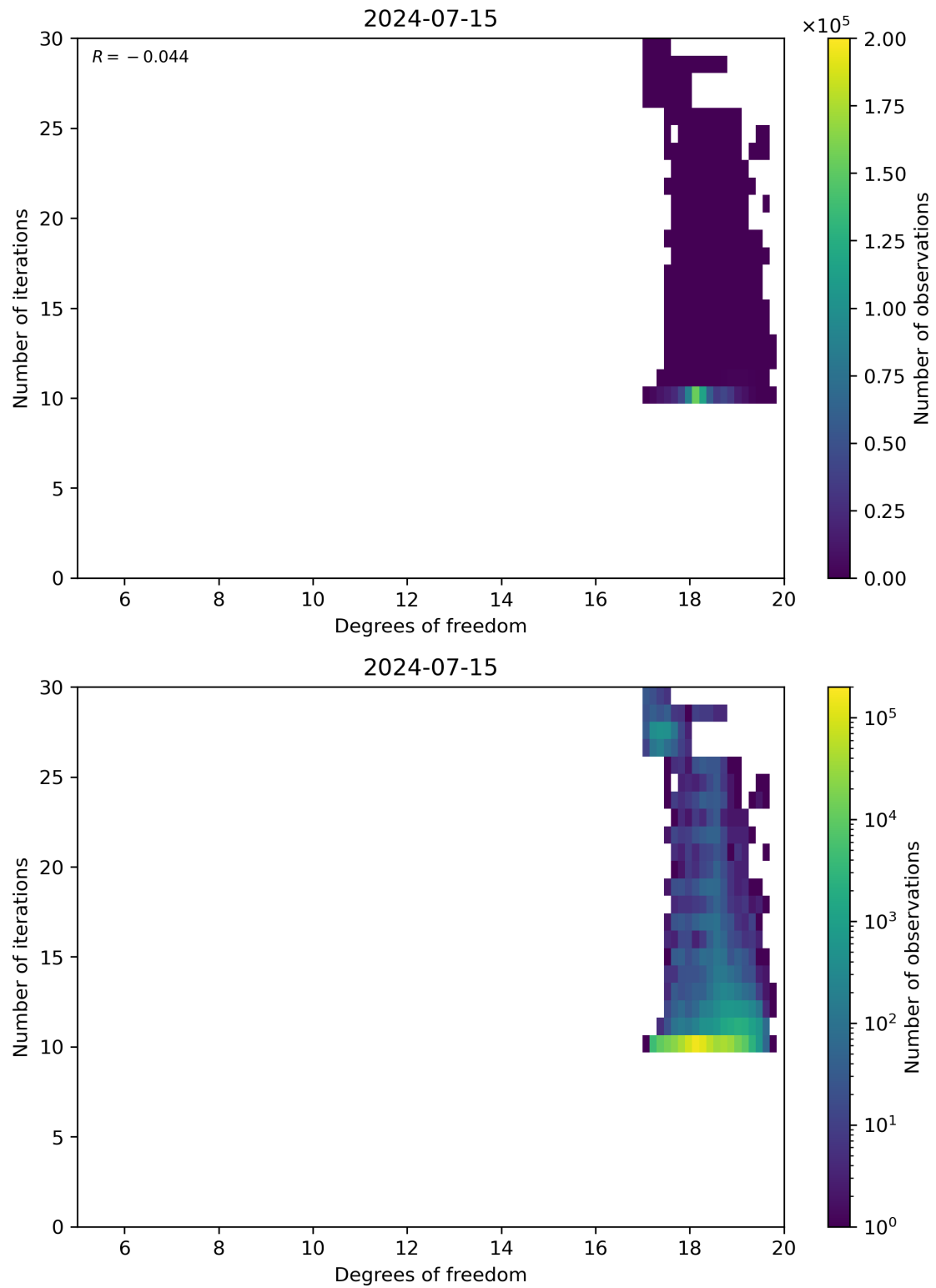
Figure 52: Scatter density plot of “Degrees of freedom” against “Number of iterations” for 2024-07-15 to 2024-07-16.
