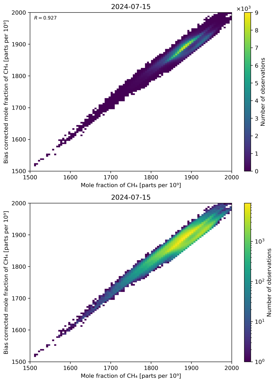
Figure 74: Scatter density plot of “Mole fraction of CH 4 ” against “Bias corrected mole fraction of CH 4 ” for 2024-07-15 to 2024-07-16.
