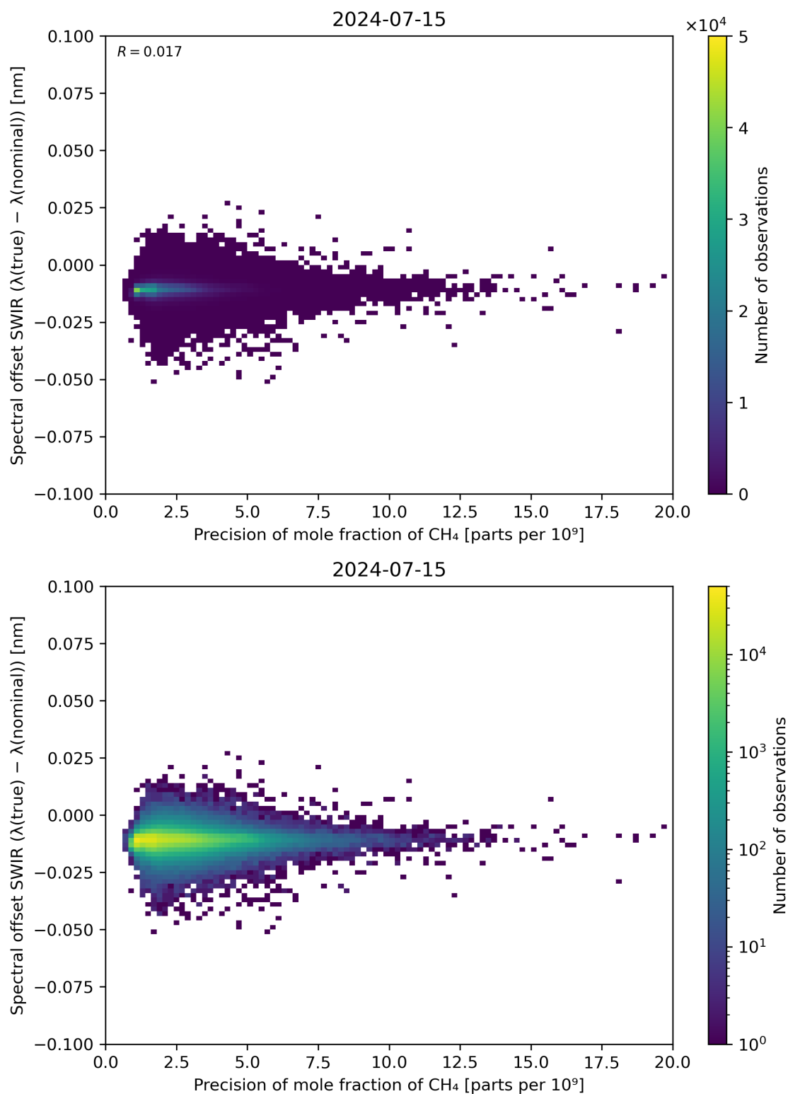
Figure 85: Scatter density plot of “Precision of mole fraction of \text{CH}_4 ” against “Spectral offset SWIR ( \lambda(\text{true}) - \lambda(\text{nominal}) )” for 2024-07-15 to 2024-07-16.
