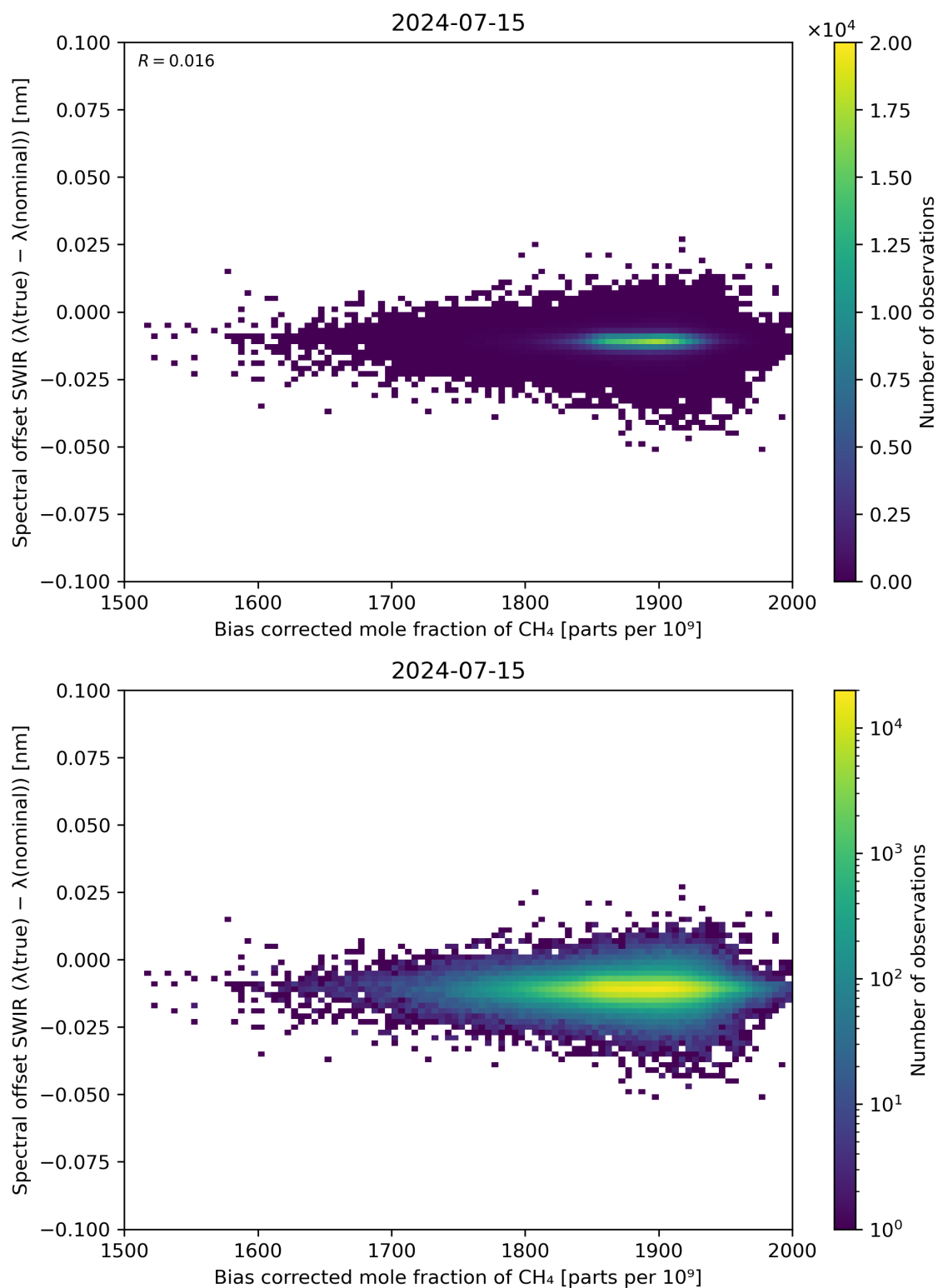
Figure 69: Scatter density plot of “Bias corrected mole fraction of \text{CH}_4 ” against “Spectral offset SWIR ( \lambda(\text{true}) - \lambda(\text{nominal}) )” for 2024-07-15 to 2024-07-16.
