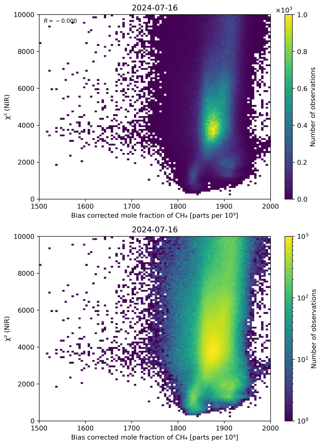
Figure 63: Scatter density plot of “Bias corrected mole fraction of CH 4 ” against “ \chi^2 (NIR)” for 2024-07-15 to 2024-07-17.
