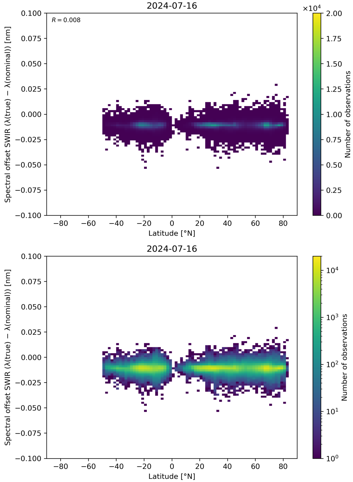
Figure 62: Scatter density plot of “Latitude” against “Spectral offset SWIR ( \lambda(\text{true}) - \lambda(\text{nominal}) )” for 2024-07-15 to 2024-07-17.
