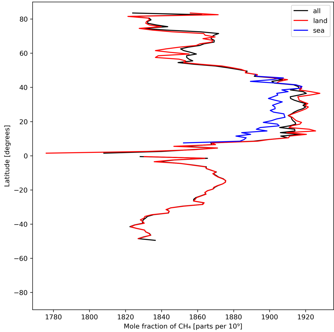
Figure 12: Zonal average of “Mole fraction of \text{CH}_4 ” for 2024-07-15 to 2024-07-17.
