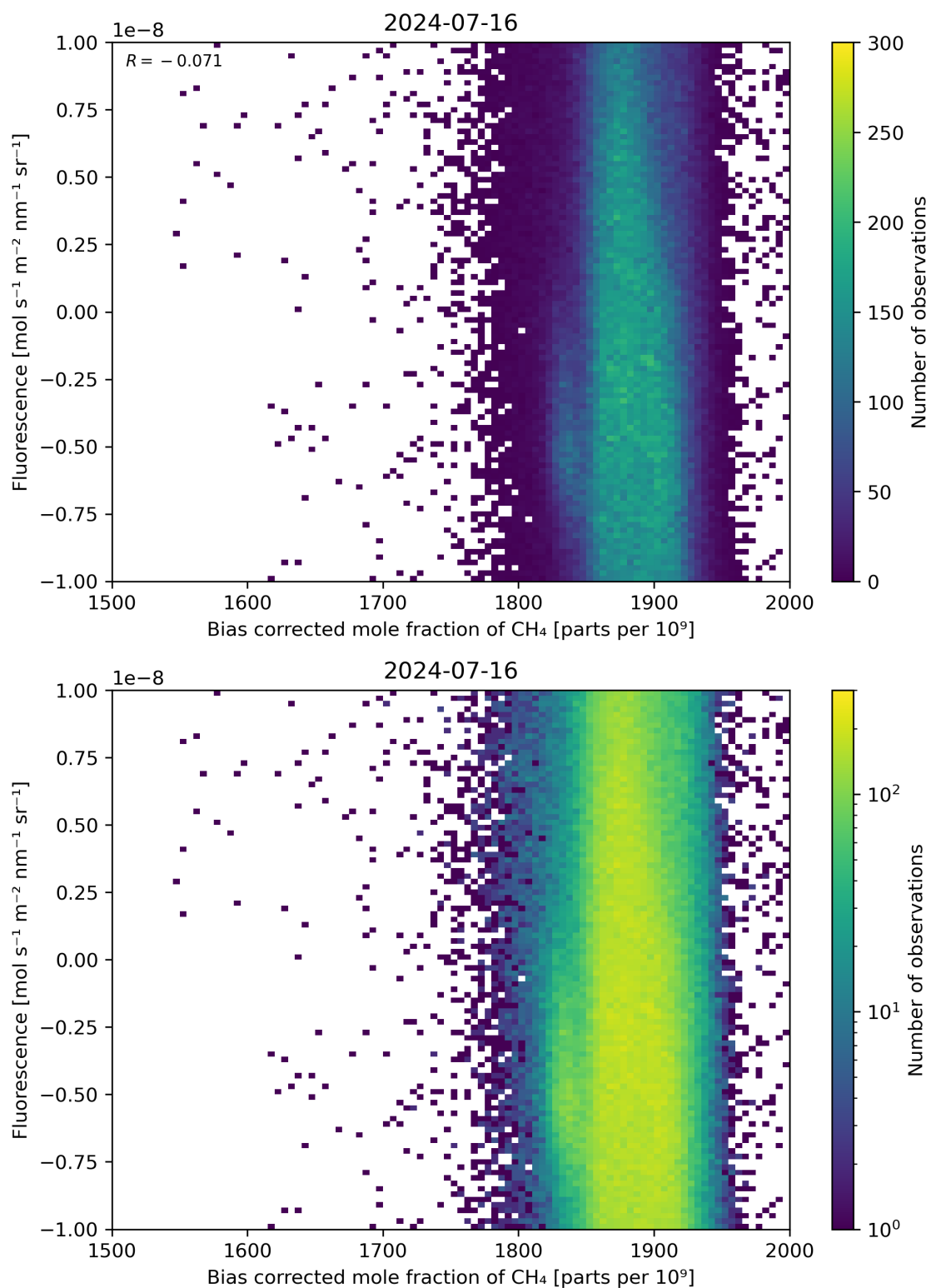
Figure 66: Scatter density plot of “Bias corrected mole fraction of \text{CH}_4 ” against “Fluorescence” for 2024-07-15 to 2024-07-17.
