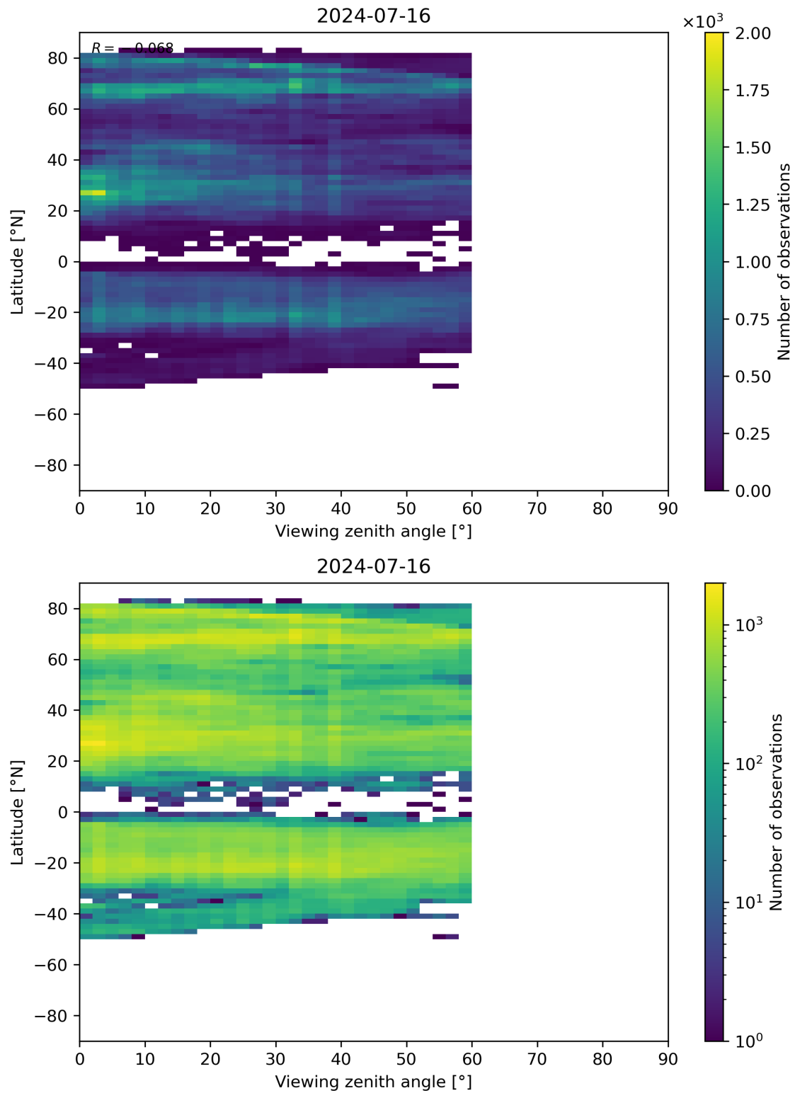
Figure 109: Scatter density plot of “Viewing zenith angle” against “Latitude” for 2024-07-15 to 2024-07-17.
