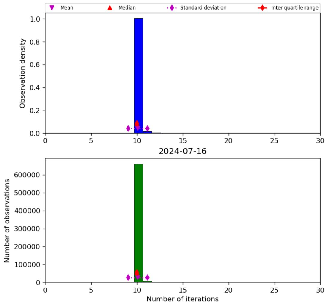
Figure 31: Histogram of “Number of iterations” for 2024-07-15 to 2024-07-17
