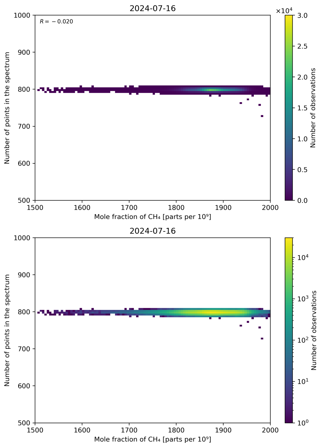
Figure 77: Scatter density plot of “Mole fraction of CH 4 ” against “Number of points in the spectrum” for 2024-07-15 to 2024-07-17.
