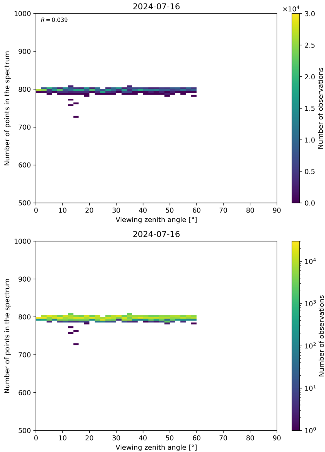
Figure 114: Scatter density plot of “Viewing zenith angle” against “Number of points in the spectrum” for 2024-07-15 to 2024-07-17.
