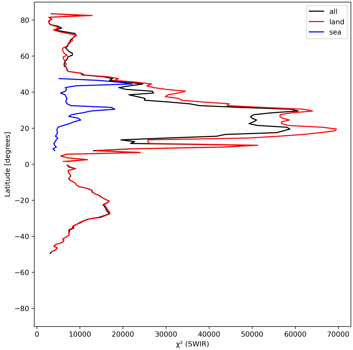
Figure 17: Zonal average of “ \chi^2 (SWIR)” for 2024-07-15 to 2024-07-17.
