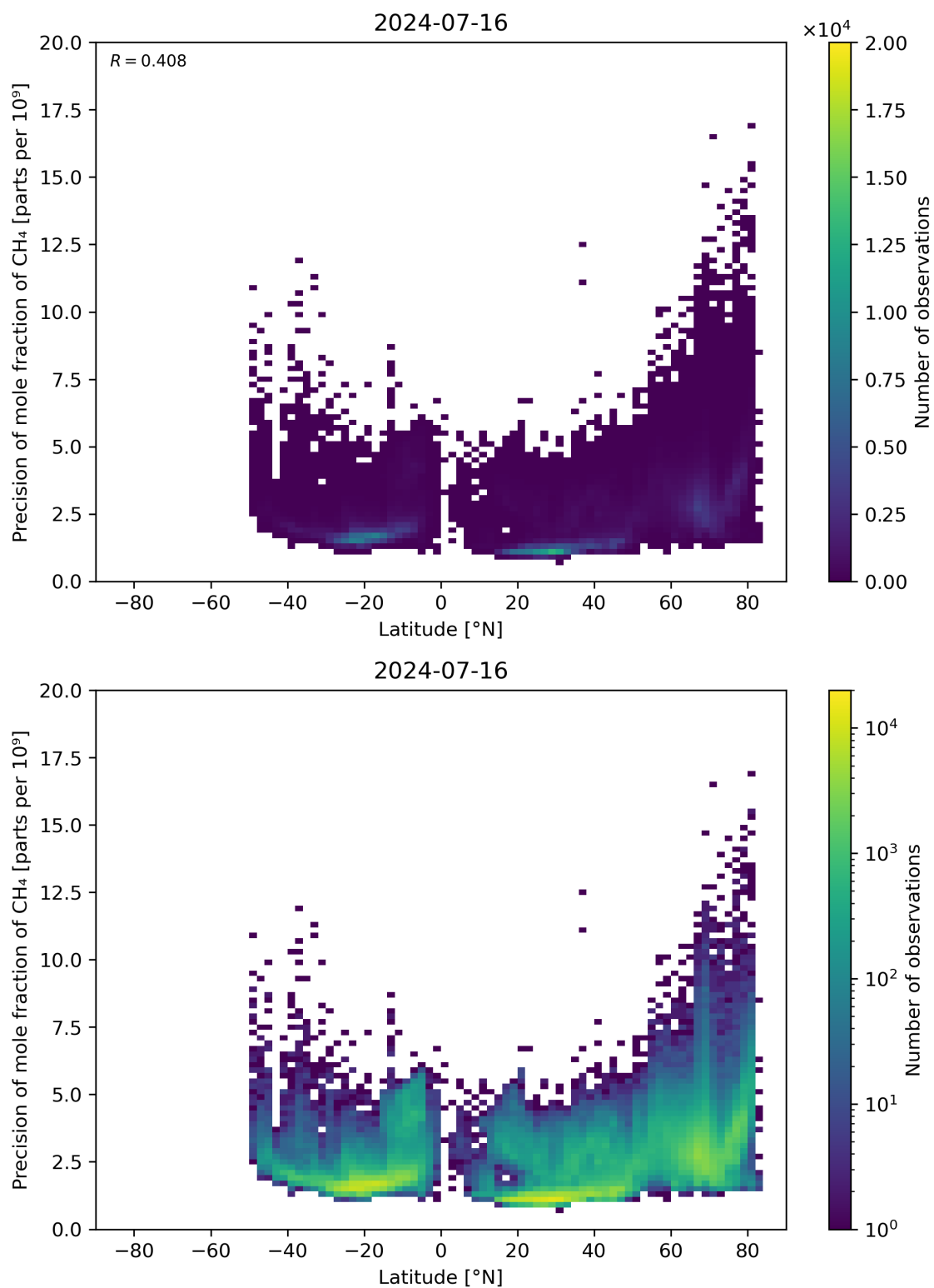
Figure 59: Scatter density plot of “Latitude” against “Precision of mole fraction of \text{CH}_4 ” for 2024-07-15 to 2024-07-17.
