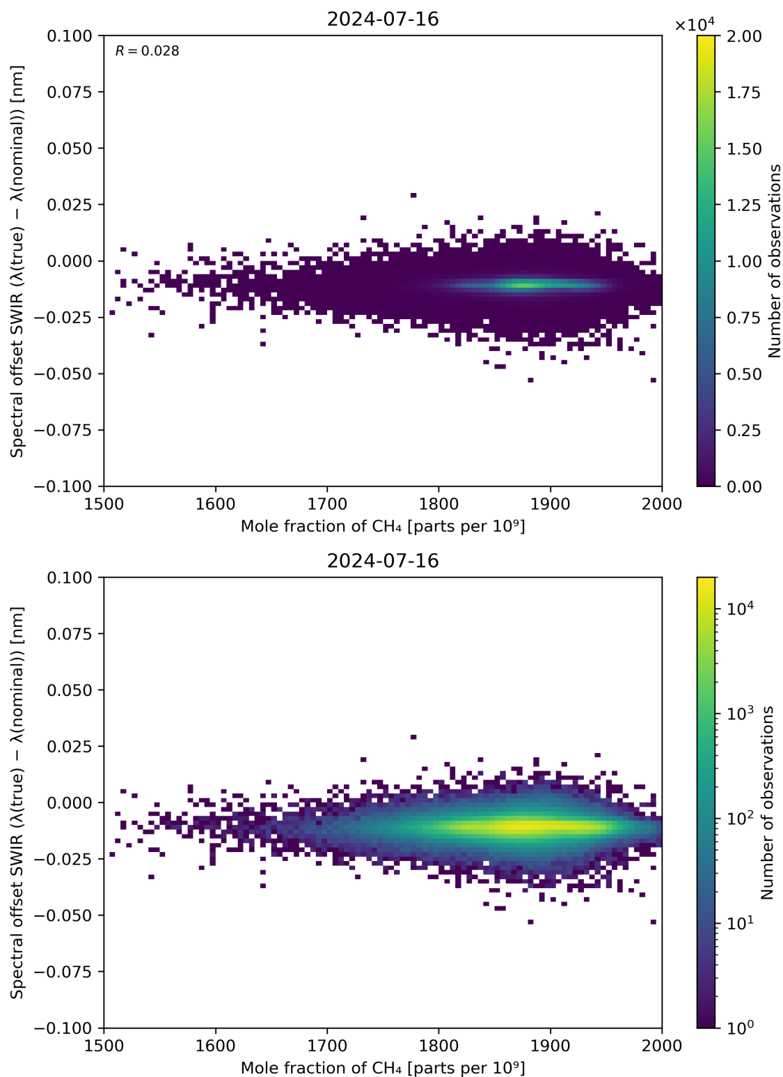
Figure 86: Scatter density plot of “Mole fraction of CH 4 ” against “Spectral offset SWIR ( \lambda(\text{true}) - \lambda(\text{nominal}) )” for 2024-07-15 to 2024-07-17.
