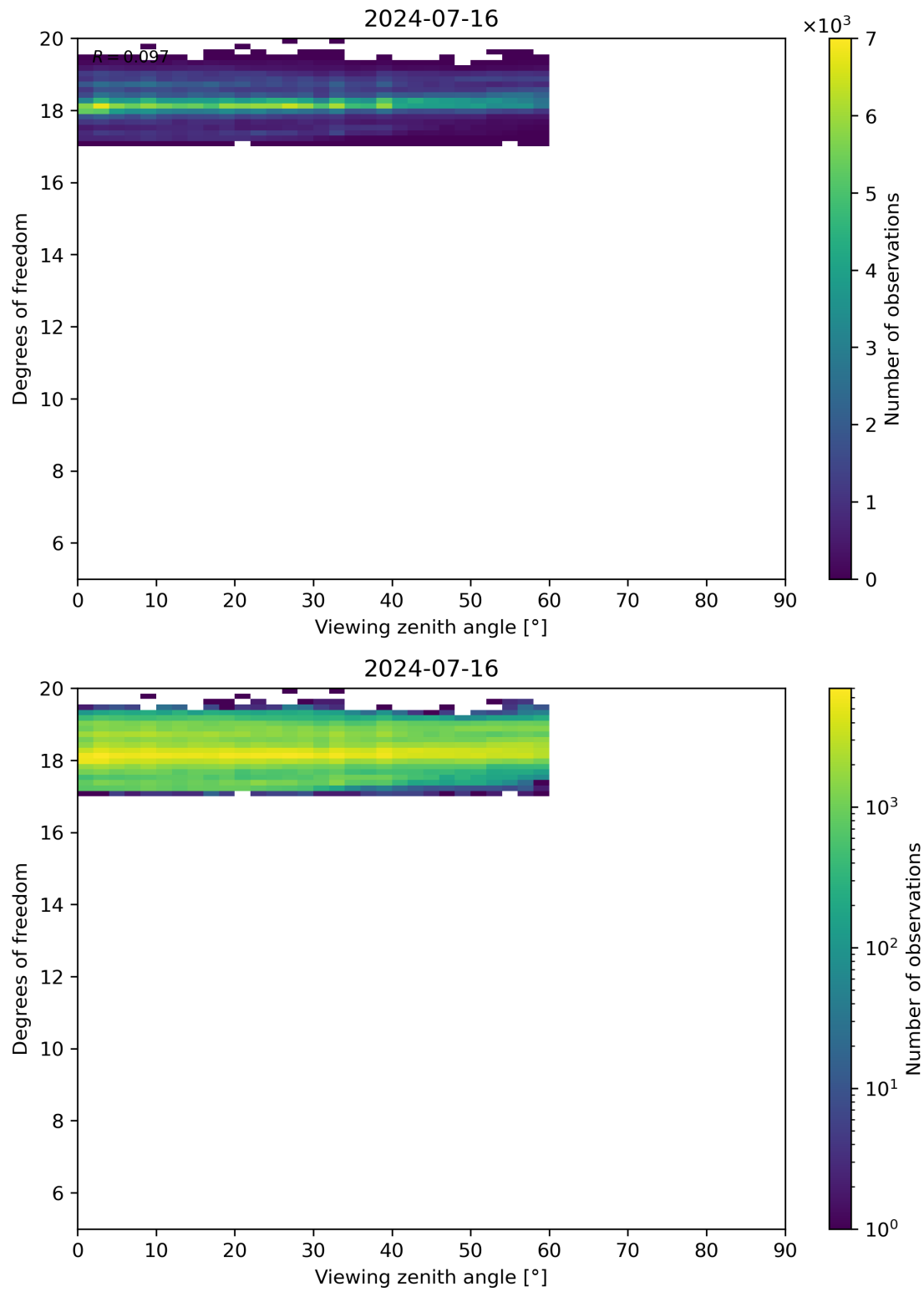
Figure 107: Scatter density plot of “Viewing zenith angle” against “Degrees of freedom” for 2024-07-15 to 2024-07-17.
