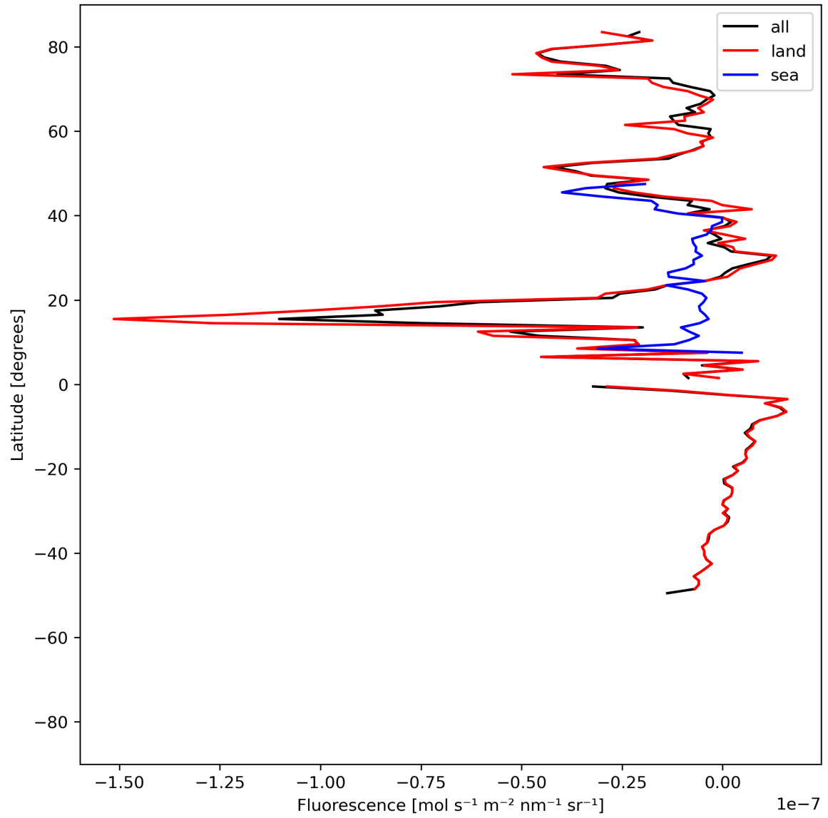
Figure 21: Zonal average of “Fluorescence” for 2024-07-15 to 2024-07-17.
