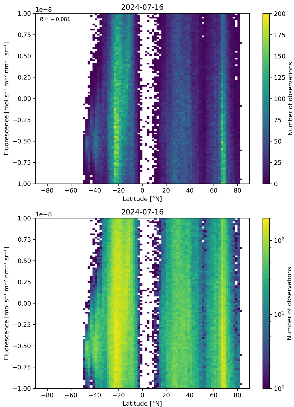
Figure 56: Scatter density plot of “Latitude” against “Fluorescence” for 2024-07-15 to 2024-07-17.
