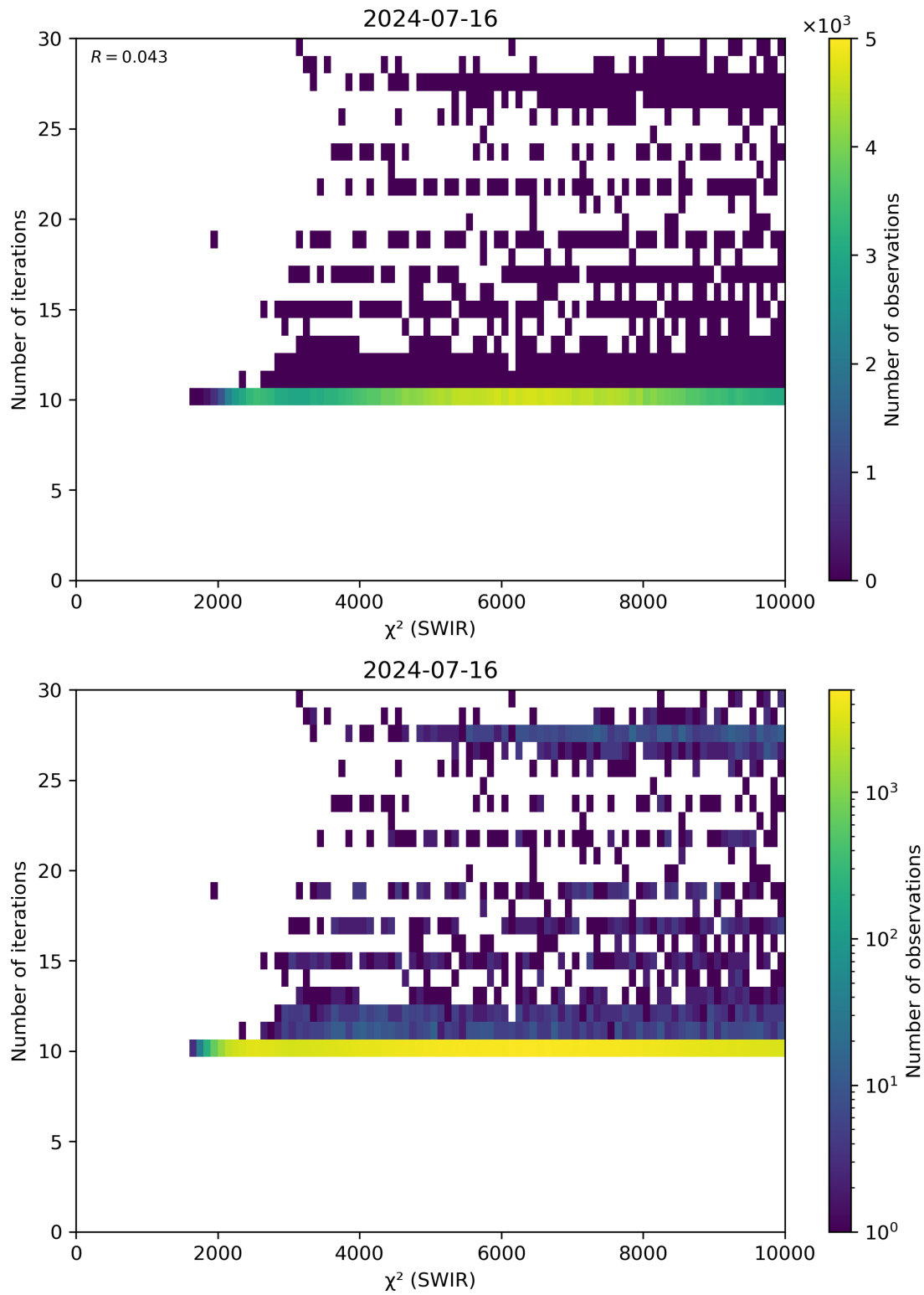
Figure 50: Scatter density plot of “ \chi^2 (SWIR)” against “Number of iterations” for 2024-07-15 to 2024-07-17.
