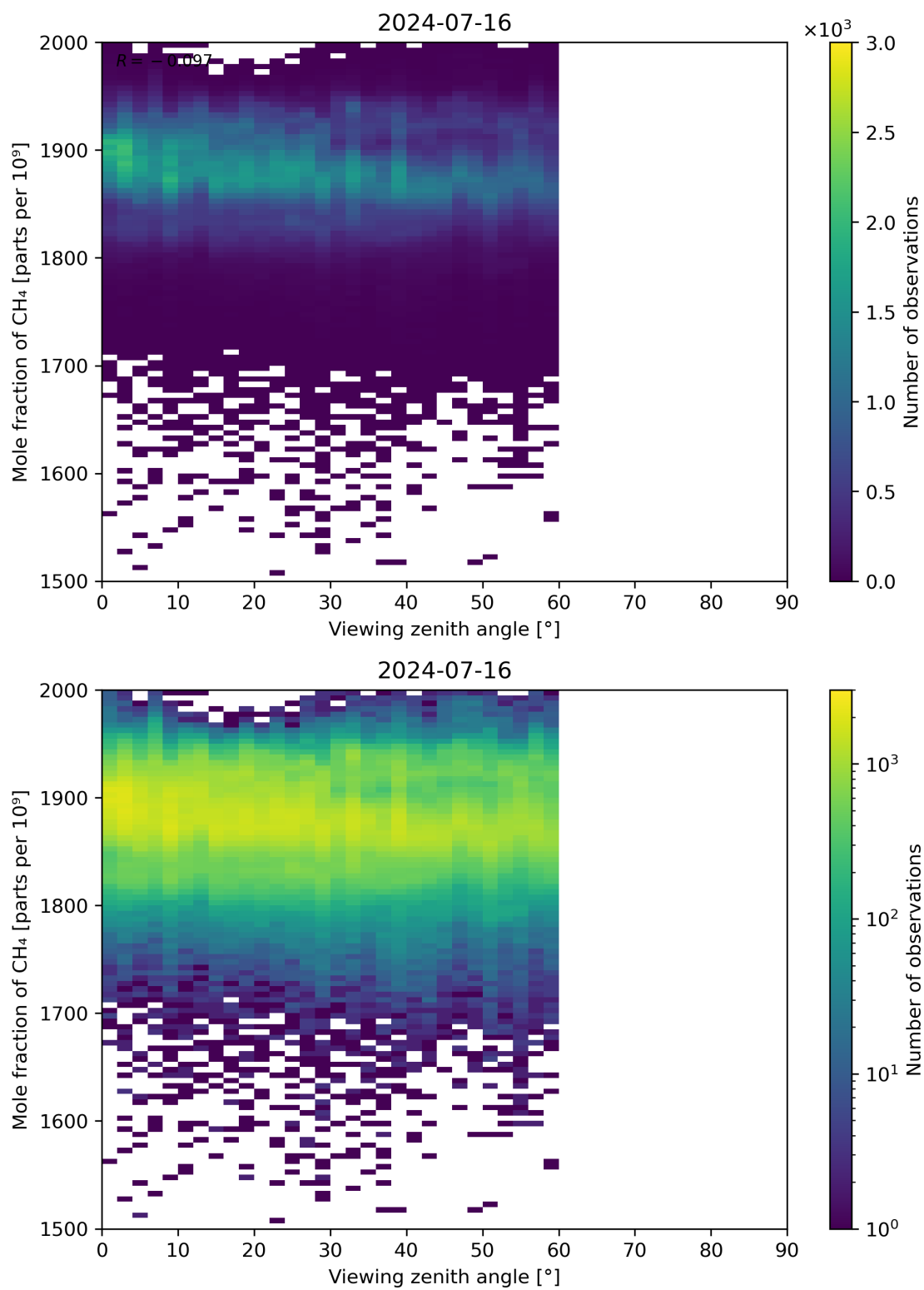
Figure 110: Scatter density plot of “Viewing zenith angle” against “Mole fraction of CH 4 ” for 2024-07-15 to 2024-07-17.
