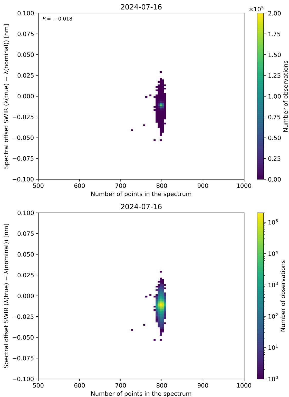
Figure 93: Scatter density plot of “Number of points in the spectrum” against “Spectral offset SWIR ( \lambda(\text{true}) - \lambda(\text{nominal}) )” for 2024-07-15 to 2024-07-17.
