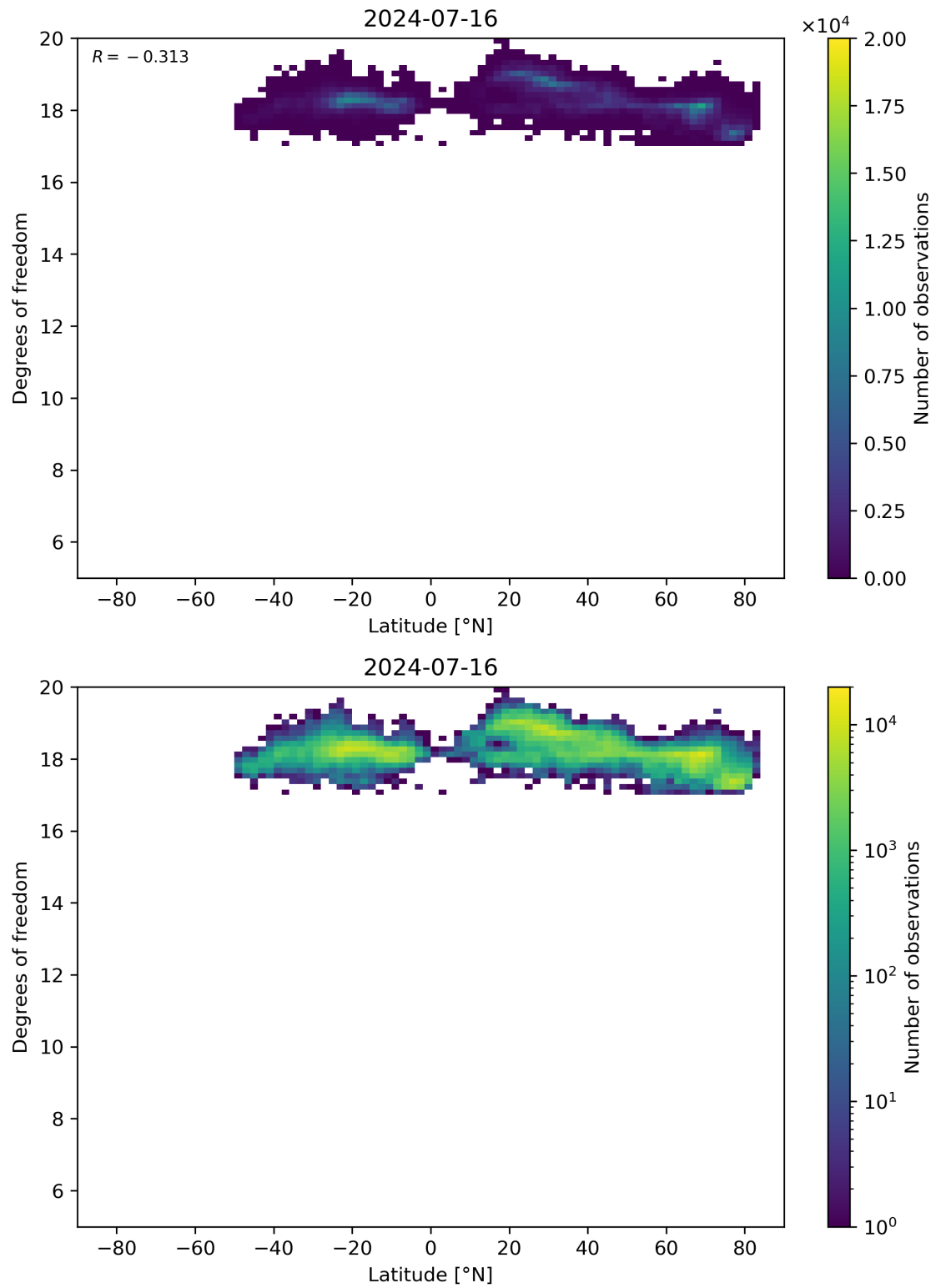
Figure 55: Scatter density plot of “Latitude” against “Degrees of freedom” for 2024-07-15 to 2024-07-17.
