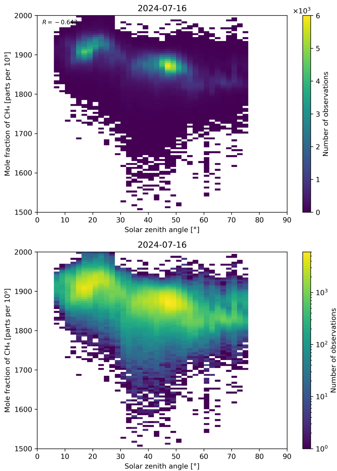
Figure 99: Scatter density plot of “Solar zenith angle” against “Mole fraction of CH 4 ” for 2024-07-15 to 2024-07-17.
