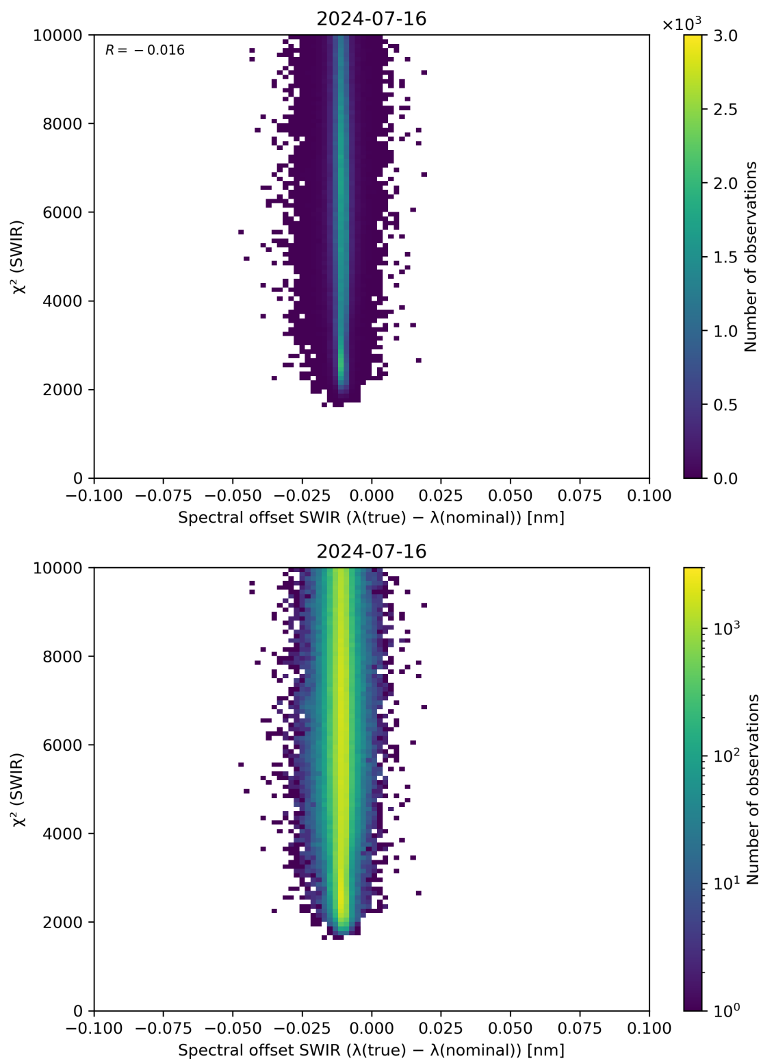
Figure 118: Scatter density plot of “Spectral offset SWIR ( \lambda(\text{true}) - \lambda(\text{nominal}) )” against “ \chi^2 (SWIR)” for 2024-07-15 to 2024-07-17.
