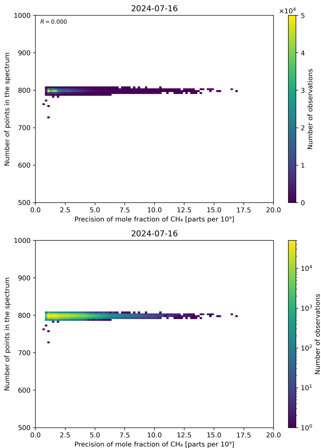
Figure 84: Scatter density plot of “Precision of mole fraction of \text{CH}_4 ” against “Number of points in the spectrum” for 2024-07-15 to 2024-07-17.
