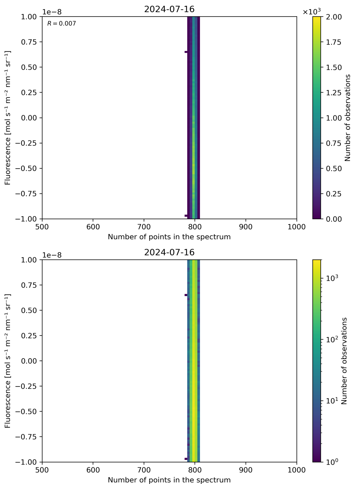
Figure 91: Scatter density plot of “Number of points in the spectrum” against “Fluorescence” for 2024-07-15 to 2024-07-17.
