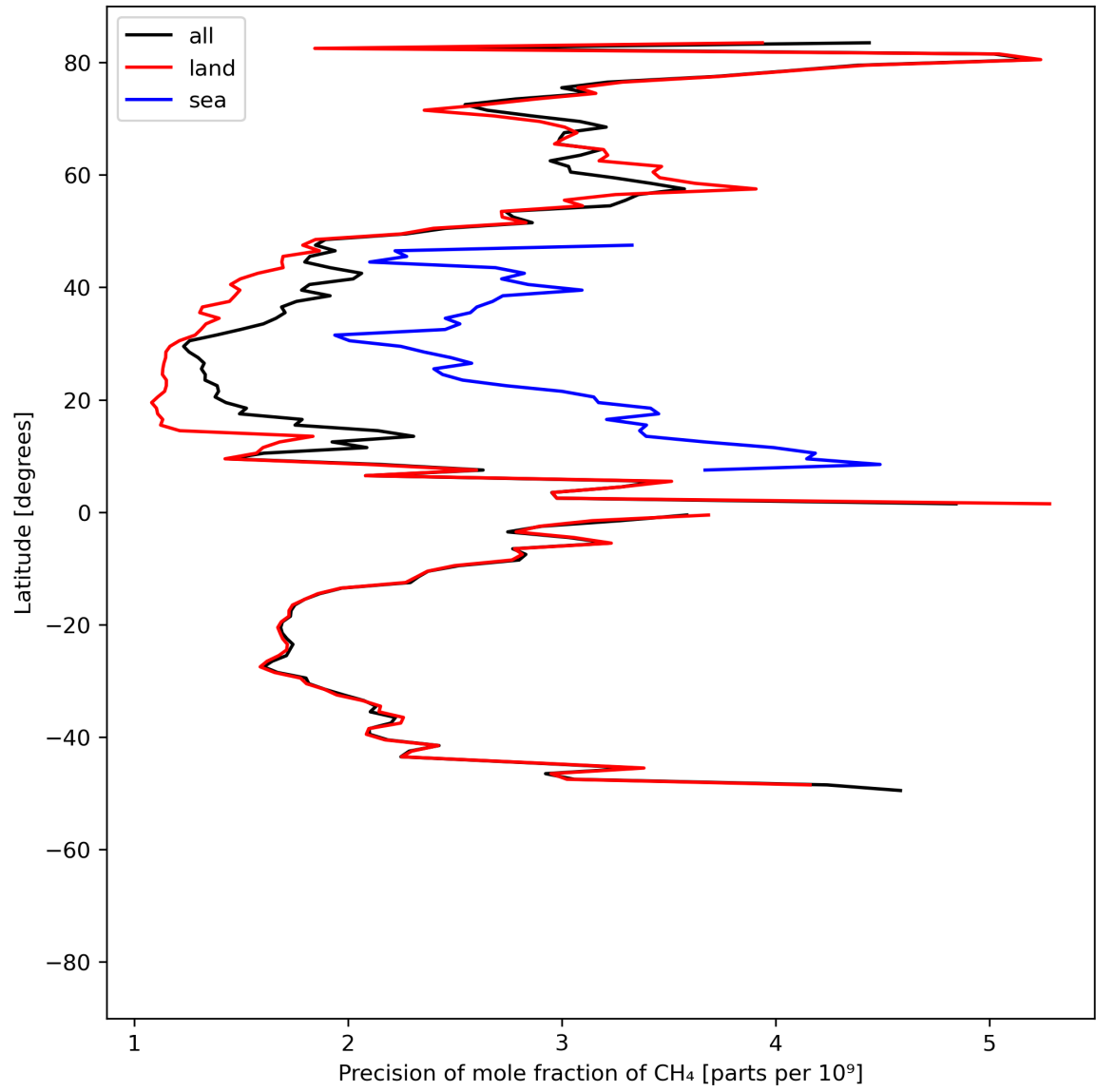
Figure 13: Zonal average of “Precision of mole fraction of CH 4 ” for 2024-07-15 to 2024-07-17.
