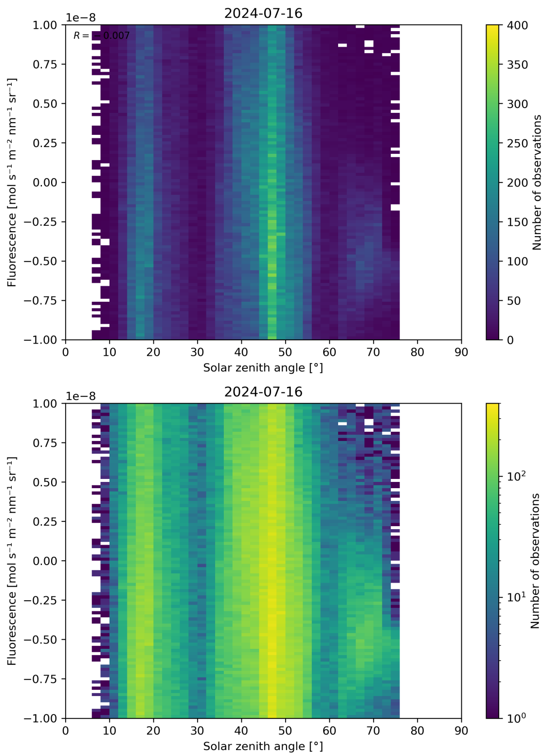
Figure 97: Scatter density plot of “Solar zenith angle” against “Fluorescence” for 2024-07-15 to 2024-07-17.
