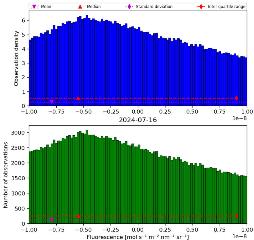
Figure 32: Histogram of “Fluorescence” for 2024-07-15 to 2024-07-17
