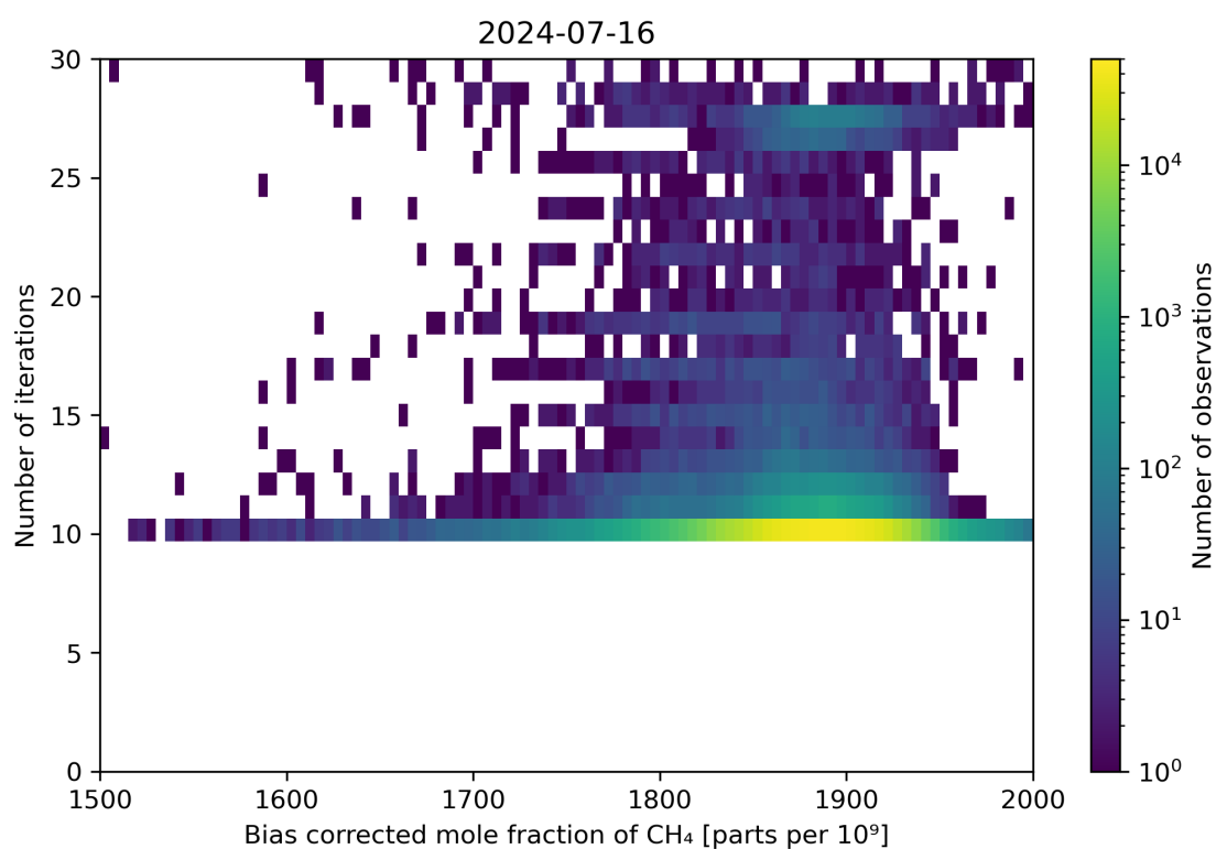
Figure 67: Scatter density plot of “Bias corrected mole fraction of CH 4 ” against “Number of iterations” for 2024-07-15 to 2024-07-17.
