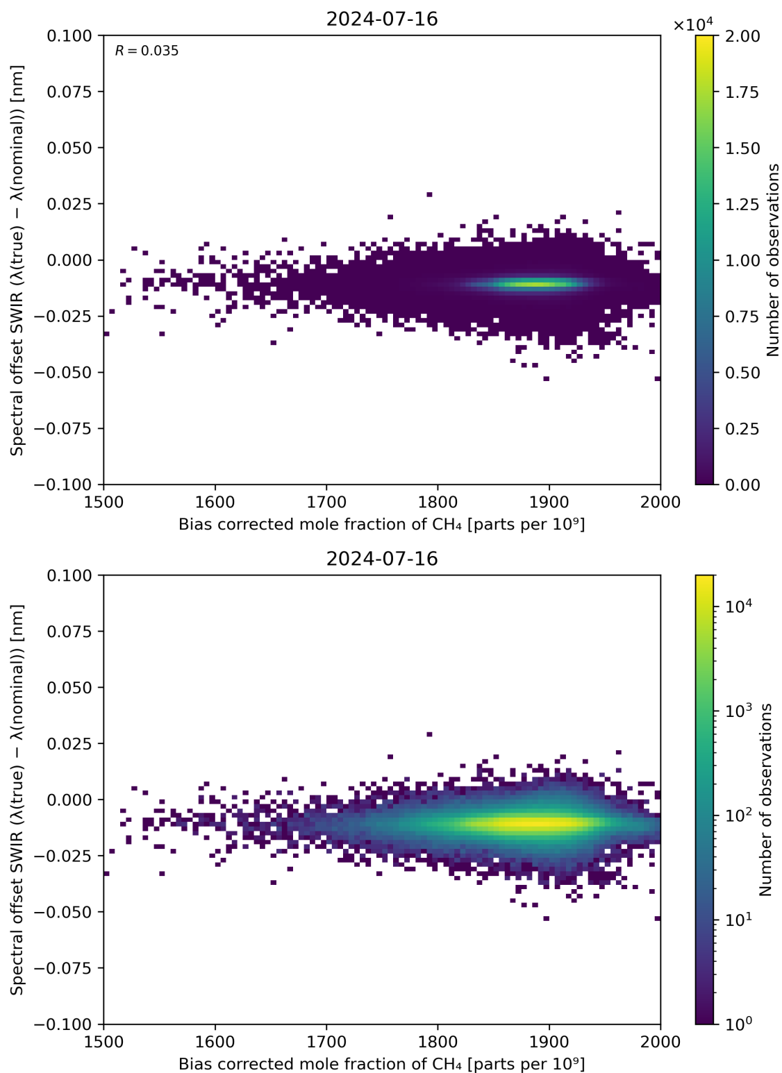
Figure 69: Scatter density plot of “Bias corrected mole fraction of \text{CH}_4 ” against “Spectral offset SWIR ( \lambda(\text{true}) - \lambda(\text{nominal}) )” for 2024-07-15 to 2024-07-17.
