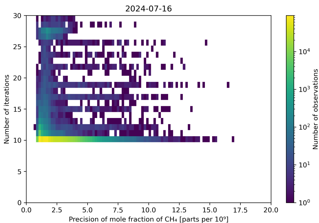
Figure 83: Scatter density plot of “Precision of mole fraction of CH 4 ” against “Number of iterations” for 2024-07-15 to 2024-07-17.
