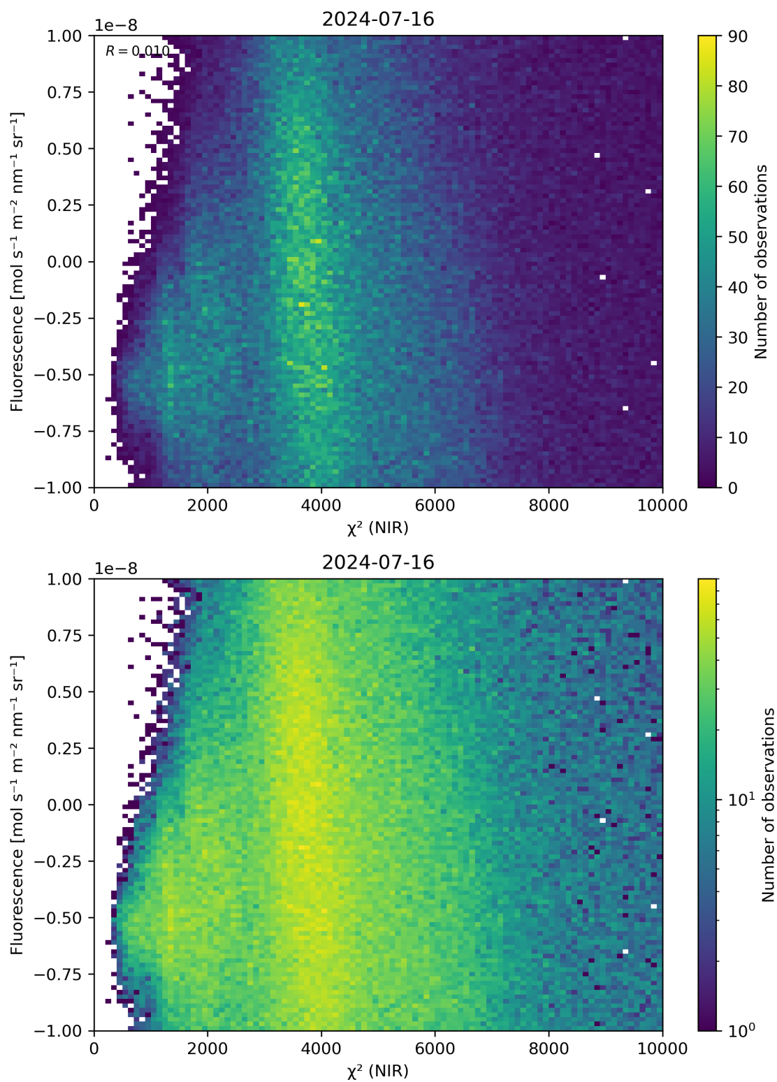
Figure 45: Scatter density plot of “ \chi^2 (NIR)” against “Fluorescence” for 2024-07-15 to 2024-07-17.
