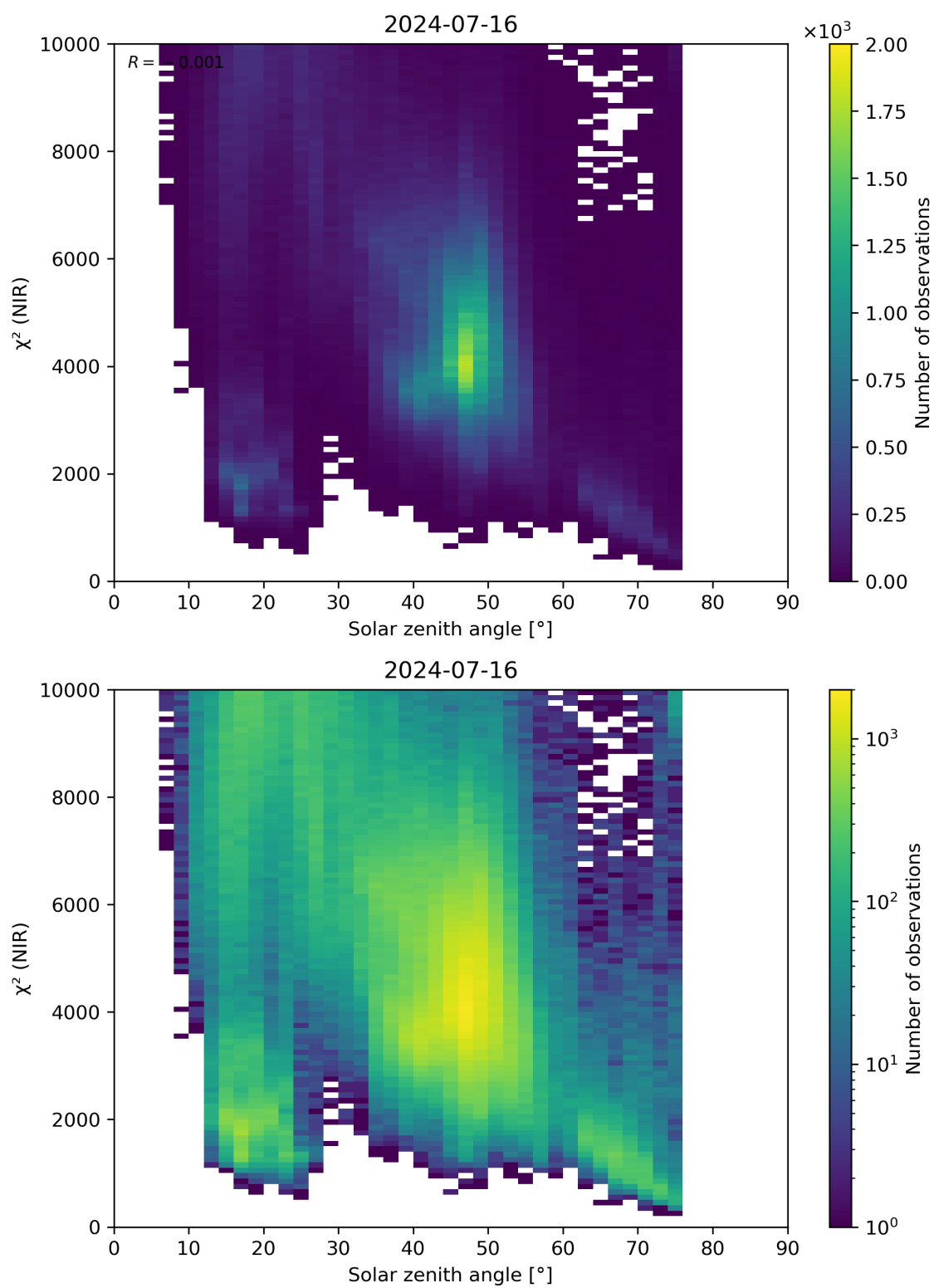
Figure 94: Scatter density plot of “Solar zenith angle” against “ \chi^2 (NIR)” for 2024-07-15 to 2024-07-17.
