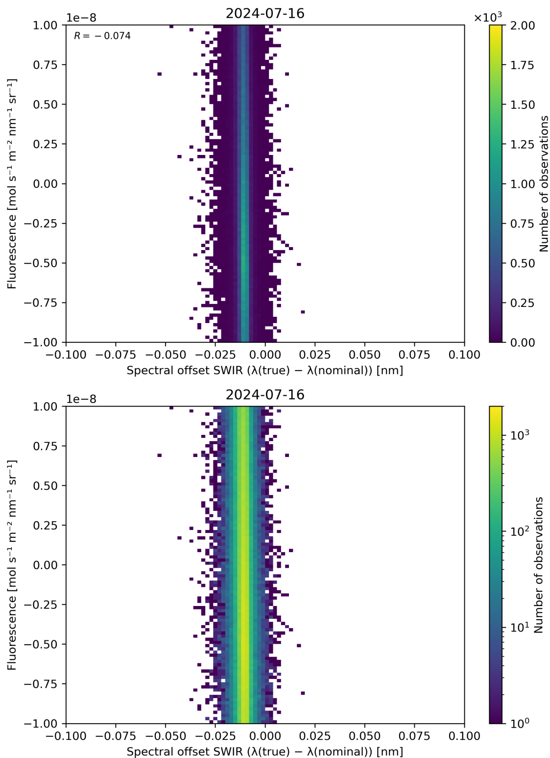
Figure 120: Scatter density plot of “Spectral offset SWIR ( \lambda(\text{true}) - \lambda(\text{nominal}) )” against “Fluorescence” for 2024-07-15 to 2024-07-17.
