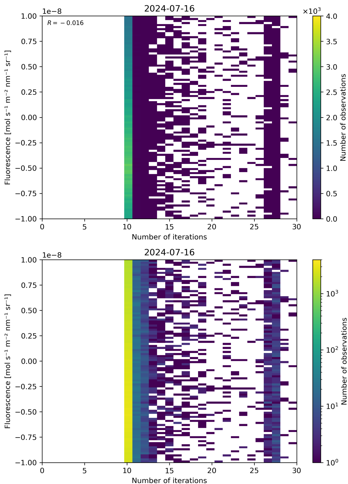
Figure 87: Scatter density plot of “Number of iterations” against “Fluorescence” for 2024-07-15 to 2024-07-17.
