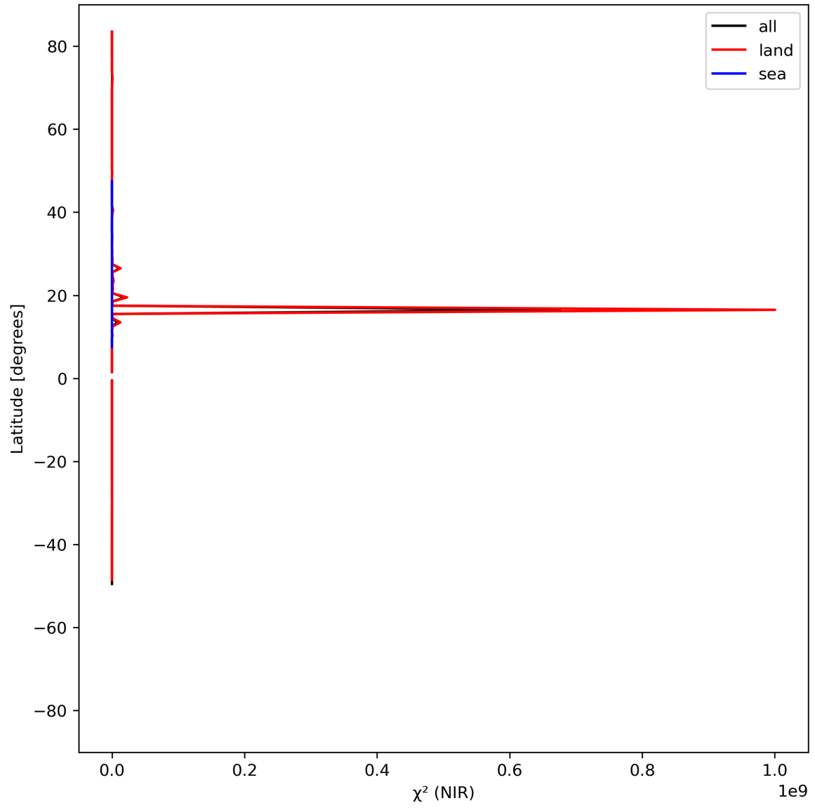
Figure 18: Zonal average of “ \chi^2 (NIR)” for 2024-07-15 to 2024-07-17.
