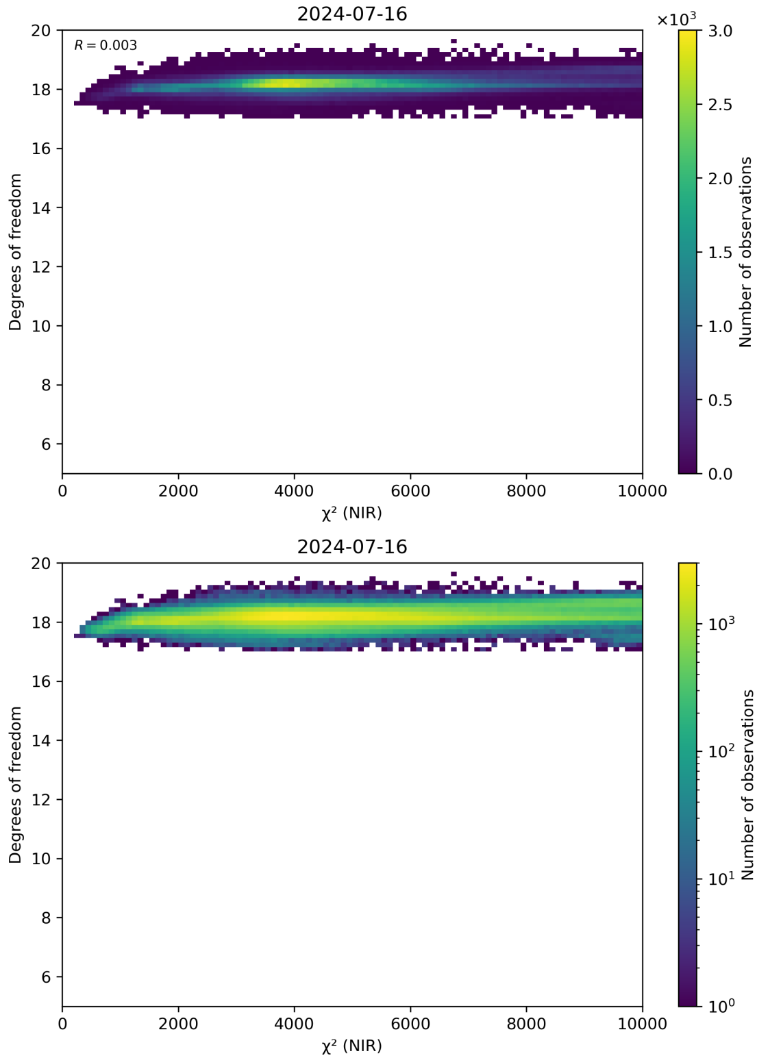
Figure 44: Scatter density plot of “ \chi^2 (NIR)” against “Degrees of freedom” for 2024-07-15 to 2024-07-17.
