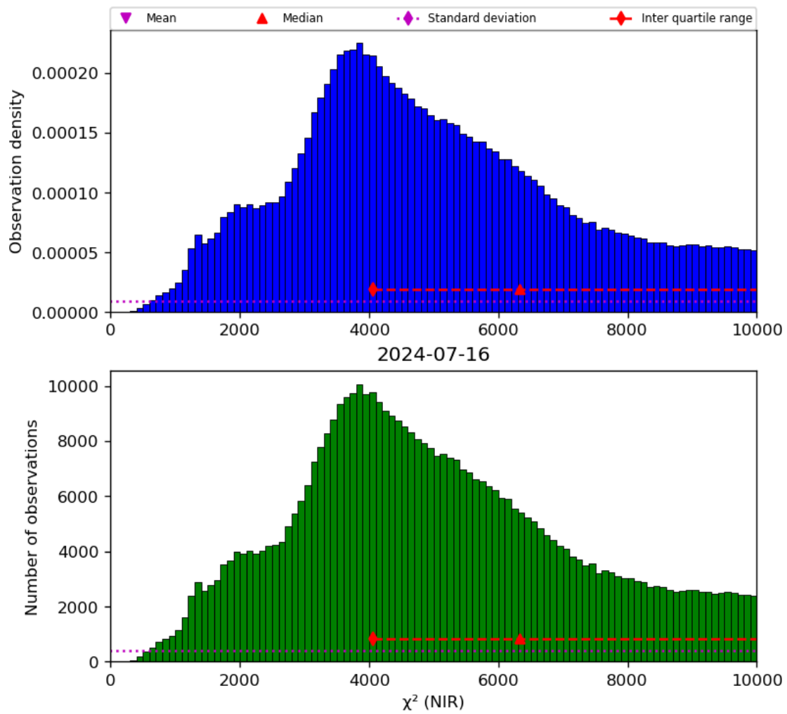
Figure 29: Histogram of “ \chi^2 (NIR)” for 2024-07-15 to 2024-07-17
