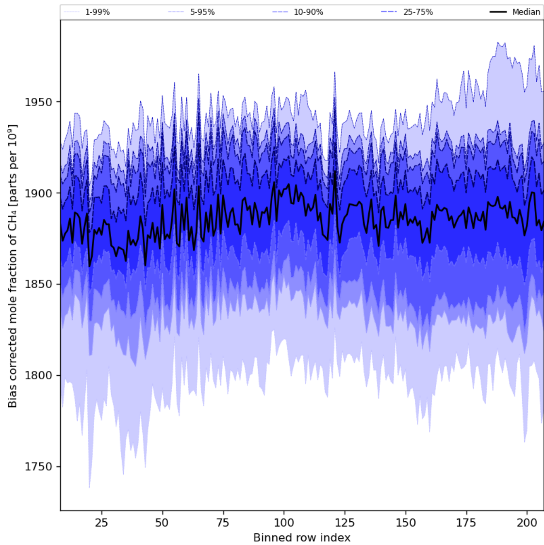
Figure 36: Along track statistics of “Bias corrected mole fraction of CH 4 ” for 2024-07-15 to 2024-07-17
