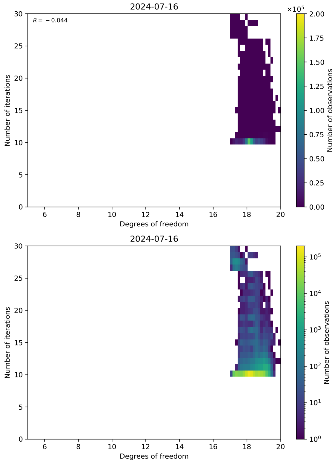
Figure 52: Scatter density plot of “Degrees of freedom” against “Number of iterations” for 2024-07-15 to 2024-07-17.
