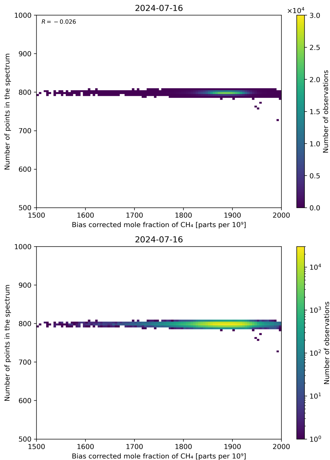
Figure 68: Scatter density plot of “Bias corrected mole fraction of CH 4 ” against “Number of points in the spectrum” for 2024-07-15 to 2024-07-17.
