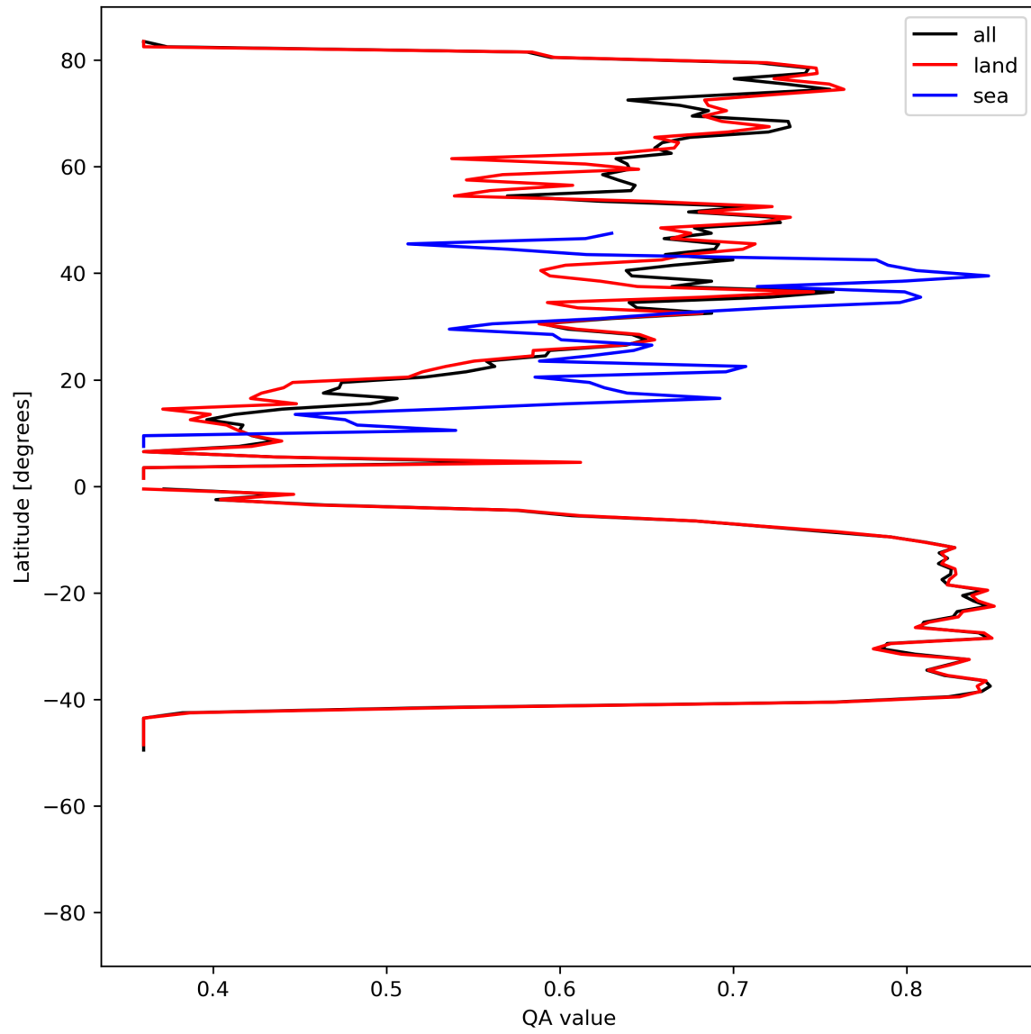
Figure 11: Zonal average of “QA value” for 2024-07-15 to 2024-07-17.
