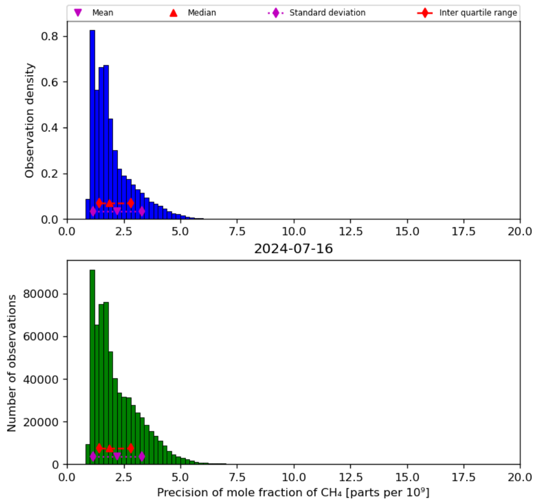
Figure 24: Histogram of “Precision of mole fraction of CH 4 ” for 2024-07-15 to 2024-07-17
