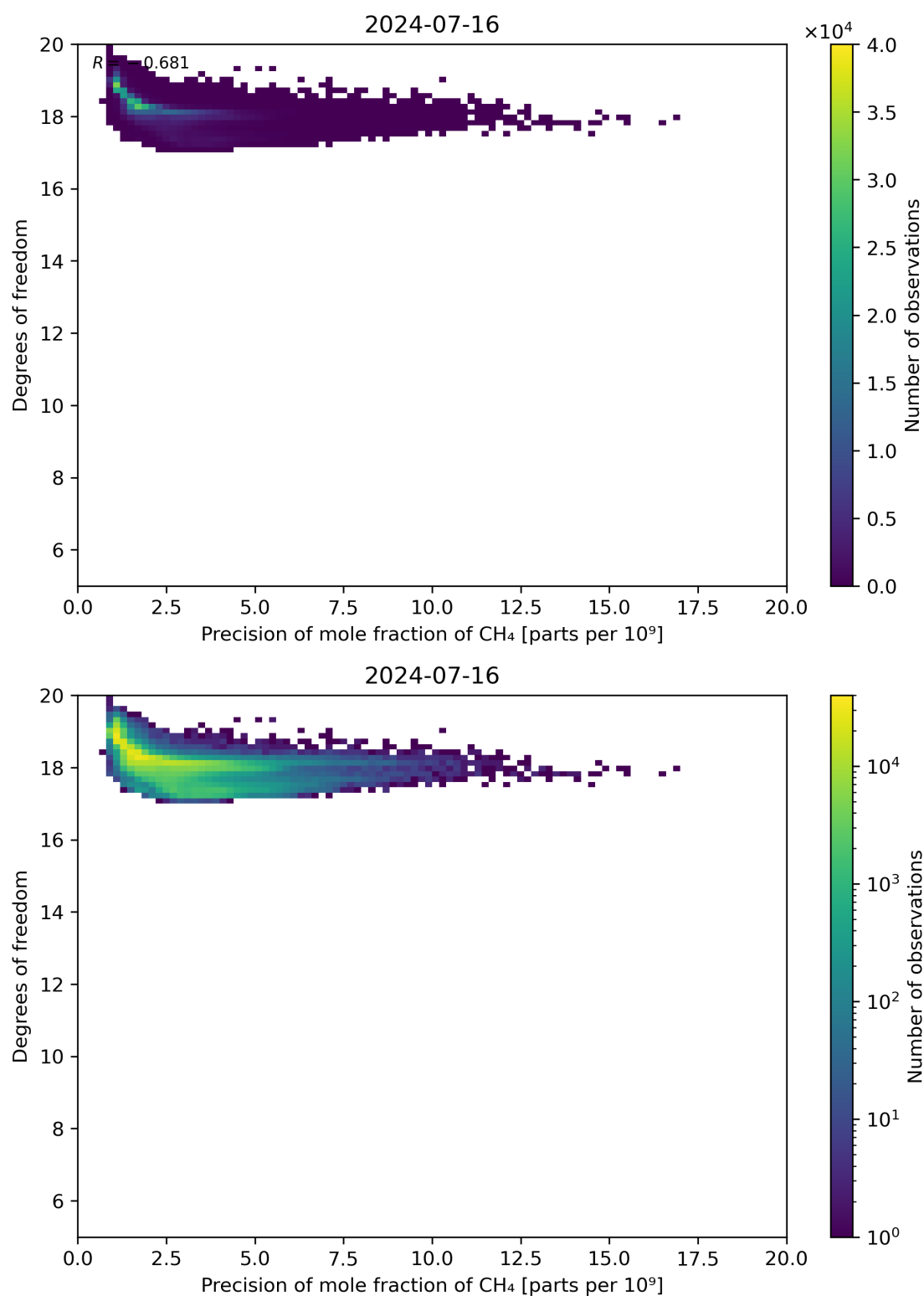
Figure 80: Scatter density plot of “Precision of mole fraction of CH 4 ” against “Degrees of freedom” for 2024-07-15 to 2024-07-17.
