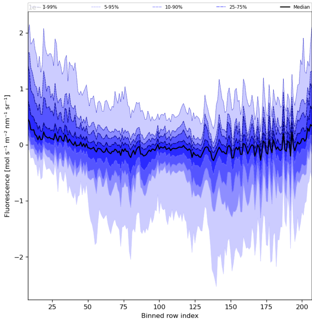
Figure 43: Along track statistics of “Fluorescence” for 2024-07-15 to 2024-07-17
