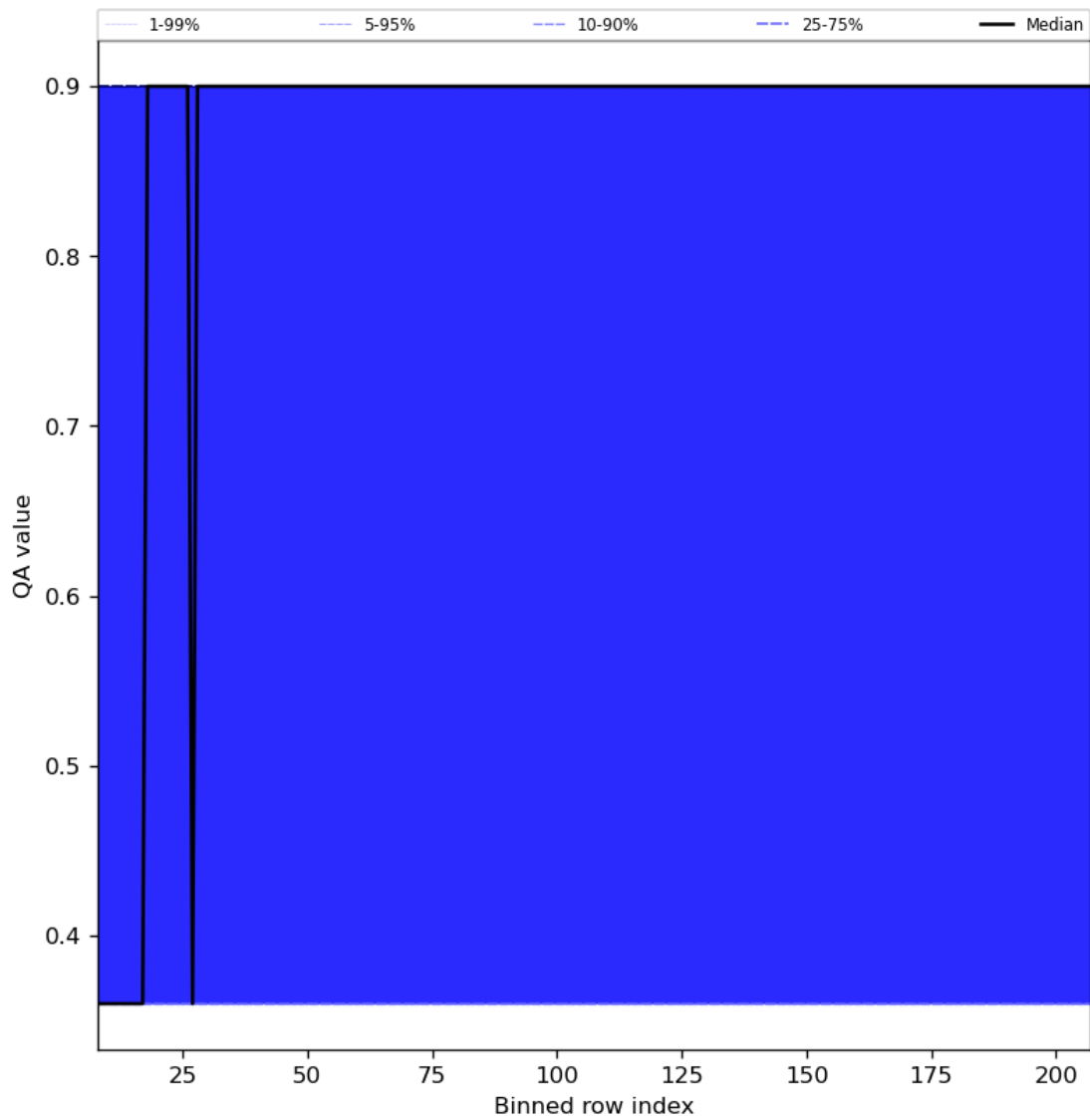
Figure 33: Along track statistics of “QA value” for 2024-07-15 to 2024-07-17
