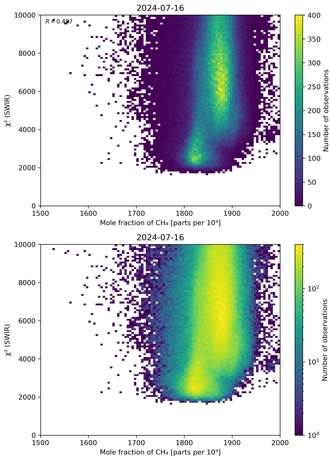
Figure 71: Scatter density plot of “Mole fraction of \text{CH}_4 ” against “ \chi^2 (SWIR)” for 2024-07-15 to 2024-07-17.
