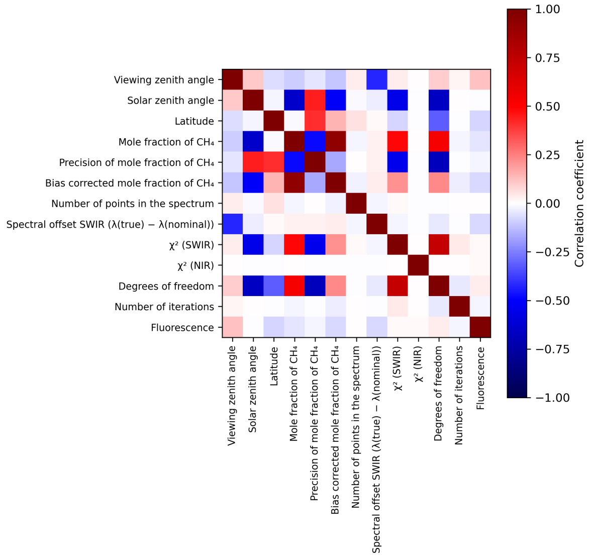
Figure 2: Map of correlation matrix for 2024-07-15 to 2024-07-17.
