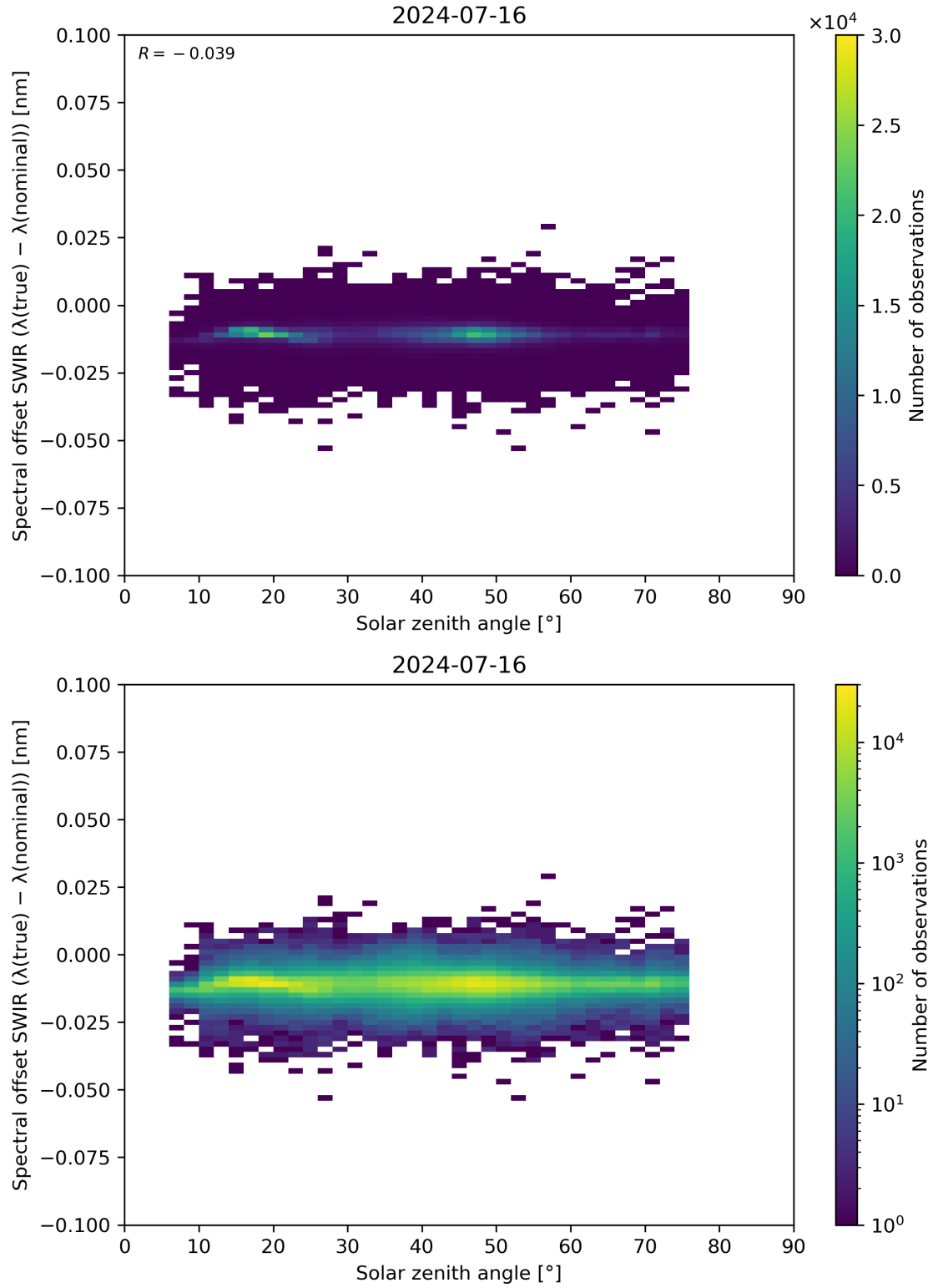
Figure 104: Scatter density plot of “Solar zenith angle” against “Spectral offset SWIR ( \lambda(\text{true}) - \lambda(\text{nominal}) )” for 2024-07-15 to 2024-07-17.
