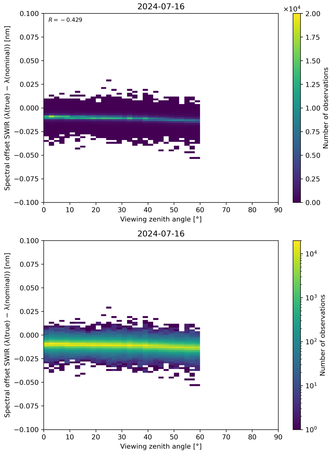
Figure 116: Scatter density plot of “Viewing zenith angle” against “Spectral offset SWIR ( \lambda(\text{true}) - \lambda(\text{nominal}) )” for 2024-07-15 to 2024-07-17.
