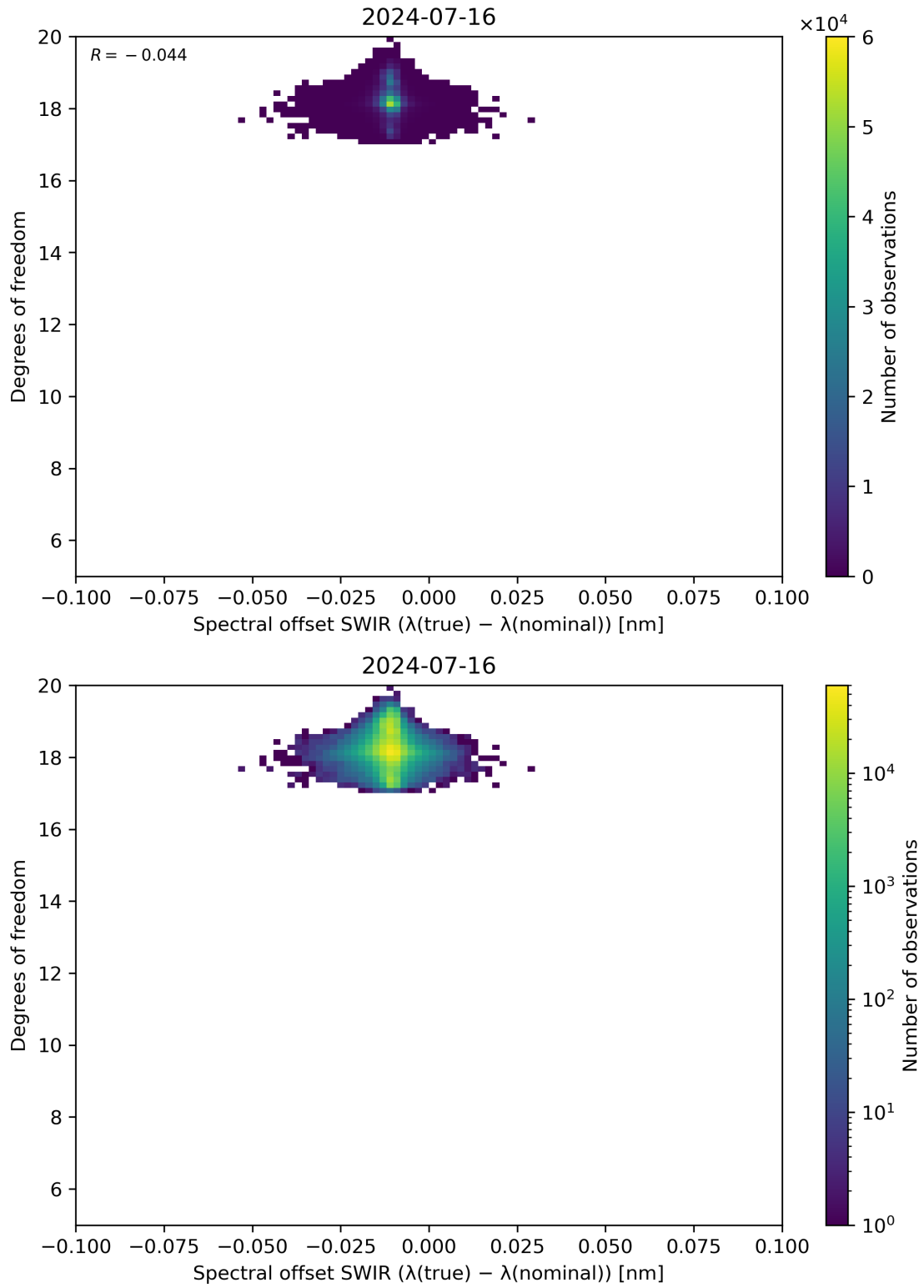
Figure 119: Scatter density plot of “Spectral offset SWIR ( \lambda(\text{true}) - \lambda(\text{nominal}) )” against “Degrees of freedom” for 2024-07-15 to 2024-07-17.
