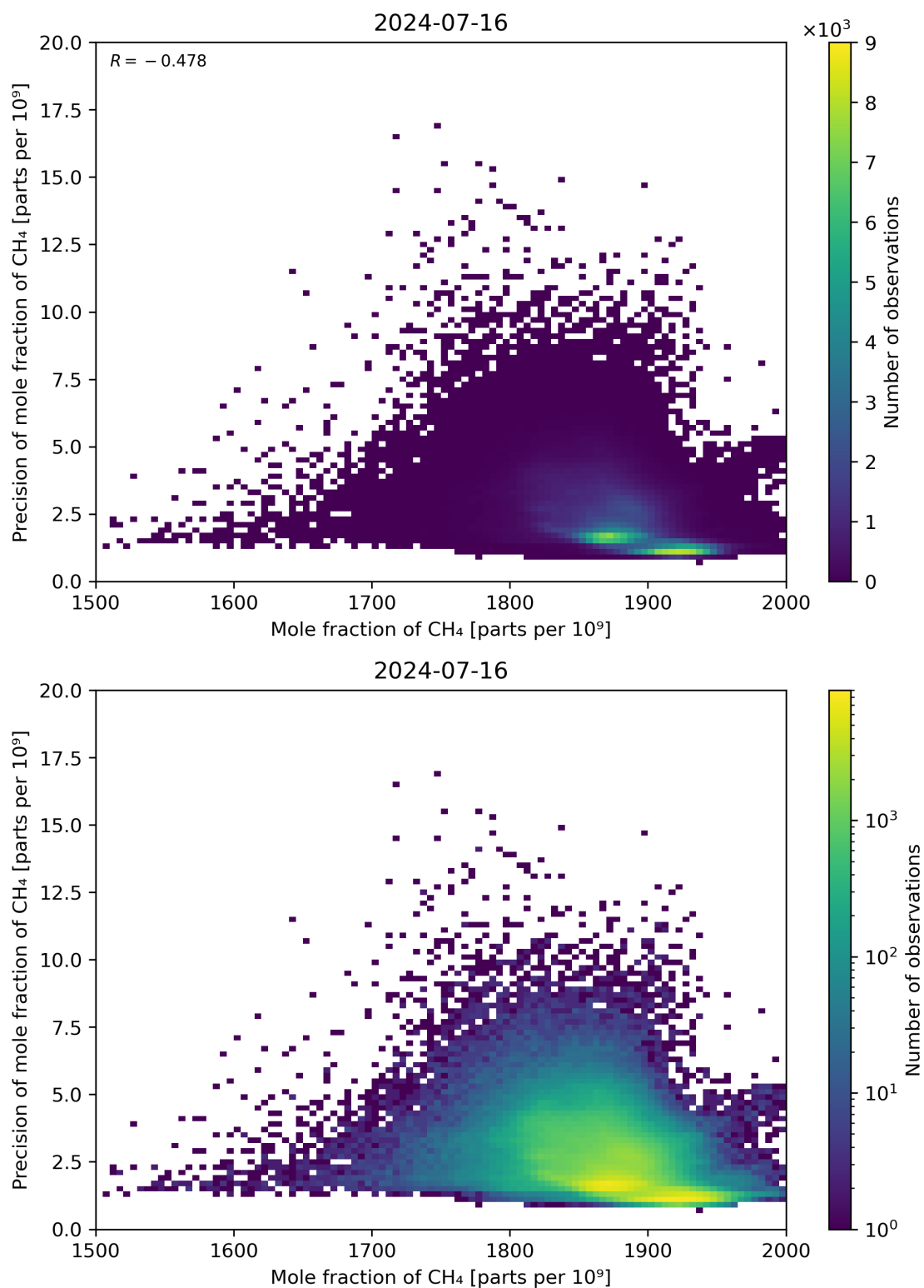
Figure 75: Scatter density plot of “Mole fraction of CH 4 ” against “Precision of mole fraction of CH 4 ” for 2024-07-15 to 2024-07-17.
