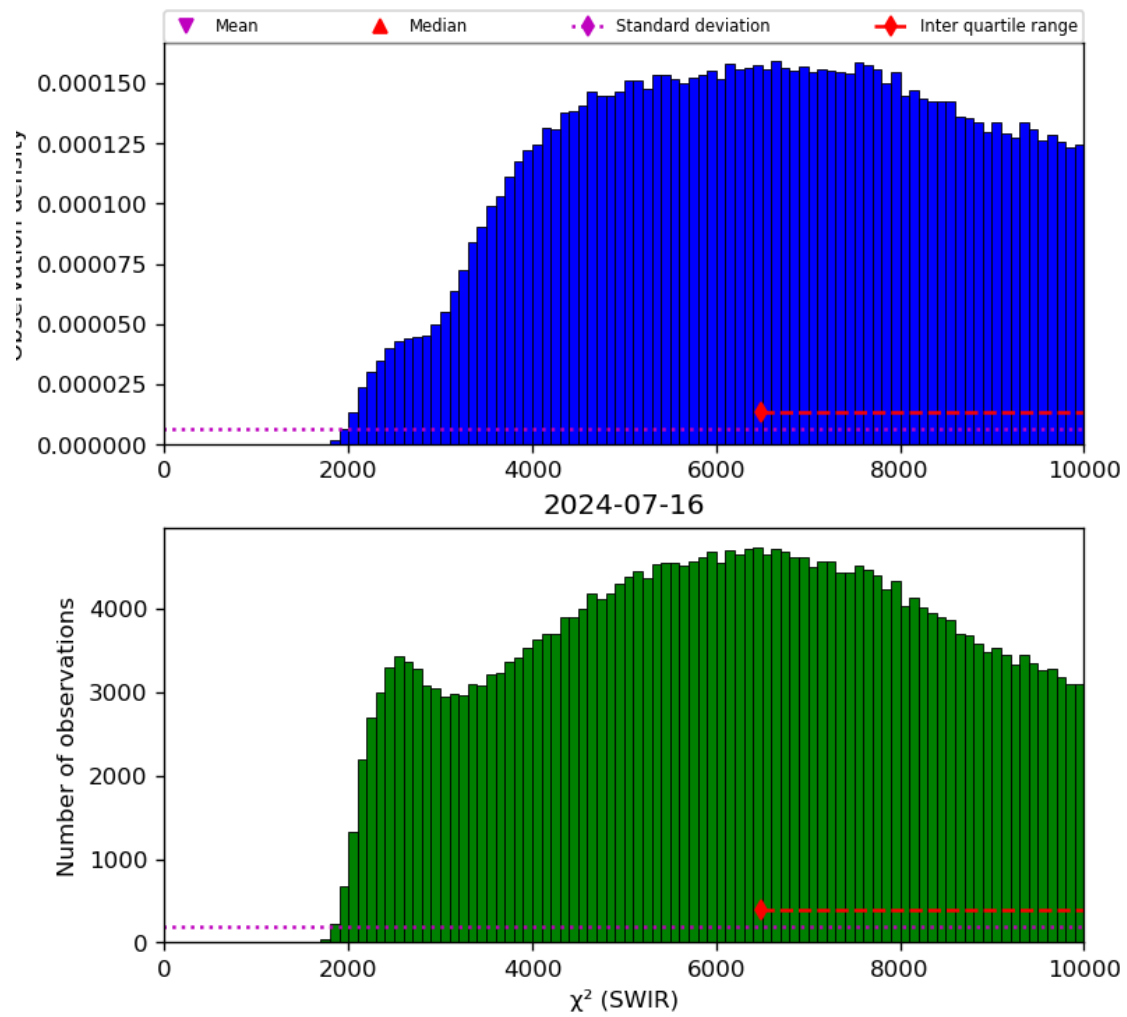
Figure 28: Histogram of “ \chi^2 (SWIR)” for 2024-07-15 to 2024-07-17
