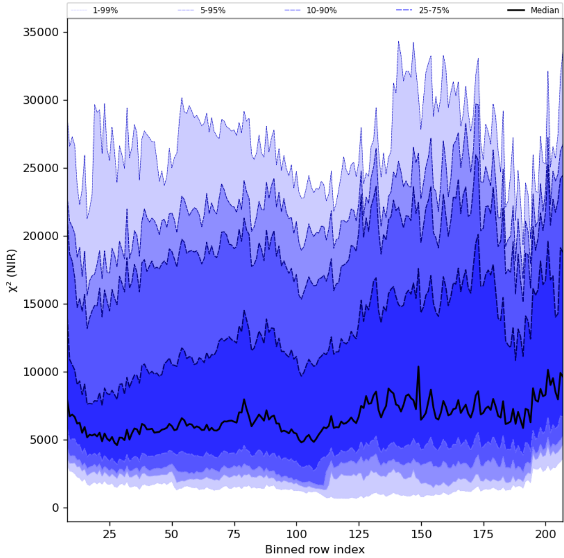
Figure 40: Along track statistics of “ \chi^2 (NIR)” for 2024-07-15 to 2024-07-17
