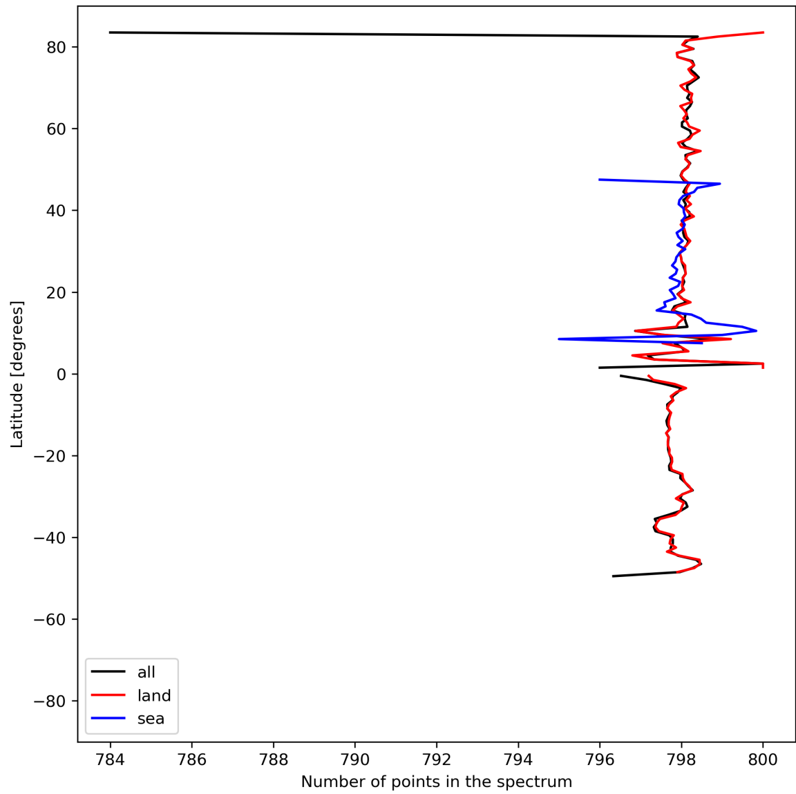
Figure 15: Zonal average of “Number of points in the spectrum” for 2024-07-15 to 2024-07-17.
