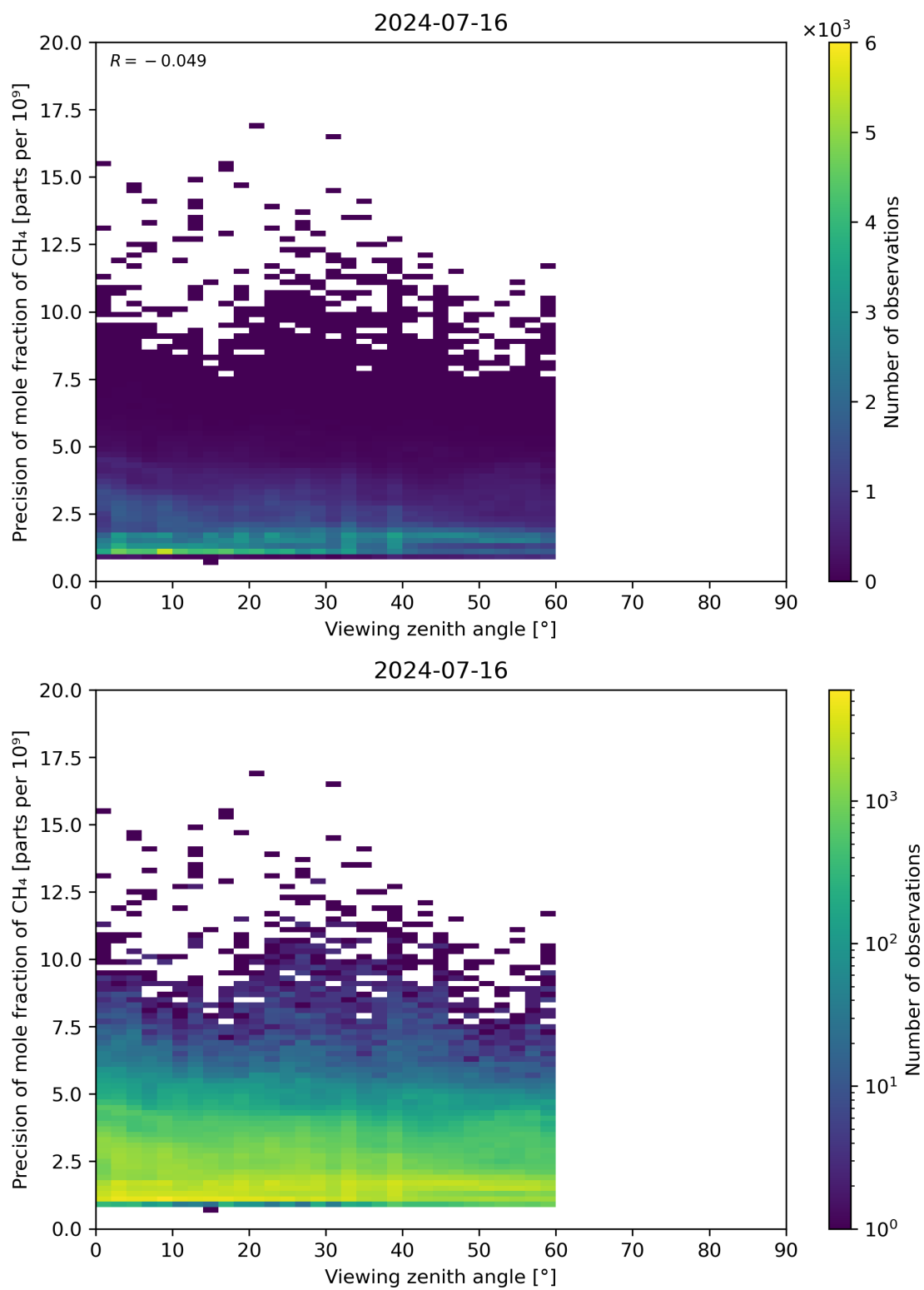
Figure 112: Scatter density plot of “Viewing zenith angle” against “Precision of mole fraction of CH 4 ” for 2024-07-15 to 2024-07-17.
