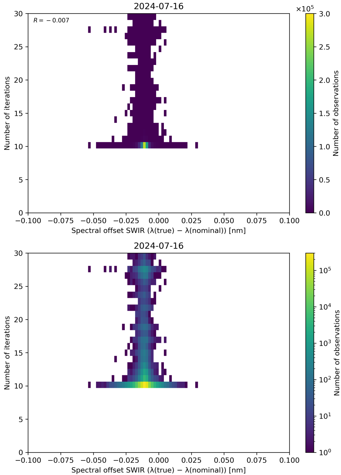
Figure 121: Scatter density plot of “Spectral offset SWIR ( \lambda(\text{true}) - \lambda(\text{nominal}) )” against “Number of iterations” for 2024-07-15 to 2024-07-17.
