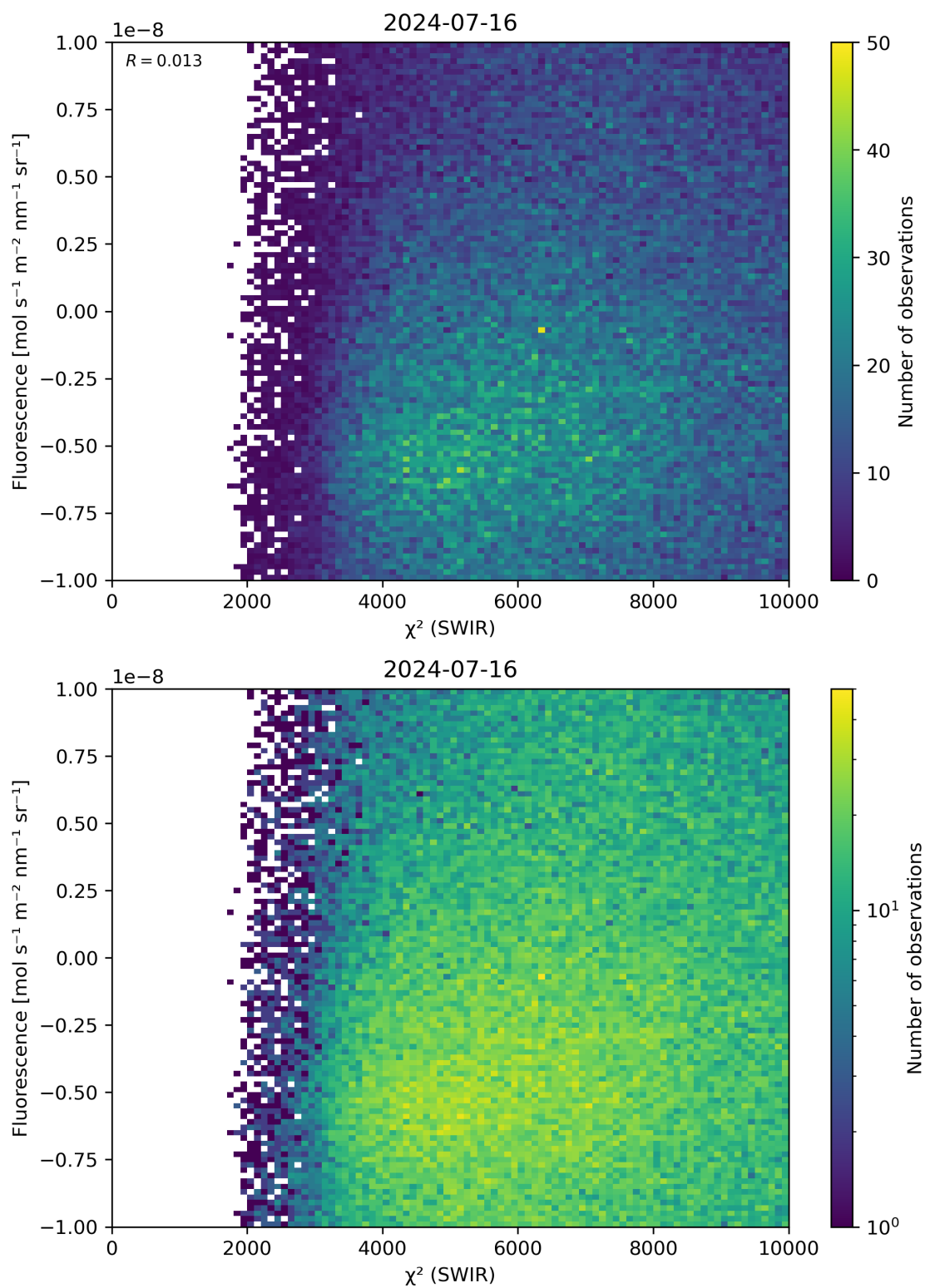
Figure 49: Scatter density plot of “ \chi^2 (SWIR)” against “Fluorescence” for 2024-07-15 to 2024-07-17.
