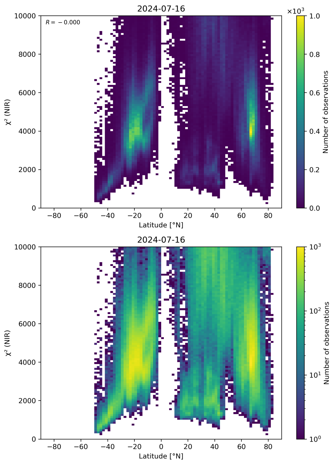
Figure 53: Scatter density plot of “Latitude” against “ \chi^2 (NIR)” for 2024-07-15 to 2024-07-17.
