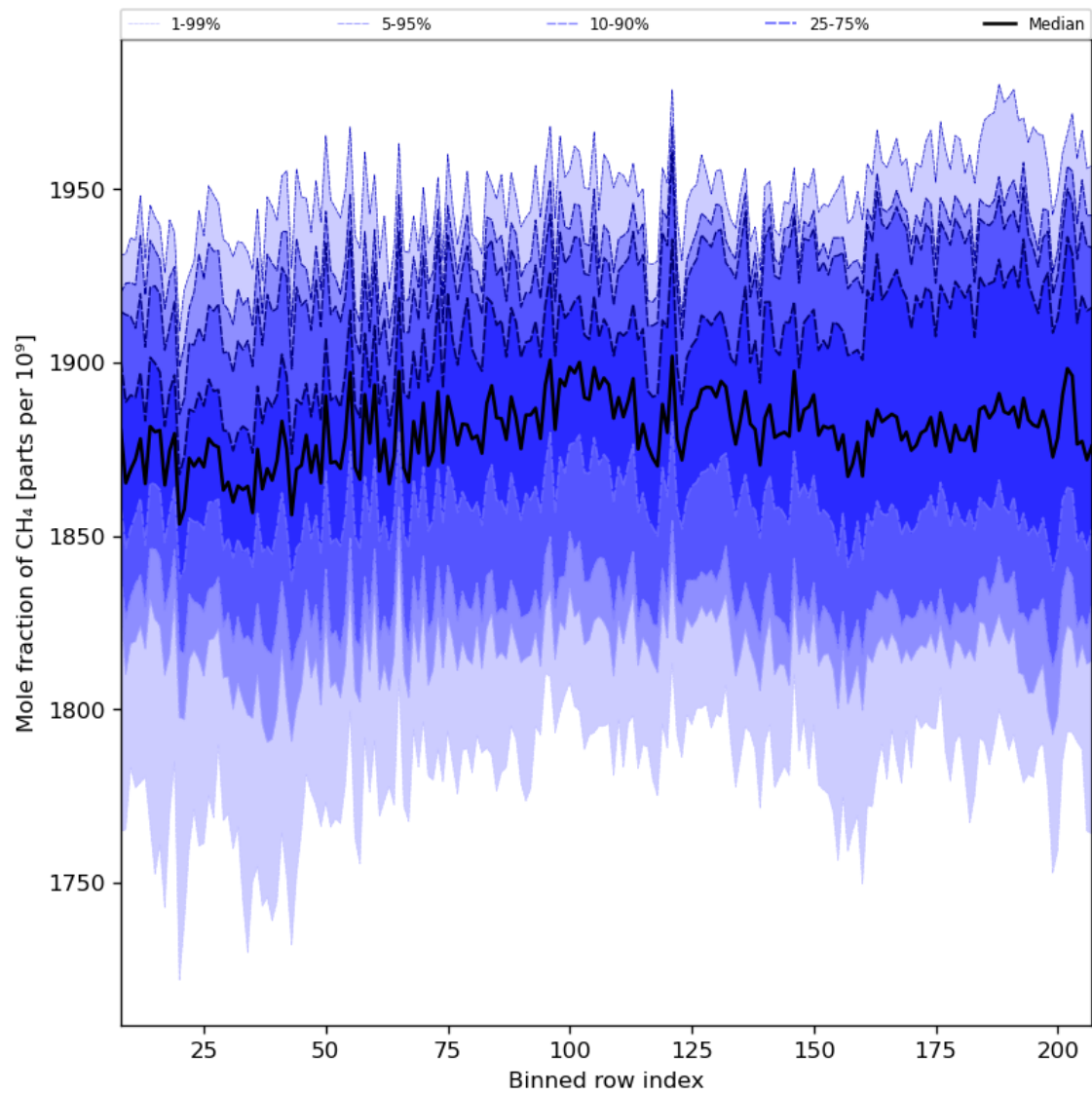
Figure 34: Along track statistics of “Mole fraction of CH 4 ” for 2024-07-15 to 2024-07-17
