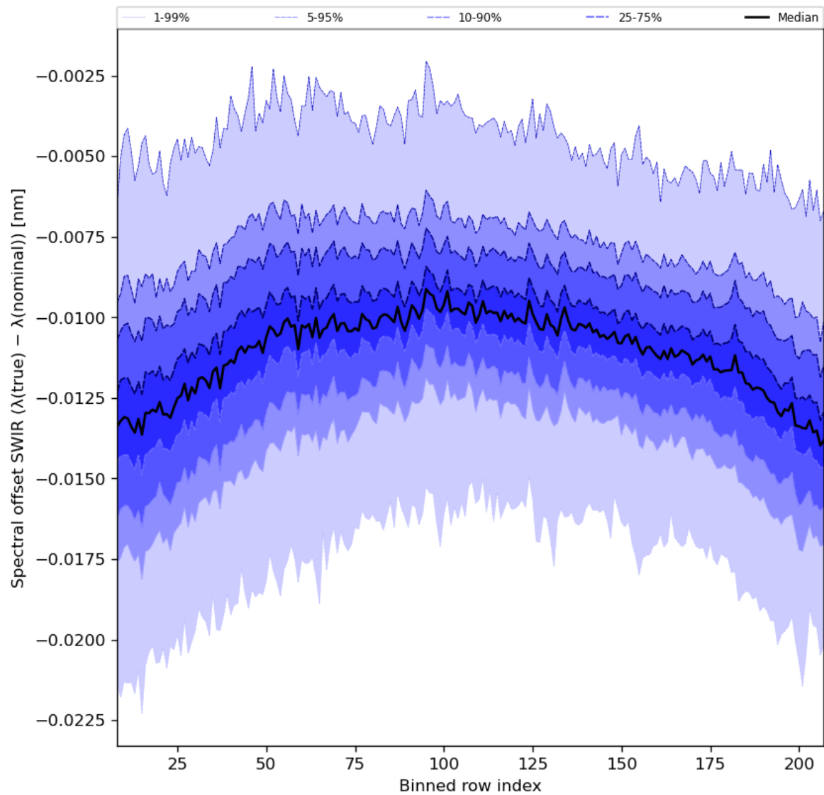
Figure 38: Along track statistics of “Spectral offset SWIR ( \lambda(\text{true}) - \lambda(\text{nominal}) )” for 2024-07-15 to 2024-07-17
