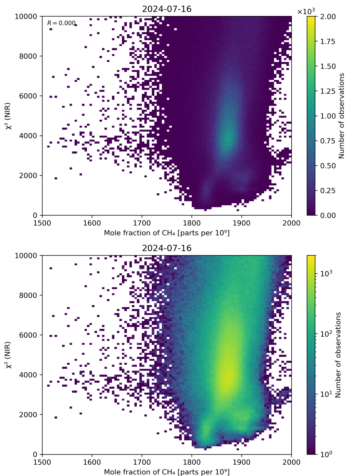
Figure 70: Scatter density plot of “Mole fraction of \text{CH}_4 ” against “ \chi^2 (NIR)” for 2024-07-15 to 2024-07-17.
