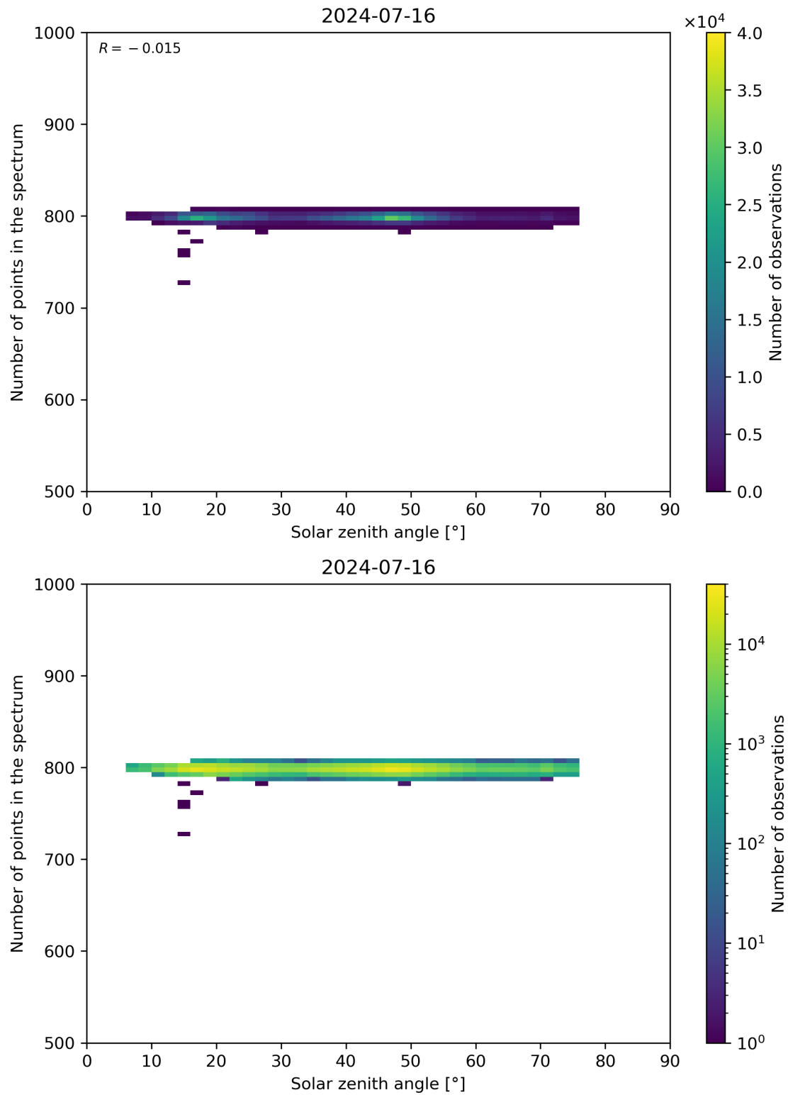
Figure 103: Scatter density plot of “Solar zenith angle” against “Number of points in the spectrum” for 2024-07-15 to 2024-07-17.
