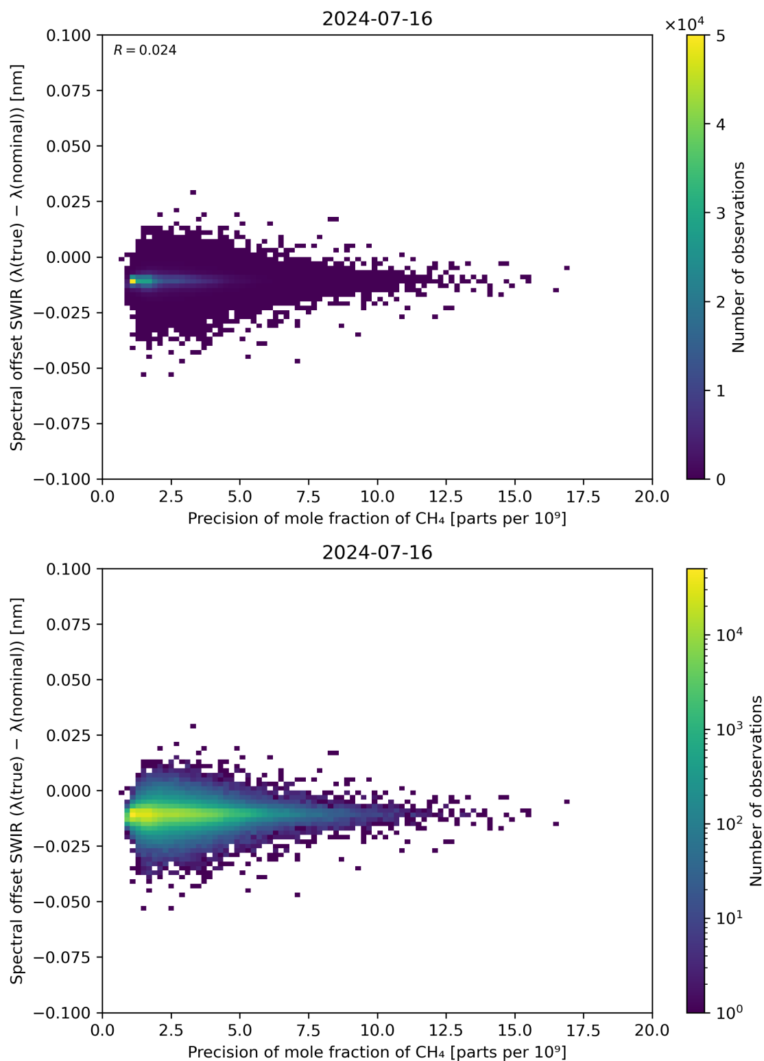
Figure 85: Scatter density plot of “Precision of mole fraction of CH 4 ” against “Spectral offset SWIR ( \lambda(\text{true}) - \lambda(\text{nominal}) )” for 2024-07-15 to 2024-07-17.
