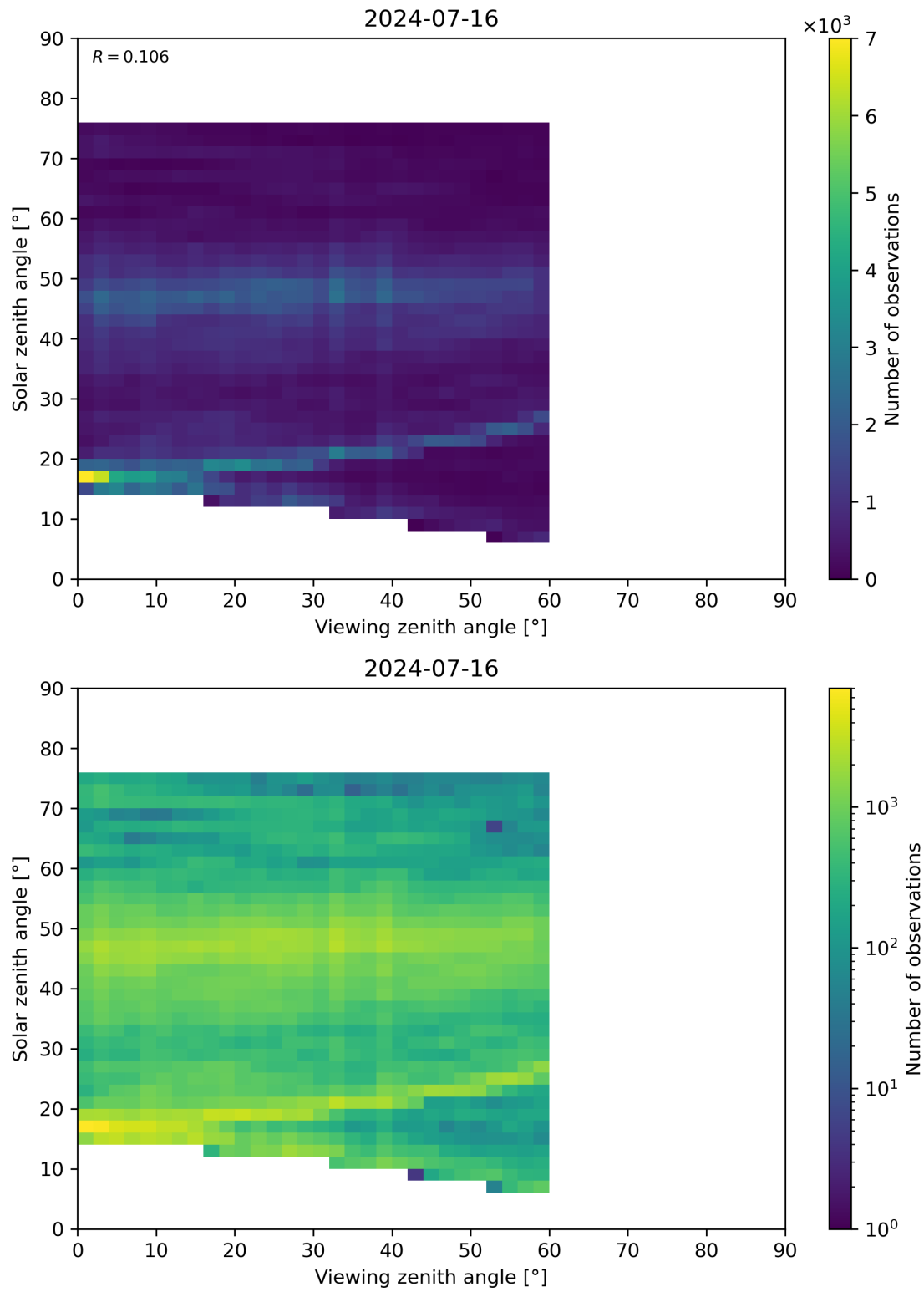
Figure 115: Scatter density plot of “Viewing zenith angle” against “Solar zenith angle” for 2024-07-15 to 2024-07-17.
