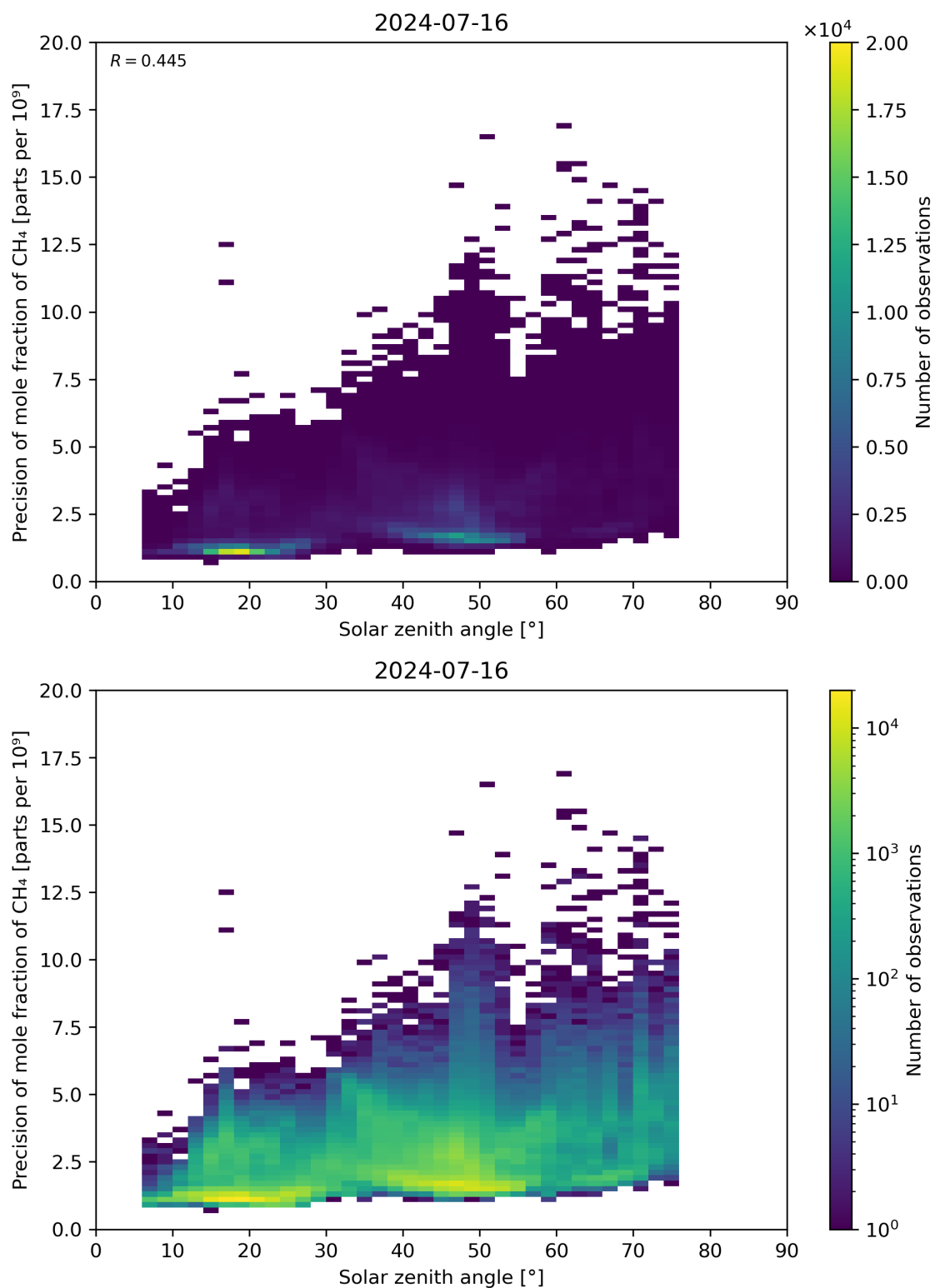
Figure 101: Scatter density plot of “Solar zenith angle” against “Precision of mole fraction of \text{CH}_4 ” for 2024-07-15 to 2024-07-17.
