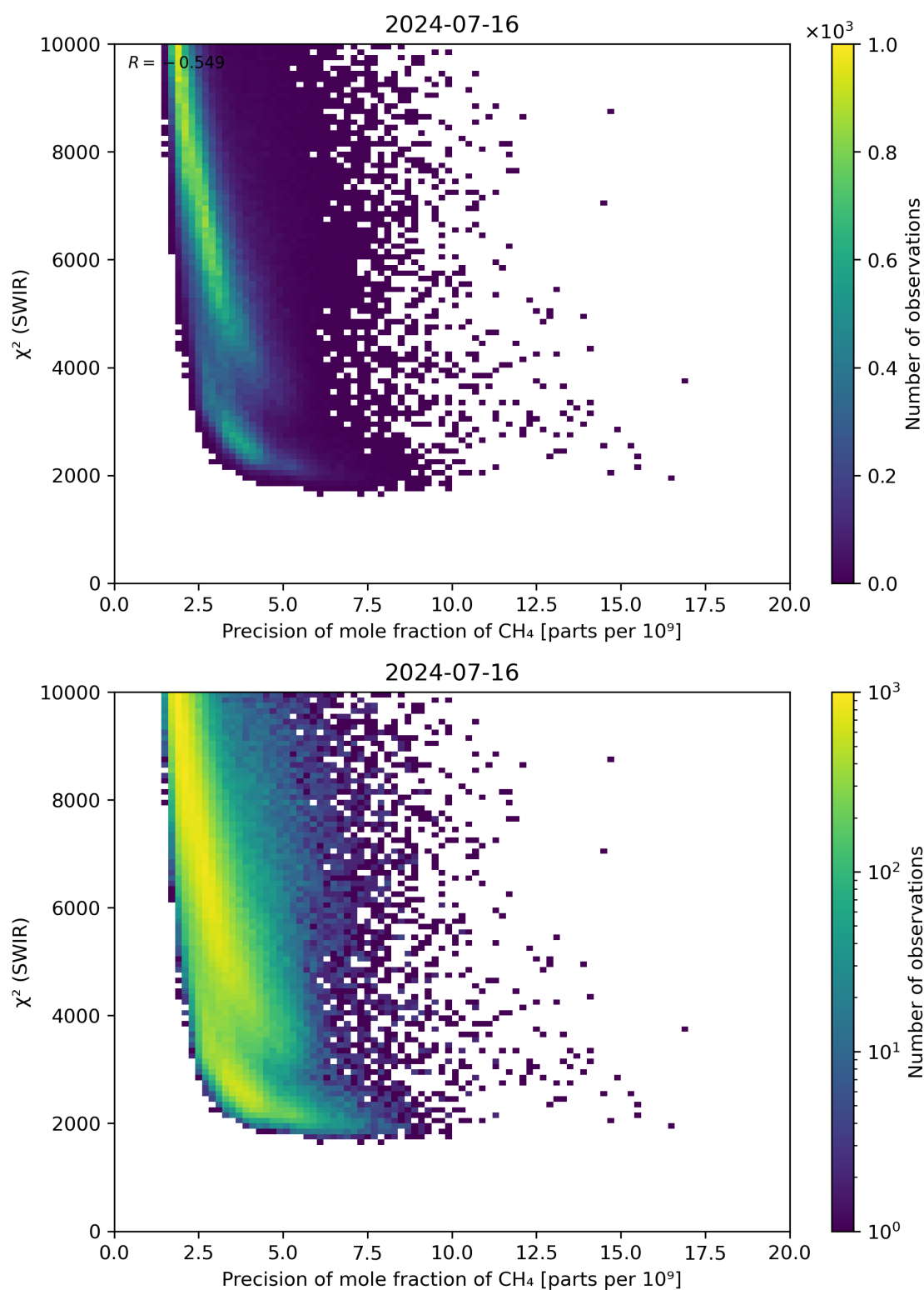
Figure 79: Scatter density plot of “Precision of mole fraction of \text{CH}_4 ” against “ \chi^2 (SWIR)” for 2024-07-15 to 2024-07-17.
