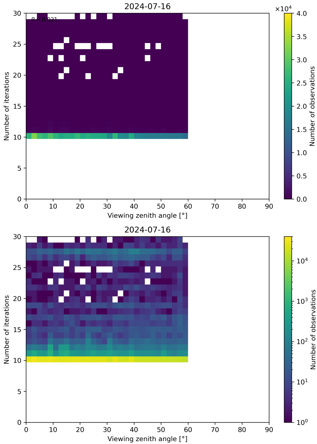
Figure 113: Scatter density plot of “Viewing zenith angle” against “Number of iterations” for 2024-07-15 to 2024-07-17.
