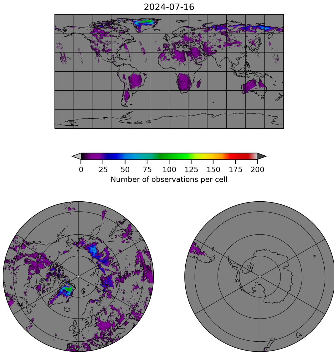
Figure 10: Map of the number of observations for 2024-07-15 to 2024-07-17
