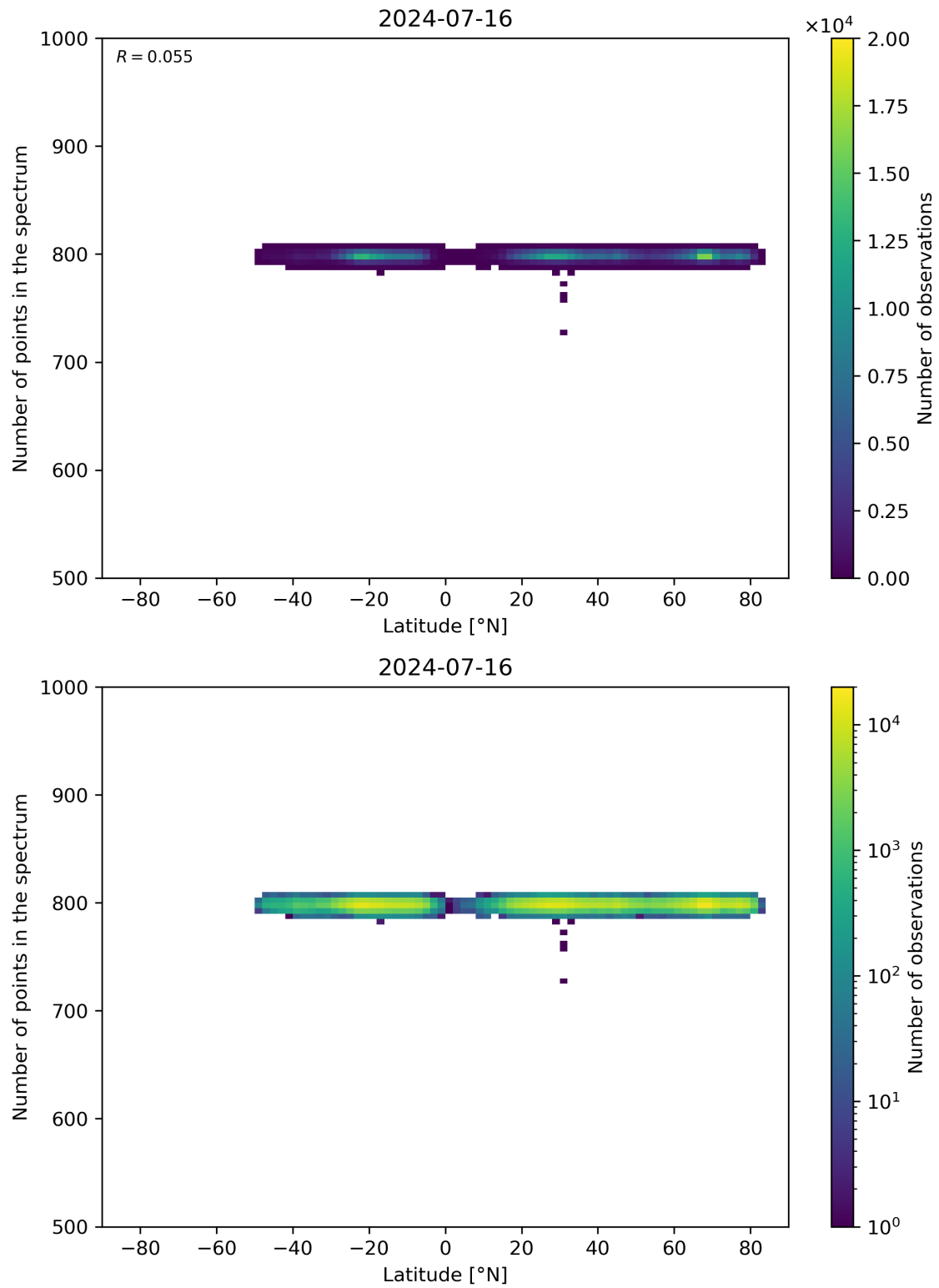
Figure 61: Scatter density plot of “Latitude” against “Number of points in the spectrum” for 2024-07-15 to 2024-07-17.
