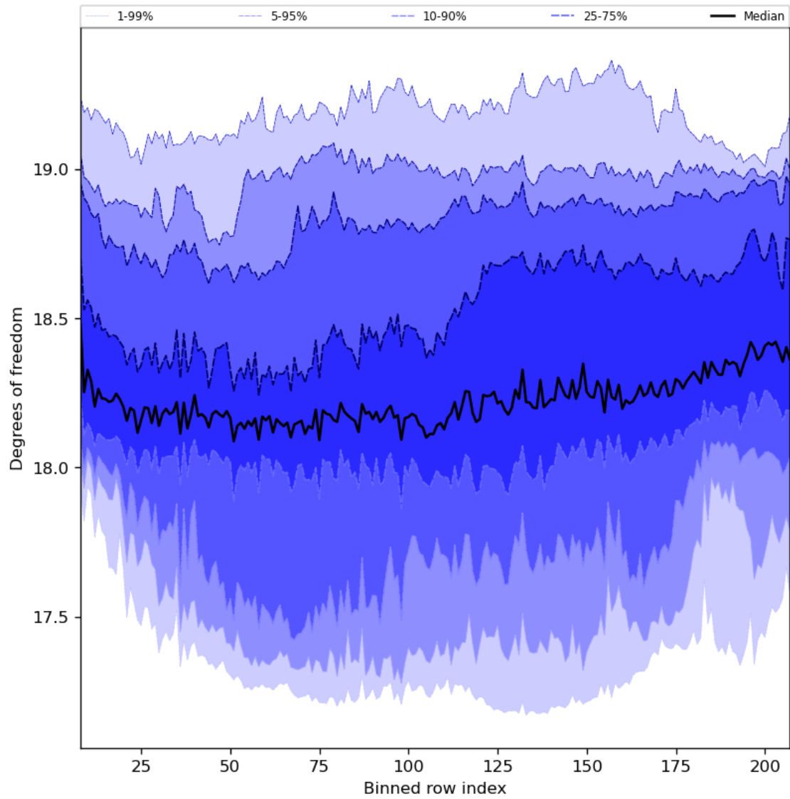
Figure 41: Along track statistics of “Degrees of freedom” for 2024-07-15 to 2024-07-17
