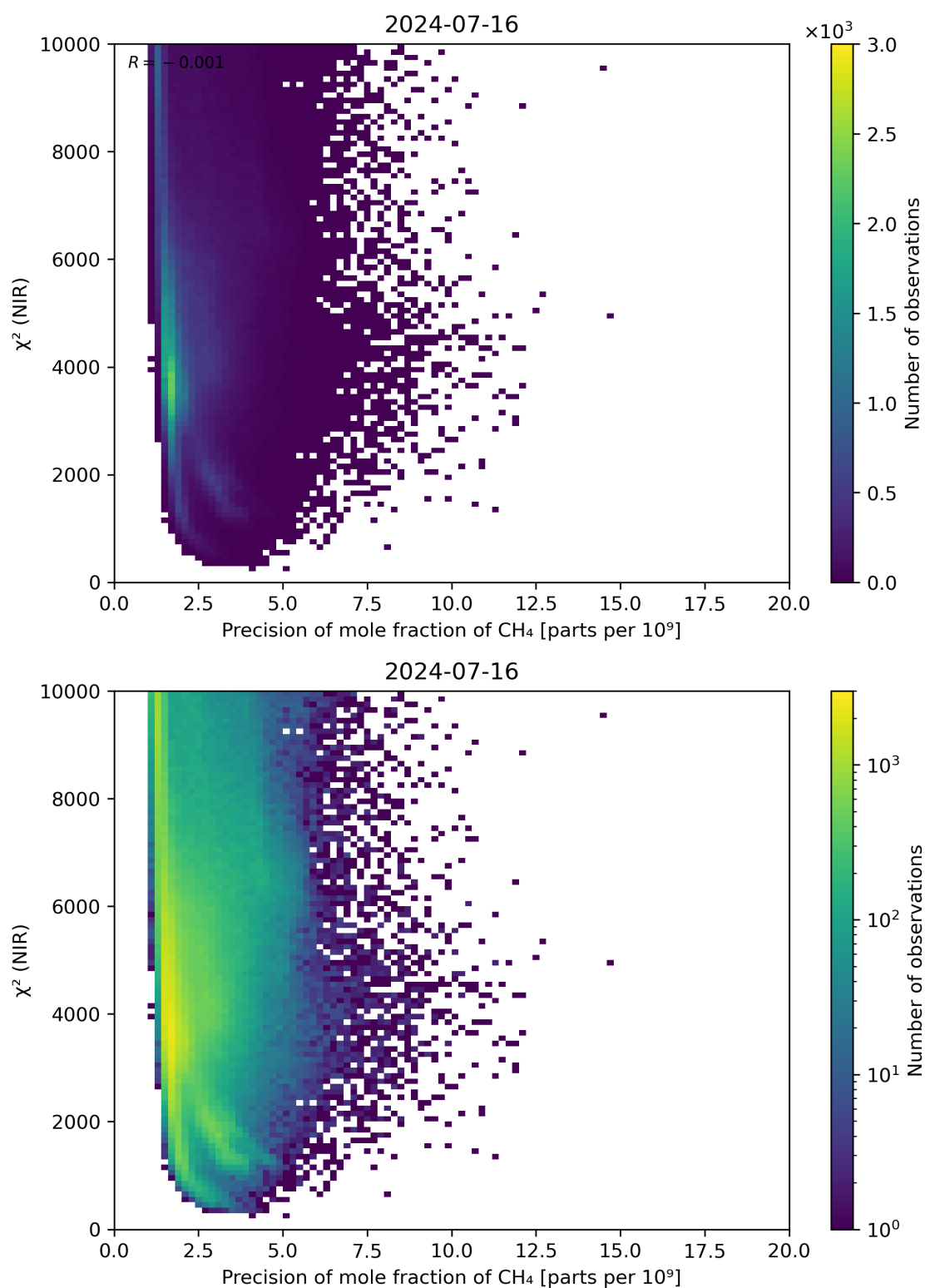
Figure 78: Scatter density plot of “Precision of mole fraction of CH 4 ” against “ \chi^2 (NIR)” for 2024-07-15 to 2024-07-17.
