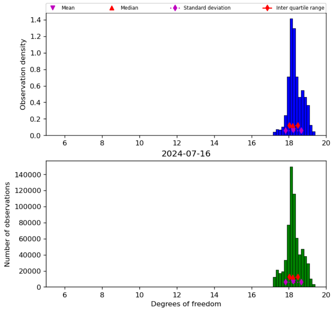
Figure 30: Histogram of “Degrees of freedom” for 2024-07-15 to 2024-07-17
