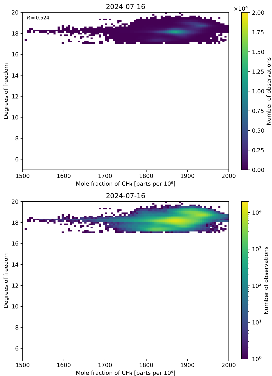
Figure 72: Scatter density plot of “Mole fraction of CH 4 ” against “Degrees of freedom” for 2024-07-15 to 2024-07-17.
