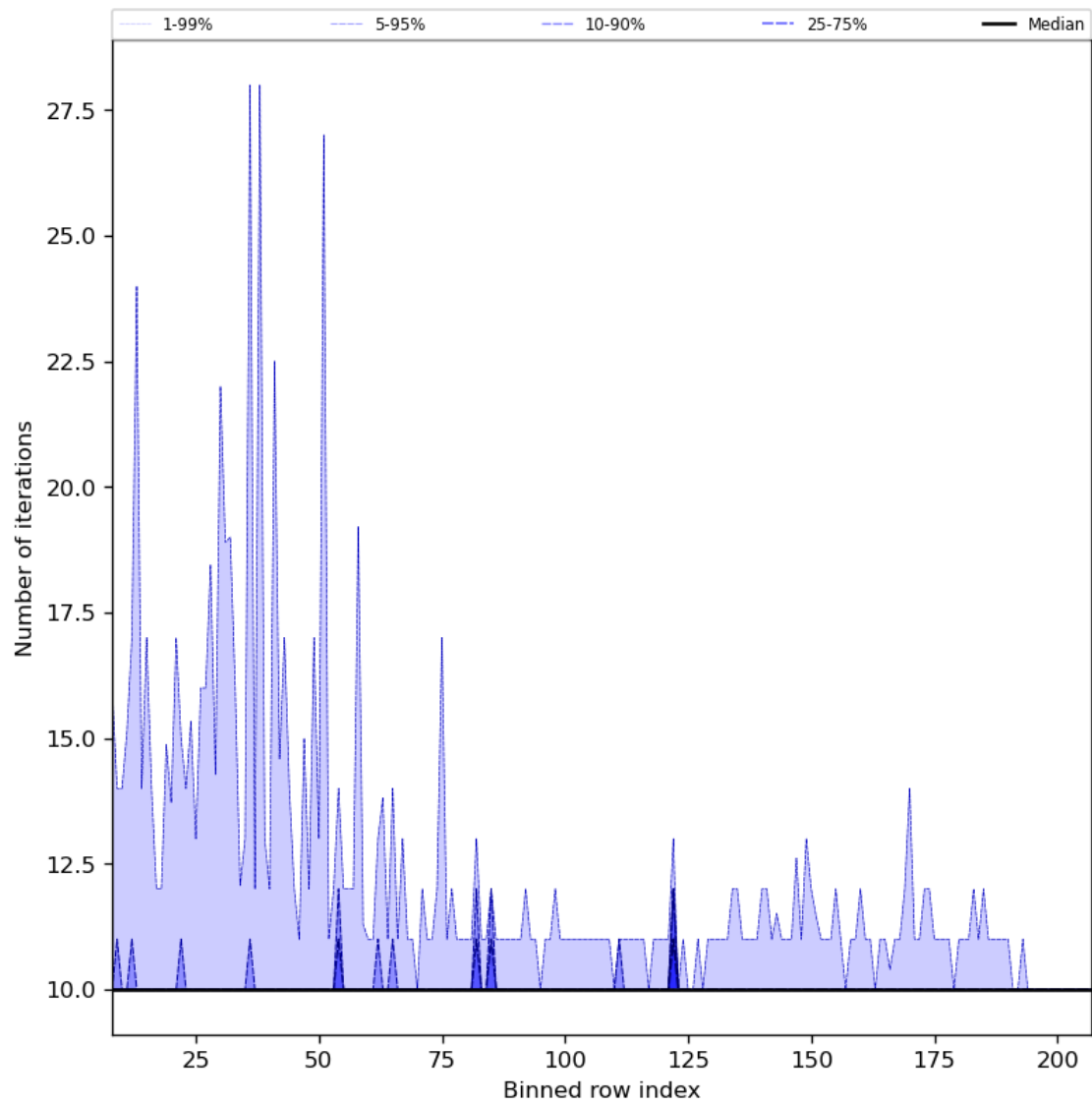
Figure 42: Along track statistics of “Number of iterations” for 2024-07-15 to 2024-07-17
