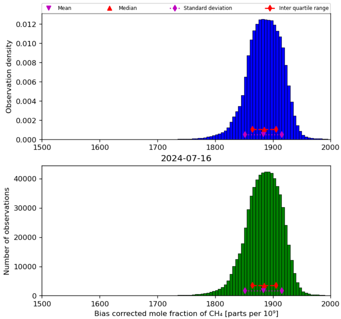
Figure 25: Histogram of “Bias corrected mole fraction of CH 4 ” for 2024-07-15 to 2024-07-17
