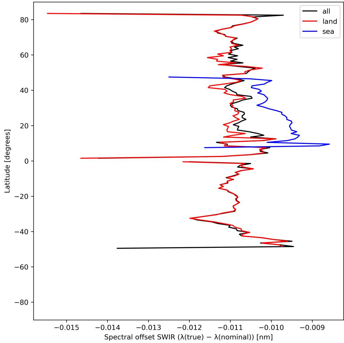
Figure 16: Zonal average of “Spectral offset SWIR ( \lambda(\text{true}) - \lambda(\text{nominal}) )” for 2024-07-15 to 2024-07-17.
