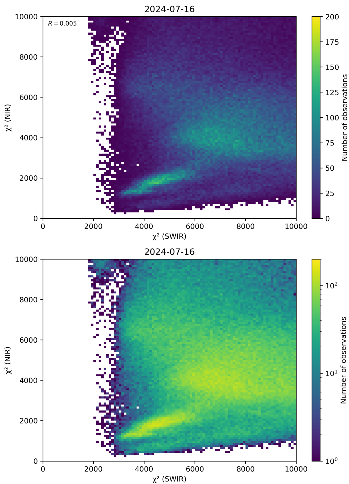
Figure 47: Scatter density plot of “ \chi^2 (SWIR)” against “ \chi^2 (NIR)” for 2024-07-15 to 2024-07-17.
