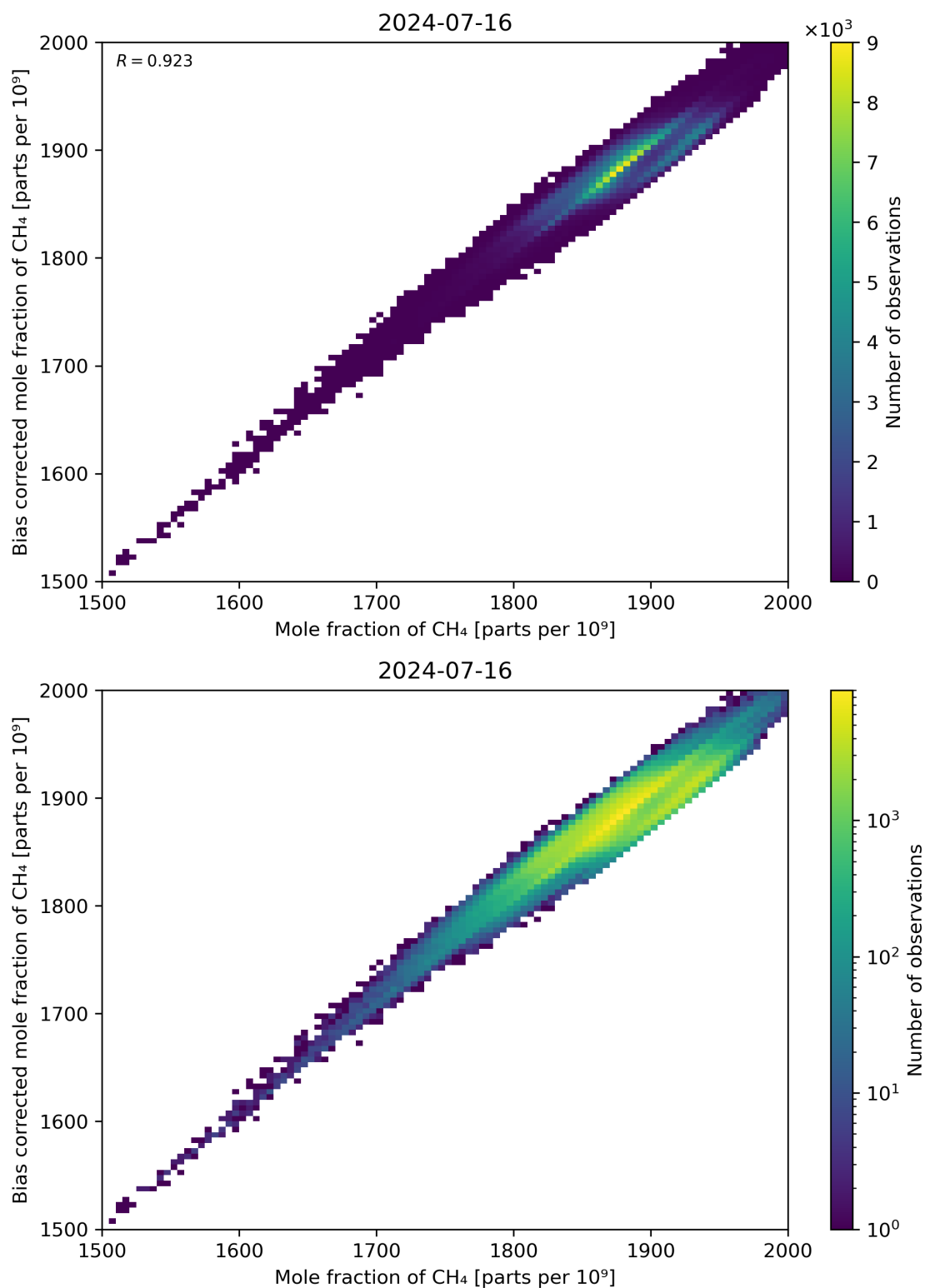
Figure 74: Scatter density plot of “Mole fraction of CH 4 ” against “Bias corrected mole fraction of CH 4 ” for 2024-07-15 to 2024-07-17.
