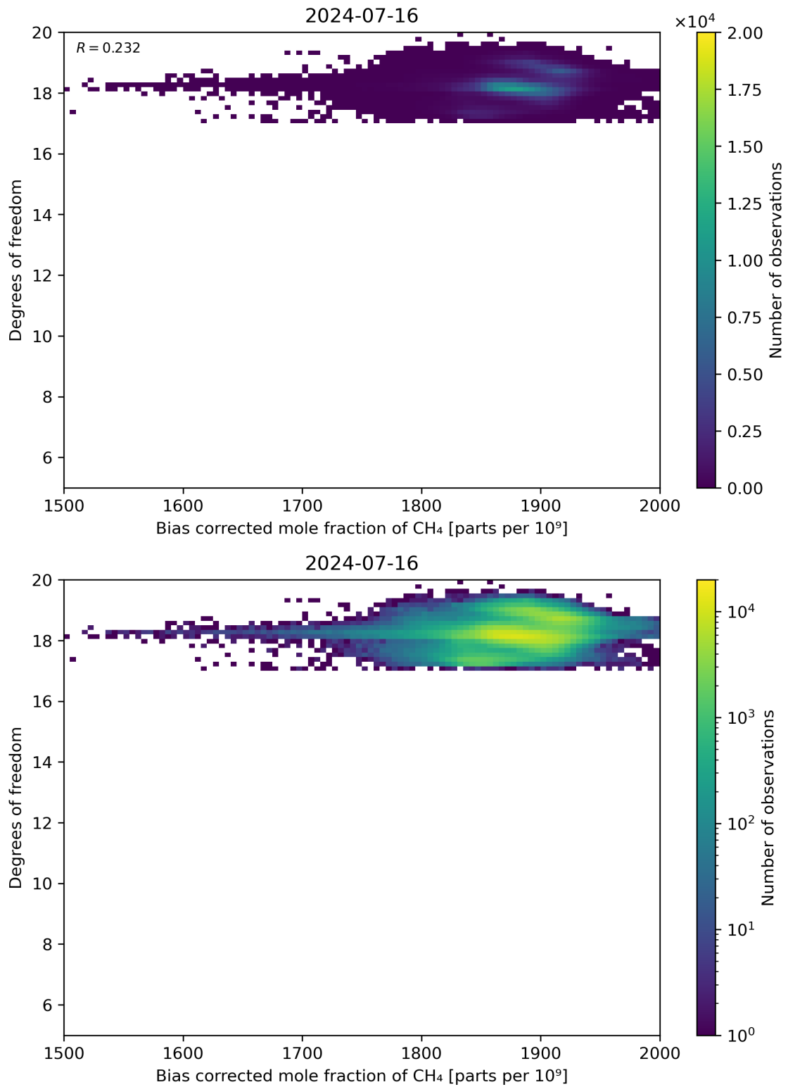
Figure 65: Scatter density plot of “Bias corrected mole fraction of CH 4 ” against “Degrees of freedom” for 2024-07-15 to 2024-07-17.
