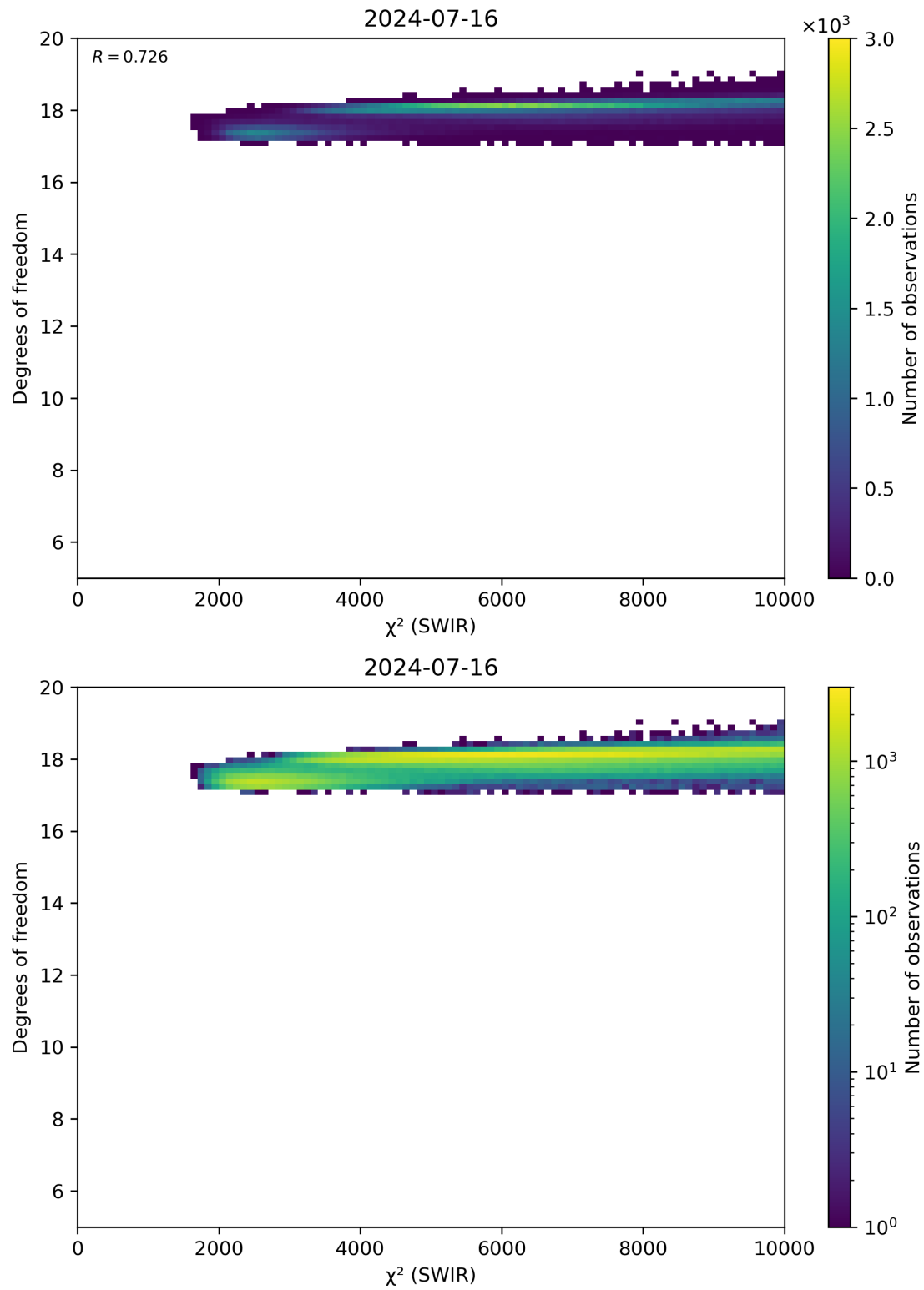
Figure 48: Scatter density plot of “ \chi^2 (SWIR)” against “Degrees of freedom” for 2024-07-15 to 2024-07-17.
