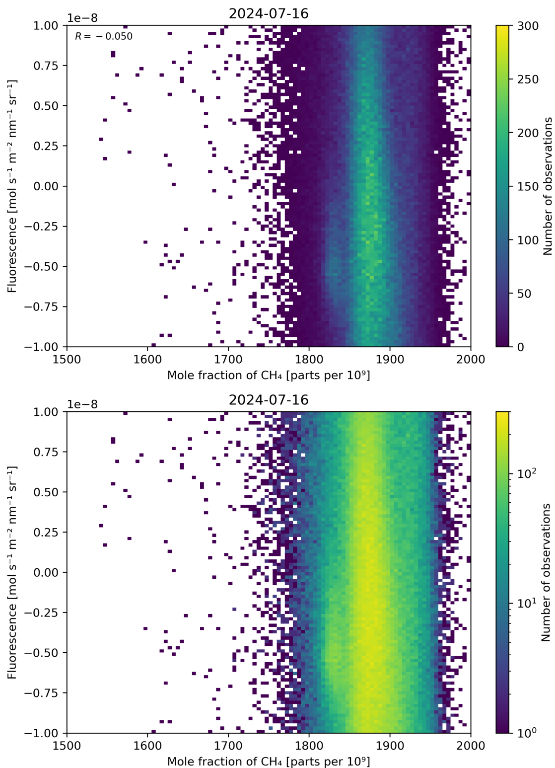
Figure 73: Scatter density plot of “Mole fraction of \text{CH}_4 ” against “Fluorescence” for 2024-07-15 to 2024-07-17.
