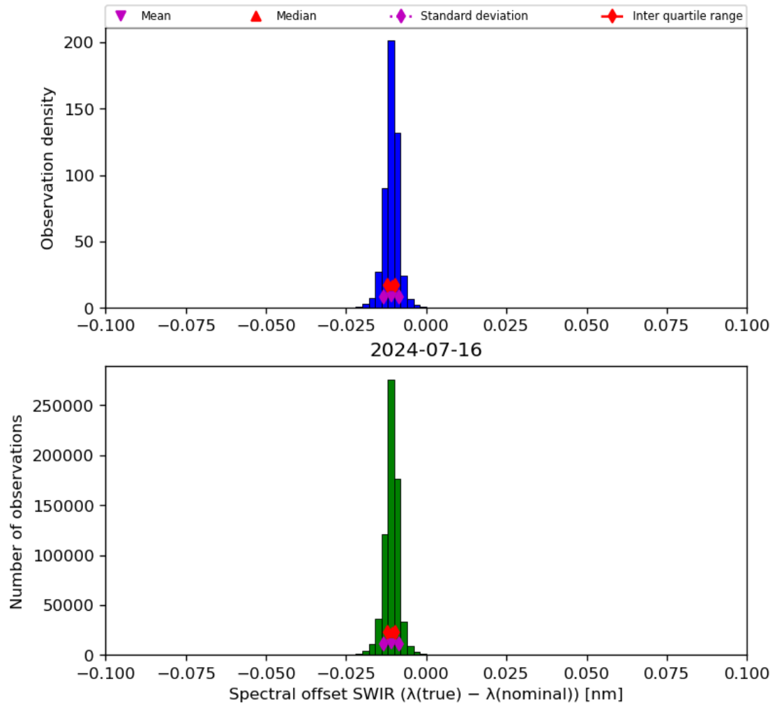
Figure 27: Histogram of “Spectral offset SWIR ( \lambda(\text{true}) - \lambda(\text{nominal}) )” for 2024-07-15 to 2024-07-17
