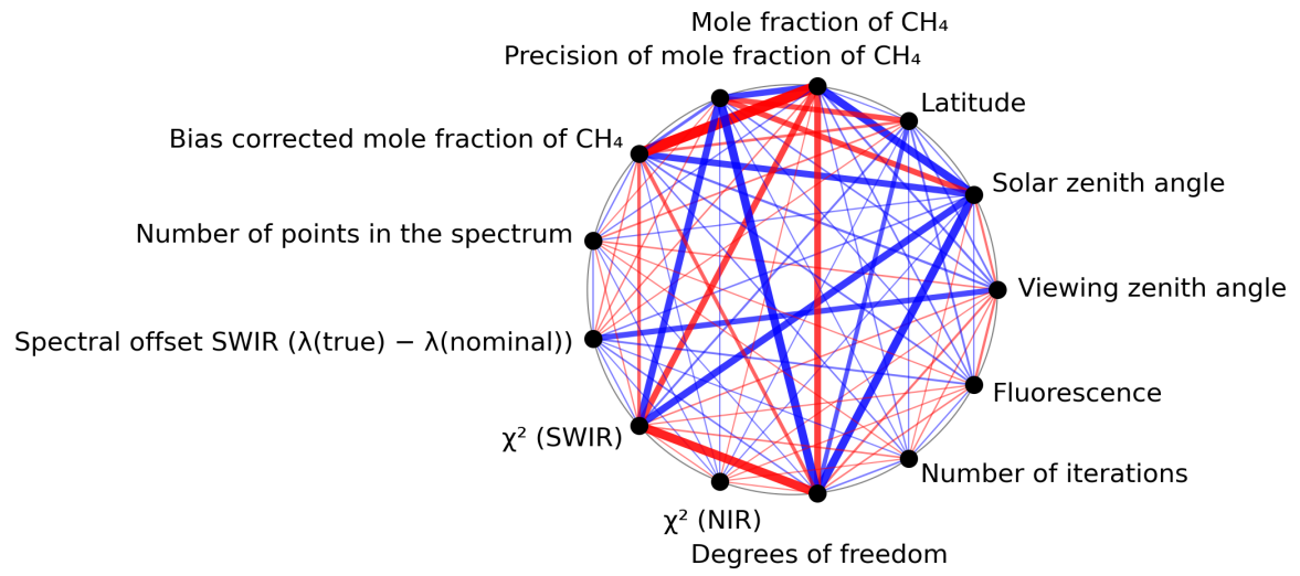
Figure 1: Map of correlation graph for 2024-07-15 to 2024-07-17.
