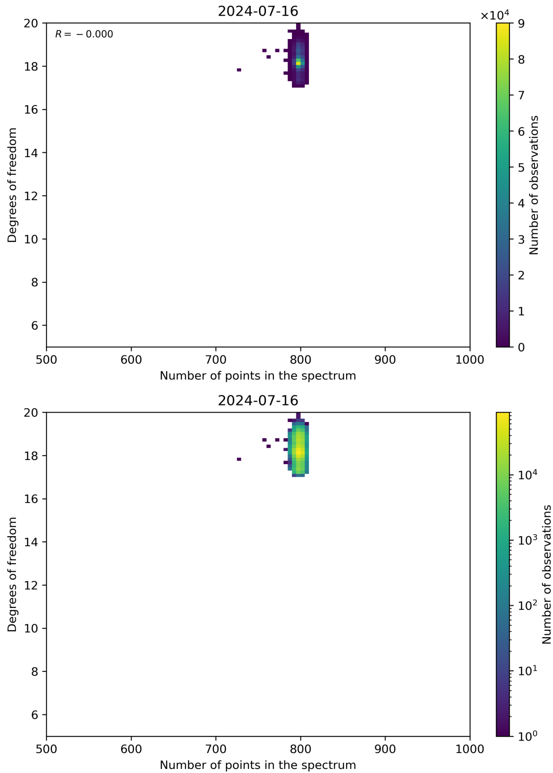
Figure 90: Scatter density plot of “Number of points in the spectrum” against “Degrees of freedom” for 2024-07-15 to 2024-07-17.
