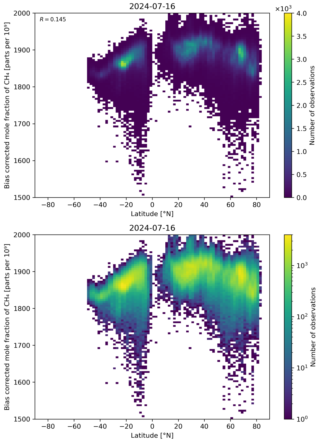
Figure 58: Scatter density plot of “Latitude” against “Bias corrected mole fraction of CH 4 ” for 2024-07-15 to 2024-07-17.
