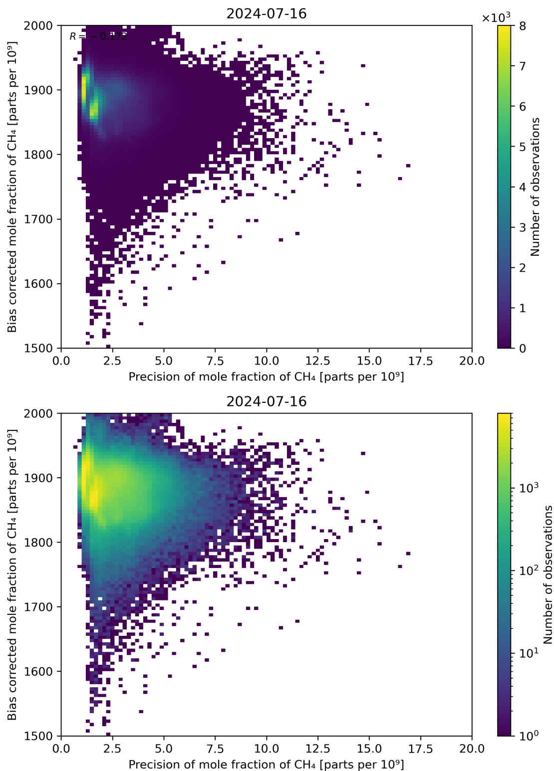
Figure 82: Scatter density plot of “Precision of mole fraction of CH 4 ” against “Bias corrected mole fraction of CH 4 ” for 2024-07-15 to 2024-07-17.
