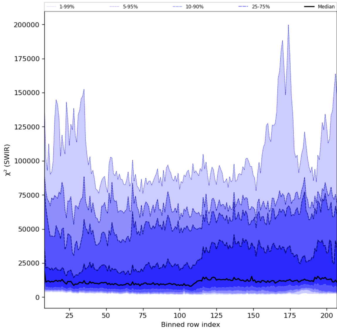
Figure 39: Along track statistics of “ \chi^2 (SWIR)” for 2024-07-15 to 2024-07-17
