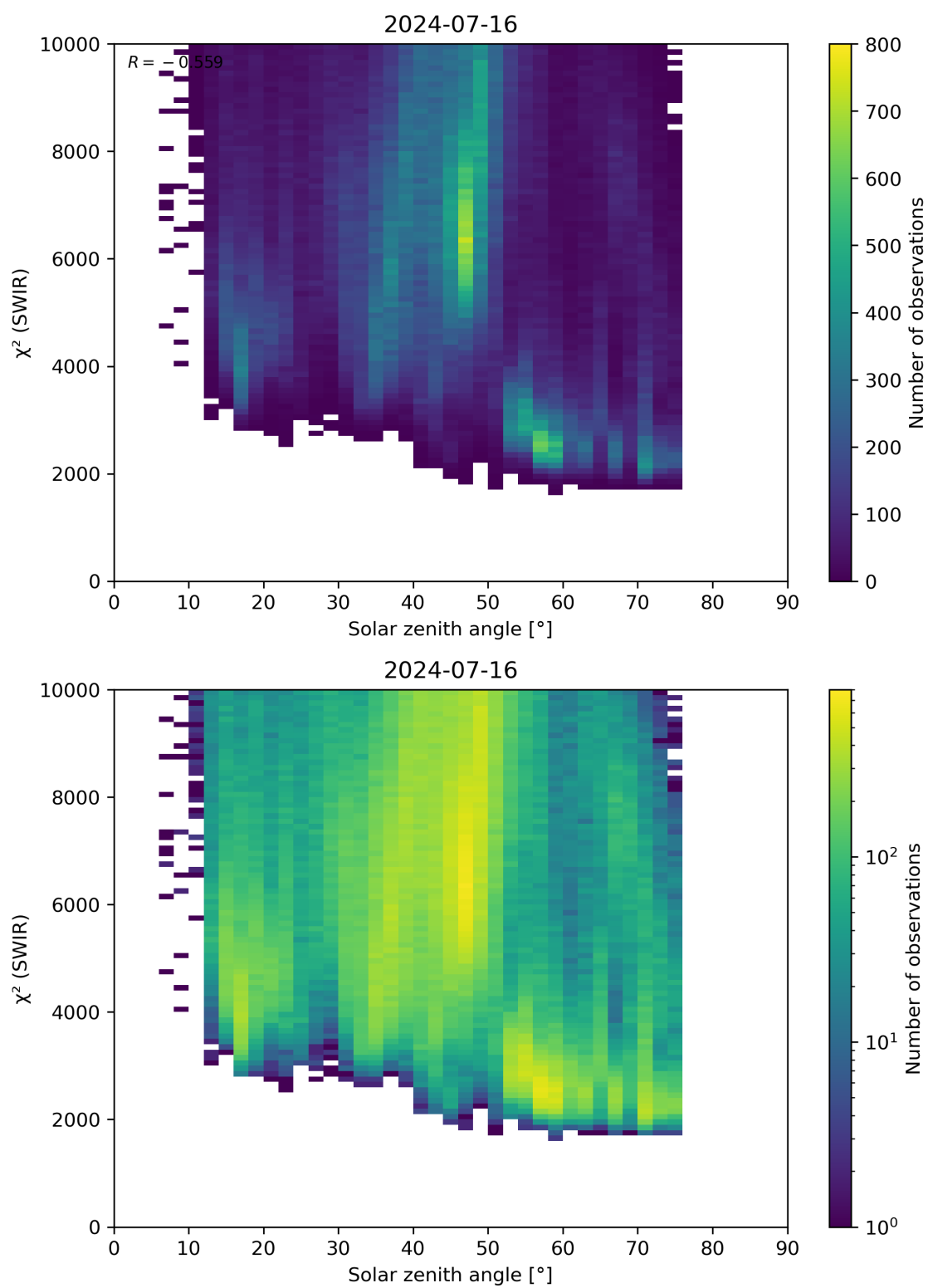
Figure 95: Scatter density plot of “Solar zenith angle” against “ \chi^2 (SWIR)” for 2024-07-15 to 2024-07-17.
