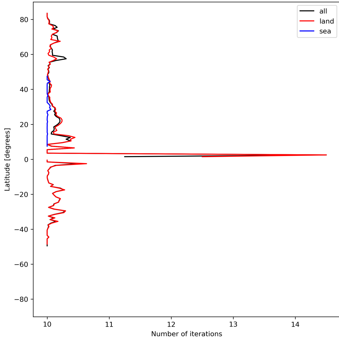
Figure 20: Zonal average of “Number of iterations” for 2024-07-15 to 2024-07-17.
