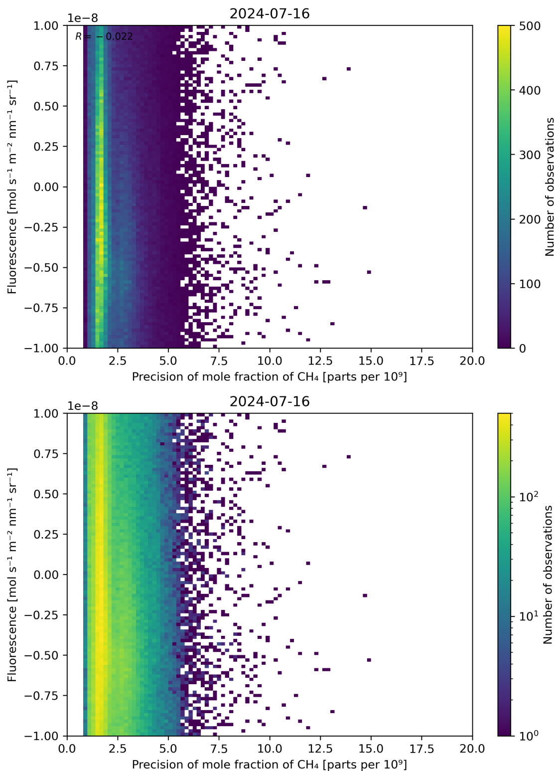
Figure 81: Scatter density plot of “Precision of mole fraction of \text{CH}_4 ” against “Fluorescence” for 2024-07-15 to 2024-07-17.
