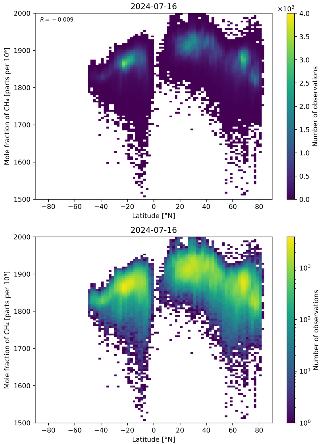
Figure 57: Scatter density plot of “Latitude” against “Mole fraction of CH 4 ” for 2024-07-15 to 2024-07-17.
