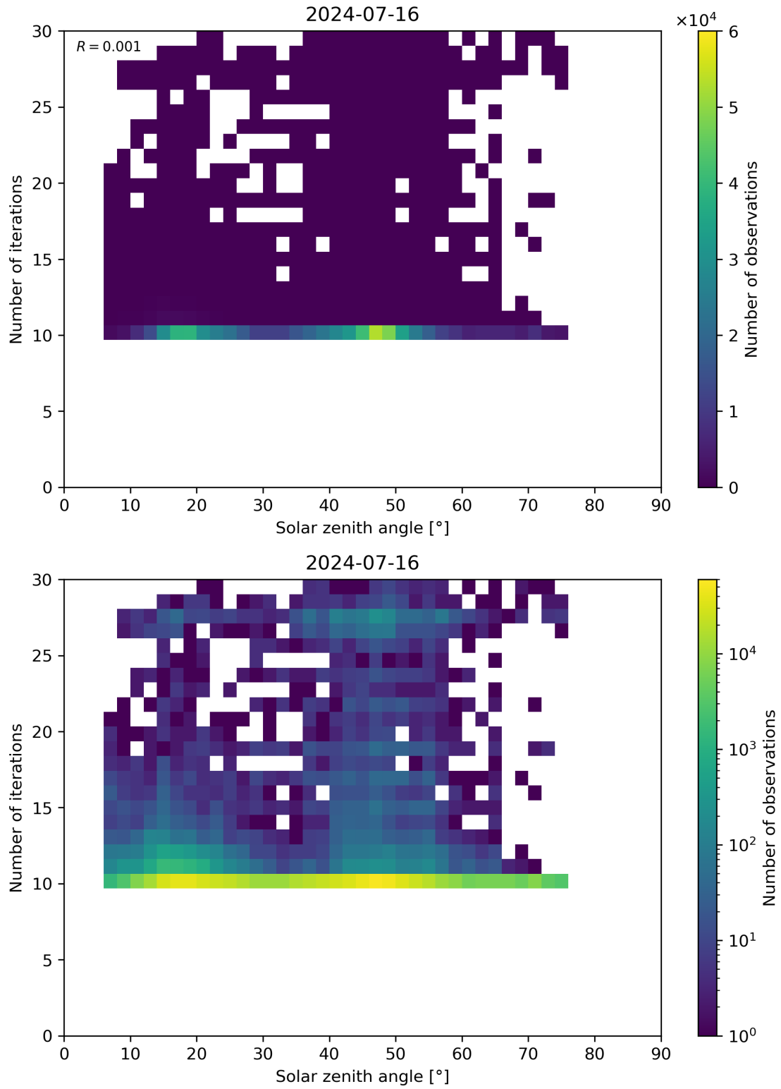
Figure 102: Scatter density plot of “Solar zenith angle” against “Number of iterations” for 2024-07-15 to 2024-07-17.
