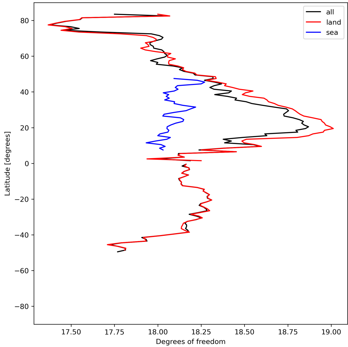
Figure 19: Zonal average of “Degrees of freedom” for 2024-07-15 to 2024-07-17.
