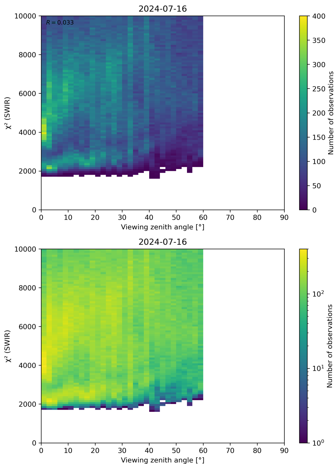
Figure 106: Scatter density plot of “Viewing zenith angle” against “ \chi^2 (SWIR)” for 2024-07-15 to 2024-07-17.
