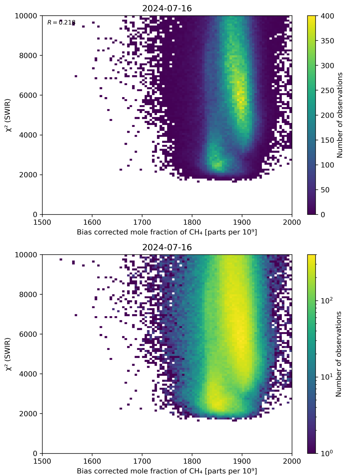
Figure 64: Scatter density plot of “Bias corrected mole fraction of CH 4 ” against “ \chi^2 (SWIR)” for 2024-07-15 to 2024-07-17.
