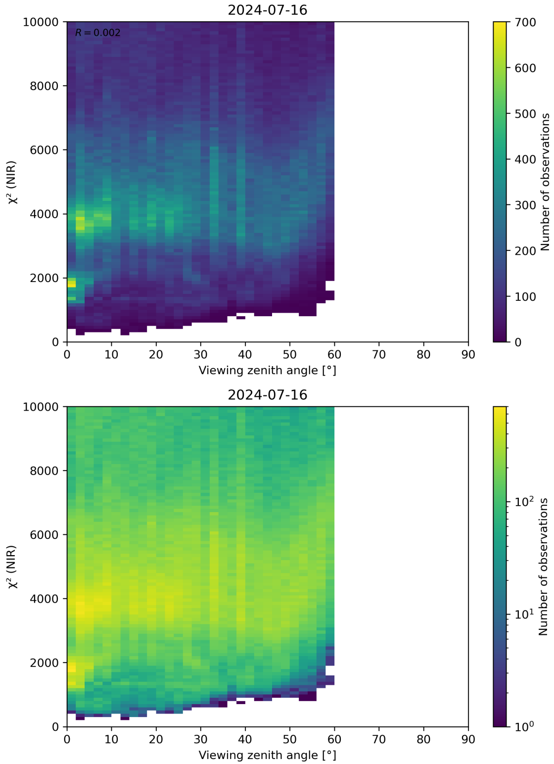
Figure 105: Scatter density plot of “Viewing zenith angle” against “ \chi^2 (NIR)” for 2024-07-15 to 2024-07-17.
