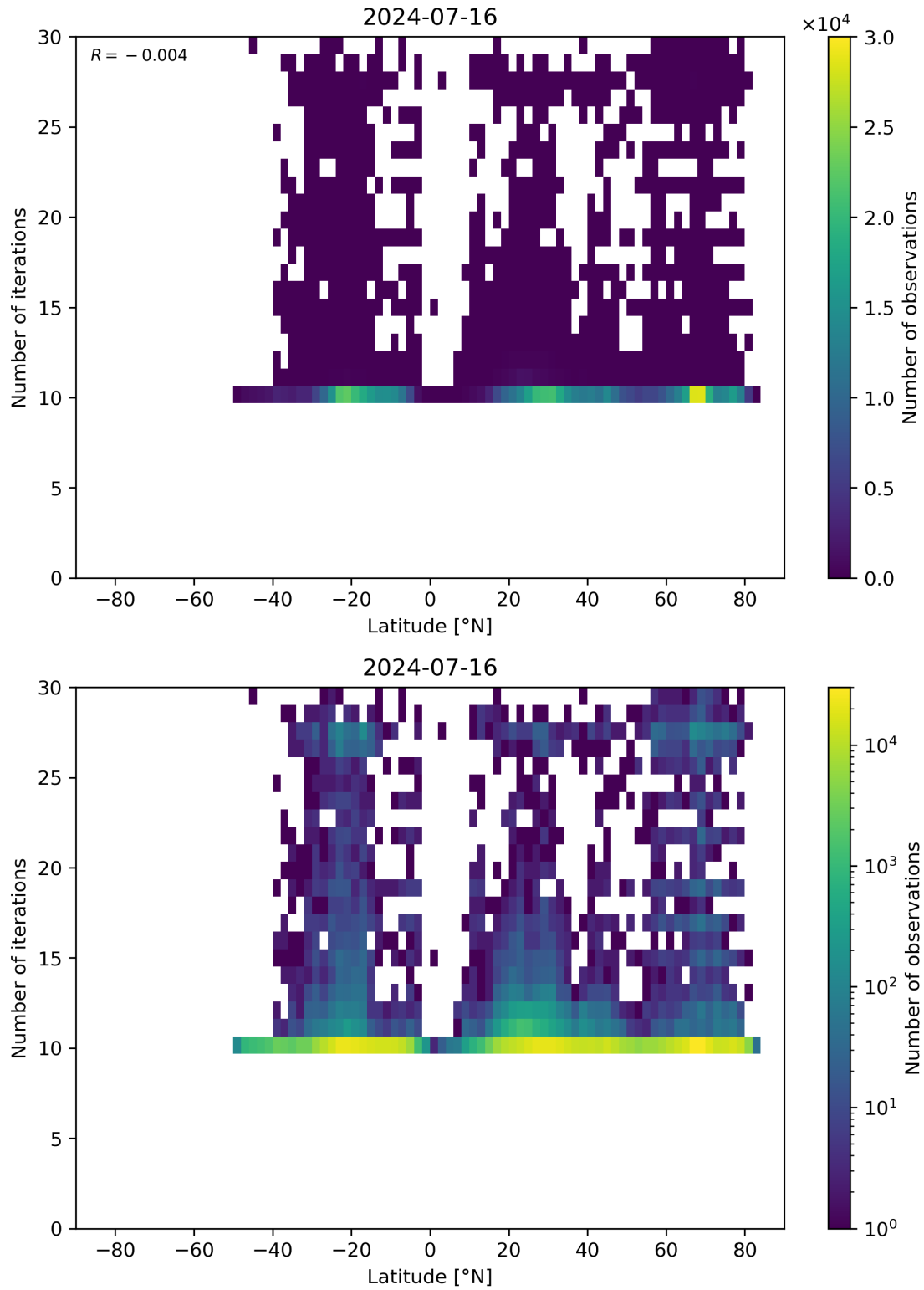
Figure 60: Scatter density plot of “Latitude” against “Number of iterations” for 2024-07-15 to 2024-07-17.
