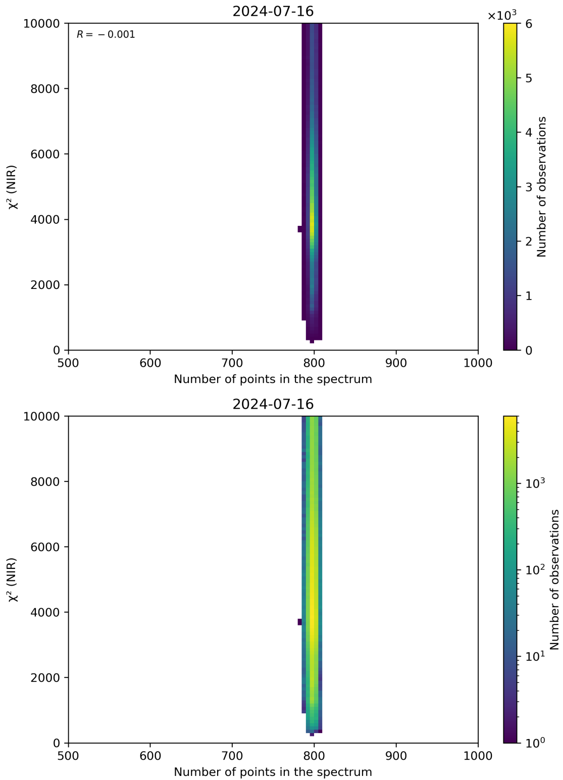
Figure 88: Scatter density plot of “Number of points in the spectrum” against “ \chi^2 (NIR)” for 2024-07-15 to 2024-07-17.
