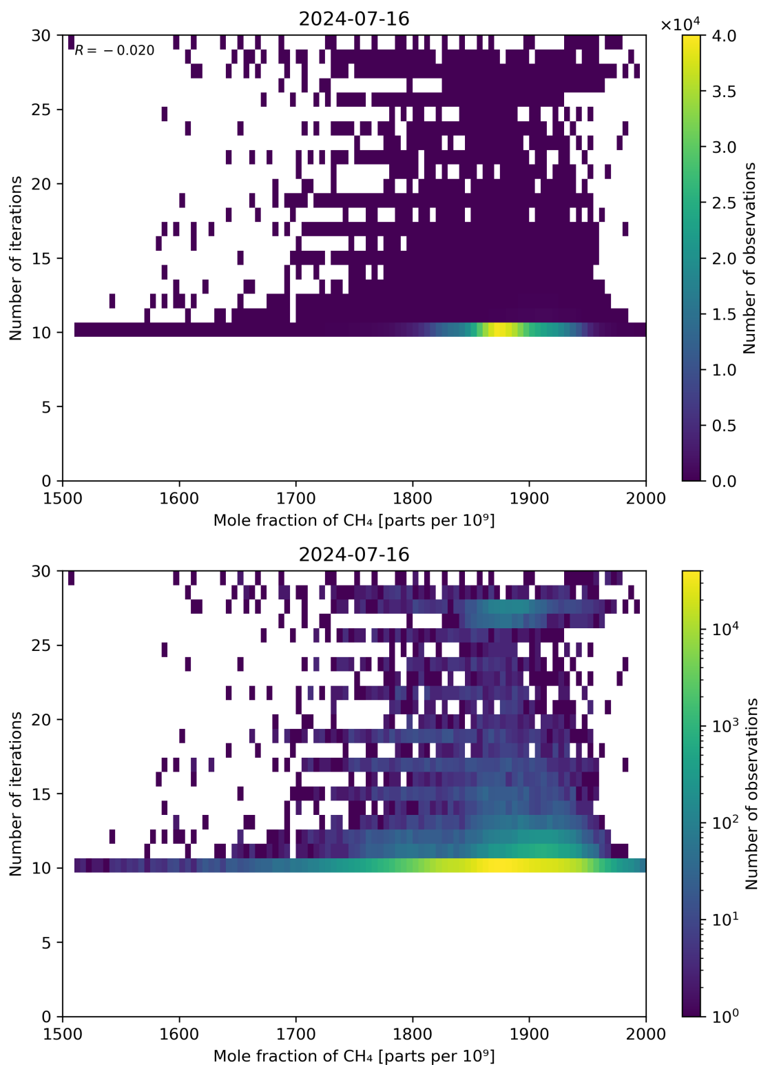
Figure 76: Scatter density plot of “Mole fraction of CH 4 ” against “Number of iterations” for 2024-07-15 to 2024-07-17.
