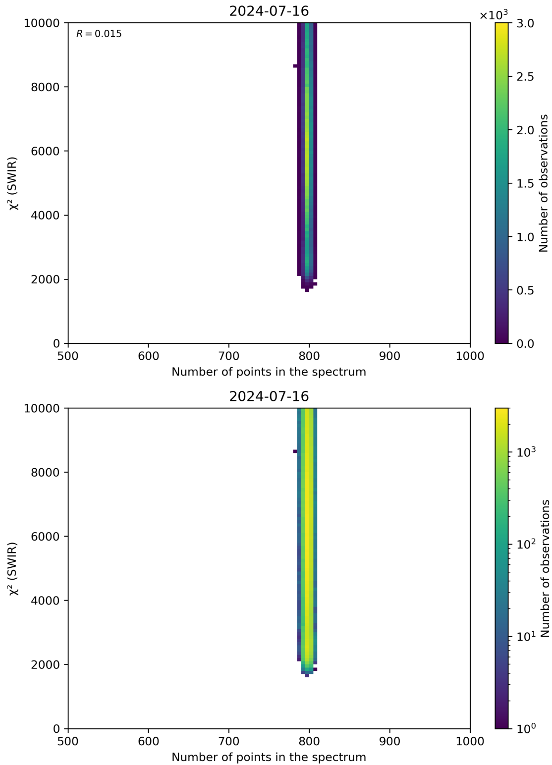
Figure 89: Scatter density plot of “Number of points in the spectrum” against “ \chi^2 (SWIR)” for 2024-07-15 to 2024-07-17.
