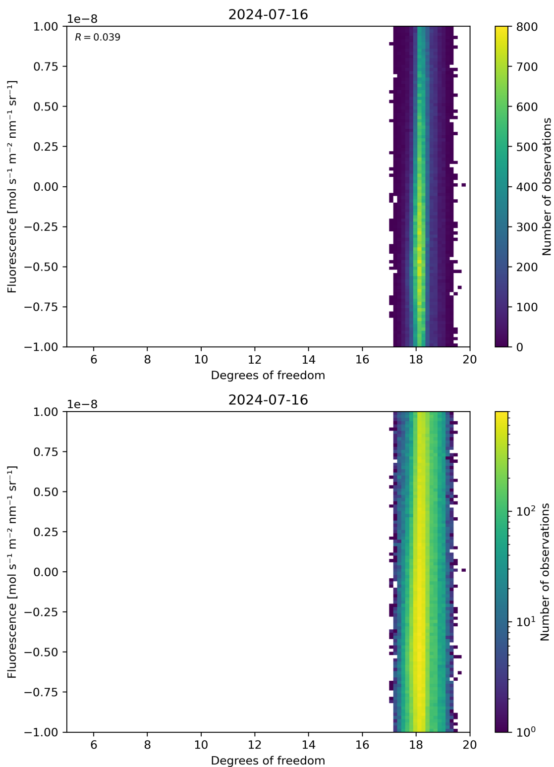
Figure 51: Scatter density plot of “Degrees of freedom” against “Fluorescence” for 2024-07-15 to 2024-07-17.
