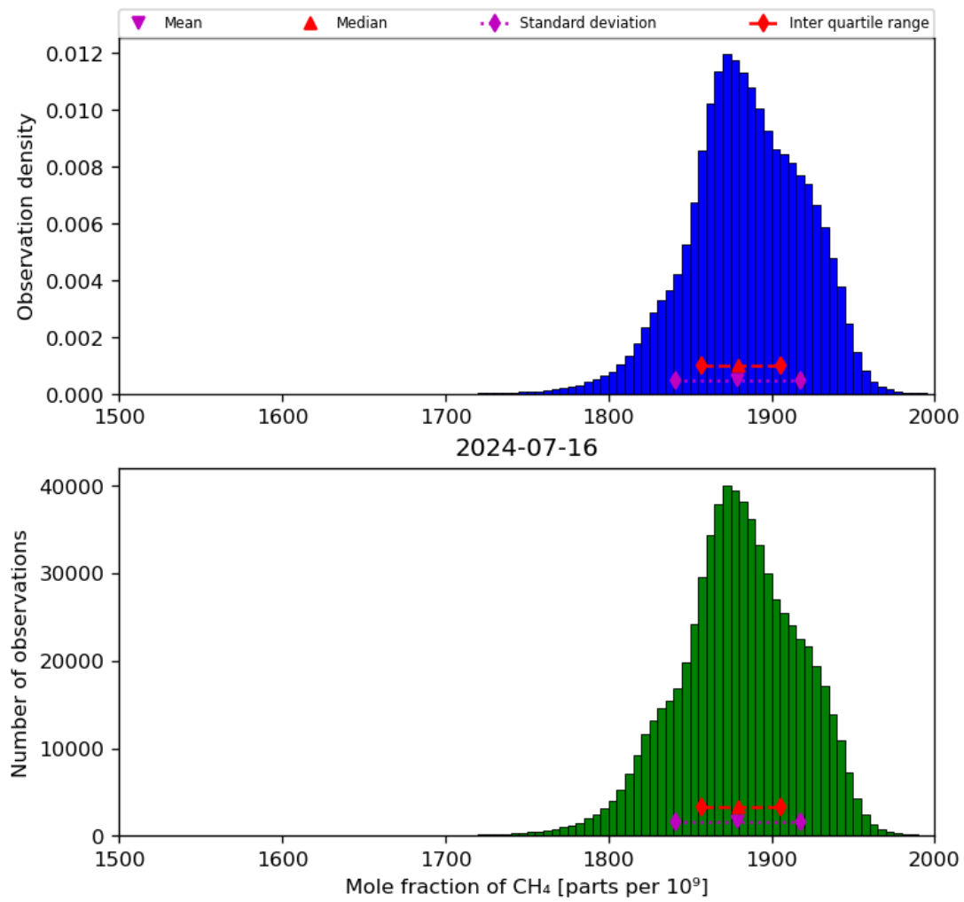
Figure 23: Histogram of “Mole fraction of CH 4 ” for 2024-07-15 to 2024-07-17
