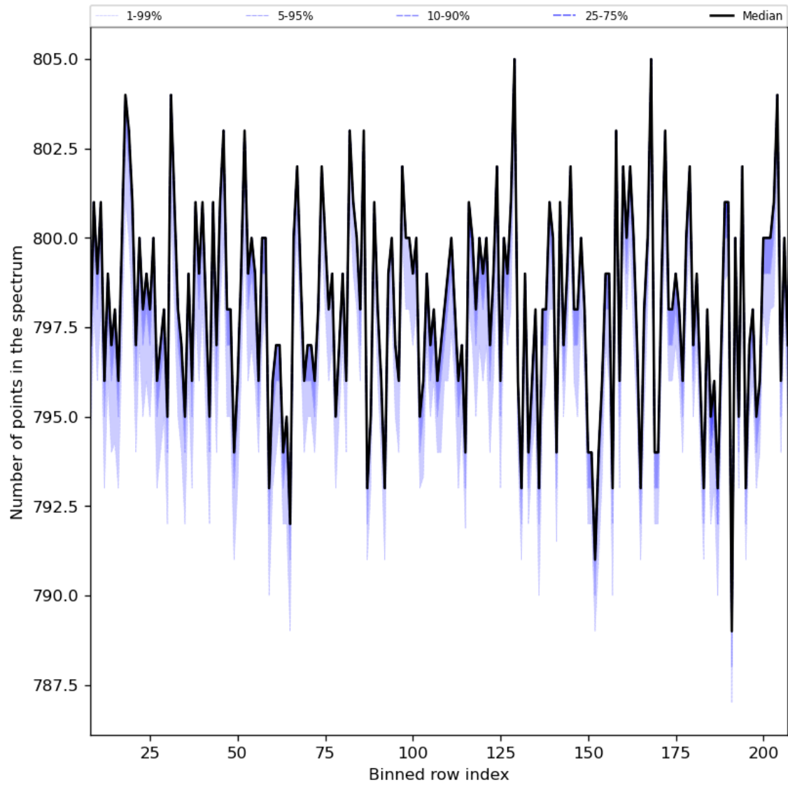
Figure 37: Along track statistics of “Number of points in the spectrum” for 2024-07-15 to 2024-07-17
