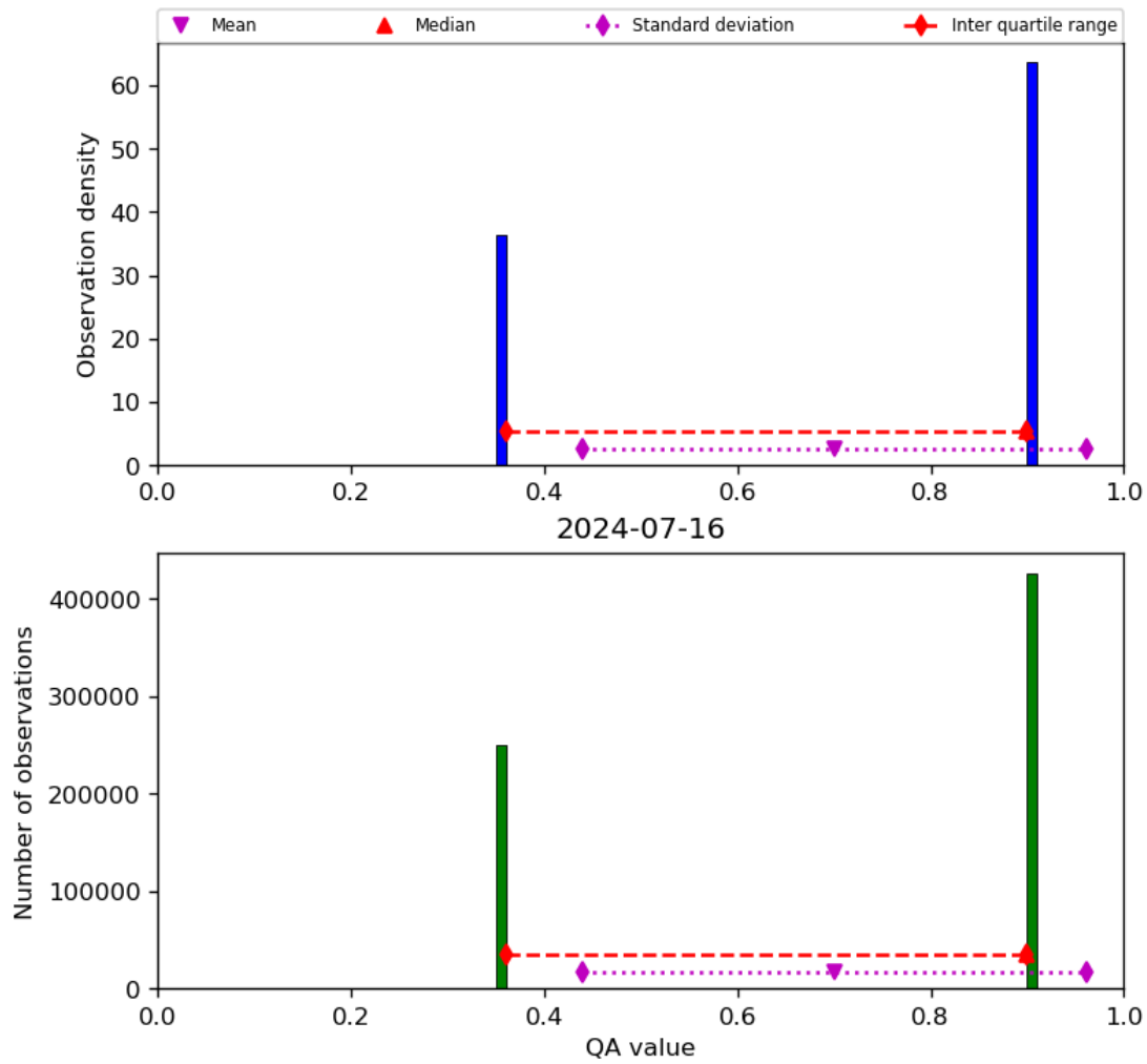
Figure 22: Histogram of “QA value” for 2024-07-15 to 2024-07-17
