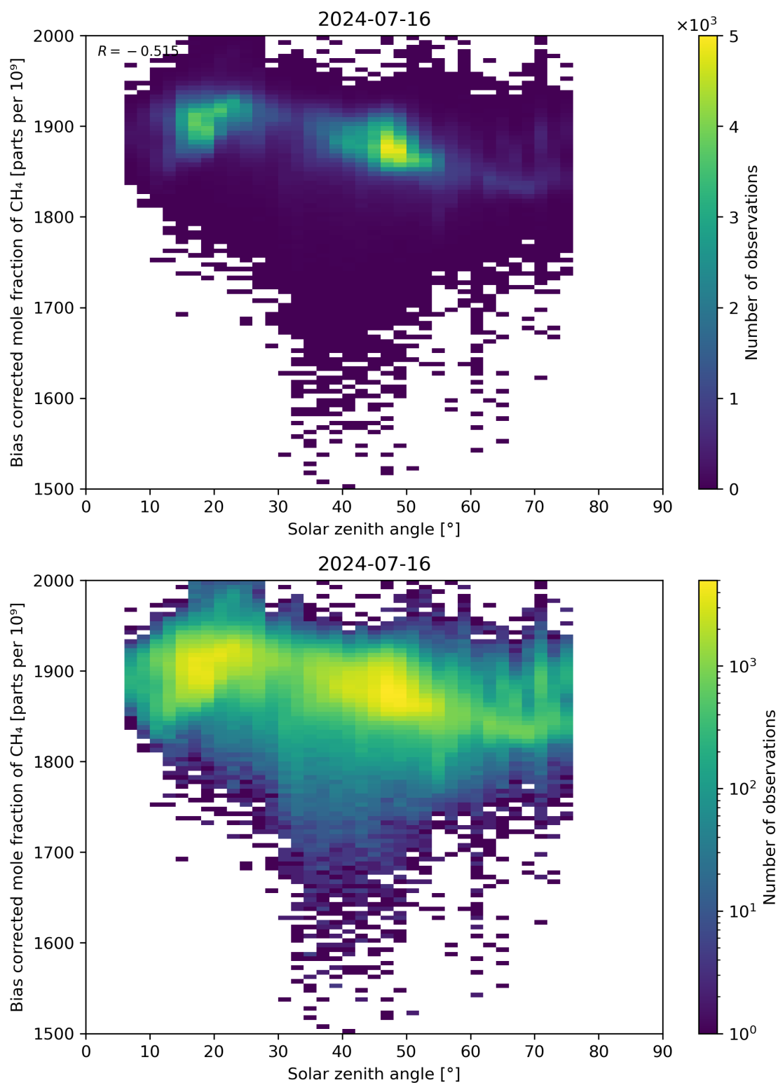
Figure 100: Scatter density plot of “Solar zenith angle” against “Bias corrected mole fraction of CH 4 ” for 2024-07-15 to 2024-07-17.
