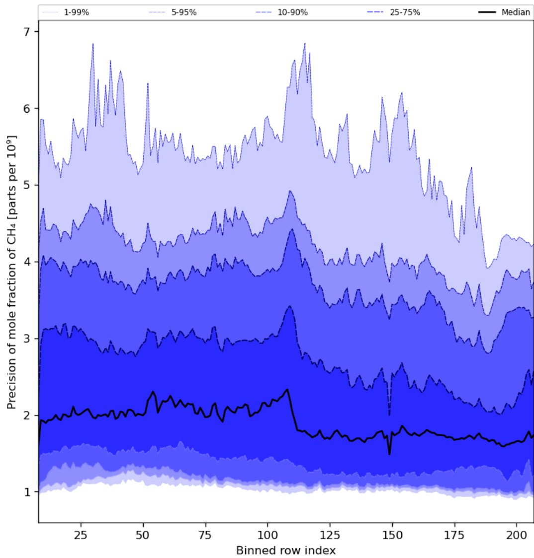
Figure 35: Along track statistics of “Precision of mole fraction of CH 4 ” for 2024-07-15 to 2024-07-17
