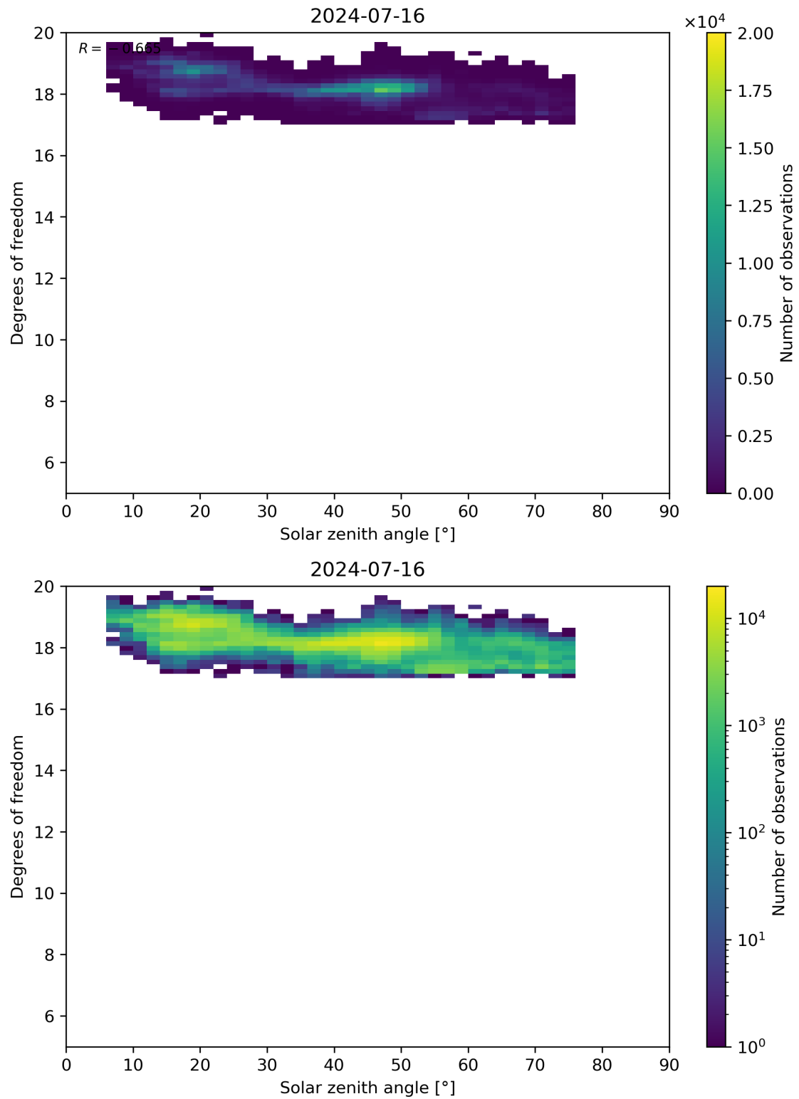
Figure 96: Scatter density plot of “Solar zenith angle” against “Degrees of freedom” for 2024-07-15 to 2024-07-17.
