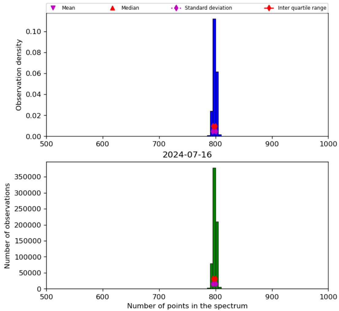
Figure 26: Histogram of “Number of points in the spectrum” for 2024-07-15 to 2024-07-17
