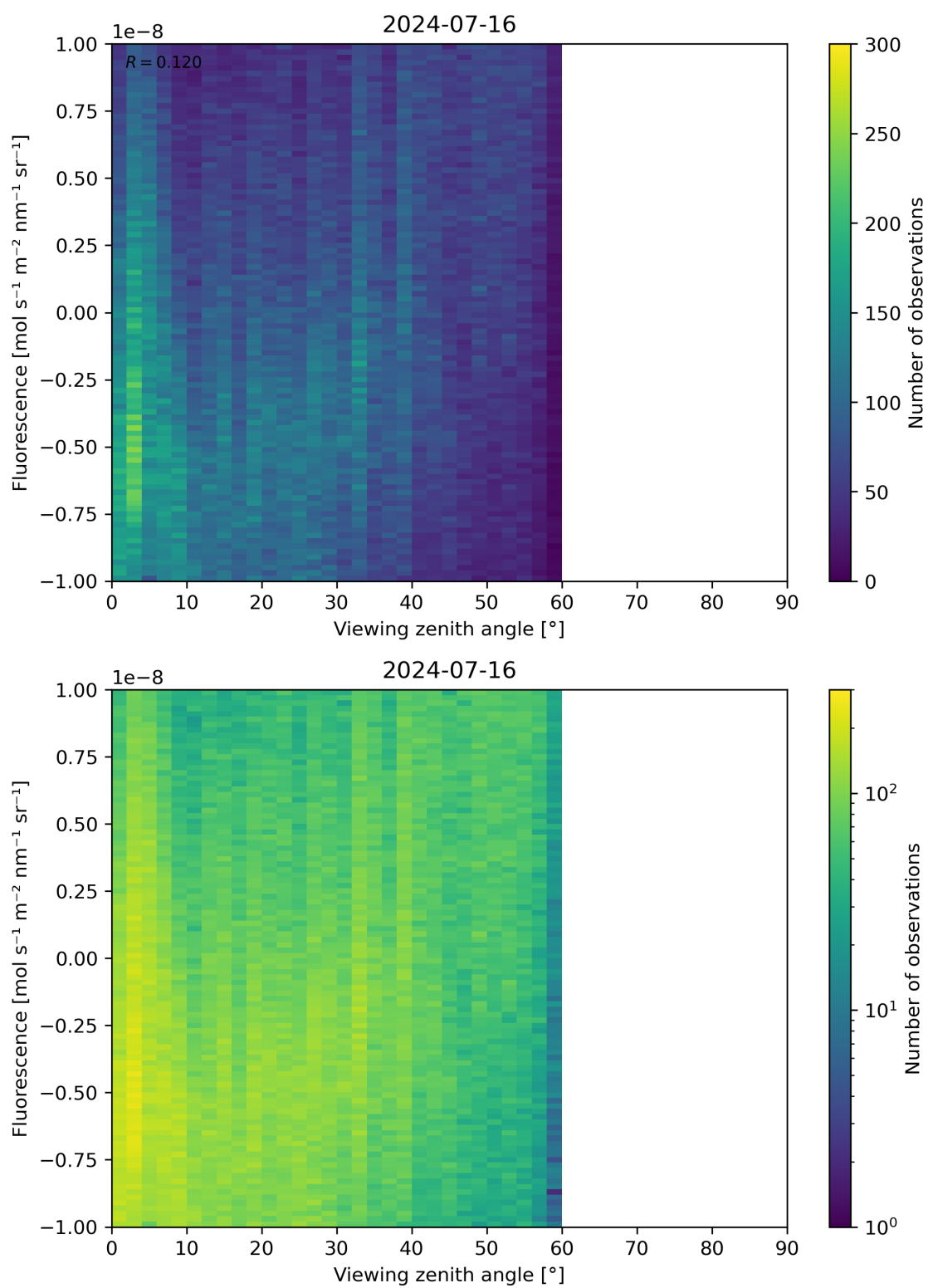
Figure 108: Scatter density plot of “Viewing zenith angle” against “Fluorescence” for 2024-07-15 to 2024-07-17.
