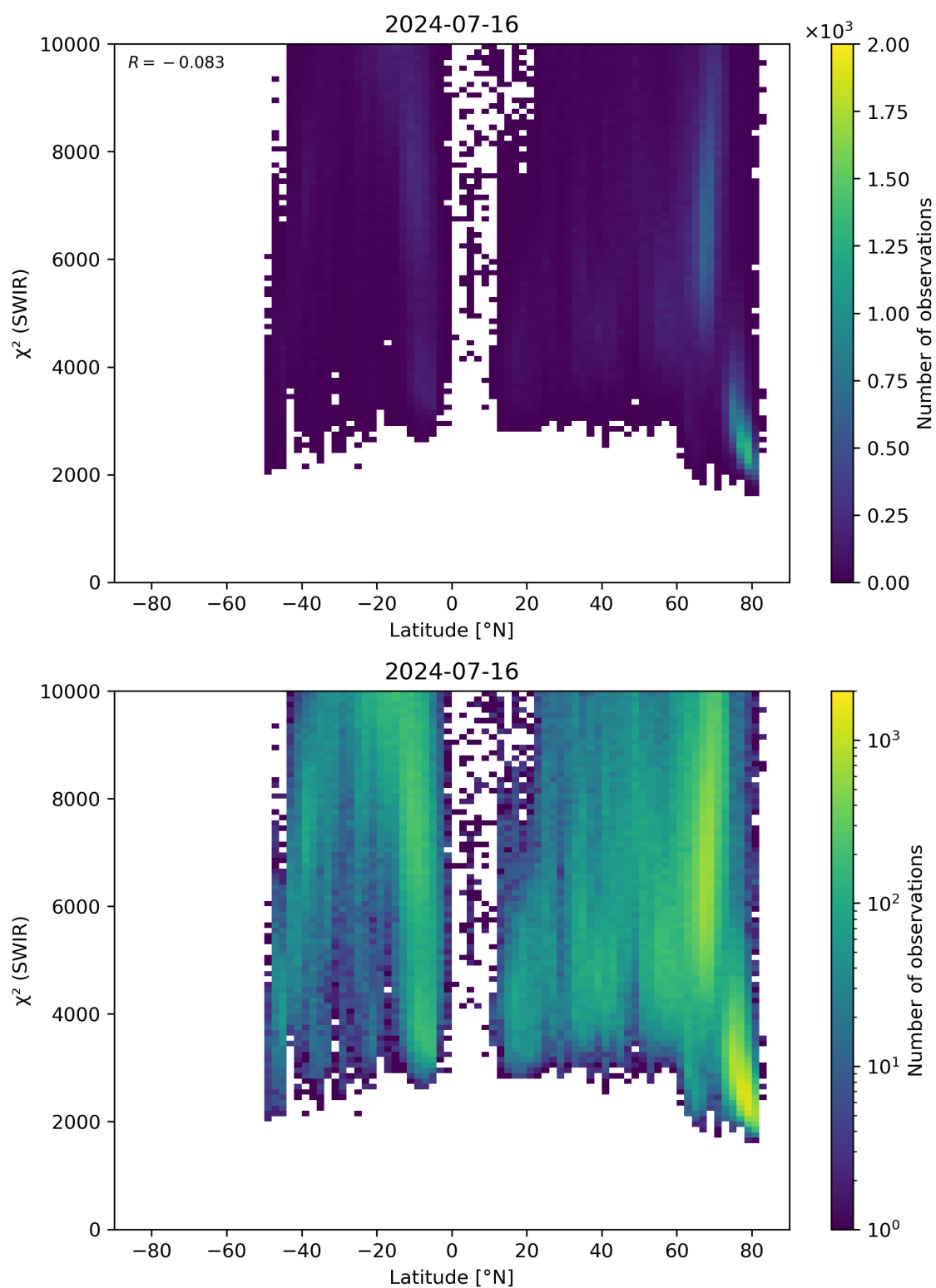
Figure 54: Scatter density plot of “Latitude” against “ \chi^2 (SWIR)” for 2024-07-15 to 2024-07-17.
