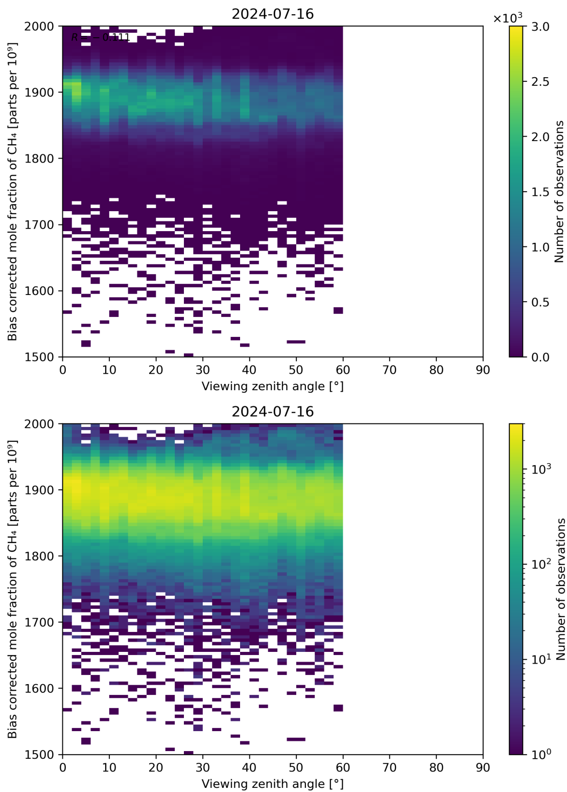
Figure 111: Scatter density plot of “Viewing zenith angle” against “Bias corrected mole fraction of CH 4 ” for 2024-07-15 to 2024-07-17.
