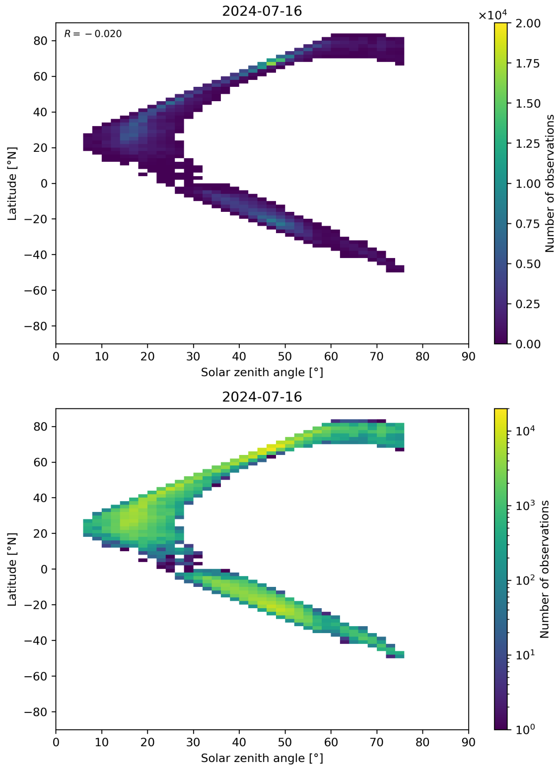
Figure 98: Scatter density plot of “Solar zenith angle” against “Latitude” for 2024-07-15 to 2024-07-17.
