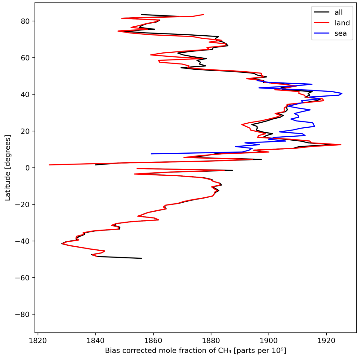
Figure 14: Zonal average of “Bias corrected mole fraction of CH 4 ” for 2024-07-15 to 2024-07-17.
