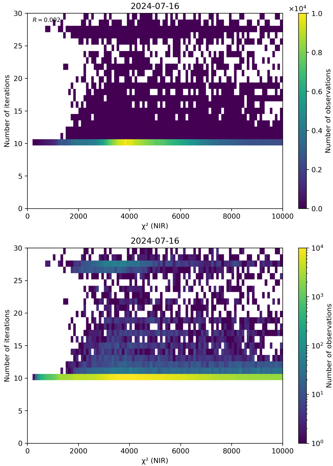
Figure 46: Scatter density plot of “ \chi^2 (NIR)” against “Number of iterations” for 2024-07-15 to 2024-07-17.
