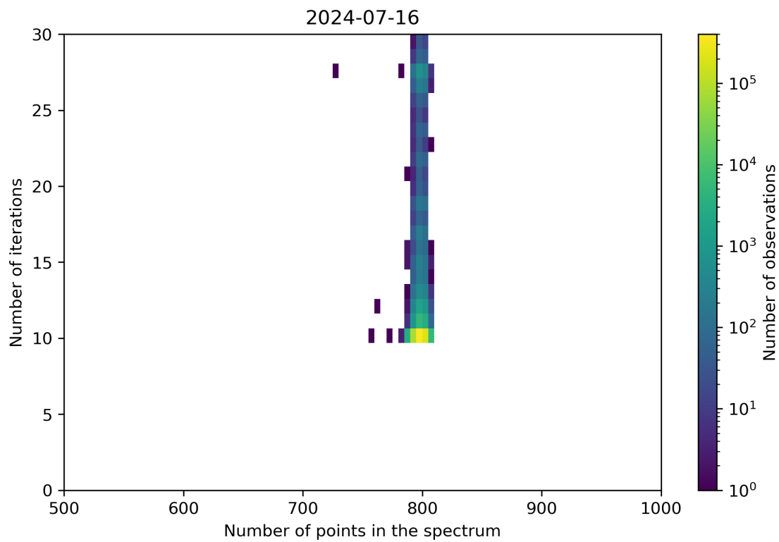
Figure 92: Scatter density plot of “Number of points in the spectrum” against “Number of iterations” for 2024-07-15 to 2024-07-17.
