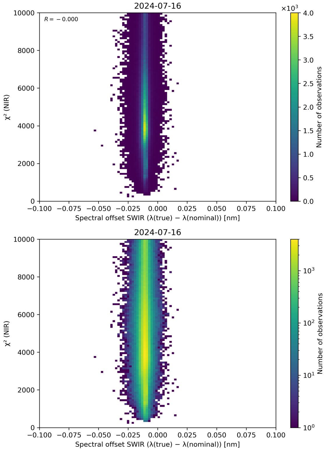
Figure 117: Scatter density plot of “Spectral offset SWIR ( \lambda(\text{true}) - \lambda(\text{nominal}) )” against “ \chi^2 (NIR)” for 2024-07-15 to 2024-07-17.
