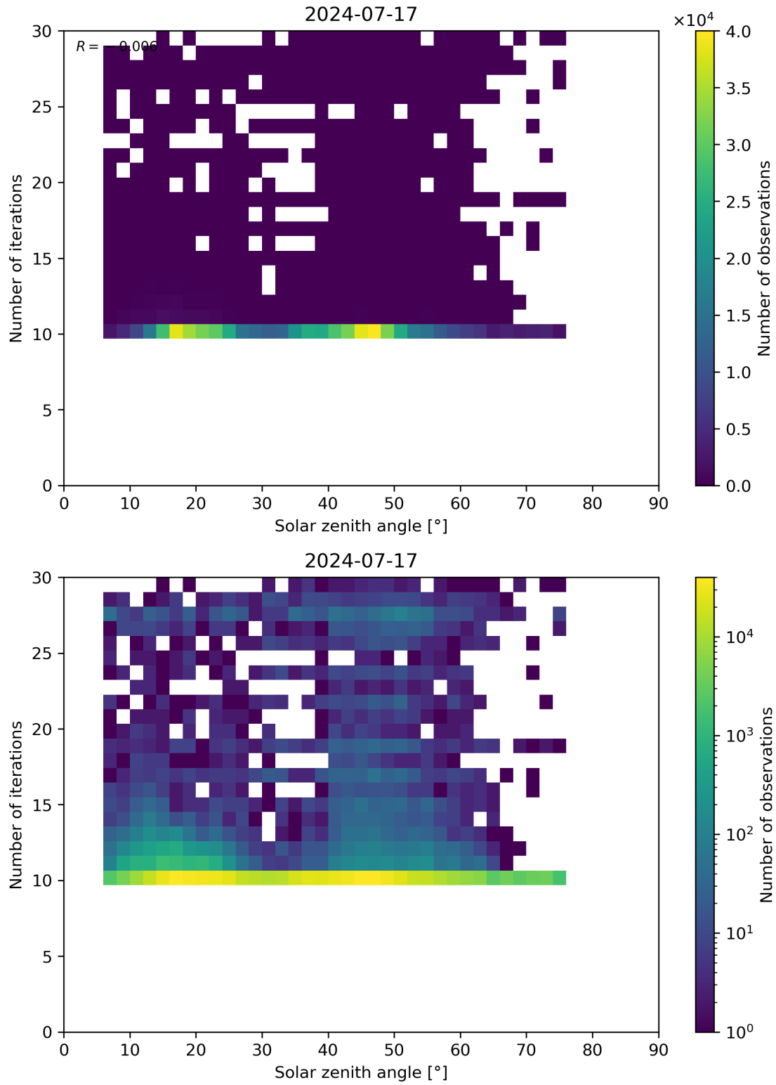
Figure 102: Scatter density plot of “Solar zenith angle” against “Number of iterations” for 2024-07-16 to 2024-07-18.
