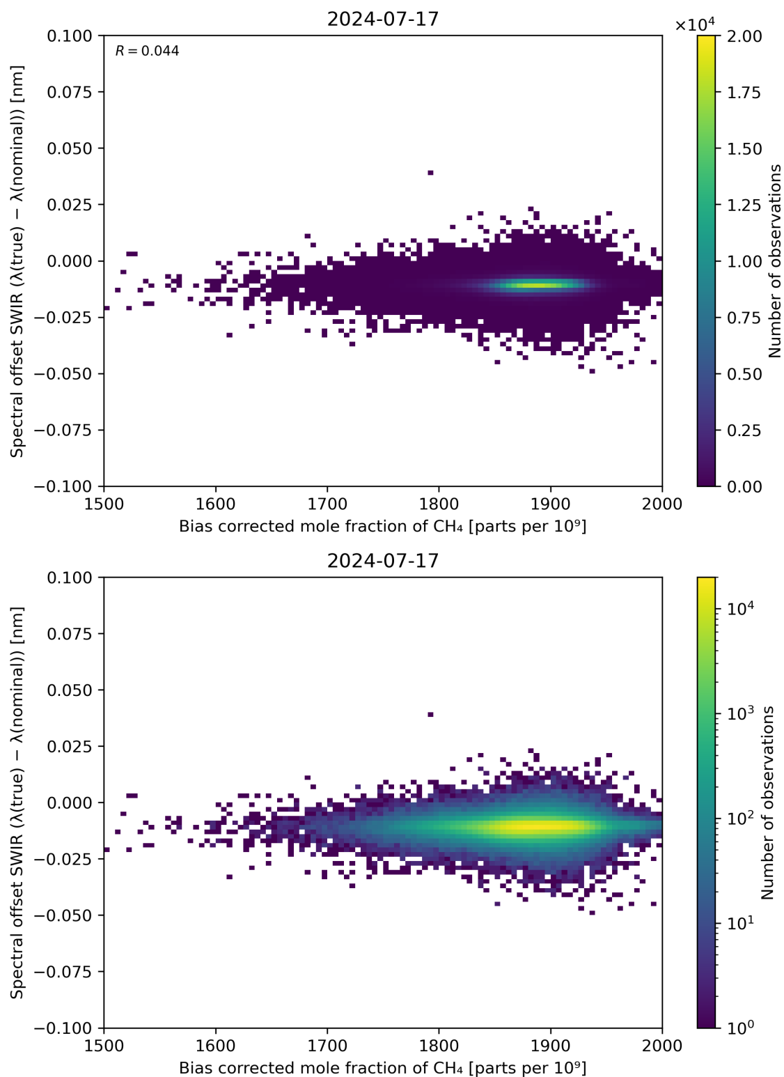
Figure 69: Scatter density plot of “Bias corrected mole fraction of \text{CH}_4 ” against “Spectral offset SWIR ( \lambda(\text{true}) - \lambda(\text{nominal}) )” for 2024-07-16 to 2024-07-18.
