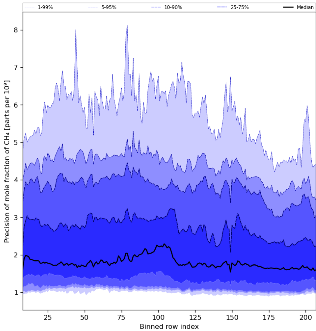
Figure 35: Along track statistics of “Precision of mole fraction of CH 4 ” for 2024-07-16 to 2024-07-18
