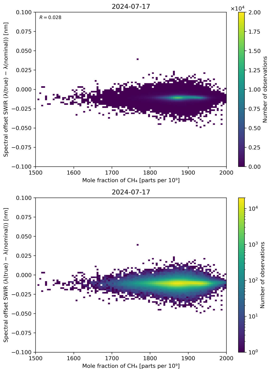
Figure 86: Scatter density plot of “Mole fraction of CH 4 ” against “Spectral offset SWIR ( \lambda(\text{true}) - \lambda(\text{nominal}) )” for 2024-07-16 to 2024-07-18.
