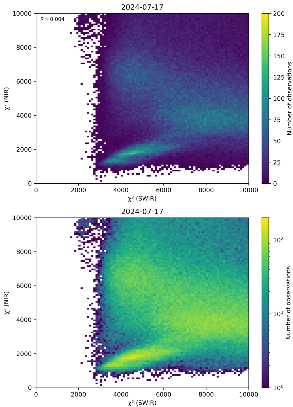
Figure 47: Scatter density plot of “ \chi^2 (SWIR)” against “ \chi^2 (NIR)” for 2024-07-16 to 2024-07-18.
