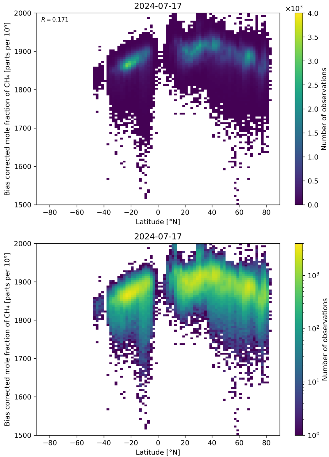
Figure 58: Scatter density plot of “Latitude” against “Bias corrected mole fraction of \text{CH}_4 ” for 2024-07-16 to 2024-07-18.
