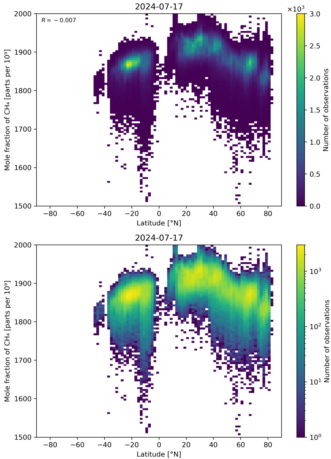
Figure 57: Scatter density plot of “Latitude” against “Mole fraction of CH 4 ” for 2024-07-16 to 2024-07-18.
