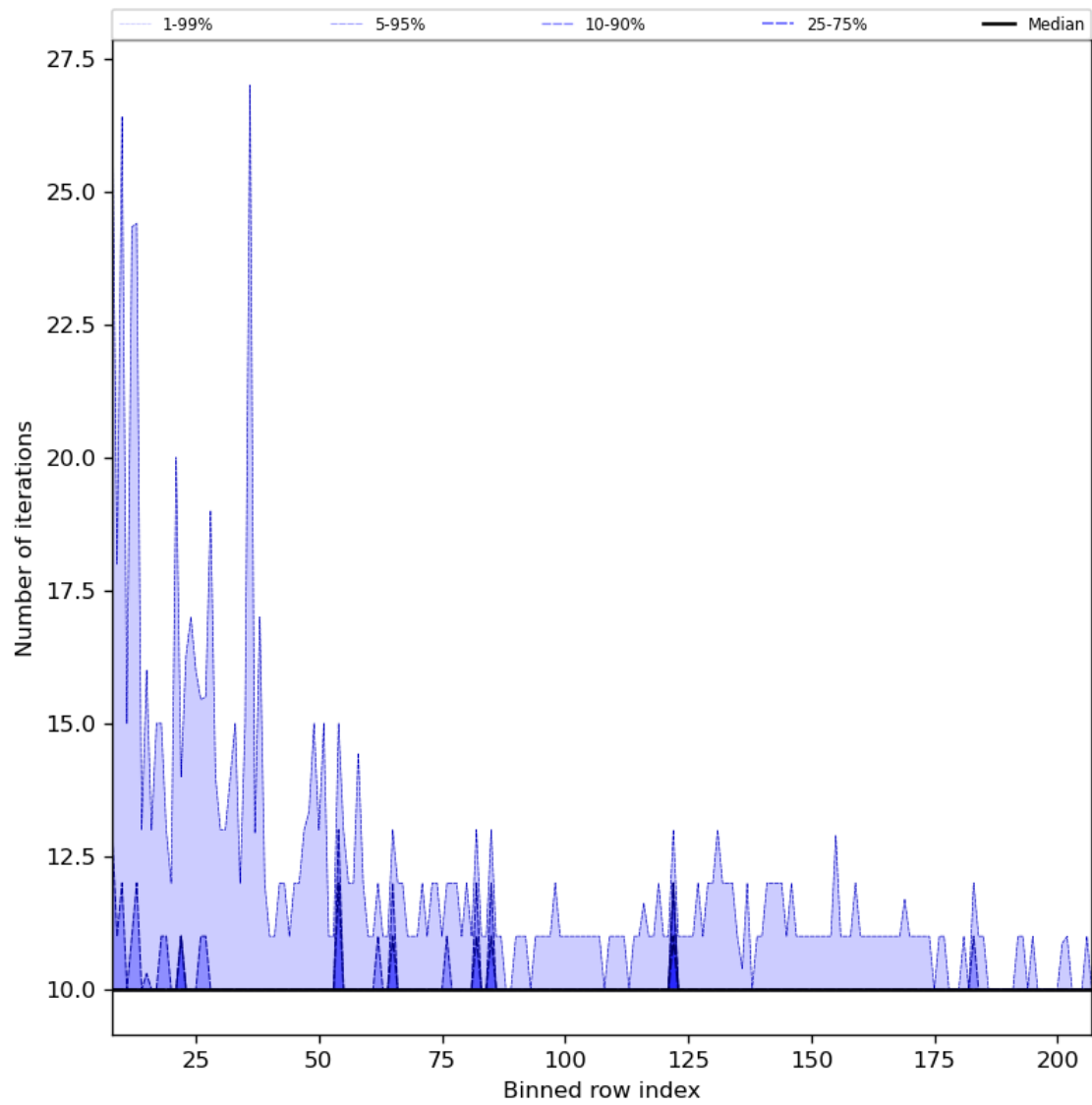
Figure 42: Along track statistics of “Number of iterations” for 2024-07-16 to 2024-07-18
