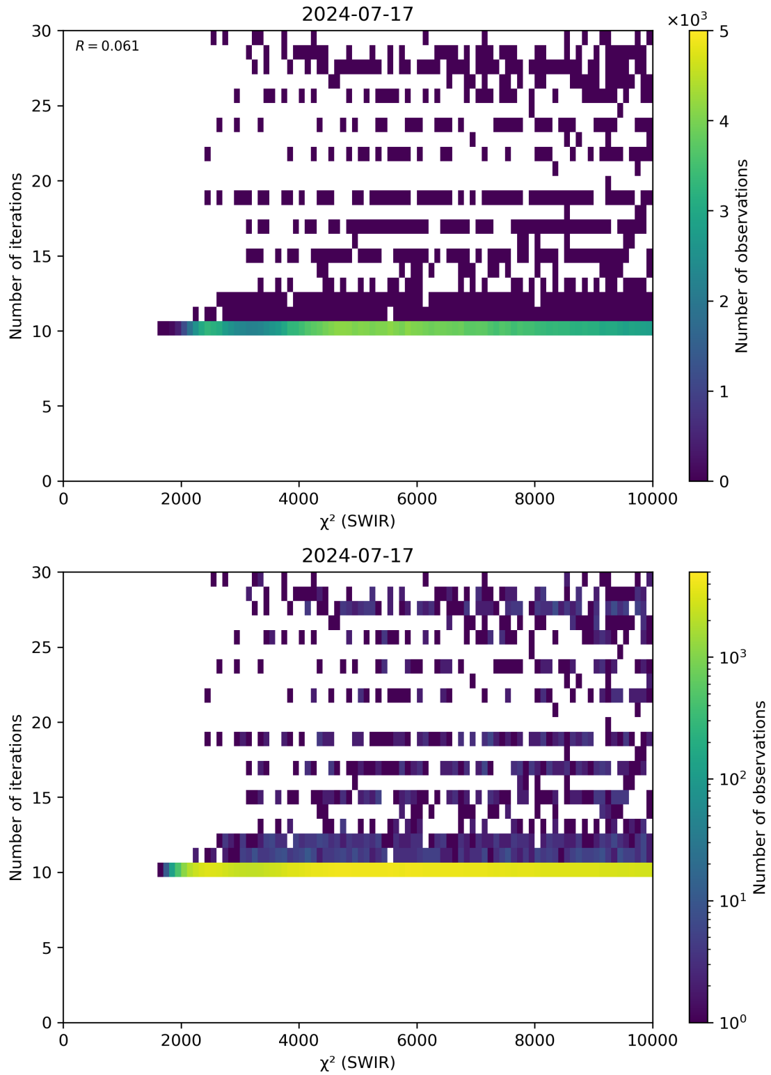
Figure 50: Scatter density plot of “ \chi^2 (SWIR)” against “Number of iterations” for 2024-07-16 to 2024-07-18.
