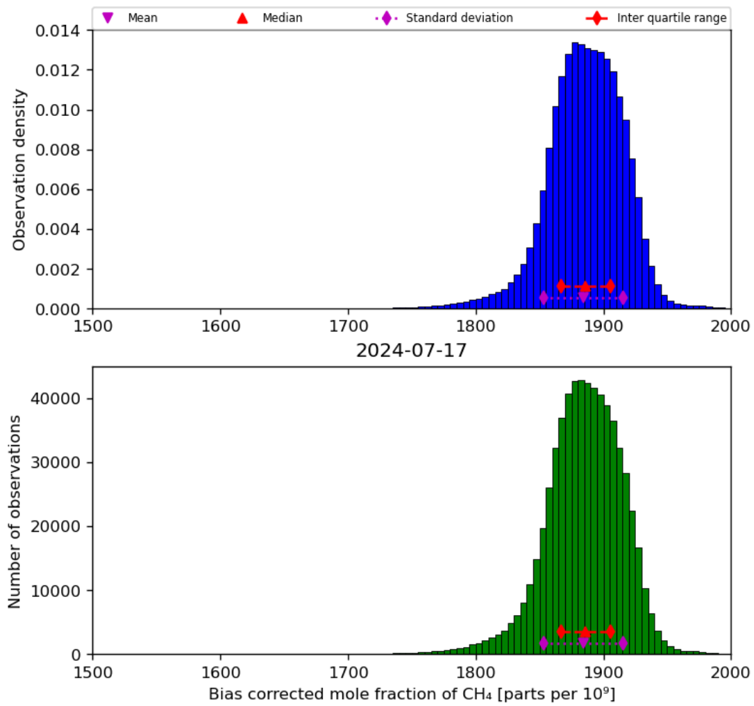
Figure 25: Histogram of “Bias corrected mole fraction of CH 4 ” for 2024-07-16 to 2024-07-18
