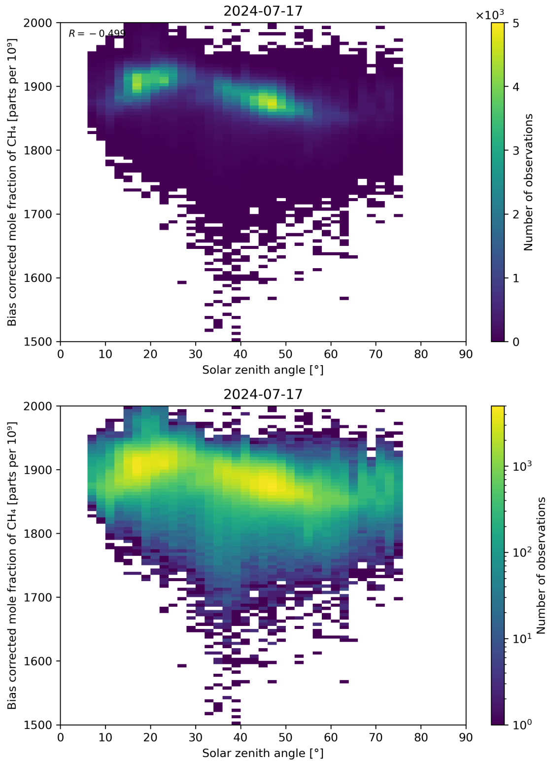
Figure 100: Scatter density plot of “Solar zenith angle” against “Bias corrected mole fraction of CH 4 ” for 2024-07-16 to 2024-07-18.
