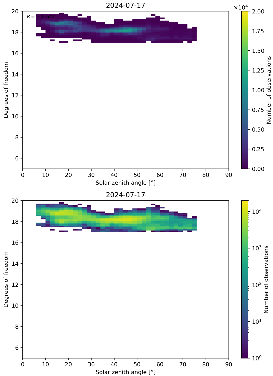
Figure 96: Scatter density plot of “Solar zenith angle” against “Degrees of freedom” for 2024-07-16 to 2024-07-18.
