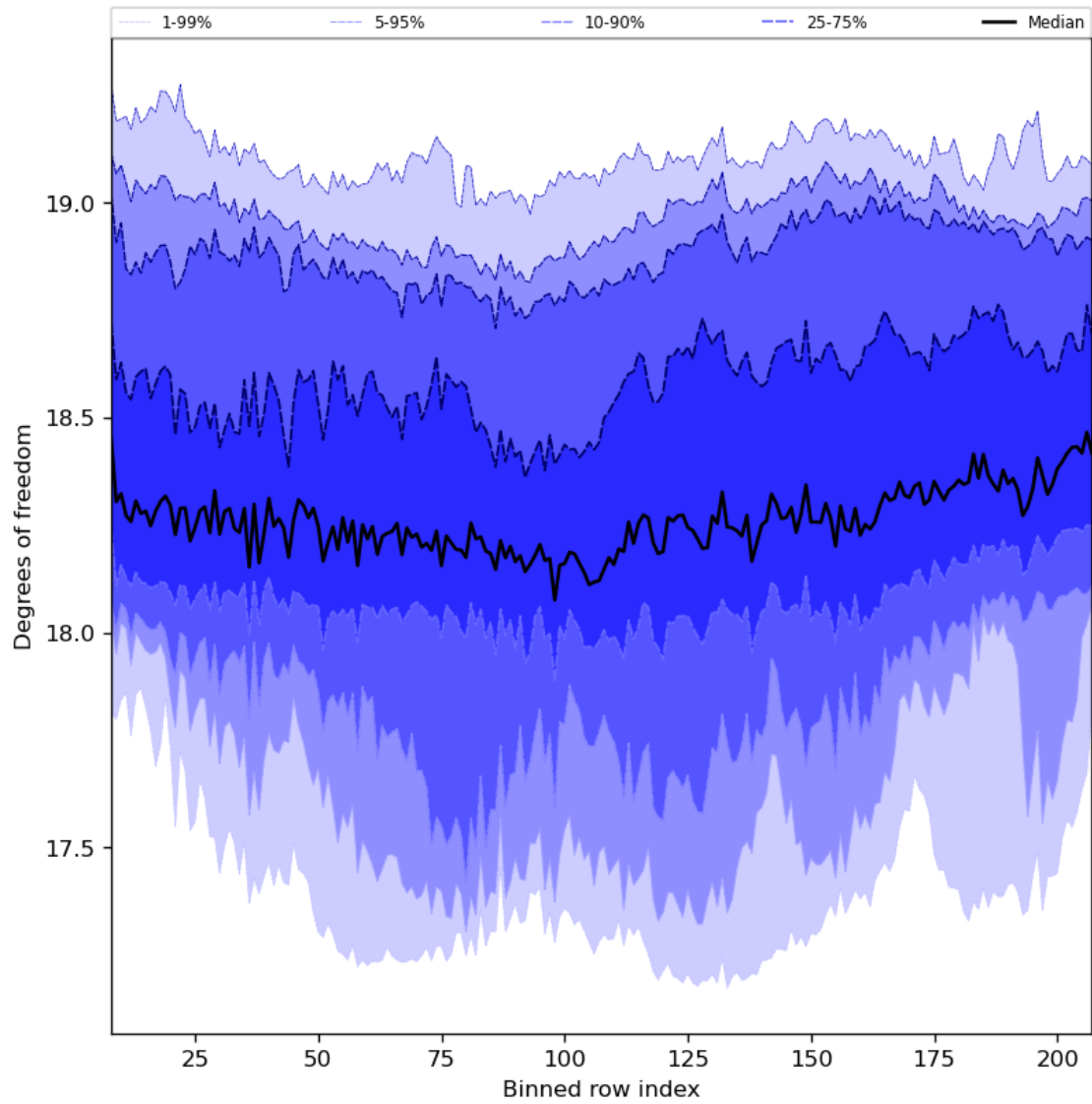
Figure 41: Along track statistics of “Degrees of freedom” for 2024-07-16 to 2024-07-18
