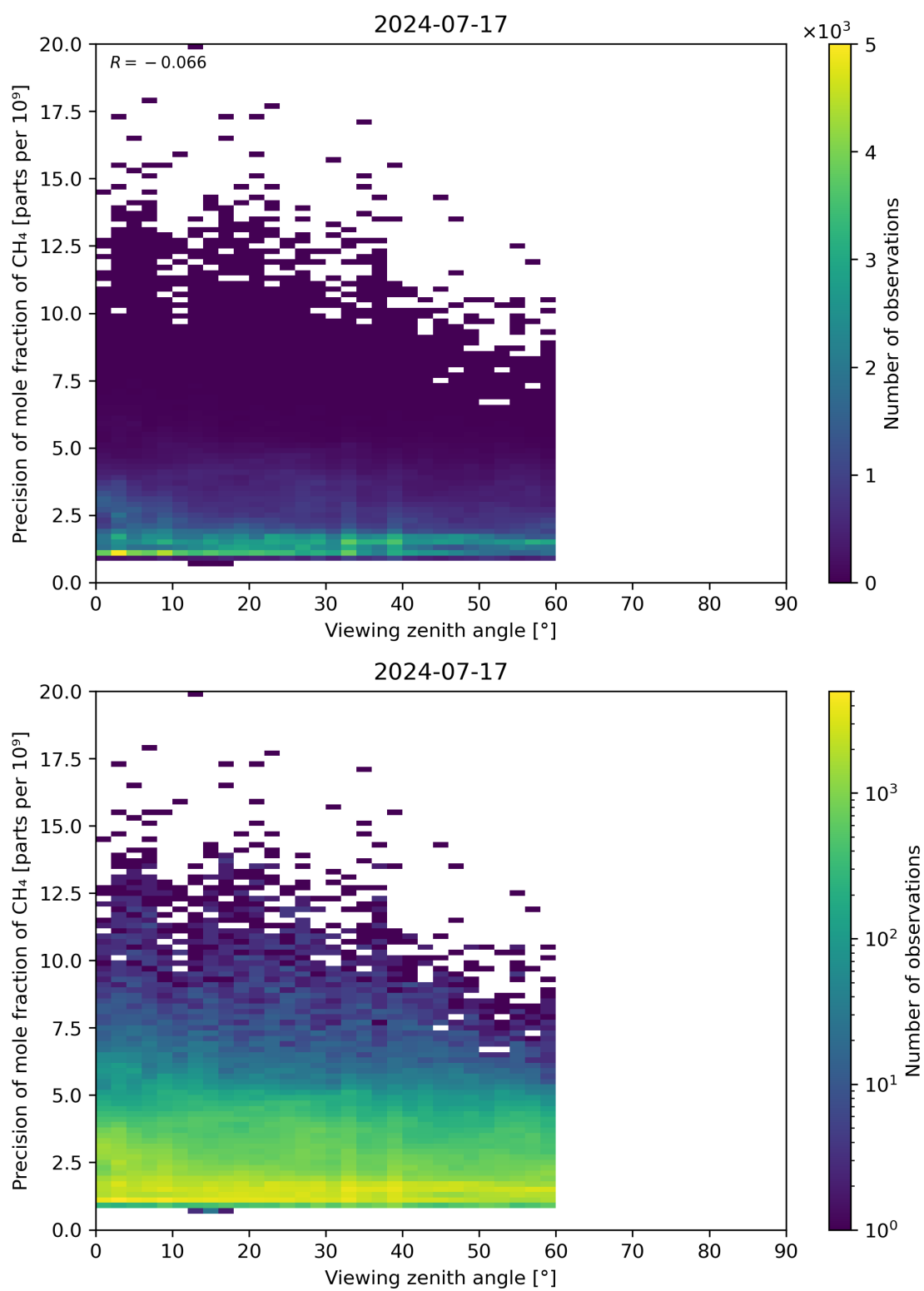
Figure 112: Scatter density plot of “Viewing zenith angle” against “Precision of mole fraction of \text{CH}_4 ” for 2024-07-16 to 2024-07-18.
