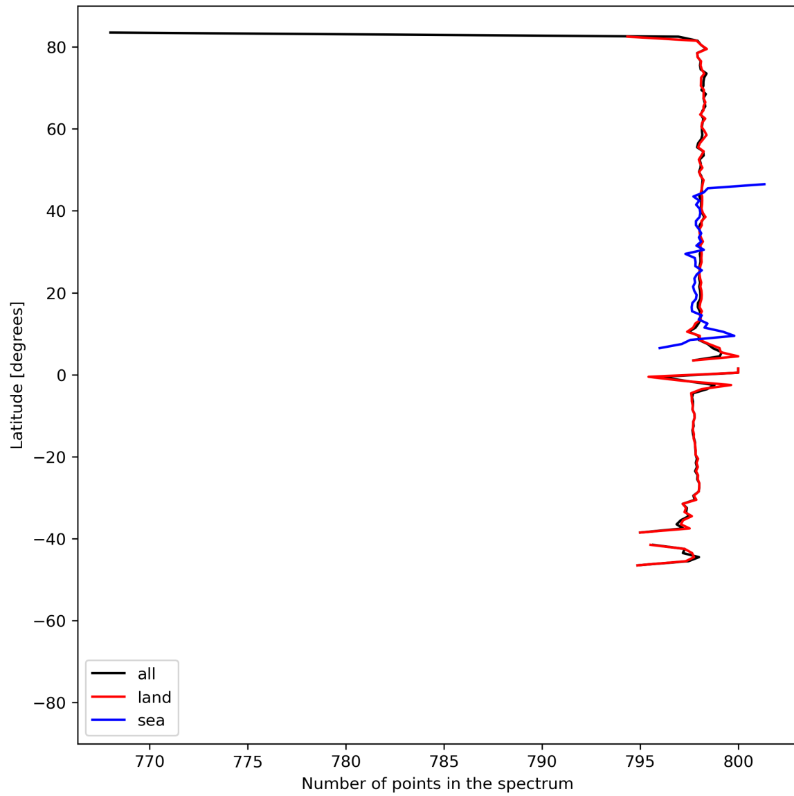
Figure 15: Zonal average of “Number of points in the spectrum” for 2024-07-16 to 2024-07-18.
