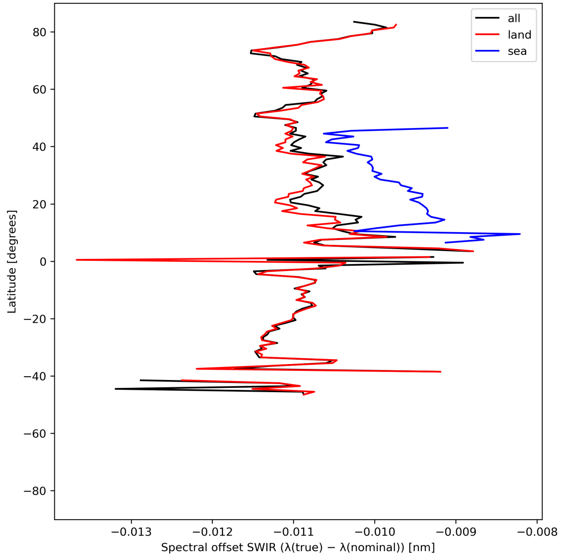
Figure 16: Zonal average of “Spectral offset SWIR ( \lambda(\text{true}) - \lambda(\text{nominal}) )” for 2024-07-16 to 2024-07-18.
