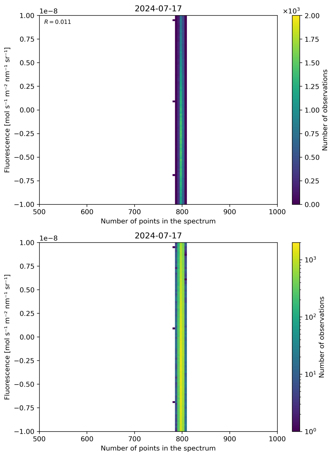
Figure 91: Scatter density plot of “Number of points in the spectrum” against “Fluorescence” for 2024-07-16 to 2024-07-18.
