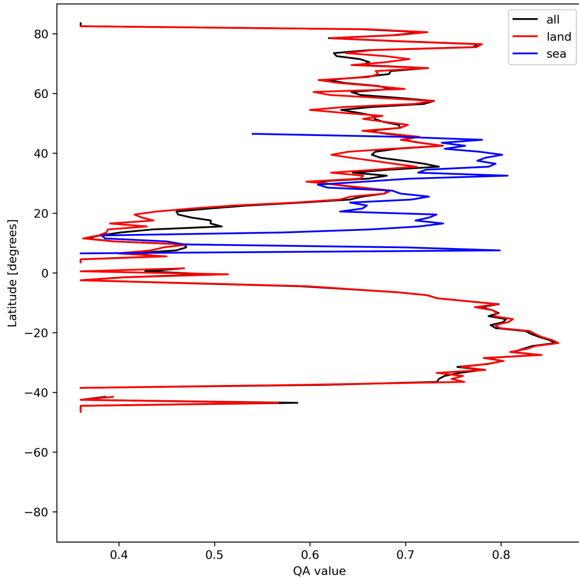
Figure 11: Zonal average of “QA value” for 2024-07-16 to 2024-07-18.
