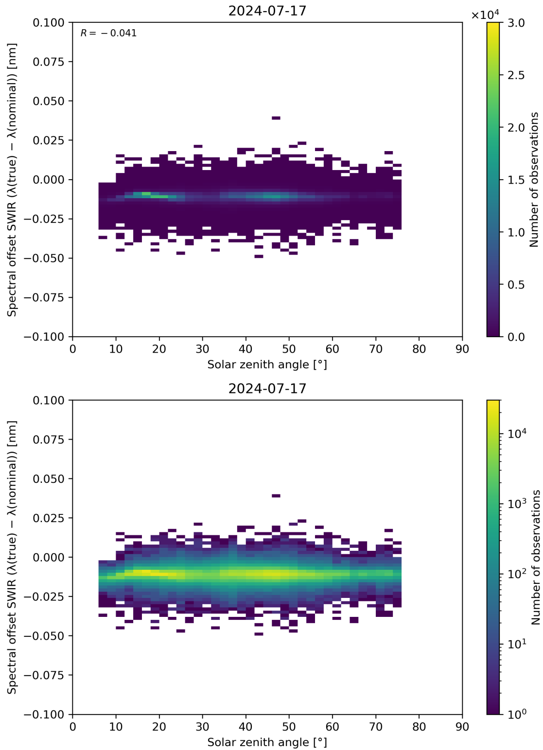
Figure 104: Scatter density plot of “Solar zenith angle” against “Spectral offset SWIR ( \lambda(\text{true}) - \lambda(\text{nominal}) )” for 2024-07-16 to 2024-07-18.
