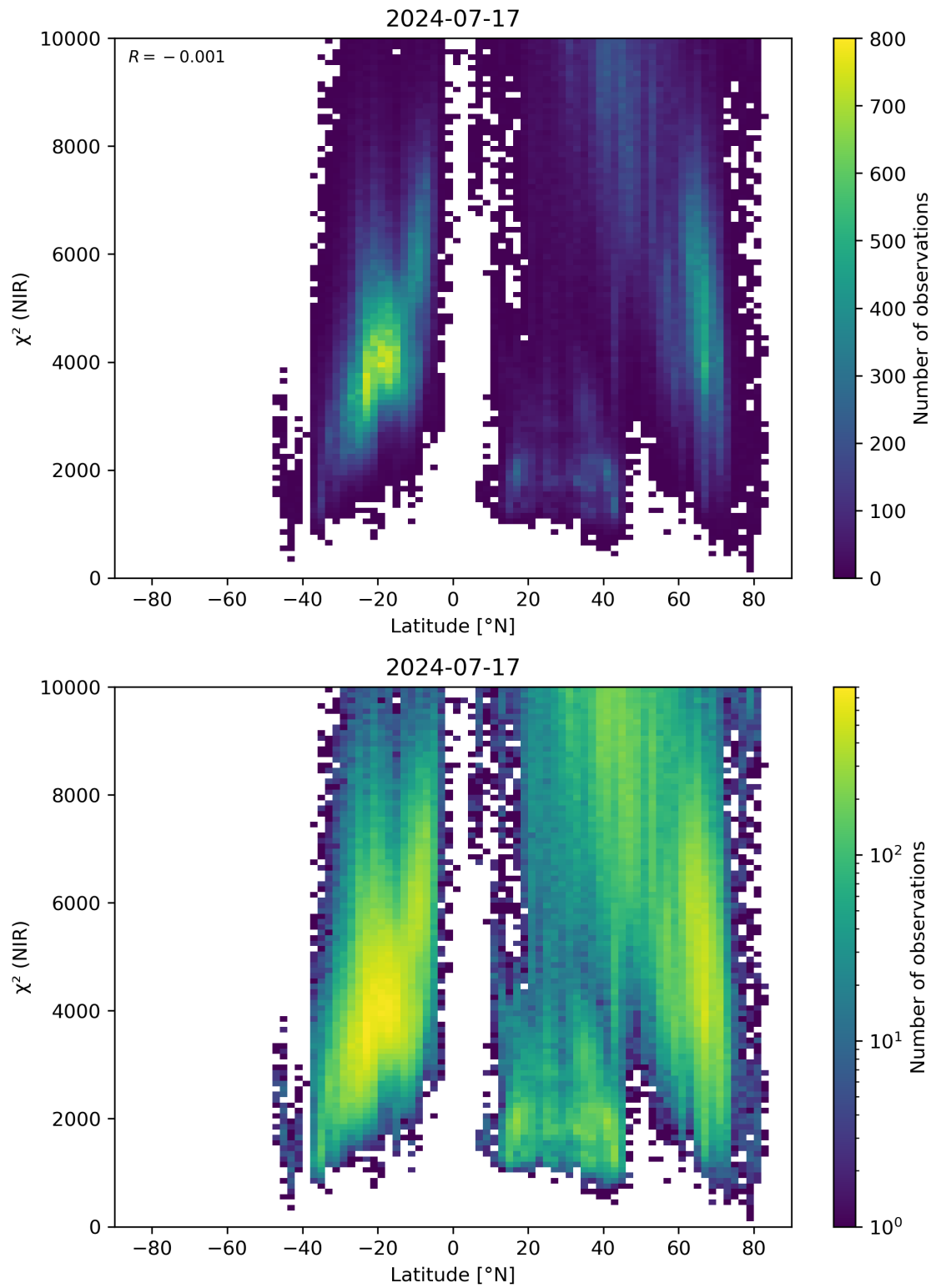
Figure 53: Scatter density plot of “Latitude” against “ \chi^2 (NIR)” for 2024-07-16 to 2024-07-18.
