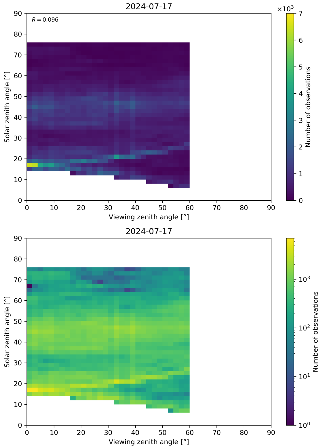
Figure 115: Scatter density plot of “Viewing zenith angle” against “Solar zenith angle” for 2024-07-16 to 2024-07-18.
