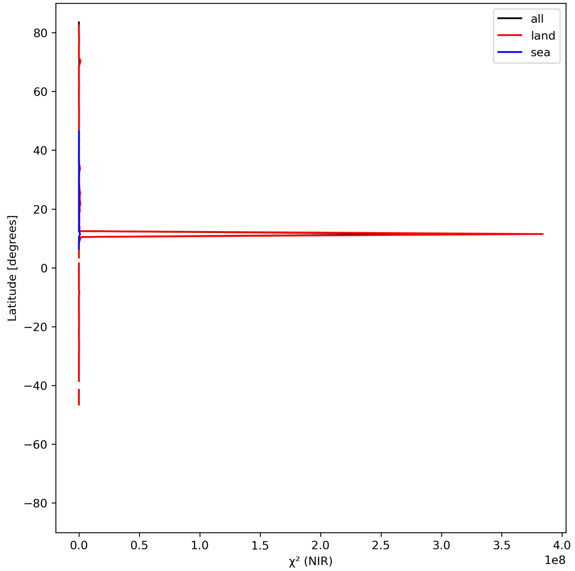
Figure 18: Zonal average of “ \chi^2 (NIR)” for 2024-07-16 to 2024-07-18.
