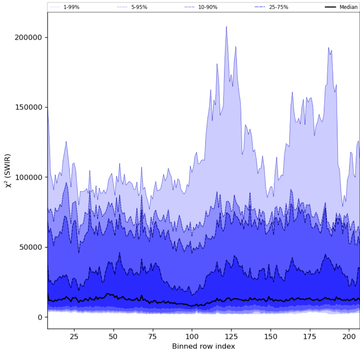
Figure 39: Along track statistics of “ \chi^2 (SWIR)” for 2024-07-16 to 2024-07-18
