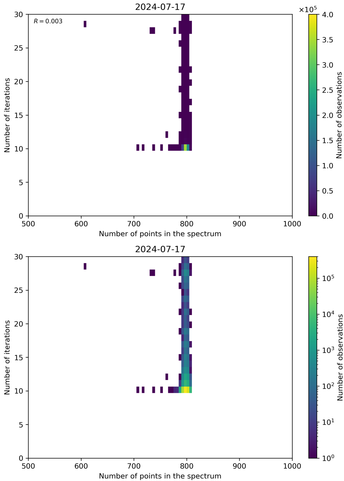
Figure 92: Scatter density plot of “Number of points in the spectrum” against “Number of iterations” for 2024-07-16 to 2024-07-18.
