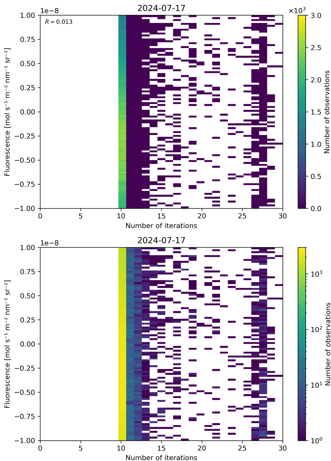
Figure 87: Scatter density plot of “Number of iterations” against “Fluorescence” for 2024-07-16 to 2024-07-18.
