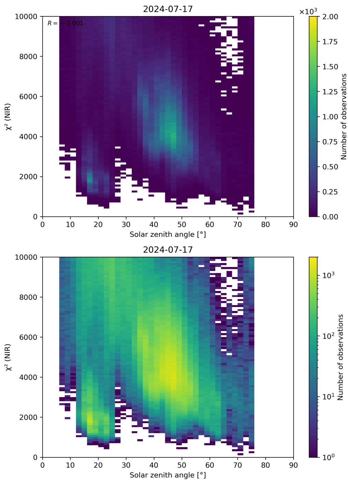
Figure 94: Scatter density plot of “Solar zenith angle” against “ \chi^2 (NIR)” for 2024-07-16 to 2024-07-18.
