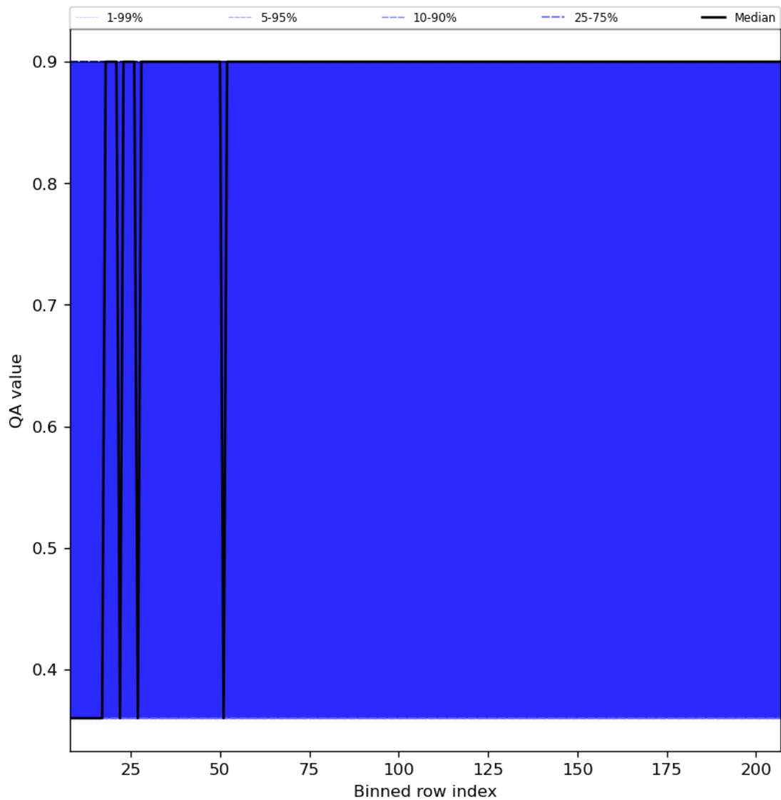
Figure 33: Along track statistics of “QA value” for 2024-07-16 to 2024-07-18
