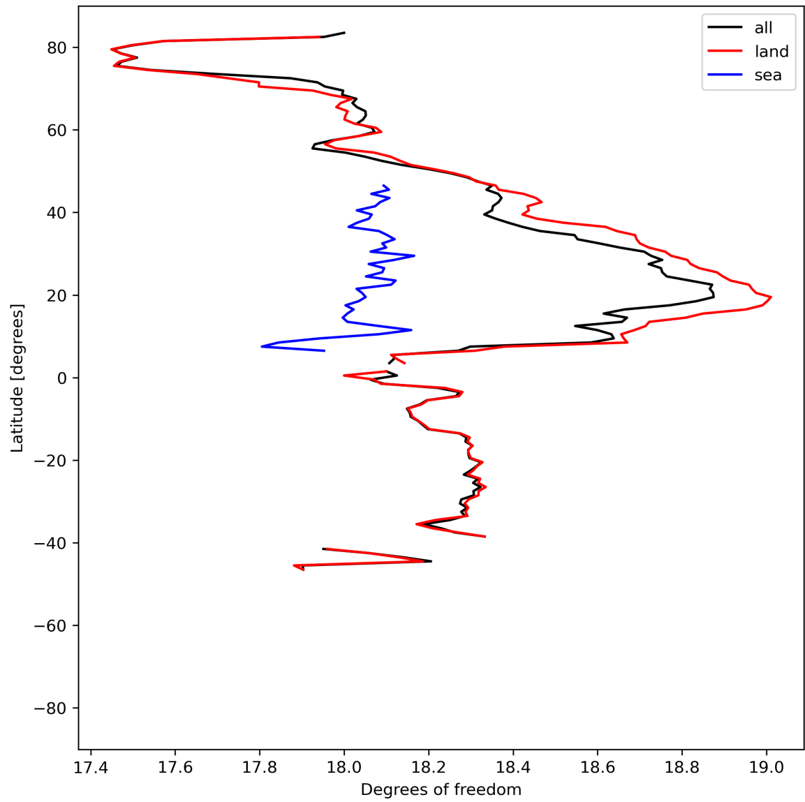
Figure 19: Zonal average of “Degrees of freedom” for 2024-07-16 to 2024-07-18.
