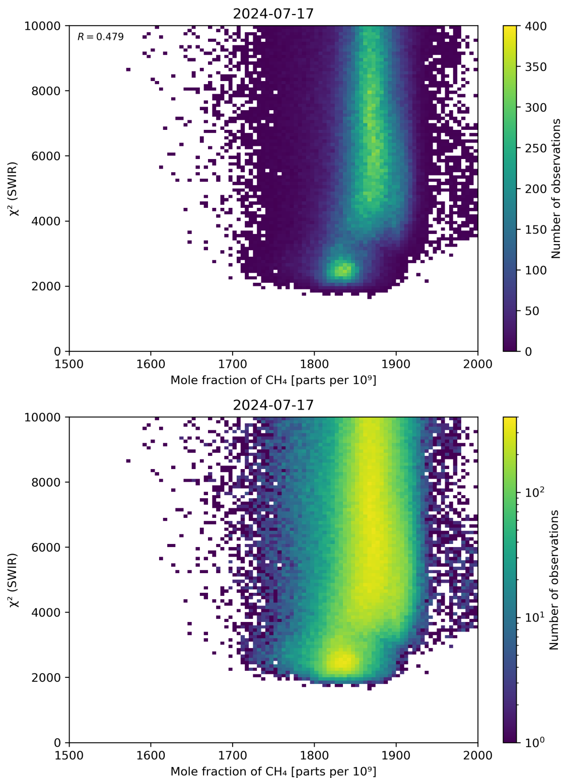
Figure 71: Scatter density plot of “Mole fraction of \text{CH}_4 ” against “ \chi^2 (SWIR)” for 2024-07-16 to 2024-07-18.
