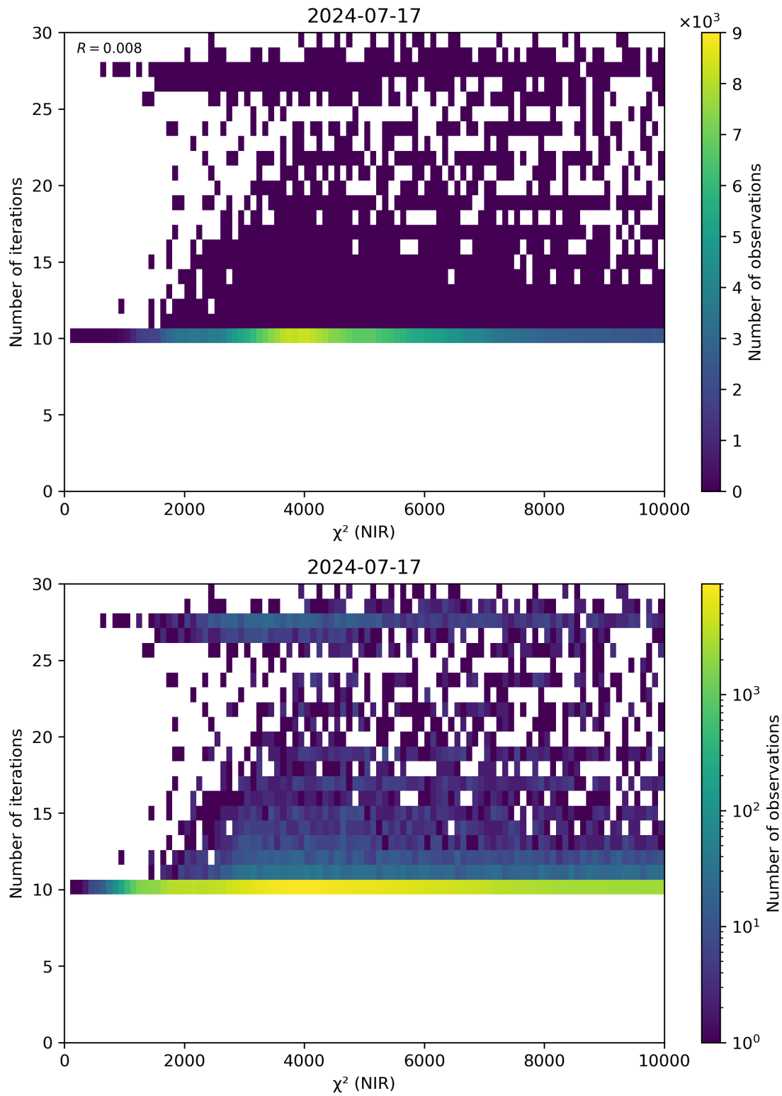
Figure 46: Scatter density plot of “ \chi^2 (NIR)” against “Number of iterations” for 2024-07-16 to 2024-07-18.
