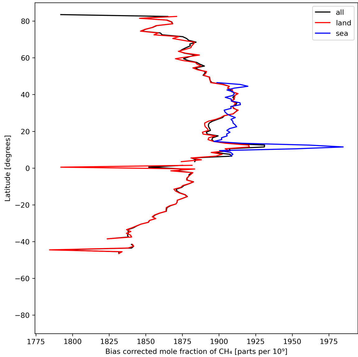
Figure 14: Zonal average of “Bias corrected mole fraction of CH 4 ” for 2024-07-16 to 2024-07-18.
