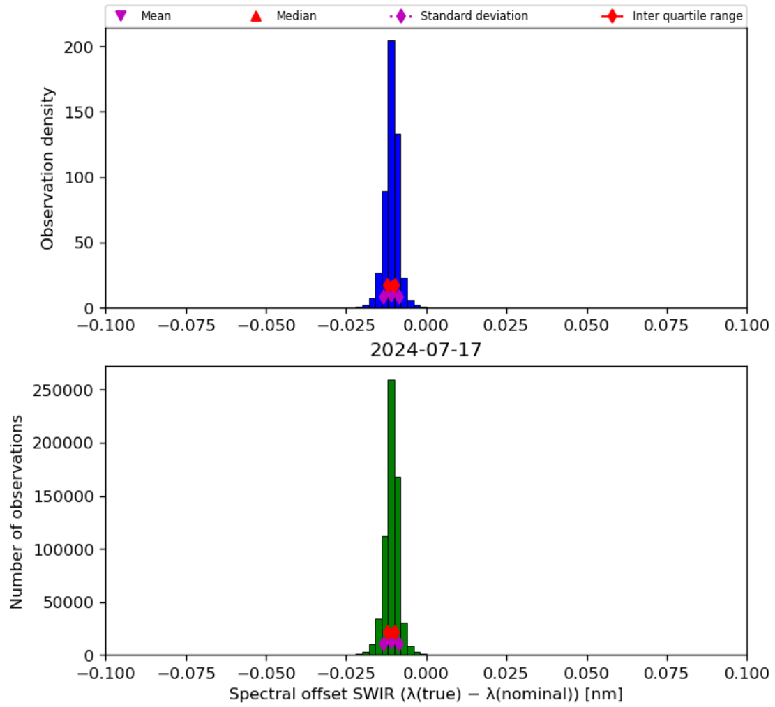
Figure 27: Histogram of “Spectral offset SWIR ( \lambda(\text{true}) - \lambda(\text{nominal}) )” for 2024-07-16 to 2024-07-18
