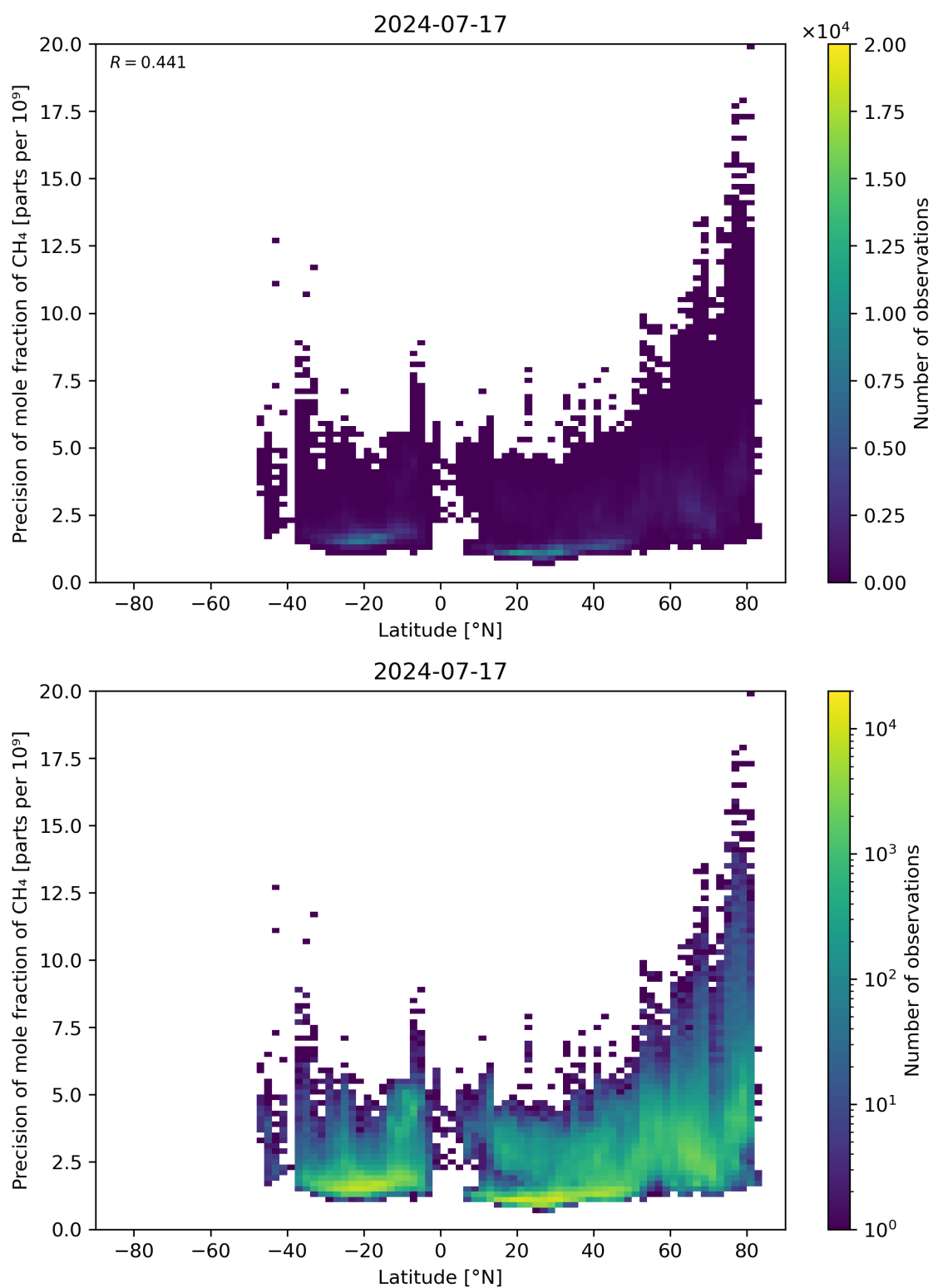
Figure 59: Scatter density plot of “Latitude” against “Precision of mole fraction of \text{CH}_4 ” for 2024-07-16 to 2024-07-18.
