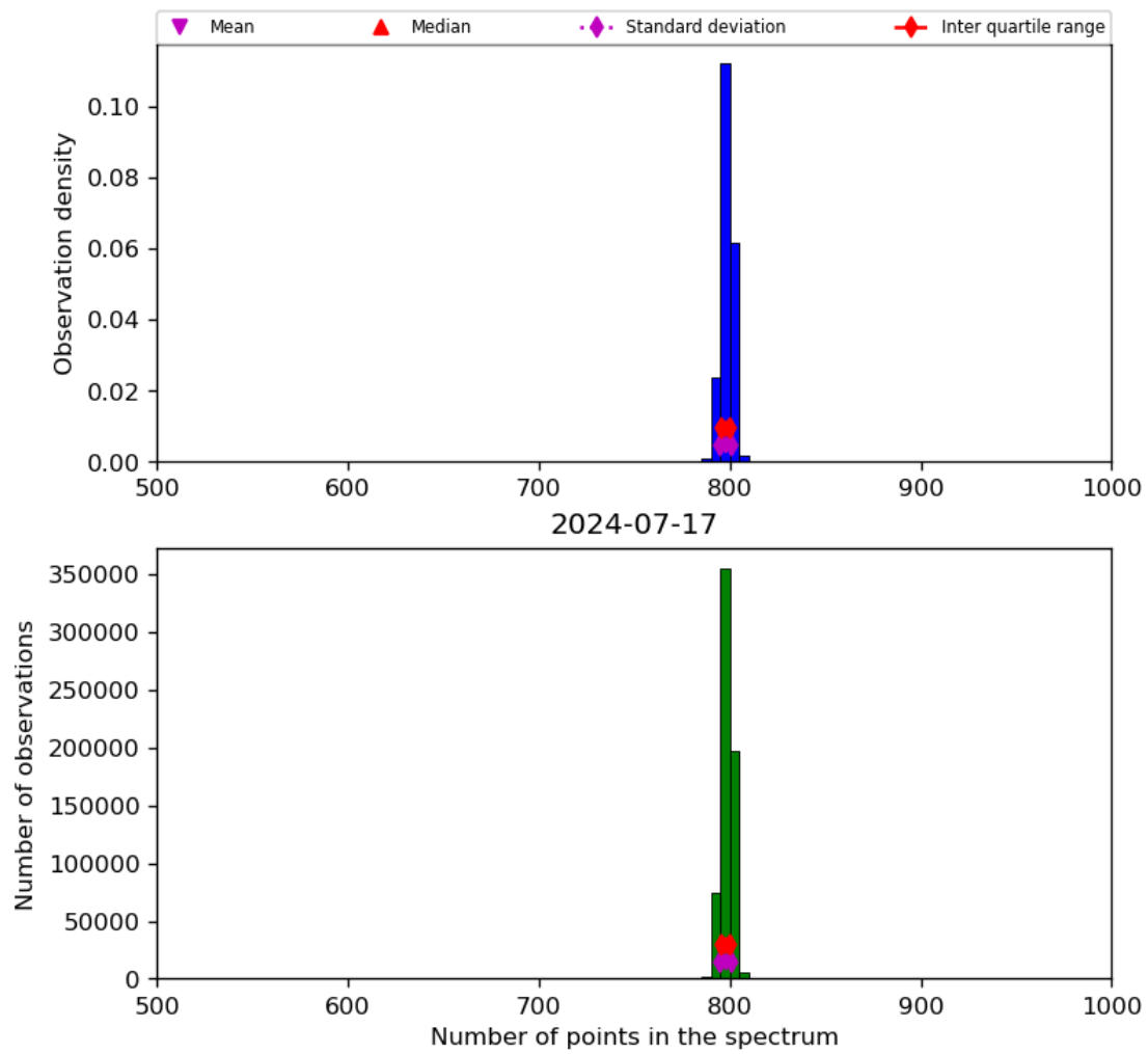
Figure 26: Histogram of “Number of points in the spectrum” for 2024-07-16 to 2024-07-18
