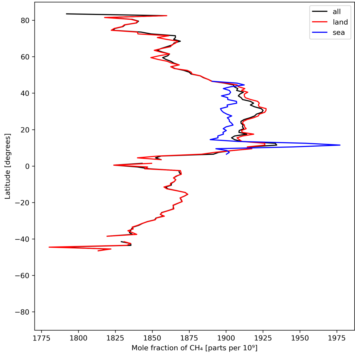
Figure 12: Zonal average of “Mole fraction of \text{CH}_4 ” for 2024-07-16 to 2024-07-18.
