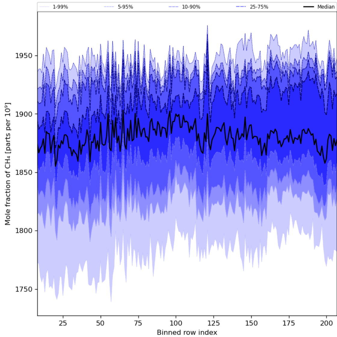
Figure 34: Along track statistics of “Mole fraction of CH 4 ” for 2024-07-16 to 2024-07-18
