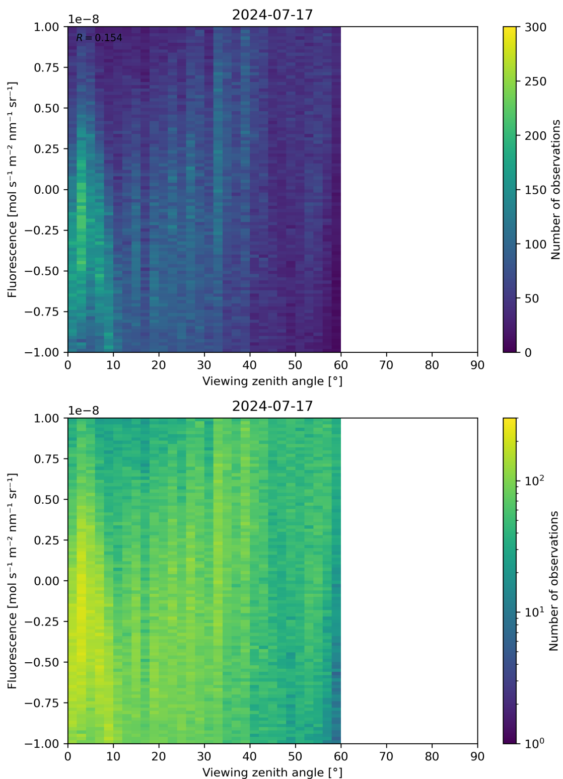
Figure 108: Scatter density plot of “Viewing zenith angle” against “Fluorescence” for 2024-07-16 to 2024-07-18.
