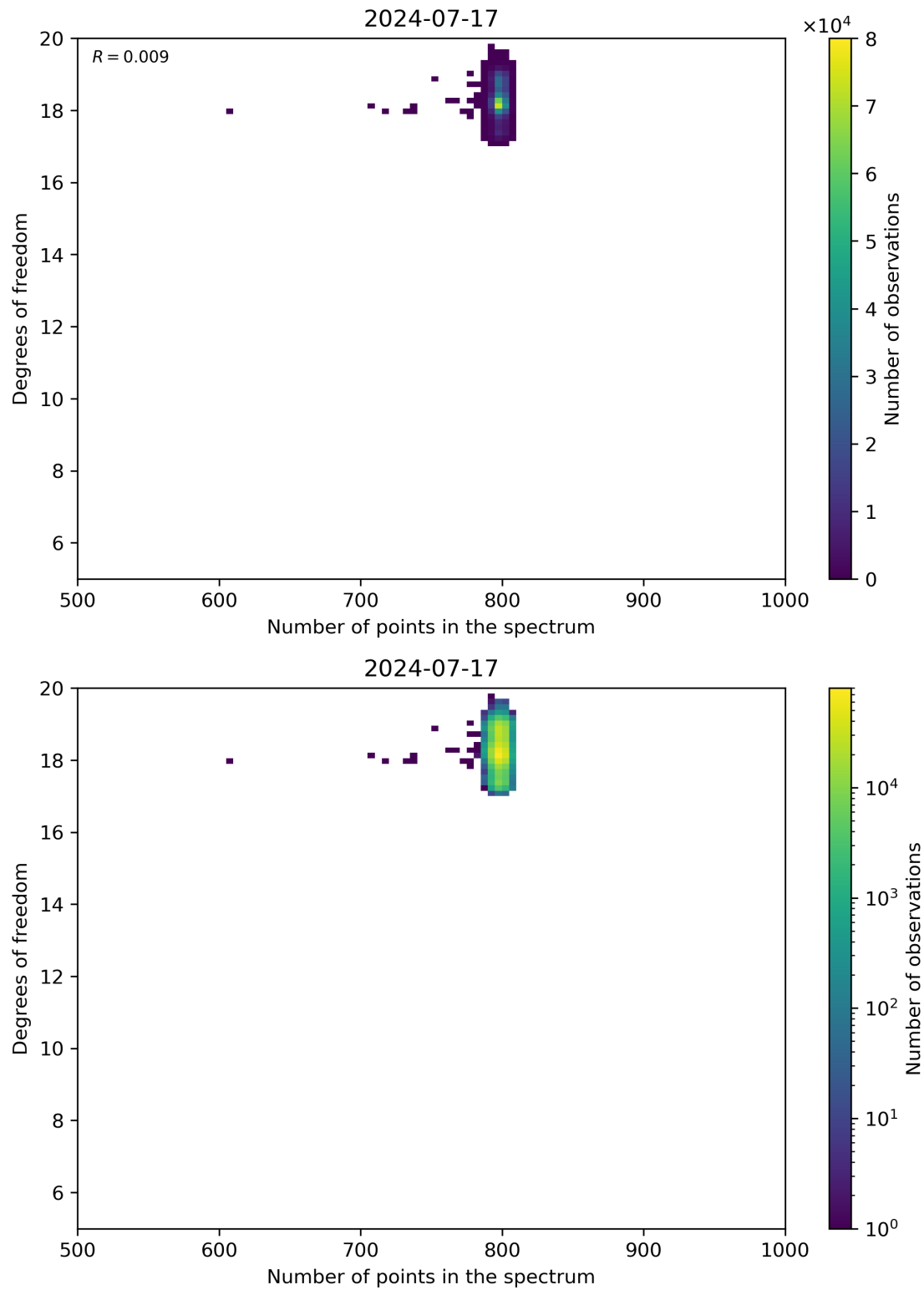
Figure 90: Scatter density plot of “Number of points in the spectrum” against “Degrees of freedom” for 2024-07-16 to 2024-07-18.
