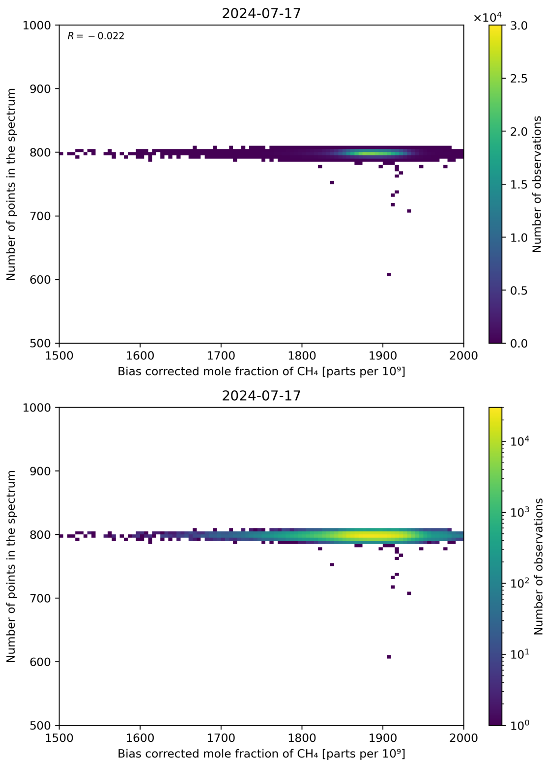
Figure 68: Scatter density plot of “Bias corrected mole fraction of CH 4 ” against “Number of points in the spectrum” for 2024-07-16 to 2024-07-18.
