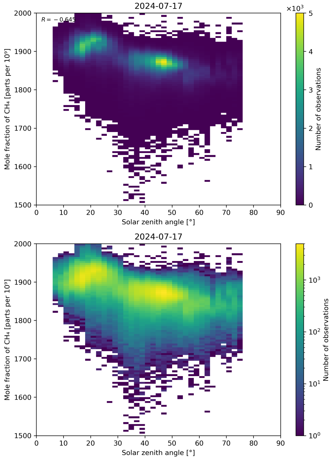
Figure 99: Scatter density plot of “Solar zenith angle” against “Mole fraction of CH 4 ” for 2024-07-16 to 2024-07-18.
