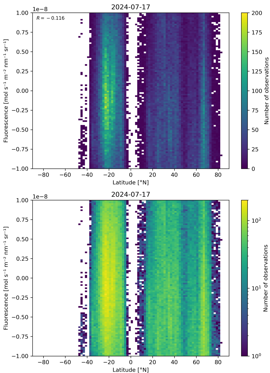
Figure 56: Scatter density plot of “Latitude” against “Fluorescence” for 2024-07-16 to 2024-07-18.
