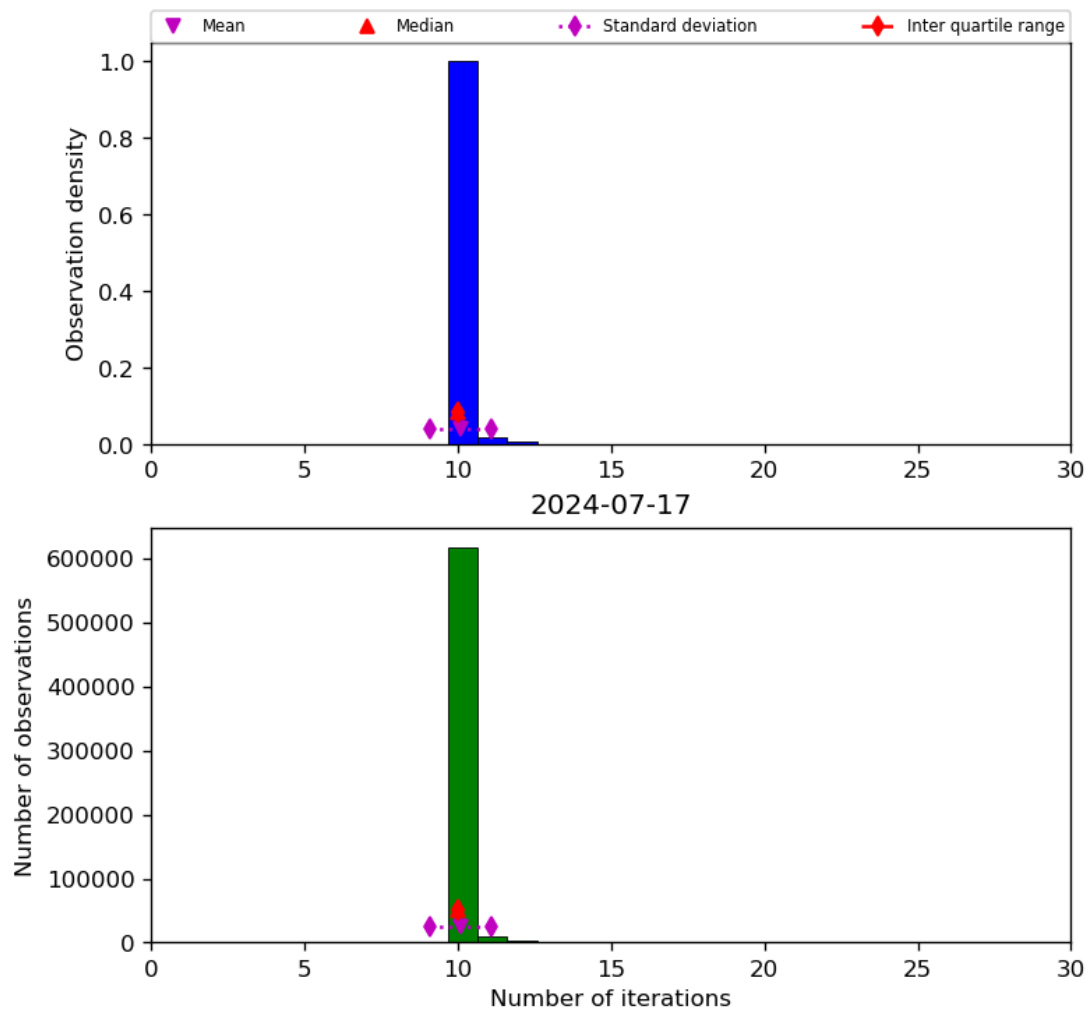
Figure 31: Histogram of “Number of iterations” for 2024-07-16 to 2024-07-18
