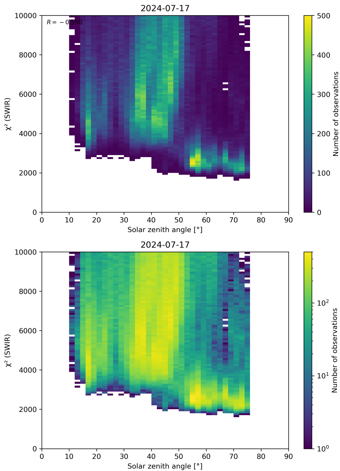
Figure 95: Scatter density plot of “Solar zenith angle” against “ \chi^2 (SWIR)” for 2024-07-16 to 2024-07-18.
