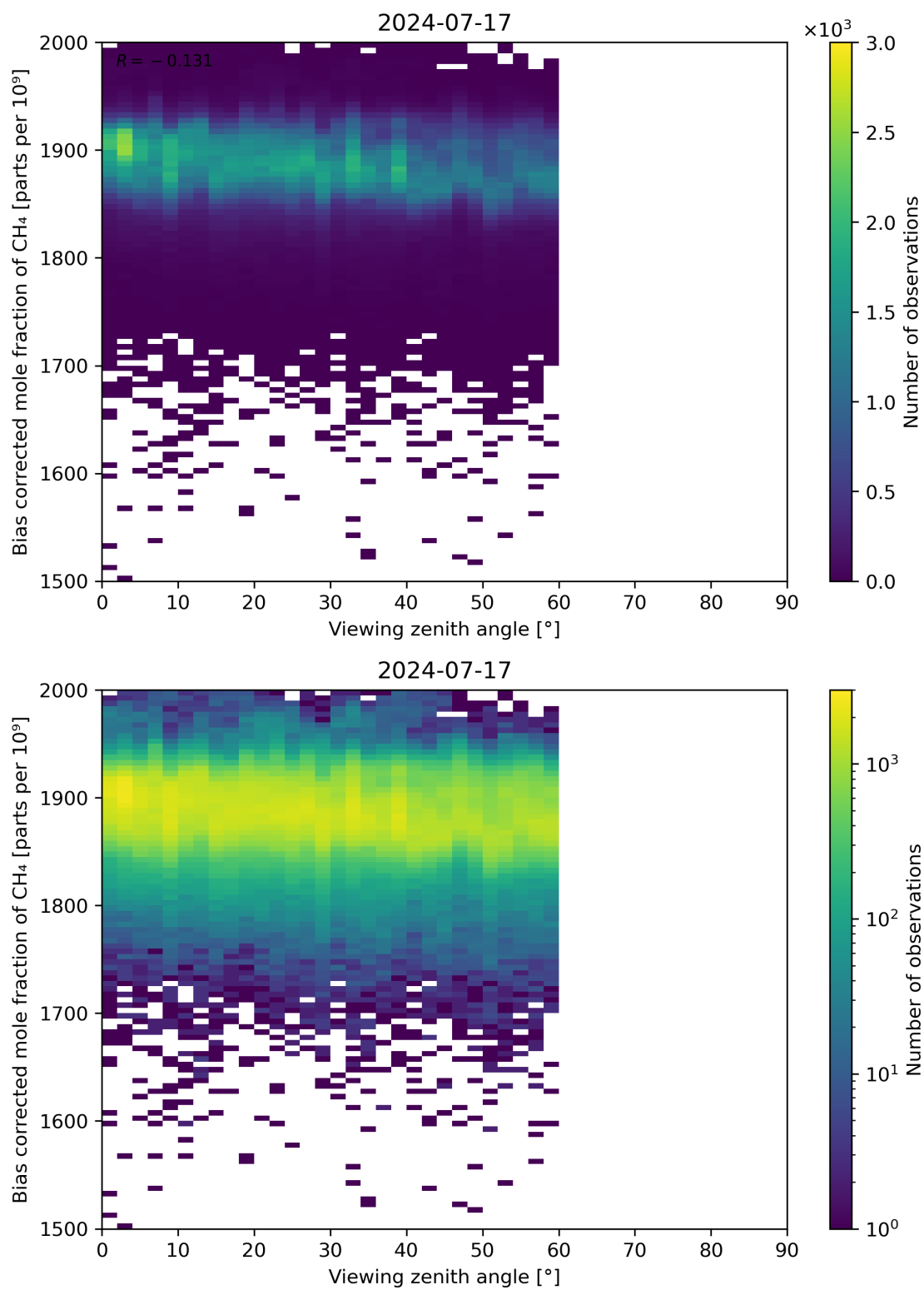
Figure 111: Scatter density plot of “Viewing zenith angle” against “Bias corrected mole fraction of CH 4 ” for 2024-07-16 to 2024-07-18.
