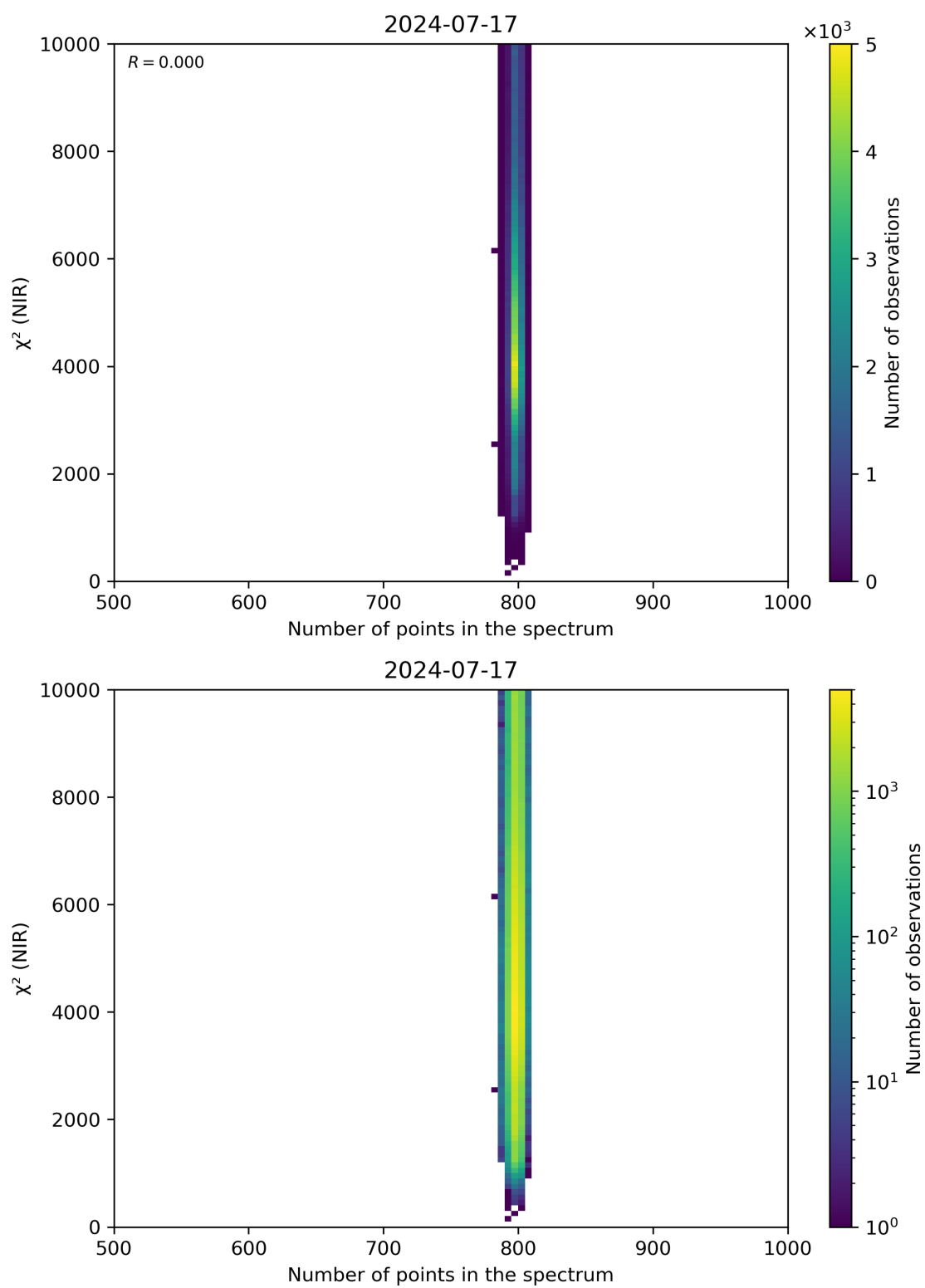
Figure 88: Scatter density plot of “Number of points in the spectrum” against “ \chi^2 (NIR)” for 2024-07-16 to 2024-07-18.
