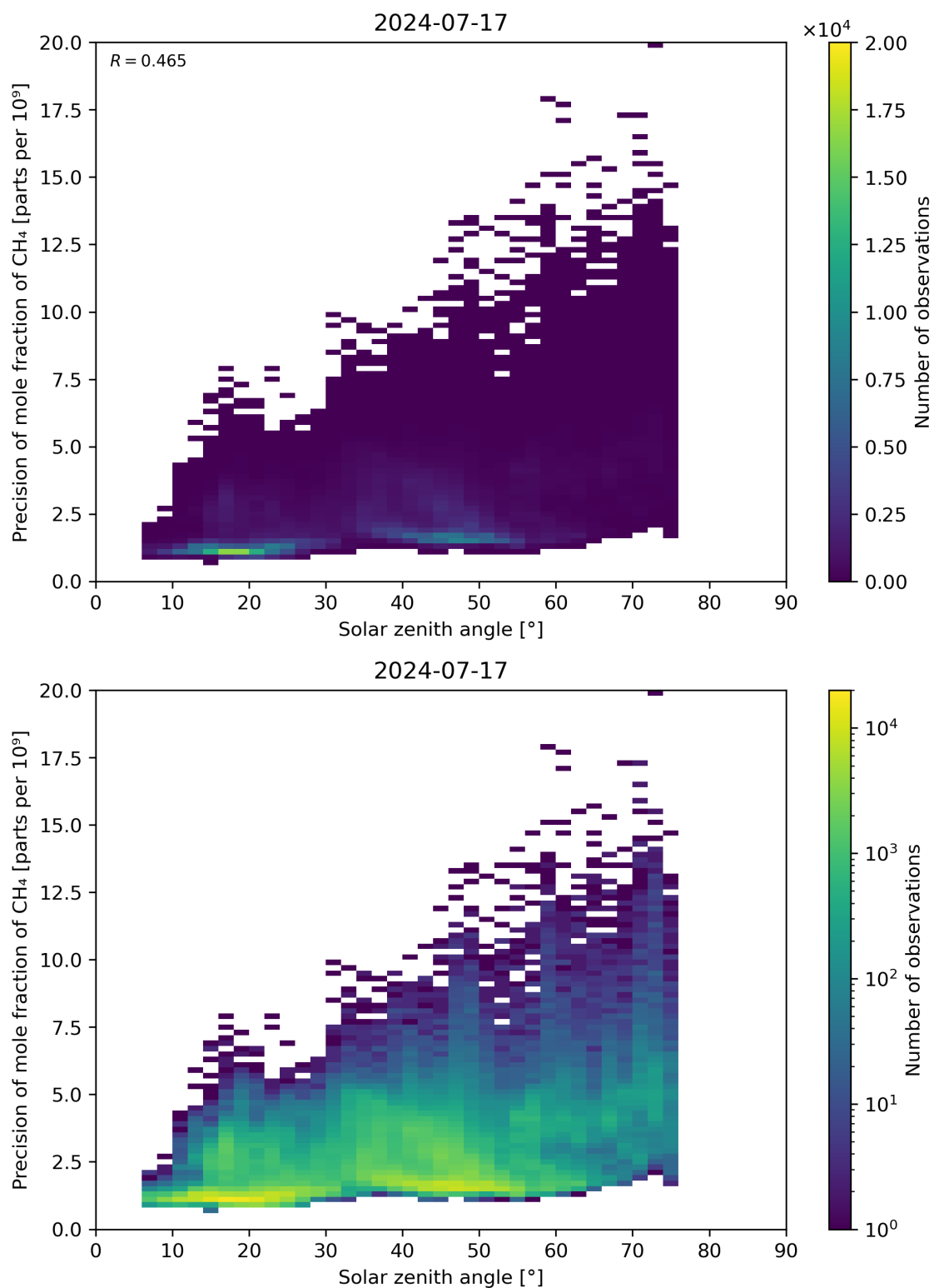
Figure 101: Scatter density plot of “Solar zenith angle” against “Precision of mole fraction of CH 4 ” for 2024-07-16 to 2024-07-18.
