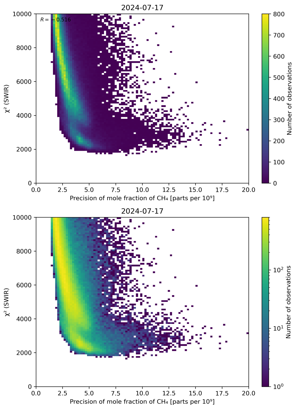
Figure 79: Scatter density plot of “Precision of mole fraction of \text{CH}_4 ” against “ \chi^2 (SWIR)” for 2024-07-16 to 2024-07-18.
