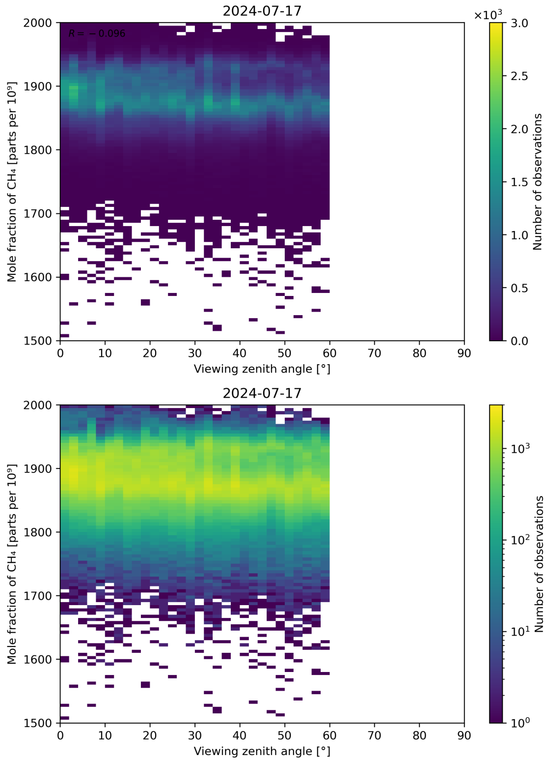
Figure 110: Scatter density plot of “Viewing zenith angle” against “Mole fraction of CH 4 ” for 2024-07-16 to 2024-07-18.
