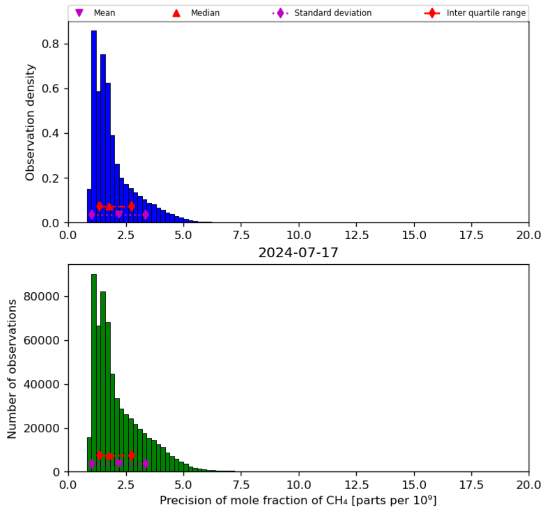
Figure 24: Histogram of “Precision of mole fraction of CH 4 ” for 2024-07-16 to 2024-07-18
