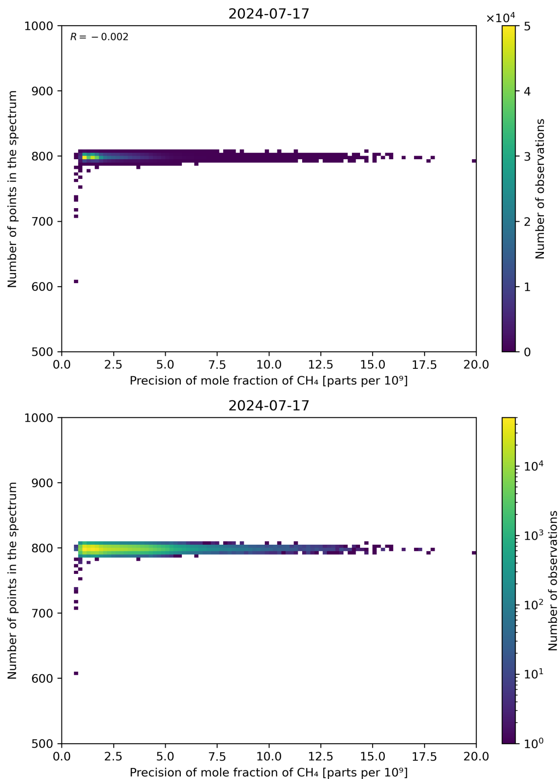
Figure 84: Scatter density plot of “Precision of mole fraction of CH 4 ” against “Number of points in the spectrum” for 2024-07-16 to 2024-07-18.
