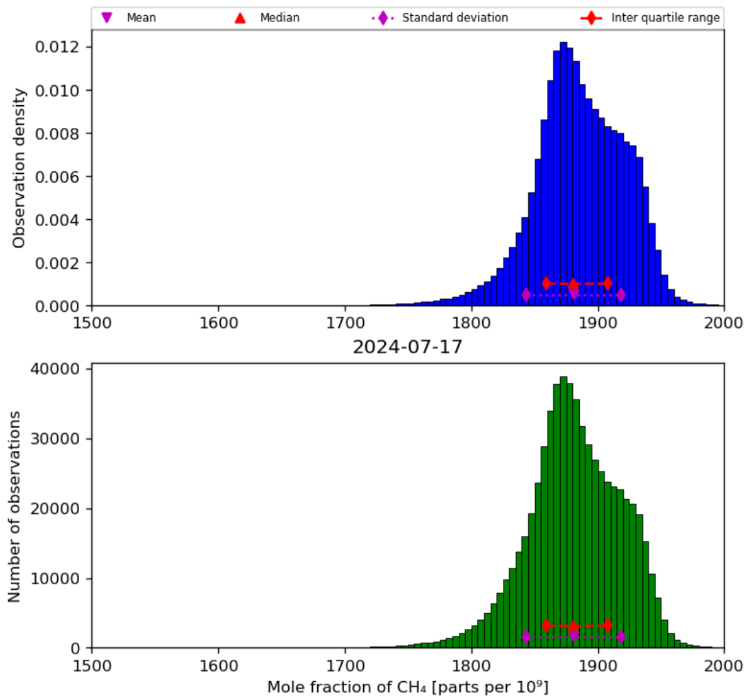
Figure 23: Histogram of “Mole fraction of CH 4 ” for 2024-07-16 to 2024-07-18
