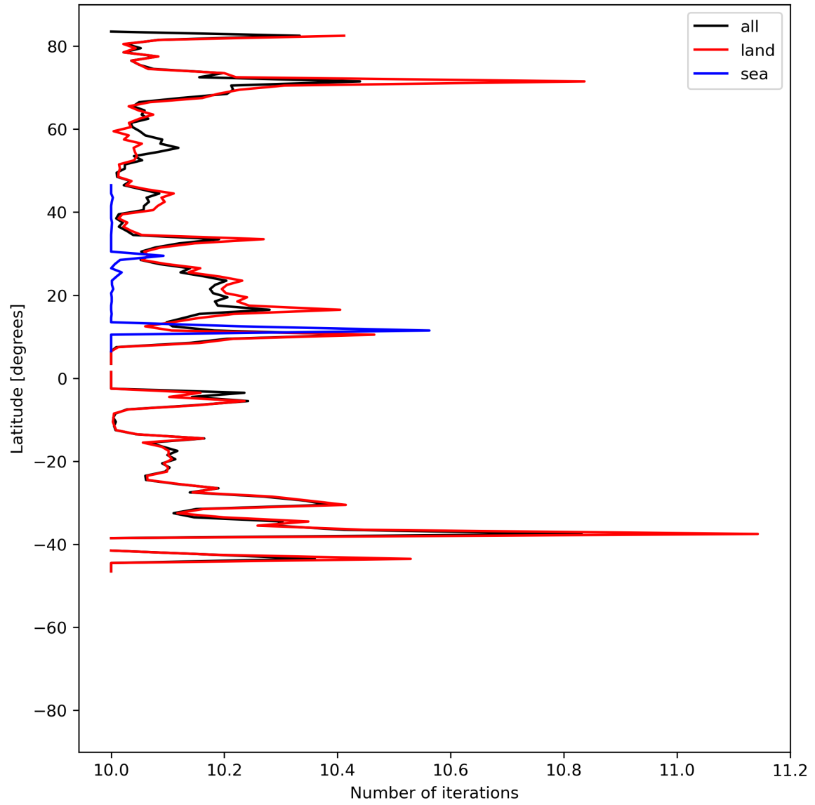
Figure 20: Zonal average of “Number of iterations” for 2024-07-16 to 2024-07-18.
