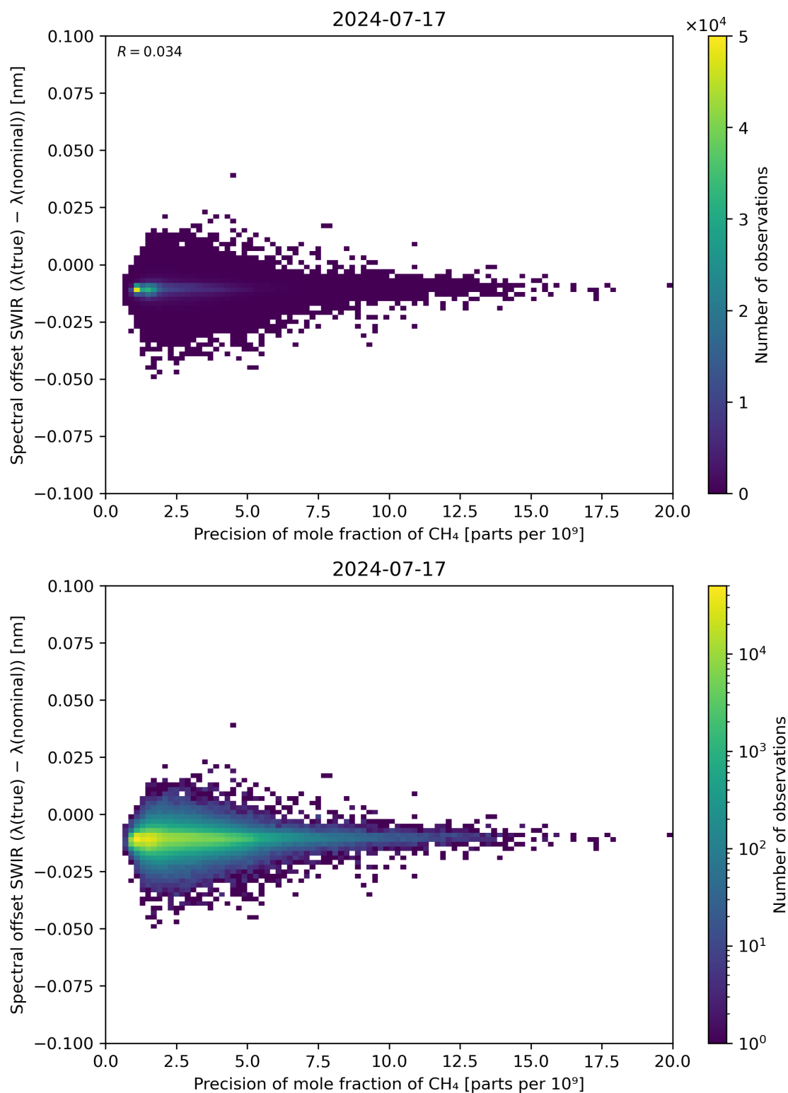
Figure 85: Scatter density plot of “Precision of mole fraction of CH 4 ” against “Spectral offset SWIR ( \lambda(\text{true}) - \lambda(\text{nominal}) )” for 2024-07-16 to 2024-07-18.
