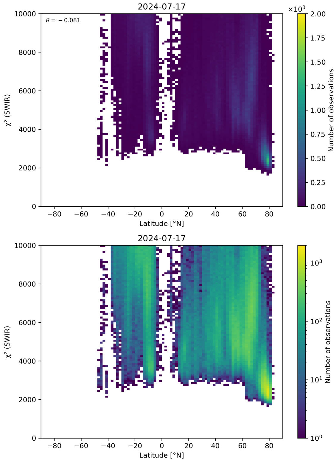
Figure 54: Scatter density plot of “Latitude” against “ \chi^2 (SWIR)” for 2024-07-16 to 2024-07-18.
