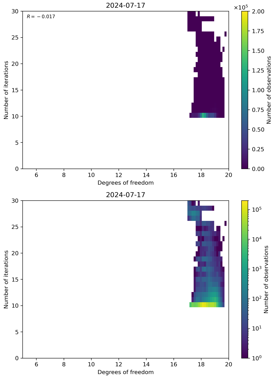
Figure 52: Scatter density plot of “Degrees of freedom” against “Number of iterations” for 2024-07-16 to 2024-07-18.
