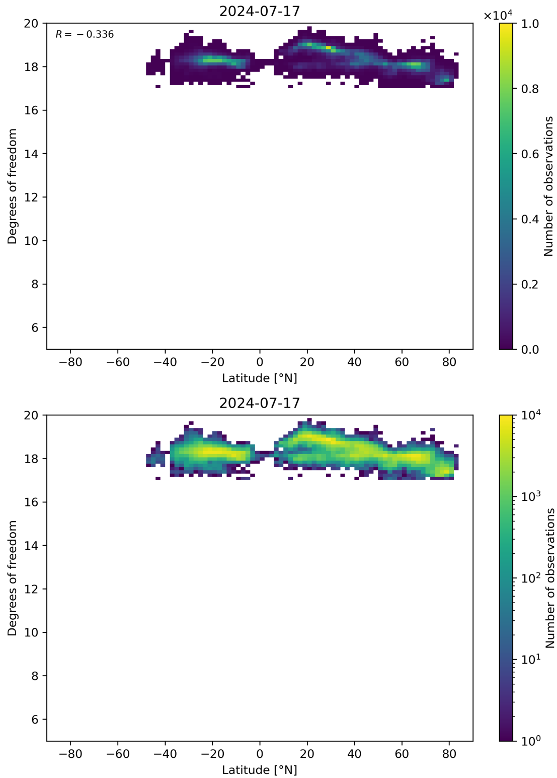
Figure 55: Scatter density plot of “Latitude” against “Degrees of freedom” for 2024-07-16 to 2024-07-18.
