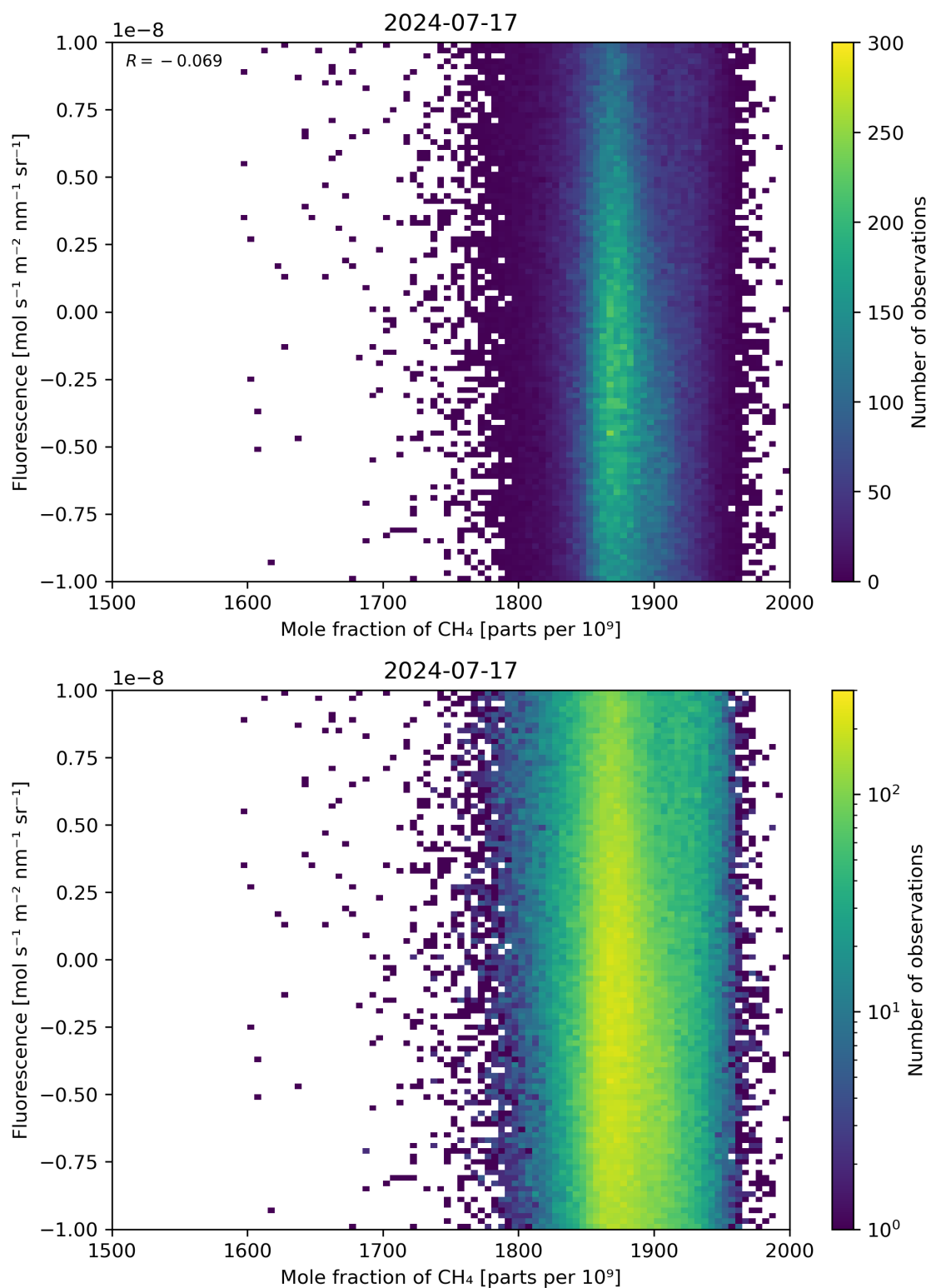
Figure 73: Scatter density plot of “Mole fraction of \text{CH}_4 ” against “Fluorescence” for 2024-07-16 to 2024-07-18.
