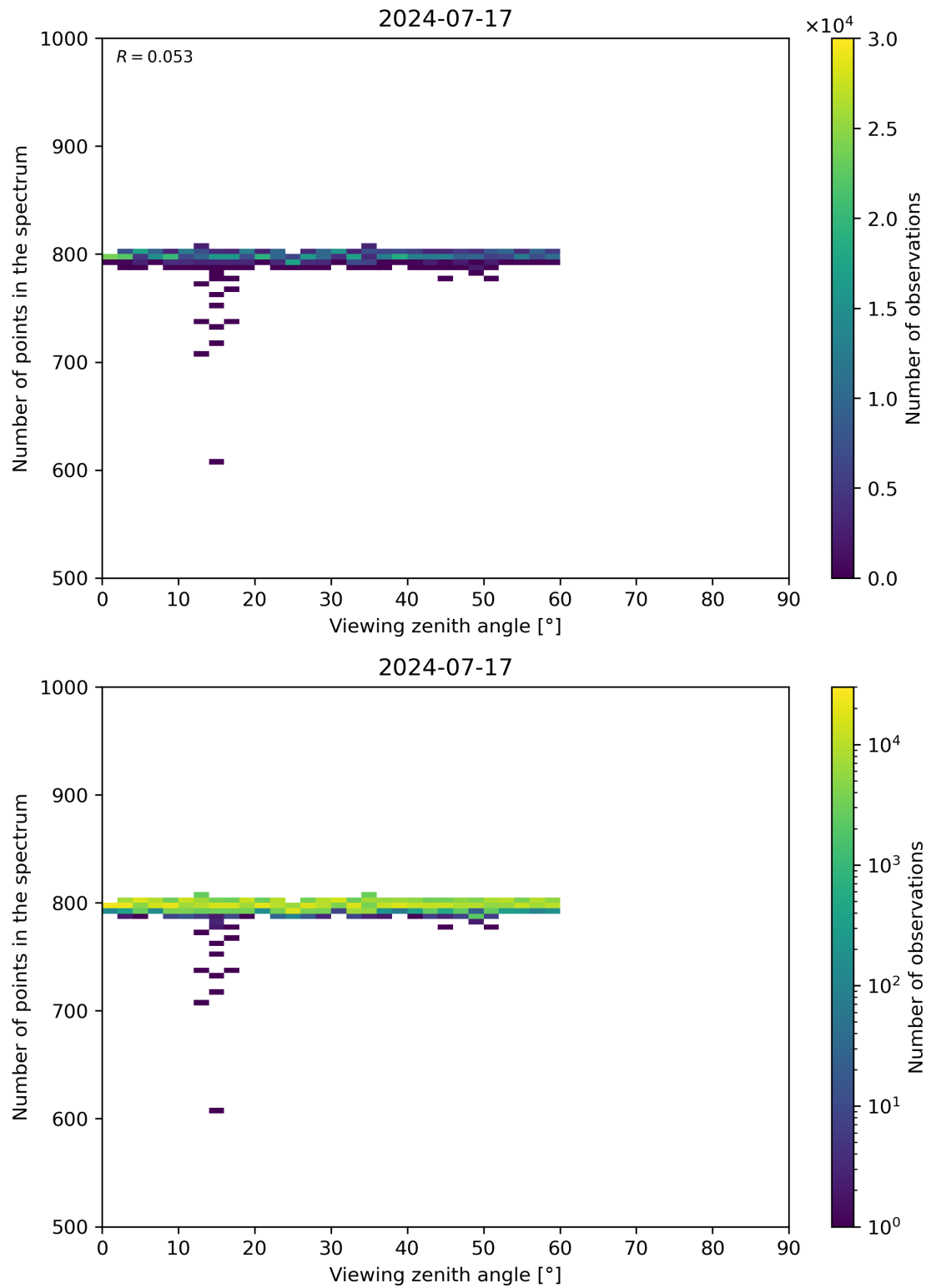
Figure 114: Scatter density plot of “Viewing zenith angle” against “Number of points in the spectrum” for 2024-07-16 to 2024-07-18.
