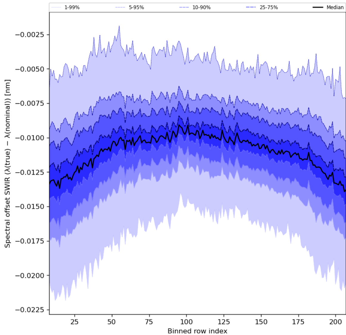
Figure 38: Along track statistics of “Spectral offset SWIR ( \lambda(\text{true}) - \lambda(\text{nominal}) )” for 2024-07-16 to 2024-07-18
