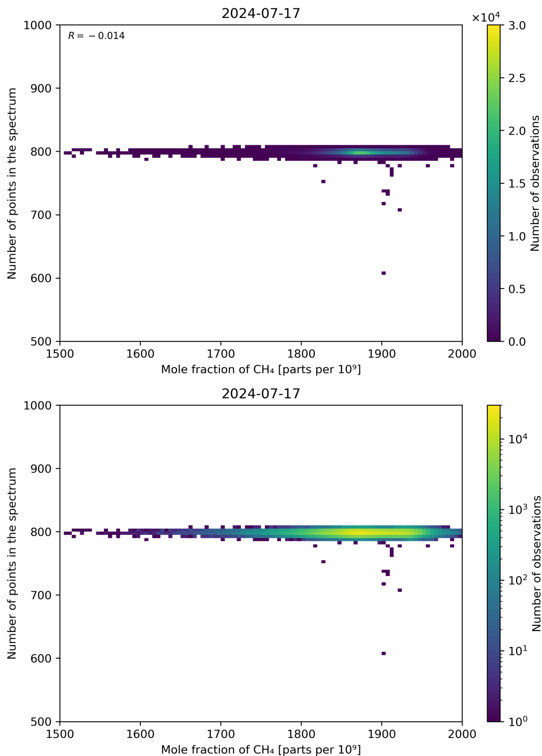
Figure 77: Scatter density plot of “Mole fraction of CH 4 ” against “Number of points in the spectrum” for 2024-07-16 to 2024-07-18.
