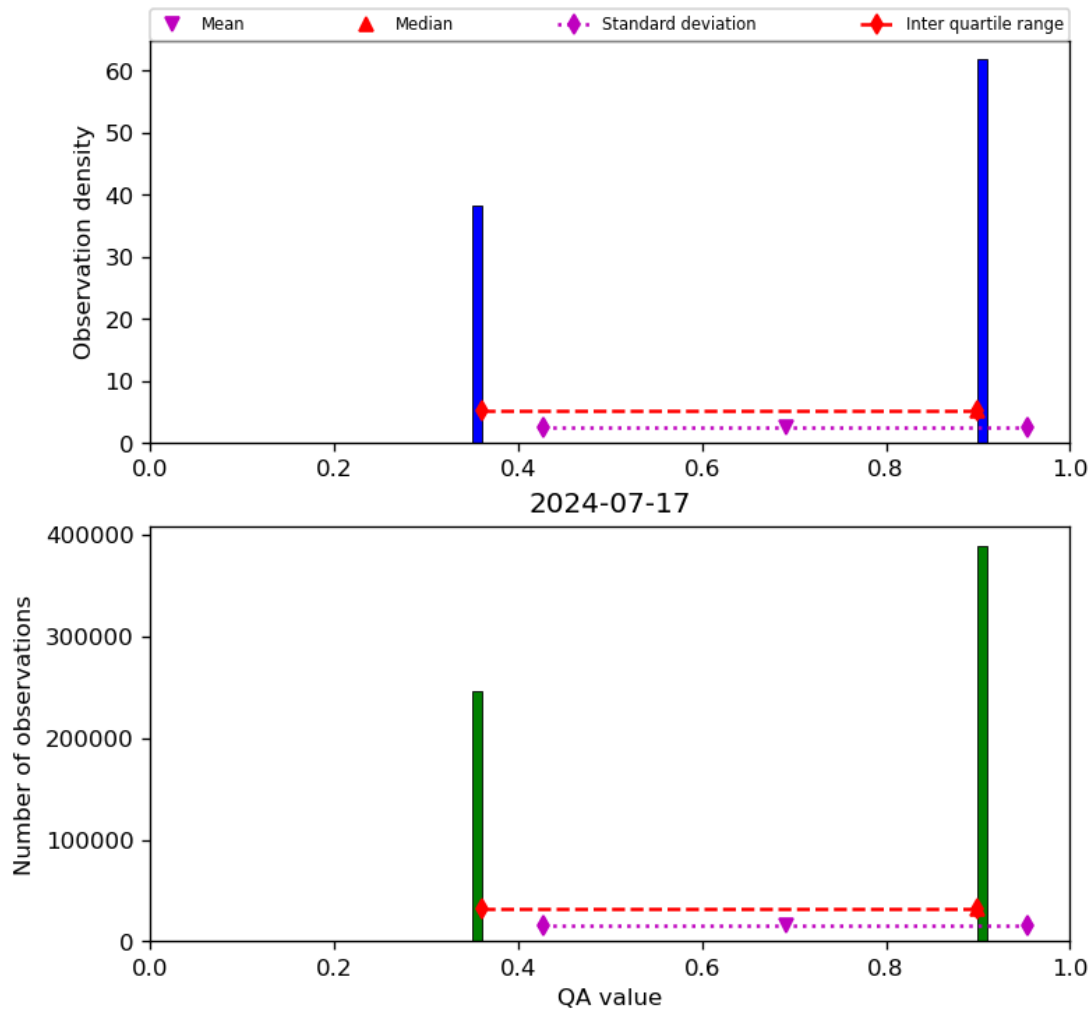
Figure 22: Histogram of “QA value” for 2024-07-16 to 2024-07-18
