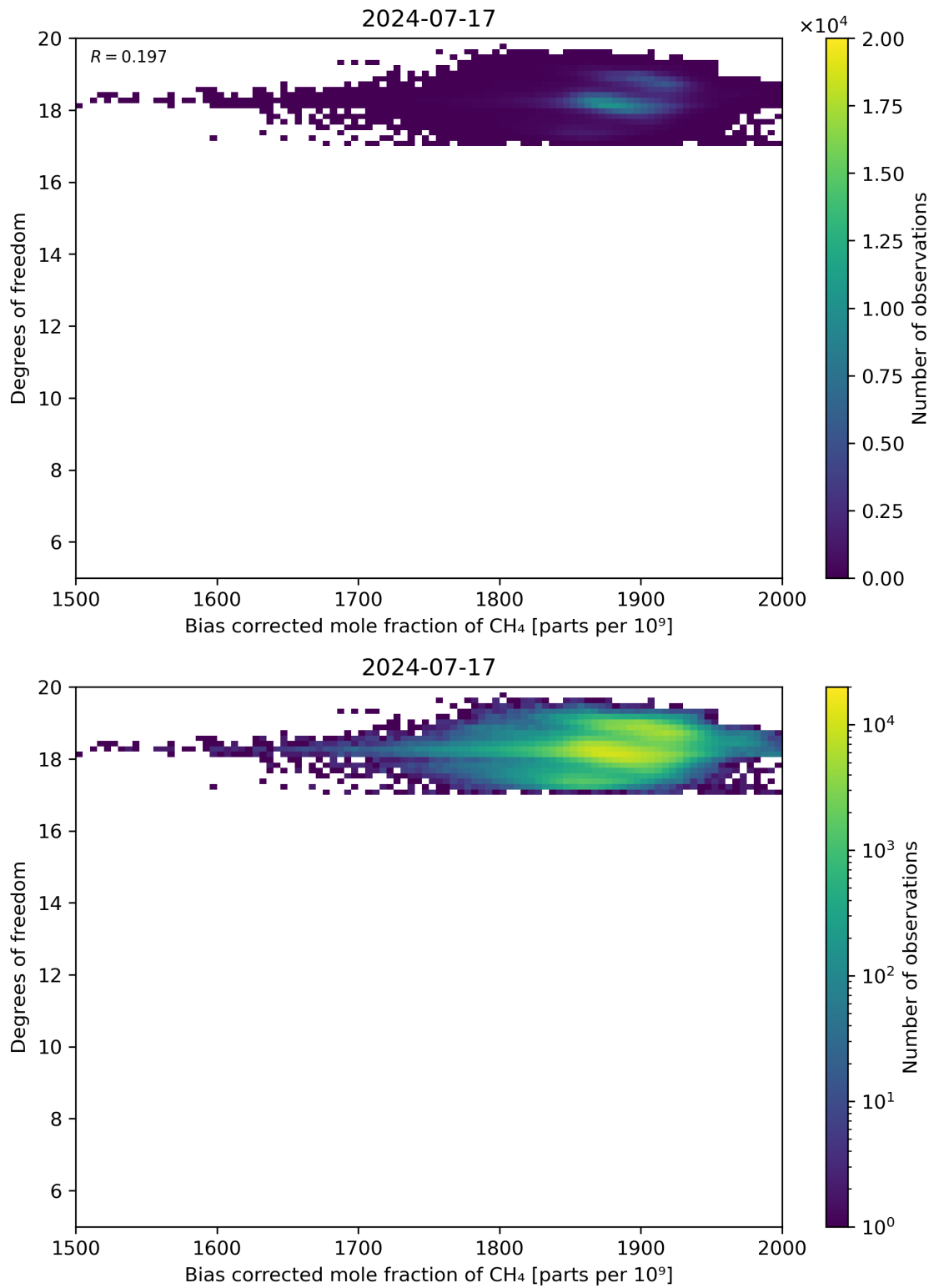
Figure 65: Scatter density plot of “Bias corrected mole fraction of CH 4 ” against “Degrees of freedom” for 2024-07-16 to 2024-07-18.
