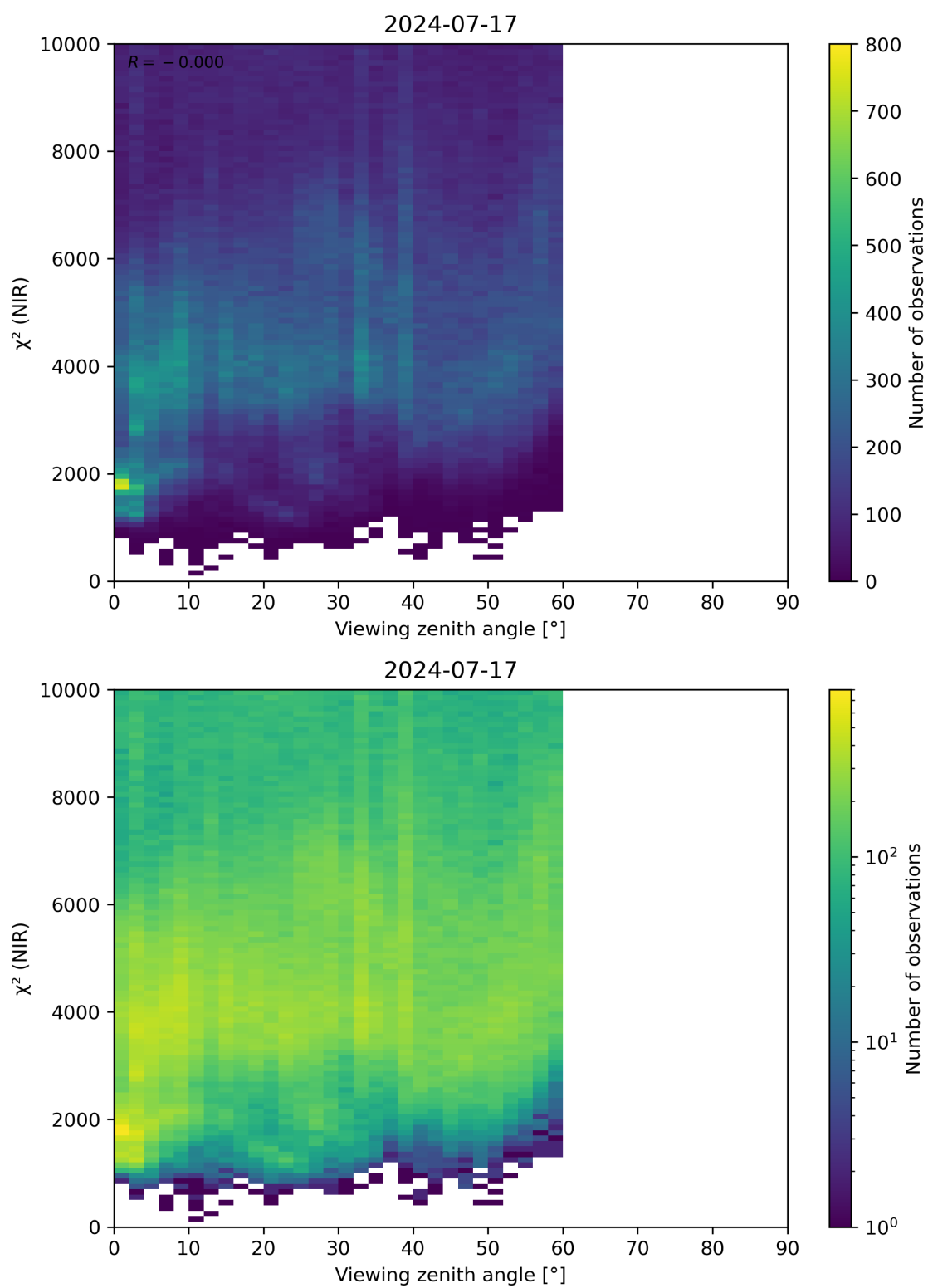
Figure 105: Scatter density plot of “Viewing zenith angle” against “ \chi^2 (NIR)” for 2024-07-16 to 2024-07-18.
