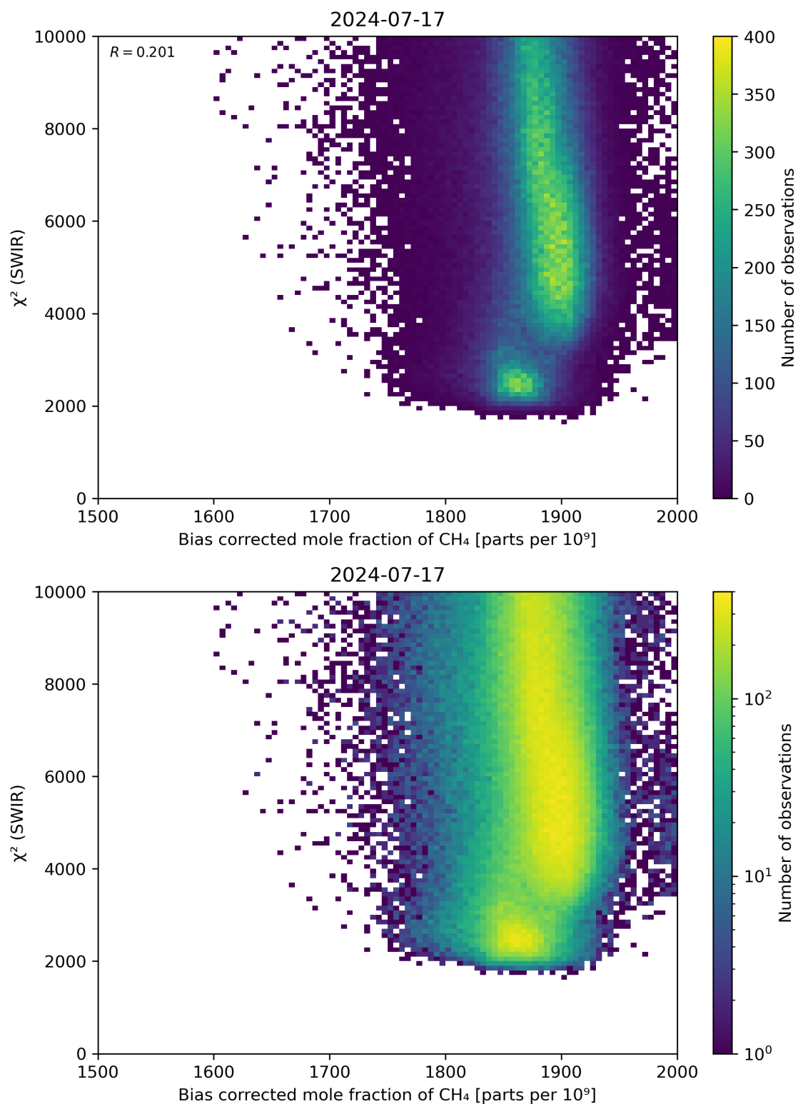
Figure 64: Scatter density plot of “Bias corrected mole fraction of CH 4 ” against “ \chi^2 (SWIR)” for 2024-07-16 to 2024-07-18.
