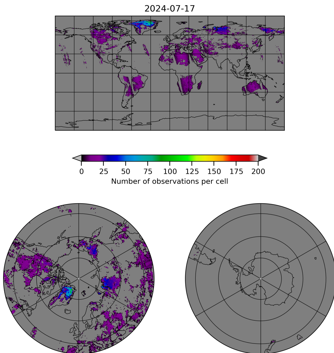
Figure 10: Map of the number of observations for 2024-07-16 to 2024-07-18
