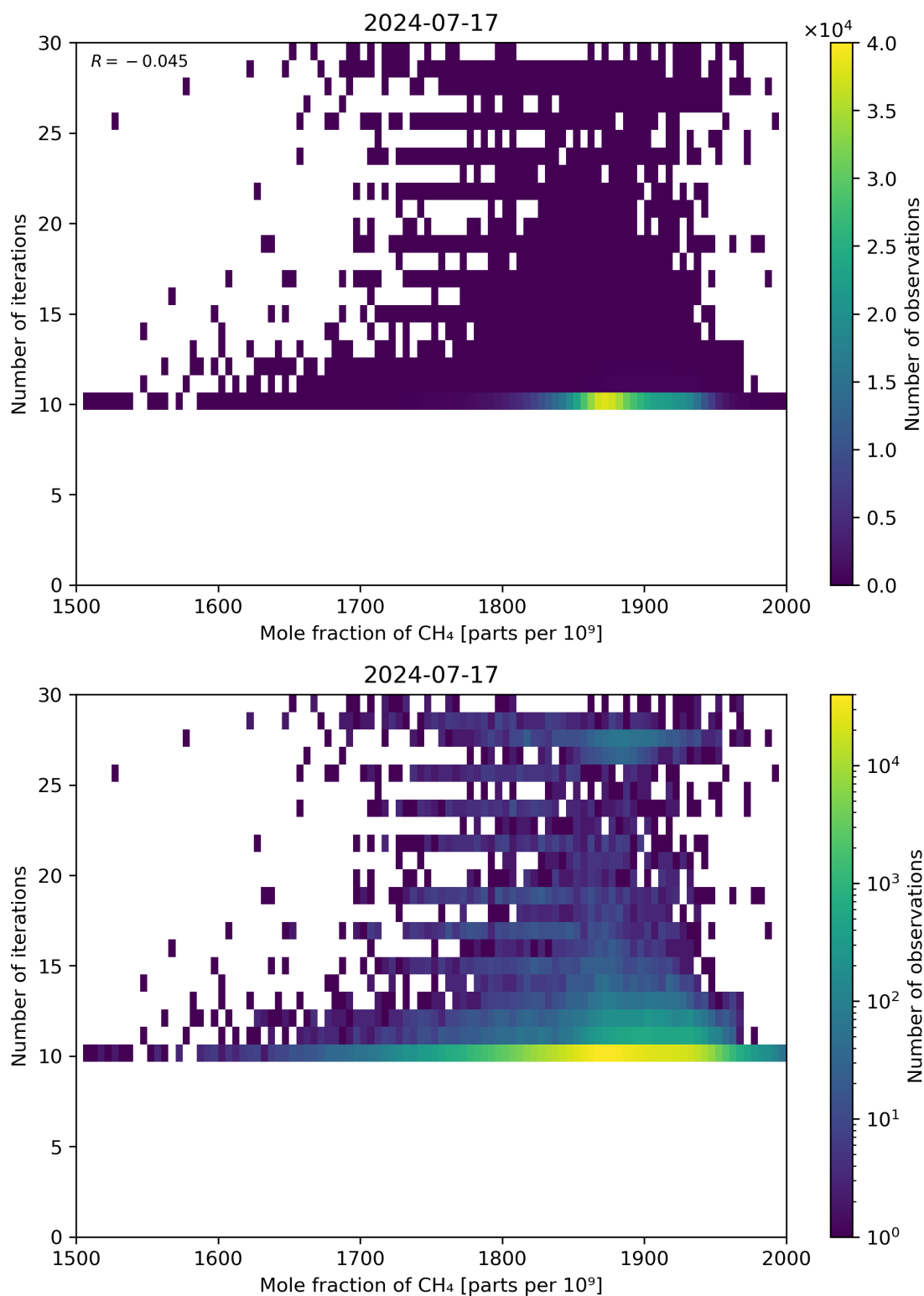
Figure 76: Scatter density plot of “Mole fraction of CH 4 ” against “Number of iterations” for 2024-07-16 to 2024-07-18.
