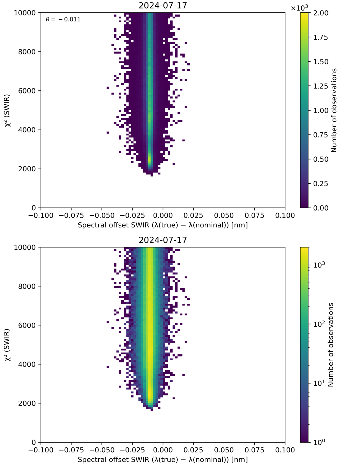
Figure 118: Scatter density plot of “Spectral offset SWIR ( \lambda(\text{true}) - \lambda(\text{nominal}) )” against “ \chi^2 (SWIR)” for 2024-07-16 to 2024-07-18.
