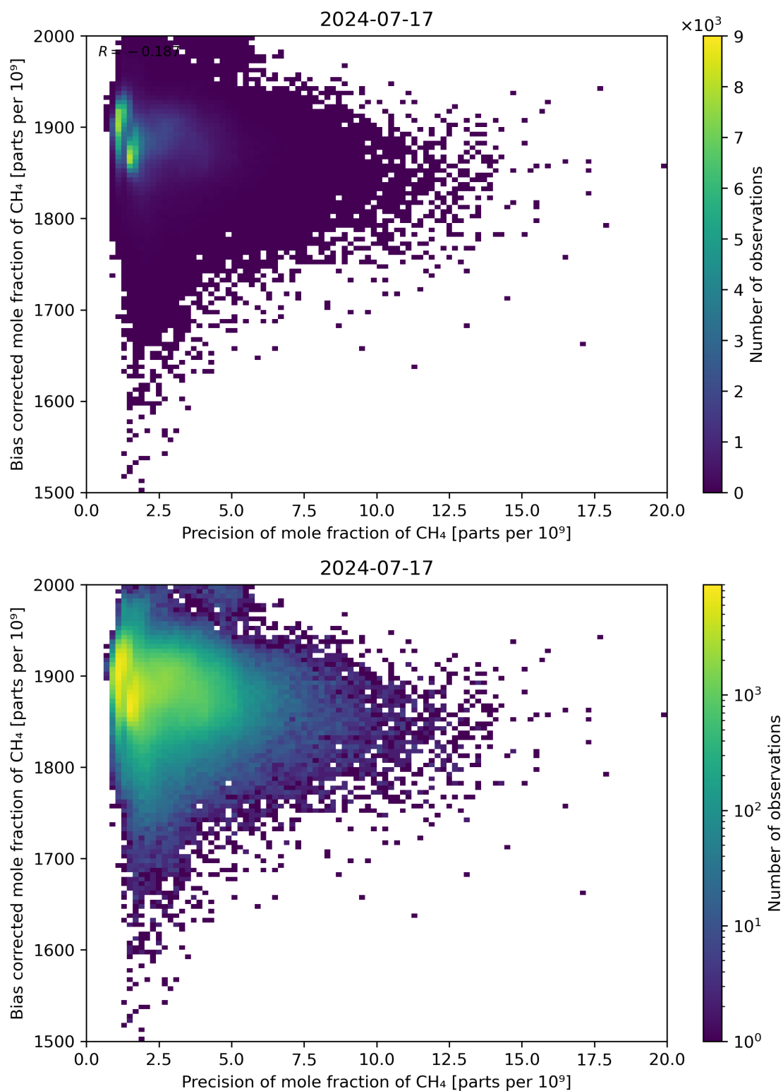
Figure 82: Scatter density plot of “Precision of mole fraction of CH 4 ” against “Bias corrected mole fraction of CH 4 ” for 2024-07-16 to 2024-07-18.
