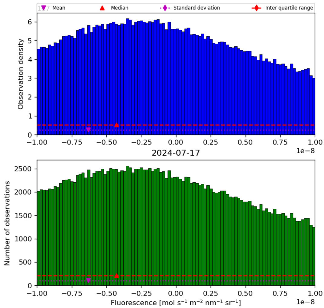
Figure 32: Histogram of “Fluorescence” for 2024-07-16 to 2024-07-18
