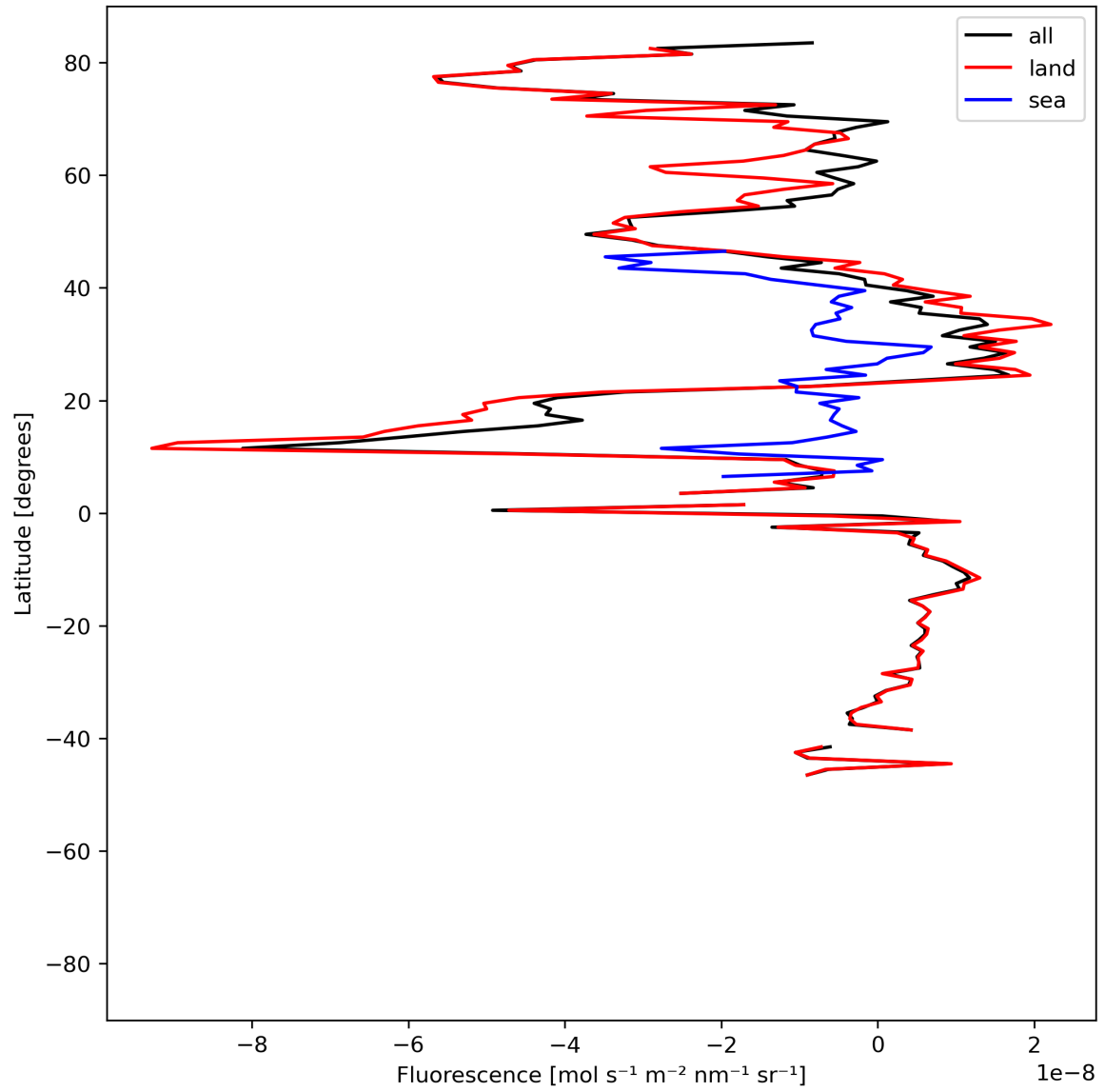
Figure 21: Zonal average of “Fluorescence” for 2024-07-16 to 2024-07-18.
