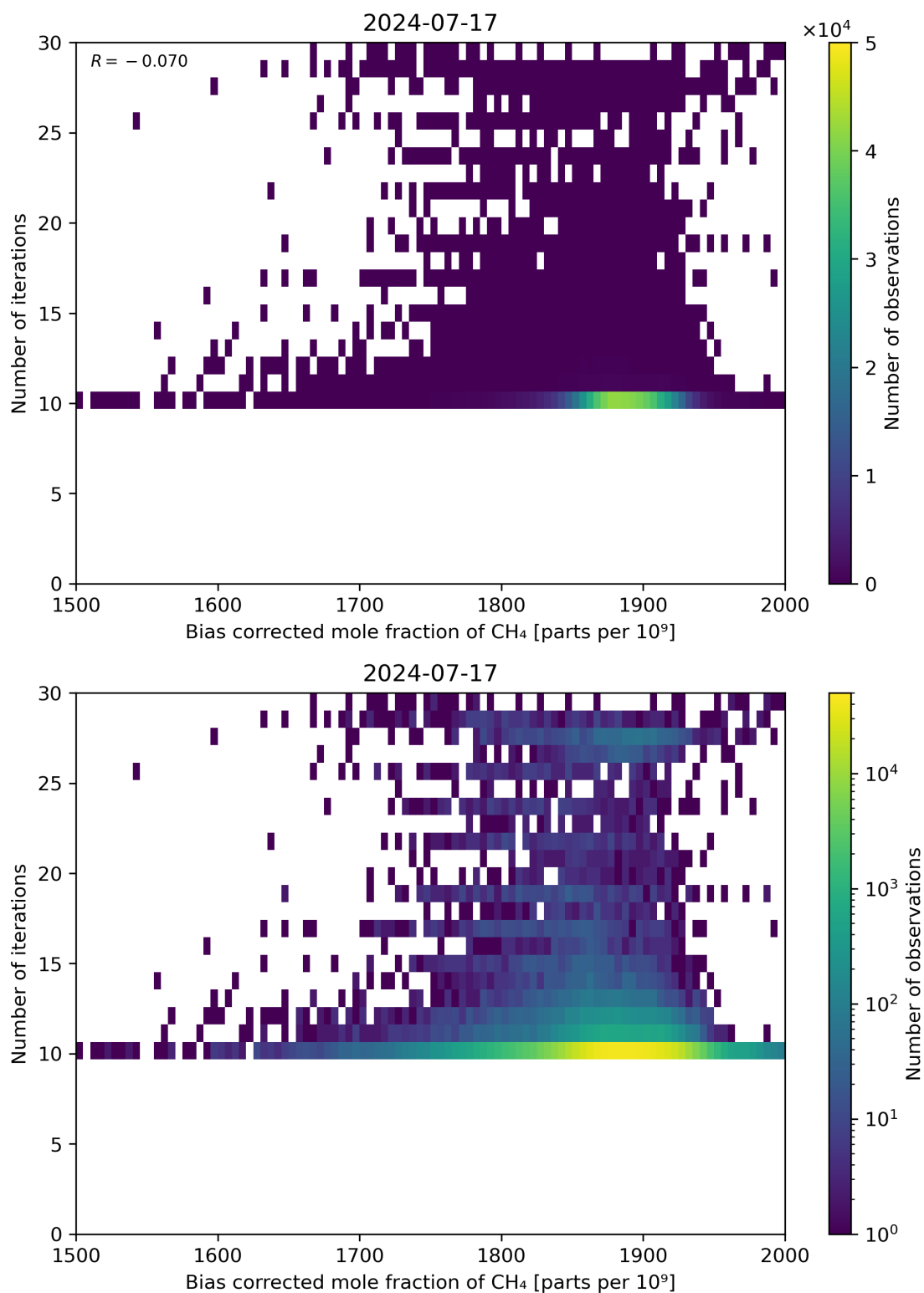
Figure 67: Scatter density plot of “Bias corrected mole fraction of \text{CH}_4 ” against “Number of iterations” for 2024-07-16 to 2024-07-18.
