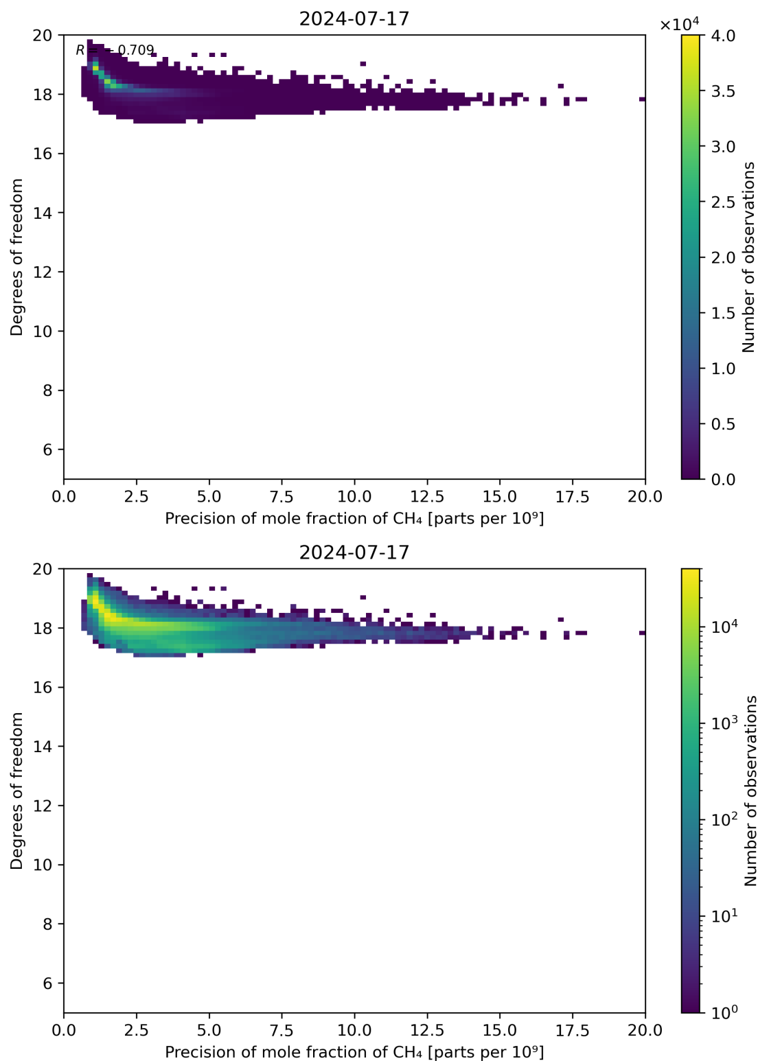
Figure 80: Scatter density plot of “Precision of mole fraction of CH 4 ” against “Degrees of freedom” for 2024-07-16 to 2024-07-18.
