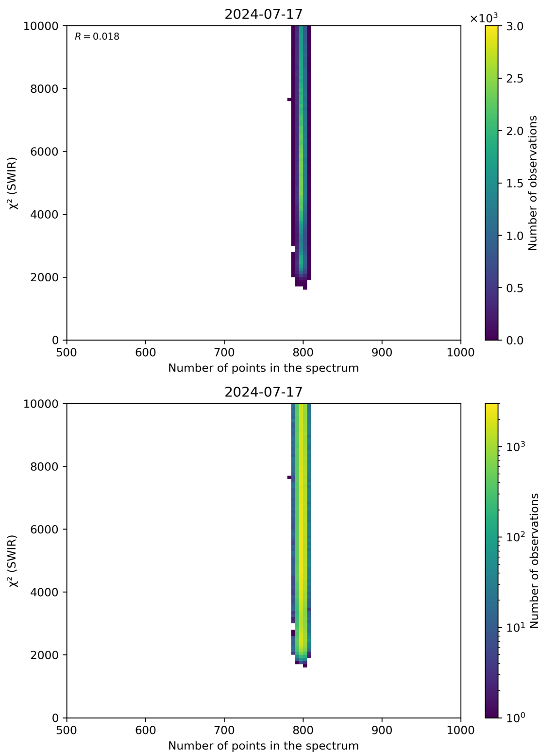
Figure 89: Scatter density plot of “Number of points in the spectrum” against “ \chi^2 (SWIR)” for 2024-07-16 to 2024-07-18.
