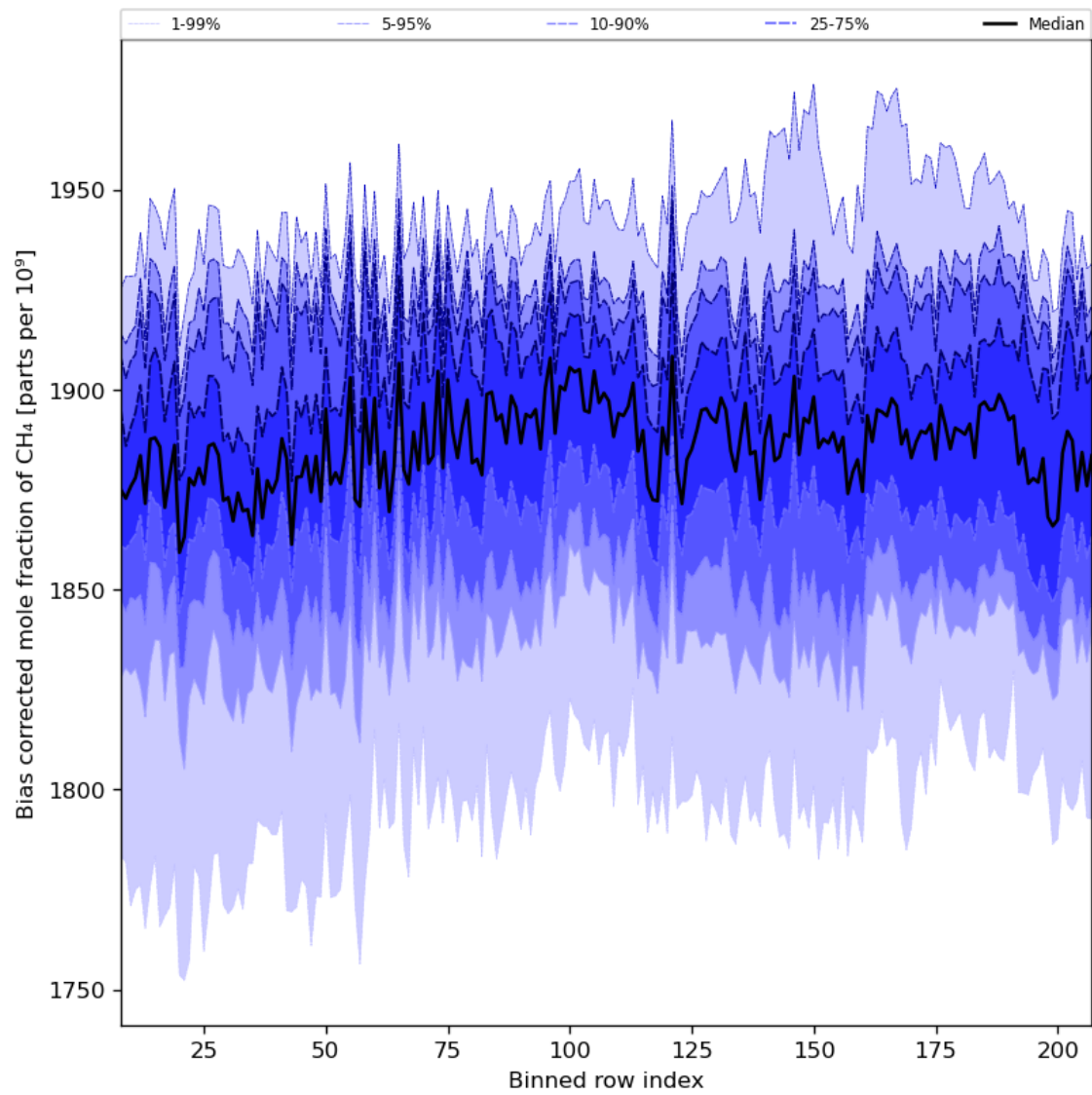
Figure 36: Along track statistics of “Bias corrected mole fraction of CH 4 ” for 2024-07-16 to 2024-07-18
