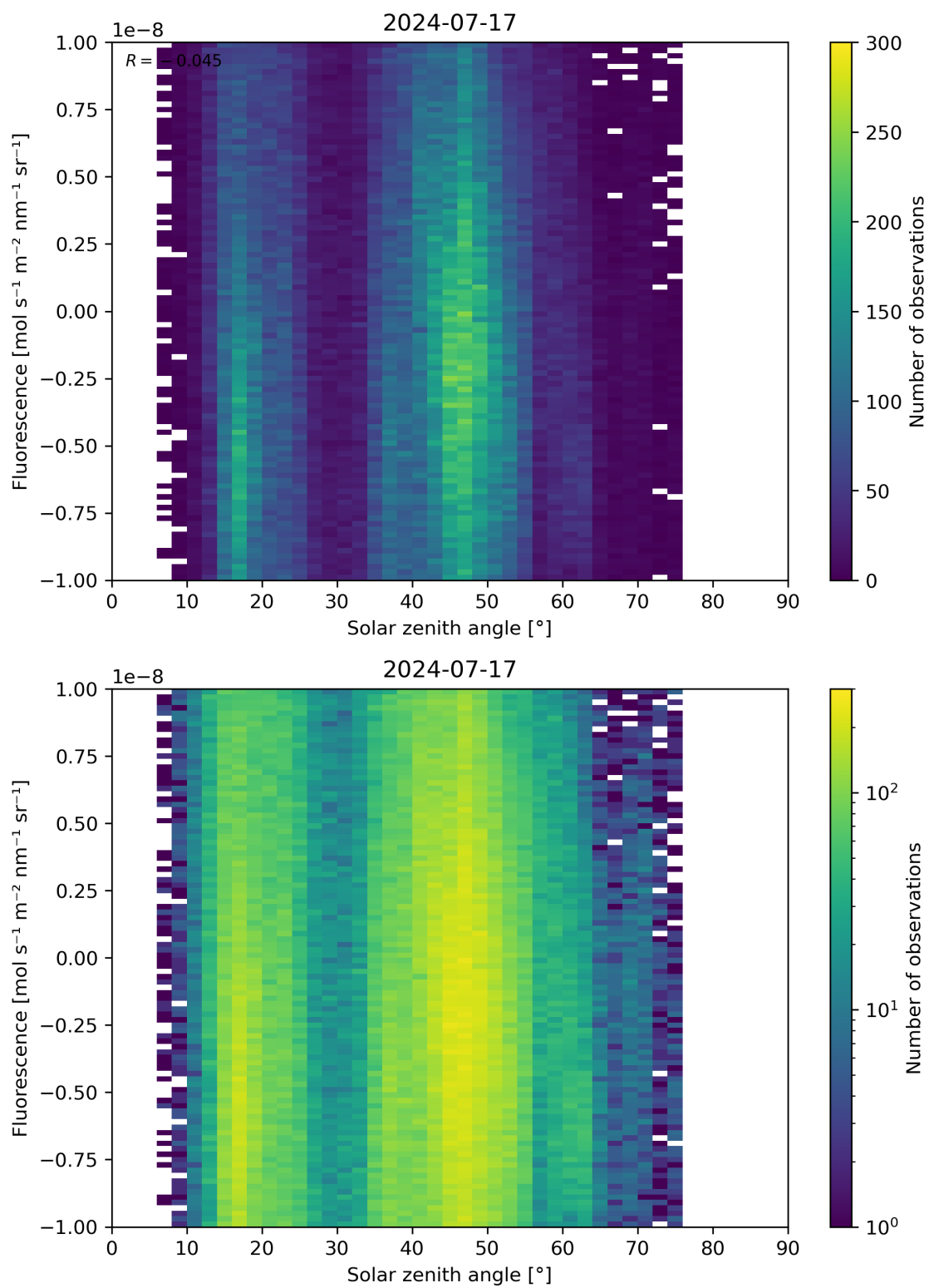
Figure 97: Scatter density plot of “Solar zenith angle” against “Fluorescence” for 2024-07-16 to 2024-07-18.
