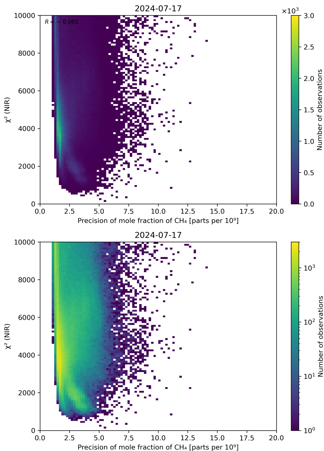
Figure 78: Scatter density plot of “Precision of mole fraction of CH 4 ” against “ \chi^2 (NIR)” for 2024-07-16 to 2024-07-18.
