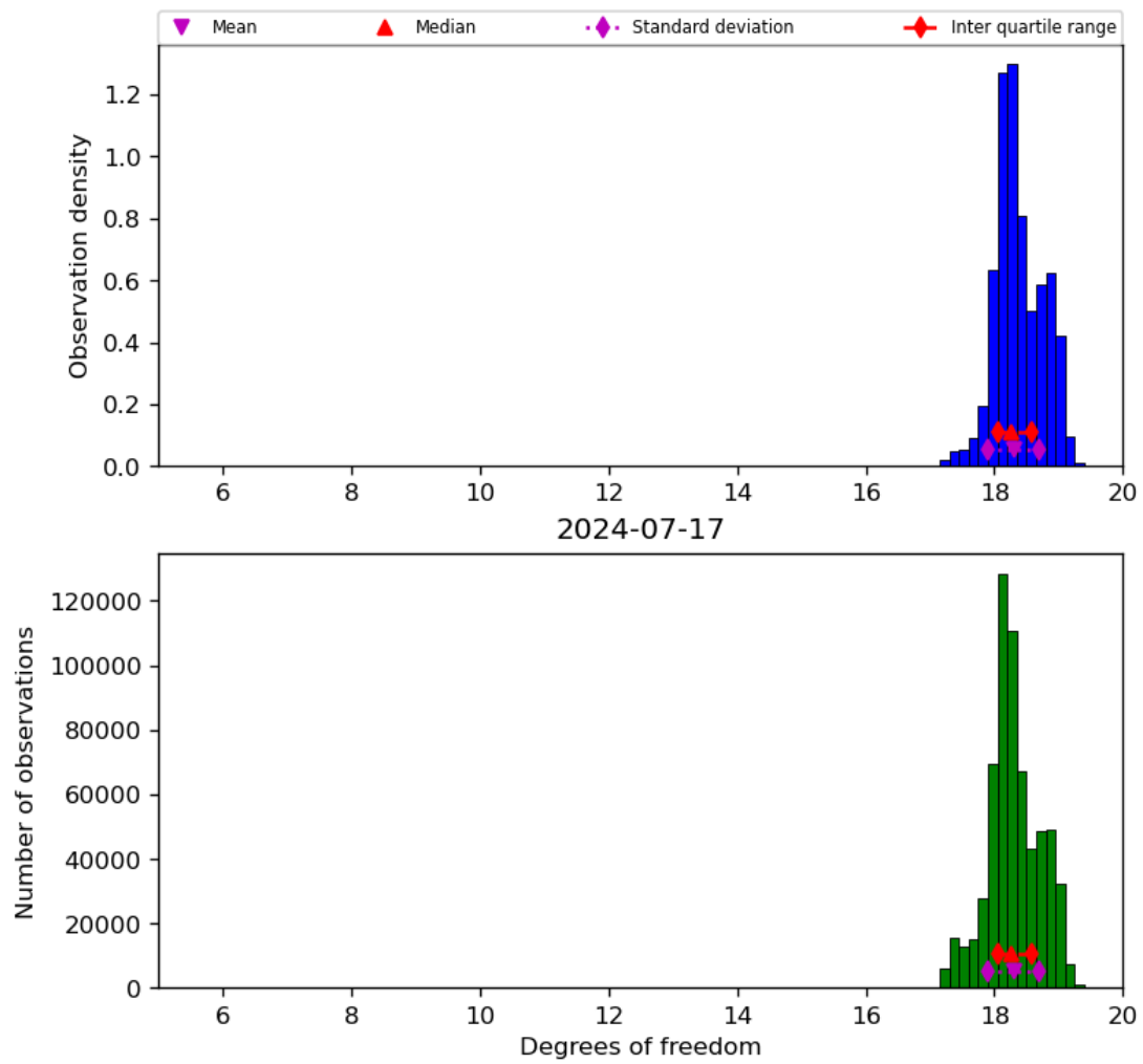
Figure 30: Histogram of “Degrees of freedom” for 2024-07-16 to 2024-07-18
