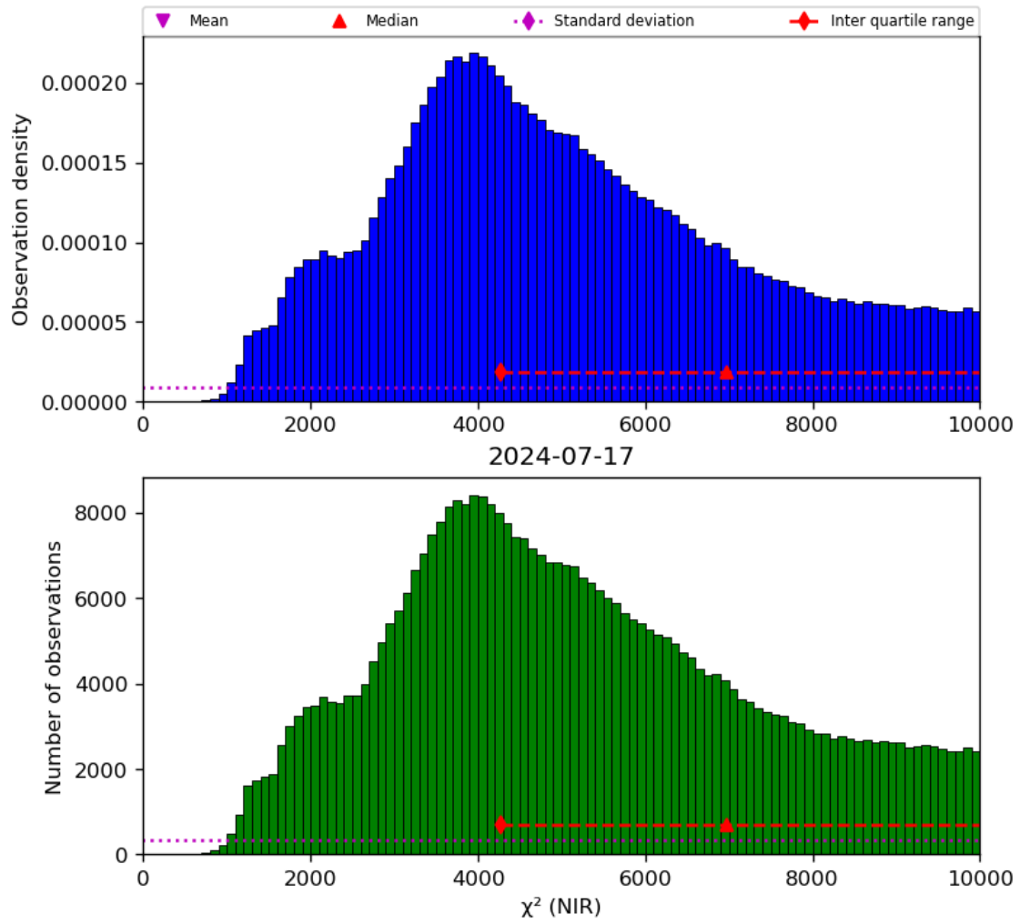
Figure 29: Histogram of “ \chi^2 (NIR)” for 2024-07-16 to 2024-07-18
