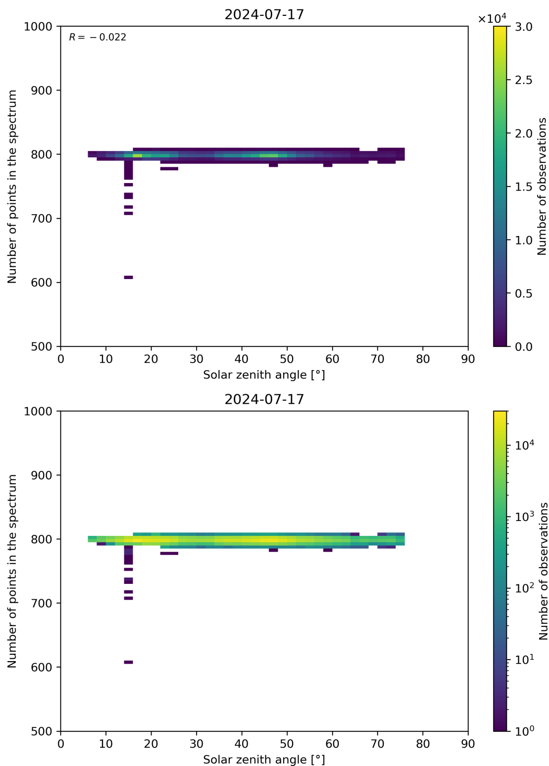
Figure 103: Scatter density plot of “Solar zenith angle” against “Number of points in the spectrum” for 2024-07-16 to 2024-07-18.
