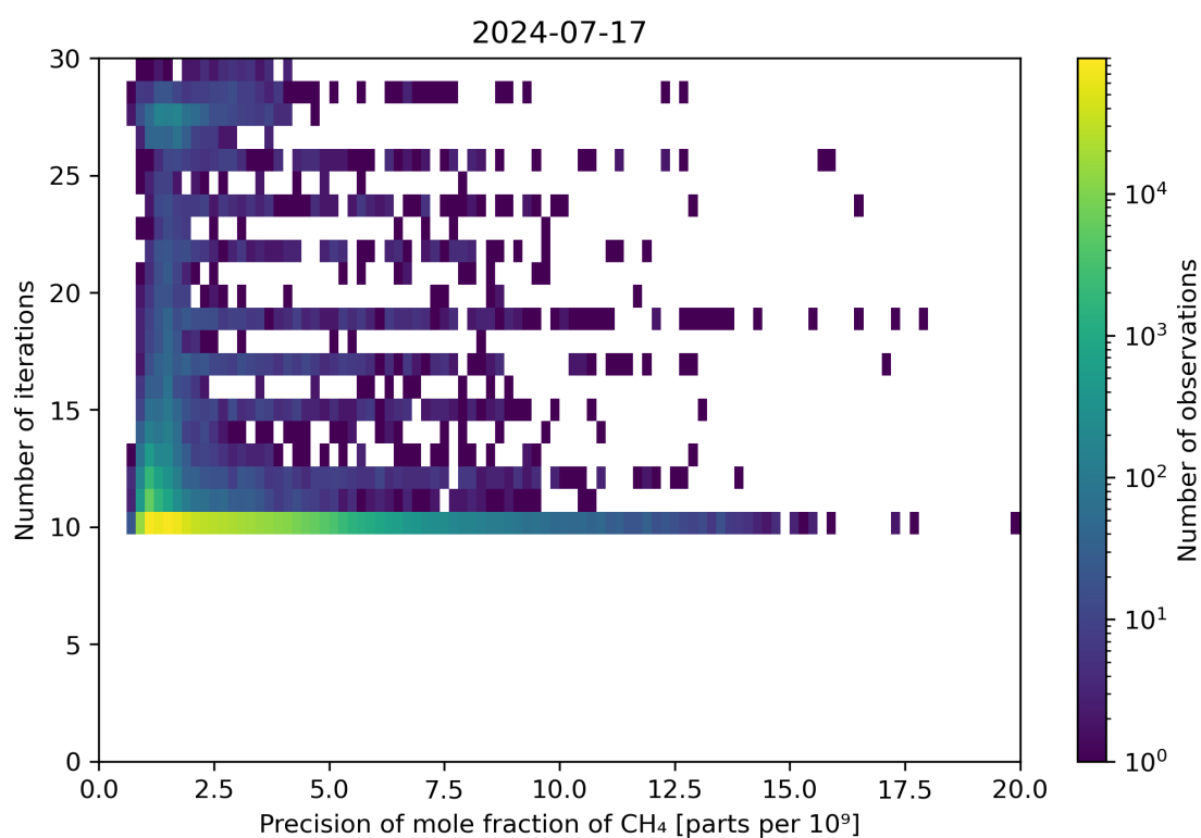
Figure 83: Scatter density plot of “Precision of mole fraction of \text{CH}_4 ” against “Number of iterations” for 2024-07-16 to 2024-07-18.
