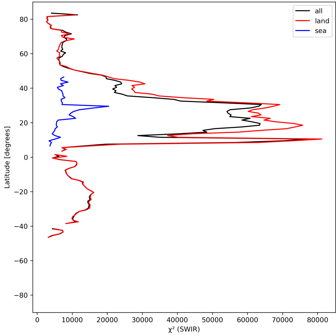
Figure 17: Zonal average of “ \chi^2 (SWIR)” for 2024-07-16 to 2024-07-18.
