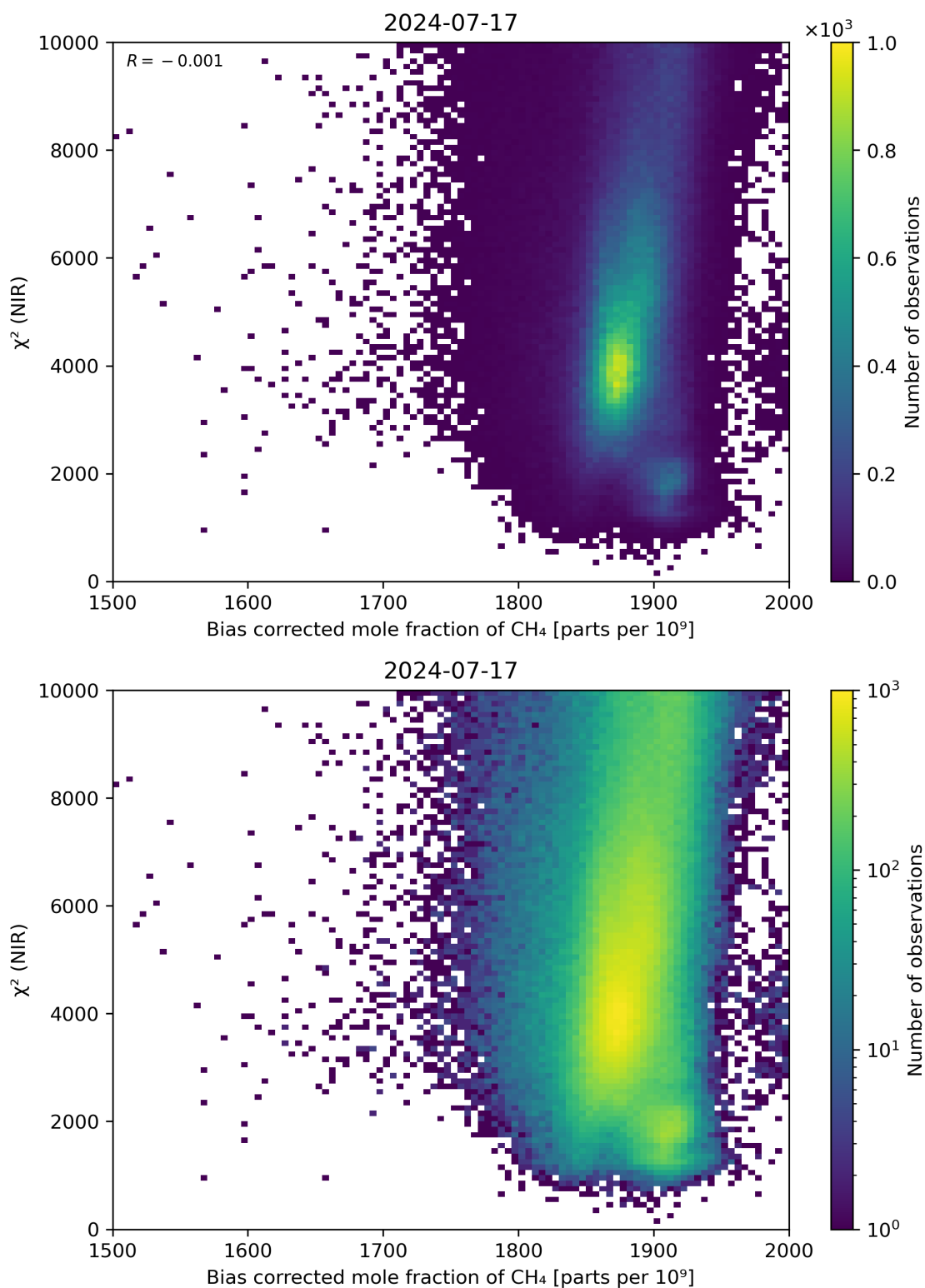
Figure 63: Scatter density plot of “Bias corrected mole fraction of CH 4 ” against “ \chi^2 (NIR)” for 2024-07-16 to 2024-07-18.
