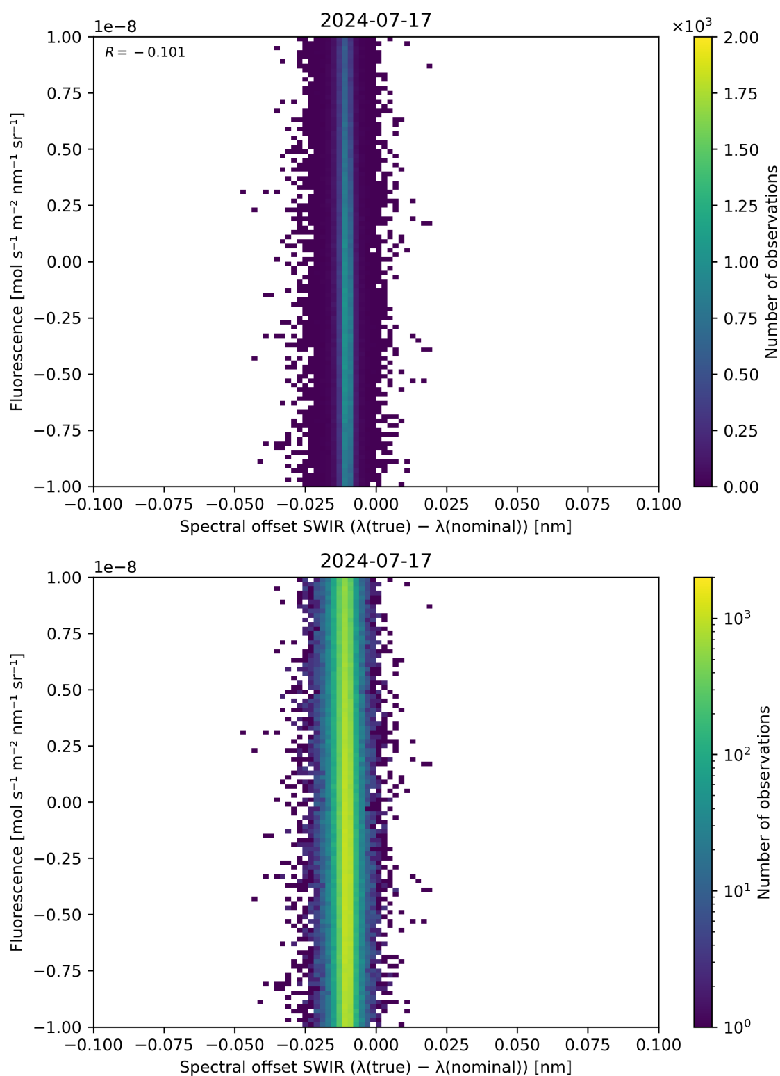
Figure 120: Scatter density plot of “Spectral offset SWIR ( \lambda(\text{true}) - \lambda(\text{nominal}) )” against “Fluorescence” for 2024-07-16 to 2024-07-18.
