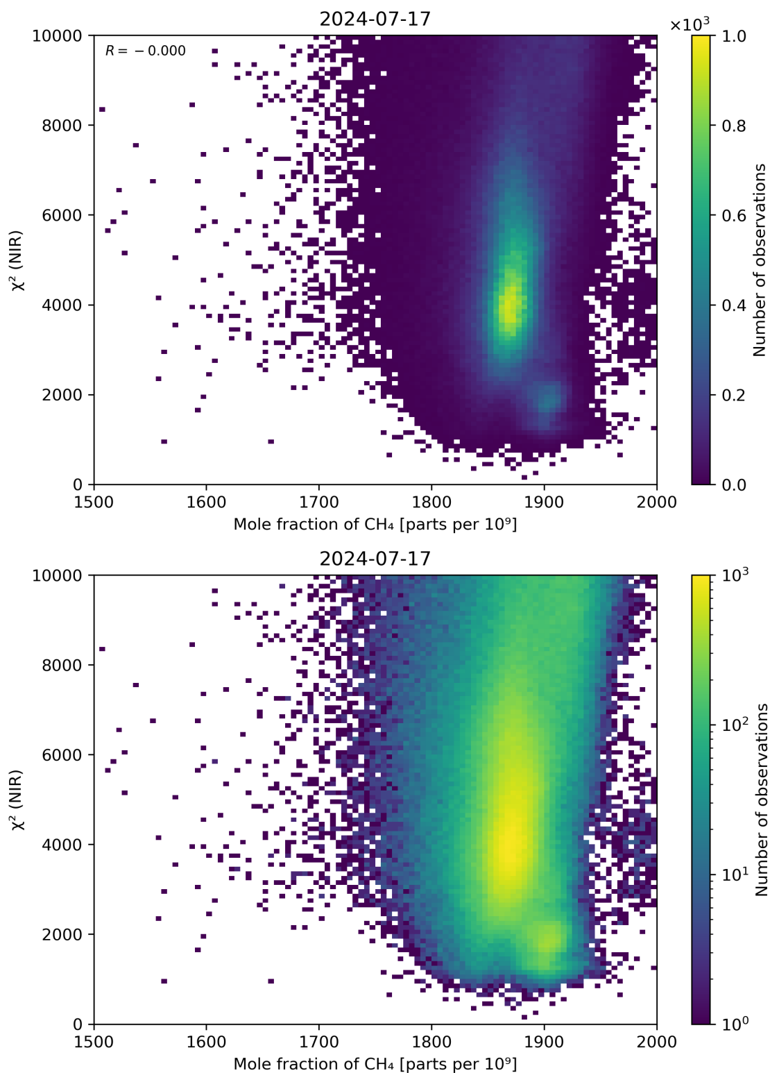
Figure 70: Scatter density plot of “Mole fraction of \text{CH}_4 ” against “ \chi^2 (NIR)” for 2024-07-16 to 2024-07-18.
