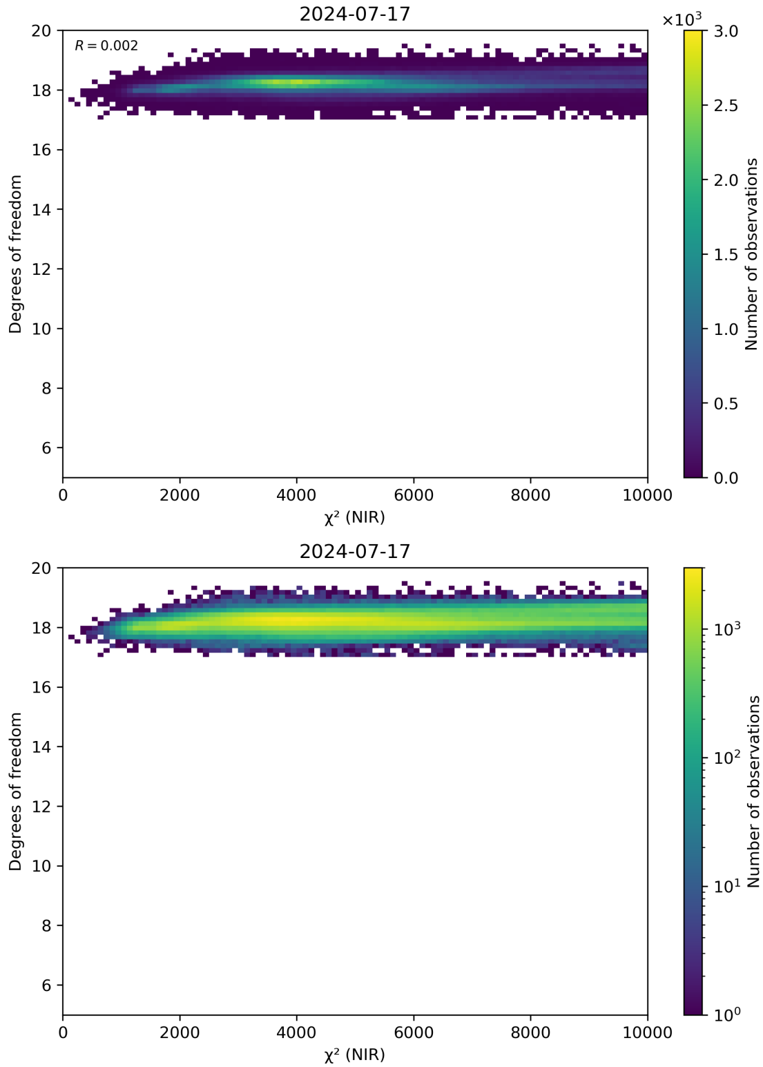
Figure 44: Scatter density plot of “ \chi^2 (NIR)” against “Degrees of freedom” for 2024-07-16 to 2024-07-18.
