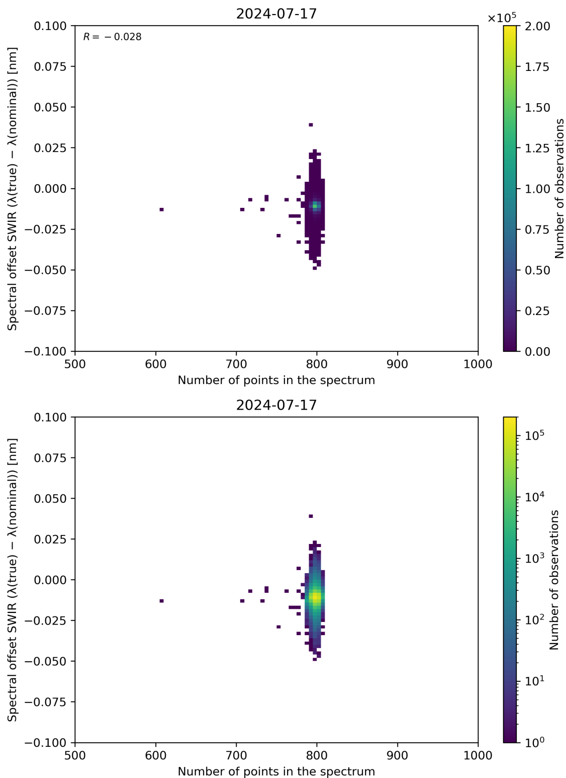
Figure 93: Scatter density plot of “Number of points in the spectrum” against “Spectral offset SWIR ( \lambda(\text{true}) - \lambda(\text{nominal}) )” for 2024-07-16 to 2024-07-18.
