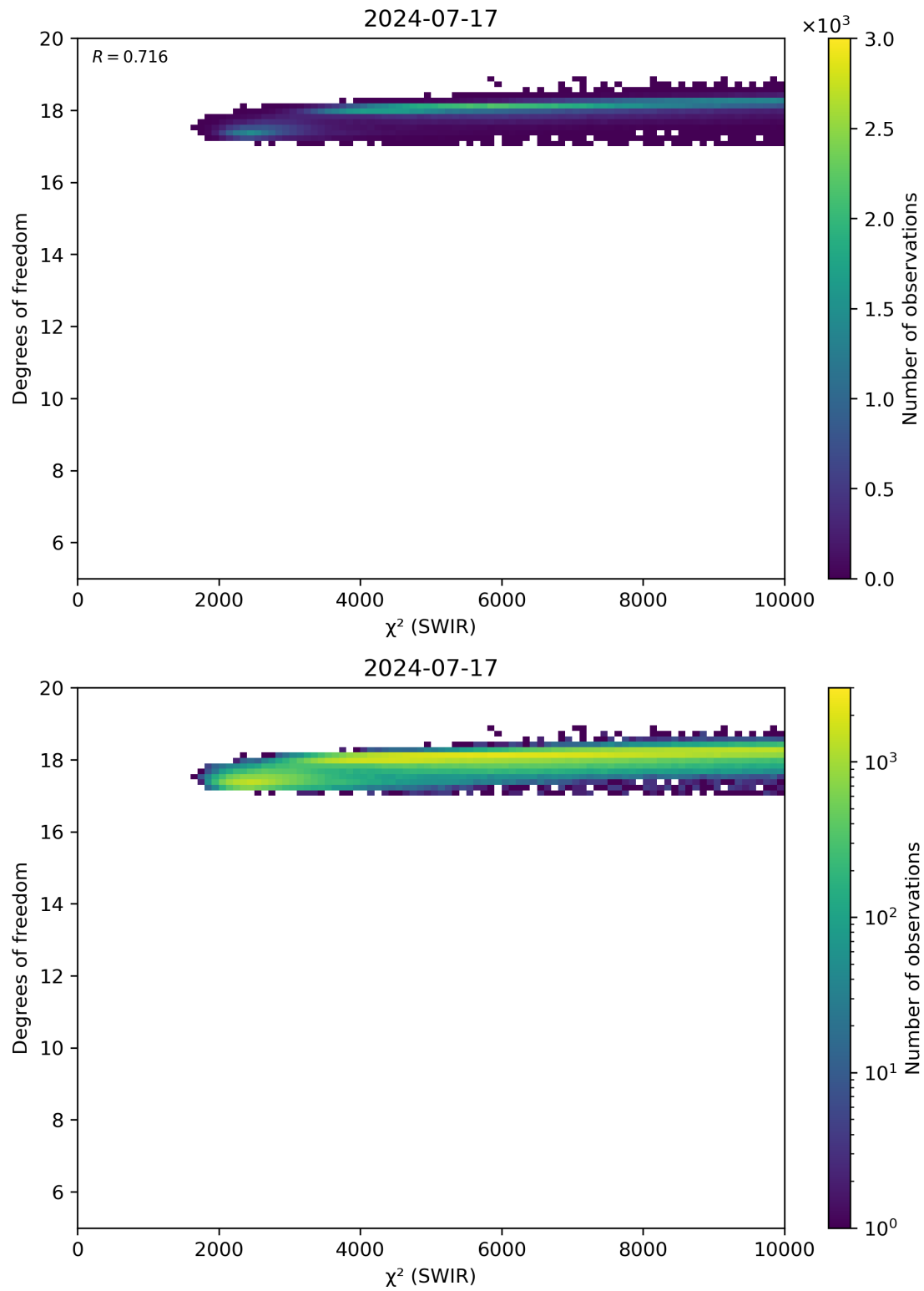
Figure 48: Scatter density plot of “ \chi^2 (SWIR)” against “Degrees of freedom” for 2024-07-16 to 2024-07-18.
