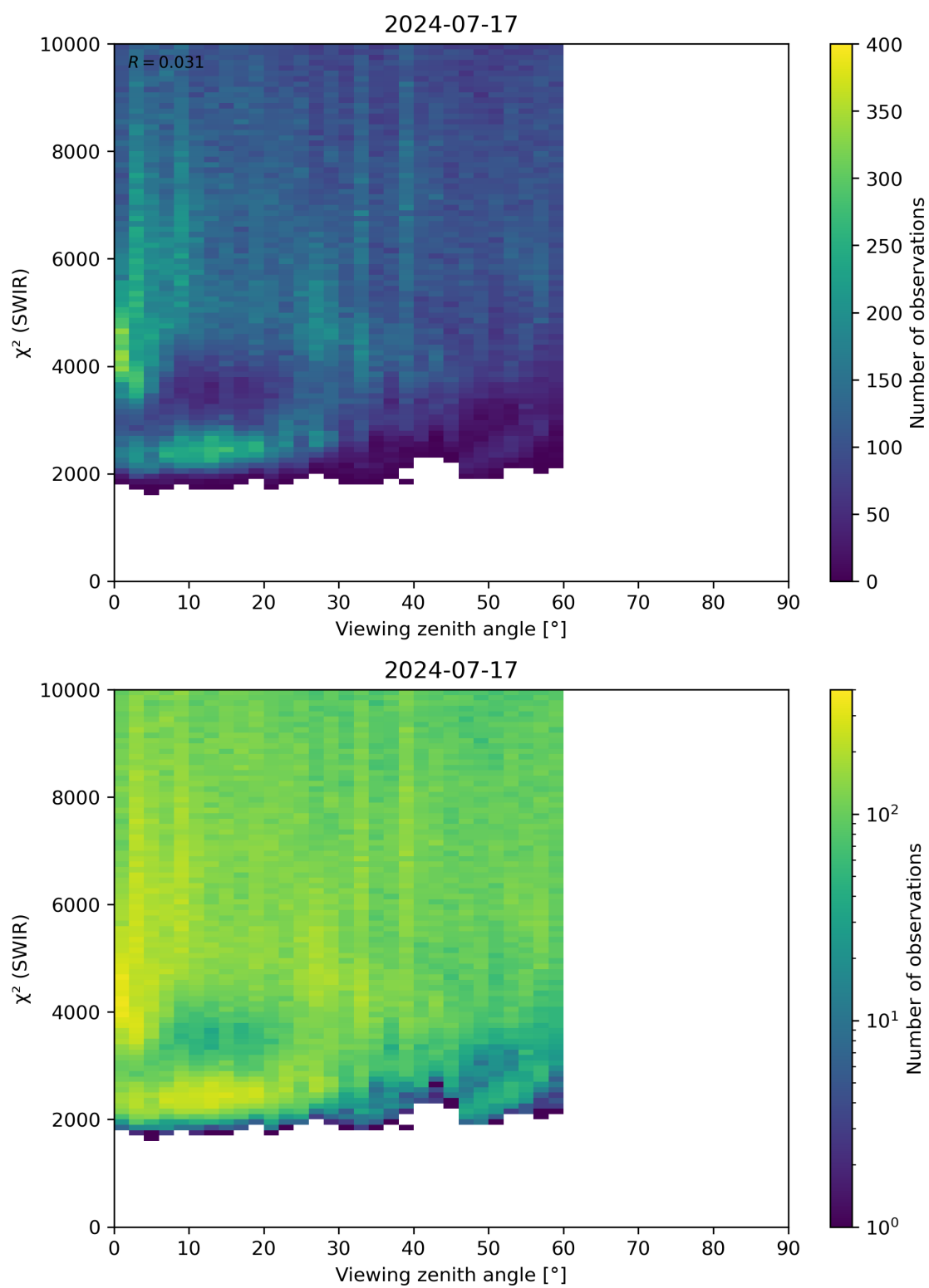
Figure 106: Scatter density plot of “Viewing zenith angle” against “ \chi^2 (SWIR)” for 2024-07-16 to 2024-07-18.
