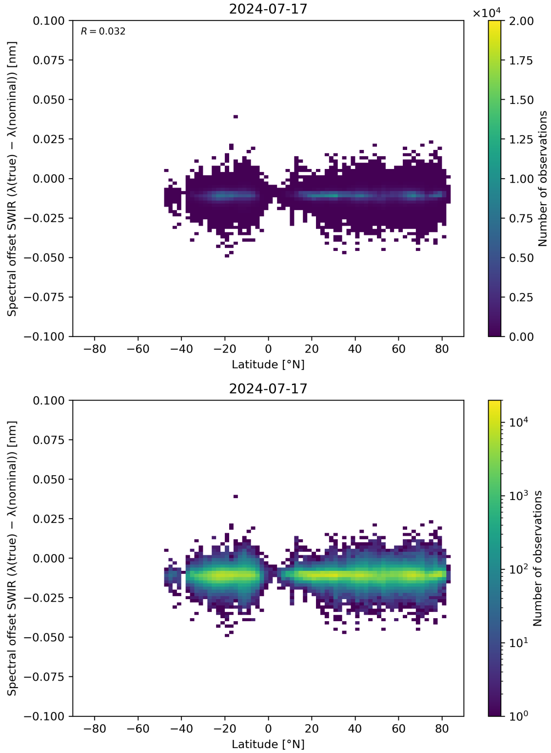
Figure 62: Scatter density plot of “Latitude” against “Spectral offset SWIR ( \lambda(\text{true}) - \lambda(\text{nominal}) )” for 2024-07-16 to 2024-07-18.
