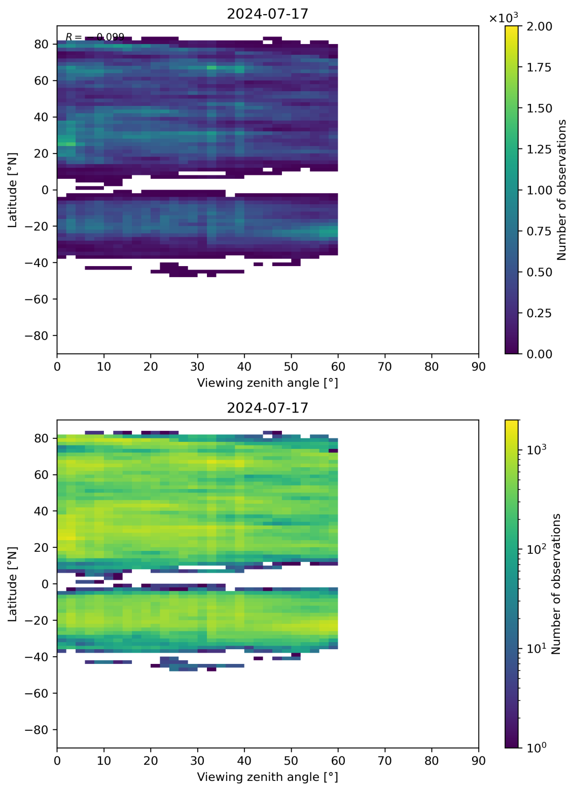
Figure 109: Scatter density plot of “Viewing zenith angle” against “Latitude” for 2024-07-16 to 2024-07-18.
