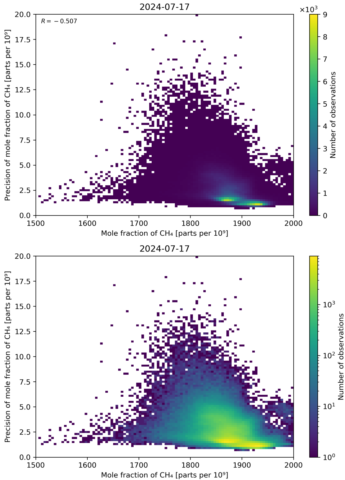
Figure 75: Scatter density plot of “Mole fraction of CH 4 ” against “Precision of mole fraction of CH 4 ” for 2024-07-16 to 2024-07-18.
