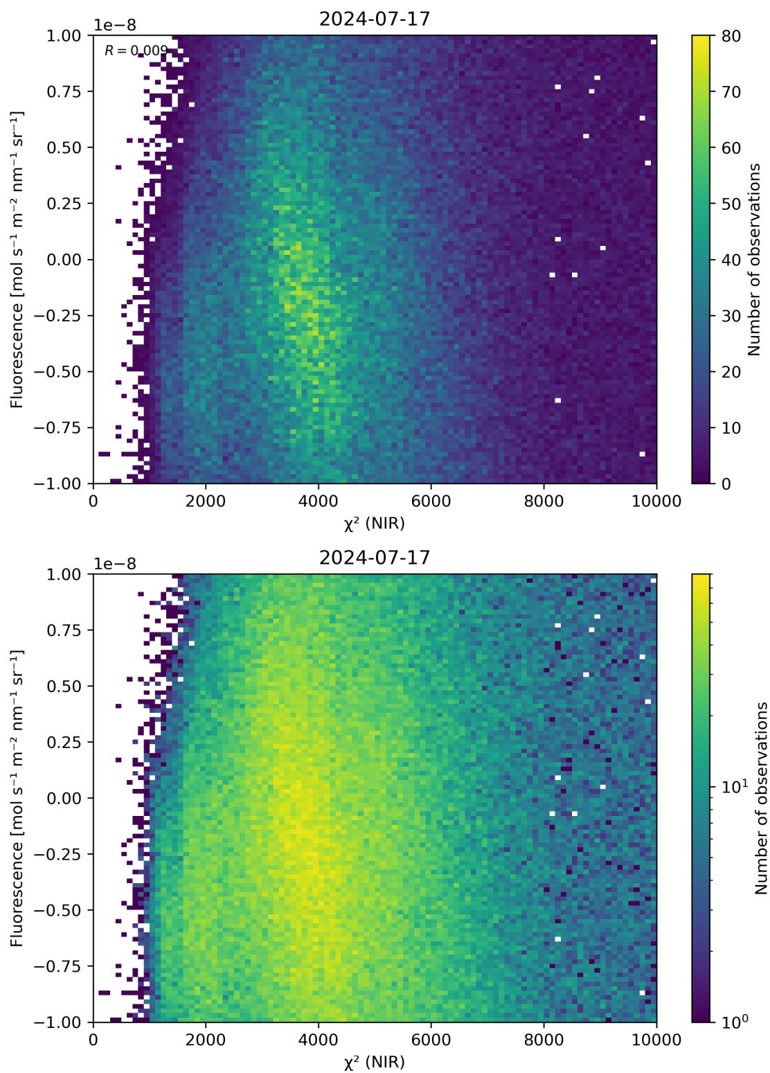
Figure 45: Scatter density plot of “ \chi^2 (NIR)” against “Fluorescence” for 2024-07-16 to 2024-07-18.
