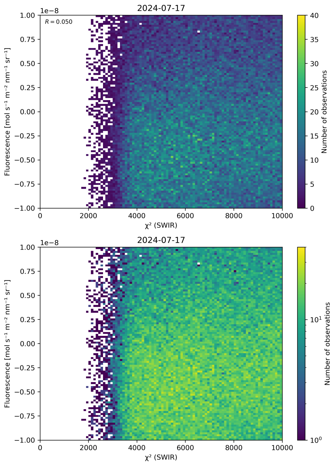
Figure 49: Scatter density plot of “ \chi^2 (SWIR)” against “Fluorescence” for 2024-07-16 to 2024-07-18.
