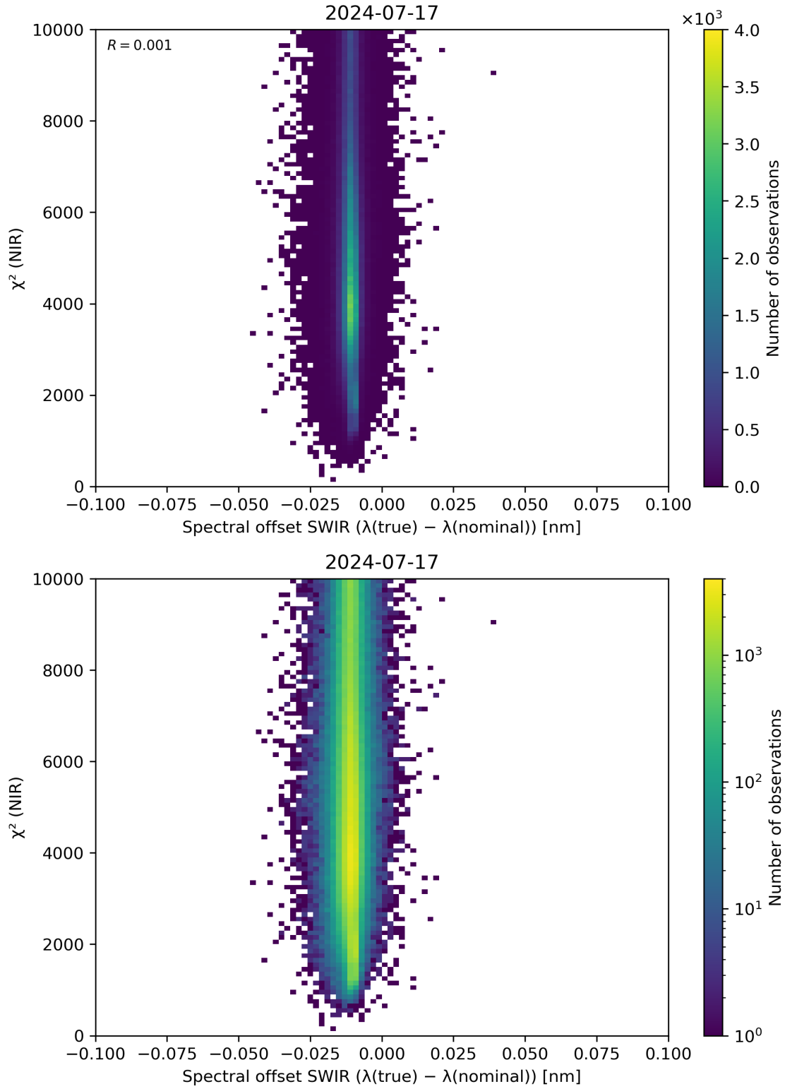
Figure 117: Scatter density plot of “Spectral offset SWIR ( \lambda(\text{true}) - \lambda(\text{nominal}) )” against “ \chi^2 (NIR)” for 2024-07-16 to 2024-07-18.
