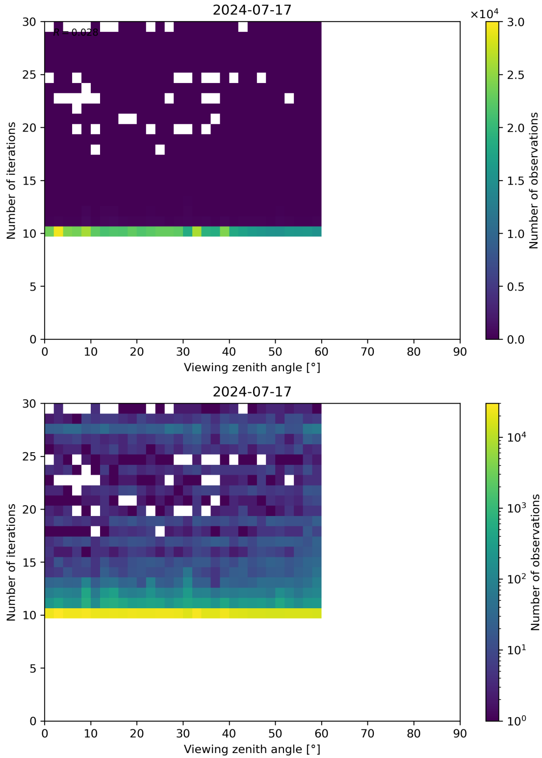
Figure 113: Scatter density plot of “Viewing zenith angle” against “Number of iterations” for 2024-07-16 to 2024-07-18.
