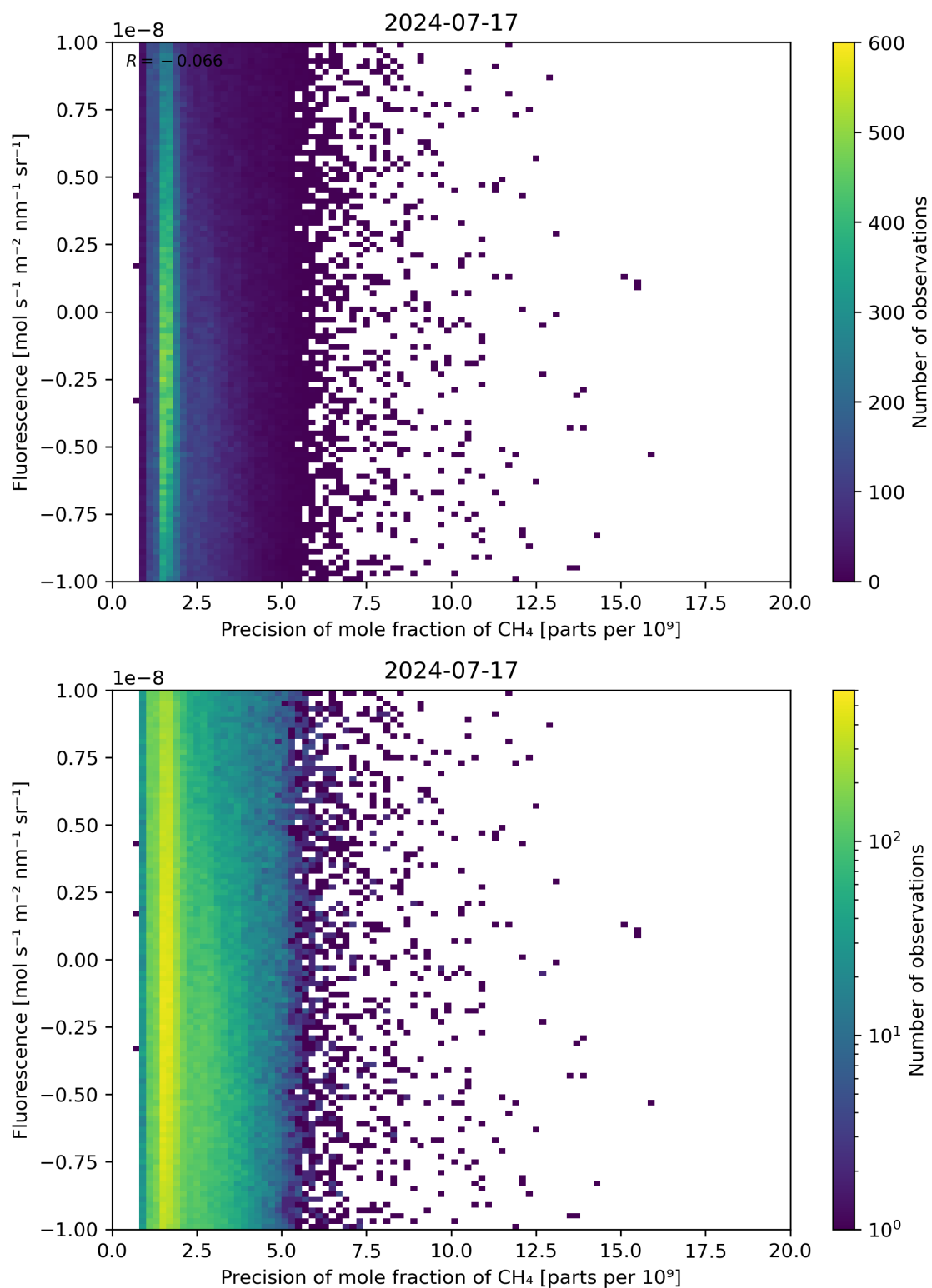
Figure 81: Scatter density plot of “Precision of mole fraction of \text{CH}_4 ” against “Fluorescence” for 2024-07-16 to 2024-07-18.
