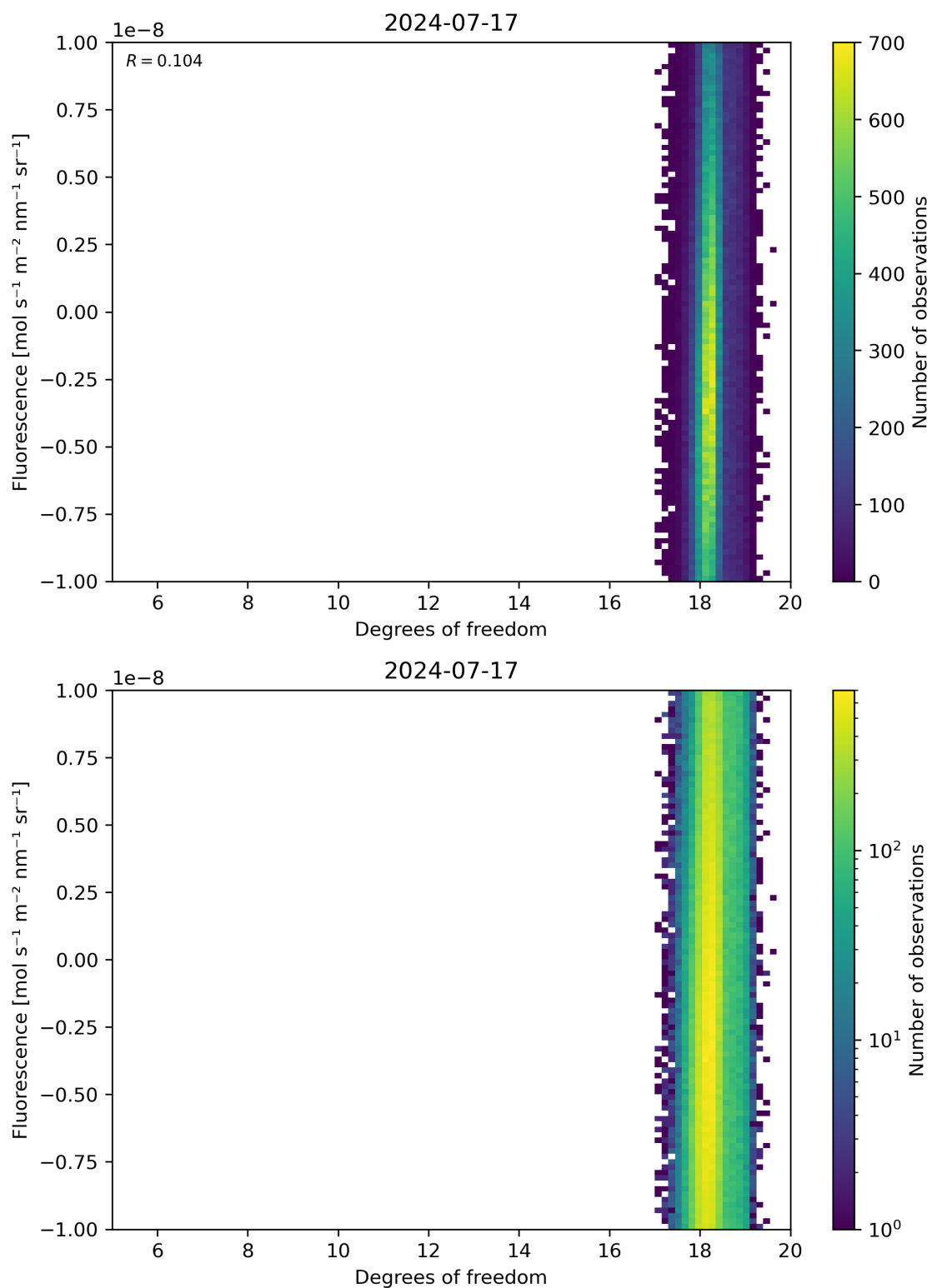
Figure 51: Scatter density plot of “Degrees of freedom” against “Fluorescence” for 2024-07-16 to 2024-07-18.
