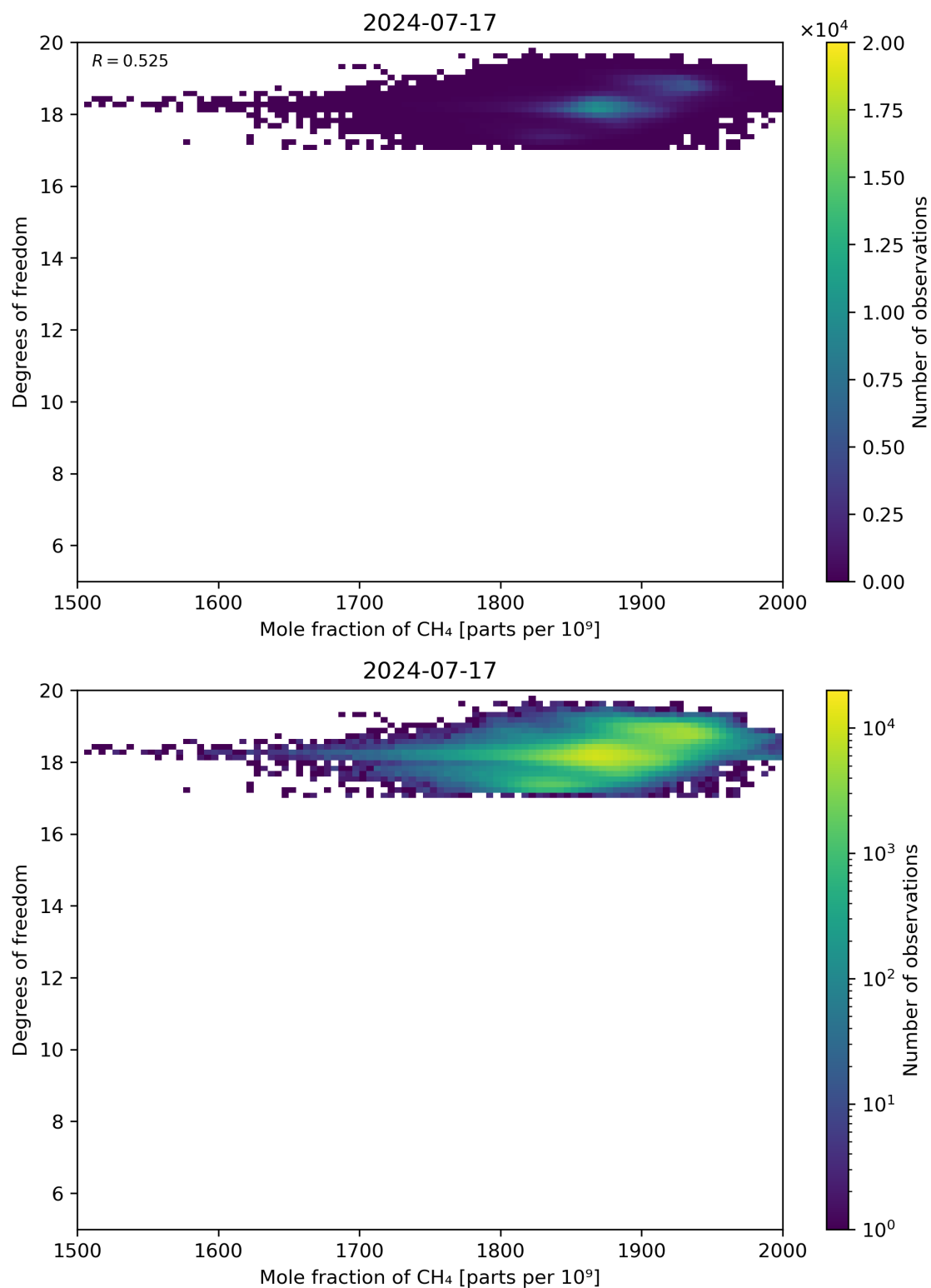
Figure 72: Scatter density plot of “Mole fraction of CH 4 ” against “Degrees of freedom” for 2024-07-16 to 2024-07-18.
