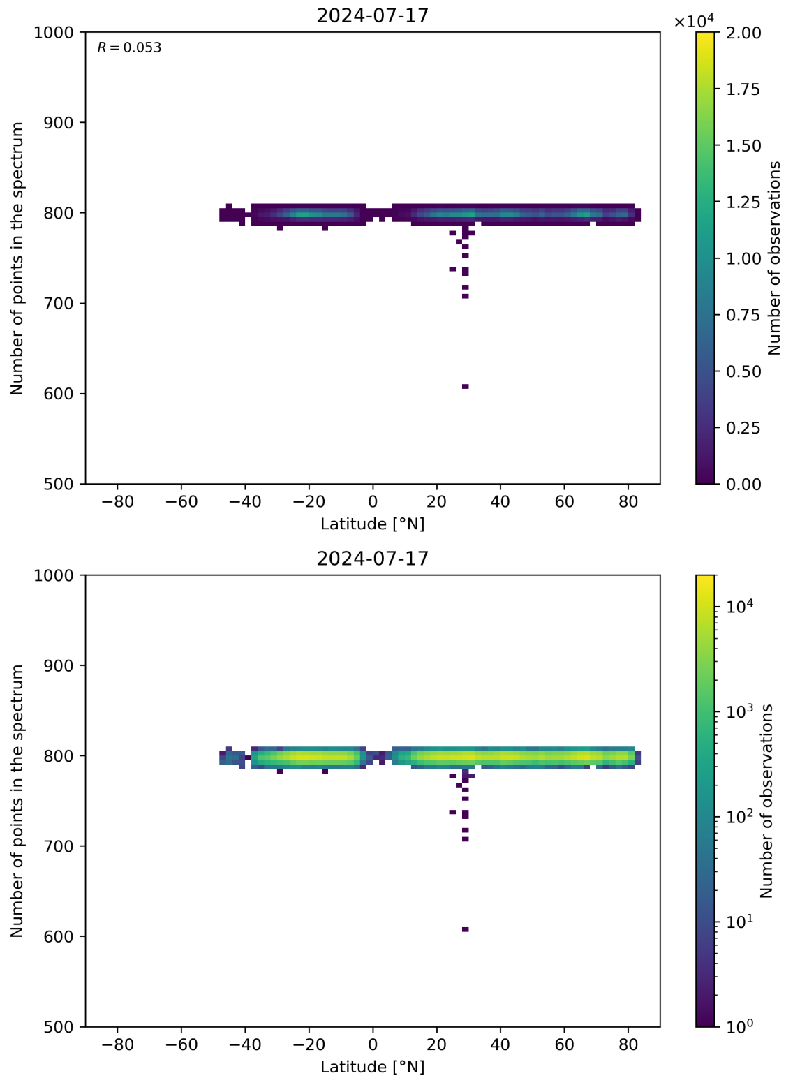
Figure 61: Scatter density plot of “Latitude” against “Number of points in the spectrum” for 2024-07-16 to 2024-07-18.
