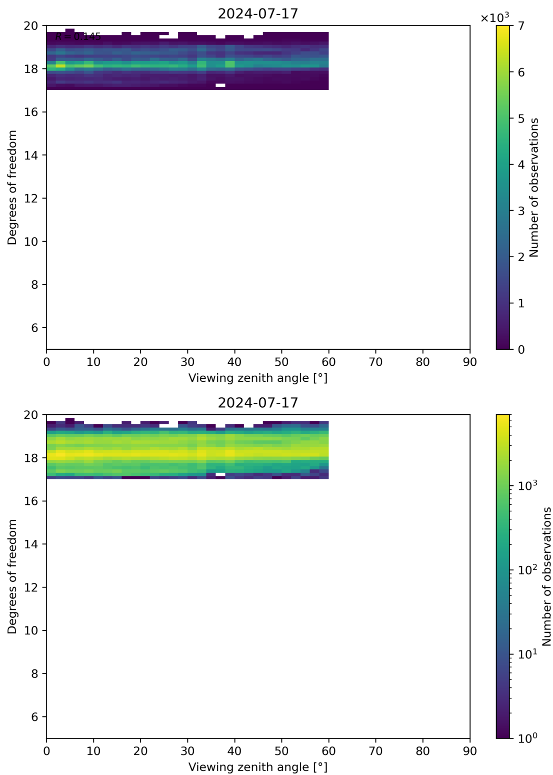
Figure 107: Scatter density plot of “Viewing zenith angle” against “Degrees of freedom” for 2024-07-16 to 2024-07-18.
