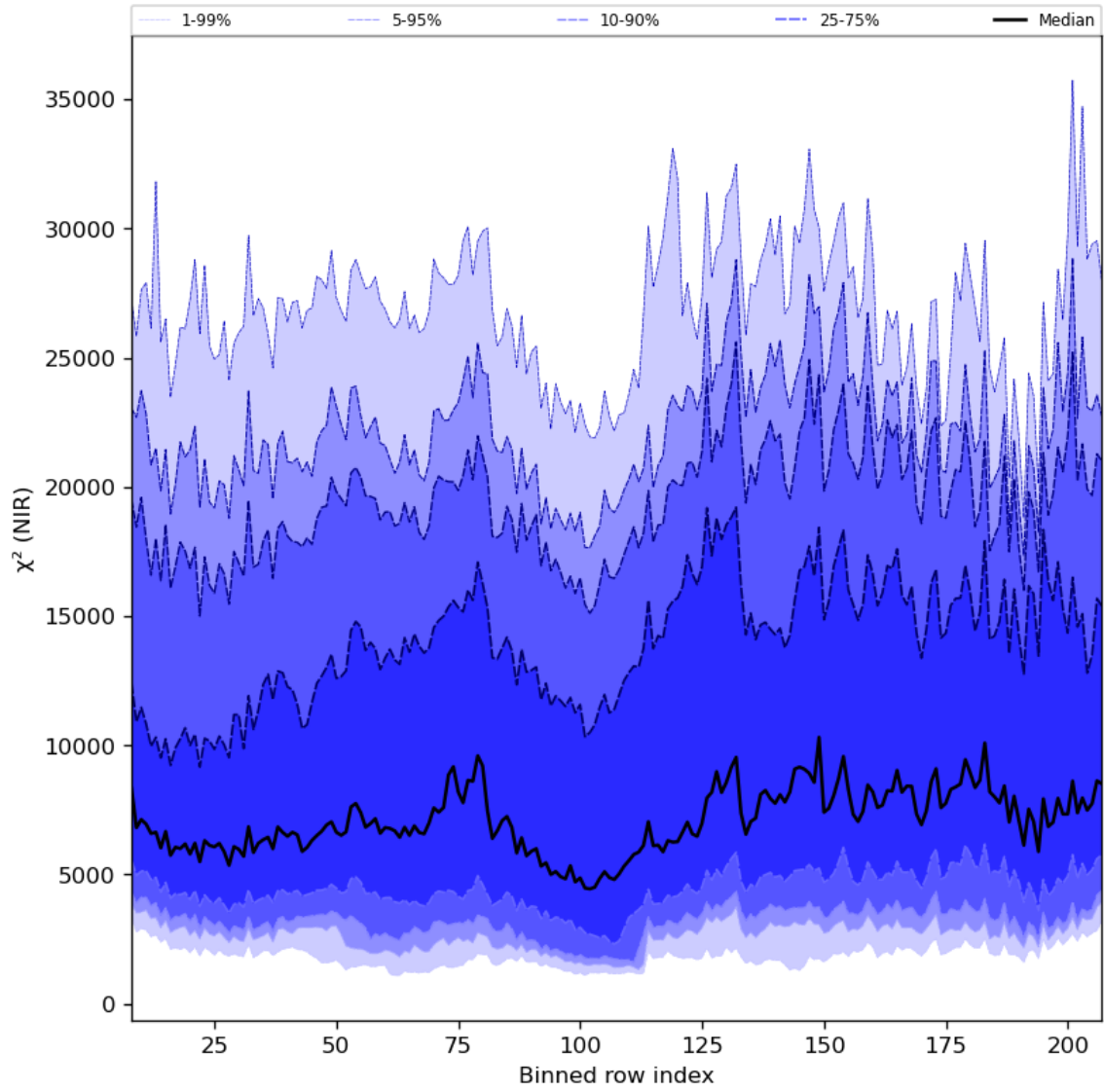
Figure 40: Along track statistics of “ \chi^2 (NIR)” for 2024-07-16 to 2024-07-18
