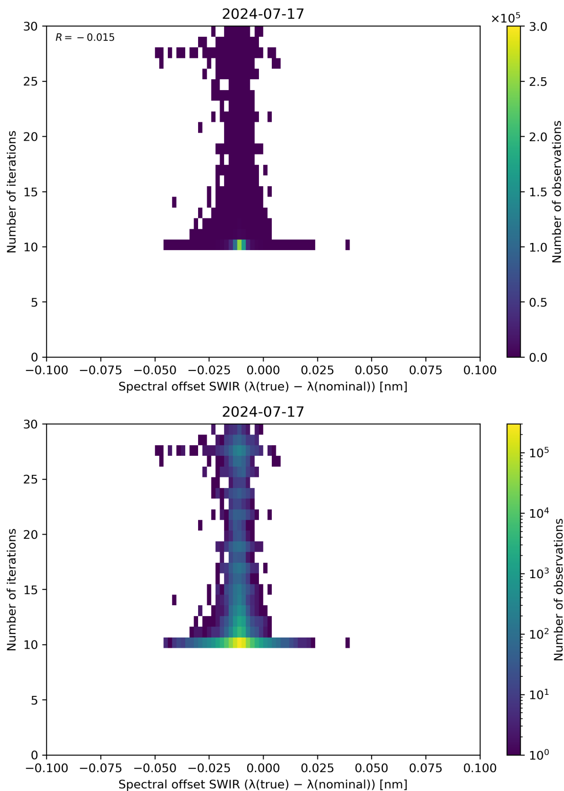
Figure 121: Scatter density plot of “Spectral offset SWIR ( \lambda(\text{true}) - \lambda(\text{nominal}) )” against “Number of iterations” for 2024-07-16 to 2024-07-18.
