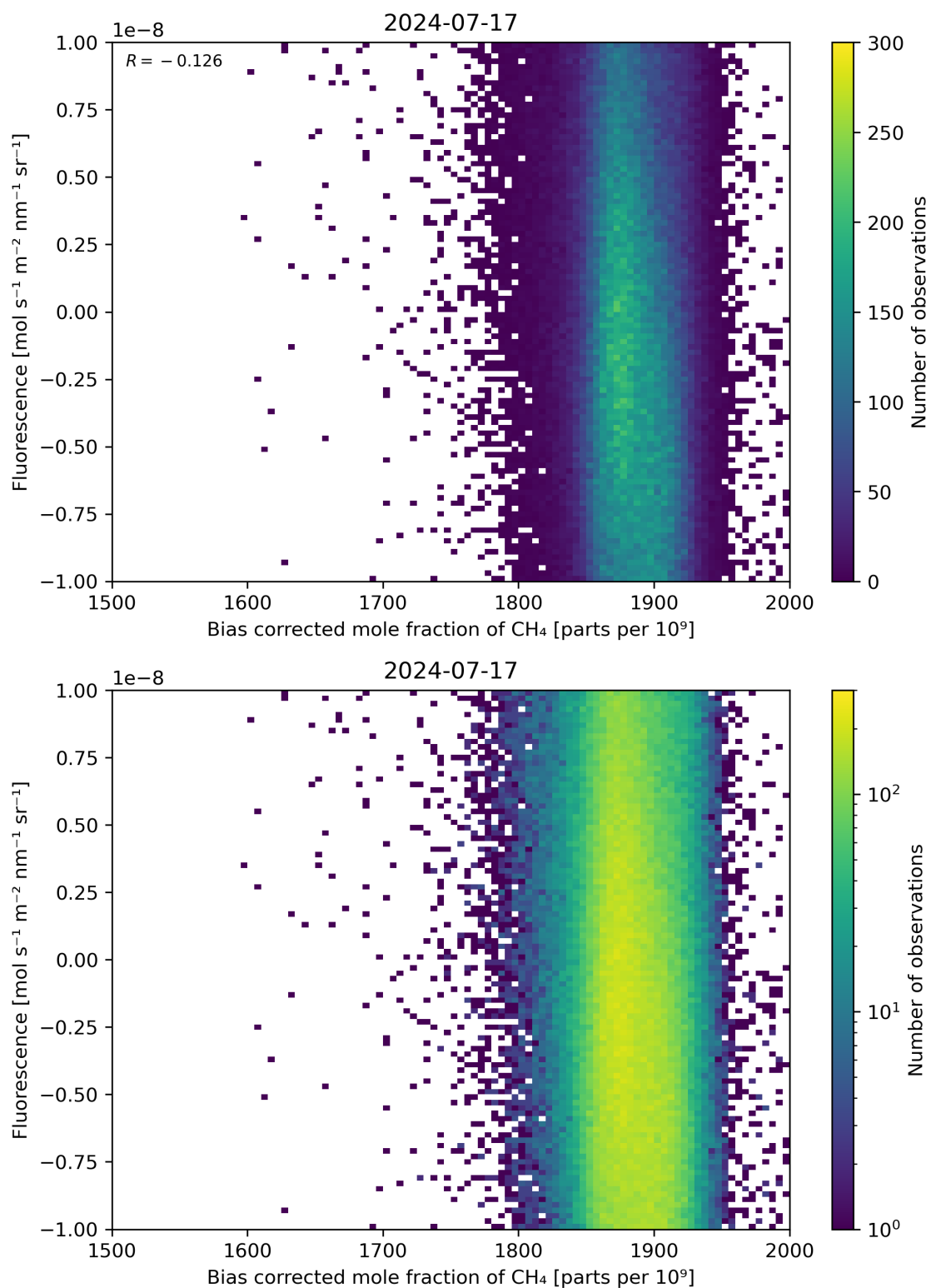
Figure 66: Scatter density plot of “Bias corrected mole fraction of \text{CH}_4 ” against “Fluorescence” for 2024-07-16 to 2024-07-18.
