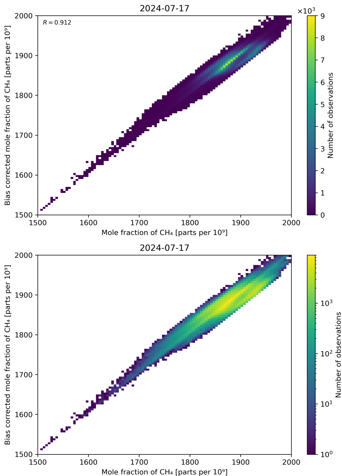
Figure 74: Scatter density plot of “Mole fraction of CH 4 ” against “Bias corrected mole fraction of CH 4 ” for 2024-07-16 to 2024-07-18.
