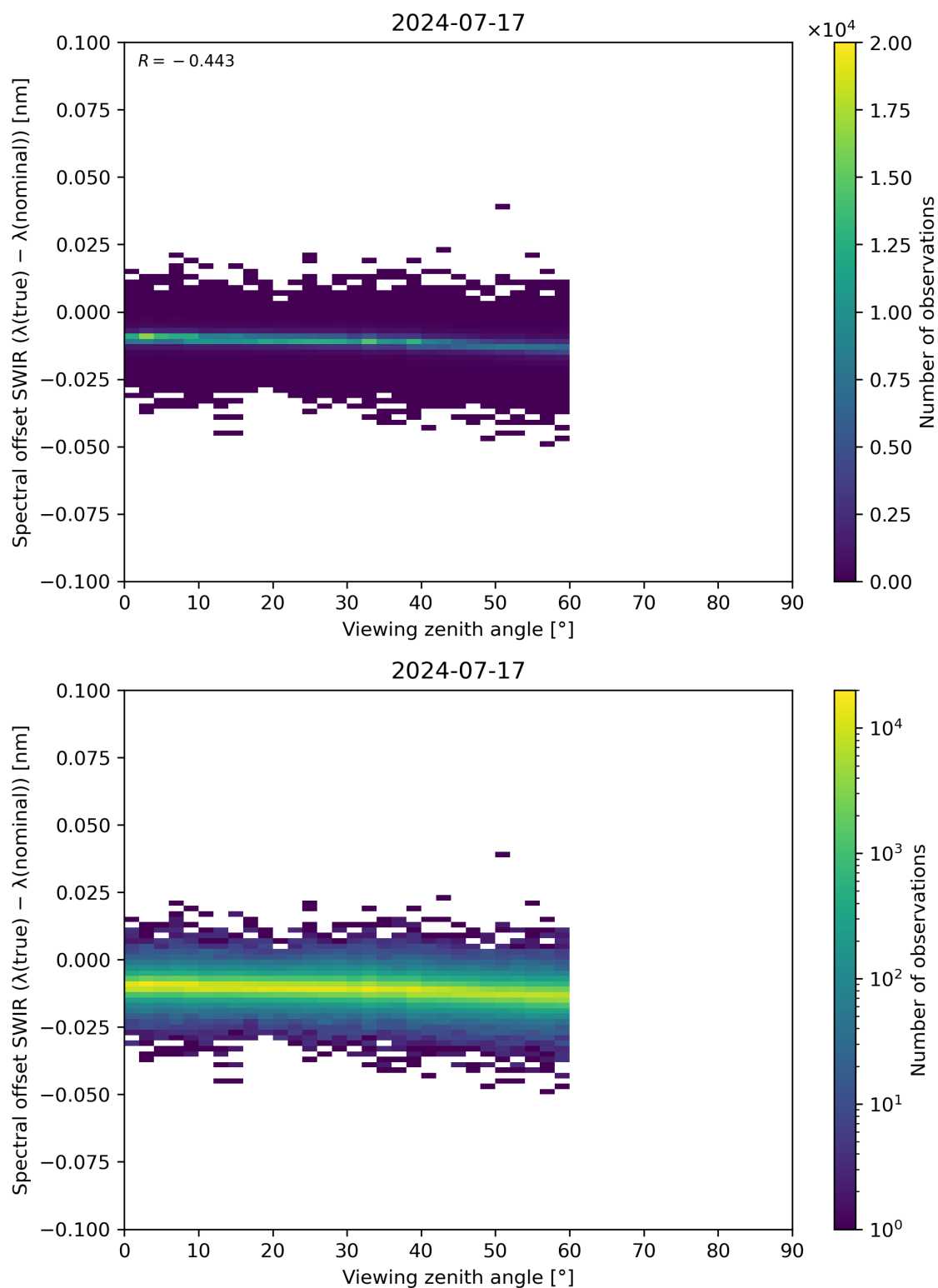
Figure 116: Scatter density plot of “Viewing zenith angle” against “Spectral offset SWIR ( \lambda(\text{true}) - \lambda(\text{nominal}) )” for 2024-07-16 to 2024-07-18.
