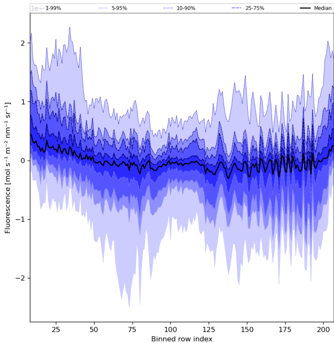
Figure 43: Along track statistics of “Fluorescence” for 2024-07-16 to 2024-07-18
