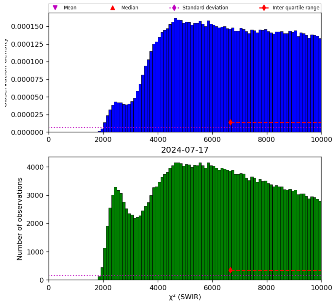
Figure 28: Histogram of “ \chi^2 (SWIR)” for 2024-07-16 to 2024-07-18
