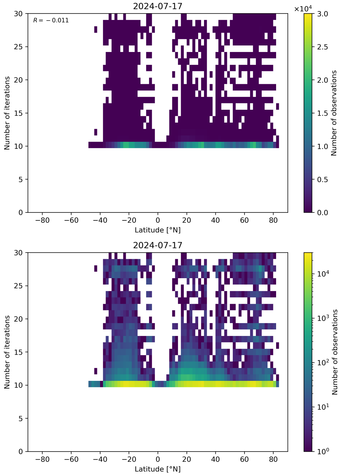
Figure 60: Scatter density plot of “Latitude” against “Number of iterations” for 2024-07-16 to 2024-07-18.
