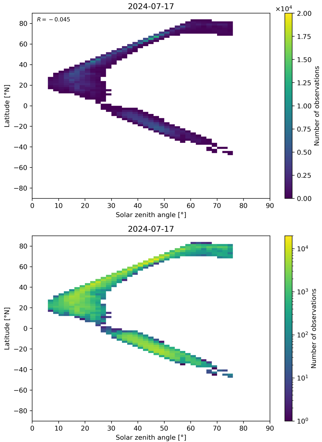
Figure 98: Scatter density plot of “Solar zenith angle” against “Latitude” for 2024-07-16 to 2024-07-18.
