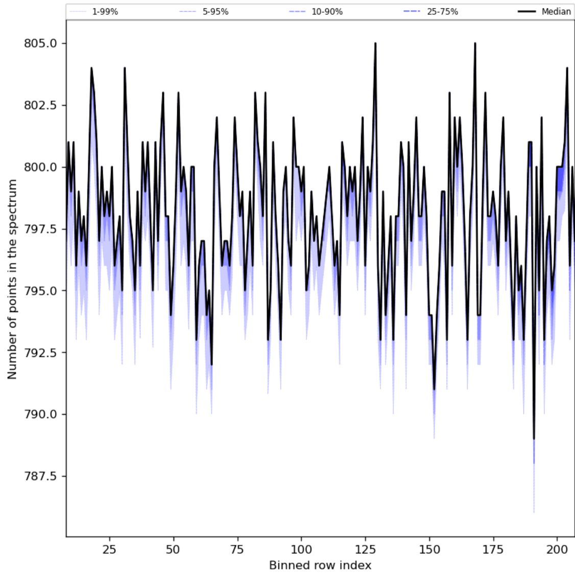
Figure 37: Along track statistics of “Number of points in the spectrum” for 2024-07-16 to 2024-07-18
