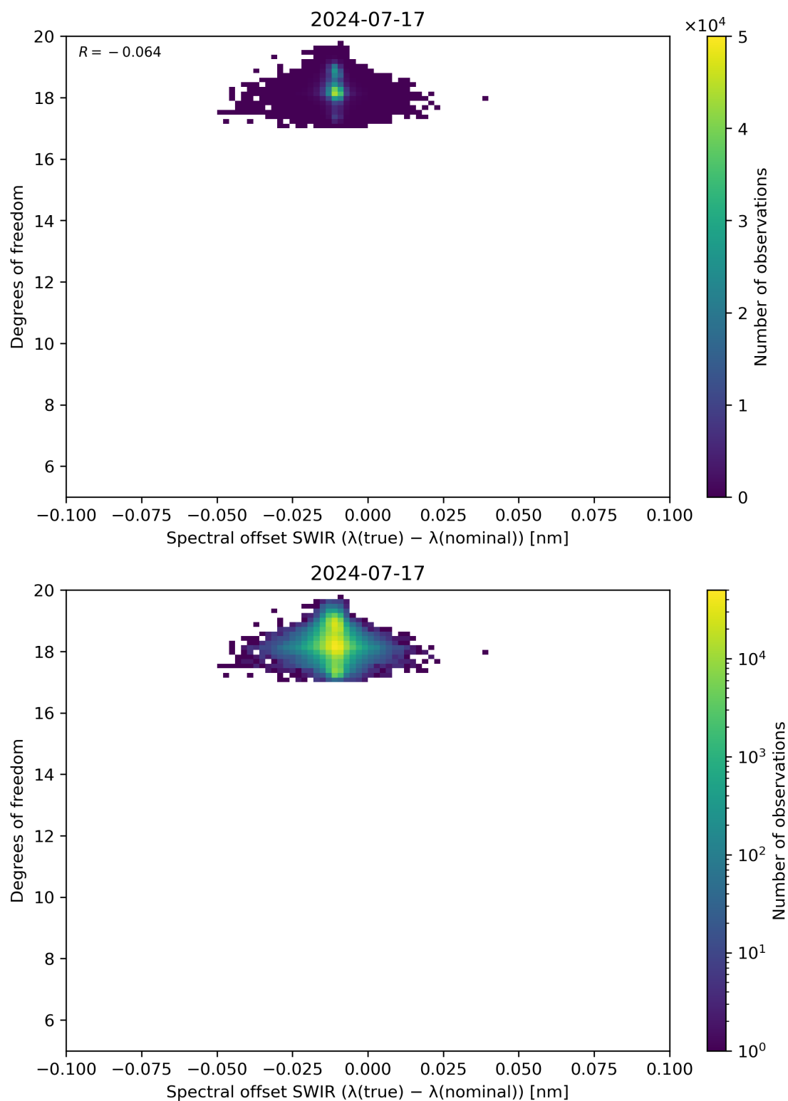
Figure 119: Scatter density plot of “Spectral offset SWIR ( \lambda(\text{true}) - \lambda(\text{nominal}) )” against “Degrees of freedom” for 2024-07-16 to 2024-07-18.
