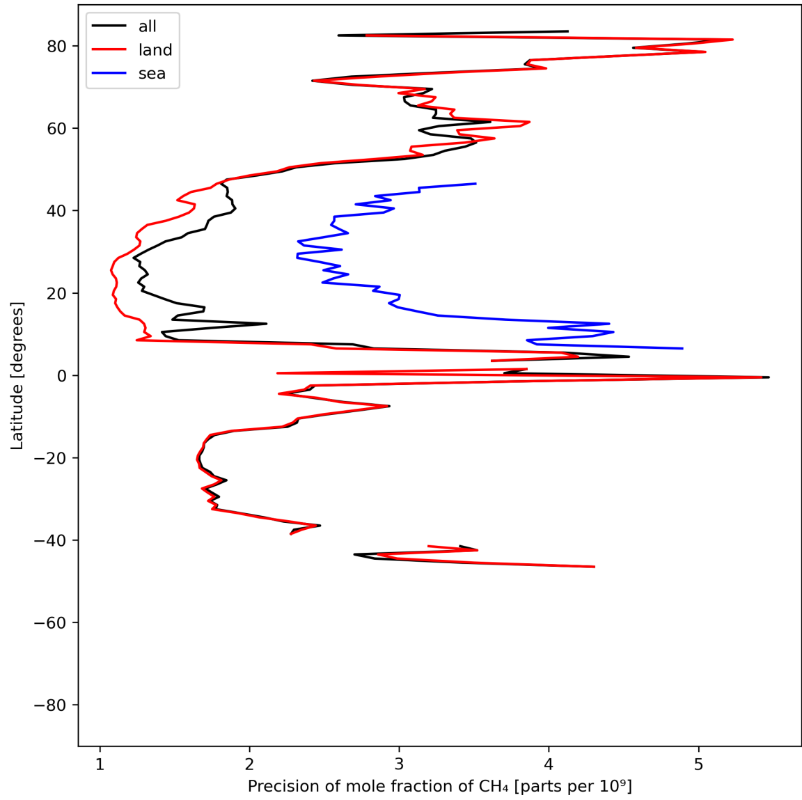
Figure 13: Zonal average of “Precision of mole fraction of CH 4 ” for 2024-07-16 to 2024-07-18.
