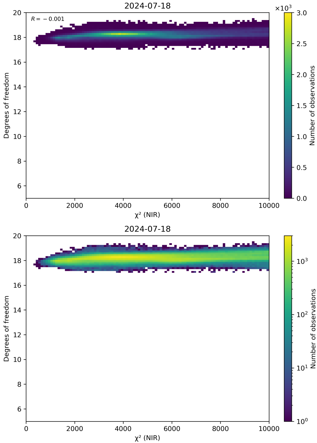
Figure 44: Scatter density plot of “ \chi^2 (NIR)” against “Degrees of freedom” for 2024-07-17 to 2024-07-19.
