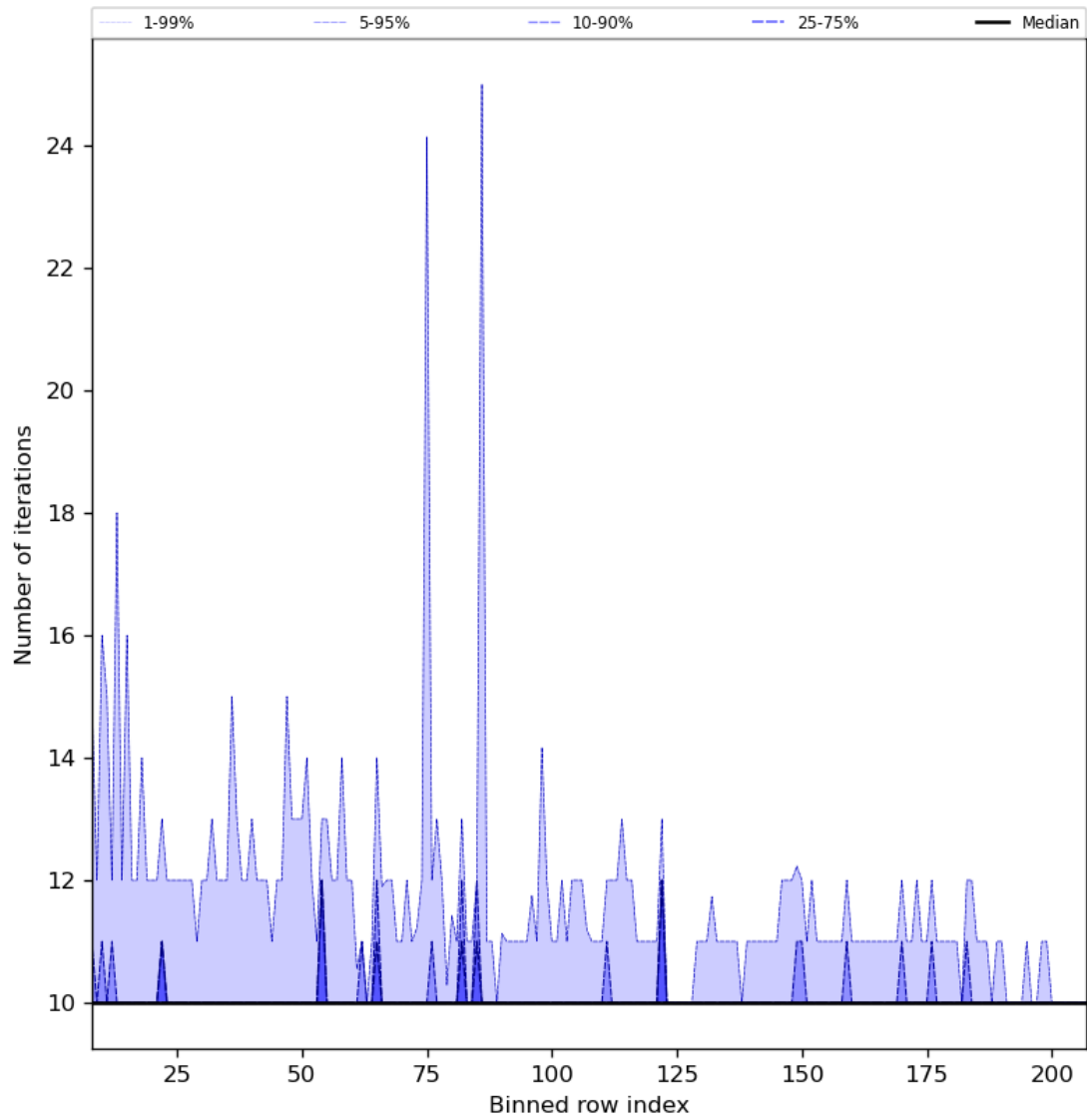
Figure 42: Along track statistics of “Number of iterations” for 2024-07-17 to 2024-07-19
