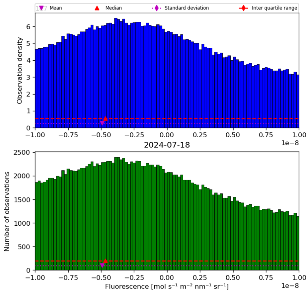
Figure 32: Histogram of “Fluorescence” for 2024-07-17 to 2024-07-19
