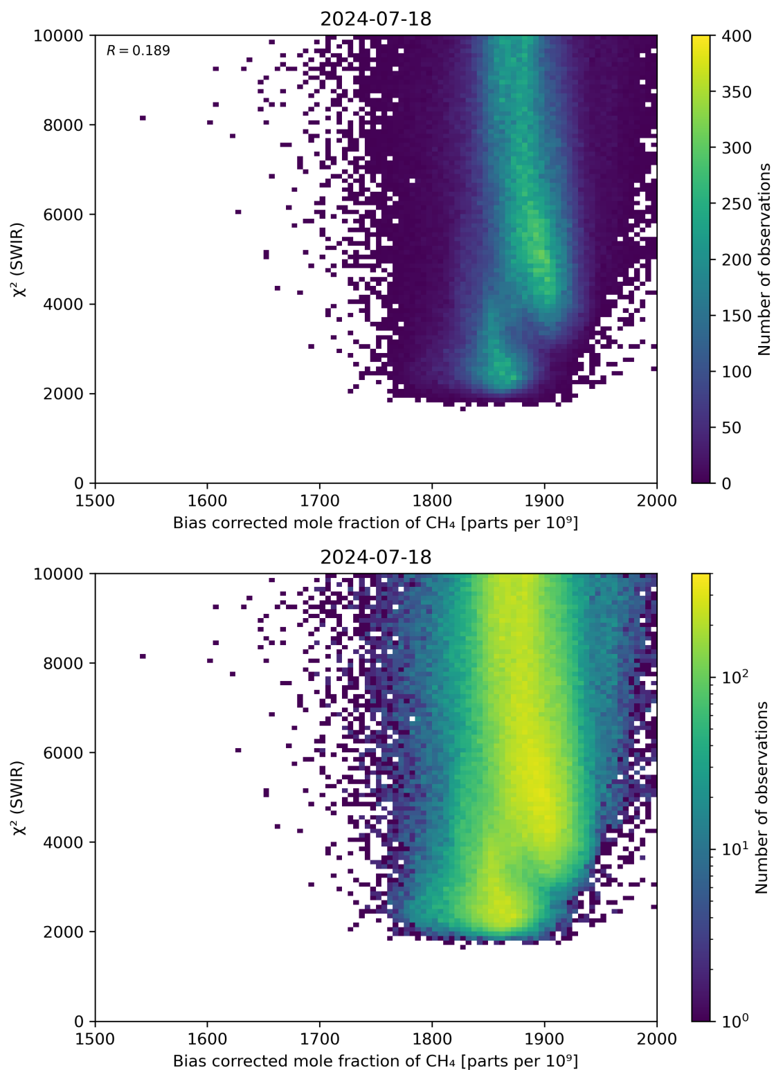
Figure 64: Scatter density plot of “Bias corrected mole fraction of \text{CH}_4 ” against “ \chi^2 (SWIR)” for 2024-07-17 to 2024-07-19.
