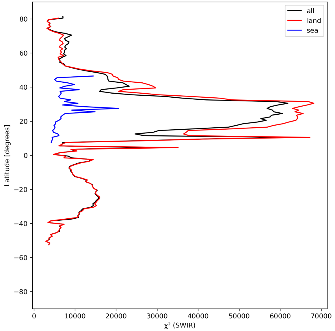
Figure 17: Zonal average of “ \chi^2 (SWIR)” for 2024-07-17 to 2024-07-19.
