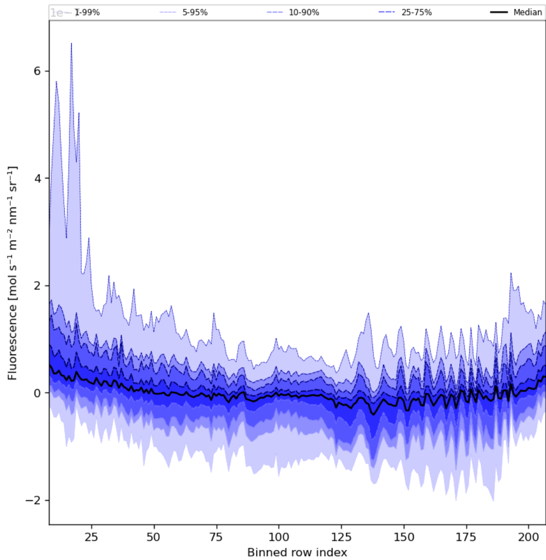
Figure 43: Along track statistics of “Fluorescence” for 2024-07-17 to 2024-07-19
