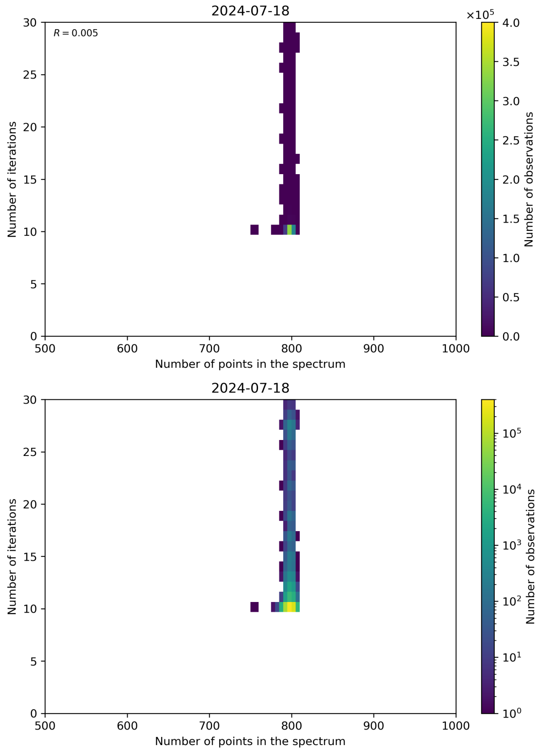
Figure 92: Scatter density plot of “Number of points in the spectrum” against “Number of iterations” for 2024-07-17 to 2024-07-19.
