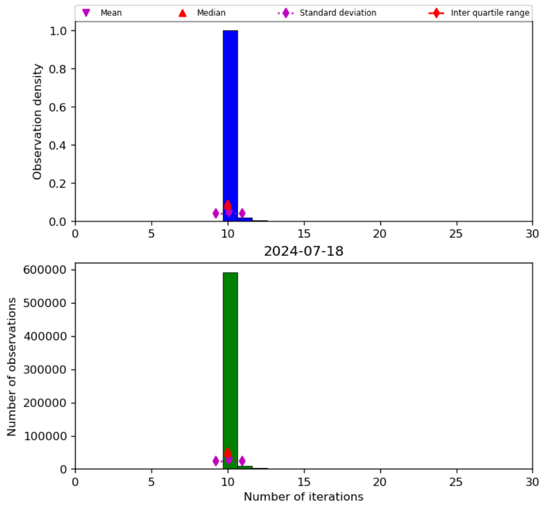
Figure 31: Histogram of “Number of iterations” for 2024-07-17 to 2024-07-19
