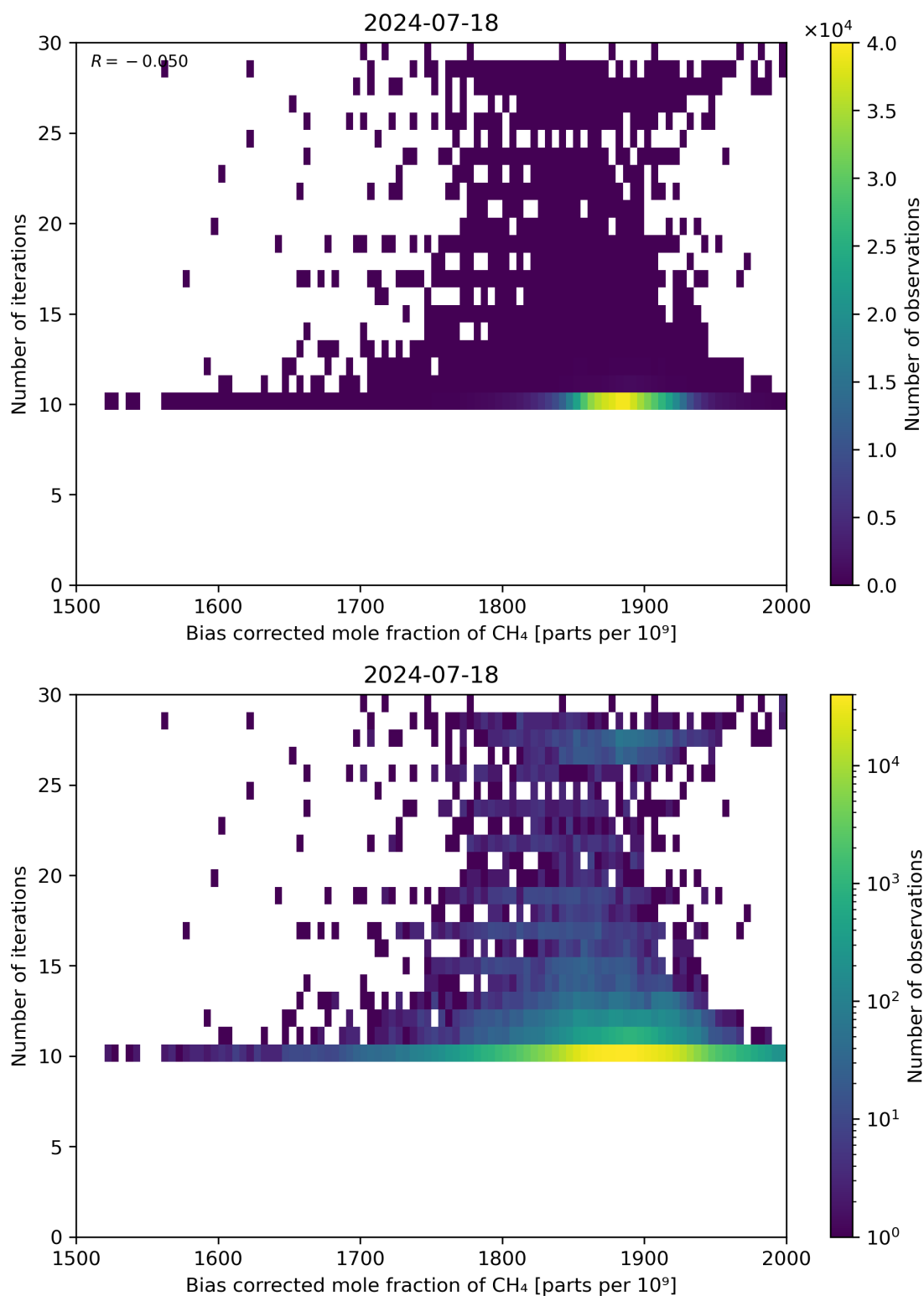
Figure 67: Scatter density plot of “Bias corrected mole fraction of CH 4 ” against “Number of iterations” for 2024-07-17 to 2024-07-19.
