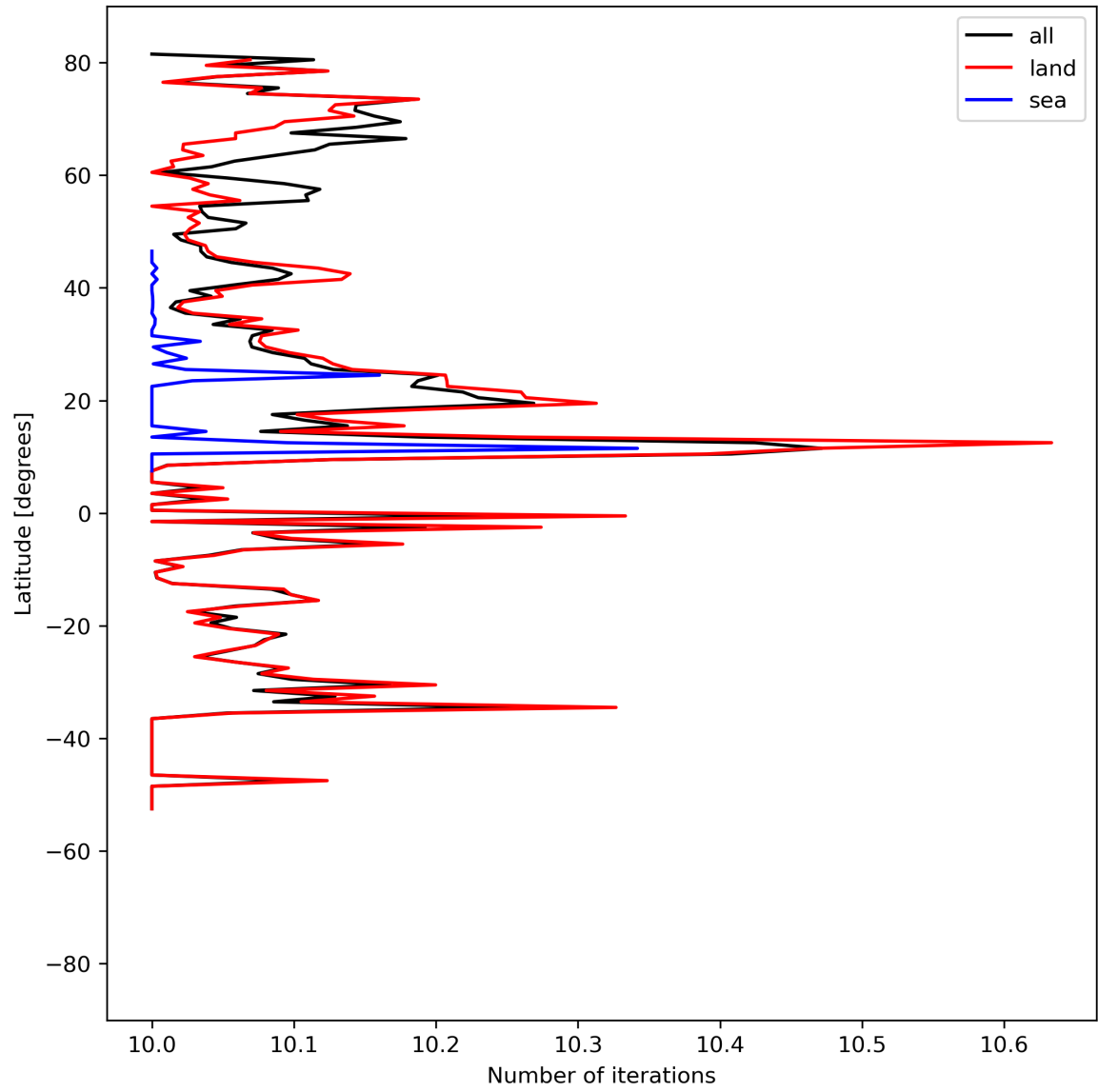
Figure 20: Zonal average of “Number of iterations” for 2024-07-17 to 2024-07-19.
