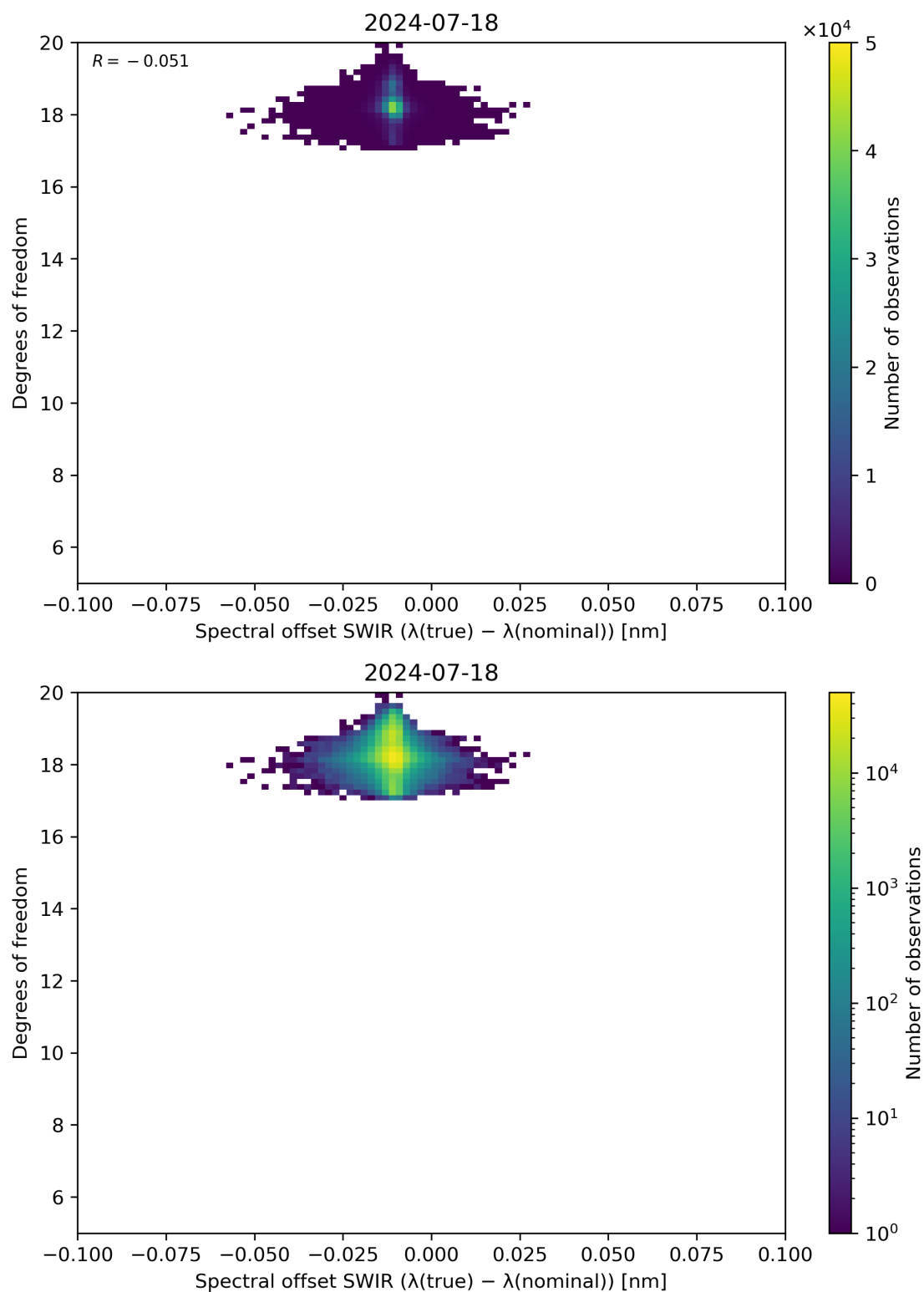
Figure 119: Scatter density plot of “Spectral offset SWIR ( \lambda(\text{true}) - \lambda(\text{nominal}) )” against “Degrees of freedom” for 2024-07-17 to 2024-07-19.
