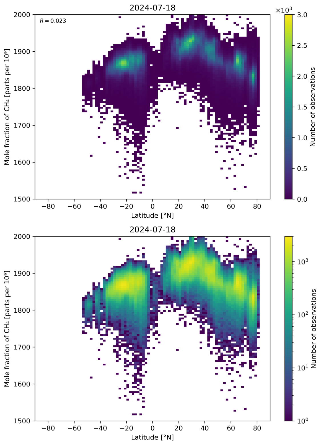
Figure 57: Scatter density plot of “Latitude” against “Mole fraction of \text{CH}_4 ” for 2024-07-17 to 2024-07-19.
