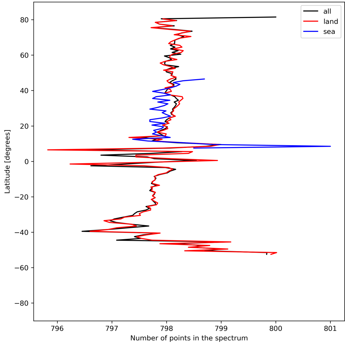
Figure 15: Zonal average of “Number of points in the spectrum” for 2024-07-17 to 2024-07-19.
