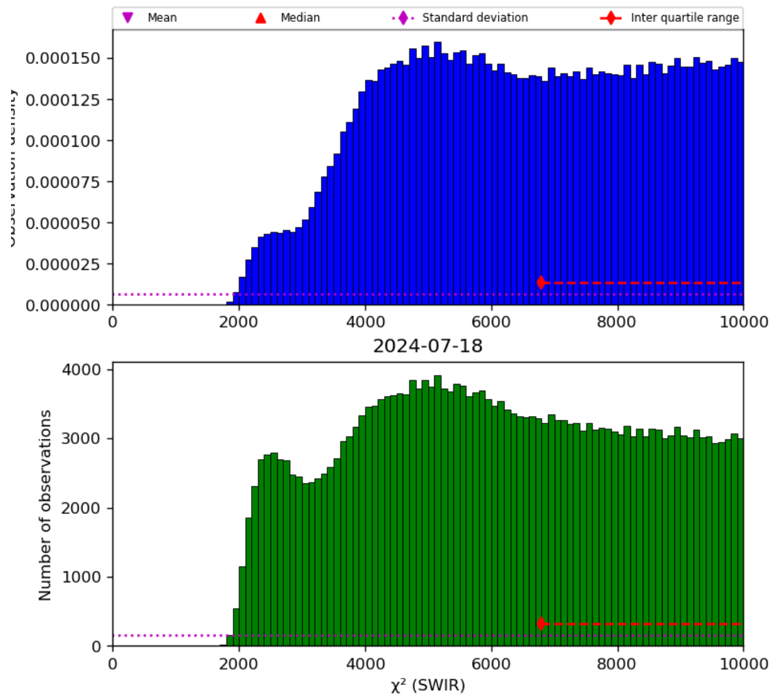
Figure 28: Histogram of “ \chi^2 (SWIR)” for 2024-07-17 to 2024-07-19
