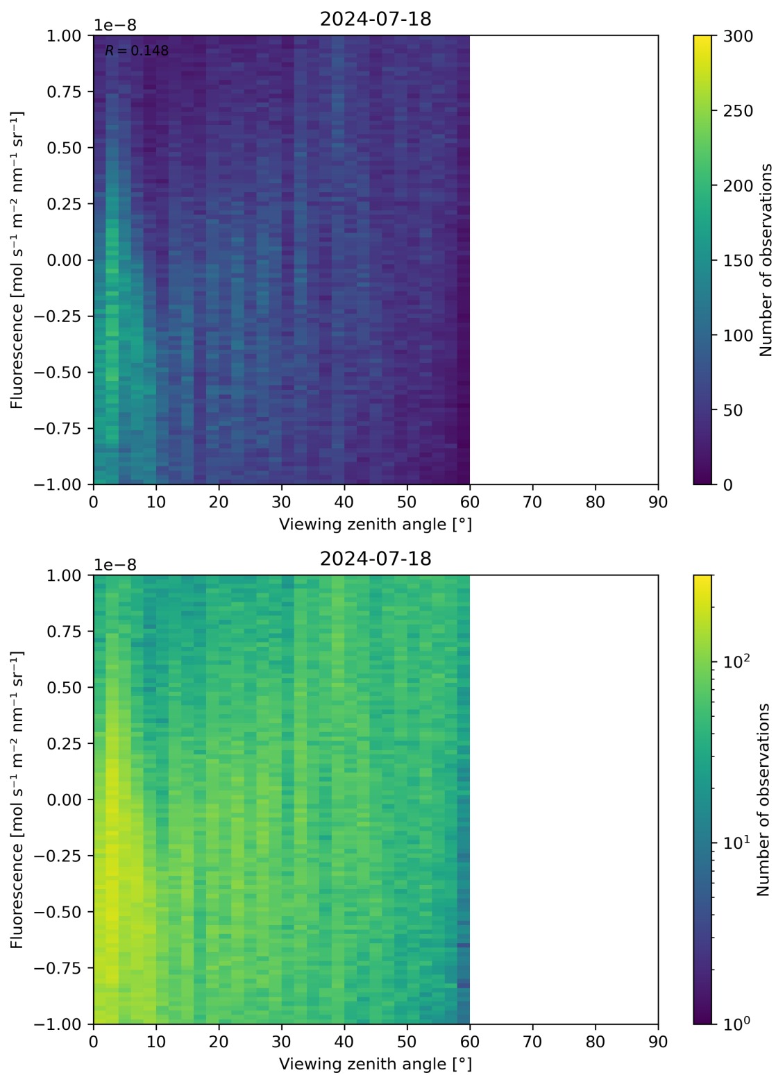
Figure 108: Scatter density plot of “Viewing zenith angle” against “Fluorescence” for 2024-07-17 to 2024-07-19.
