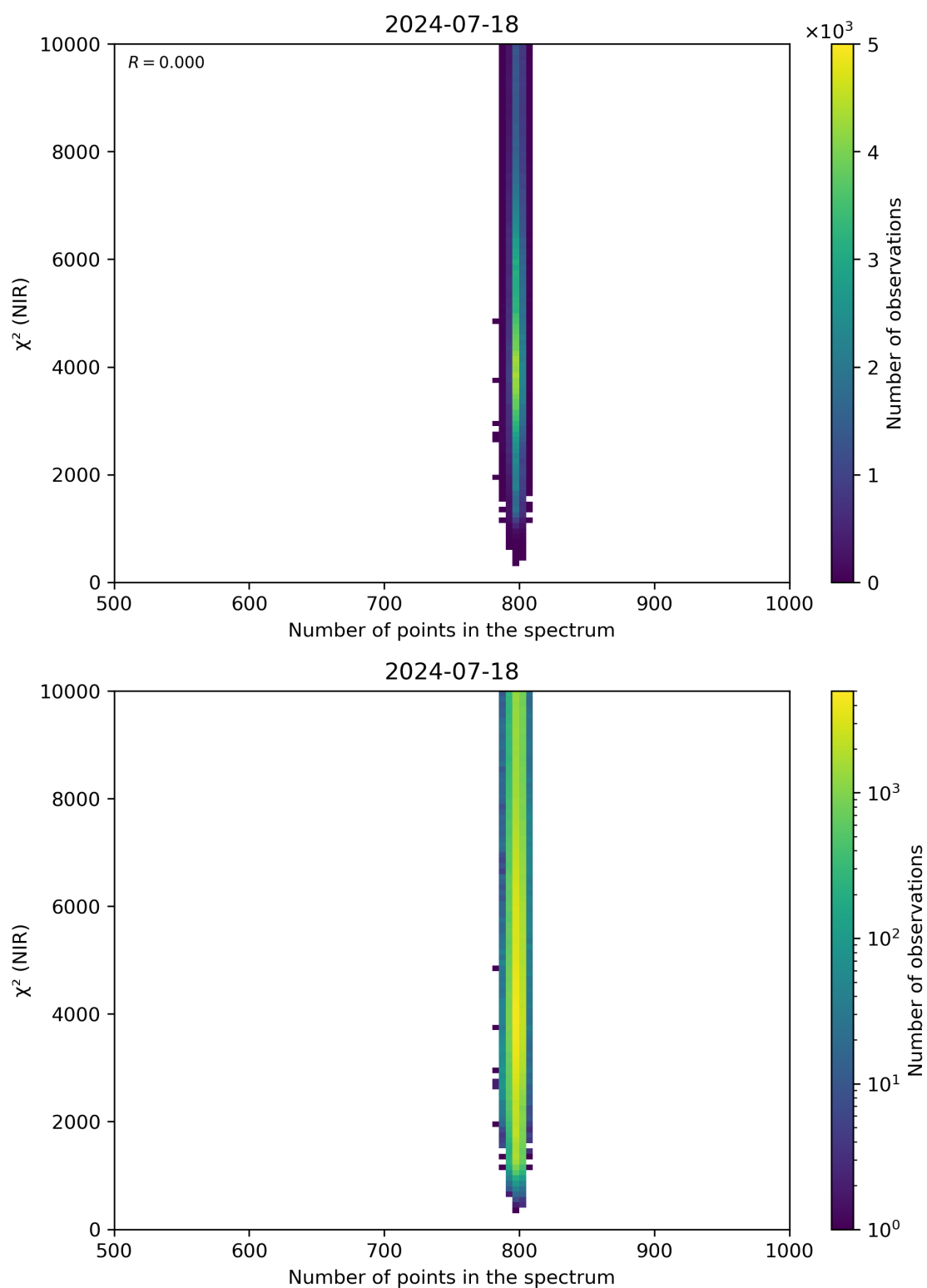
Figure 88: Scatter density plot of “Number of points in the spectrum” against “ \chi^2 (NIR)” for 2024-07-17 to 2024-07-19.
