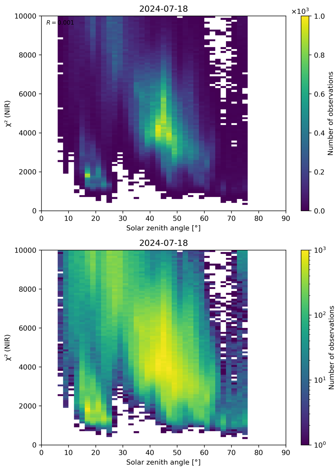
Figure 94: Scatter density plot of “Solar zenith angle” against “ \chi^2 (NIR)” for 2024-07-17 to 2024-07-19.
