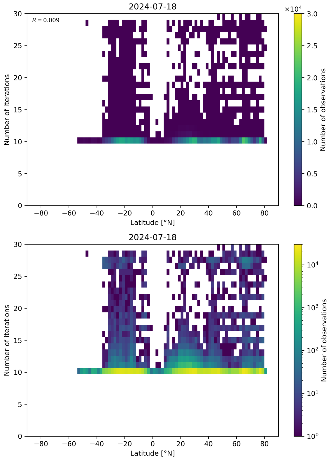
Figure 60: Scatter density plot of “Latitude” against “Number of iterations” for 2024-07-17 to 2024-07-19.
