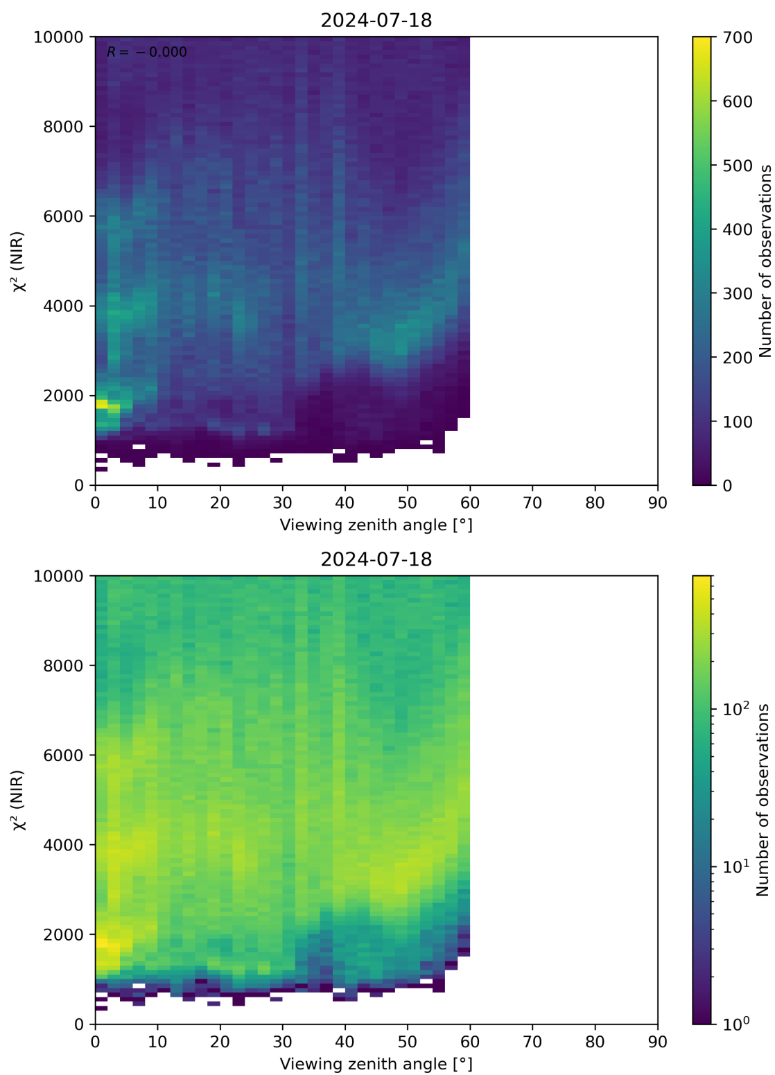
Figure 105: Scatter density plot of “Viewing zenith angle” against “ \chi^2 (NIR)” for 2024-07-17 to 2024-07-19.
