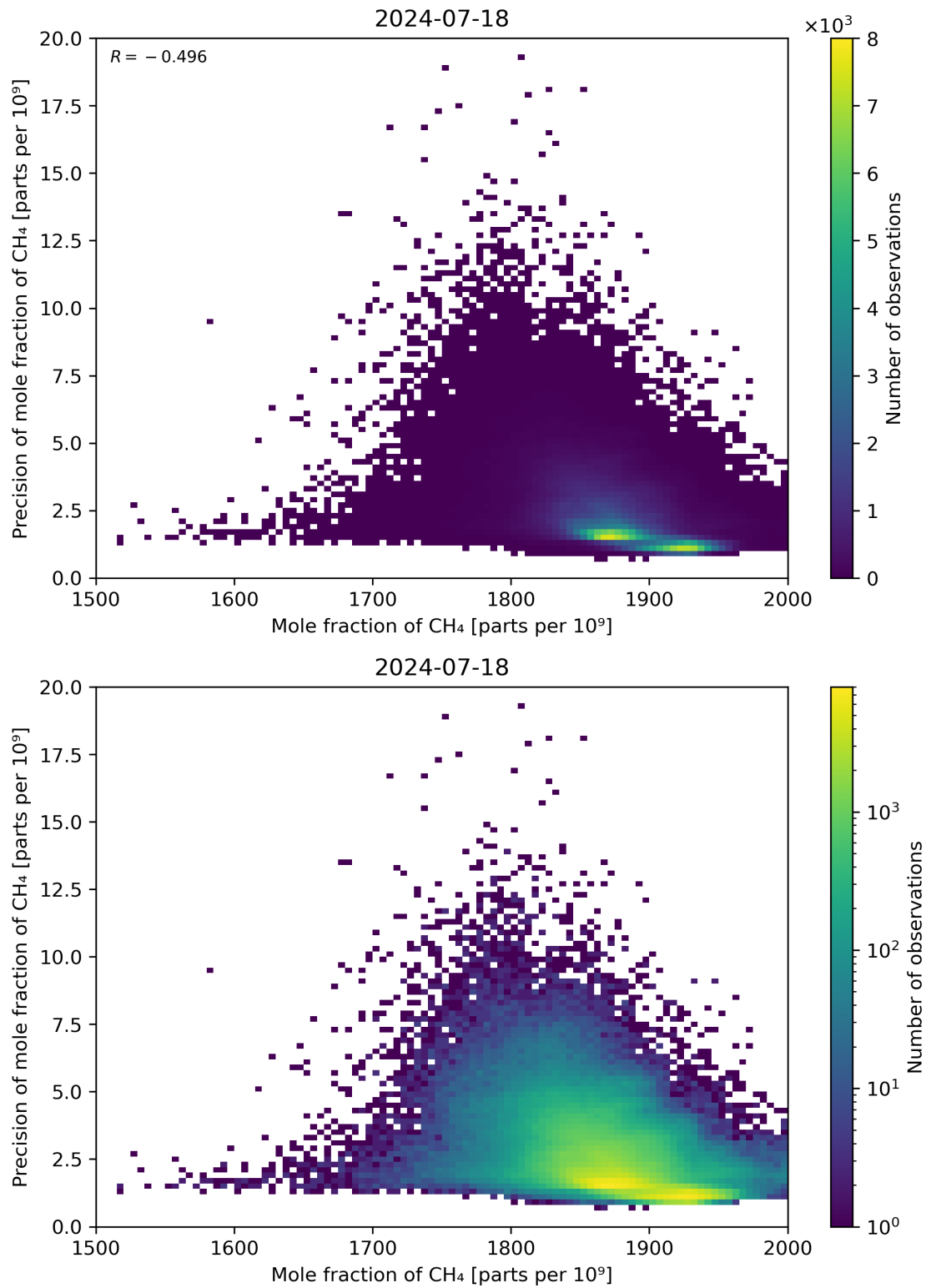
Figure 75: Scatter density plot of “Mole fraction of CH 4 ” against “Precision of mole fraction of CH 4 ” for 2024-07-17 to 2024-07-19.
