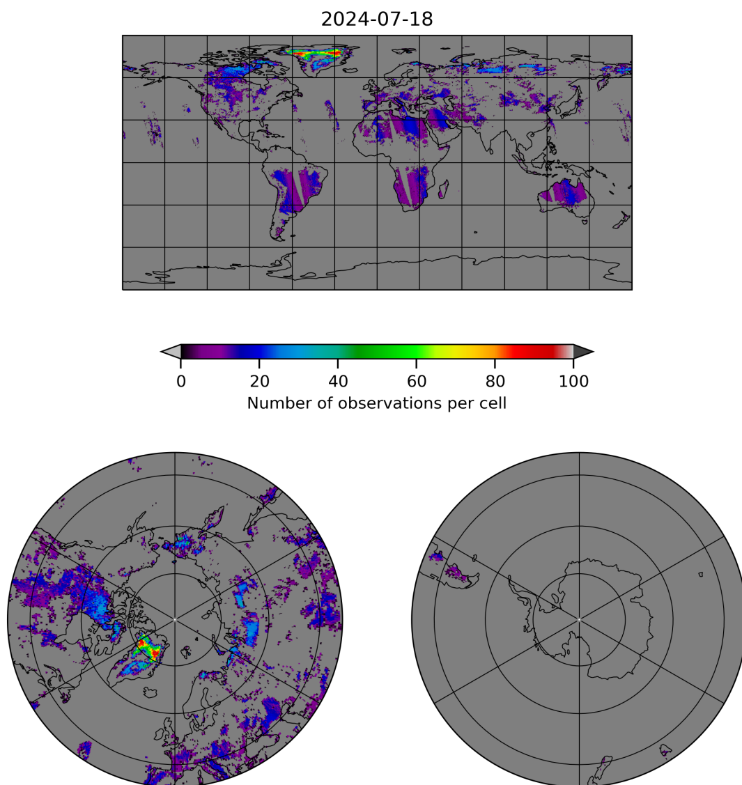
Figure 10: Map of the number of observations for 2024-07-17 to 2024-07-19
