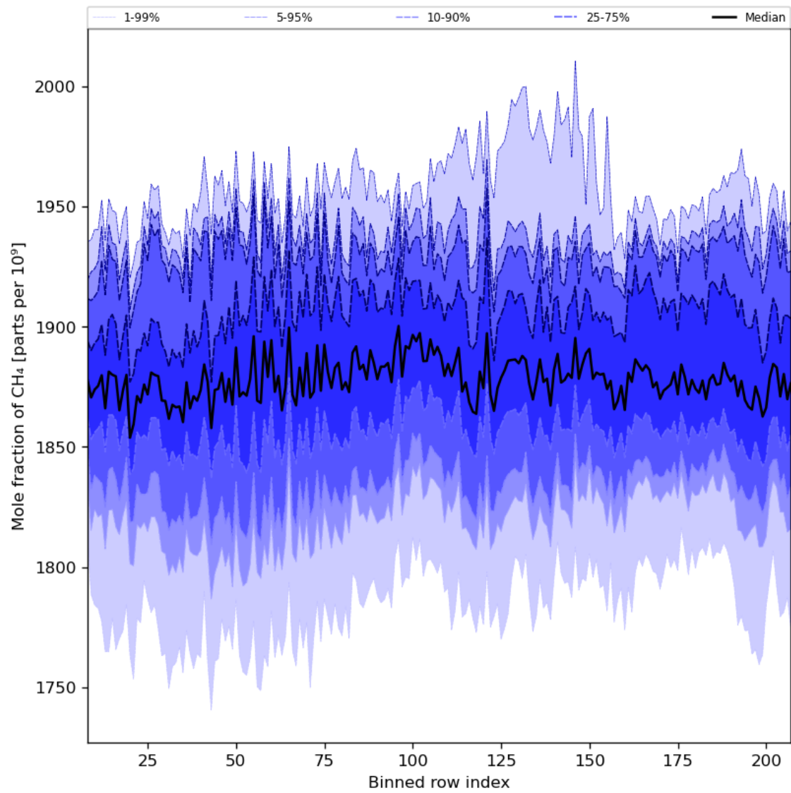
Figure 34: Along track statistics of “Mole fraction of CH 4 ” for 2024-07-17 to 2024-07-19
