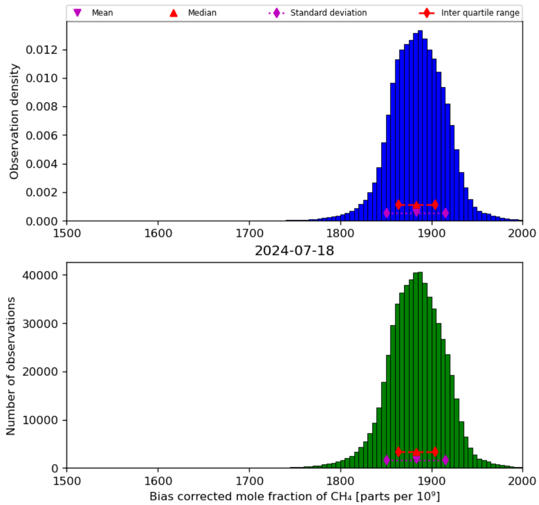
Figure 25: Histogram of “Bias corrected mole fraction of CH 4 ” for 2024-07-17 to 2024-07-19
