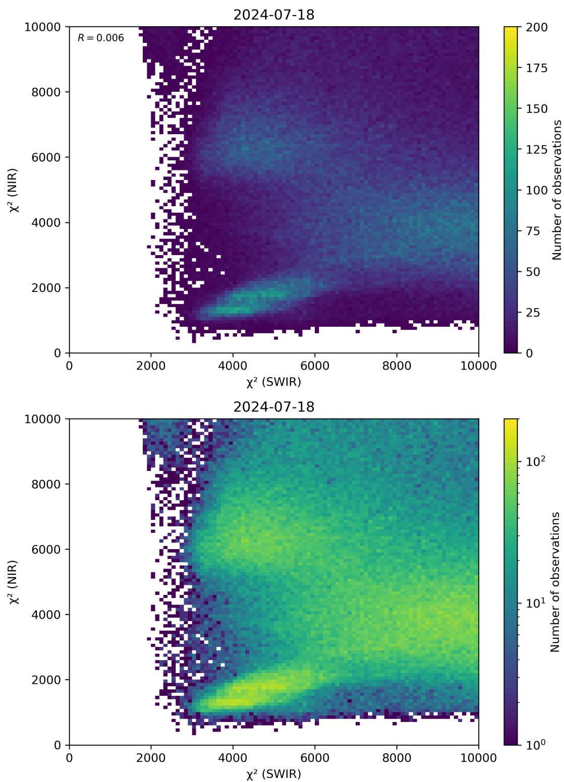
Figure 47: Scatter density plot of " \chi^2 (SWIR)" against " \chi^2 (NIR)" for 2024-07-17 to 2024-07-19.
