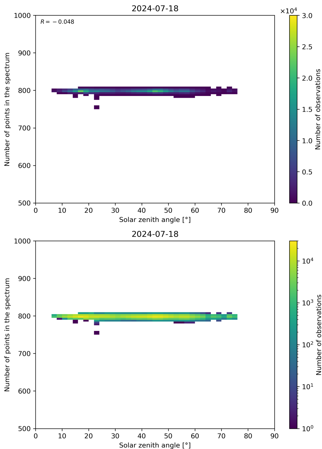
Figure 103: Scatter density plot of “Solar zenith angle” against “Number of points in the spectrum” for 2024-07-17 to 2024-07-19.
