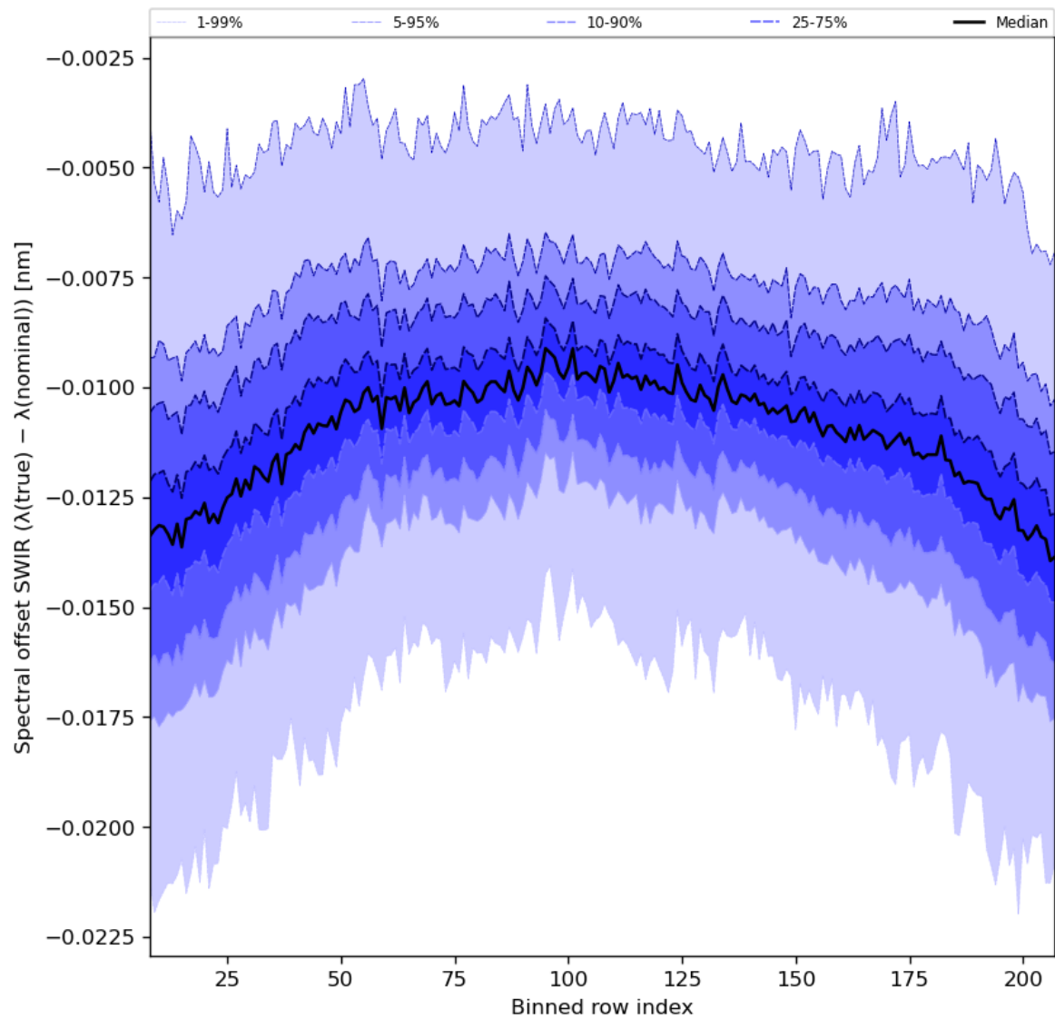
Figure 38: Along track statistics of “Spectral offset SWIR ( \lambda(\text{true}) - \lambda(\text{nominal}) )” for 2024-07-17 to 2024-07-19
