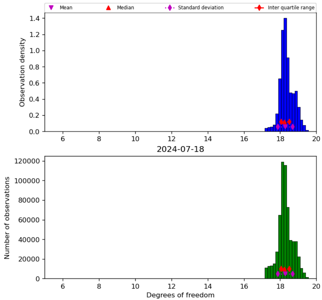
Figure 30: Histogram of “Degrees of freedom” for 2024-07-17 to 2024-07-19
