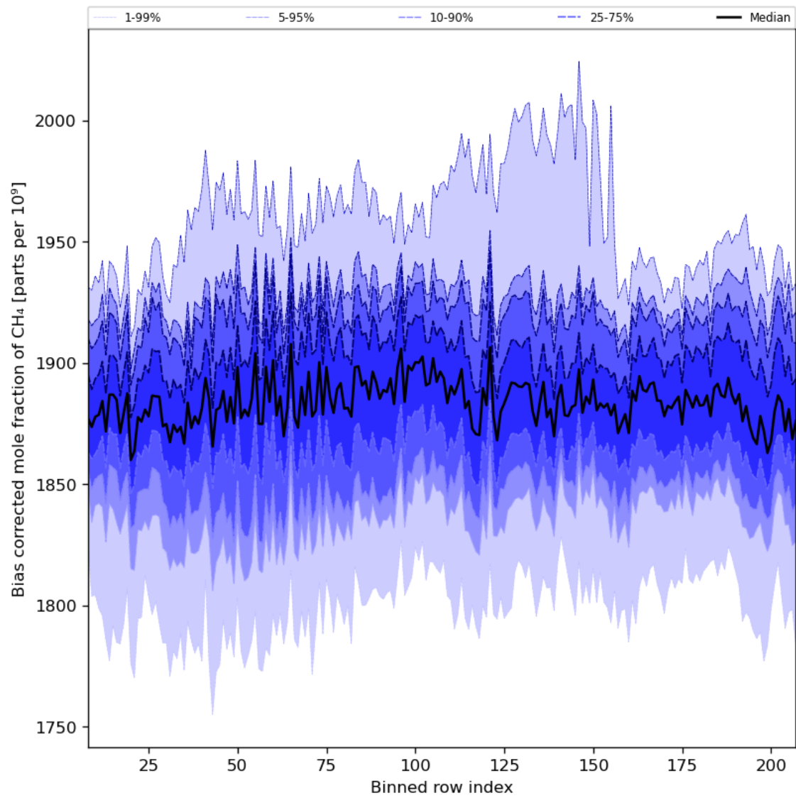
Figure 36: Along track statistics of “Bias corrected mole fraction of CH 4 ” for 2024-07-17 to 2024-07-19
