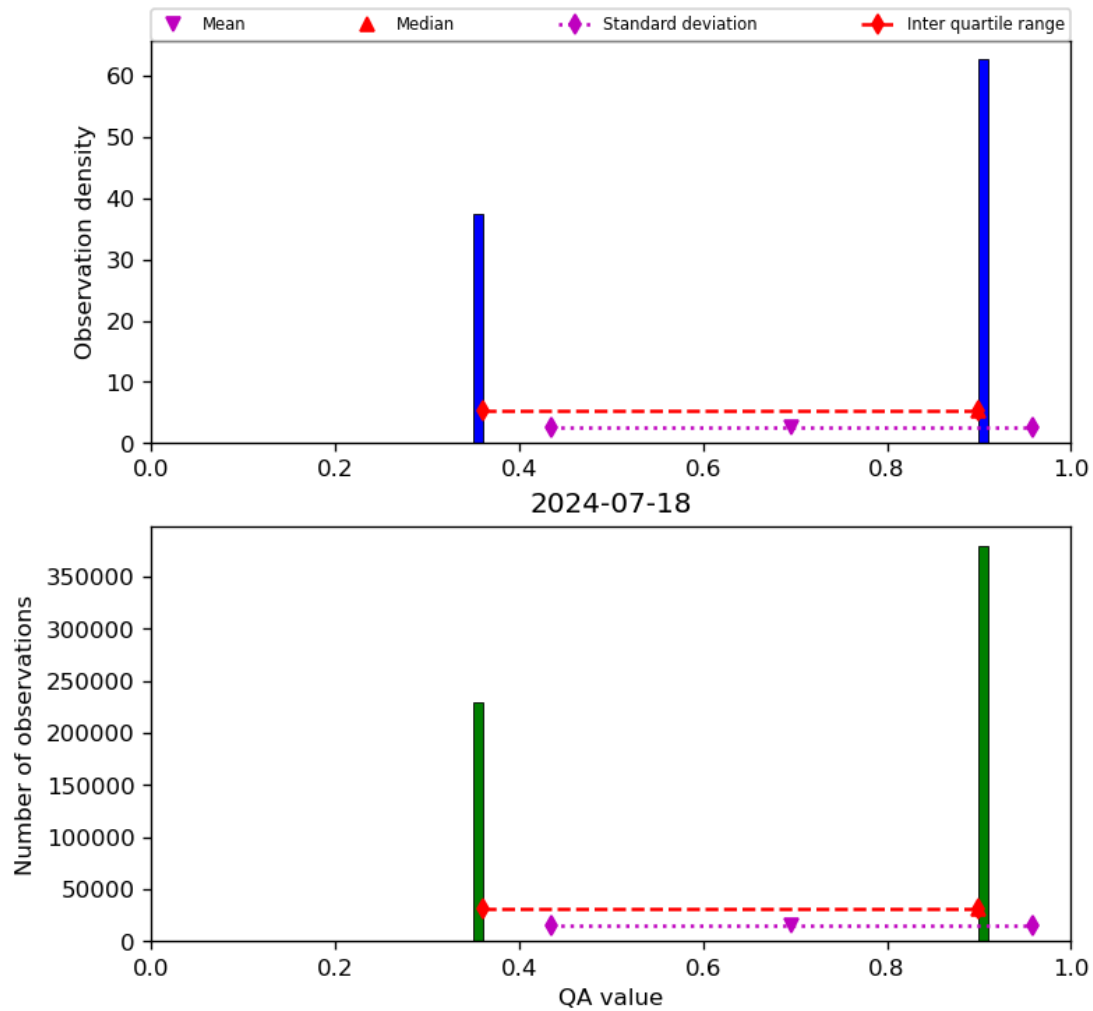
Figure 22: Histogram of “QA value” for 2024-07-17 to 2024-07-19
