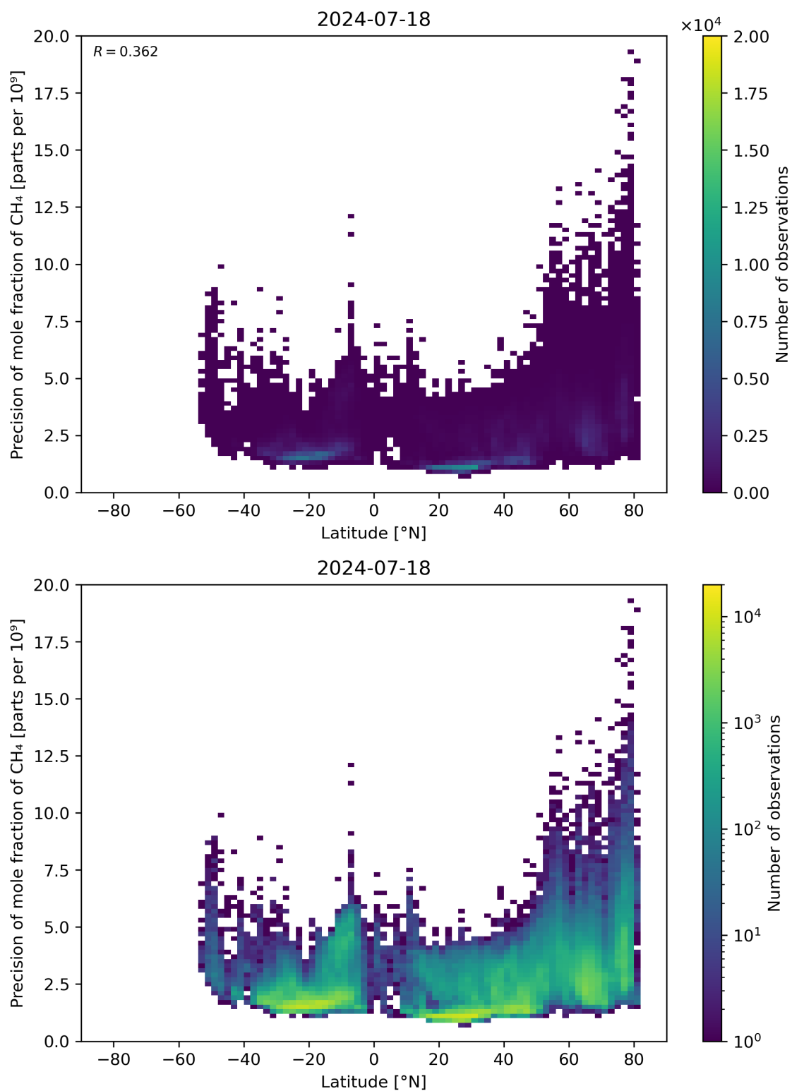
Figure 59: Scatter density plot of “Latitude” against “Precision of mole fraction of \text{CH}_4 ” for 2024-07-17 to 2024-07-19.
