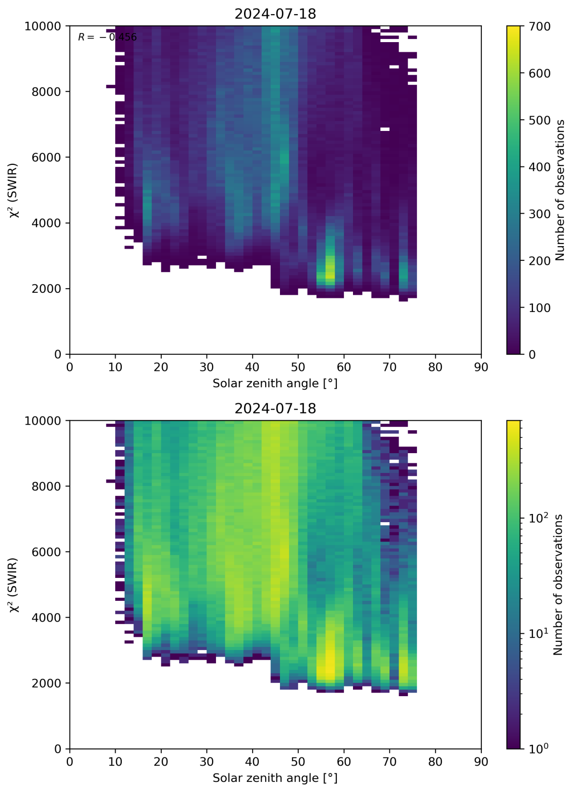
Figure 95: Scatter density plot of “Solar zenith angle” against “ \chi^2 (SWIR)” for 2024-07-17 to 2024-07-19.
