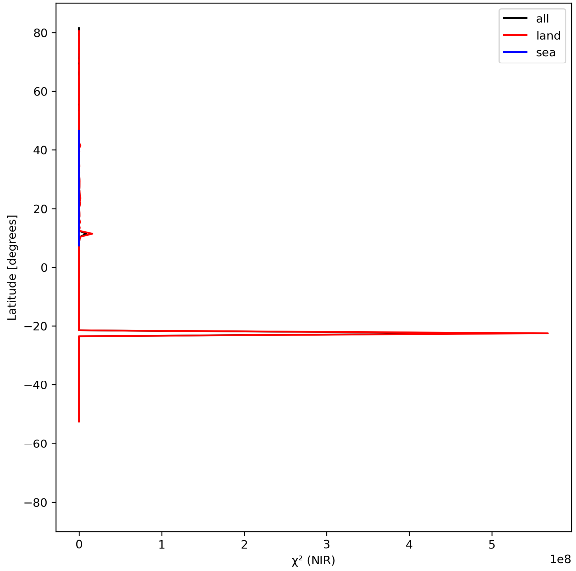
Figure 18: Zonal average of “ \chi^2 (NIR)” for 2024-07-17 to 2024-07-19.
