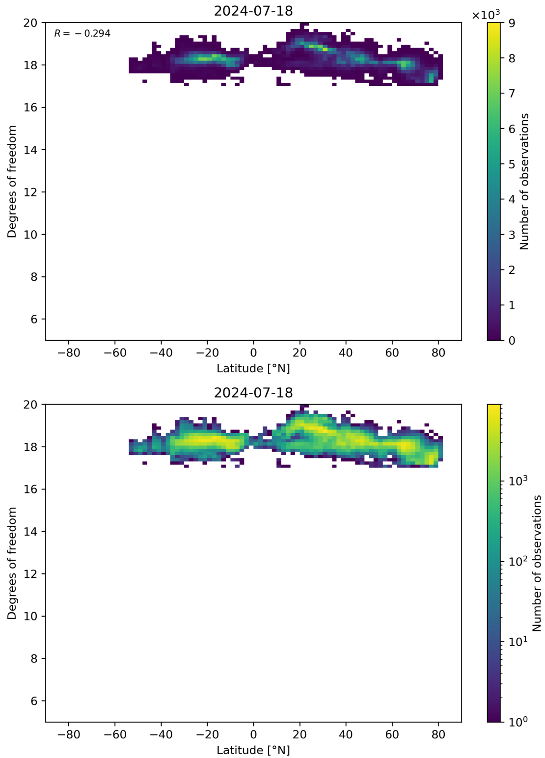
Figure 55: Scatter density plot of “Latitude” against “Degrees of freedom” for 2024-07-17 to 2024-07-19.
