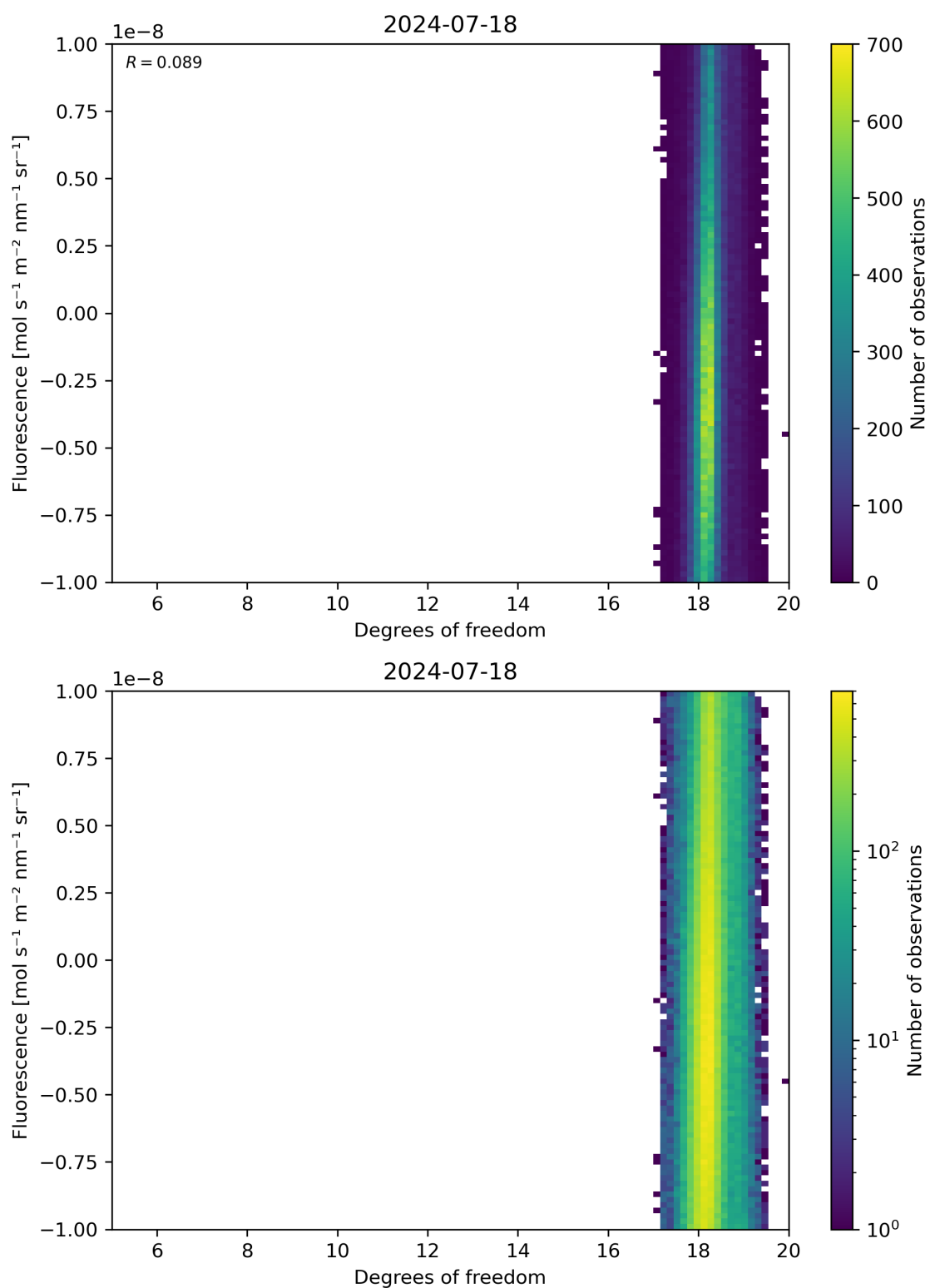
Figure 51: Scatter density plot of “Degrees of freedom” against “Fluorescence” for 2024-07-17 to 2024-07-19.
