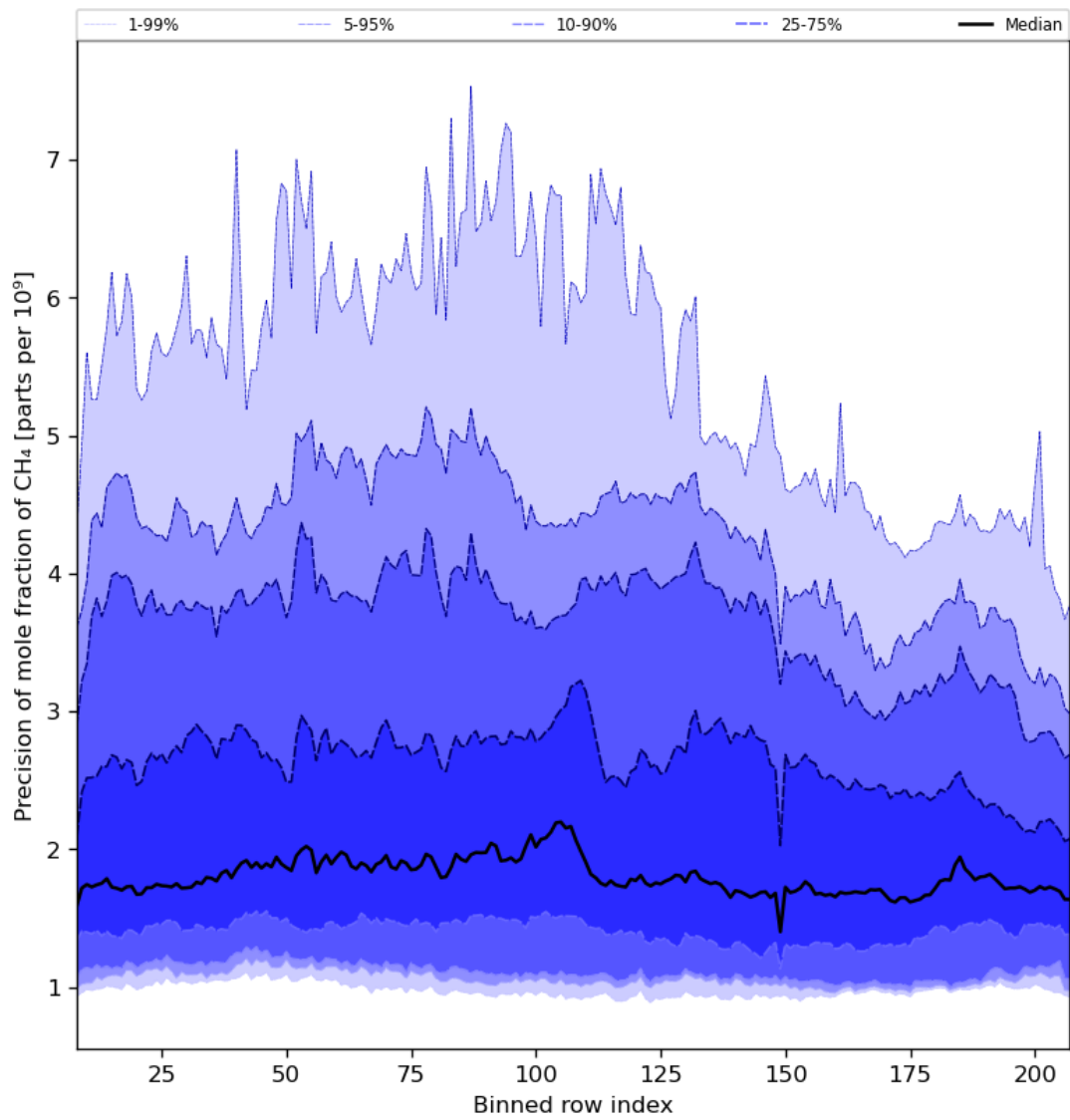
Figure 35: Along track statistics of “Precision of mole fraction of CH 4 ” for 2024-07-17 to 2024-07-19
