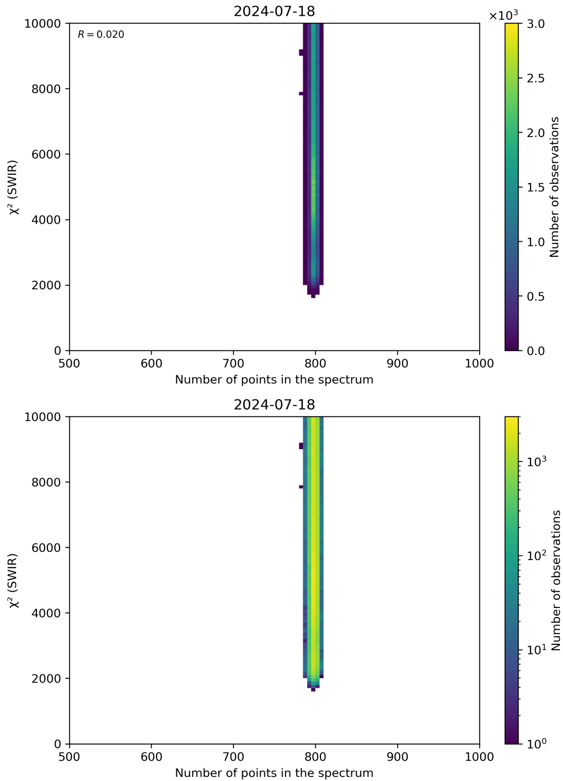
Figure 89: Scatter density plot of “Number of points in the spectrum” against “ \chi^2 (SWIR)” for 2024-07-17 to 2024-07-19.
