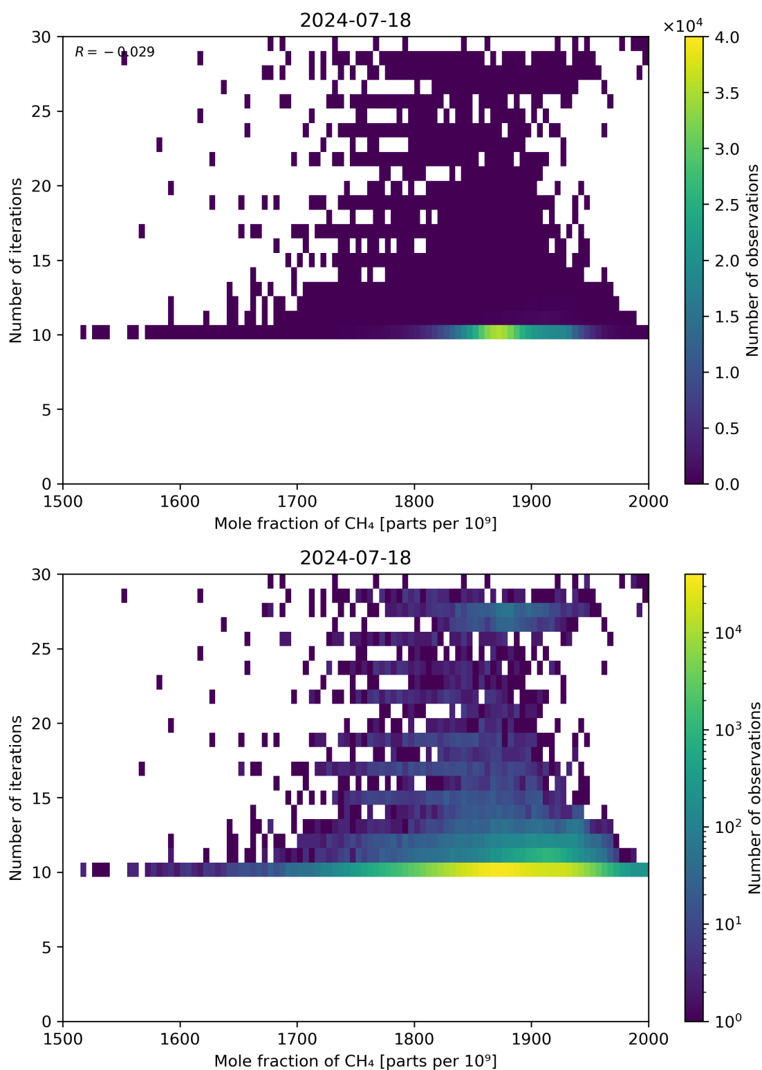
Figure 76: Scatter density plot of “Mole fraction of CH 4 ” against “Number of iterations” for 2024-07-17 to 2024-07-19.
