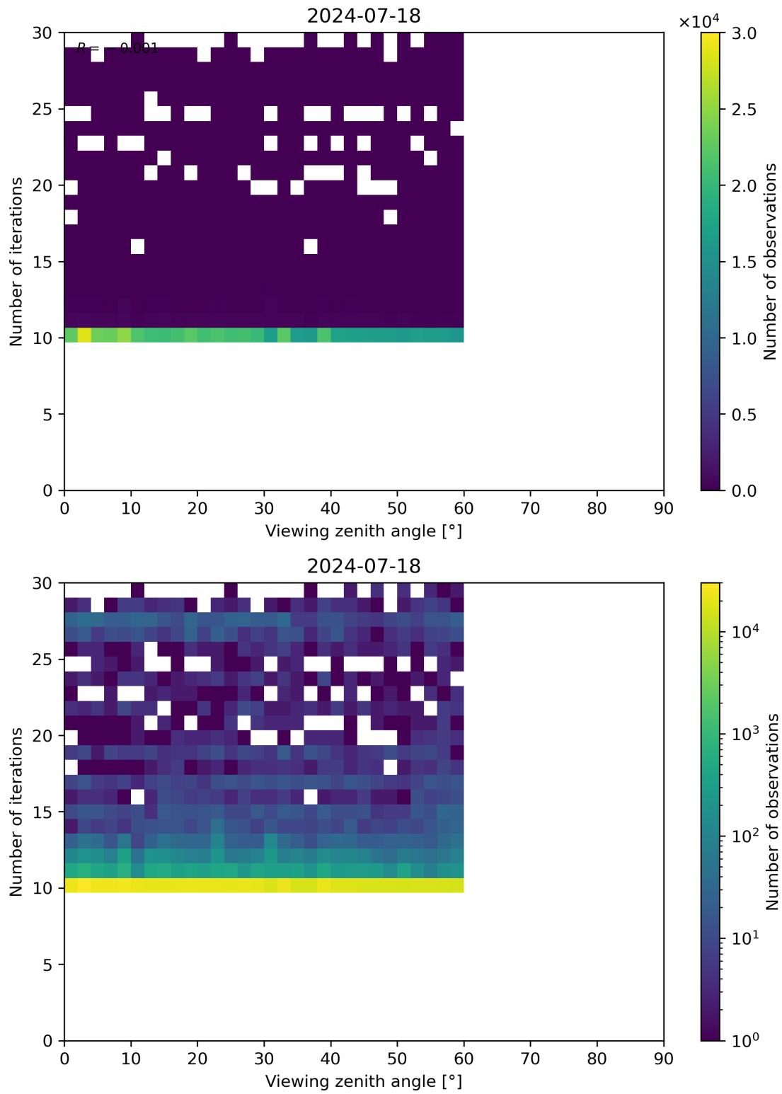
Figure 113: Scatter density plot of “Viewing zenith angle” against “Number of iterations” for 2024-07-17 to 2024-07-19.
