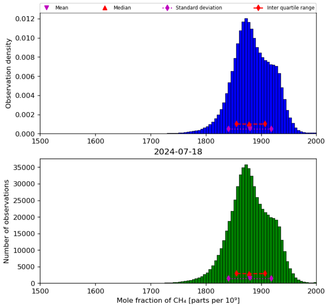
Figure 23: Histogram of “Mole fraction of CH 4 ” for 2024-07-17 to 2024-07-19
