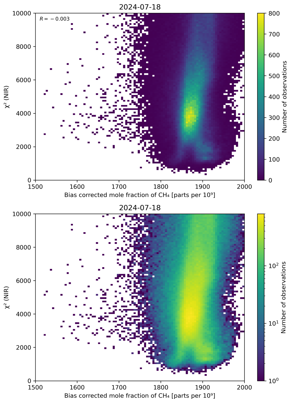
Figure 63: Scatter density plot of “Bias corrected mole fraction of CH 4 ” against “ \chi^2 (NIR)” for 2024-07-17 to 2024-07-19.
