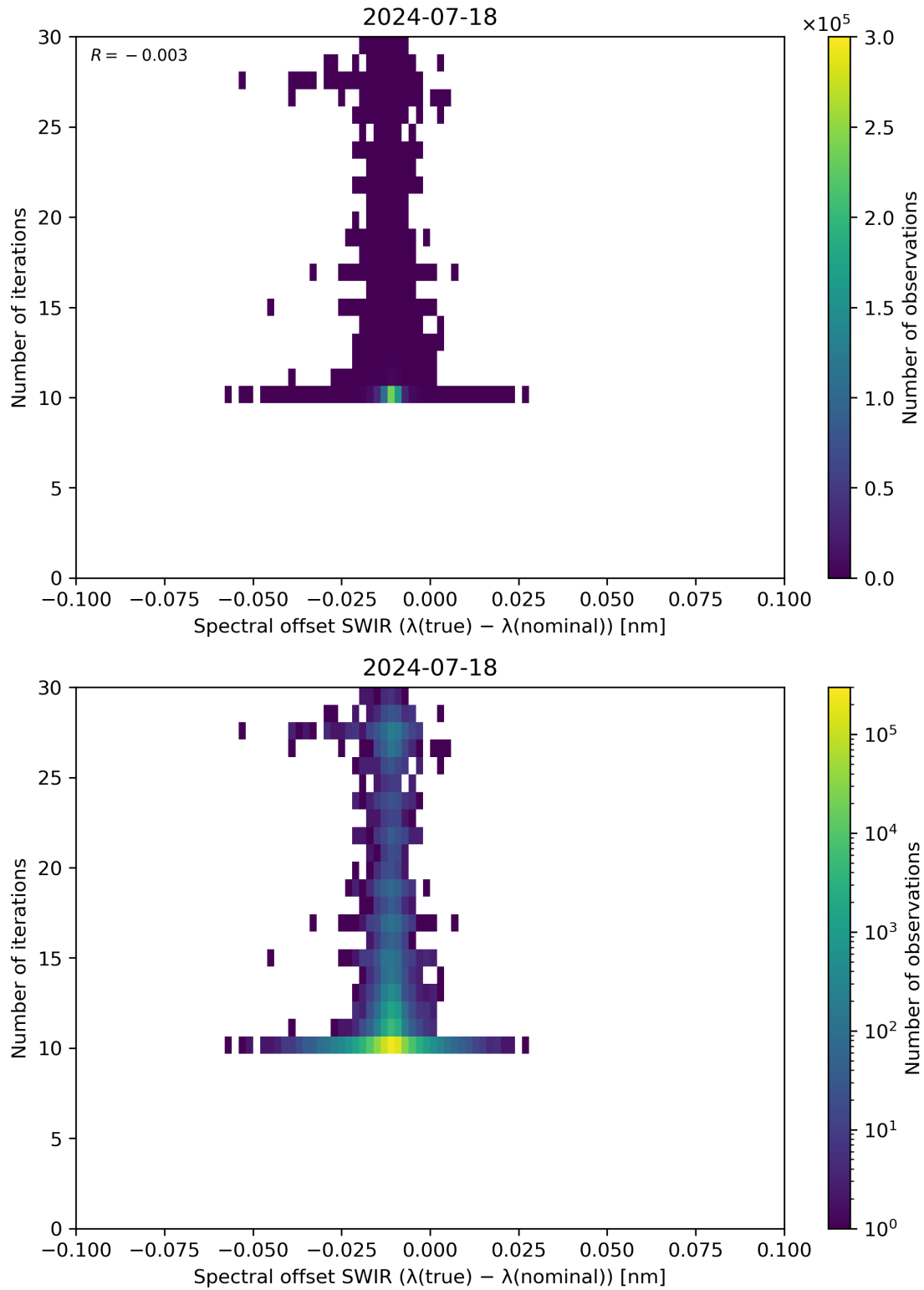
Figure 121: Scatter density plot of “Spectral offset SWIR ( \lambda(\text{true}) - \lambda(\text{nominal}) )” against “Number of iterations” for 2024-07-17 to 2024-07-19.
