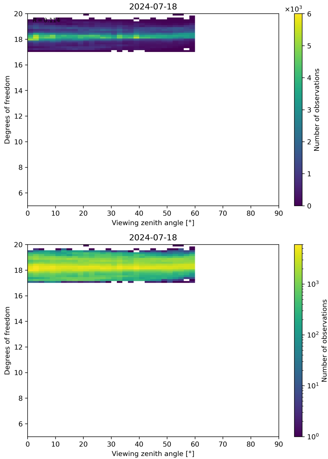
Figure 107: Scatter density plot of “Viewing zenith angle” against “Degrees of freedom” for 2024-07-17 to 2024-07-19.
