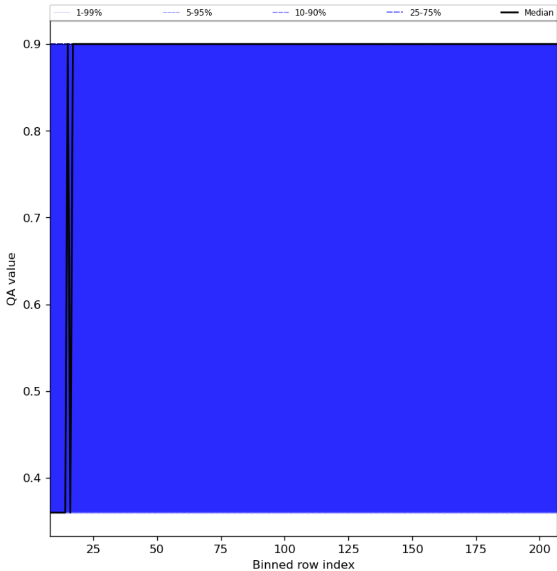
Figure 33: Along track statistics of "QA value" for 2024-07-17 to 2024-07-19
