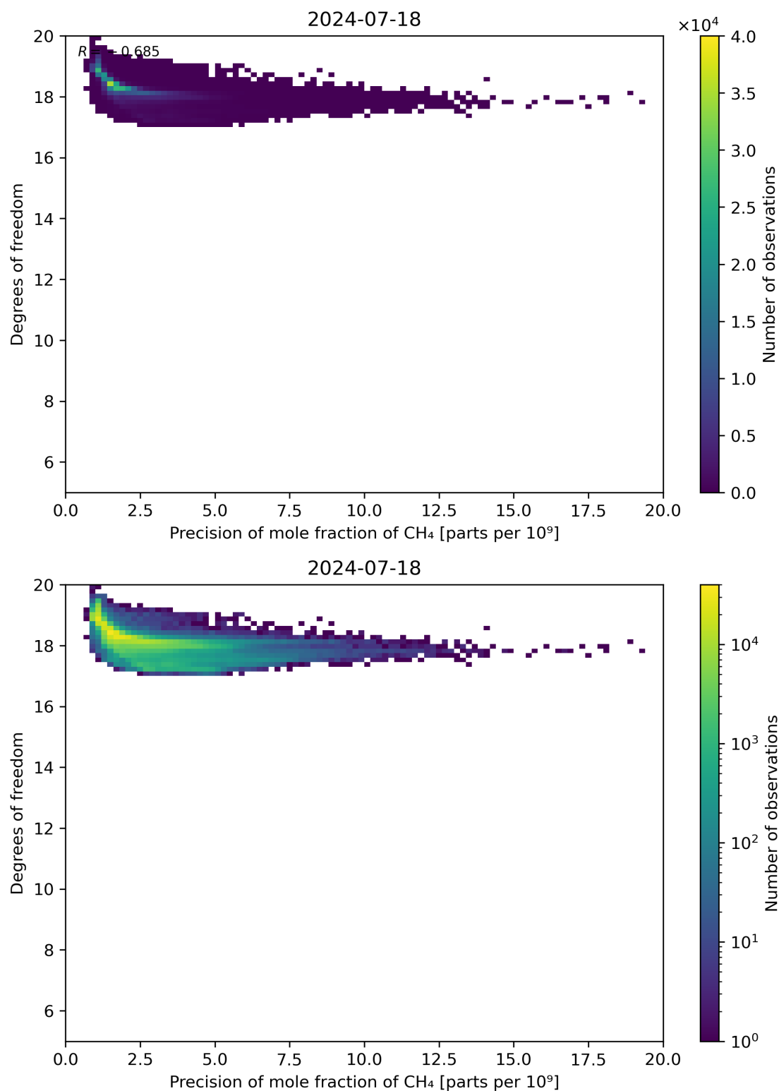
Figure 80: Scatter density plot of “Precision of mole fraction of CH 4 ” against “Degrees of freedom” for 2024-07-17 to 2024-07-19.
