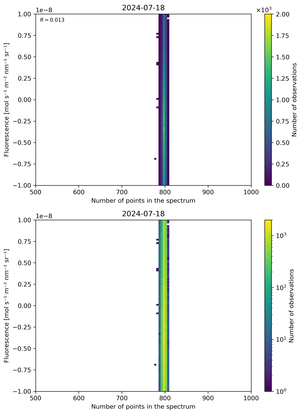
Figure 91: Scatter density plot of “Number of points in the spectrum” against “Fluorescence” for 2024-07-17 to 2024-07-19.
