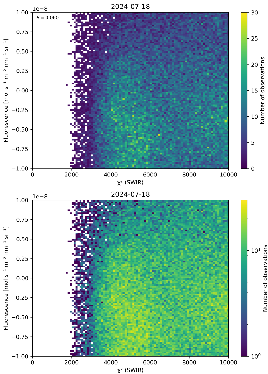
Figure 49: Scatter density plot of “ \chi^2 (SWIR)” against “Fluorescence” for 2024-07-17 to 2024-07-19.
