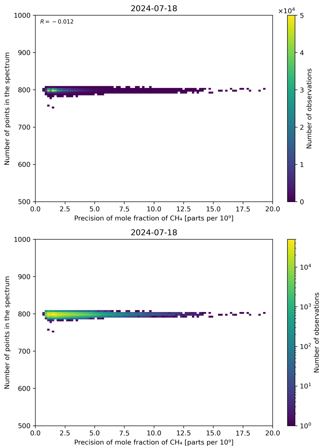
Figure 84: Scatter density plot of “Precision of mole fraction of CH 4 ” against “Number of points in the spectrum” for 2024-07-17 to 2024-07-19.
