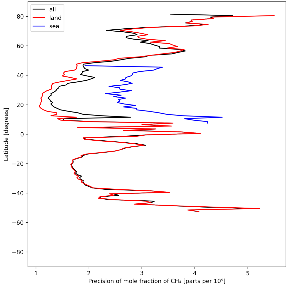
Figure 13: Zonal average of “Precision of mole fraction of \text{CH}_4 ” for 2024-07-17 to 2024-07-19.
