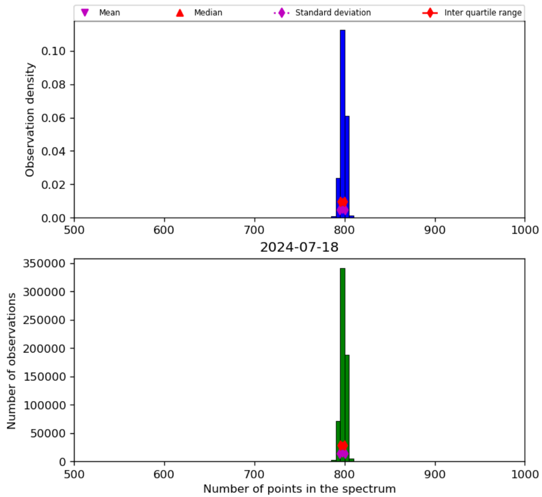
Figure 26: Histogram of “Number of points in the spectrum” for 2024-07-17 to 2024-07-19
