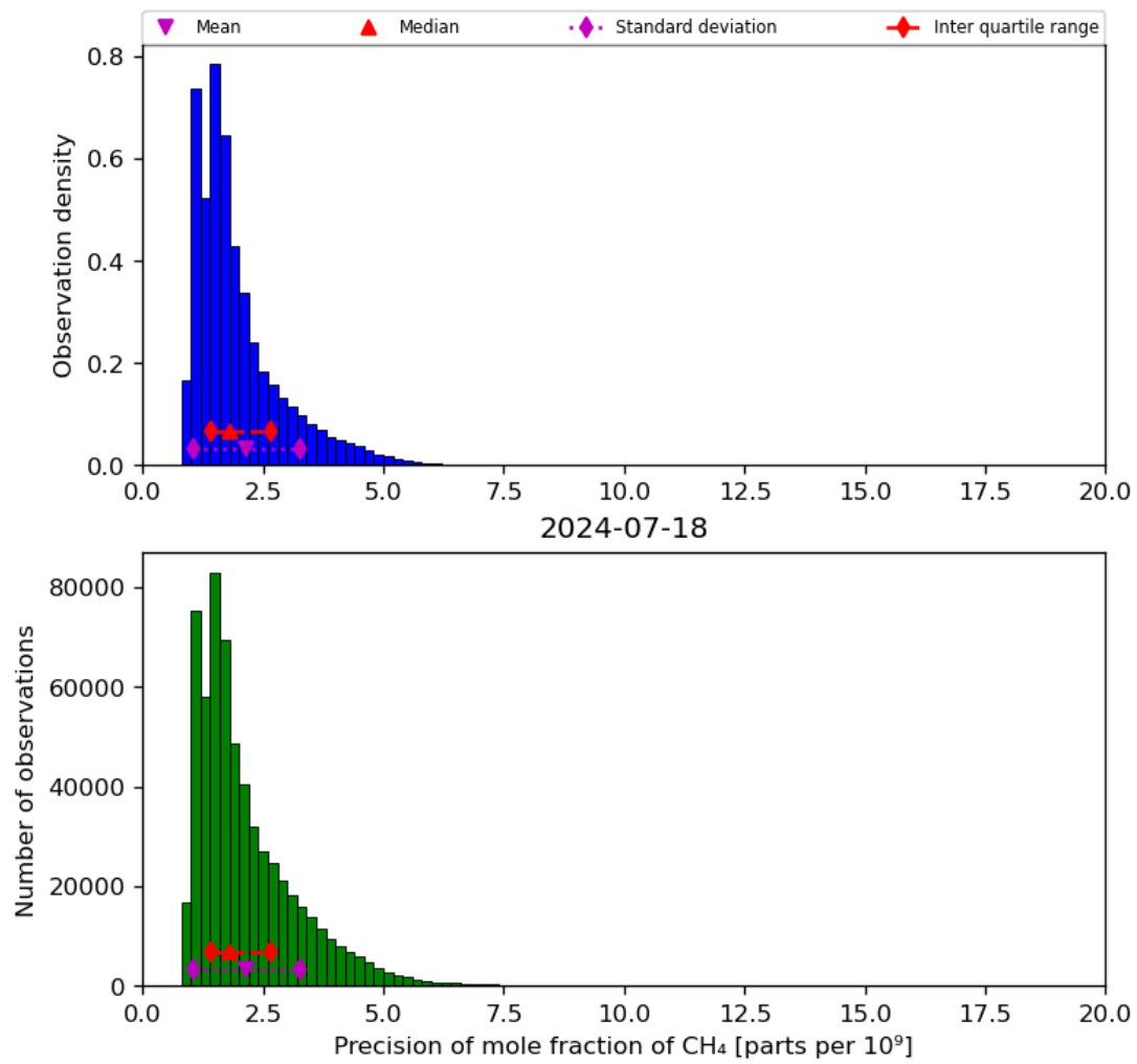
Figure 24: Histogram of “Precision of mole fraction of CH 4 ” for 2024-07-17 to 2024-07-19
