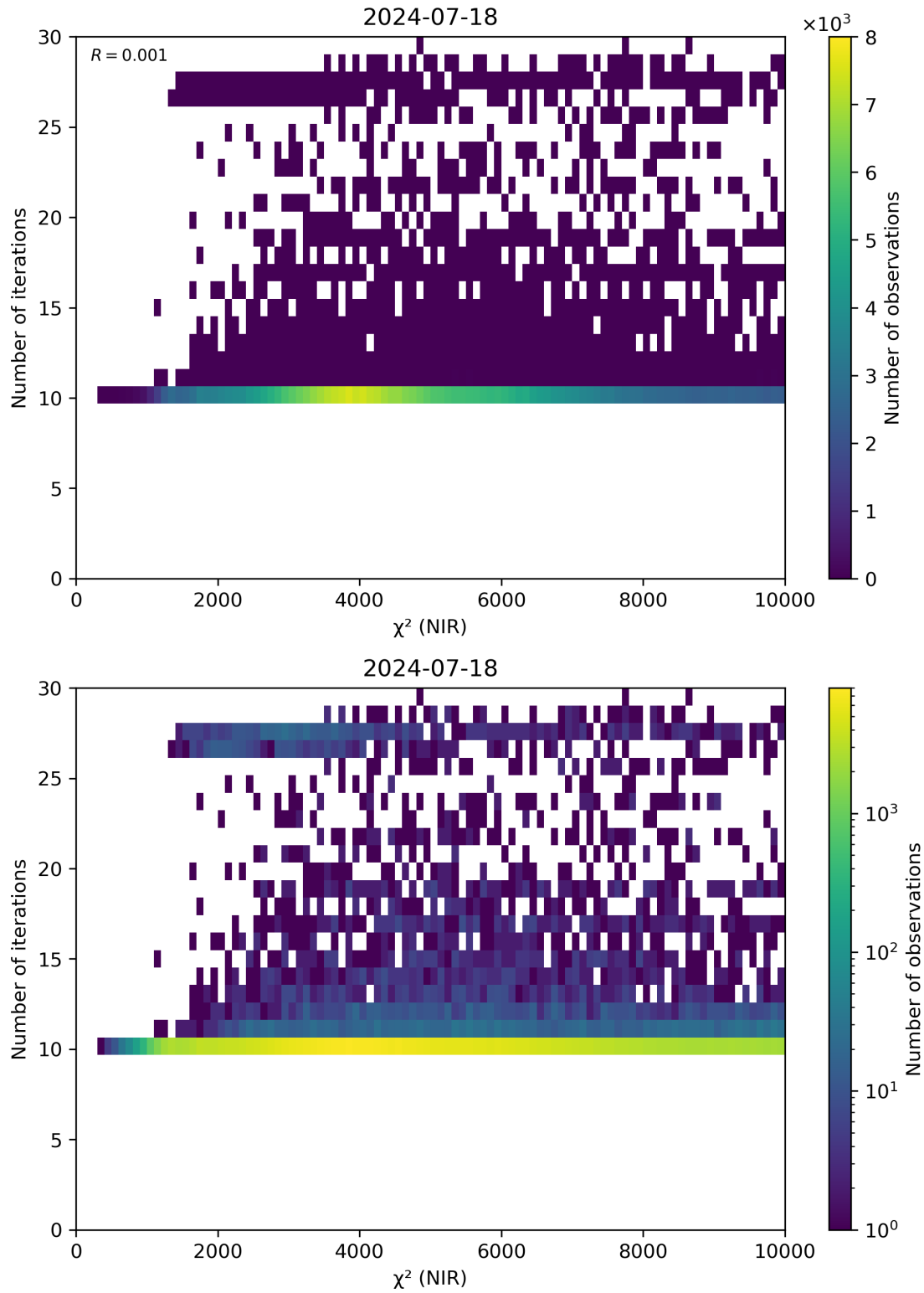
Figure 46: Scatter density plot of “ \chi^2 (NIR)” against “Number of iterations” for 2024-07-17 to 2024-07-19.
