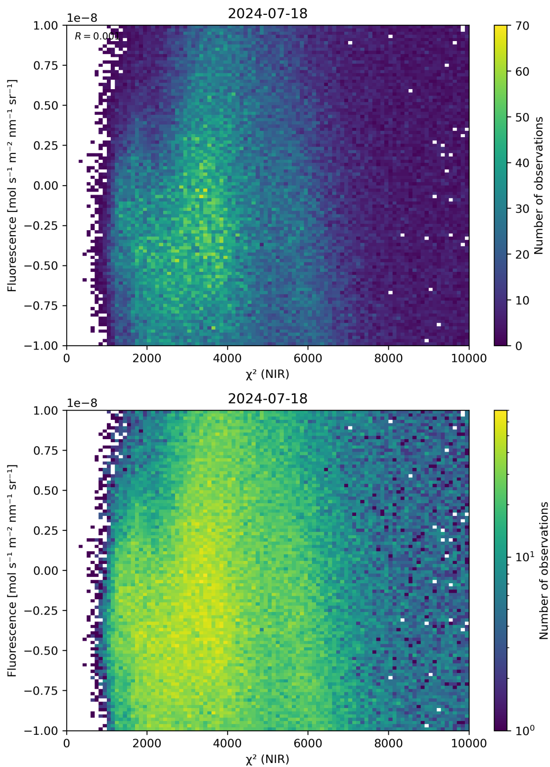
Figure 45: Scatter density plot of “ \chi^2 (NIR)” against “Fluorescence” for 2024-07-17 to 2024-07-19.
