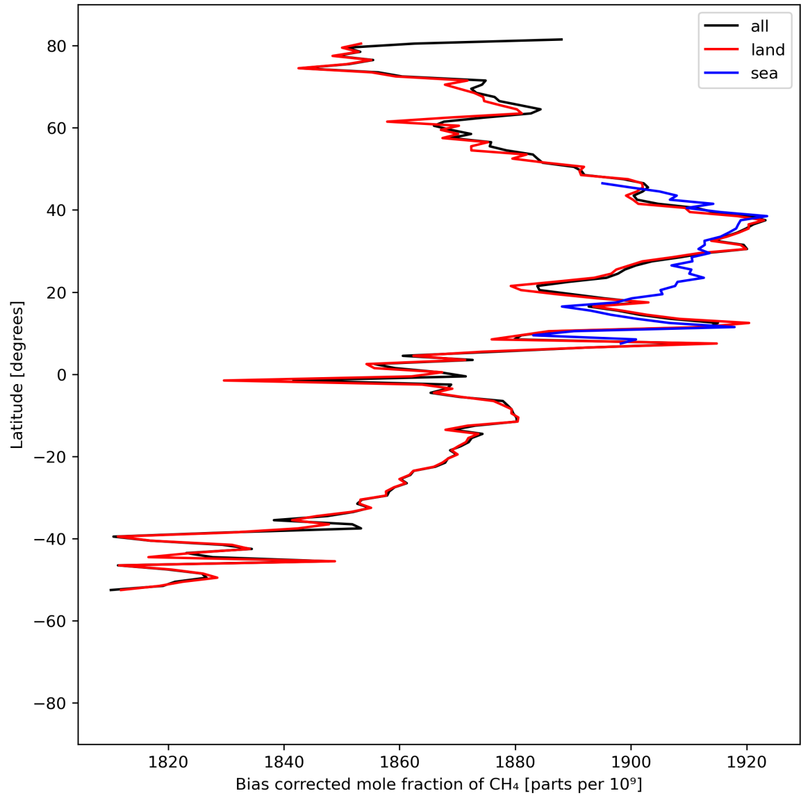
Figure 14: Zonal average of “Bias corrected mole fraction of \text{CH}_4 ” for 2024-07-17 to 2024-07-19.
