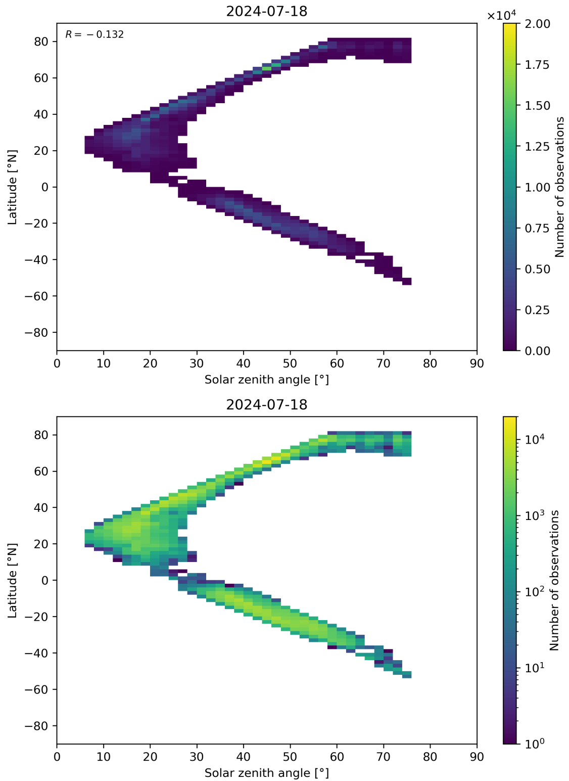
Figure 98: Scatter density plot of “Solar zenith angle” against “Latitude” for 2024-07-17 to 2024-07-19.
