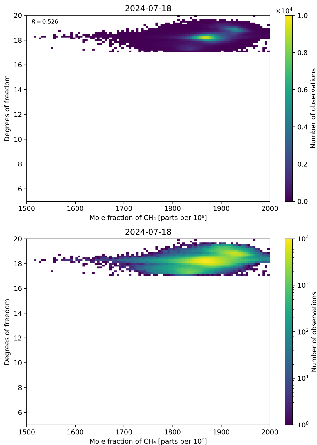
Figure 72: Scatter density plot of “Mole fraction of CH 4 ” against “Degrees of freedom” for 2024-07-17 to 2024-07-19.
