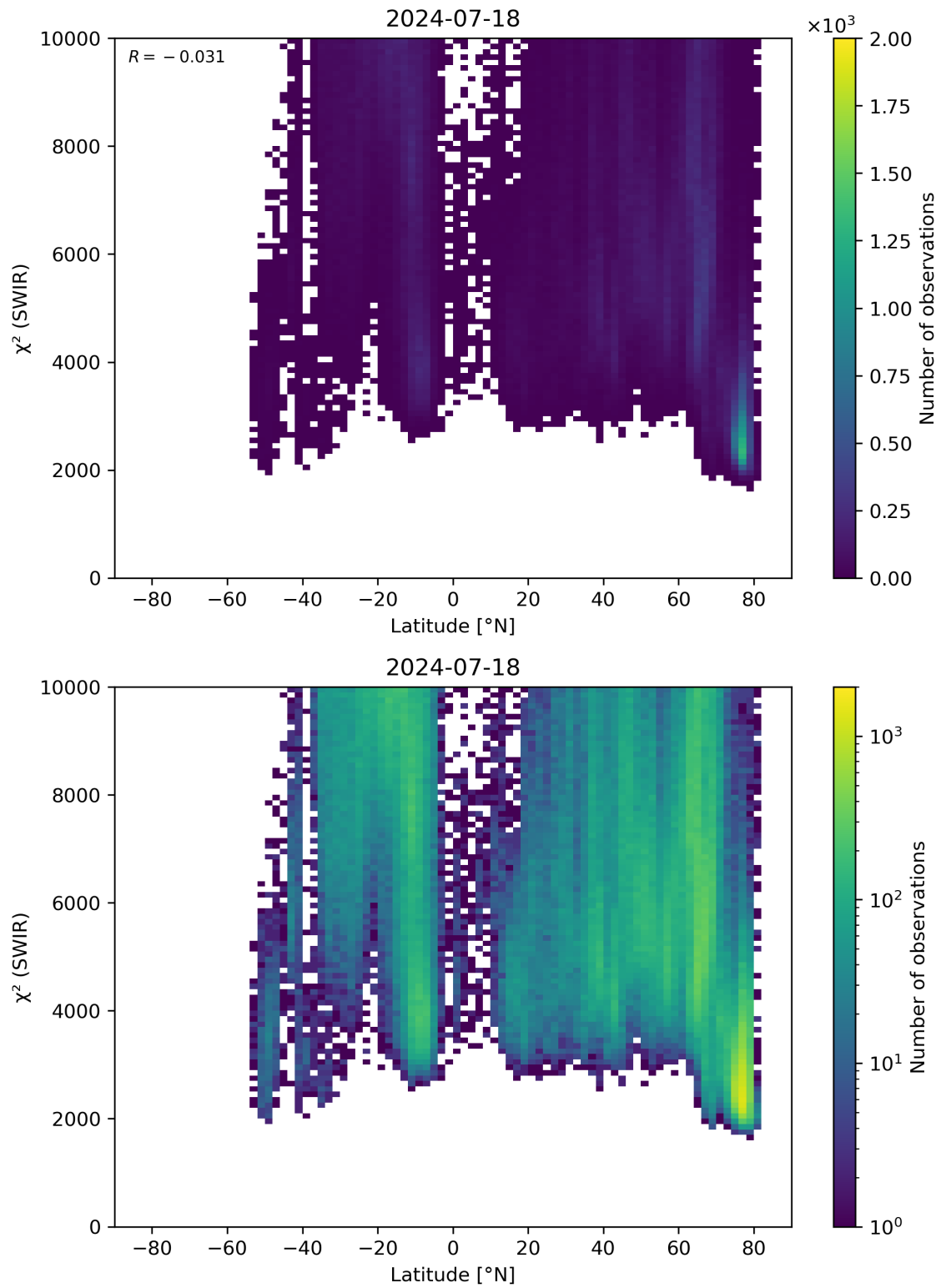
Figure 54: Scatter density plot of “Latitude” against “ \chi^2 (SWIR)” for 2024-07-17 to 2024-07-19.
