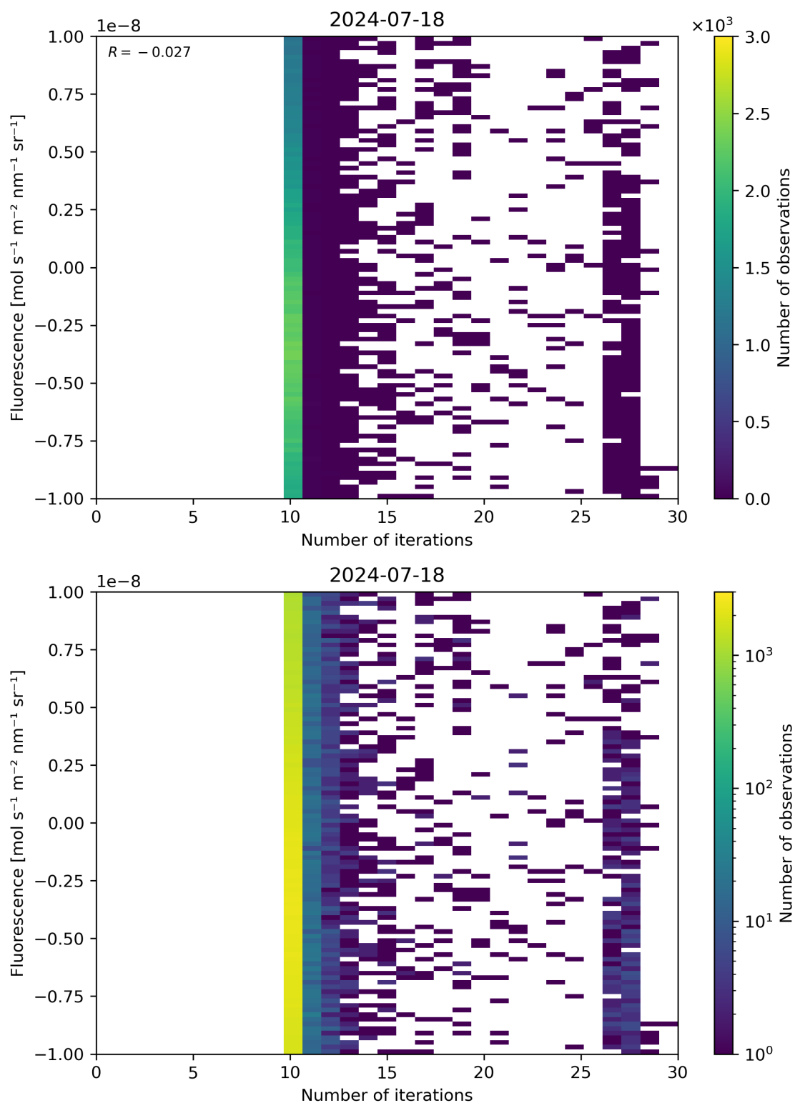
Figure 87: Scatter density plot of “Number of iterations” against “Fluorescence” for 2024-07-17 to 2024-07-19.
