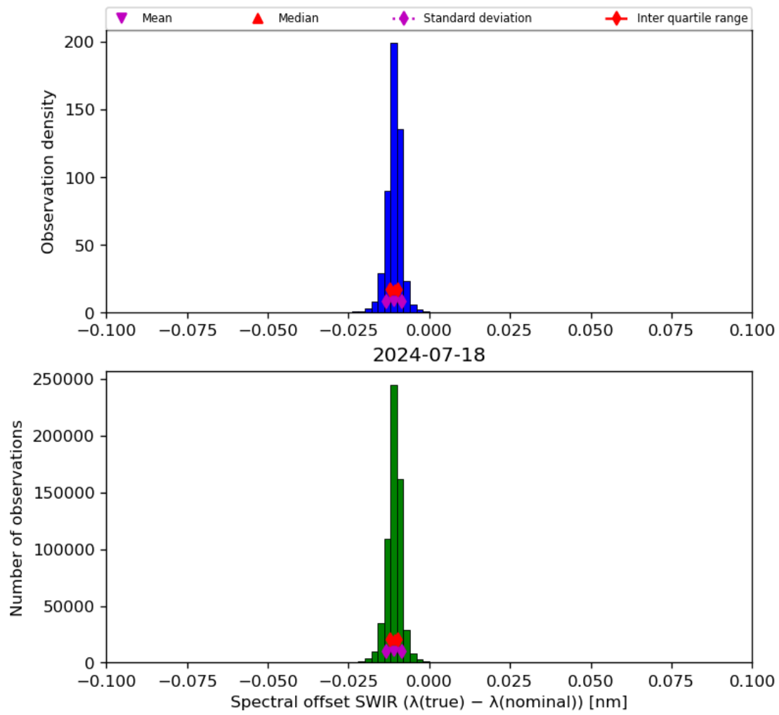
Figure 27: Histogram of “Spectral offset SWIR ( \lambda(\text{true}) - \lambda(\text{nominal}) )” for 2024-07-17 to 2024-07-19
