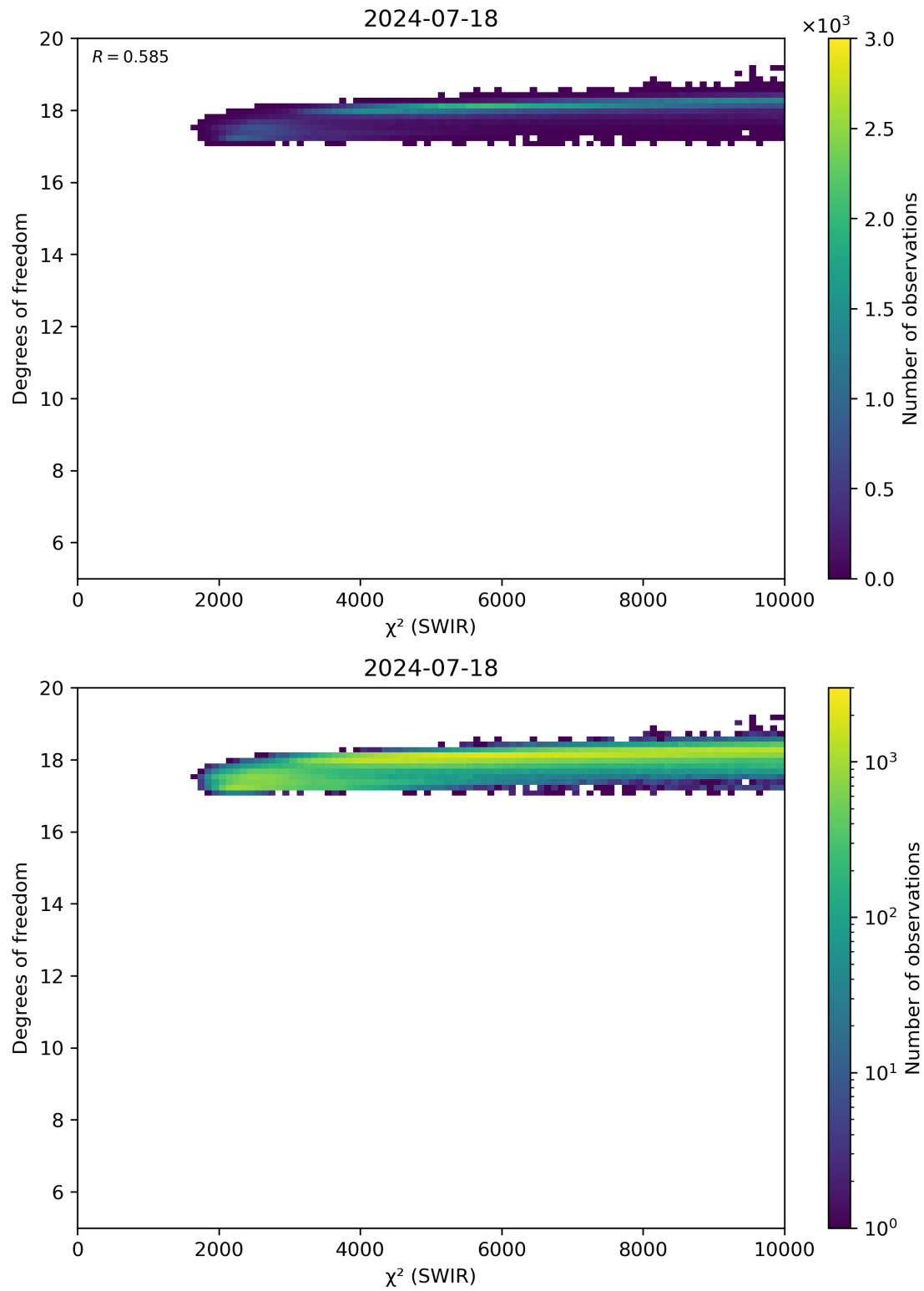
Figure 48: Scatter density plot of “ \chi^2 (SWIR)” against “Degrees of freedom” for 2024-07-17 to 2024-07-19.
