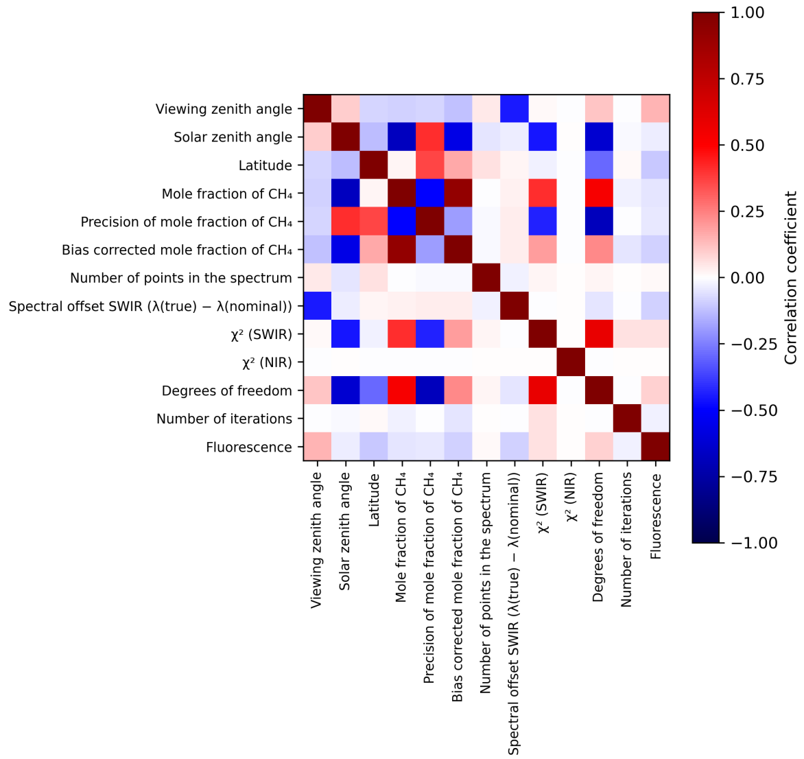
Figure 2: Map of correlation matrix for 2024-07-17 to 2024-07-19.
