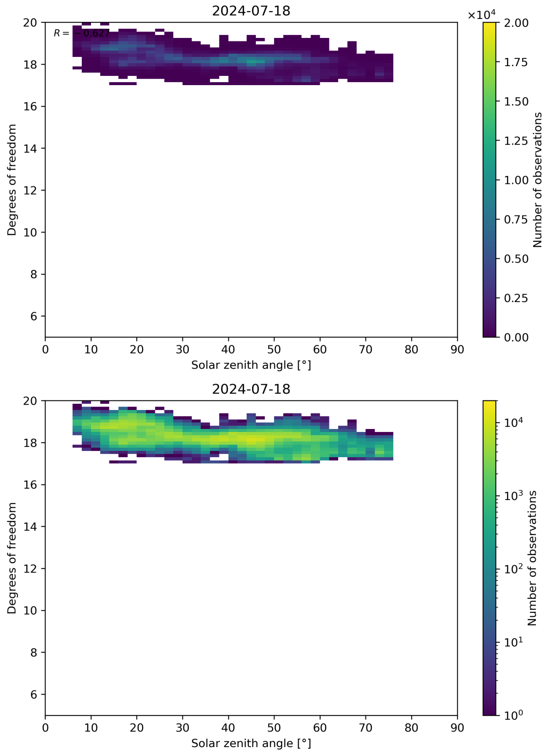
Figure 96: Scatter density plot of “Solar zenith angle” against “Degrees of freedom” for 2024-07-17 to 2024-07-19.
