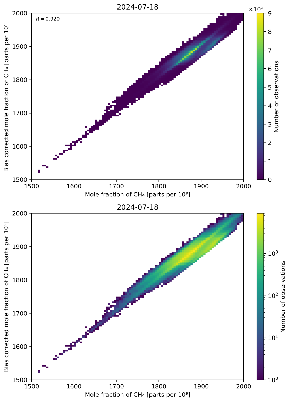
Figure 74: Scatter density plot of “Mole fraction of CH 4 ” against “Bias corrected mole fraction of CH 4 ” for 2024-07-17 to 2024-07-19.
