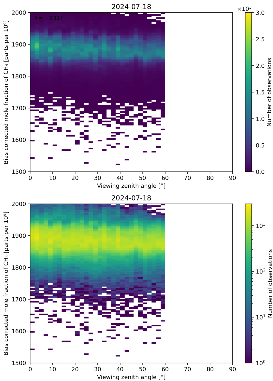
Figure 111: Scatter density plot of “Viewing zenith angle” against “Bias corrected mole fraction of CH 4 ” for 2024-07-17 to 2024-07-19.
