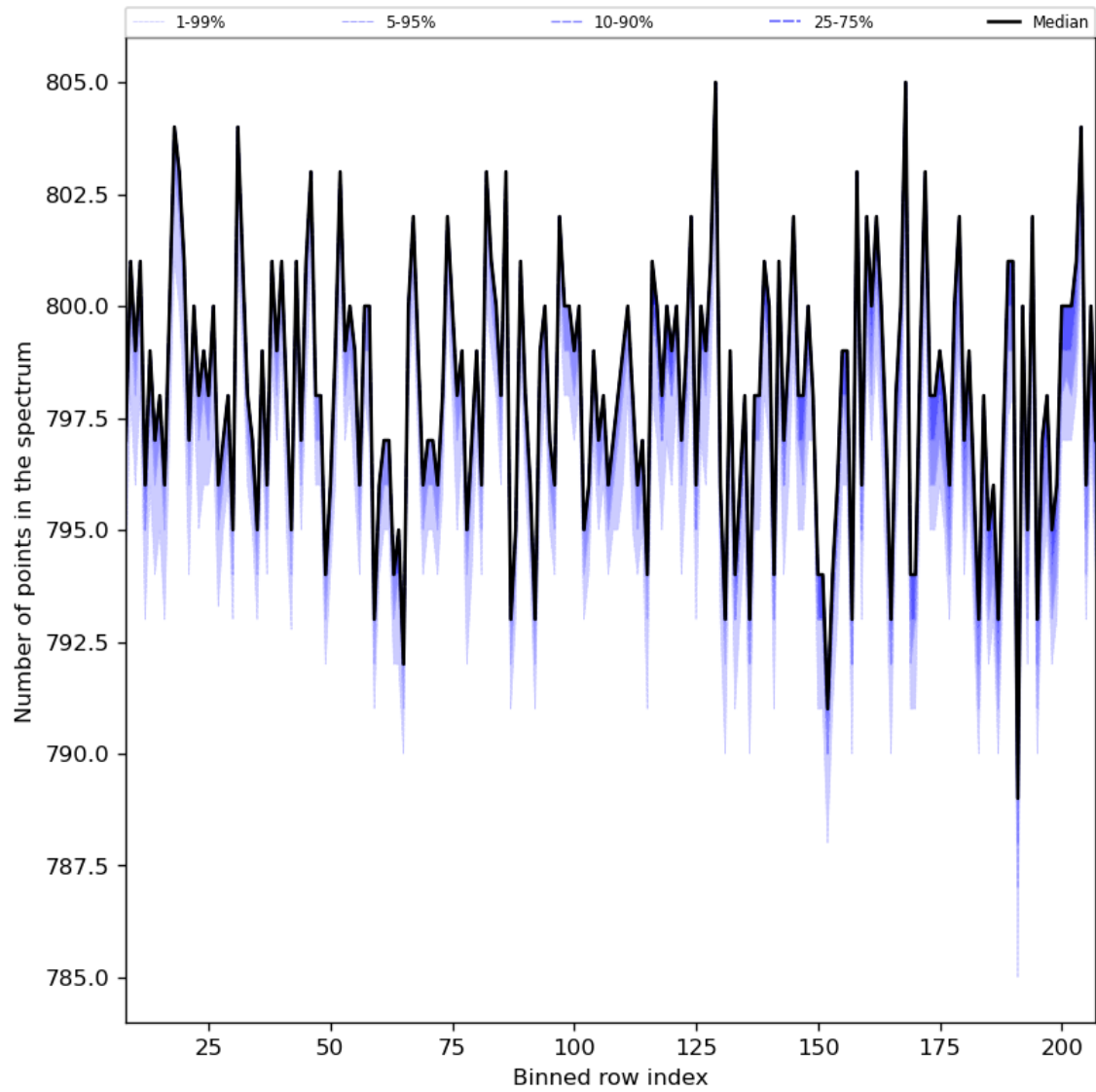
Figure 37: Along track statistics of “Number of points in the spectrum” for 2024-07-17 to 2024-07-19
