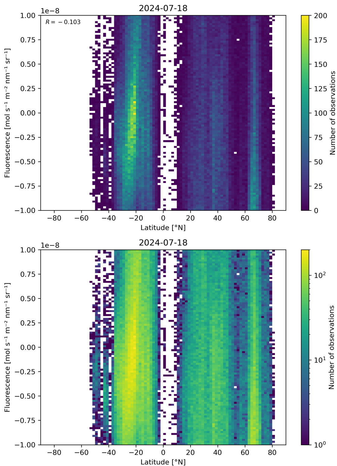
Figure 56: Scatter density plot of “Latitude” against “Fluorescence” for 2024-07-17 to 2024-07-19.
