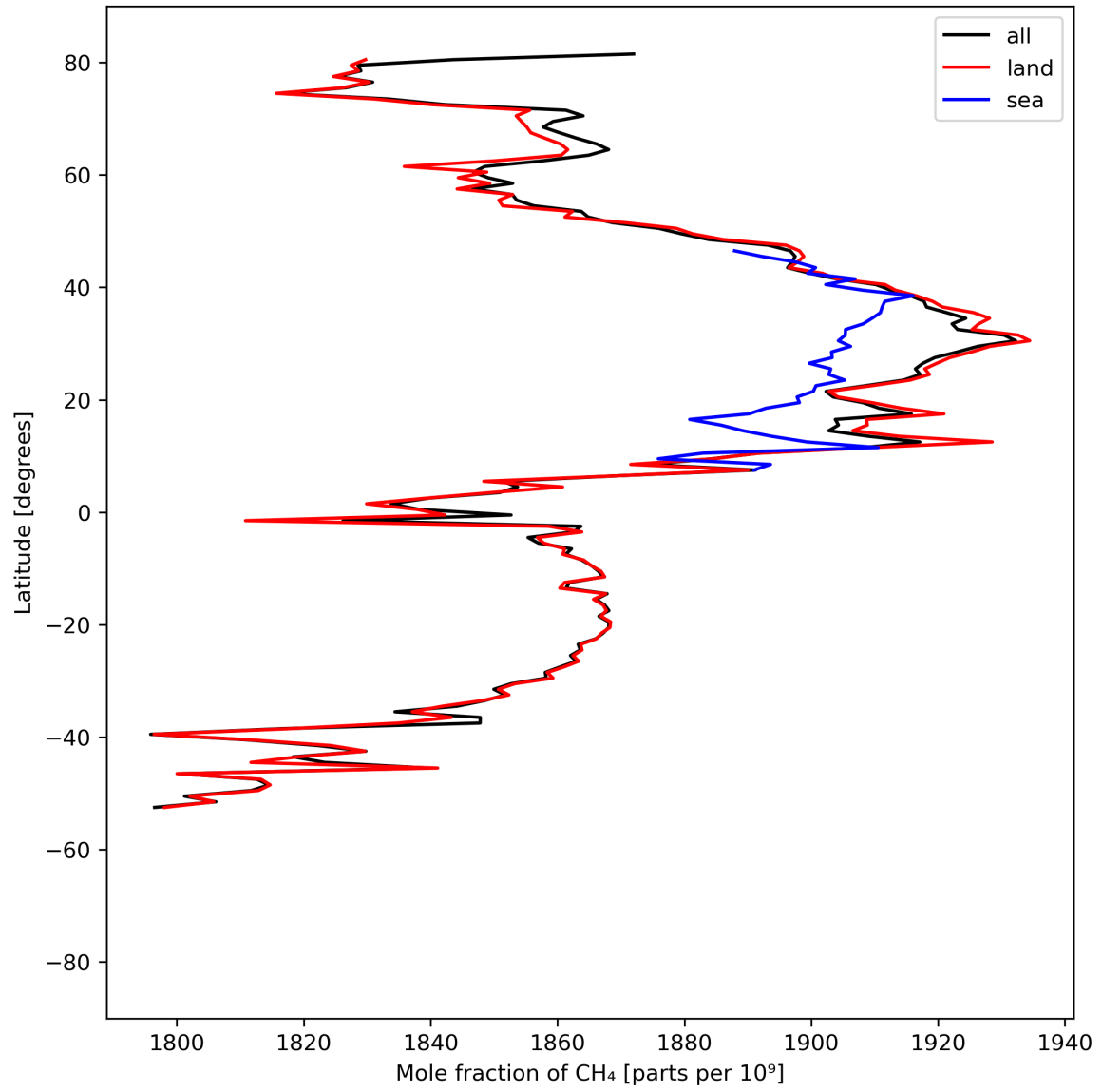
Figure 12: Zonal average of “Mole fraction of \text{CH}_4 ” for 2024-07-17 to 2024-07-19.
