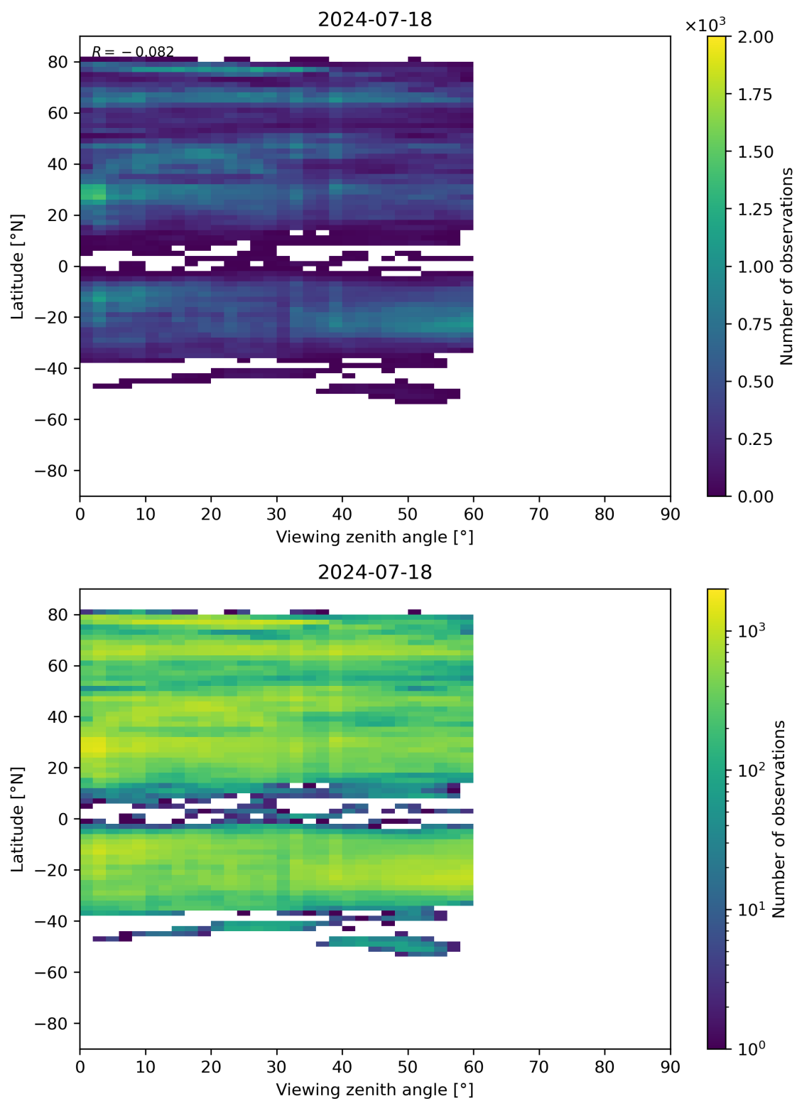
Figure 109: Scatter density plot of “Viewing zenith angle” against “Latitude” for 2024-07-17 to 2024-07-19.
