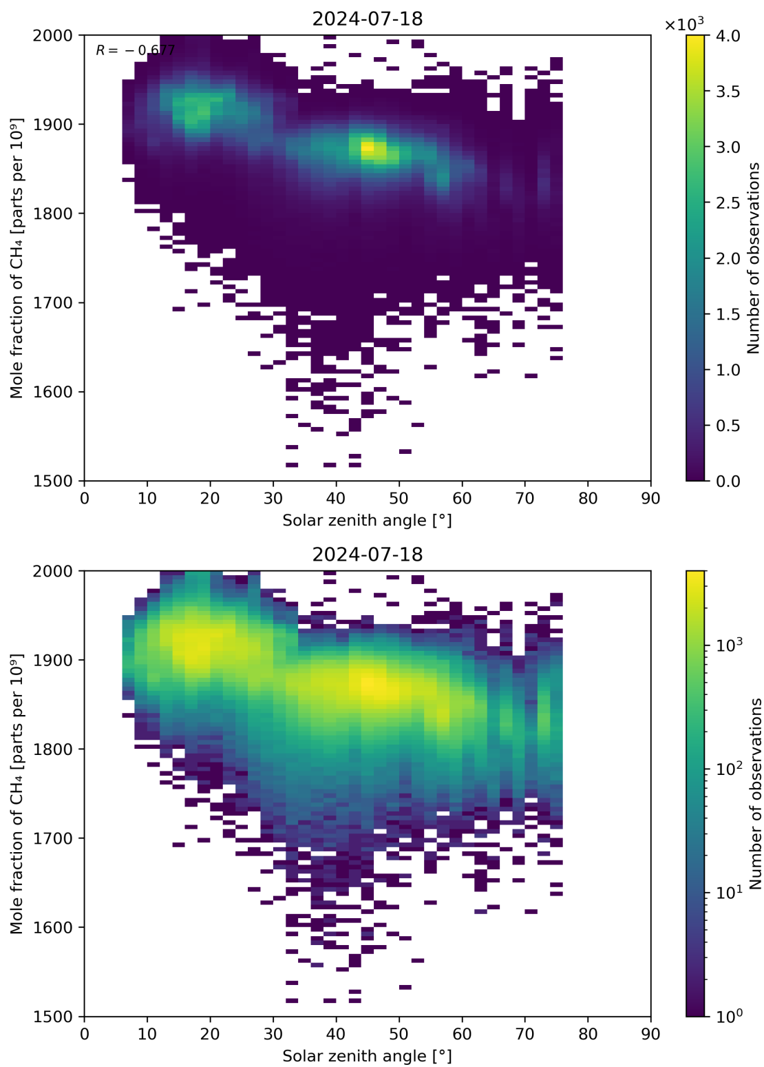
Figure 99: Scatter density plot of “Solar zenith angle” against “Mole fraction of CH 4 ” for 2024-07-17 to 2024-07-19.
