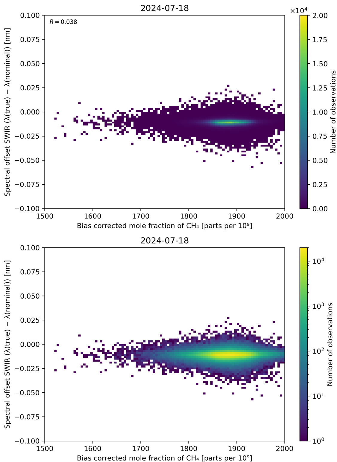
Figure 69: Scatter density plot of “Bias corrected mole fraction of \text{CH}_4 ” against “Spectral offset SWIR ( \lambda(\text{true}) - \lambda(\text{nominal}) )” for 2024-07-17 to 2024-07-19.
