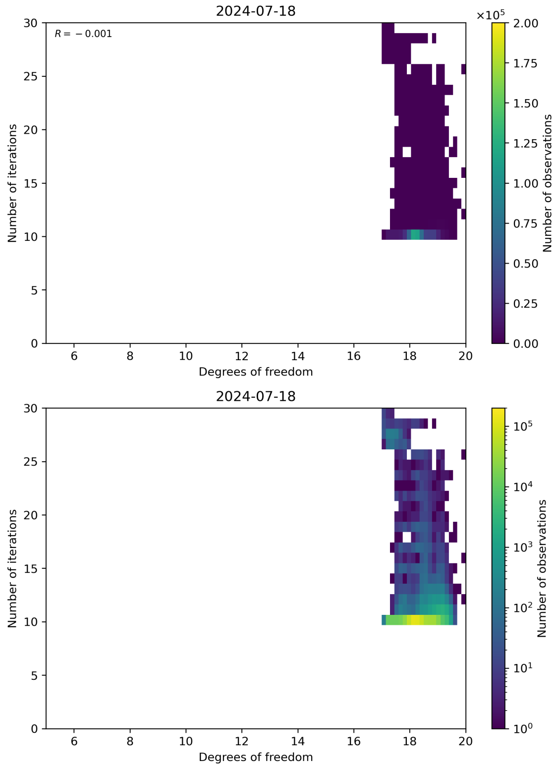
Figure 52: Scatter density plot of “Degrees of freedom” against “Number of iterations” for 2024-07-17 to 2024-07-19.
