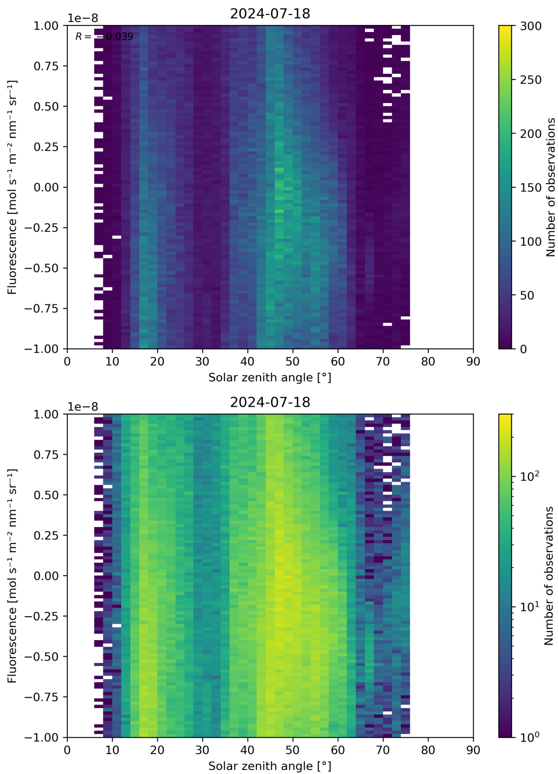
Figure 97: Scatter density plot of “Solar zenith angle” against “Fluorescence” for 2024-07-17 to 2024-07-19.
