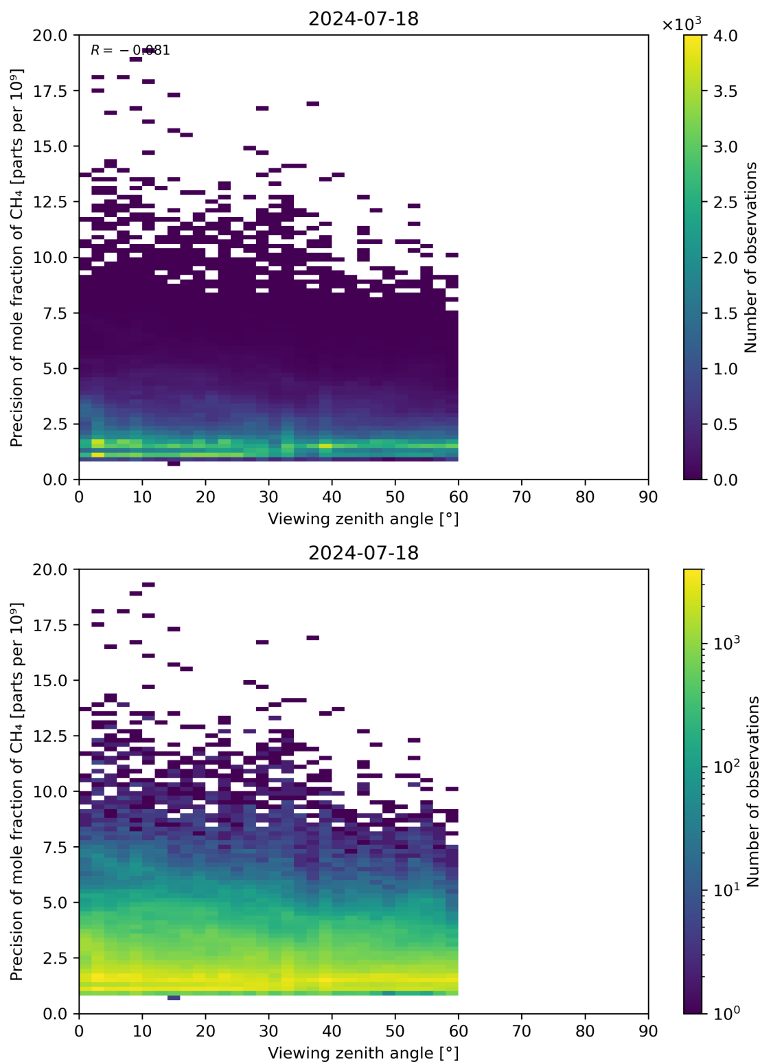
Figure 112: Scatter density plot of “Viewing zenith angle” against “Precision of mole fraction of CH 4 ” for 2024-07-17 to 2024-07-19.
