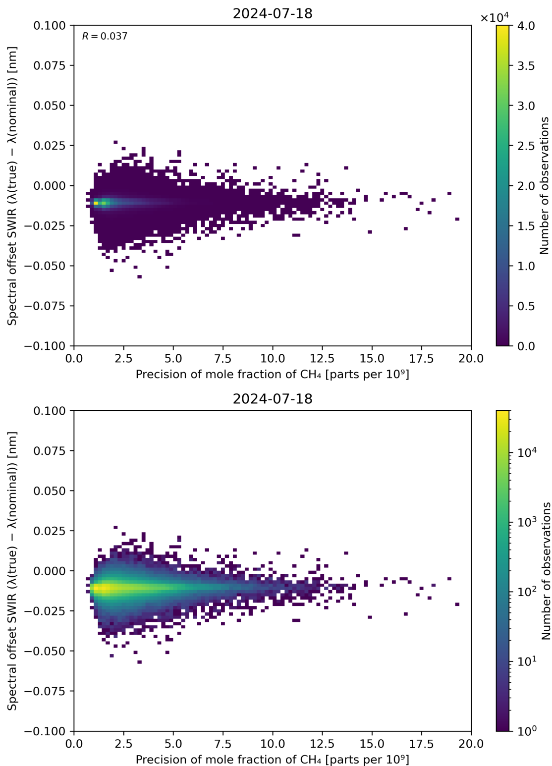
Figure 85: Scatter density plot of “Precision of mole fraction of CH 4 ” against “Spectral offset SWIR ( \lambda(\text{true}) - \lambda(\text{nominal}) )” for 2024-07-17 to 2024-07-19.
