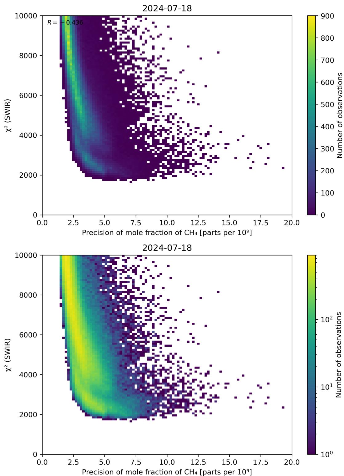
Figure 79: Scatter density plot of “Precision of mole fraction of CH 4 ” against “ \chi^2 (SWIR)” for 2024-07-17 to 2024-07-19.
