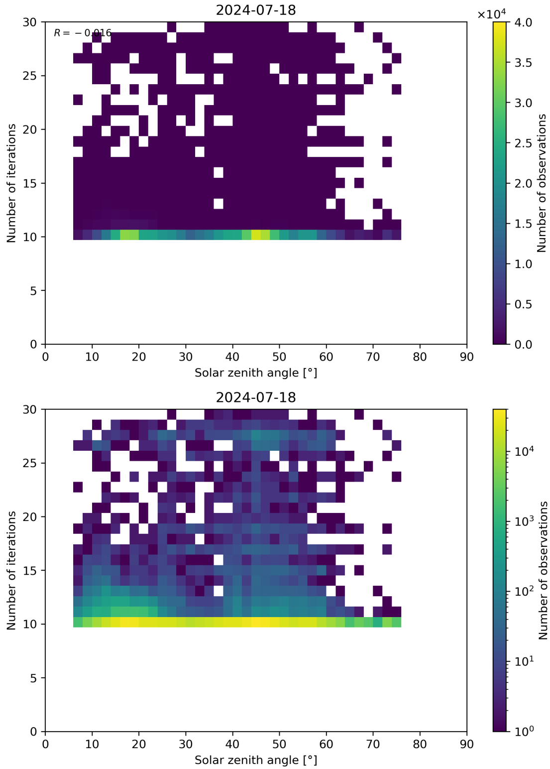
Figure 102: Scatter density plot of “Solar zenith angle” against “Number of iterations” for 2024-07-17 to 2024-07-19.
