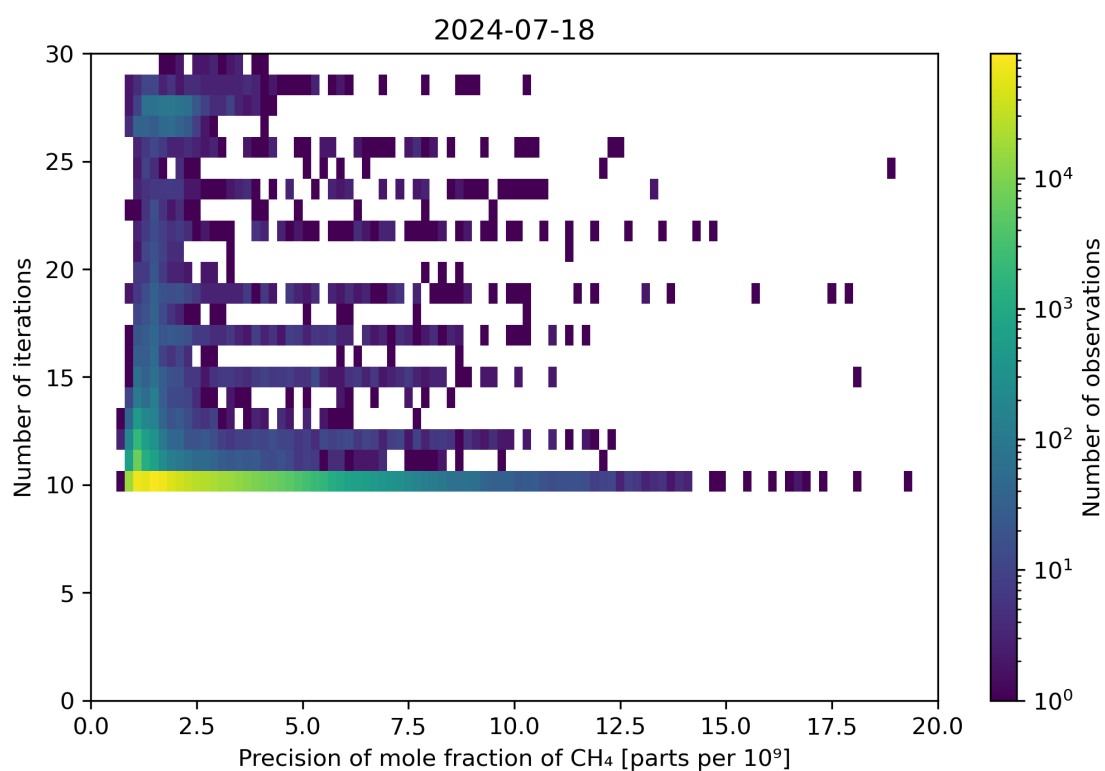
Figure 83: Scatter density plot of “Precision of mole fraction of CH 4 ” against “Number of iterations” for 2024-07-17 to 2024-07-19.
