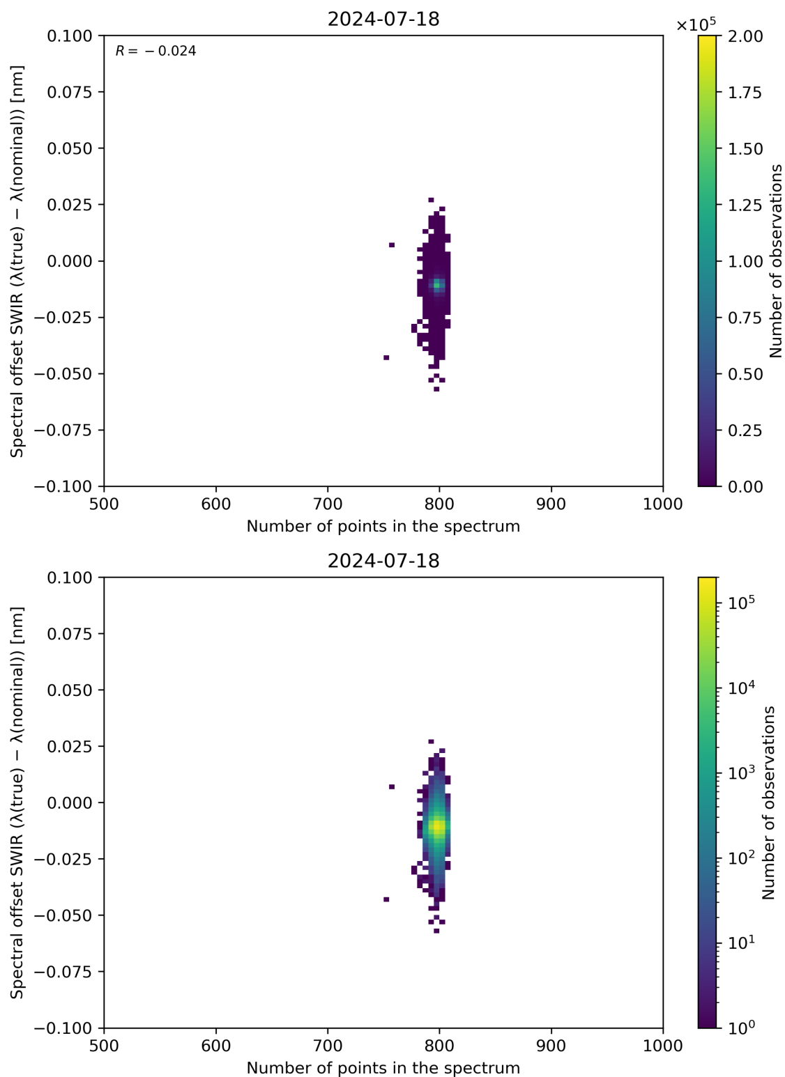
Figure 93: Scatter density plot of “Number of points in the spectrum” against “Spectral offset SWIR ( \lambda(\text{true}) - \lambda(\text{nominal}) )” for 2024-07-17 to 2024-07-19.
