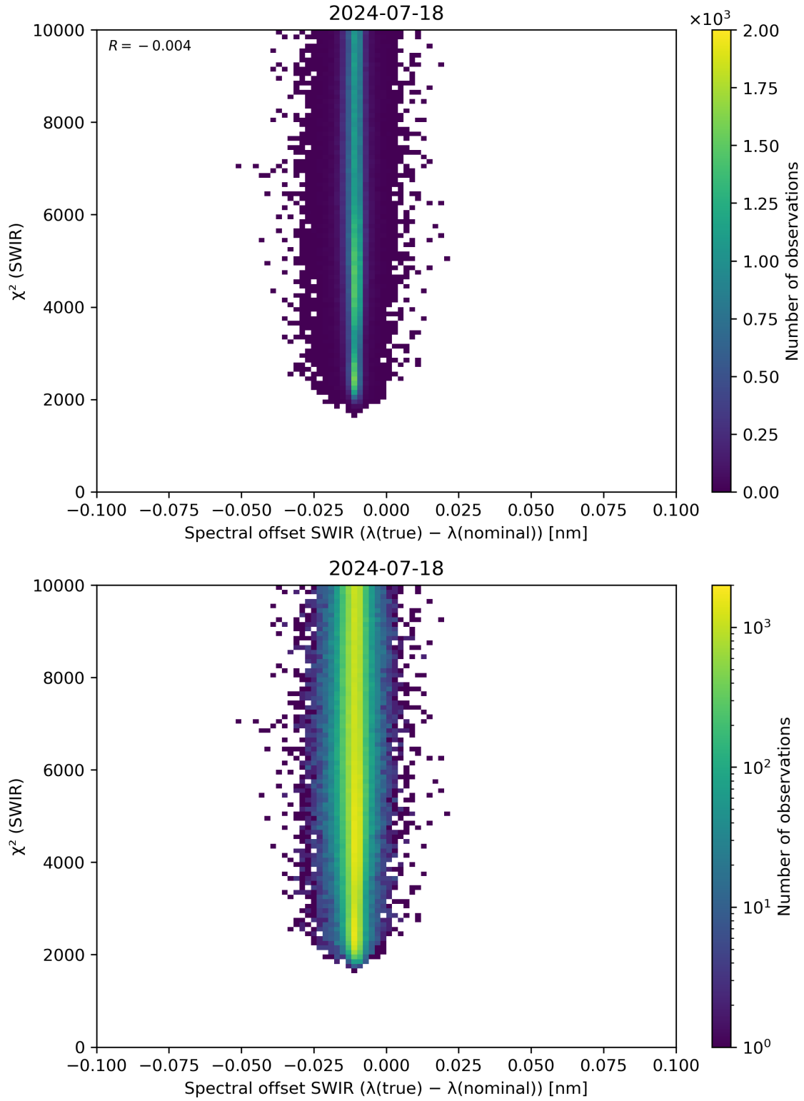
Figure 118: Scatter density plot of “Spectral offset SWIR ( \lambda(\text{true}) - \lambda(\text{nominal}) )” against “ \chi^2 (SWIR)” for 2024-07-17 to 2024-07-19.
