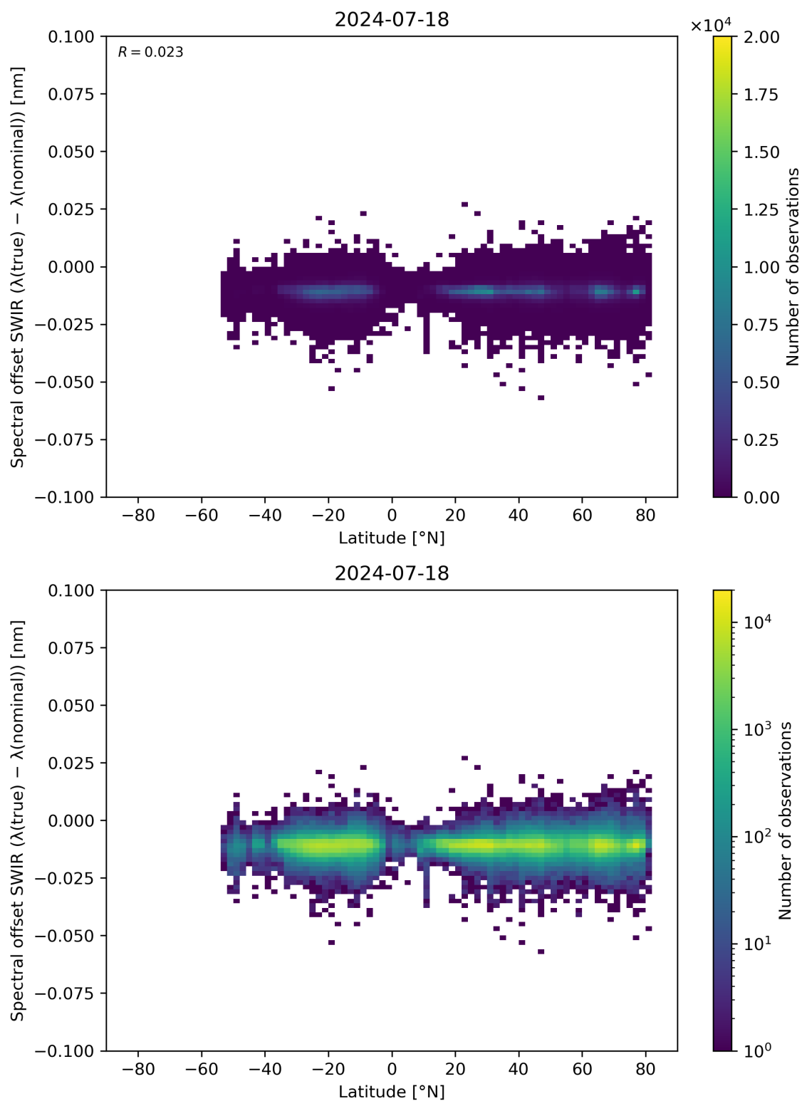
Figure 62: Scatter density plot of “Latitude” against “Spectral offset SWIR ( \lambda(\text{true}) - \lambda(\text{nominal}) )” for 2024-07-17 to 2024-07-19.
