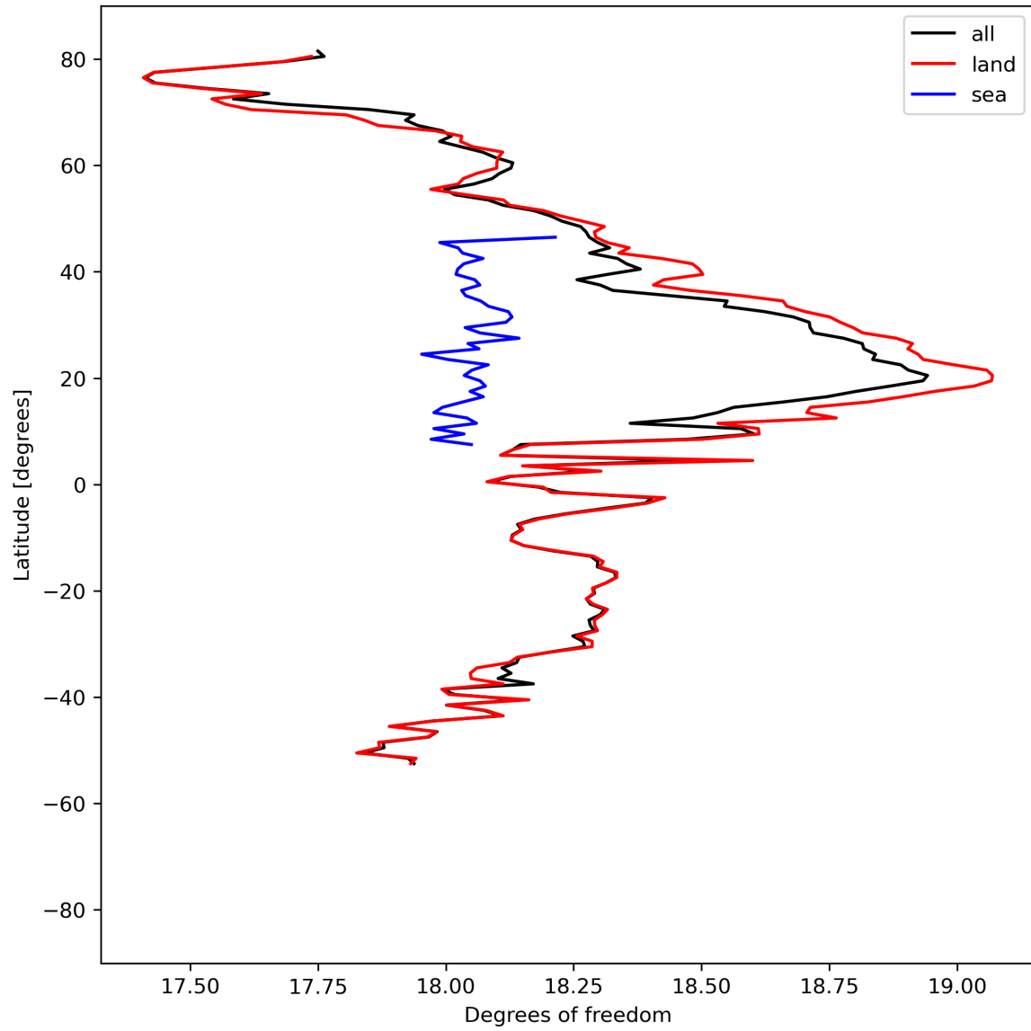
Figure 19: Zonal average of “Degrees of freedom” for 2024-07-17 to 2024-07-19.
