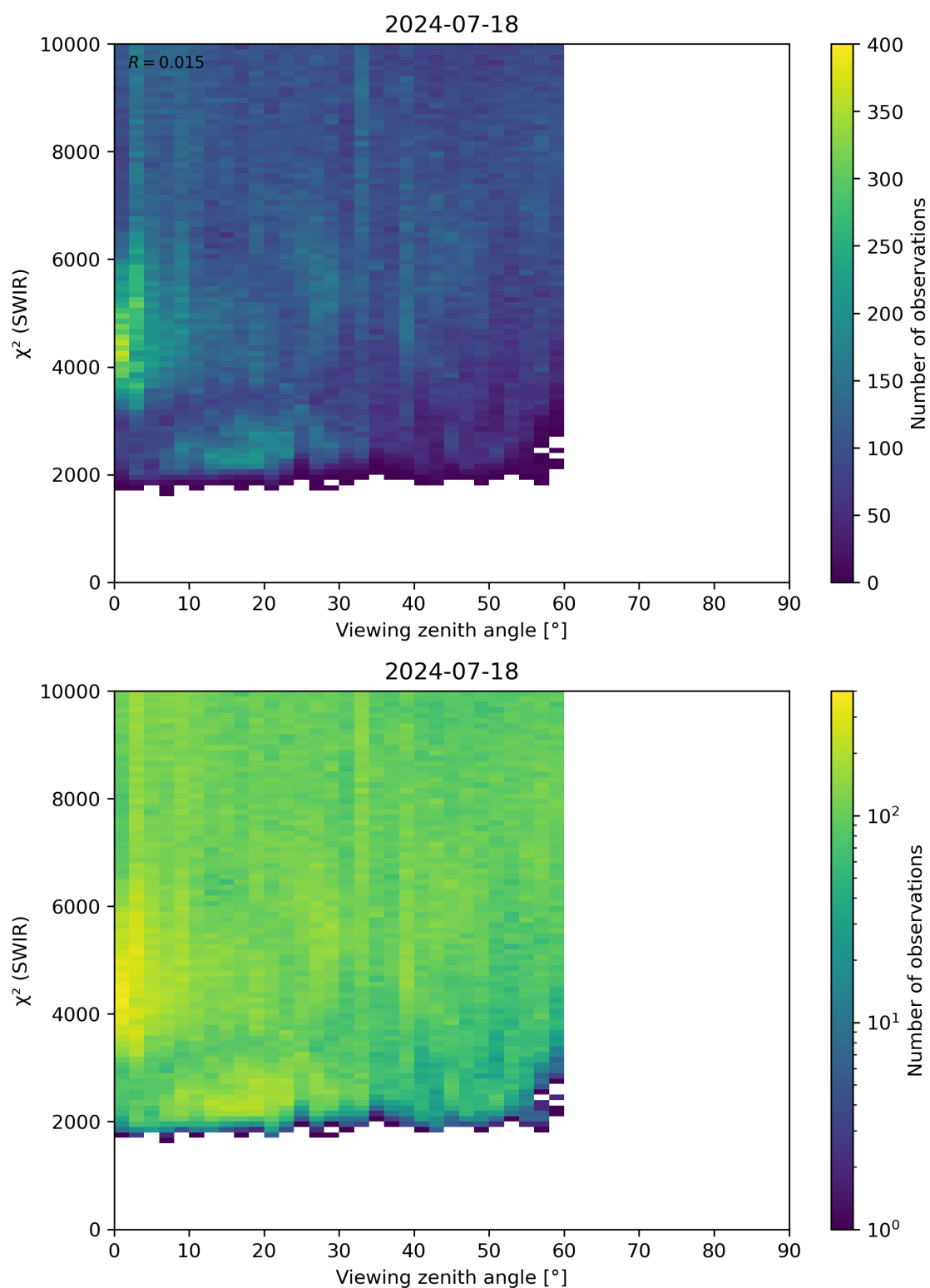
Figure 106: Scatter density plot of “Viewing zenith angle” against “ \chi^2 (SWIR)” for 2024-07-17 to 2024-07-19.
