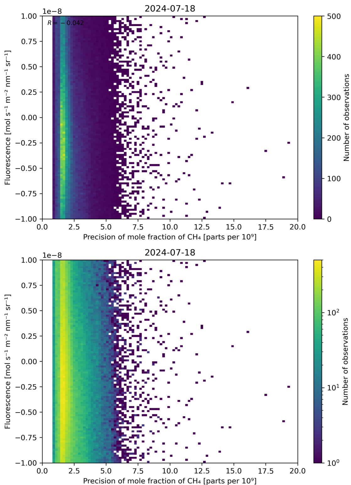
Figure 81: Scatter density plot of “Precision of mole fraction of \text{CH}_4 ” against “Fluorescence” for 2024-07-17 to 2024-07-19.
