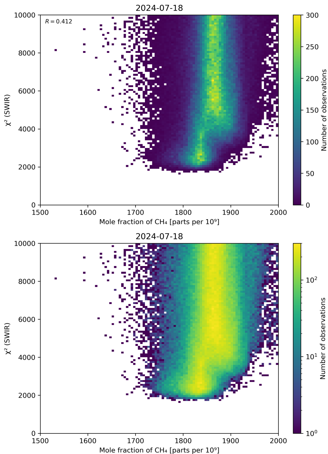
Figure 71: Scatter density plot of “Mole fraction of \text{CH}_4 ” against “ \chi^2 (SWIR)” for 2024-07-17 to 2024-07-19.
