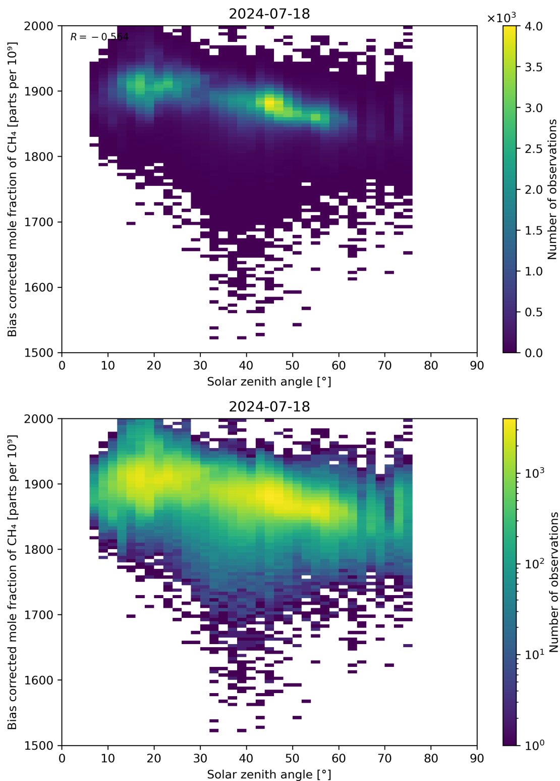
Figure 100: Scatter density plot of “Solar zenith angle” against “Bias corrected mole fraction of CH 4 ” for 2024-07-17 to 2024-07-19.
