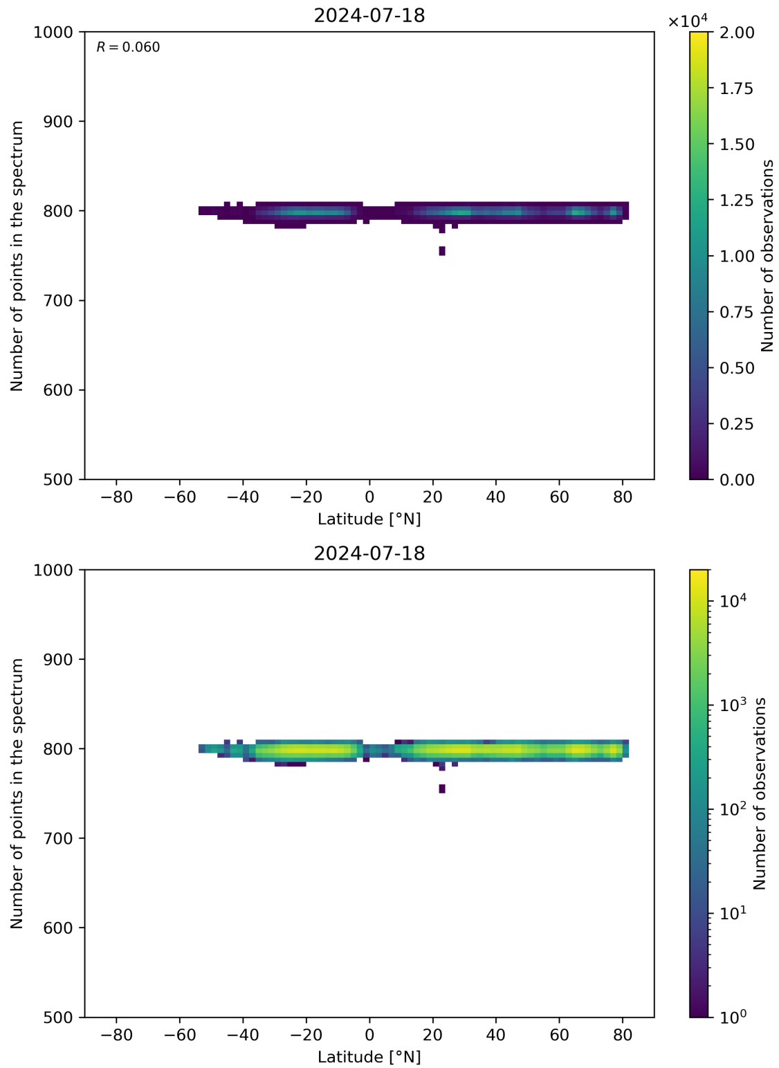
Figure 61: Scatter density plot of “Latitude” against “Number of points in the spectrum” for 2024-07-17 to 2024-07-19.
