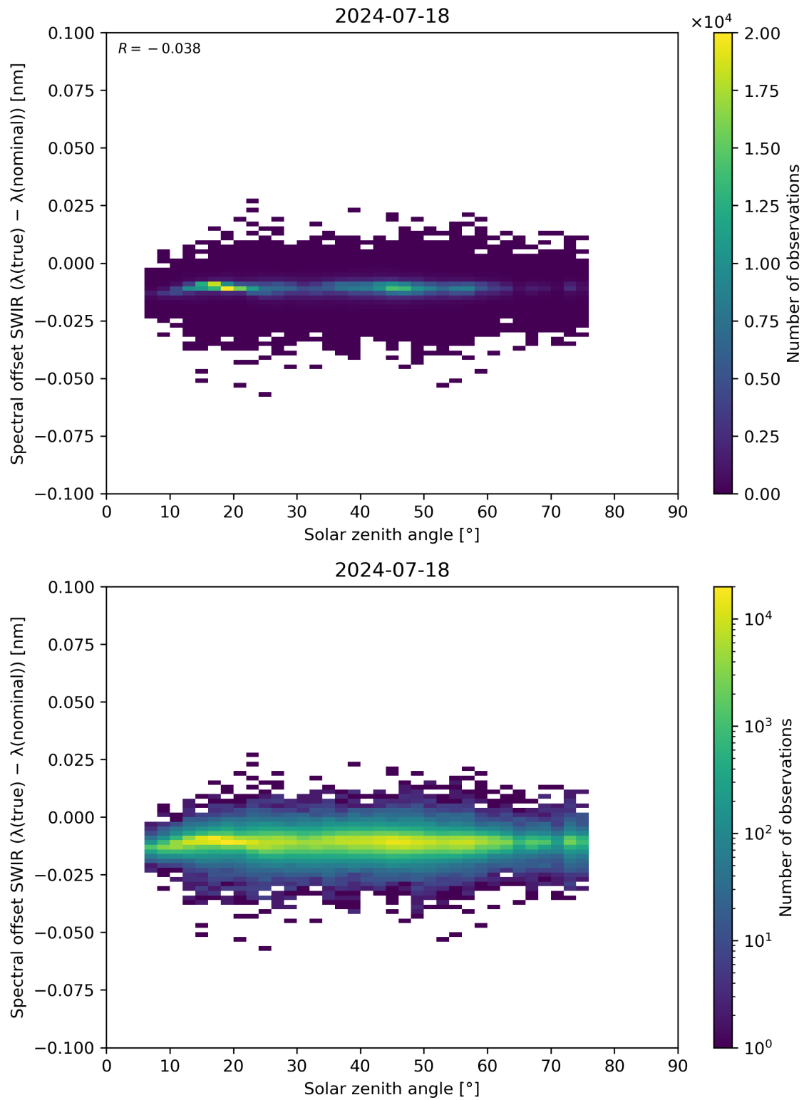
Figure 104: Scatter density plot of “Solar zenith angle” against “Spectral offset SWIR ( \lambda(\text{true}) - \lambda(\text{nominal}) )” for 2024-07-17 to 2024-07-19.
