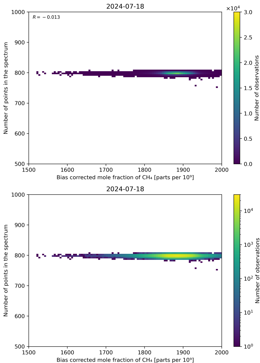
Figure 68: Scatter density plot of “Bias corrected mole fraction of CH 4 ” against “Number of points in the spectrum” for 2024-07-17 to 2024-07-19.
