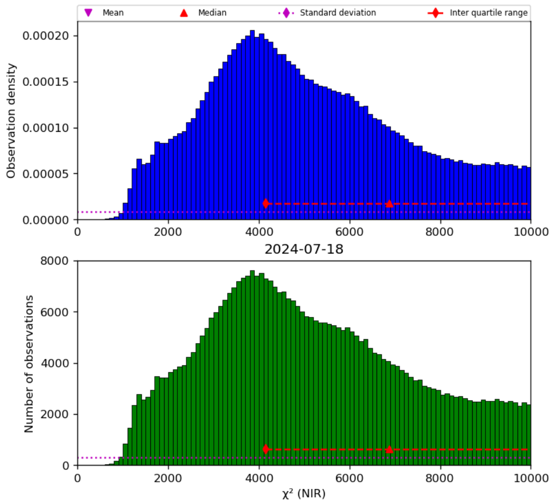
Figure 29: Histogram of “ \chi^2 (NIR)” for 2024-07-17 to 2024-07-19
