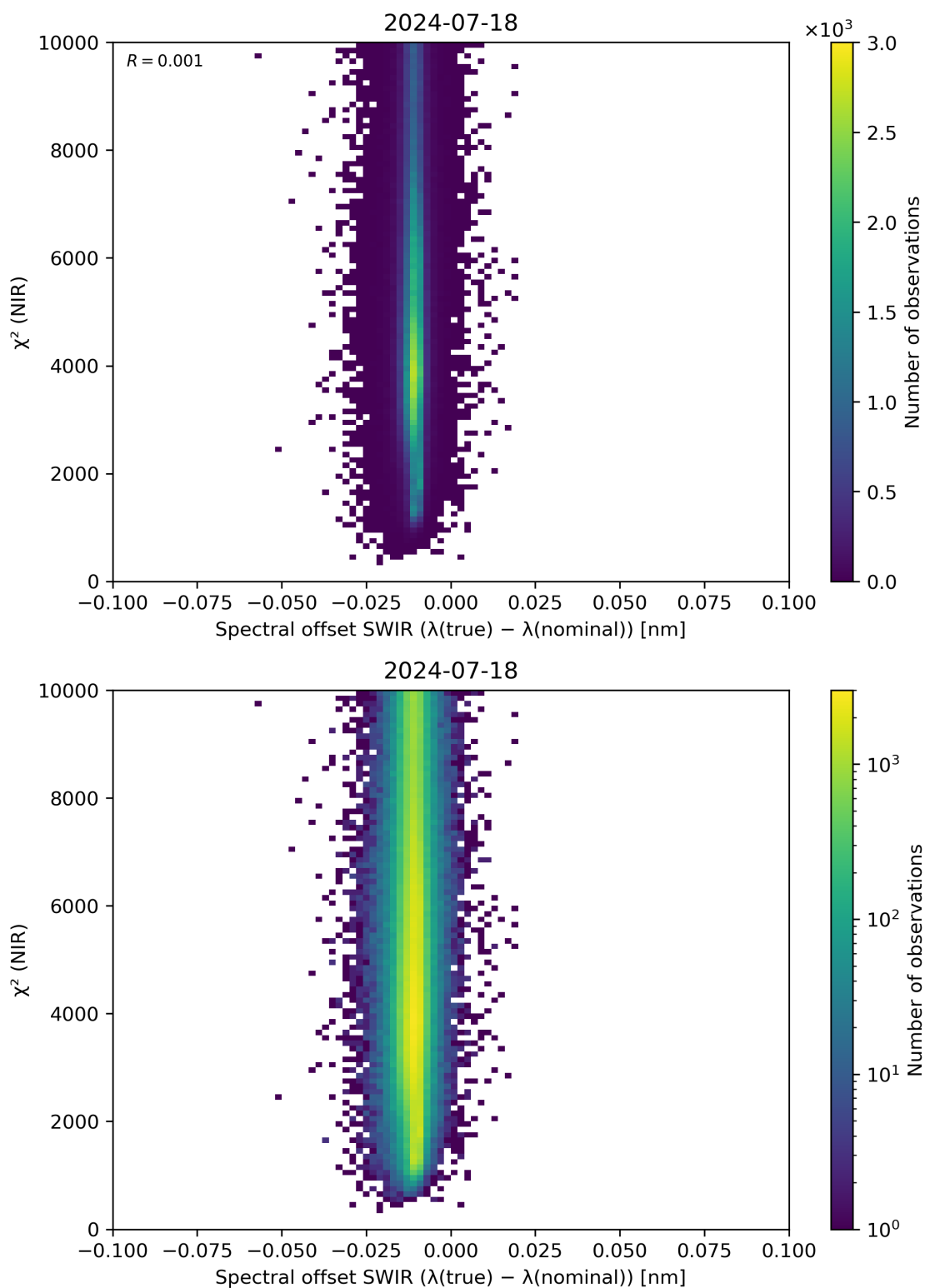
Figure 117: Scatter density plot of “Spectral offset SWIR ( \lambda(\text{true}) - \lambda(\text{nominal}) )” against “ \chi^2 (NIR)” for 2024-07-17 to 2024-07-19.
