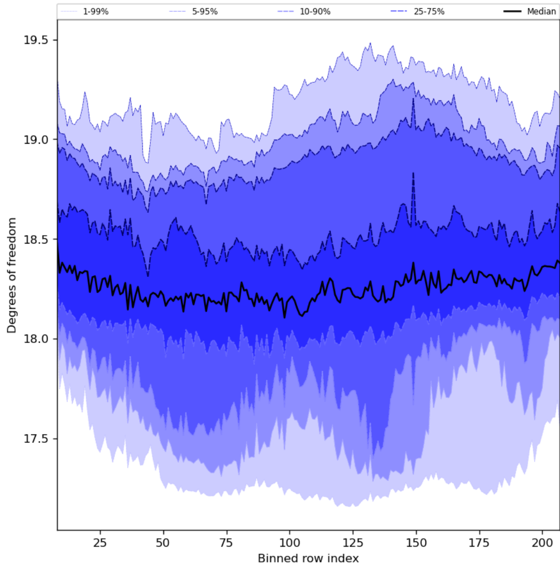
Figure 41: Along track statistics of “Degrees of freedom” for 2024-07-17 to 2024-07-19
