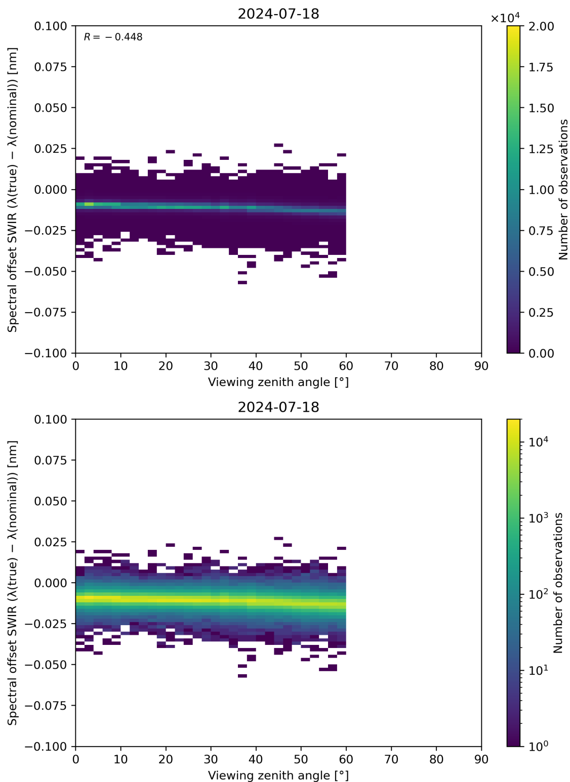
Figure 116: Scatter density plot of “Viewing zenith angle” against “Spectral offset SWIR ( \lambda(\text{true}) - \lambda(\text{nominal}) )” for 2024-07-17 to 2024-07-19.
