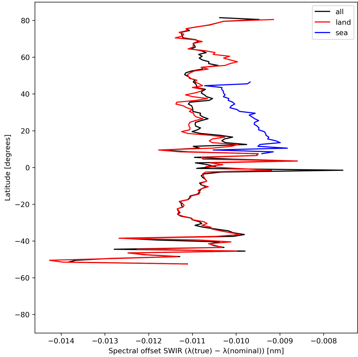
Figure 16: Zonal average of “Spectral offset SWIR ( \lambda(\text{true}) - \lambda(\text{nominal}) )” for 2024-07-17 to 2024-07-19.
