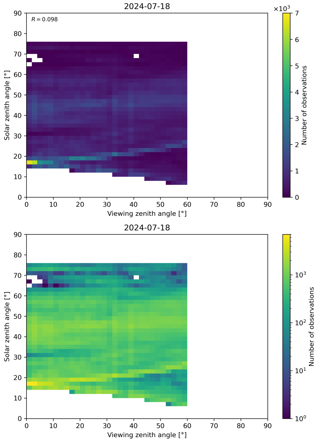
Figure 115: Scatter density plot of “Viewing zenith angle” against “Solar zenith angle” for 2024-07-17 to 2024-07-19.
