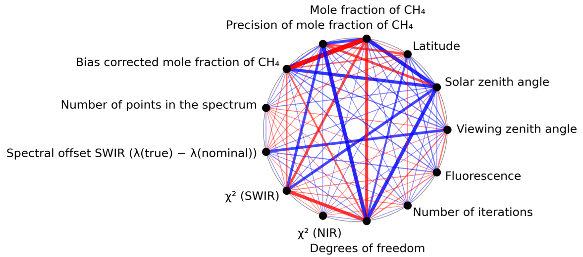
Figure 1: Map of correlation graph for 2024-07-17 to 2024-07-19.
