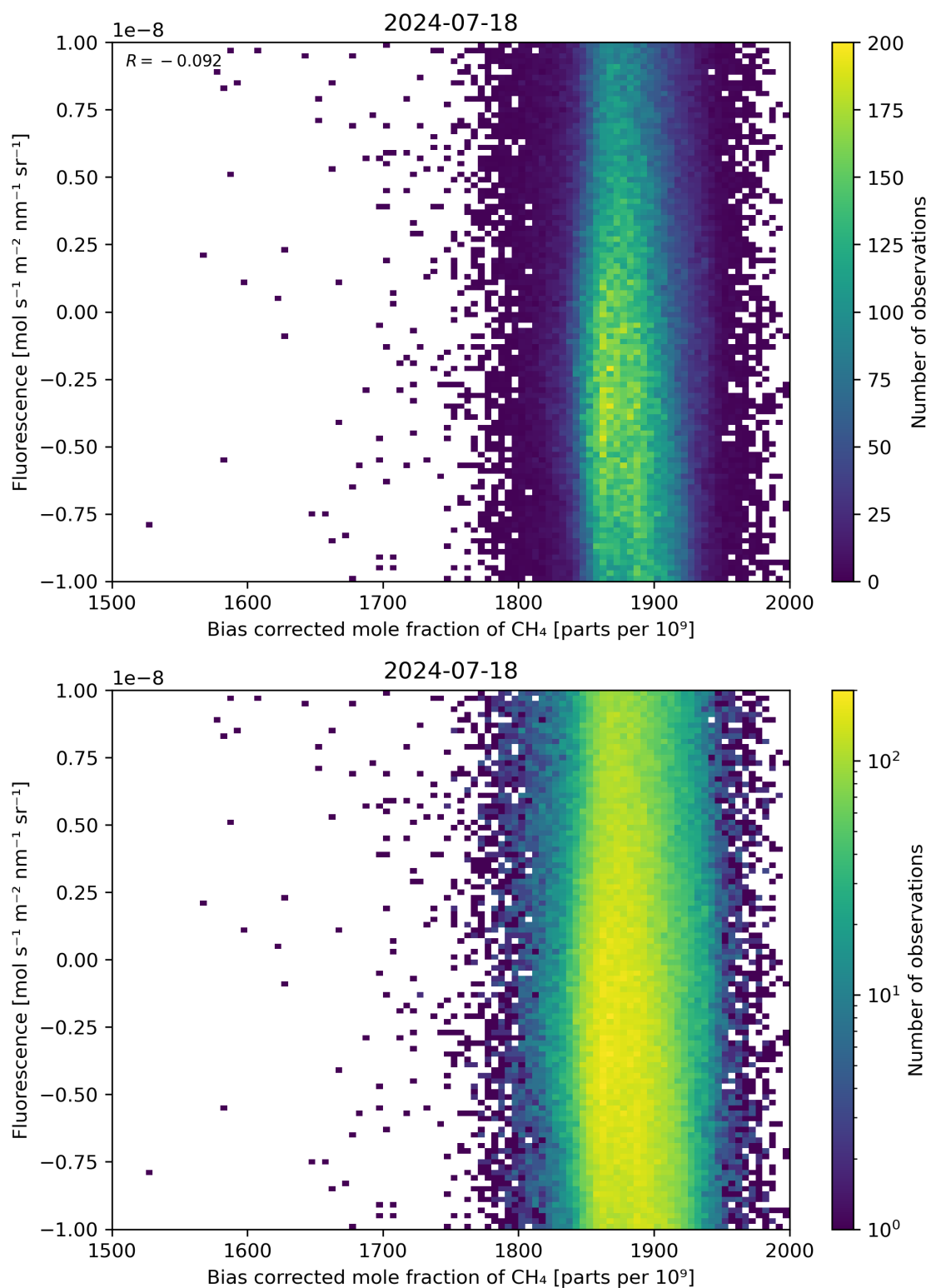
Figure 66: Scatter density plot of “Bias corrected mole fraction of \text{CH}_4 ” against “Fluorescence” for 2024-07-17 to 2024-07-19.
