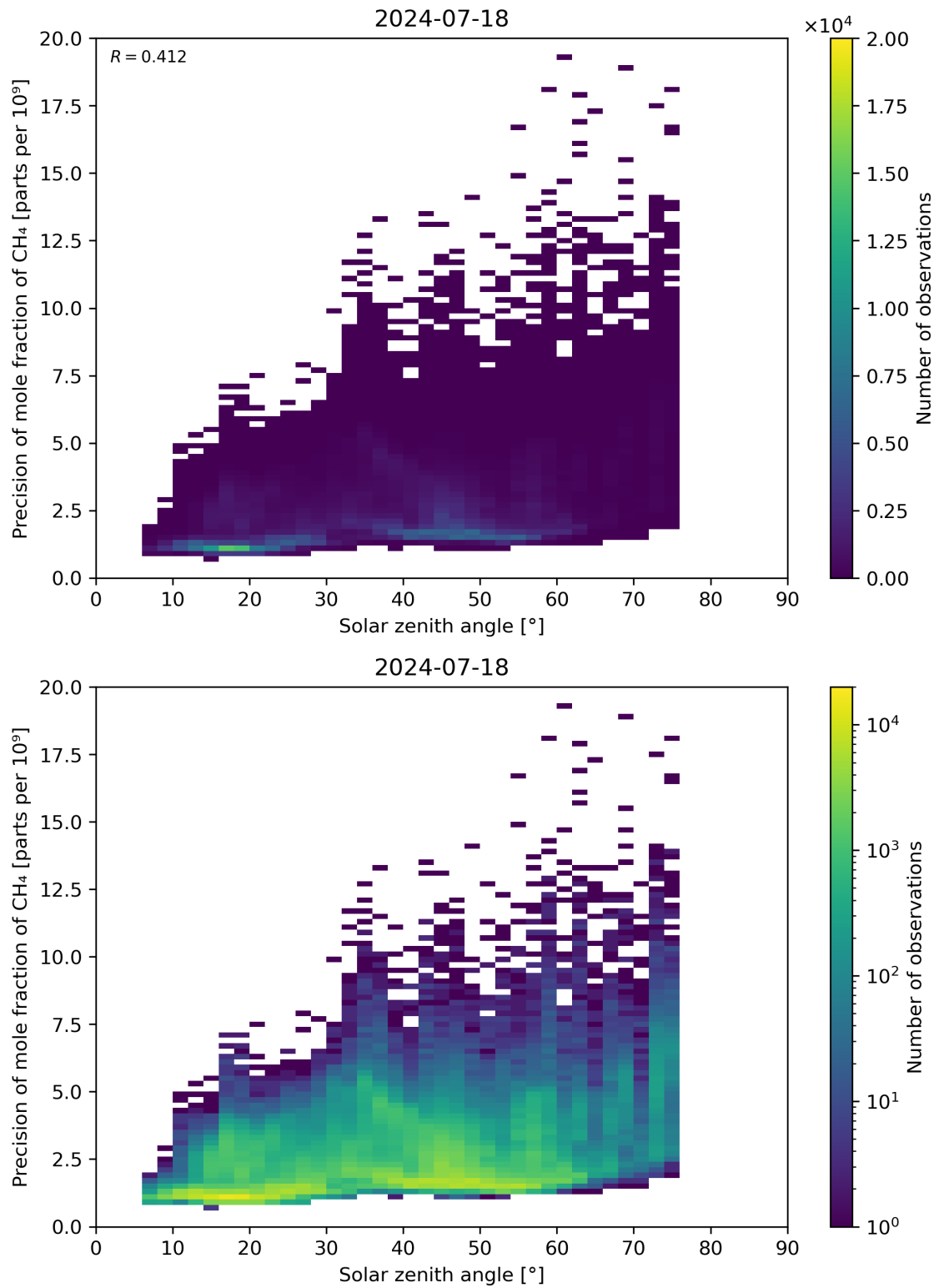
Figure 101: Scatter density plot of “Solar zenith angle” against “Precision of mole fraction of CH 4 ” for 2024-07-17 to 2024-07-19.
