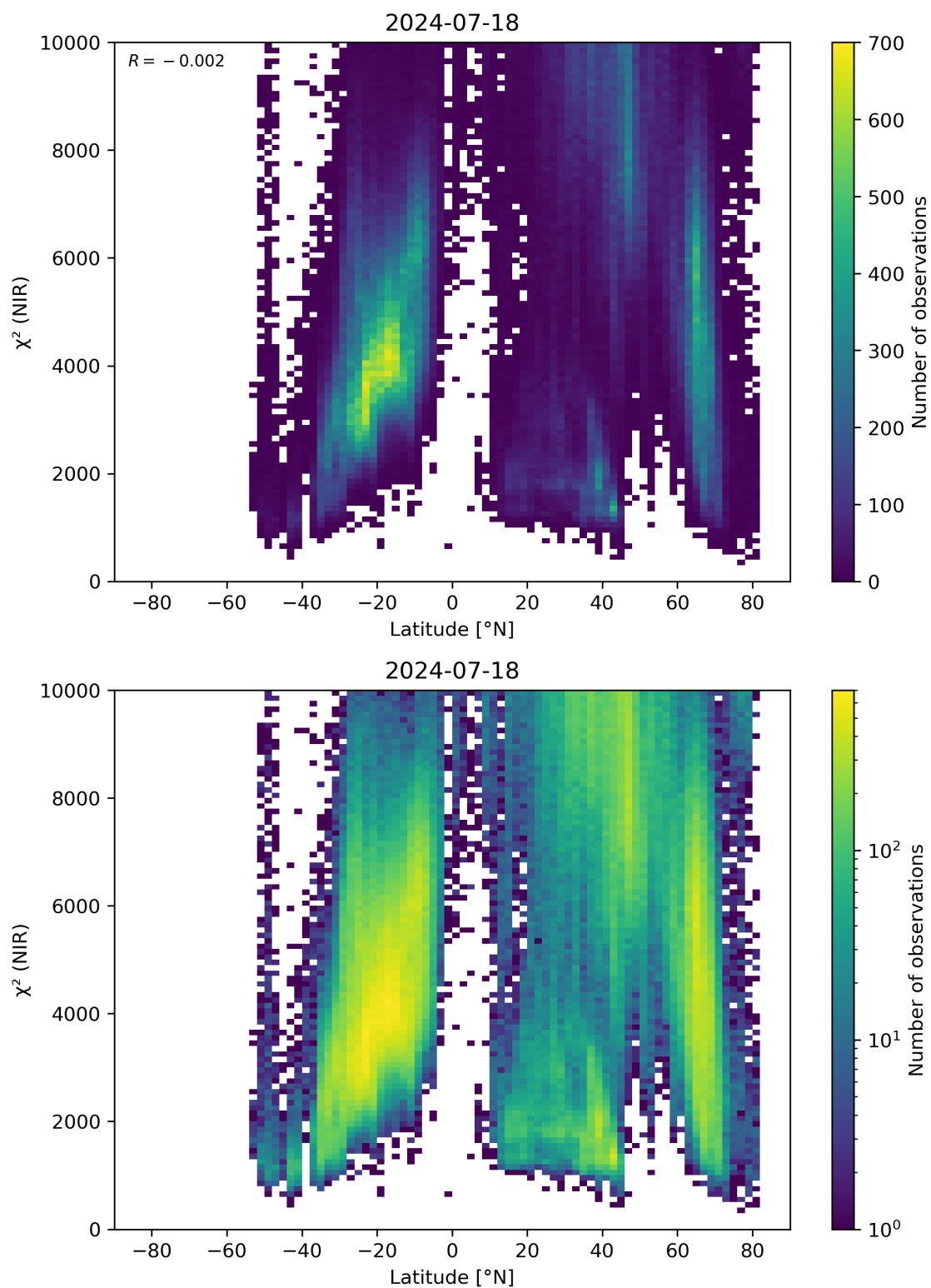
Figure 53: Scatter density plot of “Latitude” against “ \chi^2 (NIR)” for 2024-07-17 to 2024-07-19.
