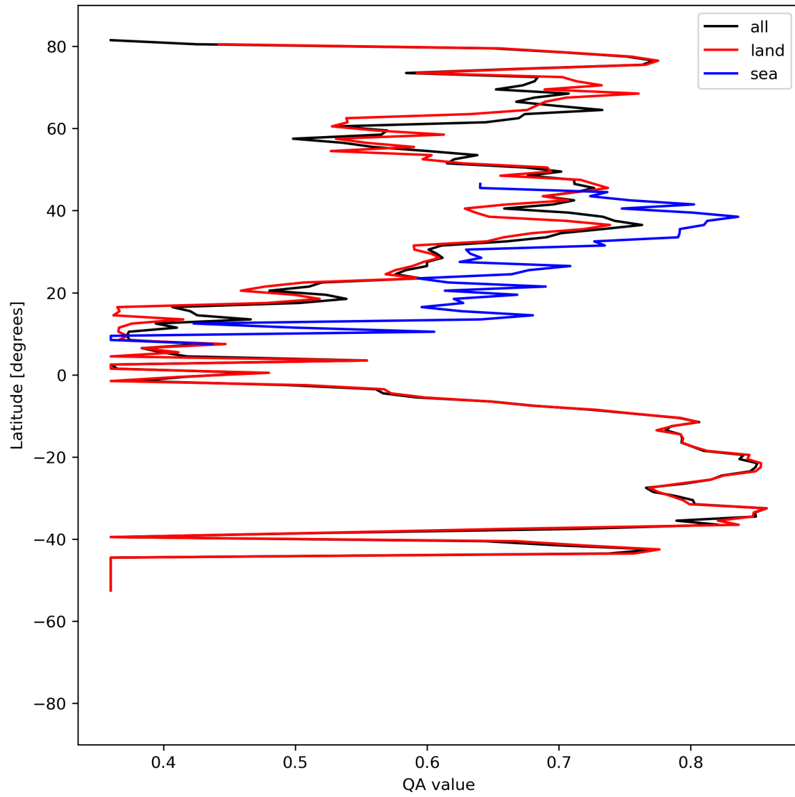
Figure 11: Zonal average of “QA value” for 2024-07-17 to 2024-07-19.
