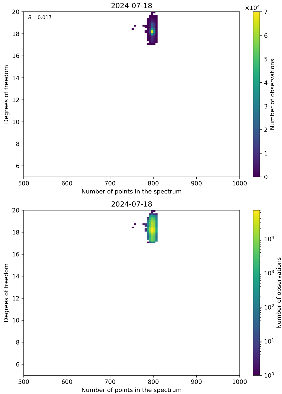
Figure 90: Scatter density plot of “Number of points in the spectrum” against “Degrees of freedom” for 2024-07-17 to 2024-07-19.
