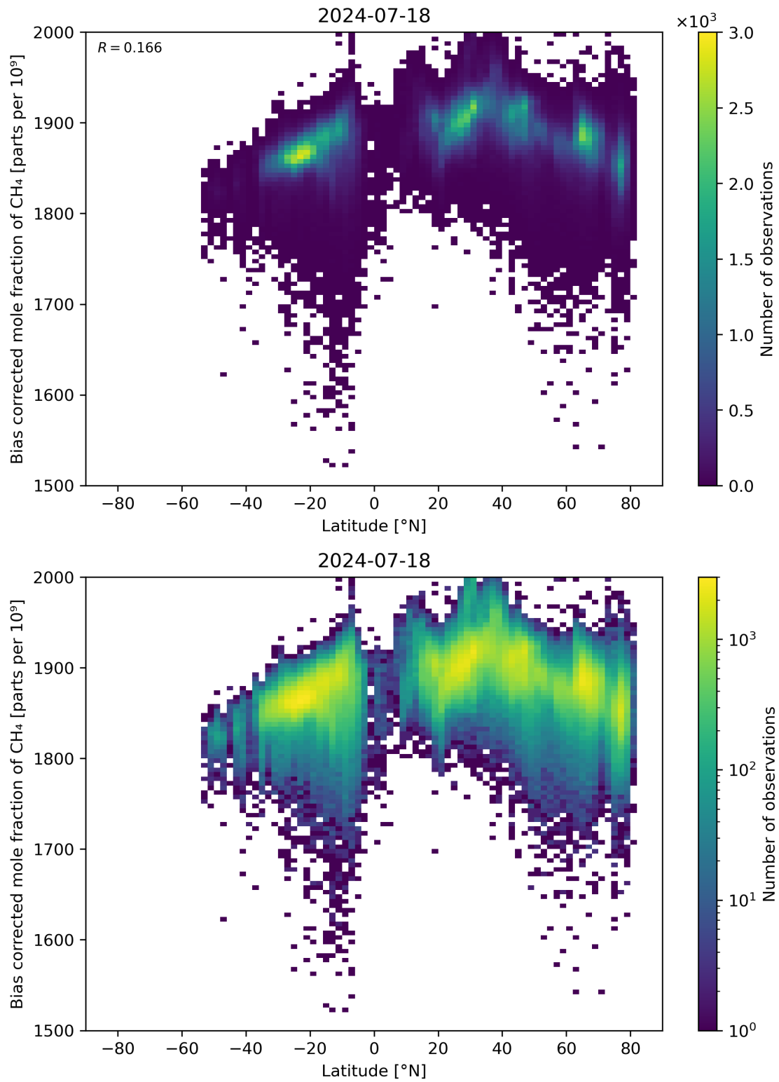
Figure 58: Scatter density plot of “Latitude” against “Bias corrected mole fraction of \text{CH}_4 ” for 2024-07-17 to 2024-07-19.
