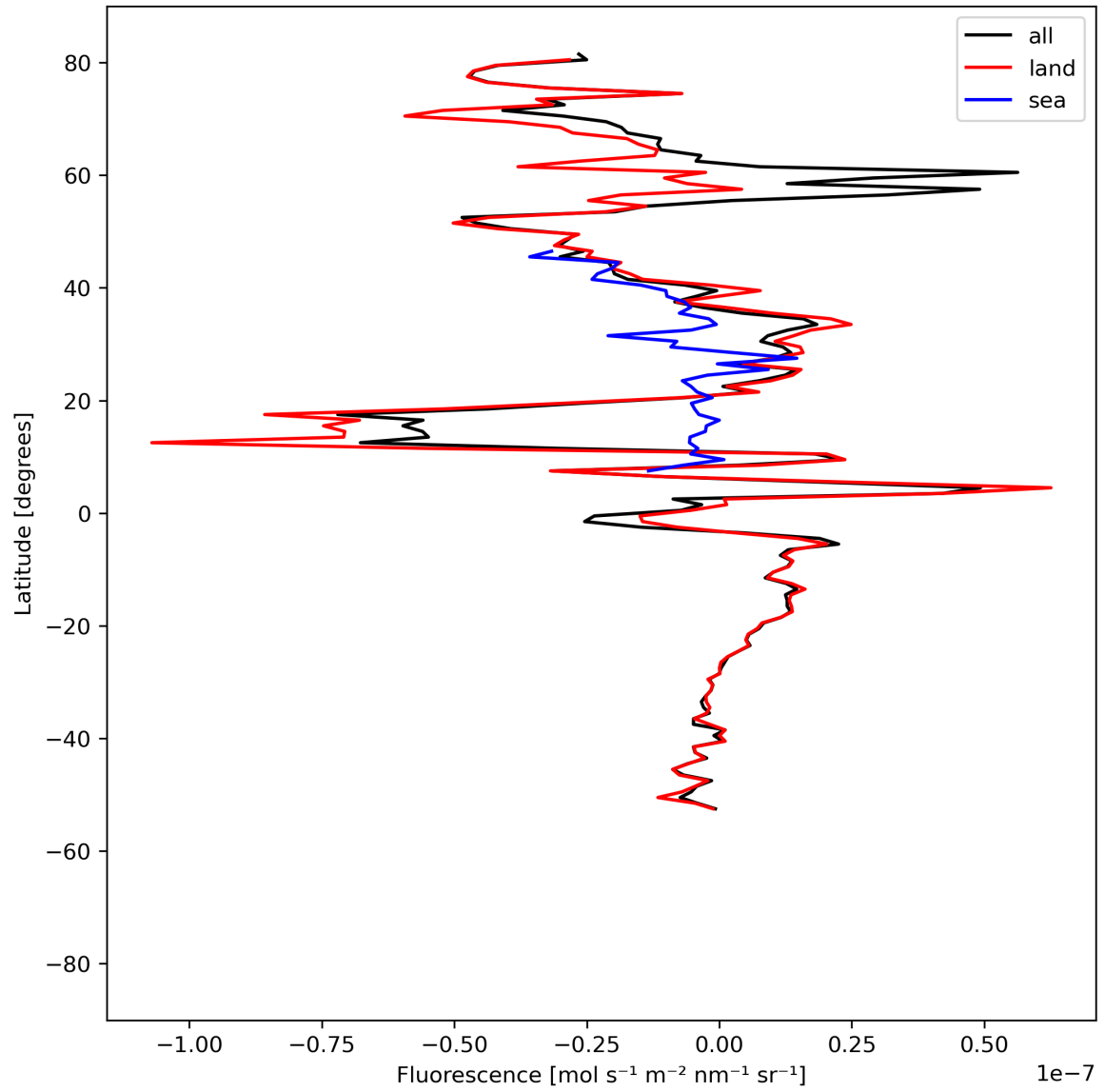
Figure 21: Zonal average of “Fluorescence” for 2024-07-17 to 2024-07-19.
