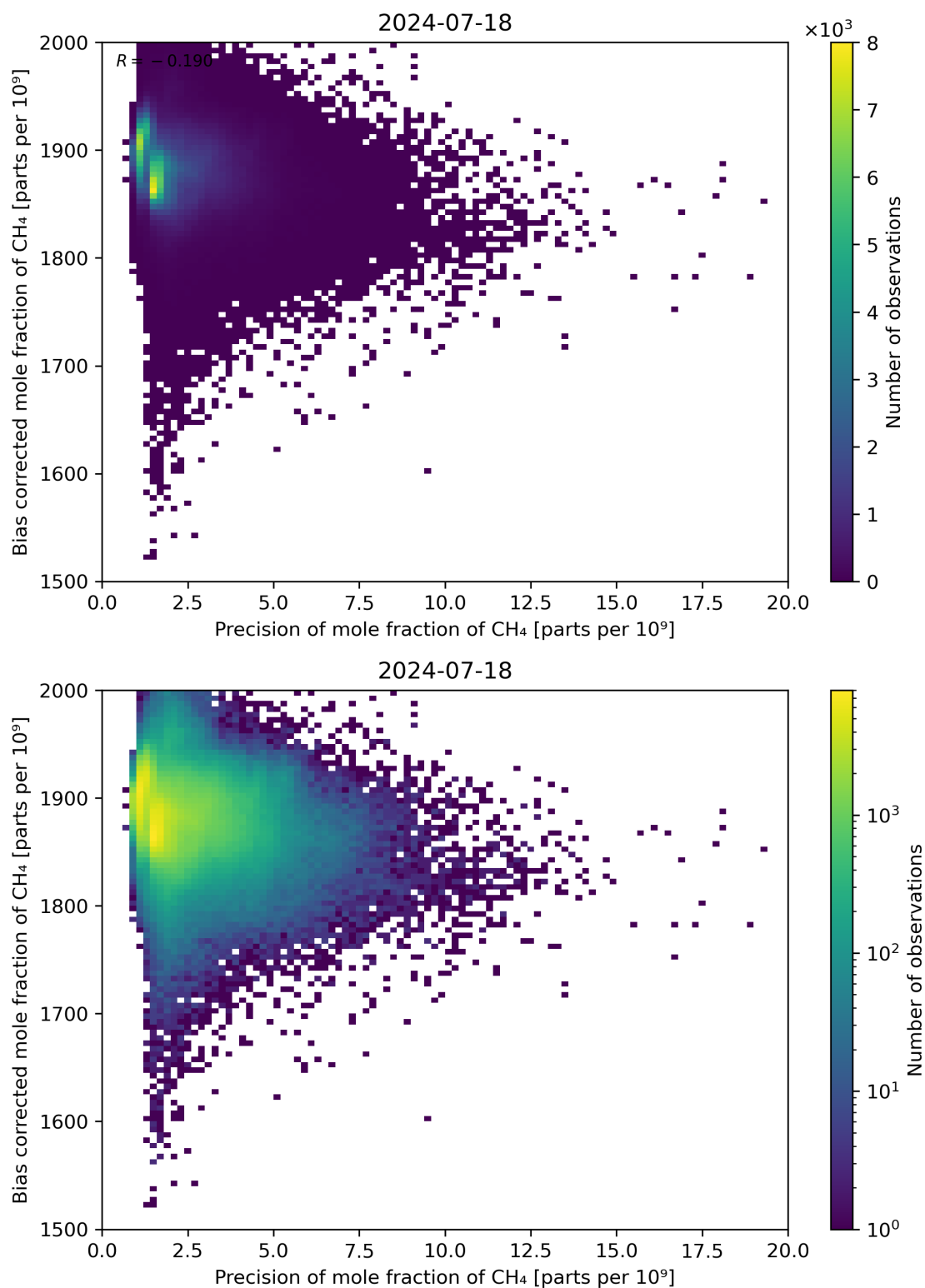
Figure 82: Scatter density plot of “Precision of mole fraction of CH 4 ” against “Bias corrected mole fraction of CH 4 ” for 2024-07-17 to 2024-07-19.
