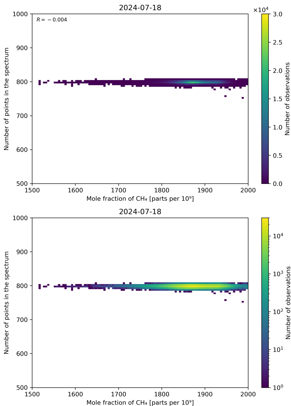
Figure 77: Scatter density plot of “Mole fraction of CH 4 ” against “Number of points in the spectrum” for 2024-07-17 to 2024-07-19.
