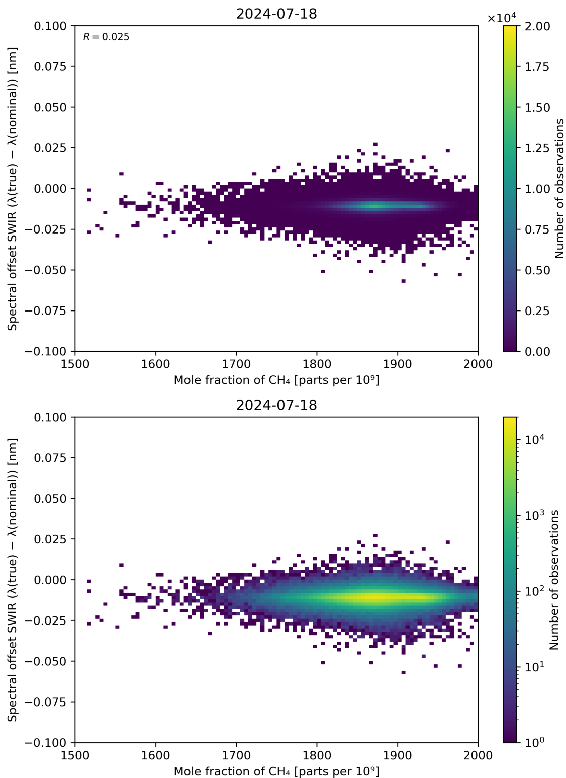
Figure 86: Scatter density plot of “Mole fraction of CH 4 ” against “Spectral offset SWIR ( \lambda(\text{true}) - \lambda(\text{nominal}) )” for 2024-07-17 to 2024-07-19.
