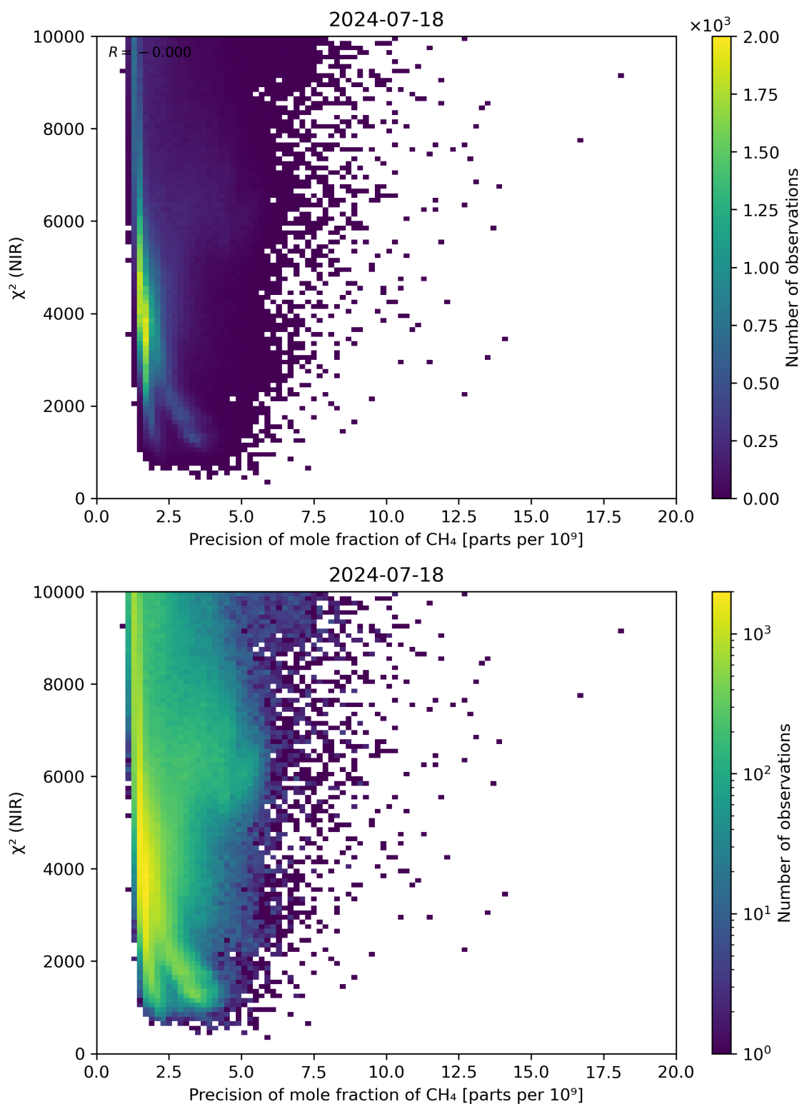
Figure 78: Scatter density plot of “Precision of mole fraction of CH 4 ” against “ \chi^2 (NIR)” for 2024-07-17 to 2024-07-19.
