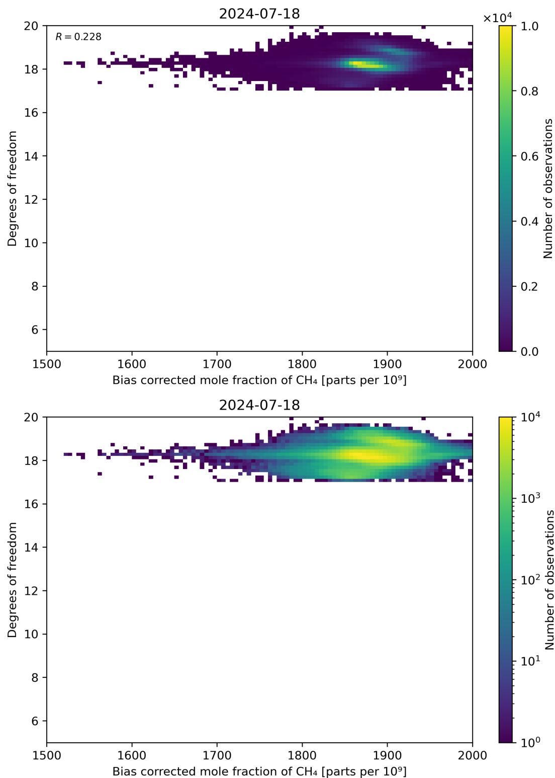
Figure 65: Scatter density plot of “Bias corrected mole fraction of CH 4 ” against “Degrees of freedom” for 2024-07-17 to 2024-07-19.
