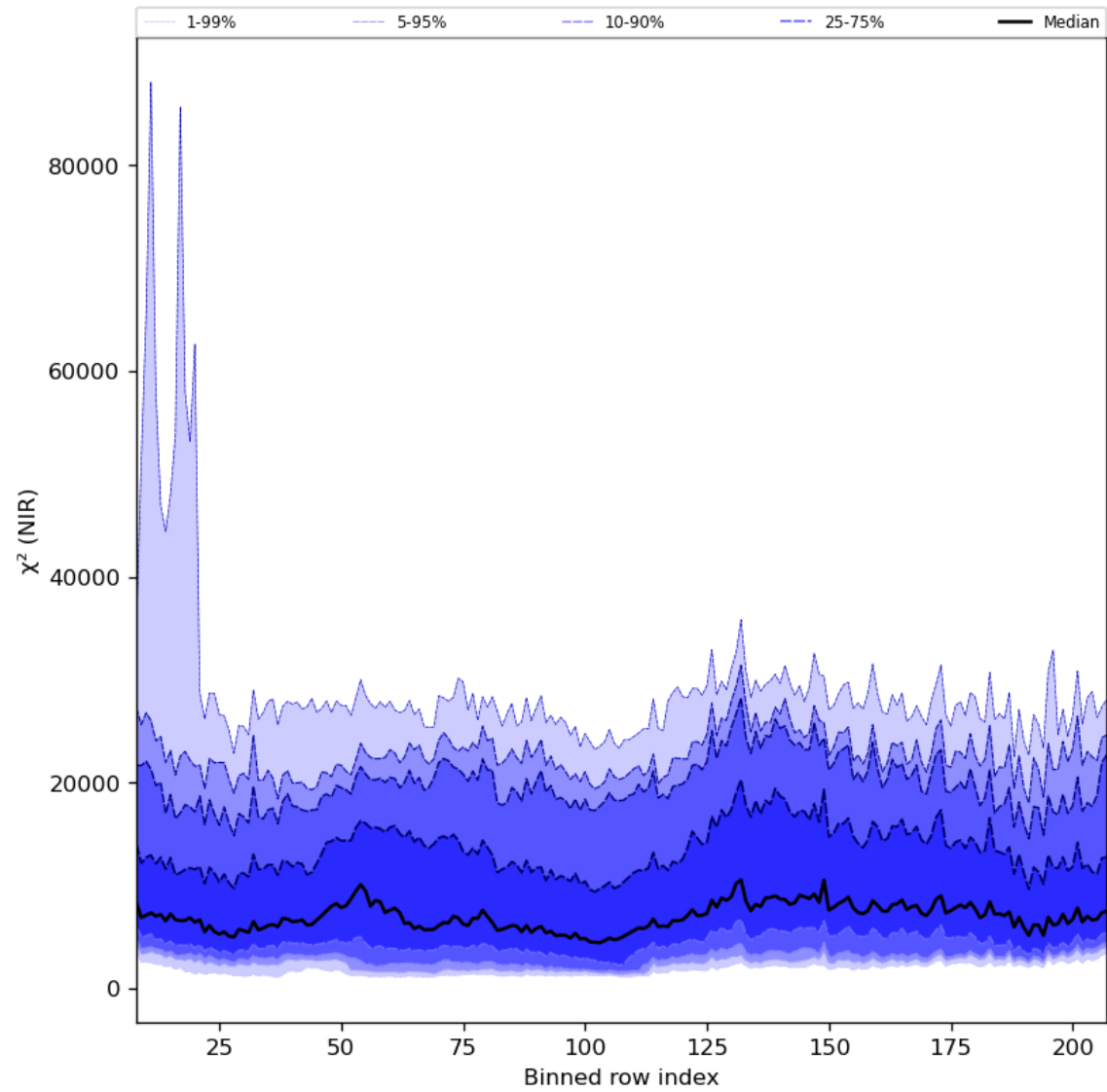
Figure 40: Along track statistics of " \chi^2 (NIR)" for 2024-07-17 to 2024-07-19
