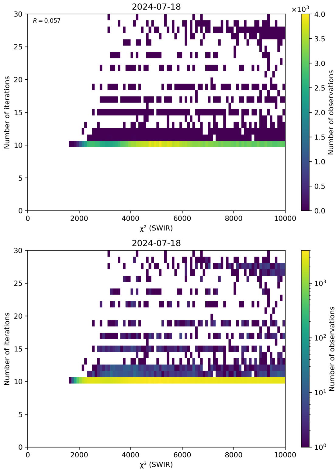
Figure 50: Scatter density plot of “ \chi^2 (SWIR)” against “Number of iterations” for 2024-07-17 to 2024-07-19.
