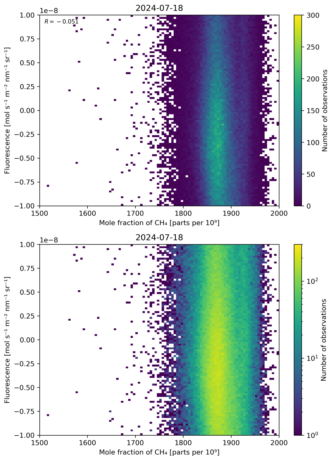
Figure 73: Scatter density plot of “Mole fraction of \text{CH}_4 ” against “Fluorescence” for 2024-07-17 to 2024-07-19.
