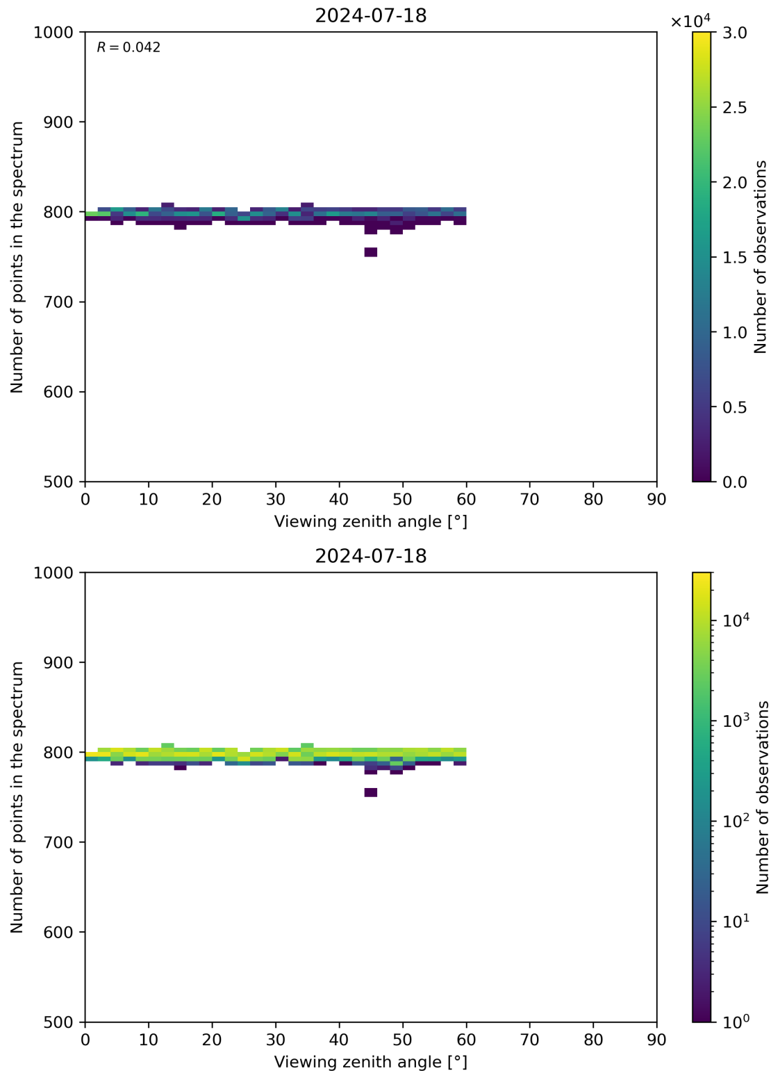
Figure 114: Scatter density plot of “Viewing zenith angle” against “Number of points in the spectrum” for 2024-07-17 to 2024-07-19.
