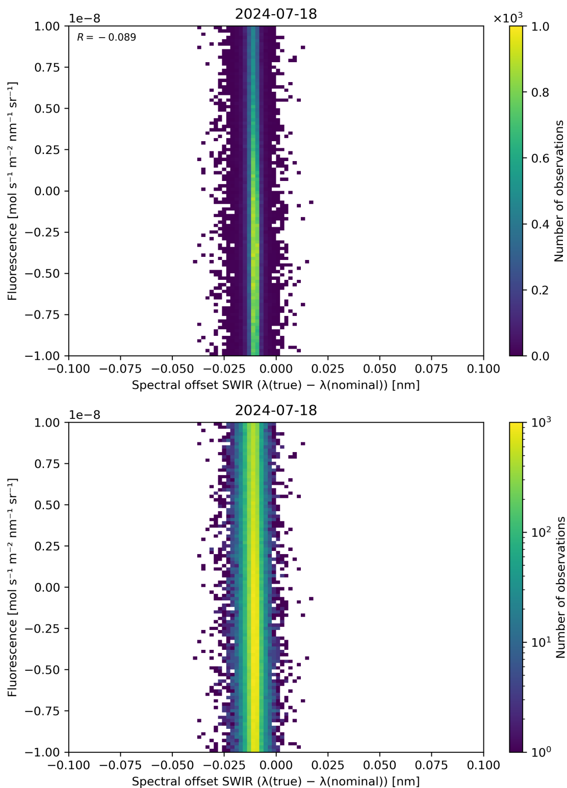
Figure 120: Scatter density plot of “Spectral offset SWIR ( \lambda(\text{true}) - \lambda(\text{nominal}) )” against “Fluorescence” for 2024-07-17 to 2024-07-19.
