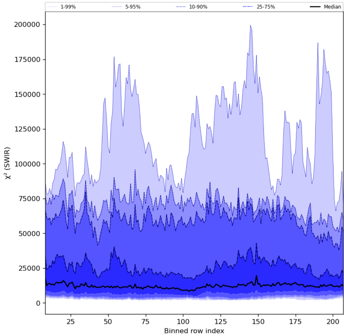
Figure 39: Along track statistics of " \chi^2 (SWIR)" for 2024-07-17 to 2024-07-19
