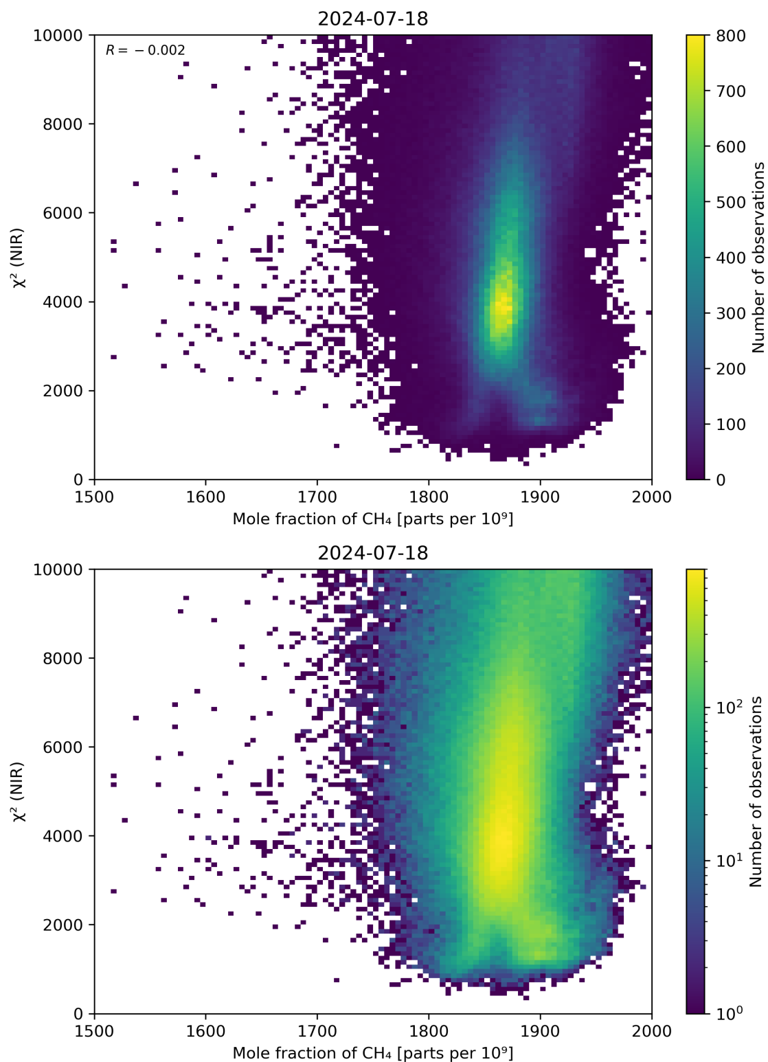
Figure 70: Scatter density plot of “Mole fraction of \text{CH}_4 ” against “ \chi^2 (NIR)” for 2024-07-17 to 2024-07-19.
