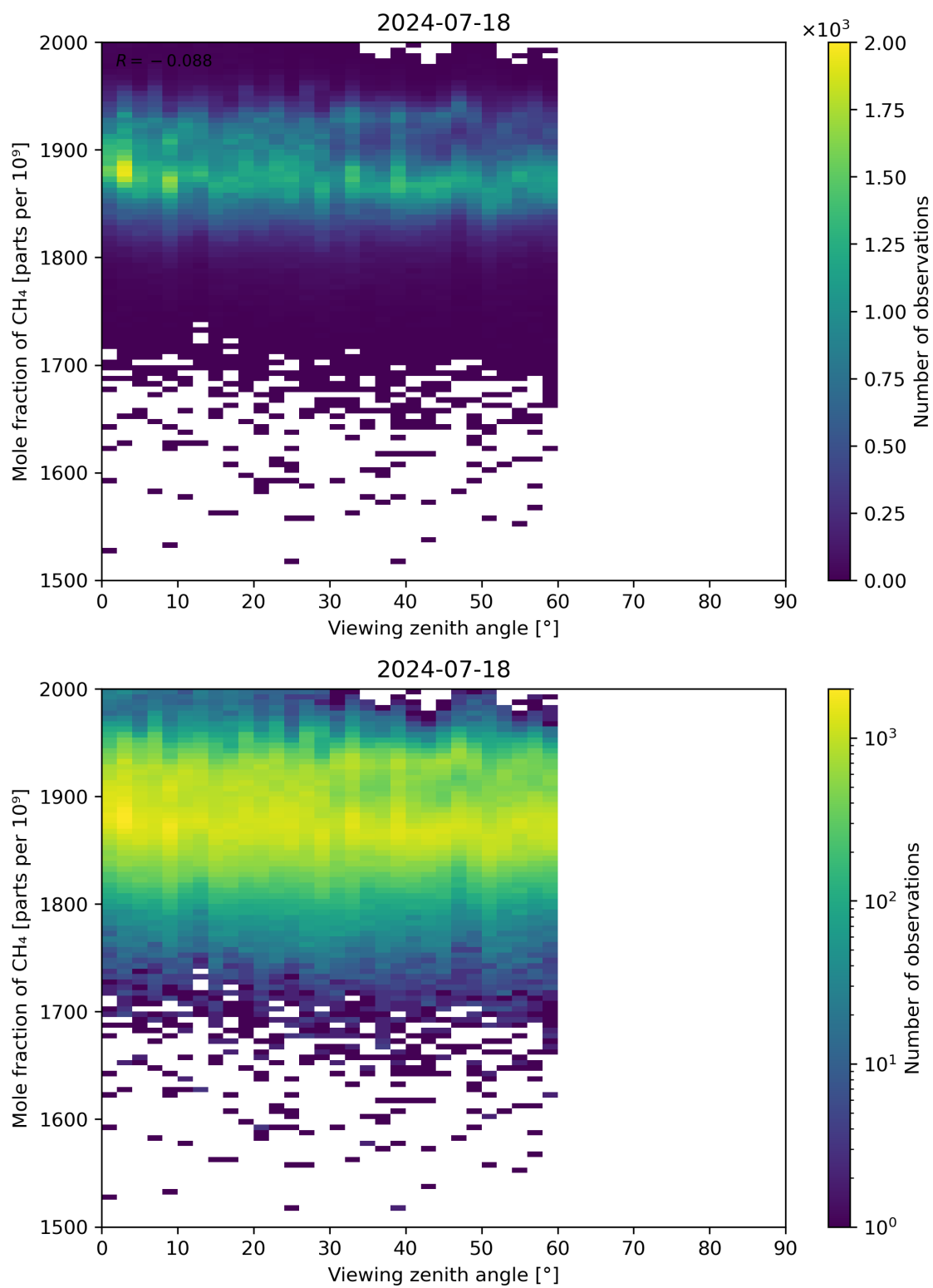
Figure 110: Scatter density plot of “Viewing zenith angle” against “Mole fraction of CH 4 ” for 2024-07-17 to 2024-07-19.
