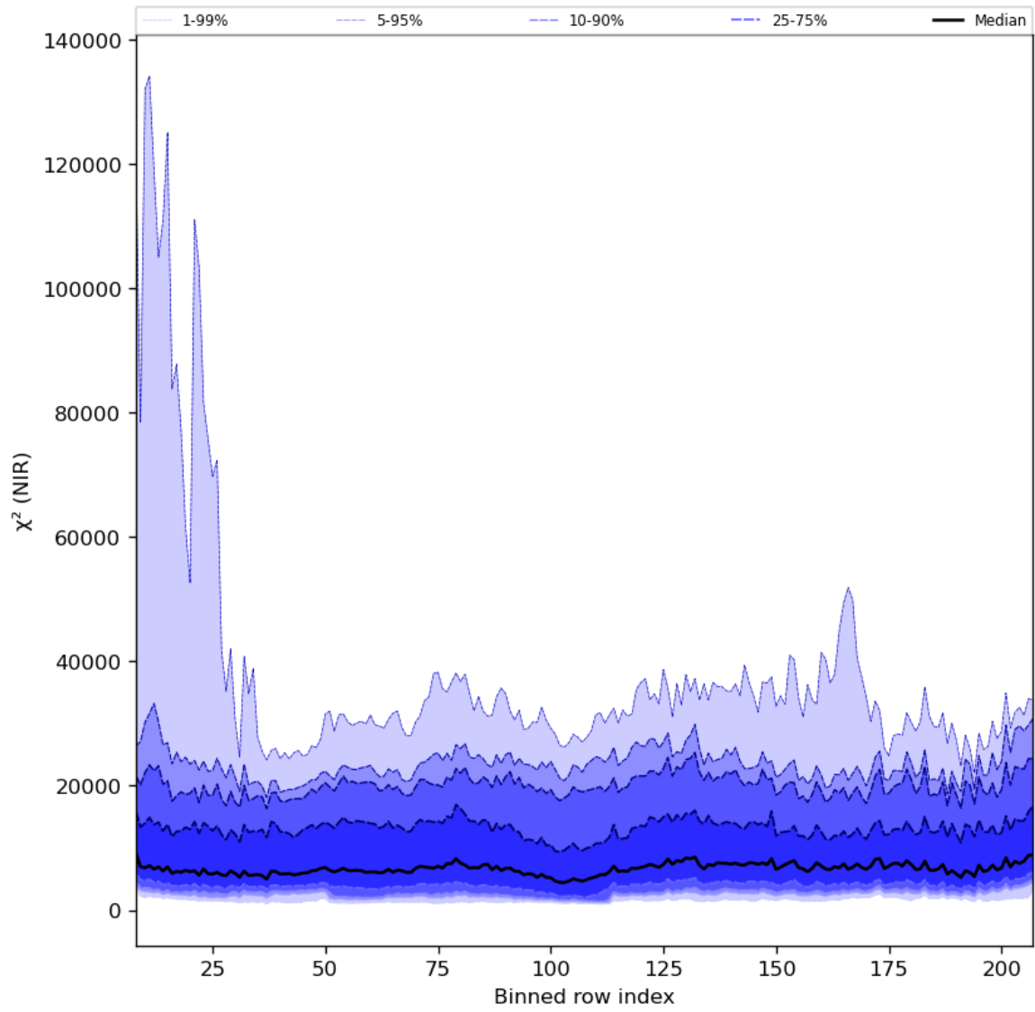
Figure 40: Along track statistics of “ \chi^2 (NIR)” for 2024-07-18 to 2024-07-20
