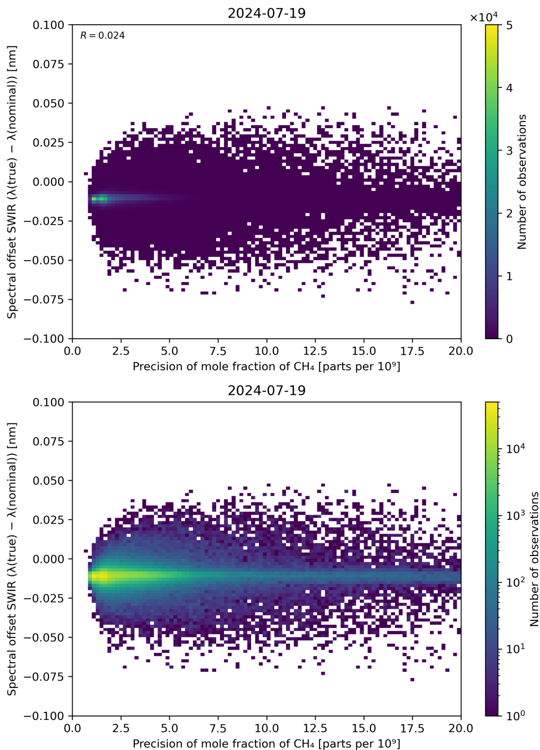
Figure 85: Scatter density plot of “Precision of mole fraction of CH 4 ” against “Spectral offset SWIR ( \lambda(\text{true}) - \lambda(\text{nominal}) )” for 2024-07-18 to 2024-07-20.
