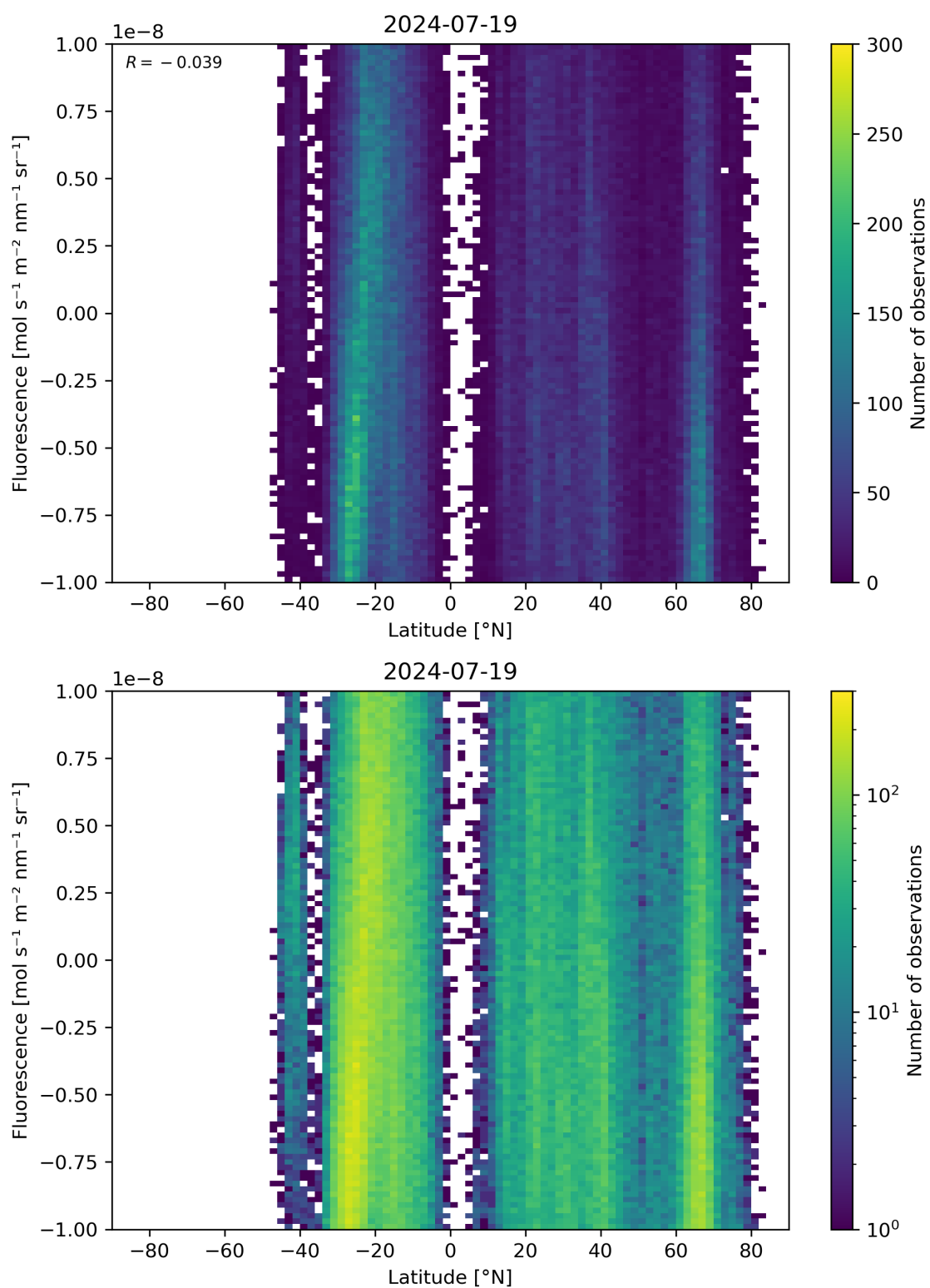
Figure 56: Scatter density plot of “Latitude” against “Fluorescence” for 2024-07-18 to 2024-07-20.
