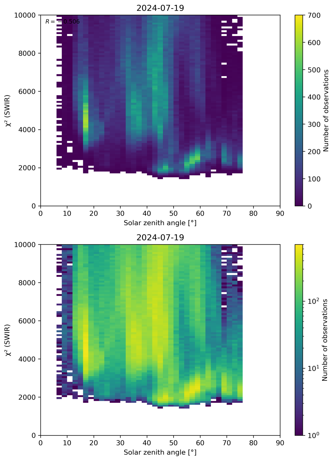
Figure 95: Scatter density plot of “Solar zenith angle” against “ \chi^2 (SWIR)” for 2024-07-18 to 2024-07-20.
