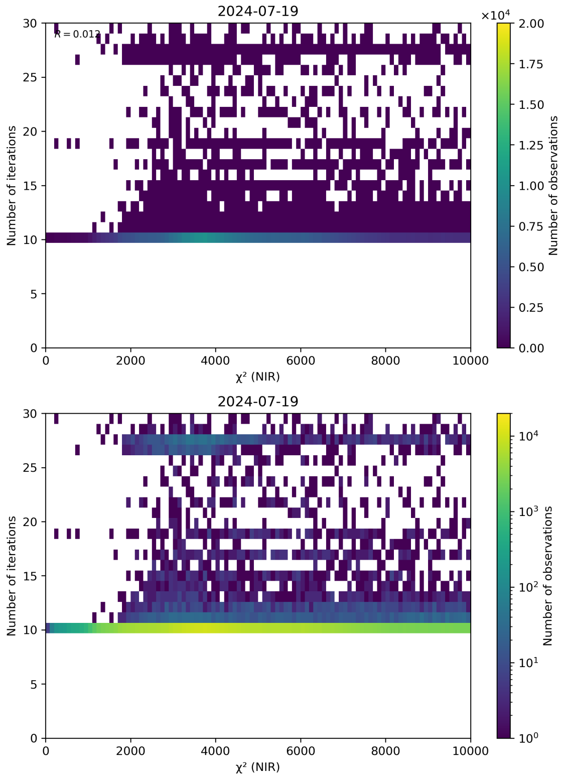
Figure 46: Scatter density plot of “ \chi^2 (NIR)” against “Number of iterations” for 2024-07-18 to 2024-07-20.
