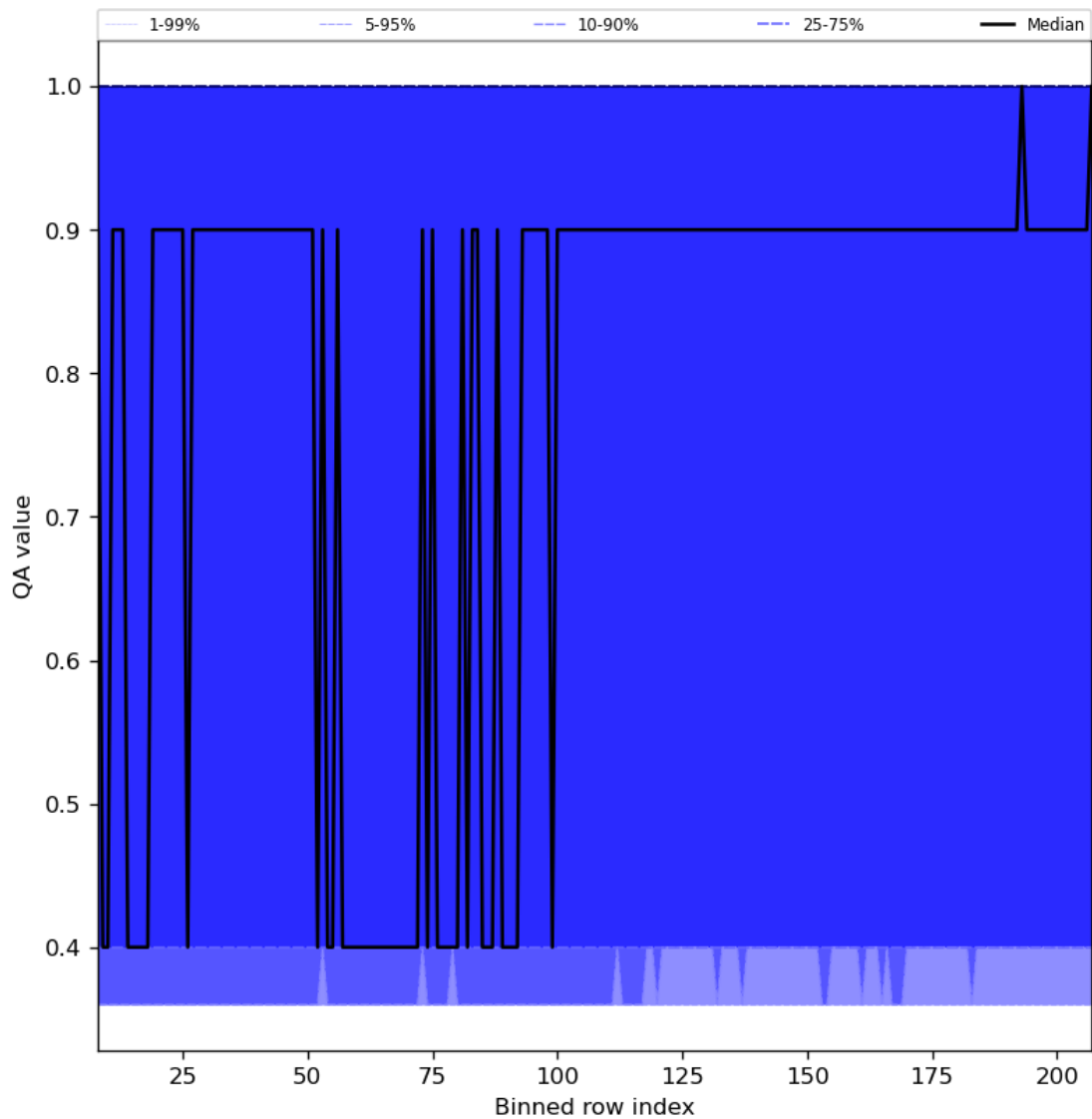
Figure 33: Along track statistics of “QA value” for 2024-07-18 to 2024-07-20
