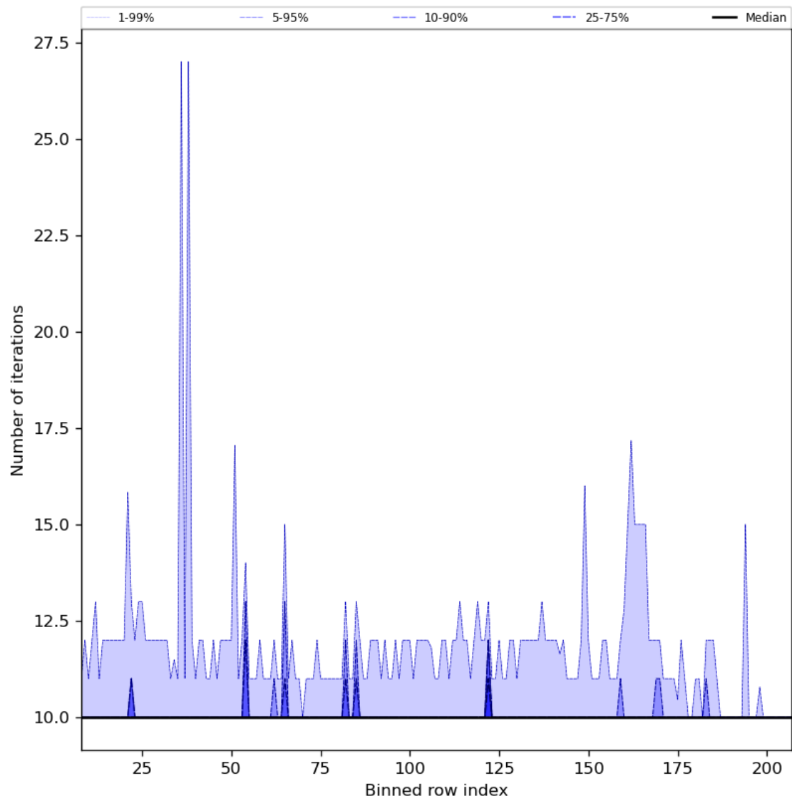
Figure 42: Along track statistics of “Number of iterations” for 2024-07-18 to 2024-07-20
