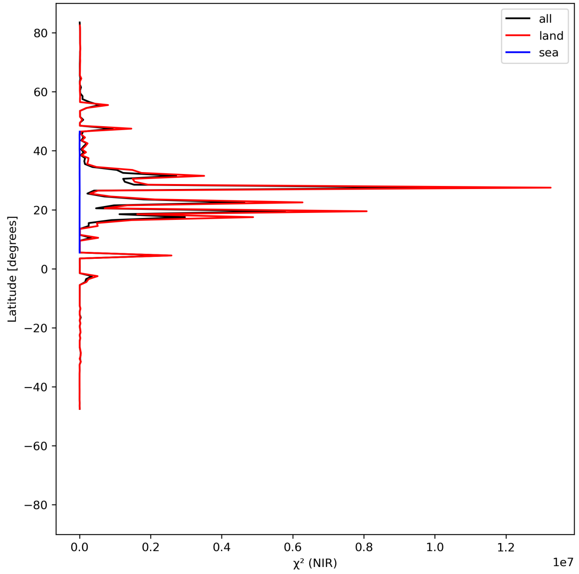
Figure 18: Zonal average of “ \chi^2 (NIR)” for 2024-07-18 to 2024-07-20.
