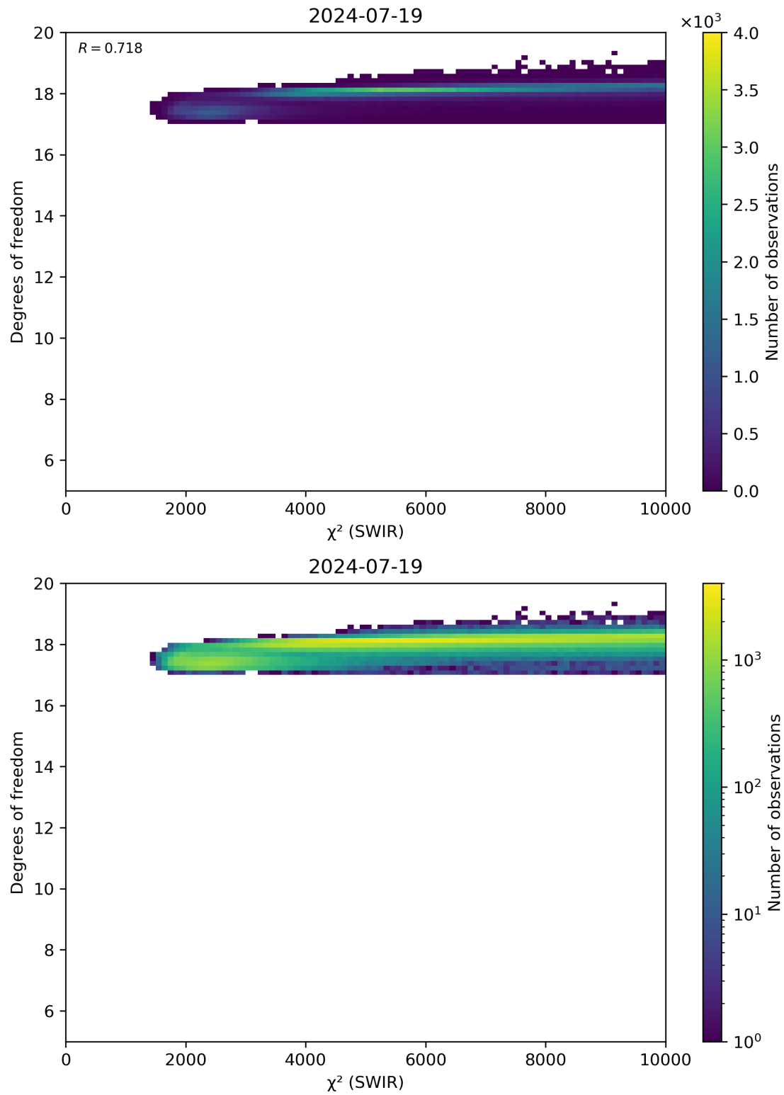
Figure 48: Scatter density plot of “ \chi^2 (SWIR)” against “Degrees of freedom” for 2024-07-18 to 2024-07-20.
