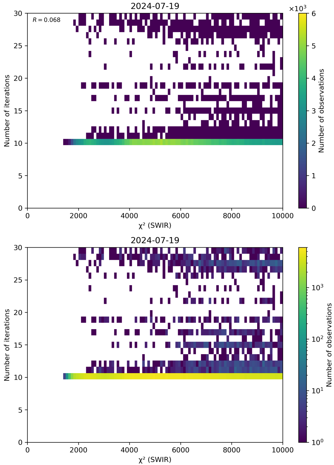
Figure 50: Scatter density plot of “ \chi^2 (SWIR)” against “Number of iterations” for 2024-07-18 to 2024-07-20.
