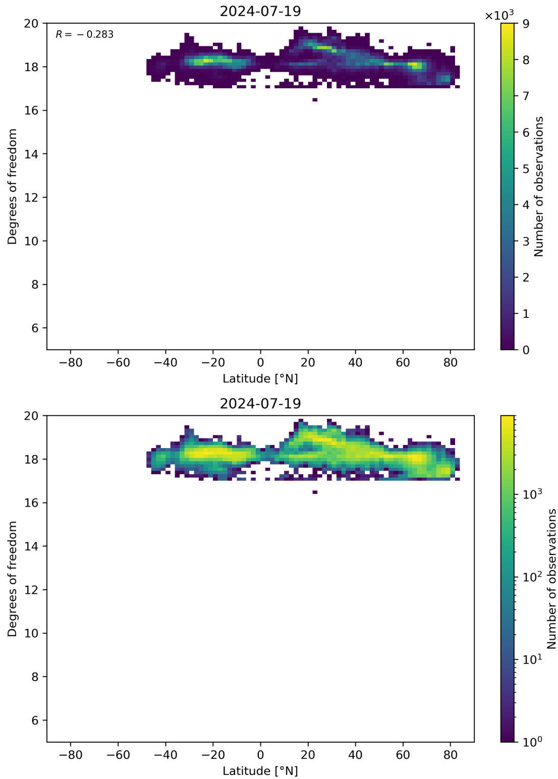
Figure 55: Scatter density plot of “Latitude” against “Degrees of freedom” for 2024-07-18 to 2024-07-20.
