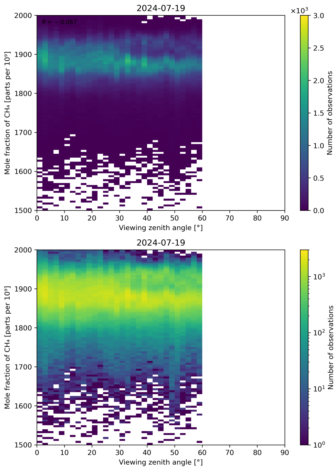
Figure 110: Scatter density plot of “Viewing zenith angle” against “Mole fraction of CH 4 ” for 2024-07-18 to 2024-07-20.
