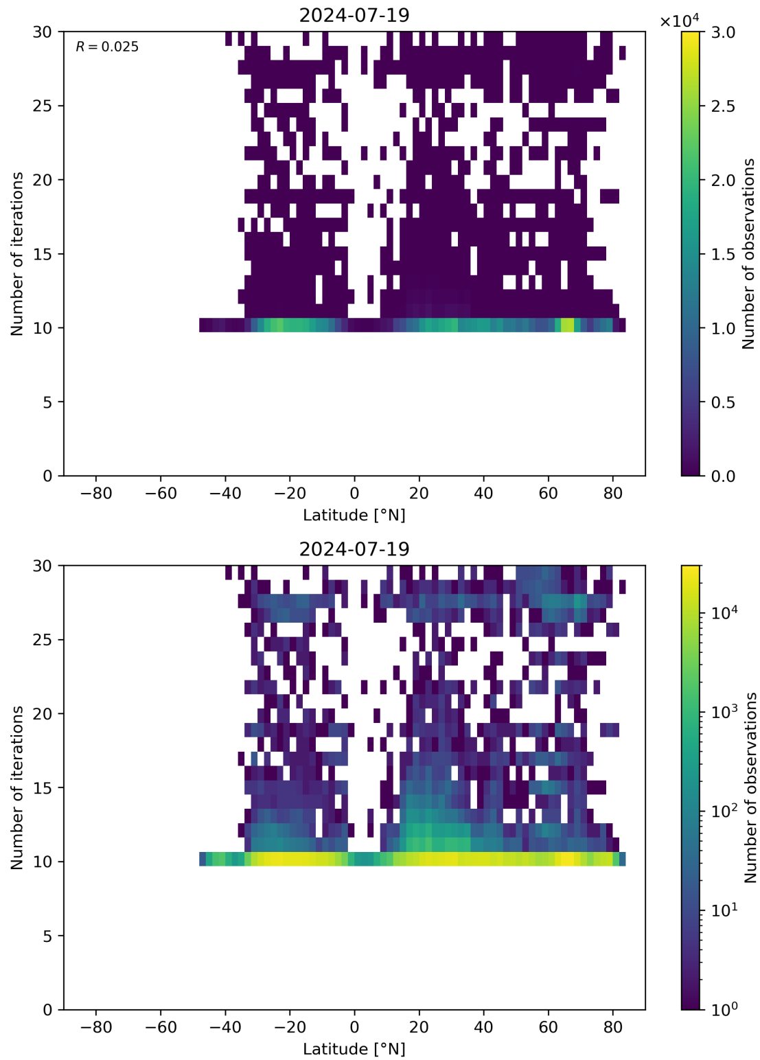
Figure 60: Scatter density plot of “Latitude” against “Number of iterations” for 2024-07-18 to 2024-07-20.
