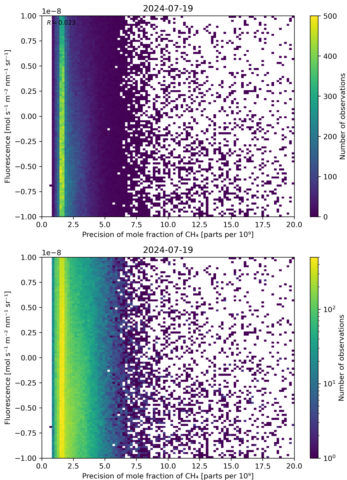
Figure 81: Scatter density plot of “Precision of mole fraction of \text{CH}_4 ” against “Fluorescence” for 2024-07-18 to 2024-07-20.
