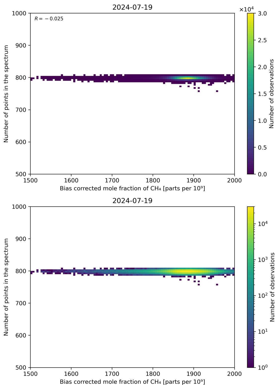
Figure 68: Scatter density plot of “Bias corrected mole fraction of CH 4 ” against “Number of points in the spectrum” for 2024-07-18 to 2024-07-20.
