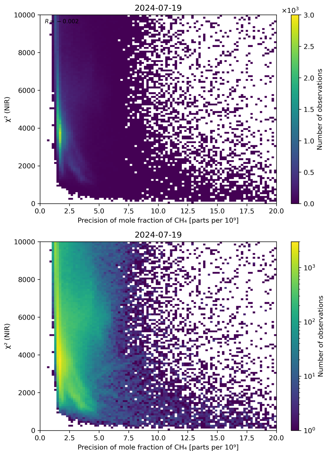
Figure 78: Scatter density plot of “Precision of mole fraction of CH 4 ” against “ \chi^2 (NIR)” for 2024-07-18 to 2024-07-20.
