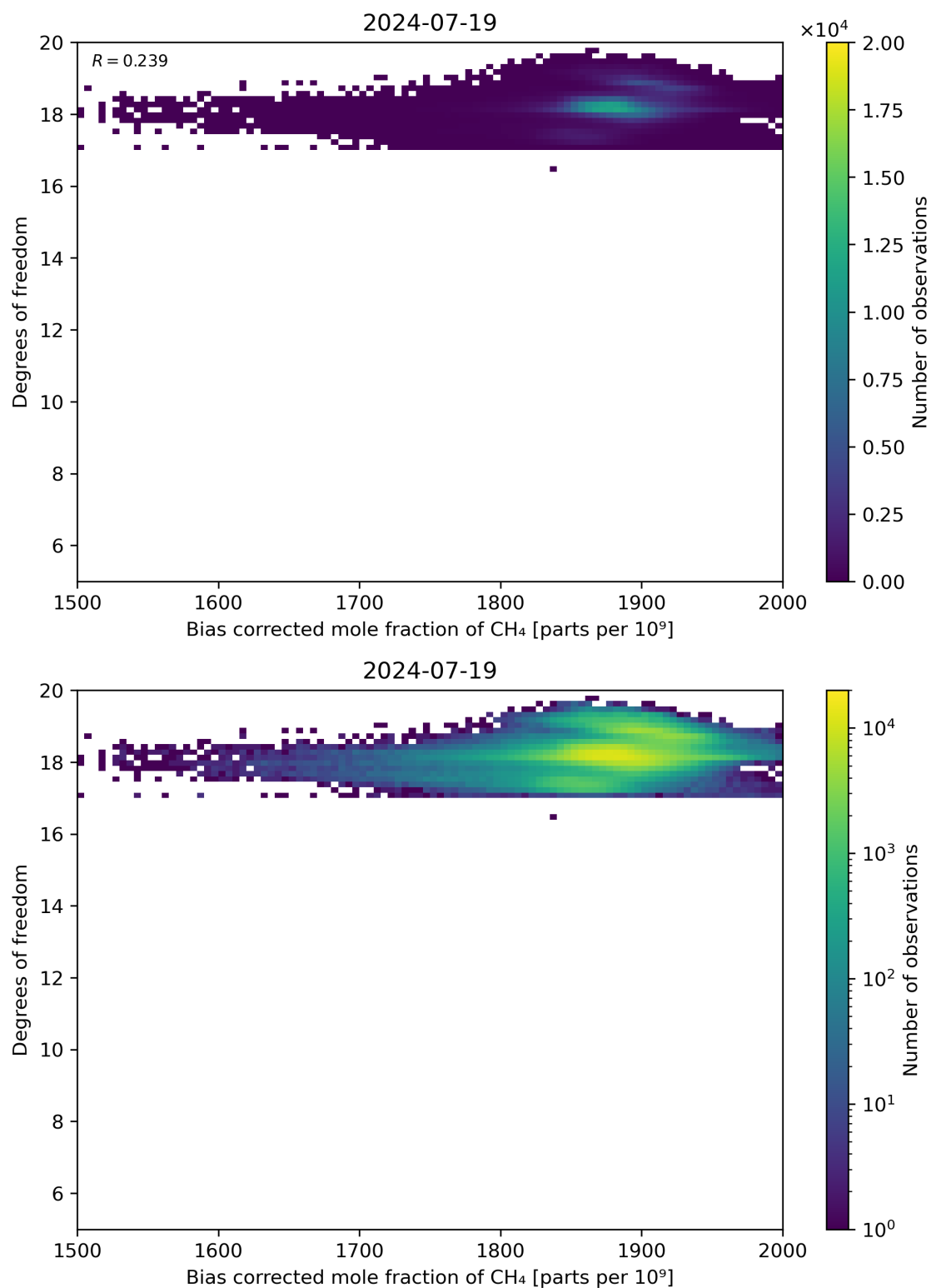
Figure 65: Scatter density plot of “Bias corrected mole fraction of CH 4 ” against “Degrees of freedom” for 2024-07-18 to 2024-07-20.
