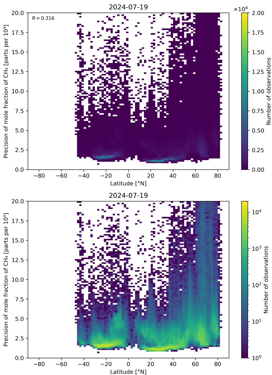
Figure 59: Scatter density plot of “Latitude” against “Precision of mole fraction of \text{CH}_4 ” for 2024-07-18 to 2024-07-20.
