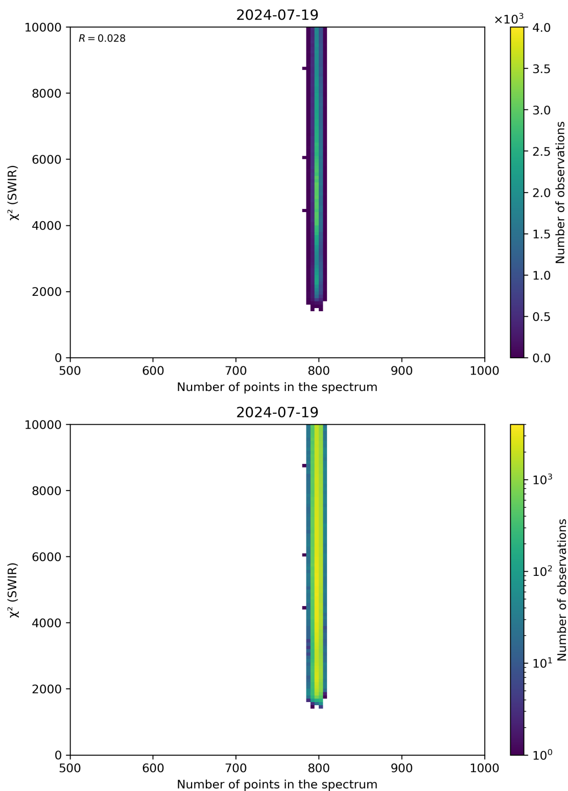
Figure 89: Scatter density plot of “Number of points in the spectrum” against “ \chi^2 (SWIR)” for 2024-07-18 to 2024-07-20.
