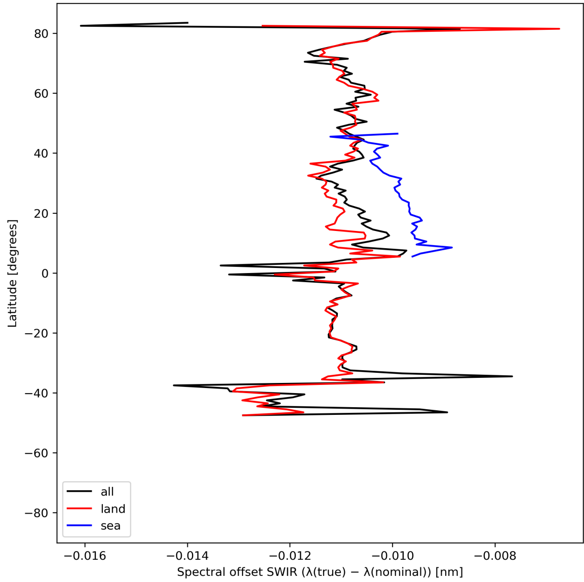
Figure 16: Zonal average of “Spectral offset SWIR ( \lambda(\text{true}) - \lambda(\text{nominal}) )” for 2024-07-18 to 2024-07-20.
