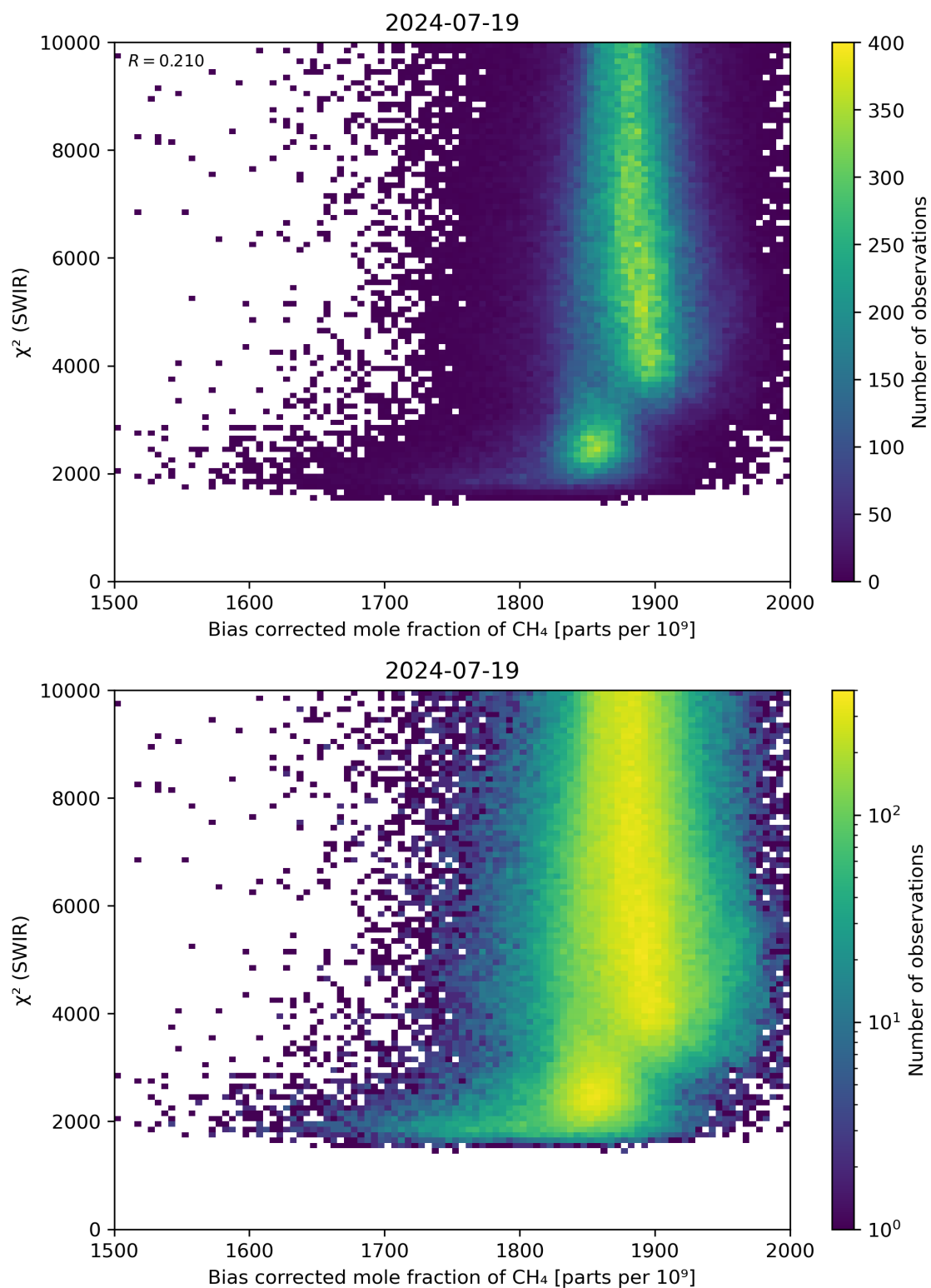
Figure 64: Scatter density plot of “Bias corrected mole fraction of \text{CH}_4 ” against “ \chi^2 (SWIR)” for 2024-07-18 to 2024-07-20.
