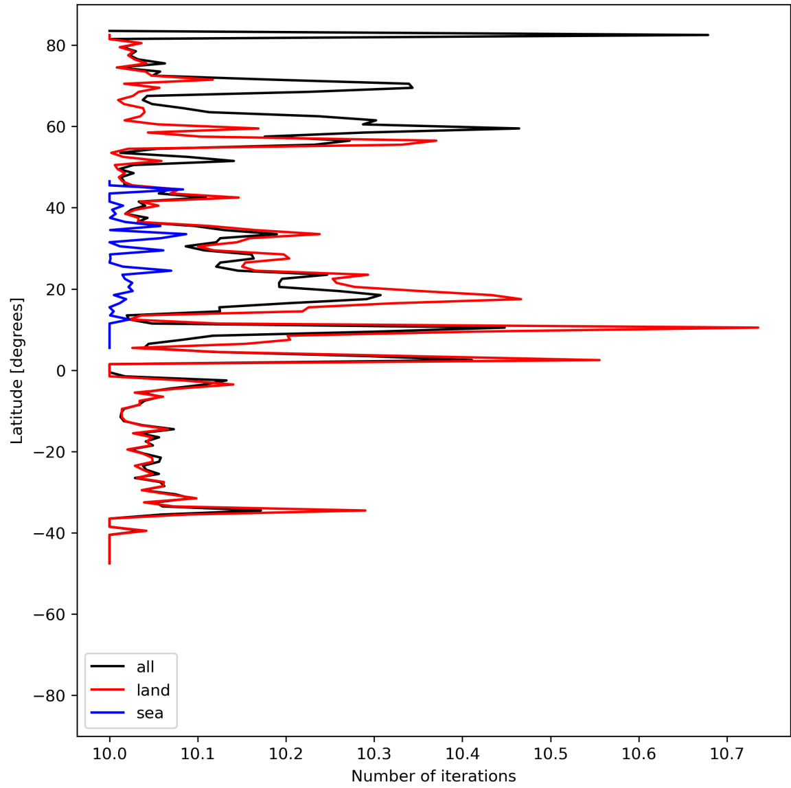
Figure 20: Zonal average of “Number of iterations” for 2024-07-18 to 2024-07-20.
