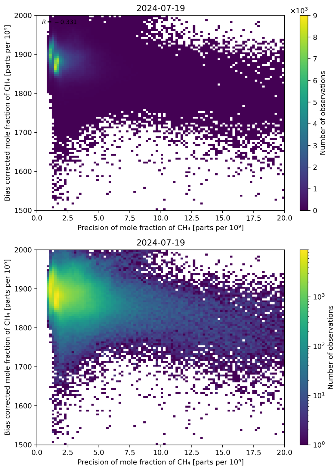
Figure 82: Scatter density plot of “Precision of mole fraction of CH 4 ” against “Bias corrected mole fraction of CH 4 ” for 2024-07-18 to 2024-07-20.
