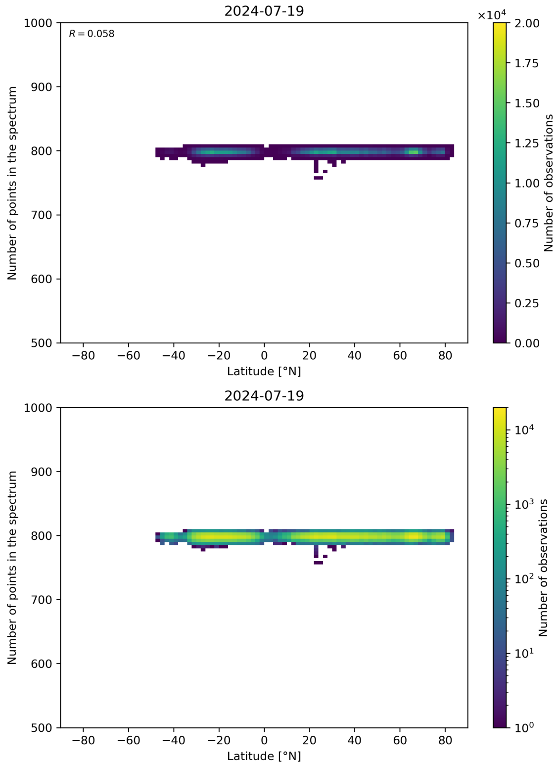
Figure 61: Scatter density plot of “Latitude” against “Number of points in the spectrum” for 2024-07-18 to 2024-07-20.
