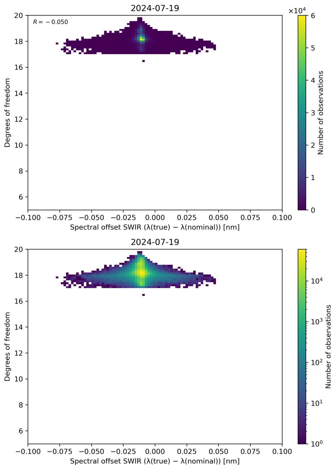
Figure 119: Scatter density plot of “Spectral offset SWIR ( \lambda(\text{true}) - \lambda(\text{nominal}) )” against “Degrees of freedom” for 2024-07-18 to 2024-07-20.
