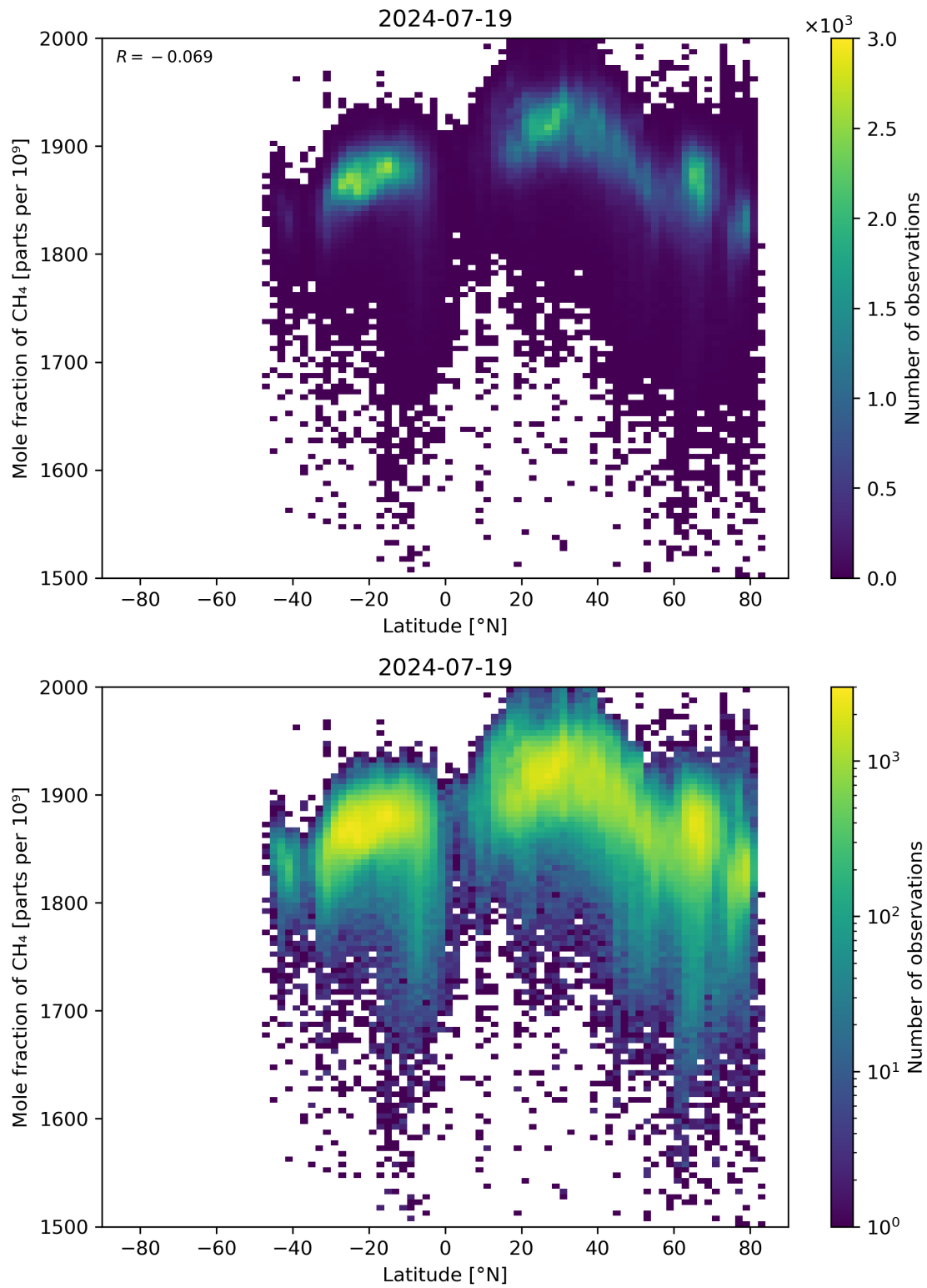
Figure 57: Scatter density plot of “Latitude” against “Mole fraction of CH 4 ” for 2024-07-18 to 2024-07-20.
