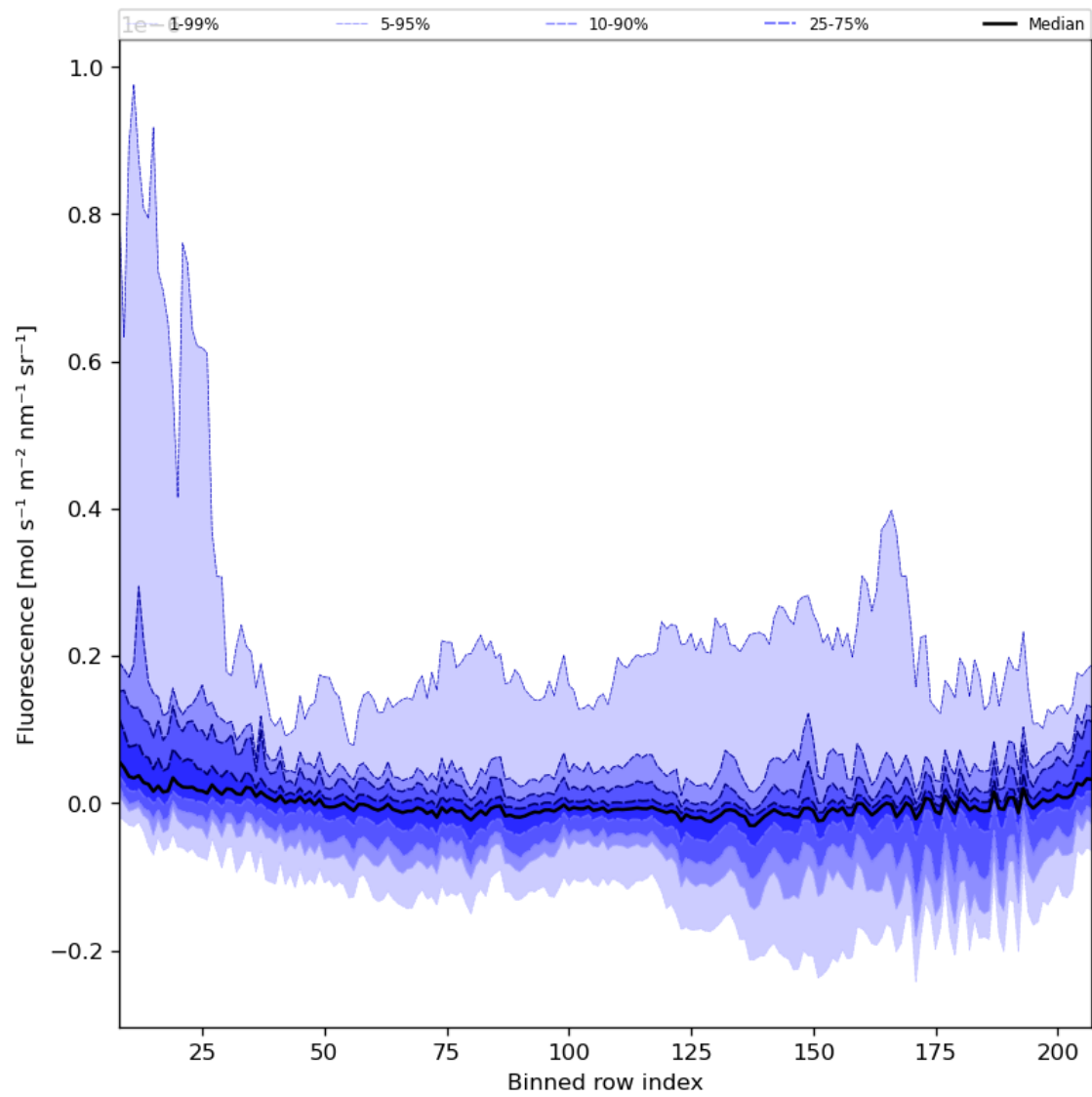
Figure 43: Along track statistics of “Fluorescence” for 2024-07-18 to 2024-07-20
