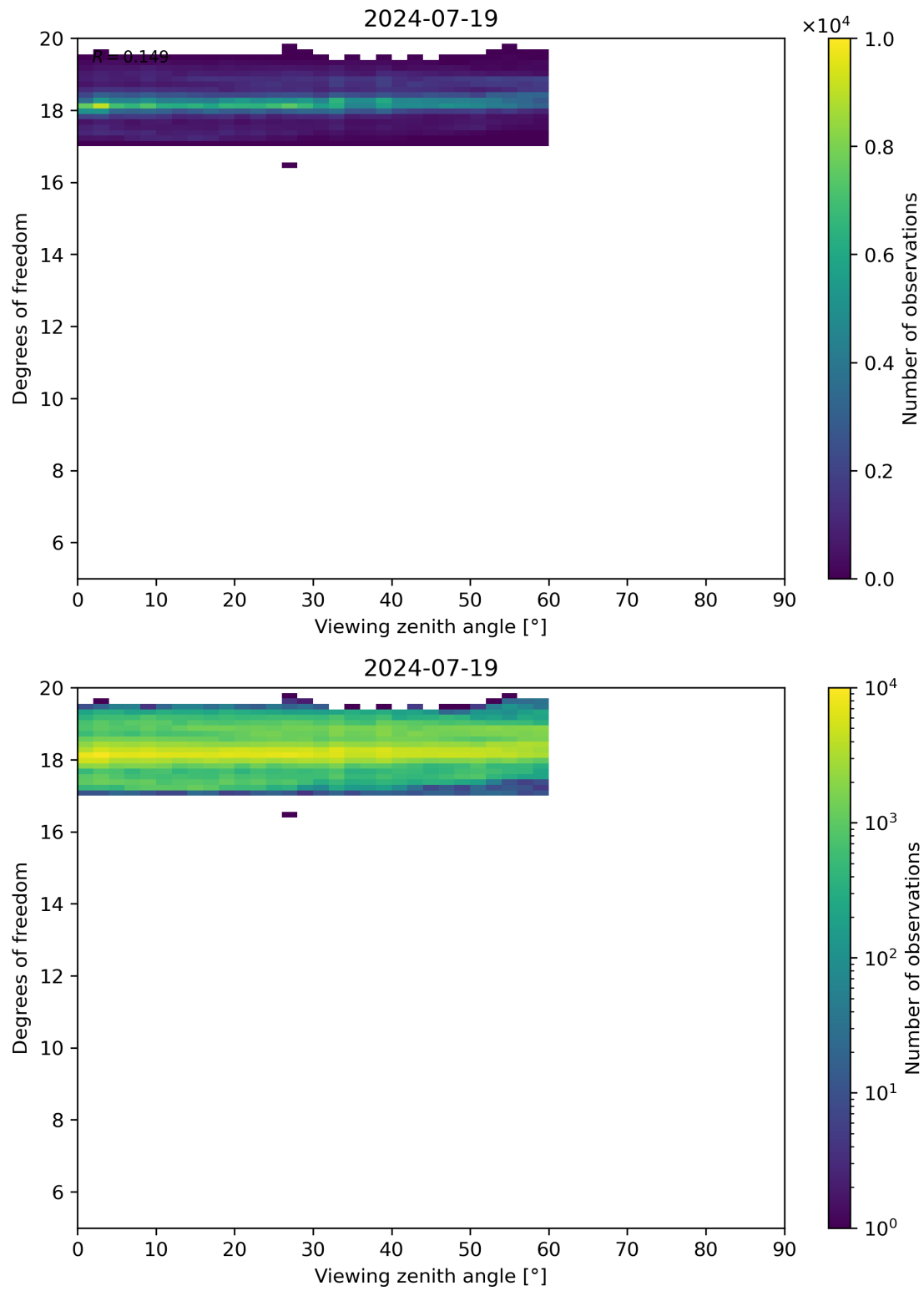
Figure 107: Scatter density plot of “Viewing zenith angle” against “Degrees of freedom” for 2024-07-18 to 2024-07-20.
