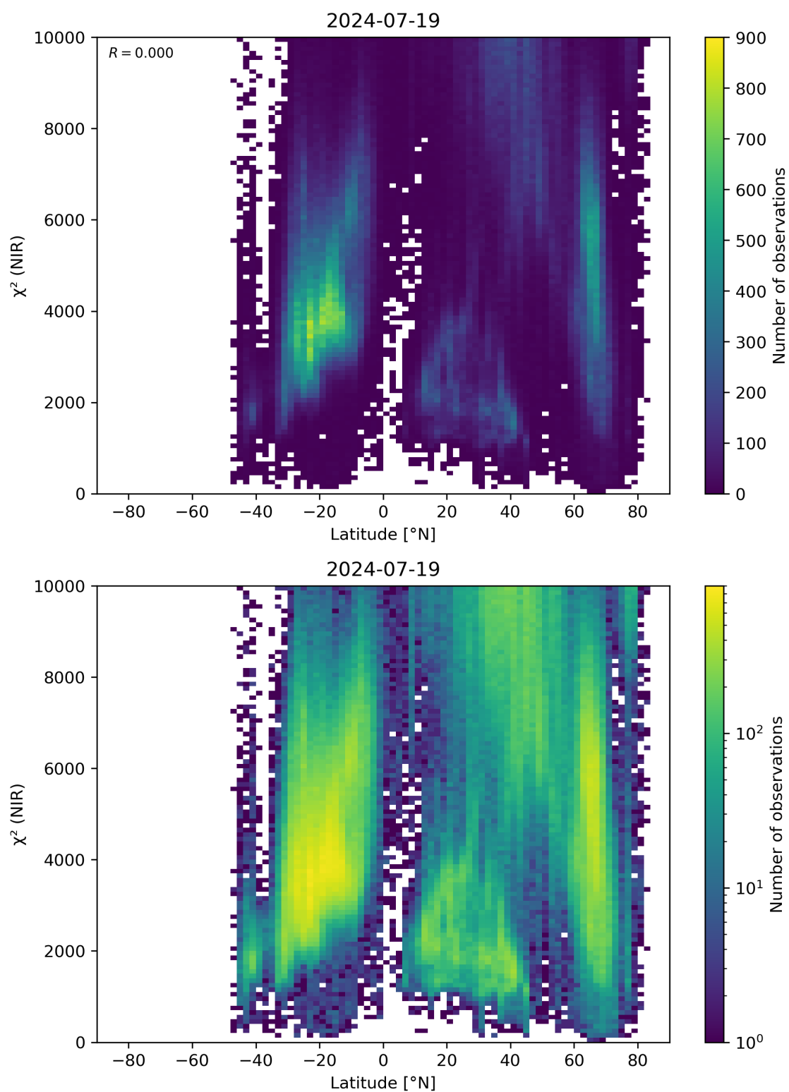
Figure 53: Scatter density plot of “Latitude” against “ \chi^2 (NIR)” for 2024-07-18 to 2024-07-20.
