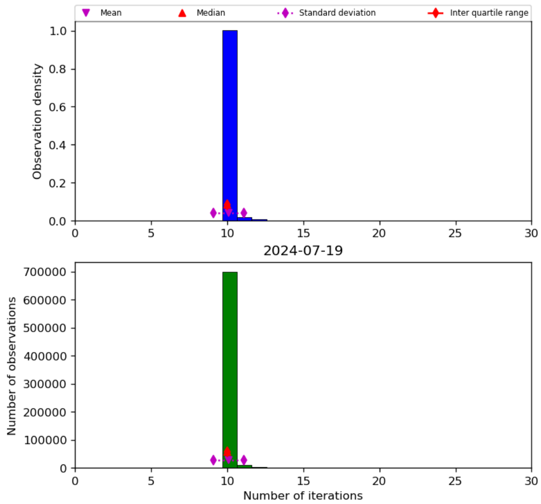
Figure 31: Histogram of “Number of iterations” for 2024-07-18 to 2024-07-20
