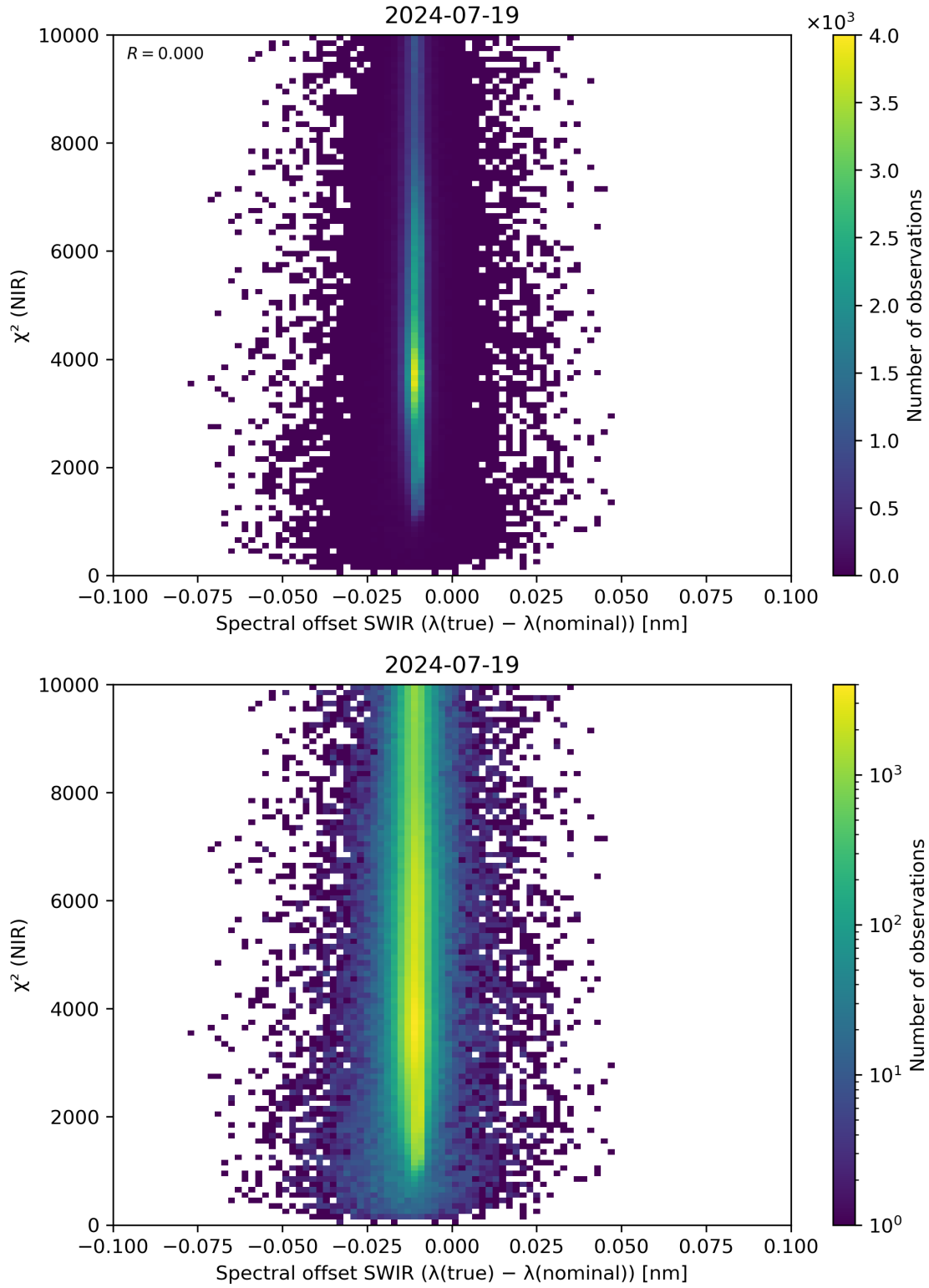
Figure 117: Scatter density plot of “Spectral offset SWIR ( \lambda(\text{true}) - \lambda(\text{nominal}) )” against “ \chi^2 (NIR)” for 2024-07-18 to 2024-07-20.
