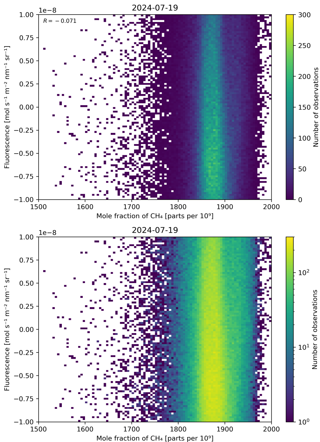
Figure 73: Scatter density plot of “Mole fraction of \text{CH}_4 ” against “Fluorescence” for 2024-07-18 to 2024-07-20.
