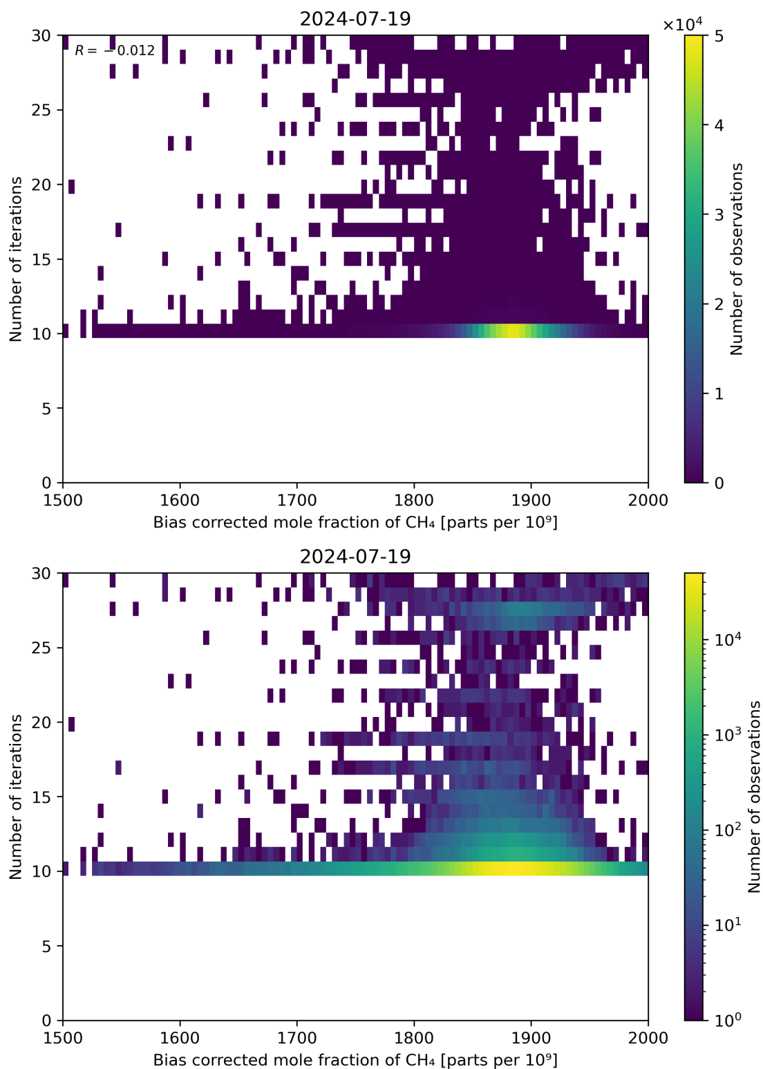
Figure 67: Scatter density plot of “Bias corrected mole fraction of CH 4 ” against “Number of iterations” for 2024-07-18 to 2024-07-20.
