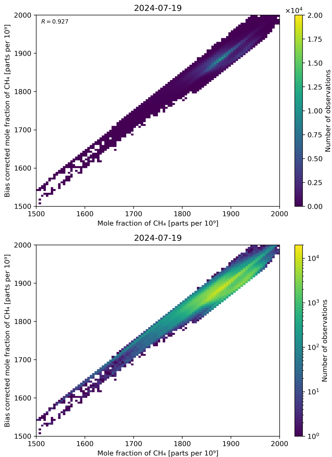
Figure 74: Scatter density plot of “Mole fraction of CH 4 ” against “Bias corrected mole fraction of CH 4 ” for 2024-07-18 to 2024-07-20.
