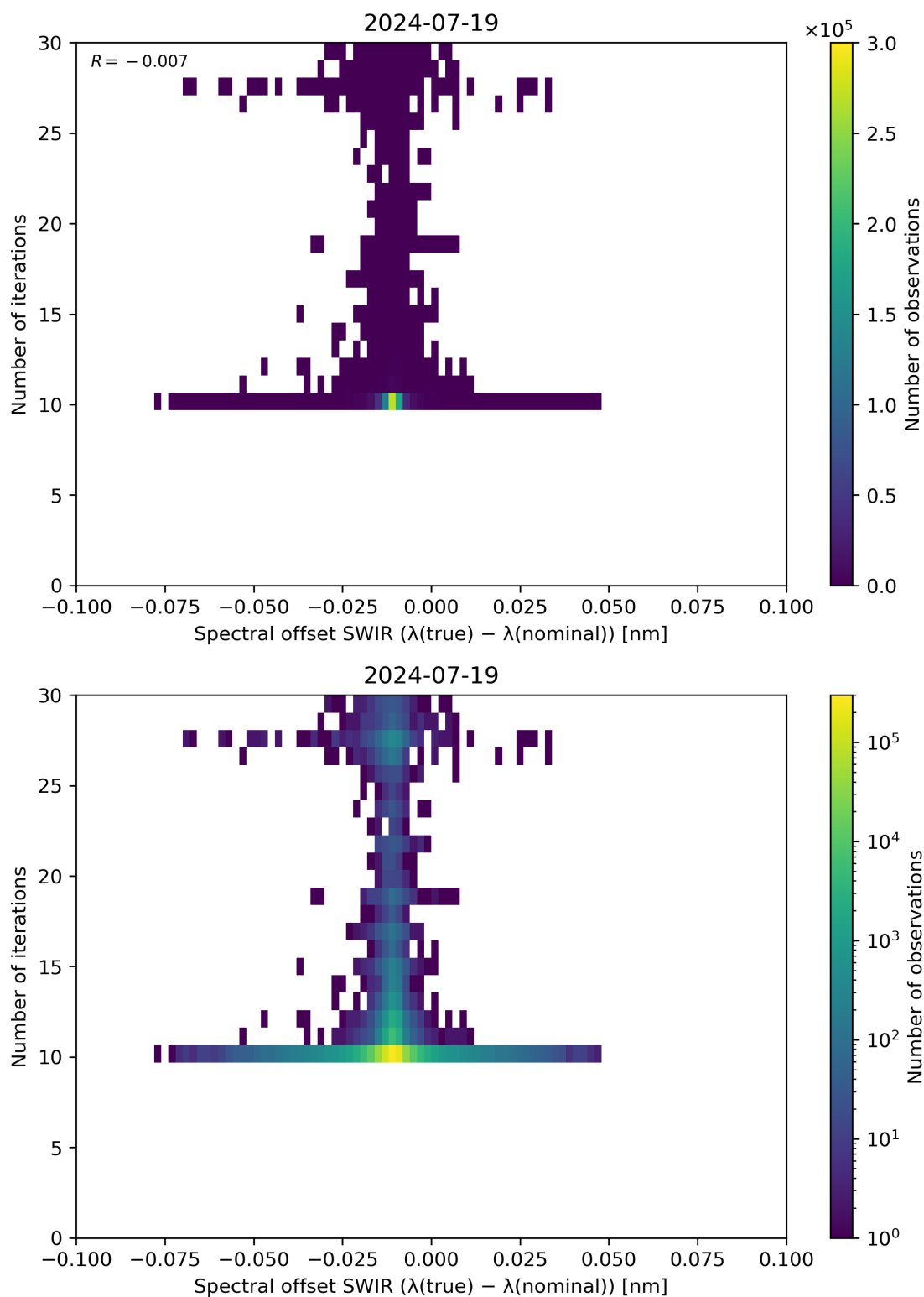
Figure 121: Scatter density plot of “Spectral offset SWIR ( \lambda(\text{true}) - \lambda(\text{nominal}) )” against “Number of iterations” for 2024-07-18 to 2024-07-20.
