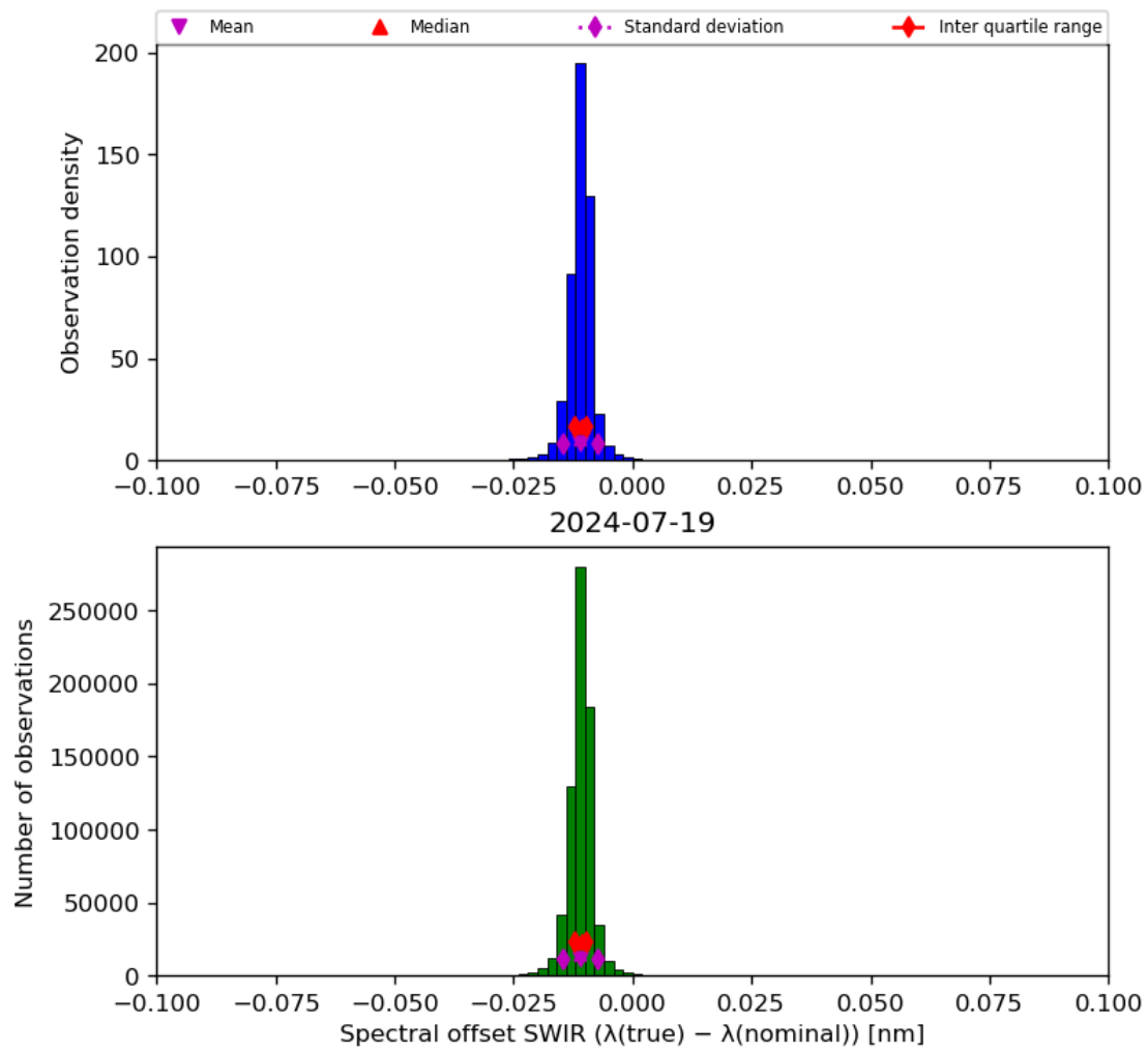
Figure 27: Histogram of “Spectral offset SWIR ( \lambda(\text{true}) - \lambda(\text{nominal}) )” for 2024-07-18 to 2024-07-20
