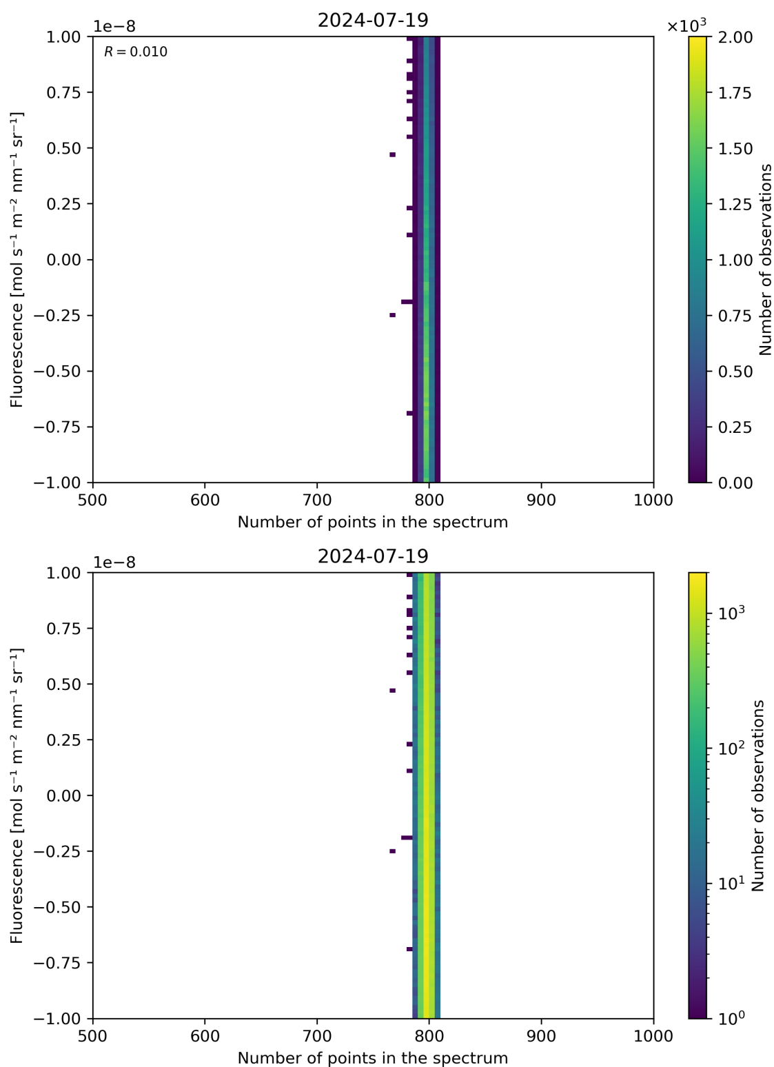
Figure 91: Scatter density plot of “Number of points in the spectrum” against “Fluorescence” for 2024-07-18 to 2024-07-20.
