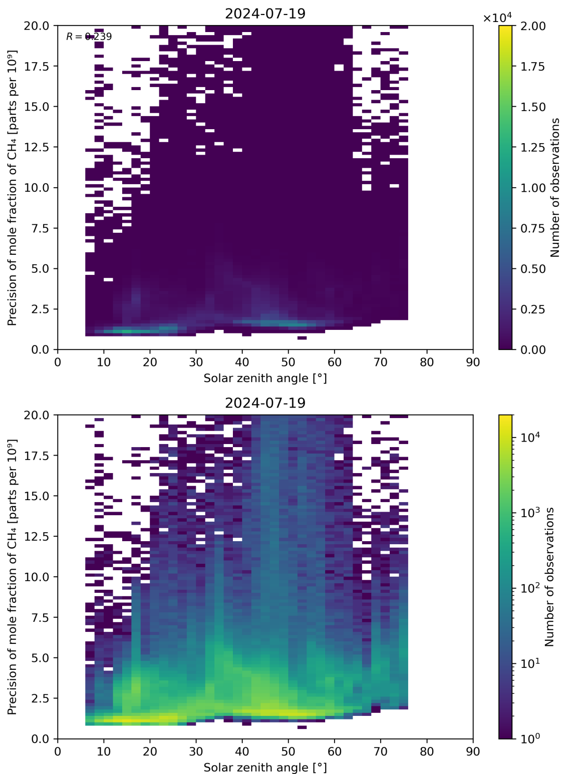
Figure 101: Scatter density plot of “Solar zenith angle” against “Precision of mole fraction of CH 4 ” for 2024-07-18 to 2024-07-20.
