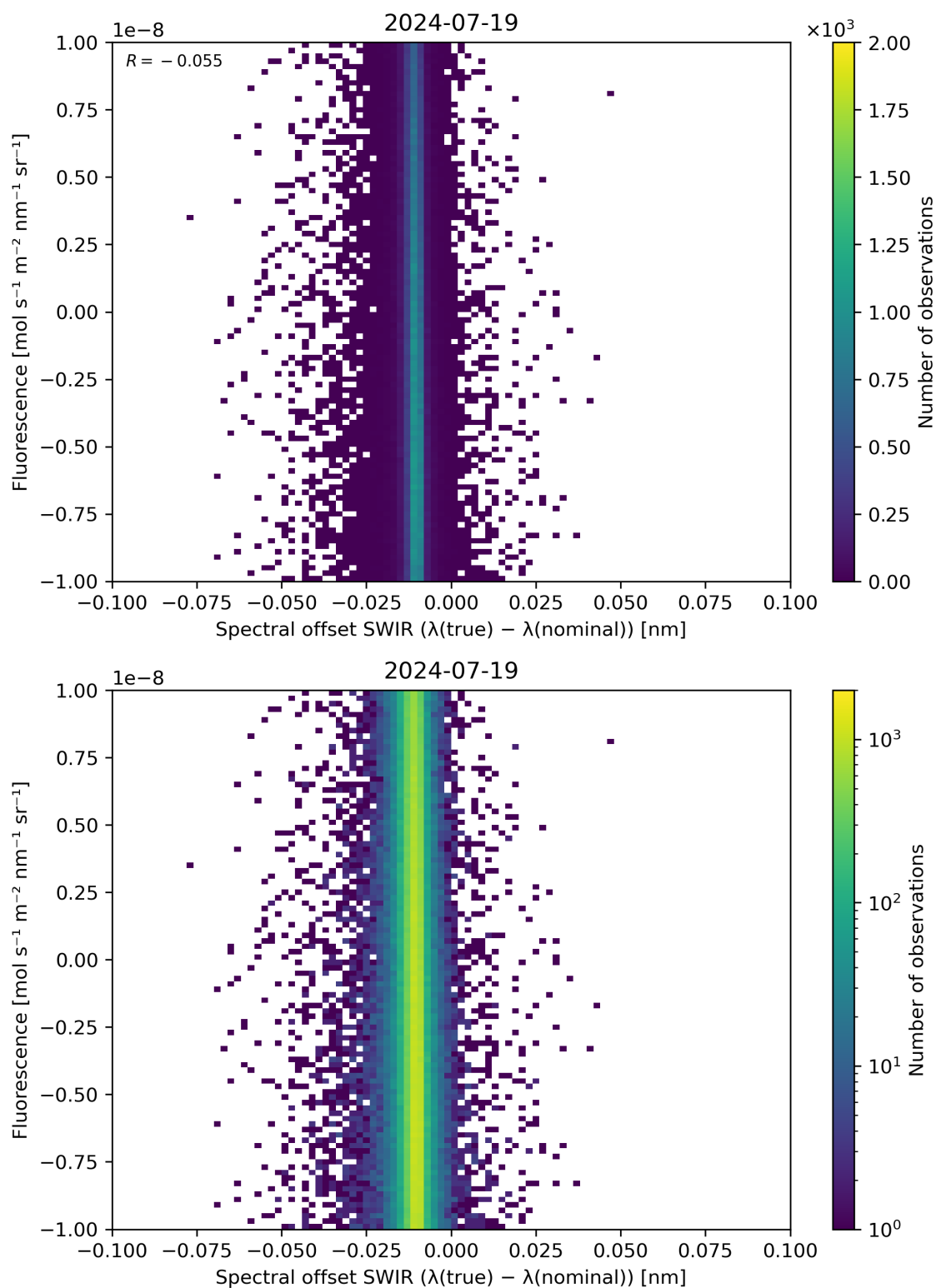
Figure 120: Scatter density plot of “Spectral offset SWIR ( \lambda(\text{true}) - \lambda(\text{nominal}) )” against “Fluorescence” for 2024-07-18 to 2024-07-20.
