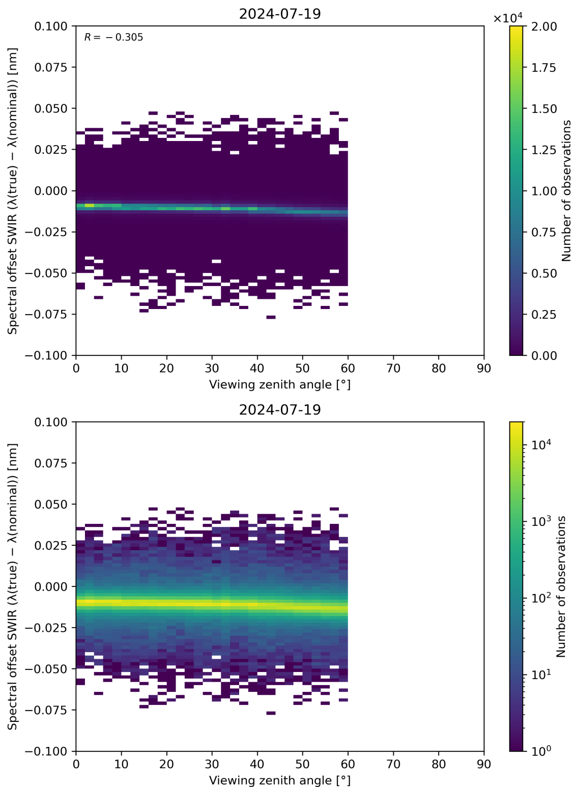
Figure 116: Scatter density plot of “Viewing zenith angle” against “Spectral offset SWIR ( \lambda(\text{true}) - \lambda(\text{nominal}) )” for 2024-07-18 to 2024-07-20.
