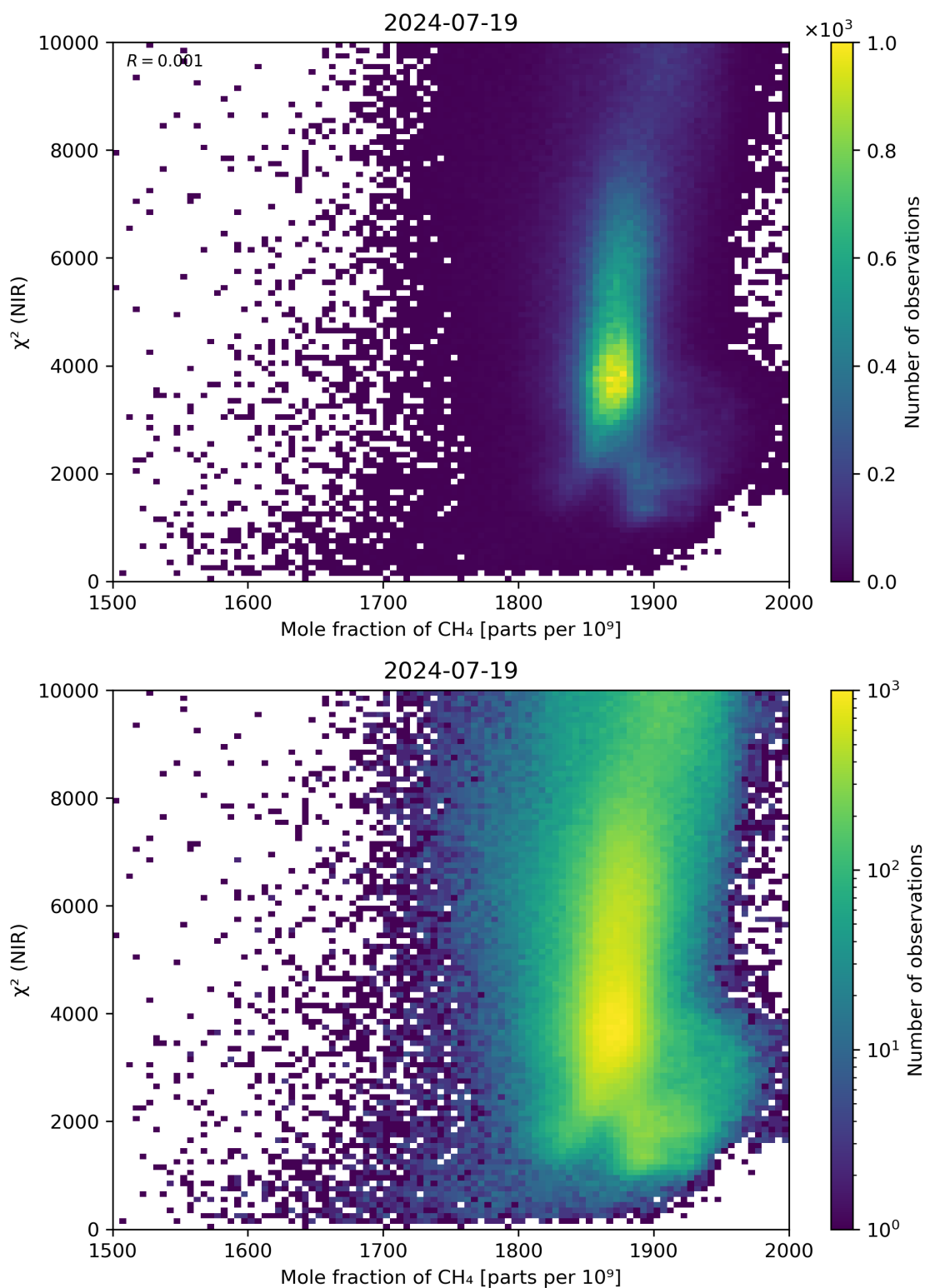
Figure 70: Scatter density plot of “Mole fraction of \text{CH}_4 ” against “ \chi^2 (NIR)” for 2024-07-18 to 2024-07-20.
