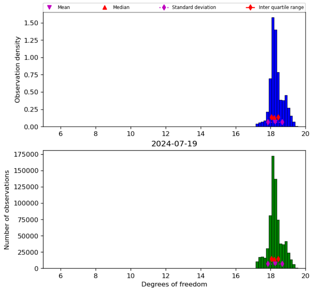
Figure 30: Histogram of “Degrees of freedom” for 2024-07-18 to 2024-07-20
