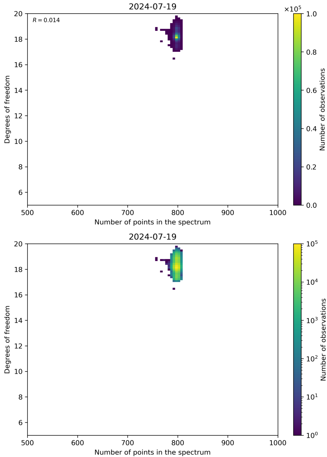
Figure 90: Scatter density plot of “Number of points in the spectrum” against “Degrees of freedom” for 2024-07-18 to 2024-07-20.
