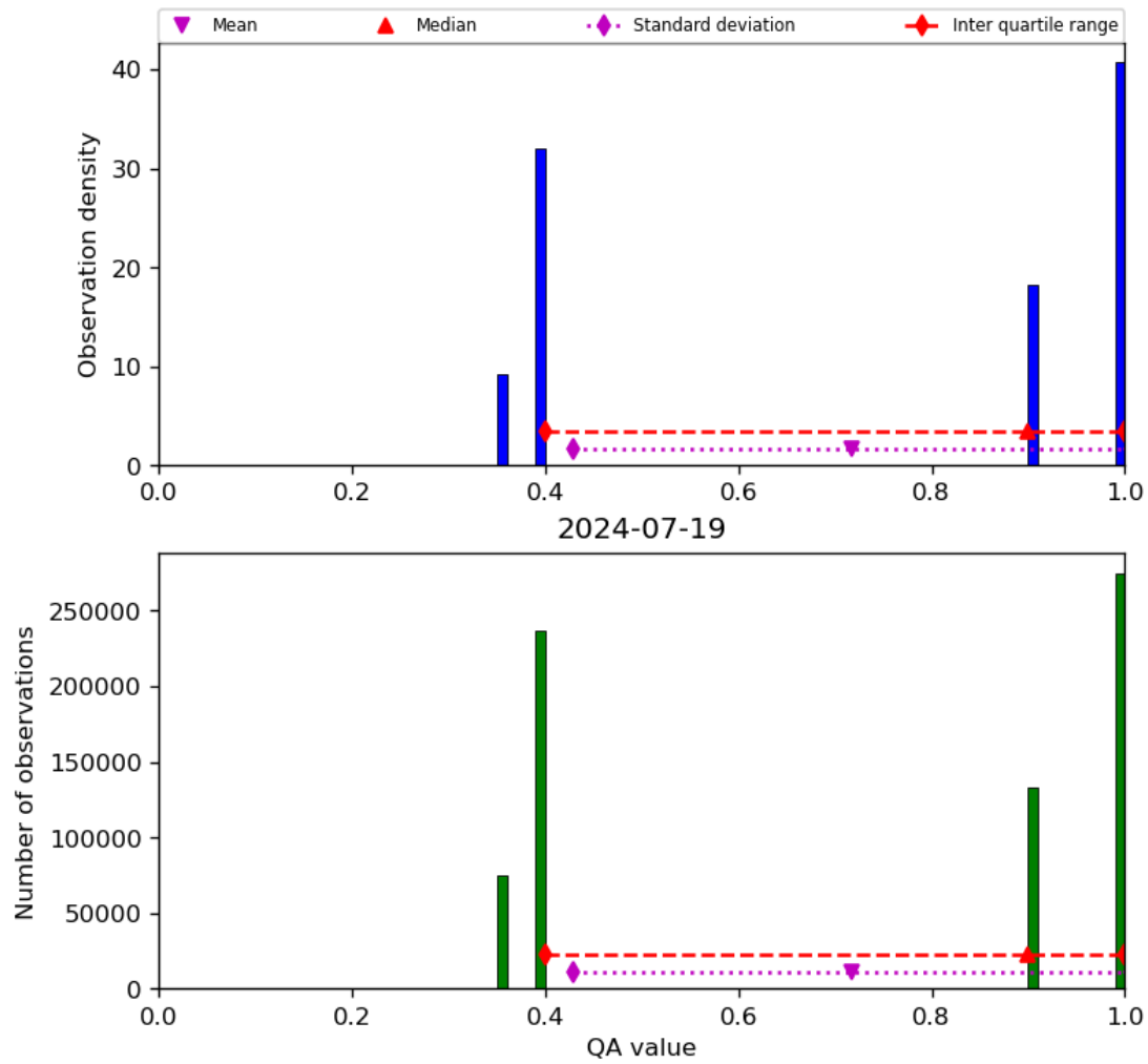
Figure 22: Histogram of “QA value” for 2024-07-18 to 2024-07-20
