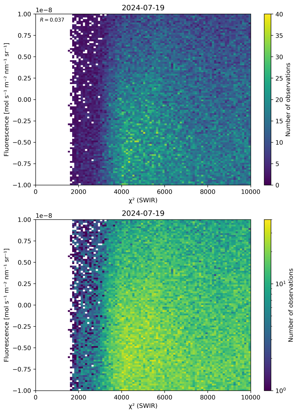
Figure 49: Scatter density plot of “ \chi^2 (SWIR)” against “Fluorescence” for 2024-07-18 to 2024-07-20.
