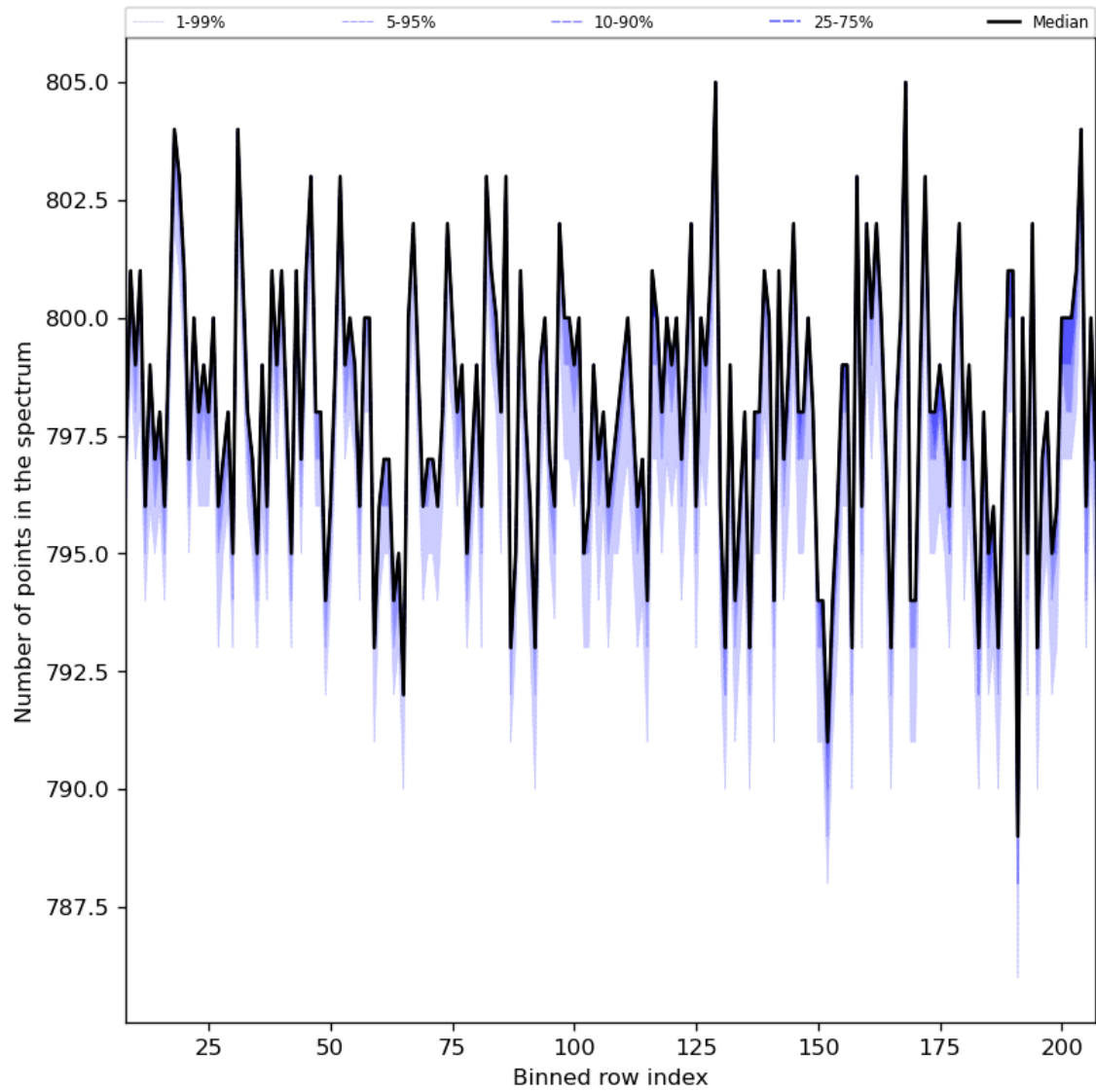
Figure 37: Along track statistics of “Number of points in the spectrum” for 2024-07-18 to 2024-07-20
