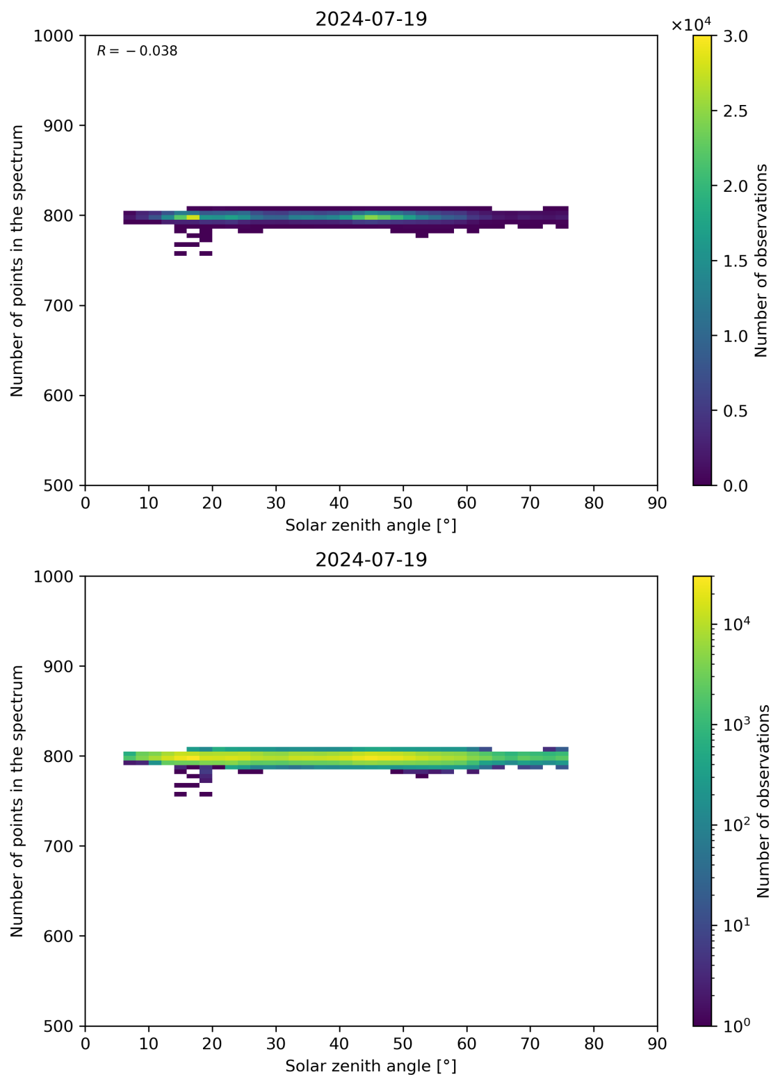
Figure 103: Scatter density plot of “Solar zenith angle” against “Number of points in the spectrum” for 2024-07-18 to 2024-07-20.
