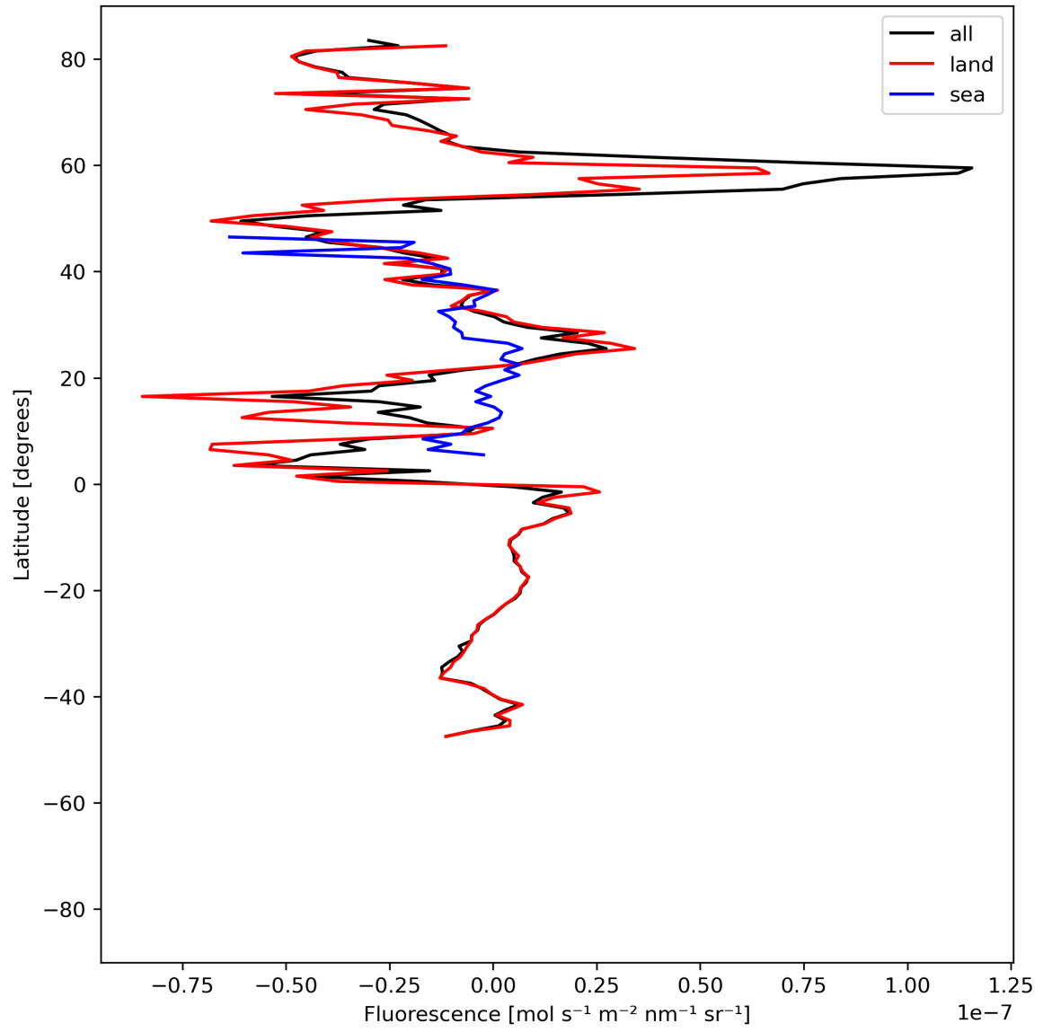
Figure 21: Zonal average of “Fluorescence” for 2024-07-18 to 2024-07-20.
