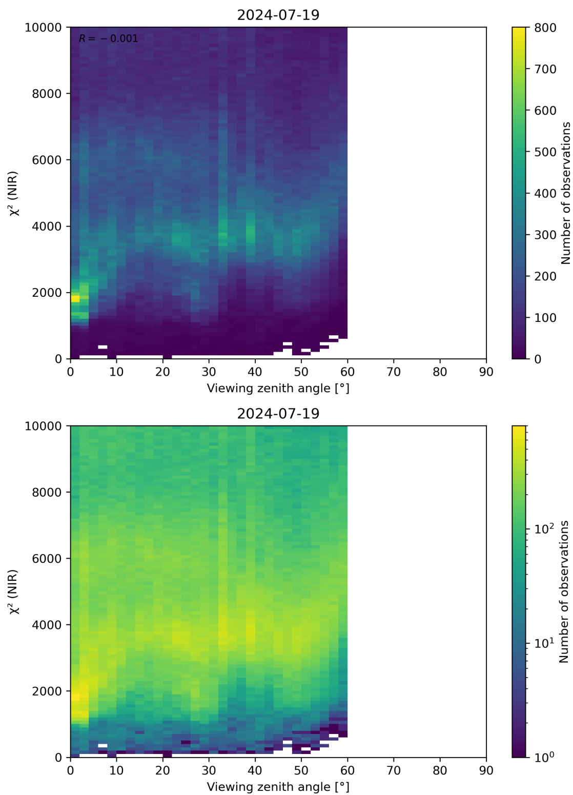
Figure 105: Scatter density plot of “Viewing zenith angle” against “ \chi^2 (NIR)” for 2024-07-18 to 2024-07-20.
