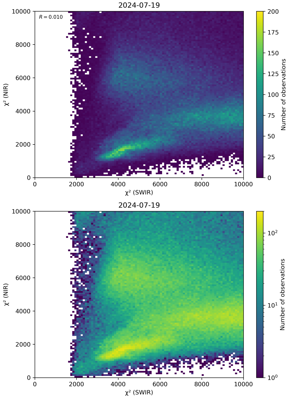
Figure 47: Scatter density plot of “ \chi^2 (SWIR)” against “ \chi^2 (NIR)” for 2024-07-18 to 2024-07-20.
