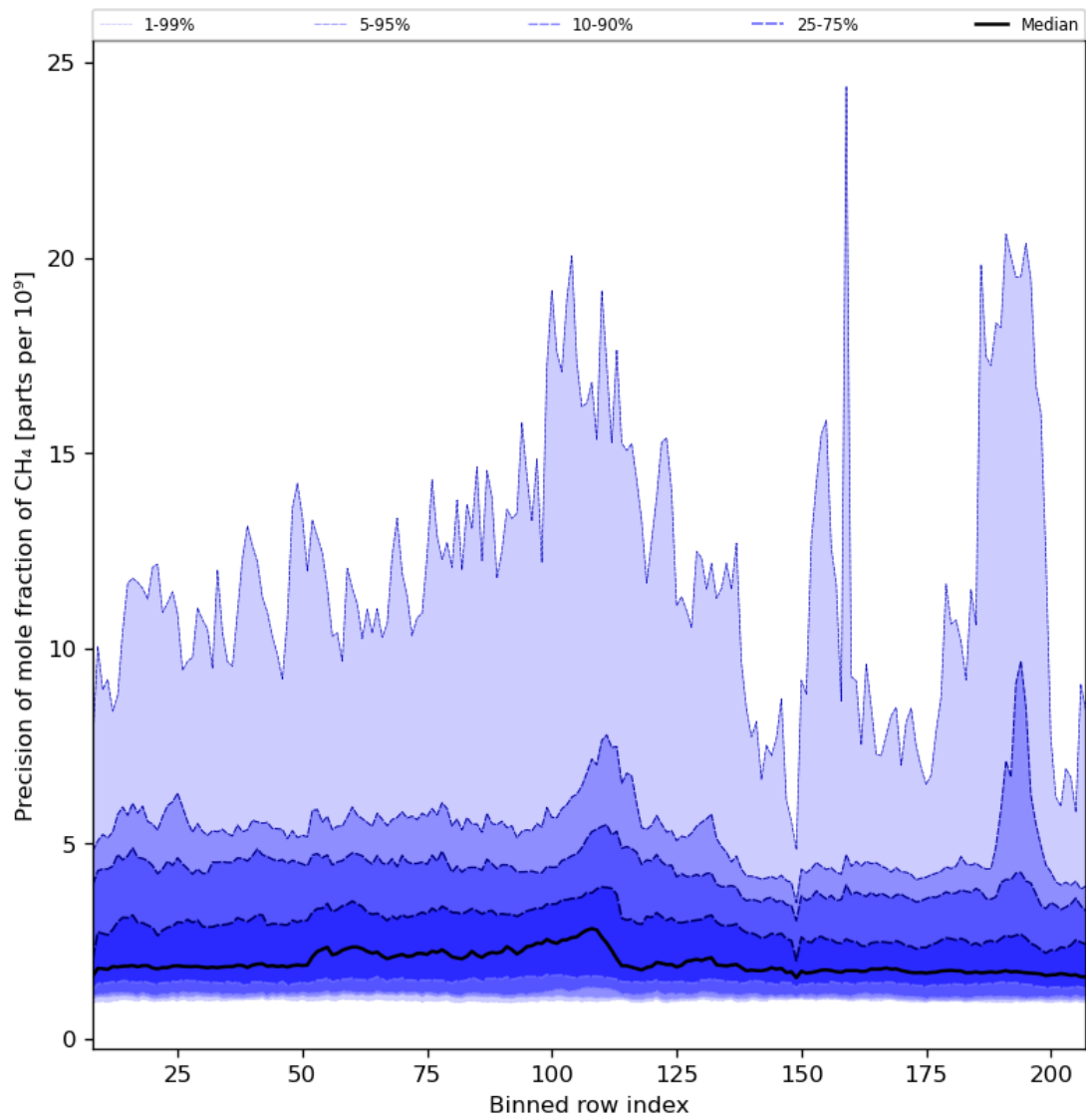
Figure 35: Along track statistics of “Precision of mole fraction of CH 4 ” for 2024-07-18 to 2024-07-20
