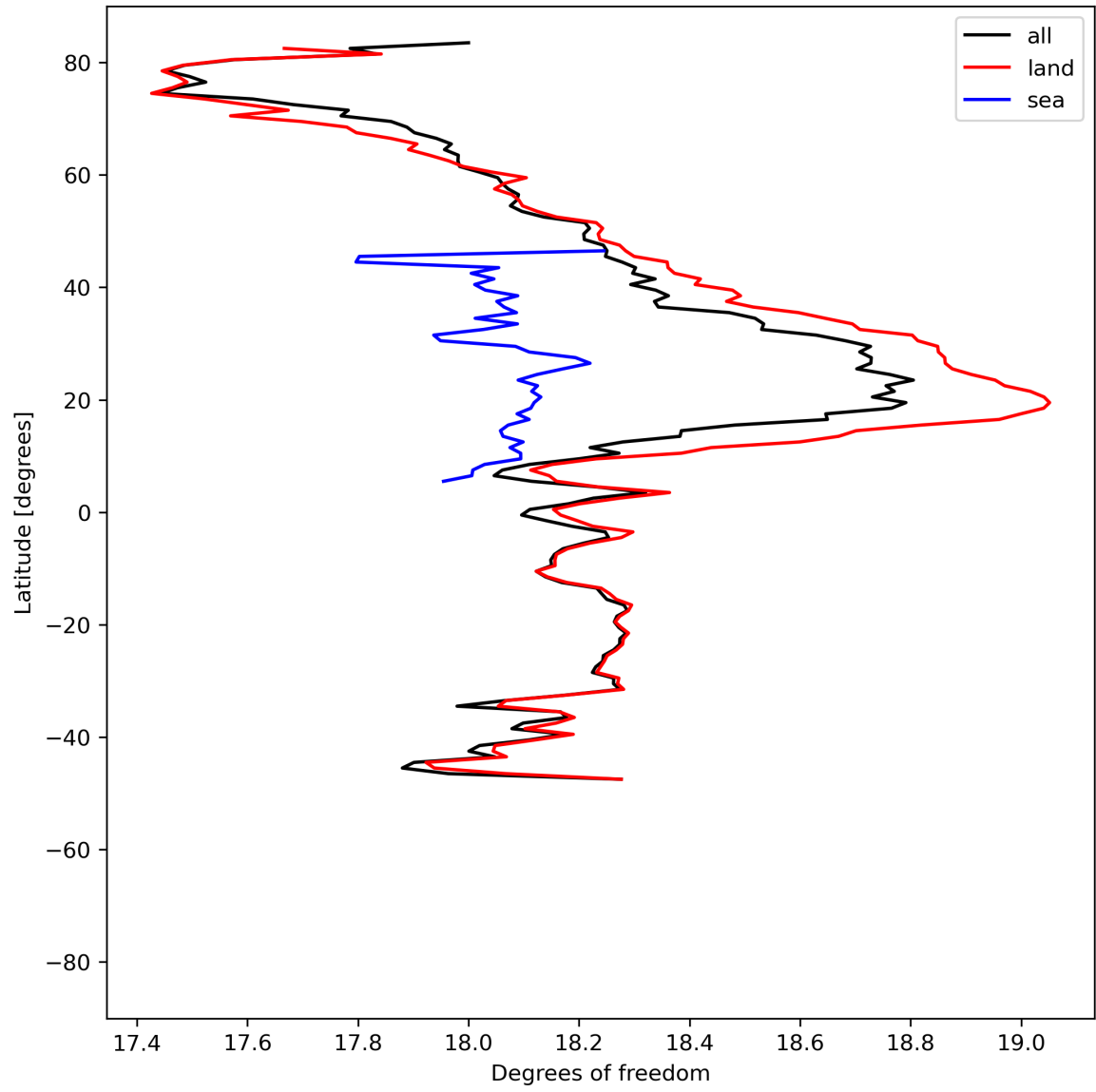
Figure 19: Zonal average of “Degrees of freedom” for 2024-07-18 to 2024-07-20.
