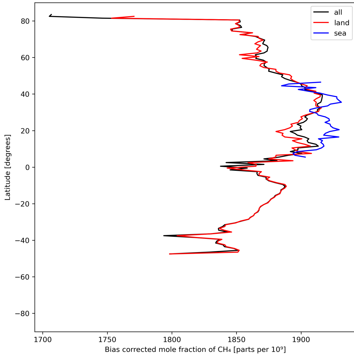
Figure 14: Zonal average of “Bias corrected mole fraction of \text{CH}_4 ” for 2024-07-18 to 2024-07-20.
