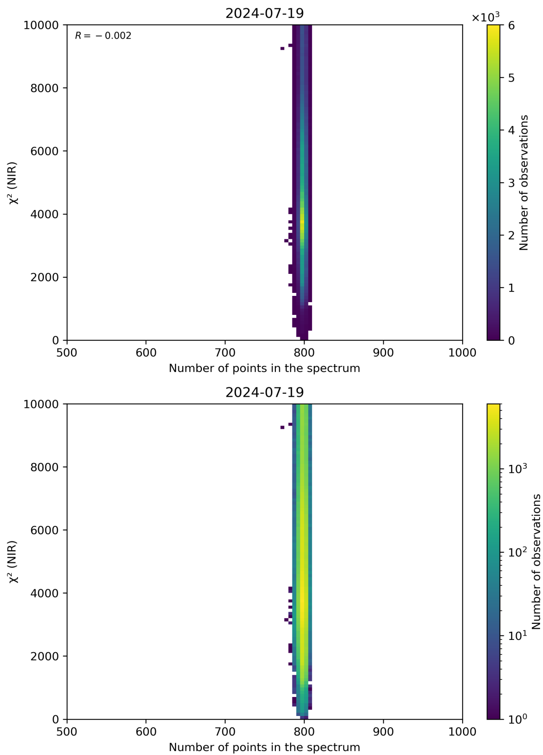
Figure 88: Scatter density plot of “Number of points in the spectrum” against “ \chi^2 (NIR)” for 2024-07-18 to 2024-07-20.
