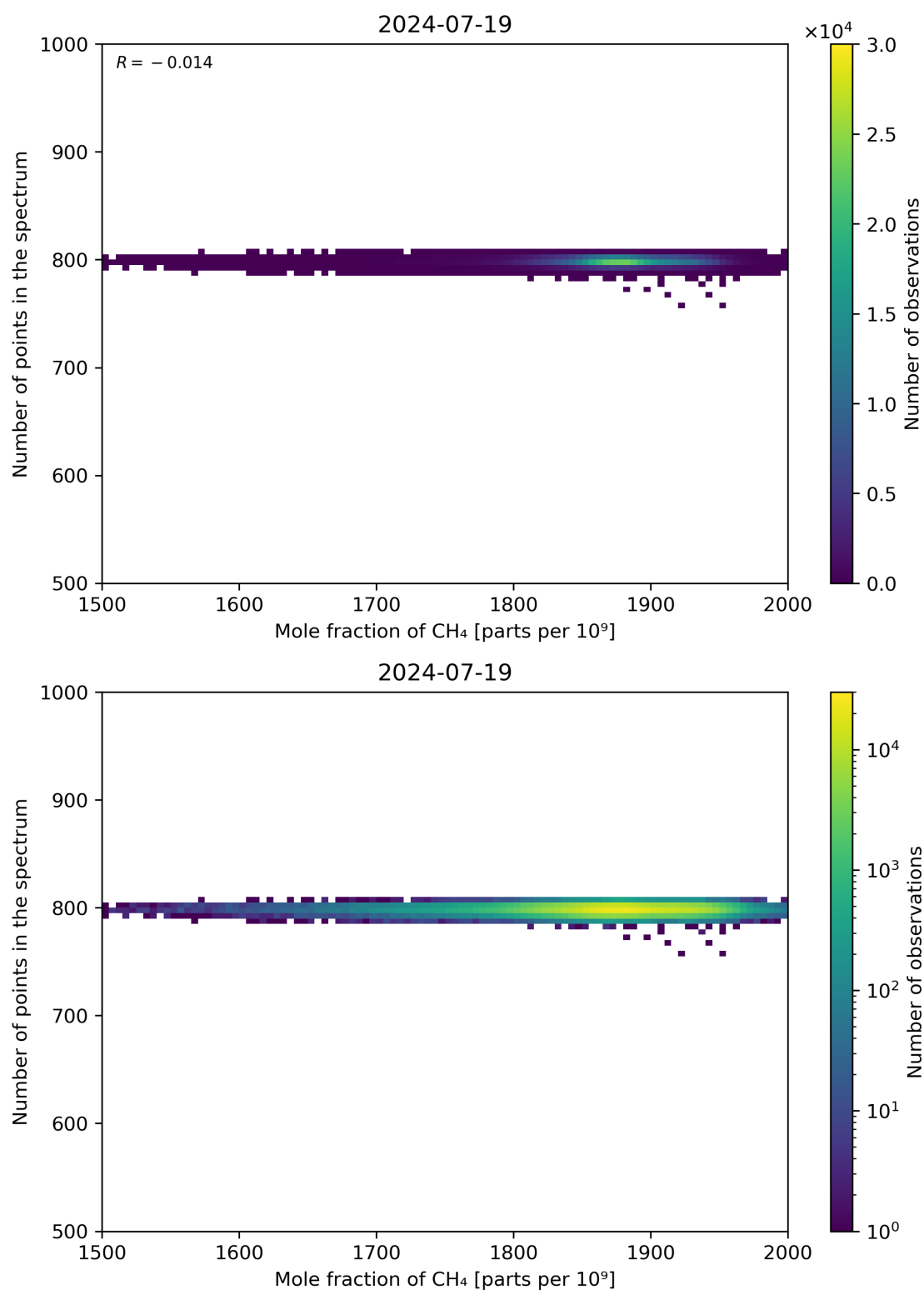
Figure 77: Scatter density plot of “Mole fraction of CH 4 ” against “Number of points in the spectrum” for 2024-07-18 to 2024-07-20.
