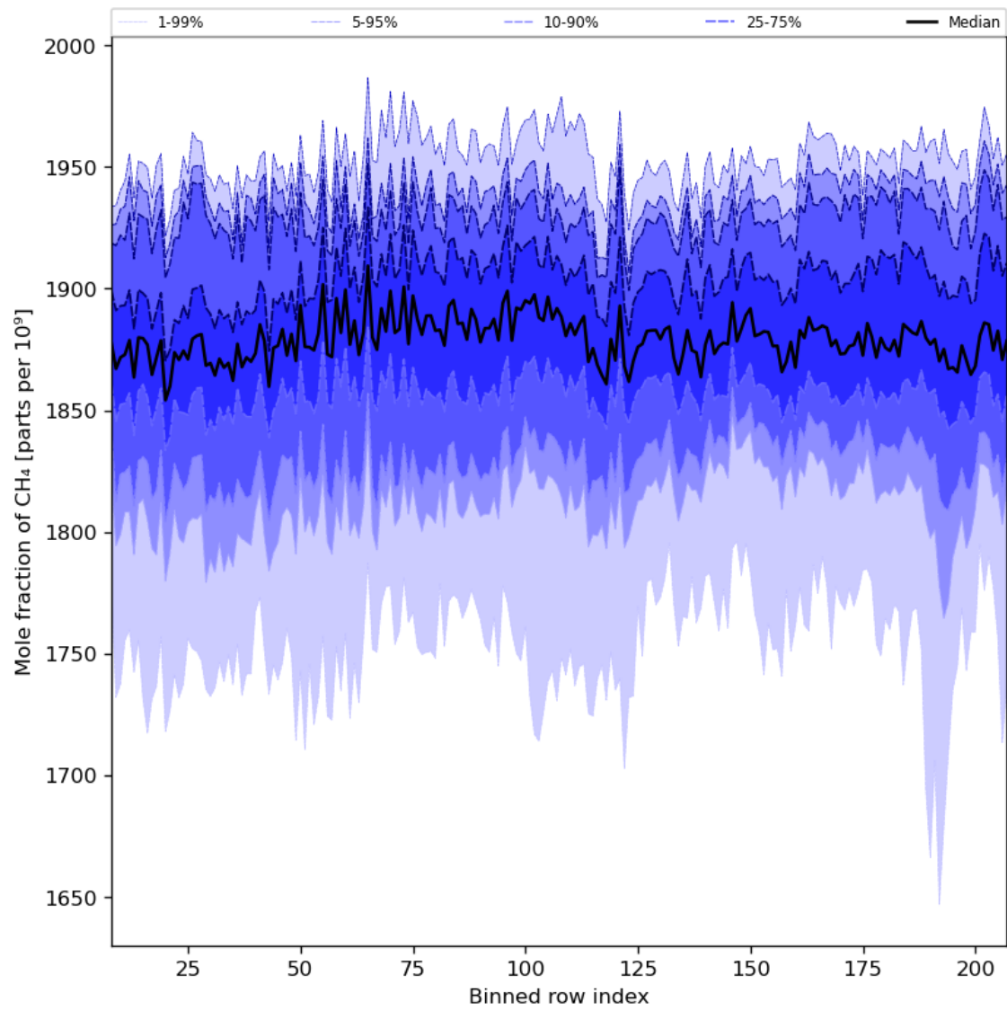
Figure 34: Along track statistics of “Mole fraction of CH 4 ” for 2024-07-18 to 2024-07-20
