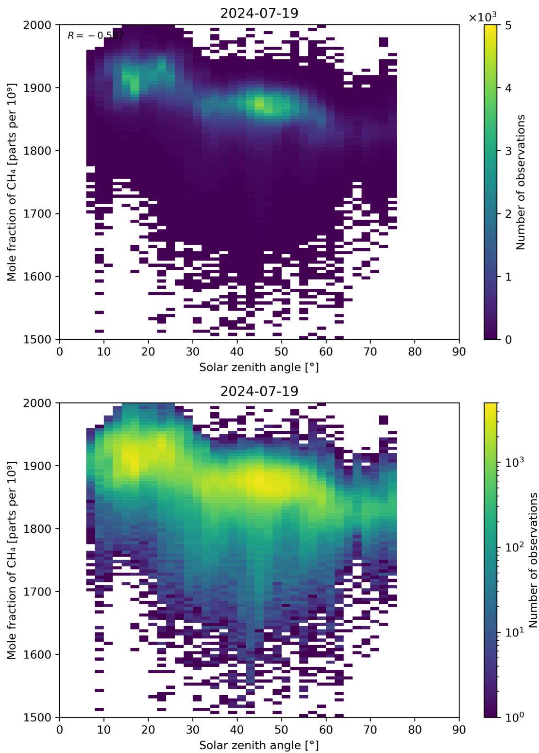
Figure 99: Scatter density plot of “Solar zenith angle” against “Mole fraction of CH 4 ” for 2024-07-18 to 2024-07-20.
