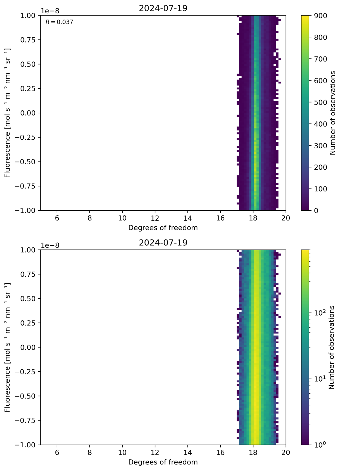
Figure 51: Scatter density plot of “Degrees of freedom” against “Fluorescence” for 2024-07-18 to 2024-07-20.
