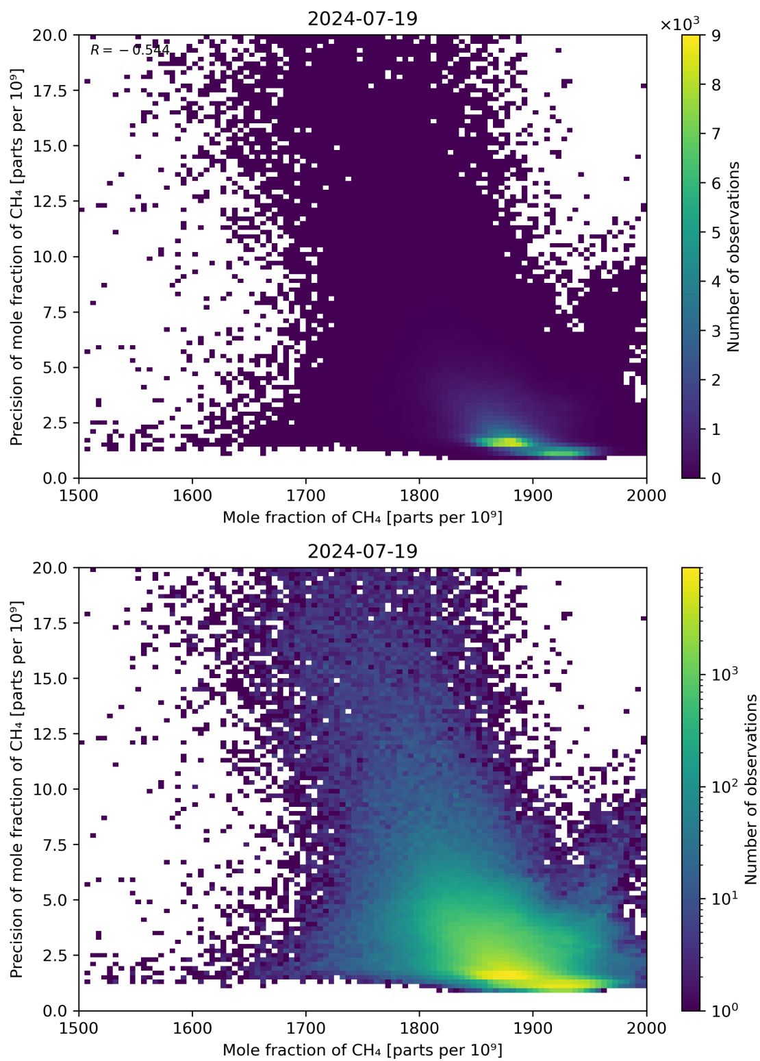
Figure 75: Scatter density plot of “Mole fraction of CH 4 ” against “Precision of mole fraction of CH 4 ” for 2024-07-18 to 2024-07-20.
