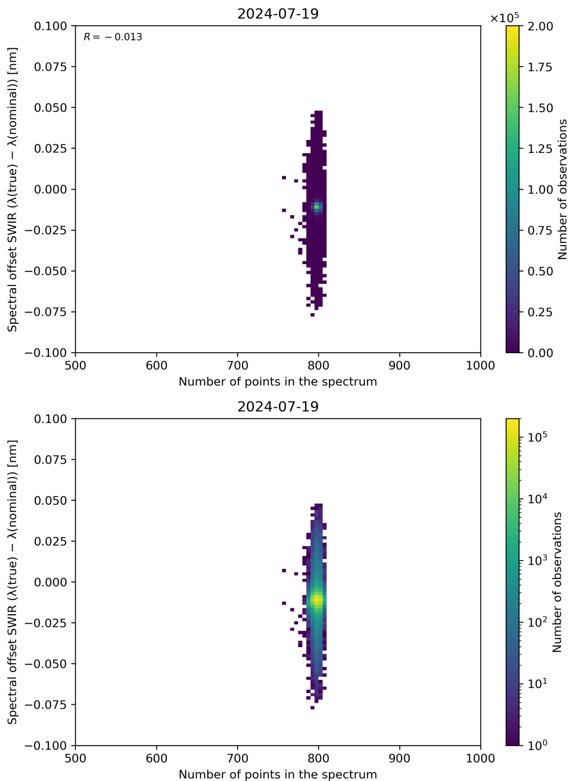
Figure 93: Scatter density plot of “Number of points in the spectrum” against “Spectral offset SWIR ( \lambda(\text{true}) - \lambda(\text{nominal}) )” for 2024-07-18 to 2024-07-20.
