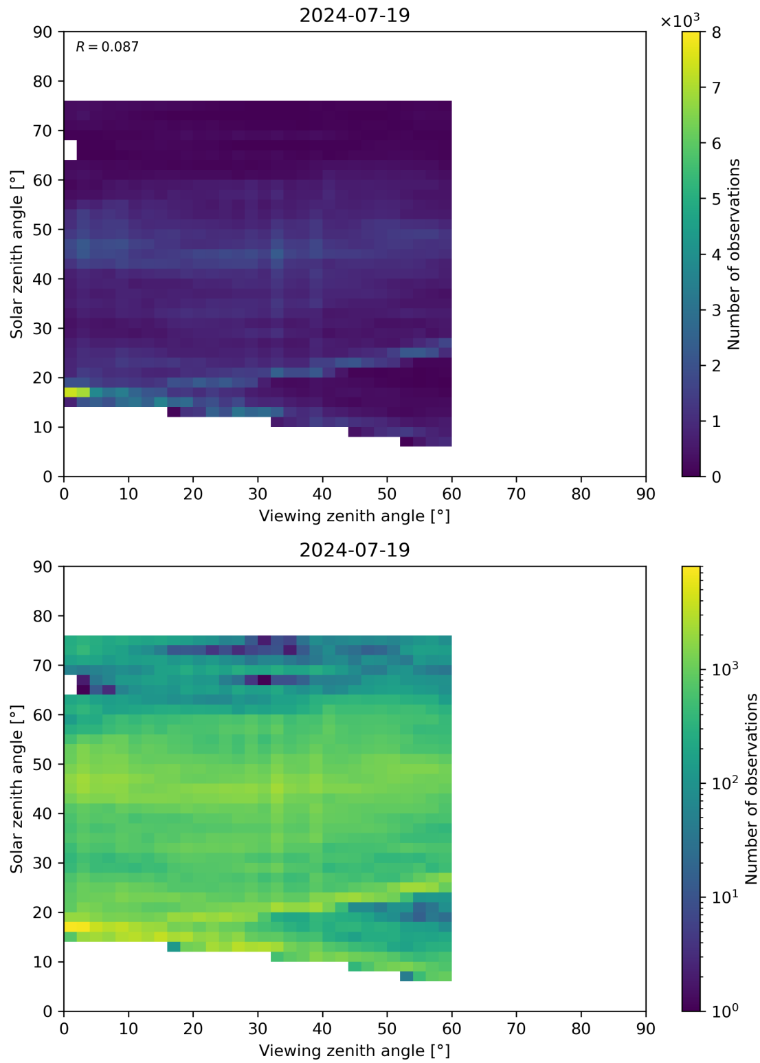
Figure 115: Scatter density plot of “Viewing zenith angle” against “Solar zenith angle” for 2024-07-18 to 2024-07-20.
