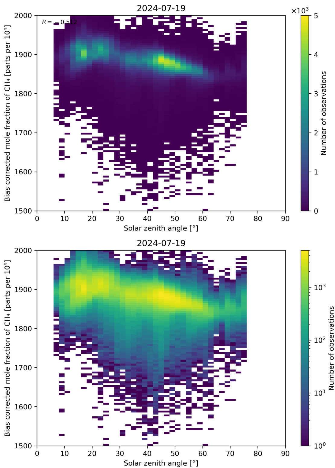
Figure 100: Scatter density plot of “Solar zenith angle” against “Bias corrected mole fraction of CH 4 ” for 2024-07-18 to 2024-07-20.
