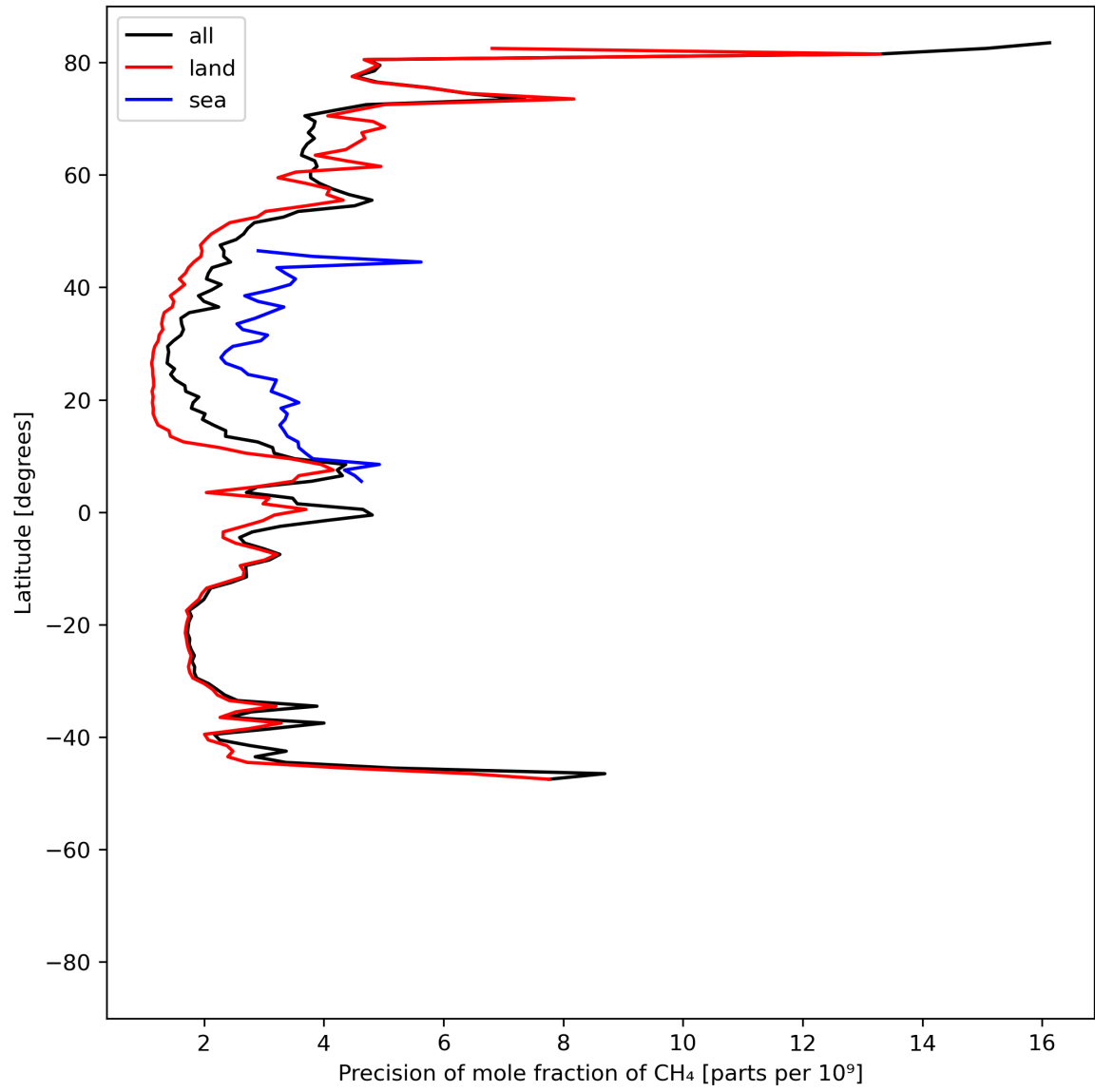
Figure 13: Zonal average of “Precision of mole fraction of CH 4 ” for 2024-07-18 to 2024-07-20.
