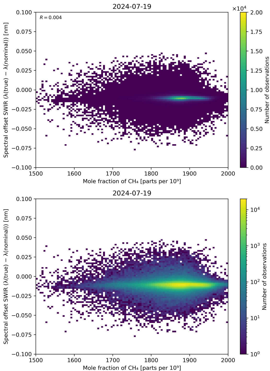
Figure 86: Scatter density plot of “Mole fraction of CH 4 ” against “Spectral offset SWIR ( \lambda(\text{true}) - \lambda(\text{nominal}) )” for 2024-07-18 to 2024-07-20.
