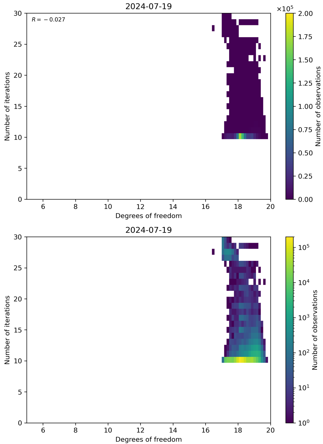
Figure 52: Scatter density plot of “Degrees of freedom” against “Number of iterations” for 2024-07-18 to 2024-07-20.
