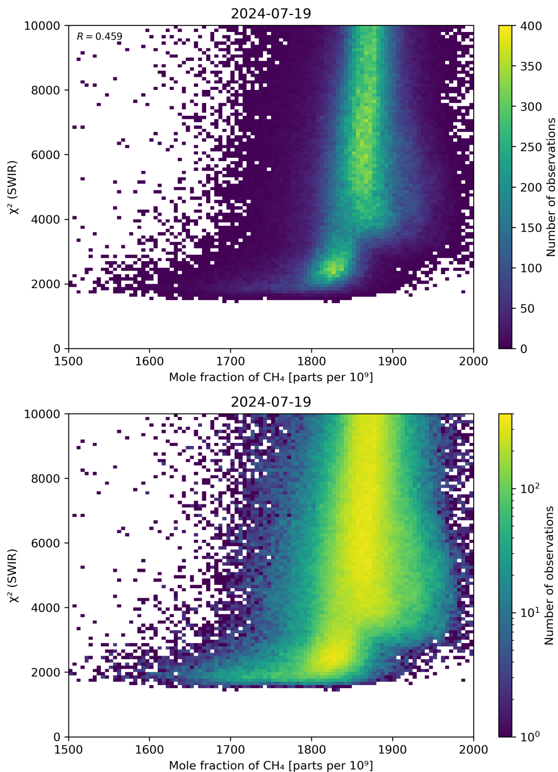
Figure 71: Scatter density plot of “Mole fraction of \text{CH}_4 ” against “ \chi^2 (SWIR)” for 2024-07-18 to 2024-07-20.
