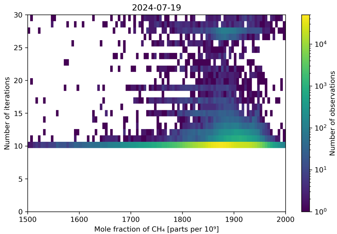
Figure 76: Scatter density plot of “Mole fraction of CH 4 ” against “Number of iterations” for 2024-07-18 to 2024-07-20.
