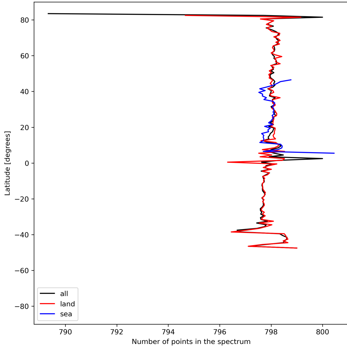
Figure 15: Zonal average of “Number of points in the spectrum” for 2024-07-18 to 2024-07-20.
