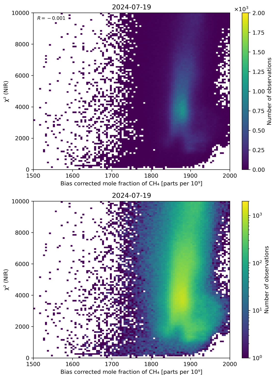
Figure 63: Scatter density plot of “Bias corrected mole fraction of CH 4 ” against “ \chi^2 (NIR)” for 2024-07-18 to 2024-07-20.
