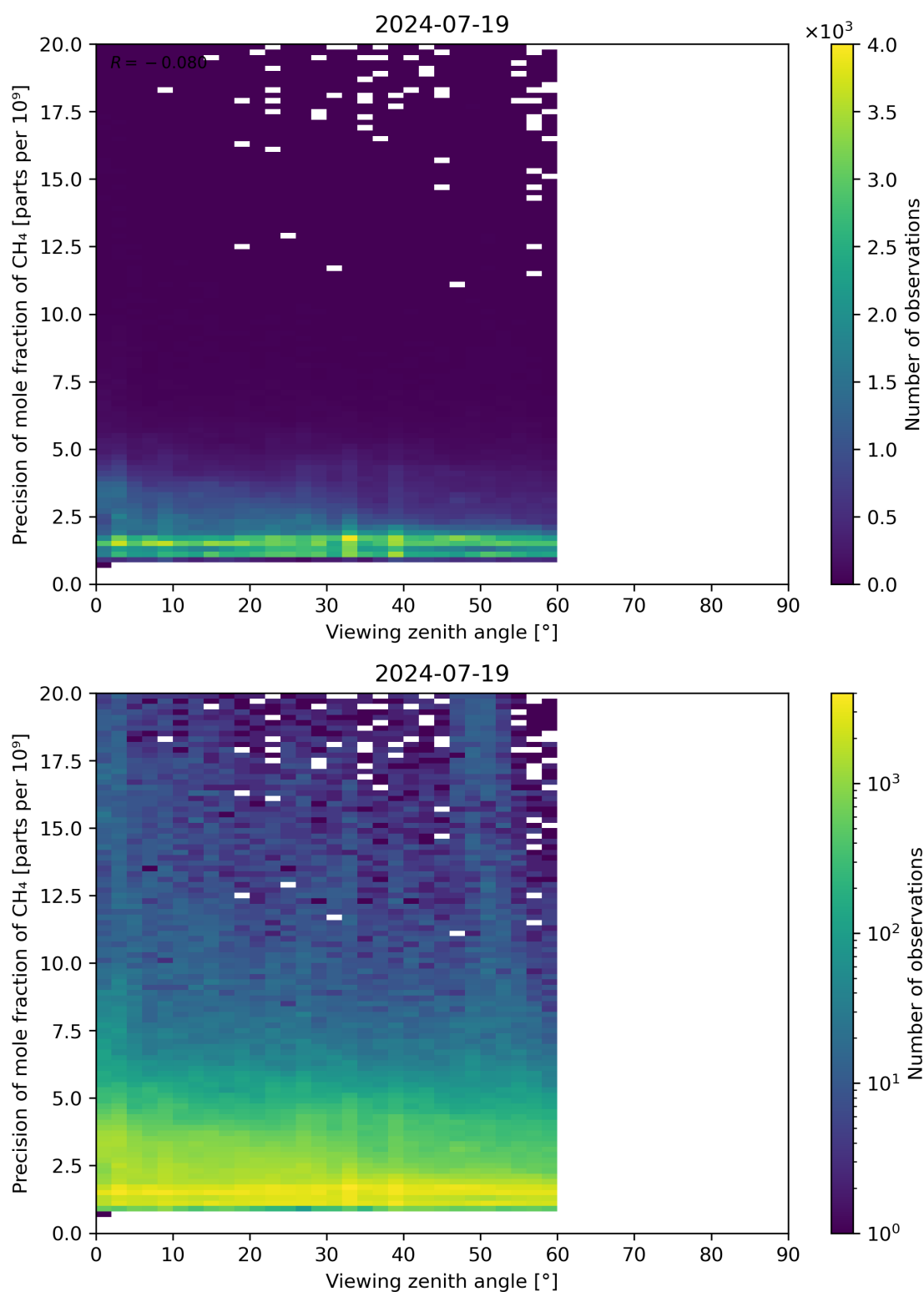
Figure 112: Scatter density plot of “Viewing zenith angle” against “Precision of mole fraction of CH 4 ” for 2024-07-18 to 2024-07-20.
