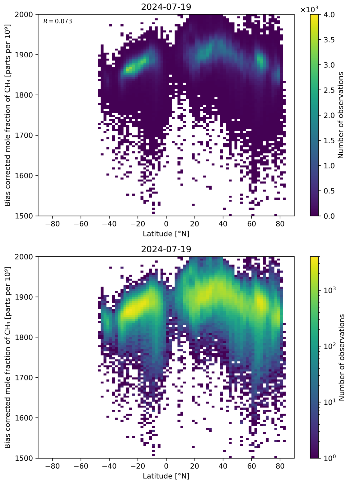
Figure 58: Scatter density plot of “Latitude” against “Bias corrected mole fraction of CH 4 ” for 2024-07-18 to 2024-07-20.
