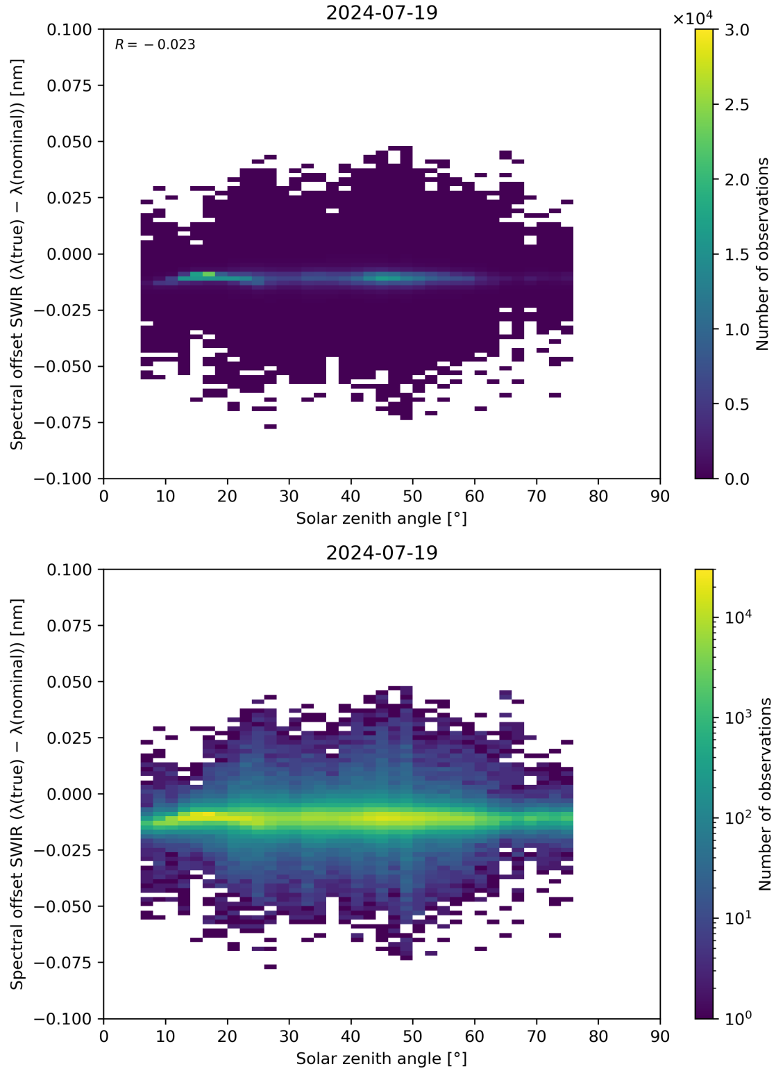
Figure 104: Scatter density plot of “Solar zenith angle” against “Spectral offset SWIR ( \lambda(\text{true}) - \lambda(\text{nominal}) )” for 2024-07-18 to 2024-07-20.
