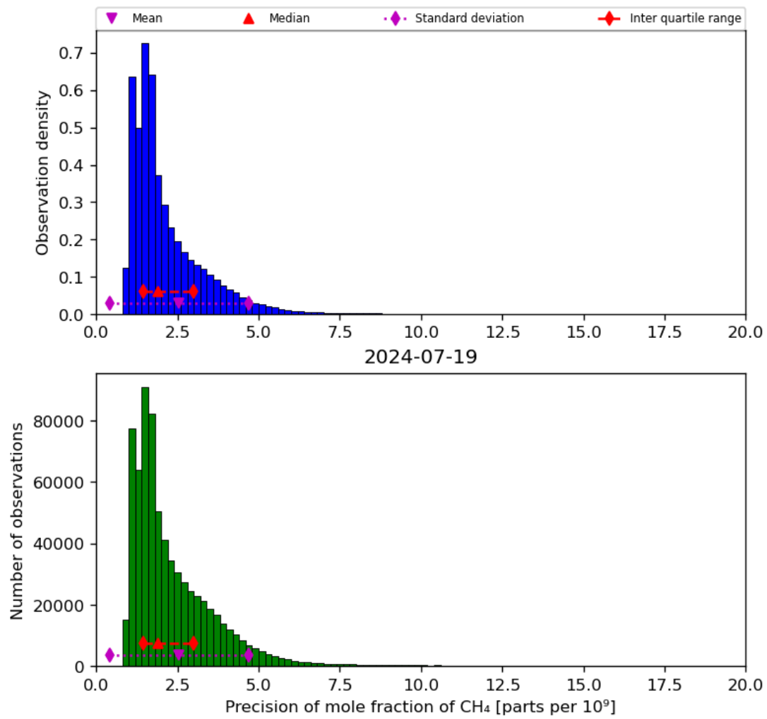
Figure 24: Histogram of “Precision of mole fraction of CH 4 ” for 2024-07-18 to 2024-07-20
