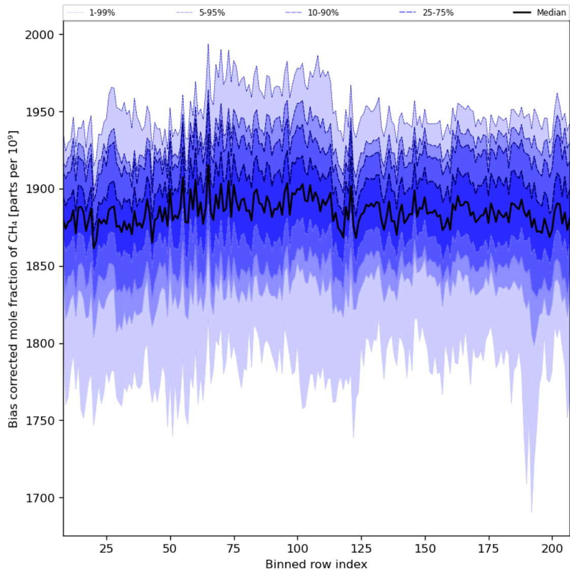
Figure 36: Along track statistics of “Bias corrected mole fraction of CH 4 ” for 2024-07-18 to 2024-07-20
