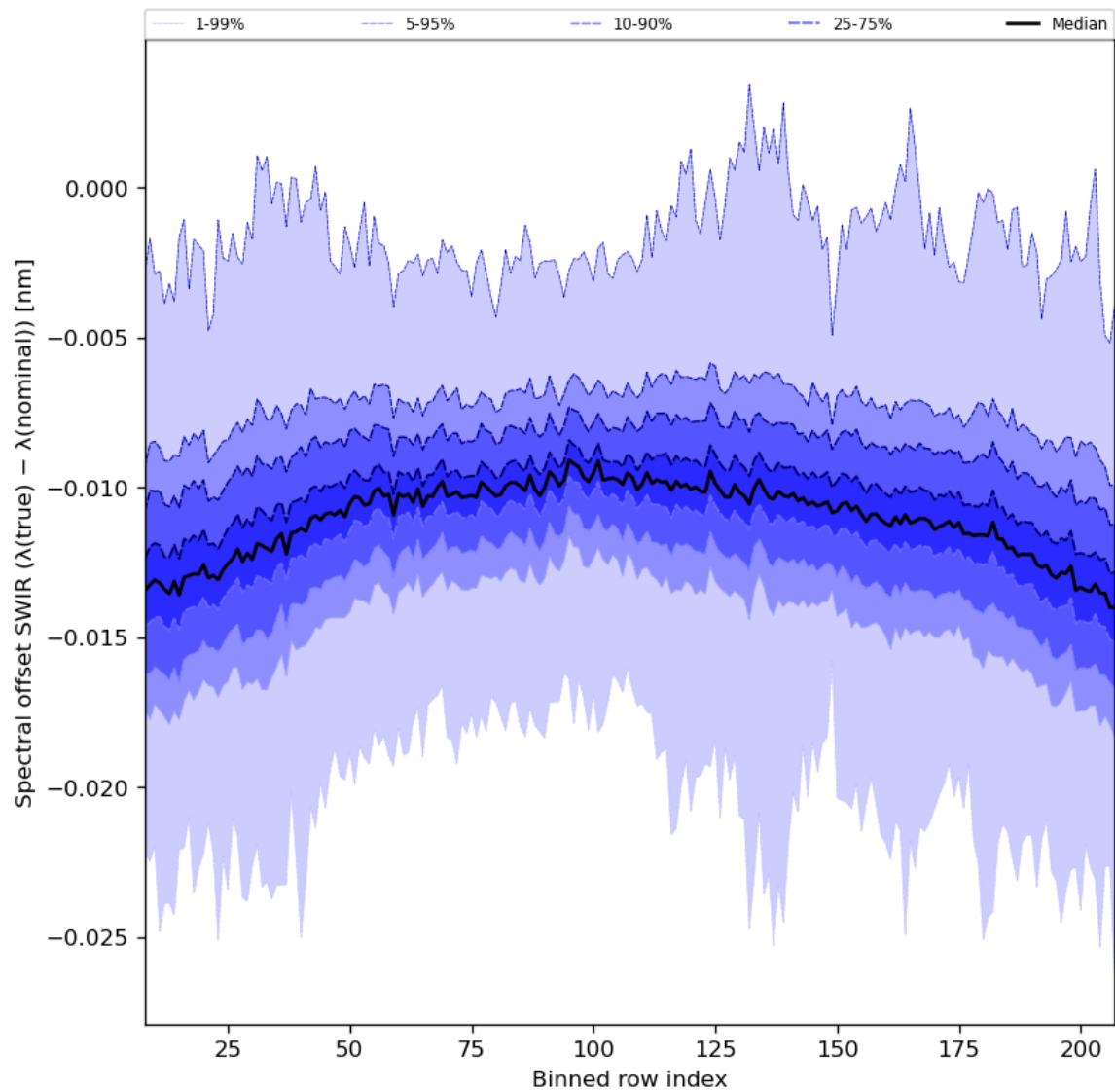
Figure 38: Along track statistics of “Spectral offset SWIR ( \lambda(\text{true}) - \lambda(\text{nominal}) )” for 2024-07-18 to 2024-07-20
