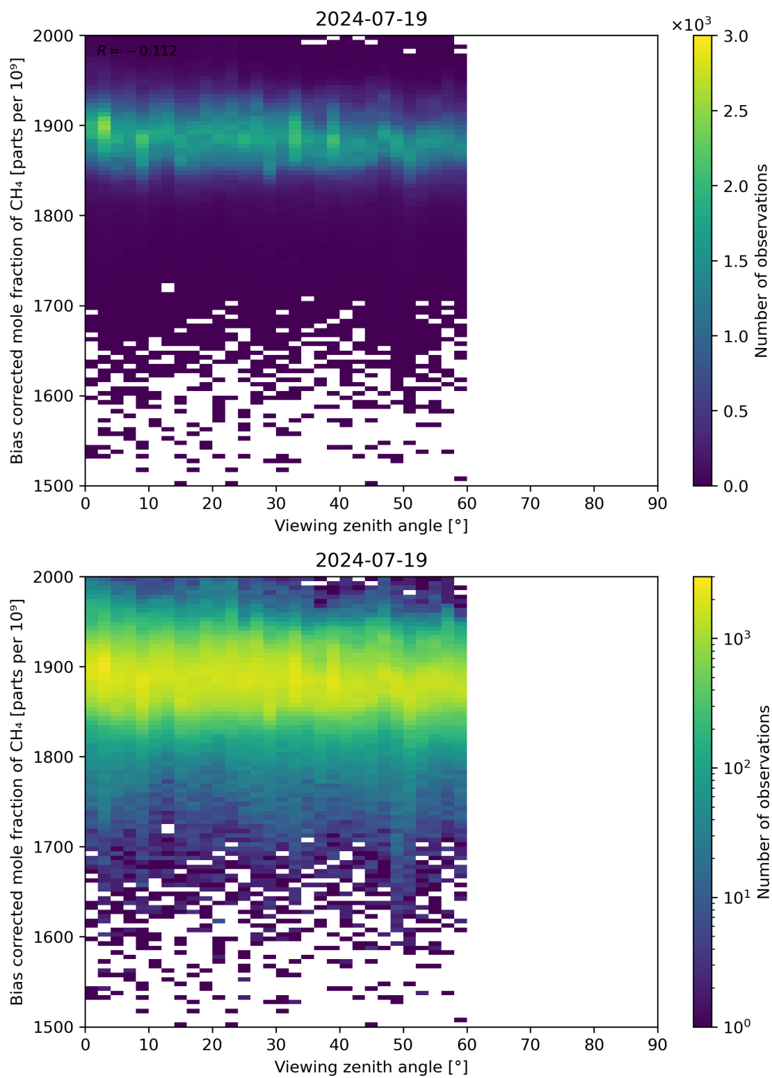
Figure 111: Scatter density plot of “Viewing zenith angle” against “Bias corrected mole fraction of CH 4 ” for 2024-07-18 to 2024-07-20.
