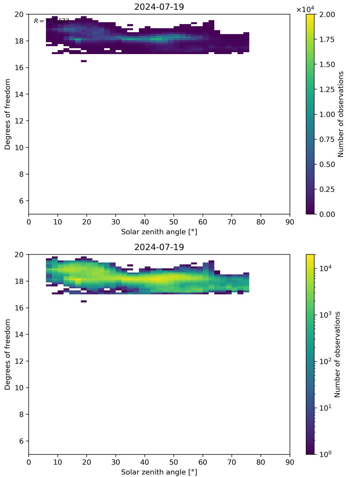
Figure 96: Scatter density plot of “Solar zenith angle” against “Degrees of freedom” for 2024-07-18 to 2024-07-20.
