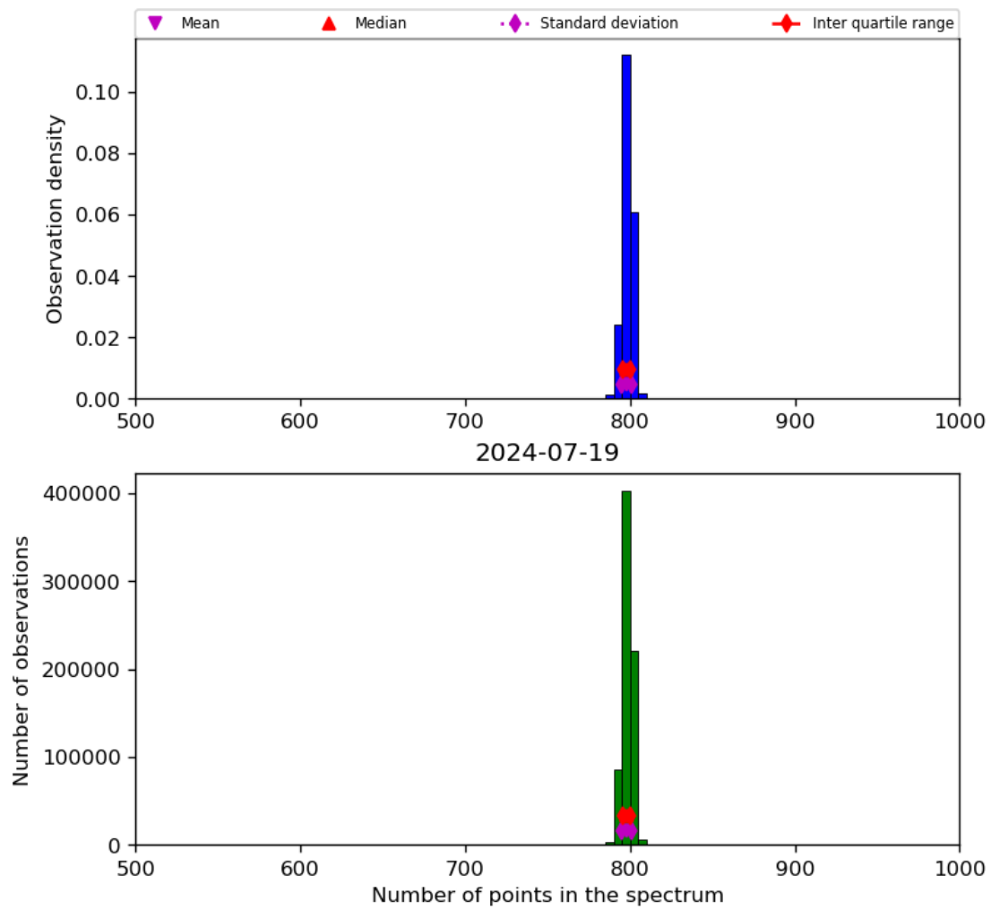
Figure 26: Histogram of “Number of points in the spectrum” for 2024-07-18 to 2024-07-20
