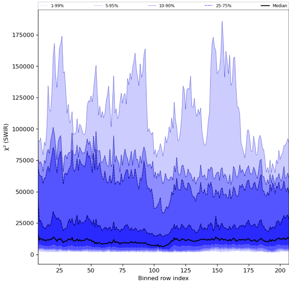
Figure 39: Along track statistics of “ \chi^2 (SWIR)” for 2024-07-18 to 2024-07-20
