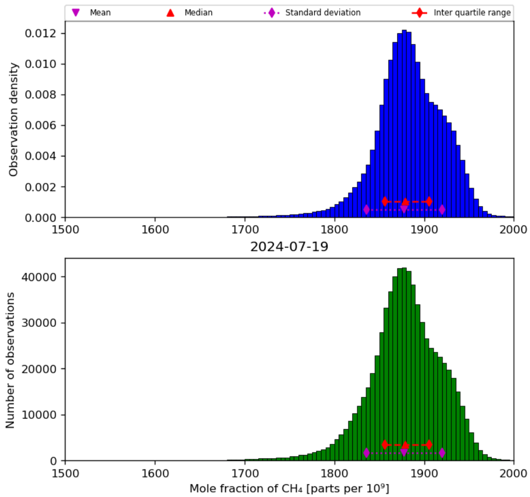
Figure 23: Histogram of “Mole fraction of CH 4 ” for 2024-07-18 to 2024-07-20
