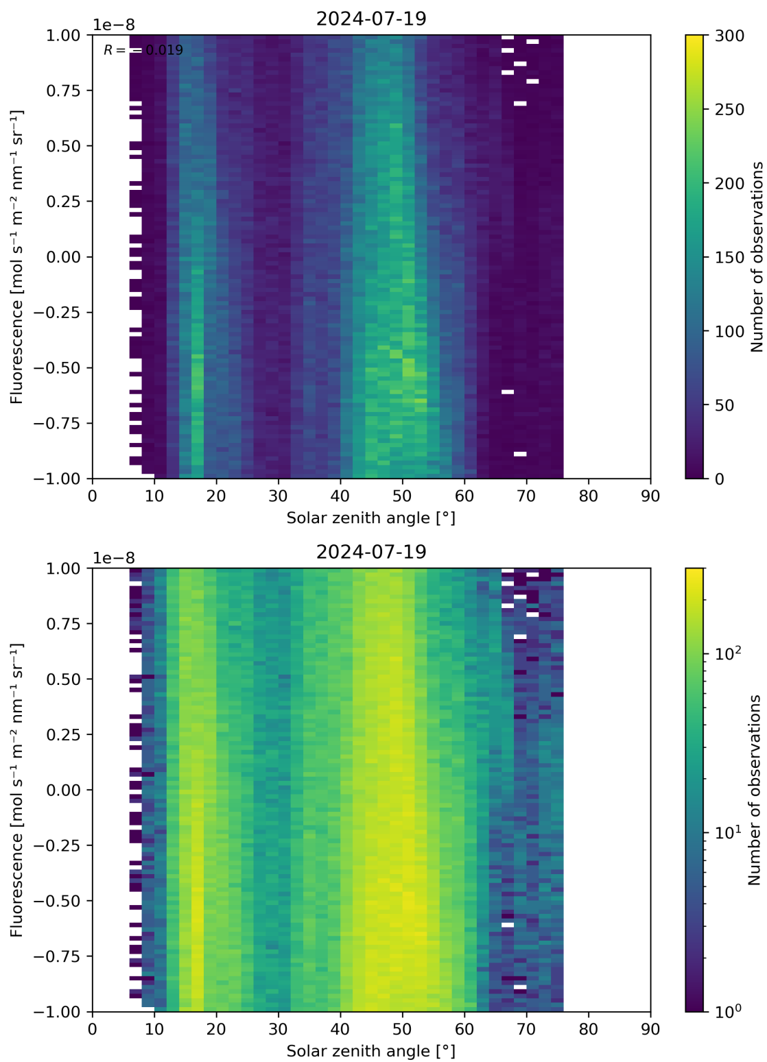
Figure 97: Scatter density plot of “Solar zenith angle” against “Fluorescence” for 2024-07-18 to 2024-07-20.
