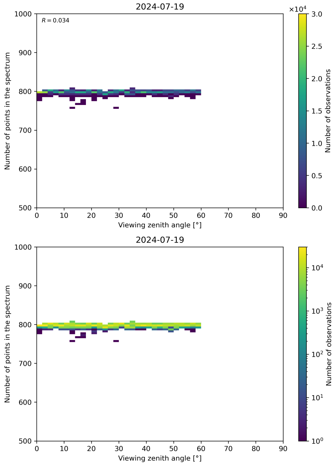
Figure 114: Scatter density plot of “Viewing zenith angle” against “Number of points in the spectrum” for 2024-07-18 to 2024-07-20.
