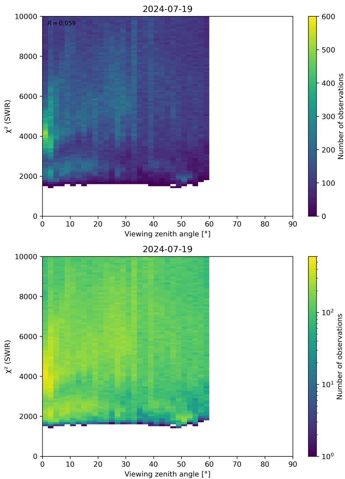
Figure 106: Scatter density plot of “Viewing zenith angle” against “ \chi^2 (SWIR)” for 2024-07-18 to 2024-07-20.
