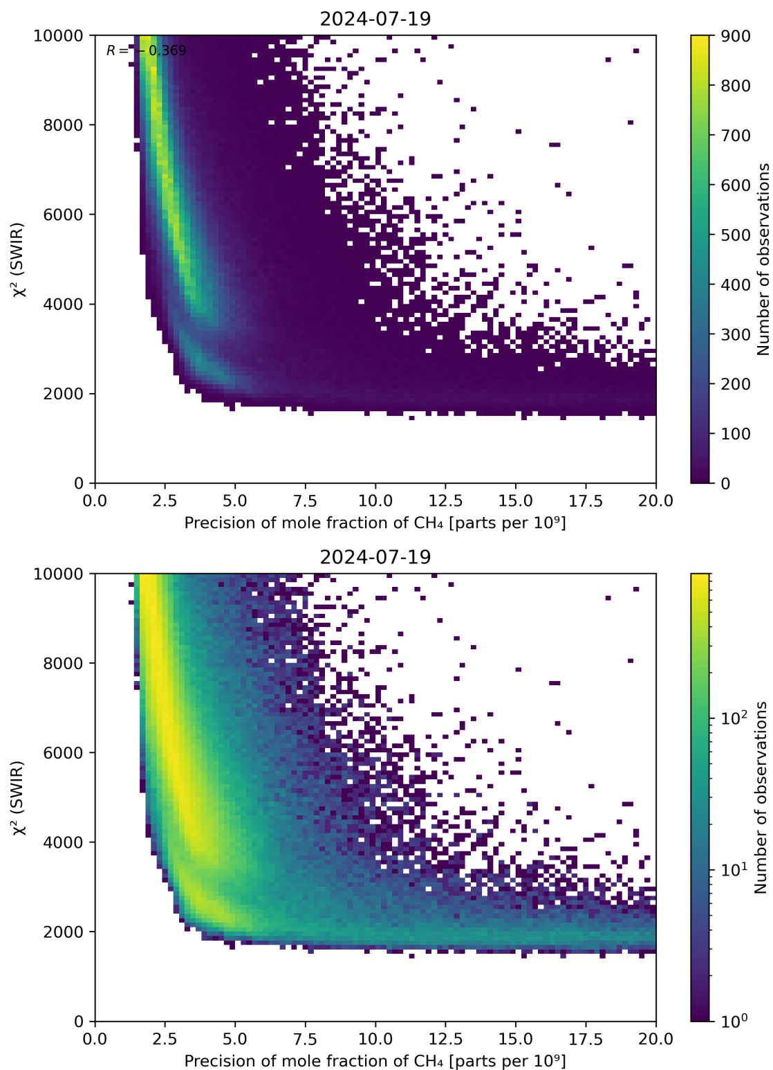
Figure 79: Scatter density plot of “Precision of mole fraction of CH 4 ” against “ \chi^2 (SWIR)” for 2024-07-18 to 2024-07-20.
