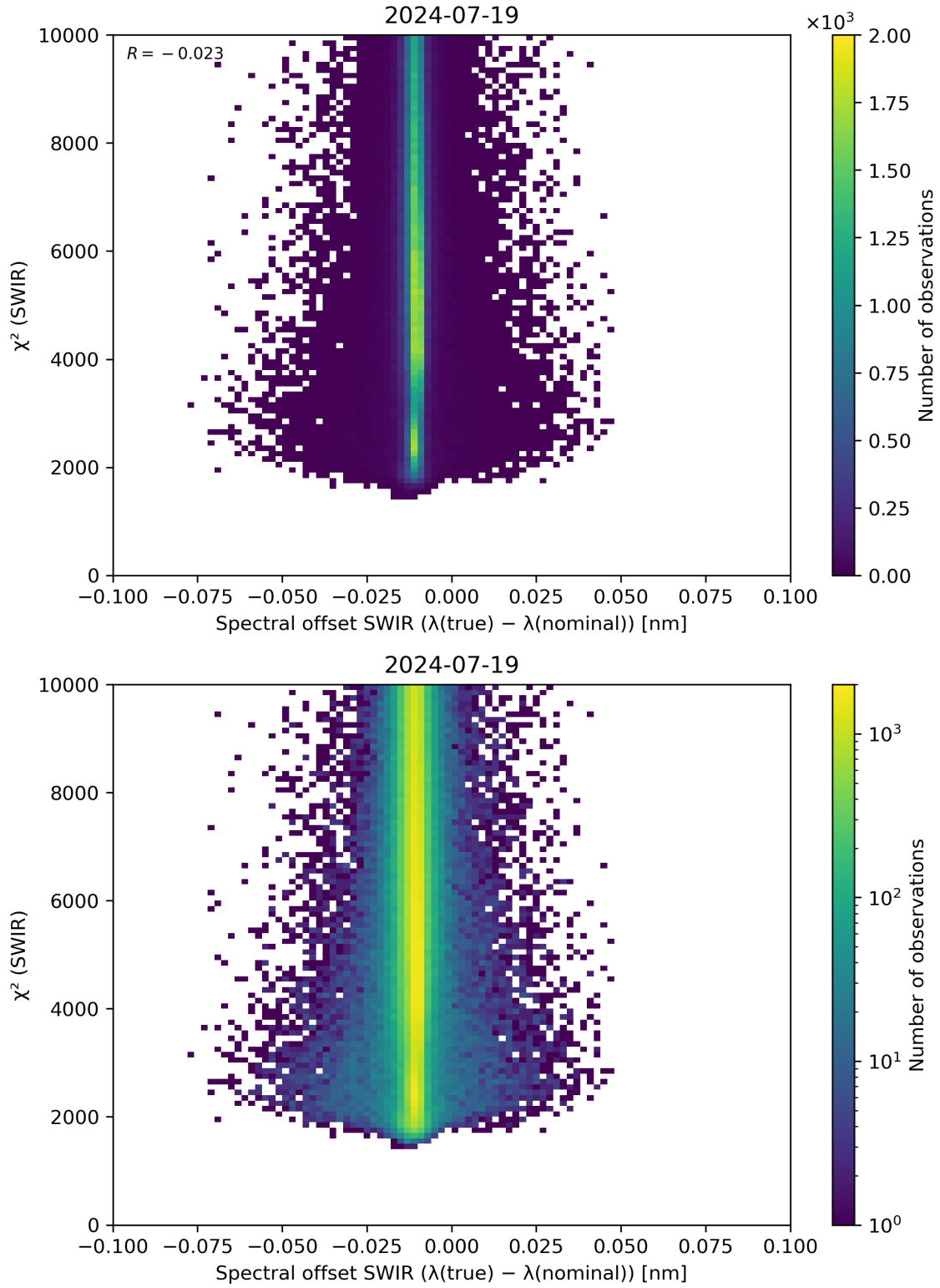
Figure 118: Scatter density plot of “Spectral offset SWIR ( \lambda(\text{true}) - \lambda(\text{nominal}) )” against “ \chi^2 (SWIR)” for 2024-07-18 to 2024-07-20.
