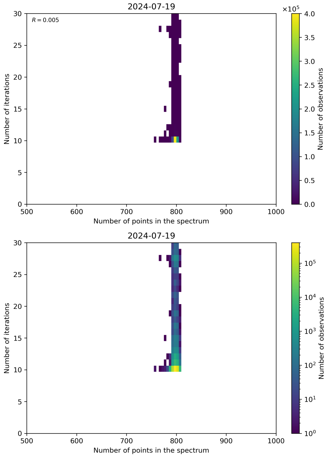
Figure 92: Scatter density plot of “Number of points in the spectrum” against “Number of iterations” for 2024-07-18 to 2024-07-20.
