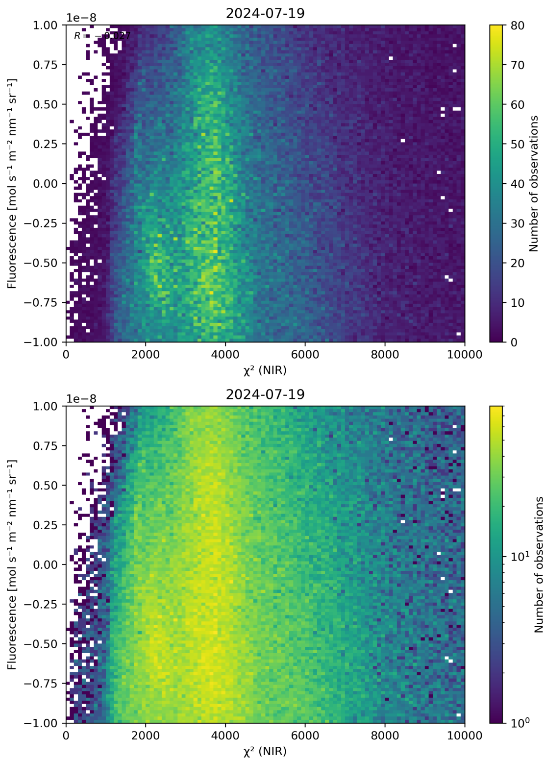
Figure 45: Scatter density plot of “ \chi^2 (NIR)” against “Fluorescence” for 2024-07-18 to 2024-07-20.
