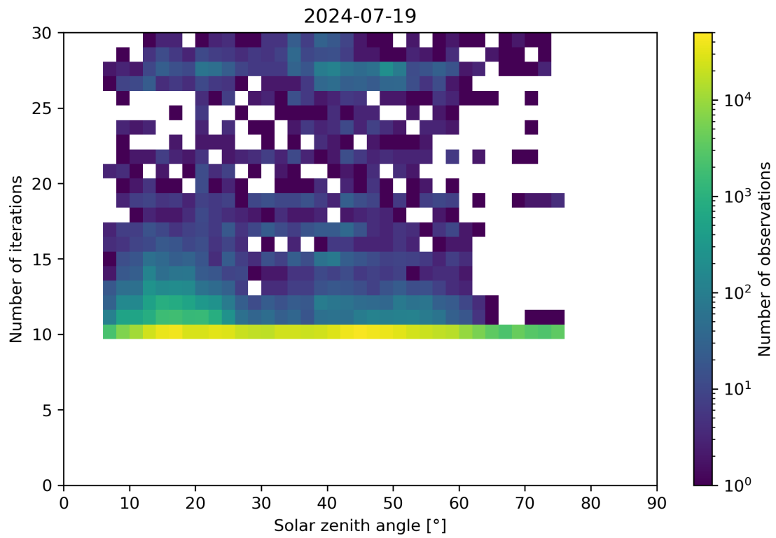
Figure 102: Scatter density plot of “Solar zenith angle” against “Number of iterations” for 2024-07-18 to 2024-07-20.
