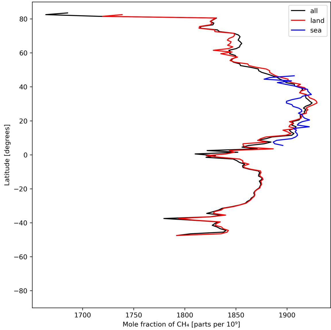
Figure 12: Zonal average of “Mole fraction of \text{CH}_4 ” for 2024-07-18 to 2024-07-20.
