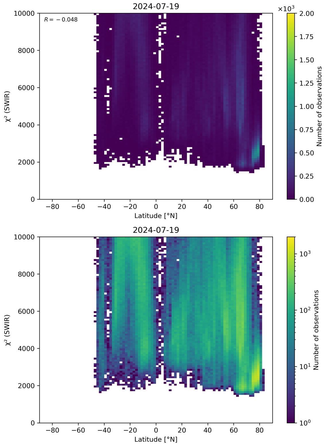
Figure 54: Scatter density plot of “Latitude” against “ \chi^2 (SWIR)” for 2024-07-18 to 2024-07-20.
