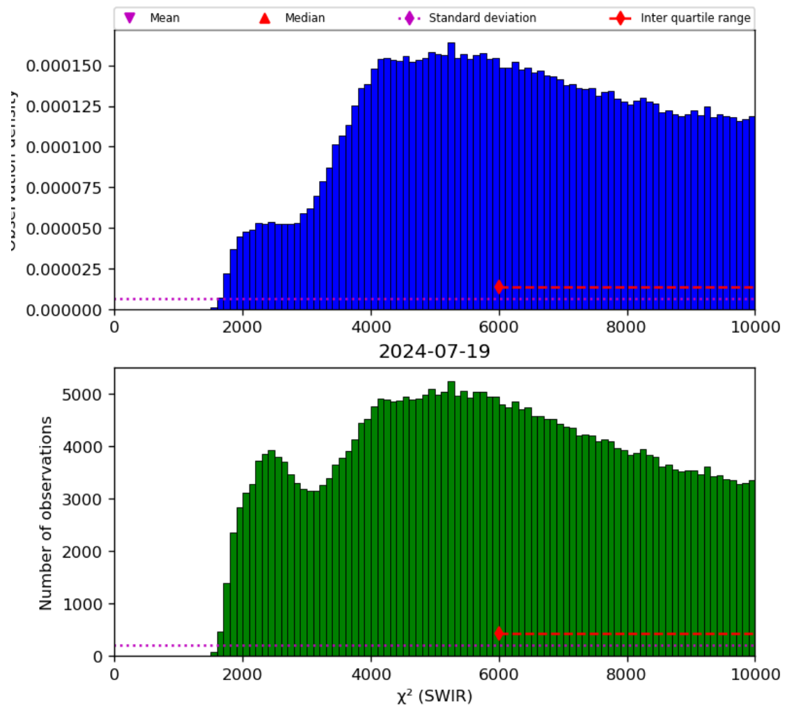
Figure 28: Histogram of “ \chi^2 (SWIR)” for 2024-07-18 to 2024-07-20
