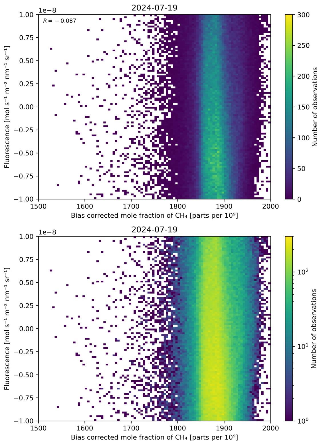
Figure 66: Scatter density plot of “Bias corrected mole fraction of \text{CH}_4 ” against “Fluorescence” for 2024-07-18 to 2024-07-20.
