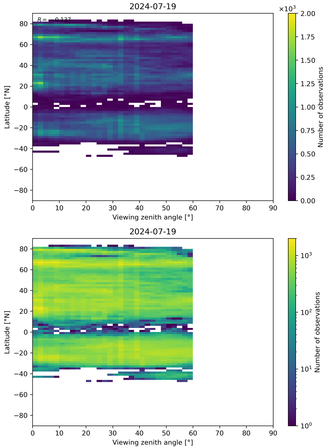
Figure 109: Scatter density plot of “Viewing zenith angle” against “Latitude” for 2024-07-18 to 2024-07-20.
