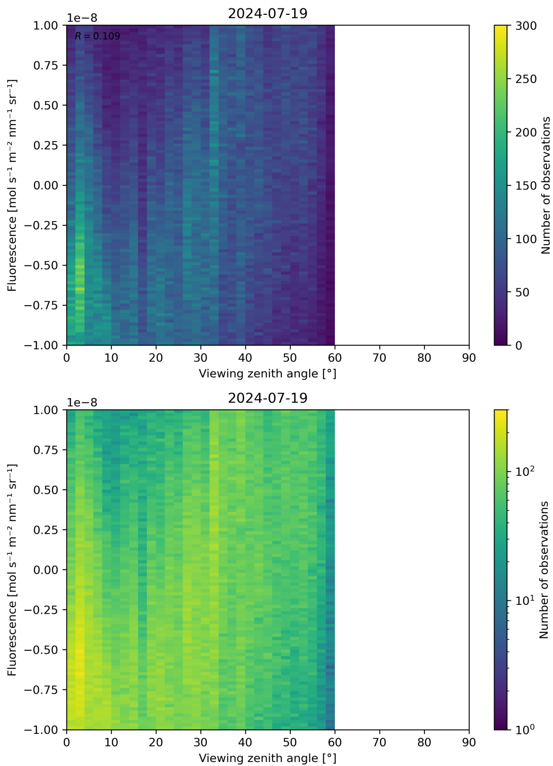
Figure 108: Scatter density plot of “Viewing zenith angle” against “Fluorescence” for 2024-07-18 to 2024-07-20.
