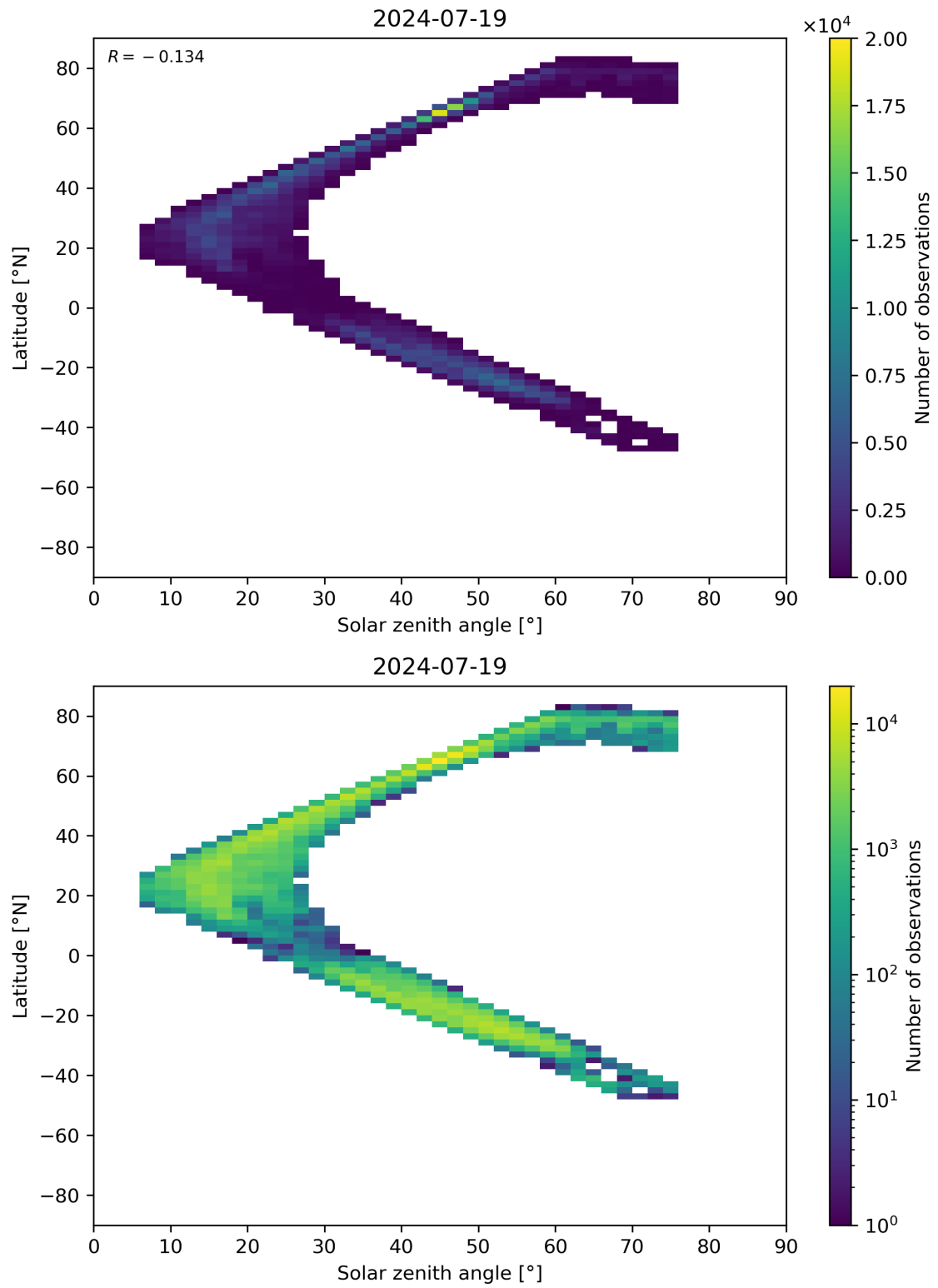
Figure 98: Scatter density plot of “Solar zenith angle” against “Latitude” for 2024-07-18 to 2024-07-20.
