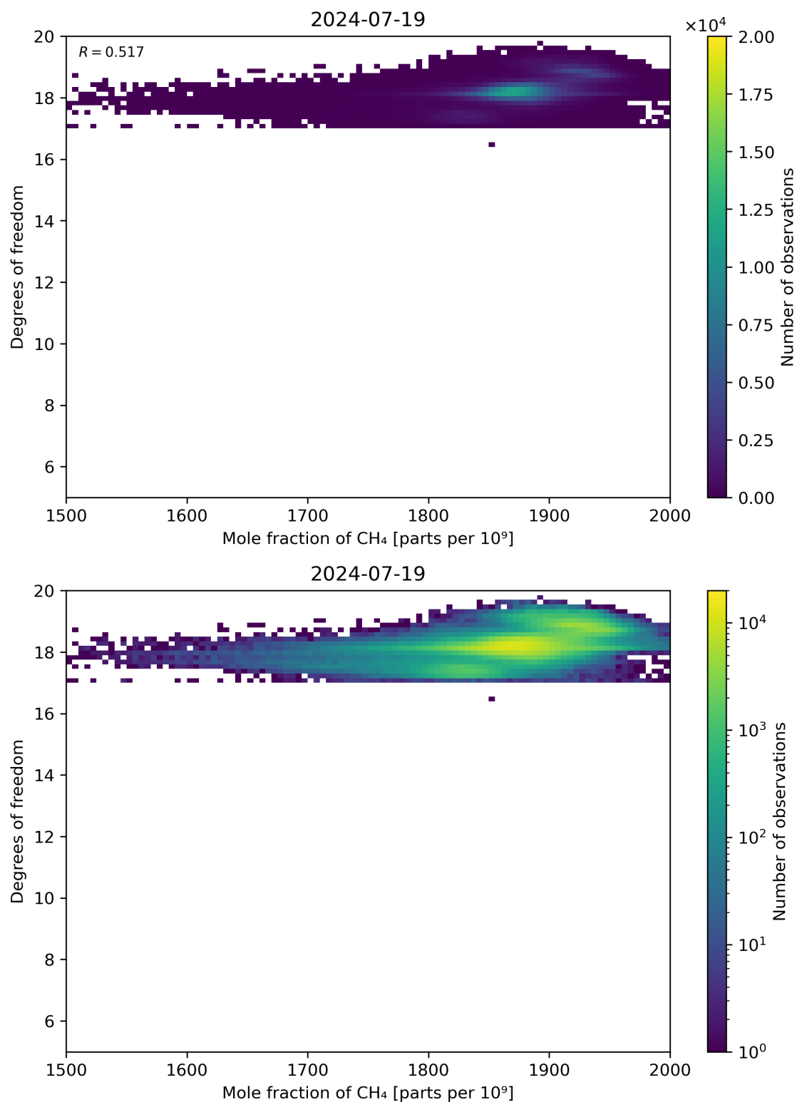
Figure 72: Scatter density plot of “Mole fraction of CH 4 ” against “Degrees of freedom” for 2024-07-18 to 2024-07-20.
