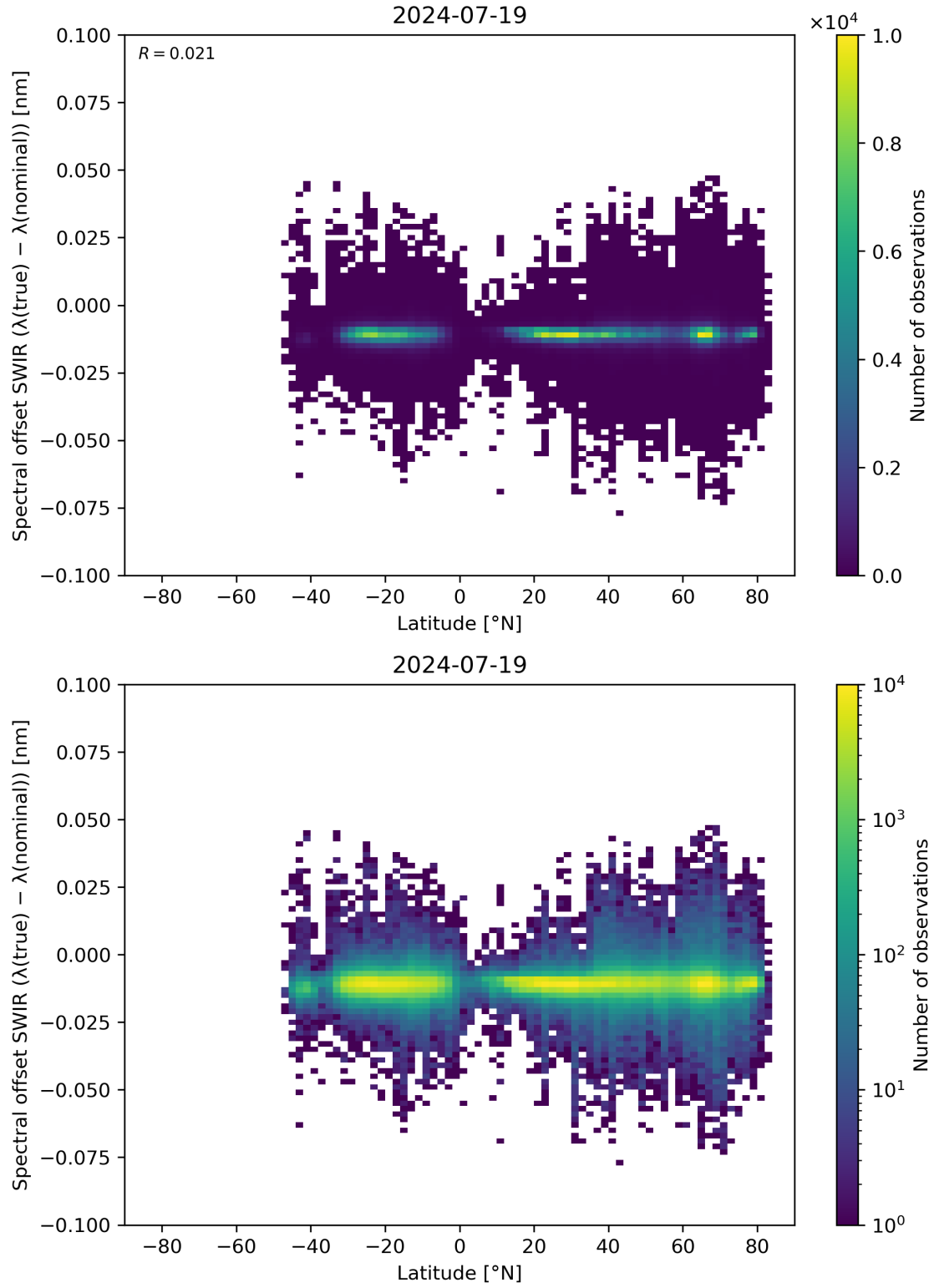
Figure 62: Scatter density plot of “Latitude” against “Spectral offset SWIR ( \lambda(\text{true}) - \lambda(\text{nominal}) )” for 2024-07-18 to 2024-07-20.
