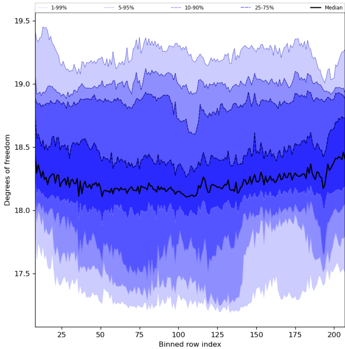
Figure 41: Along track statistics of “Degrees of freedom” for 2024-07-18 to 2024-07-20
