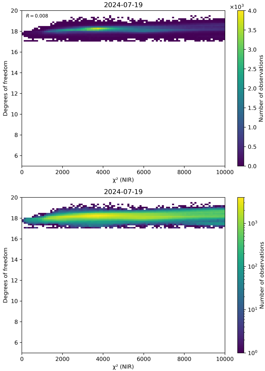
Figure 44: Scatter density plot of “ \chi^2 (NIR)” against “Degrees of freedom” for 2024-07-18 to 2024-07-20.
