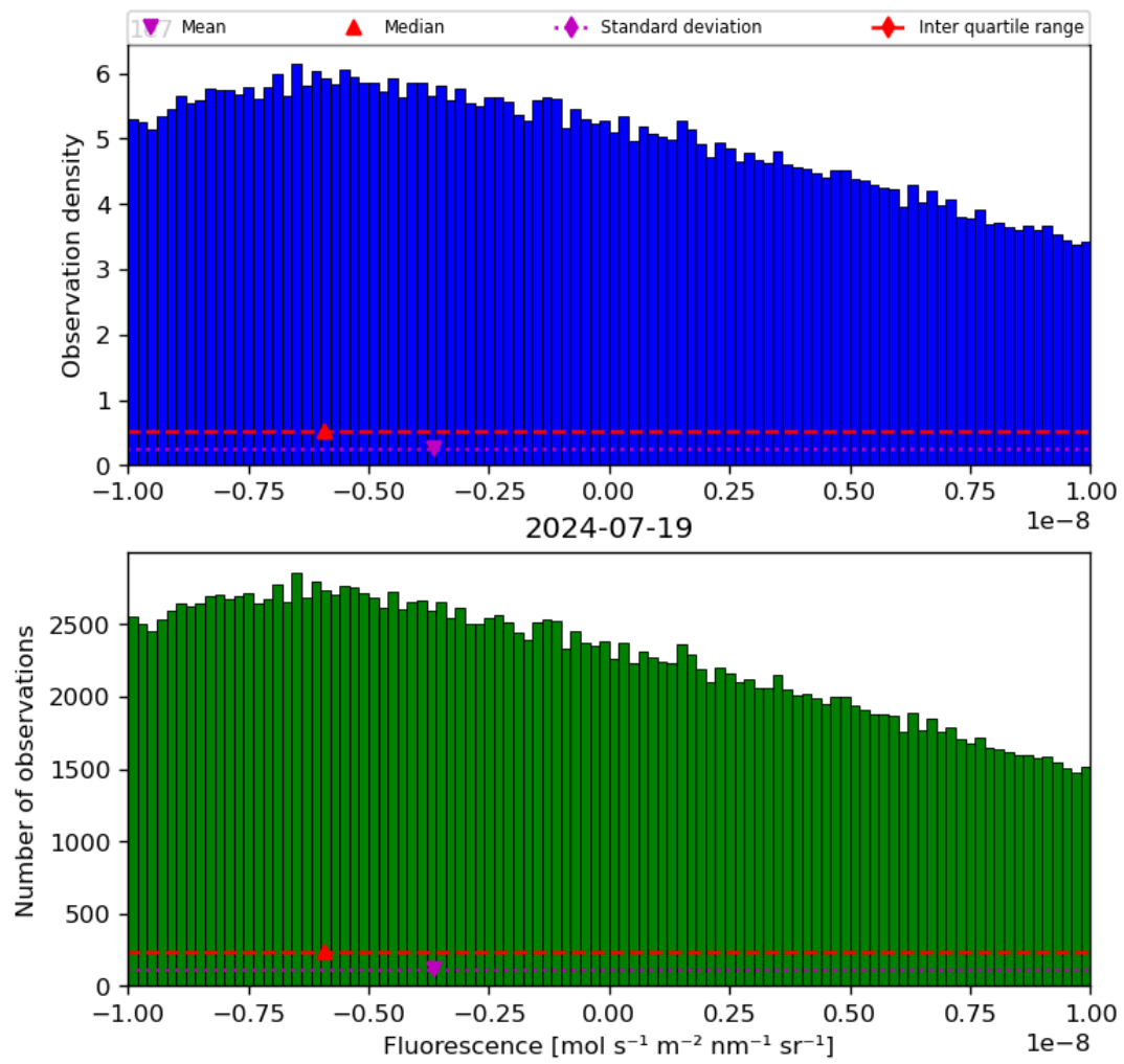
Figure 32: Histogram of “Fluorescence” for 2024-07-18 to 2024-07-20
