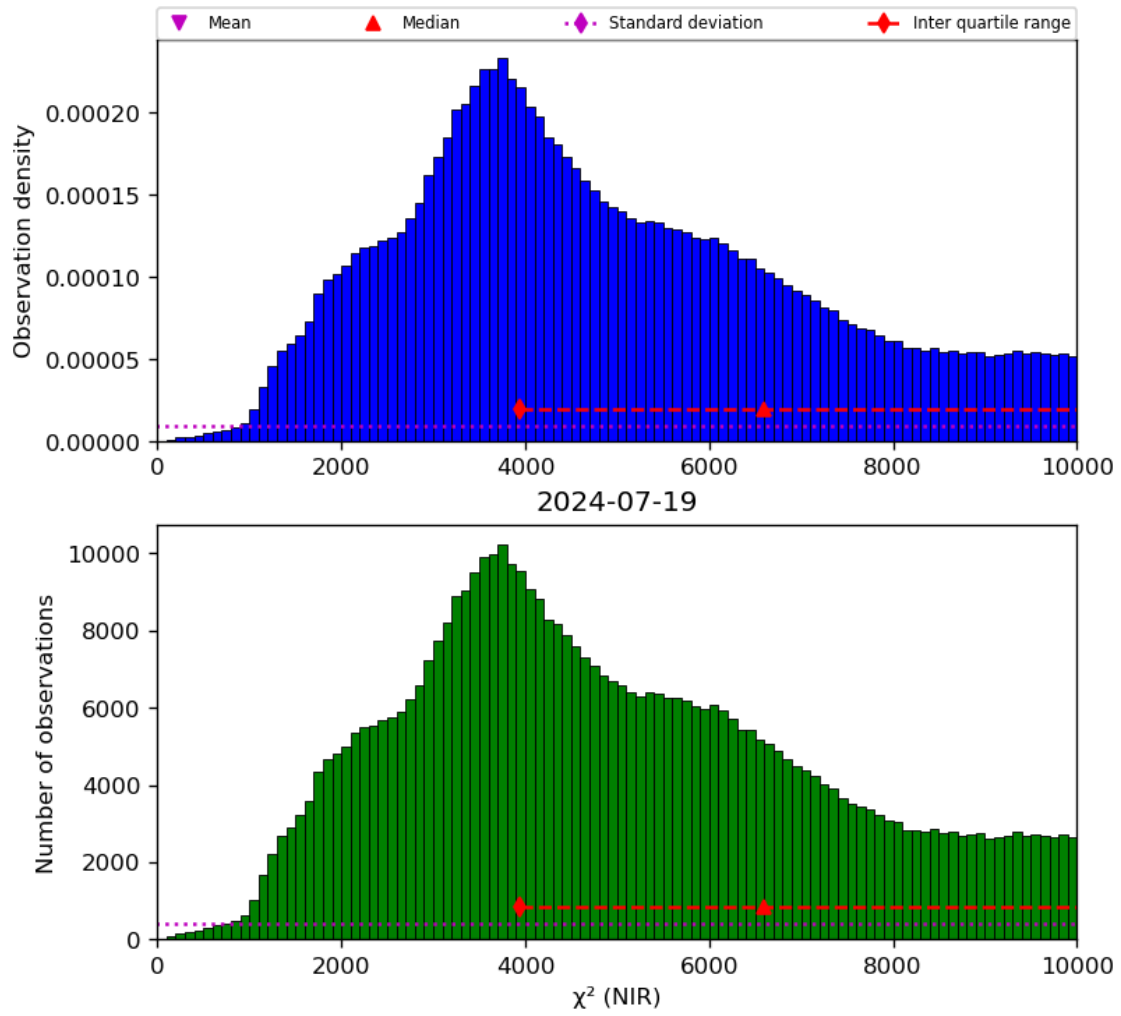
Figure 29: Histogram of “ \chi^2 (NIR)” for 2024-07-18 to 2024-07-20
