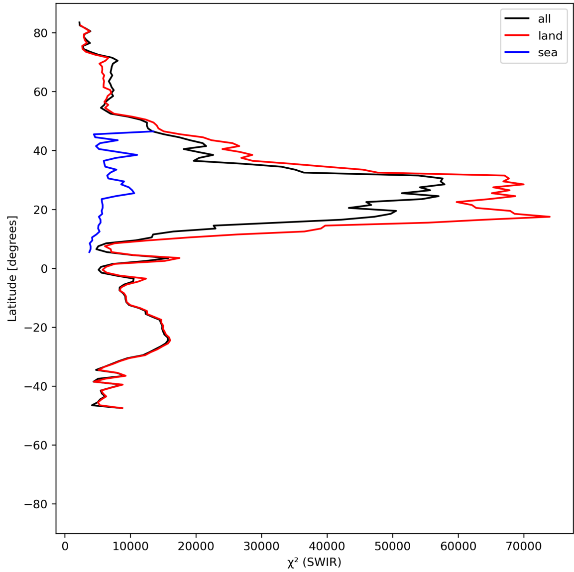
Figure 17: Zonal average of “ \chi^2 (SWIR)” for 2024-07-18 to 2024-07-20.
