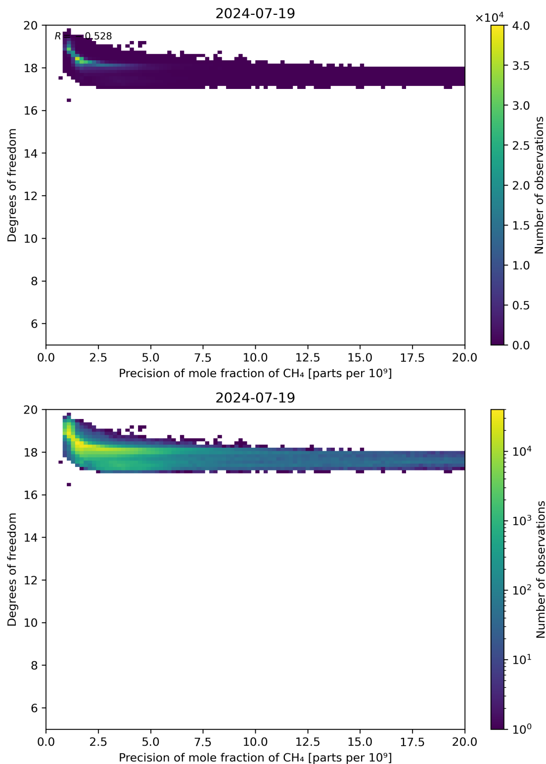
Figure 80: Scatter density plot of “Precision of mole fraction of CH 4 ” against “Degrees of freedom” for 2024-07-18 to 2024-07-20.
