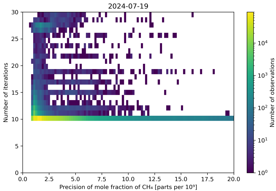
Figure 83: Scatter density plot of “Precision of mole fraction of CH 4 ” against “Number of iterations” for 2024-07-18 to 2024-07-20.
