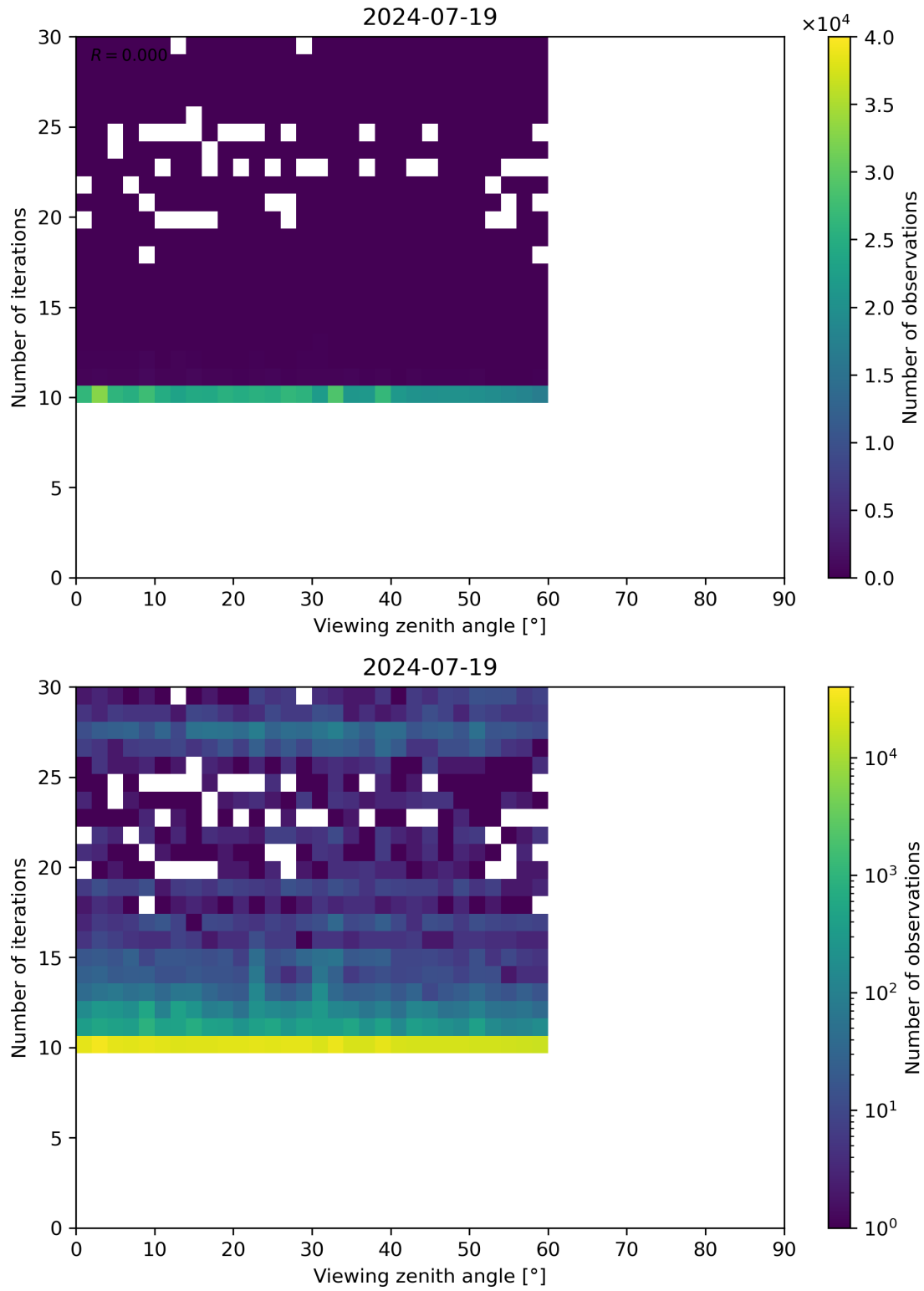
Figure 113: Scatter density plot of “Viewing zenith angle” against “Number of iterations” for 2024-07-18 to 2024-07-20.
