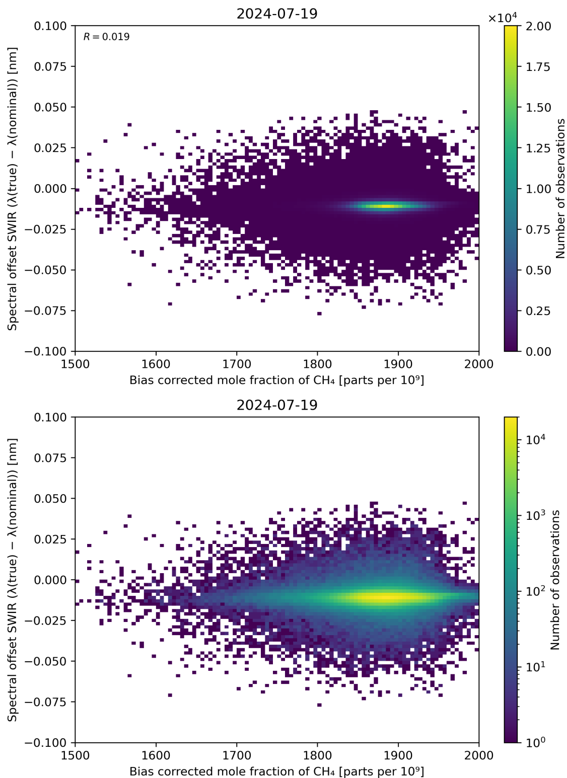
Figure 69: Scatter density plot of “Bias corrected mole fraction of \text{CH}_4 ” against “Spectral offset SWIR ( \lambda(\text{true}) - \lambda(\text{nominal}) )” for 2024-07-18 to 2024-07-20.
