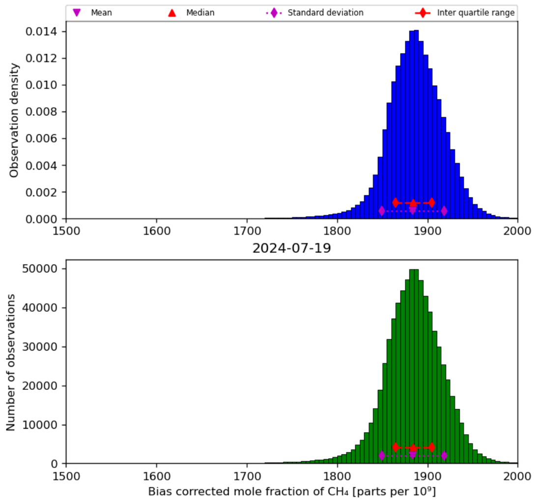
Figure 25: Histogram of “Bias corrected mole fraction of CH 4 ” for 2024-07-18 to 2024-07-20
