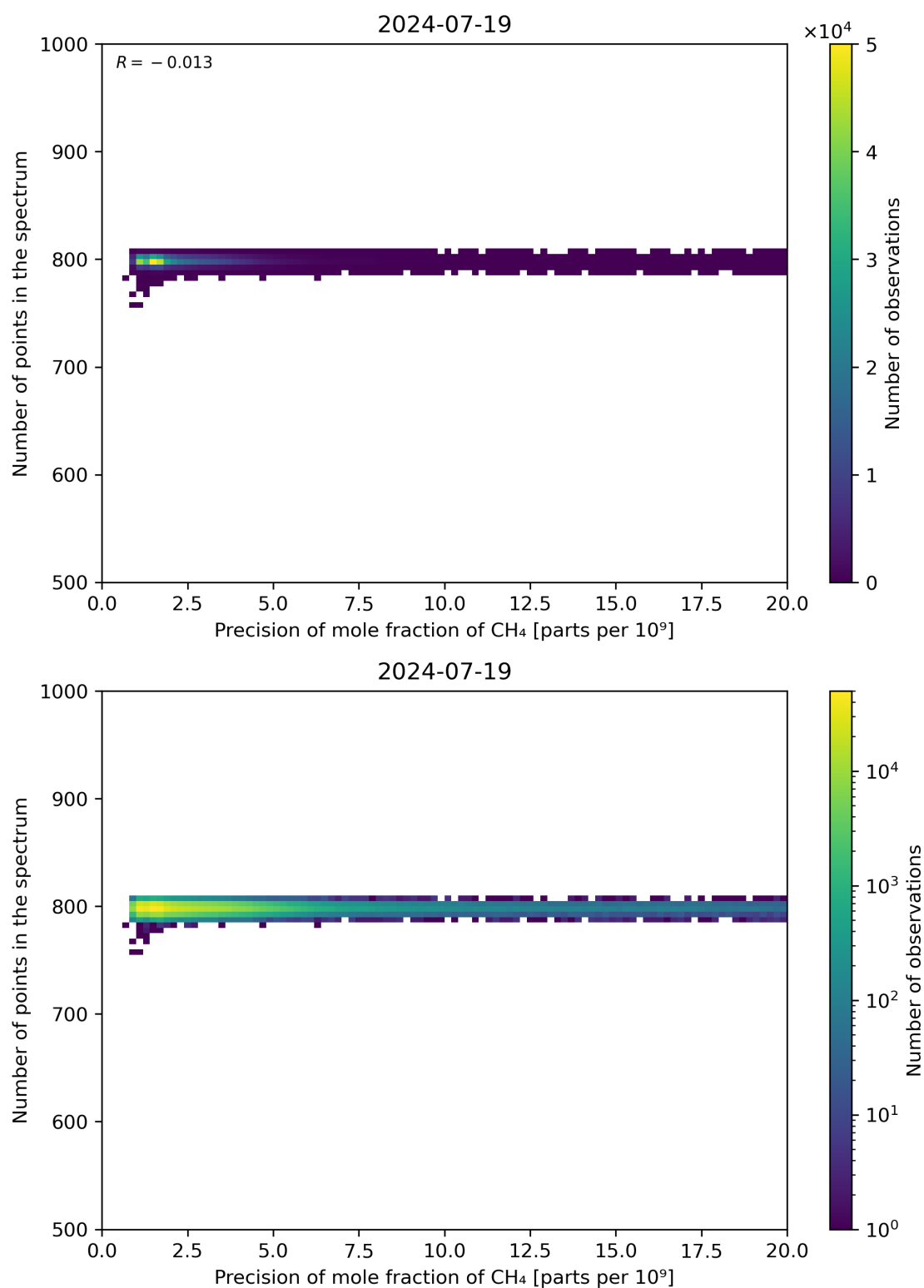
Figure 84: Scatter density plot of “Precision of mole fraction of CH 4 ” against “Number of points in the spectrum” for 2024-07-18 to 2024-07-20.
