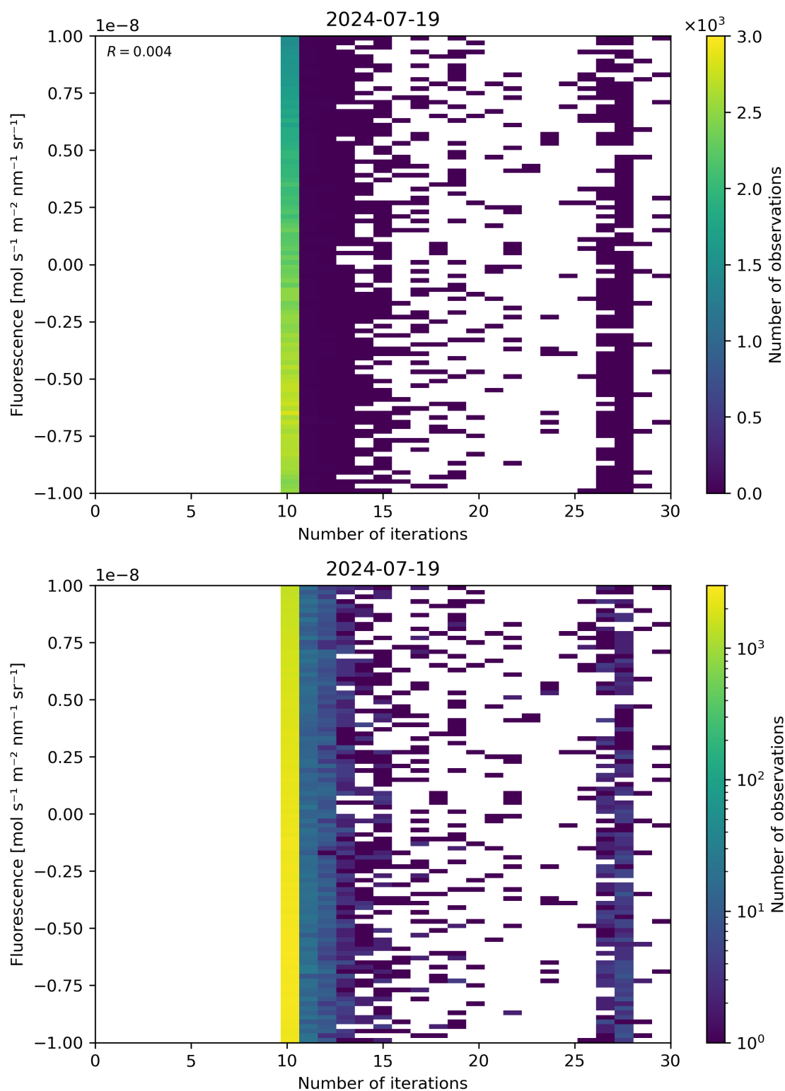
Figure 87: Scatter density plot of “Number of iterations” against “Fluorescence” for 2024-07-18 to 2024-07-20.
