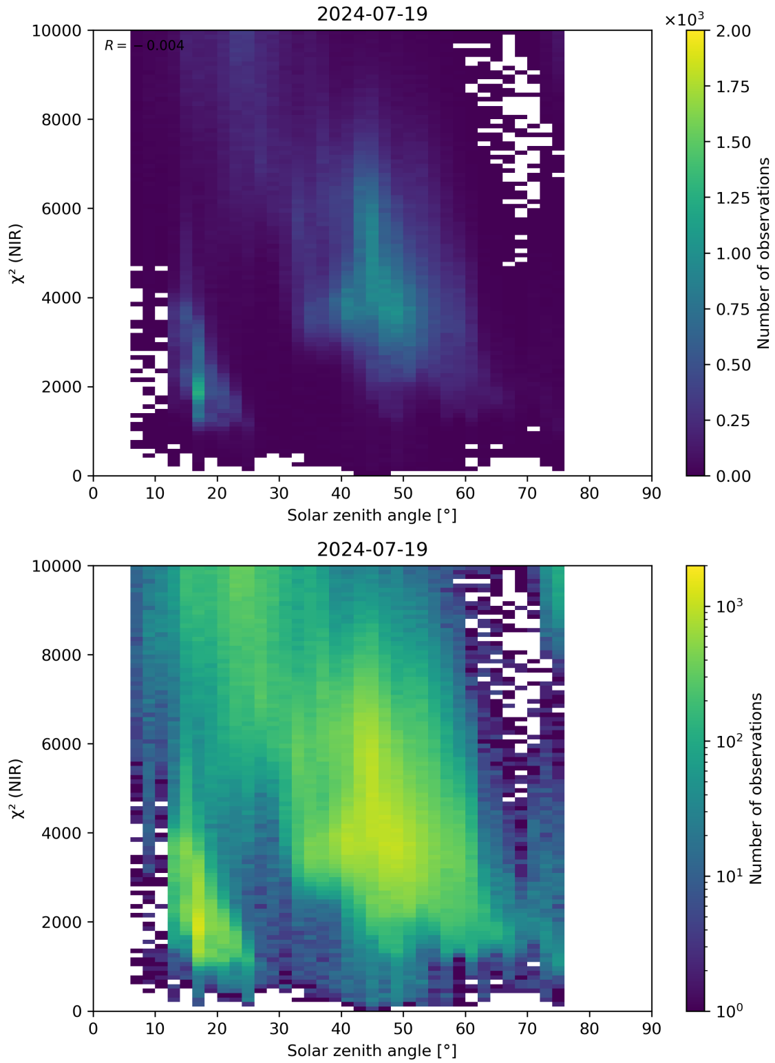
Figure 94: Scatter density plot of “Solar zenith angle” against “ \chi^2 (NIR)” for 2024-07-18 to 2024-07-20.
