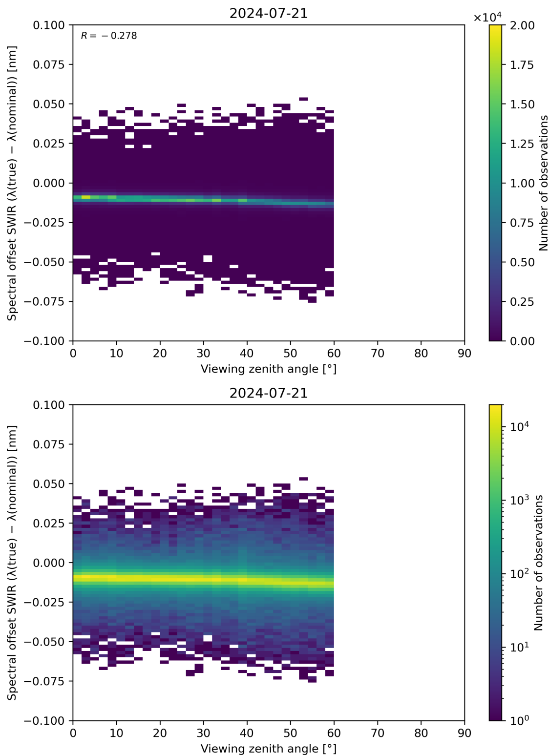
Figure 116: Scatter density plot of “Viewing zenith angle” against “Spectral offset SWIR ( \lambda(\text{true}) - \lambda(\text{nominal}) )” for 2024-07-21 to 2024-07-22.
