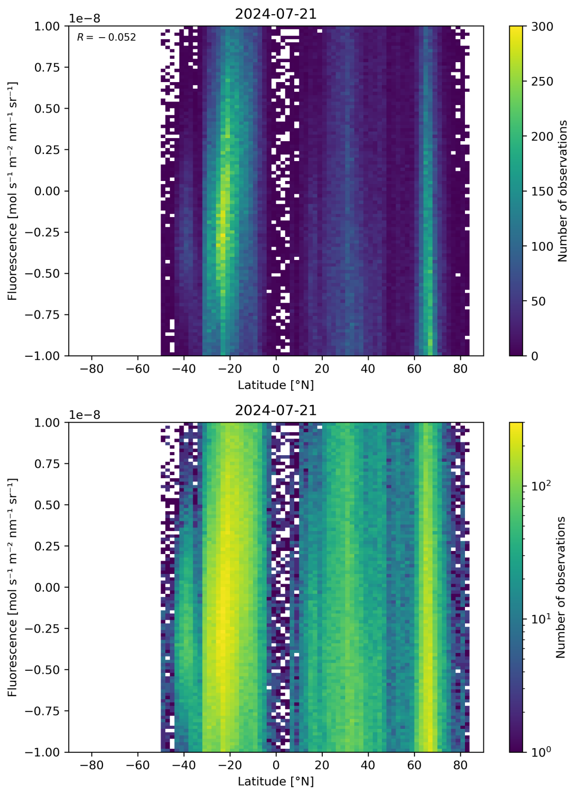
Figure 56: Scatter density plot of “Latitude” against “Fluorescence” for 2024-07-21 to 2024-07-22.
