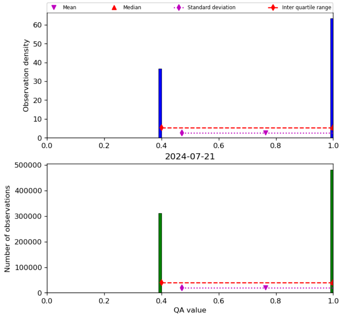
Figure 22: Histogram of “QA value” for 2024-07-21 to 2024-07-22
