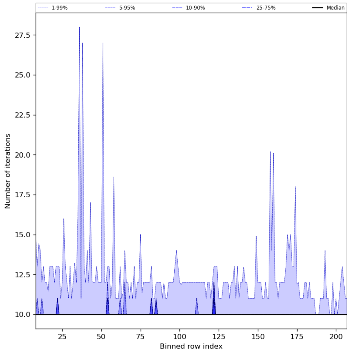
Figure 42: Along track statistics of “Number of iterations” for 2024-07-21 to 2024-07-22
