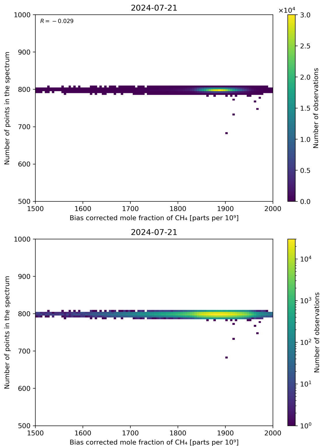
Figure 68: Scatter density plot of “Bias corrected mole fraction of CH 4 ” against “Number of points in the spectrum” for 2024-07-21 to 2024-07-22.
