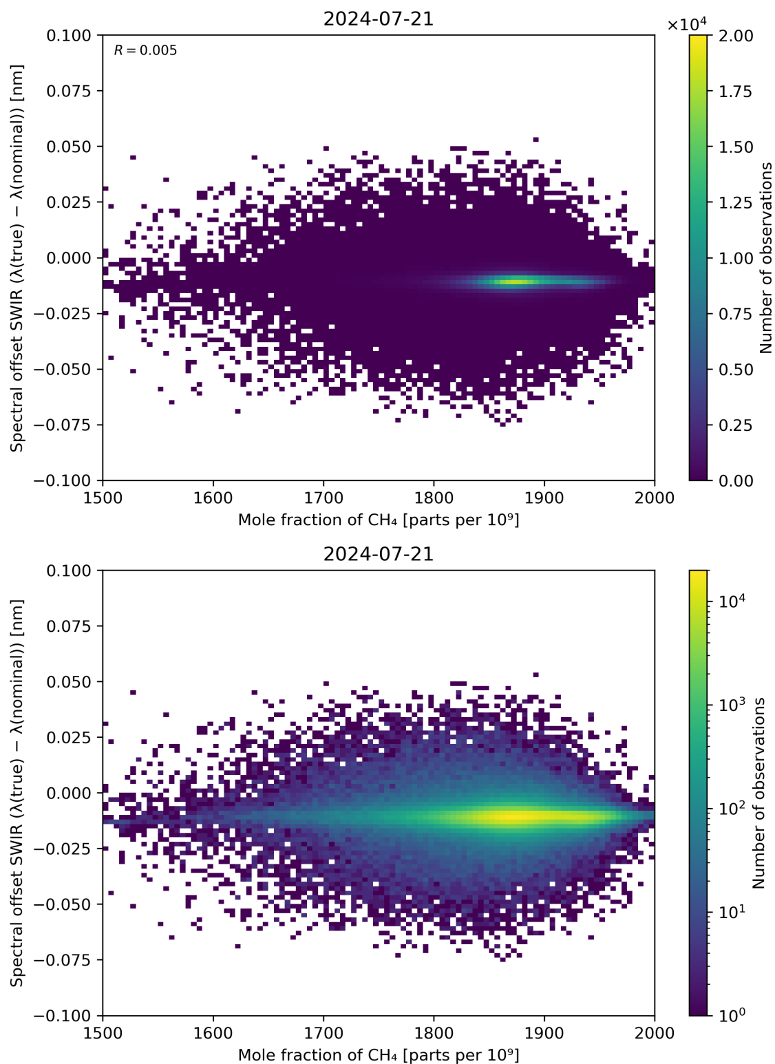
Figure 86: Scatter density plot of “Mole fraction of CH 4 ” against “Spectral offset SWIR ( \lambda(\text{true}) - \lambda(\text{nominal}) )” for 2024-07-21 to 2024-07-22.
