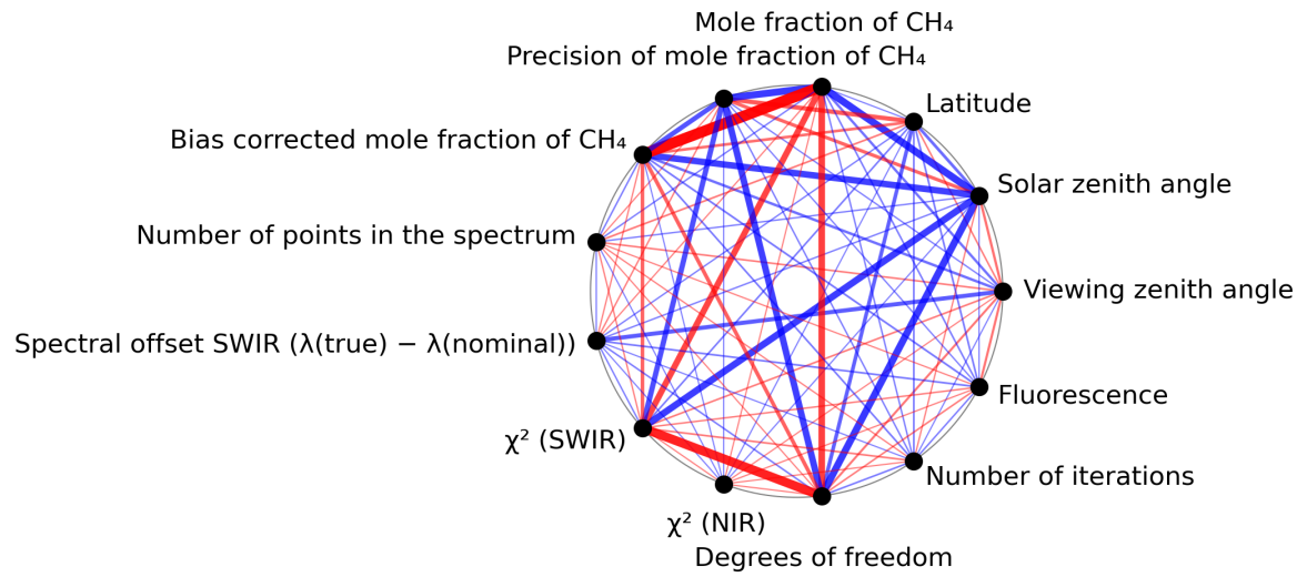
Figure 1: Map of correlation graph for 2024-07-21 to 2024-07-22.
