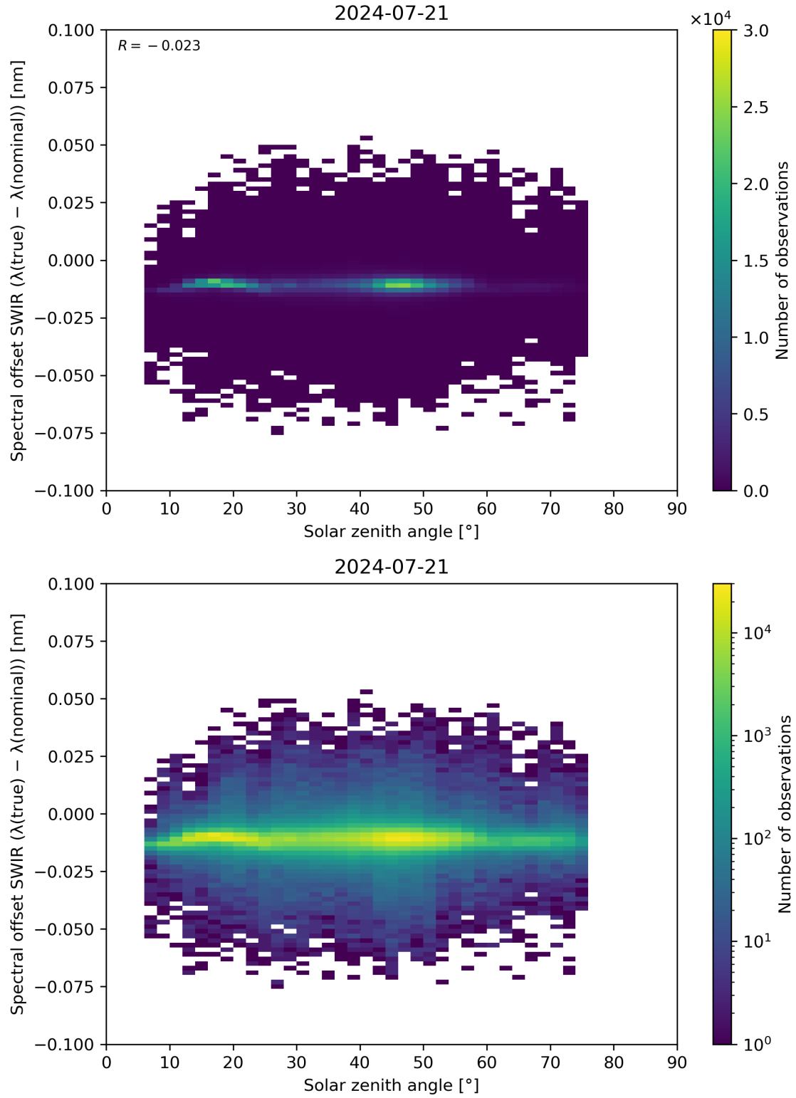
Figure 104: Scatter density plot of “Solar zenith angle” against “Spectral offset SWIR ( \lambda(\text{true}) - \lambda(\text{nominal}) )” for 2024-07-21 to 2024-07-22.
