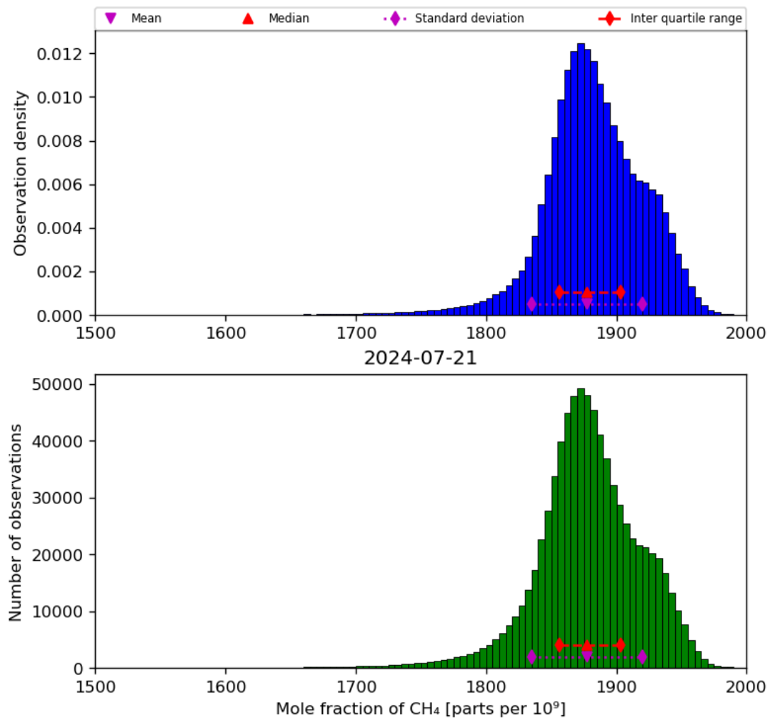
Figure 23: Histogram of “Mole fraction of CH 4 ” for 2024-07-21 to 2024-07-22
