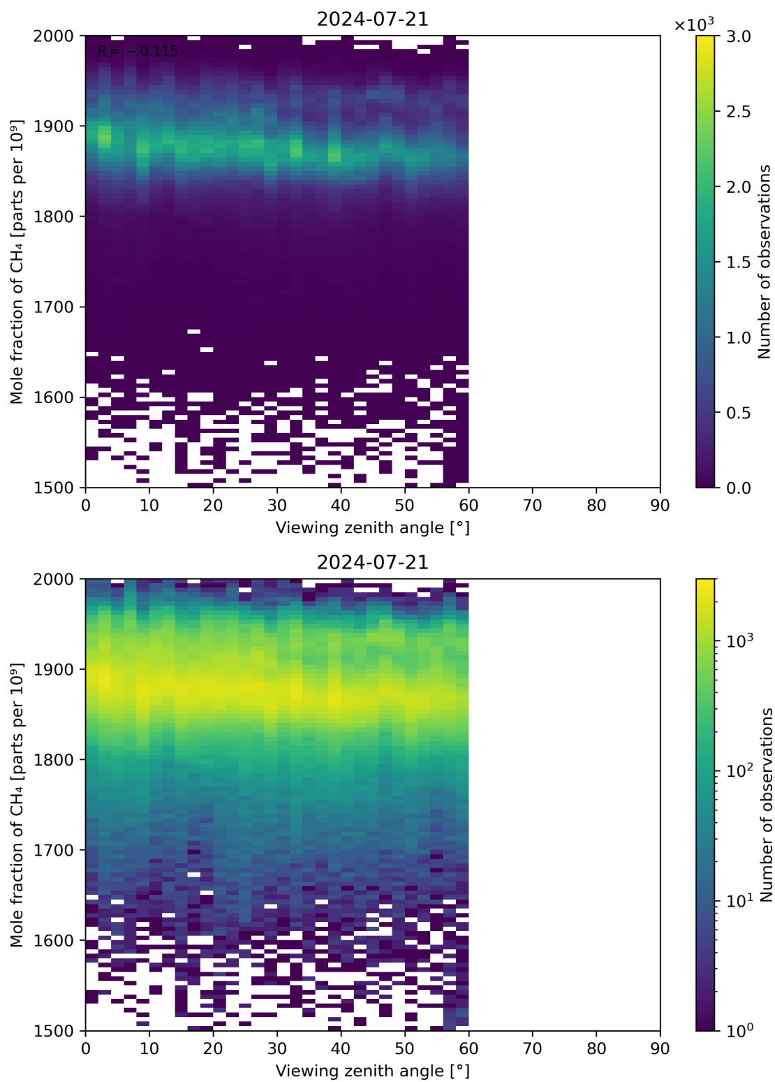
Figure 110: Scatter density plot of “Viewing zenith angle” against “Mole fraction of CH 4 ” for 2024-07-21 to 2024-07-22.
