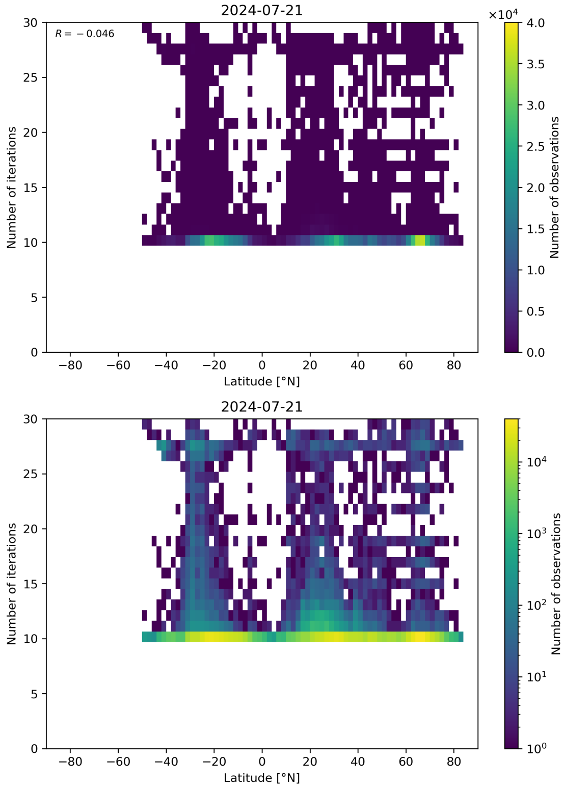
Figure 60: Scatter density plot of “Latitude” against “Number of iterations” for 2024-07-21 to 2024-07-22.
