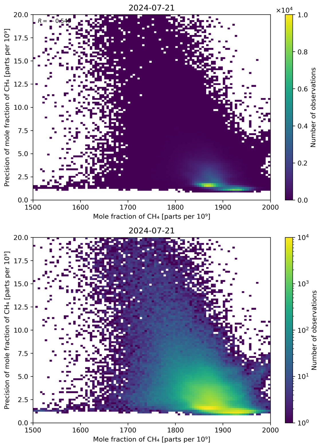
Figure 75: Scatter density plot of “Mole fraction of CH 4 ” against “Precision of mole fraction of CH 4 ” for 2024-07-21 to 2024-07-22.
