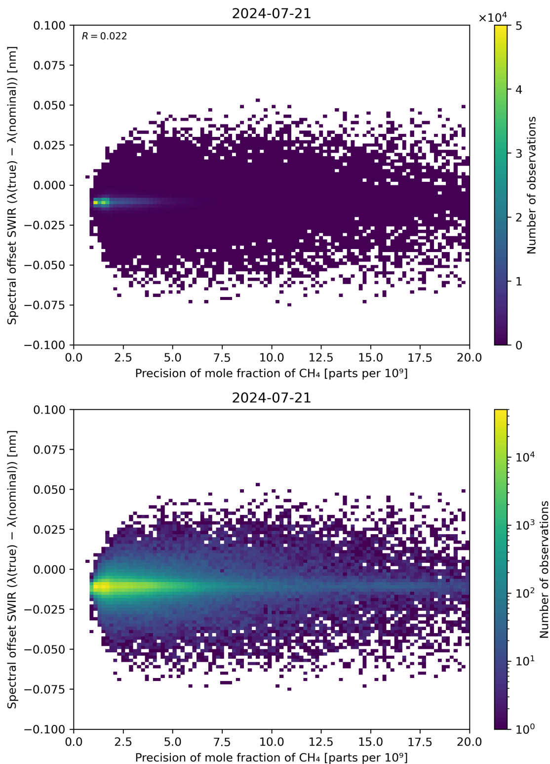
Figure 85: Scatter density plot of “Precision of mole fraction of \text{CH}_4 ” against “Spectral offset SWIR ( \lambda(\text{true}) - \lambda(\text{nominal}) )” for 2024-07-21 to 2024-07-22.
