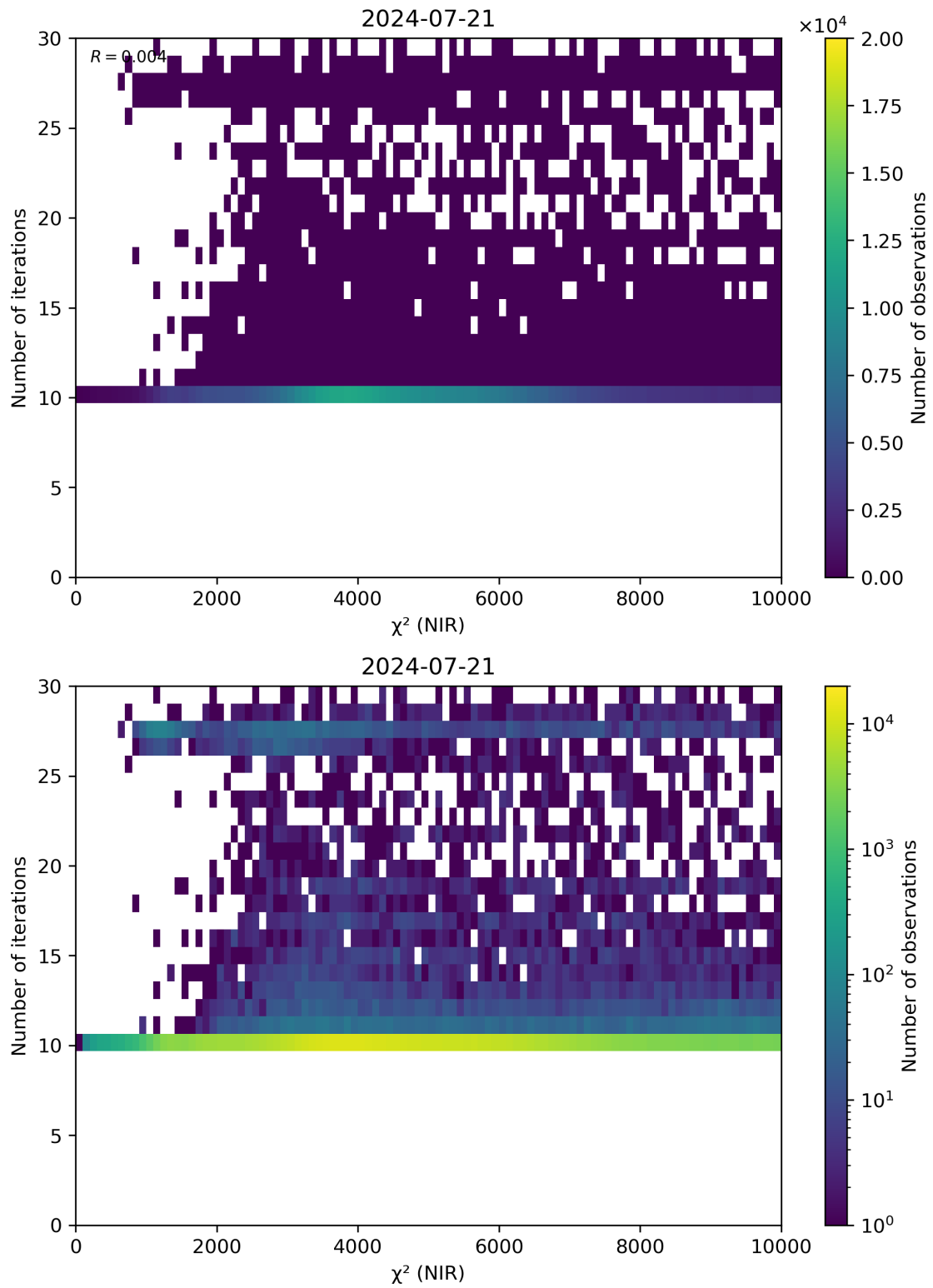
Figure 46: Scatter density plot of “ \chi^2 (NIR)” against “Number of iterations” for 2024-07-21 to 2024-07-22.
