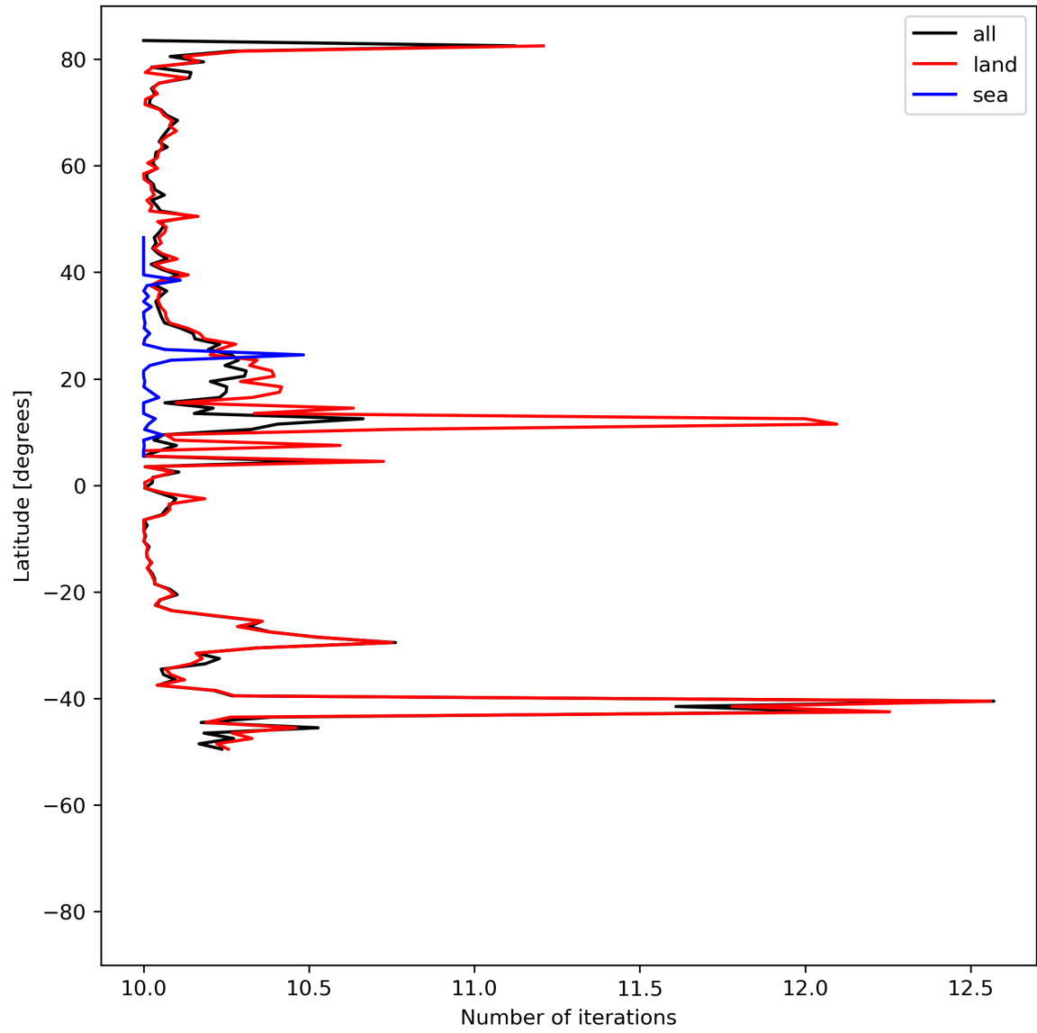
Figure 20: Zonal average of “Number of iterations” for 2024-07-21 to 2024-07-22.
