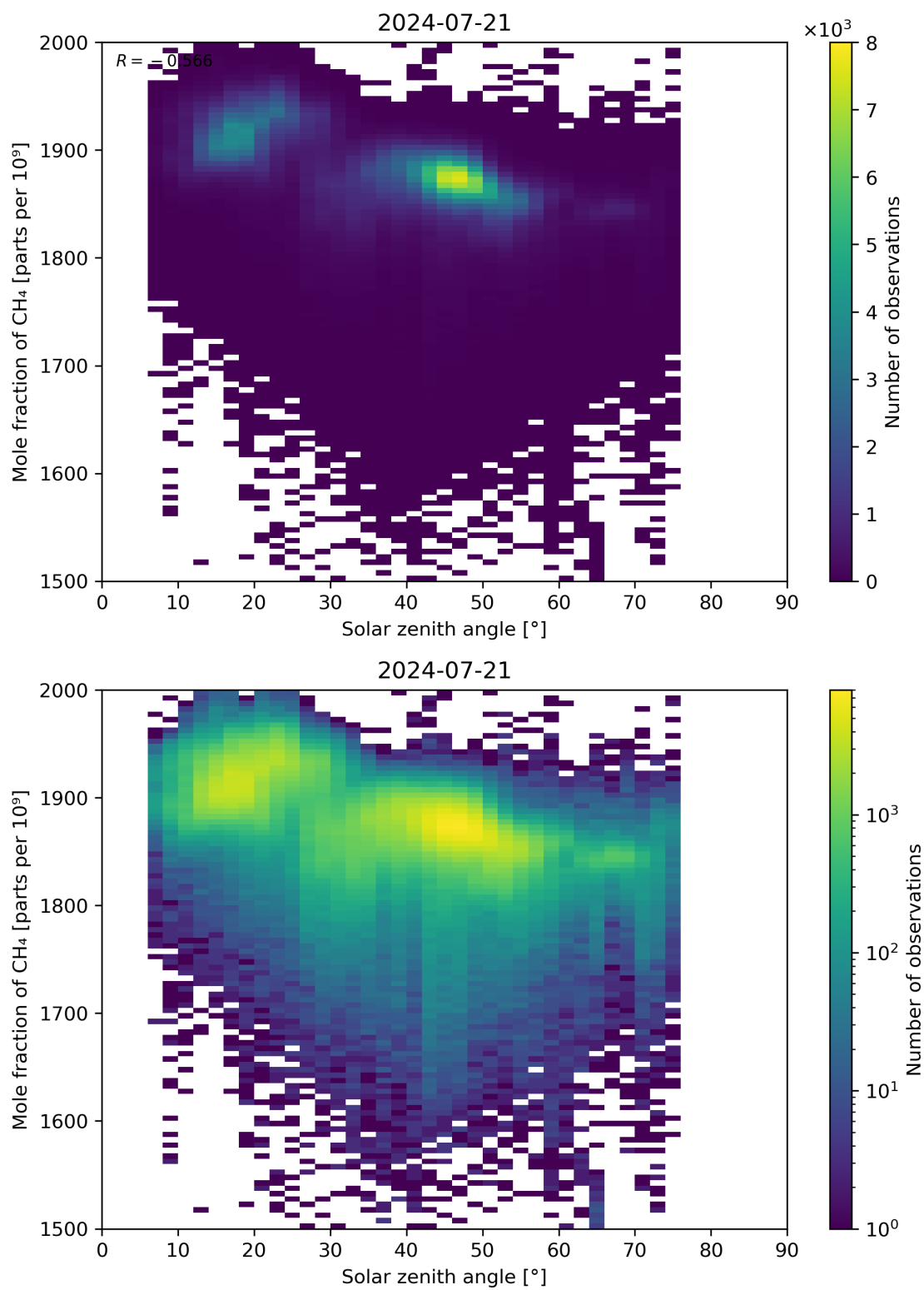
Figure 99: Scatter density plot of “Solar zenith angle” against “Mole fraction of CH 4 ” for 2024-07-21 to 2024-07-22.
