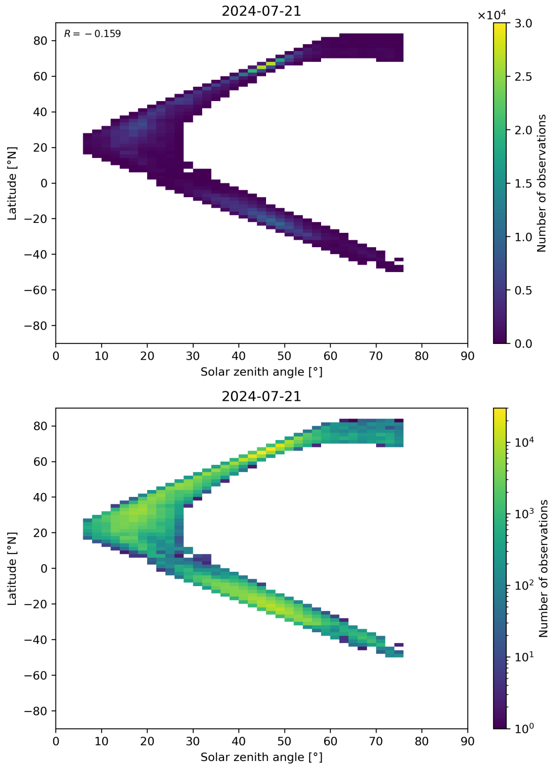
Figure 98: Scatter density plot of “Solar zenith angle” against “Latitude” for 2024-07-21 to 2024-07-22.
