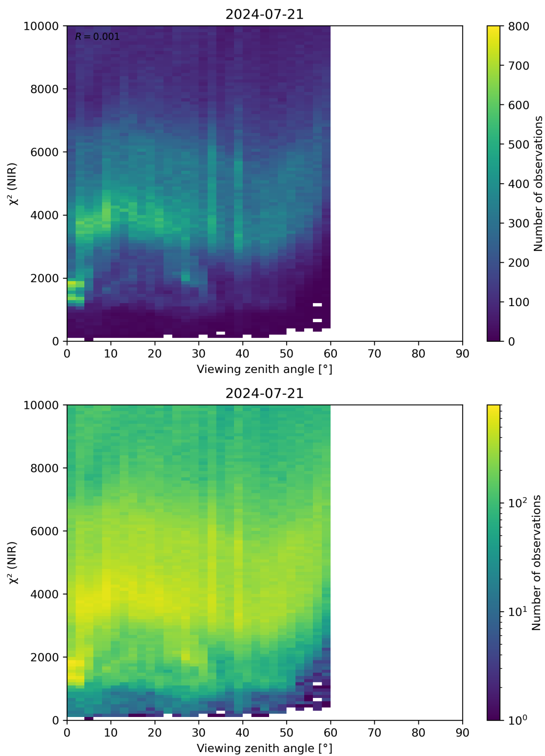
Figure 105: Scatter density plot of “Viewing zenith angle” against “ \chi^2 (NIR)” for 2024-07-21 to 2024-07-22.
