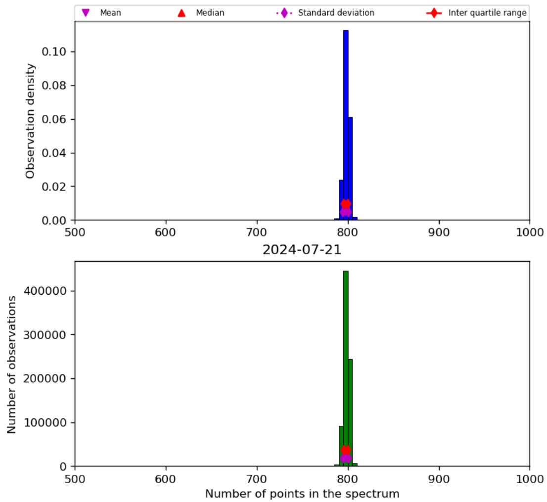
Figure 26: Histogram of “Number of points in the spectrum” for 2024-07-21 to 2024-07-22
