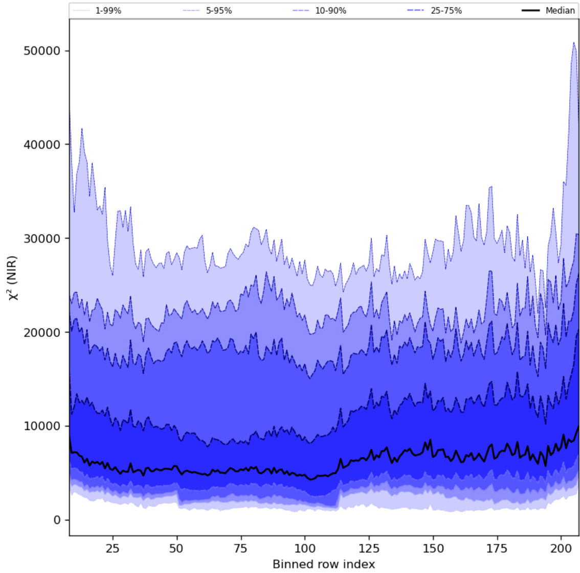
Figure 40: Along track statistics of “ \chi^2 (NIR)” for 2024-07-21 to 2024-07-22
