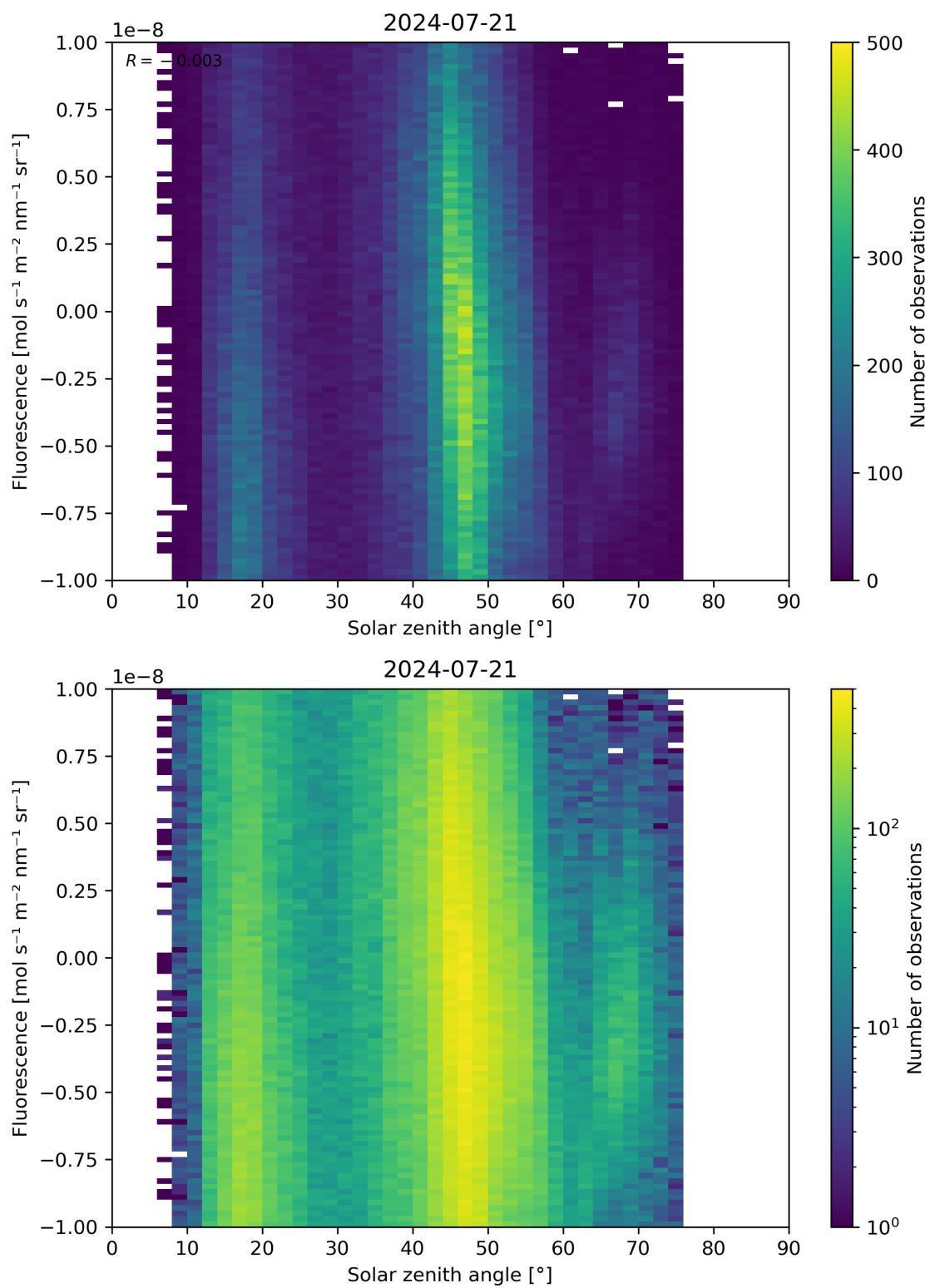
Figure 97: Scatter density plot of “Solar zenith angle” against “Fluorescence” for 2024-07-21 to 2024-07-22.
