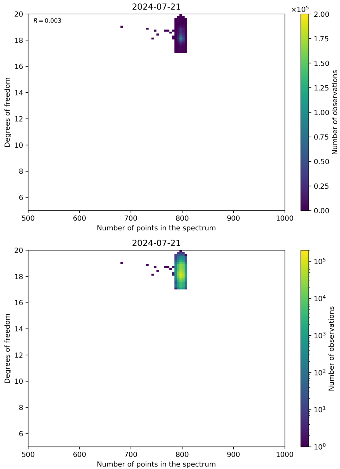
Figure 90: Scatter density plot of “Number of points in the spectrum” against “Degrees of freedom” for 2024-07-21 to 2024-07-22.
