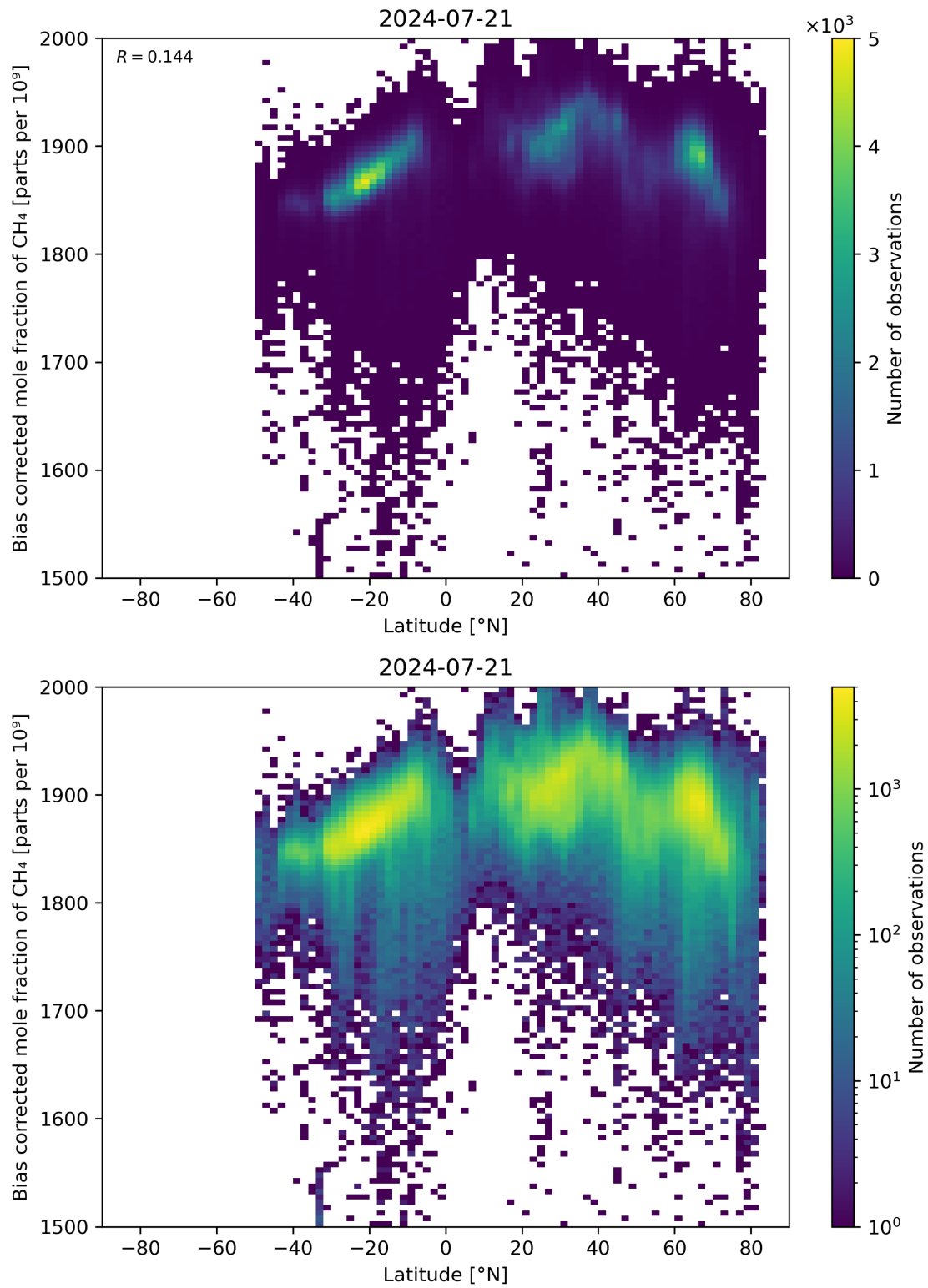
Figure 58: Scatter density plot of “Latitude” against “Bias corrected mole fraction of CH 4 ” for 2024-07-21 to 2024-07-22.
