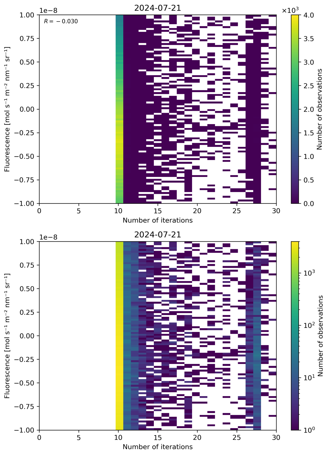
Figure 87: Scatter density plot of “Number of iterations” against “Fluorescence” for 2024-07-21 to 2024-07-22.
