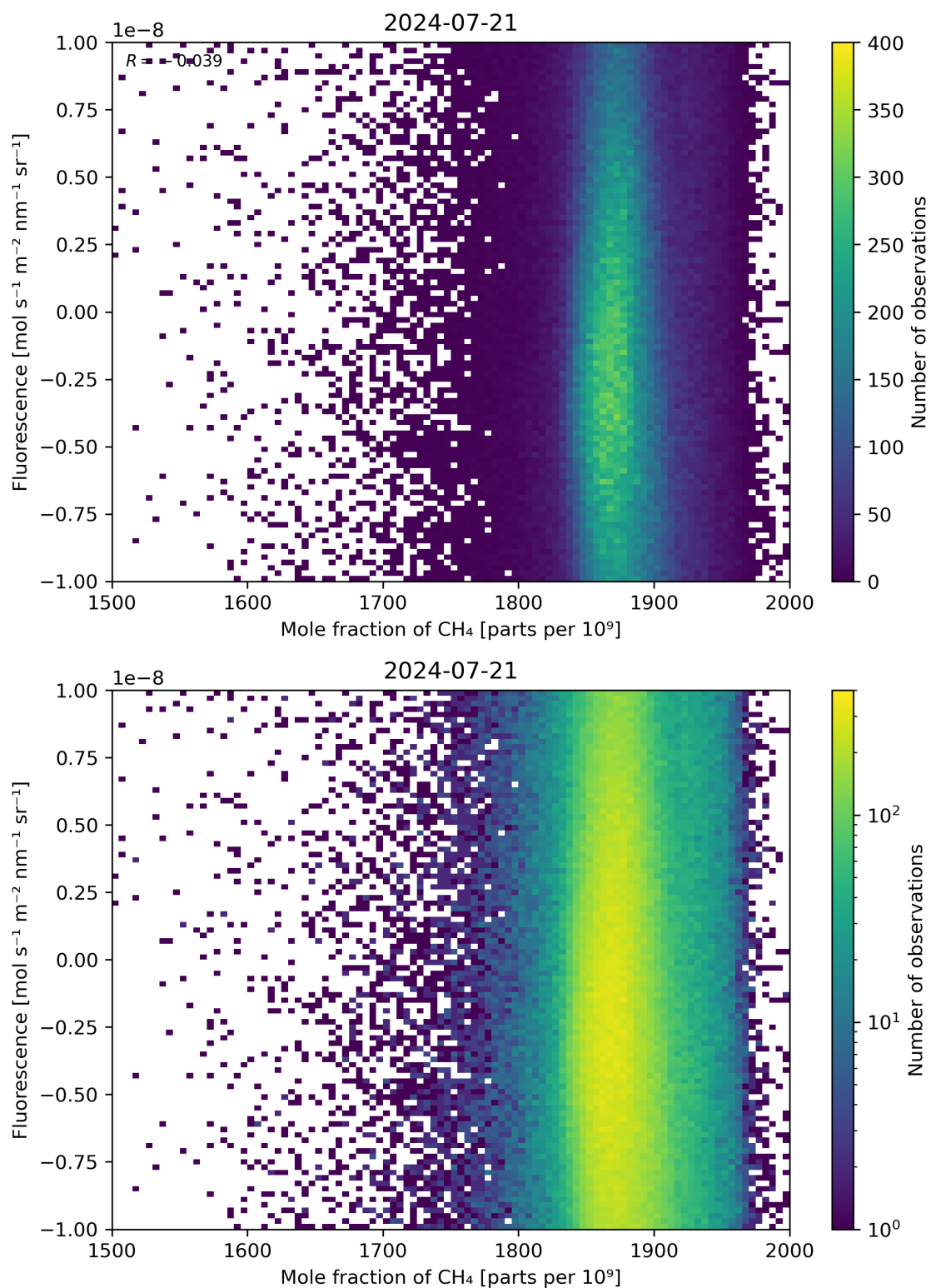
Figure 73: Scatter density plot of “Mole fraction of \text{CH}_4 ” against “Fluorescence” for 2024-07-21 to 2024-07-22.
