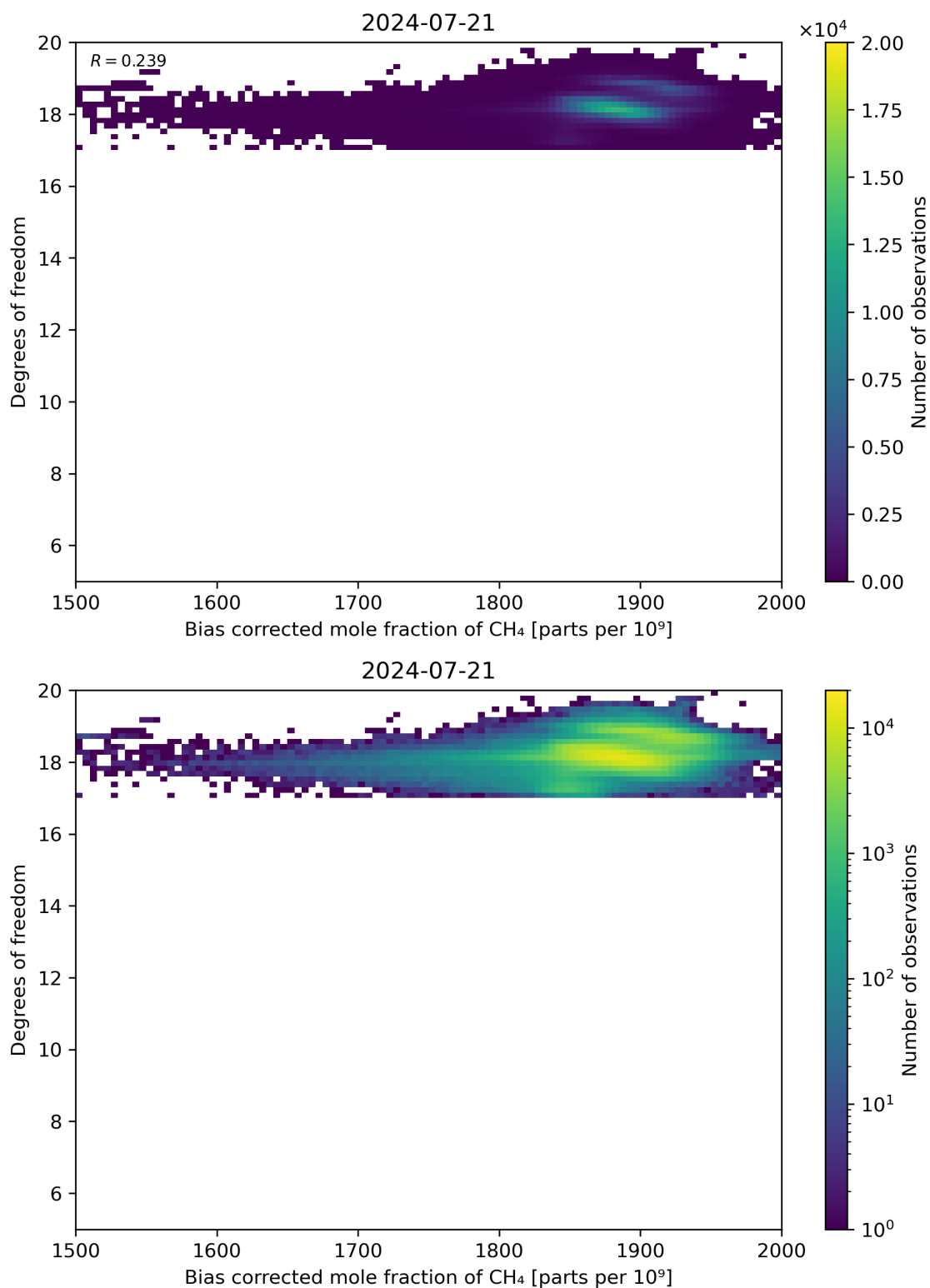
Figure 65: Scatter density plot of “Bias corrected mole fraction of CH 4 ” against “Degrees of freedom” for 2024-07-21 to 2024-07-22.
