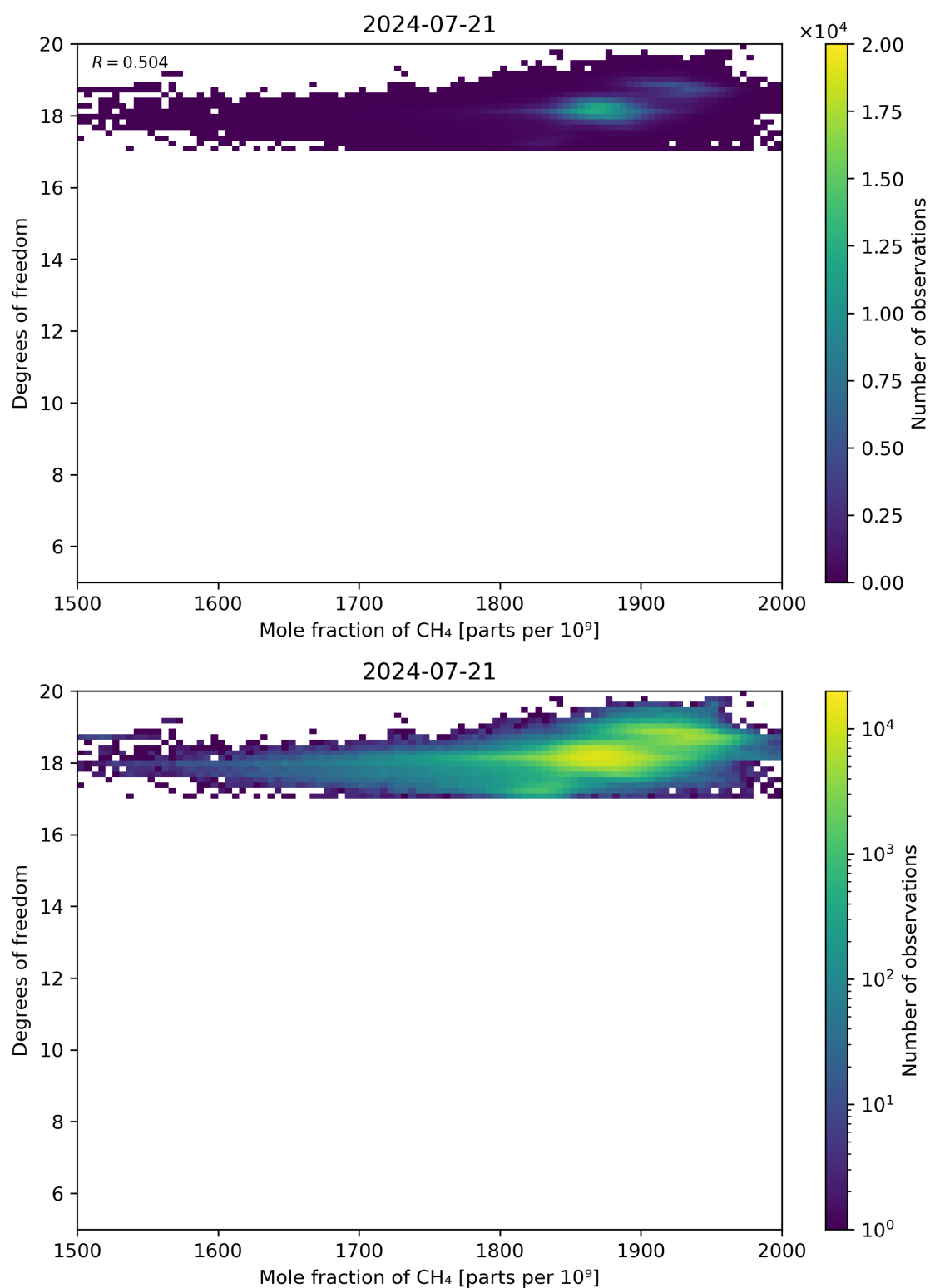
Figure 72: Scatter density plot of “Mole fraction of CH 4 ” against “Degrees of freedom” for 2024-07-21 to 2024-07-22.
