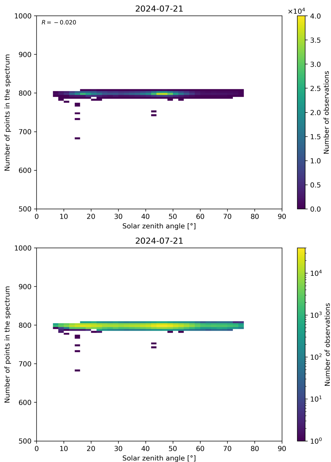
Figure 103: Scatter density plot of “Solar zenith angle” against “Number of points in the spectrum” for 2024-07-21 to 2024-07-22.
