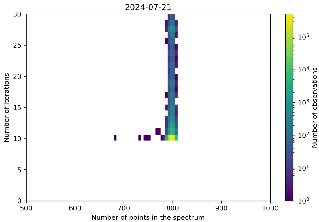
Figure 92: Scatter density plot of “Number of points in the spectrum” against “Number of iterations” for 2024-07-21 to 2024-07-22.
