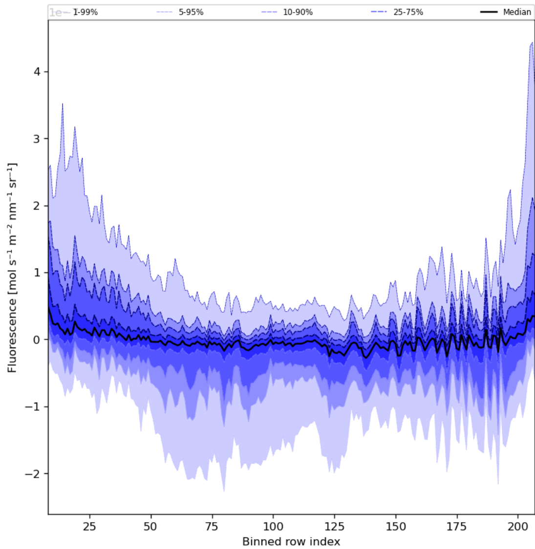
Figure 43: Along track statistics of “Fluorescence” for 2024-07-21 to 2024-07-22
