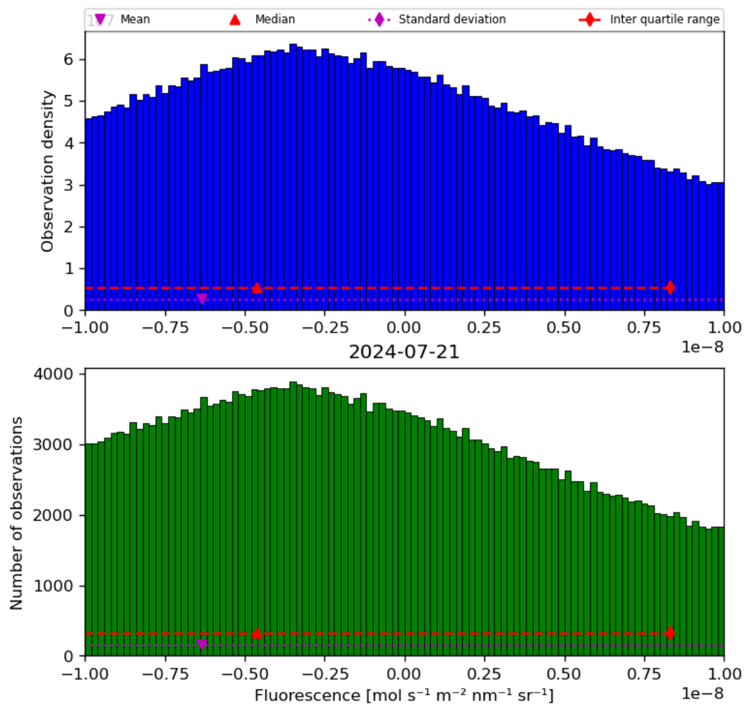
Figure 32: Histogram of “Fluorescence” for 2024-07-21 to 2024-07-22
