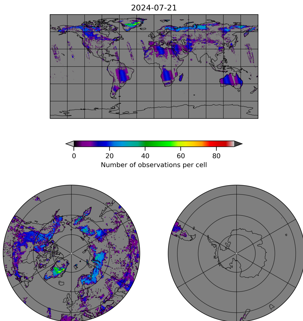
Figure 10: Map of the number of observations for 2024-07-21 to 2024-07-22
