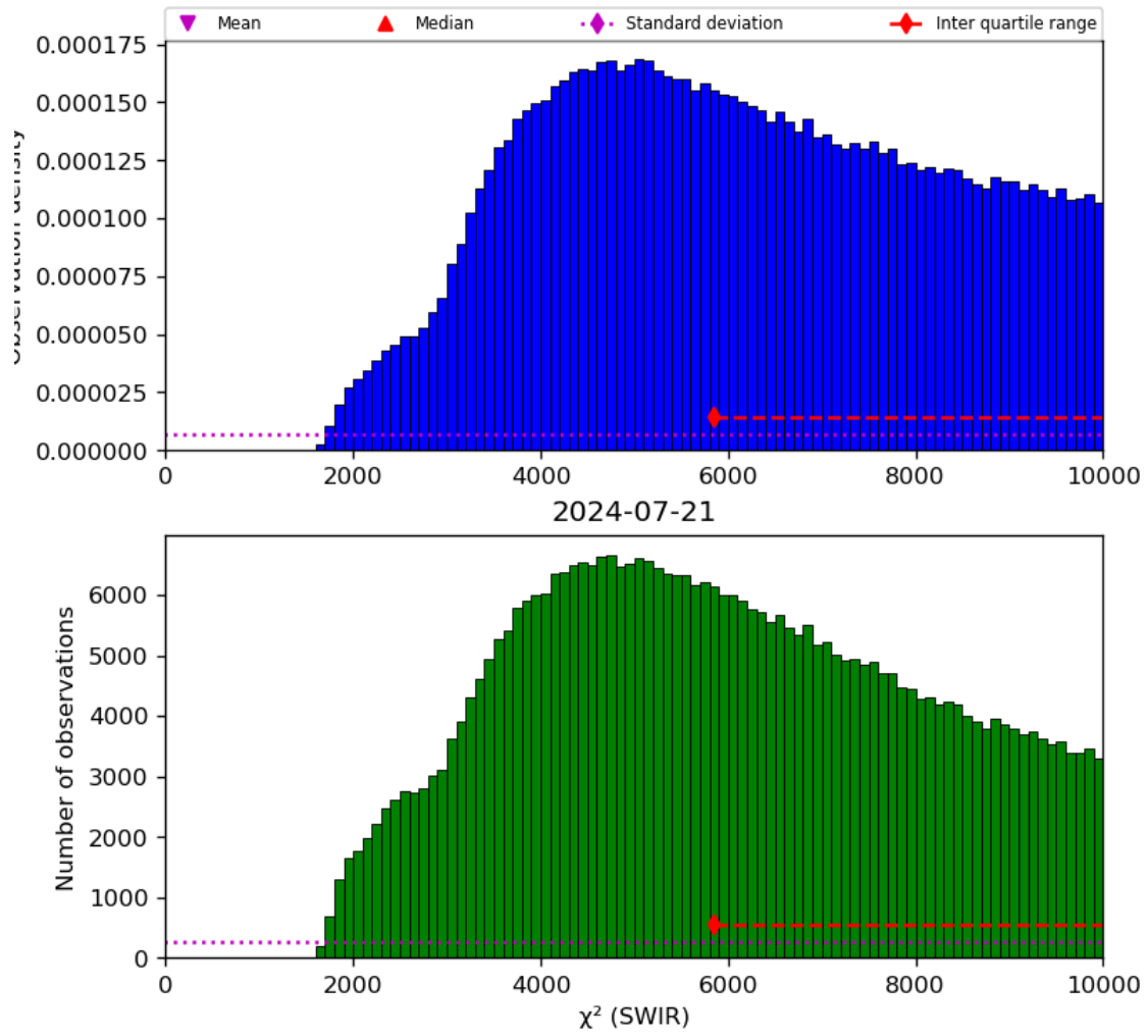
Figure 28: Histogram of “ \chi^2 (SWIR)” for 2024-07-21 to 2024-07-22
