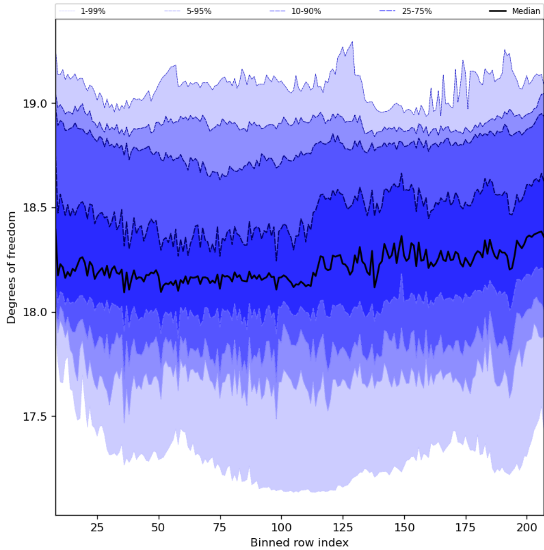
Figure 41: Along track statistics of “Degrees of freedom” for 2024-07-21 to 2024-07-22
