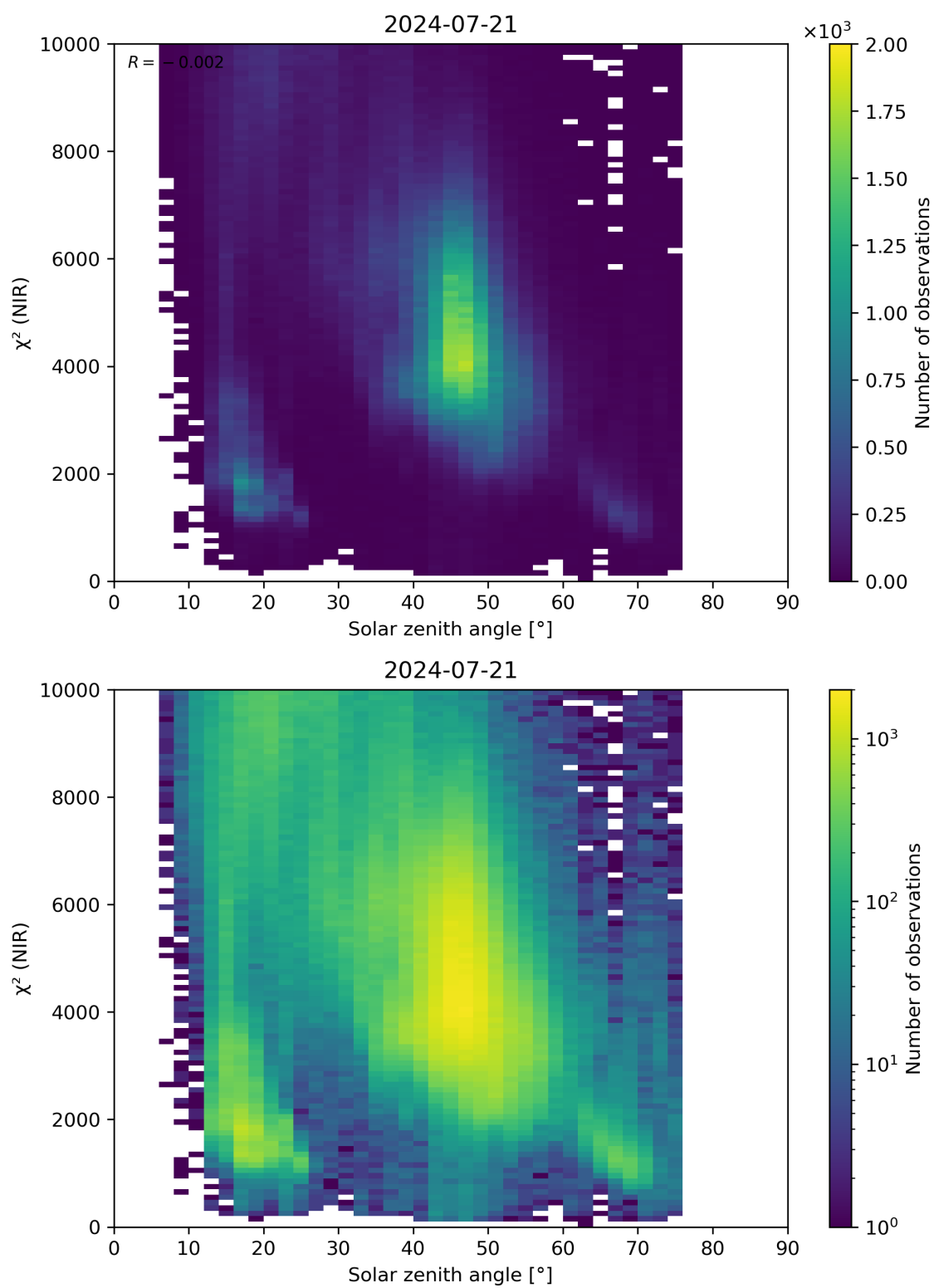
Figure 94: Scatter density plot of “Solar zenith angle” against “ \chi^2 (NIR)” for 2024-07-21 to 2024-07-22.
