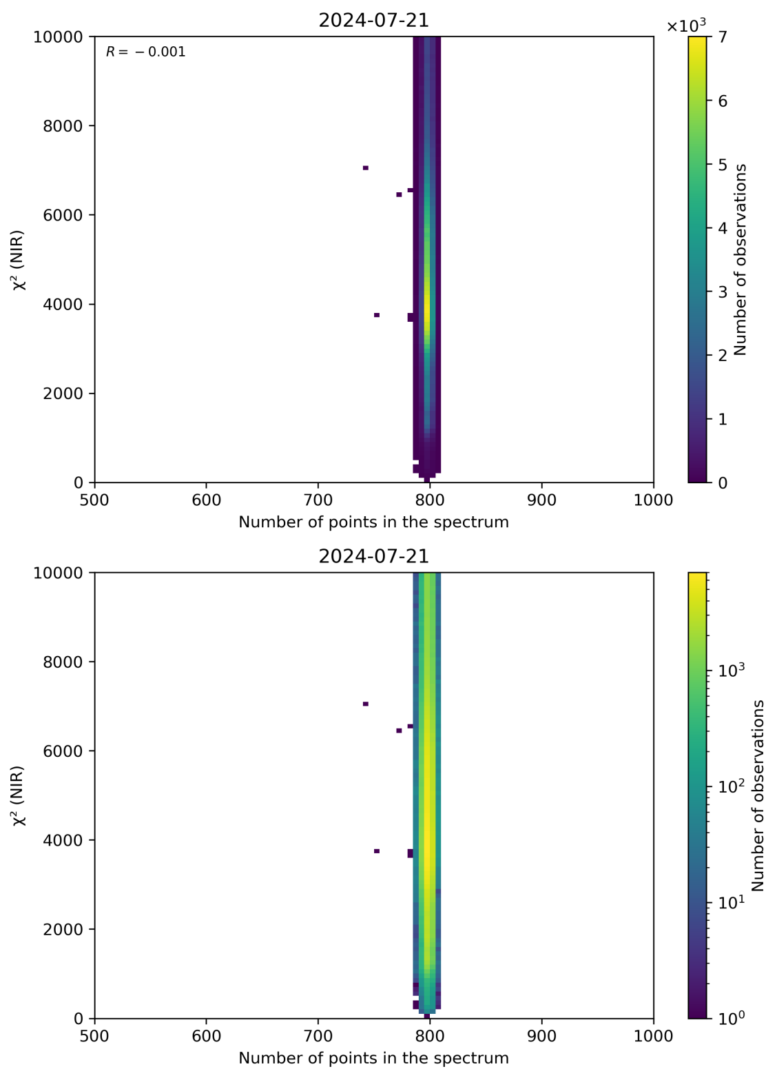
Figure 88: Scatter density plot of “Number of points in the spectrum” against “ \chi^2 (NIR)” for 2024-07-21 to 2024-07-22.
