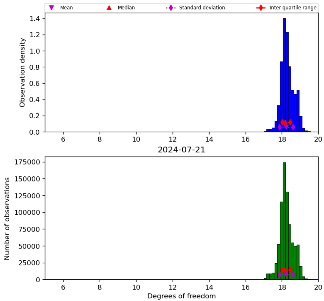
Figure 30: Histogram of “Degrees of freedom” for 2024-07-21 to 2024-07-22
