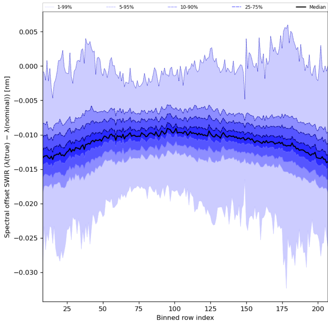
Figure 38: Along track statistics of “Spectral offset SWIR ( \lambda(\text{true}) - \lambda(\text{nominal}) )” for 2024-07-21 to 2024-07-22
