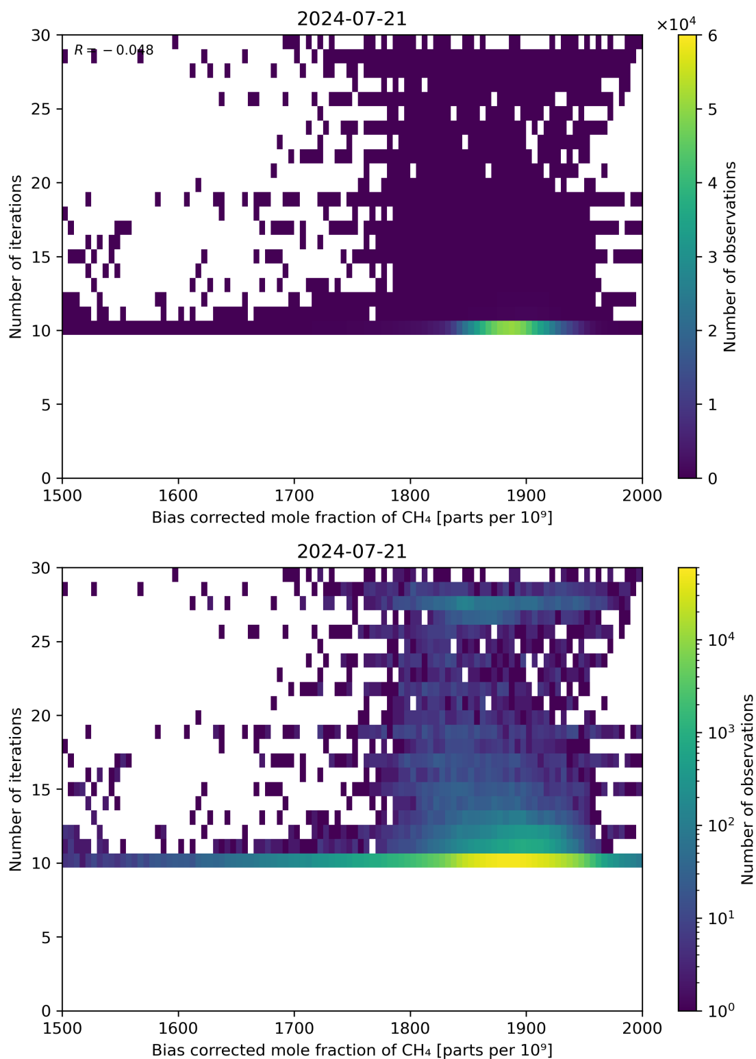
Figure 67: Scatter density plot of “Bias corrected mole fraction of CH 4 ” against “Number of iterations” for 2024-07-21 to 2024-07-22.
