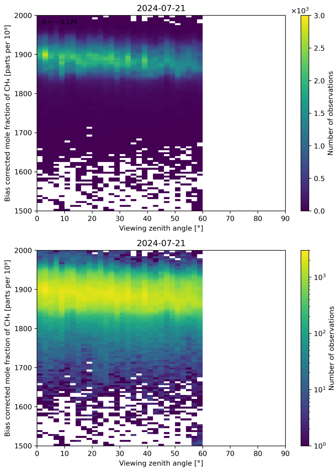
Figure 111: Scatter density plot of “Viewing zenith angle” against “Bias corrected mole fraction of CH 4 ” for 2024-07-21 to 2024-07-22.
