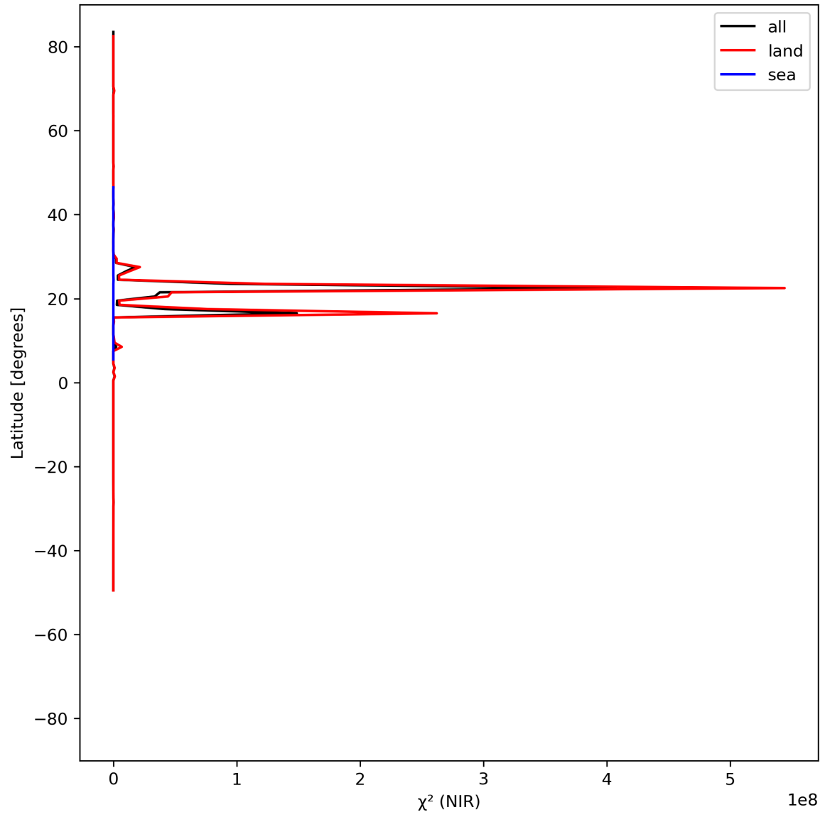
Figure 18: Zonal average of “ \chi^2 (NIR)” for 2024-07-21 to 2024-07-22.
