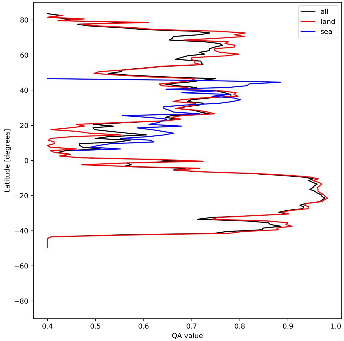
Figure 11: Zonal average of “QA value” for 2024-07-21 to 2024-07-22.
