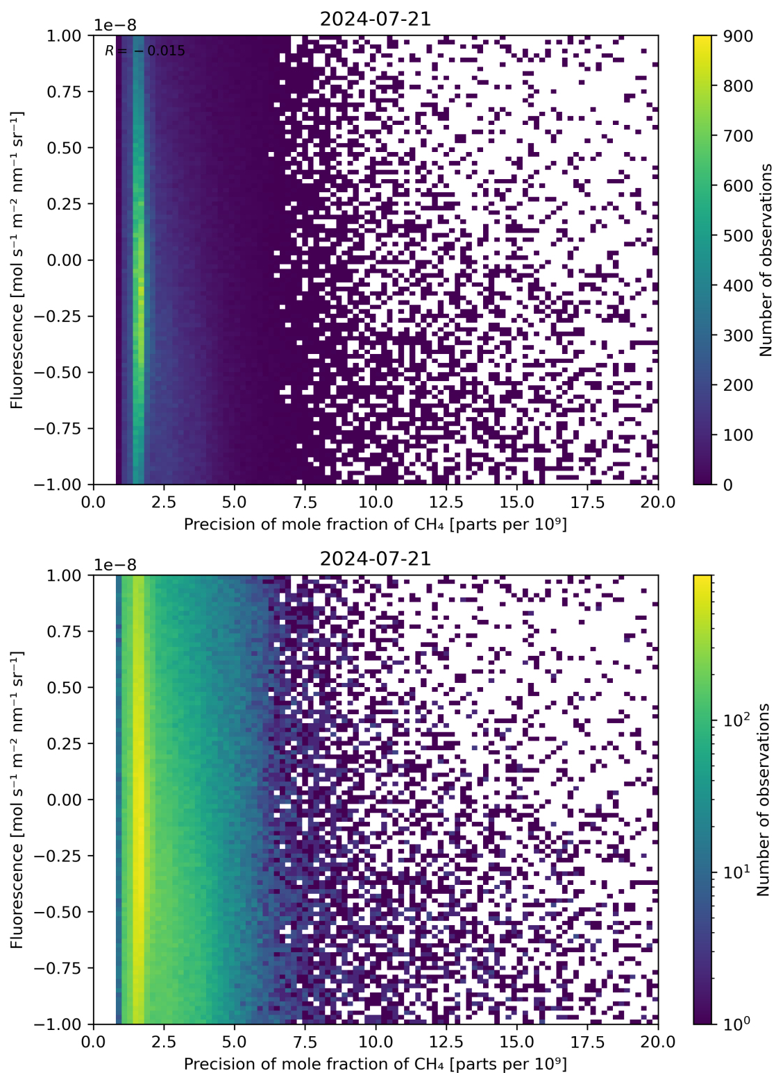
Figure 81: Scatter density plot of “Precision of mole fraction of \text{CH}_4 ” against “Fluorescence” for 2024-07-21 to 2024-07-22.
