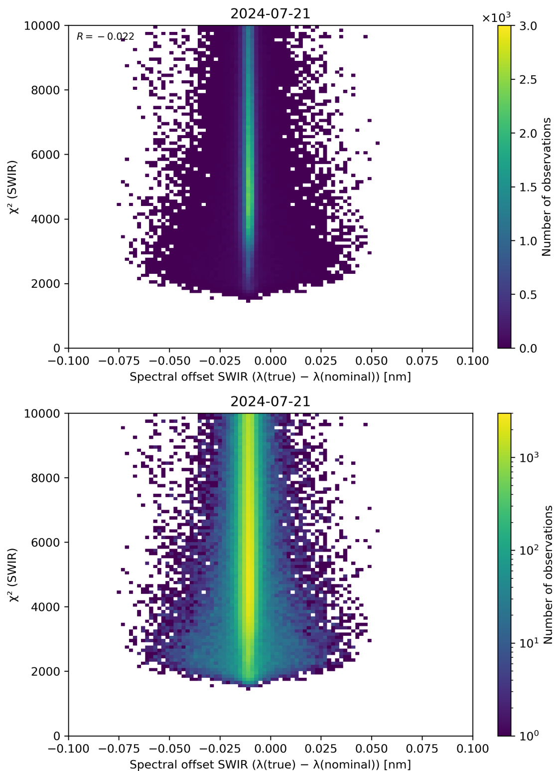
Figure 118: Scatter density plot of “Spectral offset SWIR ( \lambda(\text{true}) - \lambda(\text{nominal}) )” against “ \chi^2 (SWIR)” for 2024-07-21 to 2024-07-22.
