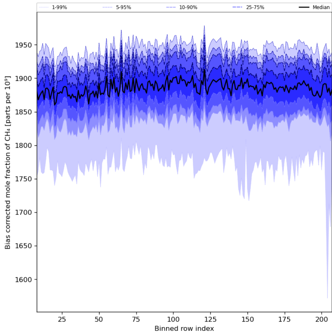
Figure 36: Along track statistics of “Bias corrected mole fraction of CH 4 ” for 2024-07-21 to 2024-07-22
