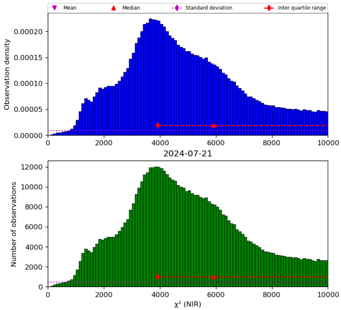
Figure 29: Histogram of “ \chi^2 (NIR)” for 2024-07-21 to 2024-07-22
