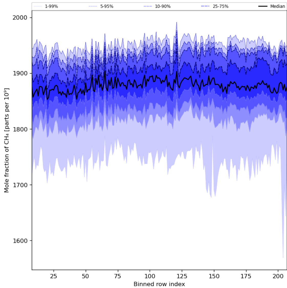
Figure 34: Along track statistics of “Mole fraction of CH 4 ” for 2024-07-21 to 2024-07-22
