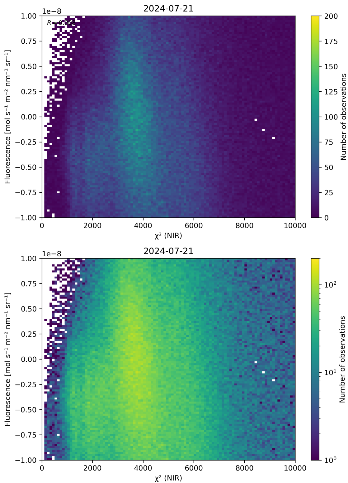
Figure 45: Scatter density plot of “ \chi^2 (NIR)” against “Fluorescence” for 2024-07-21 to 2024-07-22.
