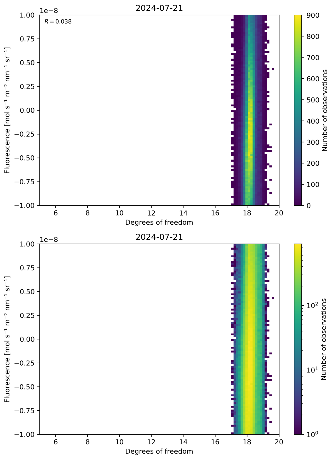
Figure 51: Scatter density plot of “Degrees of freedom” against “Fluorescence” for 2024-07-21 to 2024-07-22.
