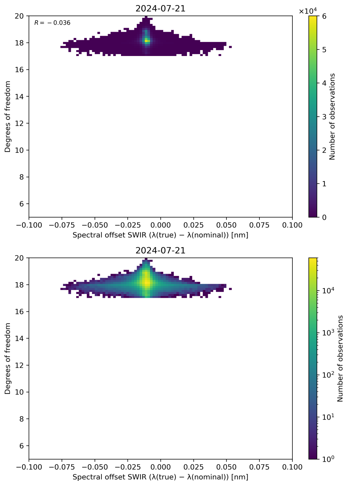
Figure 119: Scatter density plot of “Spectral offset SWIR ( \lambda(\text{true}) - \lambda(\text{nominal}) )” against “Degrees of freedom” for 2024-07-21 to 2024-07-22.
