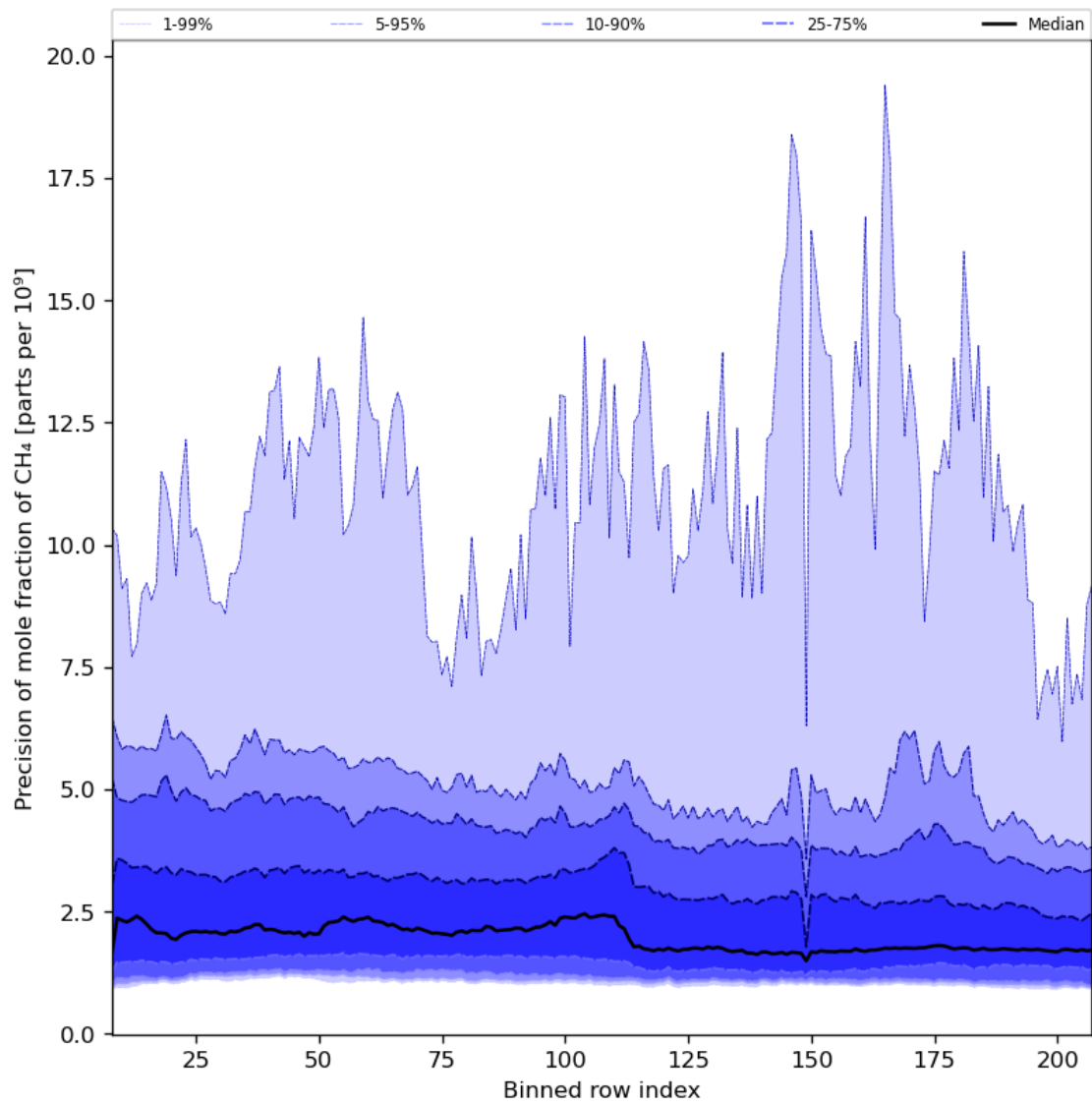
Figure 35: Along track statistics of “Precision of mole fraction of CH 4 ” for 2024-07-21 to 2024-07-22
