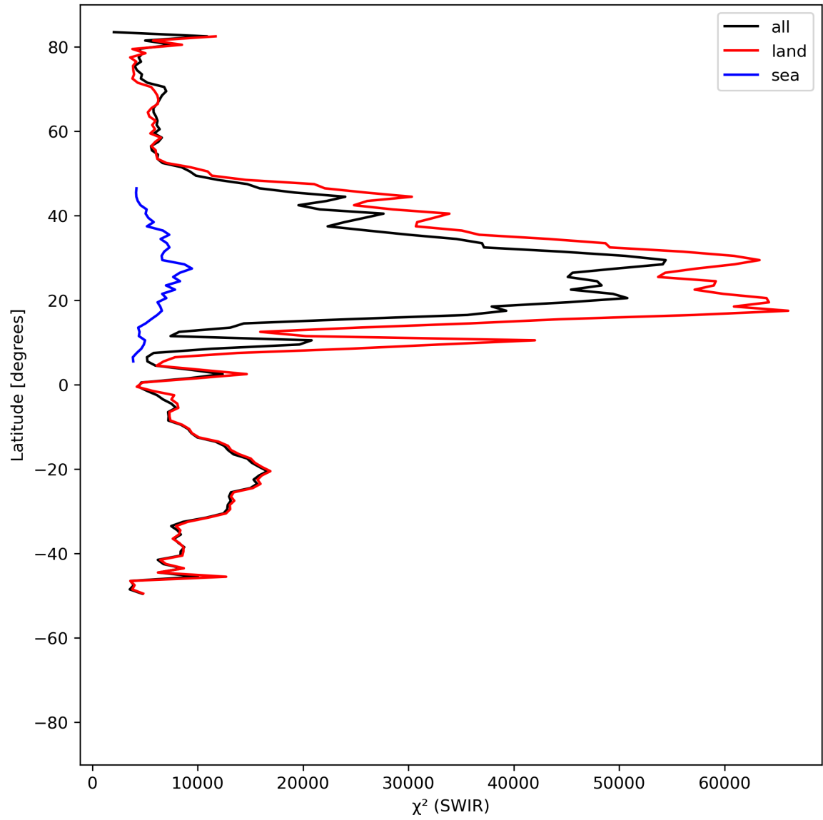
Figure 17: Zonal average of “ \chi^2 (SWIR)” for 2024-07-21 to 2024-07-22.
