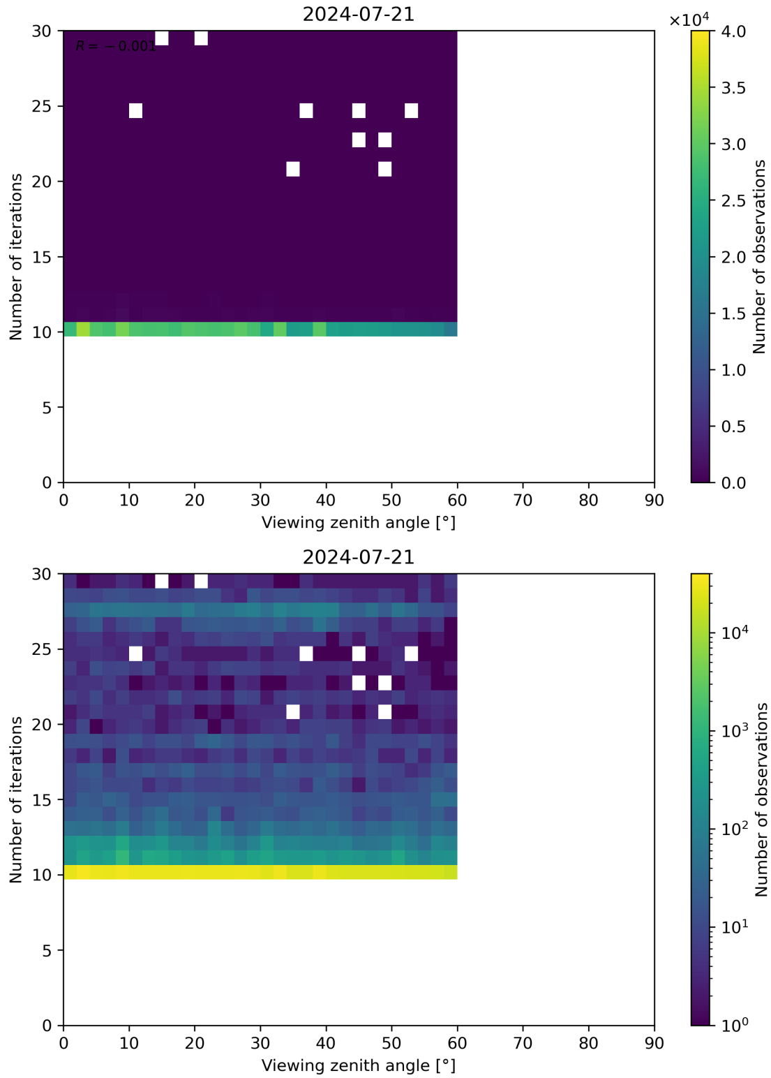
Figure 113: Scatter density plot of “Viewing zenith angle” against “Number of iterations” for 2024-07-21 to 2024-07-22.
