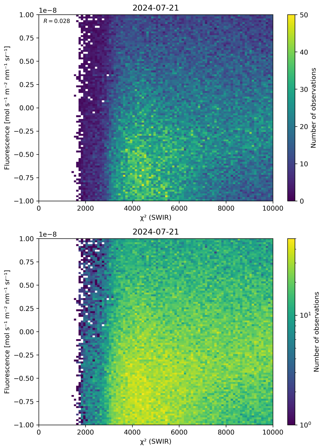
Figure 49: Scatter density plot of “ \chi^2 (SWIR)” against “Fluorescence” for 2024-07-21 to 2024-07-22.
