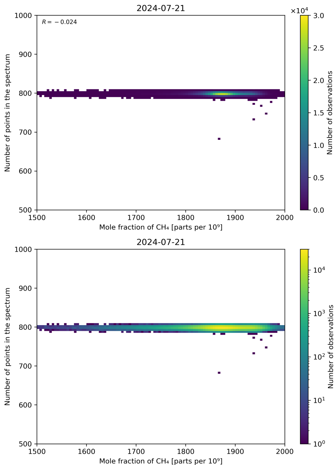
Figure 77: Scatter density plot of “Mole fraction of CH 4 ” against “Number of points in the spectrum” for 2024-07-21 to 2024-07-22.
