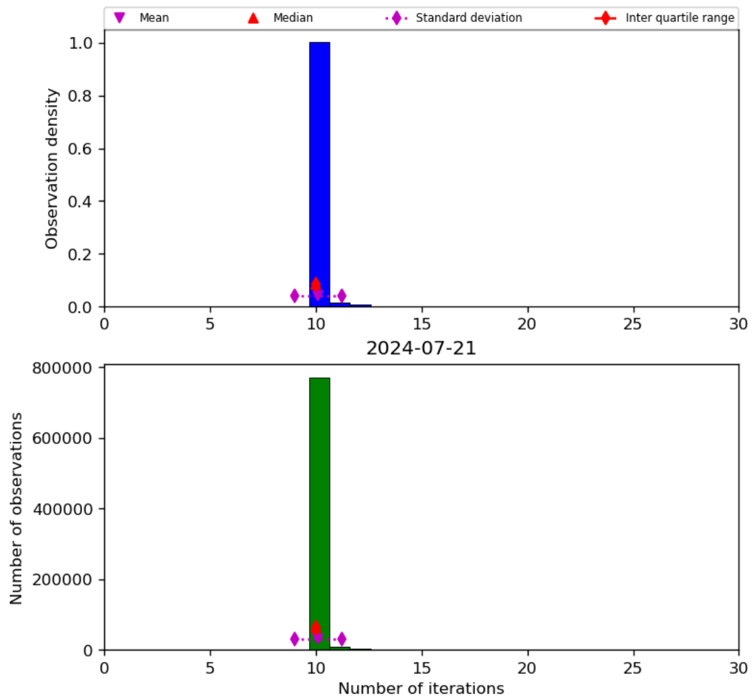
Figure 31: Histogram of “Number of iterations” for 2024-07-21 to 2024-07-22
