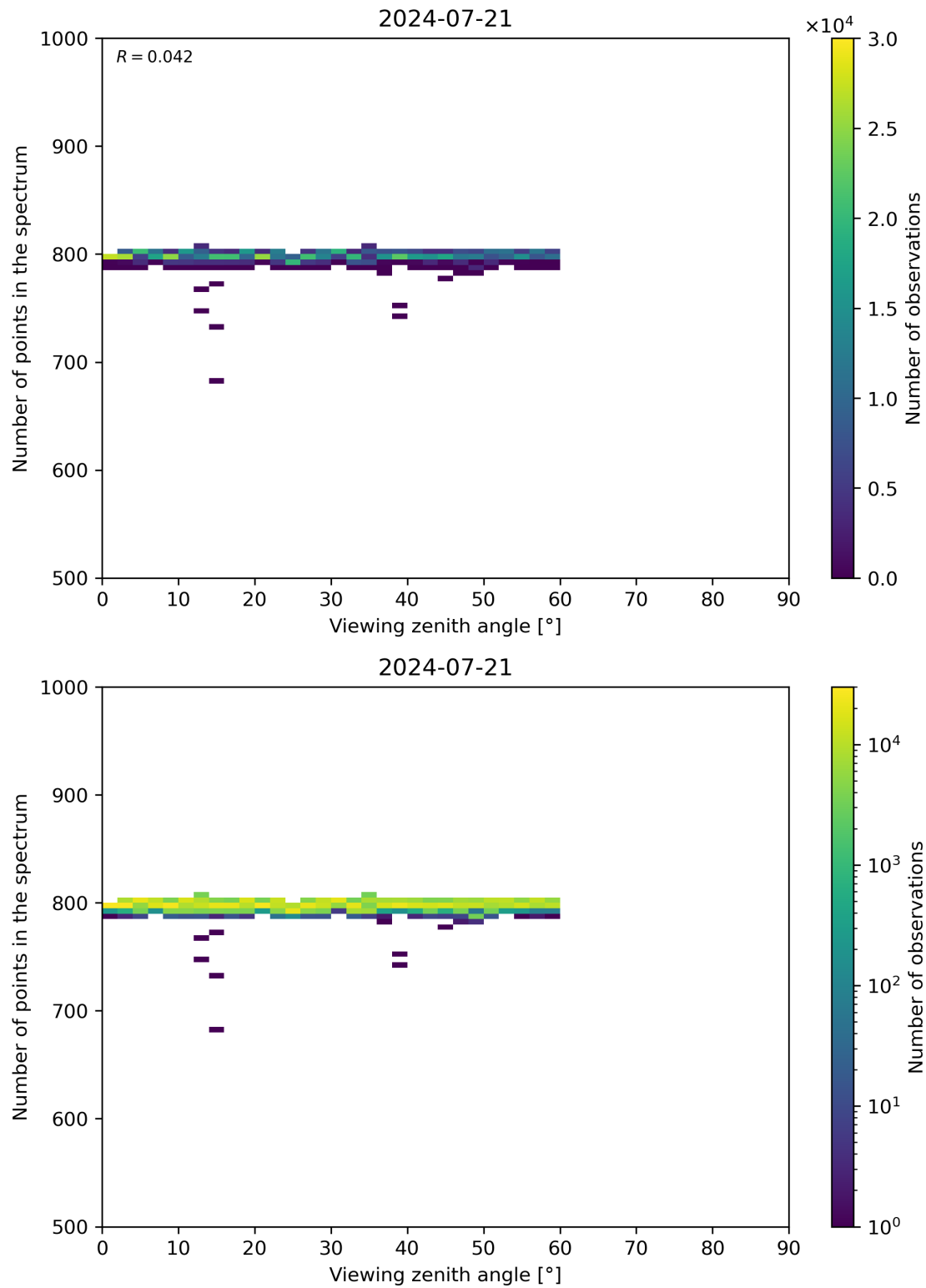
Figure 114: Scatter density plot of “Viewing zenith angle” against “Number of points in the spectrum” for 2024-07-21 to 2024-07-22.
