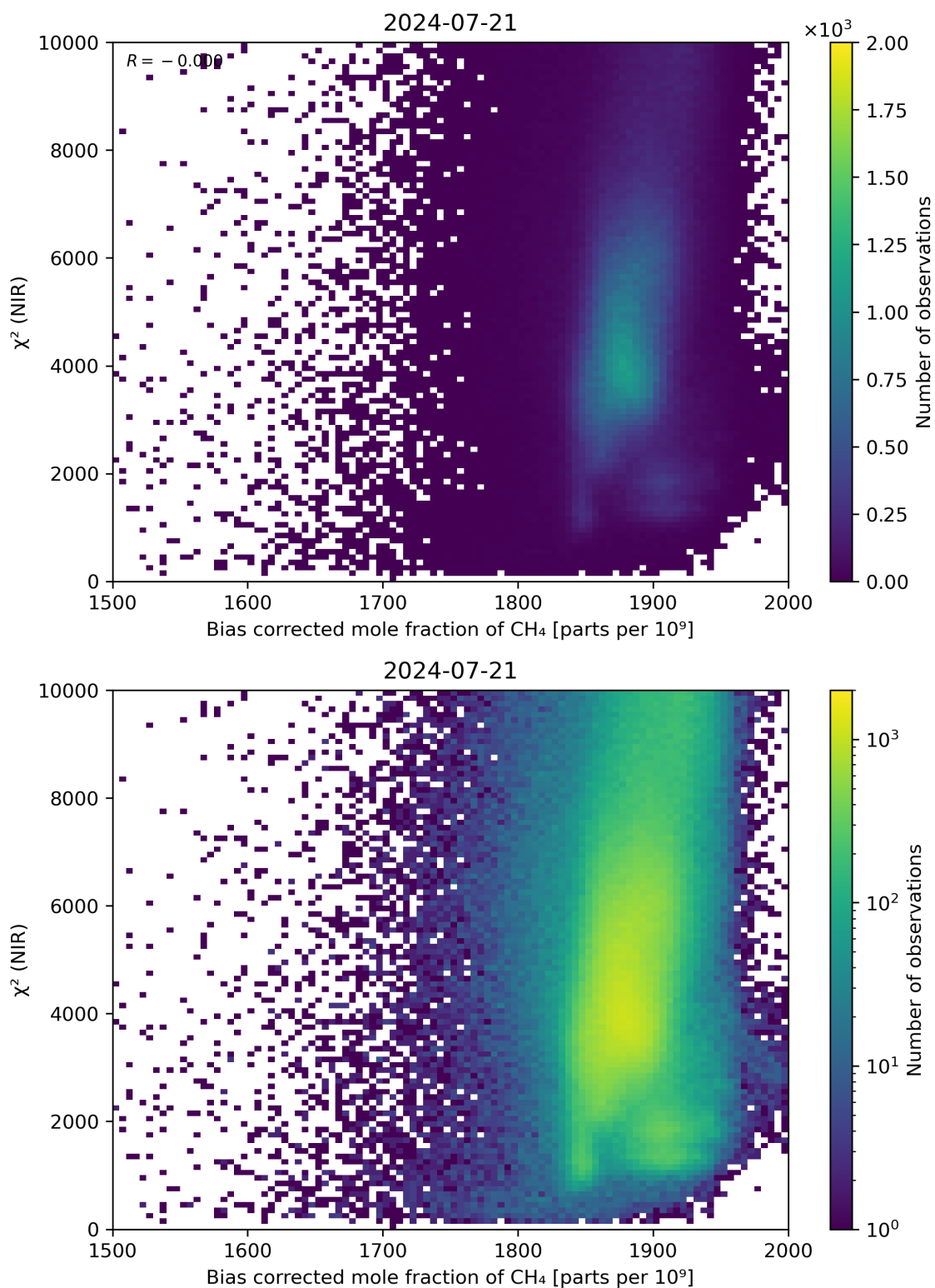
Figure 63: Scatter density plot of “Bias corrected mole fraction of \text{CH}_4 ” against “ \chi^2 (NIR)” for 2024-07-21 to 2024-07-22.
