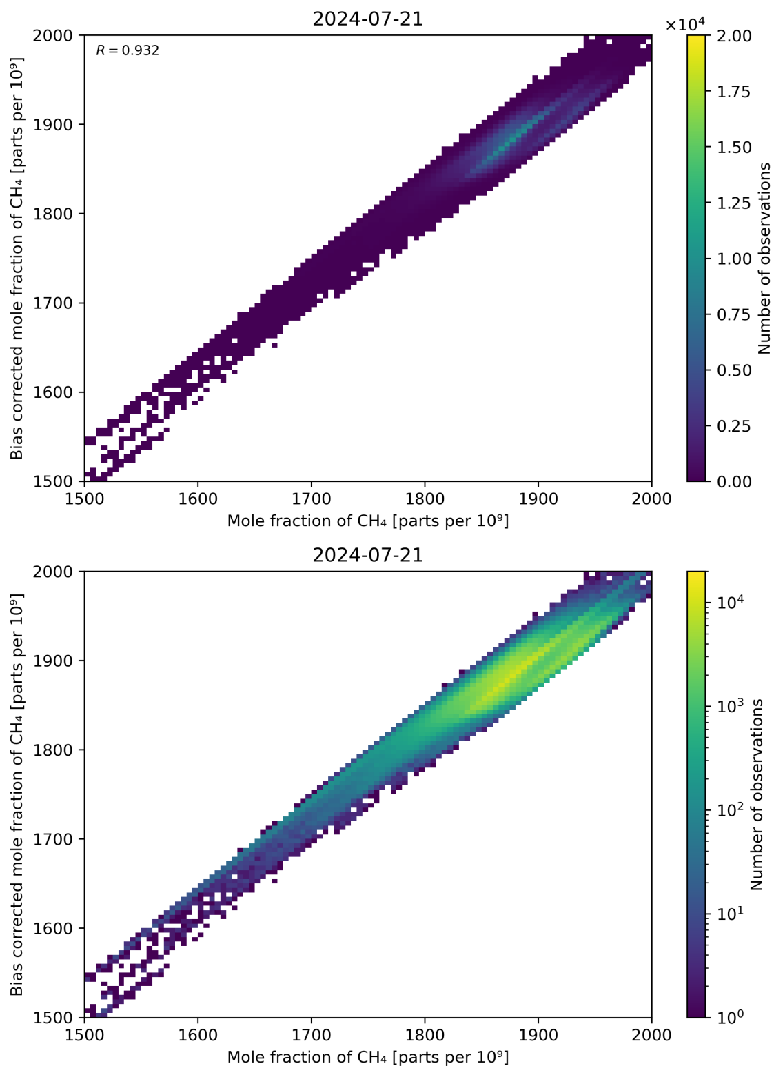
Figure 74: Scatter density plot of “Mole fraction of CH 4 ” against “Bias corrected mole fraction of CH 4 ” for 2024-07-21 to 2024-07-22.
