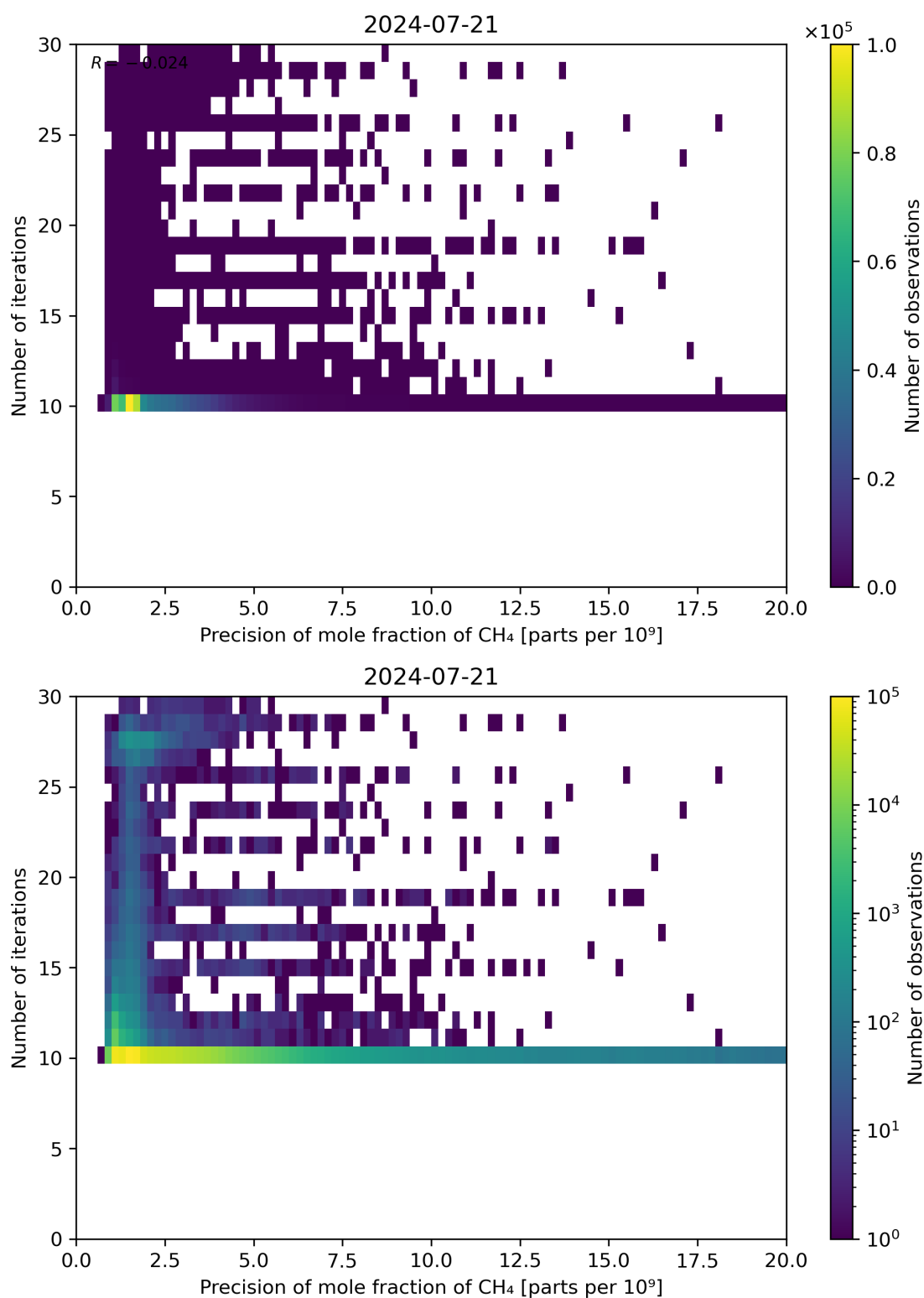
Figure 83: Scatter density plot of “Precision of mole fraction of CH 4 ” against “Number of iterations” for 2024-07-21 to 2024-07-22.
