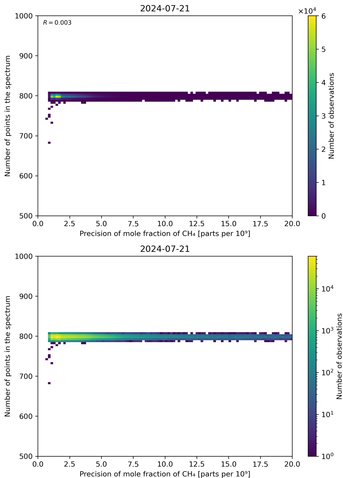
Figure 84: Scatter density plot of “Precision of mole fraction of CH 4 ” against “Number of points in the spectrum” for 2024-07-21 to 2024-07-22.
