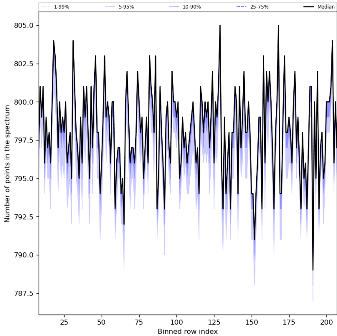
Figure 37: Along track statistics of “Number of points in the spectrum” for 2024-07-21 to 2024-07-22
