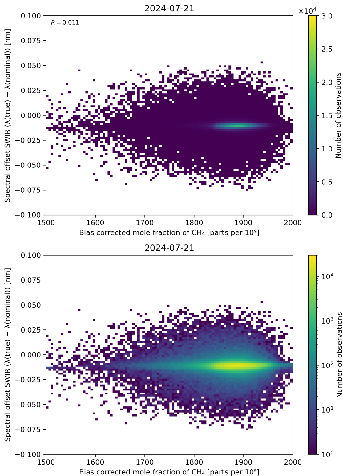
Figure 69: Scatter density plot of “Bias corrected mole fraction of \text{CH}_4 ” against “Spectral offset SWIR ( \lambda(\text{true}) - \lambda(\text{nominal}) )” for 2024-07-21 to 2024-07-22.
