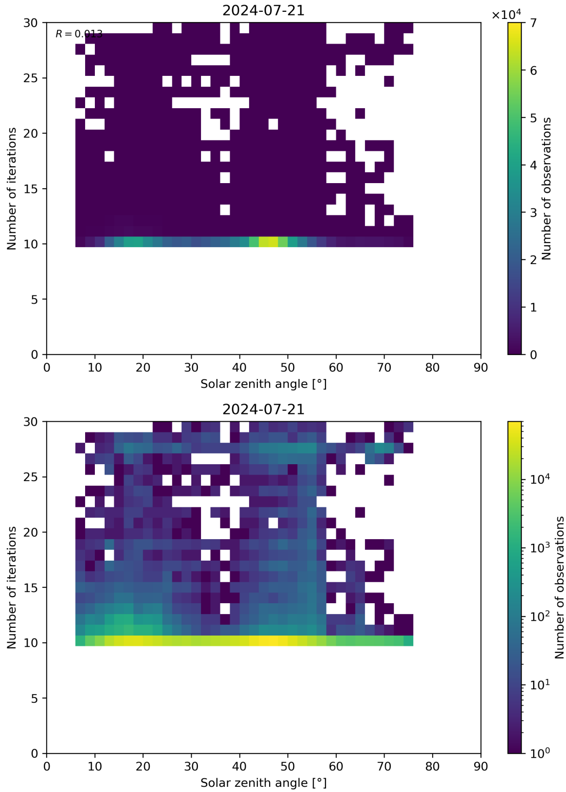
Figure 102: Scatter density plot of “Solar zenith angle” against “Number of iterations” for 2024-07-21 to 2024-07-22.
