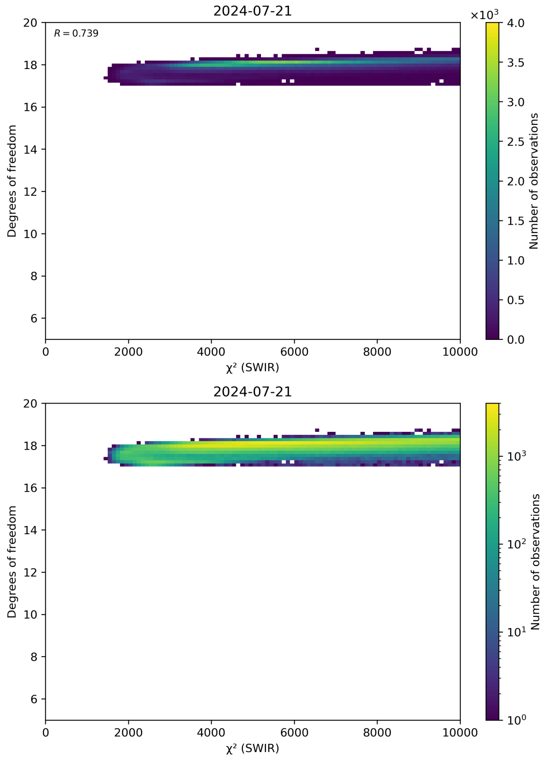
Figure 48: Scatter density plot of “ \chi^2 (SWIR)” against “Degrees of freedom” for 2024-07-21 to 2024-07-22.
