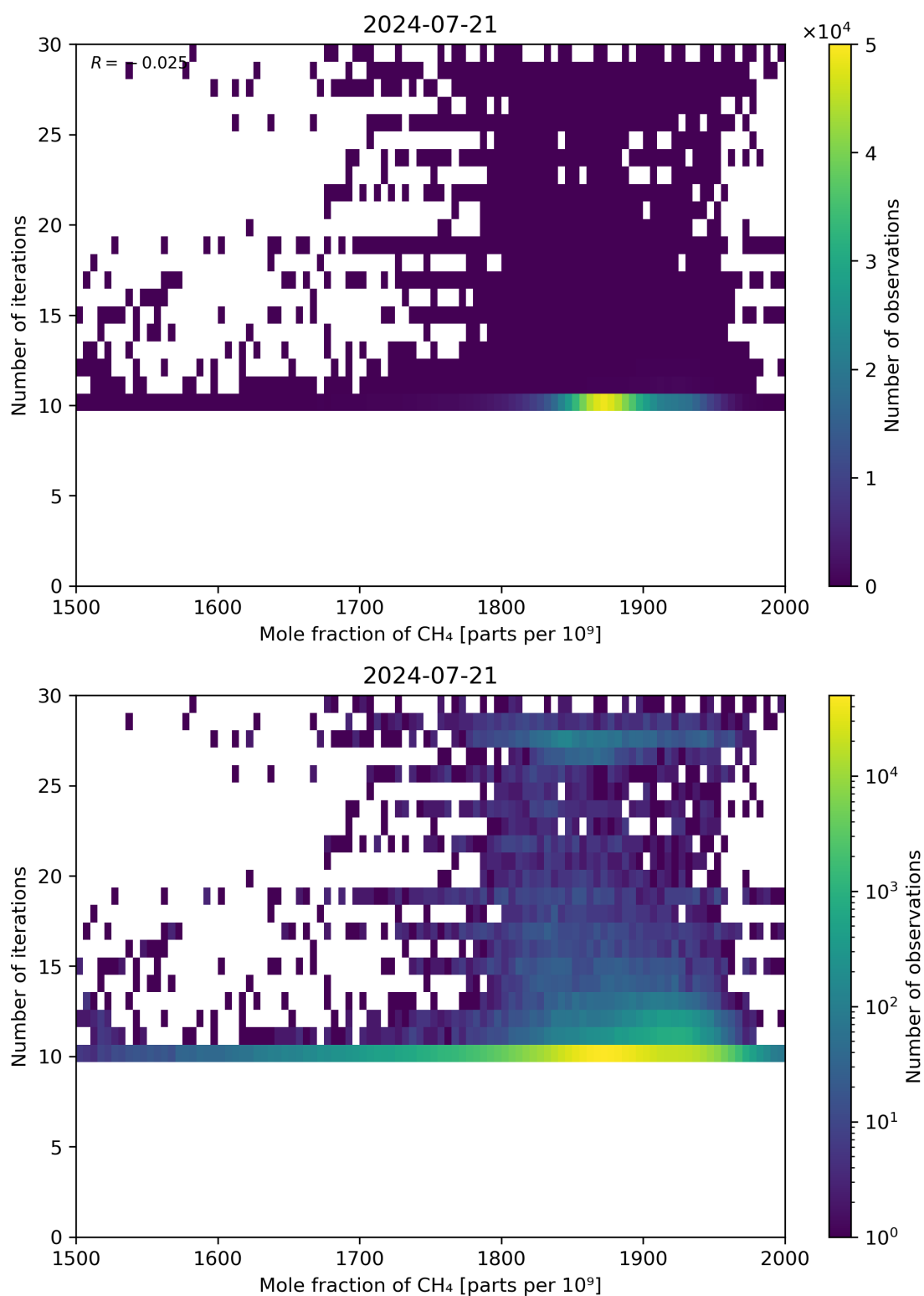
Figure 76: Scatter density plot of “Mole fraction of CH 4 ” against “Number of iterations” for 2024-07-21 to 2024-07-22.
