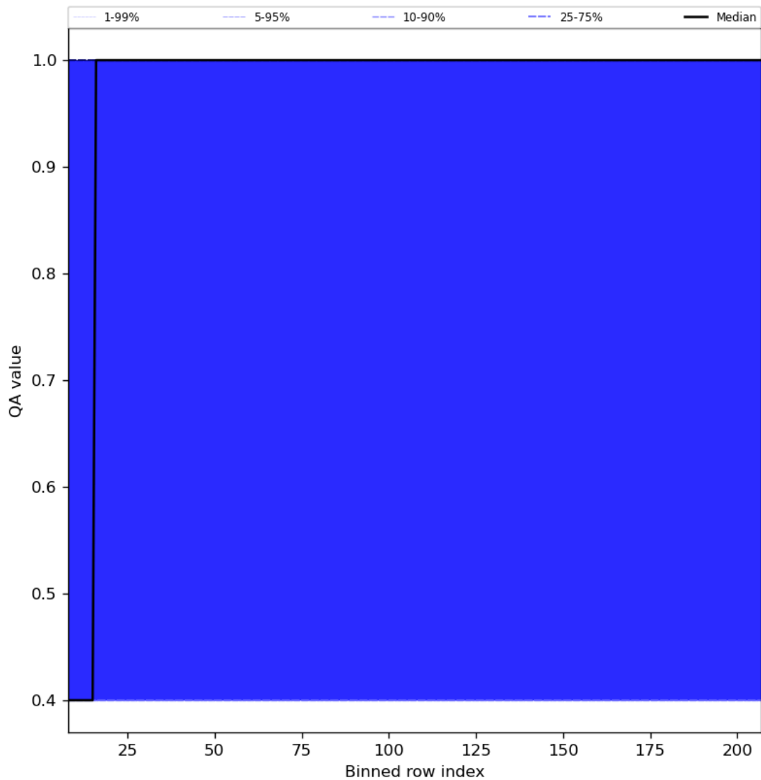
Figure 33: Along track statistics of “QA value” for 2024-07-21 to 2024-07-22
