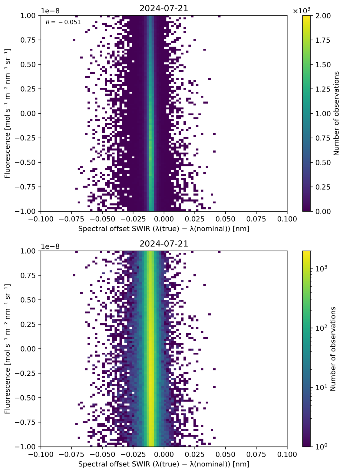
Figure 120: Scatter density plot of “Spectral offset SWIR ( \lambda(\text{true}) - \lambda(\text{nominal}) )” against “Fluorescence” for 2024-07-21 to 2024-07-22.
