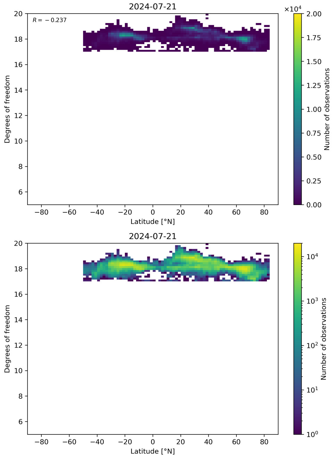
Figure 55: Scatter density plot of “Latitude” against “Degrees of freedom” for 2024-07-21 to 2024-07-22.
