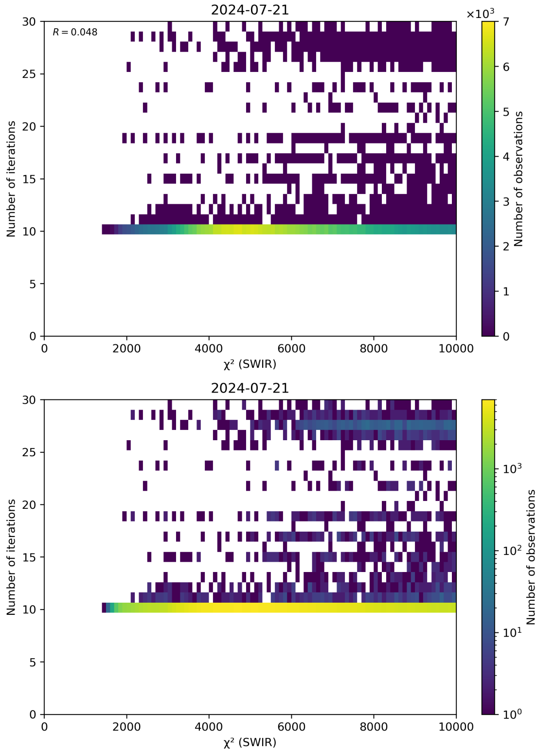
Figure 50: Scatter density plot of “ \chi^2 (SWIR)” against “Number of iterations” for 2024-07-21 to 2024-07-22.
