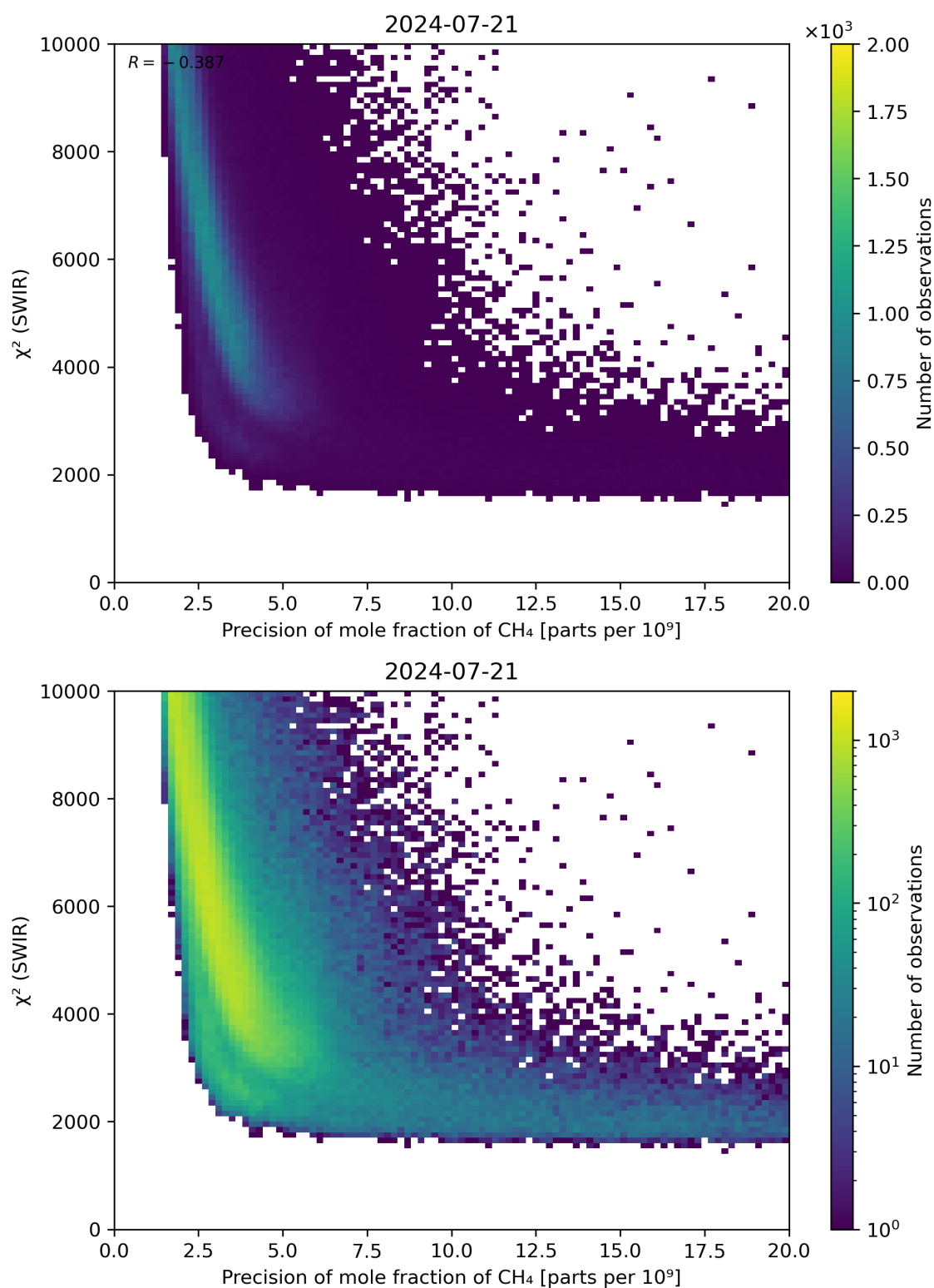
Figure 79: Scatter density plot of “Precision of mole fraction of CH 4 ” against “ \chi^2 (SWIR)” for 2024-07-21 to 2024-07-22.
