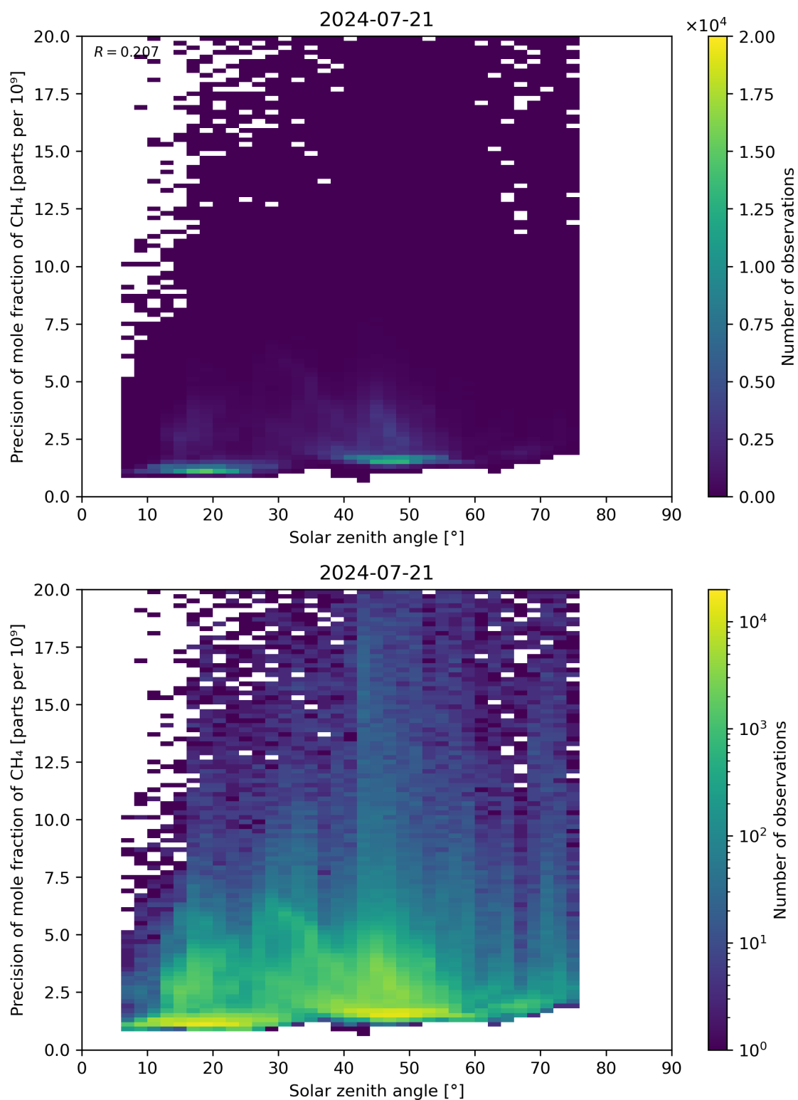
Figure 101: Scatter density plot of “Solar zenith angle” against “Precision of mole fraction of \text{CH}_4 ” for 2024-07-21 to 2024-07-22.
