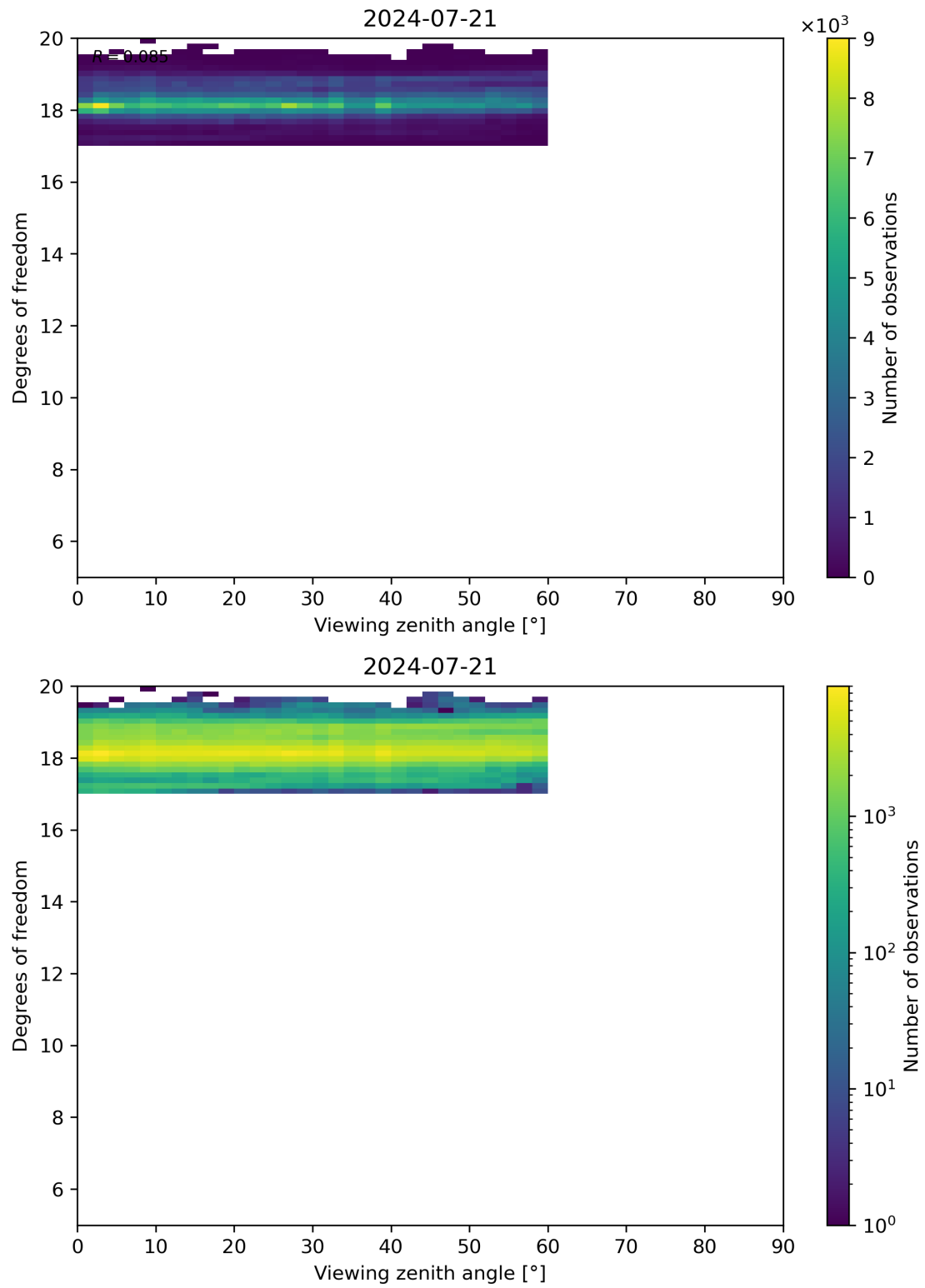
Figure 107: Scatter density plot of “Viewing zenith angle” against “Degrees of freedom” for 2024-07-21 to 2024-07-22.
