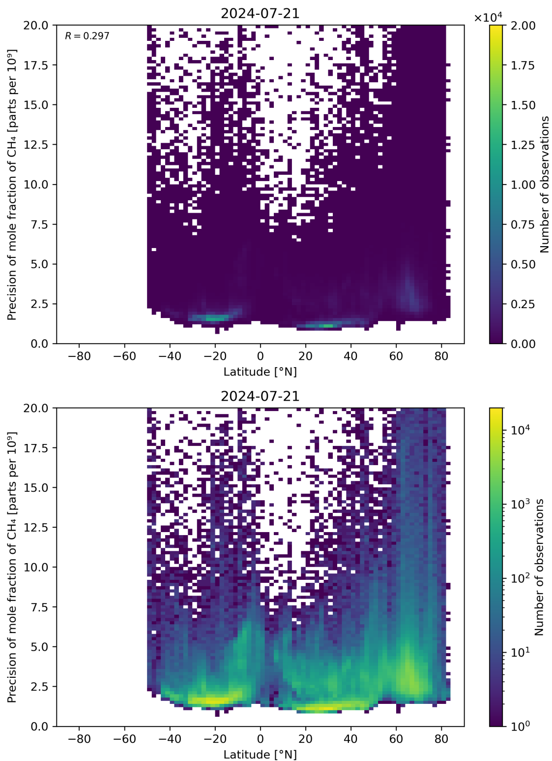
Figure 59: Scatter density plot of “Latitude” against “Precision of mole fraction of CH 4 ” for 2024-07-21 to 2024-07-22.
