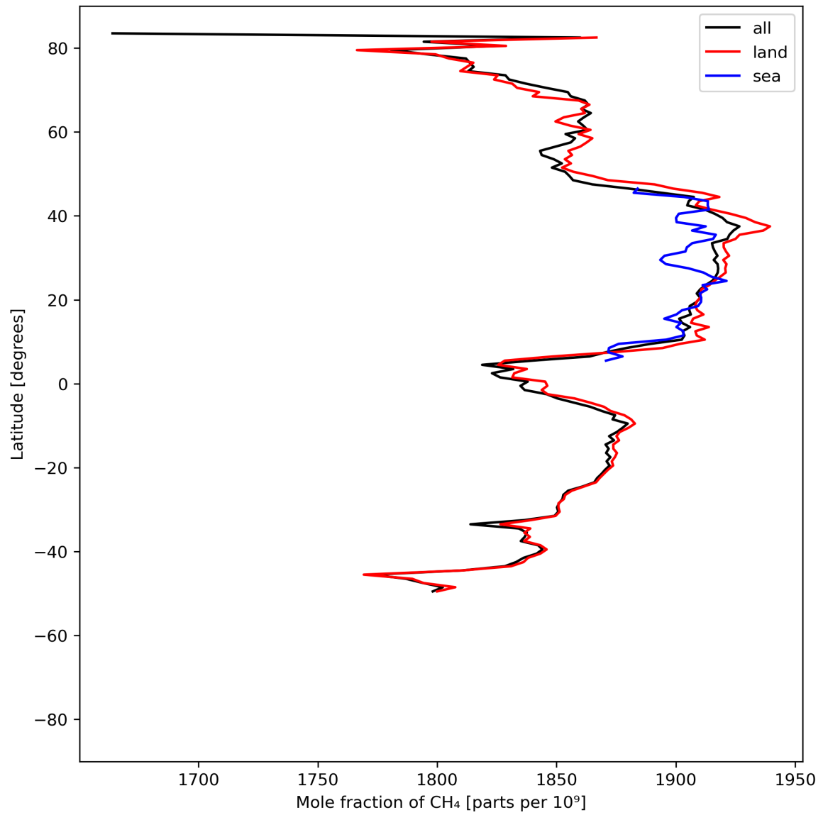
Figure 12: Zonal average of “Mole fraction of \text{CH}_4 ” for 2024-07-21 to 2024-07-22.
