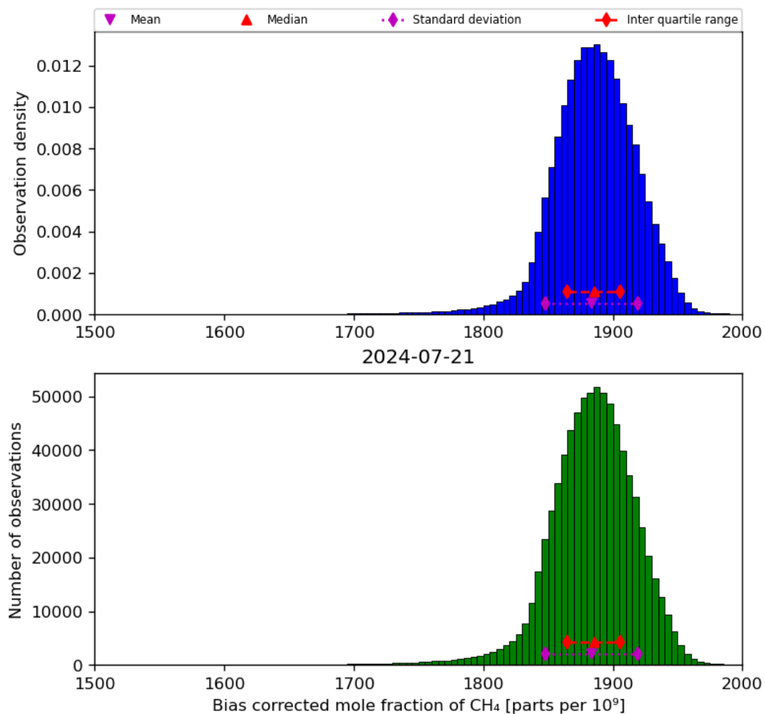
Figure 25: Histogram of “Bias corrected mole fraction of CH 4 ” for 2024-07-21 to 2024-07-22
