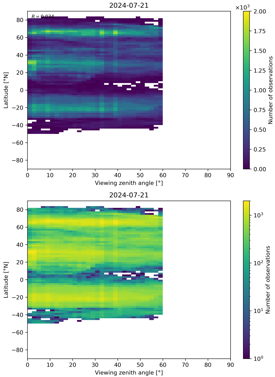
Figure 109: Scatter density plot of “Viewing zenith angle” against “Latitude” for 2024-07-21 to 2024-07-22.
