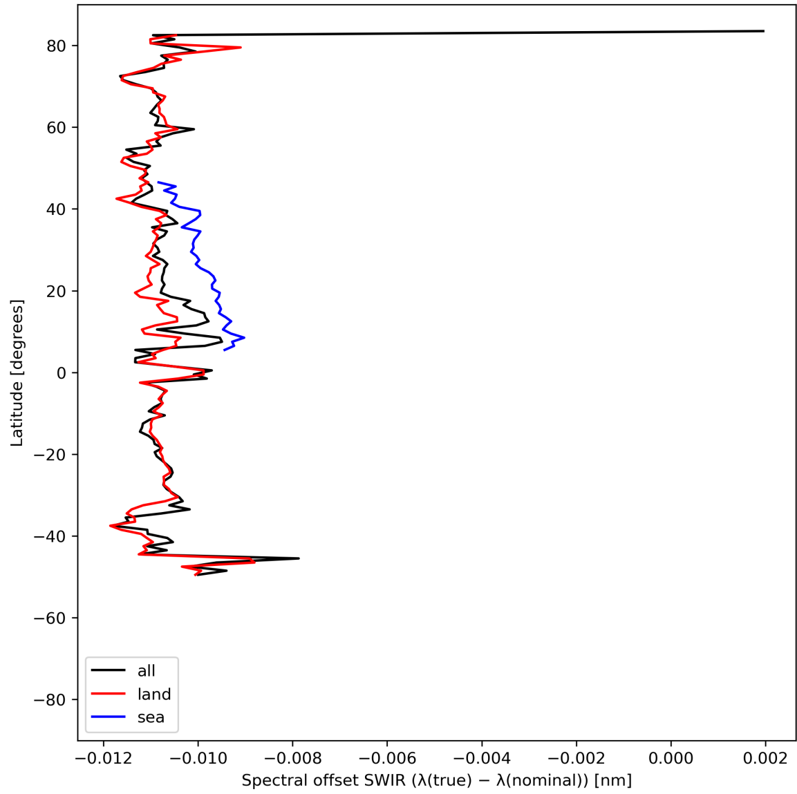
Figure 16: Zonal average of “Spectral offset SWIR ( \lambda(\text{true}) - \lambda(\text{nominal}) )” for 2024-07-21 to 2024-07-22.
