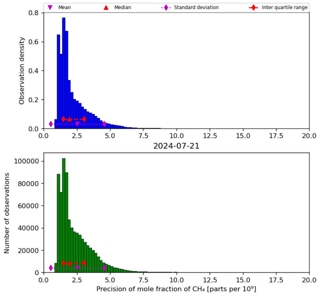
Figure 24: Histogram of “Precision of mole fraction of CH 4 ” for 2024-07-21 to 2024-07-22
