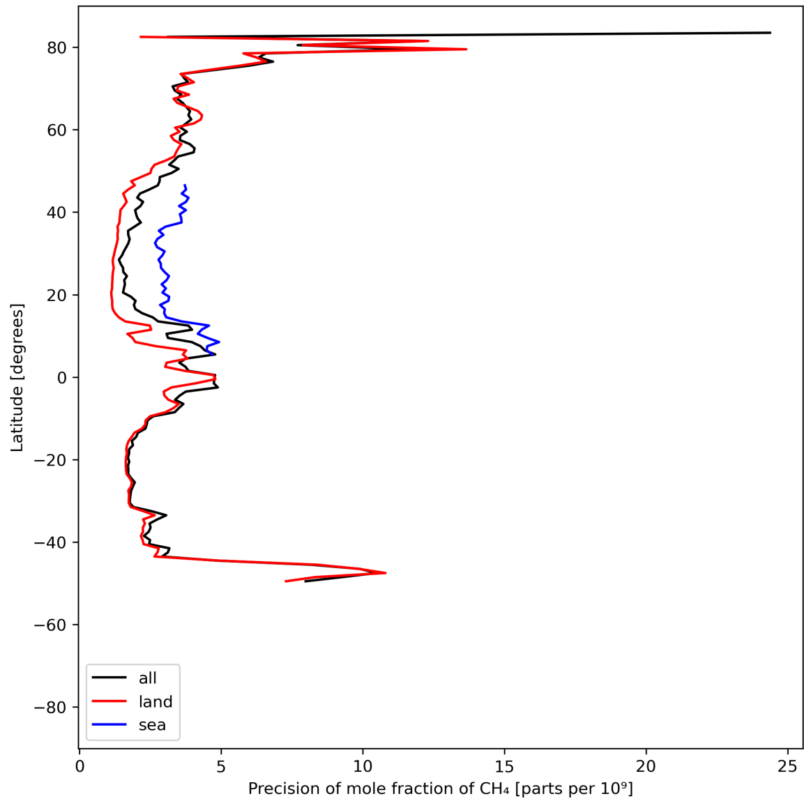
Figure 13: Zonal average of “Precision of mole fraction of CH 4 ” for 2024-07-21 to 2024-07-22.
