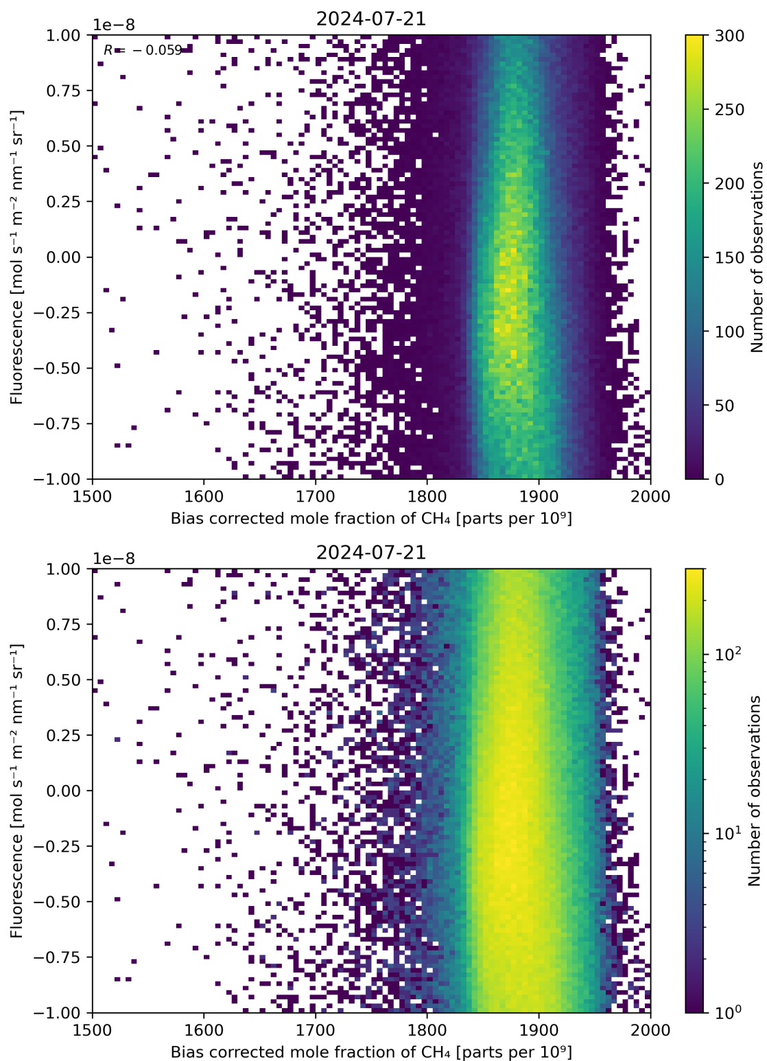
Figure 66: Scatter density plot of “Bias corrected mole fraction of \text{CH}_4 ” against “Fluorescence” for 2024-07-21 to 2024-07-22.
