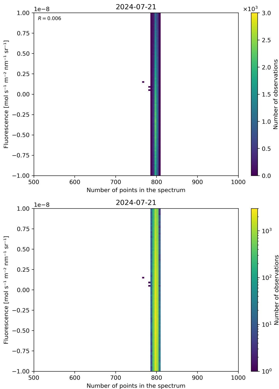
Figure 91: Scatter density plot of “Number of points in the spectrum” against “Fluorescence” for 2024-07-21 to 2024-07-22.
