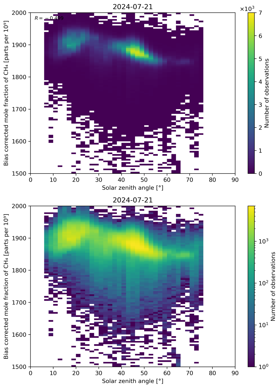
Figure 100: Scatter density plot of “Solar zenith angle” against “Bias corrected mole fraction of CH 4 ” for 2024-07-21 to 2024-07-22.
