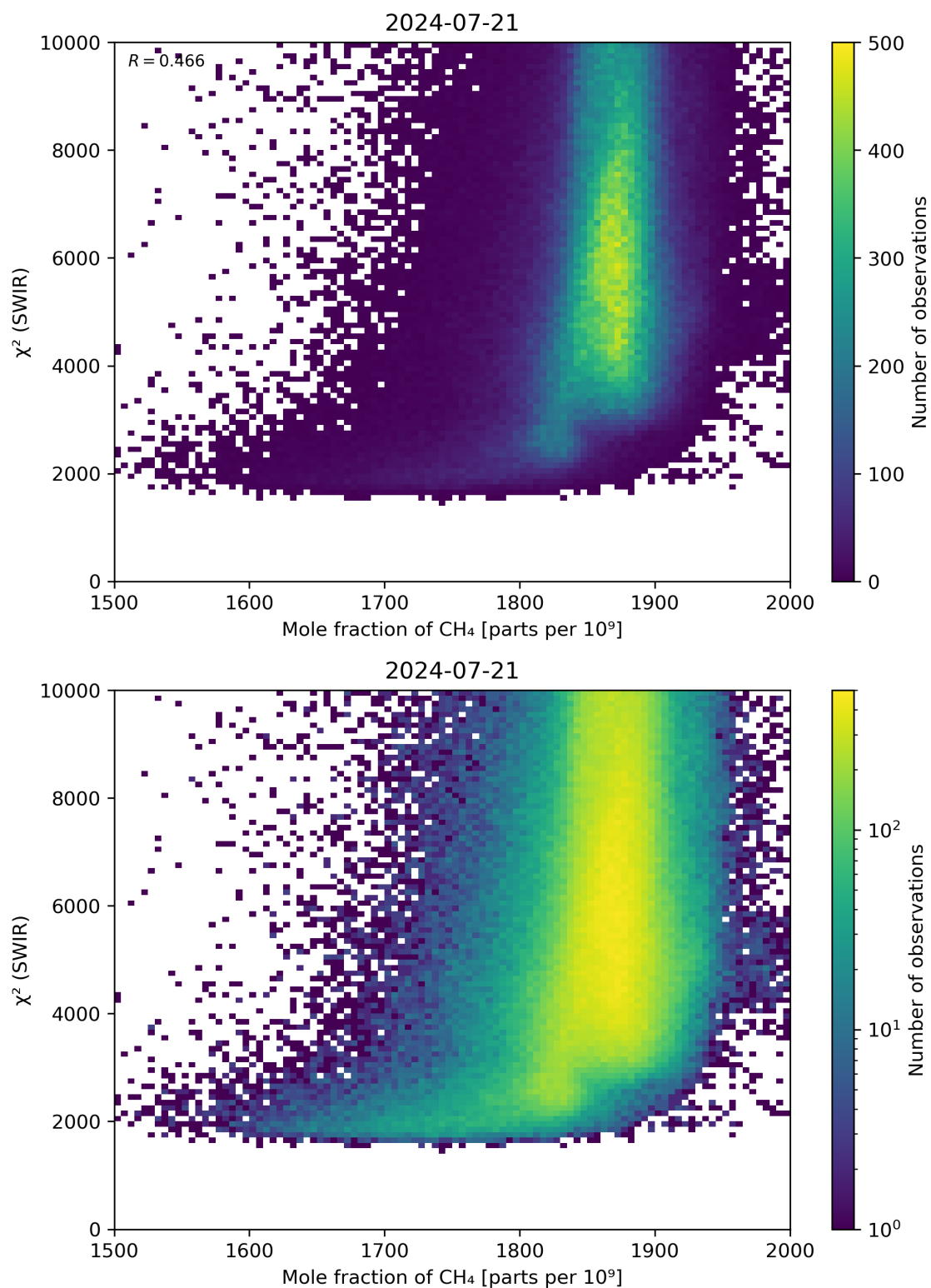
Figure 71: Scatter density plot of “Mole fraction of \text{CH}_4 ” against “ \chi^2 (SWIR)” for 2024-07-21 to 2024-07-22.
