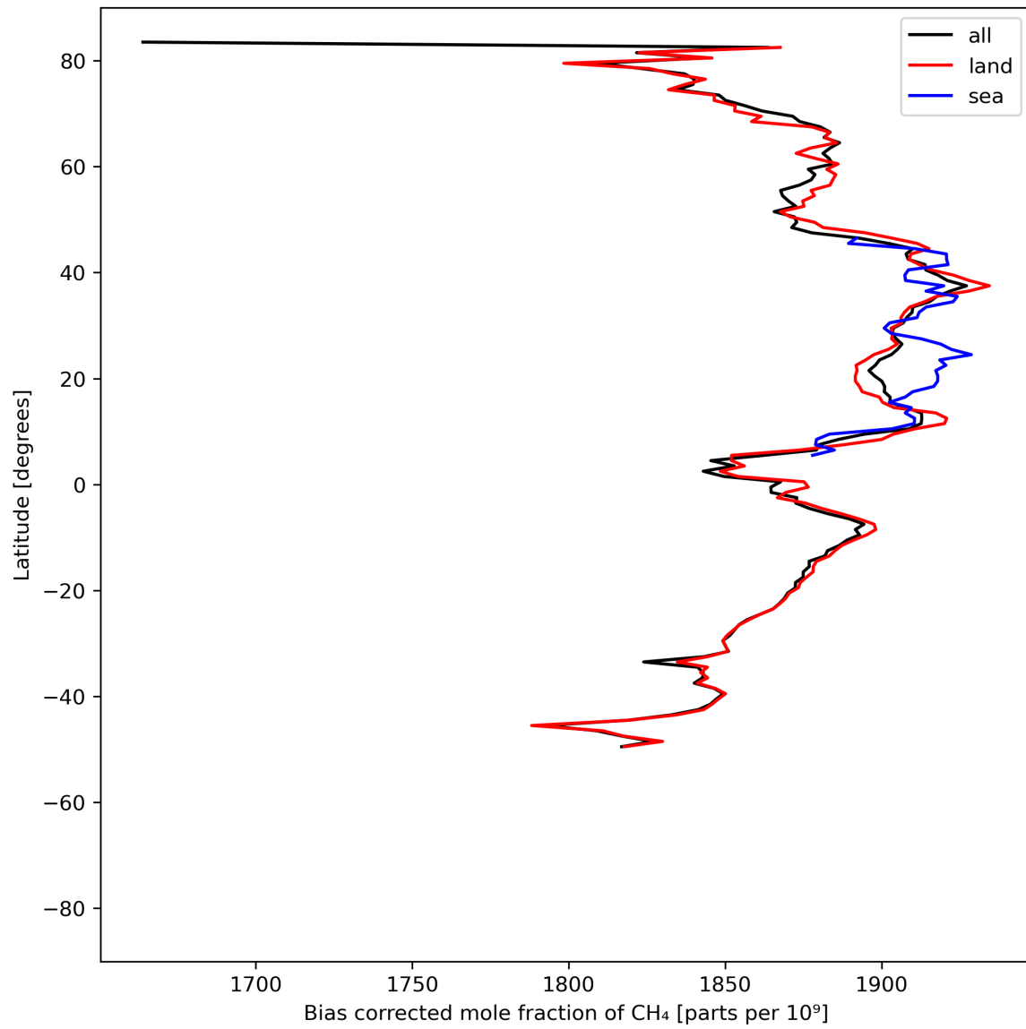
Figure 14: Zonal average of “Bias corrected mole fraction of CH 4 ” for 2024-07-21 to 2024-07-22.
