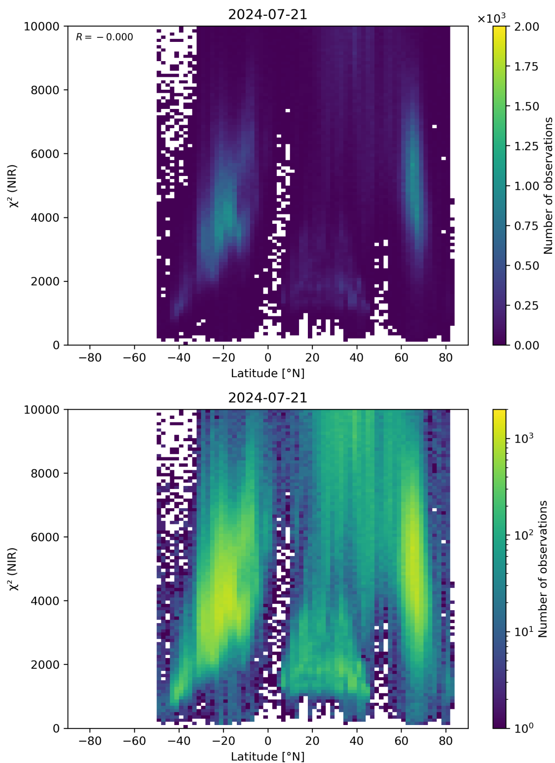
Figure 53: Scatter density plot of “Latitude” against “ \chi^2 (NIR)” for 2024-07-21 to 2024-07-22.
