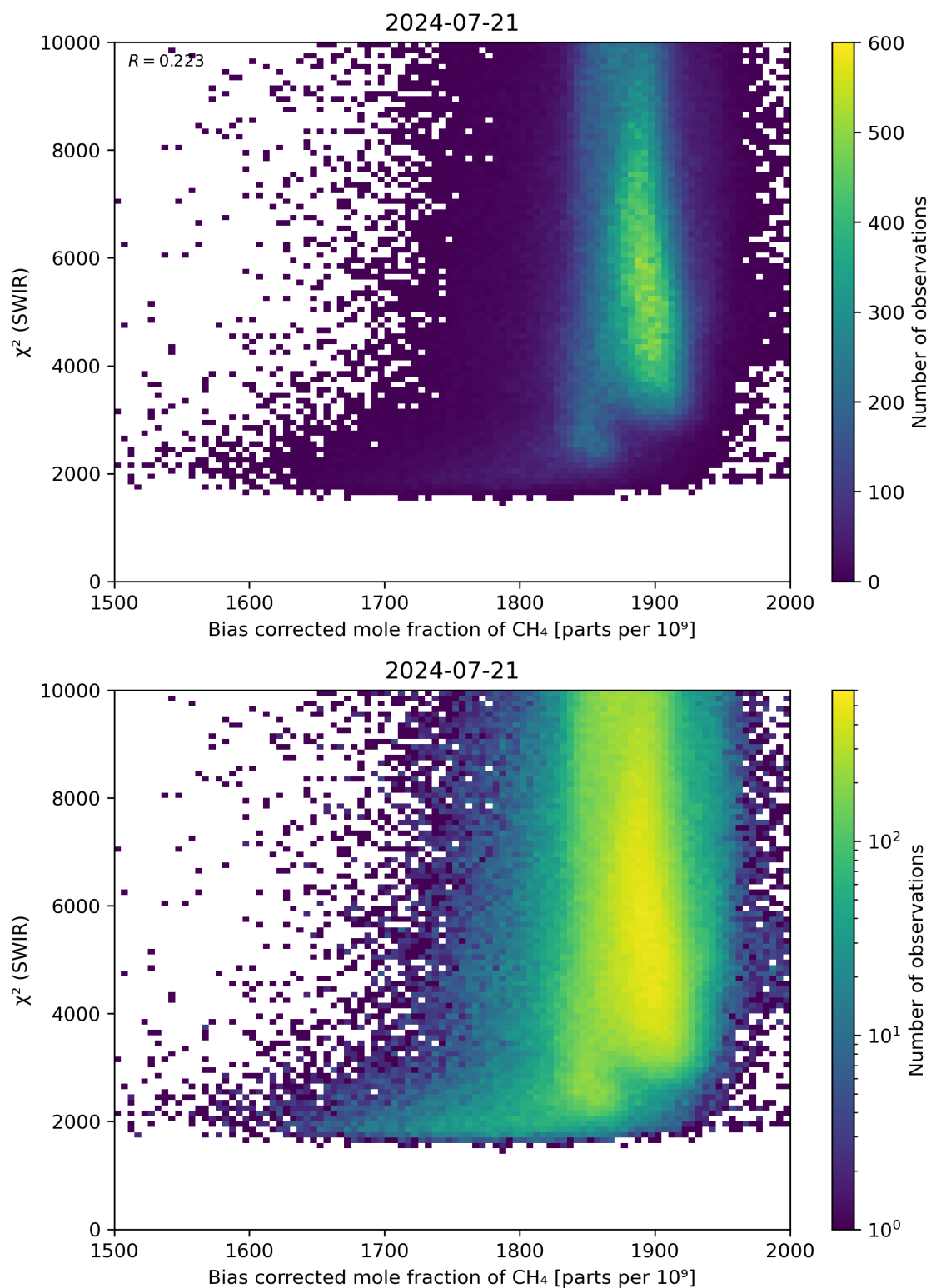
Figure 64: Scatter density plot of “Bias corrected mole fraction of \text{CH}_4 ” against “ \chi^2 (SWIR)” for 2024-07-21 to 2024-07-22.
