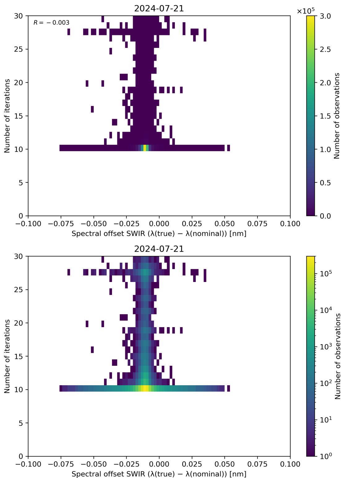
Figure 121: Scatter density plot of “Spectral offset SWIR ( \lambda(\text{true}) - \lambda(\text{nominal}) )” against “Number of iterations” for 2024-07-21 to 2024-07-22.
