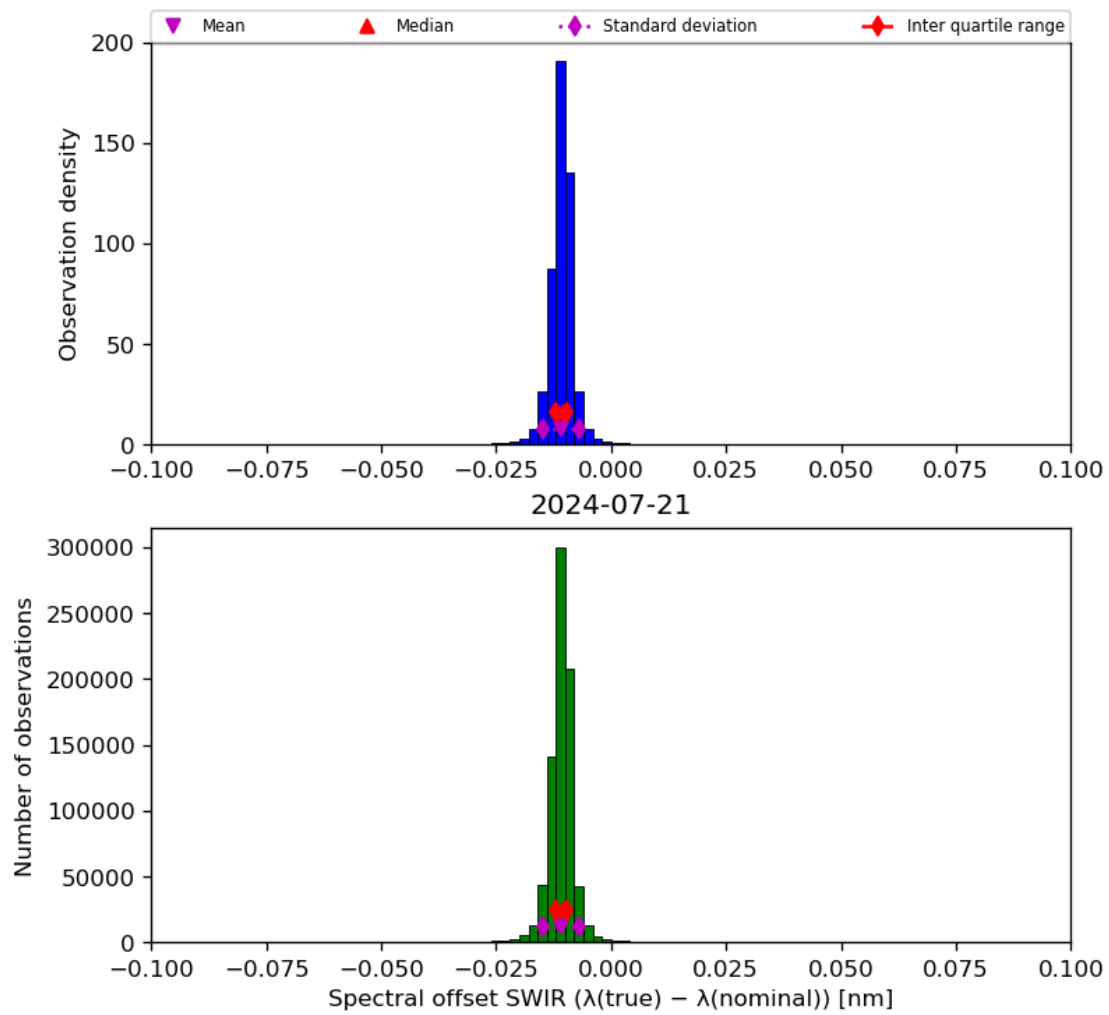
Figure 27: Histogram of “Spectral offset SWIR ( \lambda(\text{true}) - \lambda(\text{nominal}) )” for 2024-07-21 to 2024-07-22
