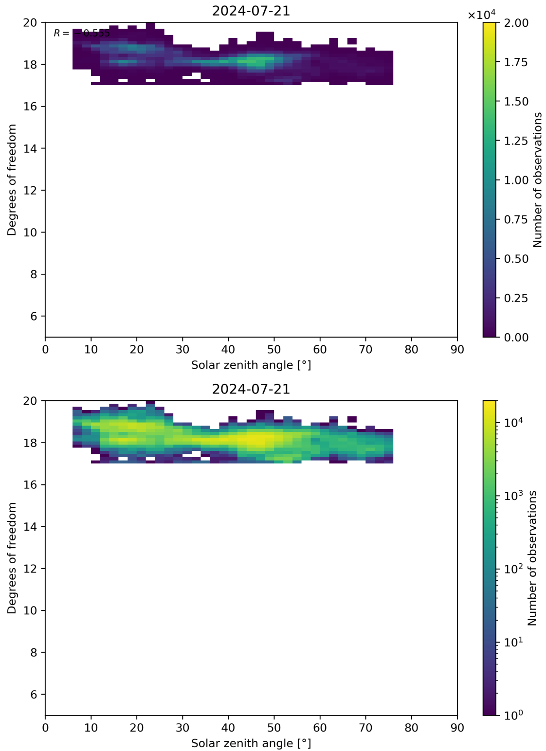
Figure 96: Scatter density plot of “Solar zenith angle” against “Degrees of freedom” for 2024-07-21 to 2024-07-22.
