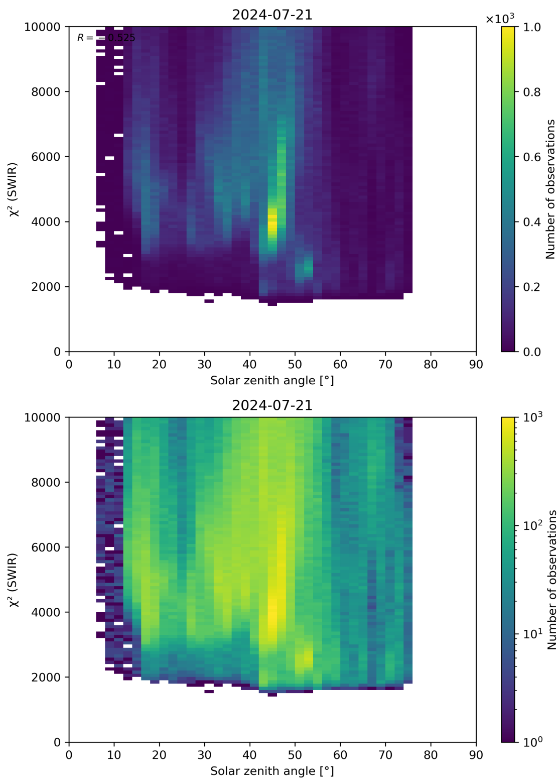
Figure 95: Scatter density plot of “Solar zenith angle” against “ \chi^2 (SWIR)” for 2024-07-21 to 2024-07-22.
