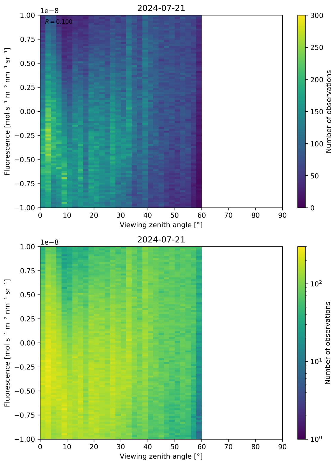
Figure 108: Scatter density plot of “Viewing zenith angle” against “Fluorescence” for 2024-07-21 to 2024-07-22.
