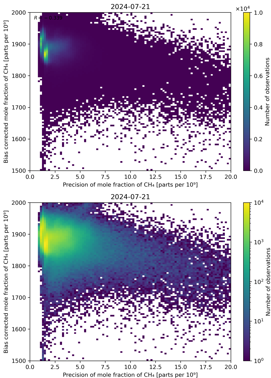
Figure 82: Scatter density plot of “Precision of mole fraction of CH 4 ” against “Bias corrected mole fraction of CH 4 ” for 2024-07-21 to 2024-07-22.
