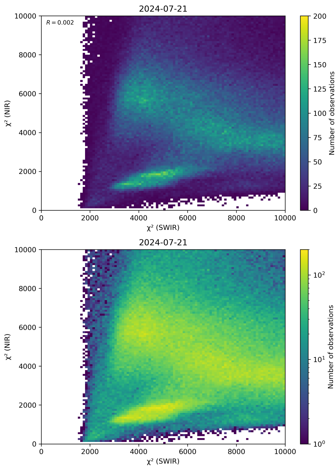
Figure 47: Scatter density plot of “ \chi^2 (SWIR)” against “ \chi^2 (NIR)” for 2024-07-21 to 2024-07-22.
