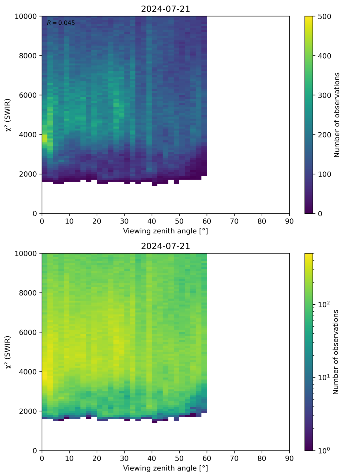
Figure 106: Scatter density plot of “Viewing zenith angle” against “ \chi^2 (SWIR)” for 2024-07-21 to 2024-07-22.
