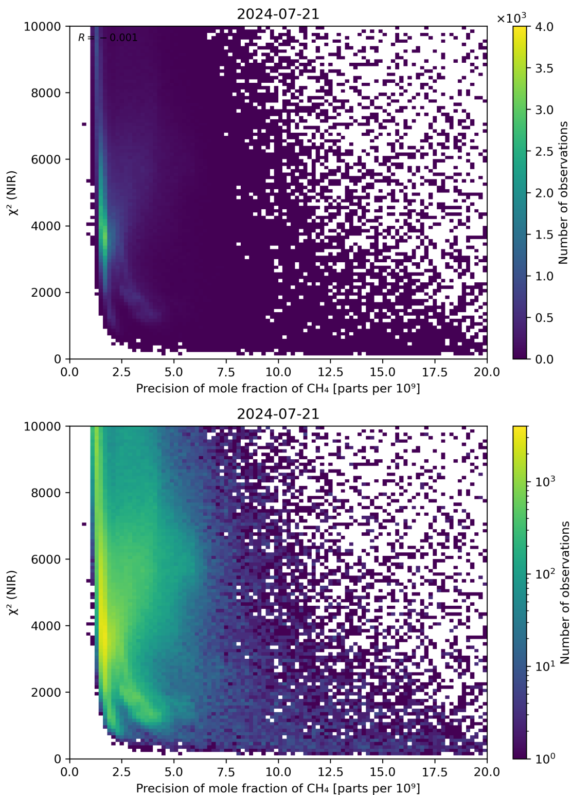
Figure 78: Scatter density plot of “Precision of mole fraction of CH 4 ” against “ \chi^2 (NIR)” for 2024-07-21 to 2024-07-22.
