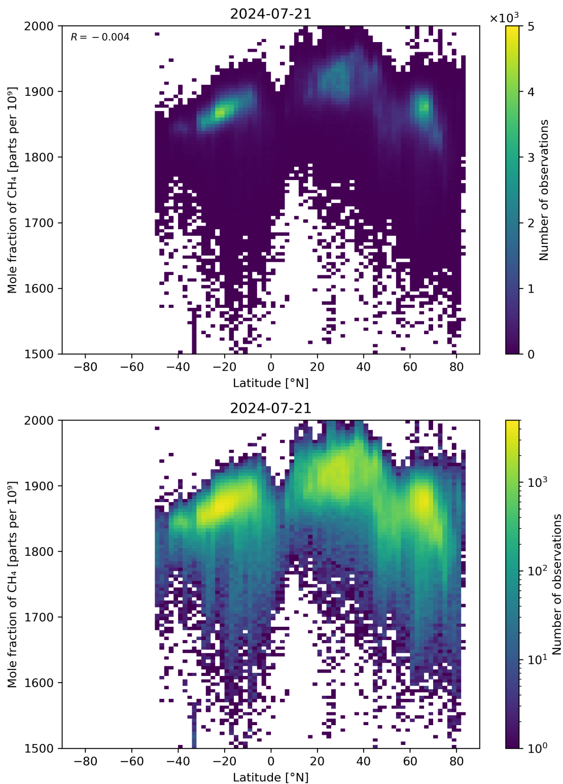
Figure 57: Scatter density plot of “Latitude” against “Mole fraction of CH 4 ” for 2024-07-21 to 2024-07-22.
