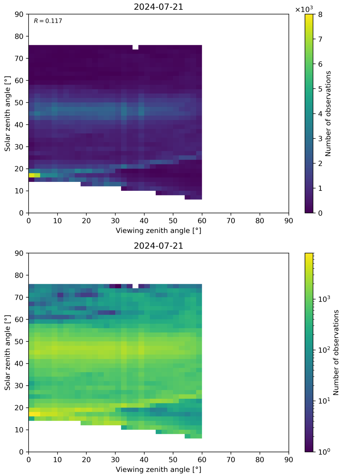
Figure 115: Scatter density plot of “Viewing zenith angle” against “Solar zenith angle” for 2024-07-21 to 2024-07-22.
