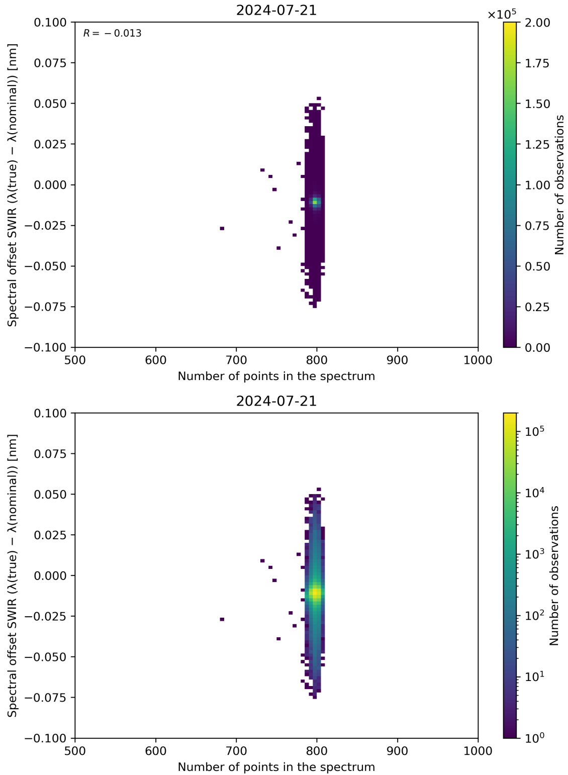
Figure 93: Scatter density plot of “Number of points in the spectrum” against “Spectral offset SWIR ( \lambda(\text{true}) - \lambda(\text{nominal}) )” for 2024-07-21 to 2024-07-22.
