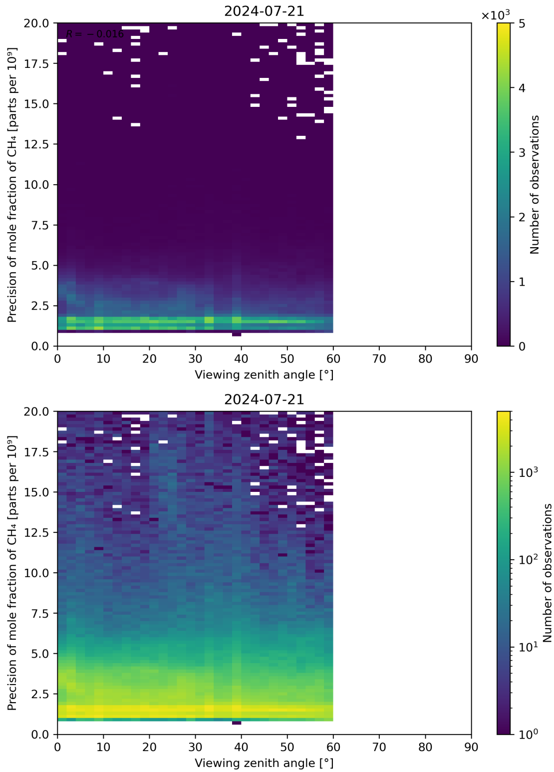
Figure 112: Scatter density plot of “Viewing zenith angle” against “Precision of mole fraction of CH 4 ” for 2024-07-21 to 2024-07-22.
