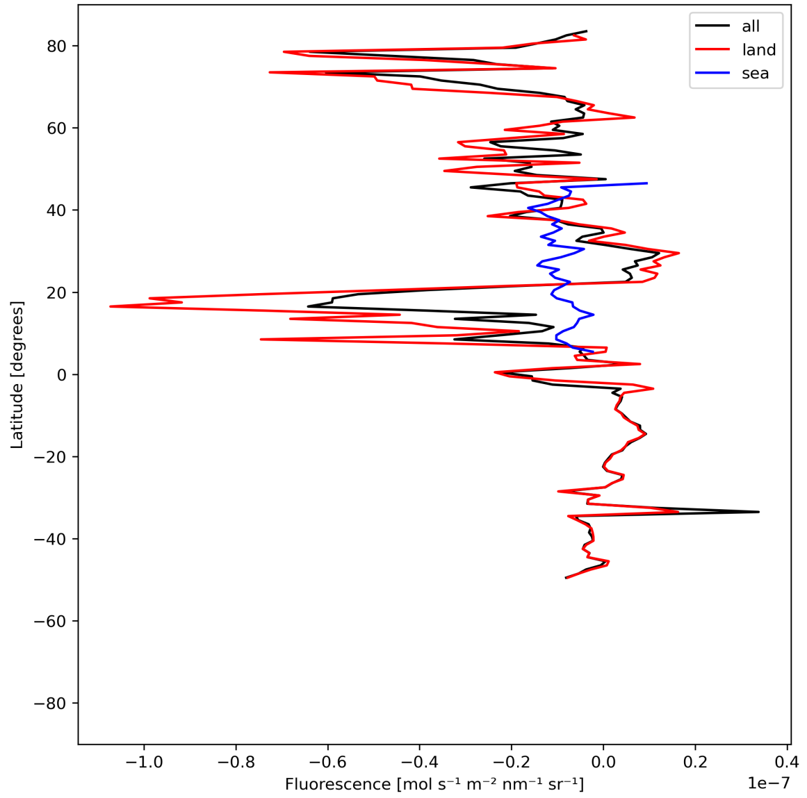
Figure 21: Zonal average of “Fluorescence” for 2024-07-21 to 2024-07-22.
