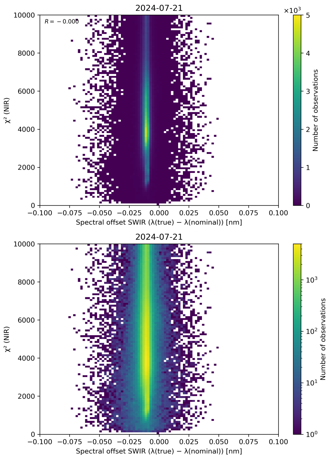
Figure 117: Scatter density plot of “Spectral offset SWIR ( \lambda(\text{true}) - \lambda(\text{nominal}) )” against “ \chi^2 (NIR)” for 2024-07-21 to 2024-07-22.
