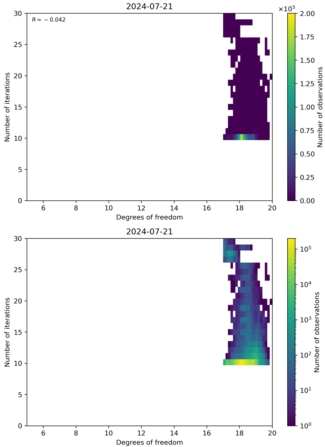
Figure 52: Scatter density plot of “Degrees of freedom” against “Number of iterations” for 2024-07-21 to 2024-07-22.
