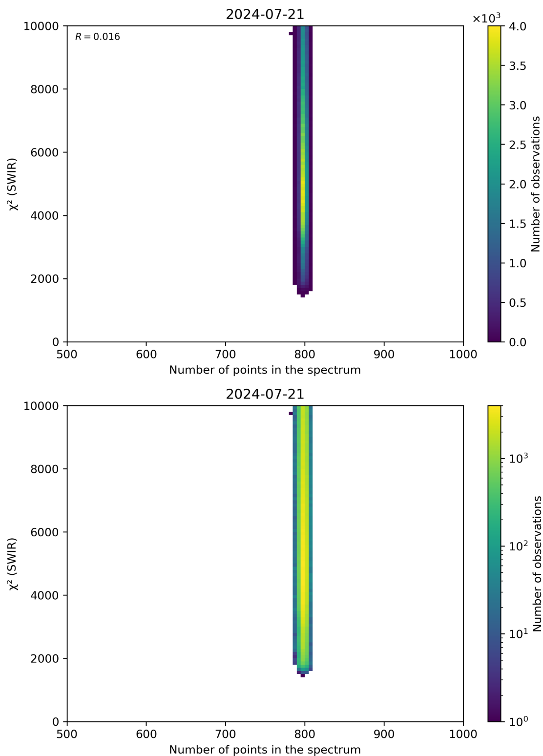
Figure 89: Scatter density plot of “Number of points in the spectrum” against “ \chi^2 (SWIR)” for 2024-07-21 to 2024-07-22.
