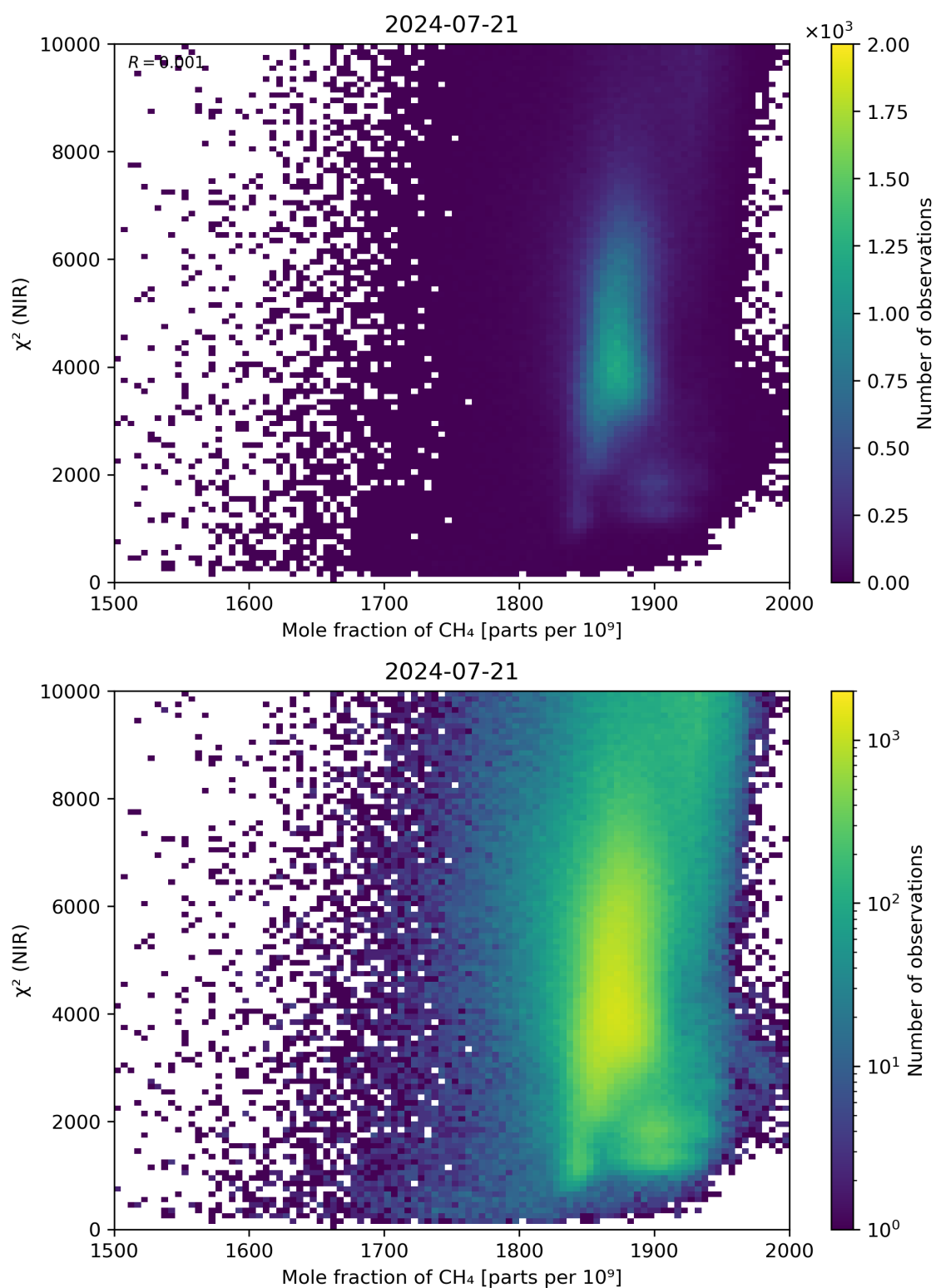
Figure 70: Scatter density plot of “Mole fraction of \text{CH}_4 ” against “ \chi^2 (NIR)” for 2024-07-21 to 2024-07-22.
