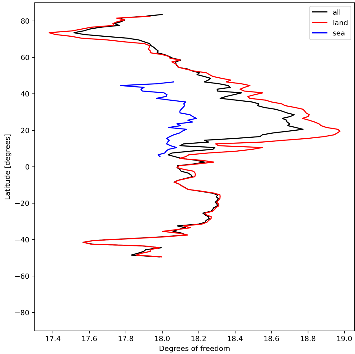
Figure 19: Zonal average of “Degrees of freedom” for 2024-07-21 to 2024-07-22.
