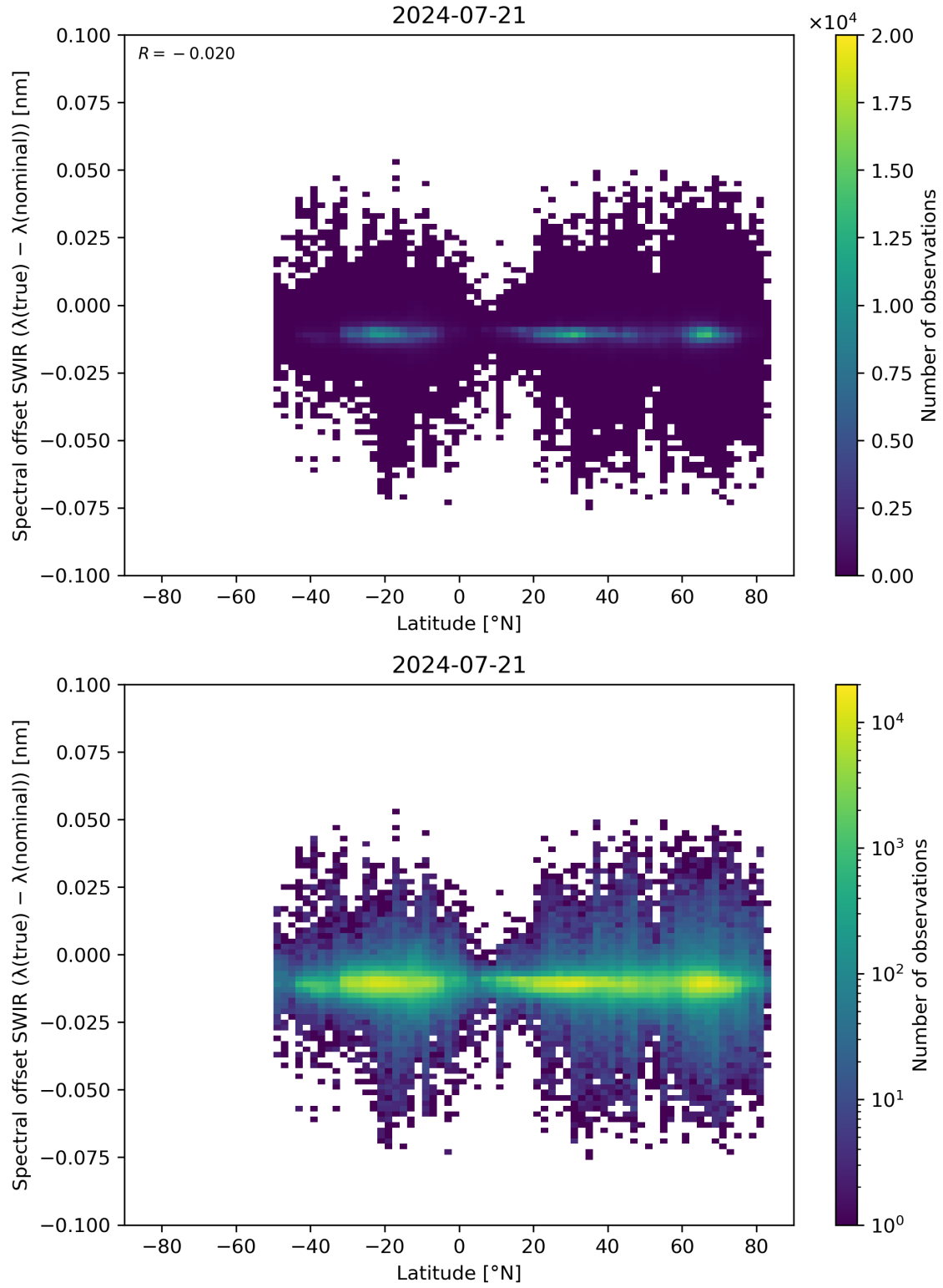
Figure 62: Scatter density plot of “Latitude” against “Spectral offset SWIR ( \lambda(\text{true}) - \lambda(\text{nominal}) )” for 2024-07-21 to 2024-07-22.
