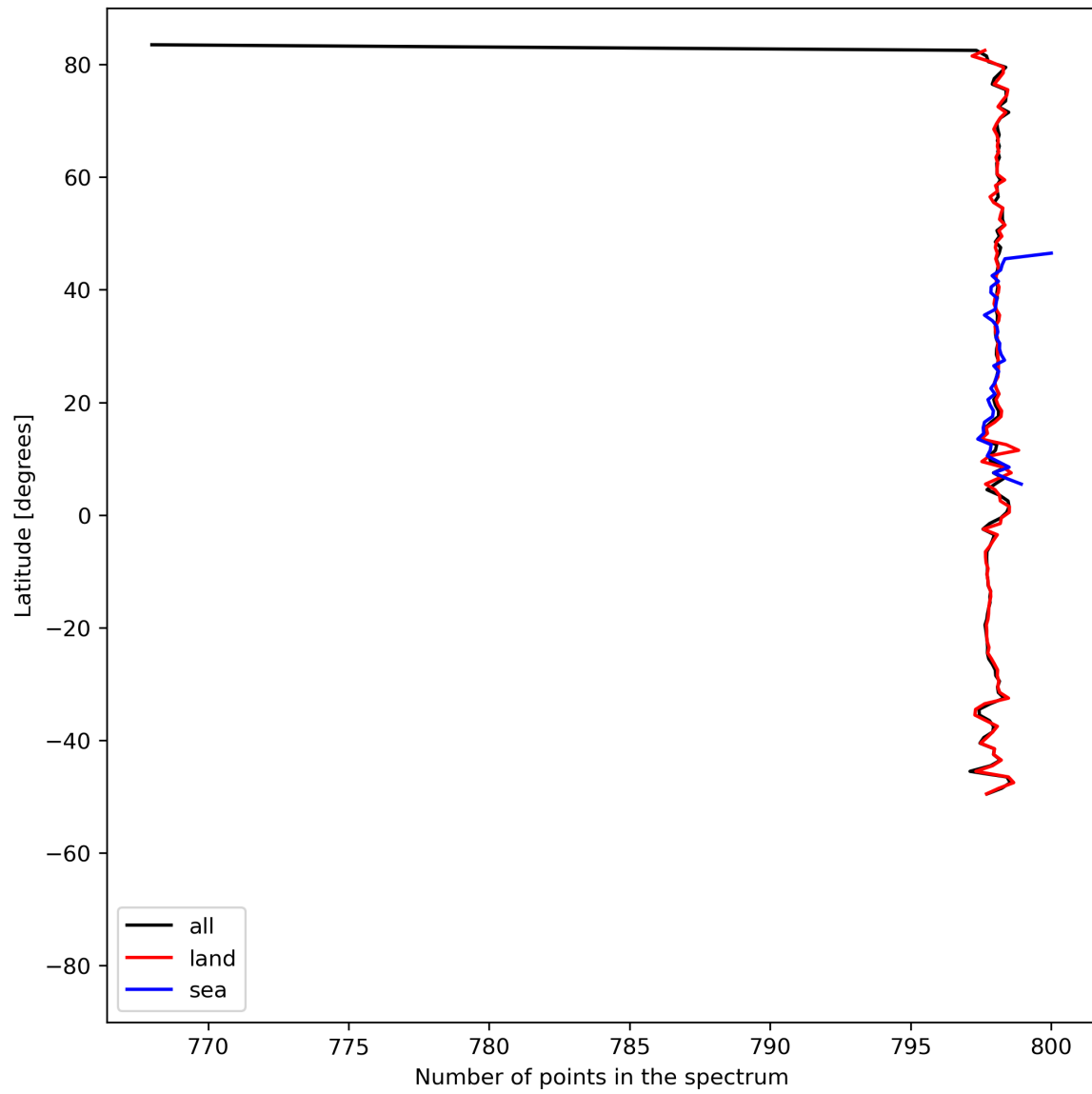
Figure 15: Zonal average of “Number of points in the spectrum” for 2024-07-21 to 2024-07-22.
