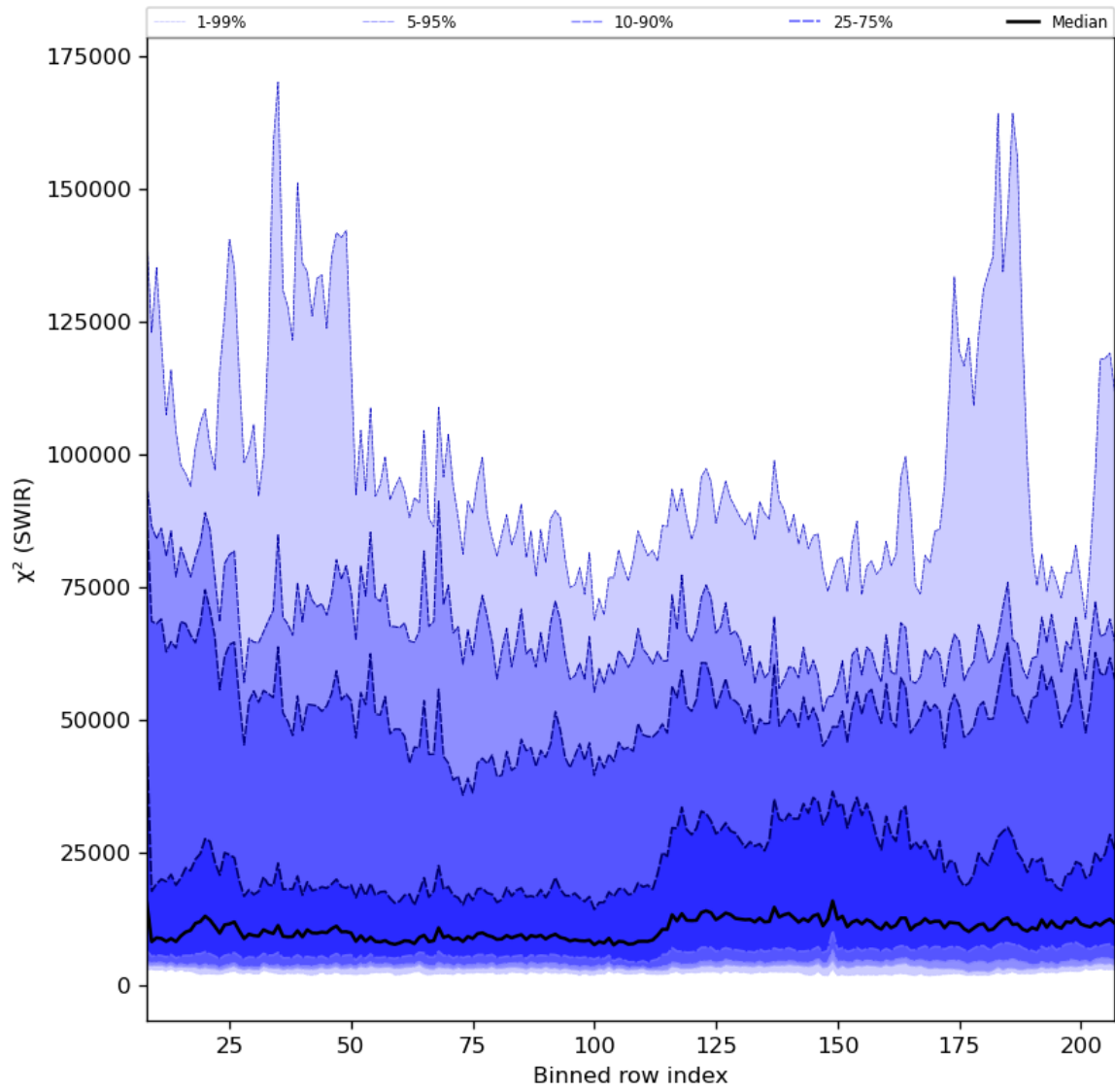
Figure 39: Along track statistics of " \chi^2 (SWIR)" for 2024-07-21 to 2024-07-22
