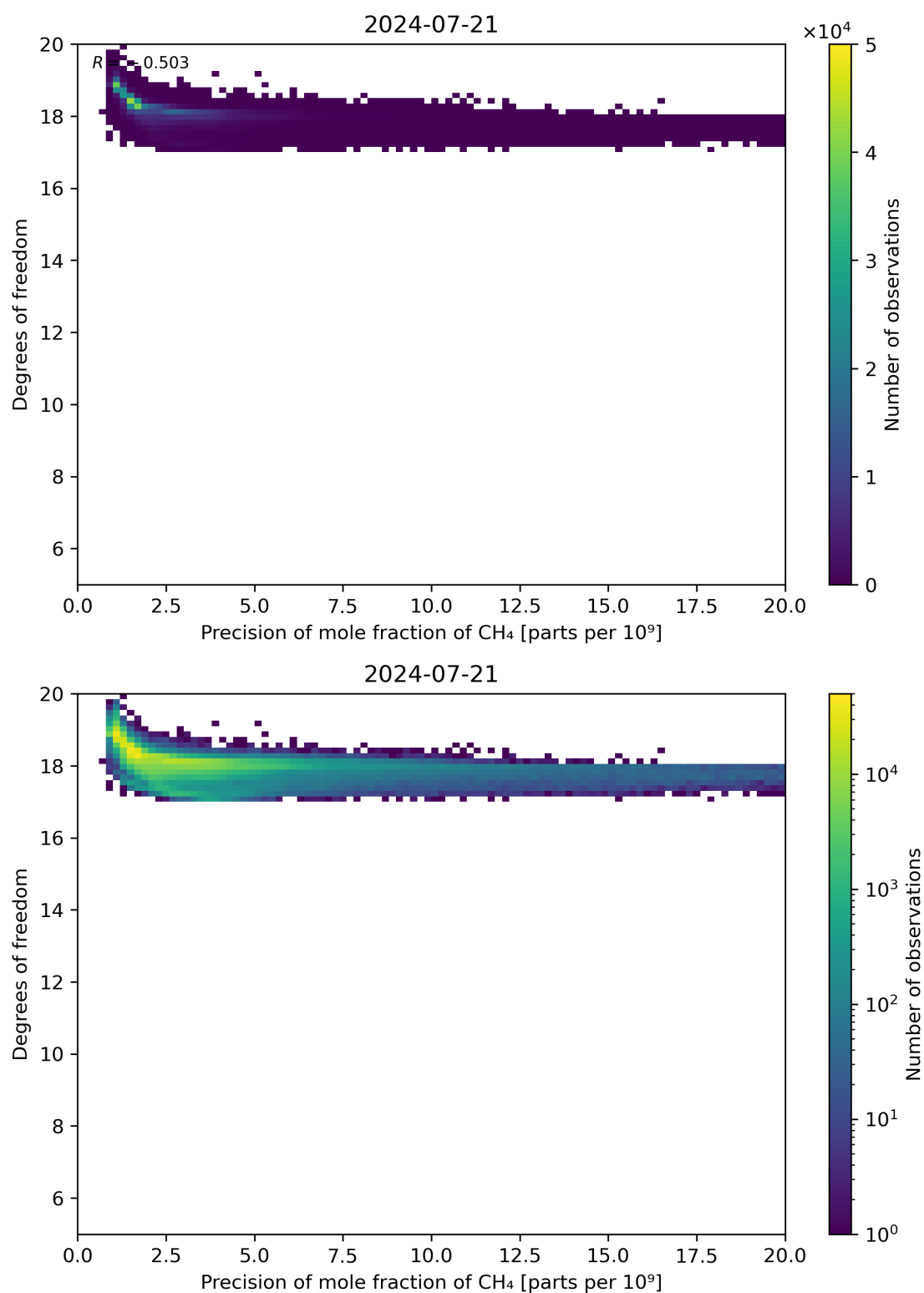
Figure 80: Scatter density plot of “Precision of mole fraction of CH 4 ” against “Degrees of freedom” for 2024-07-21 to 2024-07-22.
