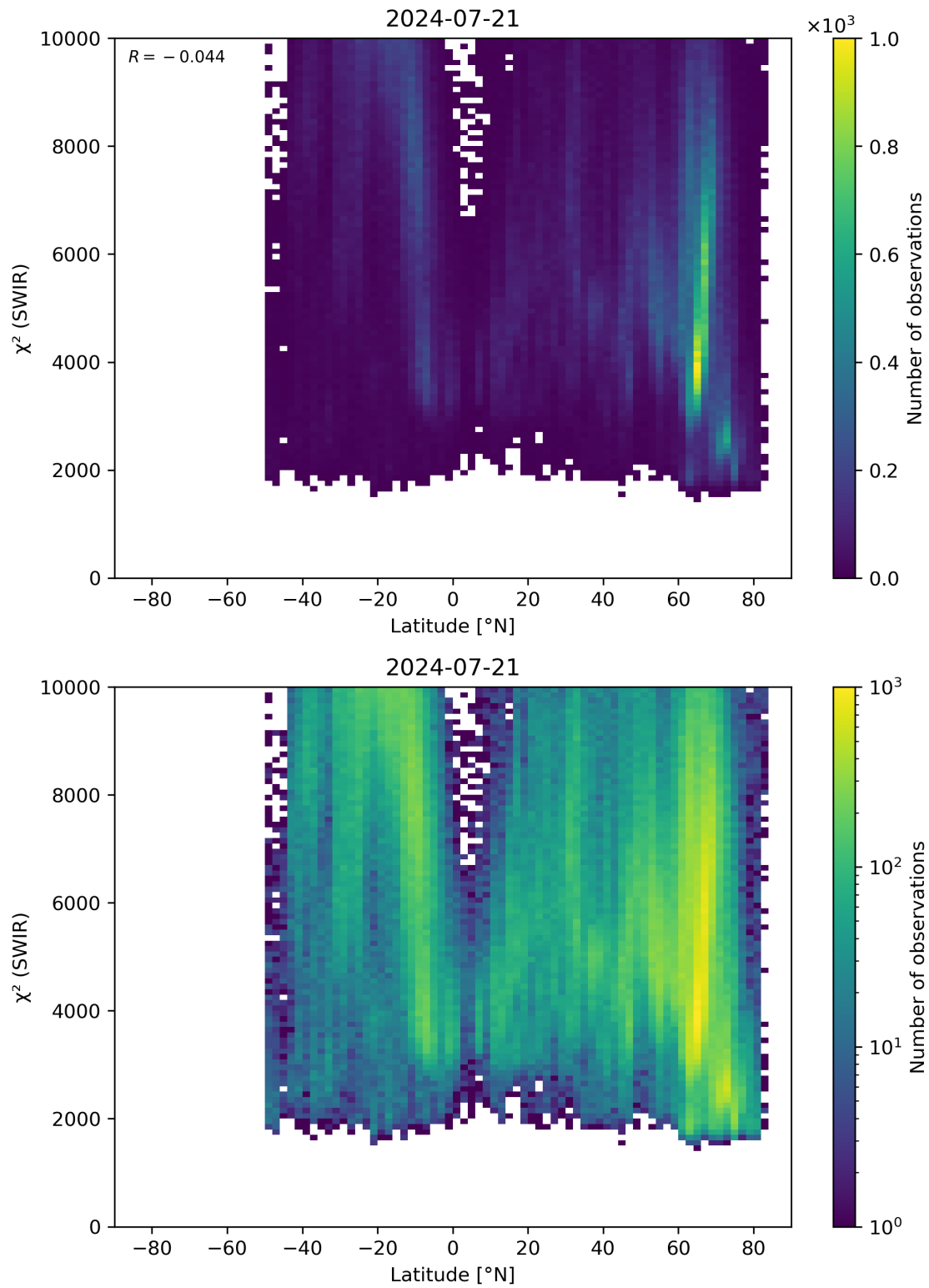
Figure 54: Scatter density plot of “Latitude” against “ \chi^2 (SWIR)” for 2024-07-21 to 2024-07-22.
