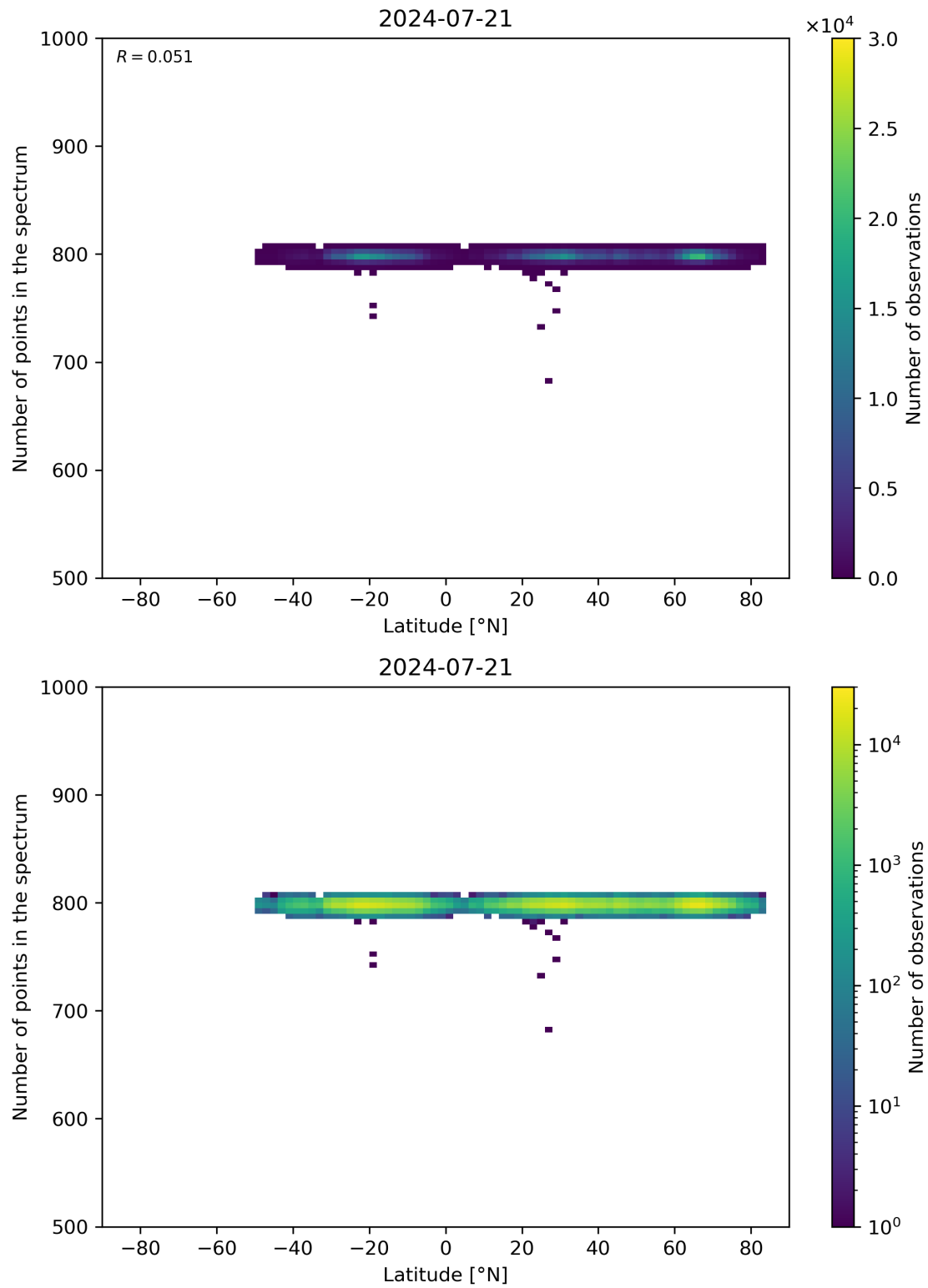
Figure 61: Scatter density plot of “Latitude” against “Number of points in the spectrum” for 2024-07-21 to 2024-07-22.
