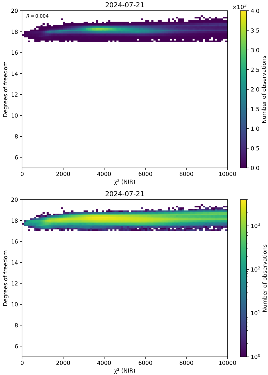
Figure 44: Scatter density plot of “ \chi^2 (NIR)” against “Degrees of freedom” for 2024-07-21 to 2024-07-22.
