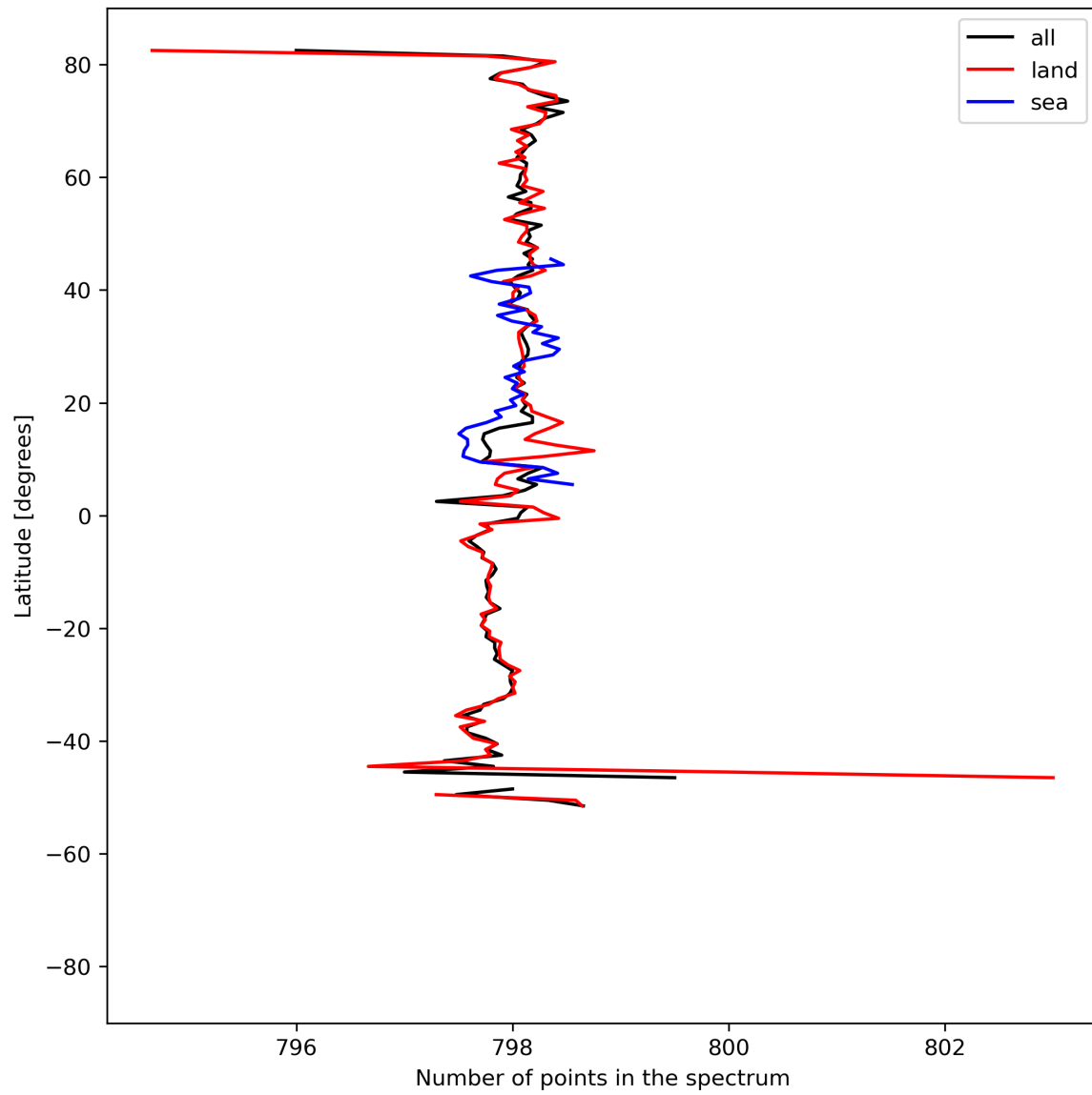
Figure 15: Zonal average of “Number of points in the spectrum” for 2024-07-21 to 2024-07-23.
