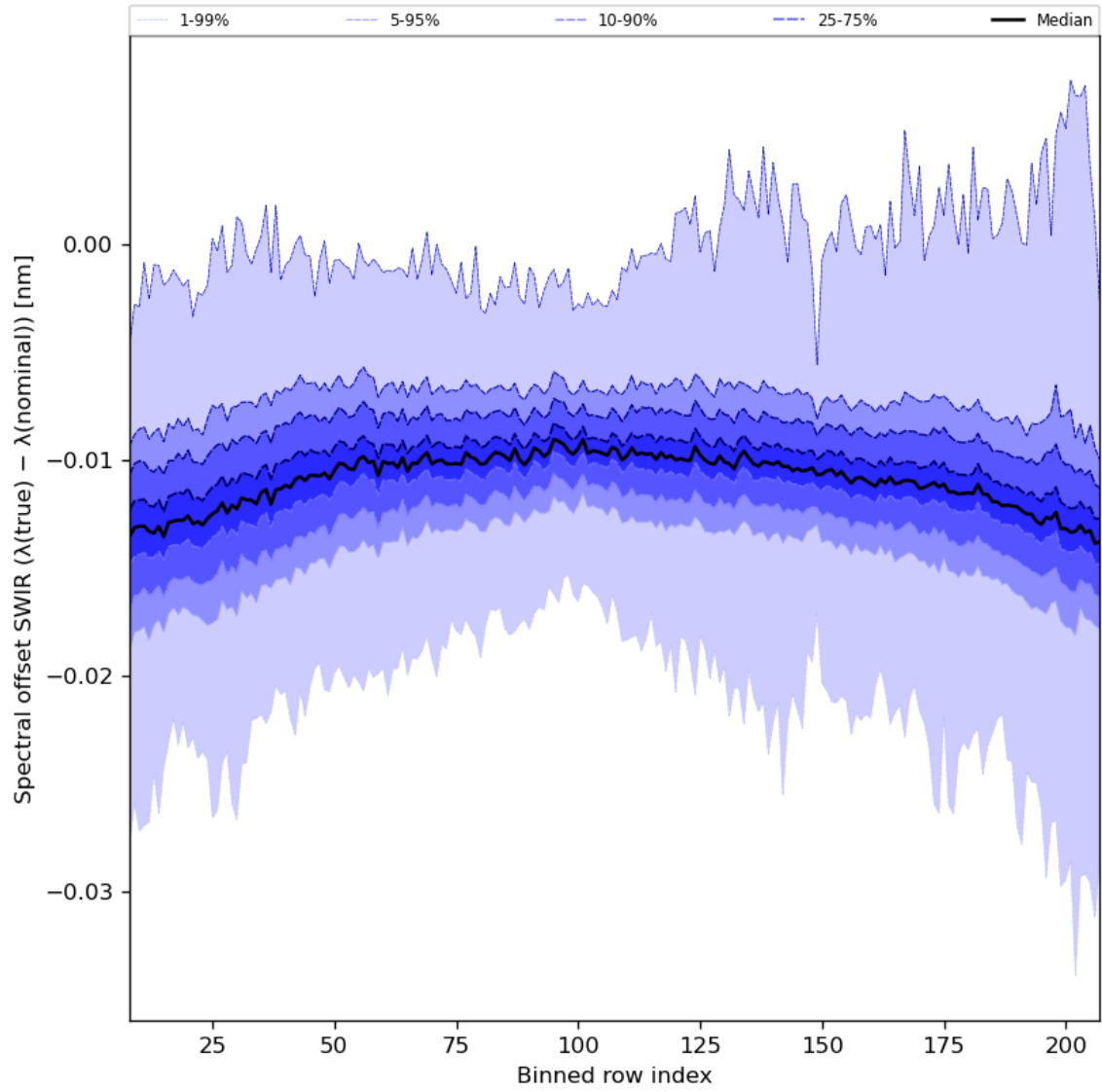
Figure 38: Along track statistics of “Spectral offset SWIR ( \lambda(\text{true}) - \lambda(\text{nominal}) )” for 2024-07-21 to 2024-07-23
