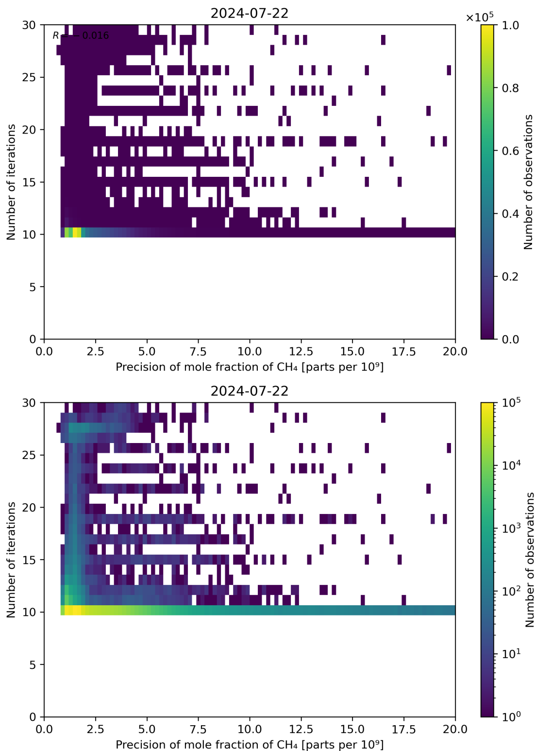
Figure 83: Scatter density plot of “Precision of mole fraction of CH 4 ” against “Number of iterations” for 2024-07-21 to 2024-07-23.
