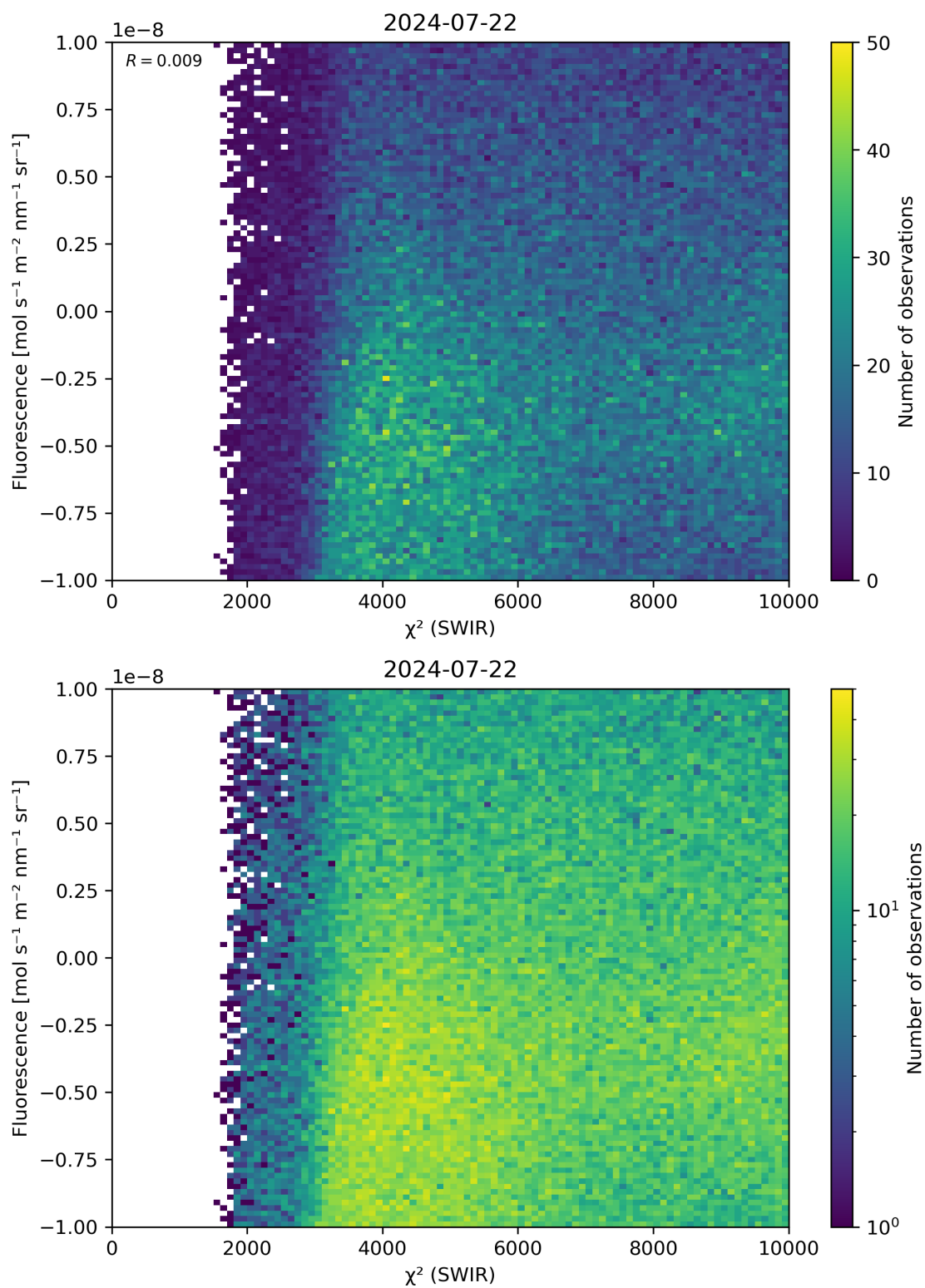
Figure 49: Scatter density plot of “ \chi^2 (SWIR)” against “Fluorescence” for 2024-07-21 to 2024-07-23.
