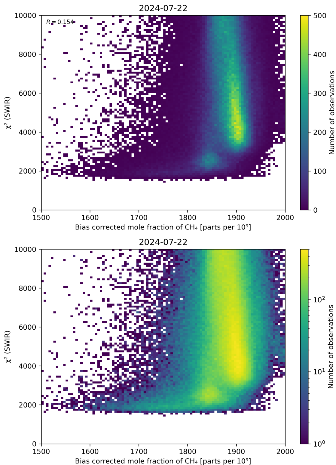
Figure 64: Scatter density plot of “Bias corrected mole fraction of CH 4 ” against “ \chi^2 (SWIR)” for 2024-07-21 to 2024-07-23.
