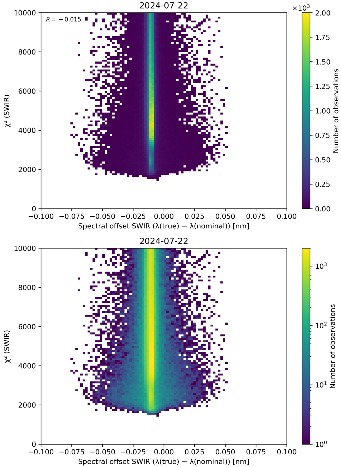
Figure 118: Scatter density plot of “Spectral offset SWIR ( \lambda(\text{true}) - \lambda(\text{nominal}) )” against “ \chi^2 (SWIR)” for 2024-07-21 to 2024-07-23.
