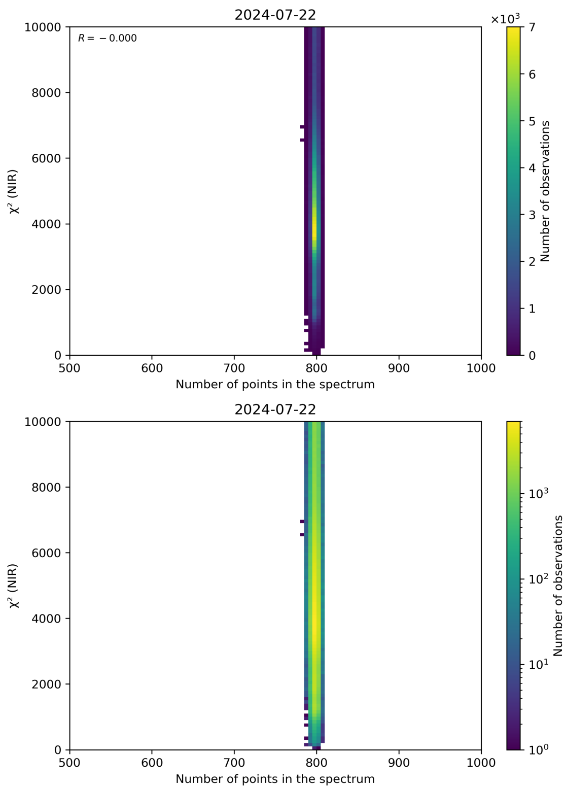
Figure 88: Scatter density plot of “Number of points in the spectrum” against “ \chi^2 (NIR)” for 2024-07-21 to 2024-07-23.
