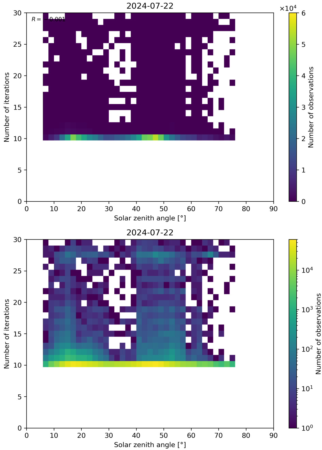
Figure 102: Scatter density plot of “Solar zenith angle” against “Number of iterations” for 2024-07-21 to 2024-07-23.
