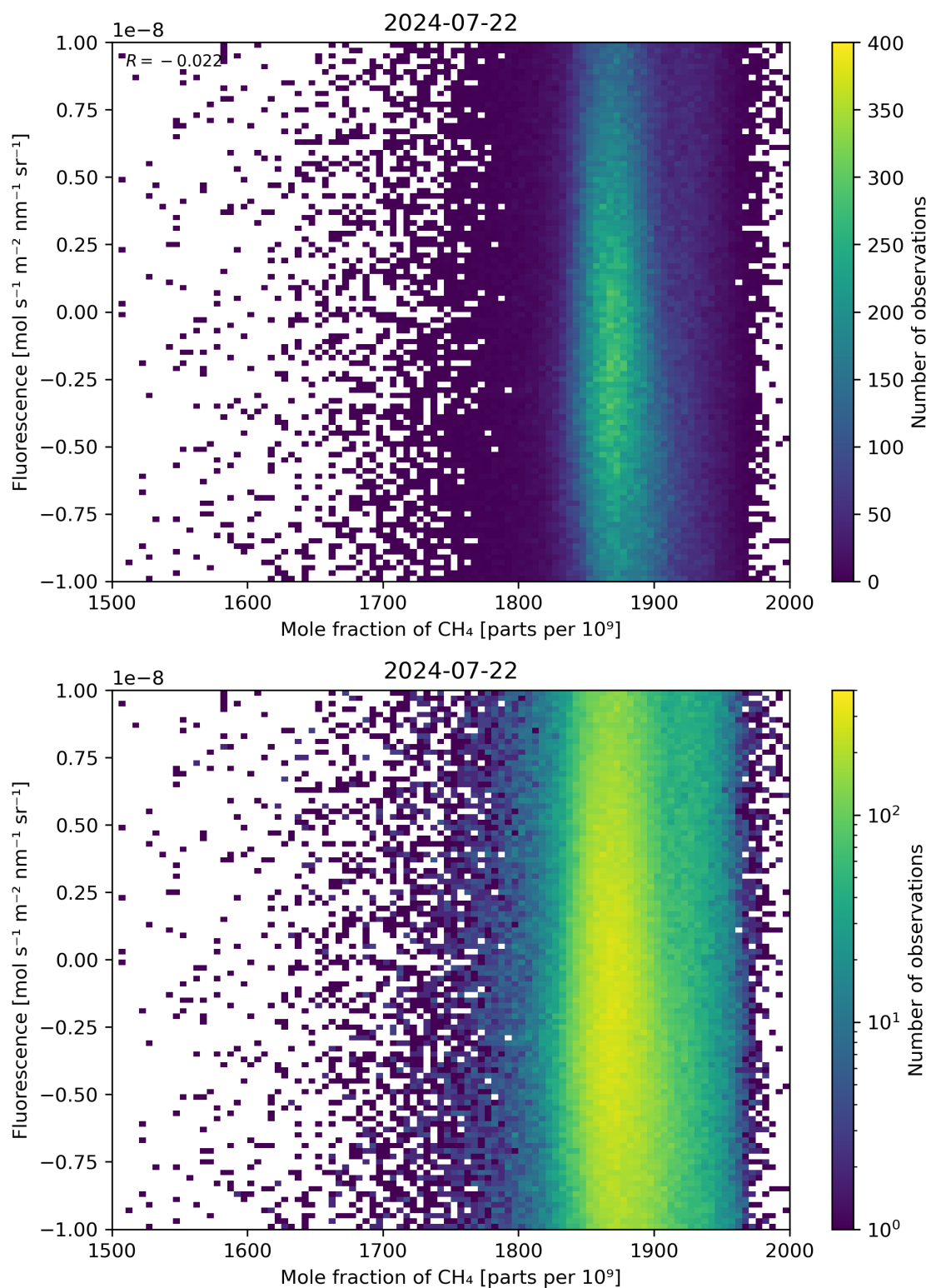
Figure 73: Scatter density plot of “Mole fraction of \text{CH}_4 ” against “Fluorescence” for 2024-07-21 to 2024-07-23.
