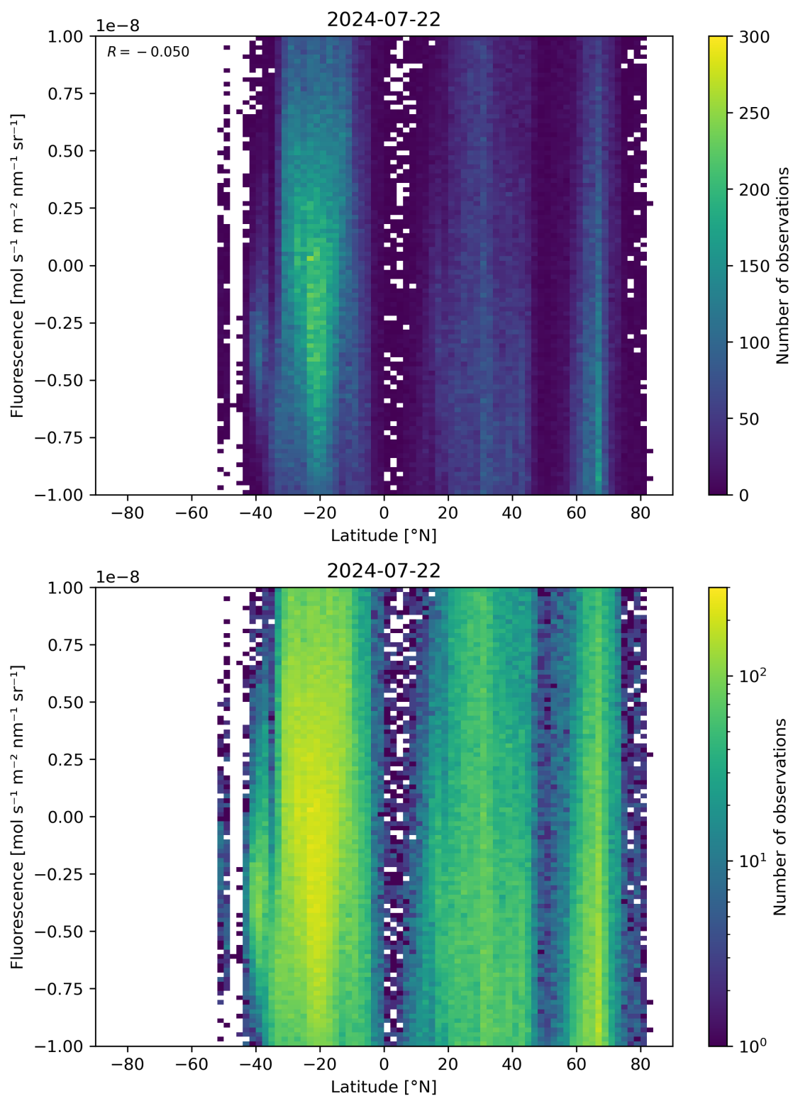
Figure 56: Scatter density plot of “Latitude” against “Fluorescence” for 2024-07-21 to 2024-07-23.
