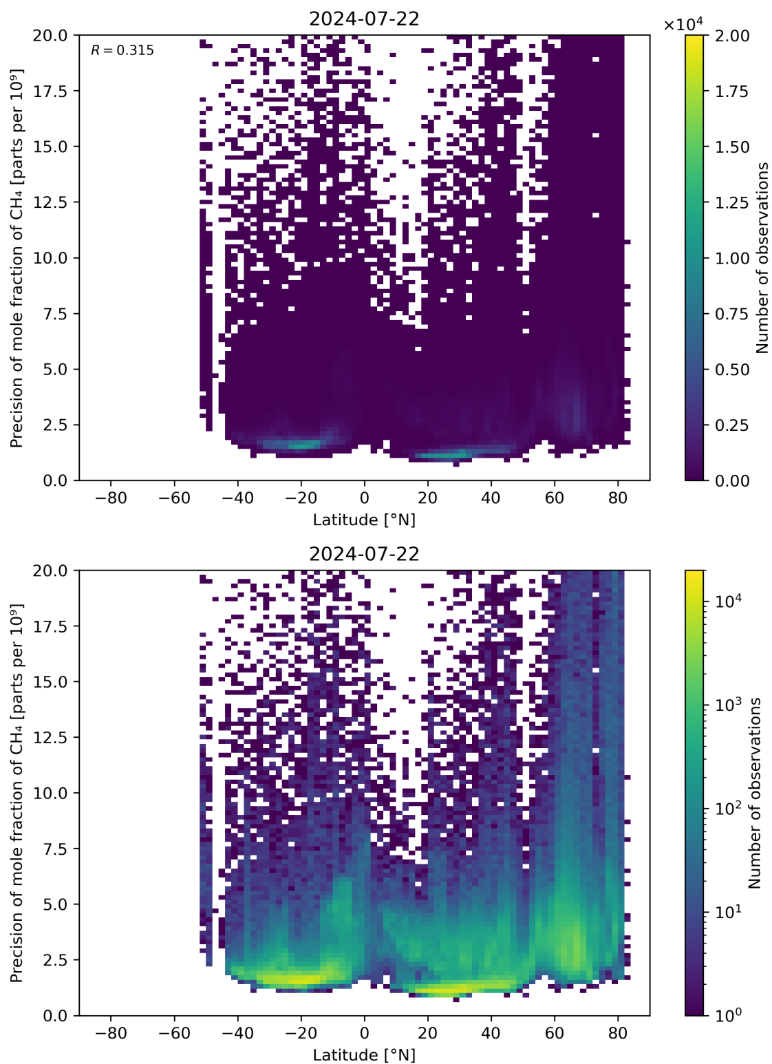
Figure 59: Scatter density plot of “Latitude” against “Precision of mole fraction of \text{CH}_4 ” for 2024-07-21 to 2024-07-23.
