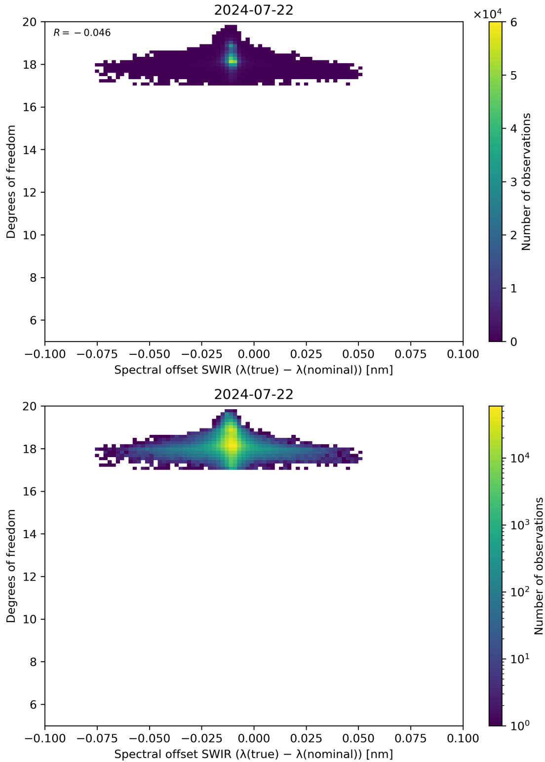
Figure 119: Scatter density plot of “Spectral offset SWIR ( \lambda(\text{true}) - \lambda(\text{nominal}) )” against “Degrees of freedom” for 2024-07-21 to 2024-07-23.
