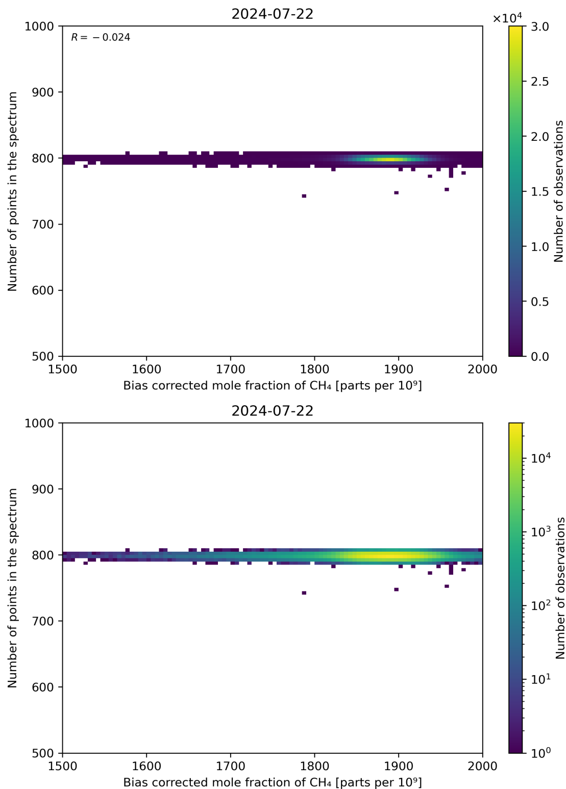
Figure 68: Scatter density plot of “Bias corrected mole fraction of CH 4 ” against “Number of points in the spectrum” for 2024-07-21 to 2024-07-23.
