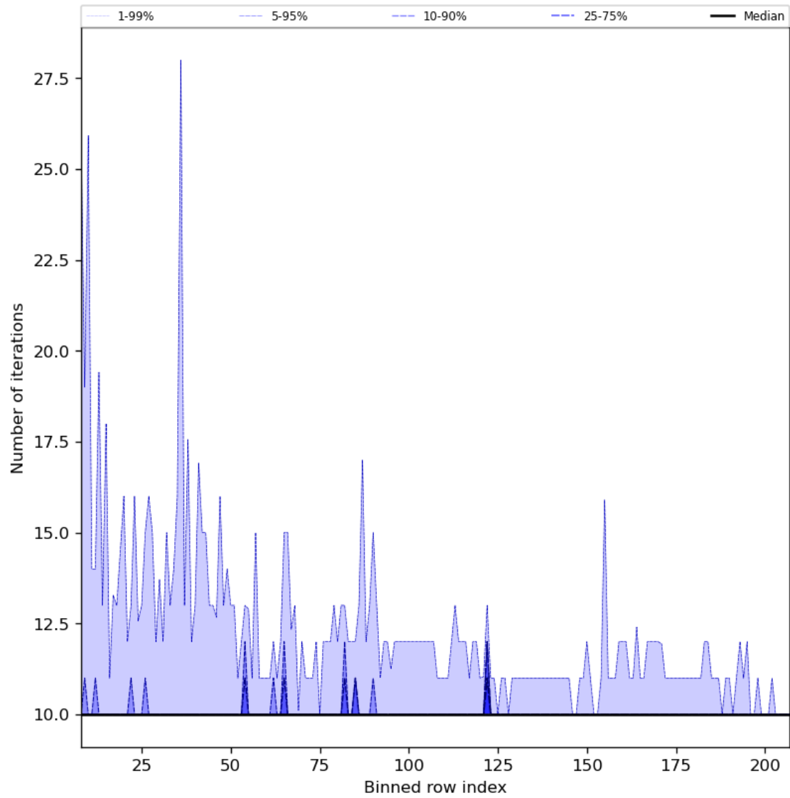
Figure 42: Along track statistics of “Number of iterations” for 2024-07-21 to 2024-07-23
