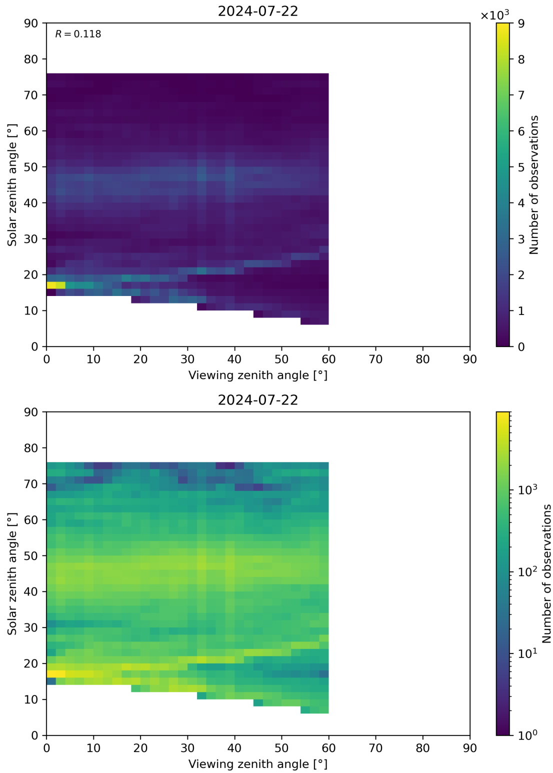
Figure 115: Scatter density plot of “Viewing zenith angle” against “Solar zenith angle” for 2024-07-21 to 2024-07-23.
