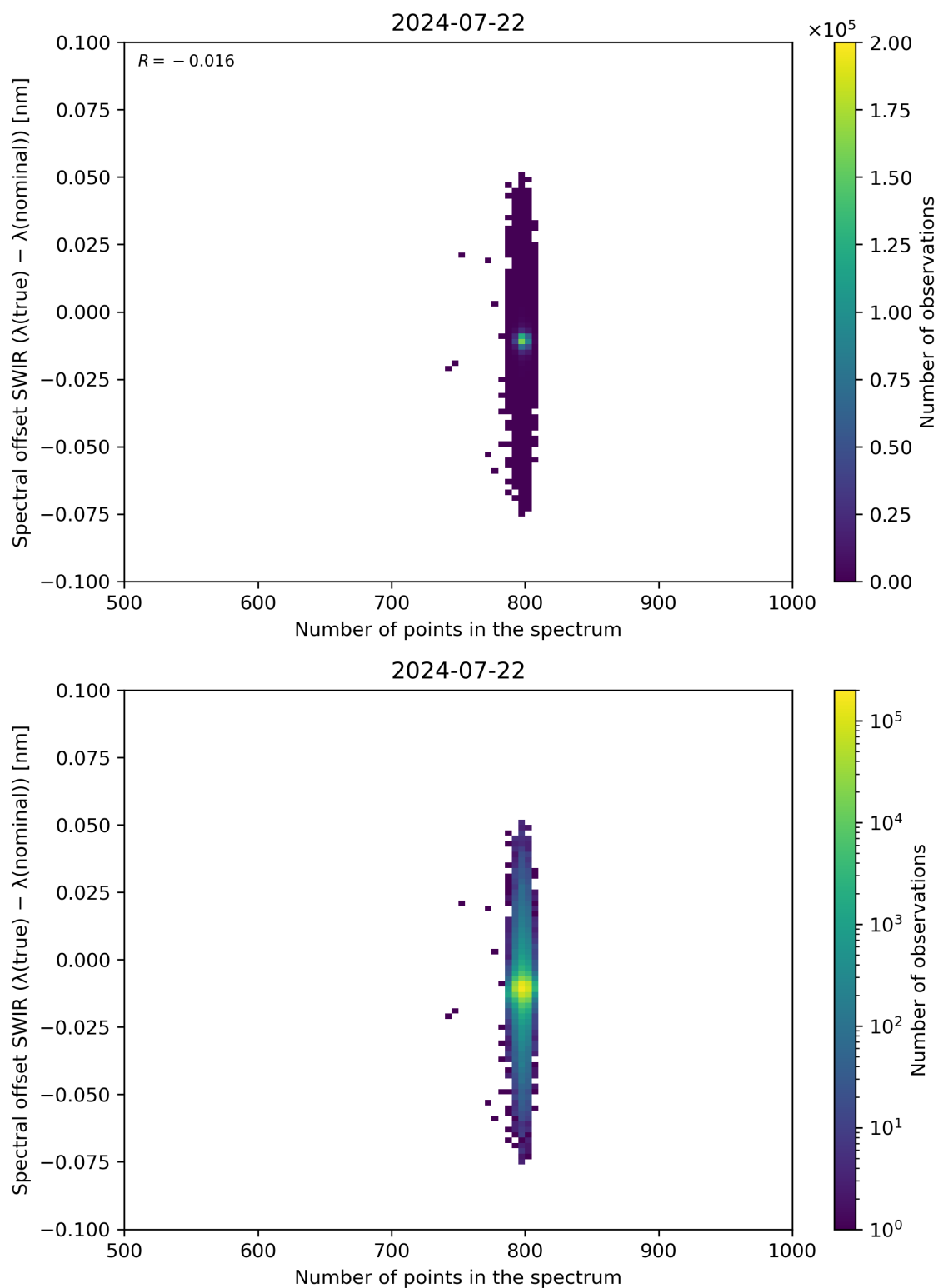
Figure 93: Scatter density plot of “Number of points in the spectrum” against “Spectral offset SWIR ( \lambda(\text{true}) - \lambda(\text{nominal}) )” for 2024-07-21 to 2024-07-23.
