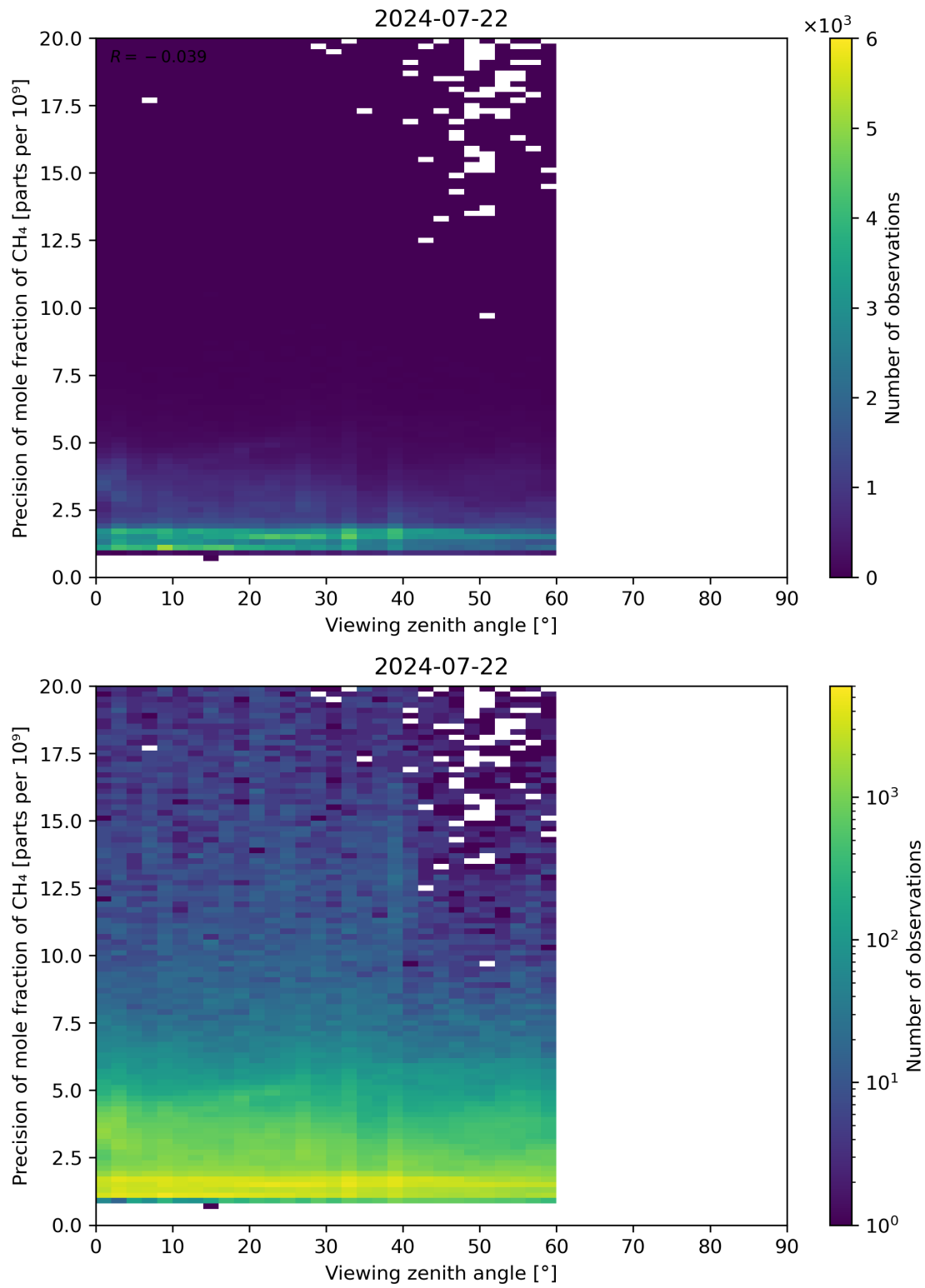
Figure 112: Scatter density plot of “Viewing zenith angle” against “Precision of mole fraction of \text{CH}_4 ” for 2024-07-21 to 2024-07-23.
