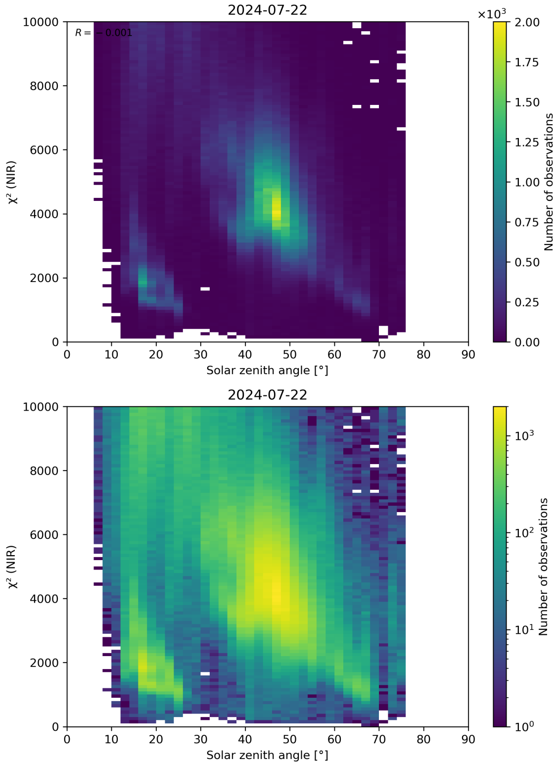
Figure 94: Scatter density plot of “Solar zenith angle” against “ \chi^2 (NIR)” for 2024-07-21 to 2024-07-23.
