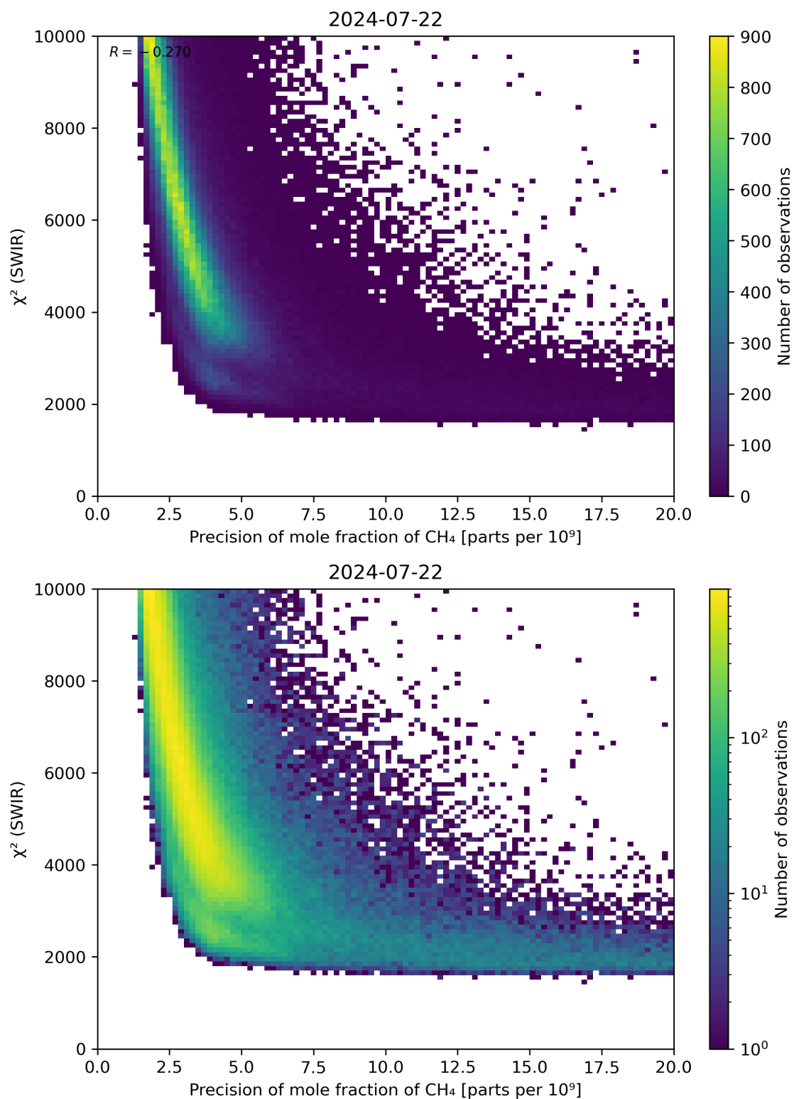
Figure 79: Scatter density plot of “Precision of mole fraction of \text{CH}_4 ” against “ \chi^2 (SWIR)” for 2024-07-21 to 2024-07-23.
