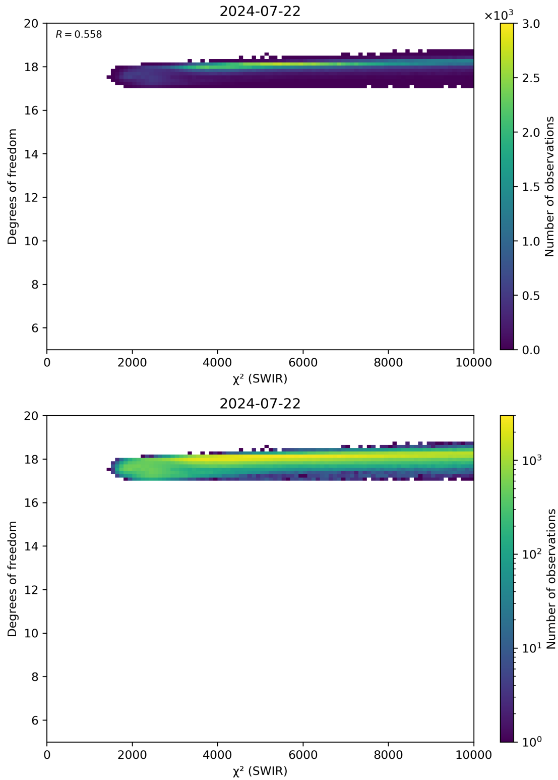
Figure 48: Scatter density plot of “ \chi^2 (SWIR)” against “Degrees of freedom” for 2024-07-21 to 2024-07-23.
