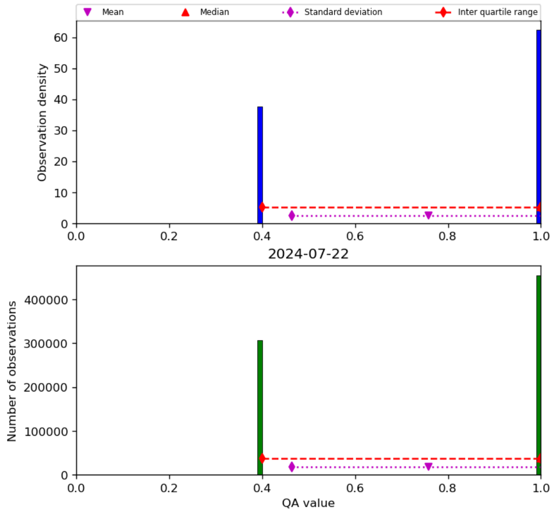
Figure 22: Histogram of “QA value” for 2024-07-21 to 2024-07-23
