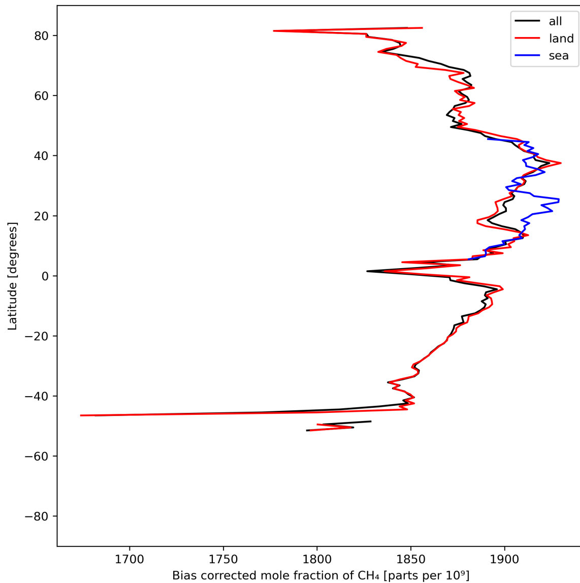
Figure 14: Zonal average of “Bias corrected mole fraction of CH 4 ” for 2024-07-21 to 2024-07-23.
