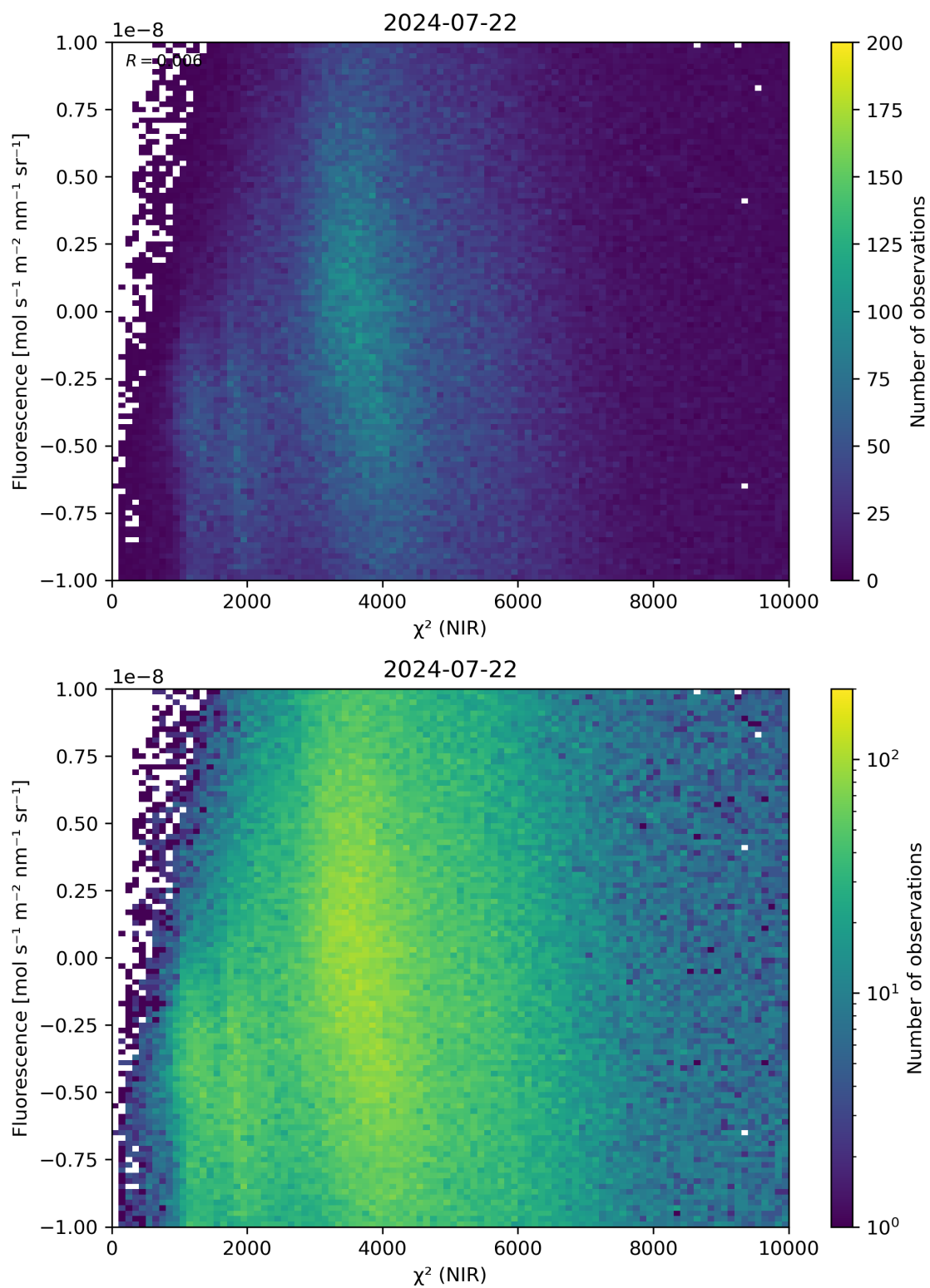
Figure 45: Scatter density plot of “ \chi^2 (NIR)” against “Fluorescence” for 2024-07-21 to 2024-07-23.
