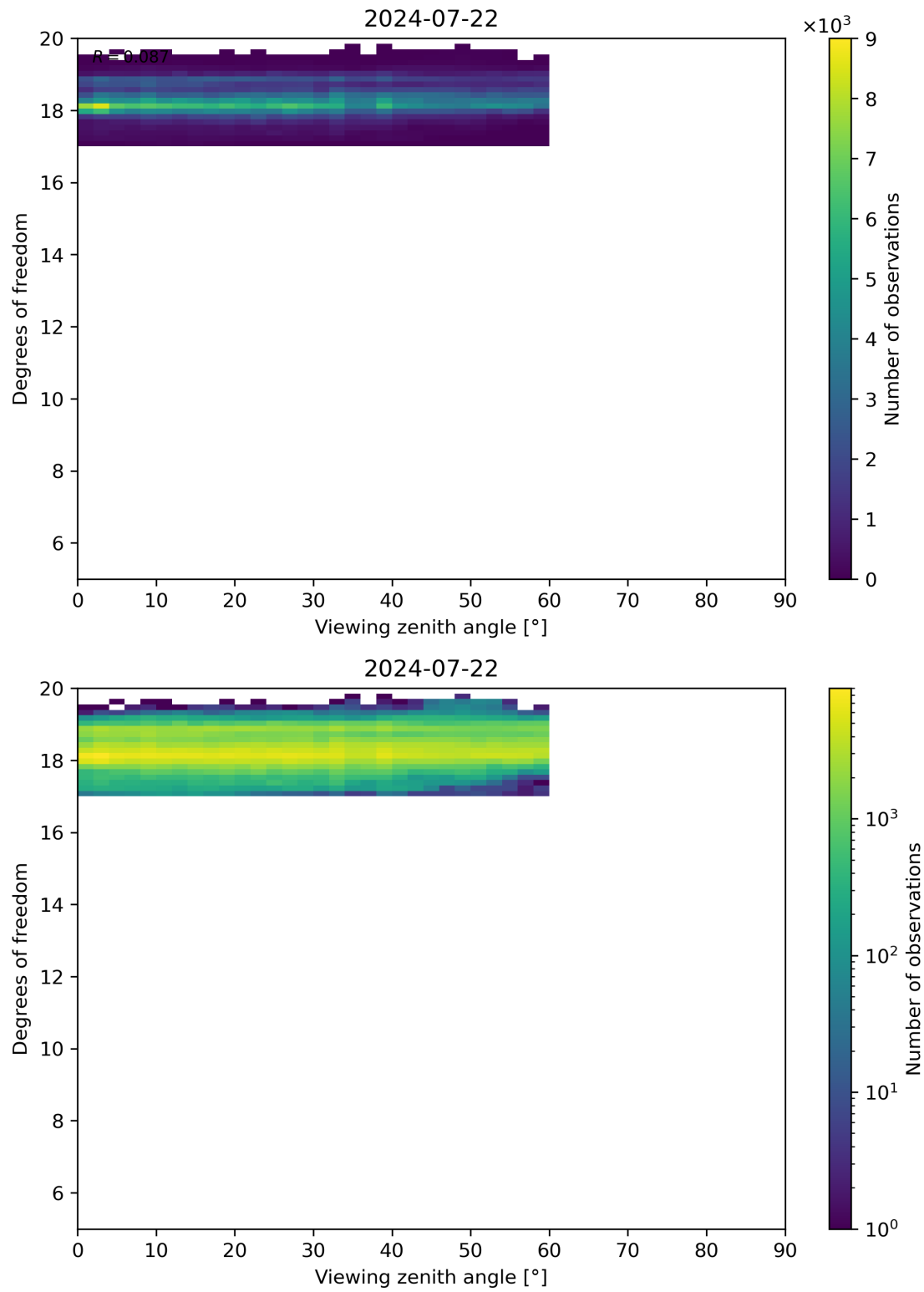
Figure 107: Scatter density plot of “Viewing zenith angle” against “Degrees of freedom” for 2024-07-21 to 2024-07-23.
