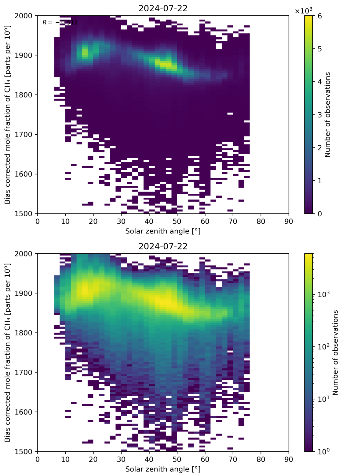
Figure 100: Scatter density plot of “Solar zenith angle” against “Bias corrected mole fraction of CH 4 ” for 2024-07-21 to 2024-07-23.
