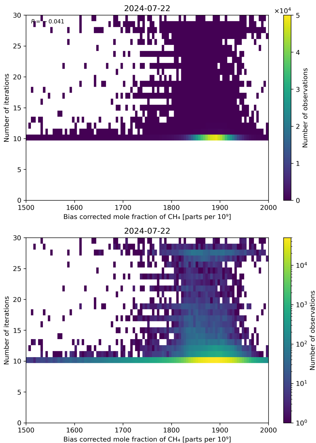
Figure 67: Scatter density plot of “Bias corrected mole fraction of CH 4 ” against “Number of iterations” for 2024-07-21 to 2024-07-23.
