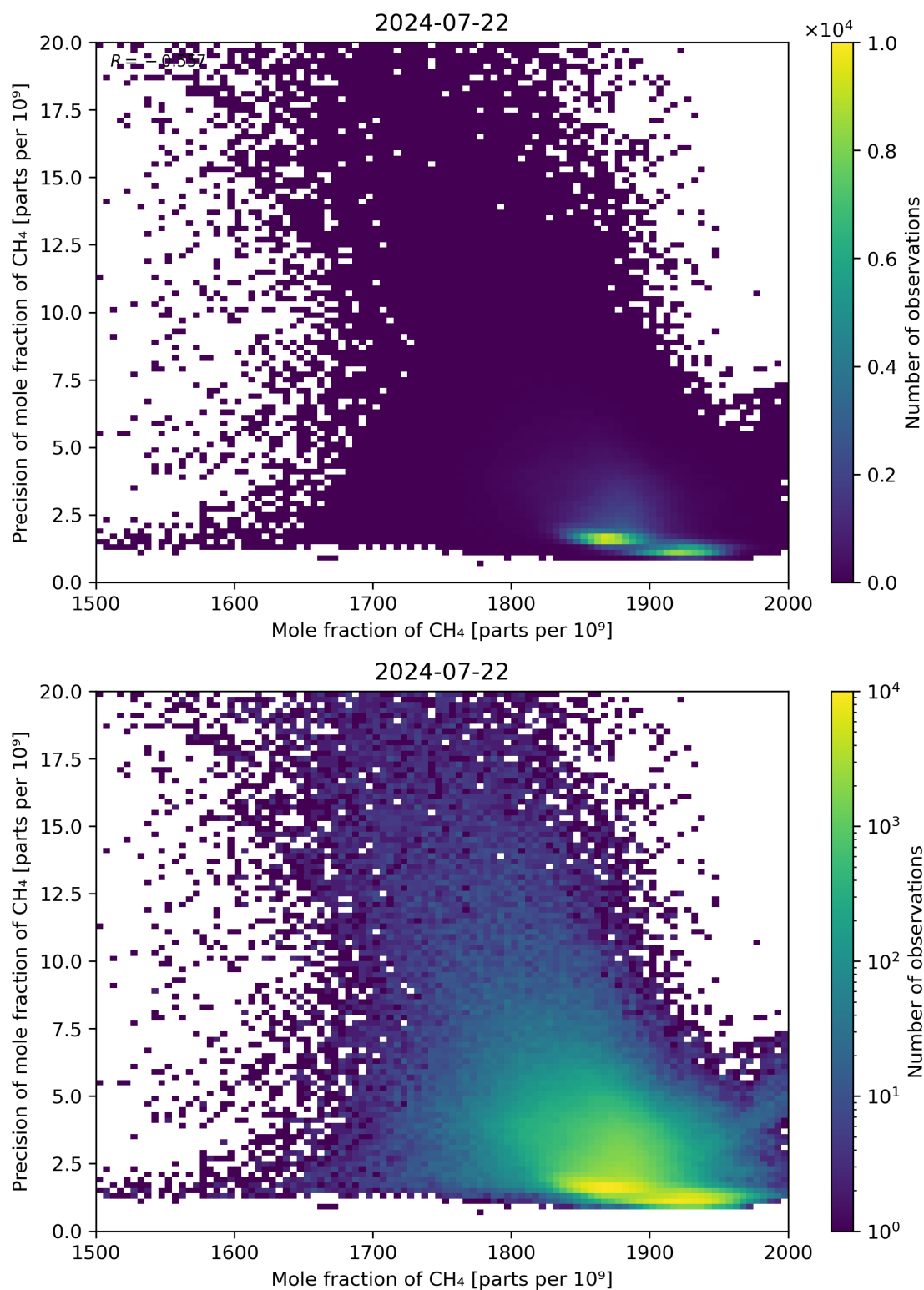
Figure 75: Scatter density plot of “Mole fraction of CH 4 ” against “Precision of mole fraction of CH 4 ” for 2024-07-21 to 2024-07-23.
