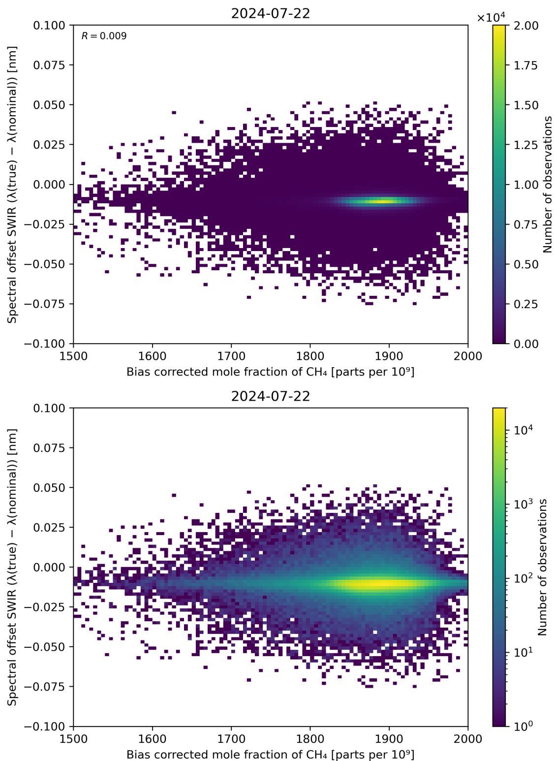
Figure 69: Scatter density plot of “Bias corrected mole fraction of \text{CH}_4 ” against “Spectral offset SWIR ( \lambda(\text{true}) - \lambda(\text{nominal}) )” for 2024-07-21 to 2024-07-23.
