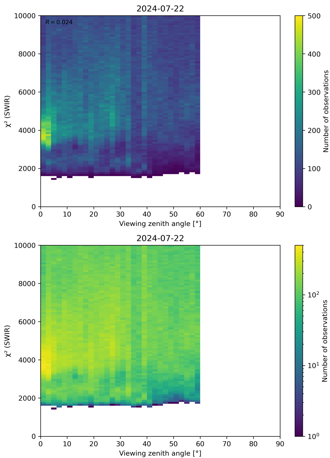
Figure 106: Scatter density plot of “Viewing zenith angle” against “ \chi^2 (SWIR)” for 2024-07-21 to 2024-07-23.
