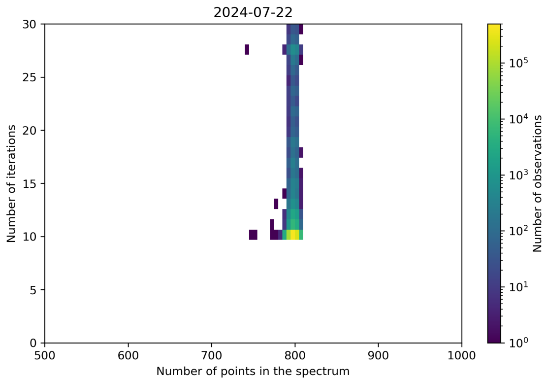
Figure 92: Scatter density plot of “Number of points in the spectrum” against “Number of iterations” for 2024-07-21 to 2024-07-23.
