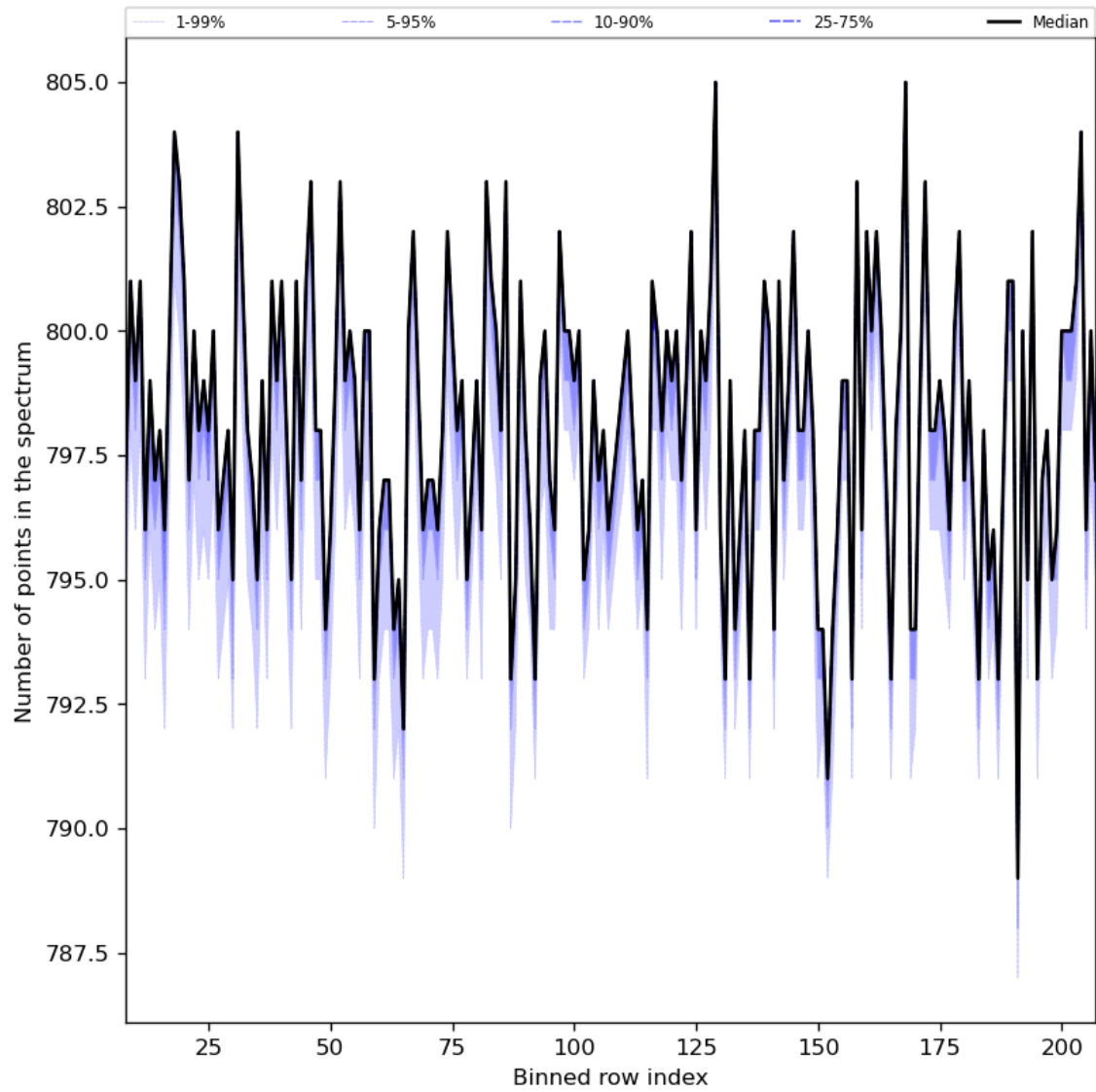
Figure 37: Along track statistics of “Number of points in the spectrum” for 2024-07-21 to 2024-07-23
