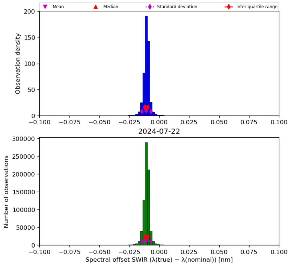
Figure 27: Histogram of “Spectral offset SWIR ( \lambda(\text{true}) - \lambda(\text{nominal}) )” for 2024-07-21 to 2024-07-23
