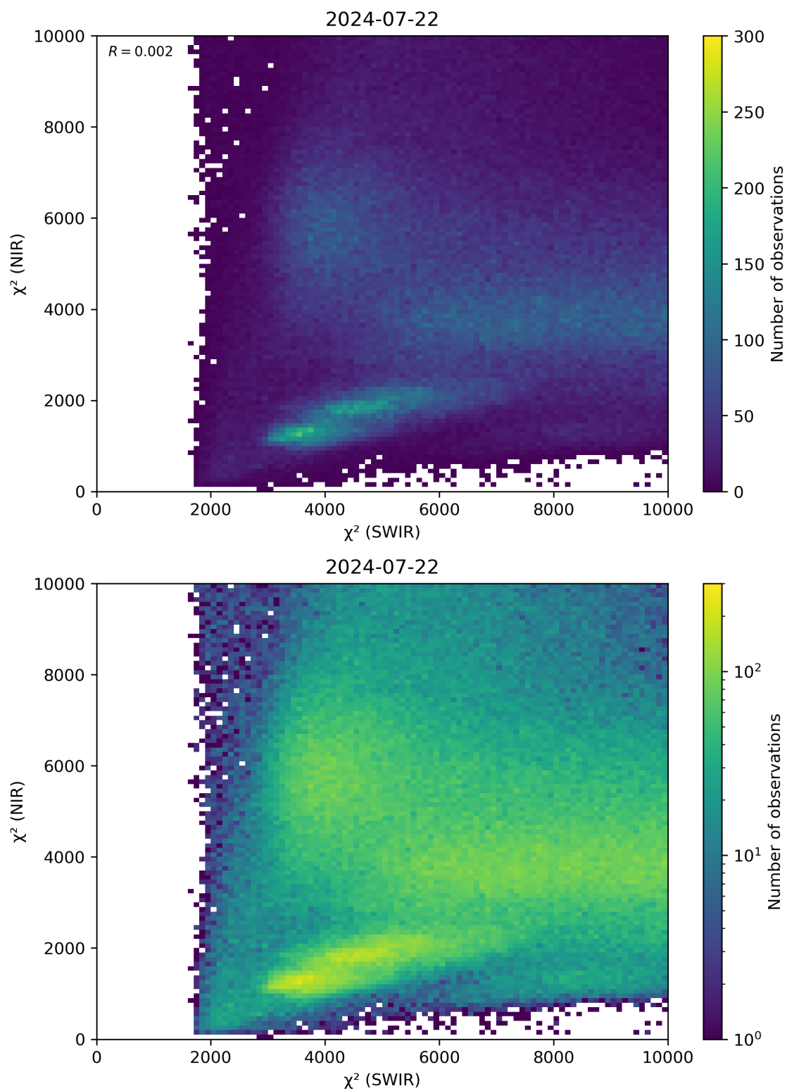
Figure 47: Scatter density plot of “ \chi^2 (SWIR)” against “ \chi^2 (NIR)” for 2024-07-21 to 2024-07-23.
