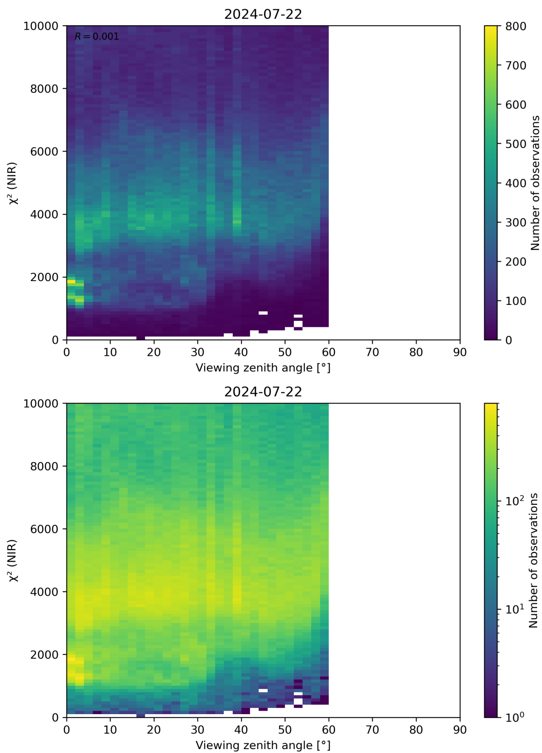
Figure 105: Scatter density plot of “Viewing zenith angle” against “ \chi^2 (NIR)” for 2024-07-21 to 2024-07-23.
