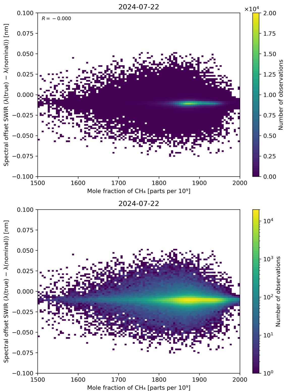
Figure 86: Scatter density plot of “Mole fraction of CH 4 ” against “Spectral offset SWIR ( \lambda(\text{true}) - \lambda(\text{nominal}) )” for 2024-07-21 to 2024-07-23.
