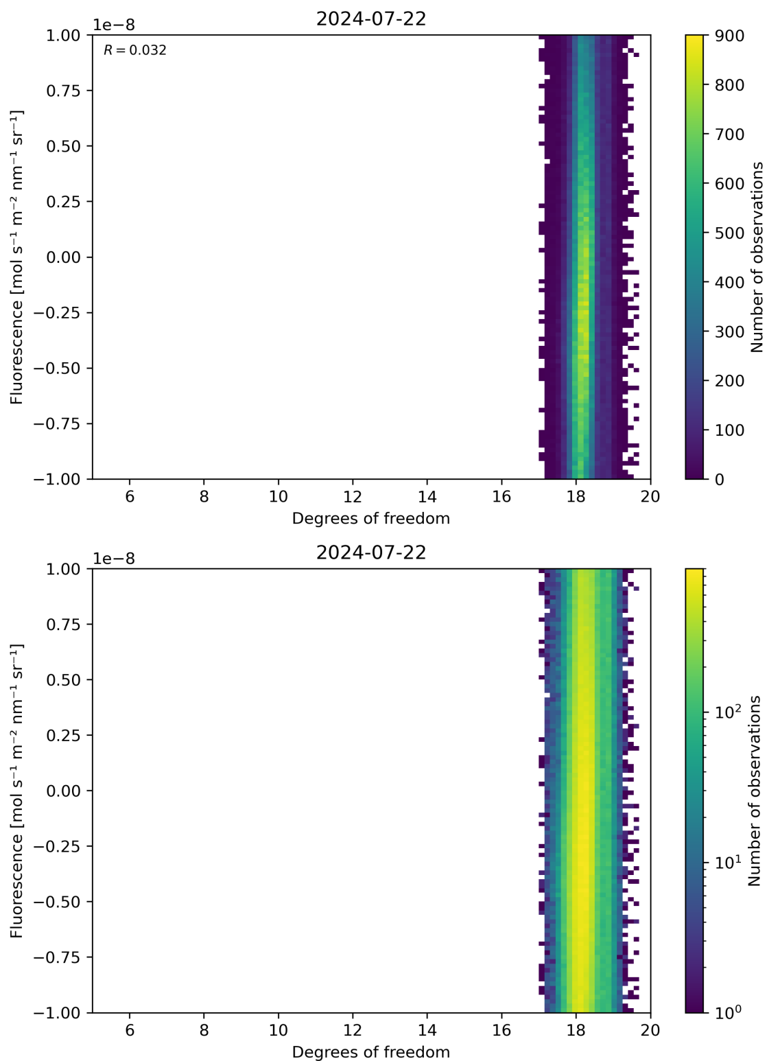
Figure 51: Scatter density plot of “Degrees of freedom” against “Fluorescence” for 2024-07-21 to 2024-07-23.
