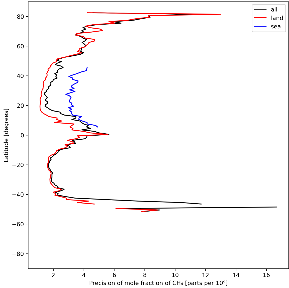
Figure 13: Zonal average of “Precision of mole fraction of CH 4 ” for 2024-07-21 to 2024-07-23.
