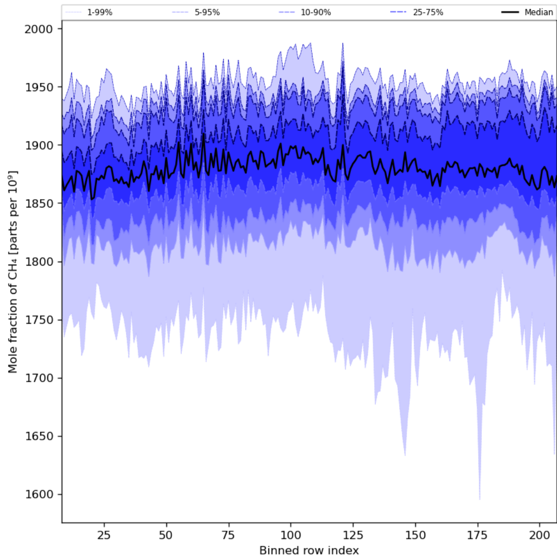
Figure 34: Along track statistics of “Mole fraction of CH 4 ” for 2024-07-21 to 2024-07-23
