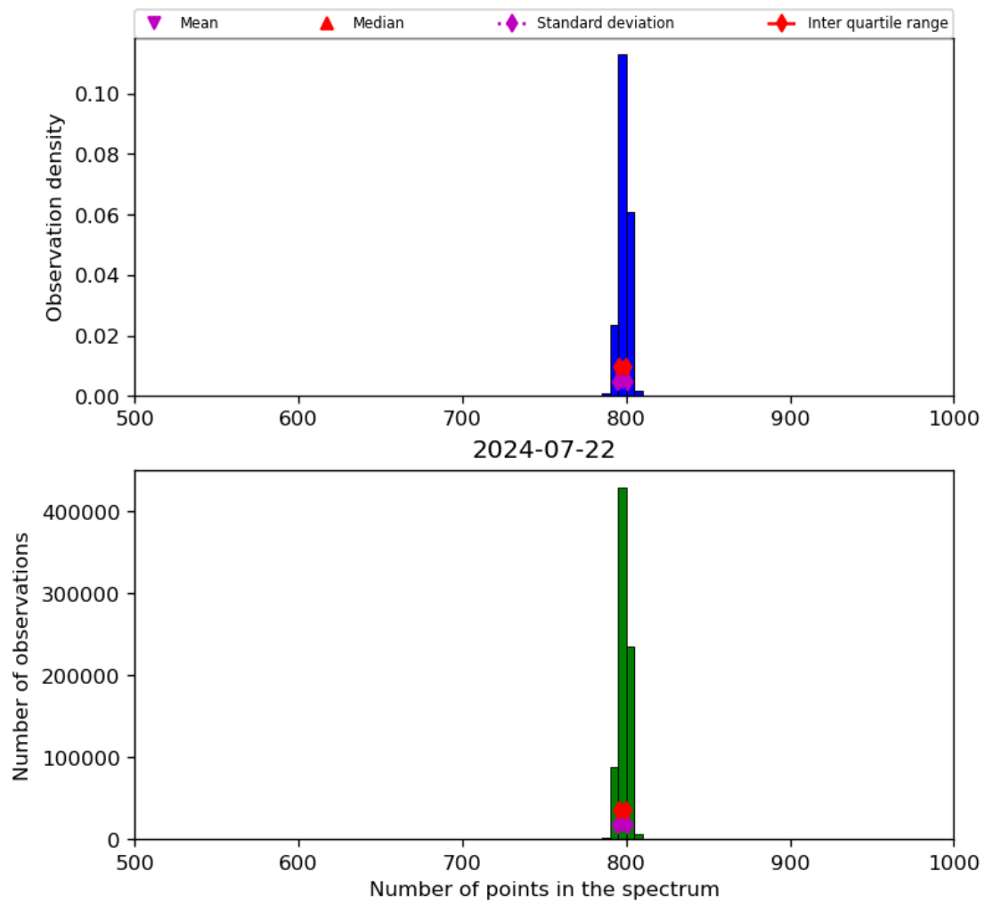
Figure 26: Histogram of “Number of points in the spectrum” for 2024-07-21 to 2024-07-23
