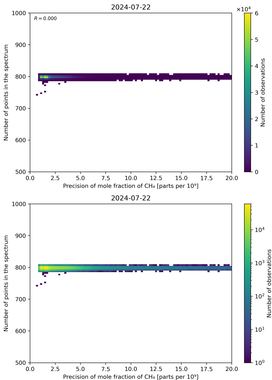
Figure 84: Scatter density plot of “Precision of mole fraction of CH 4 ” against “Number of points in the spectrum” for 2024-07-21 to 2024-07-23.
