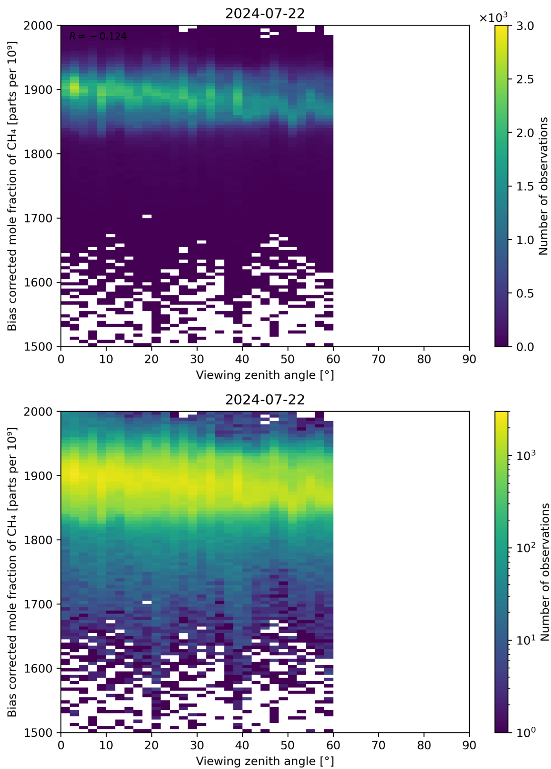
Figure 111: Scatter density plot of “Viewing zenith angle” against “Bias corrected mole fraction of CH 4 ” for 2024-07-21 to 2024-07-23.
