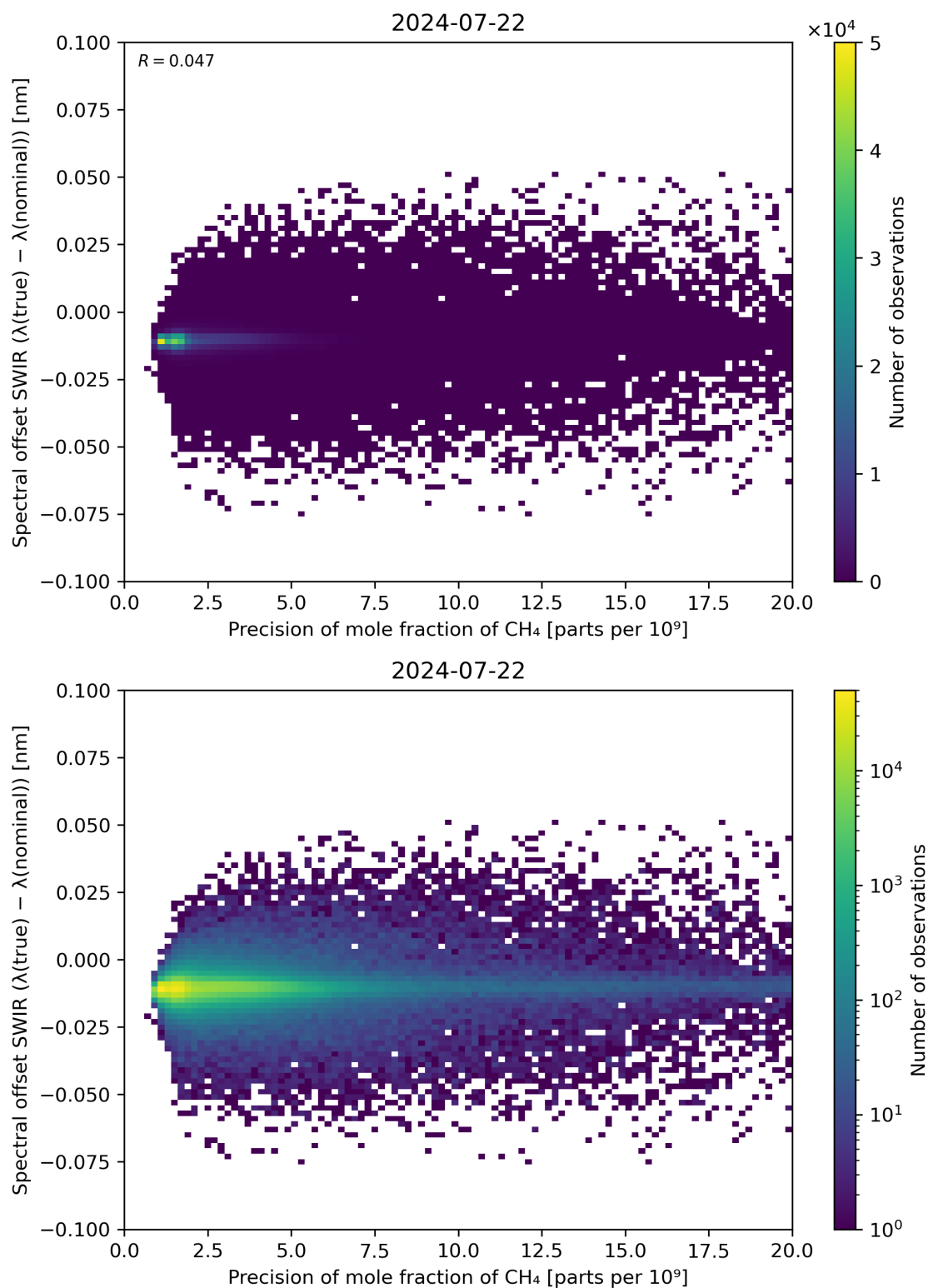
Figure 85: Scatter density plot of “Precision of mole fraction of \text{CH}_4 ” against “Spectral offset SWIR ( \lambda(\text{true}) - \lambda(\text{nominal}) )” for 2024-07-21 to 2024-07-23.
