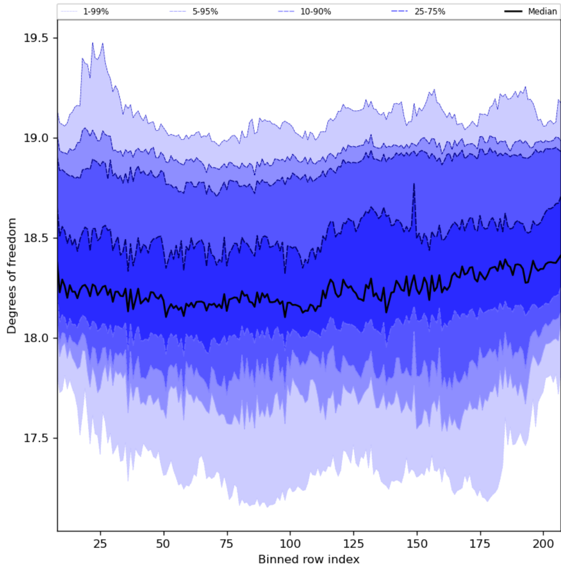
Figure 41: Along track statistics of “Degrees of freedom” for 2024-07-21 to 2024-07-23
