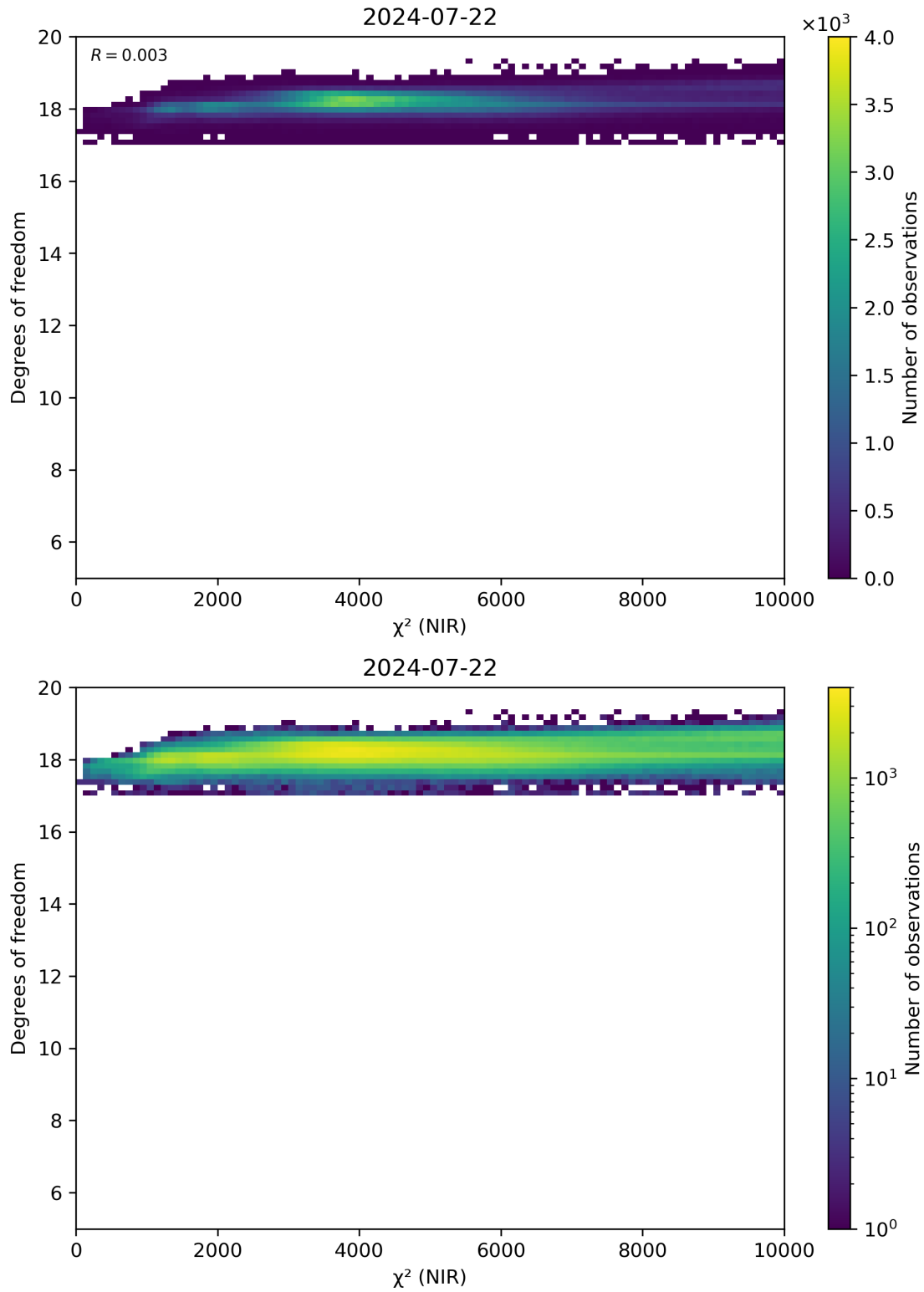
Figure 44: Scatter density plot of “ \chi^2 (NIR)” against “Degrees of freedom” for 2024-07-21 to 2024-07-23.
