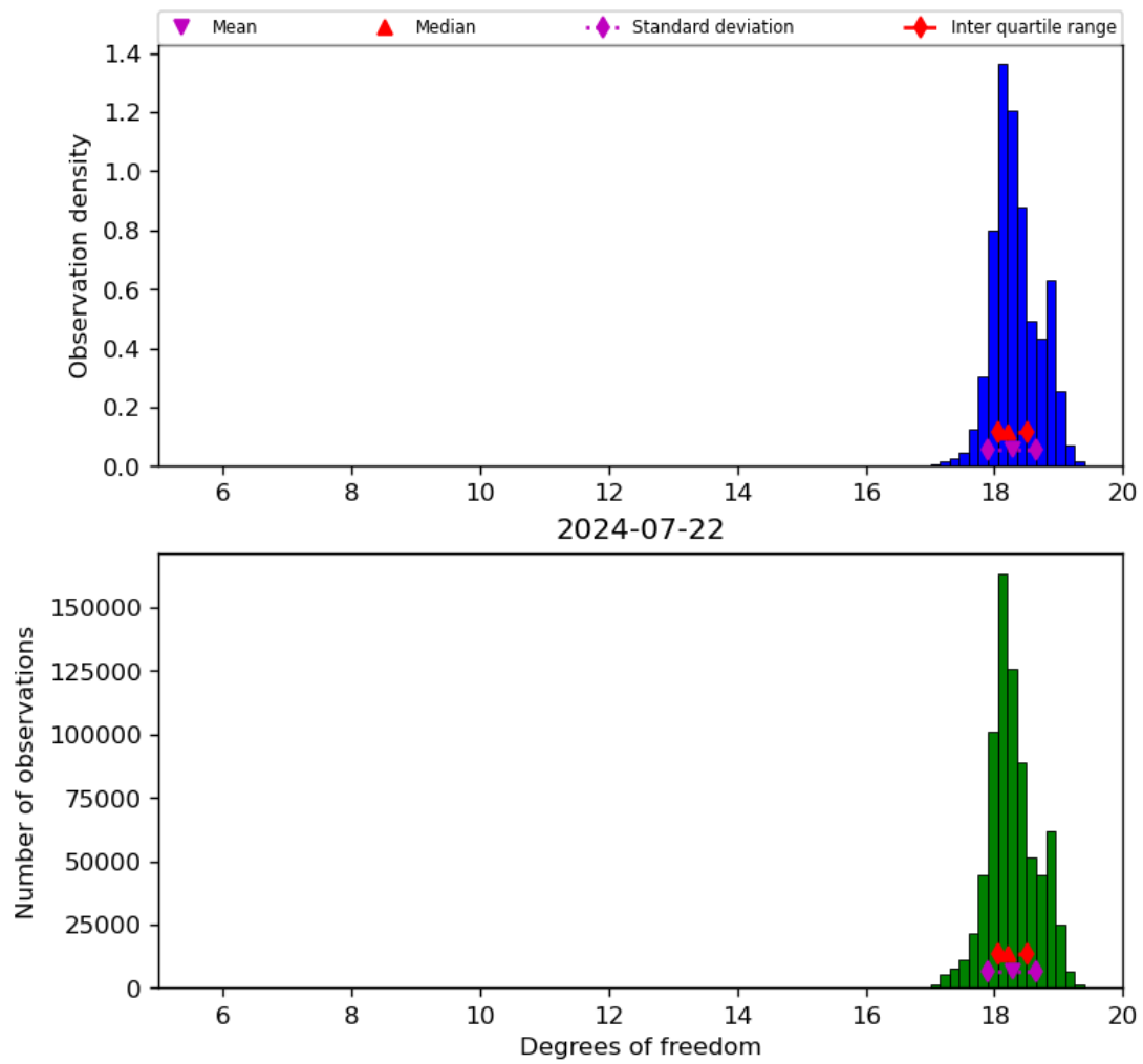
Figure 30: Histogram of “Degrees of freedom” for 2024-07-21 to 2024-07-23
