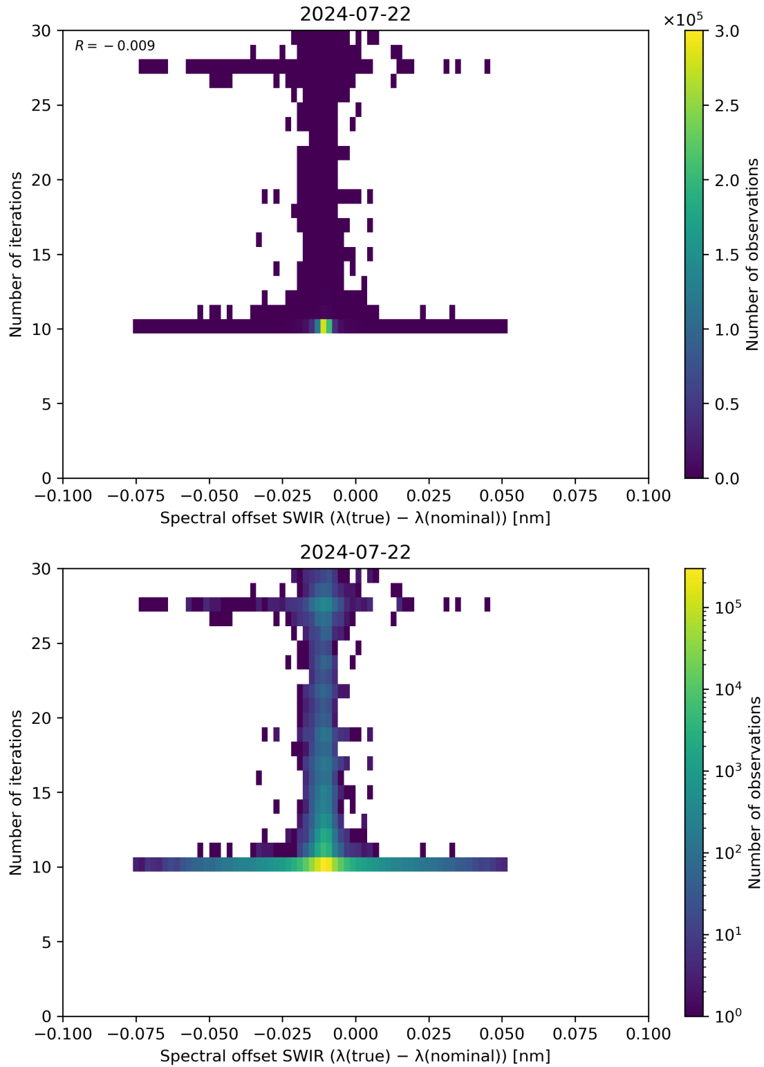
Figure 121: Scatter density plot of “Spectral offset SWIR ( \lambda(\text{true}) - \lambda(\text{nominal}) )” against “Number of iterations” for 2024-07-21 to 2024-07-23.
