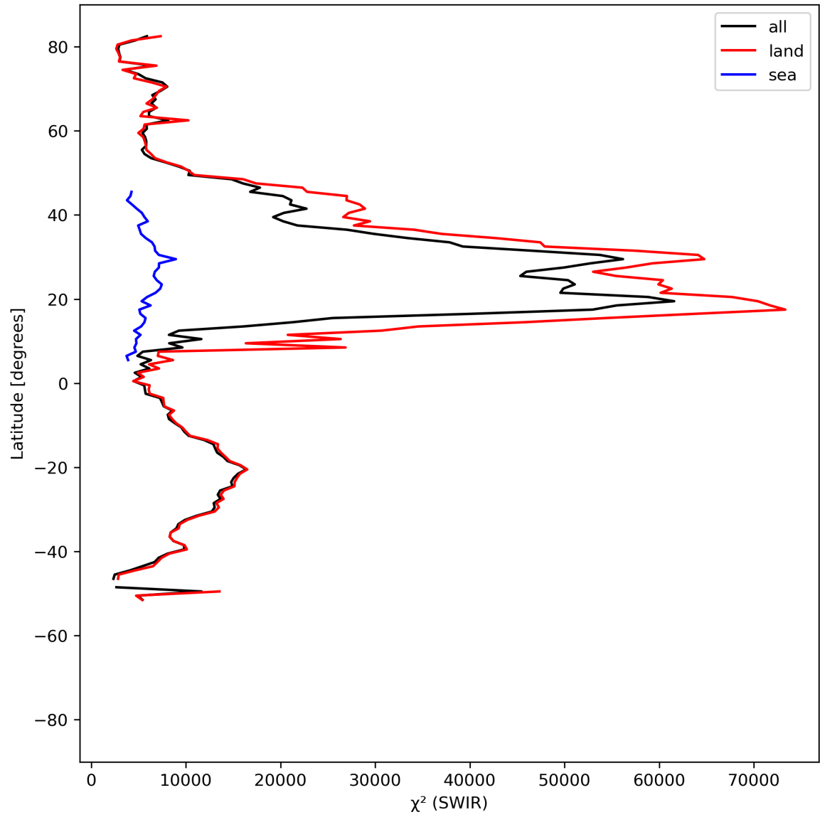
Figure 17: Zonal average of “ \chi^2 (SWIR)” for 2024-07-21 to 2024-07-23.
