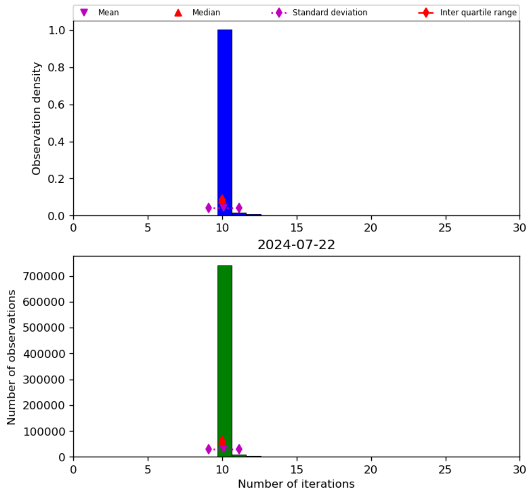
Figure 31: Histogram of “Number of iterations” for 2024-07-21 to 2024-07-23
