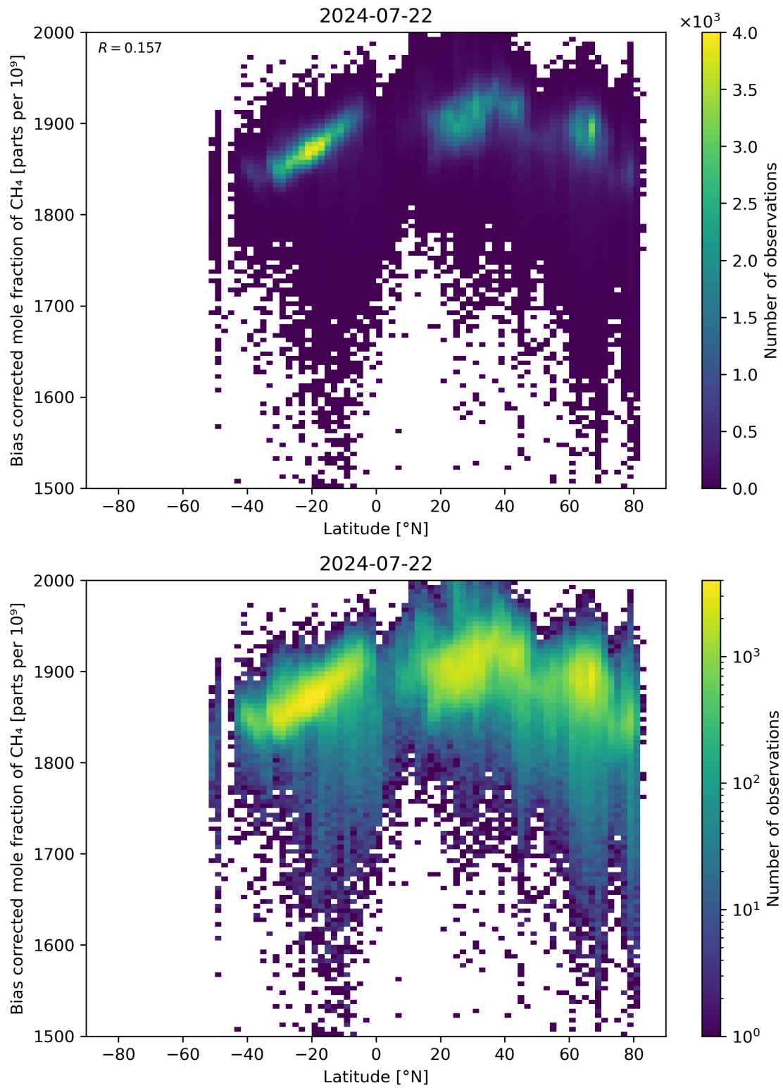
Figure 58: Scatter density plot of “Latitude” against “Bias corrected mole fraction of CH 4 ” for 2024-07-21 to 2024-07-23.
