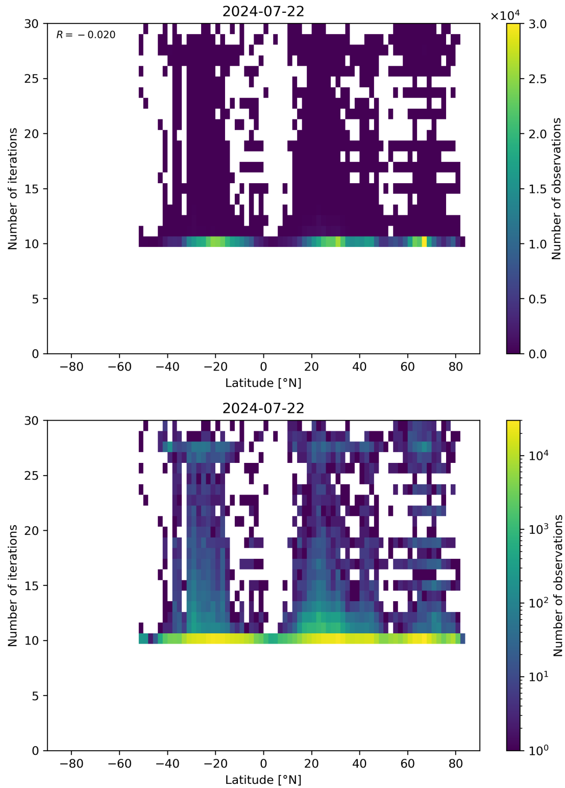
Figure 60: Scatter density plot of “Latitude” against “Number of iterations” for 2024-07-21 to 2024-07-23.
