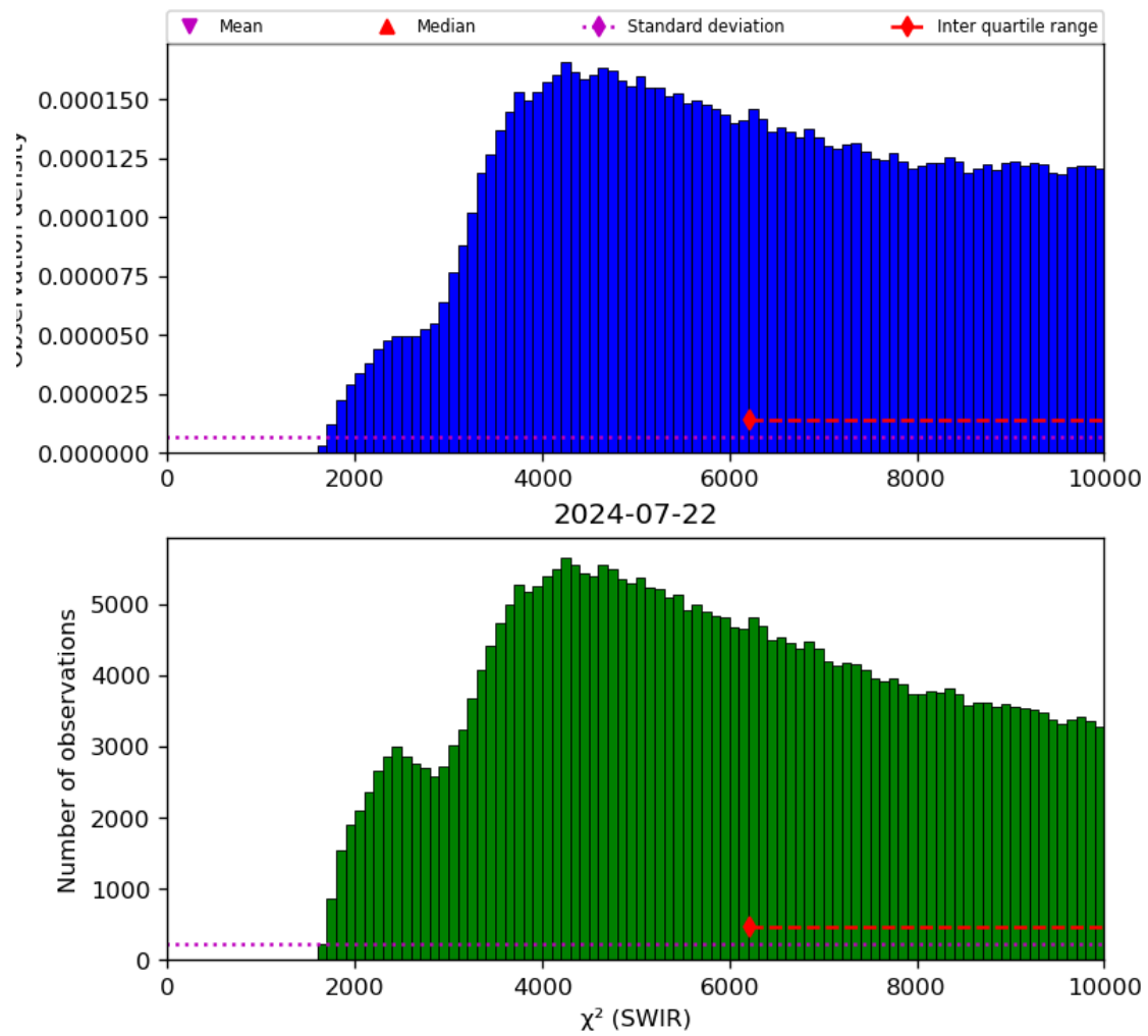
Figure 28: Histogram of “ \chi^2 (SWIR)” for 2024-07-21 to 2024-07-23
