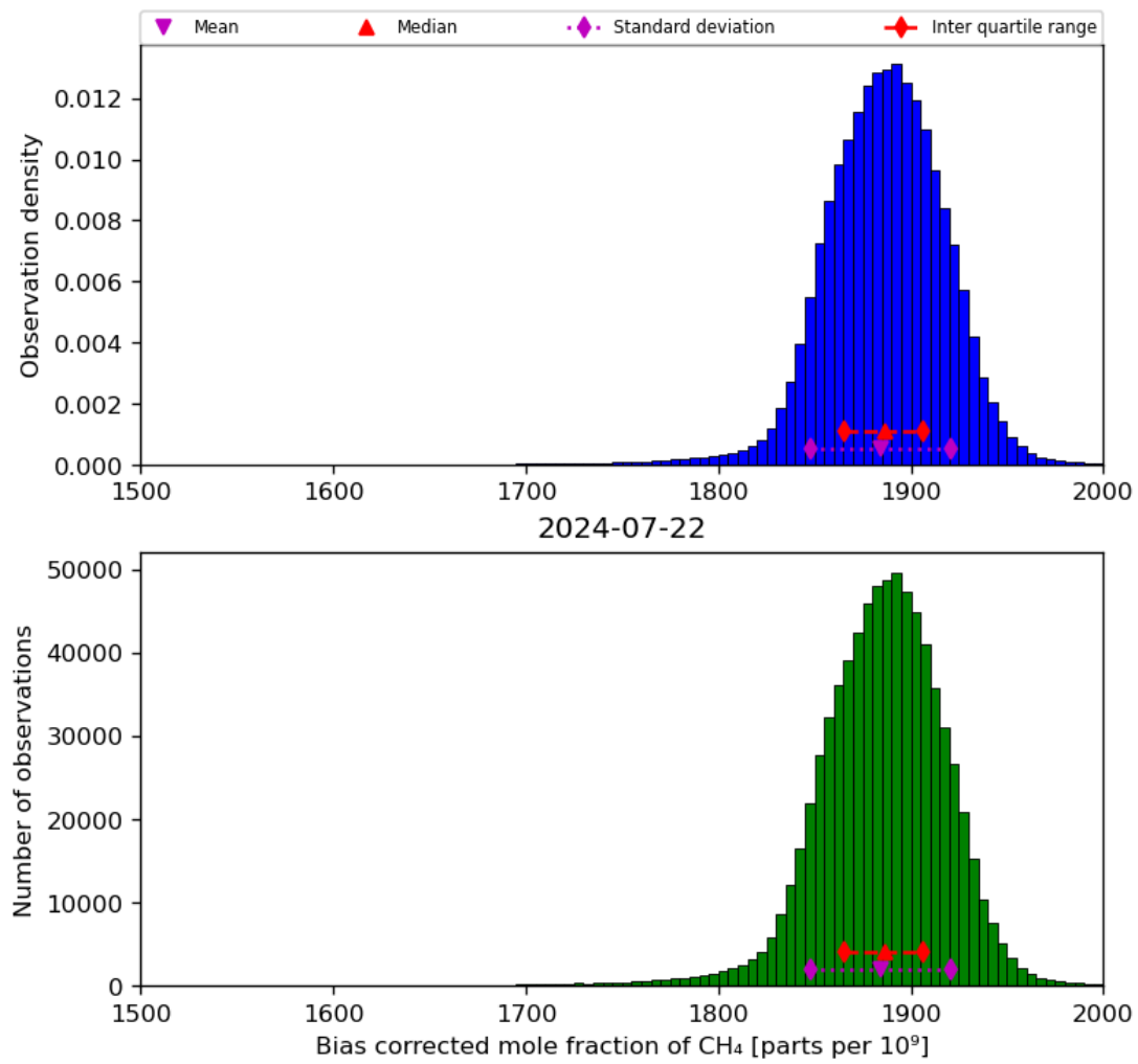
Figure 25: Histogram of “Bias corrected mole fraction of CH 4 ” for 2024-07-21 to 2024-07-23
