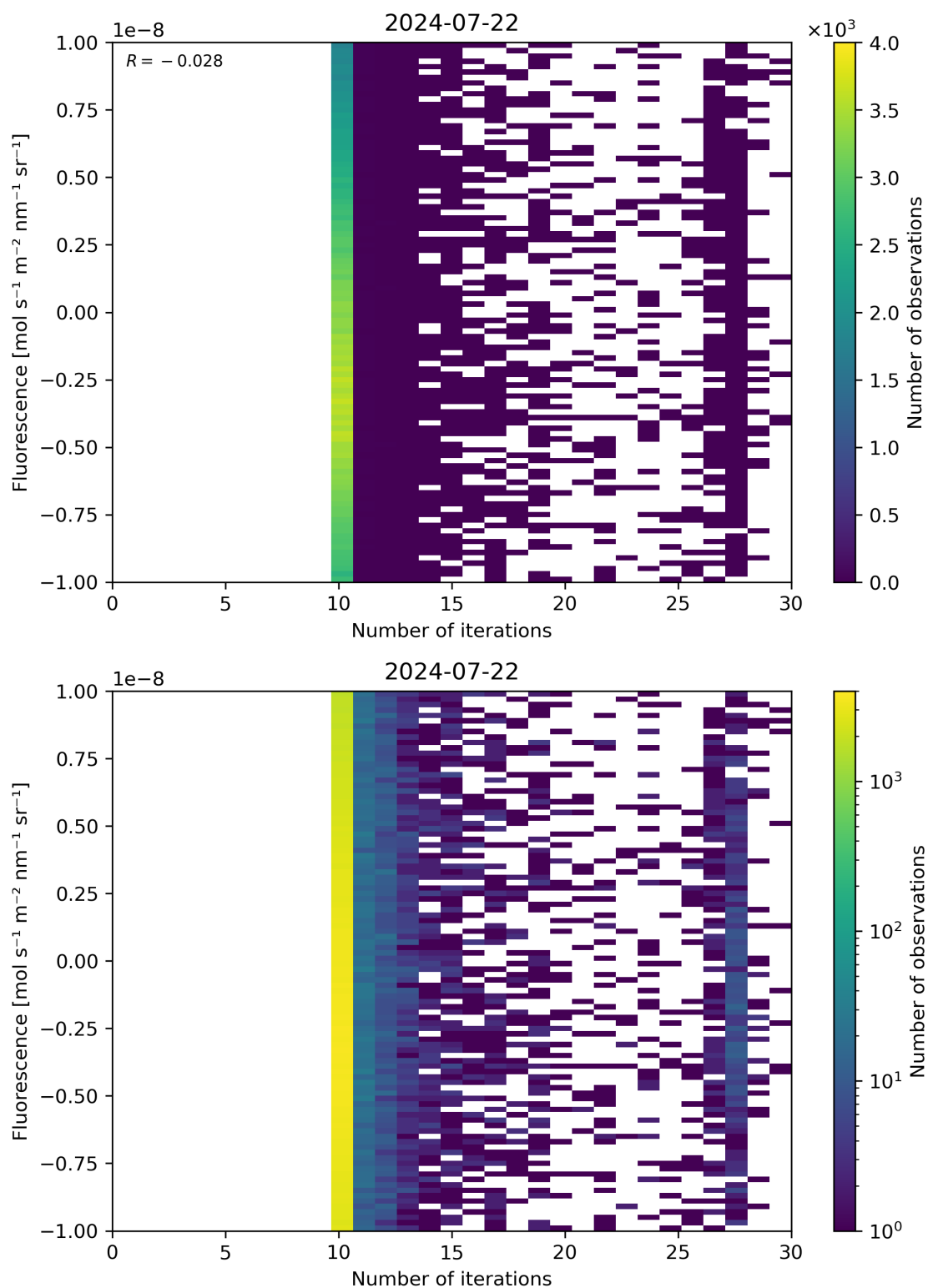
Figure 87: Scatter density plot of “Number of iterations” against “Fluorescence” for 2024-07-21 to 2024-07-23.
