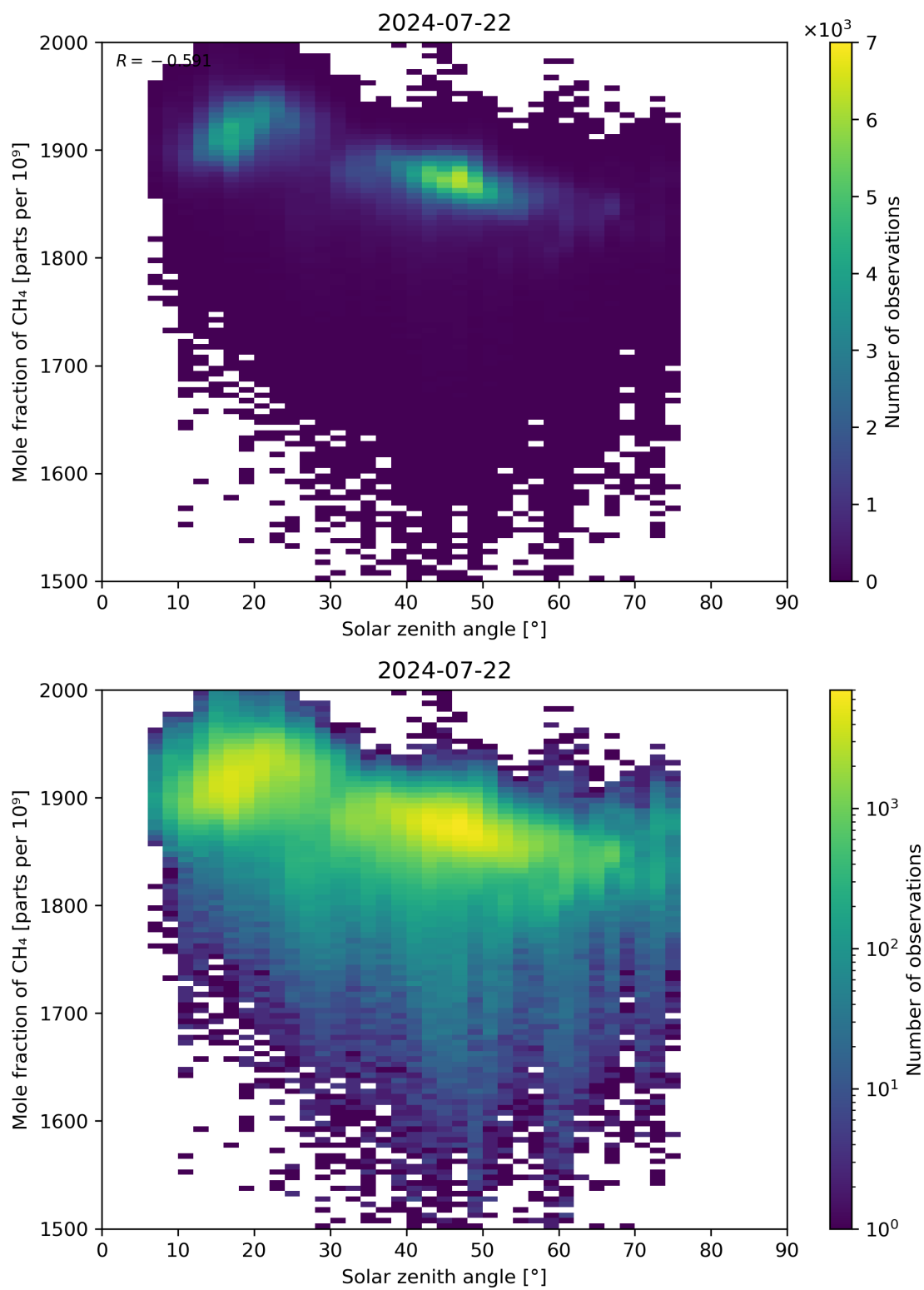
Figure 99: Scatter density plot of “Solar zenith angle” against “Mole fraction of CH 4 ” for 2024-07-21 to 2024-07-23.
