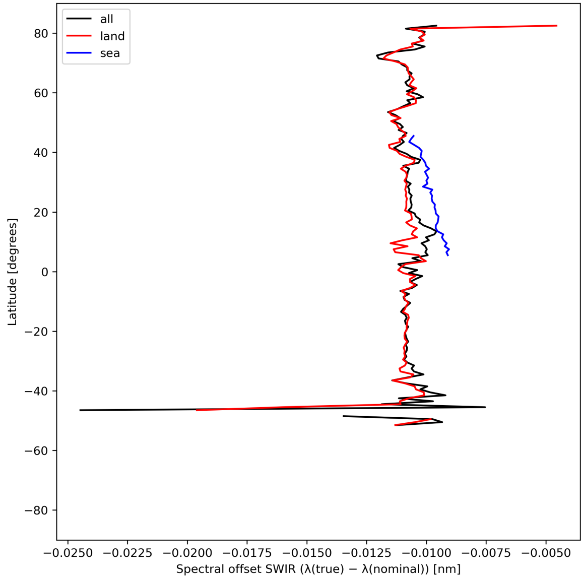
Figure 16: Zonal average of “Spectral offset SWIR ( \lambda(\text{true}) - \lambda(\text{nominal}) )” for 2024-07-21 to 2024-07-23.
