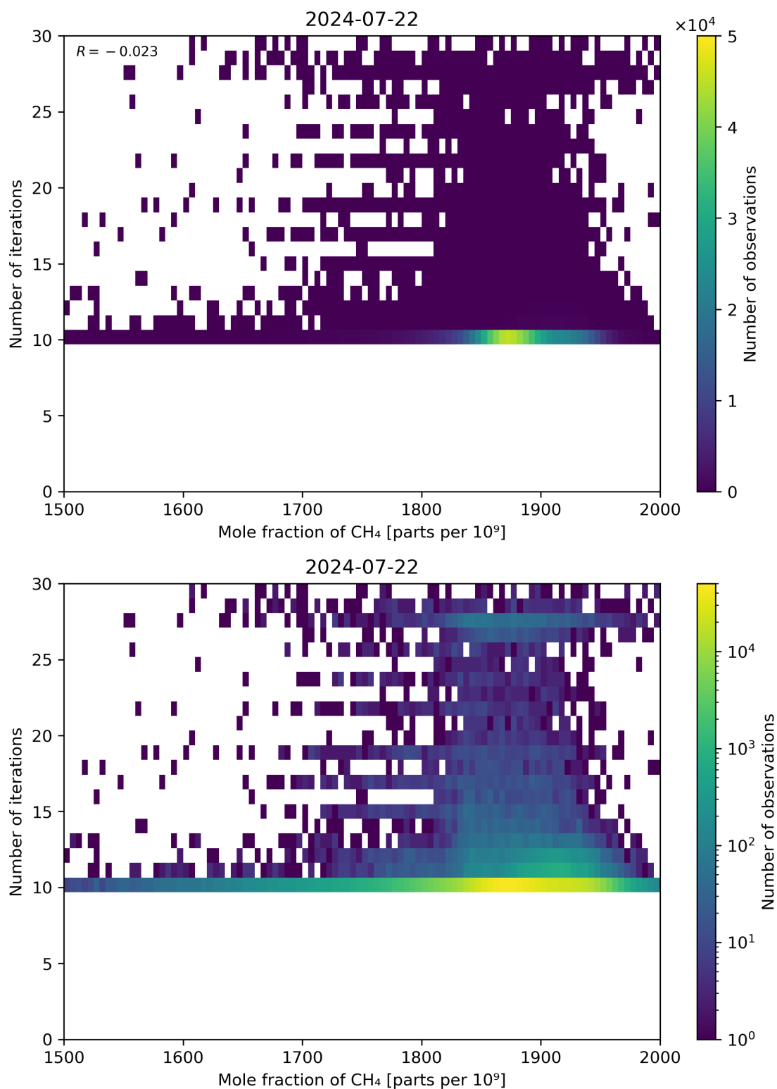
Figure 76: Scatter density plot of “Mole fraction of CH 4 ” against “Number of iterations” for 2024-07-21 to 2024-07-23.
