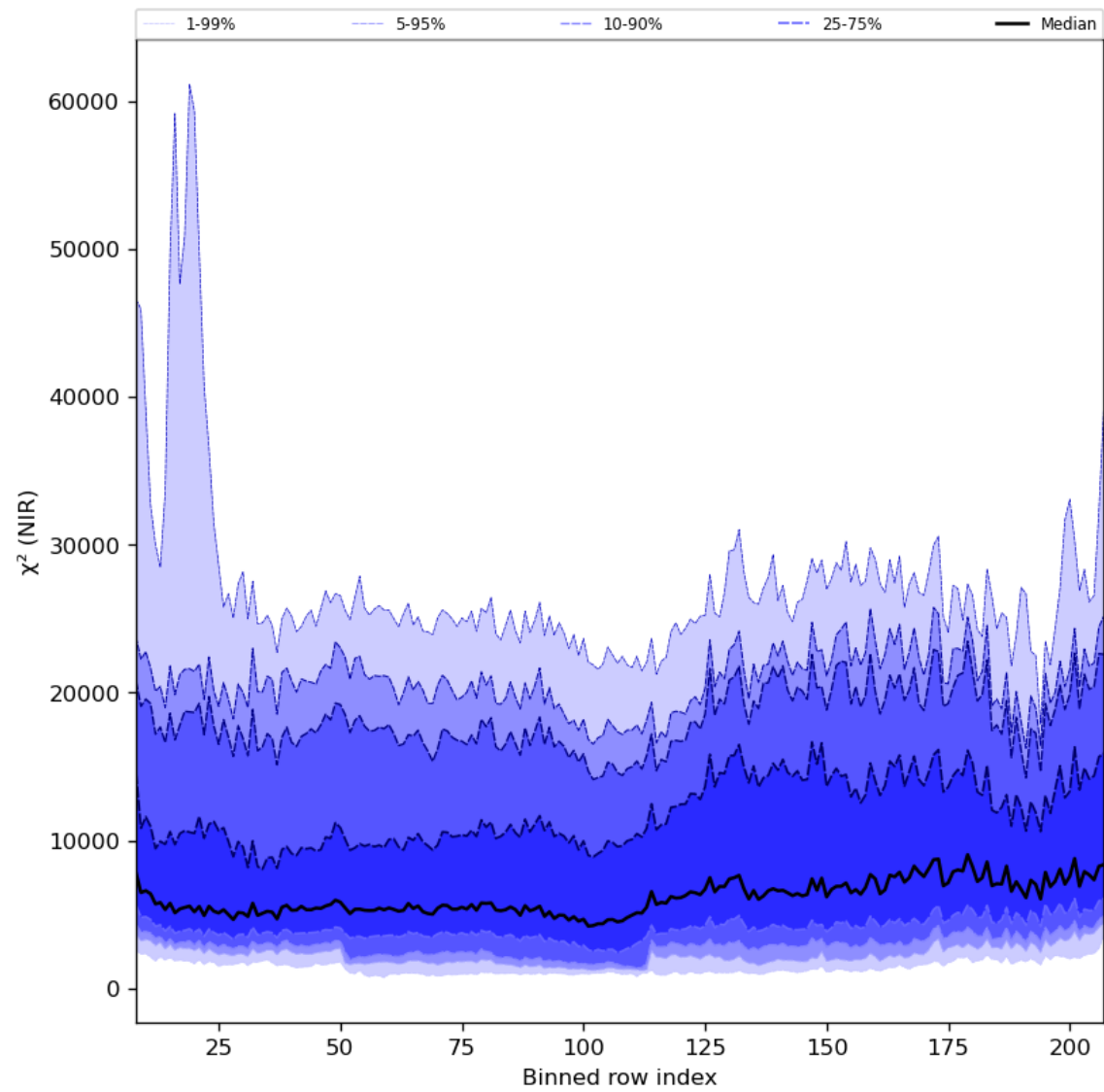
Figure 40: Along track statistics of " \chi^2 (NIR)" for 2024-07-21 to 2024-07-23
