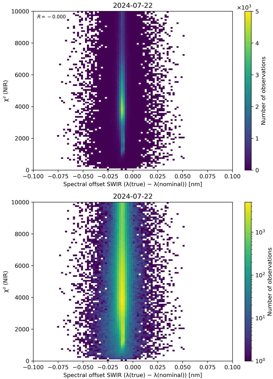
Figure 117: Scatter density plot of “Spectral offset SWIR ( \lambda(\text{true}) - \lambda(\text{nominal}) )” against “ \chi^2 (NIR)” for 2024-07-21 to 2024-07-23.
