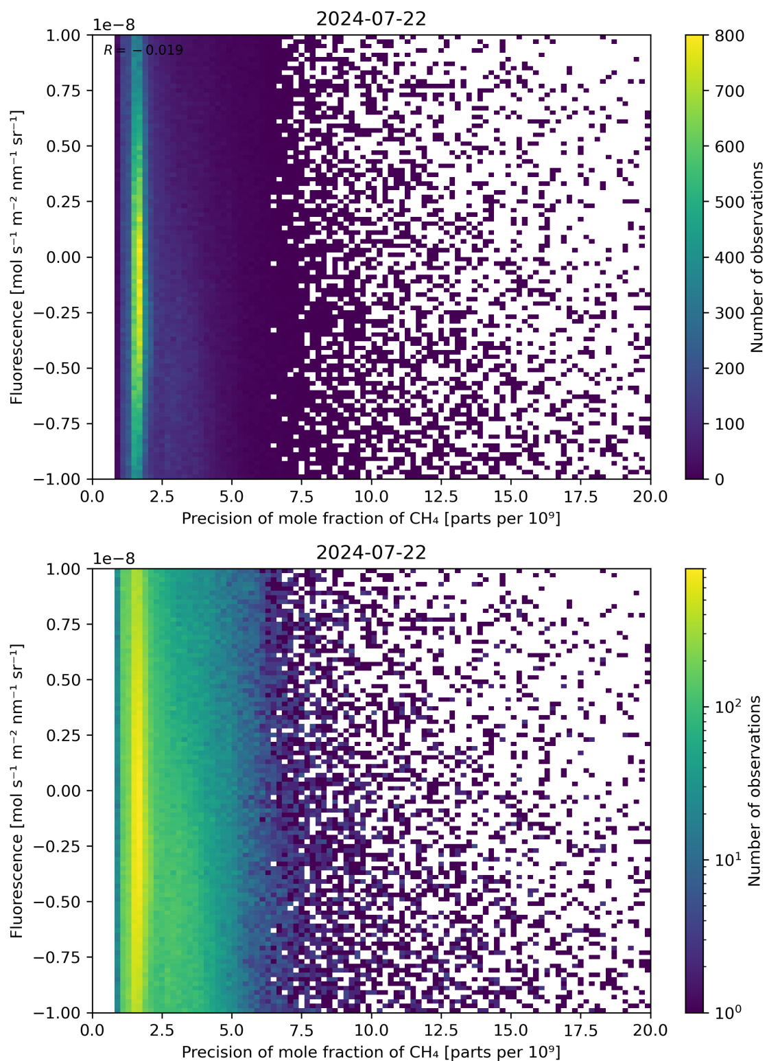
Figure 81: Scatter density plot of “Precision of mole fraction of \text{CH}_4 ” against “Fluorescence” for 2024-07-21 to 2024-07-23.
