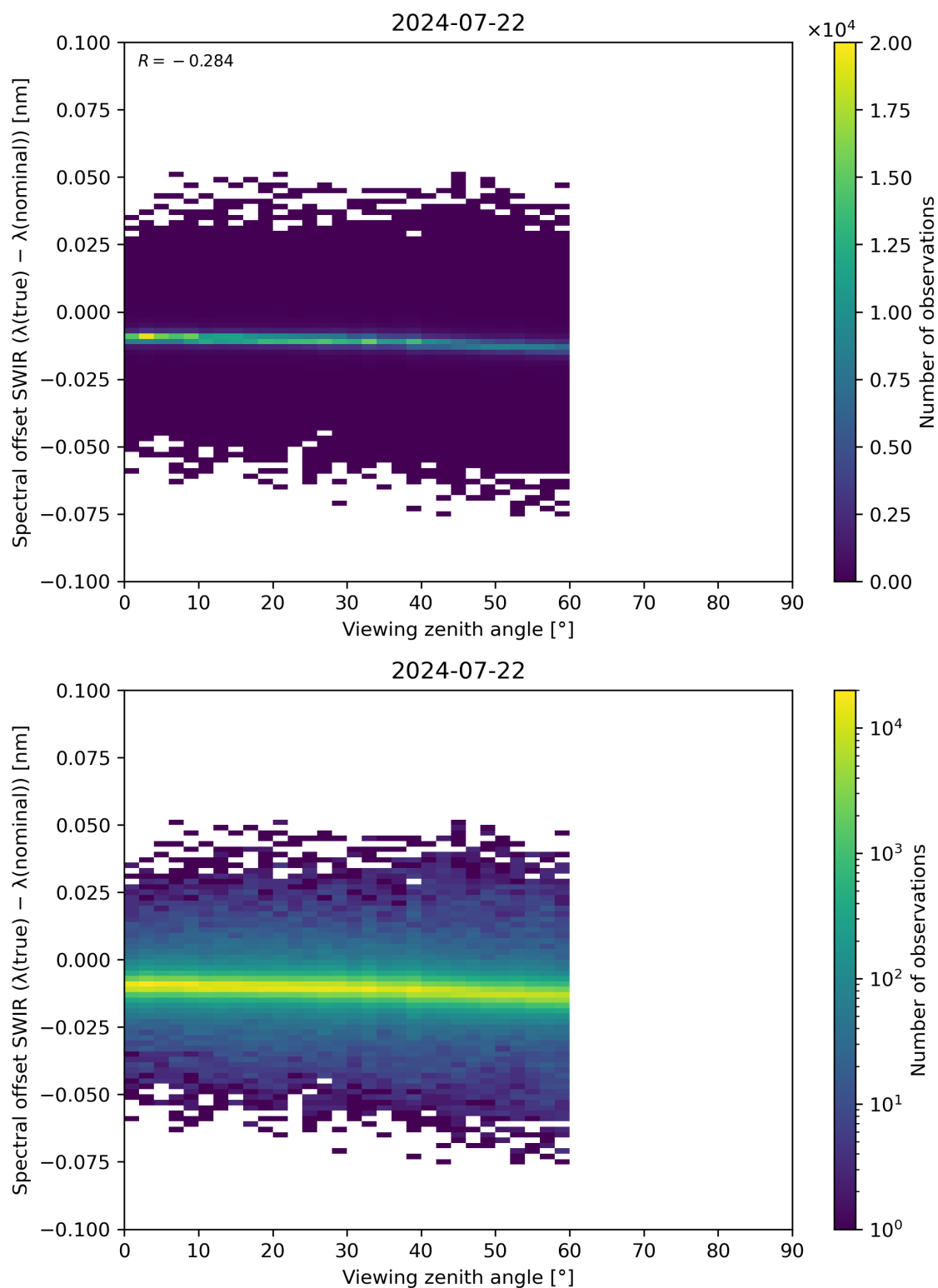
Figure 116: Scatter density plot of “Viewing zenith angle” against “Spectral offset SWIR ( \lambda(\text{true}) - \lambda(\text{nominal}) )” for 2024-07-21 to 2024-07-23.
