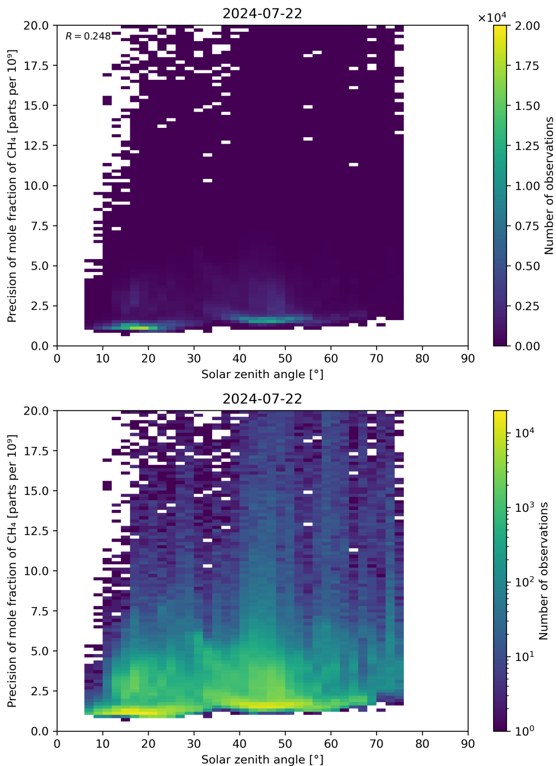
Figure 101: Scatter density plot of “Solar zenith angle” against “Precision of mole fraction of CH 4 ” for 2024-07-21 to 2024-07-23.
