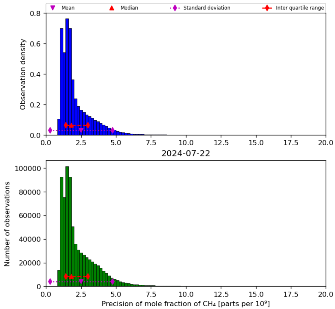
Figure 24: Histogram of “Precision of mole fraction of CH 4 ” for 2024-07-21 to 2024-07-23
