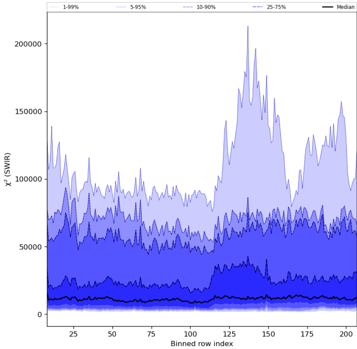
Figure 39: Along track statistics of “ \chi^2 (SWIR)” for 2024-07-21 to 2024-07-23
