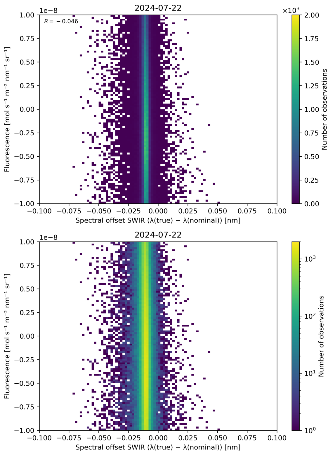
Figure 120: Scatter density plot of “Spectral offset SWIR ( \lambda(\text{true}) - \lambda(\text{nominal}) )” against “Fluorescence” for 2024-07-21 to 2024-07-23.
