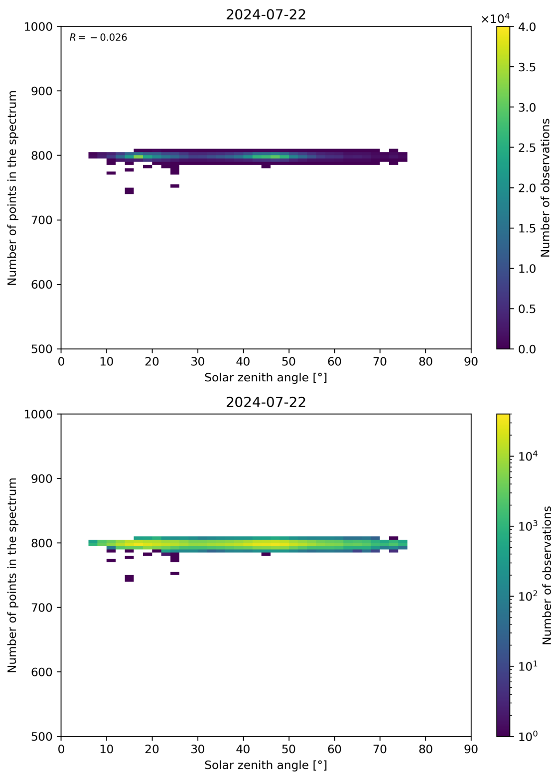
Figure 103: Scatter density plot of “Solar zenith angle” against “Number of points in the spectrum” for 2024-07-21 to 2024-07-23.
