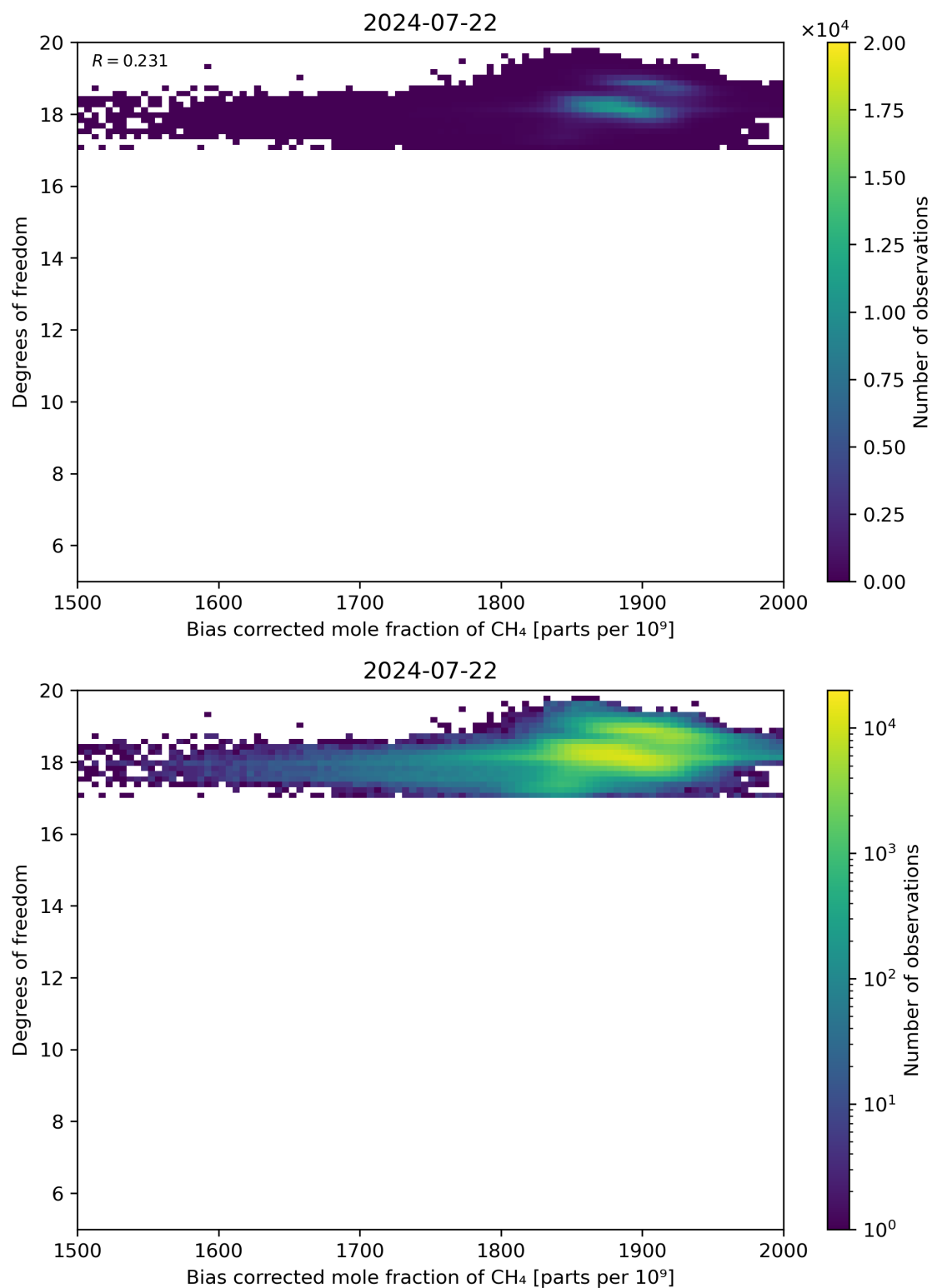
Figure 65: Scatter density plot of “Bias corrected mole fraction of CH 4 ” against “Degrees of freedom” for 2024-07-21 to 2024-07-23.
