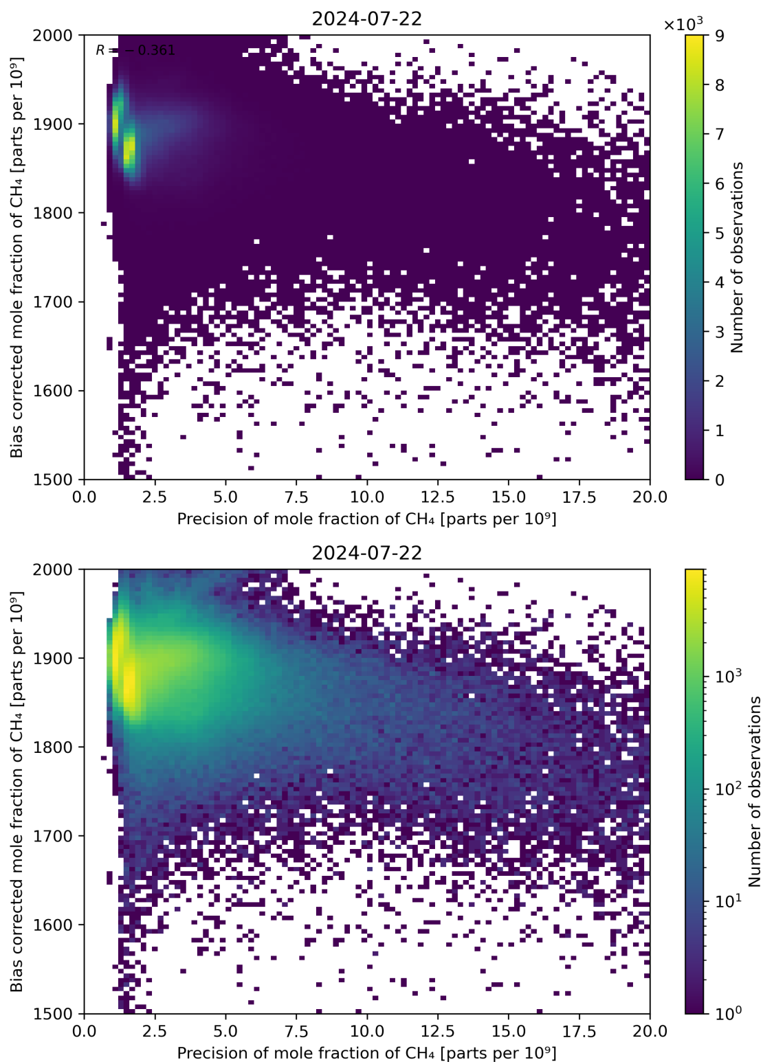
Figure 82: Scatter density plot of “Precision of mole fraction of CH 4 ” against “Bias corrected mole fraction of CH 4 ” for 2024-07-21 to 2024-07-23.
