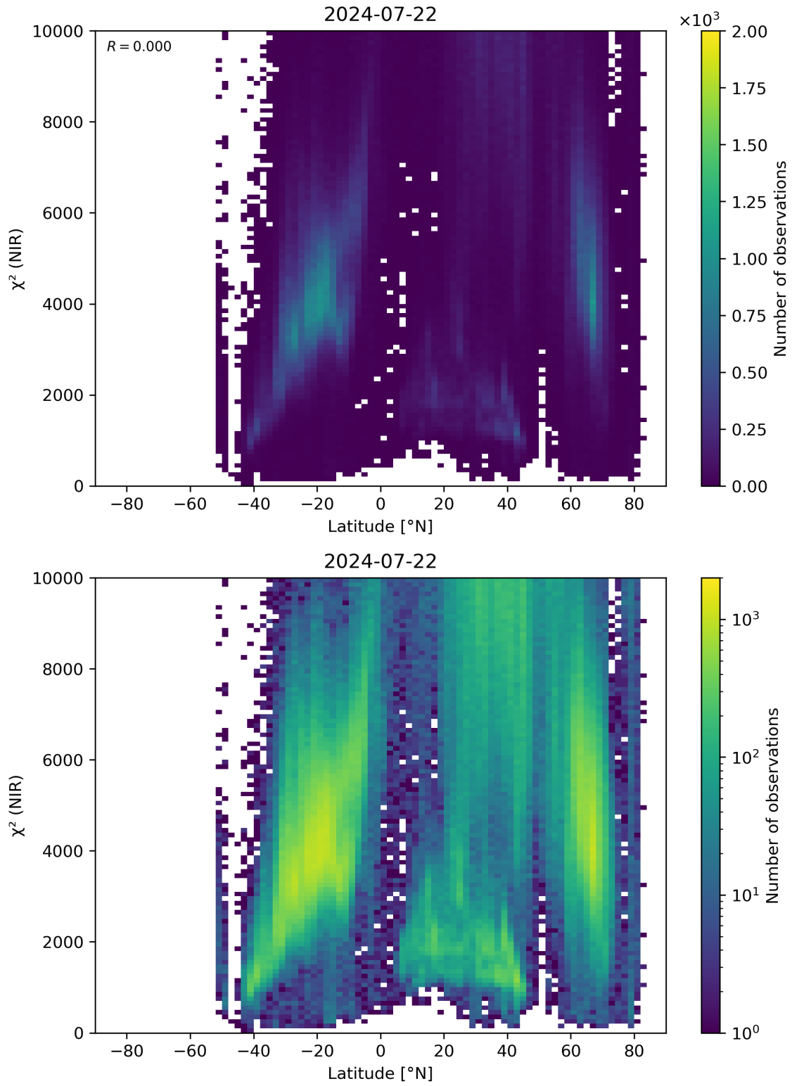
Figure 53: Scatter density plot of “Latitude” against “ \chi^2 (NIR)” for 2024-07-21 to 2024-07-23.
