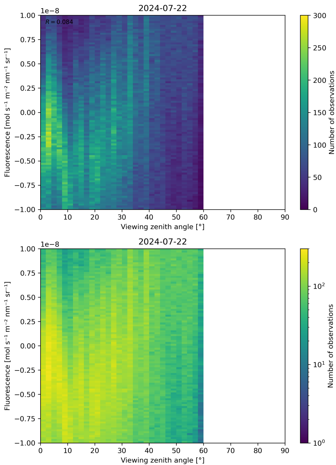
Figure 108: Scatter density plot of “Viewing zenith angle” against “Fluorescence” for 2024-07-21 to 2024-07-23.
