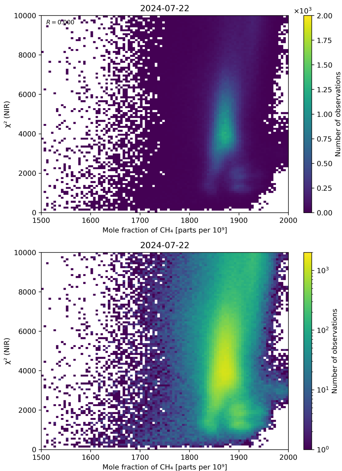
Figure 70: Scatter density plot of “Mole fraction of \text{CH}_4 ” against “ \chi^2 (NIR)” for 2024-07-21 to 2024-07-23.
