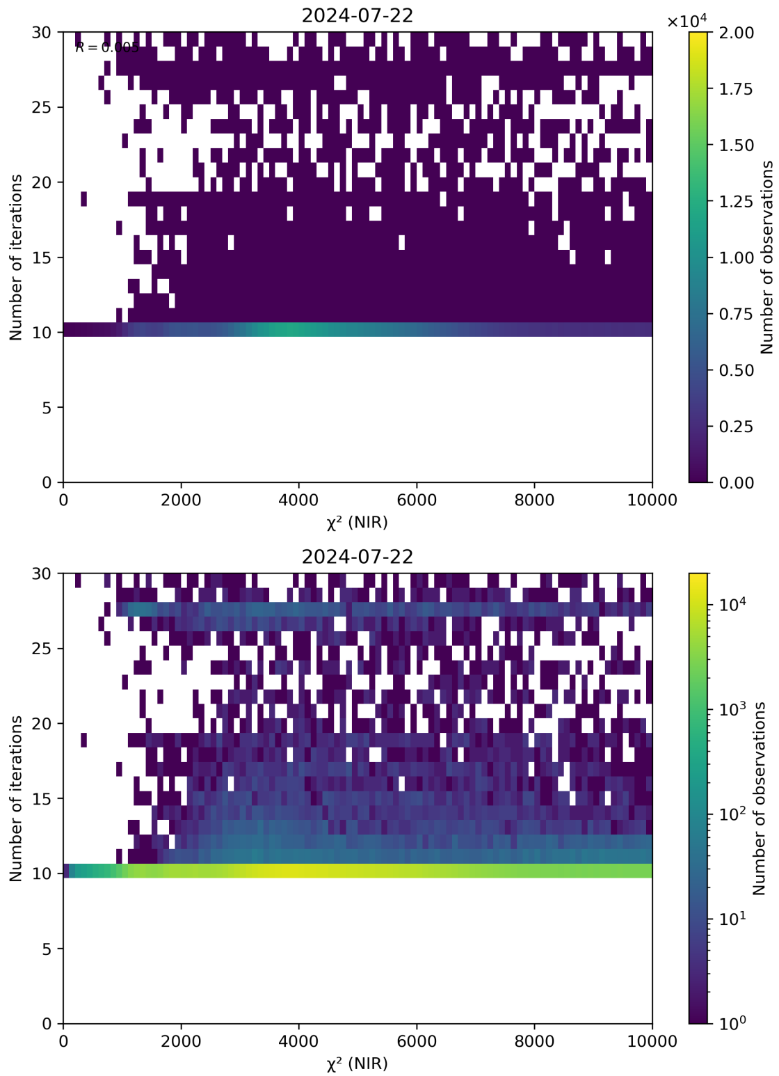
Figure 46: Scatter density plot of “ \chi^2 (NIR)” against “Number of iterations” for 2024-07-21 to 2024-07-23.
