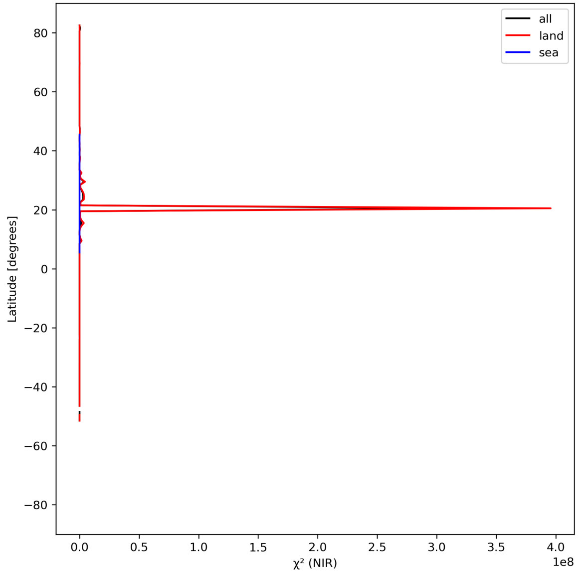
Figure 18: Zonal average of “ \chi^2 (NIR)” for 2024-07-21 to 2024-07-23.
