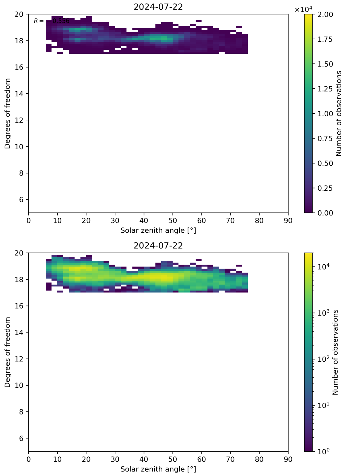
Figure 96: Scatter density plot of “Solar zenith angle” against “Degrees of freedom” for 2024-07-21 to 2024-07-23.
