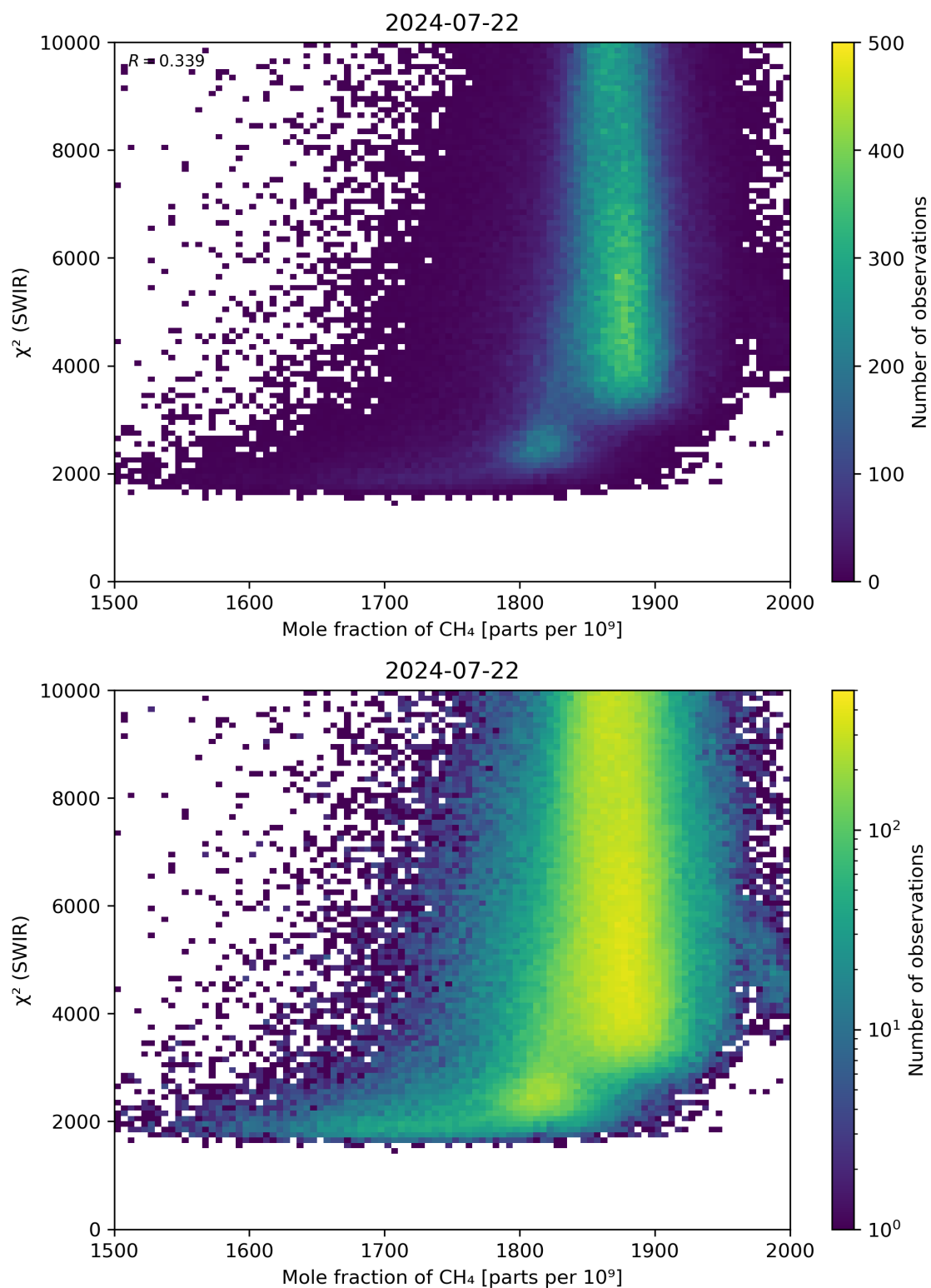
Figure 71: Scatter density plot of “Mole fraction of \text{CH}_4 ” against “ \chi^2 (SWIR)” for 2024-07-21 to 2024-07-23.
