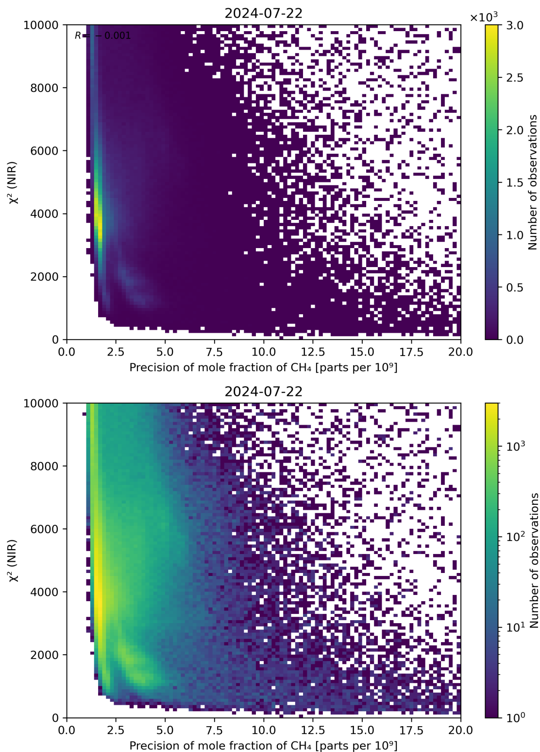
Figure 78: Scatter density plot of “Precision of mole fraction of \text{CH}_4 ” against “ \chi^2 (NIR)” for 2024-07-21 to 2024-07-23.
