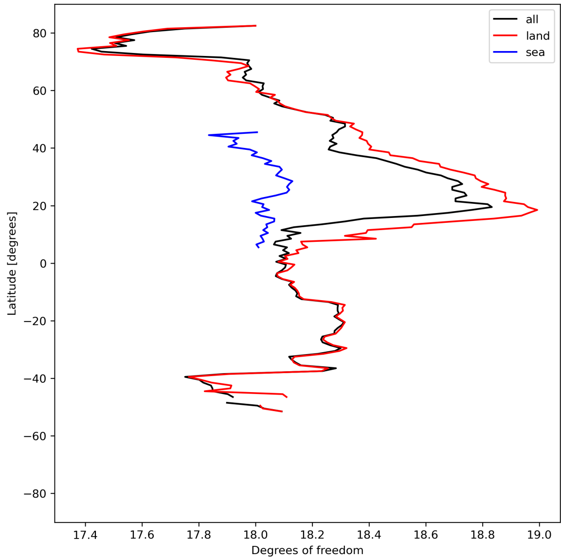
Figure 19: Zonal average of “Degrees of freedom” for 2024-07-21 to 2024-07-23.
