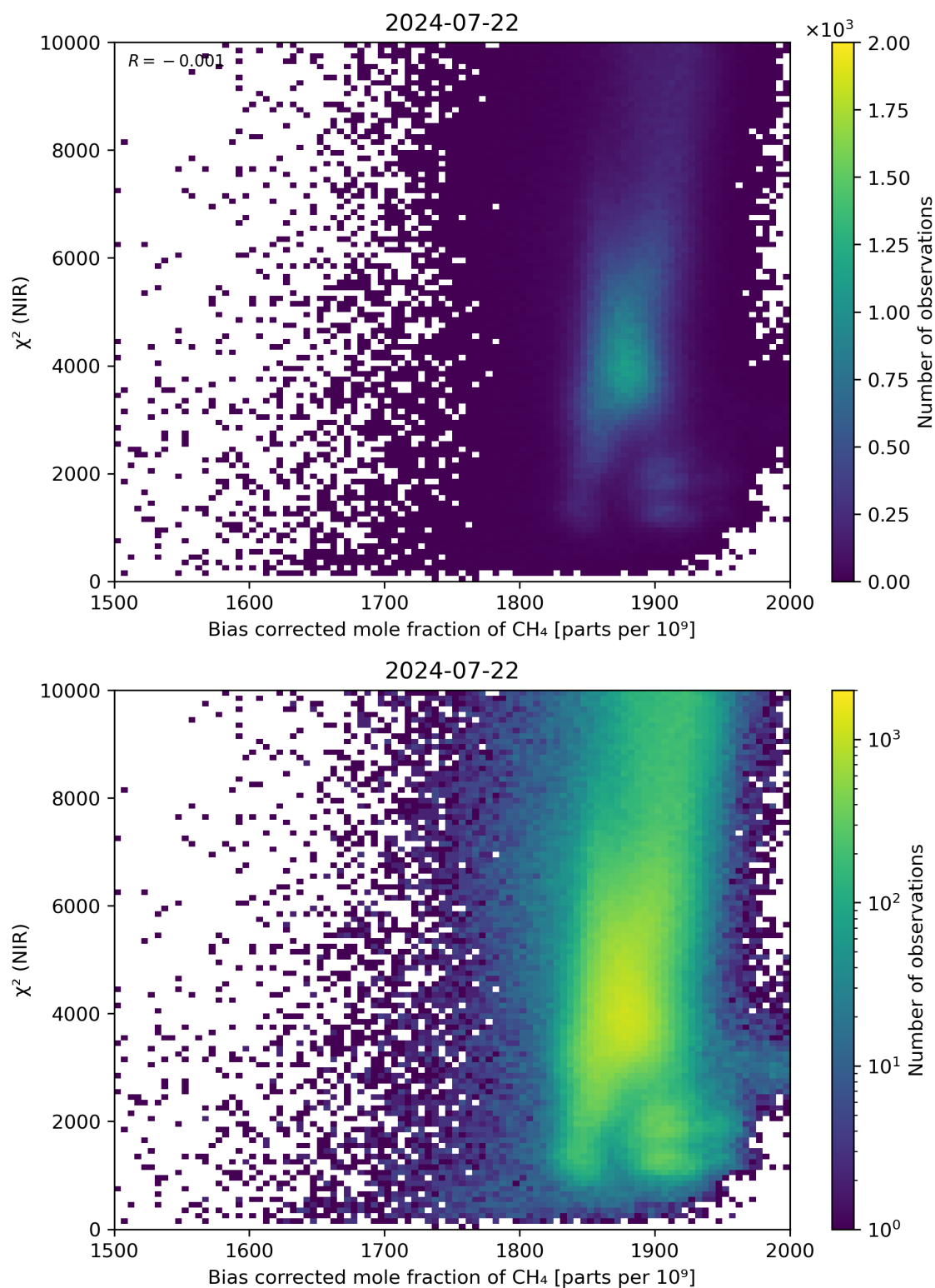
Figure 63: Scatter density plot of “Bias corrected mole fraction of CH 4 ” against “ \chi^2 (NIR)” for 2024-07-21 to 2024-07-23.
