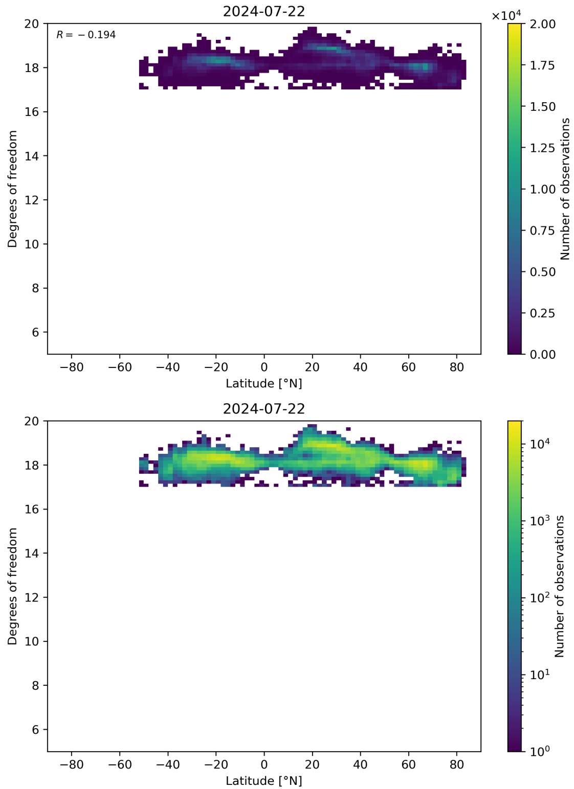
Figure 55: Scatter density plot of “Latitude” against “Degrees of freedom” for 2024-07-21 to 2024-07-23.
