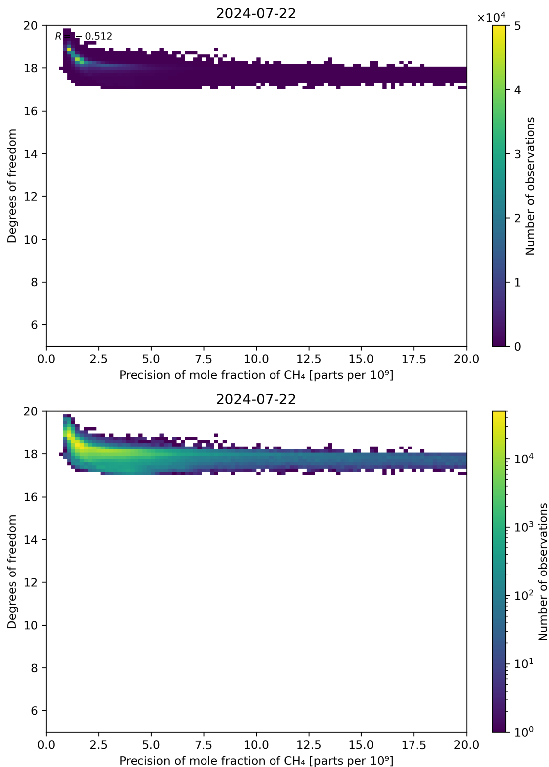
Figure 80: Scatter density plot of “Precision of mole fraction of CH 4 ” against “Degrees of freedom” for 2024-07-21 to 2024-07-23.
