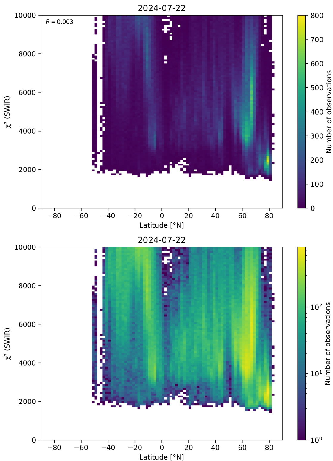
Figure 54: Scatter density plot of “Latitude” against “ \chi^2 (SWIR)” for 2024-07-21 to 2024-07-23.
