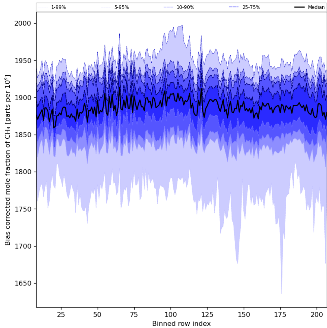
Figure 36: Along track statistics of “Bias corrected mole fraction of CH 4 ” for 2024-07-21 to 2024-07-23
