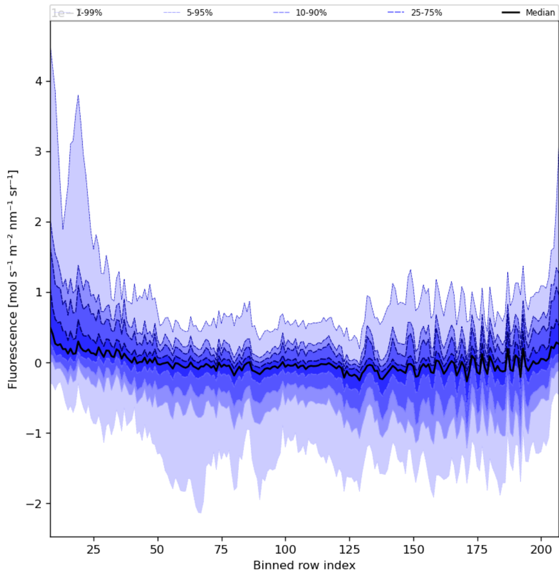
Figure 43: Along track statistics of “Fluorescence” for 2024-07-21 to 2024-07-23
