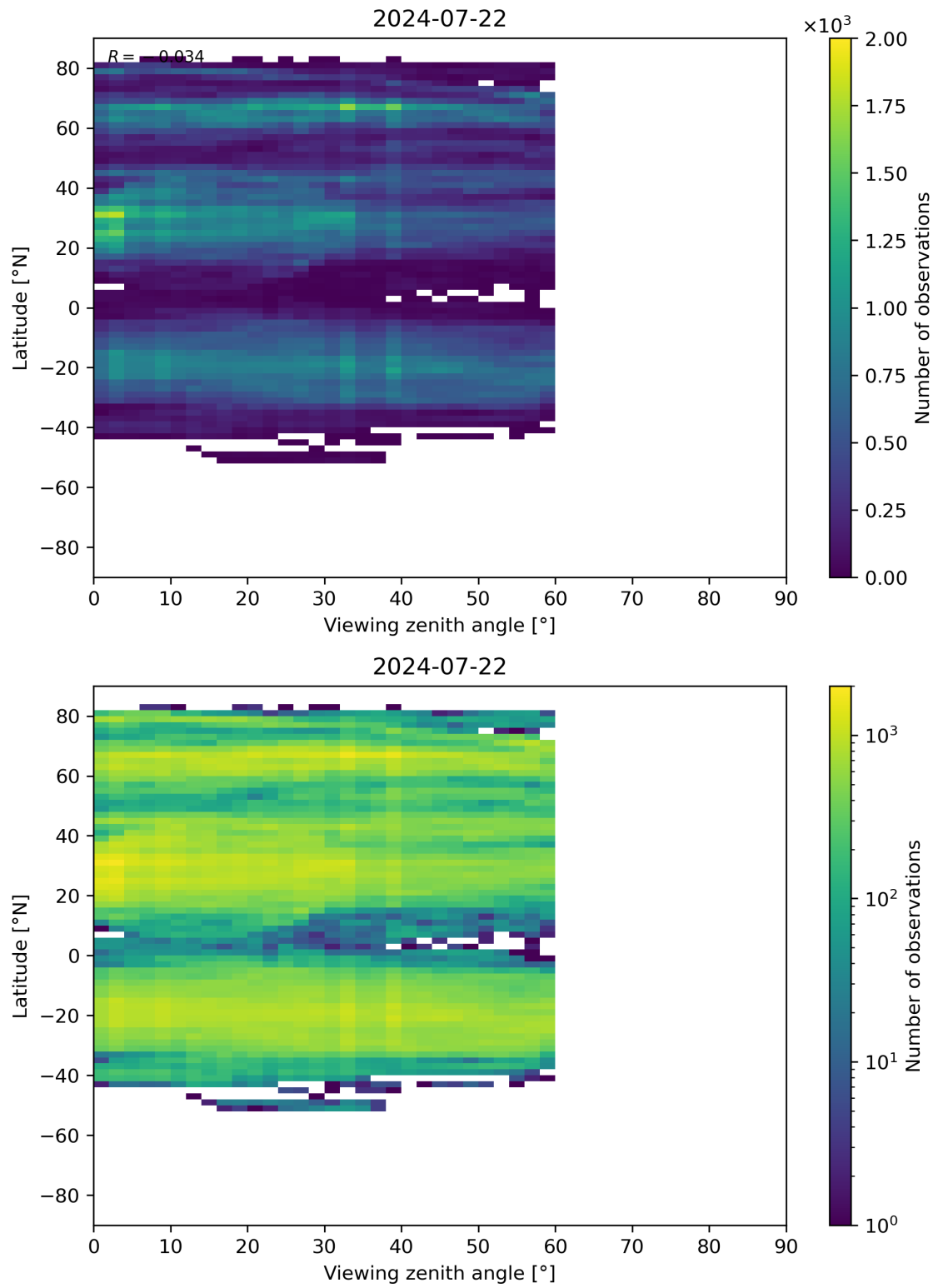
Figure 109: Scatter density plot of “Viewing zenith angle” against “Latitude” for 2024-07-21 to 2024-07-23.
