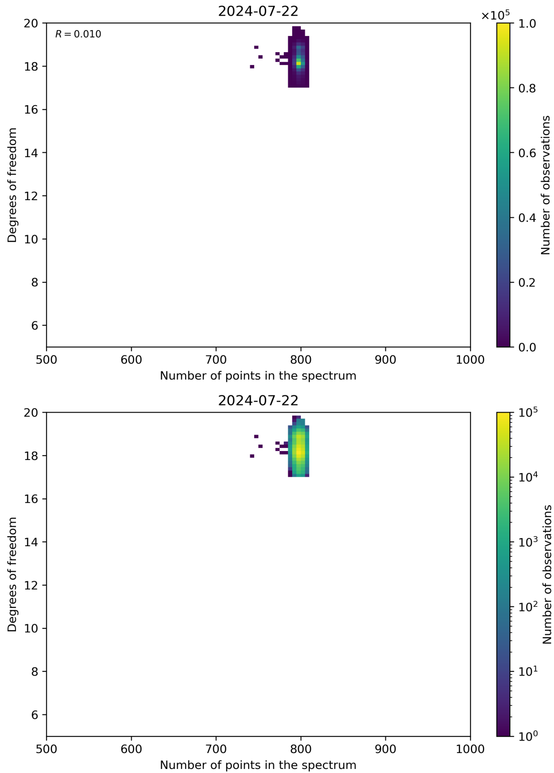
Figure 90: Scatter density plot of “Number of points in the spectrum” against “Degrees of freedom” for 2024-07-21 to 2024-07-23.
