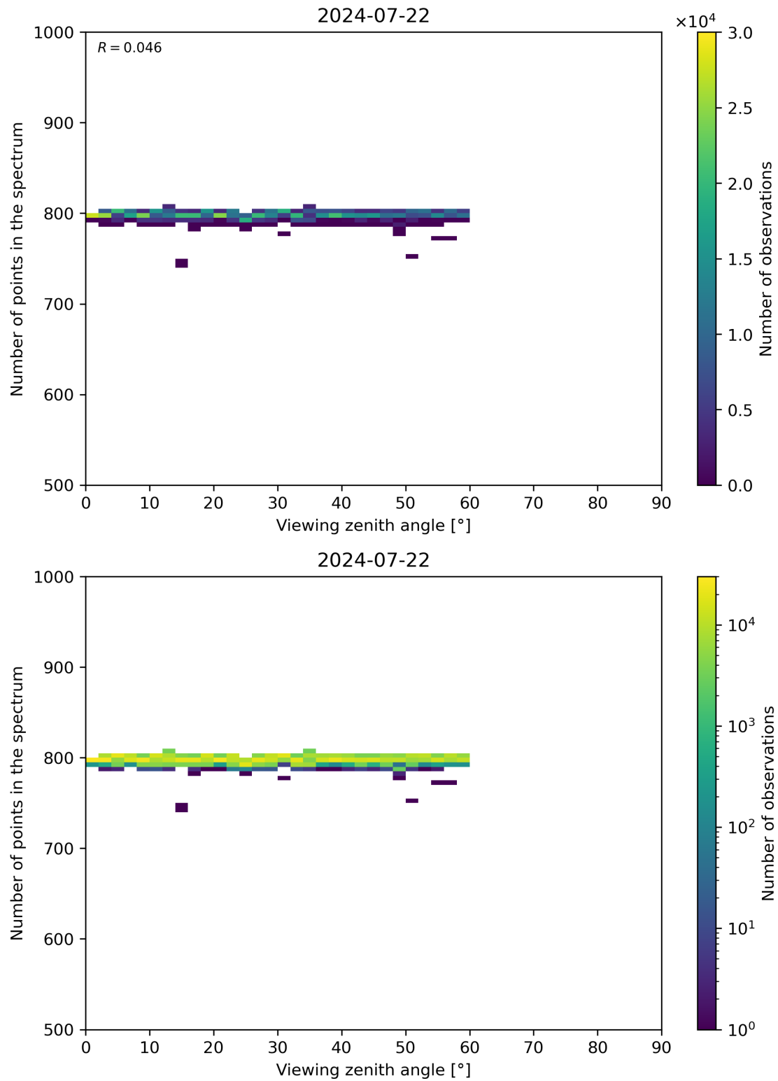
Figure 114: Scatter density plot of “Viewing zenith angle” against “Number of points in the spectrum” for 2024-07-21 to 2024-07-23.
