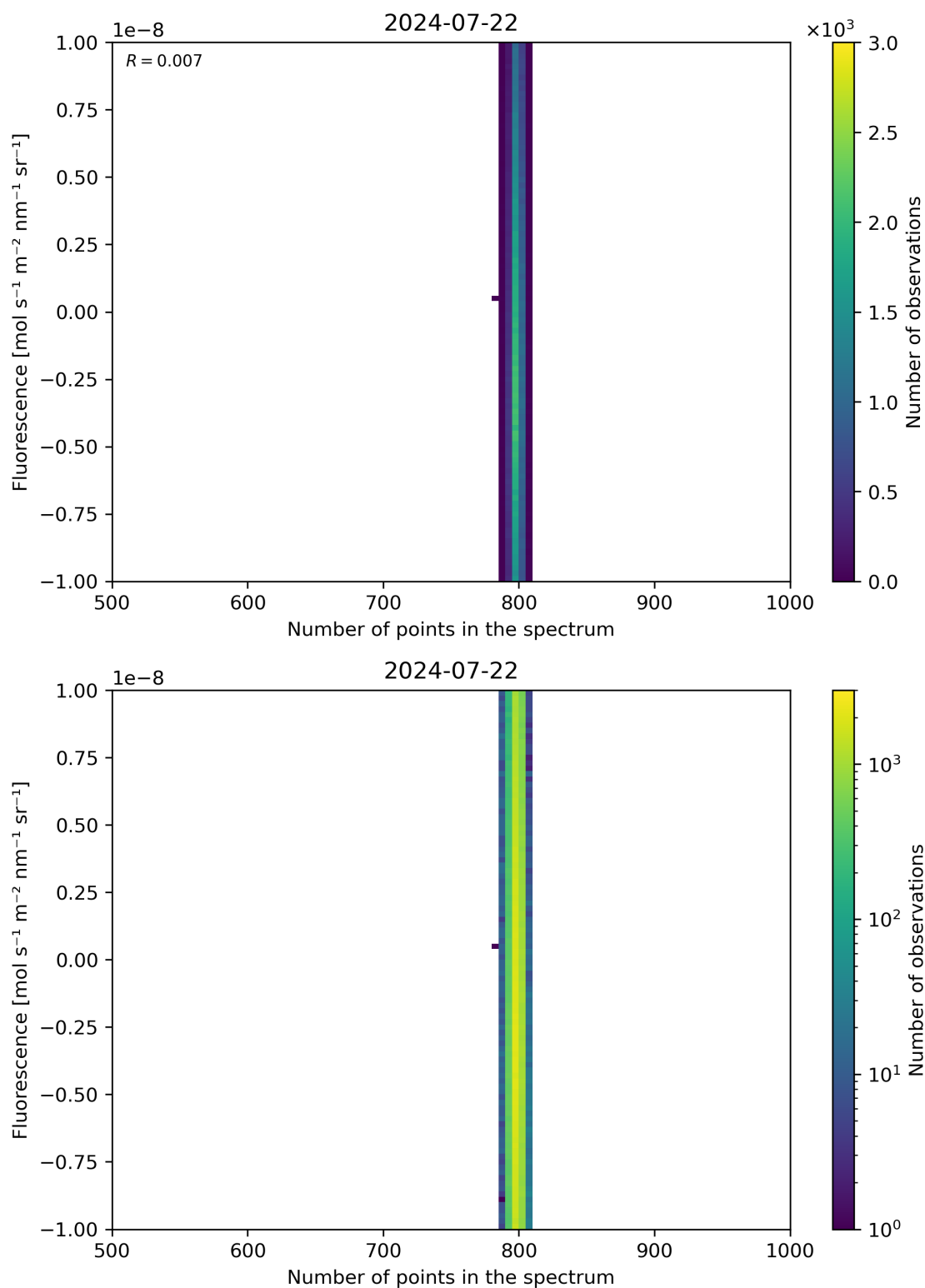
Figure 91: Scatter density plot of “Number of points in the spectrum” against “Fluorescence” for 2024-07-21 to 2024-07-23.
