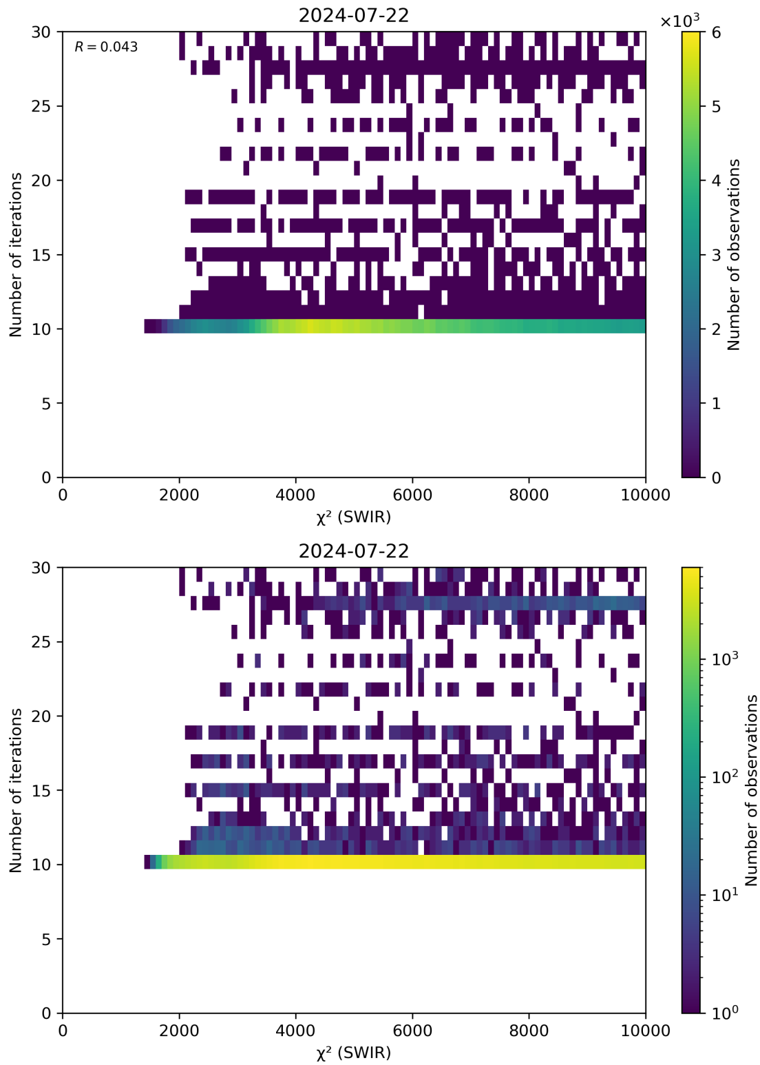
Figure 50: Scatter density plot of “ \chi^2 (SWIR)” against “Number of iterations” for 2024-07-21 to 2024-07-23.
