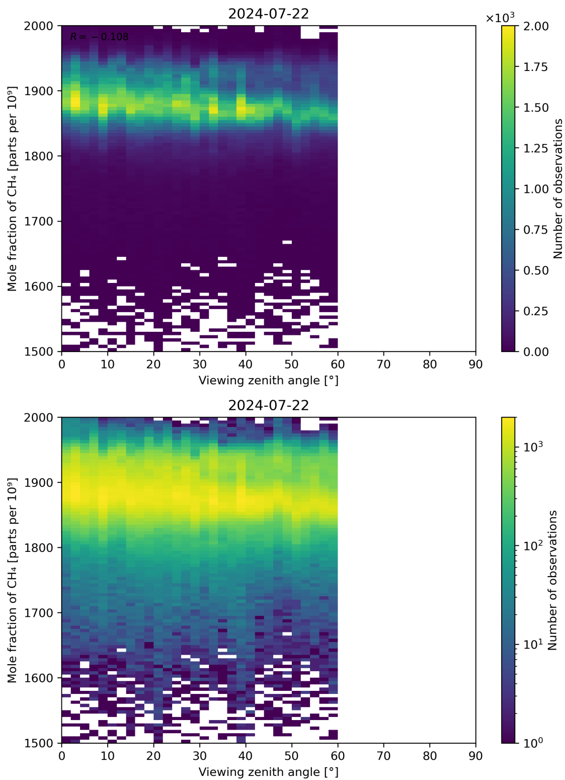
Figure 110: Scatter density plot of “Viewing zenith angle” against “Mole fraction of CH 4 ” for 2024-07-21 to 2024-07-23.
