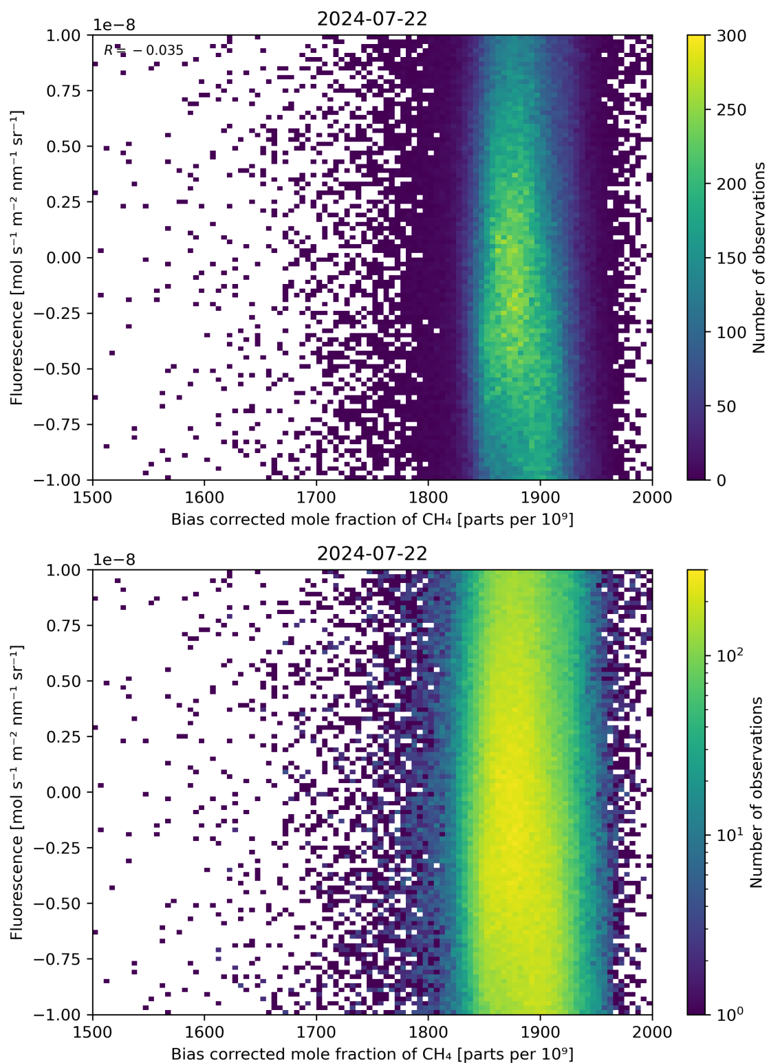
Figure 66: Scatter density plot of “Bias corrected mole fraction of \text{CH}_4 ” against “Fluorescence” for 2024-07-21 to 2024-07-23.
