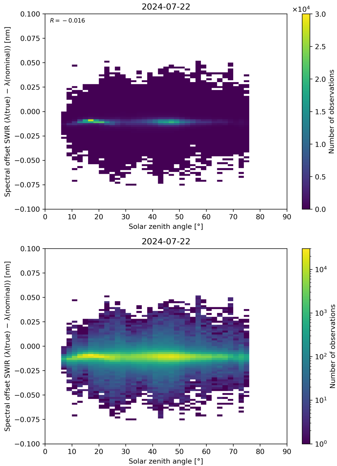
Figure 104: Scatter density plot of “Solar zenith angle” against “Spectral offset SWIR ( \lambda(\text{true}) - \lambda(\text{nominal}) )” for 2024-07-21 to 2024-07-23.
