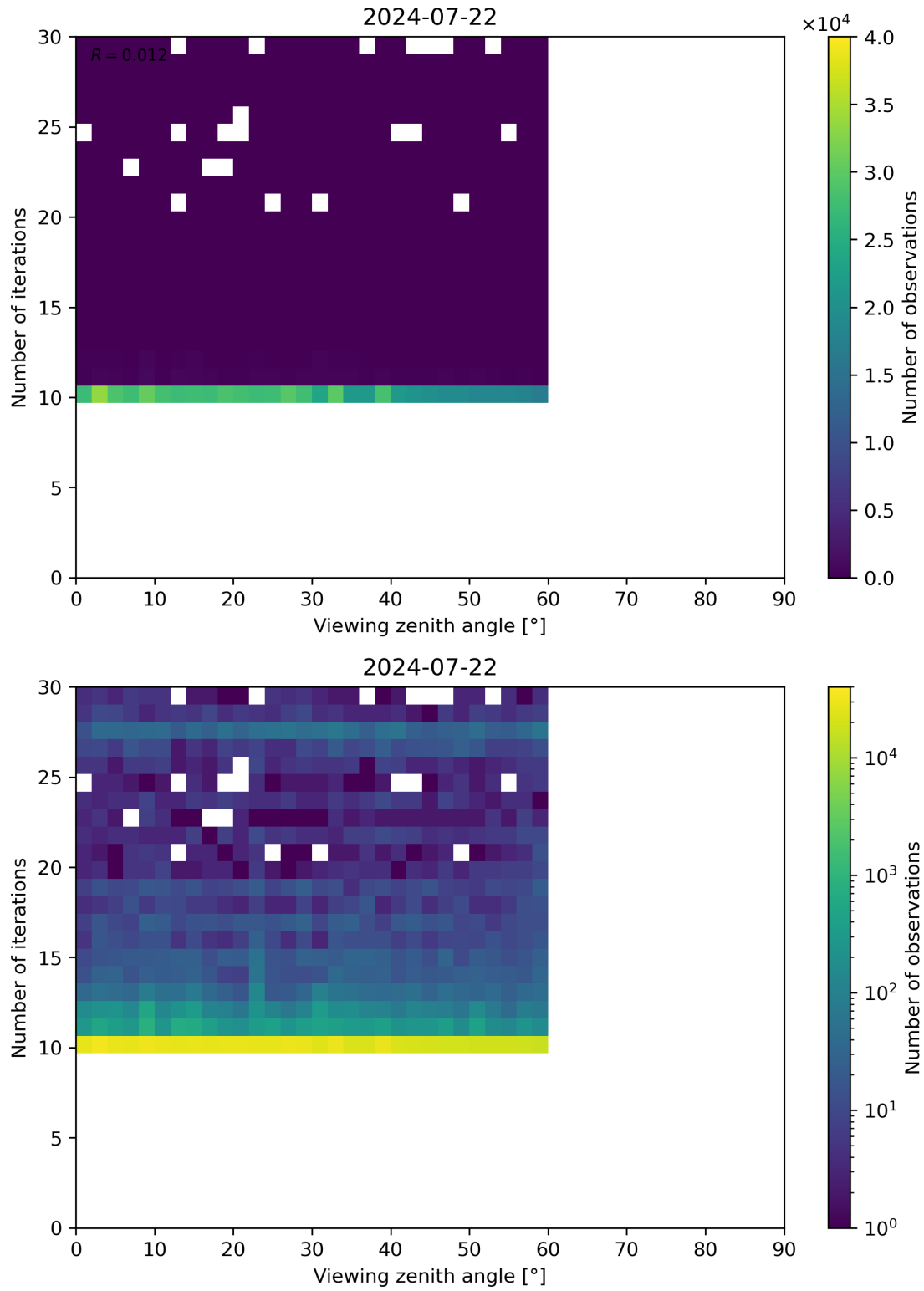
Figure 113: Scatter density plot of “Viewing zenith angle” against “Number of iterations” for 2024-07-21 to 2024-07-23.
