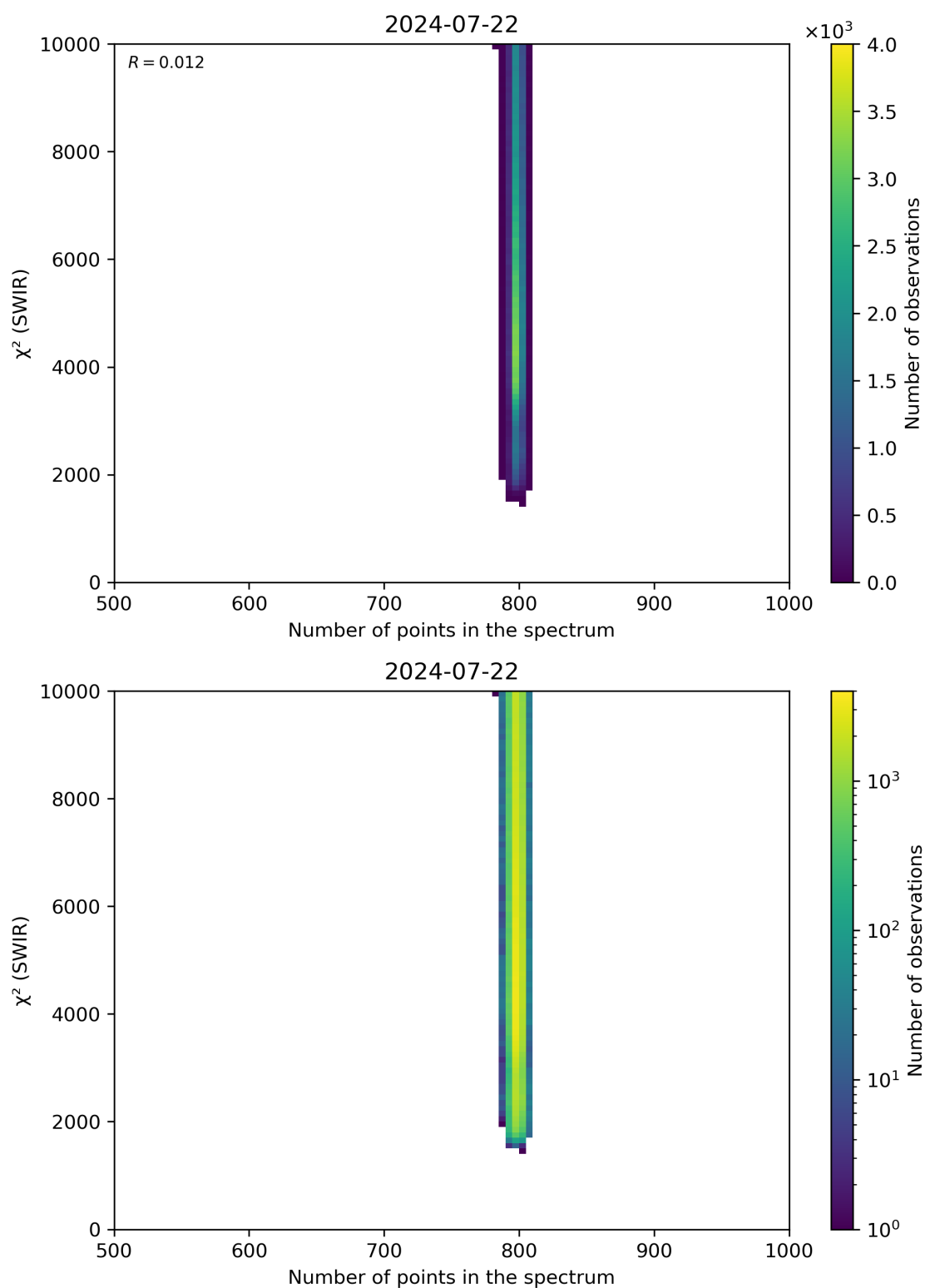
Figure 89: Scatter density plot of “Number of points in the spectrum” against “ \chi^2 (SWIR)” for 2024-07-21 to 2024-07-23.
