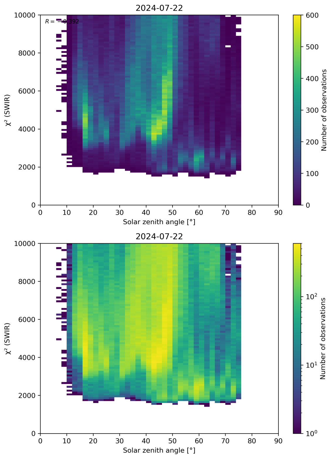
Figure 95: Scatter density plot of “Solar zenith angle” against “ \chi^2 (SWIR)” for 2024-07-21 to 2024-07-23.
