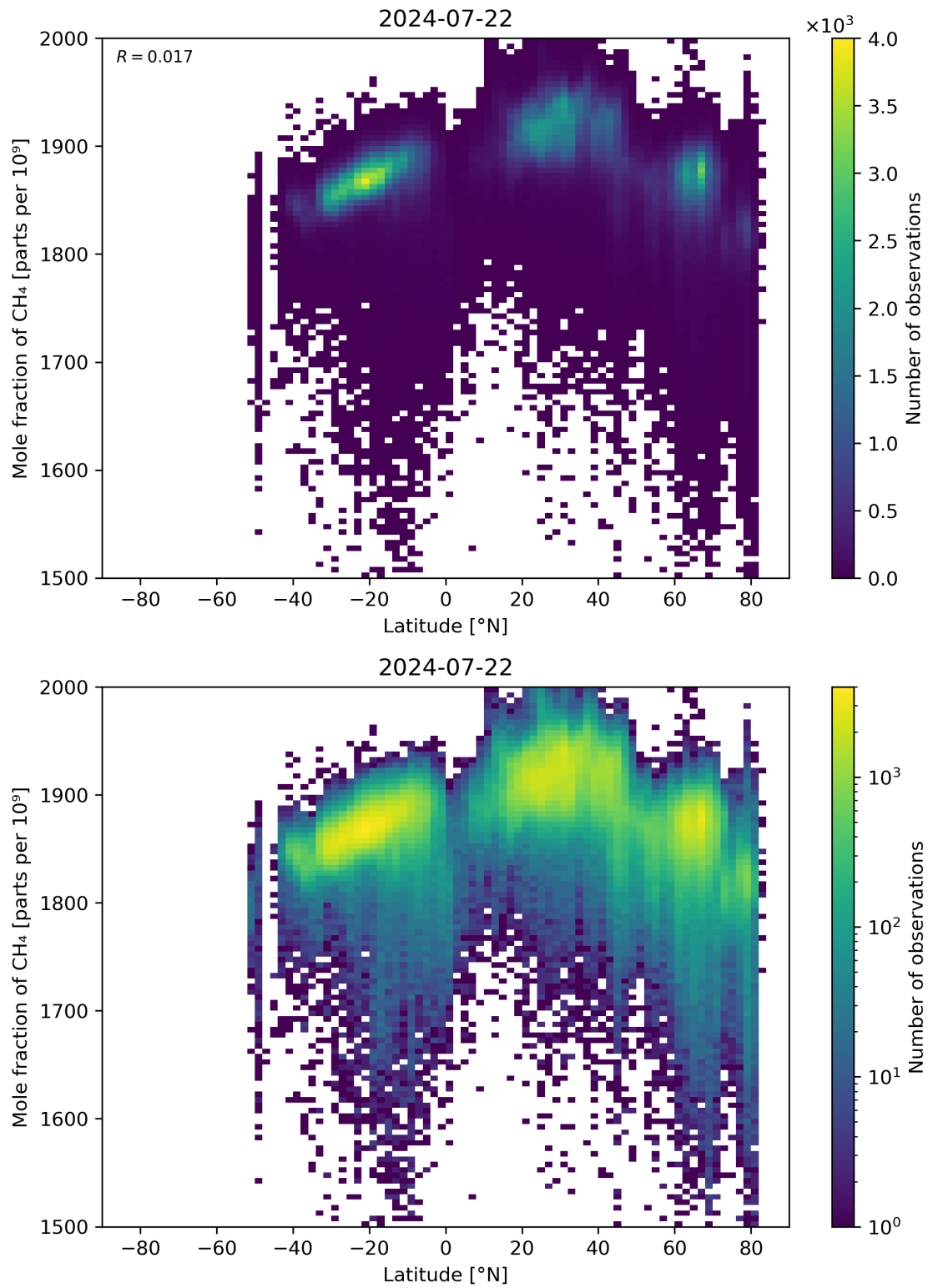
Figure 57: Scatter density plot of “Latitude” against “Mole fraction of \text{CH}_4 ” for 2024-07-21 to 2024-07-23.
