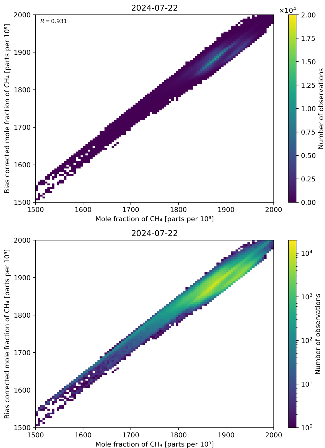
Figure 74: Scatter density plot of “Mole fraction of CH 4 ” against “Bias corrected mole fraction of CH 4 ” for 2024-07-21 to 2024-07-23.
