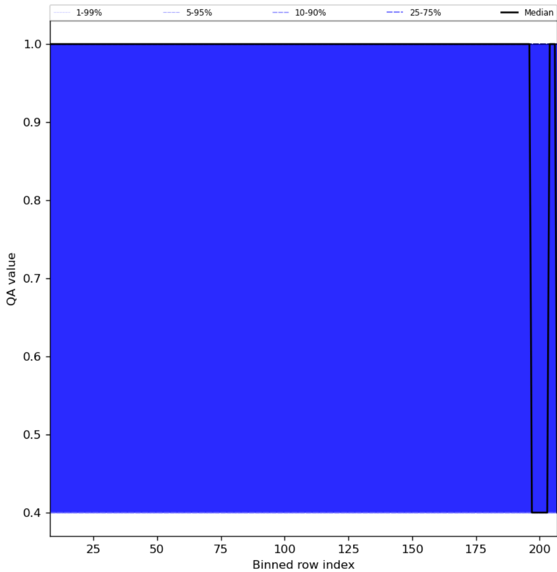
Figure 33: Along track statistics of “QA value” for 2024-07-21 to 2024-07-23
