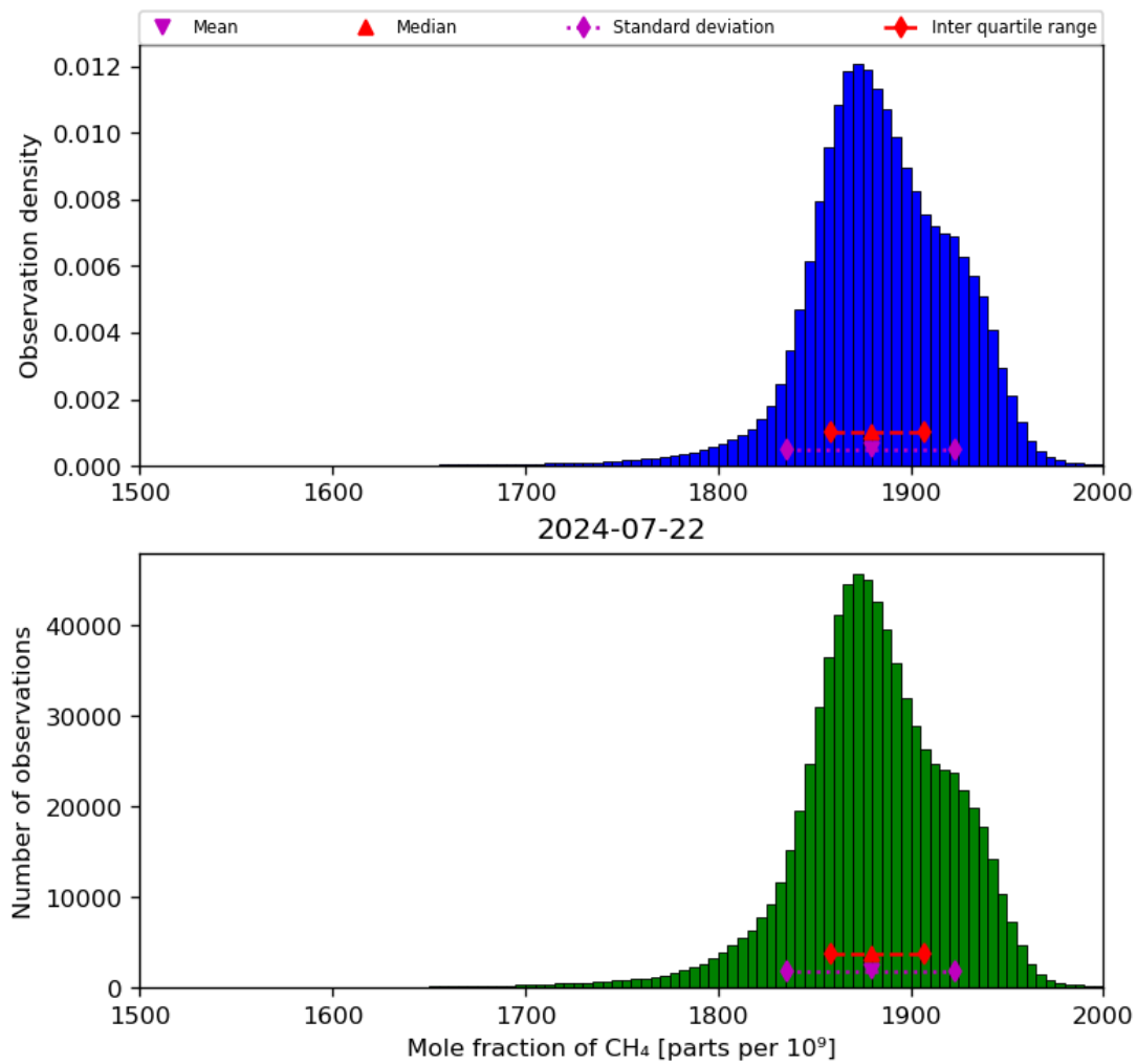
Figure 23: Histogram of “Mole fraction of CH 4 ” for 2024-07-21 to 2024-07-23
