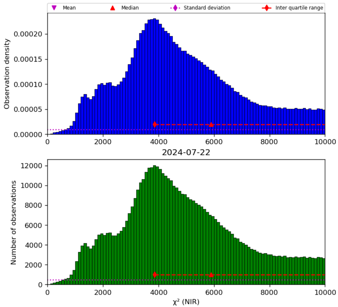
Figure 29: Histogram of " \chi^2 (NIR)" for 2024-07-21 to 2024-07-23
