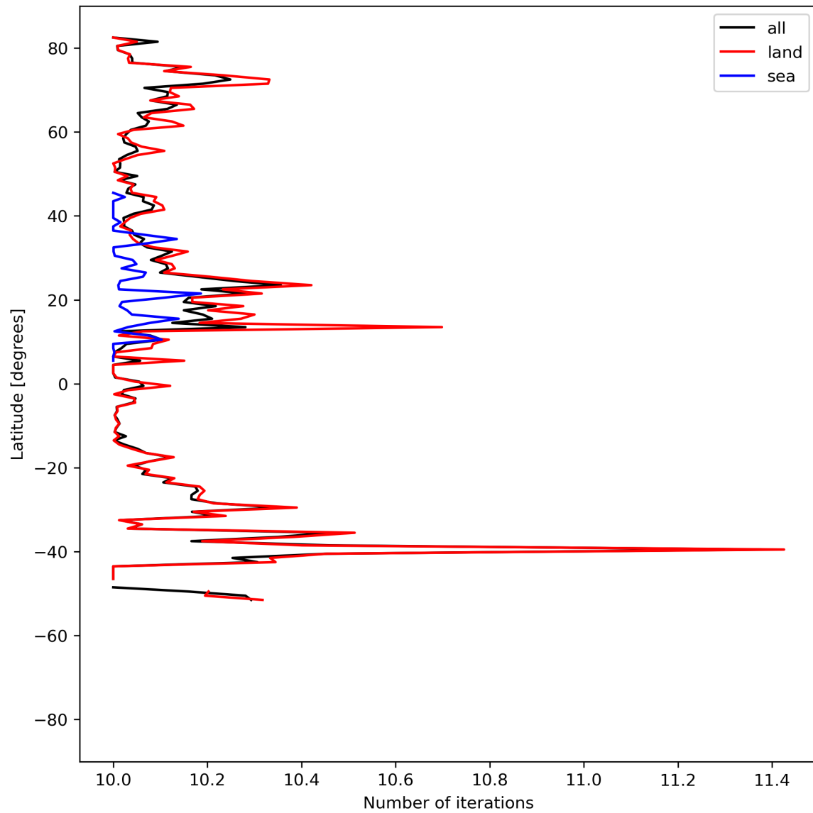
Figure 20: Zonal average of “Number of iterations” for 2024-07-21 to 2024-07-23.
