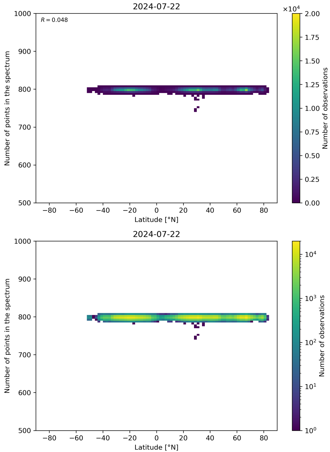
Figure 61: Scatter density plot of “Latitude” against “Number of points in the spectrum” for 2024-07-21 to 2024-07-23.
