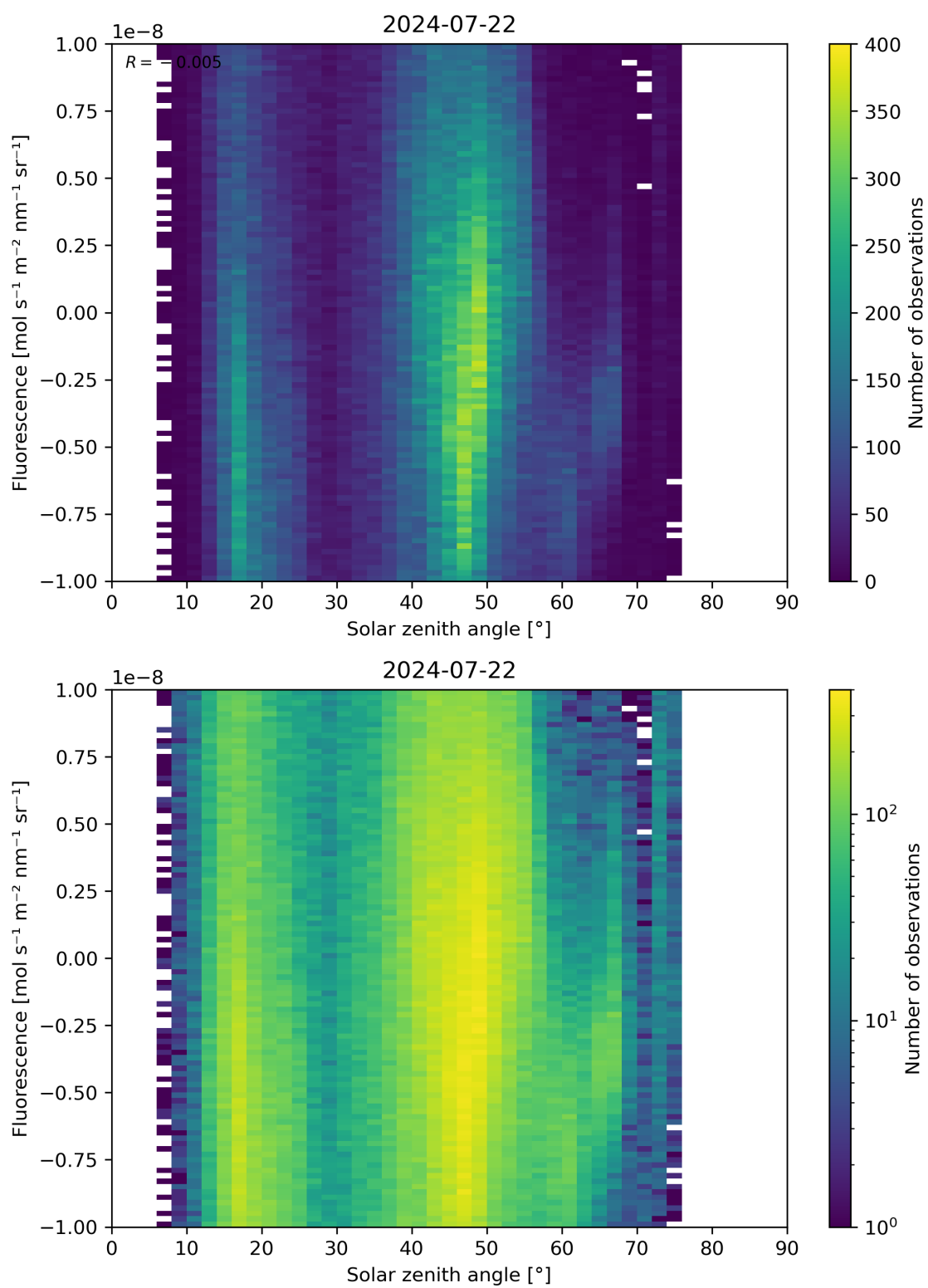
Figure 97: Scatter density plot of “Solar zenith angle” against “Fluorescence” for 2024-07-21 to 2024-07-23.
