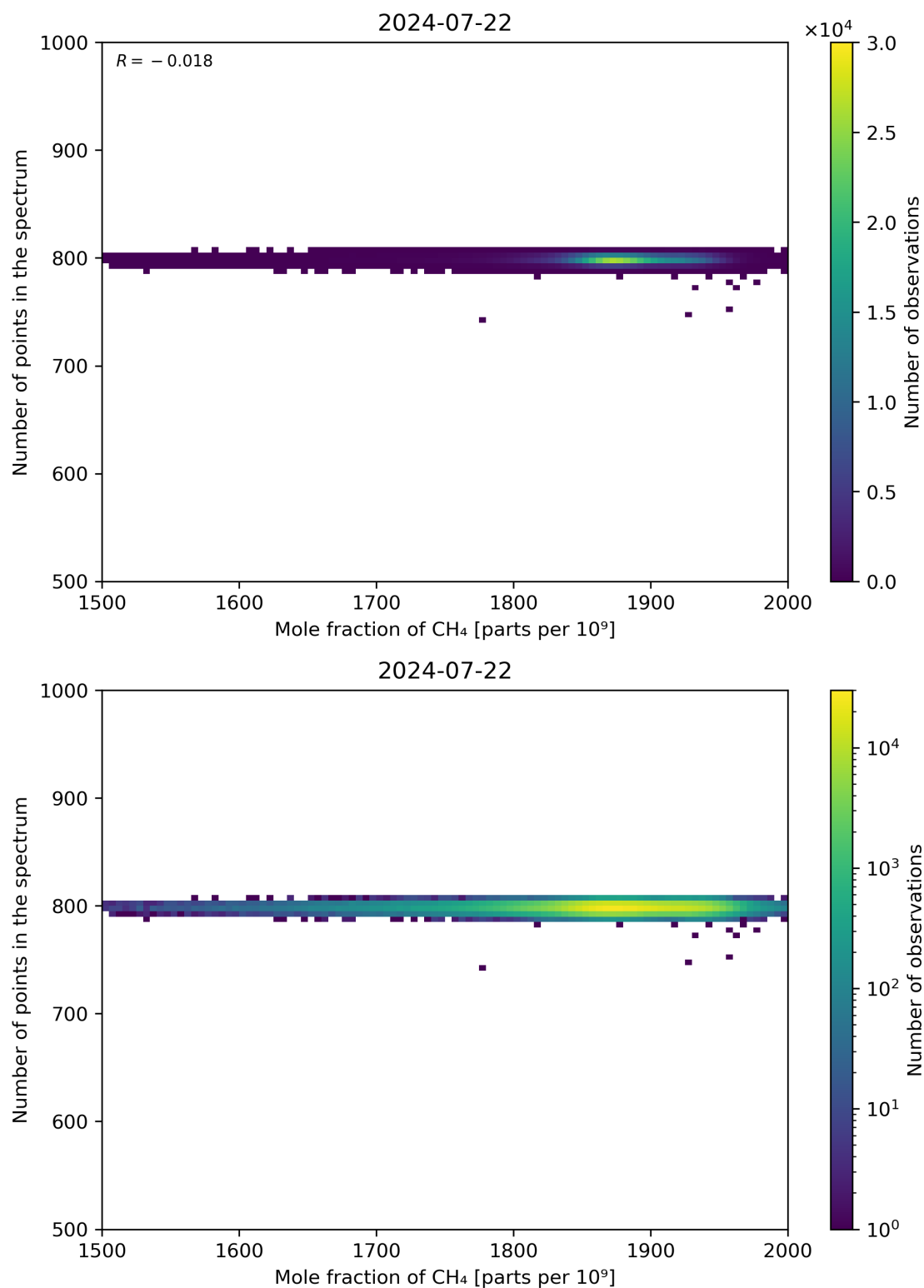
Figure 77: Scatter density plot of “Mole fraction of CH 4 ” against “Number of points in the spectrum” for 2024-07-21 to 2024-07-23.
