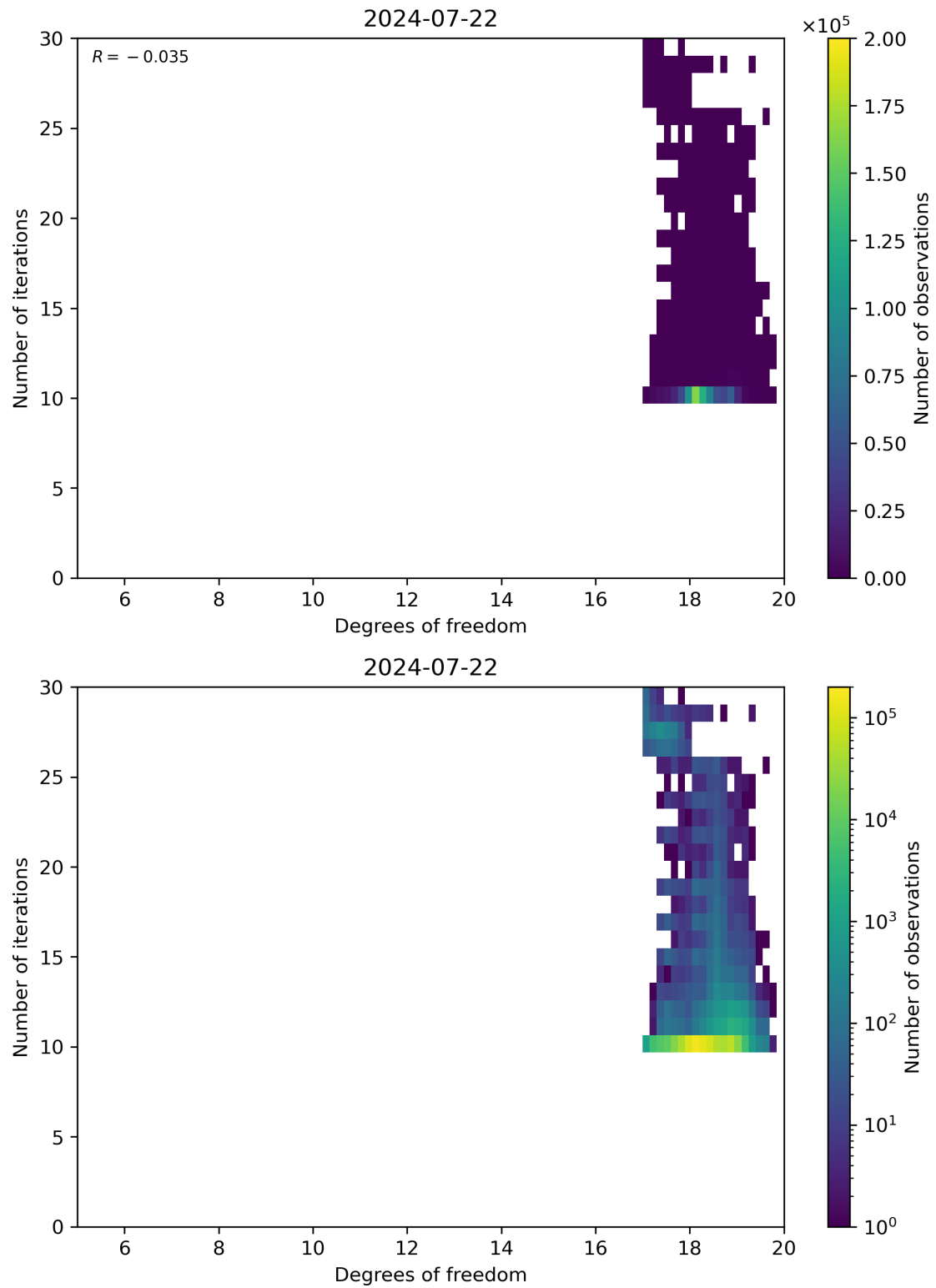
Figure 52: Scatter density plot of “Degrees of freedom” against “Number of iterations” for 2024-07-21 to 2024-07-23.
