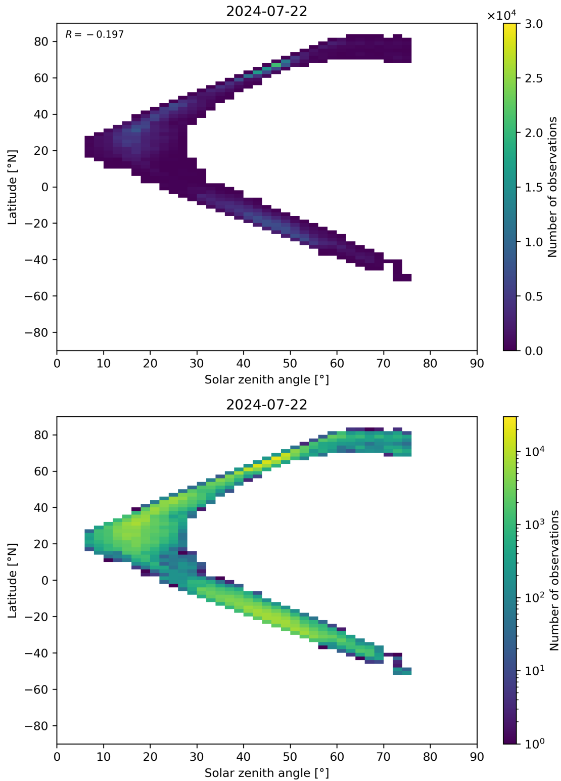
Figure 98: Scatter density plot of “Solar zenith angle” against “Latitude” for 2024-07-21 to 2024-07-23.
