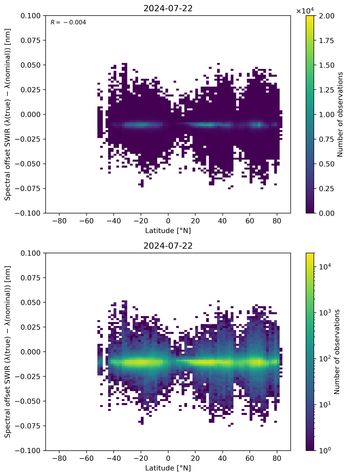
Figure 62: Scatter density plot of “Latitude” against “Spectral offset SWIR ( \lambda(\text{true}) - \lambda(\text{nominal}) )” for 2024-07-21 to 2024-07-23.
