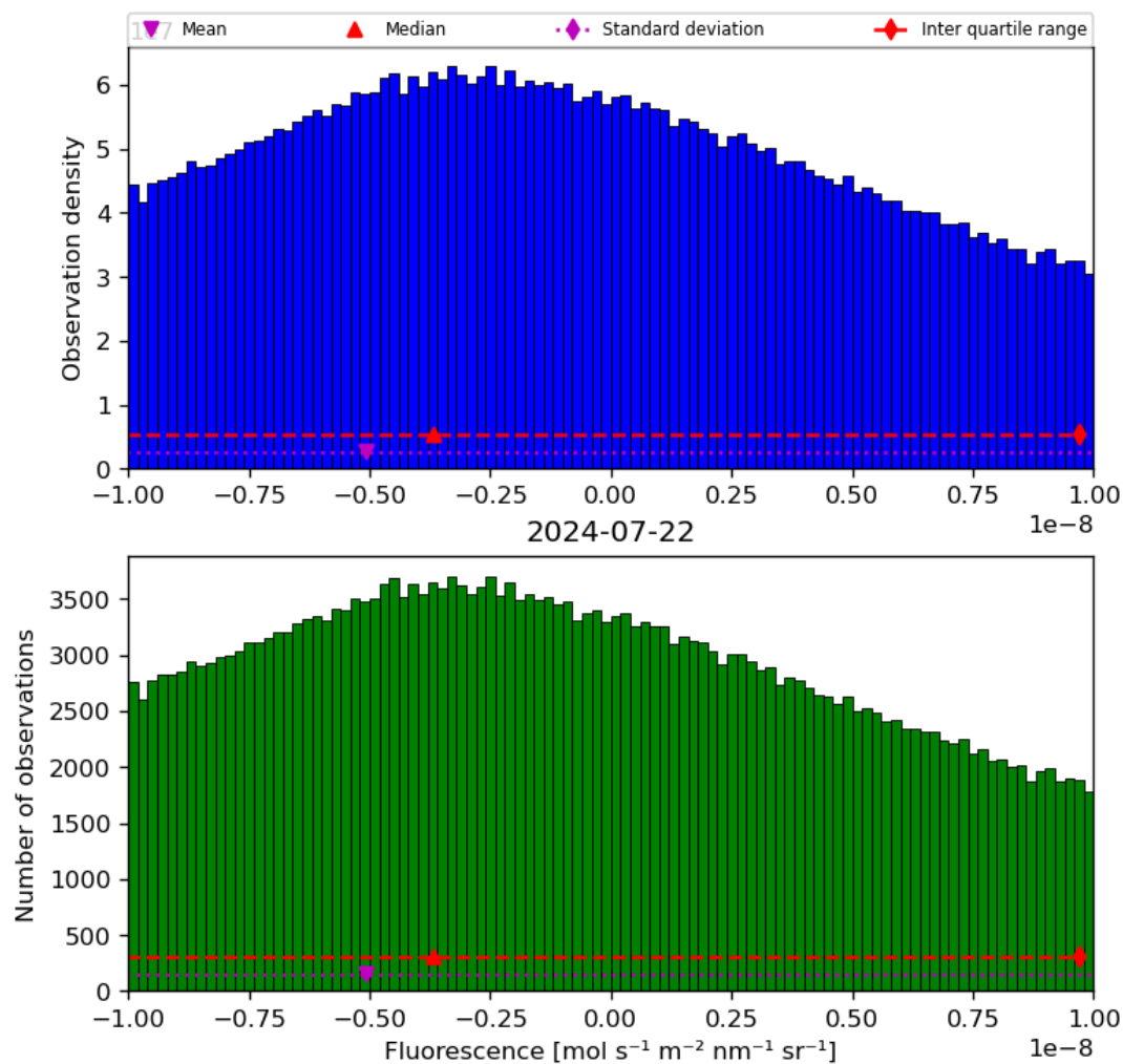
Figure 32: Histogram of “Fluorescence” for 2024-07-21 to 2024-07-23
