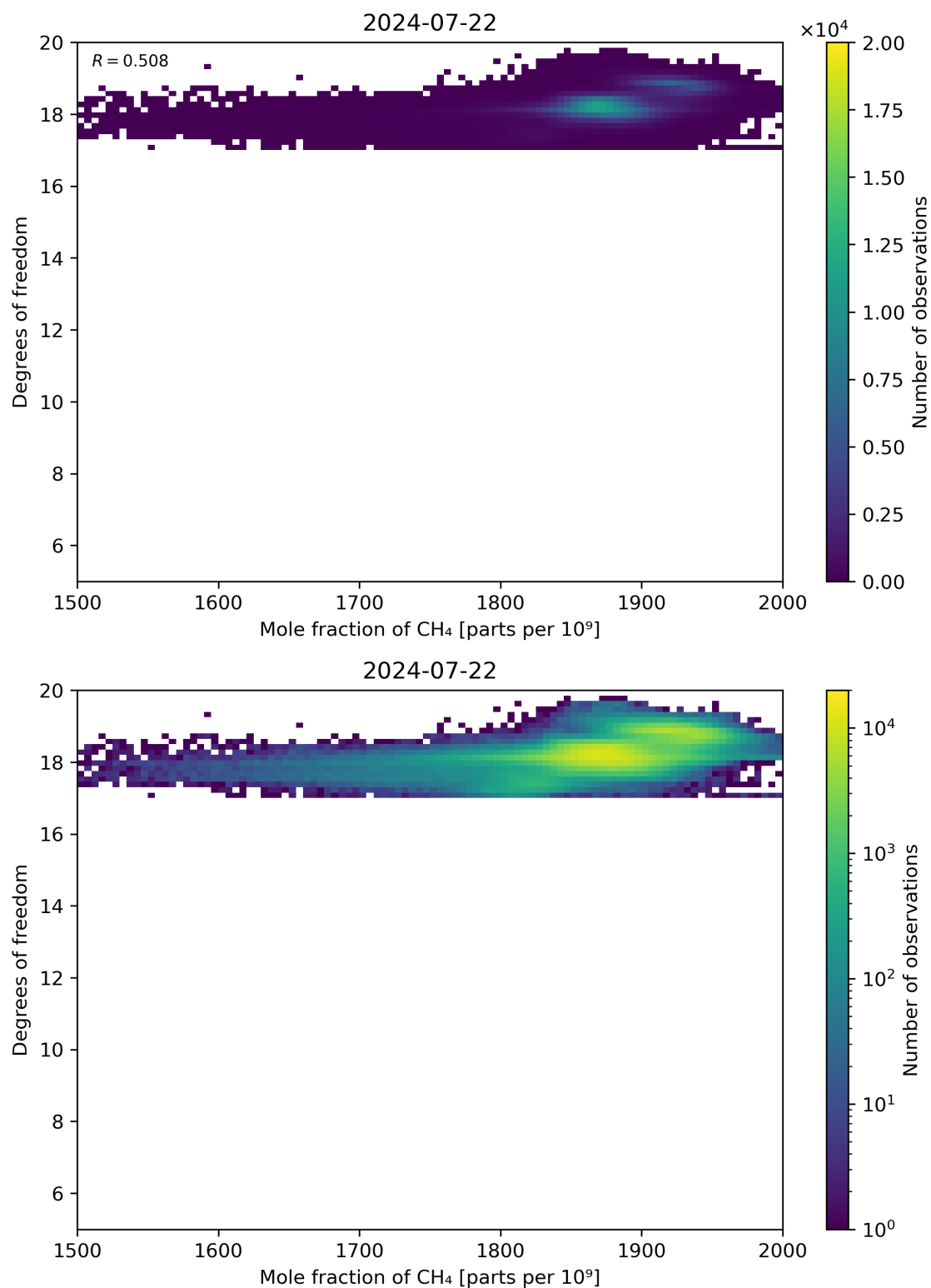
Figure 72: Scatter density plot of “Mole fraction of CH 4 ” against “Degrees of freedom” for 2024-07-21 to 2024-07-23.
