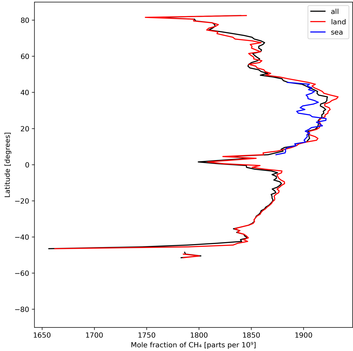
Figure 12: Zonal average of “Mole fraction of CH 4 ” for 2024-07-21 to 2024-07-23.
