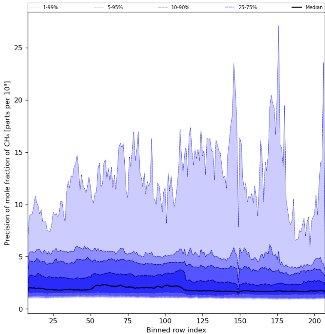
Figure 35: Along track statistics of “Precision of mole fraction of CH 4 ” for 2024-07-21 to 2024-07-23
