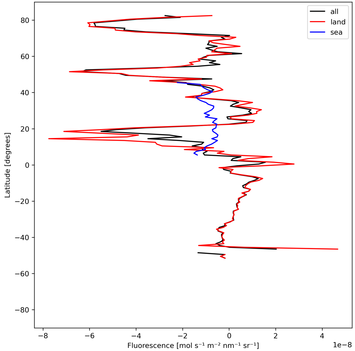
Figure 21: Zonal average of “Fluorescence” for 2024-07-21 to 2024-07-23.
