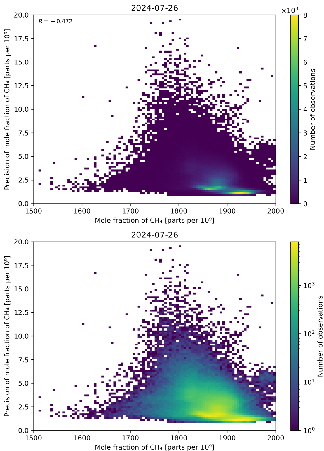
Figure 75: Scatter density plot of “Mole fraction of CH 4 ” against “Precision of mole fraction of CH 4 ” for 2024-07-26 to 2024-07-27.
