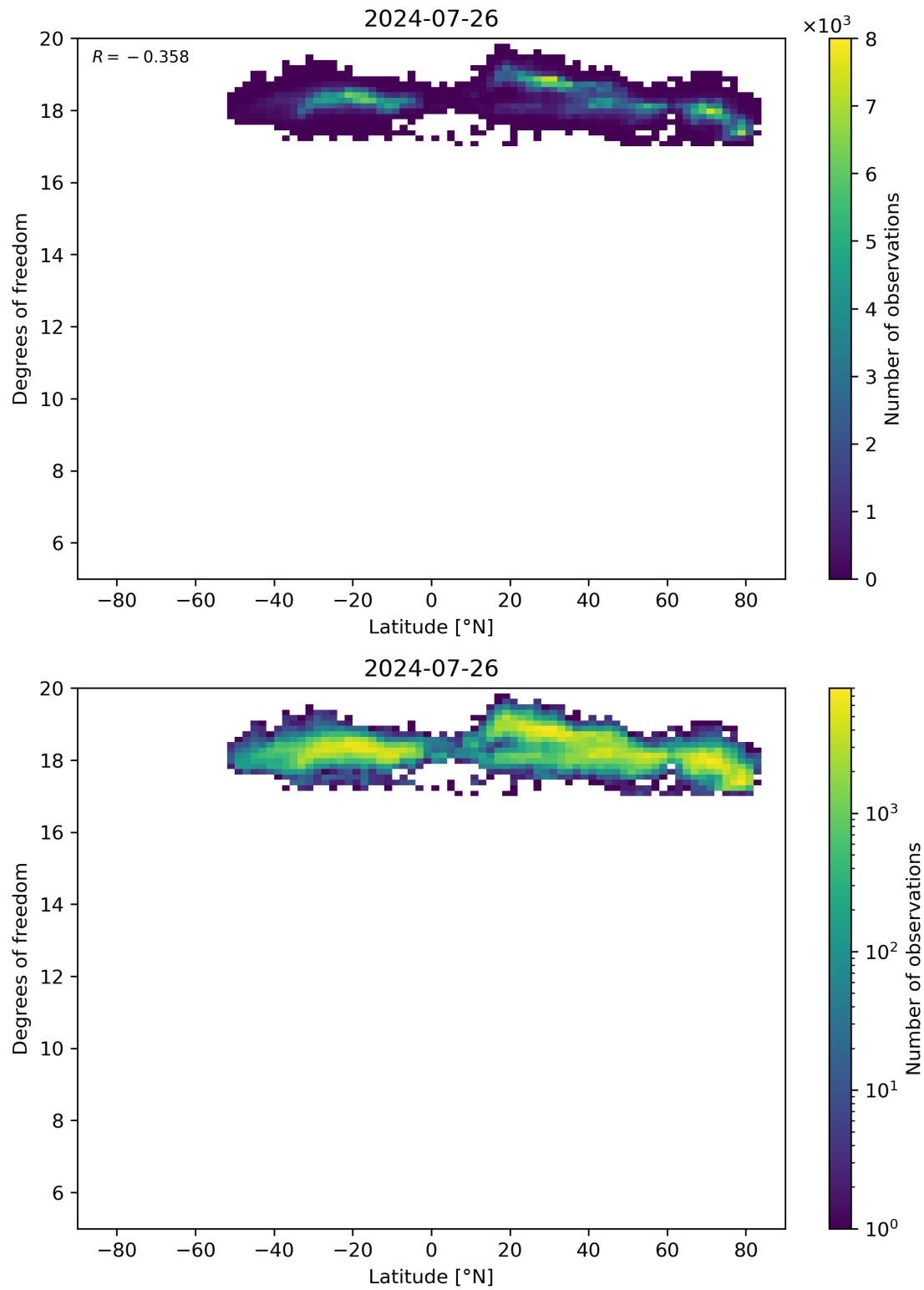
Figure 55: Scatter density plot of “Latitude” against “Degrees of freedom” for 2024-07-26 to 2024-07-27.
