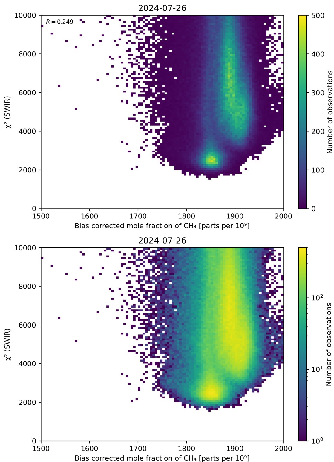
Figure 64: Scatter density plot of “Bias corrected mole fraction of CH 4 ” against “ \chi^2 (SWIR)” for 2024-07-26 to 2024-07-27.
