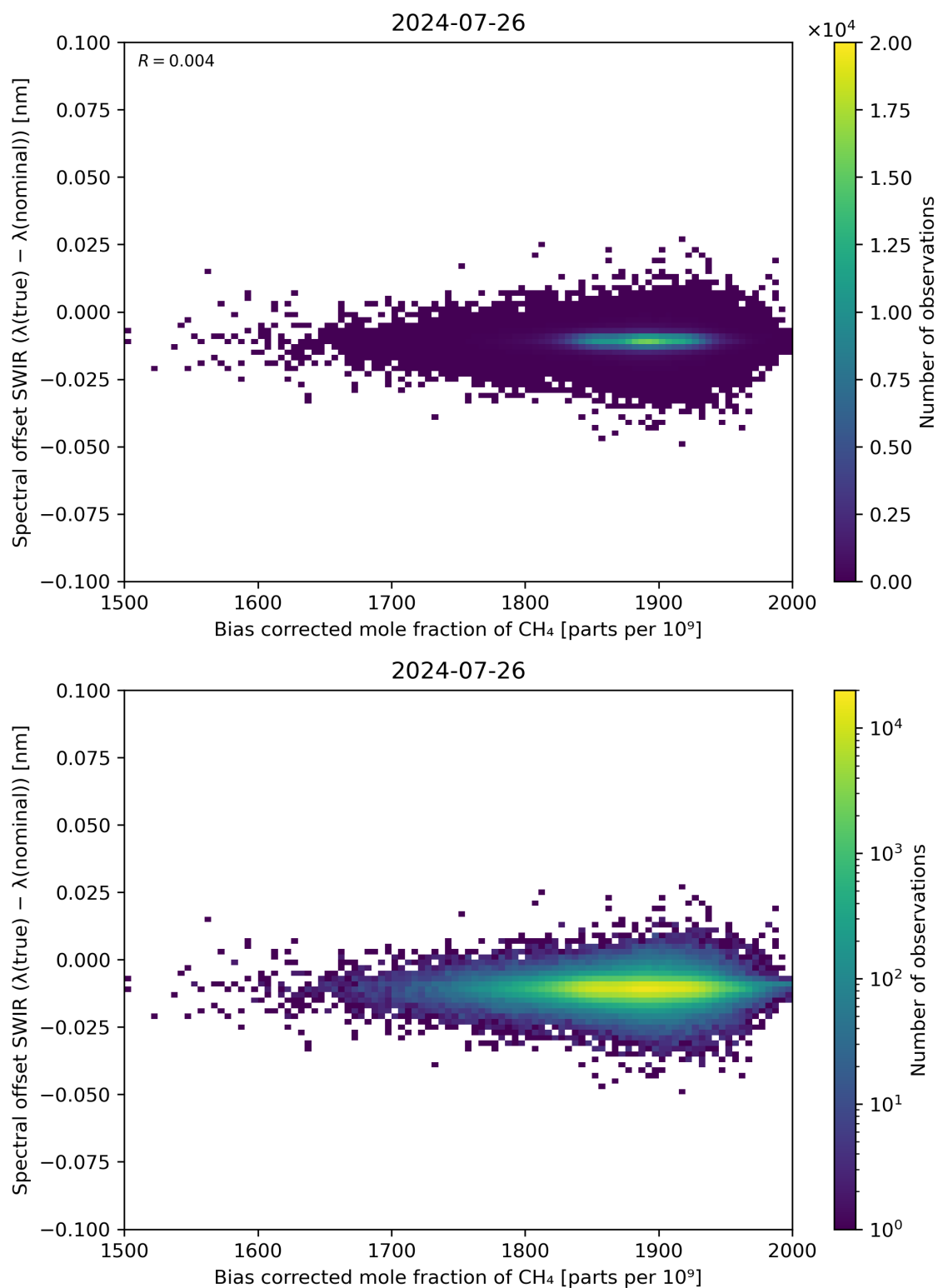
Figure 69: Scatter density plot of “Bias corrected mole fraction of \text{CH}_4 ” against “Spectral offset SWIR ( \lambda(\text{true}) - \lambda(\text{nominal}) )” for 2024-07-26 to 2024-07-27.
