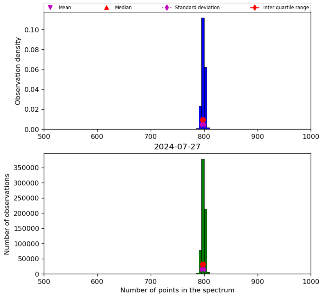
Figure 26: Histogram of “Number of points in the spectrum” for 2024-07-26 to 2024-07-28
