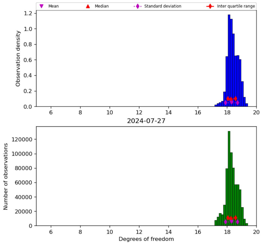
Figure 30: Histogram of “Degrees of freedom” for 2024-07-26 to 2024-07-28
