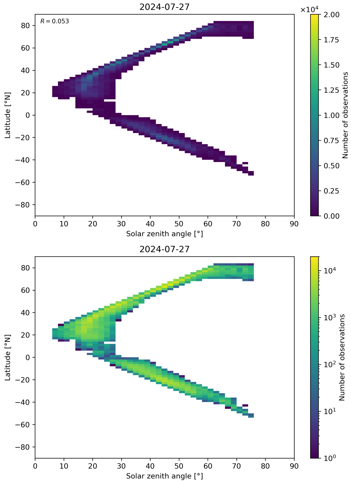
Figure 98: Scatter density plot of “Solar zenith angle” against “Latitude” for 2024-07-26 to 2024-07-28.
