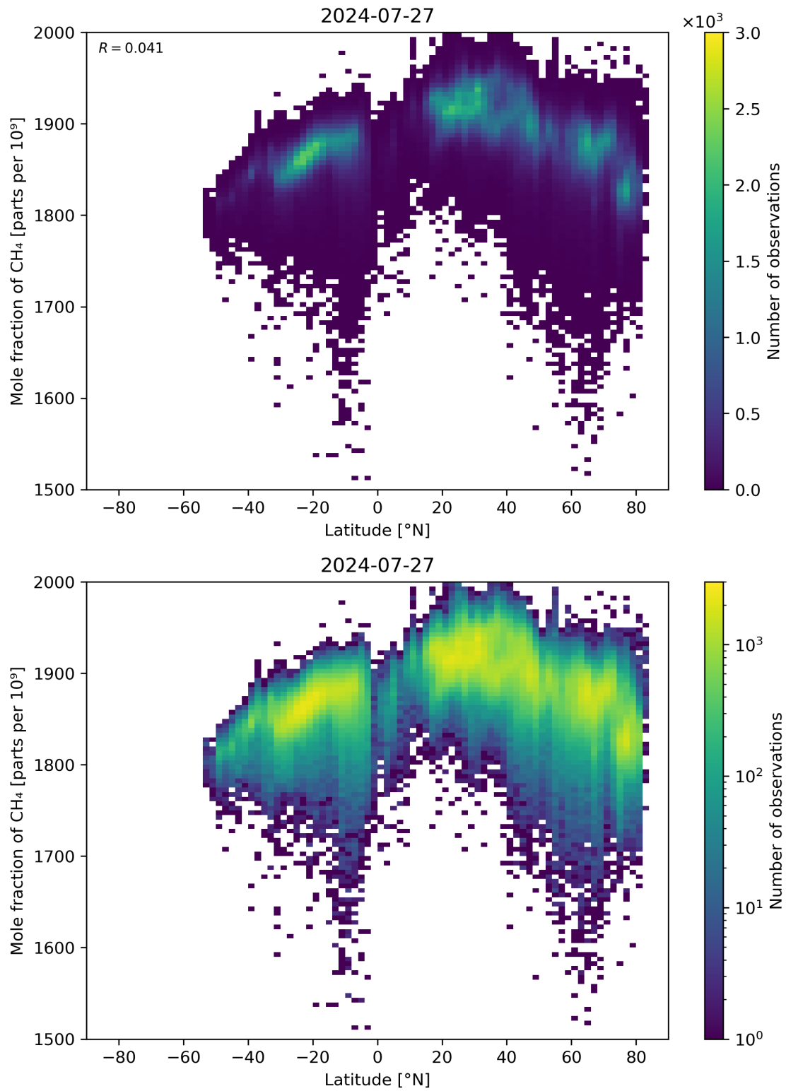
Figure 57: Scatter density plot of “Latitude” against “Mole fraction of \text{CH}_4 ” for 2024-07-26 to 2024-07-28.
