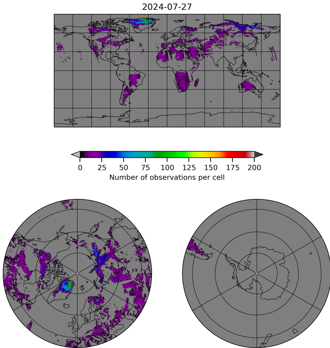
Figure 10: Map of the number of observations for 2024-07-26 to 2024-07-28
