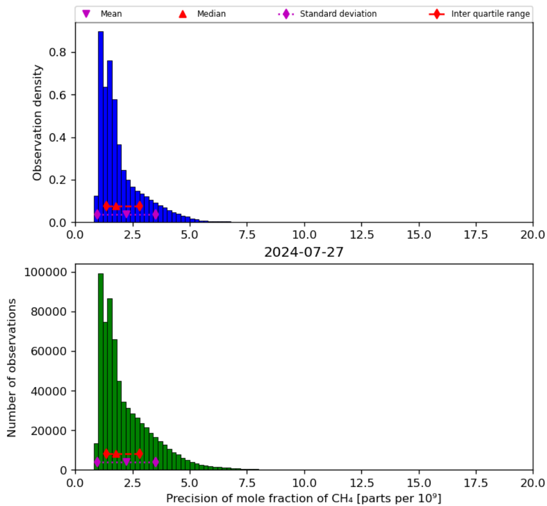
Figure 24: Histogram of “Precision of mole fraction of CH 4 ” for 2024-07-26 to 2024-07-28
