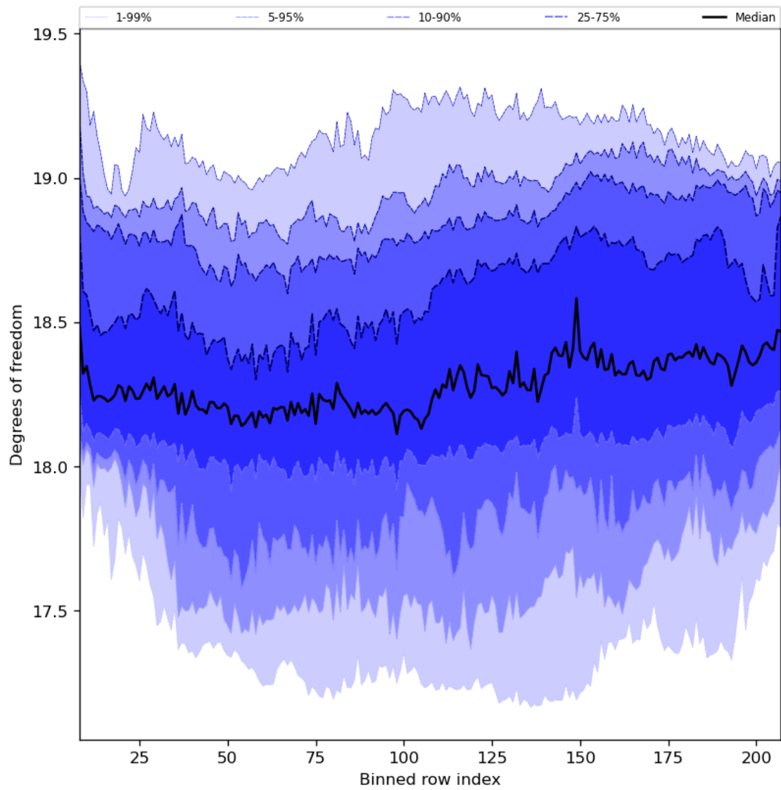
Figure 41: Along track statistics of “Degrees of freedom” for 2024-07-26 to 2024-07-28
