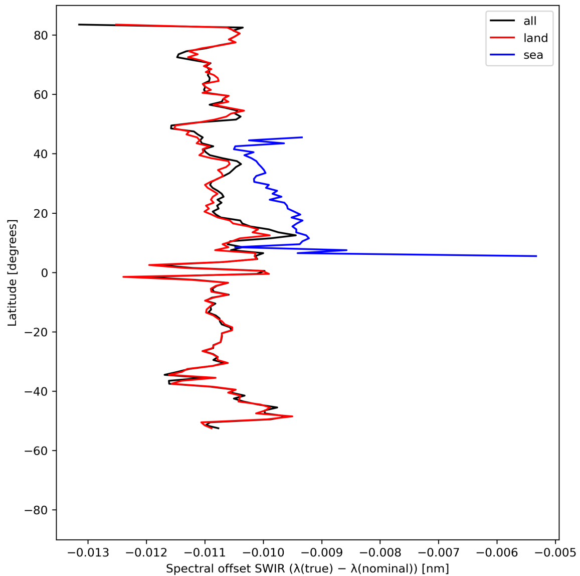
Figure 16: Zonal average of “Spectral offset SWIR ( \lambda(\text{true}) - \lambda(\text{nominal}) )” for 2024-07-26 to 2024-07-28.
