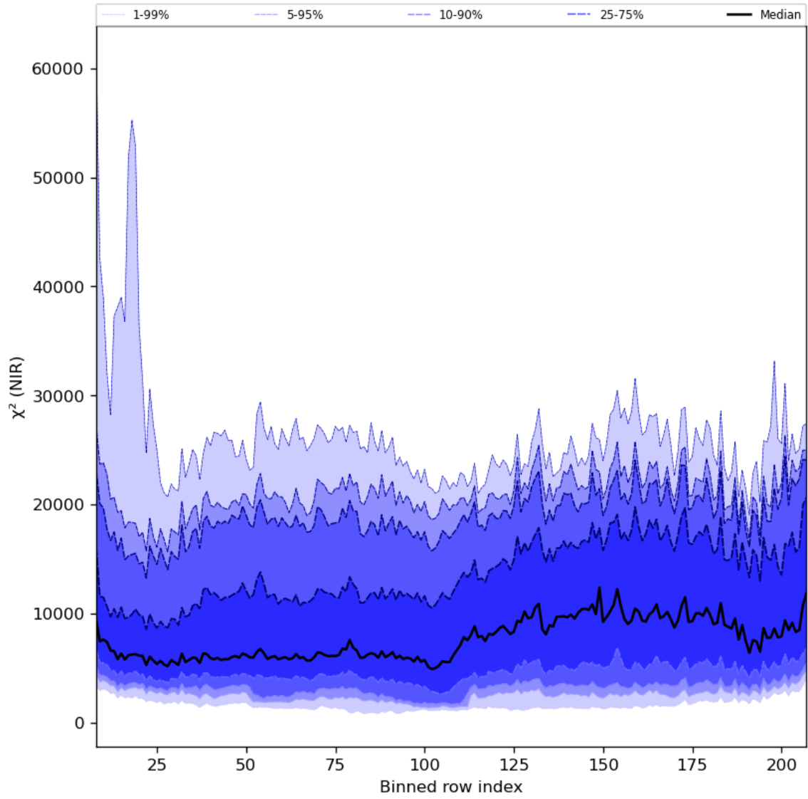
Figure 40: Along track statistics of “ \chi^2 (NIR)” for 2024-07-26 to 2024-07-28
