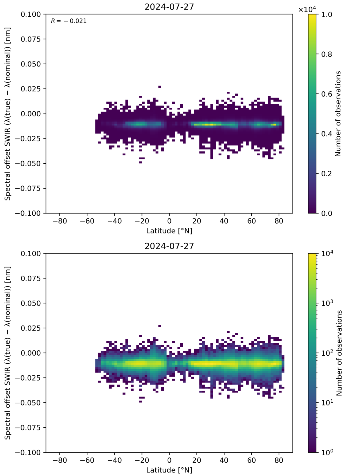
Figure 62: Scatter density plot of “Latitude” against “Spectral offset SWIR ( \lambda(\text{true}) - \lambda(\text{nominal}) )” for 2024-07-26 to 2024-07-28.
