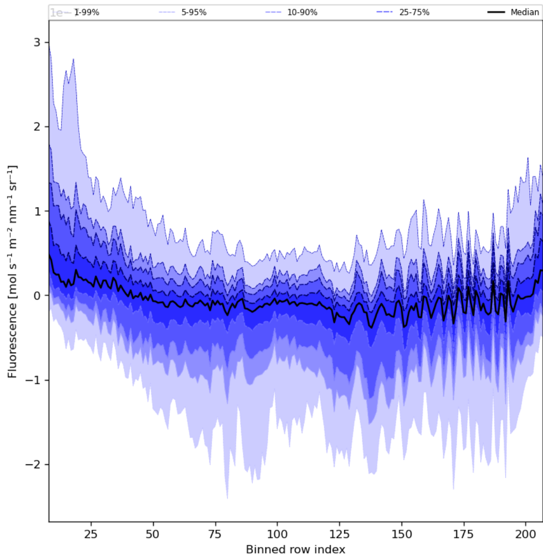
Figure 43: Along track statistics of "Fluorescence" for 2024-07-26 to 2024-07-28
