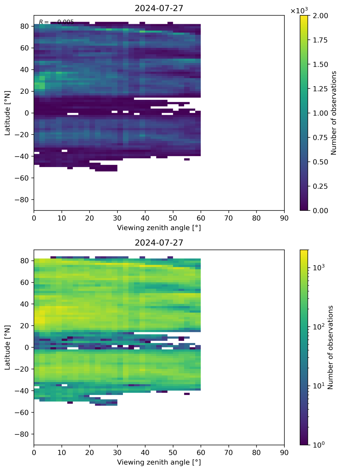
Figure 109: Scatter density plot of “Viewing zenith angle” against “Latitude” for 2024-07-26 to 2024-07-28.
