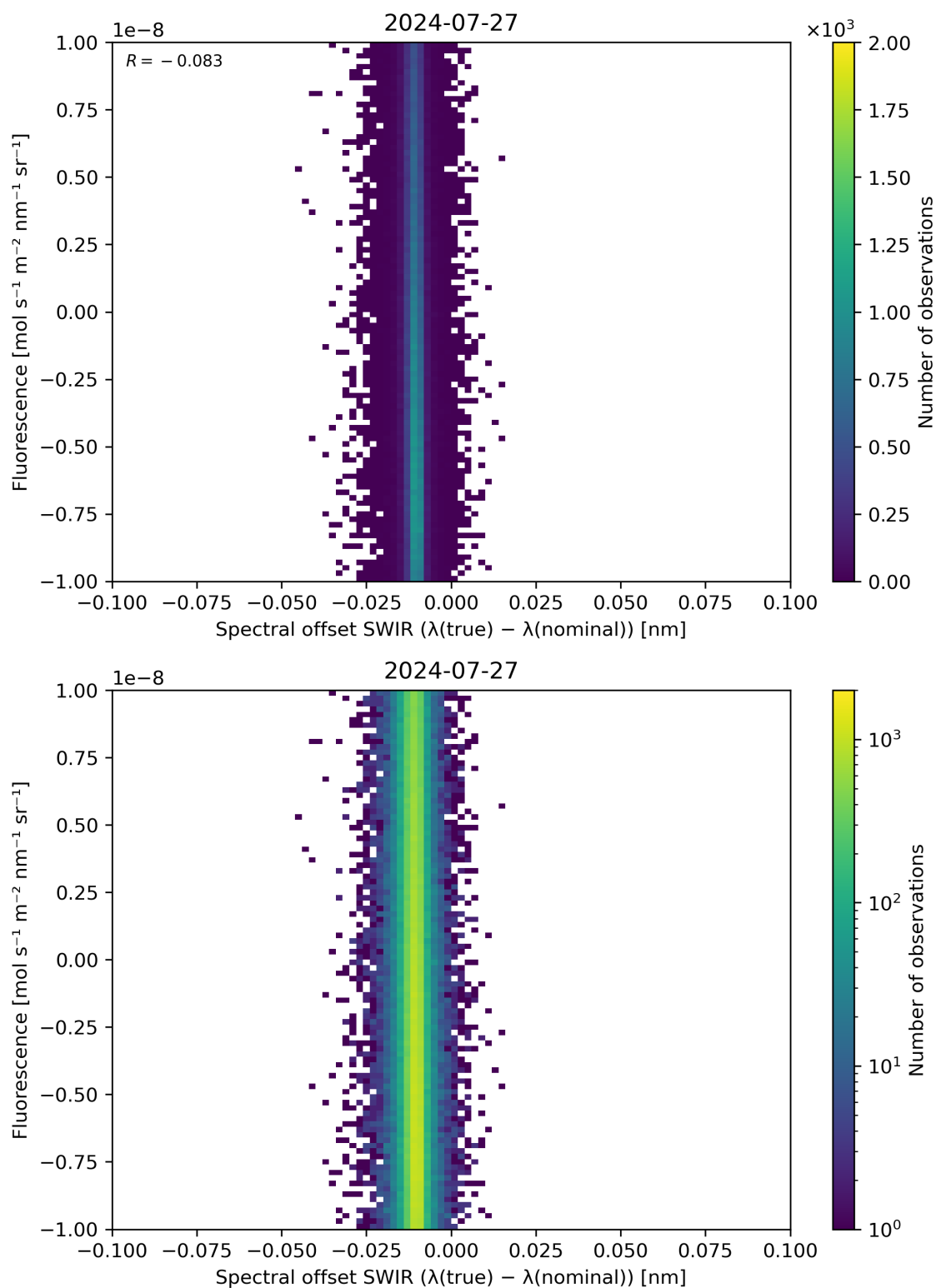
Figure 120: Scatter density plot of “Spectral offset SWIR ( \lambda(\text{true}) - \lambda(\text{nominal}) )” against “Fluorescence” for 2024-07-26 to 2024-07-28.
