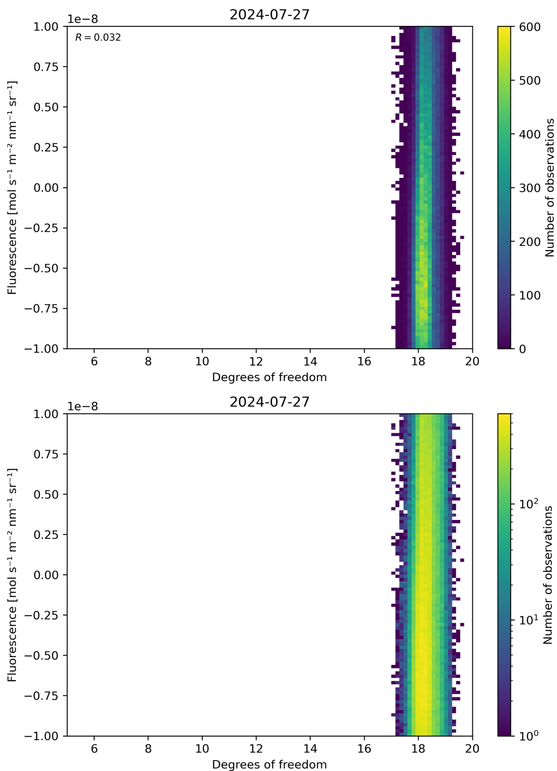
Figure 51: Scatter density plot of “Degrees of freedom” against “Fluorescence” for 2024-07-26 to 2024-07-28.
