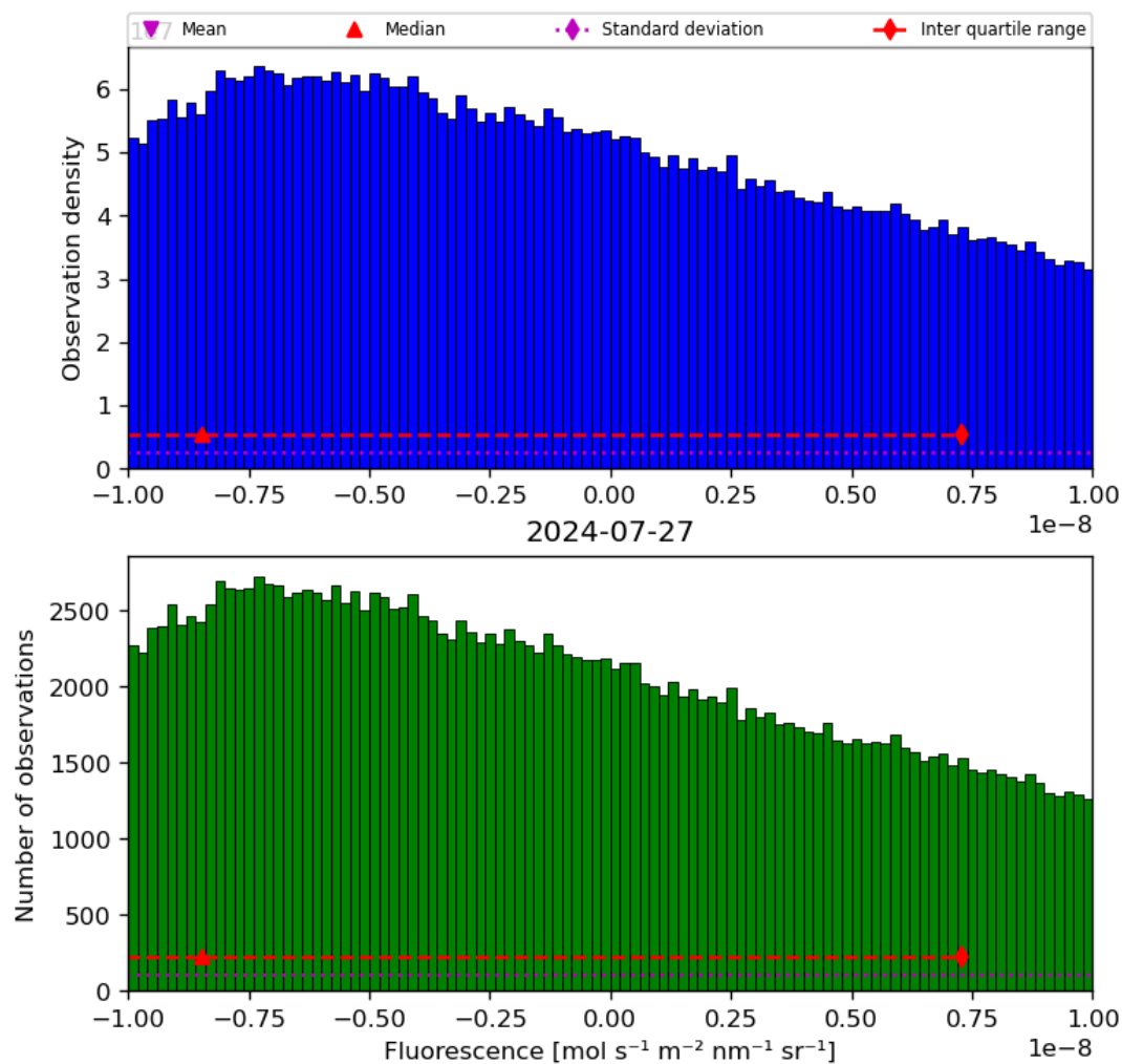
Figure 32: Histogram of “Fluorescence” for 2024-07-26 to 2024-07-28
