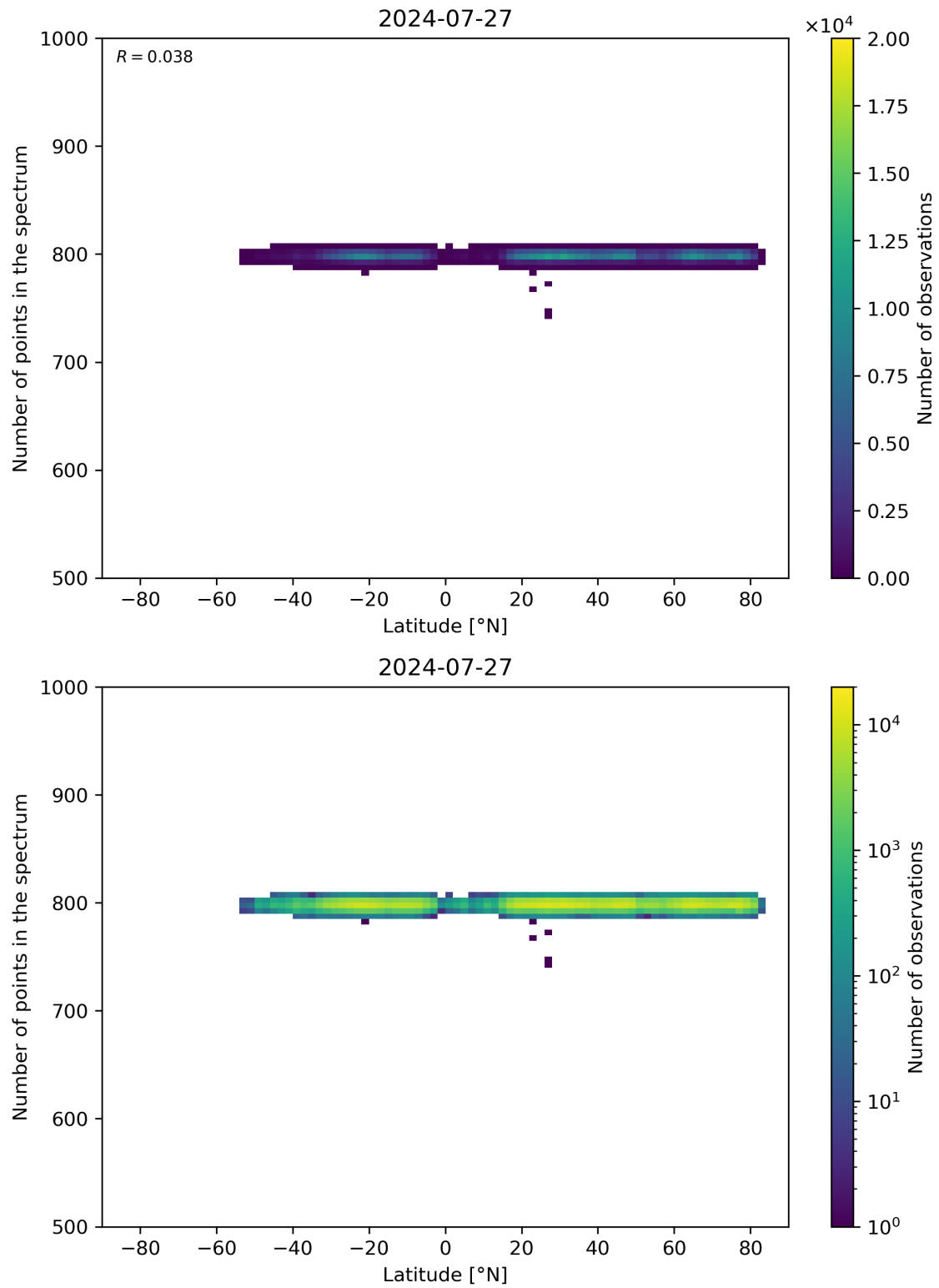
Figure 61: Scatter density plot of “Latitude” against “Number of points in the spectrum” for 2024-07-26 to 2024-07-28.
