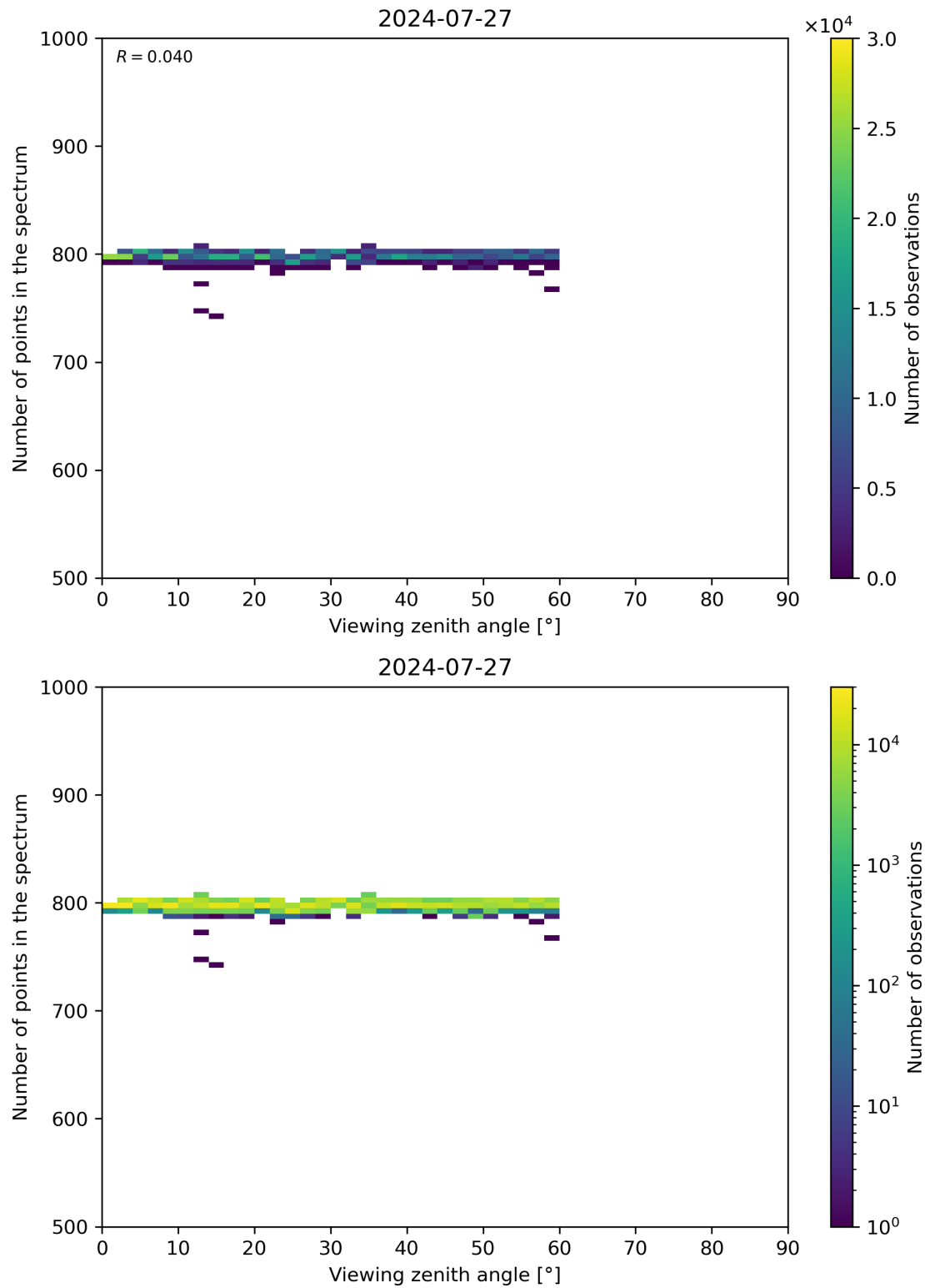
Figure 114: Scatter density plot of “Viewing zenith angle” against “Number of points in the spectrum” for 2024-07-26 to 2024-07-28.
