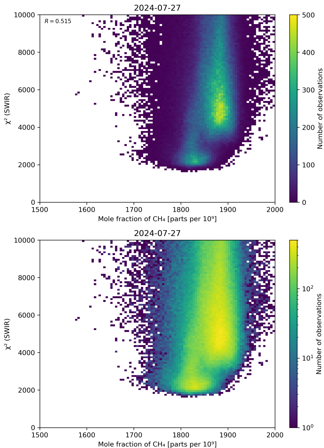
Figure 71: Scatter density plot of “Mole fraction of \text{CH}_4 ” against “ \chi^2 (SWIR)” for 2024-07-26 to 2024-07-28.
