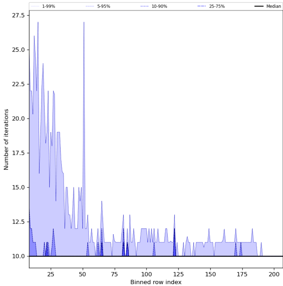
Figure 42: Along track statistics of “Number of iterations” for 2024-07-26 to 2024-07-28
