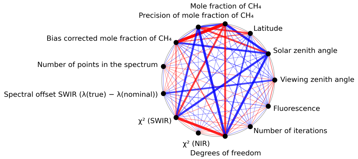
Figure 1: Map of correlation graph for 2024-07-26 to 2024-07-28.
