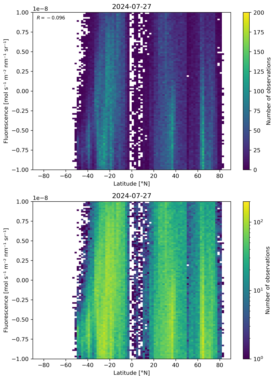
Figure 56: Scatter density plot of “Latitude” against “Fluorescence” for 2024-07-26 to 2024-07-28.
