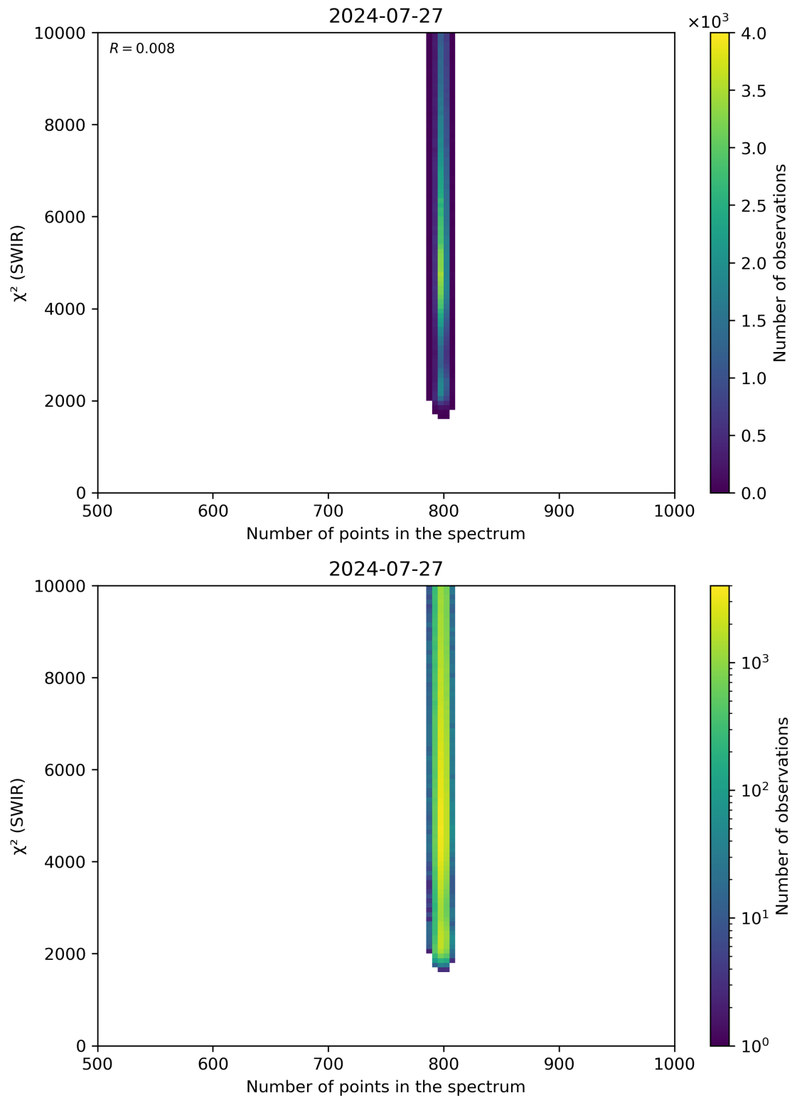
Figure 89: Scatter density plot of “Number of points in the spectrum” against “ \chi^2 (SWIR)” for 2024-07-26 to 2024-07-28.
