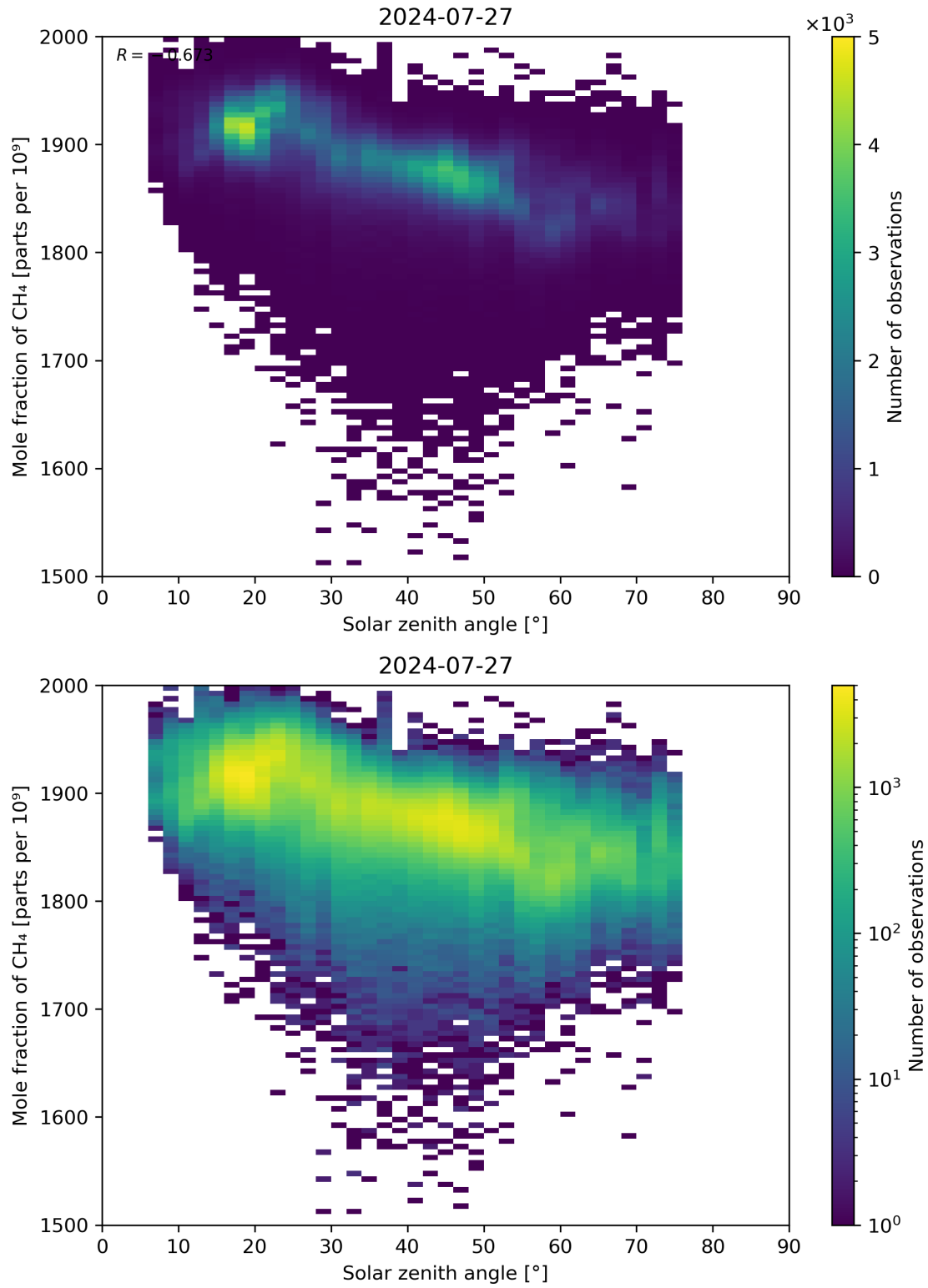
Figure 99: Scatter density plot of “Solar zenith angle” against “Mole fraction of CH 4 ” for 2024-07-26 to 2024-07-28.
