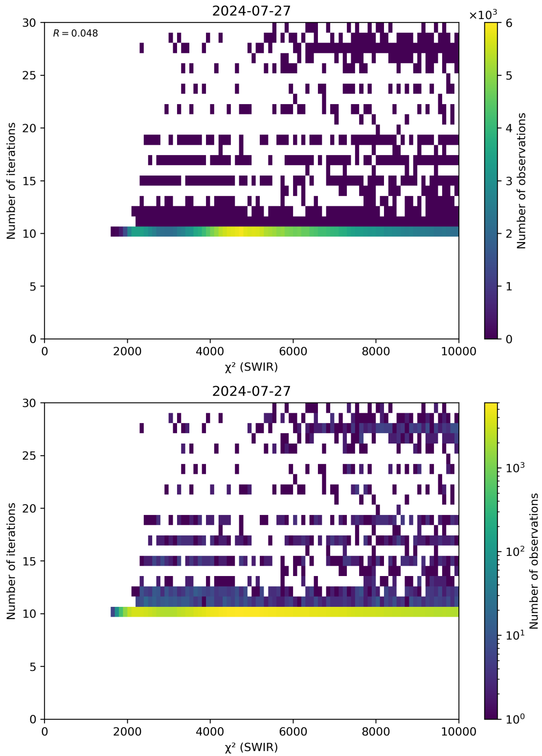
Figure 50: Scatter density plot of “ \chi^2 (SWIR)” against “Number of iterations” for 2024-07-26 to 2024-07-28.
