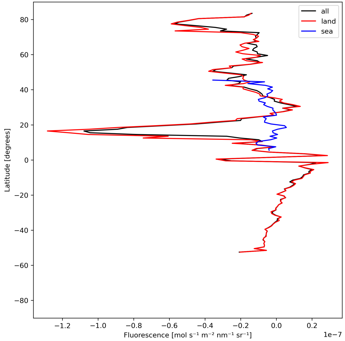
Figure 21: Zonal average of “Fluorescence” for 2024-07-26 to 2024-07-28.
