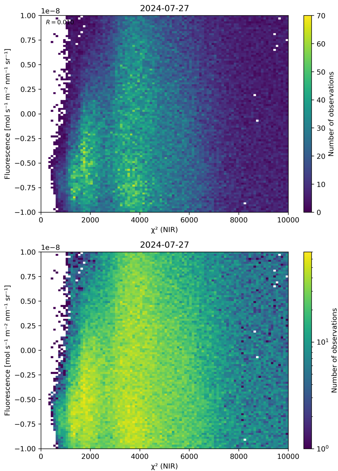
Figure 45: Scatter density plot of “ \chi^2 (NIR)” against “Fluorescence” for 2024-07-26 to 2024-07-28.
