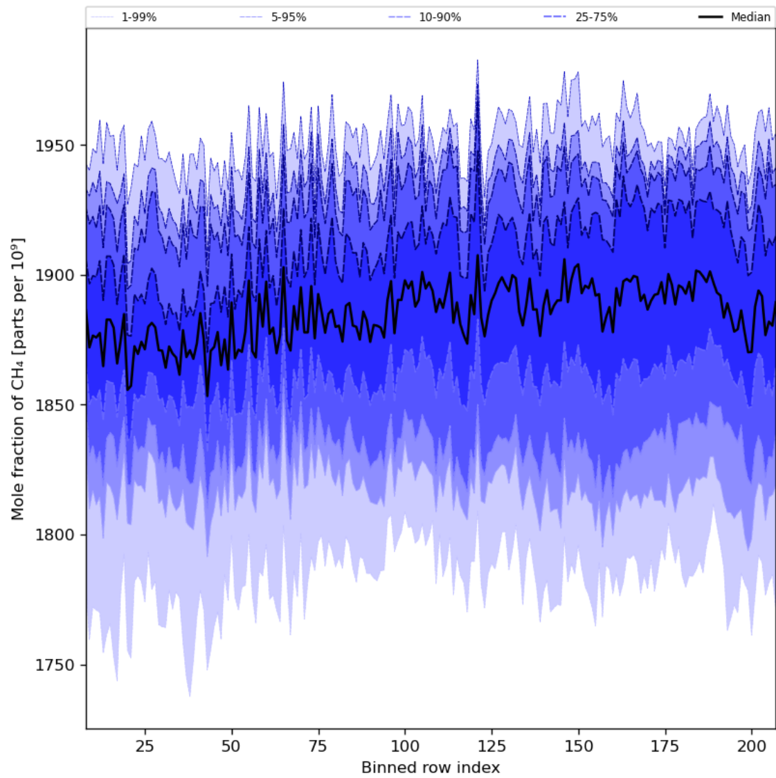
Figure 34: Along track statistics of “Mole fraction of CH 4 ” for 2024-07-26 to 2024-07-28
