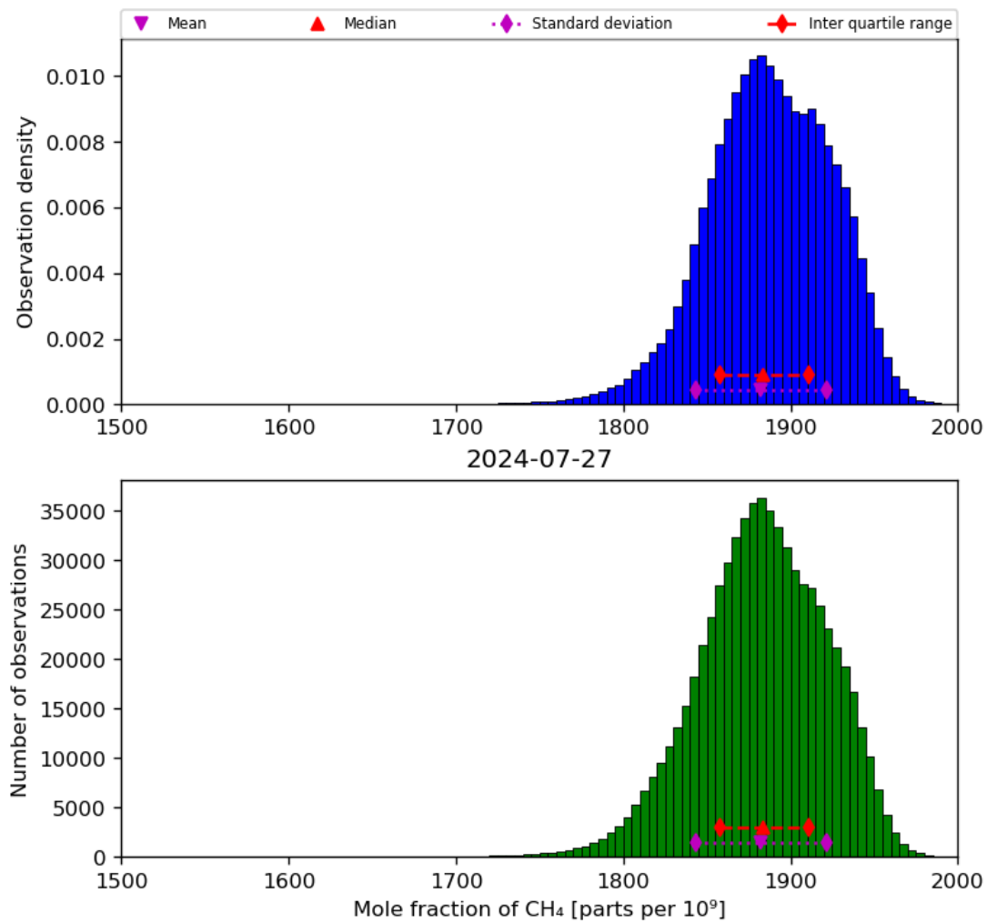
Figure 23: Histogram of “Mole fraction of CH 4 ” for 2024-07-26 to 2024-07-28
