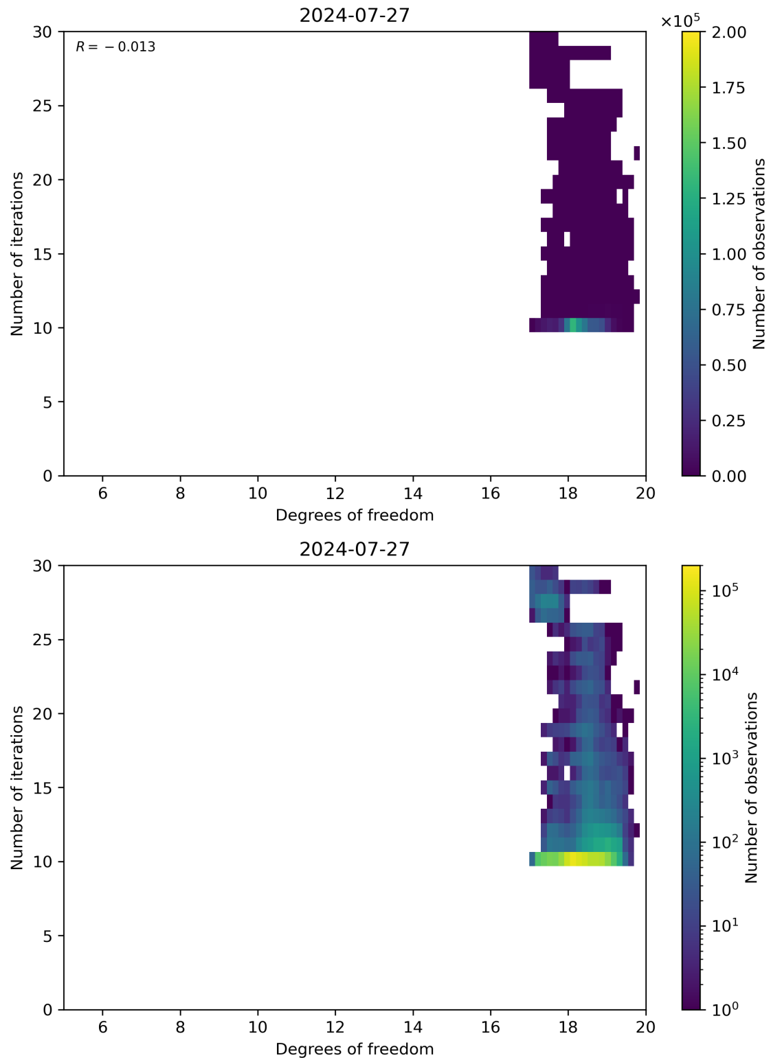
Figure 52: Scatter density plot of “Degrees of freedom” against “Number of iterations” for 2024-07-26 to 2024-07-28.
