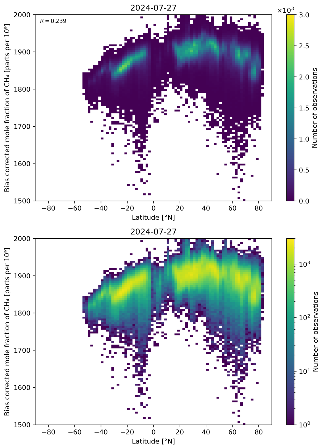
Figure 58: Scatter density plot of “Latitude” against “Bias corrected mole fraction of CH 4 ” for 2024-07-26 to 2024-07-28.
