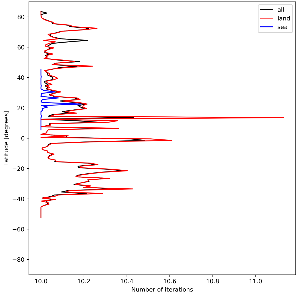
Figure 20: Zonal average of “Number of iterations” for 2024-07-26 to 2024-07-28.
