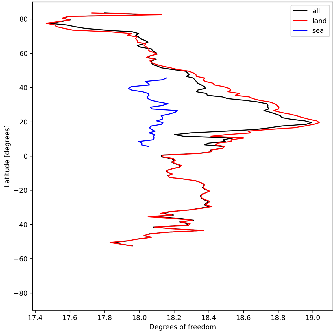
Figure 19: Zonal average of “Degrees of freedom” for 2024-07-26 to 2024-07-28.
