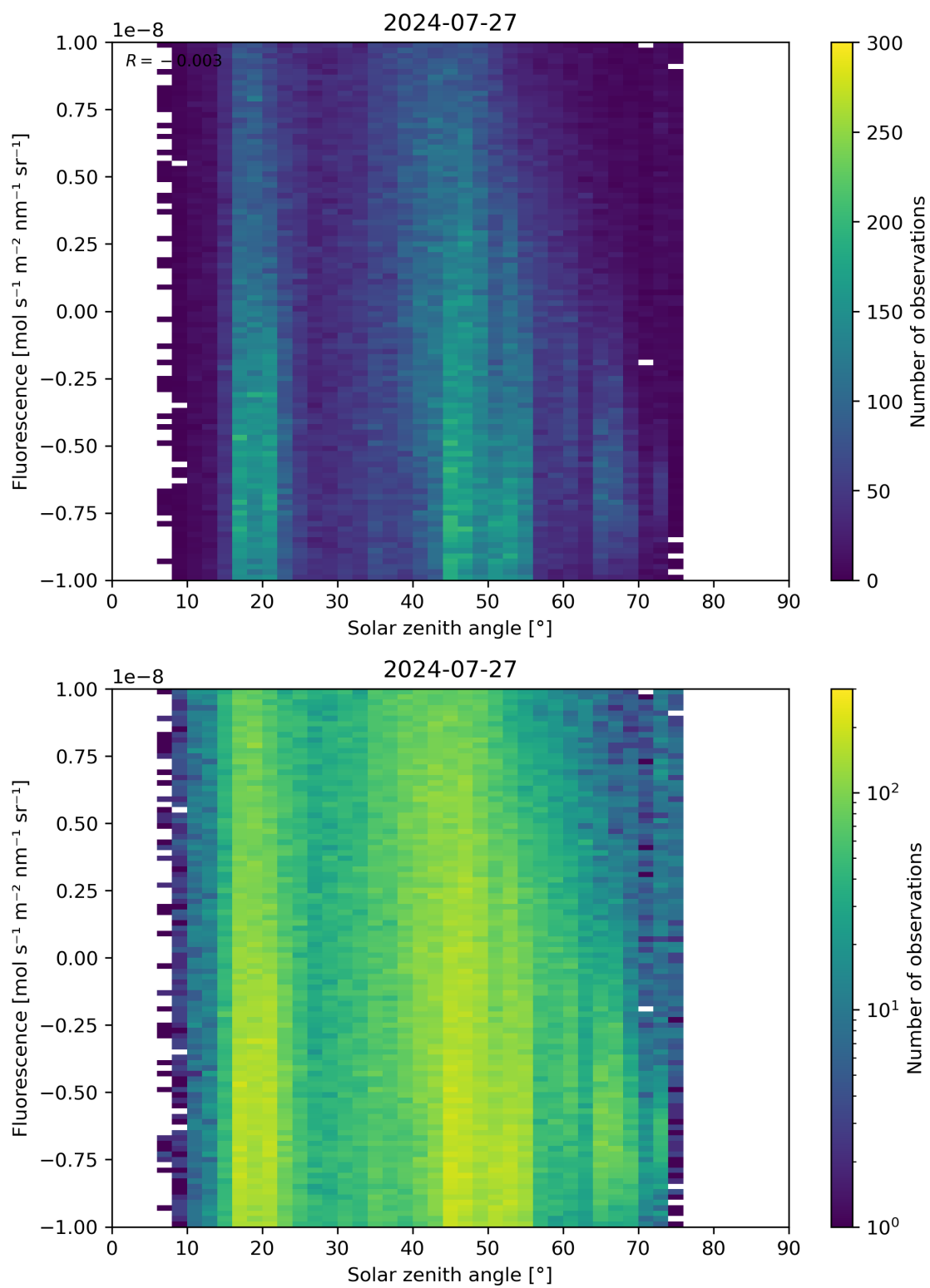
Figure 97: Scatter density plot of “Solar zenith angle” against “Fluorescence” for 2024-07-26 to 2024-07-28.
