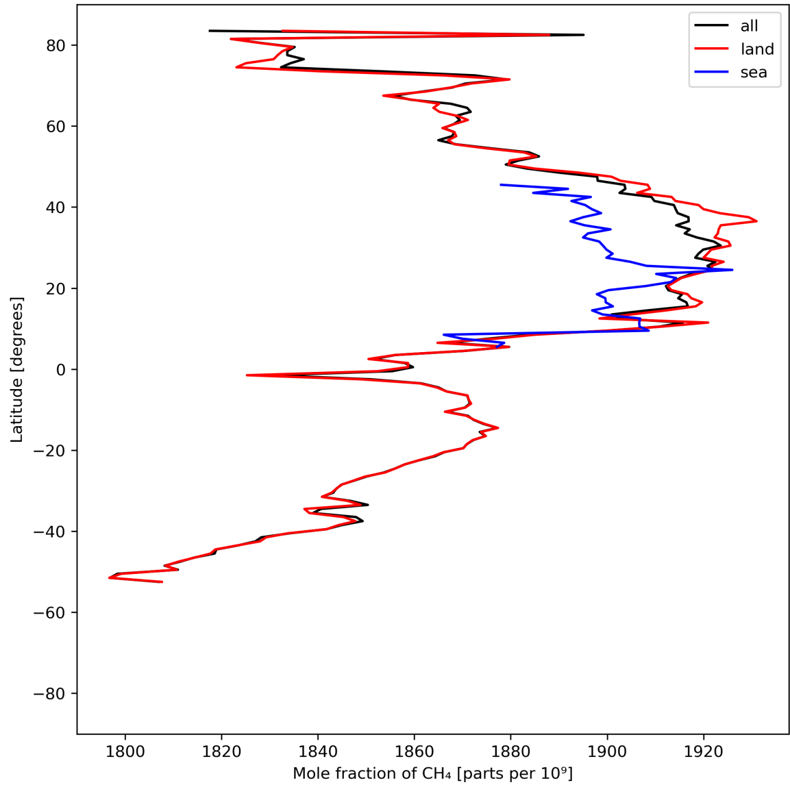
Figure 12: Zonal average of “Mole fraction of \text{CH}_4 ” for 2024-07-26 to 2024-07-28.
