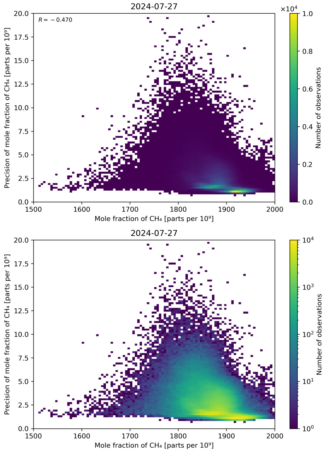
Figure 75: Scatter density plot of “Mole fraction of CH 4 ” against “Precision of mole fraction of CH 4 ” for 2024-07-26 to 2024-07-28.
