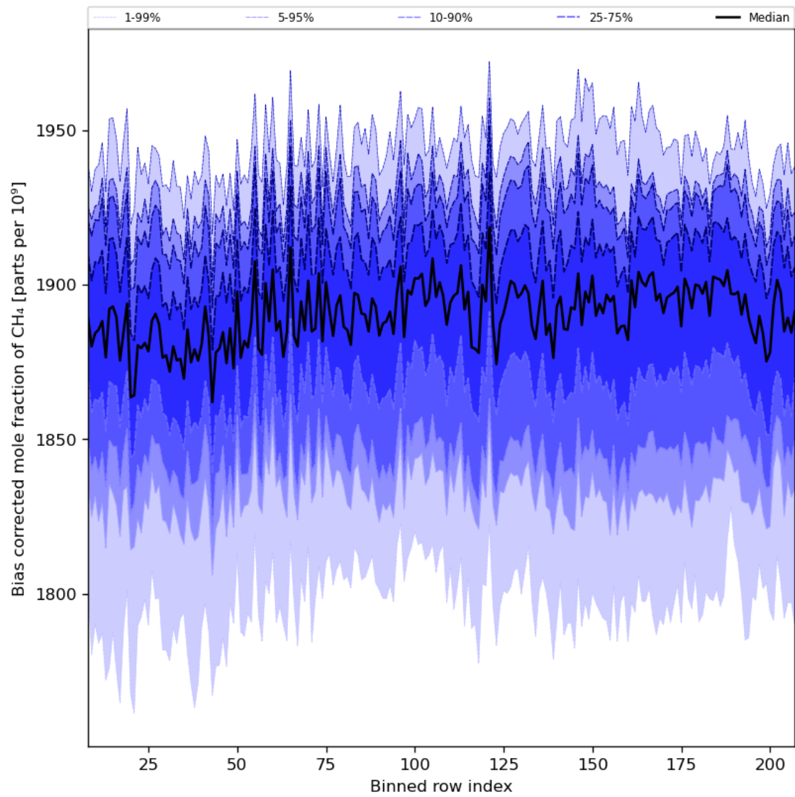
Figure 36: Along track statistics of “Bias corrected mole fraction of CH 4 ” for 2024-07-26 to 2024-07-28
