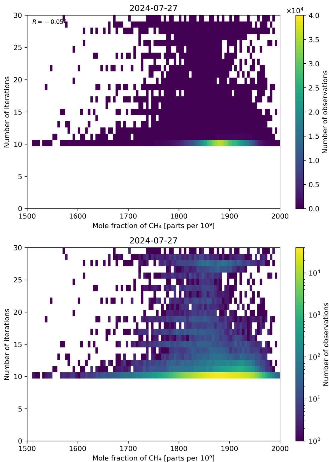
Figure 76: Scatter density plot of “Mole fraction of CH 4 ” against “Number of iterations” for 2024-07-26 to 2024-07-28.
