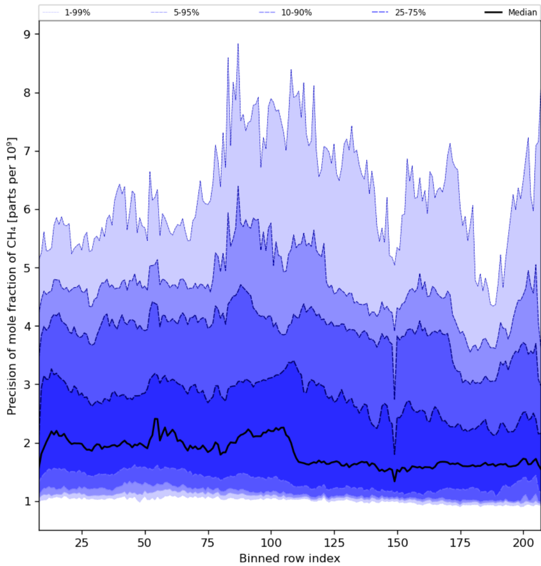
Figure 35: Along track statistics of “Precision of mole fraction of CH 4 ” for 2024-07-26 to 2024-07-28
