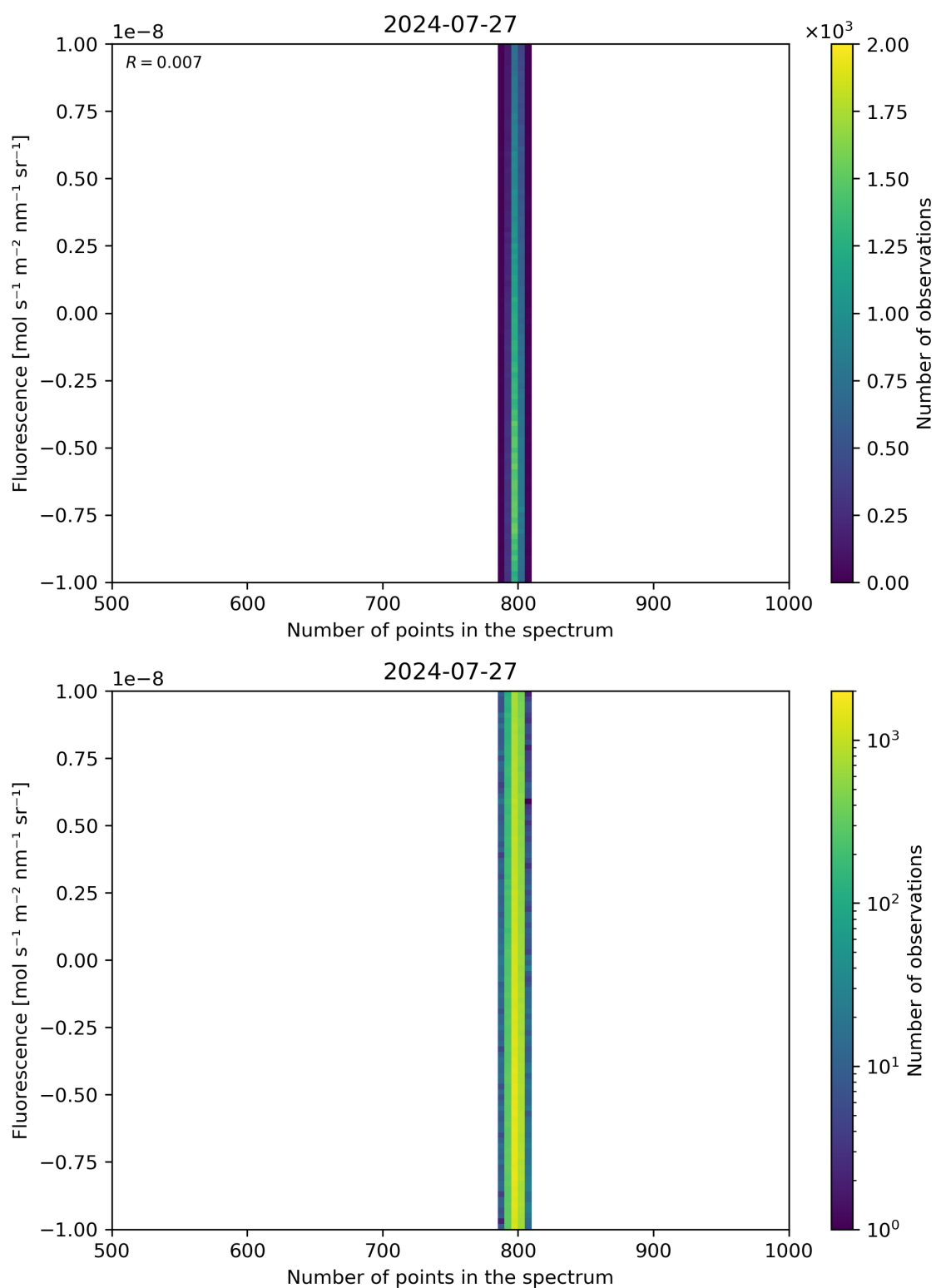
Figure 91: Scatter density plot of “Number of points in the spectrum” against “Fluorescence” for 2024-07-26 to 2024-07-28.
