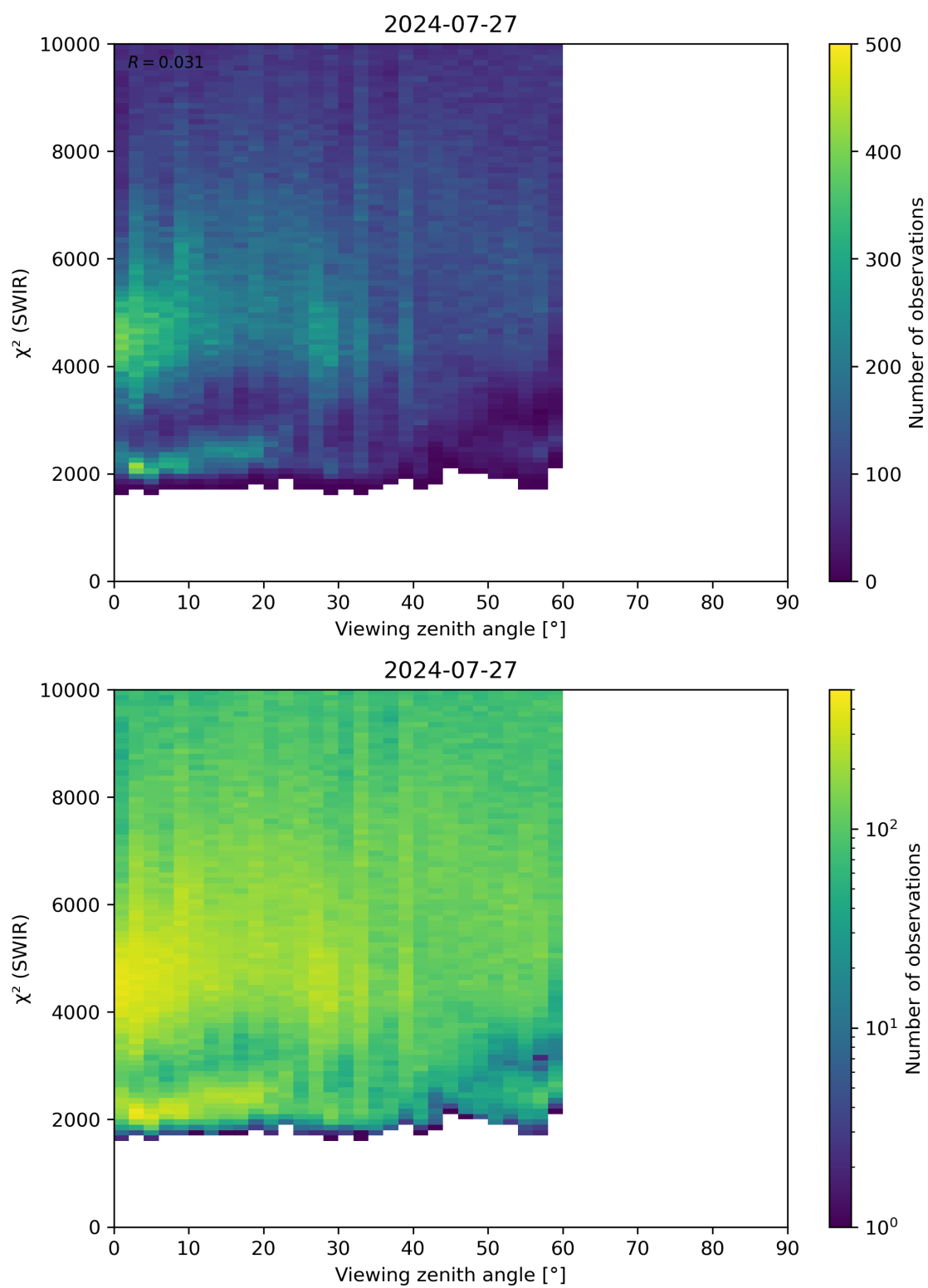
Figure 106: Scatter density plot of “Viewing zenith angle” against “ \chi^2 (SWIR)” for 2024-07-26 to 2024-07-28.
