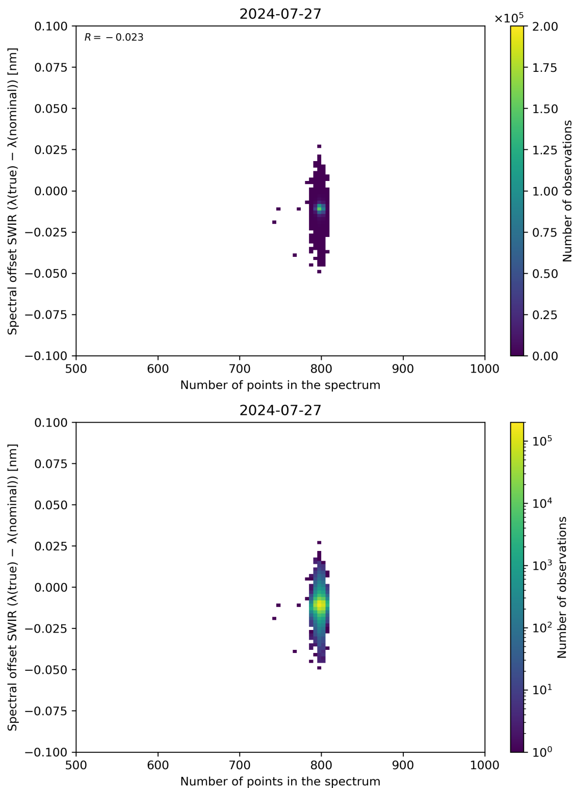
Figure 93: Scatter density plot of “Number of points in the spectrum” against “Spectral offset SWIR ( \lambda(\text{true}) - \lambda(\text{nominal}) )” for 2024-07-26 to 2024-07-28.
