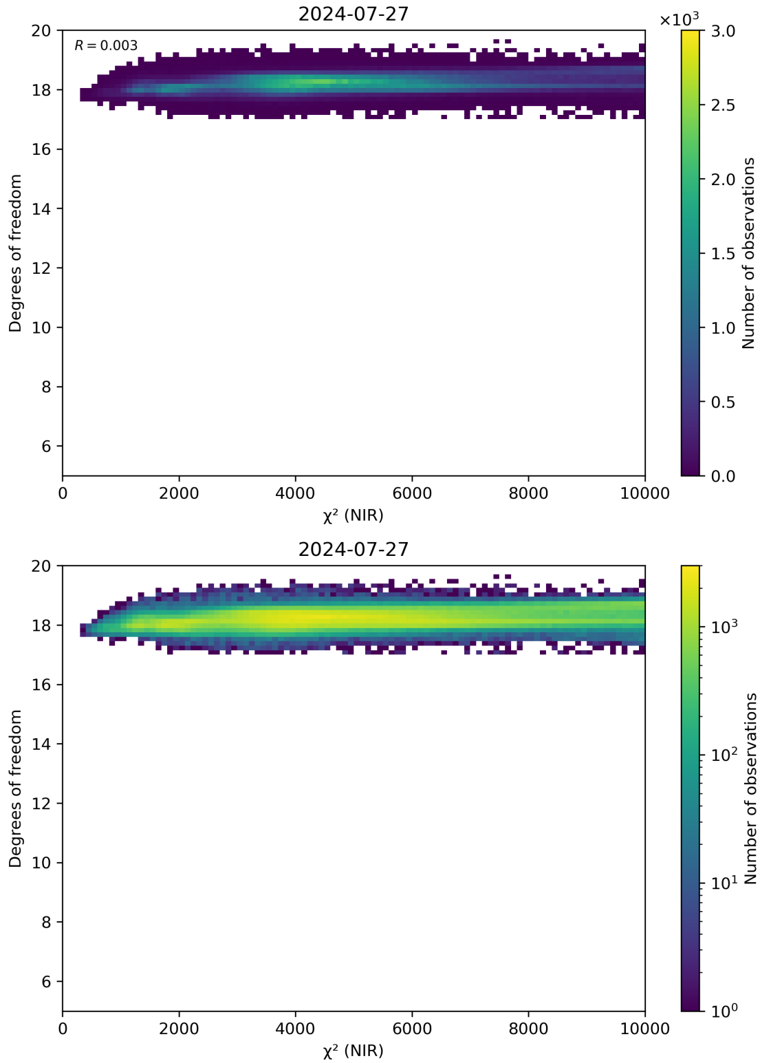
Figure 44: Scatter density plot of “ \chi^2 (NIR)” against “Degrees of freedom” for 2024-07-26 to 2024-07-28.
