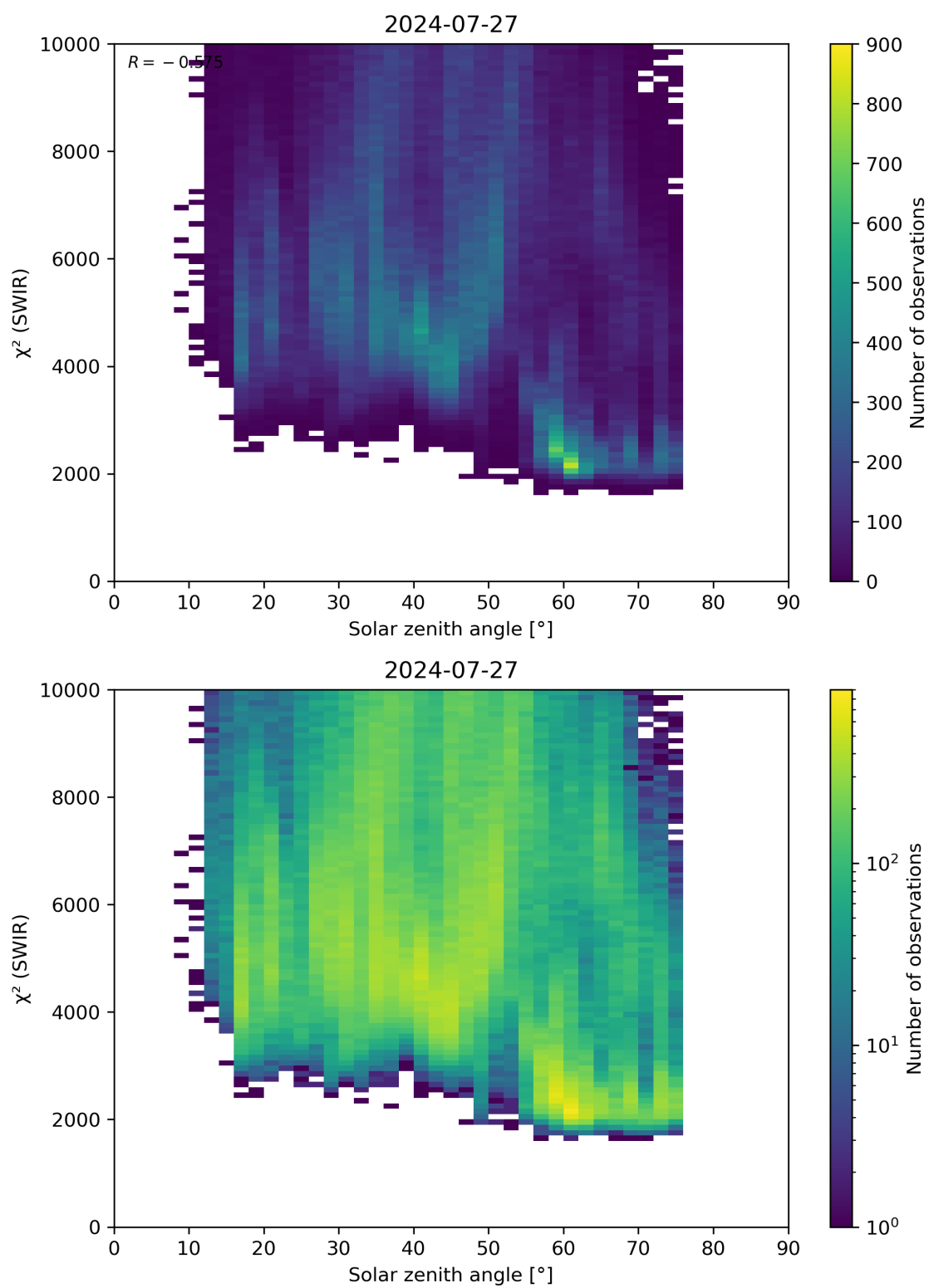
Figure 95: Scatter density plot of “Solar zenith angle” against “ \chi^2 (SWIR)” for 2024-07-26 to 2024-07-28.
