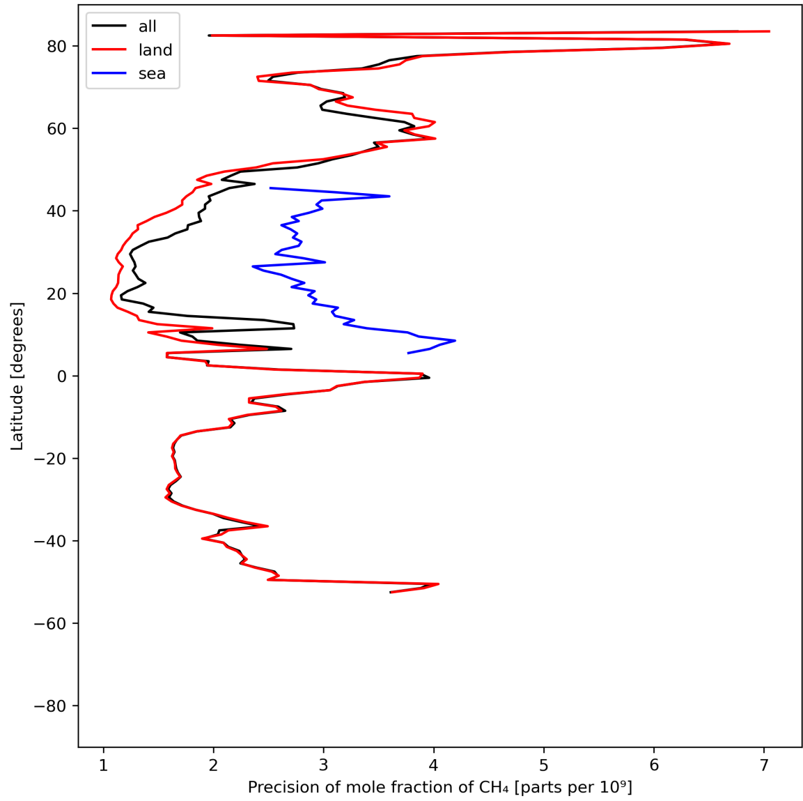
Figure 13: Zonal average of “Precision of mole fraction of CH 4 ” for 2024-07-26 to 2024-07-28.
