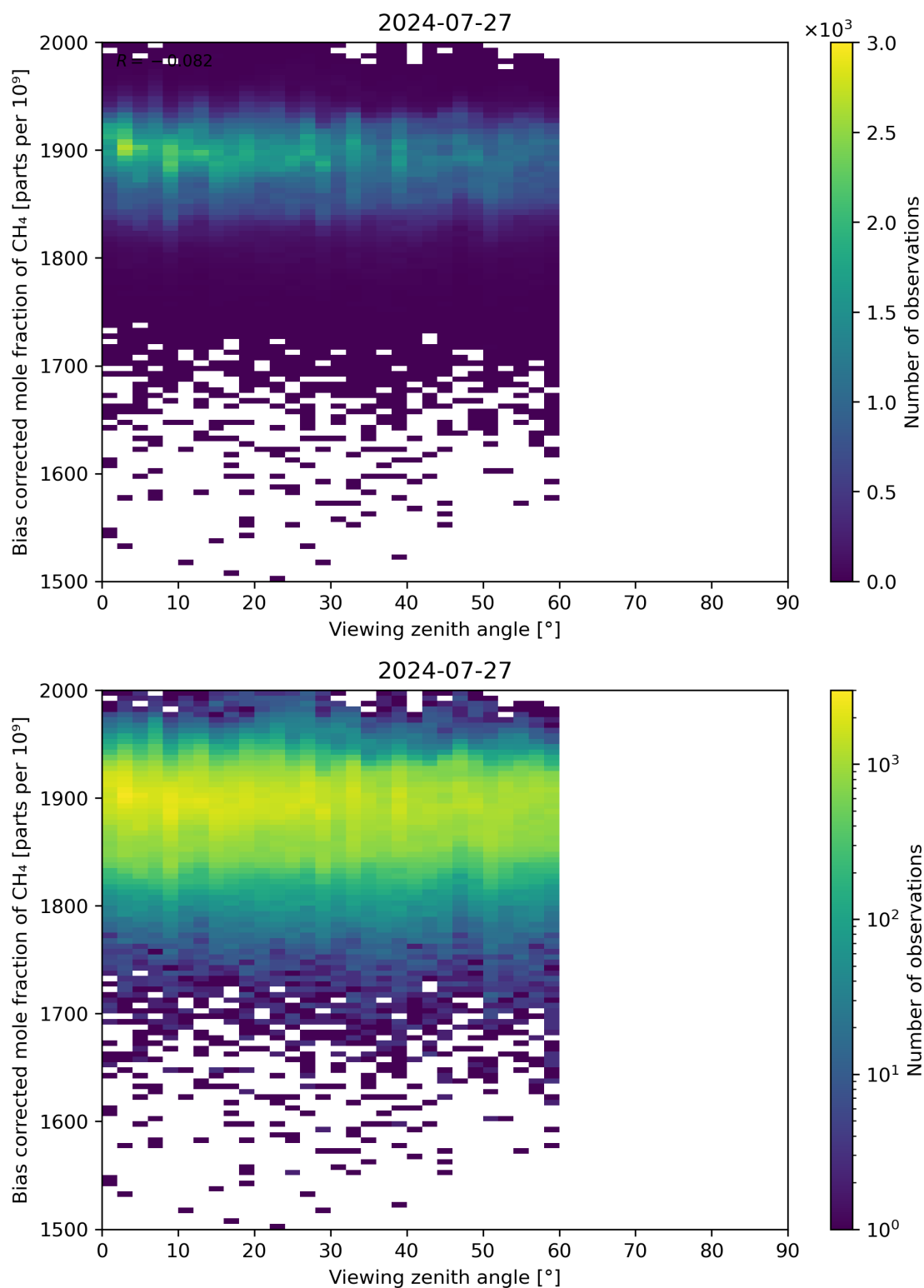
Figure 111: Scatter density plot of “Viewing zenith angle” against “Bias corrected mole fraction of CH 4 ” for 2024-07-26 to 2024-07-28.
