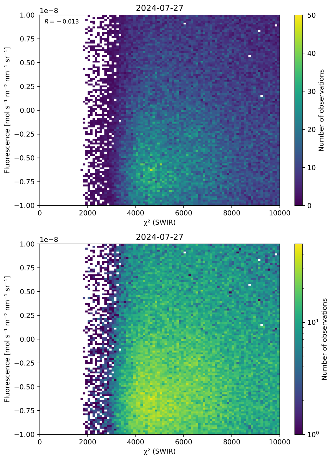
Figure 49: Scatter density plot of “ \chi^2 (SWIR)” against “Fluorescence” for 2024-07-26 to 2024-07-28.
