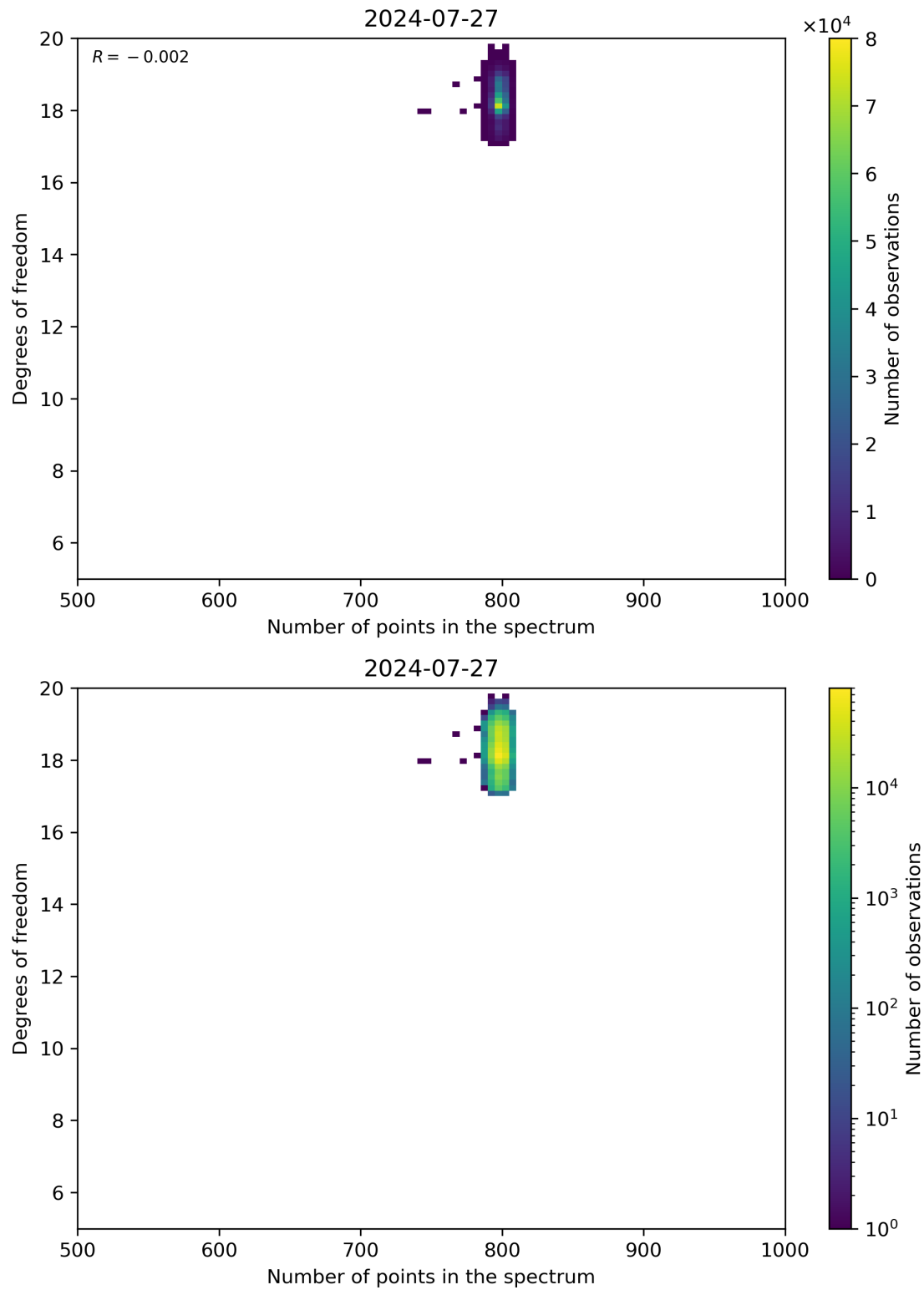
Figure 90: Scatter density plot of “Number of points in the spectrum” against “Degrees of freedom” for 2024-07-26 to 2024-07-28.
