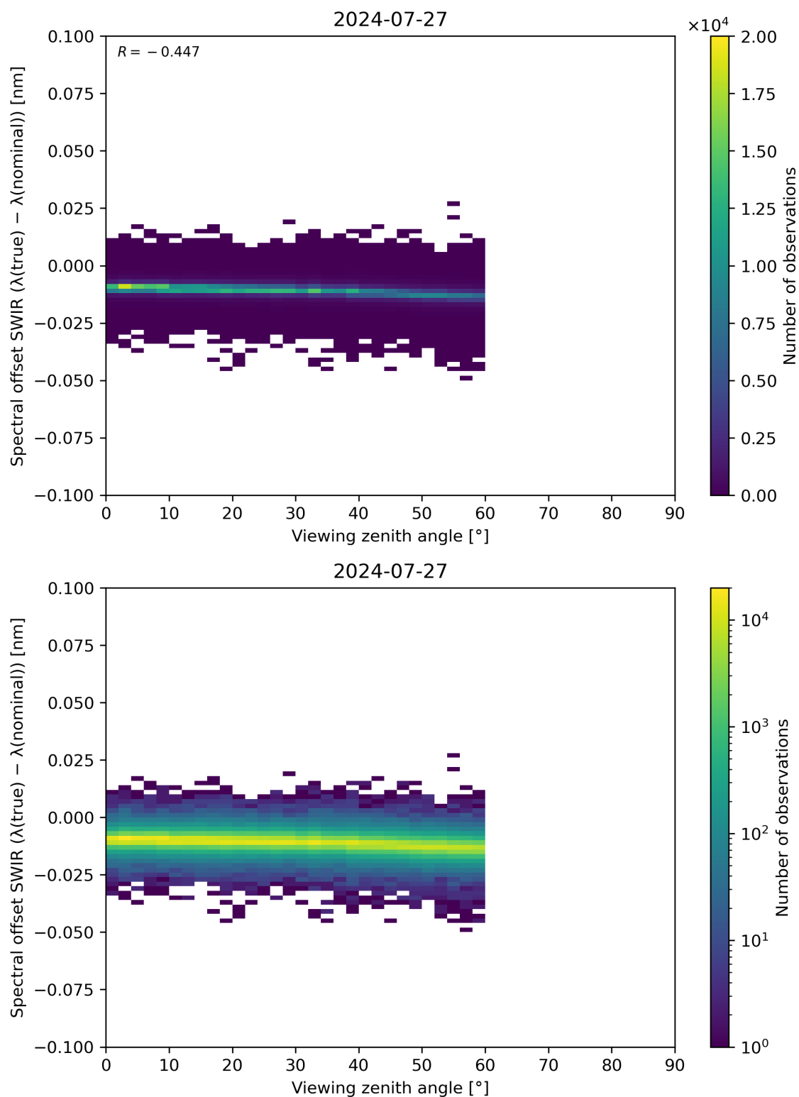
Figure 116: Scatter density plot of “Viewing zenith angle” against “Spectral offset SWIR ( \lambda(\text{true}) - \lambda(\text{nominal}) )” for 2024-07-26 to 2024-07-28.
