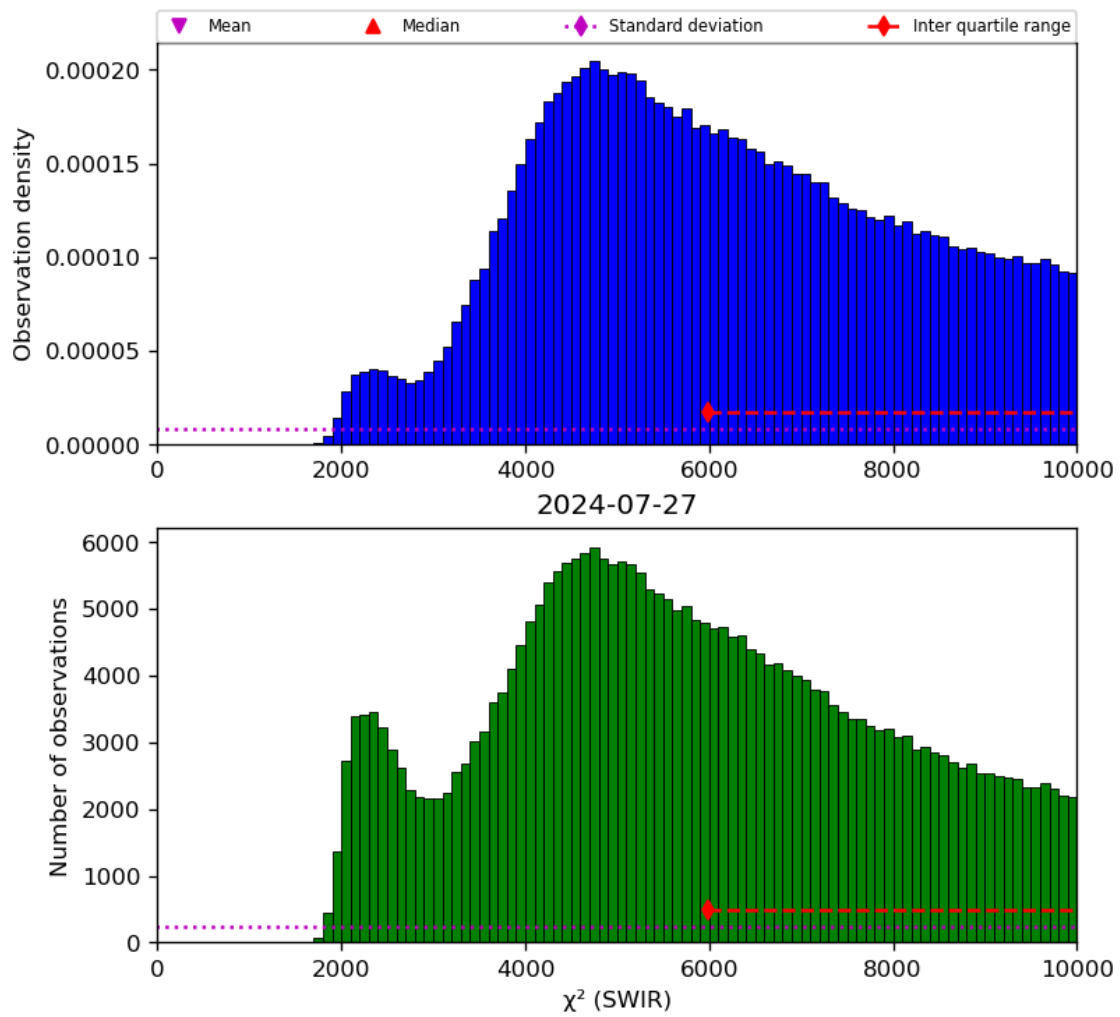
Figure 28: Histogram of “ \chi^2 (SWIR)” for 2024-07-26 to 2024-07-28
