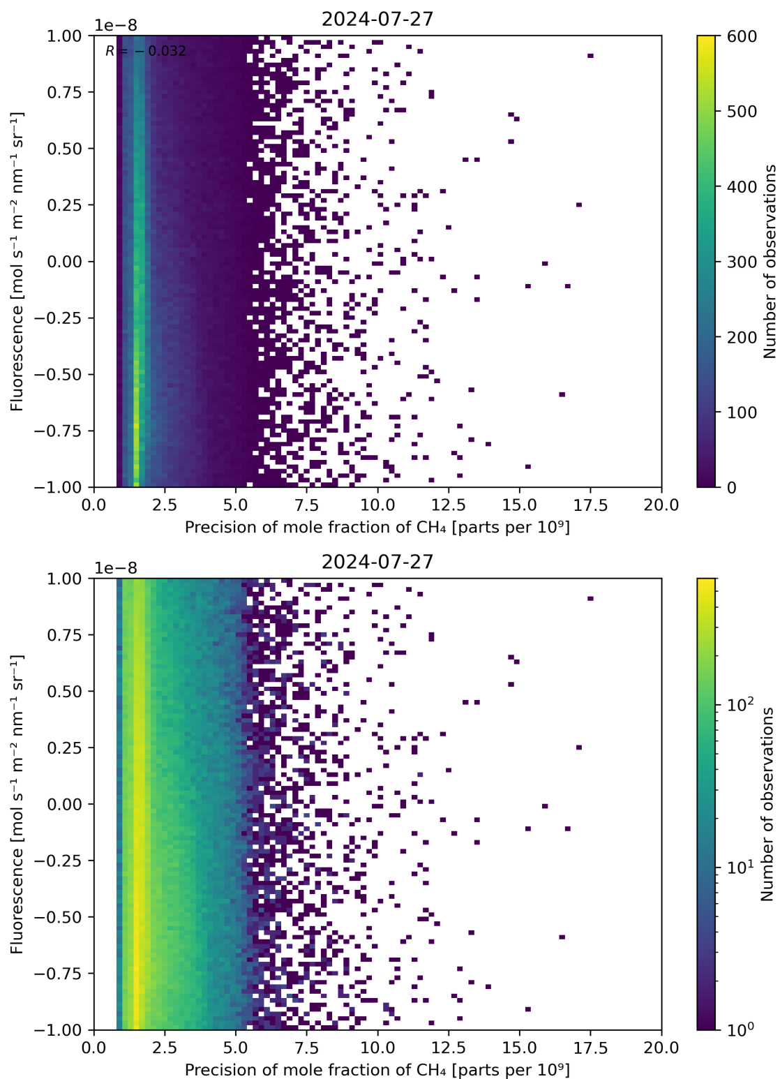
Figure 81: Scatter density plot of “Precision of mole fraction of \text{CH}_4 ” against “Fluorescence” for 2024-07-26 to 2024-07-28.
