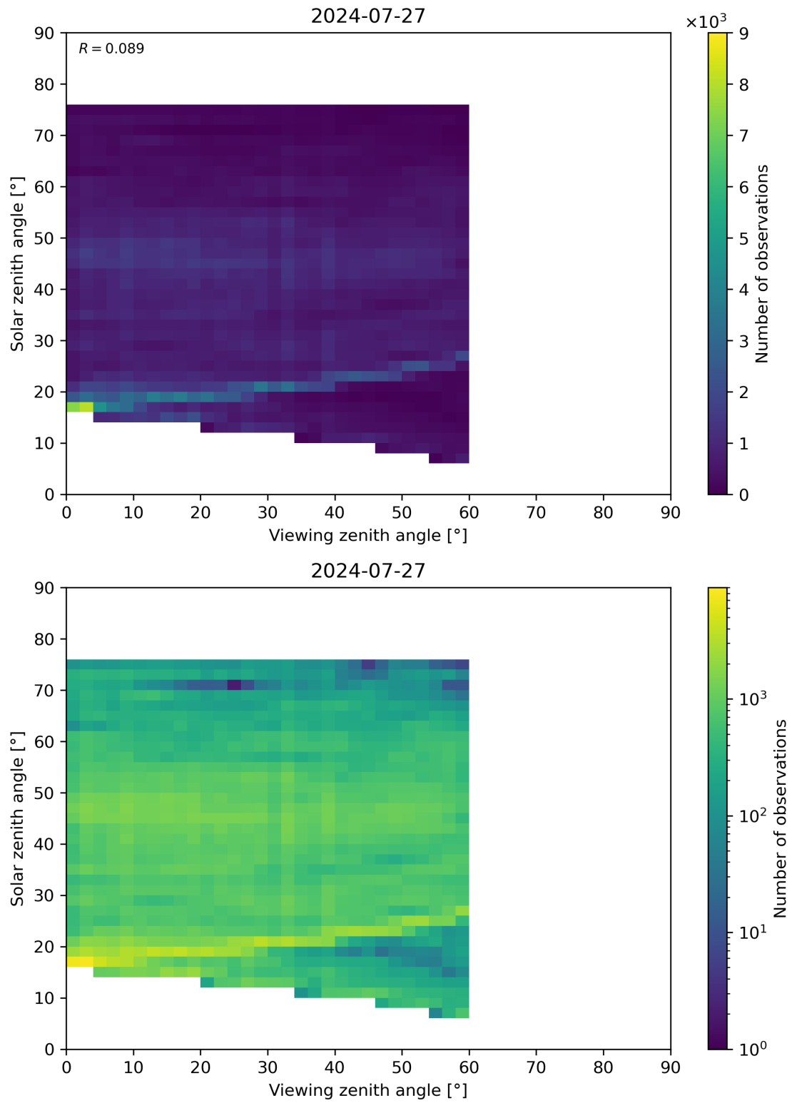
Figure 115: Scatter density plot of “Viewing zenith angle” against “Solar zenith angle” for 2024-07-26 to 2024-07-28.
