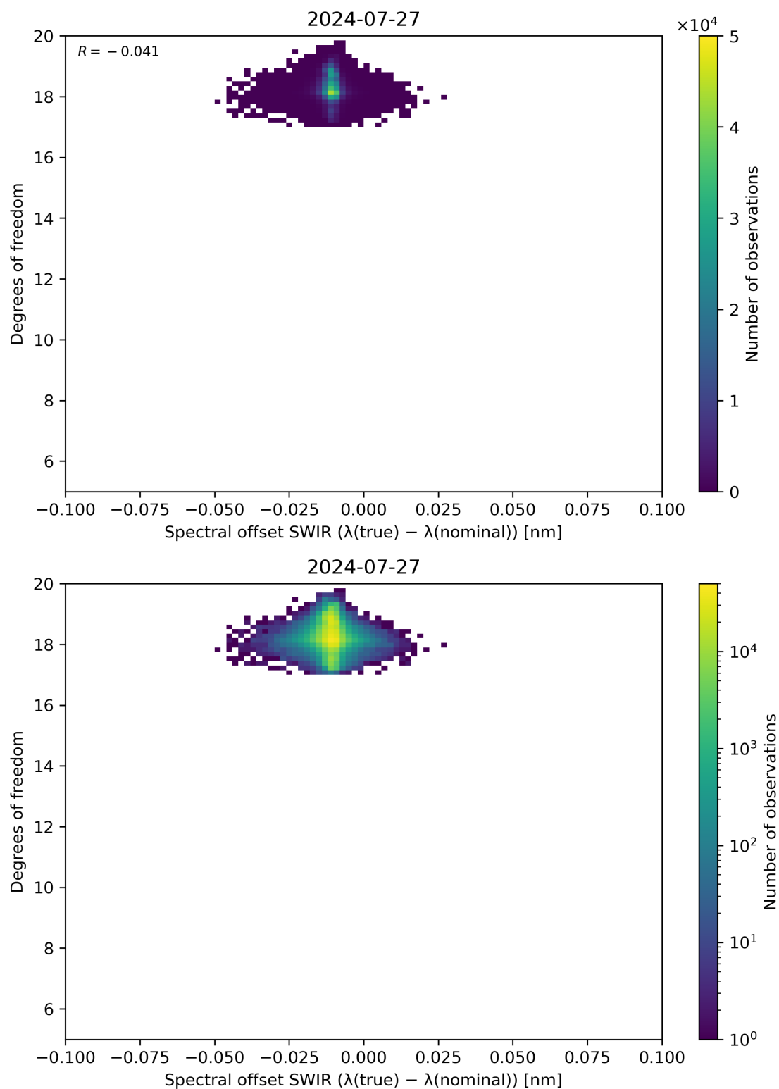
Figure 119: Scatter density plot of “Spectral offset SWIR ( \lambda(\text{true}) - \lambda(\text{nominal}) )” against “Degrees of freedom” for 2024-07-26 to 2024-07-28.
