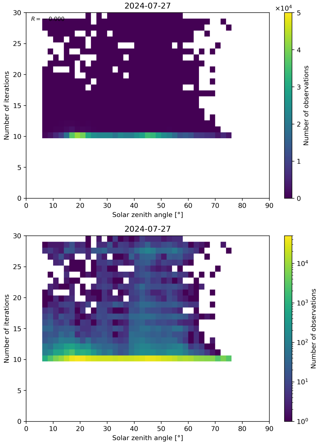
Figure 102: Scatter density plot of “Solar zenith angle” against “Number of iterations” for 2024-07-26 to 2024-07-28.
