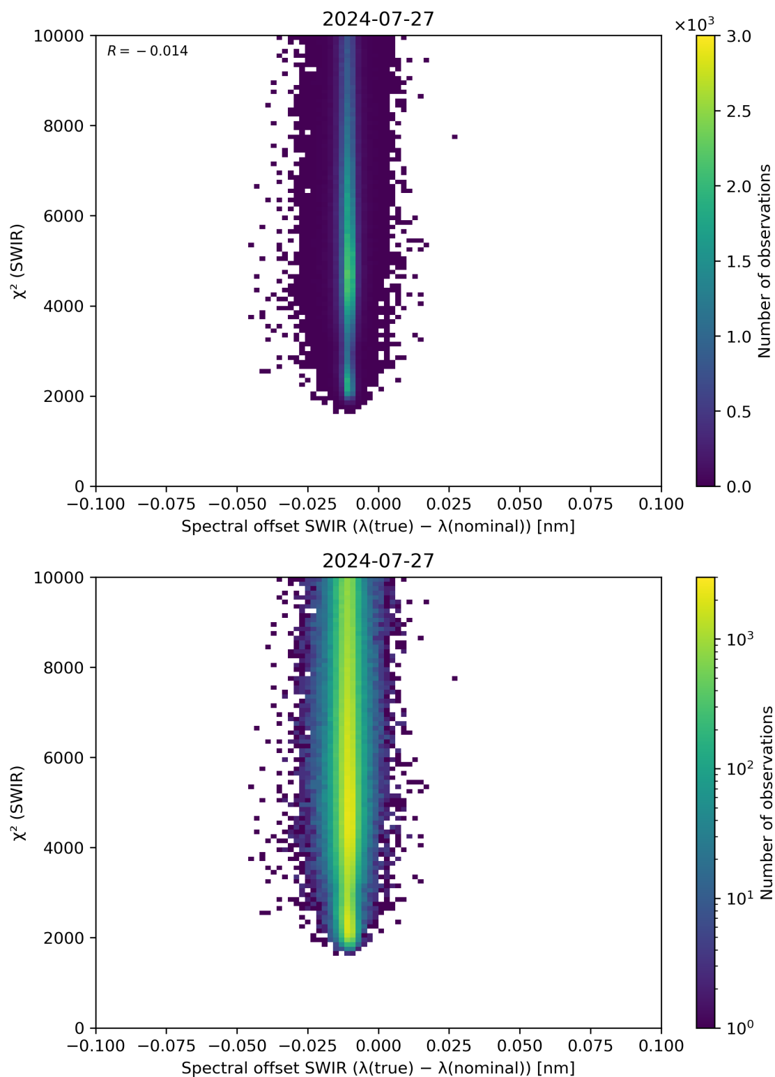
Figure 118: Scatter density plot of “Spectral offset SWIR ( \lambda(\text{true}) - \lambda(\text{nominal}) )” against “ \chi^2 (SWIR)” for 2024-07-26 to 2024-07-28.
