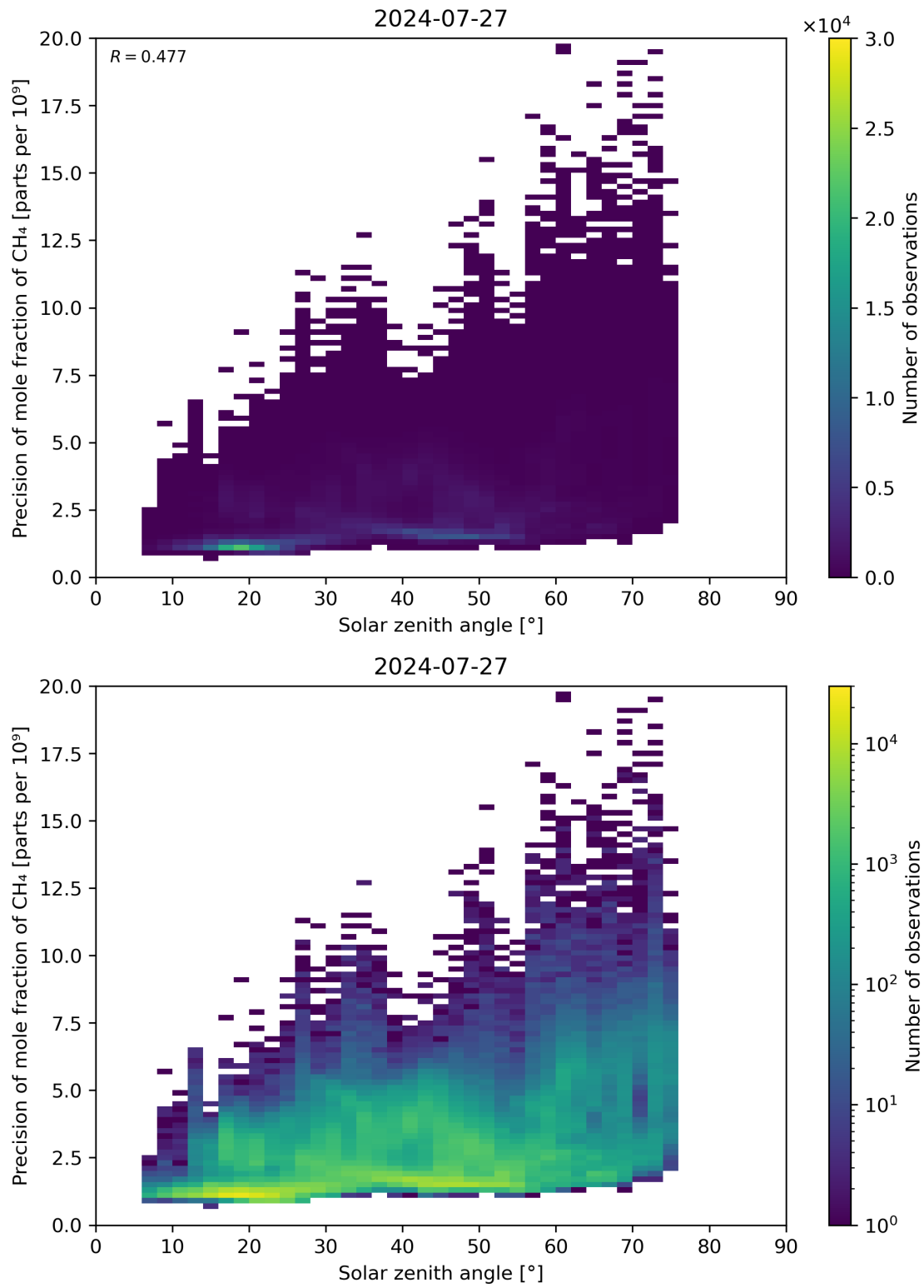
Figure 101: Scatter density plot of “Solar zenith angle” against “Precision of mole fraction of \text{CH}_4 ” for 2024-07-26 to 2024-07-28.
