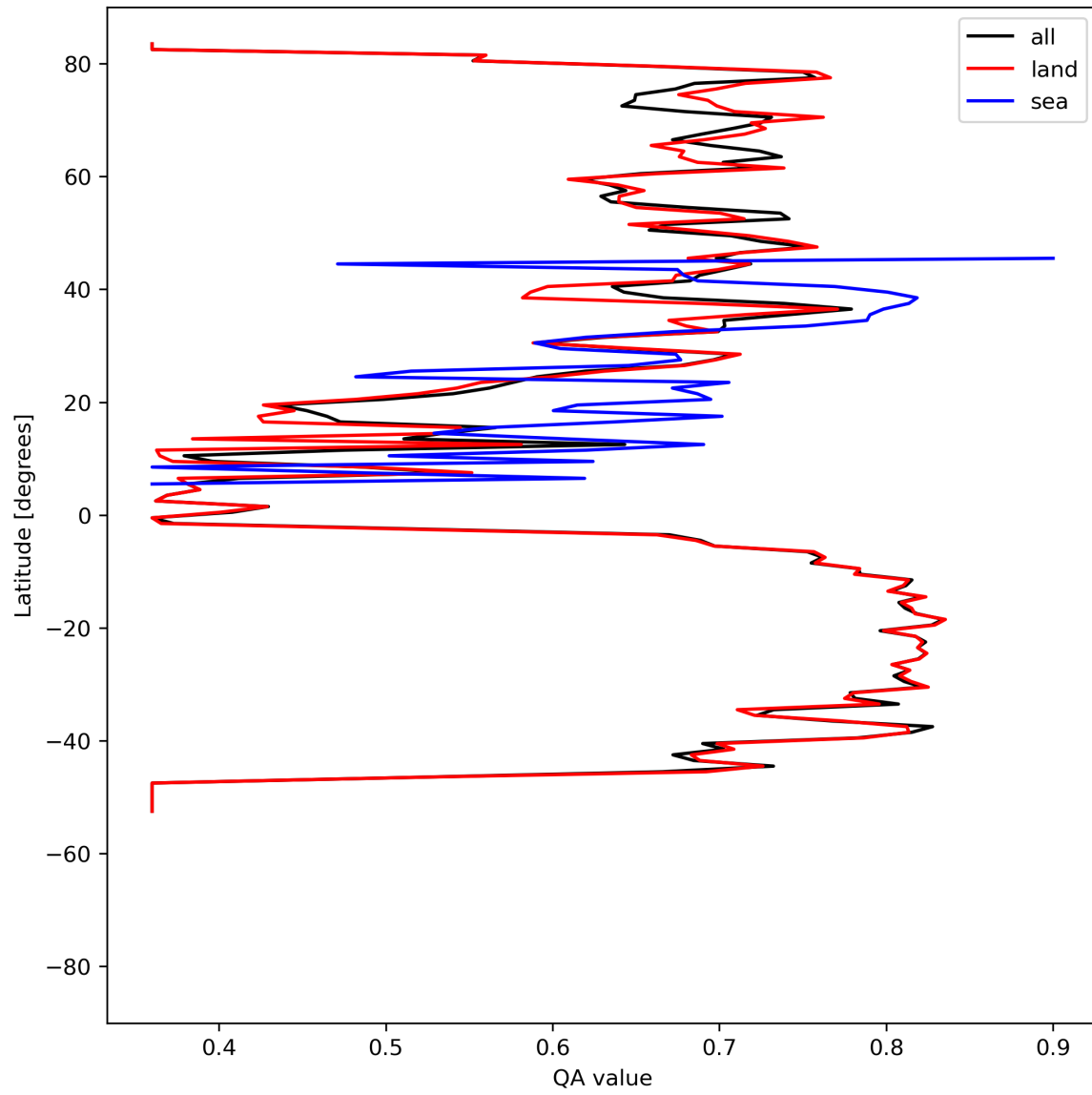
Figure 11: Zonal average of “QA value” for 2024-07-26 to 2024-07-28.
