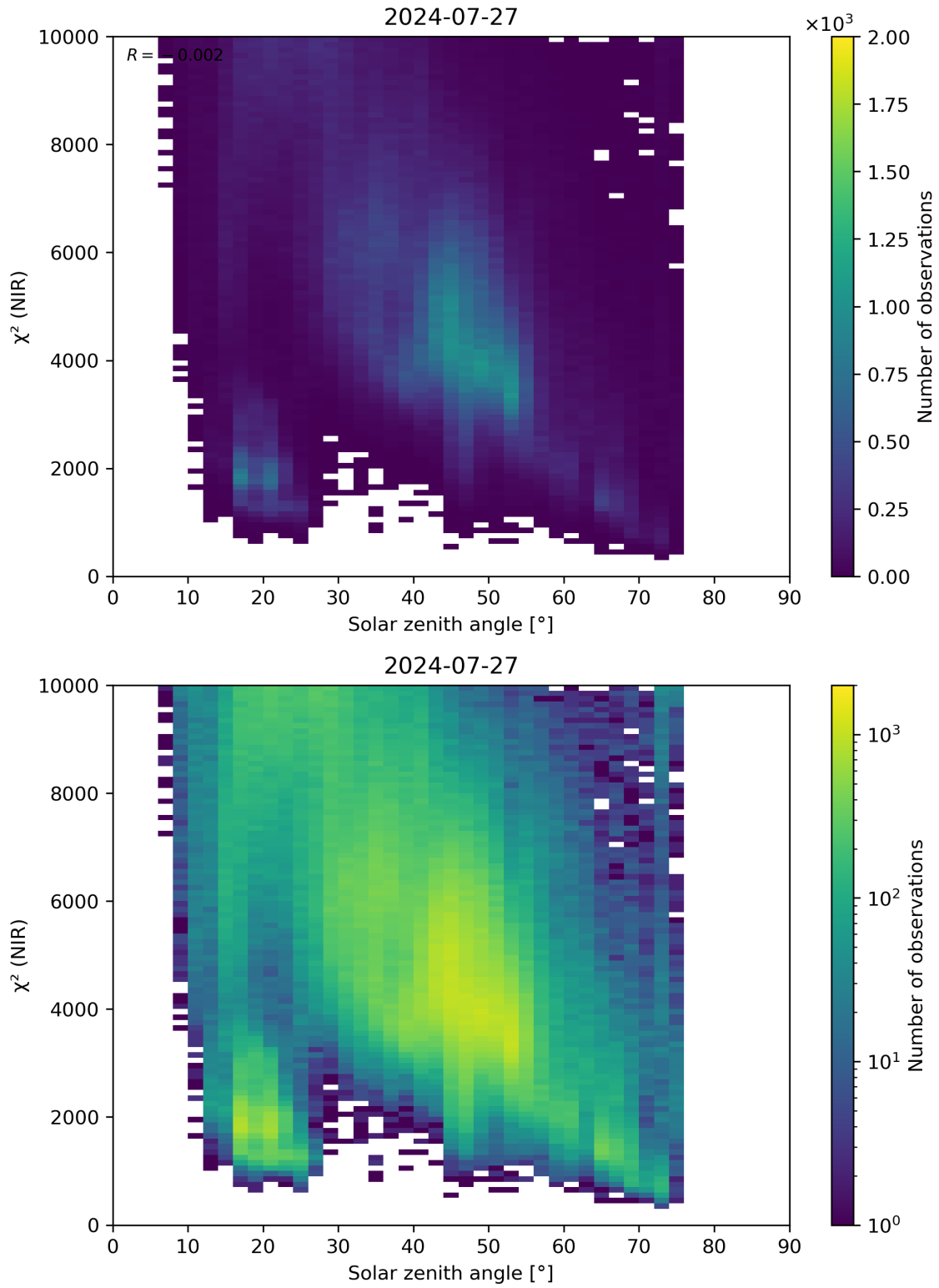
Figure 94: Scatter density plot of “Solar zenith angle” against “ \chi^2 (NIR)” for 2024-07-26 to 2024-07-28.
