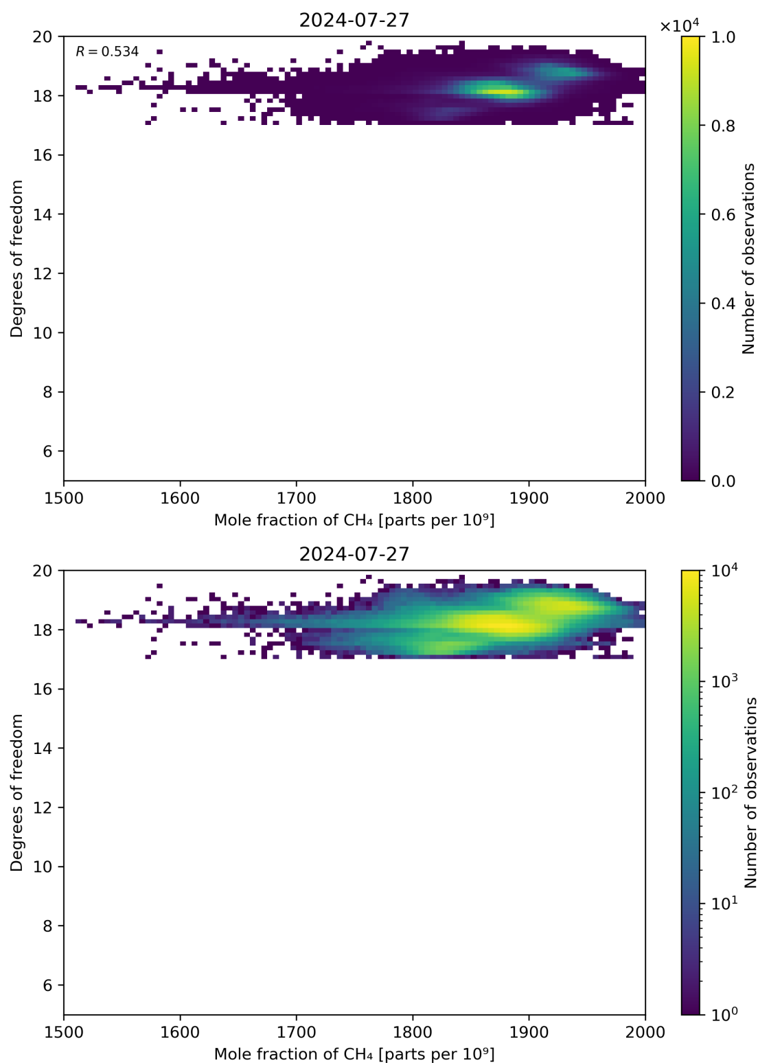
Figure 72: Scatter density plot of “Mole fraction of CH 4 ” against “Degrees of freedom” for 2024-07-26 to 2024-07-28.
