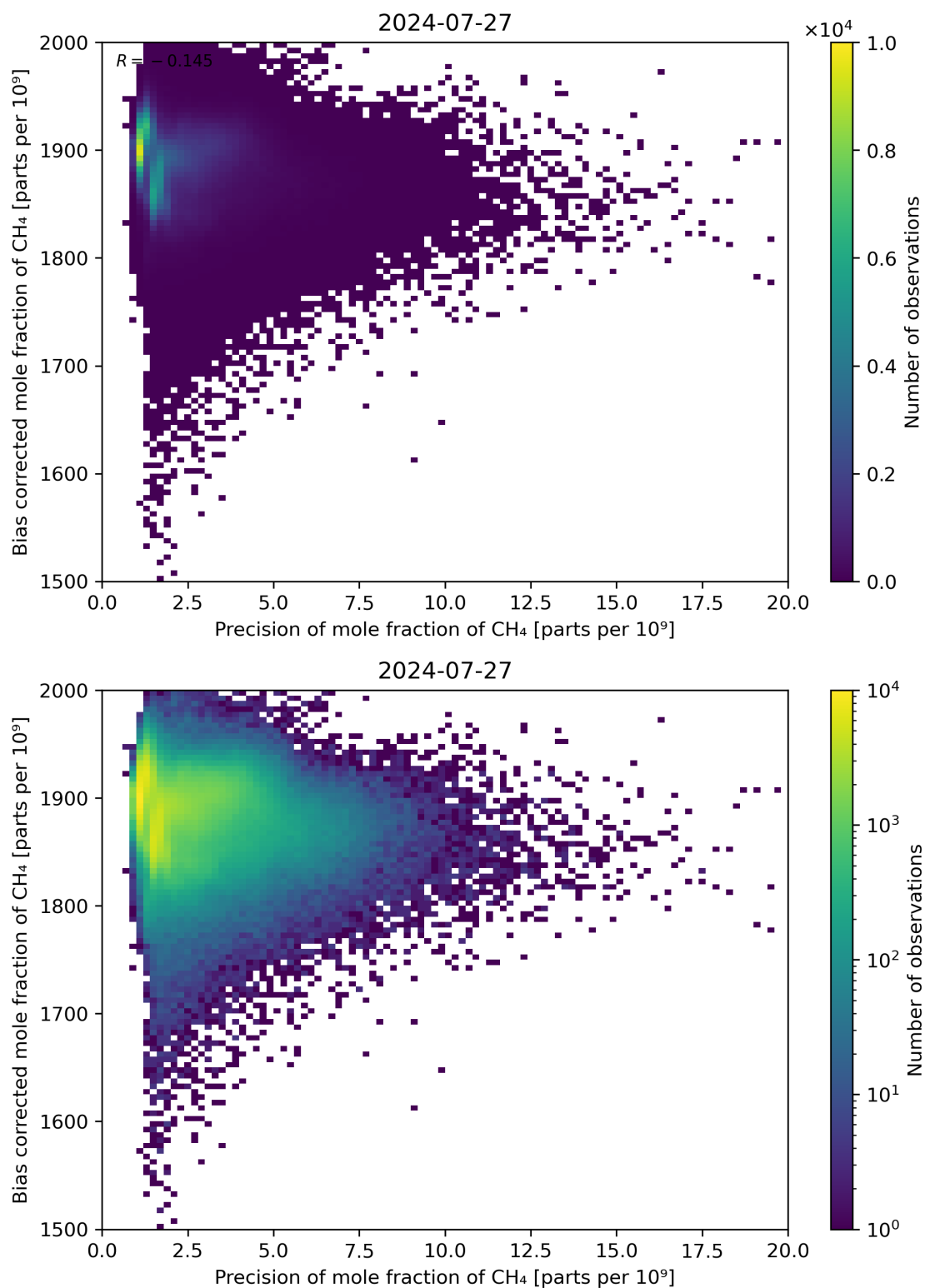
Figure 82: Scatter density plot of “Precision of mole fraction of CH 4 ” against “Bias corrected mole fraction of CH 4 ” for 2024-07-26 to 2024-07-28.
