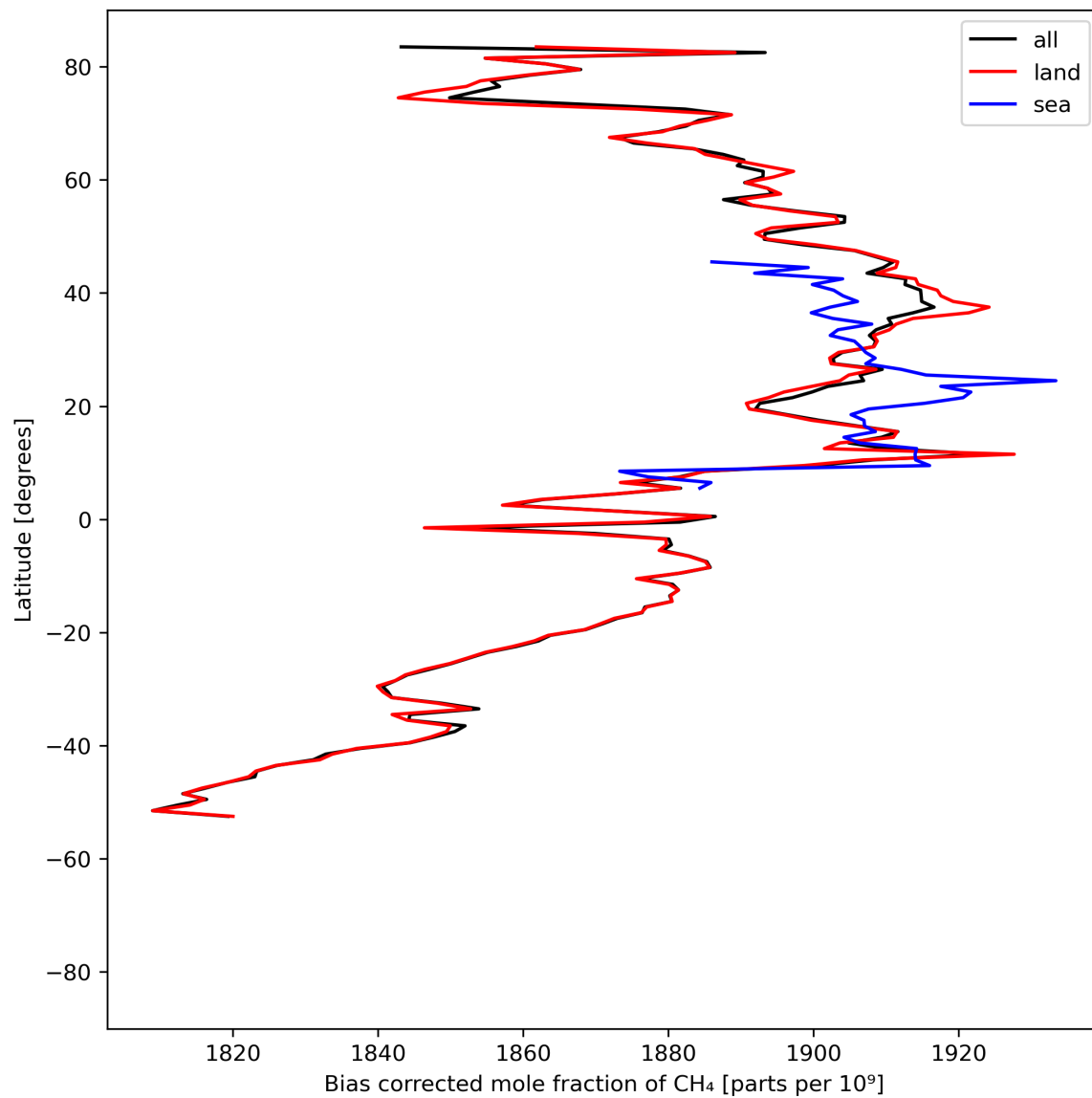
Figure 14: Zonal average of “Bias corrected mole fraction of CH 4 ” for 2024-07-26 to 2024-07-28.
