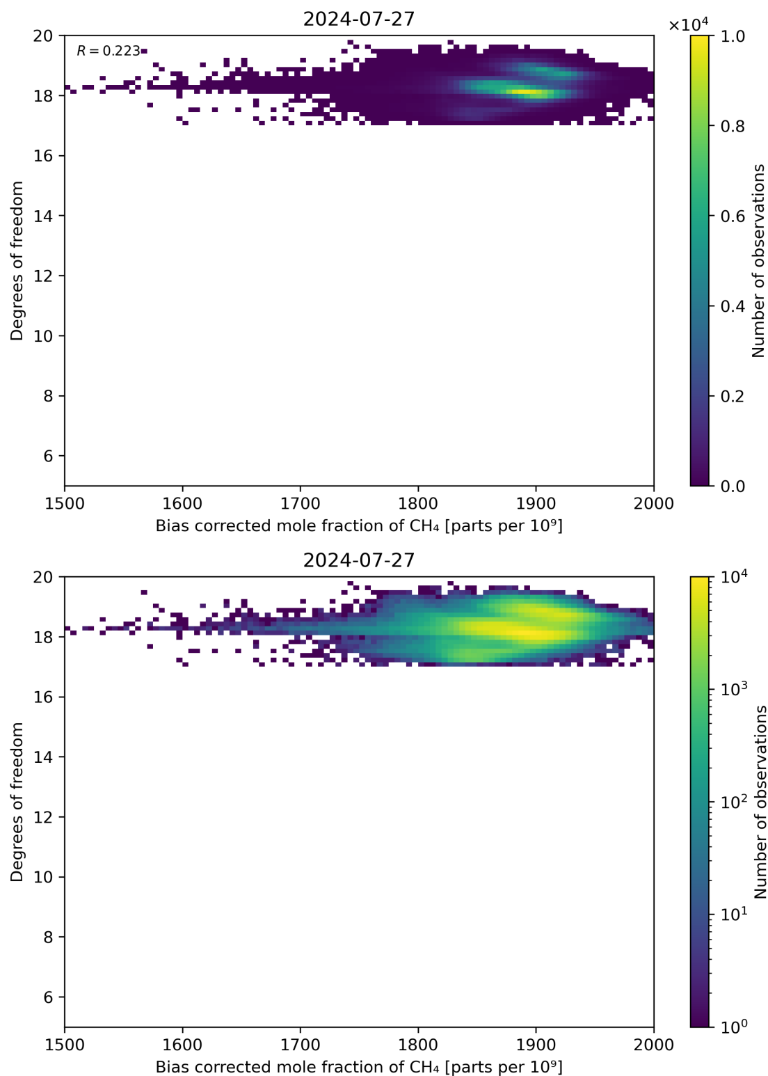
Figure 65: Scatter density plot of “Bias corrected mole fraction of CH 4 ” against “Degrees of freedom” for 2024-07-26 to 2024-07-28.
