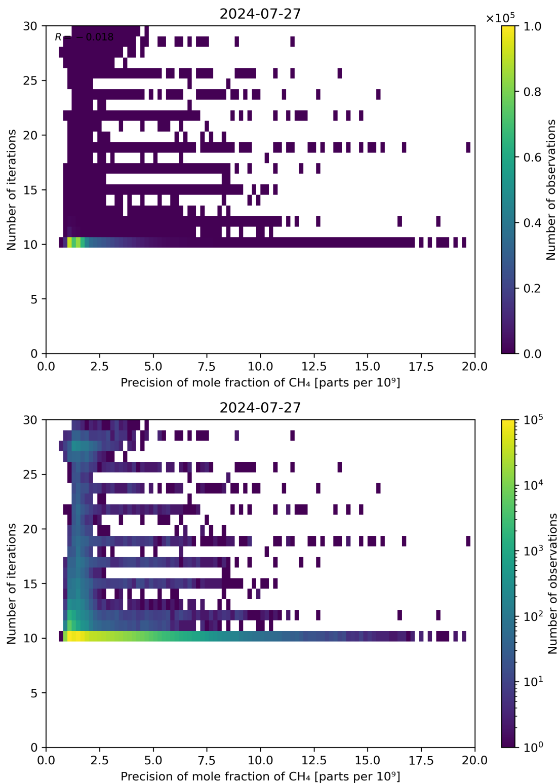
Figure 83: Scatter density plot of “Precision of mole fraction of CH 4 ” against “Number of iterations” for 2024-07-26 to 2024-07-28.
