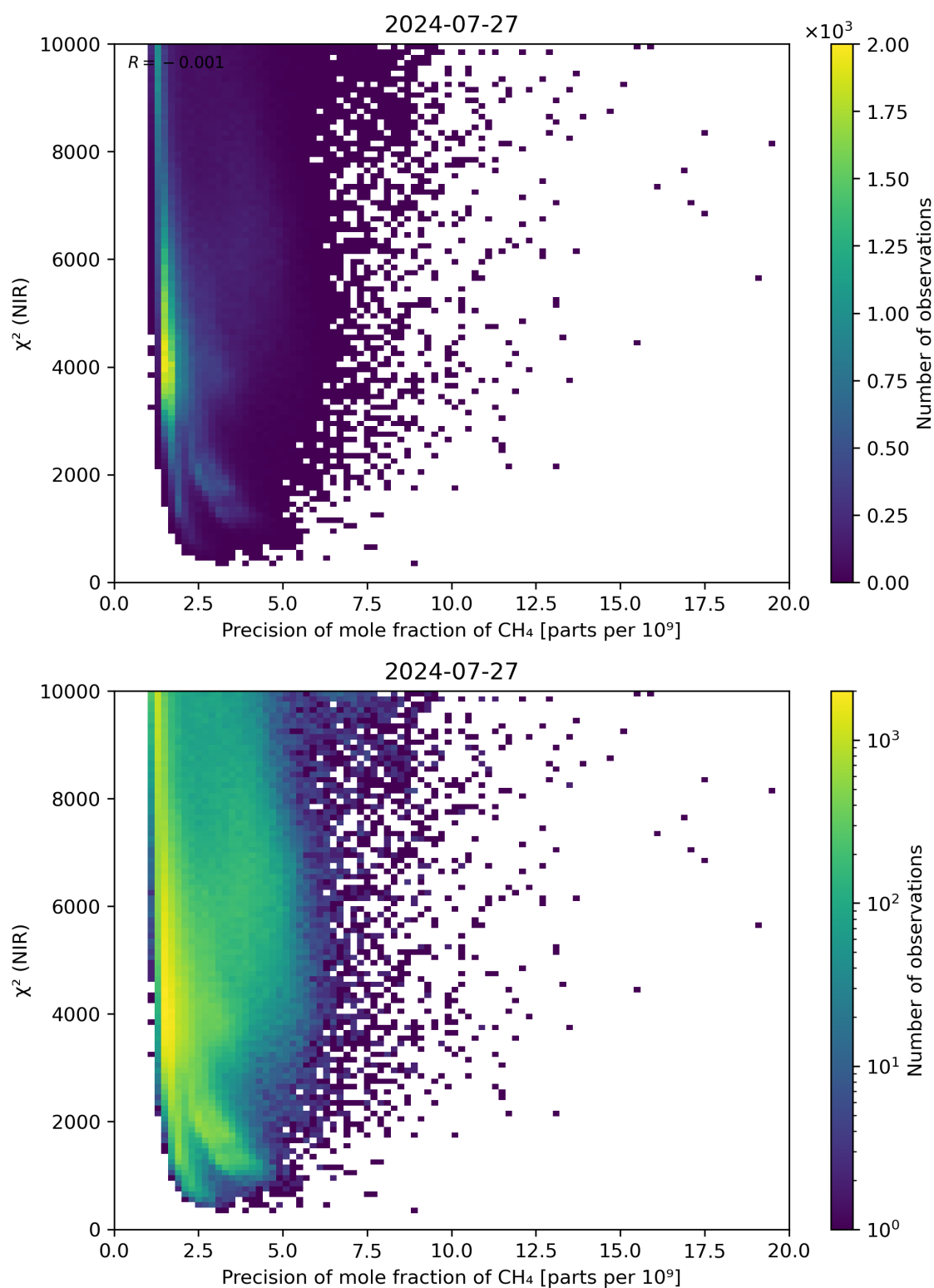
Figure 78: Scatter density plot of “Precision of mole fraction of CH 4 ” against “ \chi^2 (NIR)” for 2024-07-26 to 2024-07-28.
