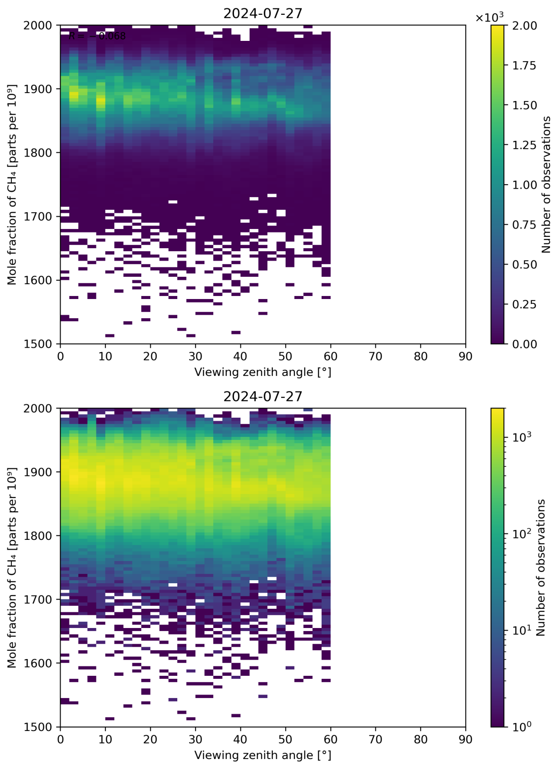
Figure 110: Scatter density plot of “Viewing zenith angle” against “Mole fraction of CH 4 ” for 2024-07-26 to 2024-07-28.
