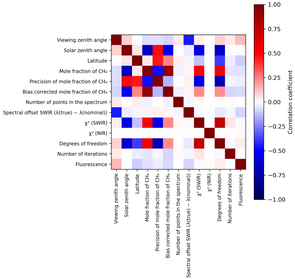
Figure 2: Map of correlation matrix for 2024-07-26 to 2024-07-28.
