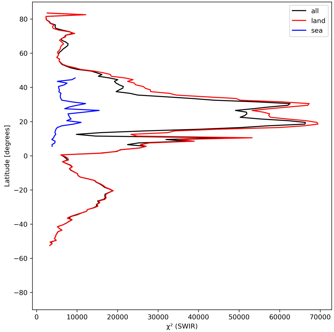
Figure 17: Zonal average of “ \chi^2 (SWIR)” for 2024-07-26 to 2024-07-28.
