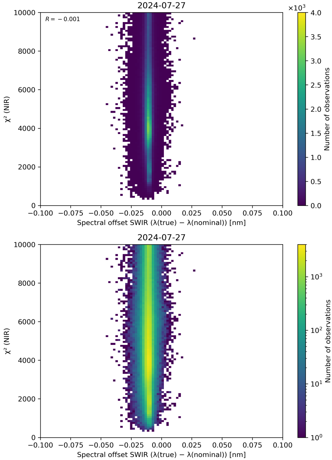
Figure 117: Scatter density plot of “Spectral offset SWIR ( \lambda(\text{true}) - \lambda(\text{nominal}) )” against “ \chi^2 (NIR)” for 2024-07-26 to 2024-07-28.
