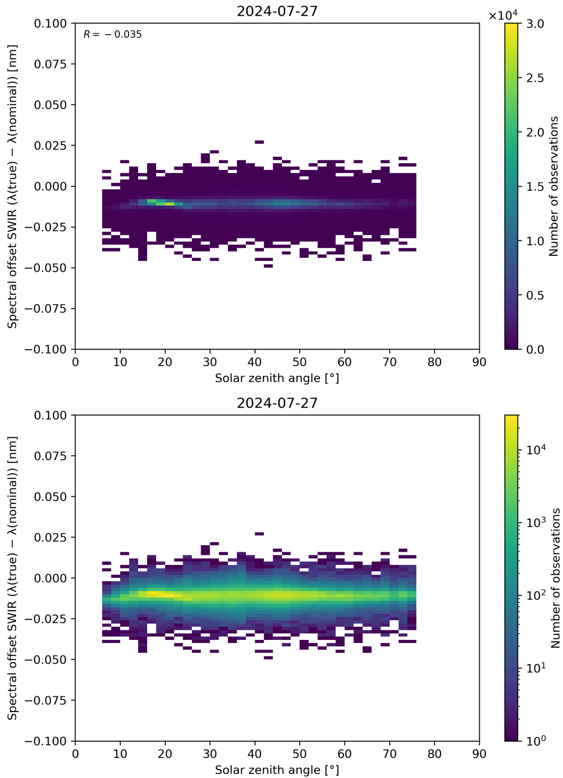
Figure 104: Scatter density plot of “Solar zenith angle” against “Spectral offset SWIR ( \lambda(\text{true}) - \lambda(\text{nominal}) )” for 2024-07-26 to 2024-07-28.
