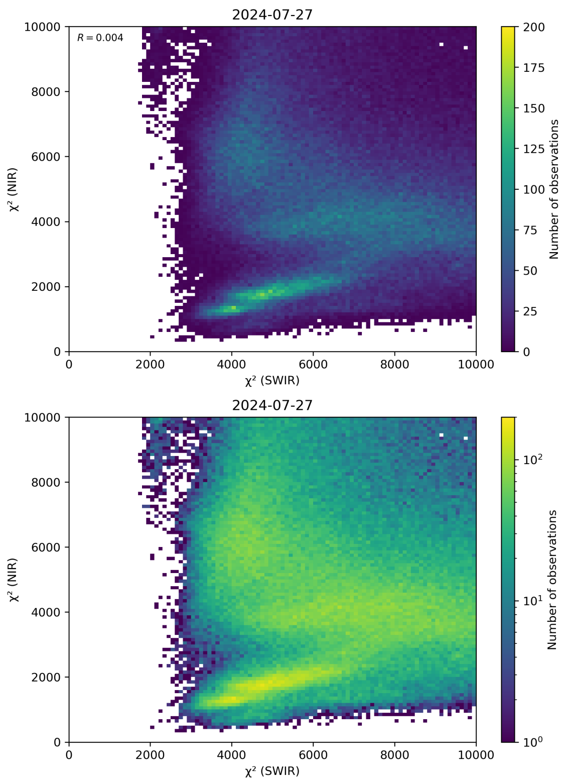
Figure 47: Scatter density plot of “ \chi^2 (SWIR)” against “ \chi^2 (NIR)” for 2024-07-26 to 2024-07-28.
