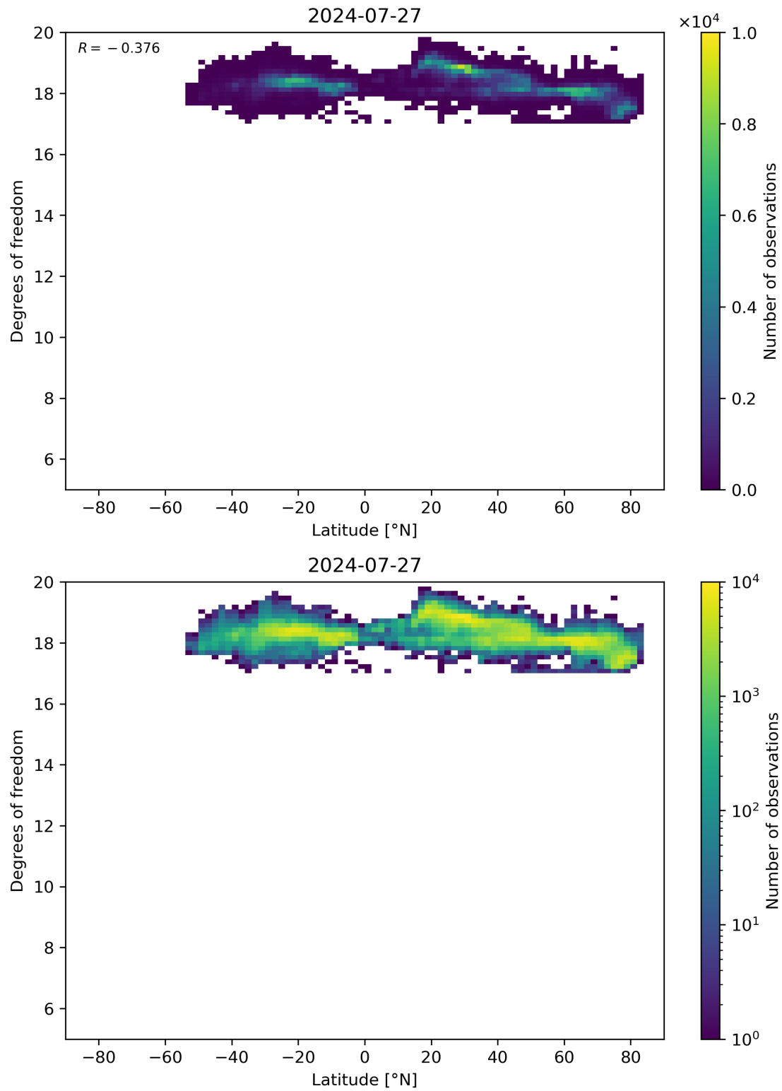
Figure 55: Scatter density plot of “Latitude” against “Degrees of freedom” for 2024-07-26 to 2024-07-28.
