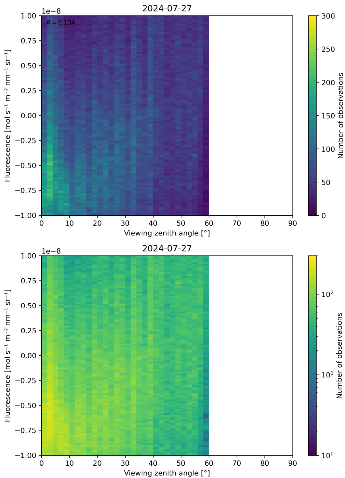
Figure 108: Scatter density plot of “Viewing zenith angle” against “Fluorescence” for 2024-07-26 to 2024-07-28.
