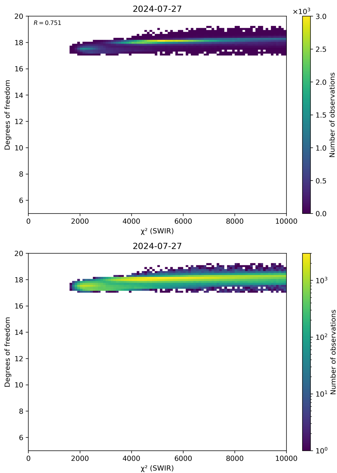
Figure 48: Scatter density plot of “ \chi^2 (SWIR)” against “Degrees of freedom” for 2024-07-26 to 2024-07-28.
