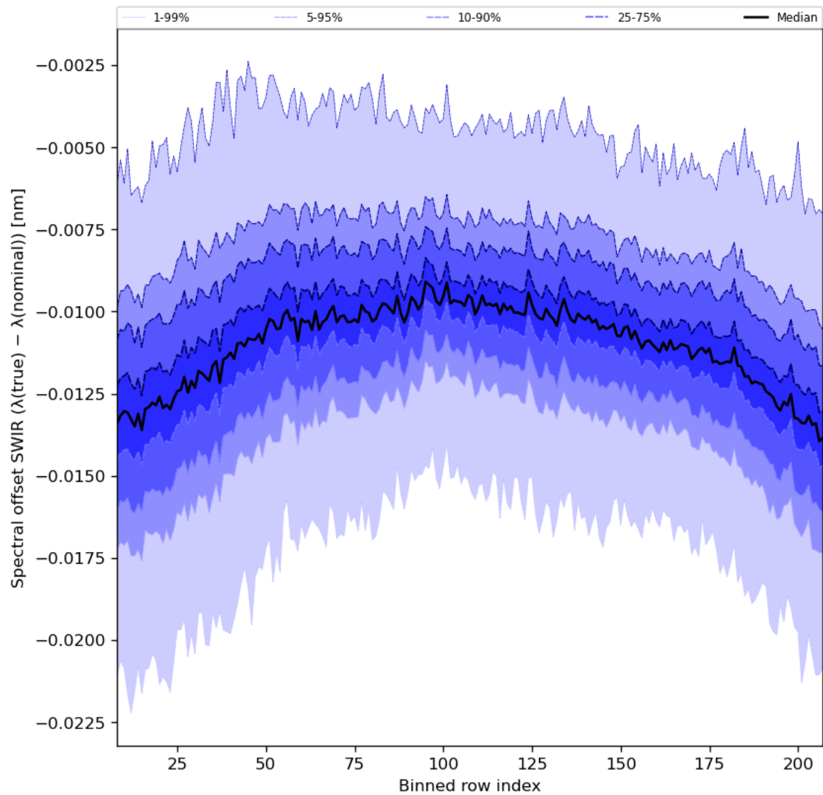
Figure 38: Along track statistics of “Spectral offset SWIR ( \lambda(\text{true}) - \lambda(\text{nominal}) )” for 2024-07-26 to 2024-07-28
