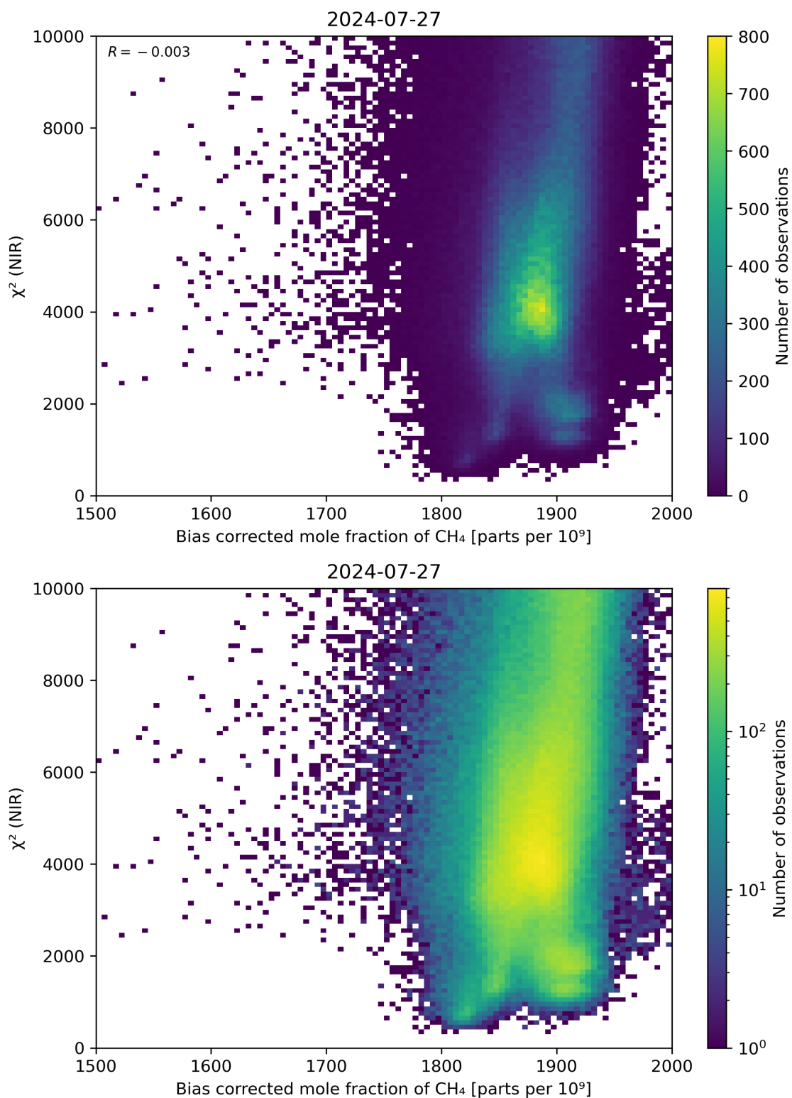
Figure 63: Scatter density plot of “Bias corrected mole fraction of CH 4 ” against “ \chi^2 (NIR)” for 2024-07-26 to 2024-07-28.
