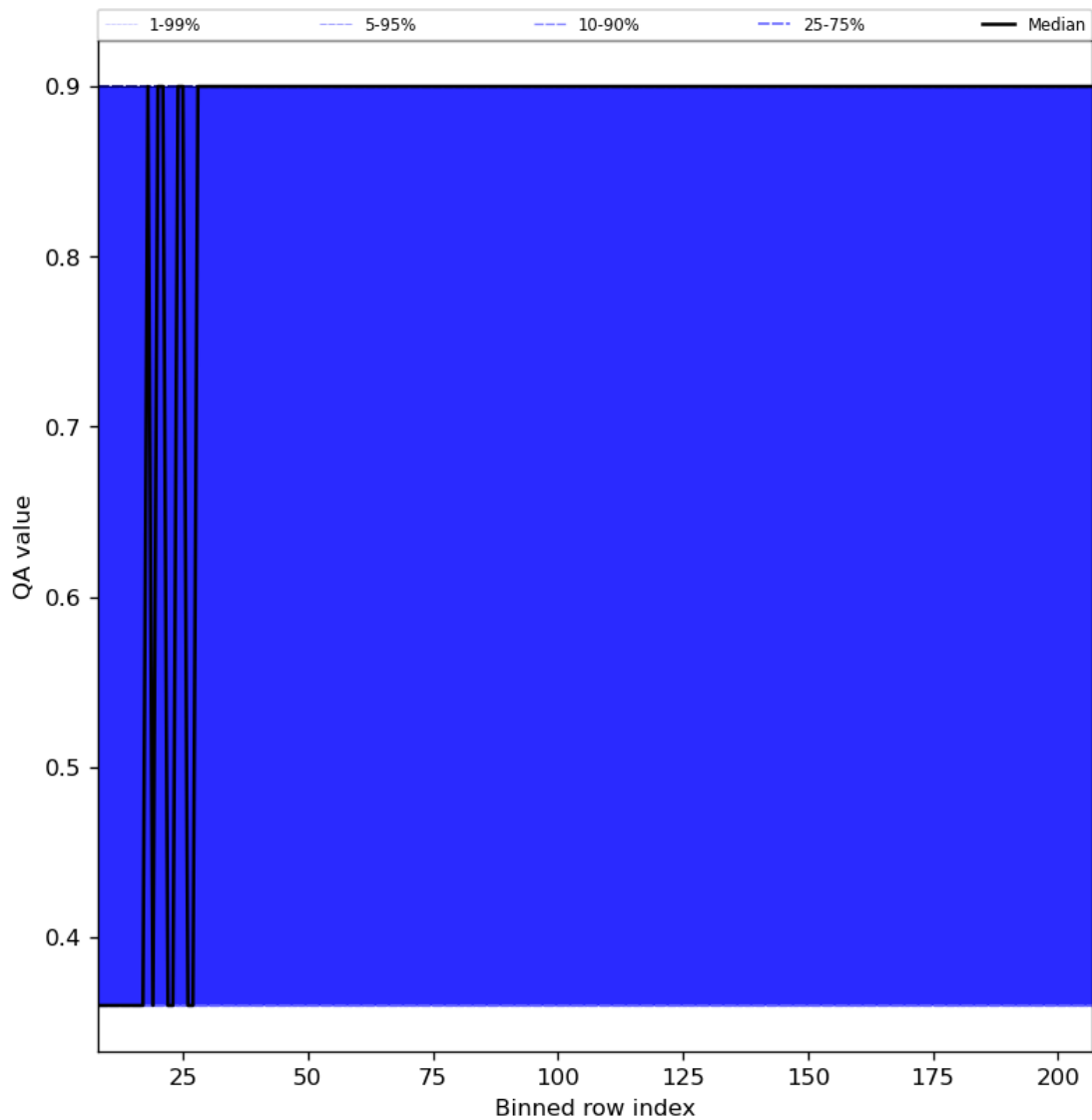
Figure 33: Along track statistics of “QA value” for 2024-07-26 to 2024-07-28
