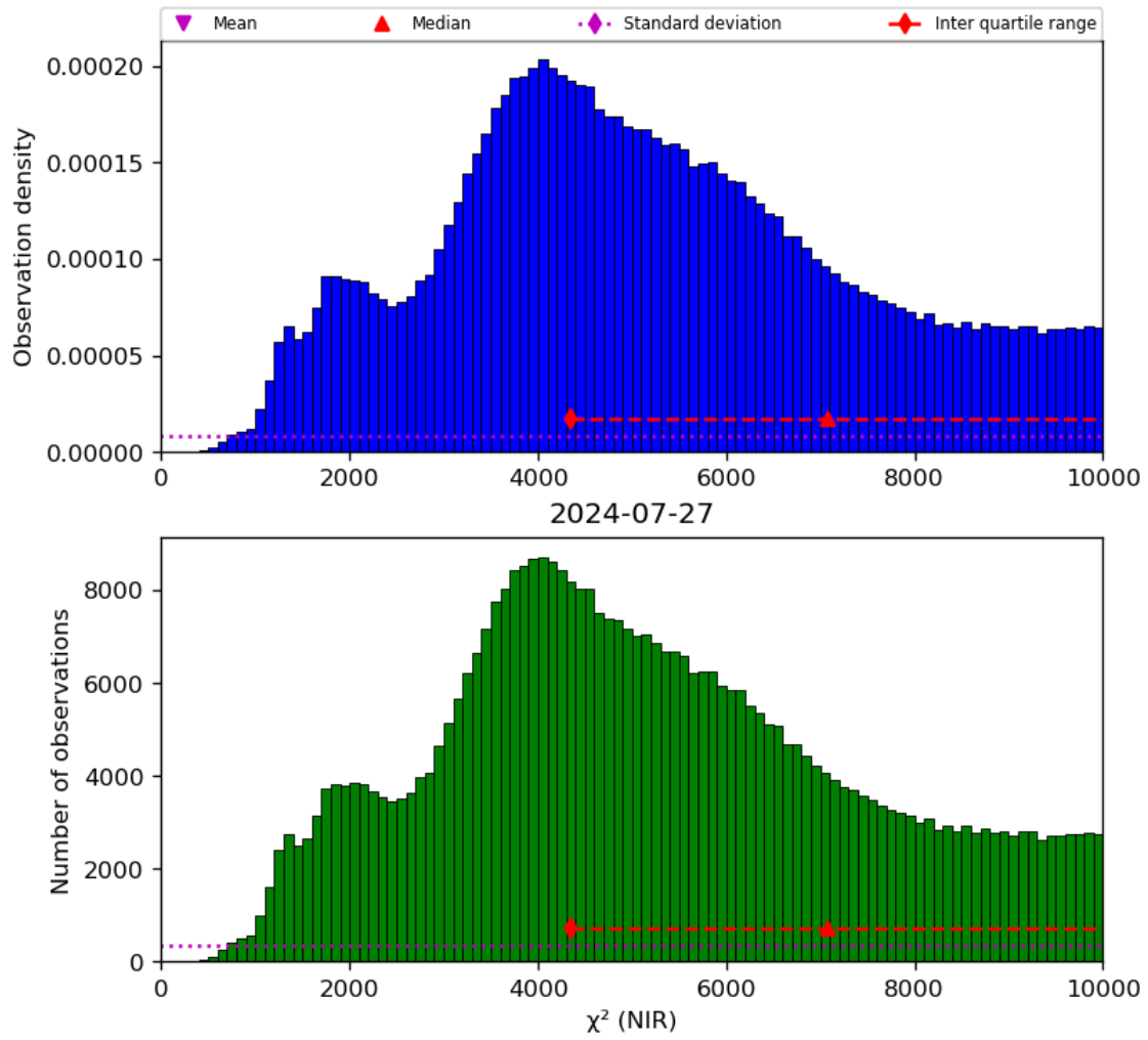
Figure 29: Histogram of “ \chi^2 (NIR)” for 2024-07-26 to 2024-07-28
