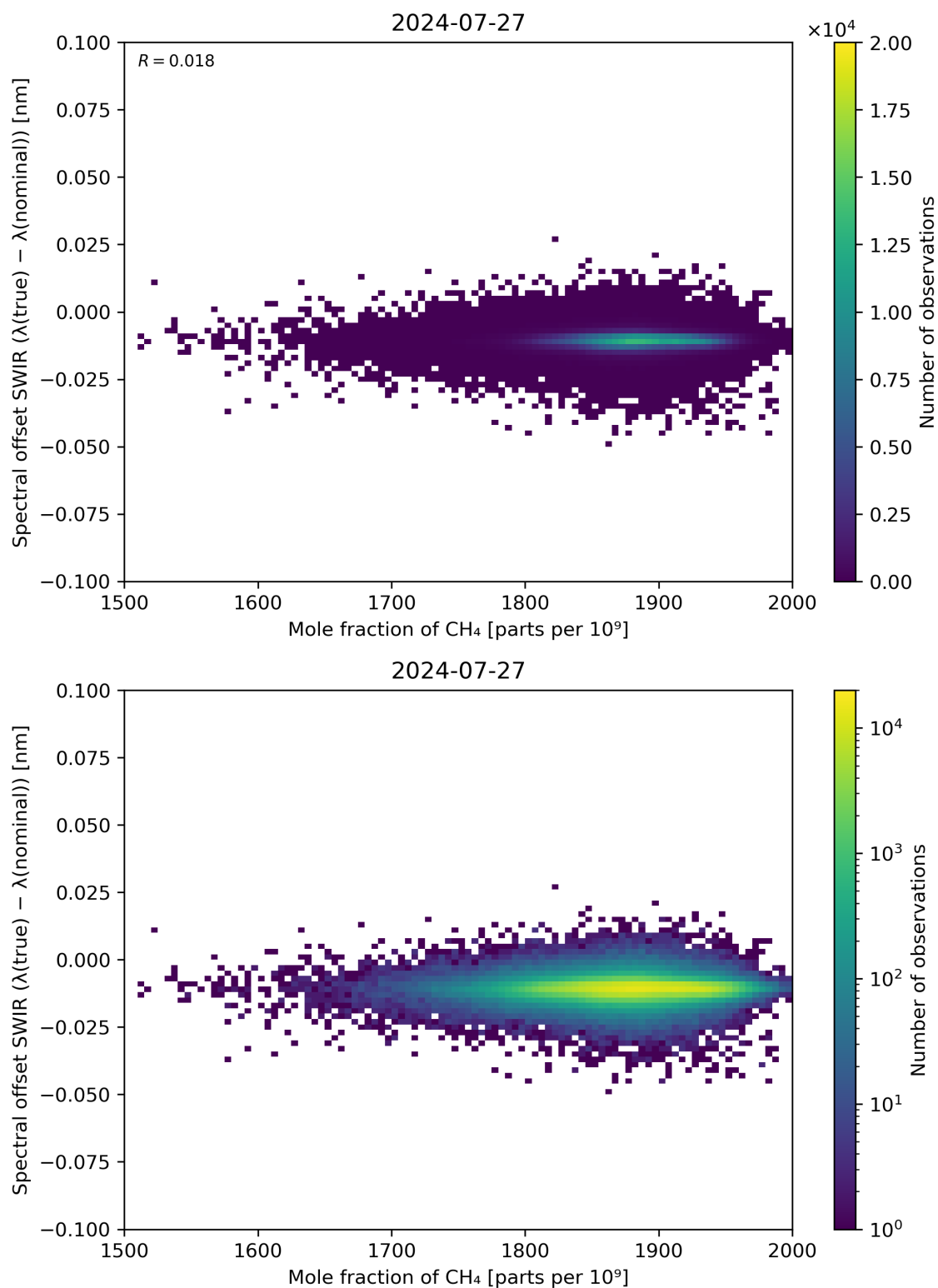
Figure 86: Scatter density plot of “Mole fraction of CH 4 ” against “Spectral offset SWIR ( \lambda(\text{true}) - \lambda(\text{nominal}) )” for 2024-07-26 to 2024-07-28.
