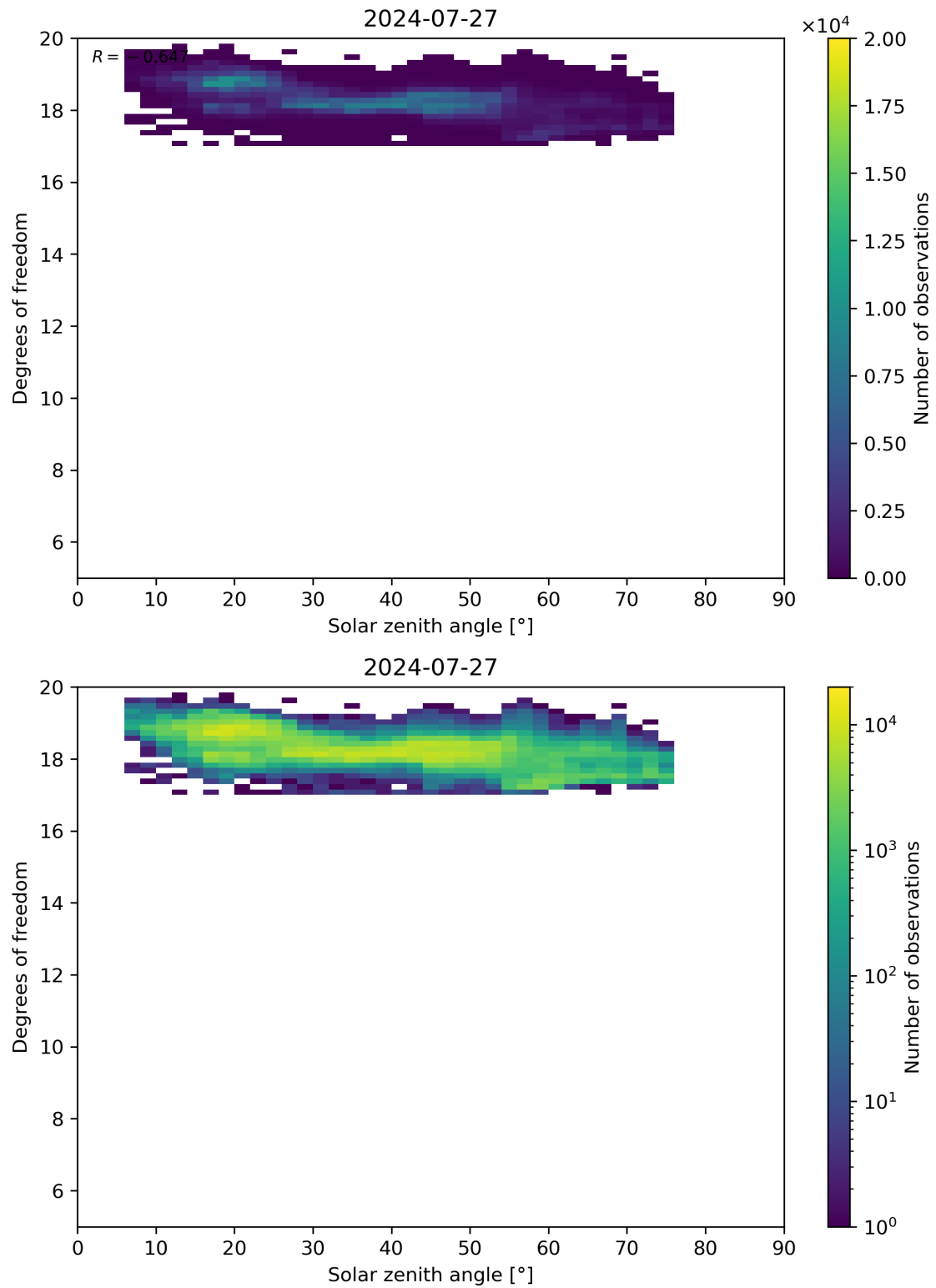
Figure 96: Scatter density plot of “Solar zenith angle” against “Degrees of freedom” for 2024-07-26 to 2024-07-28.
