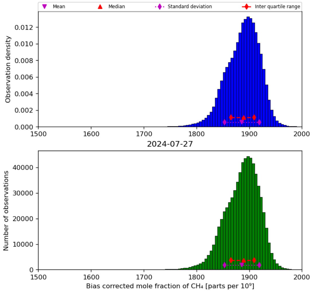
Figure 25: Histogram of “Bias corrected mole fraction of \text{CH}_4 ” for 2024-07-26 to 2024-07-28
