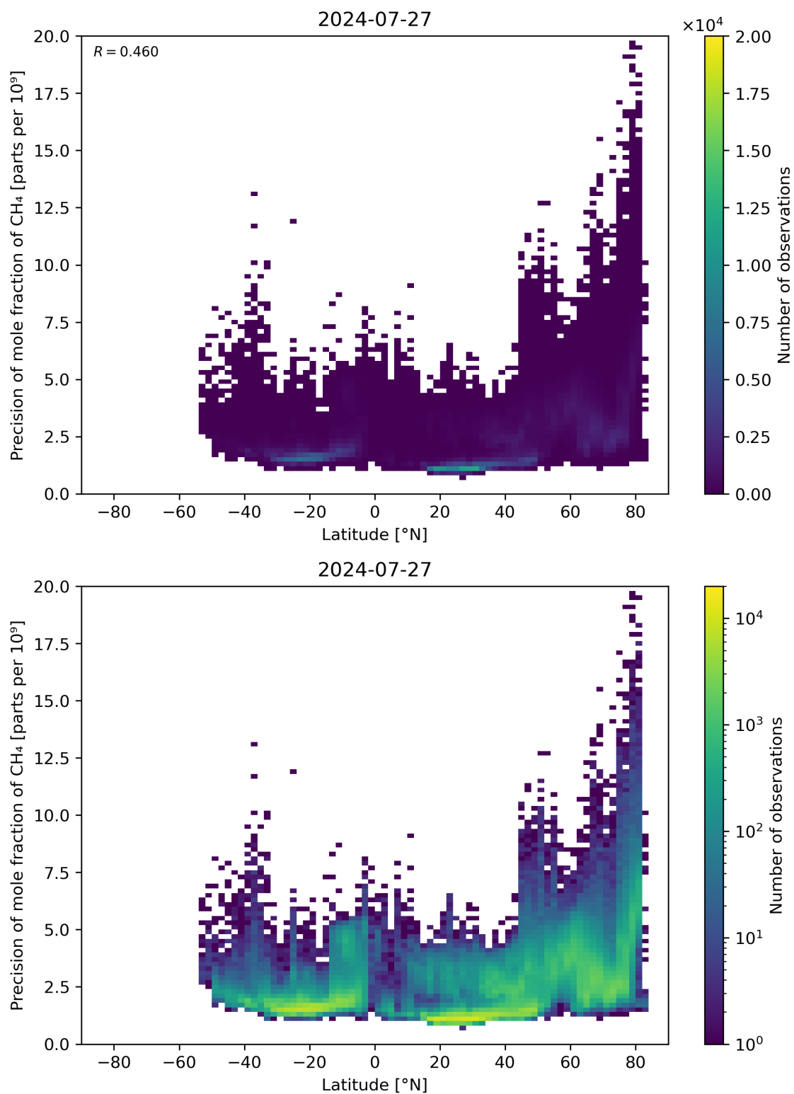
Figure 59: Scatter density plot of “Latitude” against “Precision of mole fraction of \text{CH}_4 ” for 2024-07-26 to 2024-07-28.
