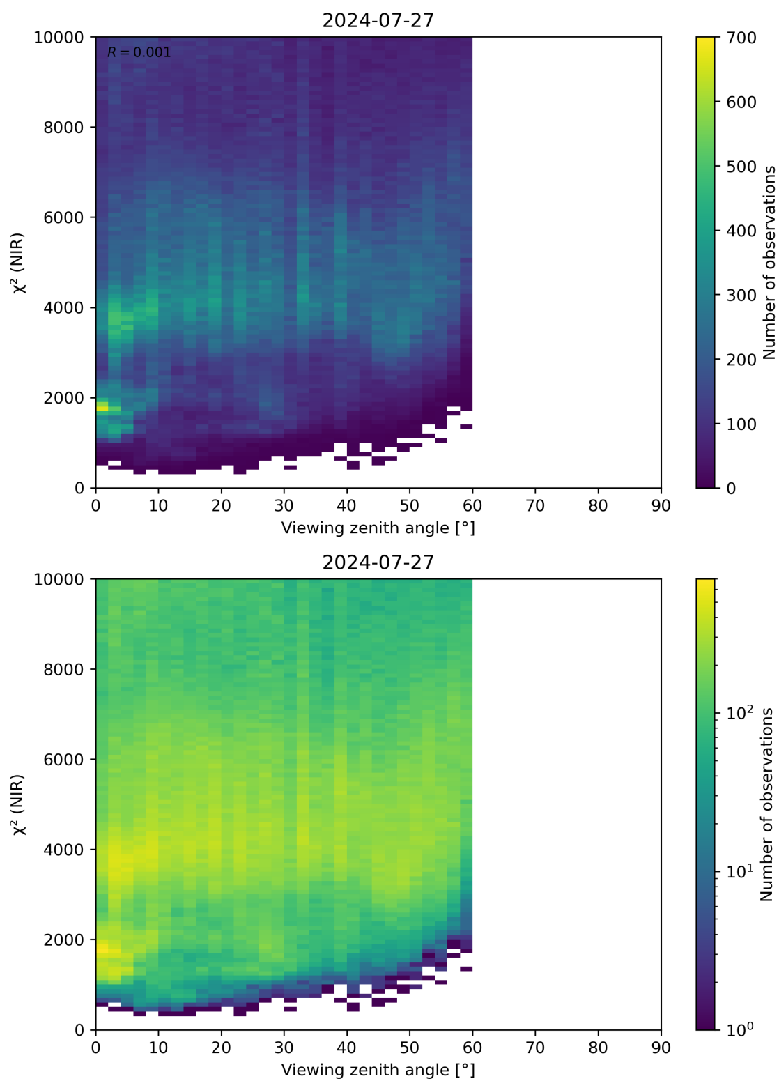
Figure 105: Scatter density plot of “Viewing zenith angle” against “ \chi^2 (NIR)” for 2024-07-26 to 2024-07-28.
