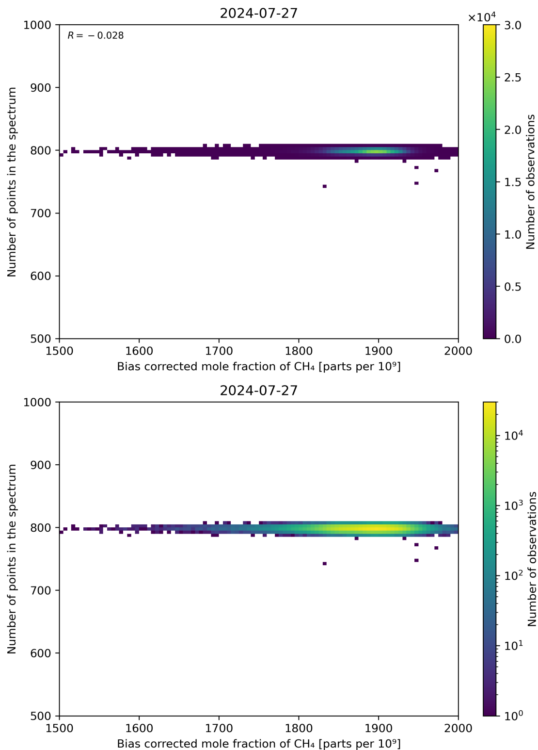
Figure 68: Scatter density plot of “Bias corrected mole fraction of CH 4 ” against “Number of points in the spectrum” for 2024-07-26 to 2024-07-28.
