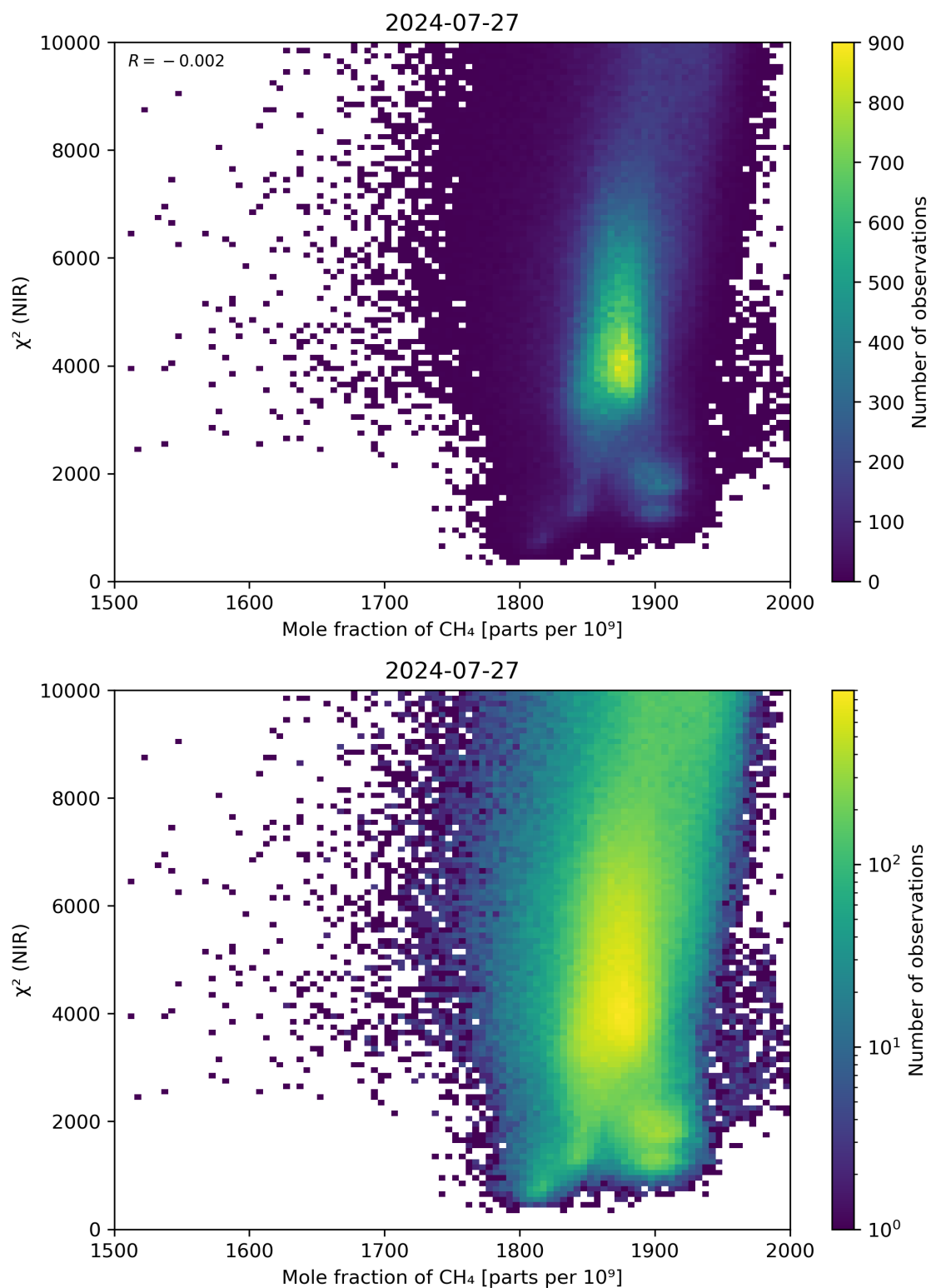
Figure 70: Scatter density plot of “Mole fraction of CH 4 ” against “ \chi^2 (NIR)” for 2024-07-26 to 2024-07-28.
