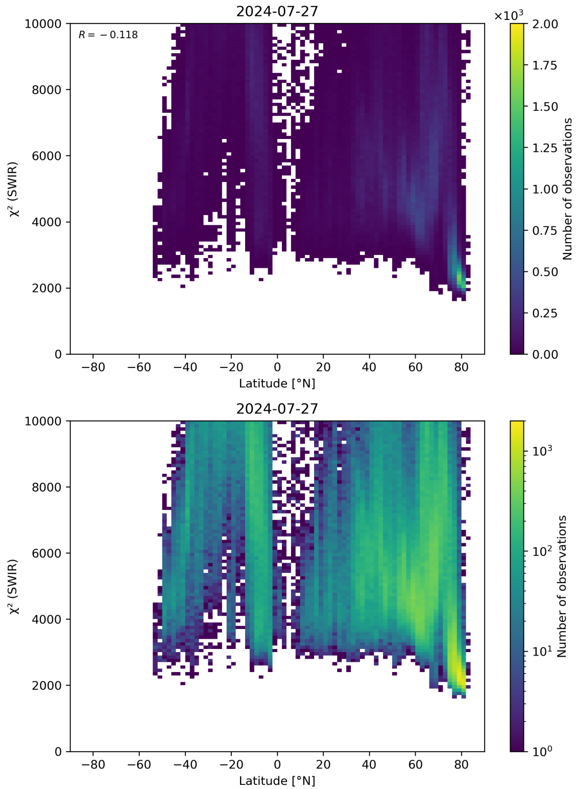
Figure 54: Scatter density plot of “Latitude” against “ \chi^2 (SWIR)” for 2024-07-26 to 2024-07-28.
