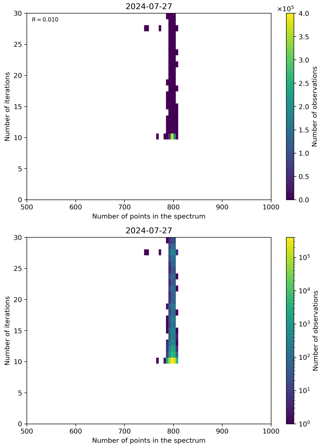
Figure 92: Scatter density plot of “Number of points in the spectrum” against “Number of iterations” for 2024-07-26 to 2024-07-28.
