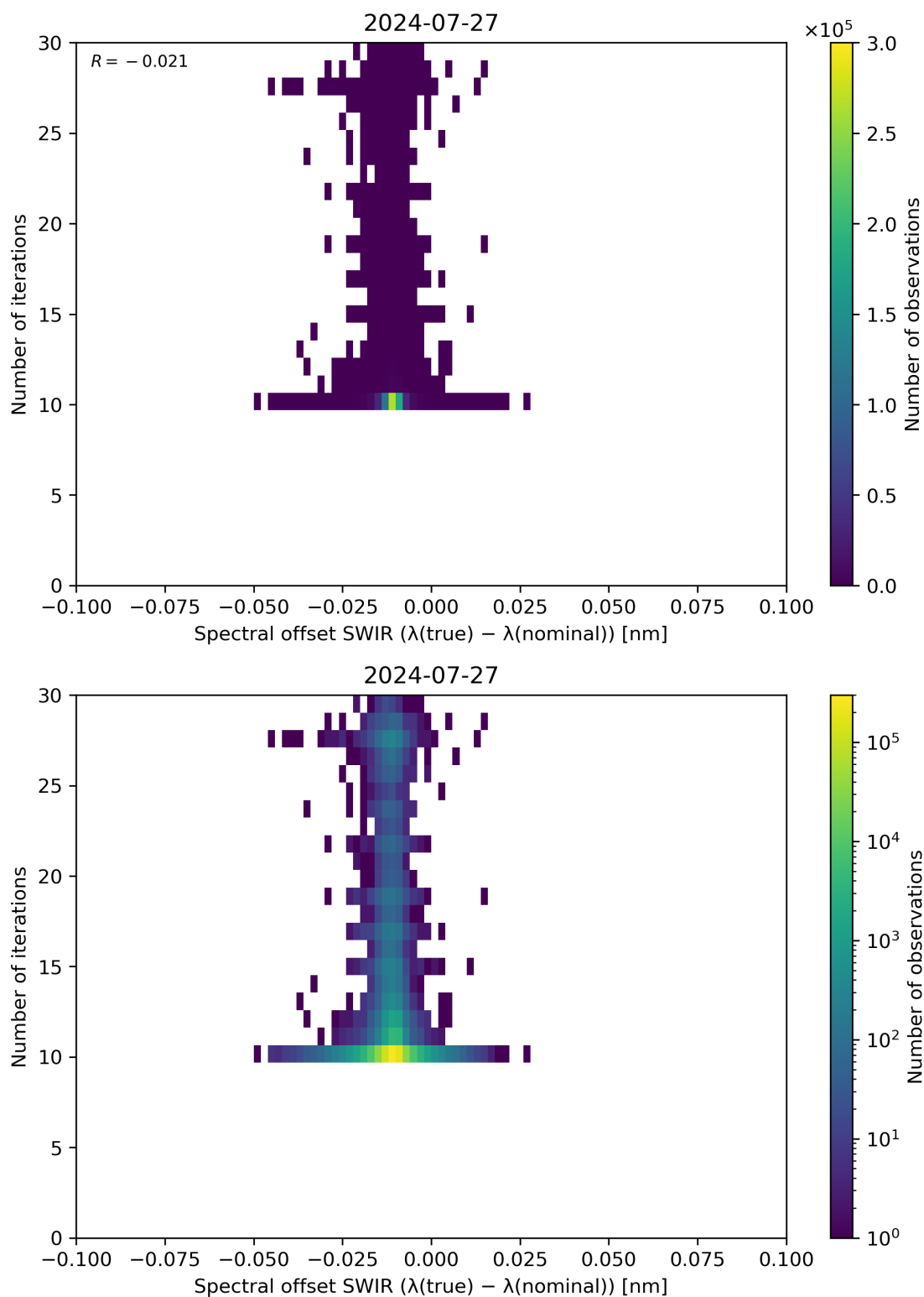
Figure 121: Scatter density plot of “Spectral offset SWIR ( \lambda(\text{true}) - \lambda(\text{nominal}) )” against “Number of iterations” for 2024-07-26 to 2024-07-28.
