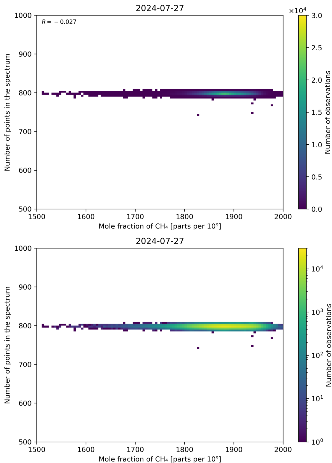
Figure 77: Scatter density plot of “Mole fraction of CH 4 ” against “Number of points in the spectrum” for 2024-07-26 to 2024-07-28.
