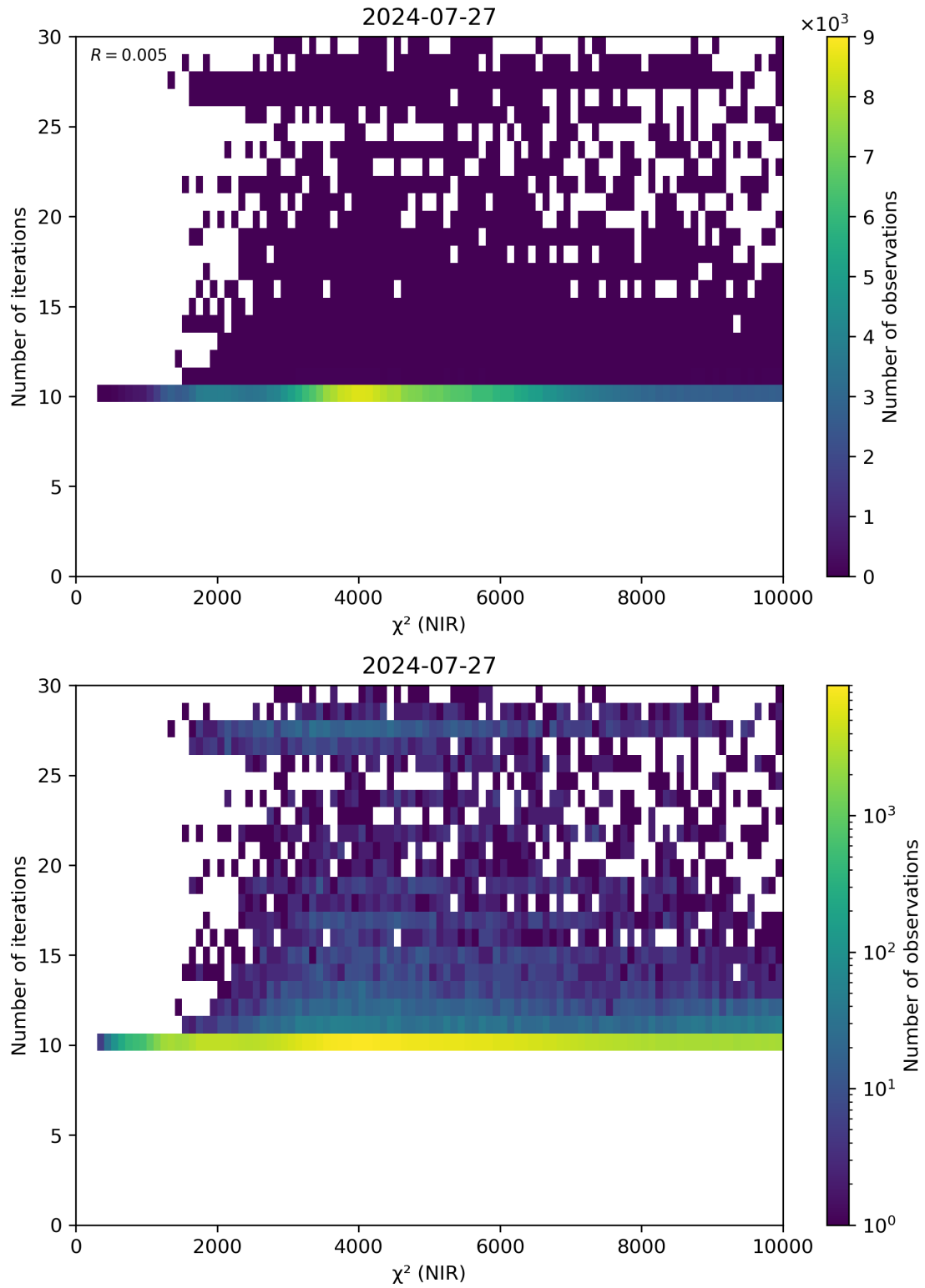
Figure 46: Scatter density plot of “ \chi^2 (NIR)” against “Number of iterations” for 2024-07-26 to 2024-07-28.
