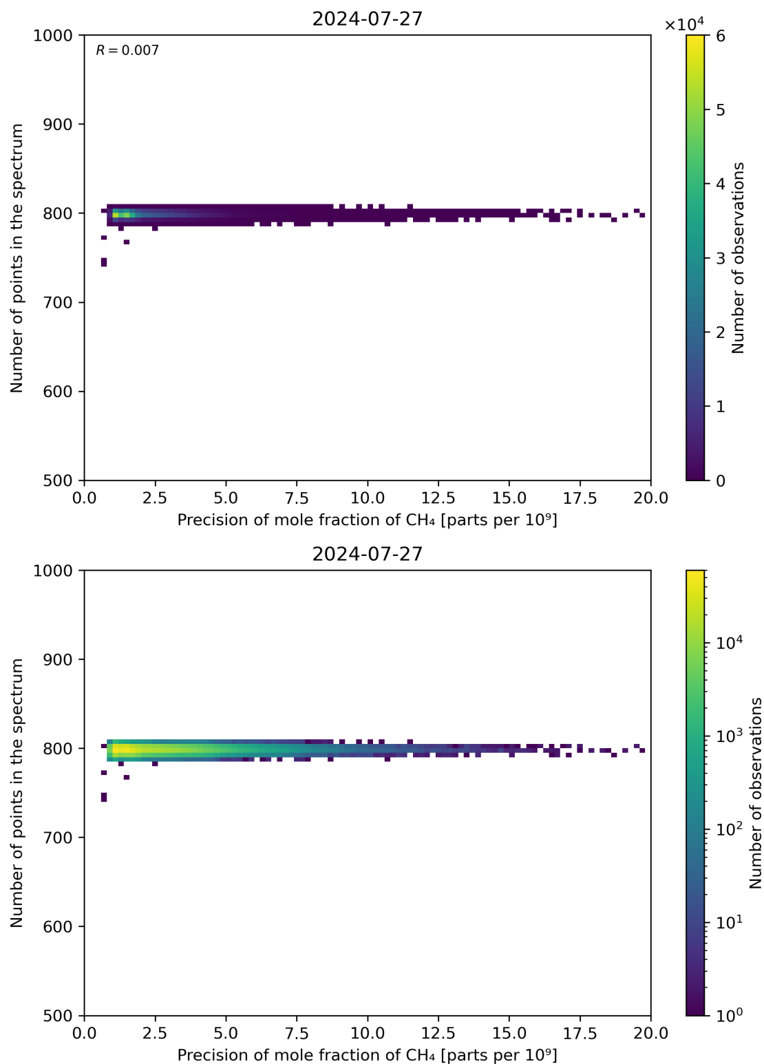
Figure 84: Scatter density plot of “Precision of mole fraction of CH 4 ” against “Number of points in the spectrum” for 2024-07-26 to 2024-07-28.
