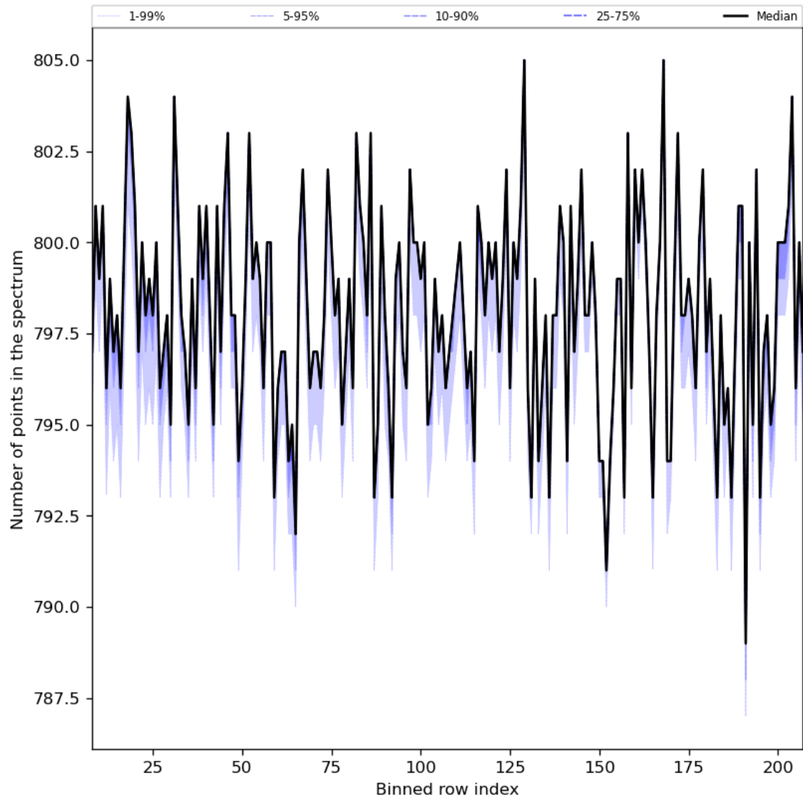
Figure 37: Along track statistics of “Number of points in the spectrum” for 2024-07-26 to 2024-07-28
