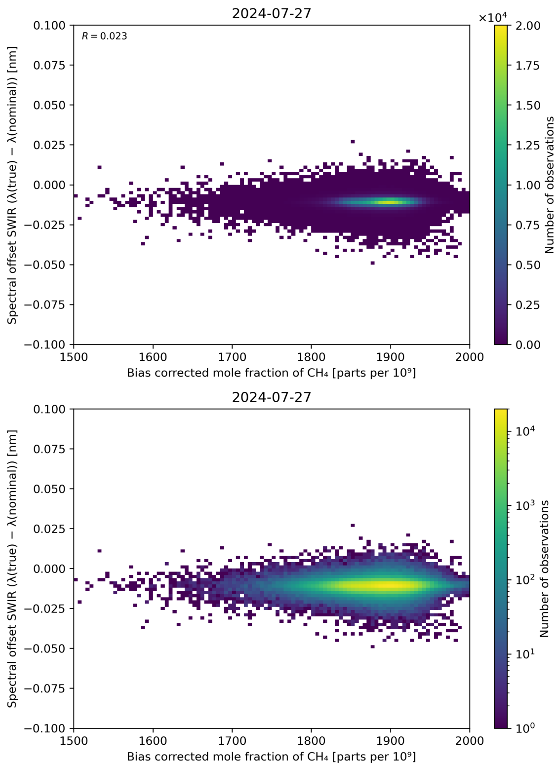
Figure 69: Scatter density plot of “Bias corrected mole fraction of \text{CH}_4 ” against “Spectral offset SWIR ( \lambda(\text{true}) - \lambda(\text{nominal}) )” for 2024-07-26 to 2024-07-28.
