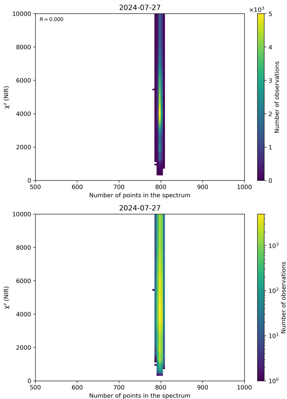
Figure 88: Scatter density plot of “Number of points in the spectrum” against “ \chi^2 (NIR)” for 2024-07-26 to 2024-07-28.
