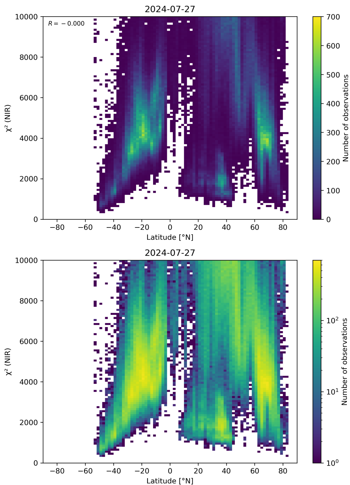
Figure 53: Scatter density plot of “Latitude” against “ \chi^2 (NIR)” for 2024-07-26 to 2024-07-28.
