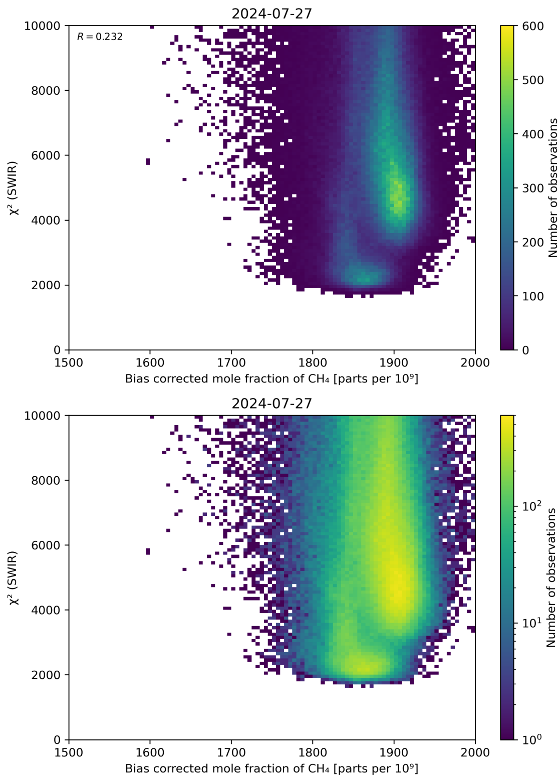
Figure 64: Scatter density plot of “Bias corrected mole fraction of \text{CH}_4 ” against “ \chi^2 (SWIR)” for 2024-07-26 to 2024-07-28.
