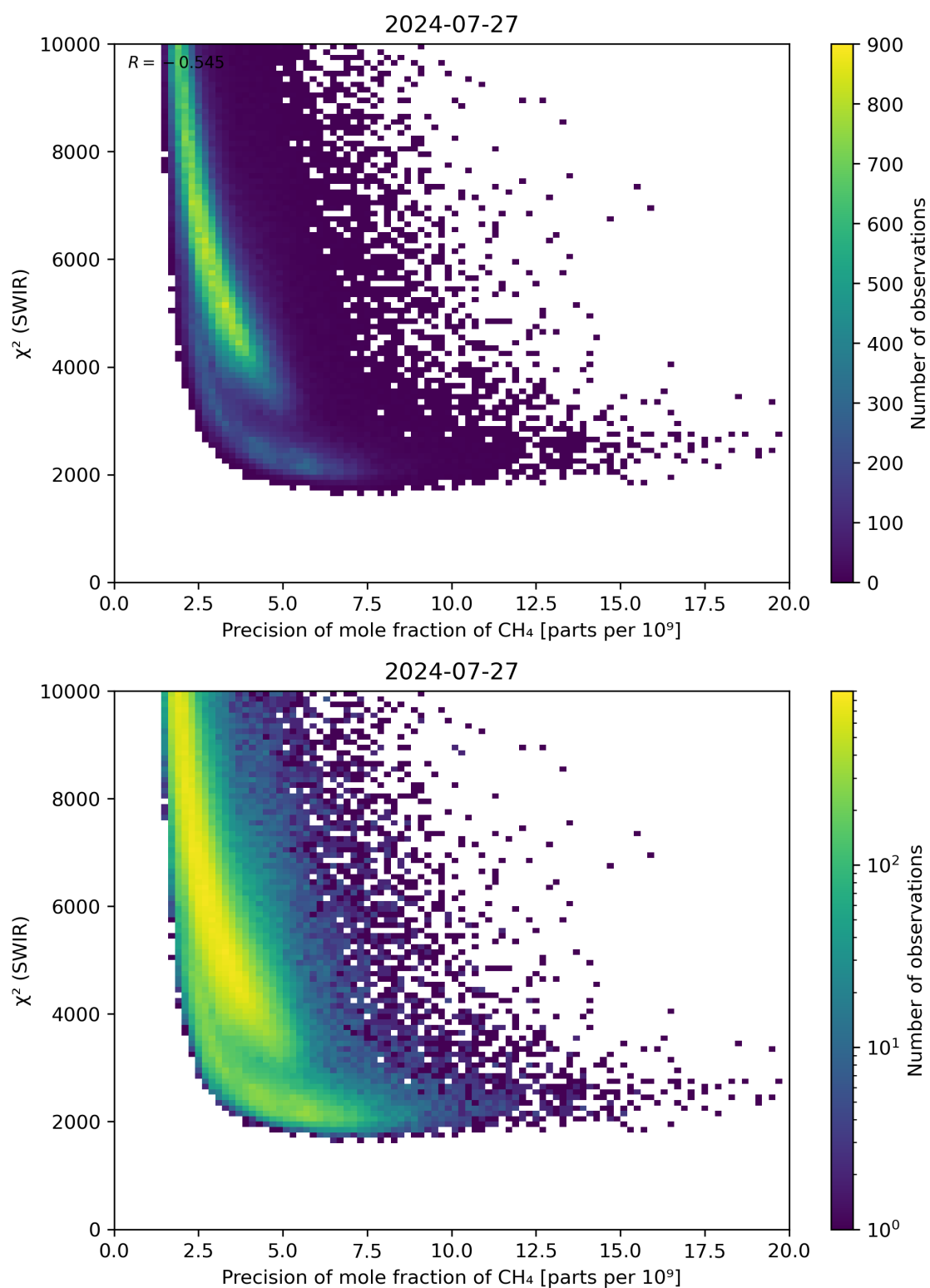
Figure 79: Scatter density plot of “Precision of mole fraction of \text{CH}_4 ” against “ \chi^2 (SWIR)” for 2024-07-26 to 2024-07-28.
