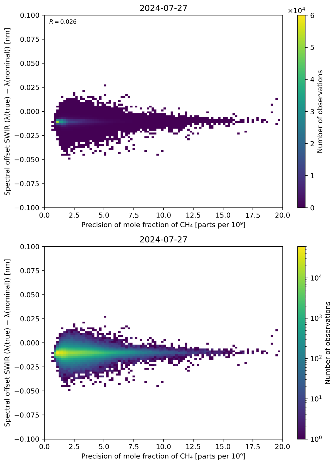
Figure 85: Scatter density plot of “Precision of mole fraction of CH 4 ” against “Spectral offset SWIR ( \lambda(\text{true}) - \lambda(\text{nominal}) )” for 2024-07-26 to 2024-07-28.
