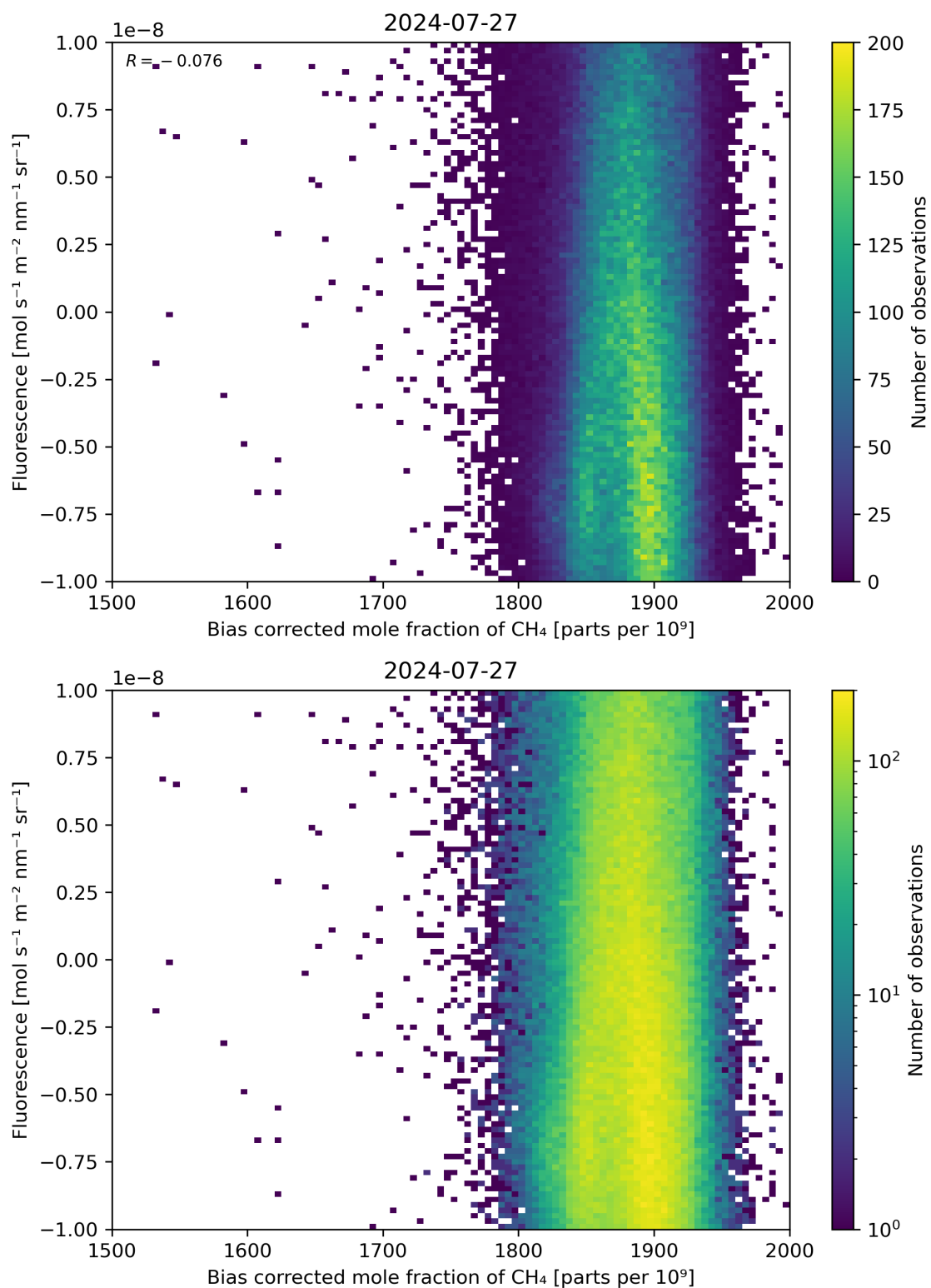
Figure 66: Scatter density plot of “Bias corrected mole fraction of \text{CH}_4 ” against “Fluorescence” for 2024-07-26 to 2024-07-28.
