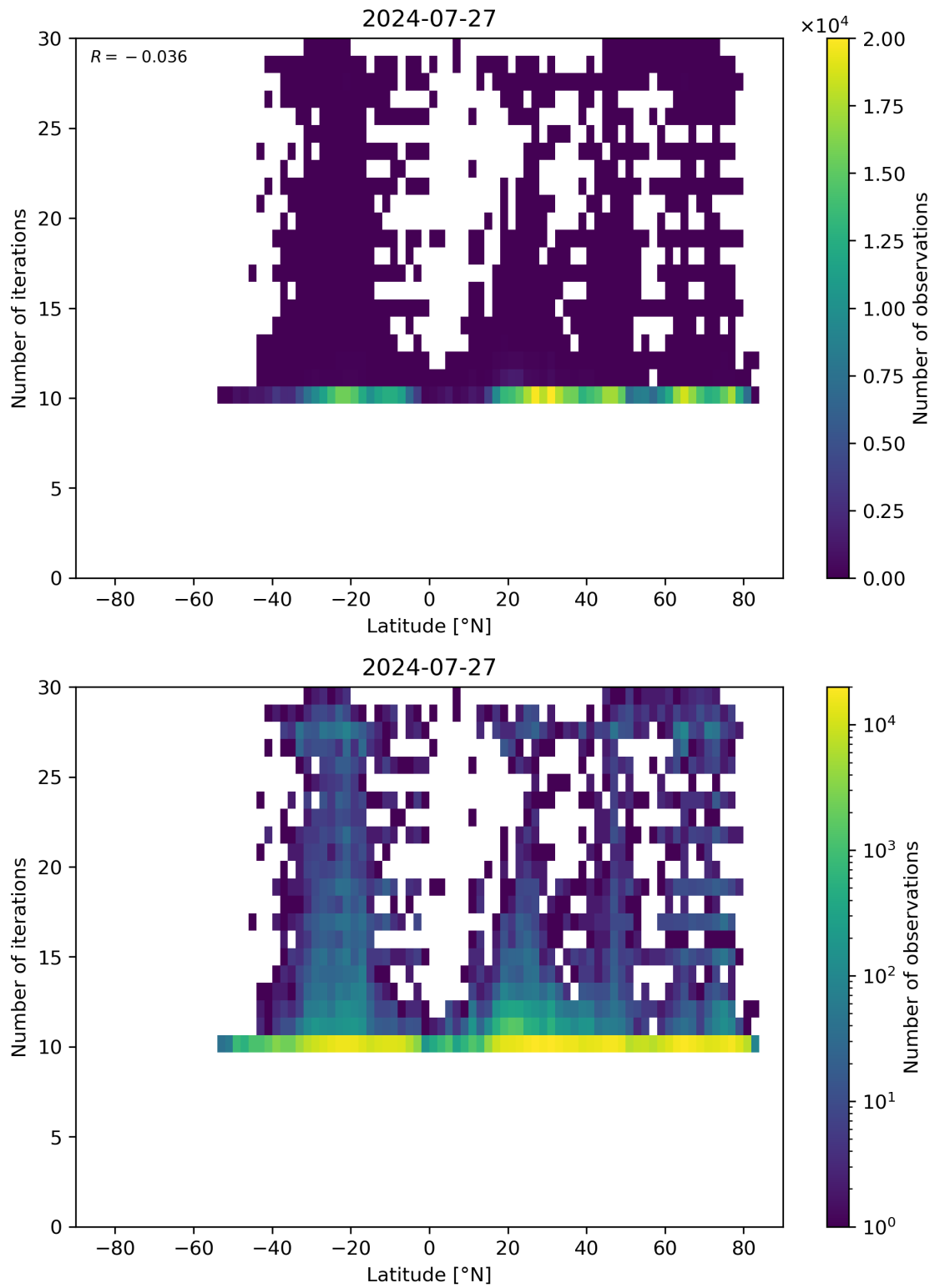
Figure 60: Scatter density plot of “Latitude” against “Number of iterations” for 2024-07-26 to 2024-07-28.
