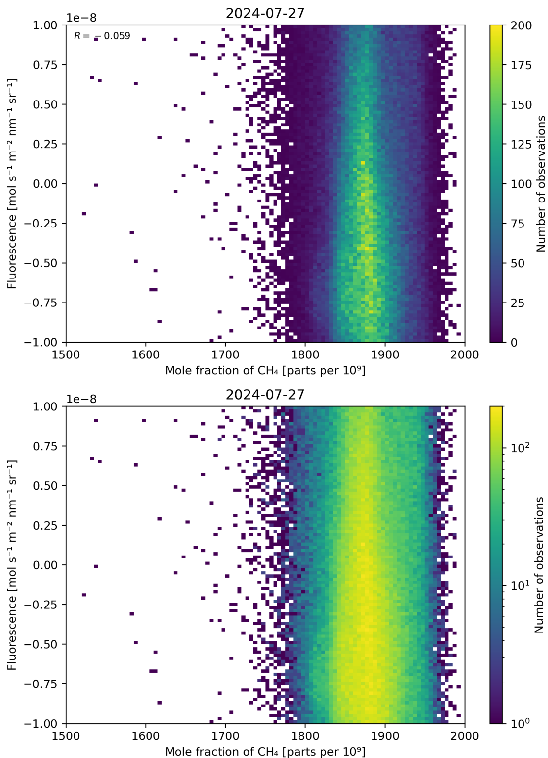
Figure 73: Scatter density plot of “Mole fraction of \text{CH}_4 ” against “Fluorescence” for 2024-07-26 to 2024-07-28.
