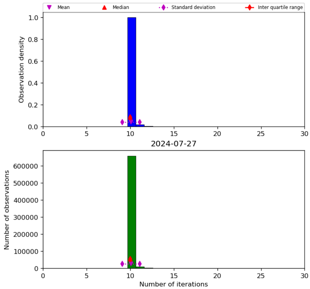
Figure 31: Histogram of “Number of iterations” for 2024-07-26 to 2024-07-28
