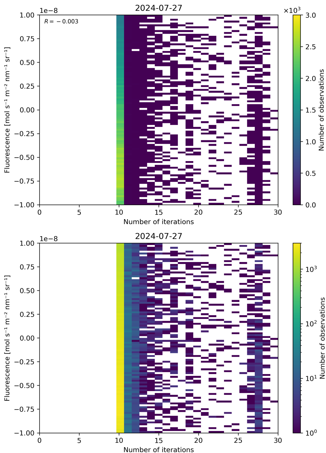
Figure 87: Scatter density plot of “Number of iterations” against “Fluorescence” for 2024-07-26 to 2024-07-28.
