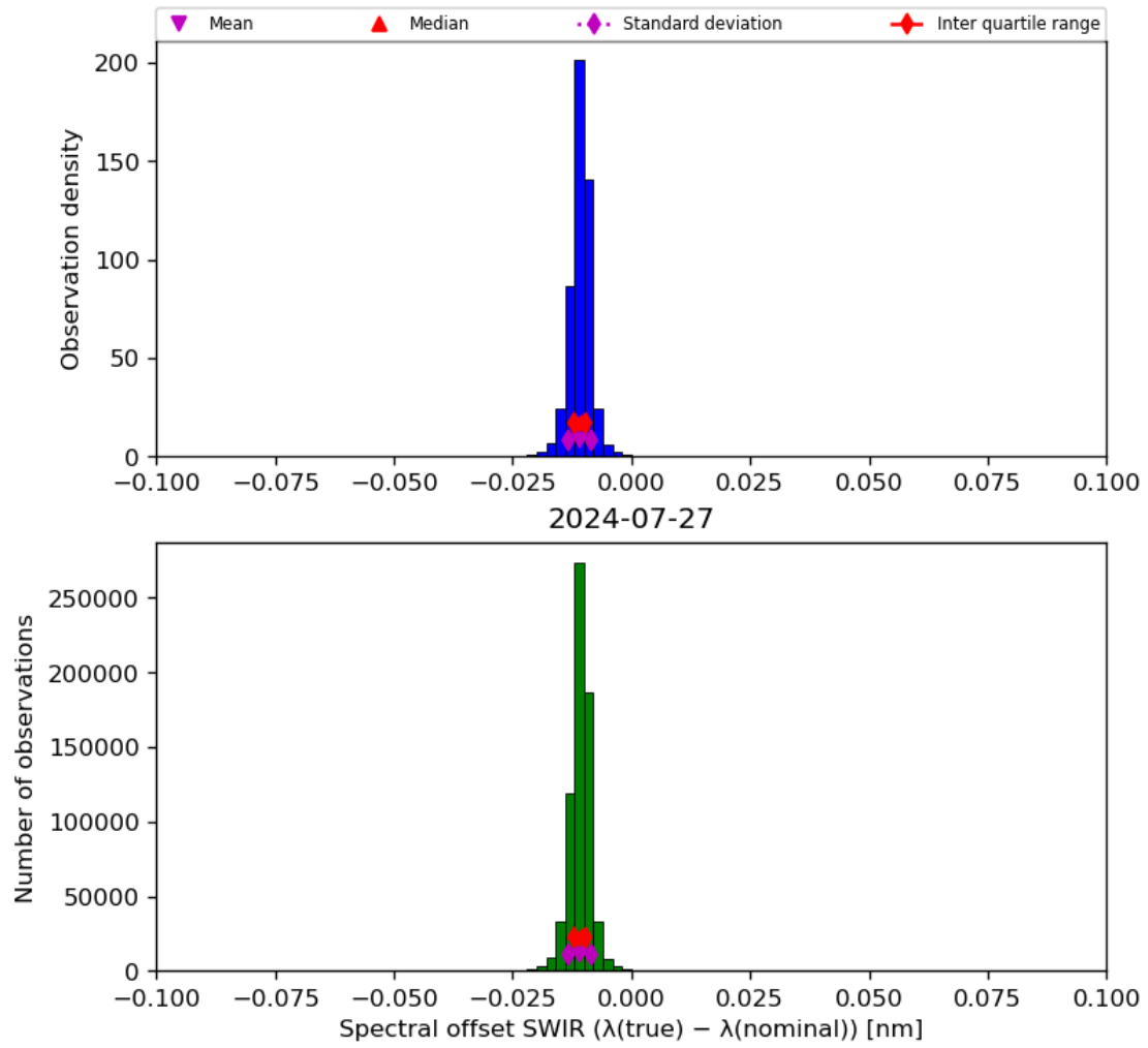
Figure 27: Histogram of “Spectral offset SWIR ( \lambda(\text{true}) - \lambda(\text{nominal}) )” for 2024-07-26 to 2024-07-28
