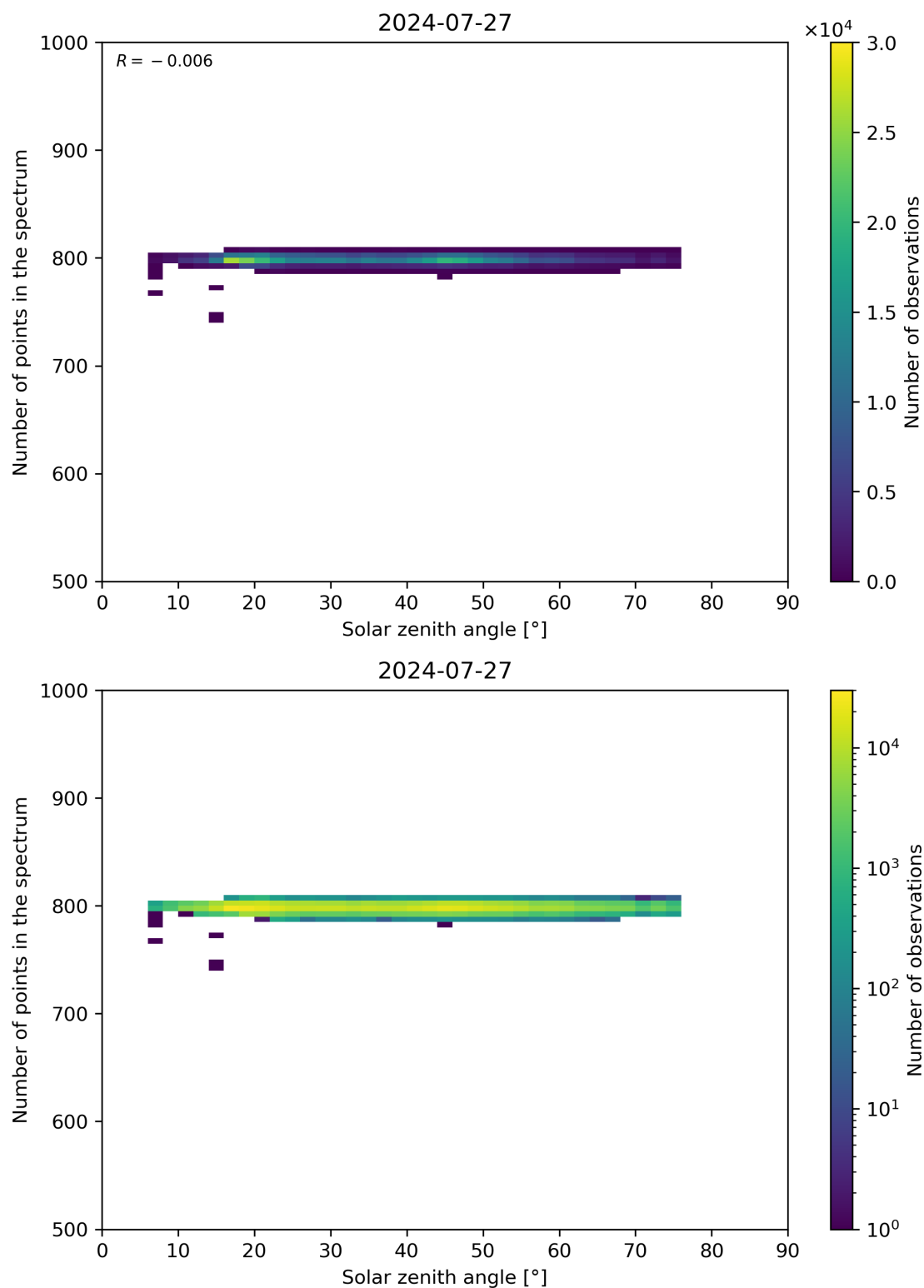
Figure 103: Scatter density plot of “Solar zenith angle” against “Number of points in the spectrum” for 2024-07-26 to 2024-07-28.
