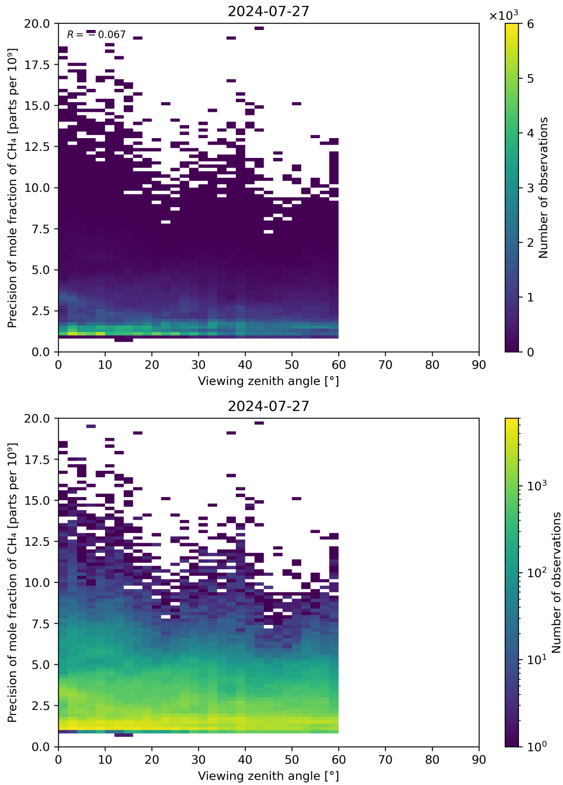
Figure 112: Scatter density plot of “Viewing zenith angle” against “Precision of mole fraction of CH 4 ” for 2024-07-26 to 2024-07-28.
