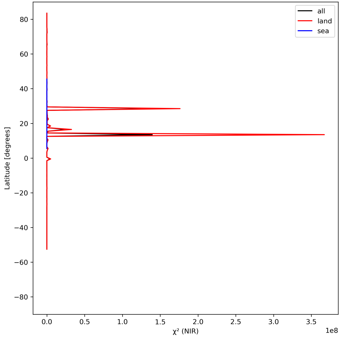
Figure 18: Zonal average of “ \chi^2 (NIR)” for 2024-07-26 to 2024-07-28.
