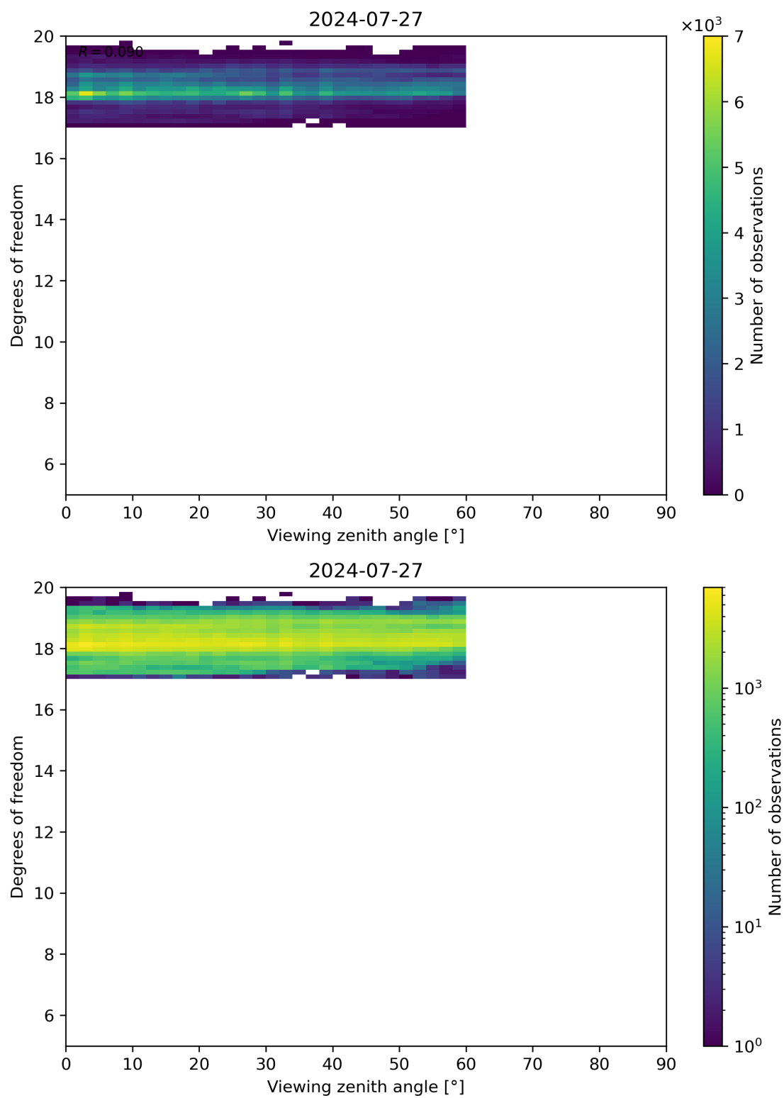
Figure 107: Scatter density plot of “Viewing zenith angle” against “Degrees of freedom” for 2024-07-26 to 2024-07-28.
