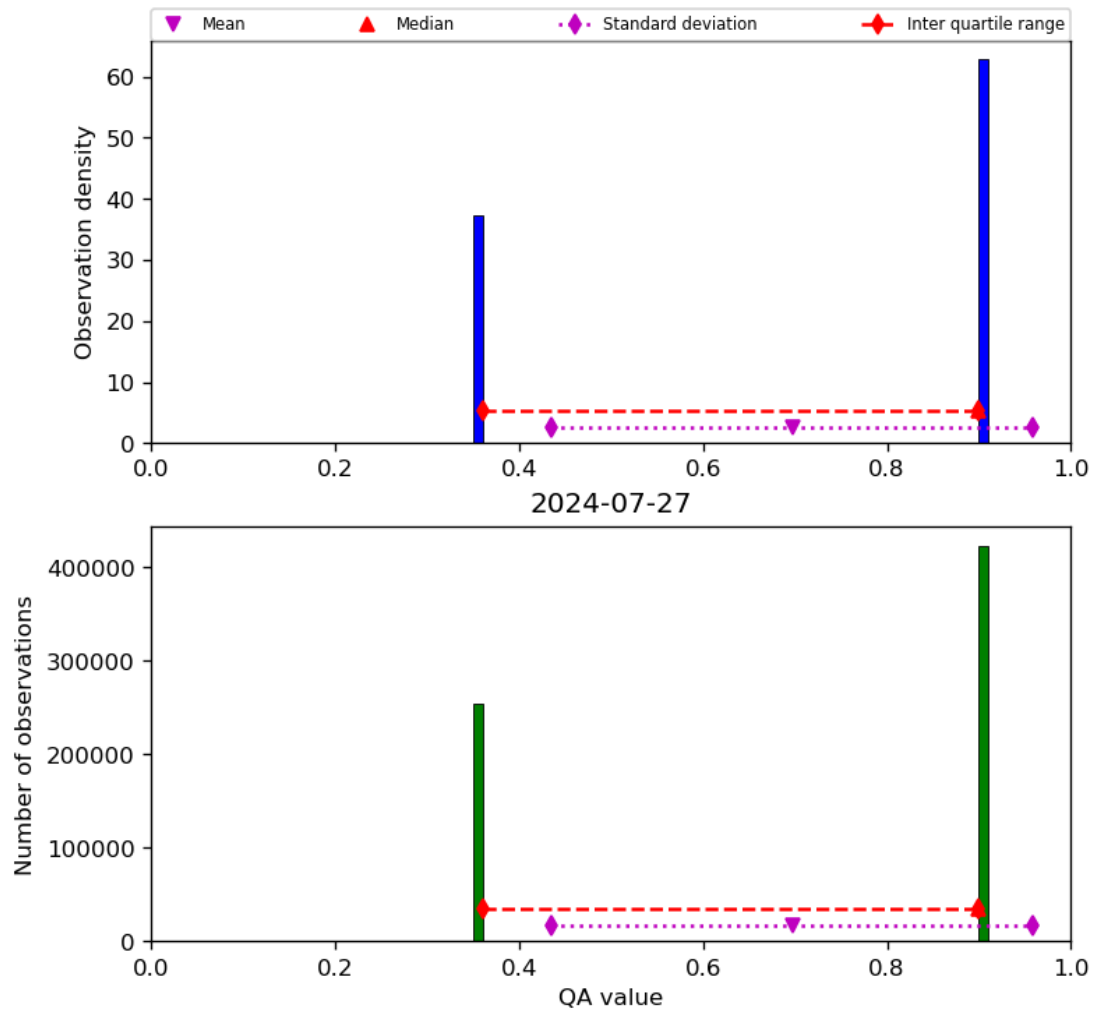
Figure 22: Histogram of “QA value” for 2024-07-26 to 2024-07-28
