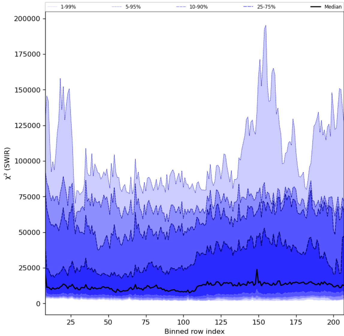
Figure 39: Along track statistics of “ \chi^2 (SWIR)” for 2024-07-26 to 2024-07-28
