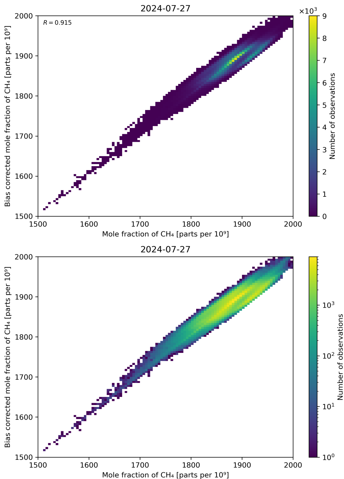
Figure 74: Scatter density plot of “Mole fraction of CH 4 ” against “Bias corrected mole fraction of CH 4 ” for 2024-07-26 to 2024-07-28.
