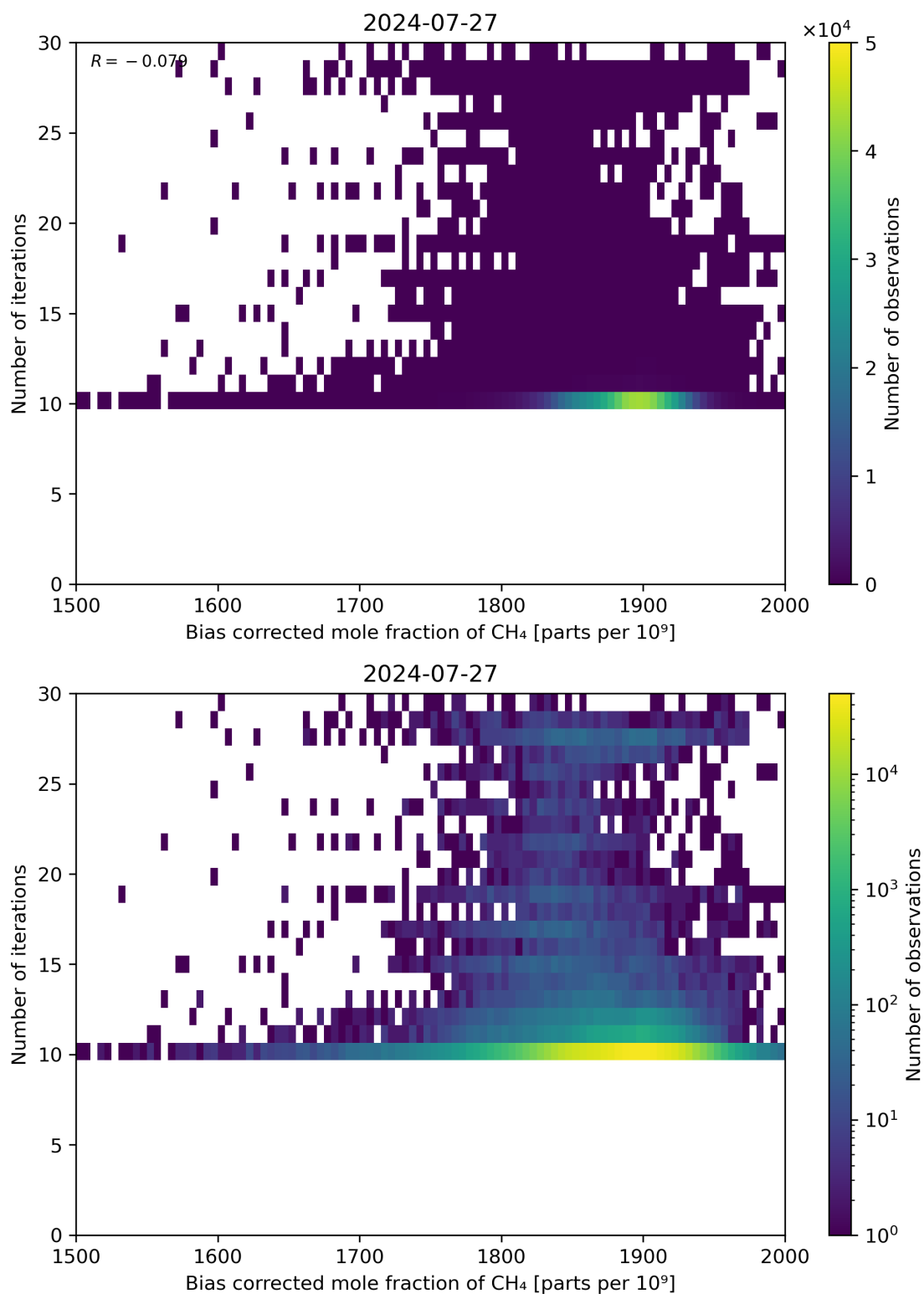
Figure 67: Scatter density plot of “Bias corrected mole fraction of CH 4 ” against “Number of iterations” for 2024-07-26 to 2024-07-28.
