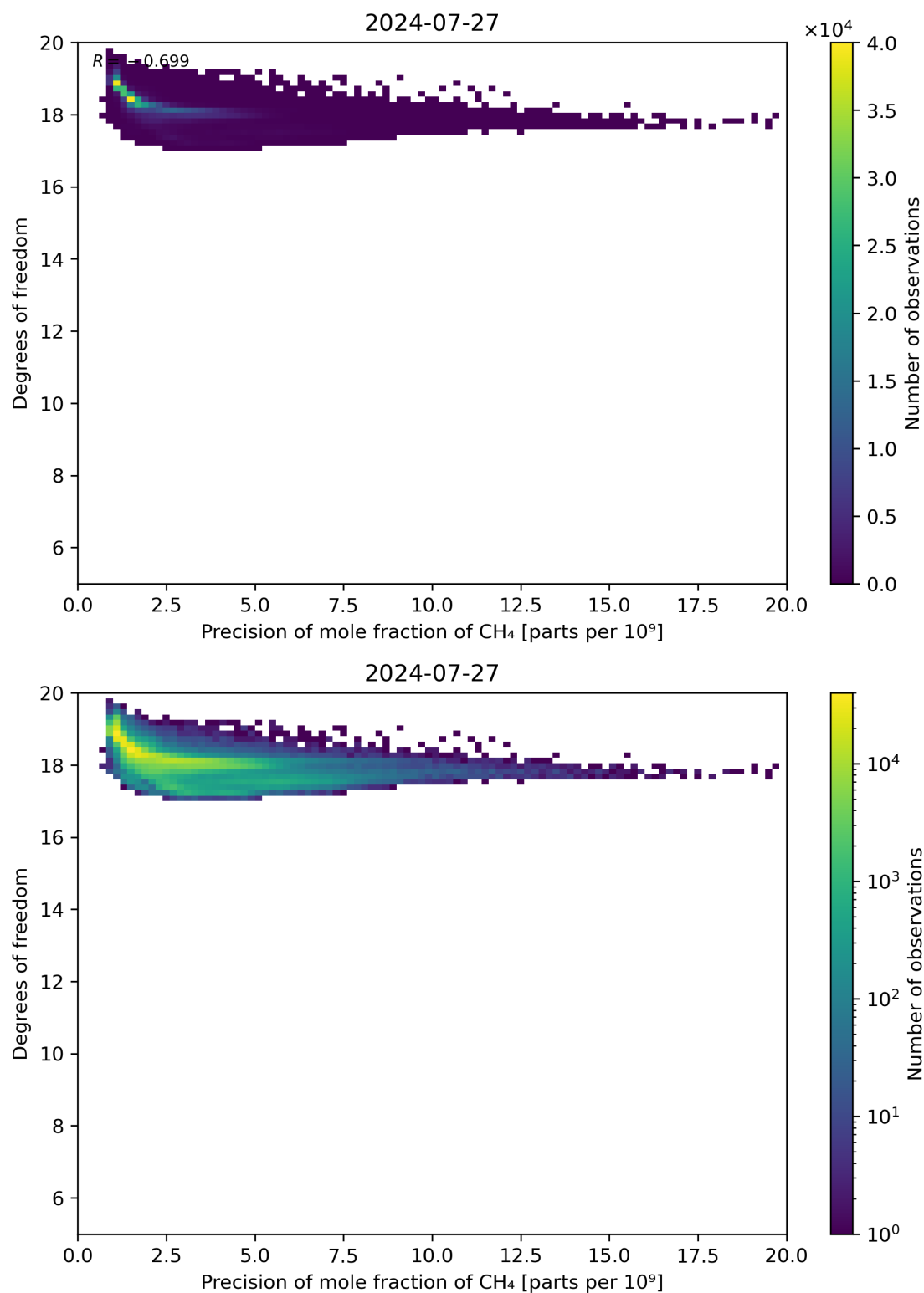
Figure 80: Scatter density plot of “Precision of mole fraction of CH 4 ” against “Degrees of freedom” for 2024-07-26 to 2024-07-28.
