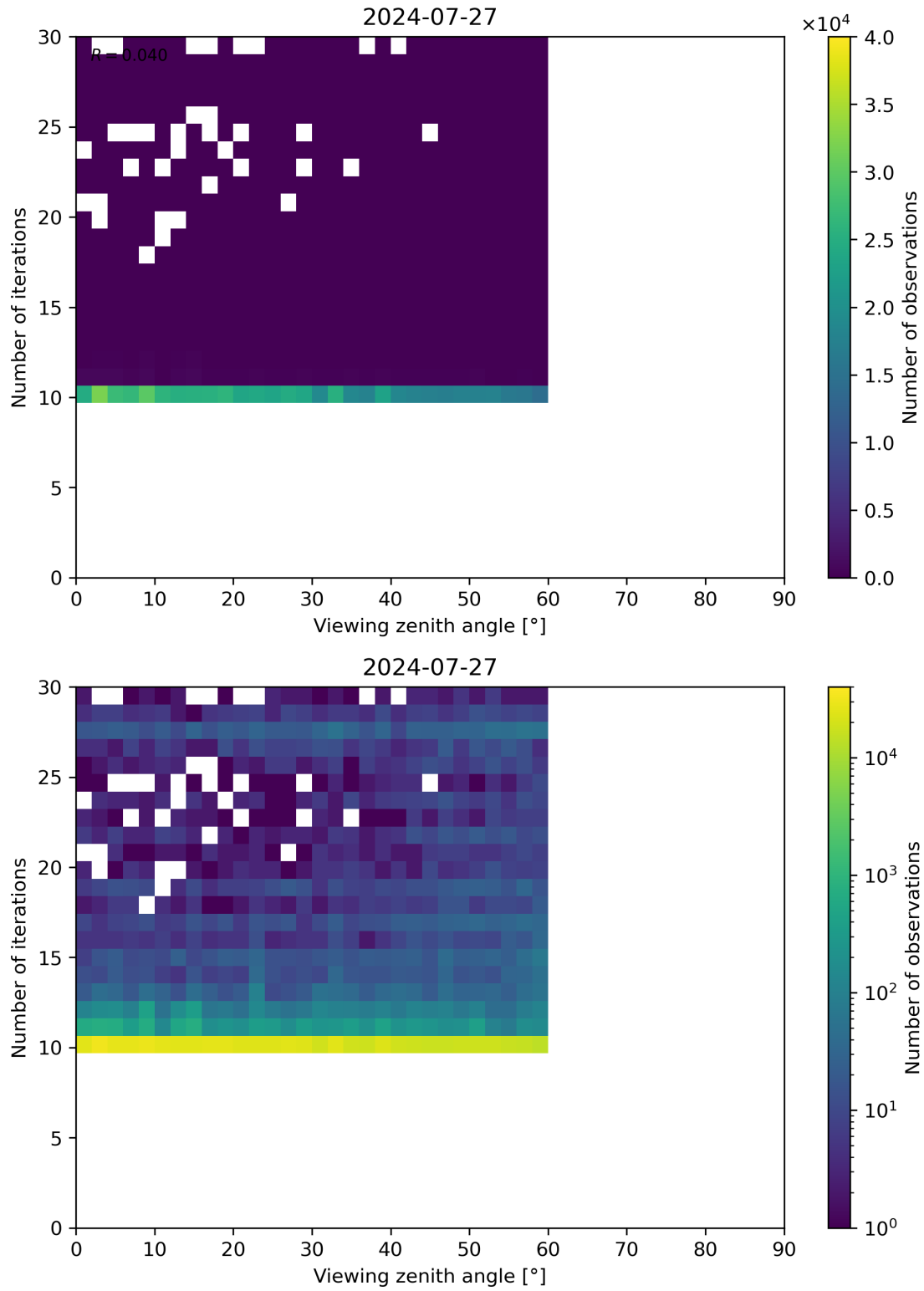
Figure 113: Scatter density plot of “Viewing zenith angle” against “Number of iterations” for 2024-07-26 to 2024-07-28.
