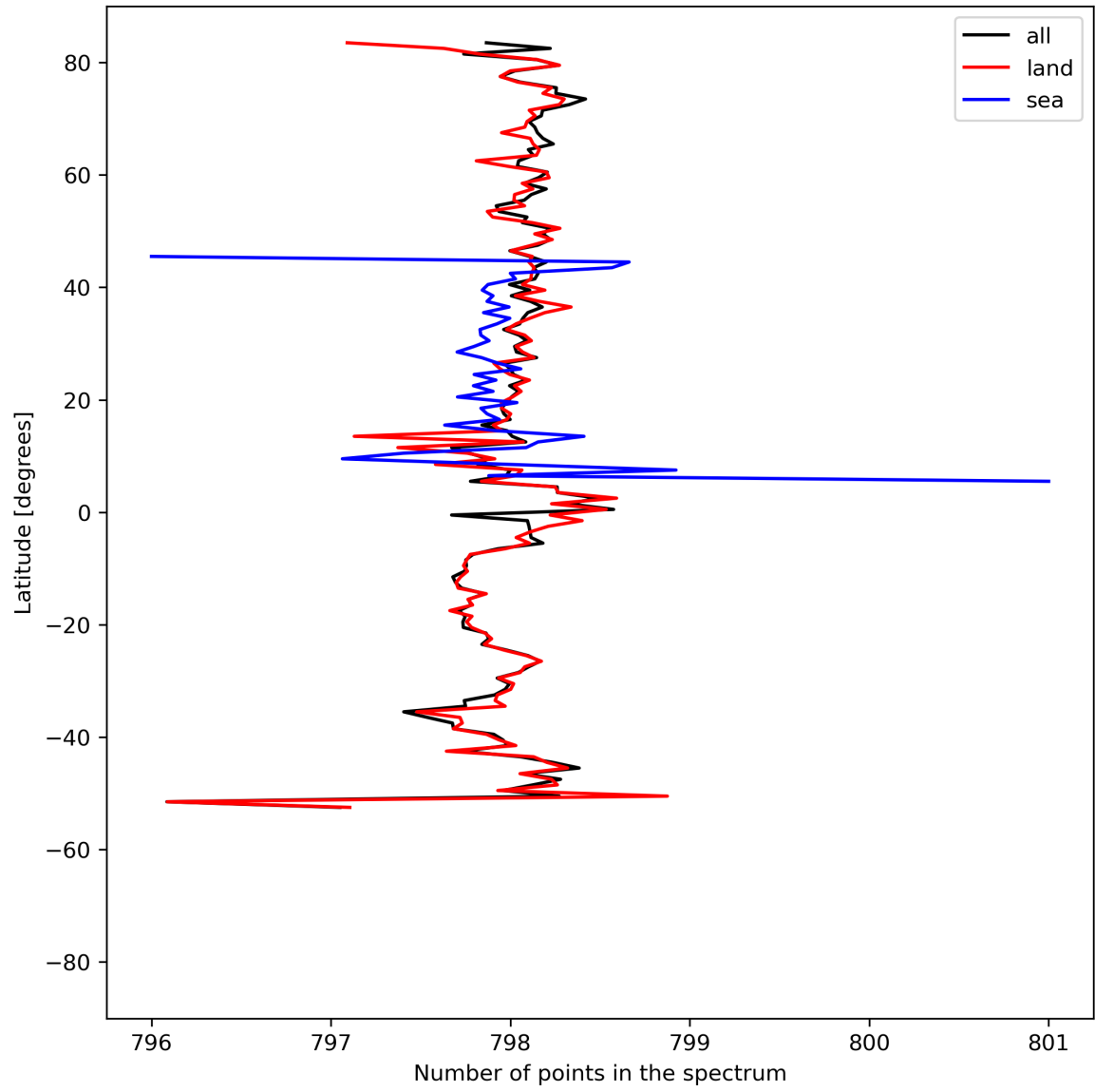
Figure 15: Zonal average of “Number of points in the spectrum” for 2024-07-26 to 2024-07-28.
