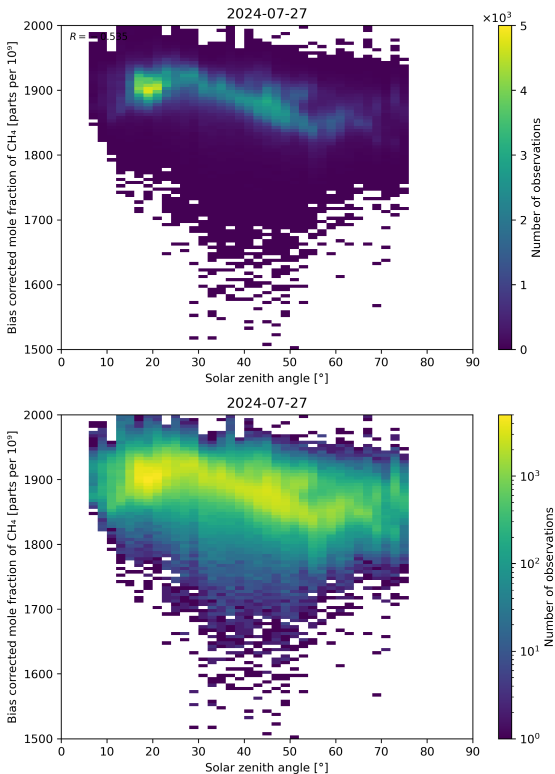
Figure 100: Scatter density plot of “Solar zenith angle” against “Bias corrected mole fraction of CH 4 ” for 2024-07-26 to 2024-07-28.
