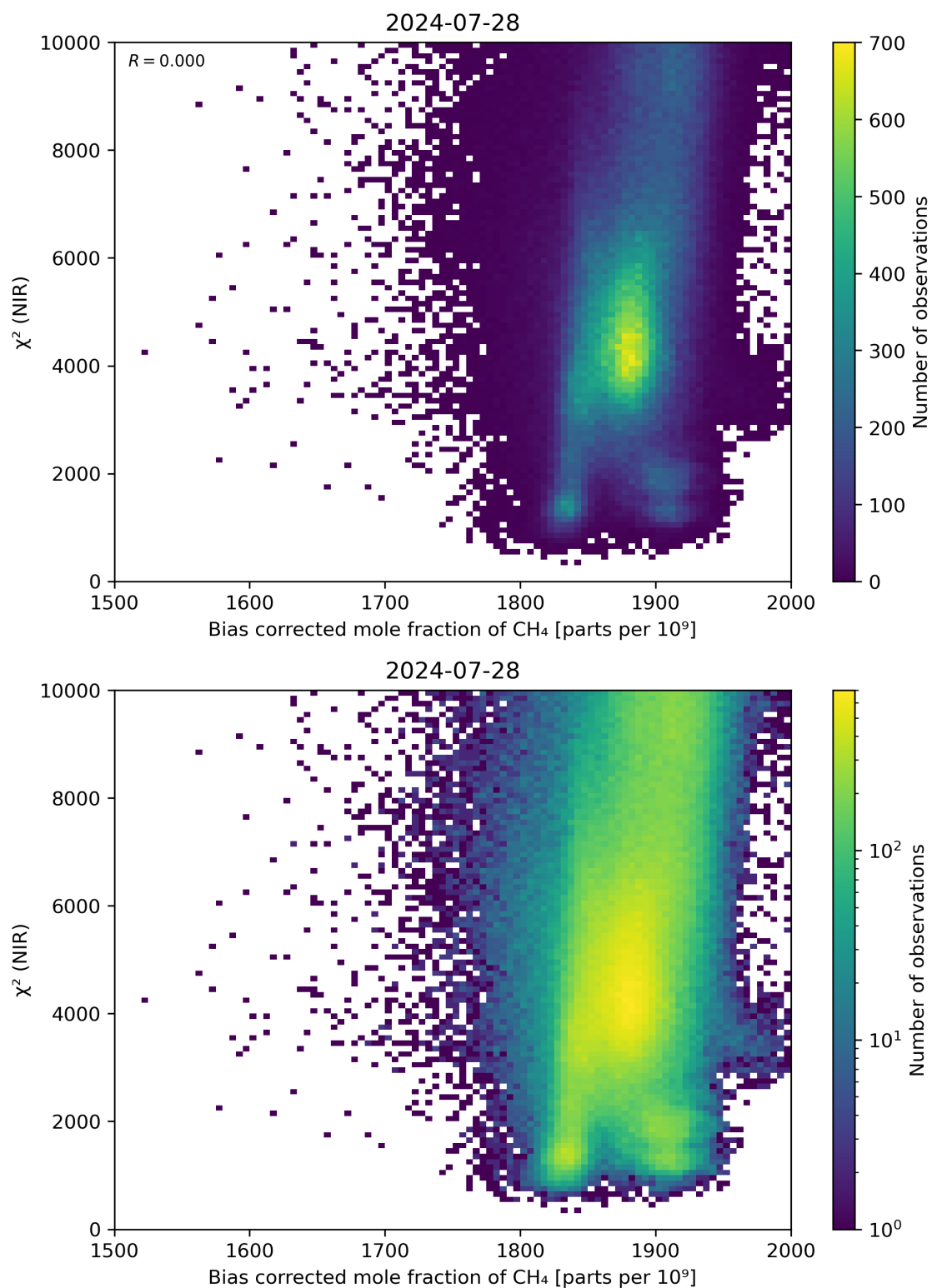
Figure 63: Scatter density plot of “Bias corrected mole fraction of CH 4 ” against “ \chi^2 (NIR)” for 2024-07-27 to 2024-07-29.
