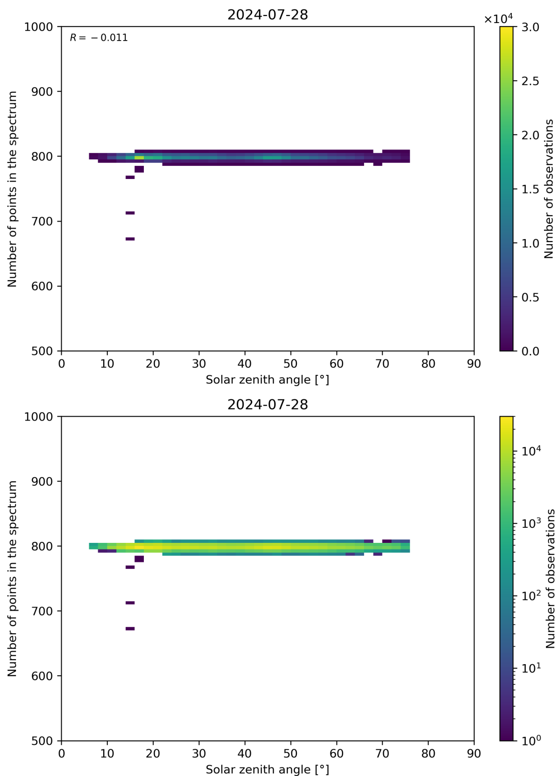
Figure 103: Scatter density plot of “Solar zenith angle” against “Number of points in the spectrum” for 2024-07-27 to 2024-07-29.
