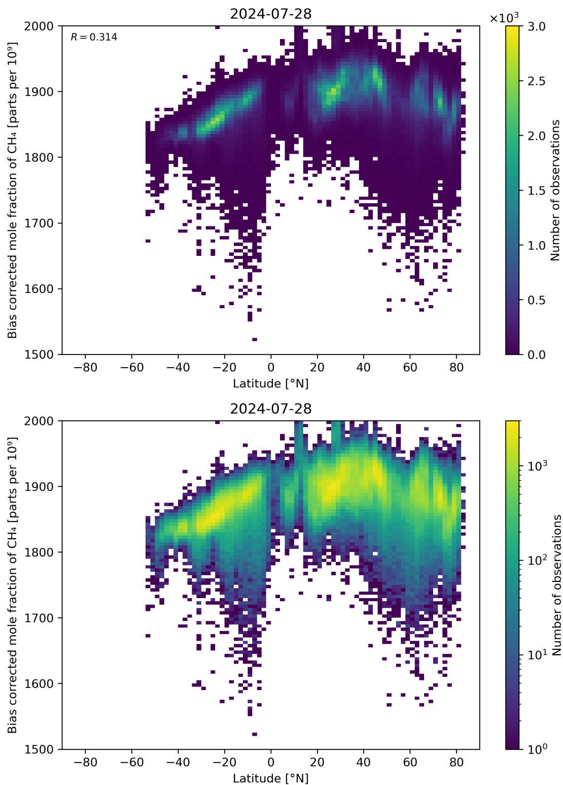
Figure 58: Scatter density plot of “Latitude” against “Bias corrected mole fraction of CH 4 ” for 2024-07-27 to 2024-07-29.
