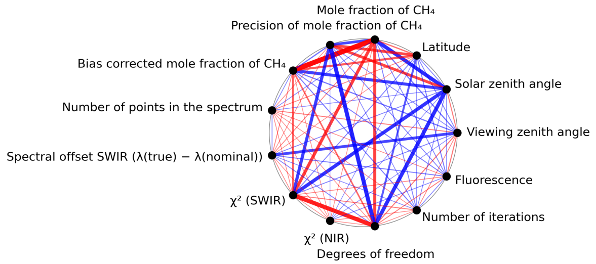
Figure 1: Map of correlation graph for 2024-07-27 to 2024-07-29.
