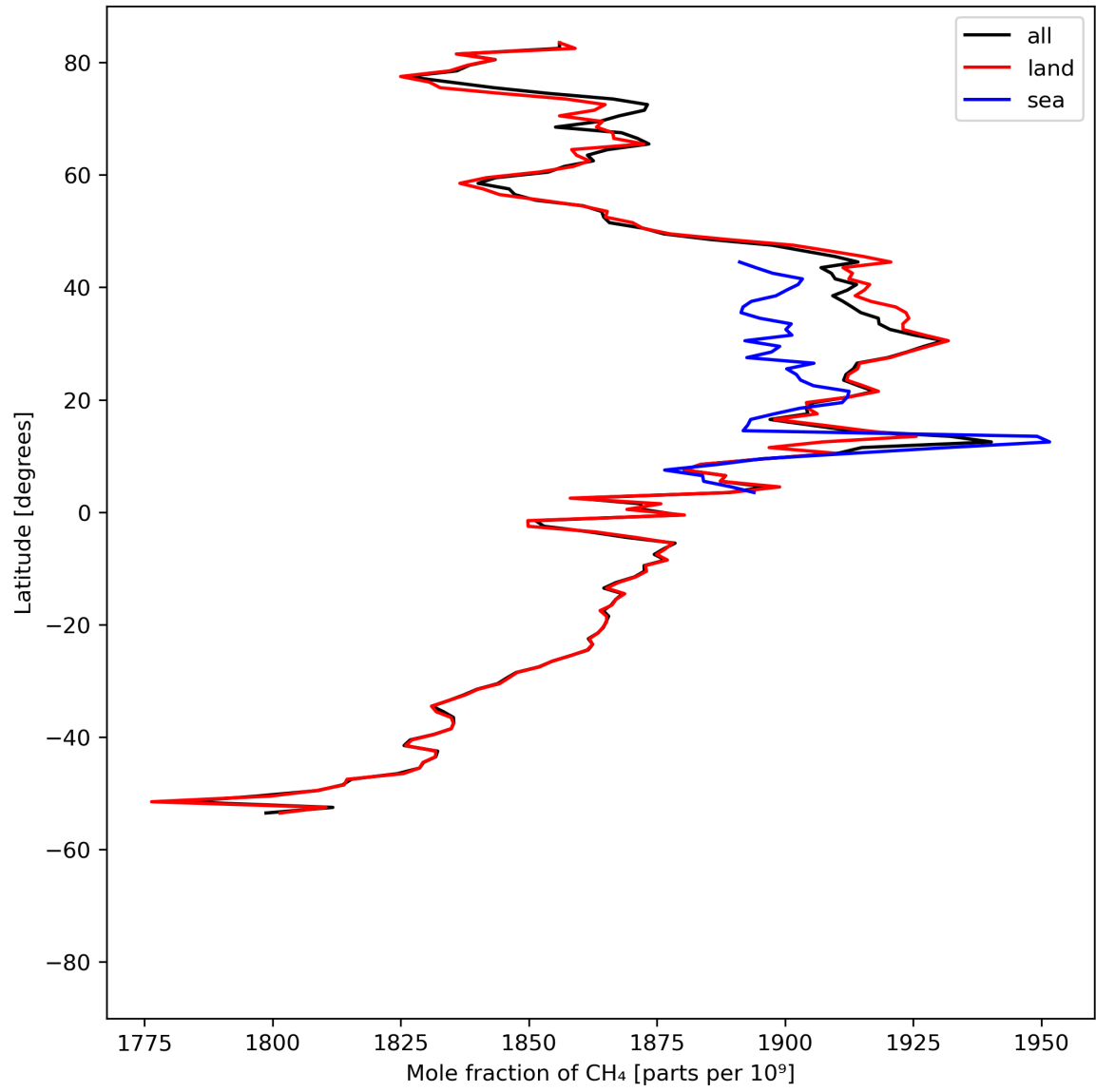
Figure 12: Zonal average of “Mole fraction of \text{CH}_4 ” for 2024-07-27 to 2024-07-29.
