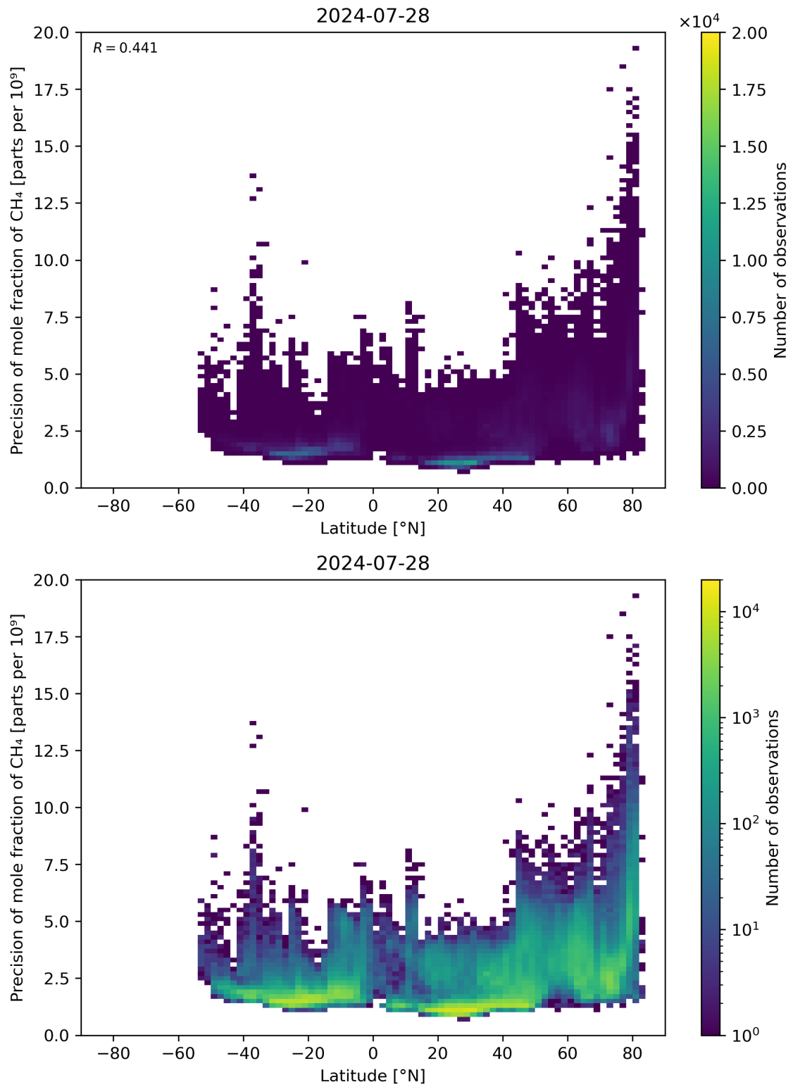
Figure 59: Scatter density plot of “Latitude” against “Precision of mole fraction of CH 4 ” for 2024-07-27 to 2024-07-29.
