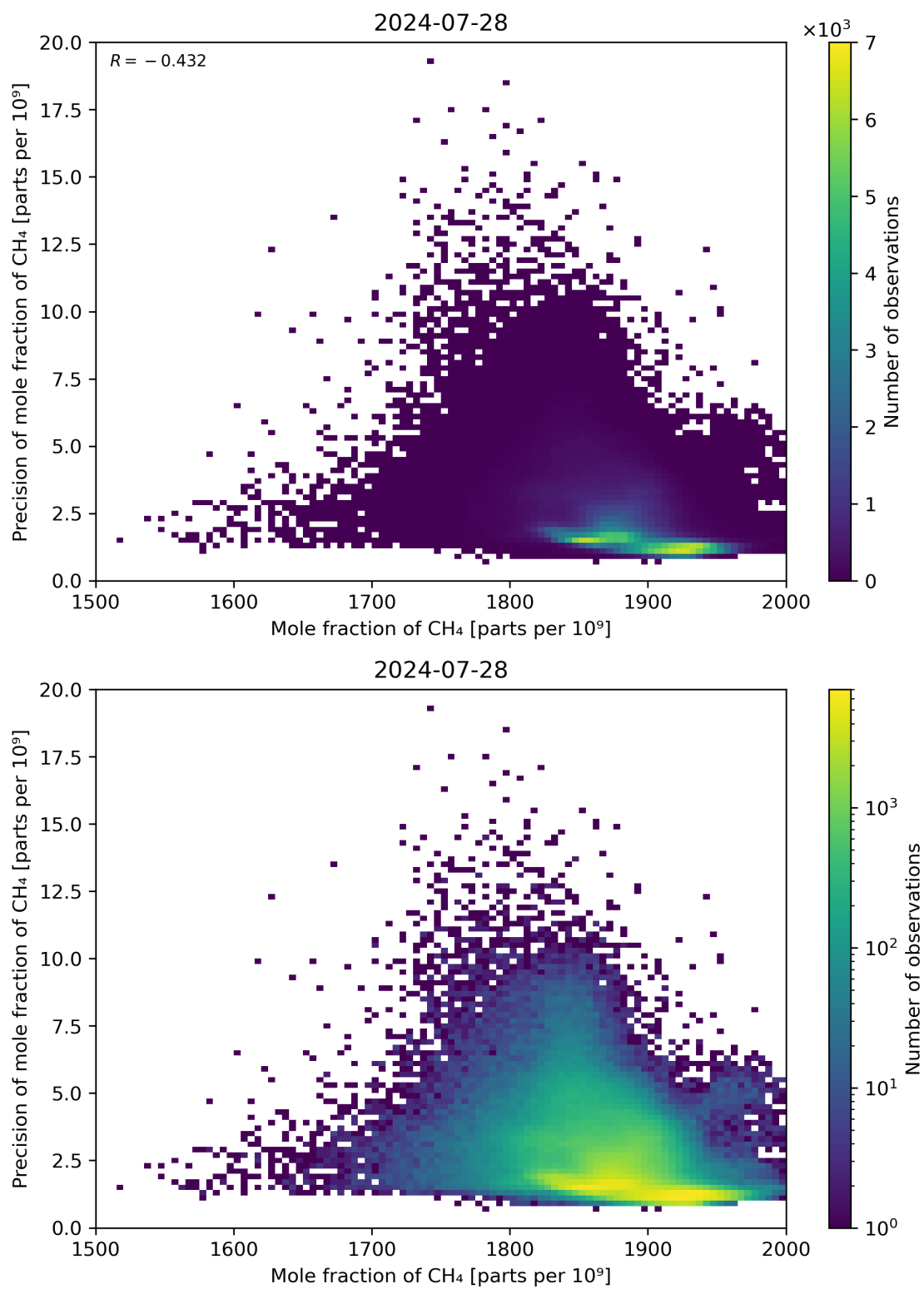
Figure 75: Scatter density plot of “Mole fraction of CH 4 ” against “Precision of mole fraction of CH 4 ” for 2024-07-27 to 2024-07-29.
