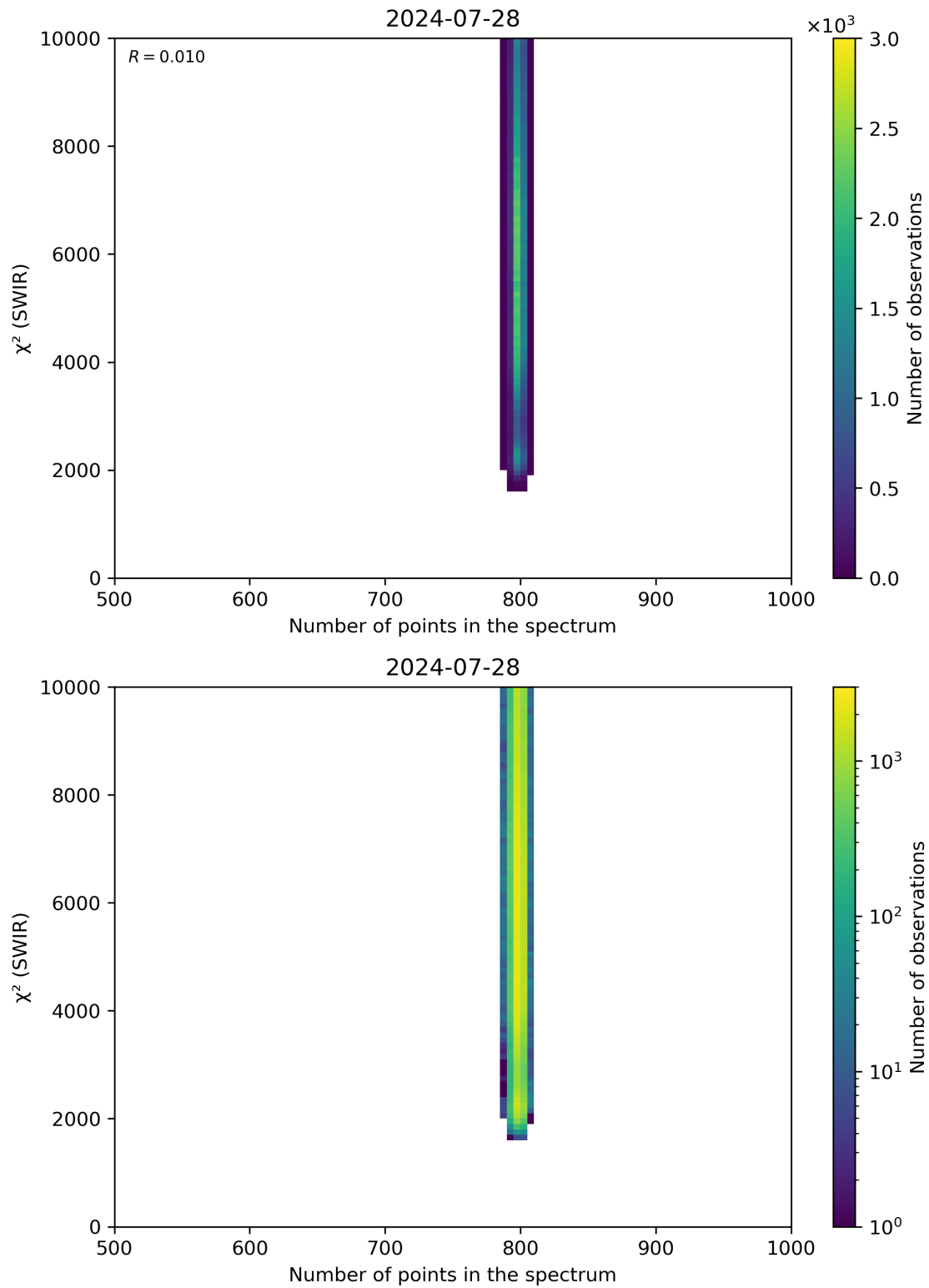
Figure 89: Scatter density plot of “Number of points in the spectrum” against “ \chi^2 (SWIR)” for 2024-07-27 to 2024-07-29.
