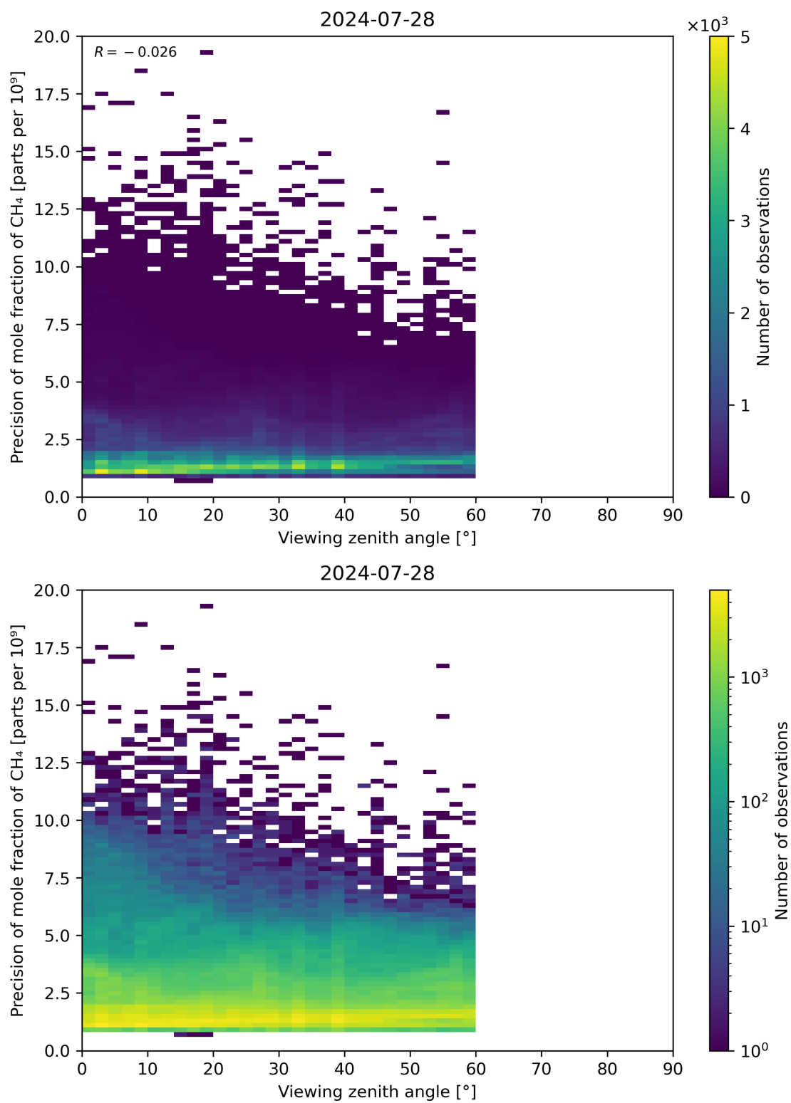
Figure 112: Scatter density plot of “Viewing zenith angle” against “Precision of mole fraction of CH 4 ” for 2024-07-27 to 2024-07-29.
