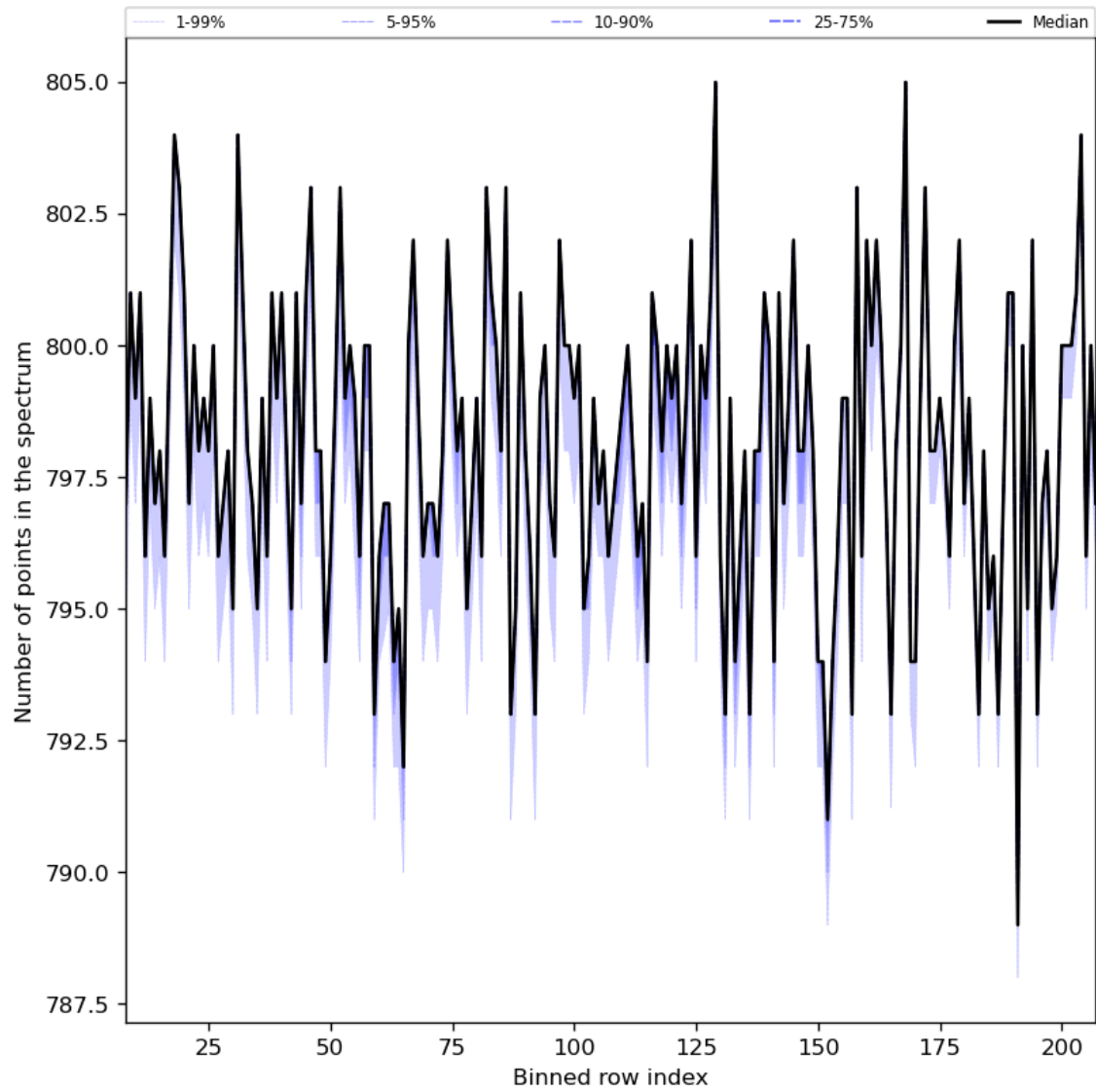
Figure 37: Along track statistics of “Number of points in the spectrum” for 2024-07-27 to 2024-07-29
