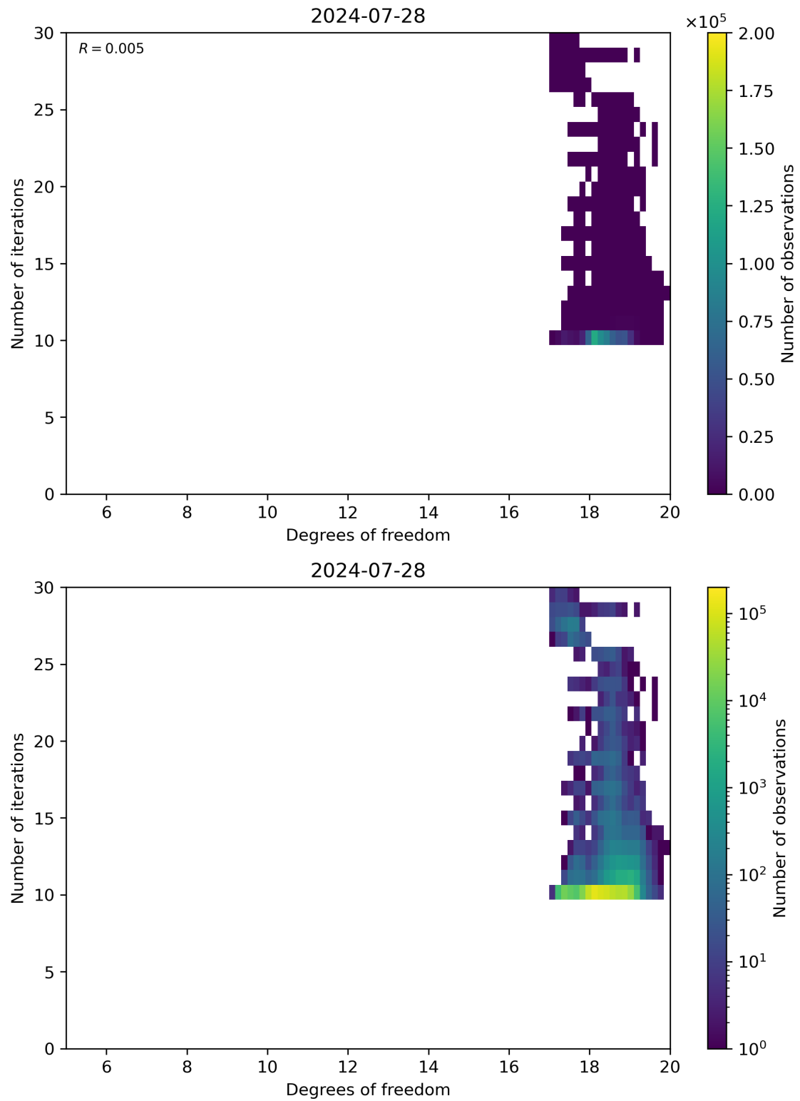
Figure 52: Scatter density plot of “Degrees of freedom” against “Number of iterations” for 2024-07-27 to 2024-07-29.
