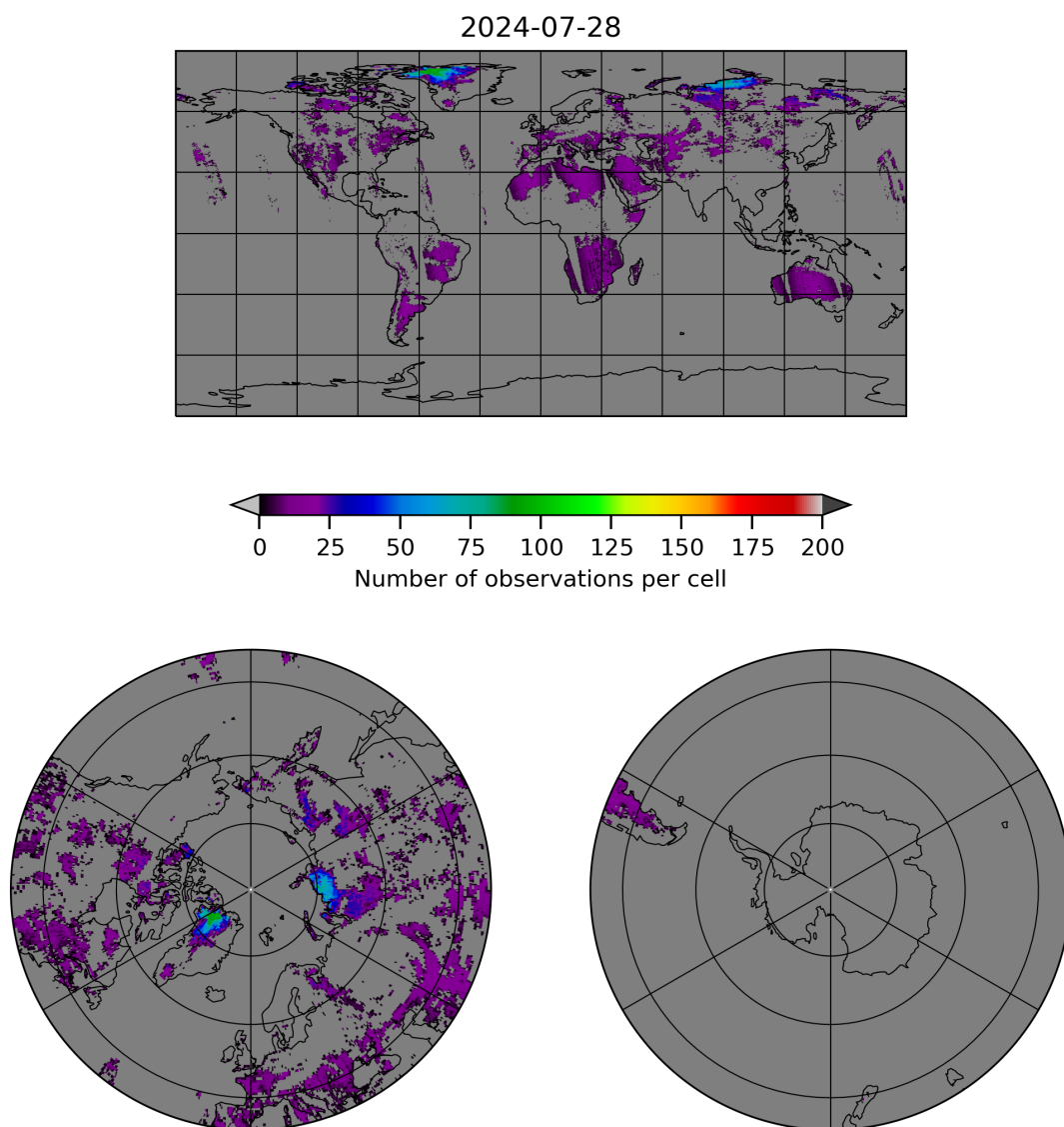
Figure 10: Map of the number of observations for 2024-07-27 to 2024-07-29
