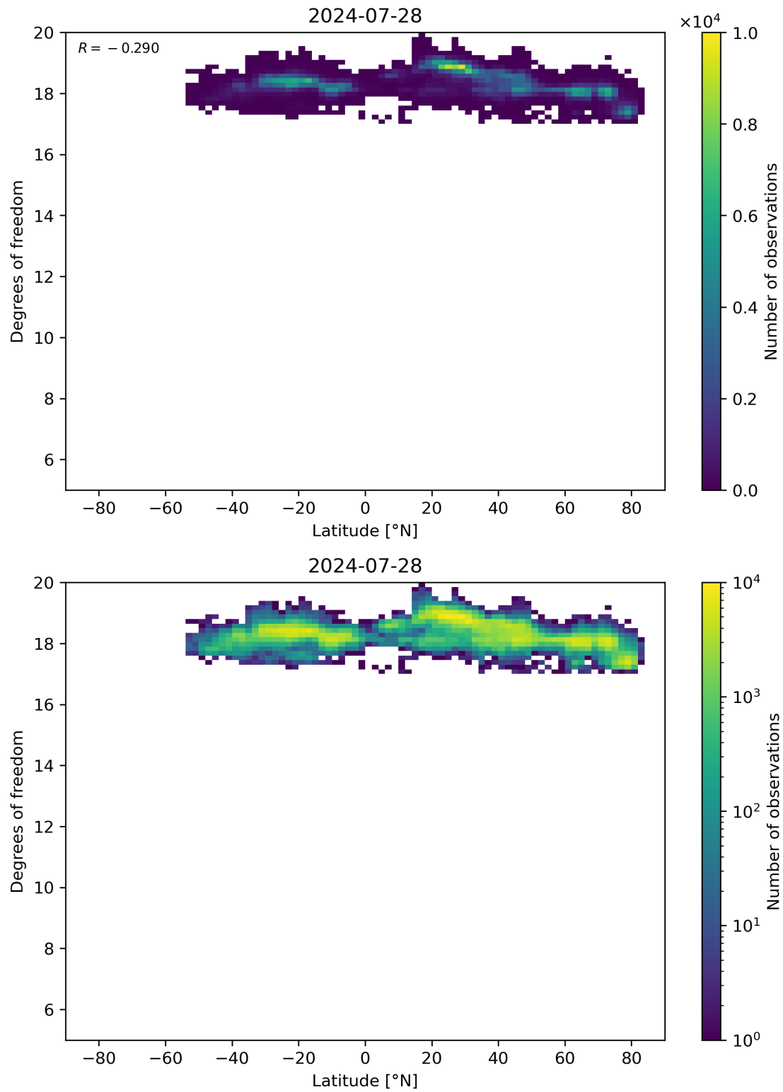
Figure 55: Scatter density plot of “Latitude” against “Degrees of freedom” for 2024-07-27 to 2024-07-29.
