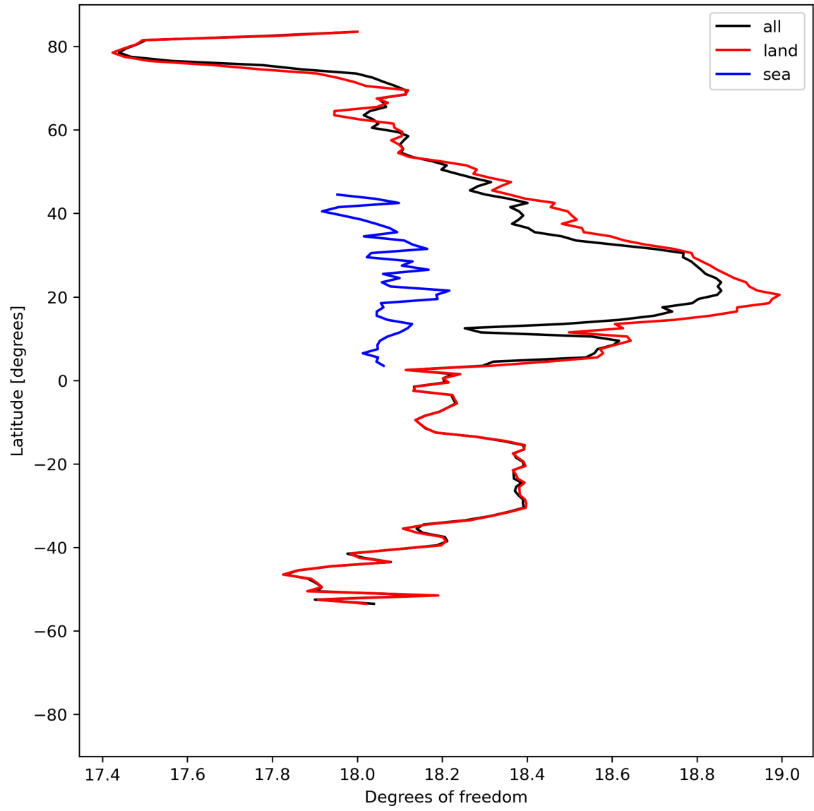
Figure 19: Zonal average of “Degrees of freedom” for 2024-07-27 to 2024-07-29.
