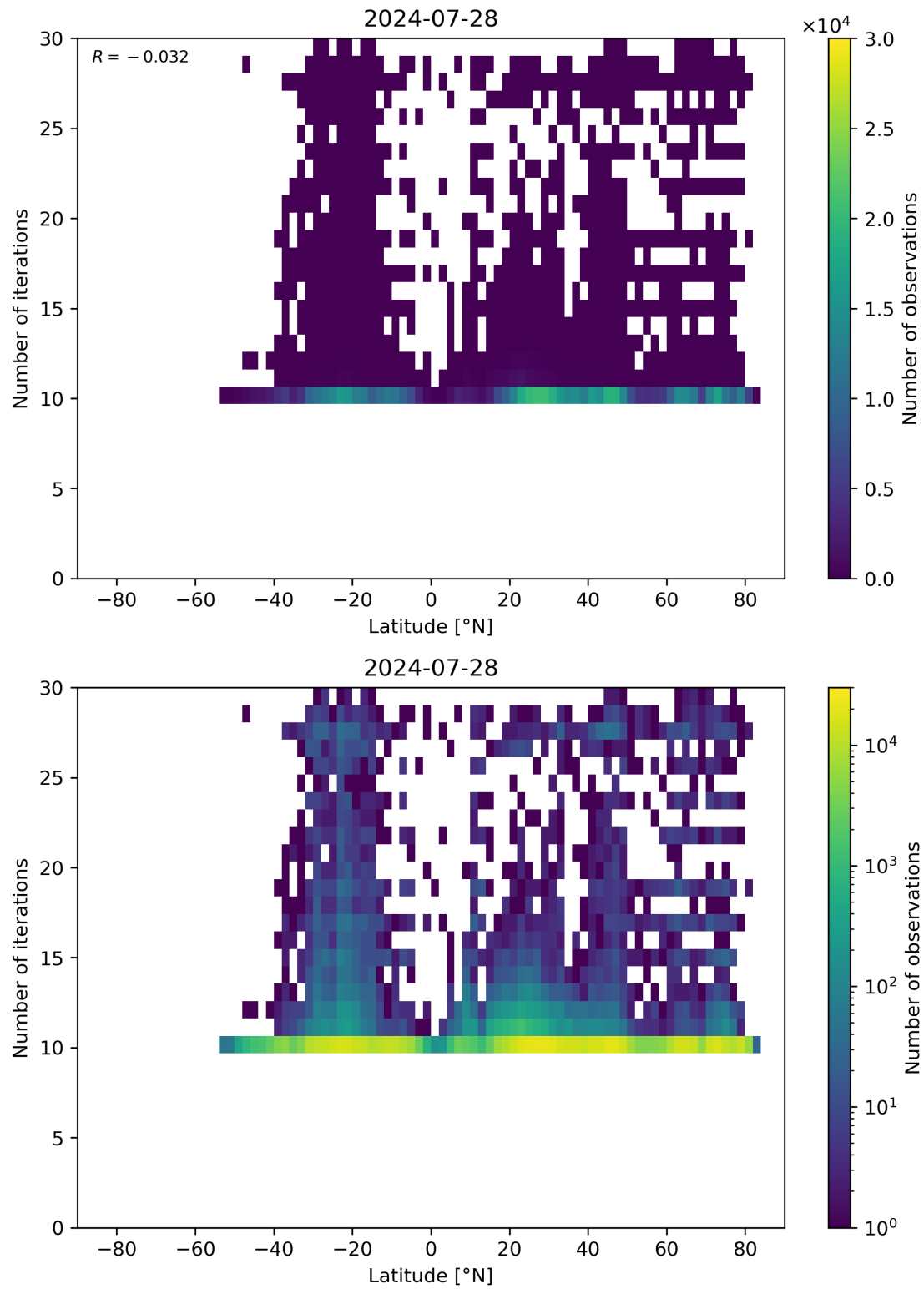
Figure 60: Scatter density plot of “Latitude” against “Number of iterations” for 2024-07-27 to 2024-07-29.
