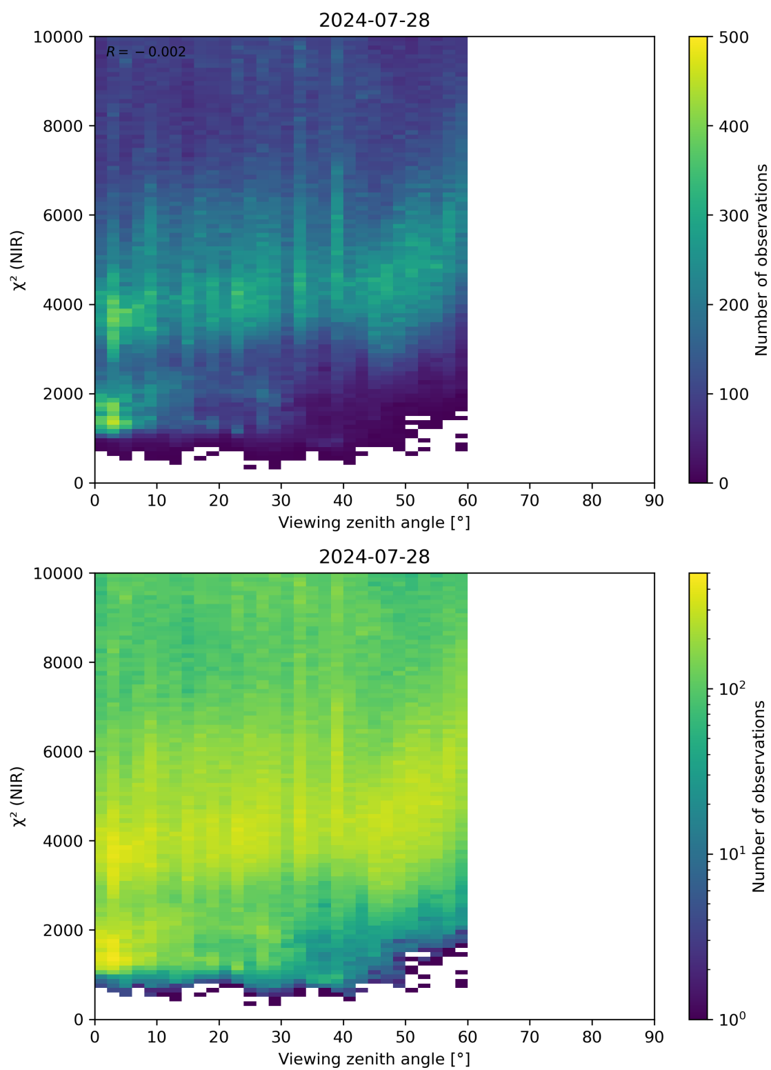
Figure 105: Scatter density plot of “Viewing zenith angle” against “ \chi^2 (NIR)” for 2024-07-27 to 2024-07-29.
