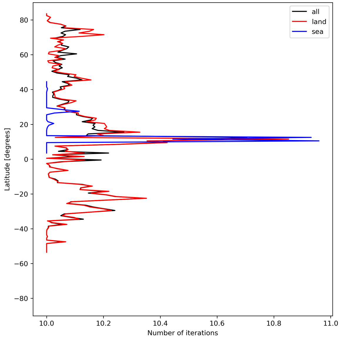
Figure 20: Zonal average of “Number of iterations” for 2024-07-27 to 2024-07-29.
