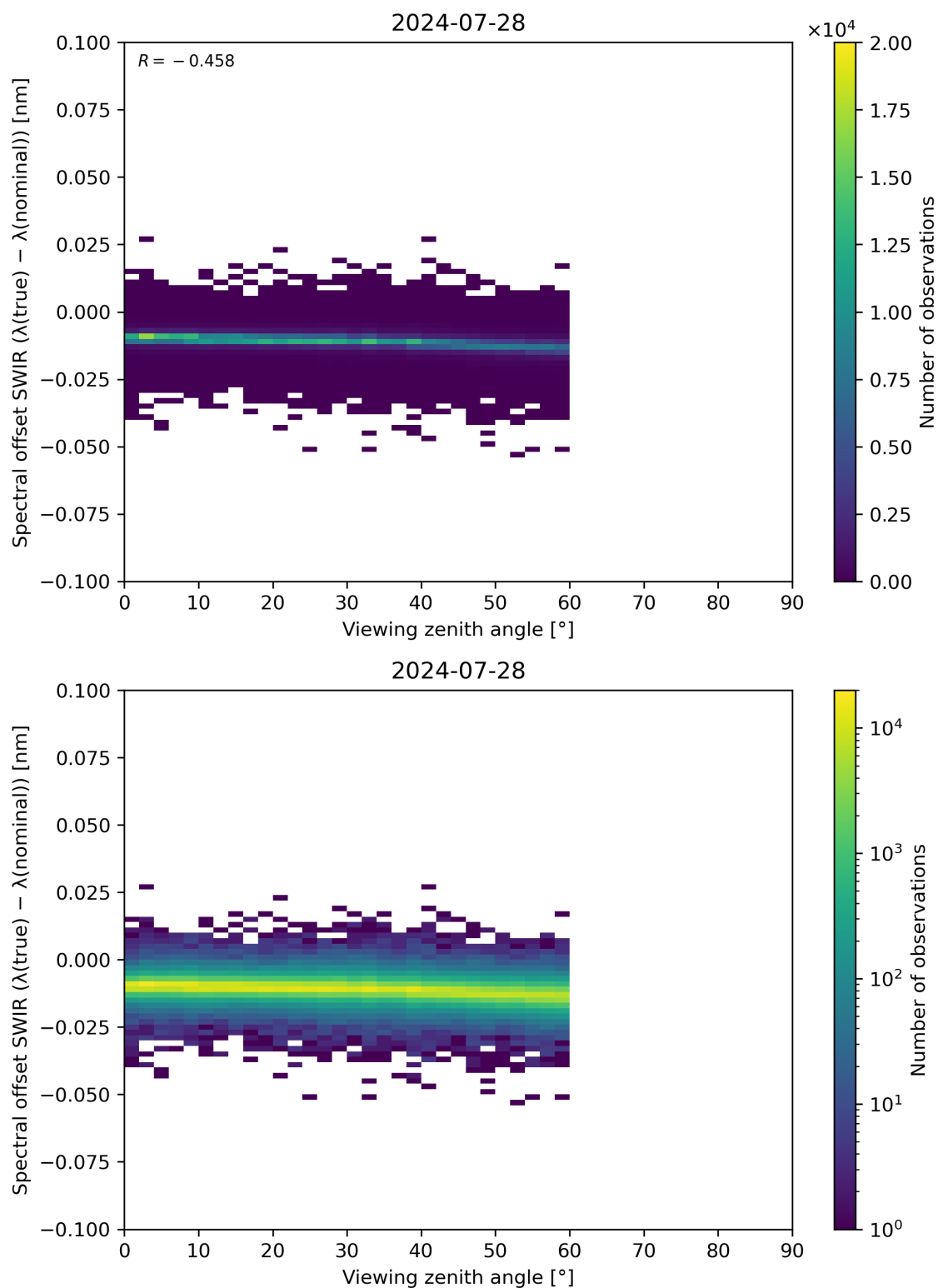
Figure 116: Scatter density plot of “Viewing zenith angle” against “Spectral offset SWIR ( \lambda(\text{true}) - \lambda(\text{nominal}) )” for 2024-07-27 to 2024-07-29.
