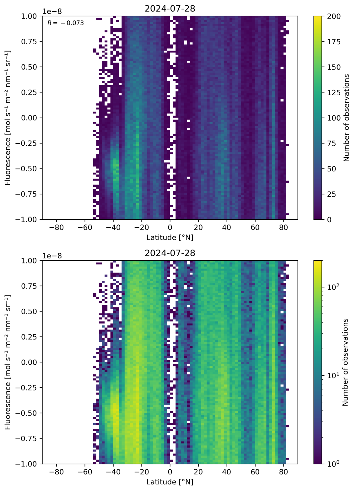
Figure 56: Scatter density plot of “Latitude” against “Fluorescence” for 2024-07-27 to 2024-07-29.
