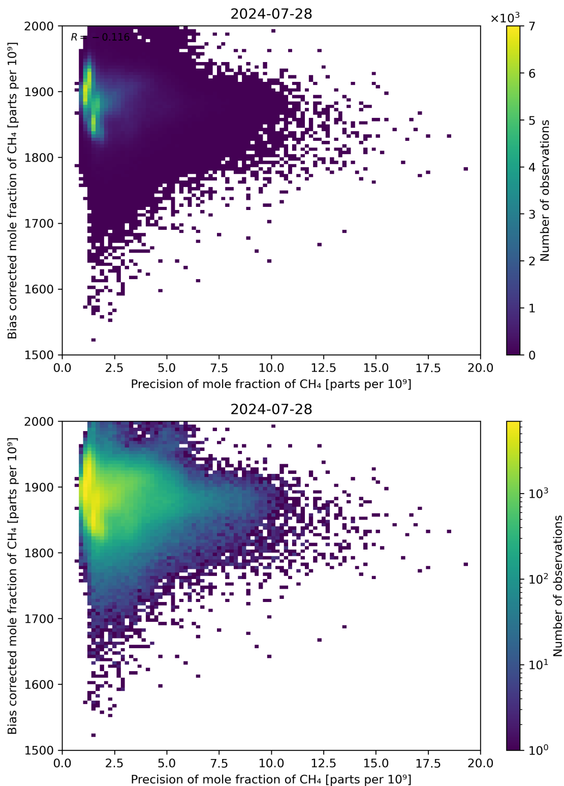
Figure 82: Scatter density plot of “Precision of mole fraction of CH 4 ” against “Bias corrected mole fraction of CH 4 ” for 2024-07-27 to 2024-07-29.
