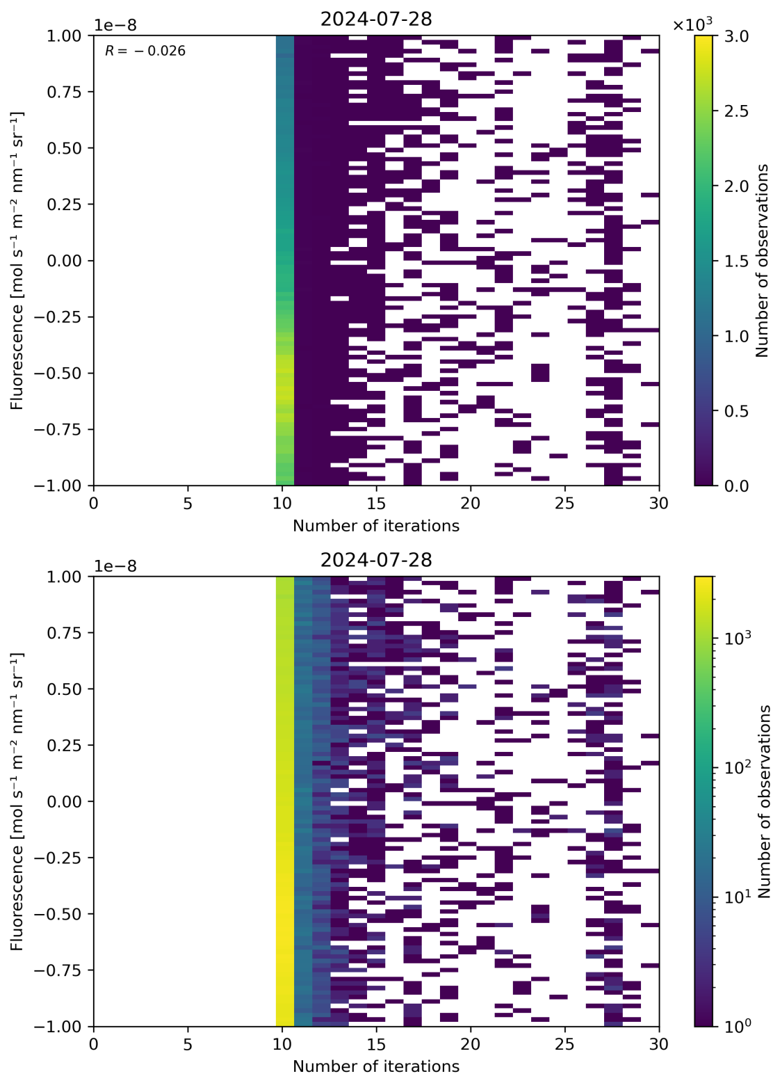
Figure 87: Scatter density plot of “Number of iterations” against “Fluorescence” for 2024-07-27 to 2024-07-29.
