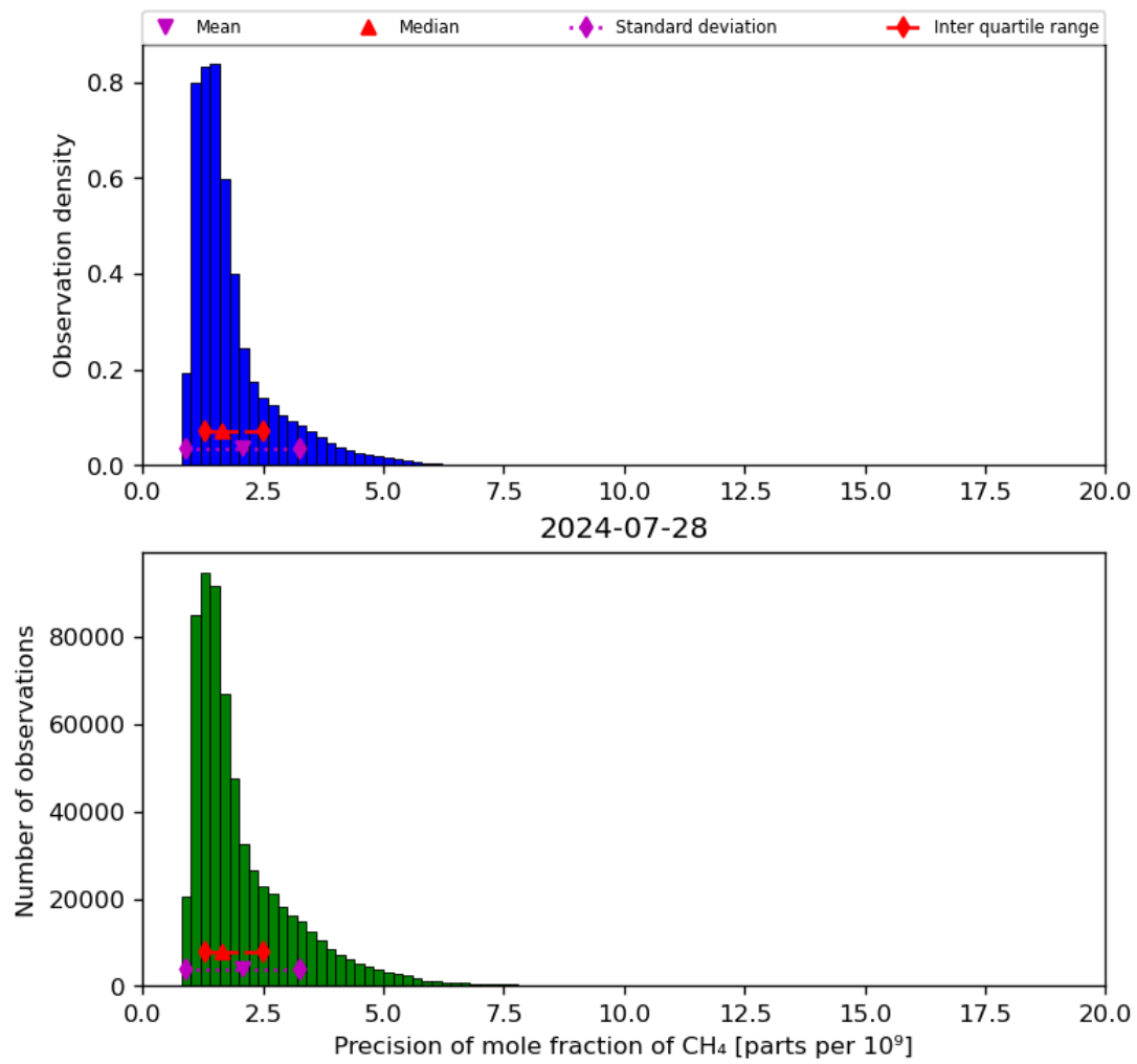
Figure 24: Histogram of “Precision of mole fraction of CH 4 ” for 2024-07-27 to 2024-07-29
