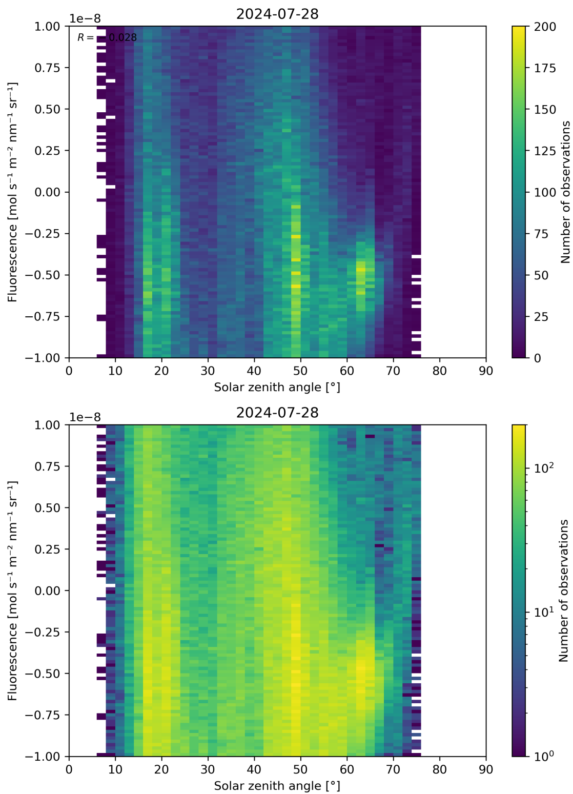
Figure 97: Scatter density plot of “Solar zenith angle” against “Fluorescence” for 2024-07-27 to 2024-07-29.
