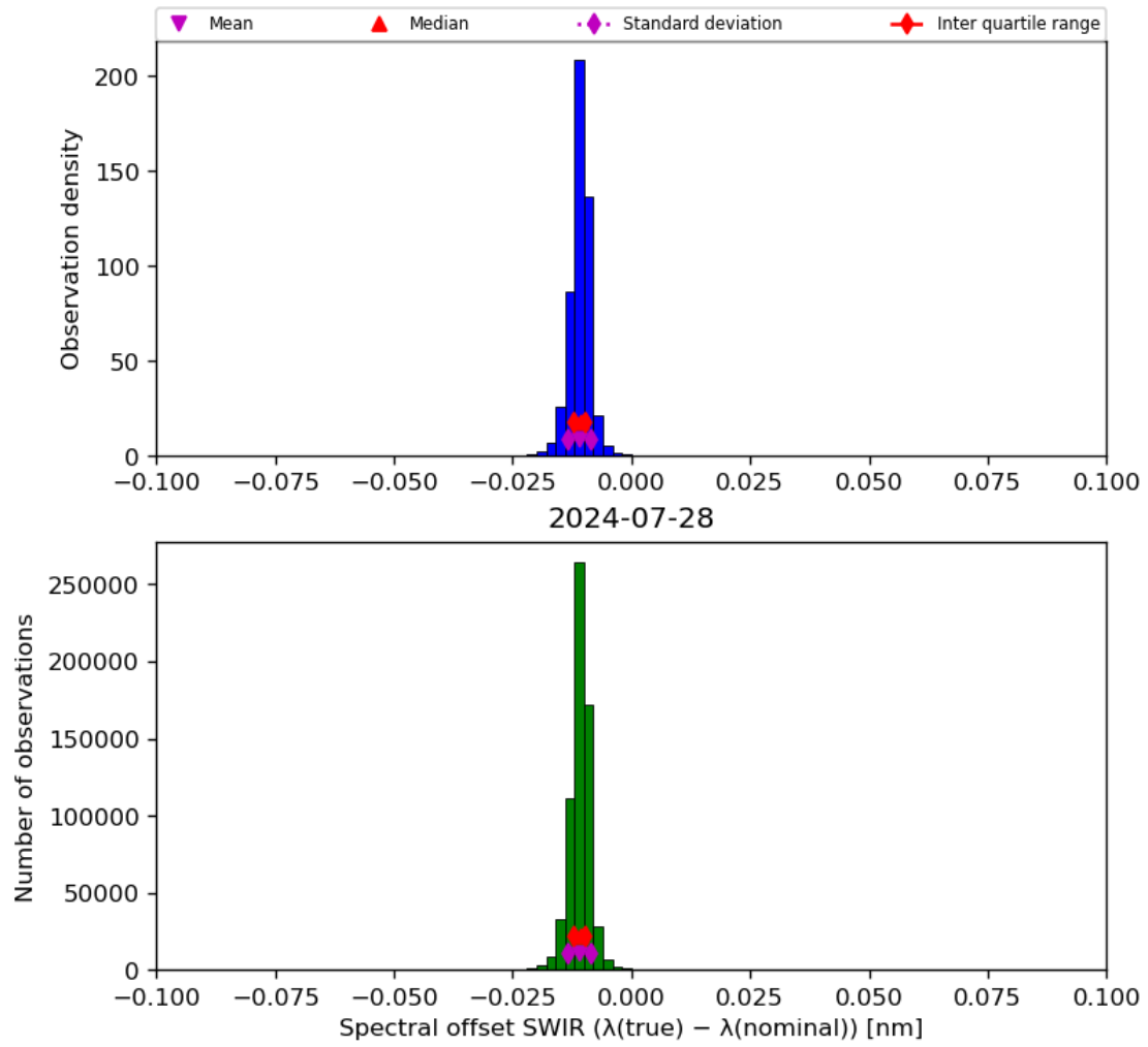
Figure 27: Histogram of “Spectral offset SWIR ( \lambda(\text{true}) - \lambda(\text{nominal}) )” for 2024-07-27 to 2024-07-29
