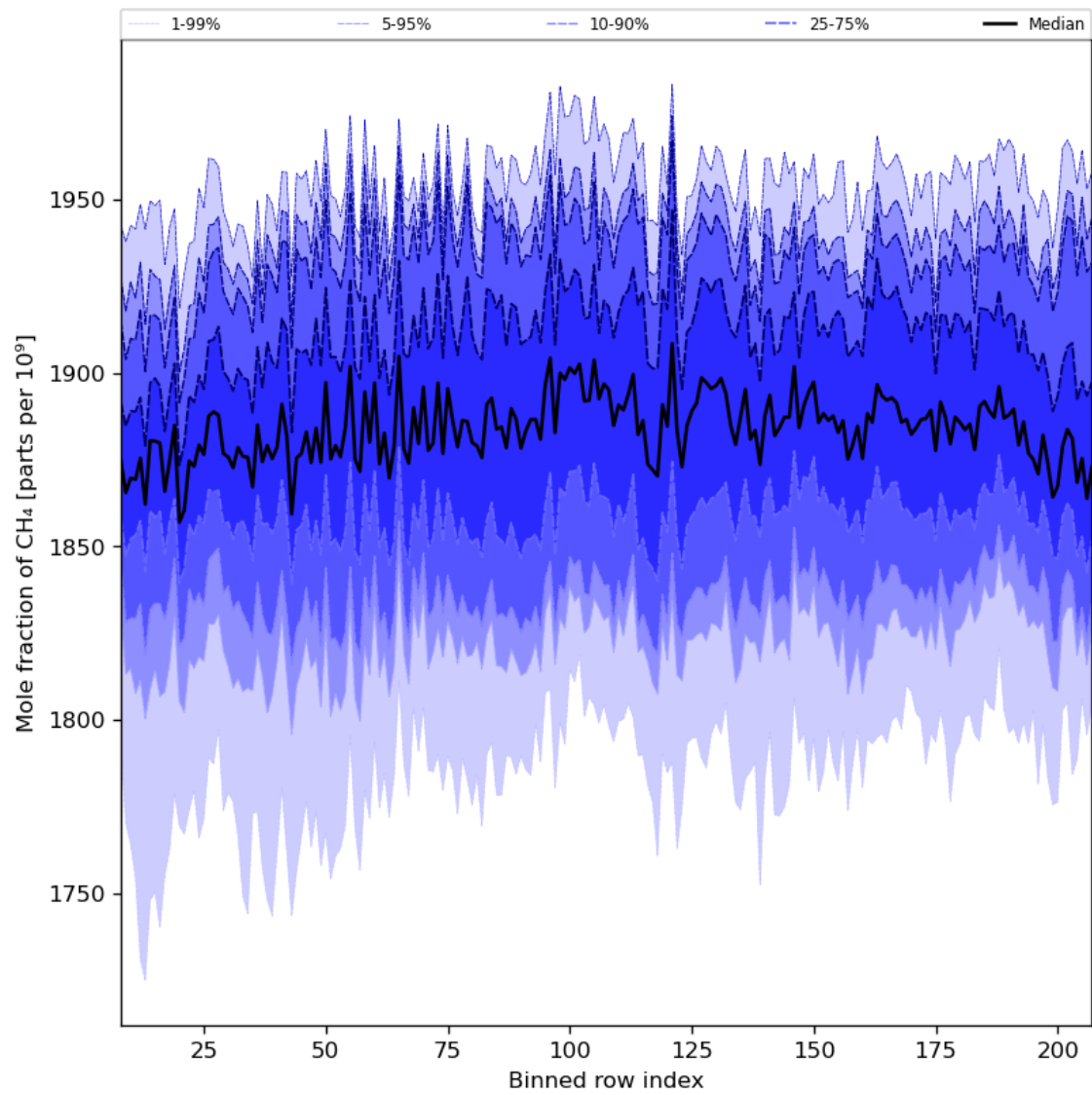
Figure 34: Along track statistics of “Mole fraction of CH 4 ” for 2024-07-27 to 2024-07-29
