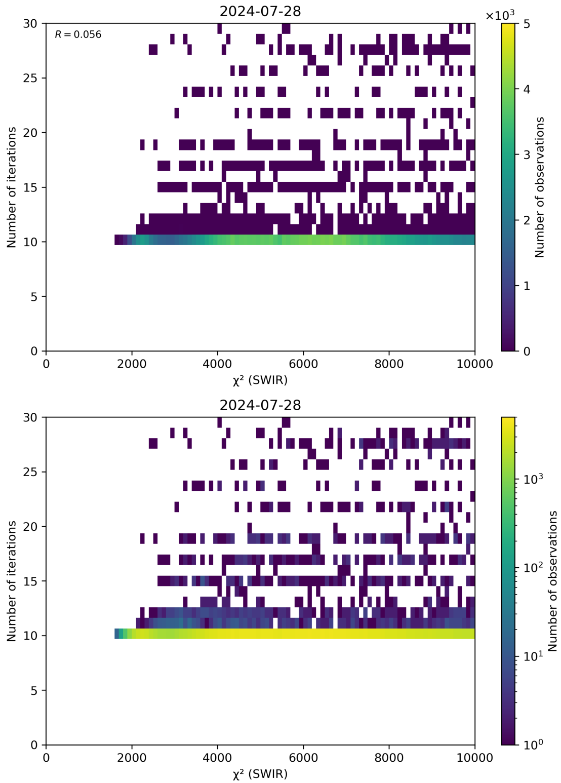
Figure 50: Scatter density plot of “ \chi^2 (SWIR)” against “Number of iterations” for 2024-07-27 to 2024-07-29.
