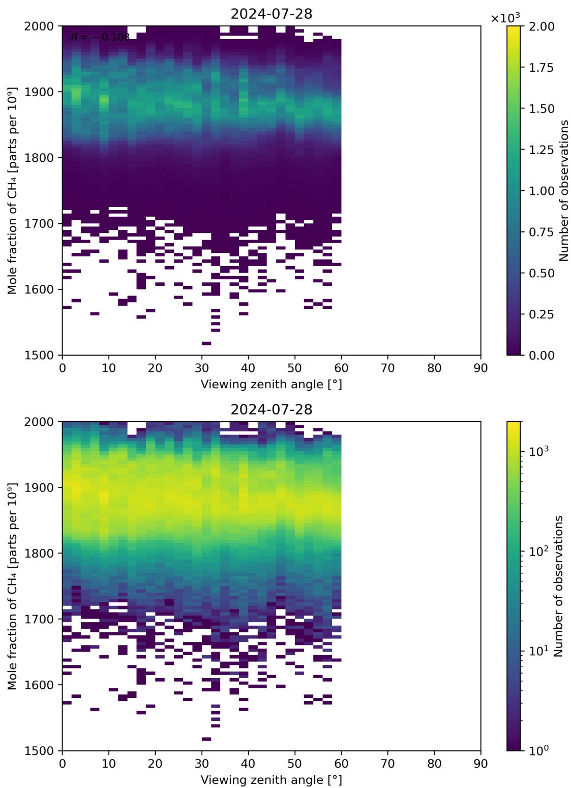
Figure 110: Scatter density plot of “Viewing zenith angle” against “Mole fraction of CH 4 ” for 2024-07-27 to 2024-07-29.
