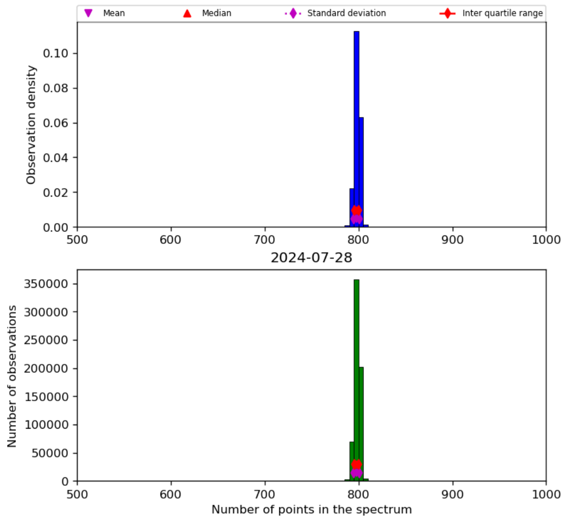
Figure 26: Histogram of “Number of points in the spectrum” for 2024-07-27 to 2024-07-29
