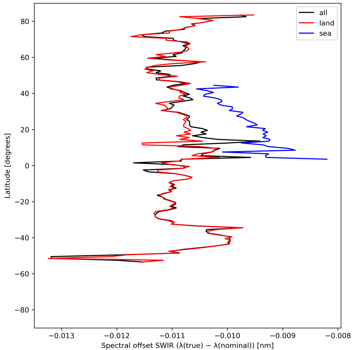
Figure 16: Zonal average of “Spectral offset SWIR ( \lambda(\text{true}) - \lambda(\text{nominal}) )” for 2024-07-27 to 2024-07-29.
