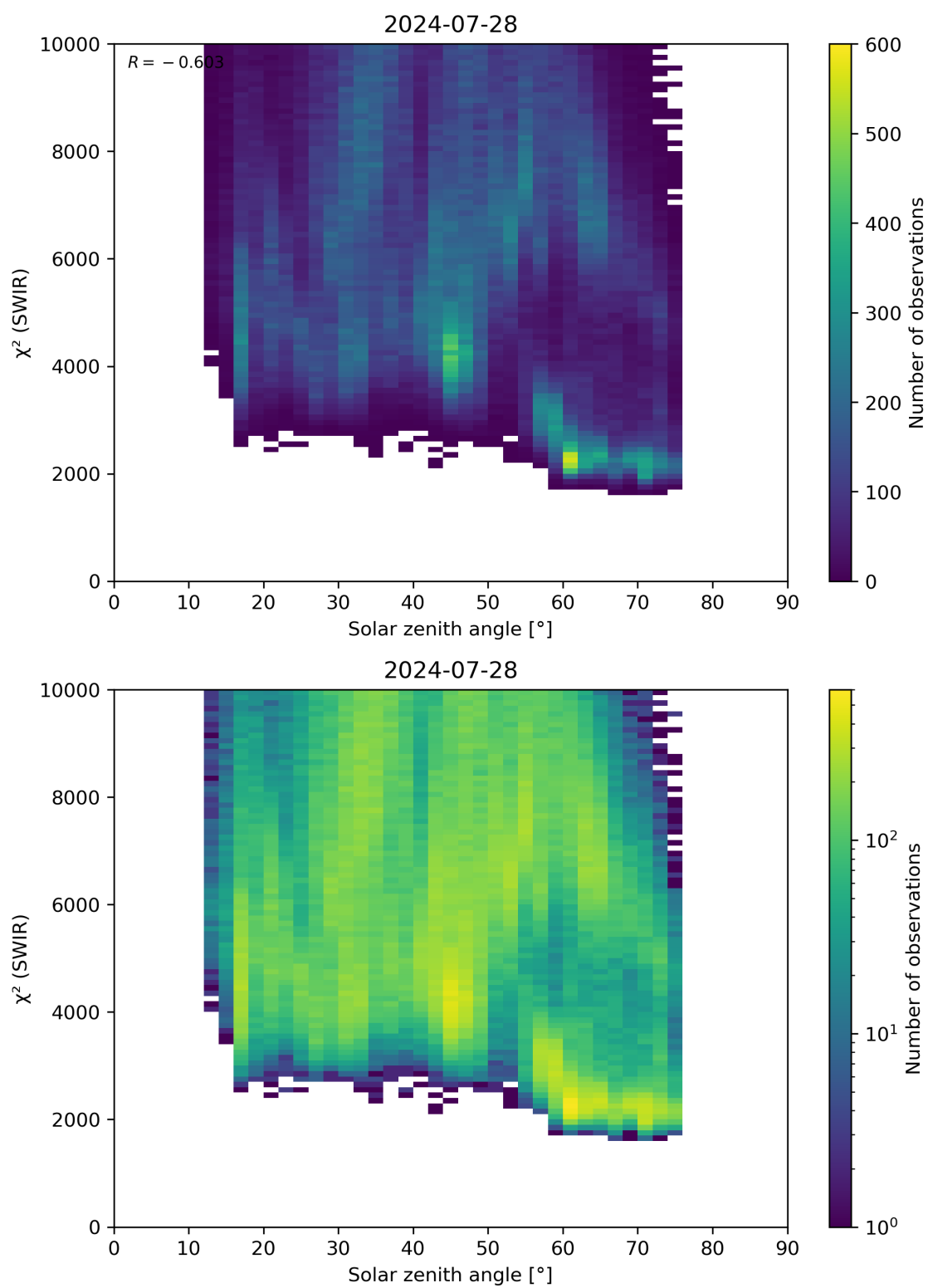
Figure 95: Scatter density plot of “Solar zenith angle” against “ \chi^2 (SWIR)” for 2024-07-27 to 2024-07-29.
