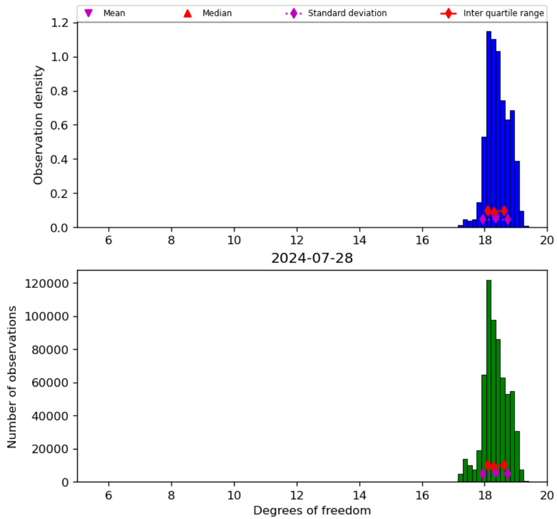
Figure 30: Histogram of “Degrees of freedom” for 2024-07-27 to 2024-07-29
