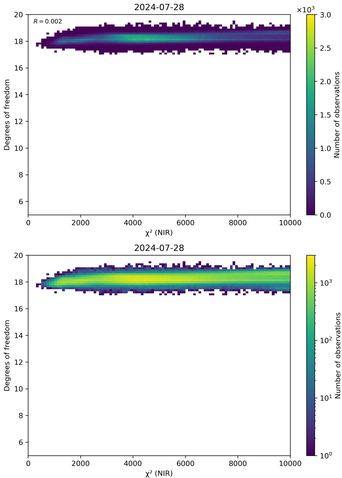
Figure 44: Scatter density plot of “ \chi^2 (NIR)” against “Degrees of freedom” for 2024-07-27 to 2024-07-29.
