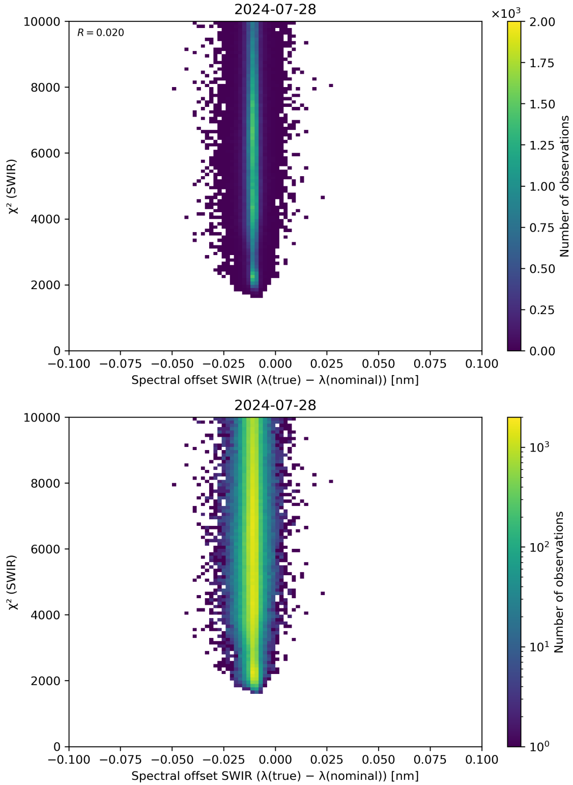
Figure 118: Scatter density plot of “Spectral offset SWIR ( \lambda(\text{true}) - \lambda(\text{nominal}) )” against “ \chi^2 (SWIR)” for 2024-07-27 to 2024-07-29.
