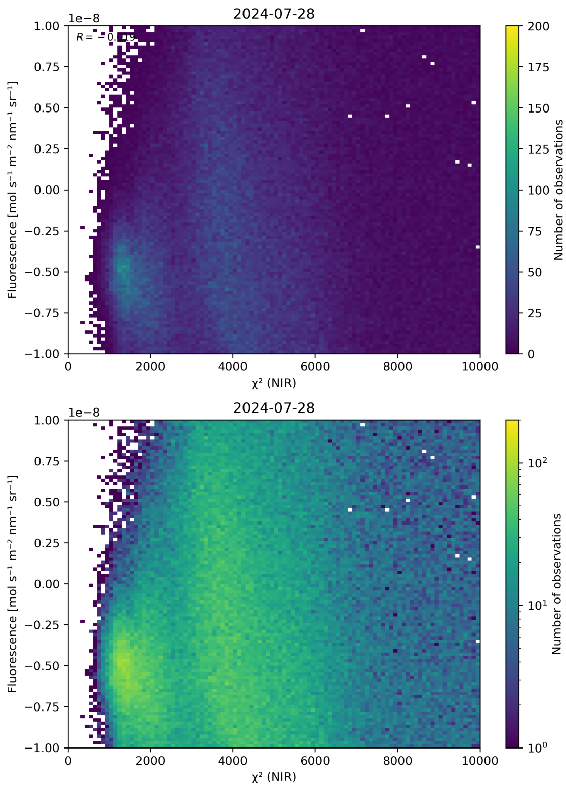
Figure 45: Scatter density plot of “ \chi^2 (NIR)” against “Fluorescence” for 2024-07-27 to 2024-07-29.
