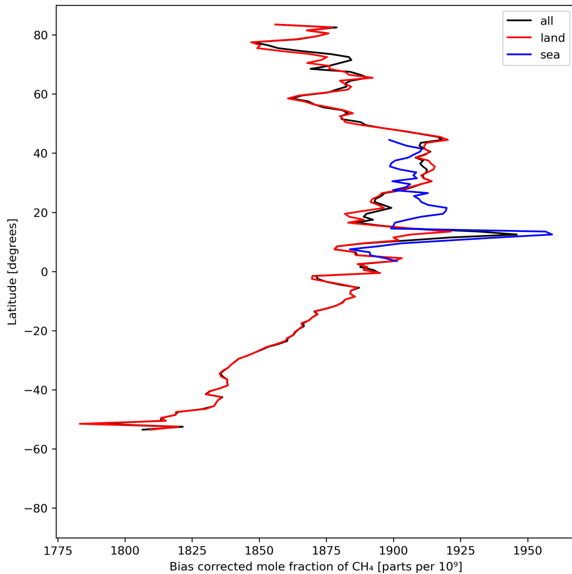
Figure 14: Zonal average of “Bias corrected mole fraction of CH 4 ” for 2024-07-27 to 2024-07-29.
