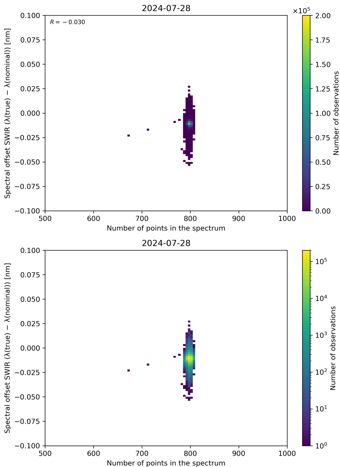
Figure 93: Scatter density plot of “Number of points in the spectrum” against “Spectral offset SWIR ( \lambda(\text{true}) - \lambda(\text{nominal}) )” for 2024-07-27 to 2024-07-29.
