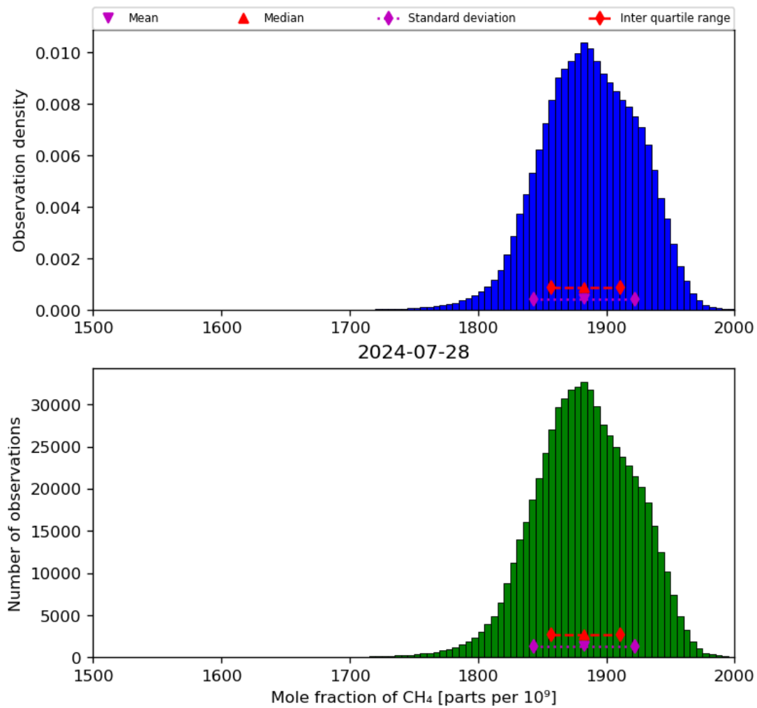
Figure 23: Histogram of “Mole fraction of CH 4 ” for 2024-07-27 to 2024-07-29
