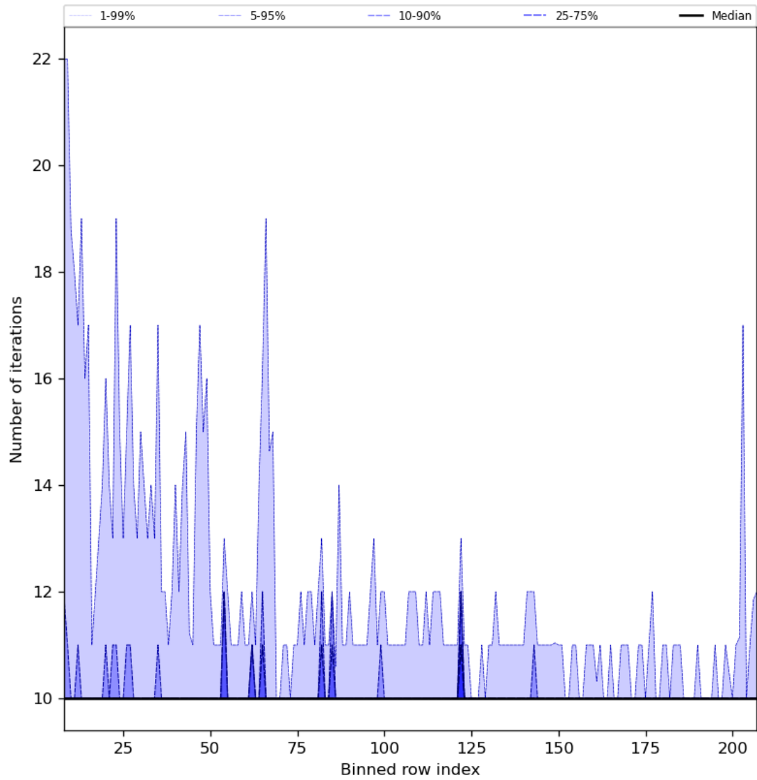
Figure 42: Along track statistics of “Number of iterations” for 2024-07-27 to 2024-07-29
