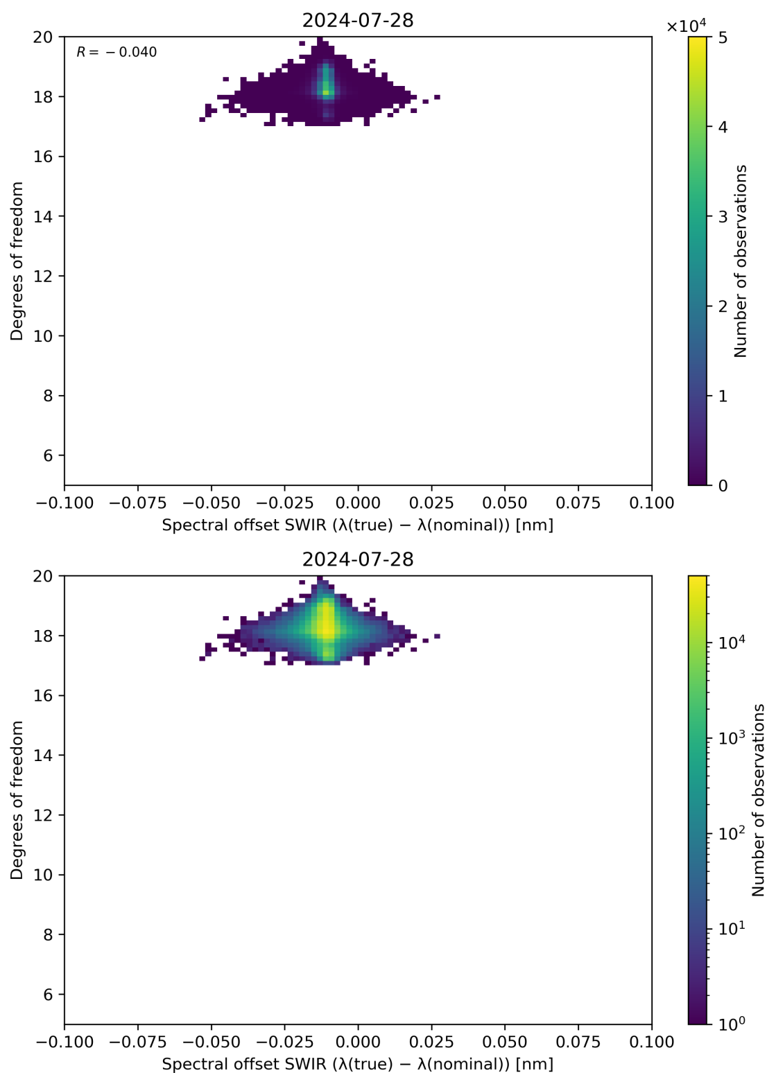
Figure 119: Scatter density plot of “Spectral offset SWIR ( \lambda(\text{true}) - \lambda(\text{nominal}) )” against “Degrees of freedom” for 2024-07-27 to 2024-07-29.
