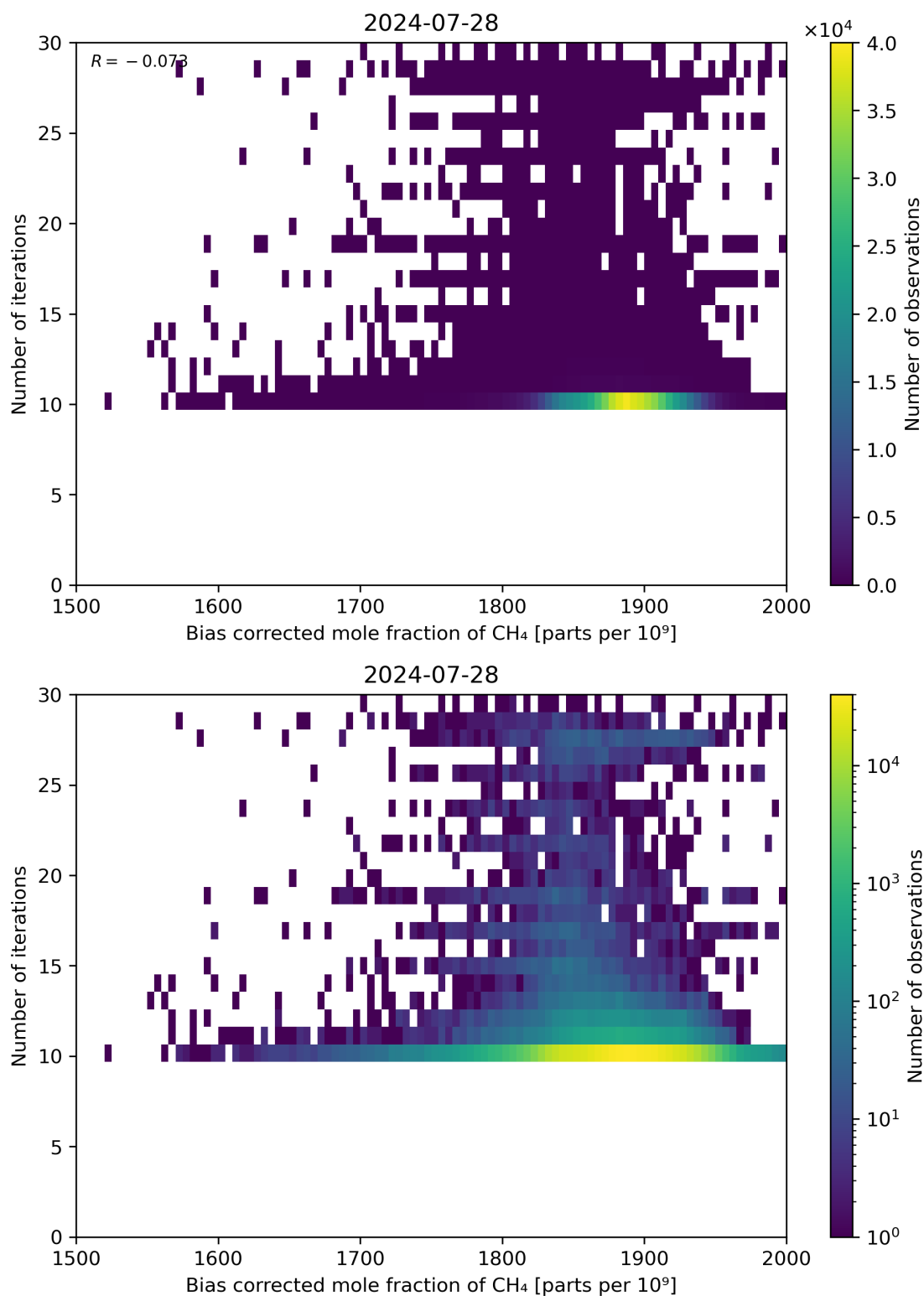
Figure 67: Scatter density plot of “Bias corrected mole fraction of CH 4 ” against “Number of iterations” for 2024-07-27 to 2024-07-29.
