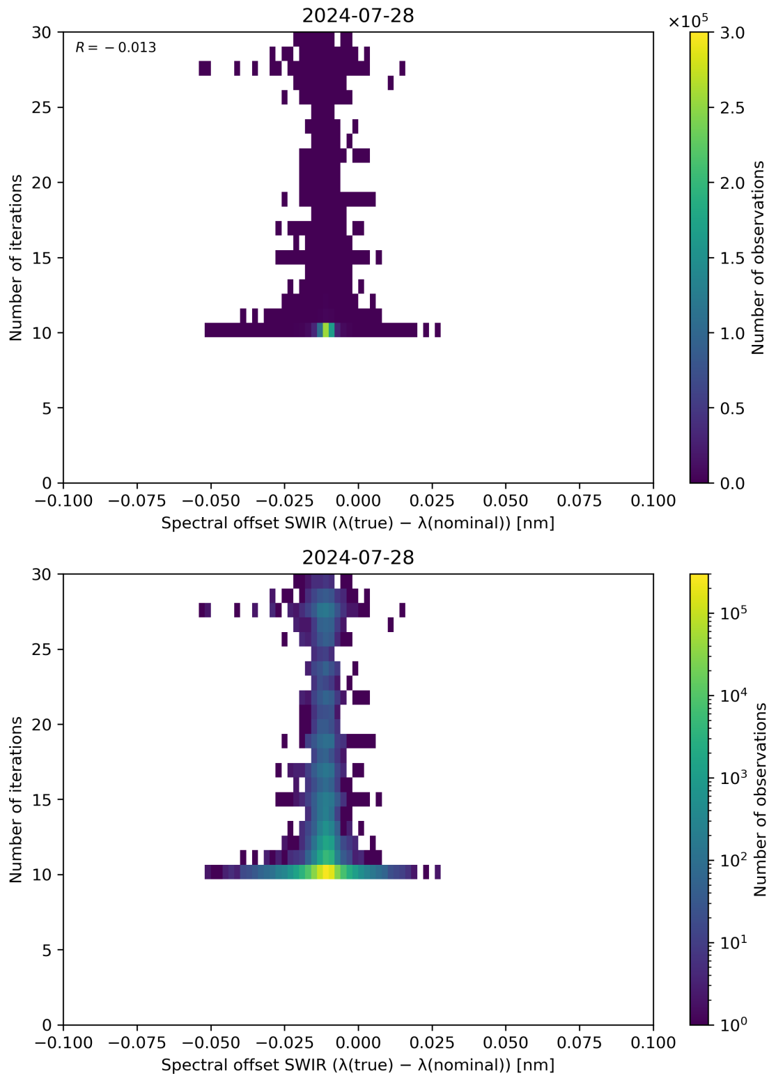
Figure 121: Scatter density plot of “Spectral offset SWIR ( \lambda(\text{true}) - \lambda(\text{nominal}) )” against “Number of iterations” for 2024-07-27 to 2024-07-29.
