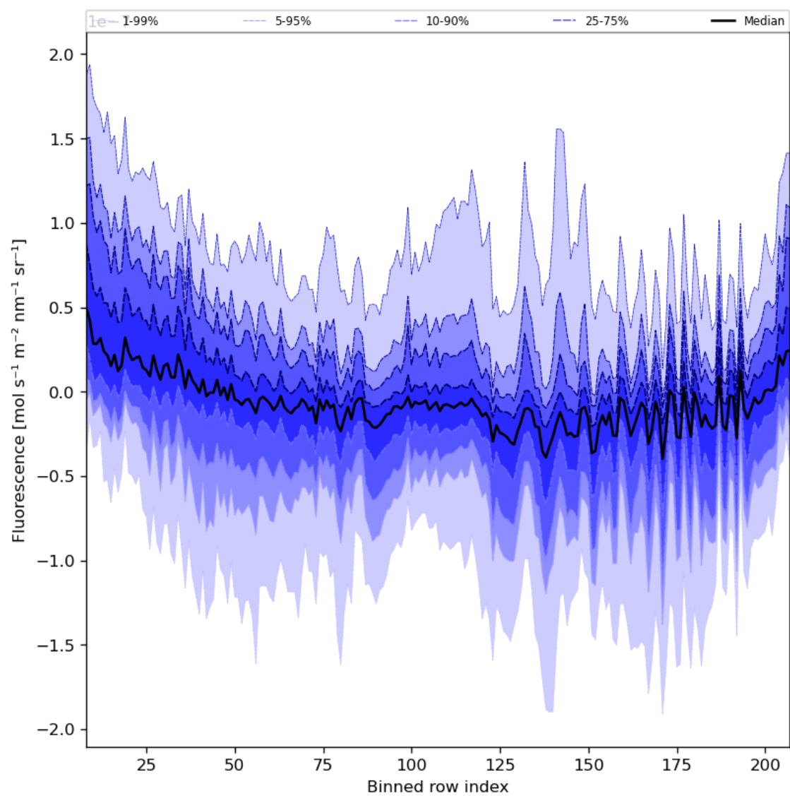
Figure 43: Along track statistics of “Fluorescence” for 2024-07-27 to 2024-07-29
