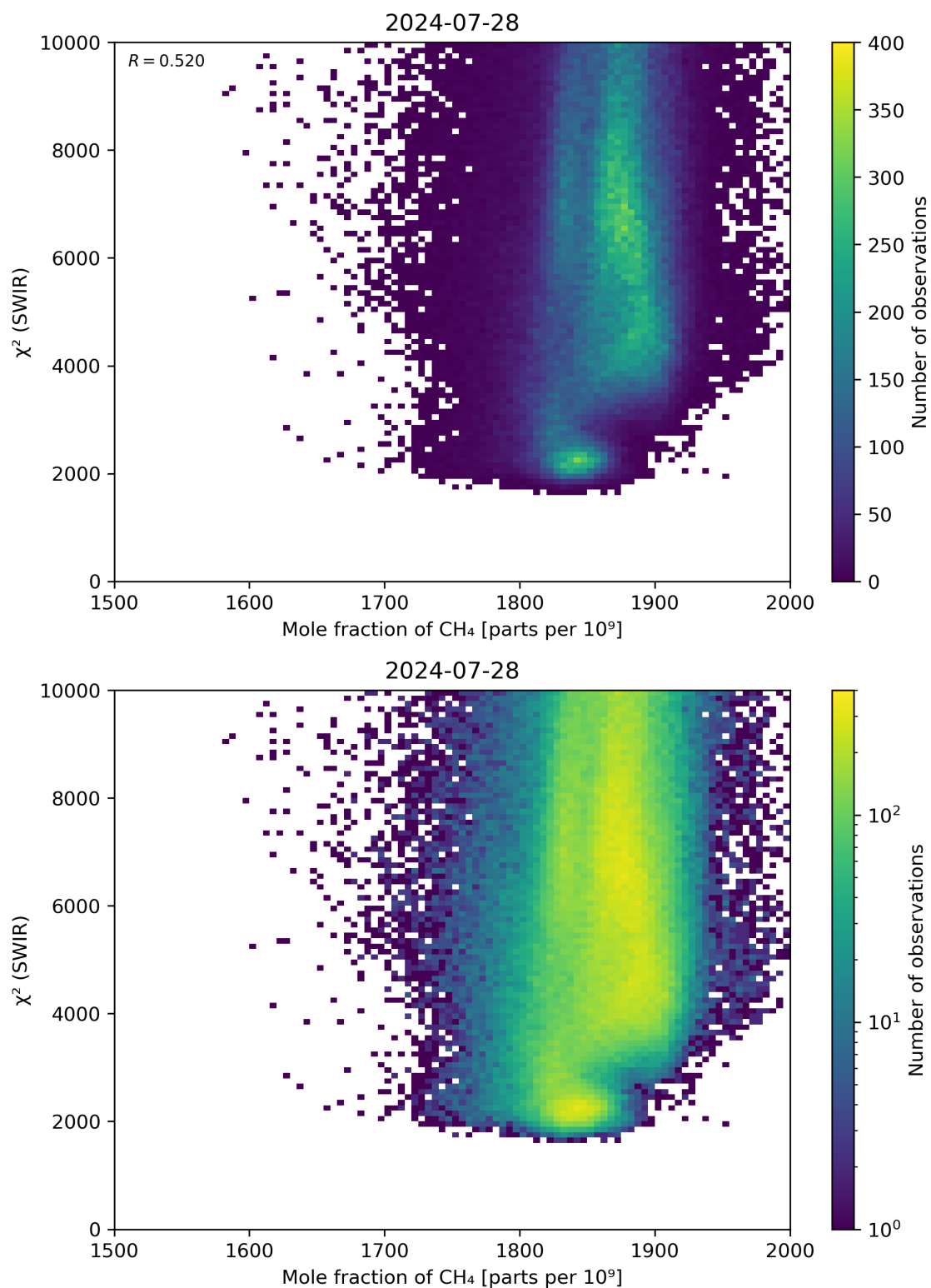
Figure 71: Scatter density plot of “Mole fraction of \text{CH}_4 ” against “ \chi^2 (SWIR)” for 2024-07-27 to 2024-07-29.
