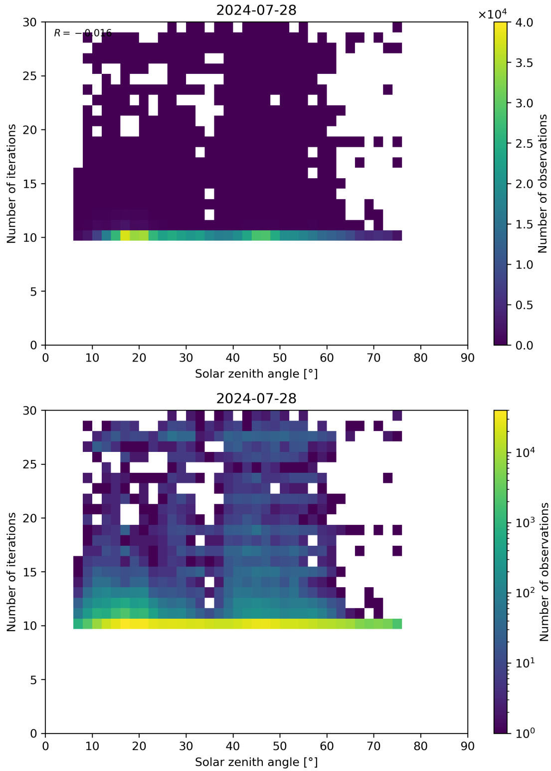
Figure 102: Scatter density plot of “Solar zenith angle” against “Number of iterations” for 2024-07-27 to 2024-07-29.
