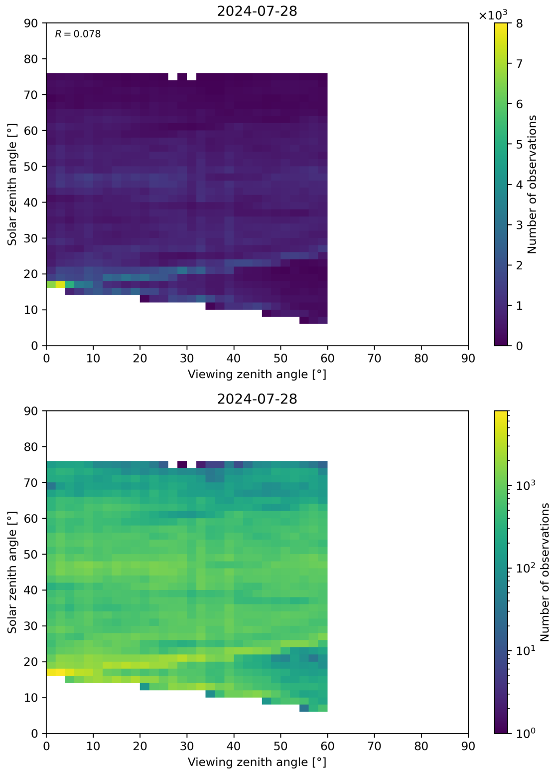
Figure 115: Scatter density plot of “Viewing zenith angle” against “Solar zenith angle” for 2024-07-27 to 2024-07-29.
