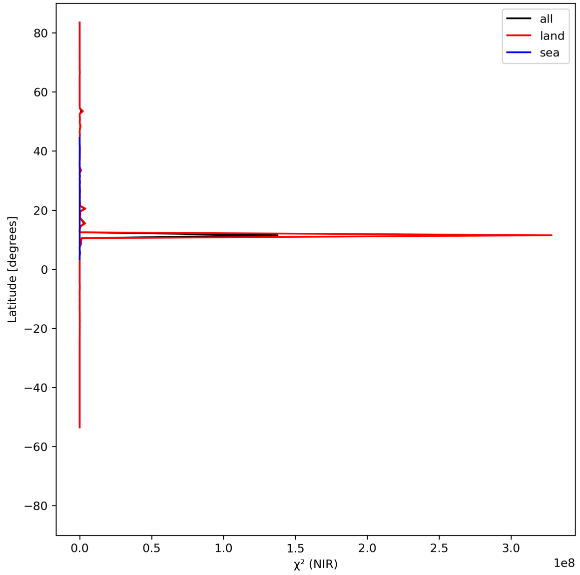
Figure 18: Zonal average of “ \chi^2 (NIR)” for 2024-07-27 to 2024-07-29.
