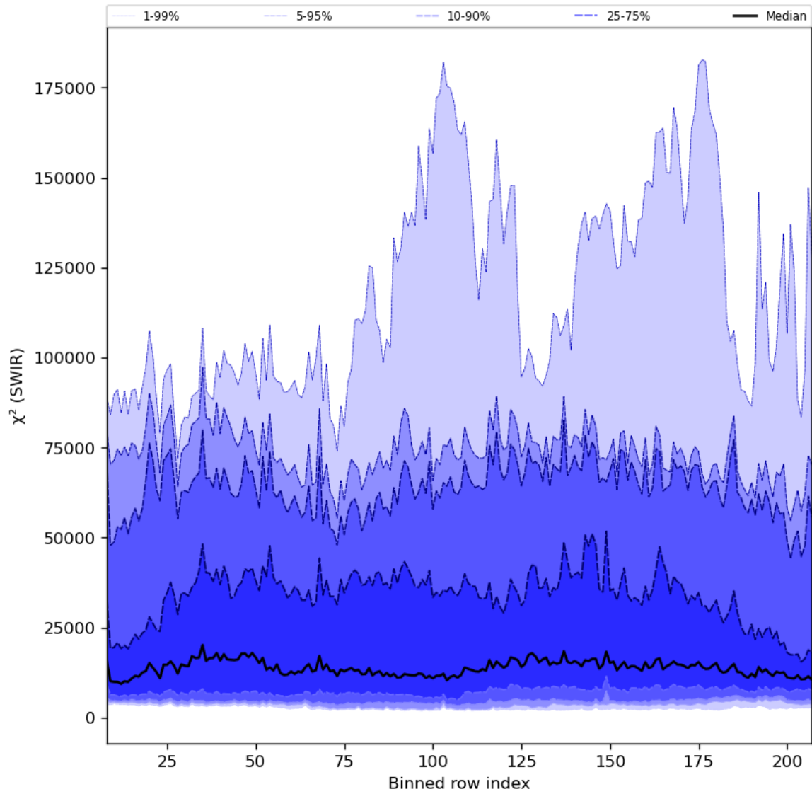
Figure 39: Along track statistics of " \chi^2 (SWIR)" for 2024-07-27 to 2024-07-29
