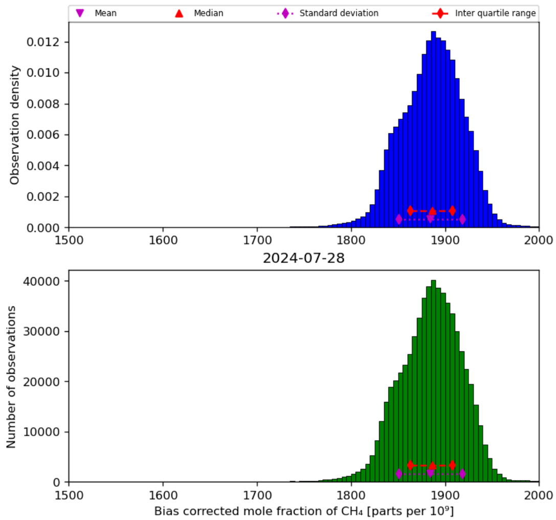
Figure 25: Histogram of “Bias corrected mole fraction of CH 4 ” for 2024-07-27 to 2024-07-29
