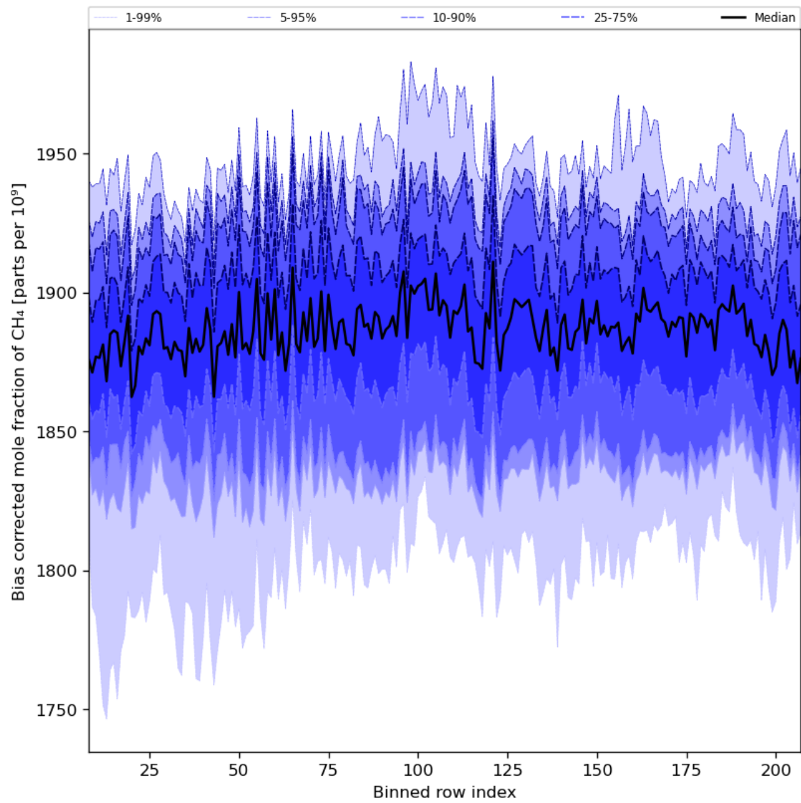
Figure 36: Along track statistics of “Bias corrected mole fraction of CH 4 ” for 2024-07-27 to 2024-07-29
