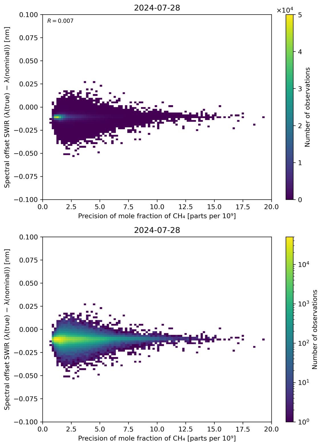
Figure 85: Scatter density plot of “Precision of mole fraction of CH 4 ” against “Spectral offset SWIR ( \lambda(\text{true}) - \lambda(\text{nominal}) )” for 2024-07-27 to 2024-07-29.
