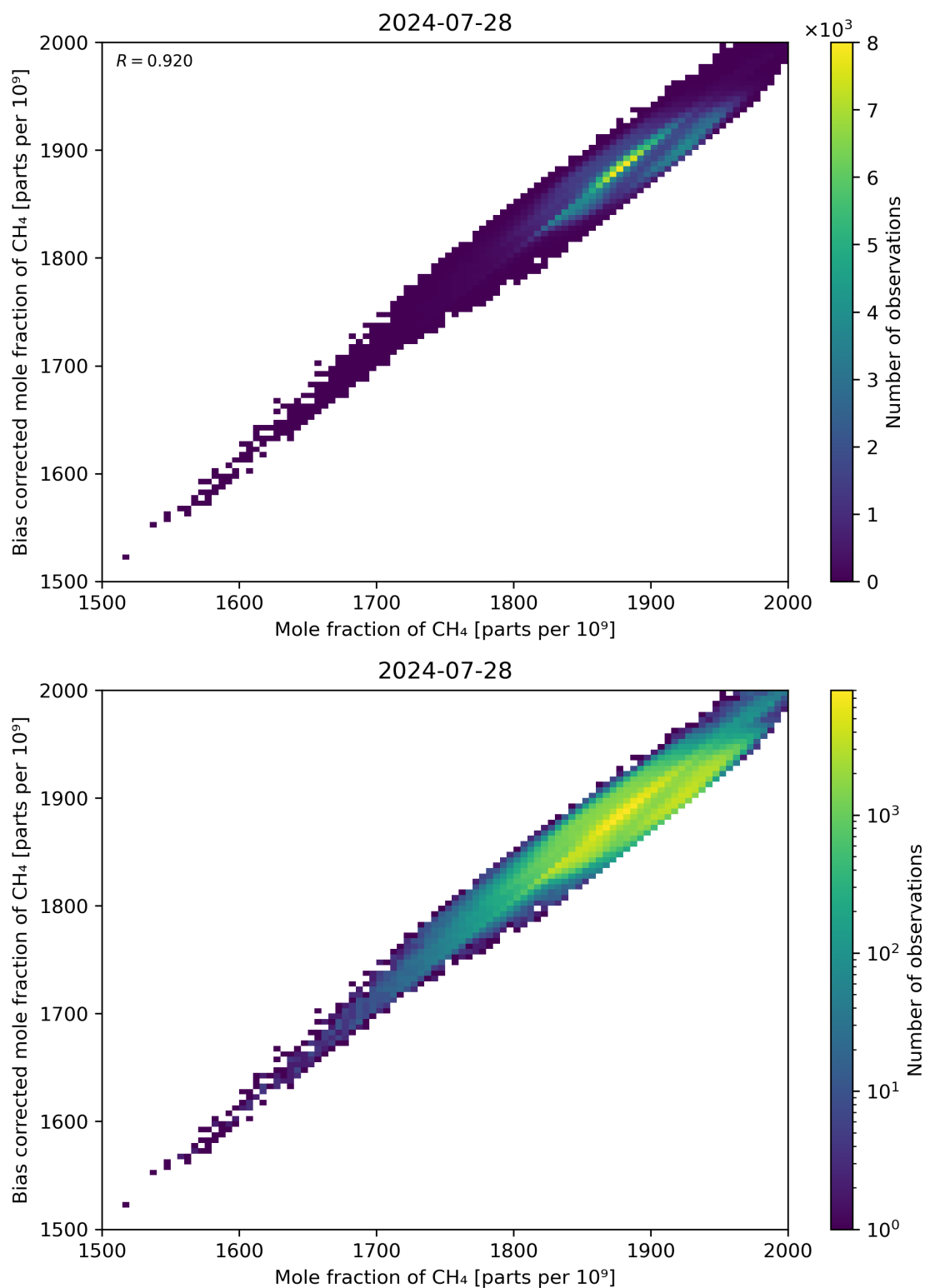
Figure 74: Scatter density plot of “Mole fraction of CH 4 ” against “Bias corrected mole fraction of CH 4 ” for 2024-07-27 to 2024-07-29.
