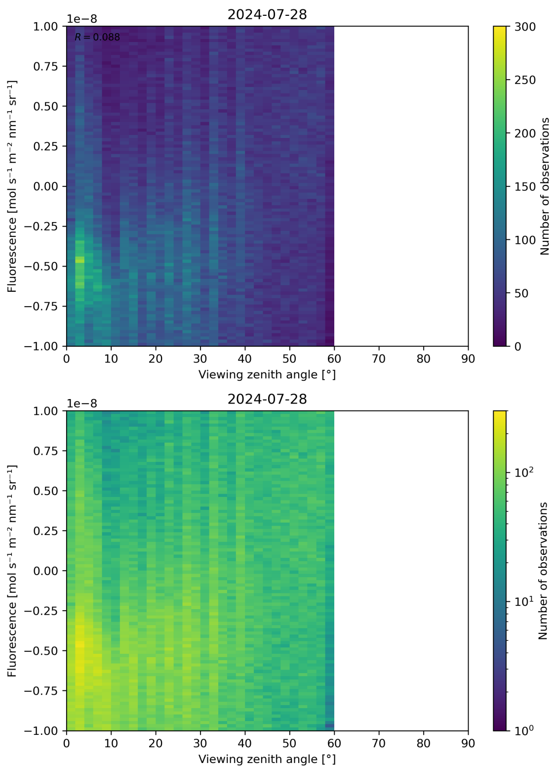
Figure 108: Scatter density plot of “Viewing zenith angle” against “Fluorescence” for 2024-07-27 to 2024-07-29.
