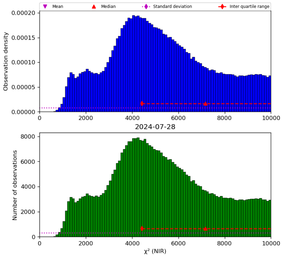
Figure 29: Histogram of “ \chi^2 (NIR)” for 2024-07-27 to 2024-07-29
