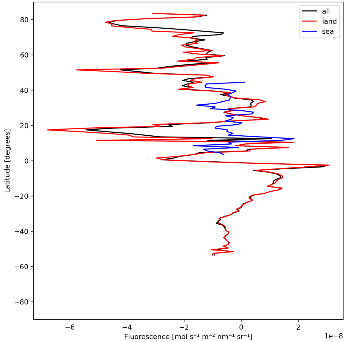
Figure 21: Zonal average of “Fluorescence” for 2024-07-27 to 2024-07-29.
