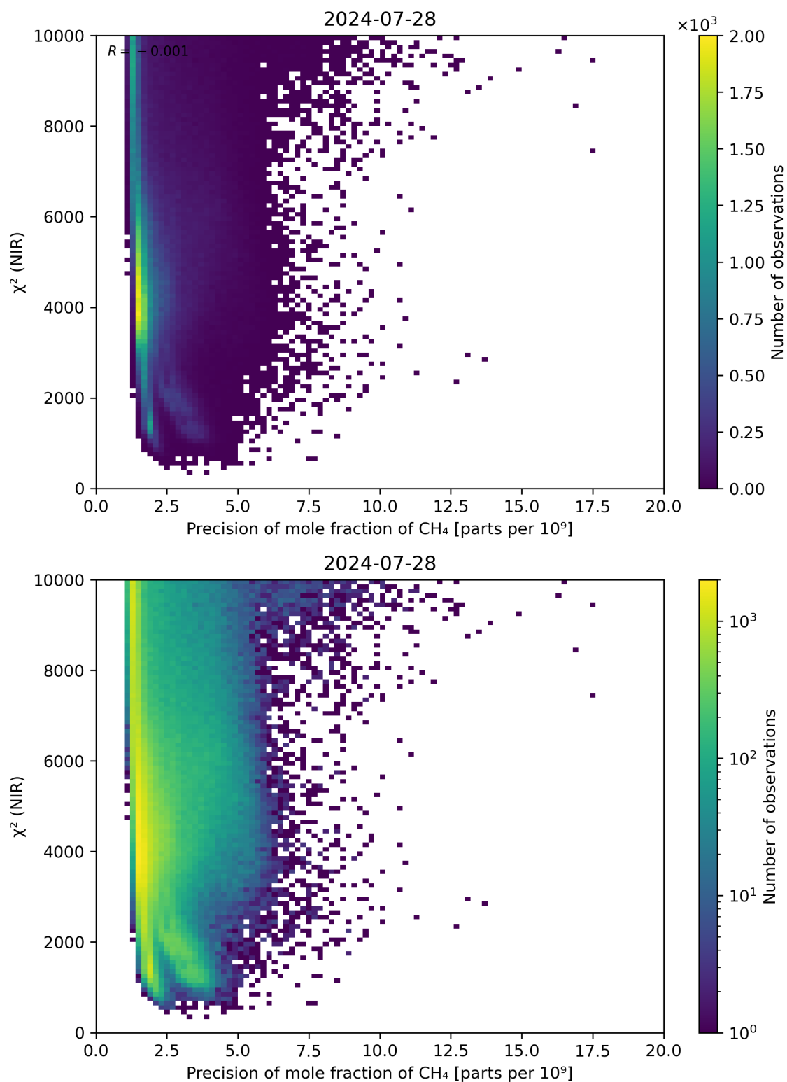
Figure 78: Scatter density plot of “Precision of mole fraction of CH 4 ” against “ \chi^2 (NIR)” for 2024-07-27 to 2024-07-29.
