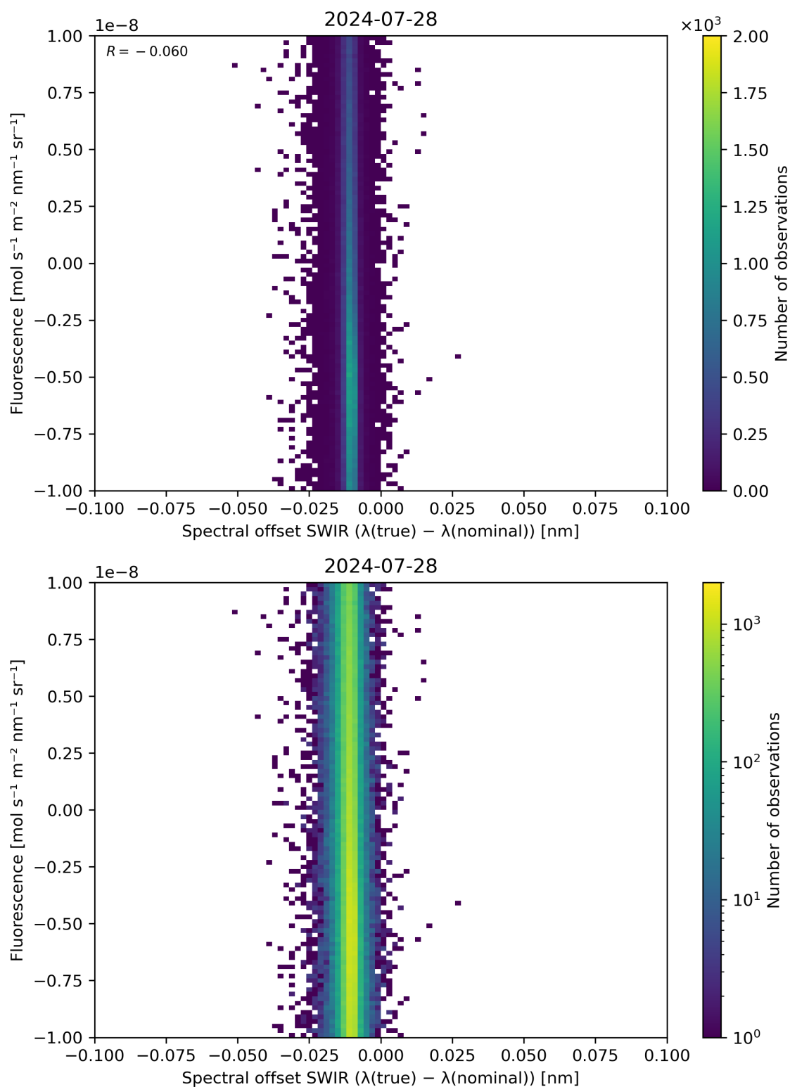
Figure 120: Scatter density plot of “Spectral offset SWIR ( \lambda(\text{true}) - \lambda(\text{nominal}) )” against “Fluorescence” for 2024-07-27 to 2024-07-29.
