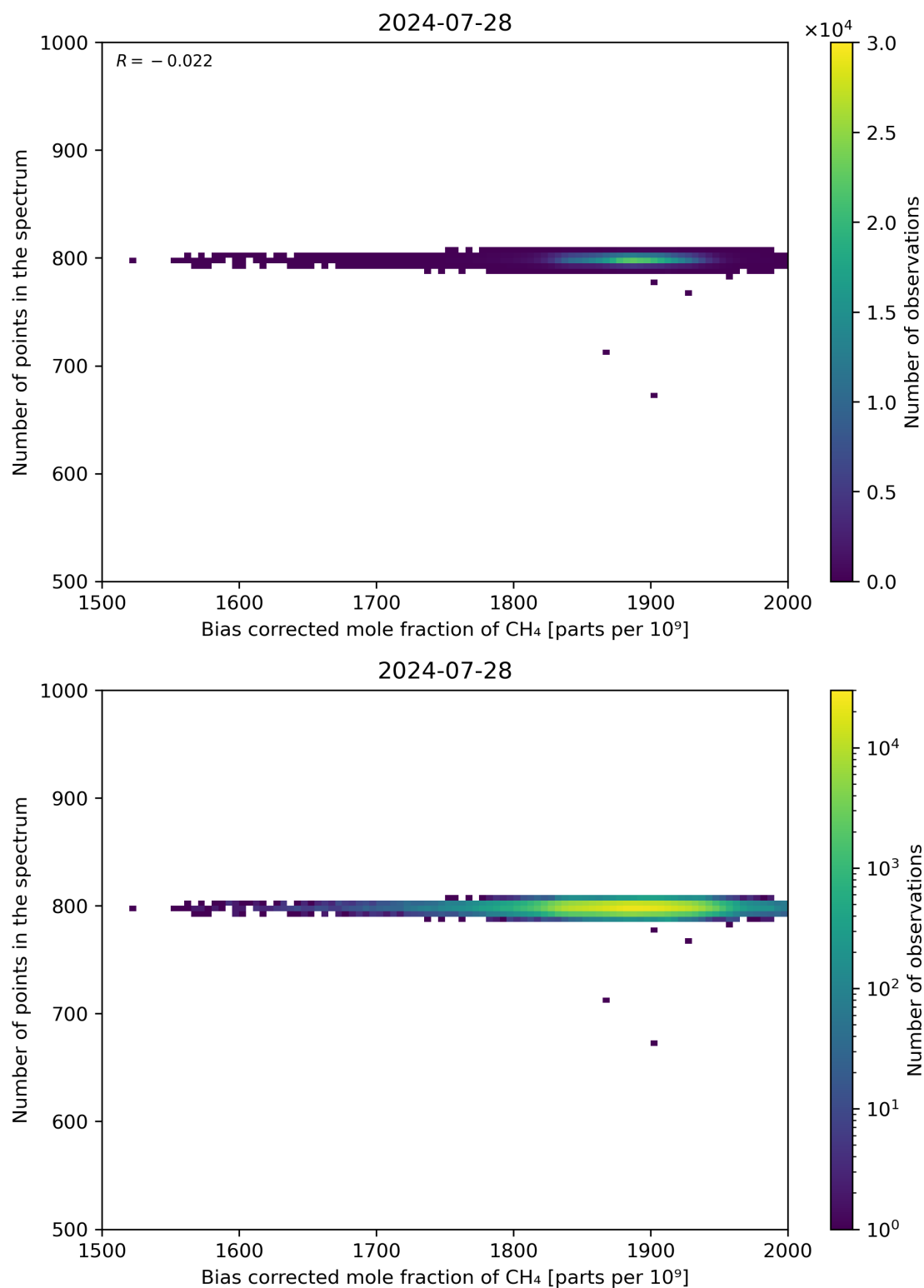
Figure 68: Scatter density plot of “Bias corrected mole fraction of CH 4 ” against “Number of points in the spectrum” for 2024-07-27 to 2024-07-29.
