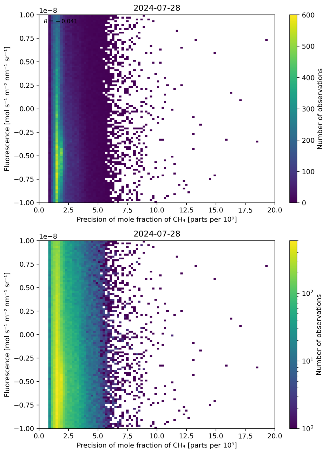
Figure 81: Scatter density plot of “Precision of mole fraction of \text{CH}_4 ” against “Fluorescence” for 2024-07-27 to 2024-07-29.
