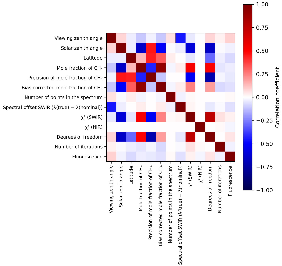
Figure 2: Map of correlation matrix for 2024-07-27 to 2024-07-29.
