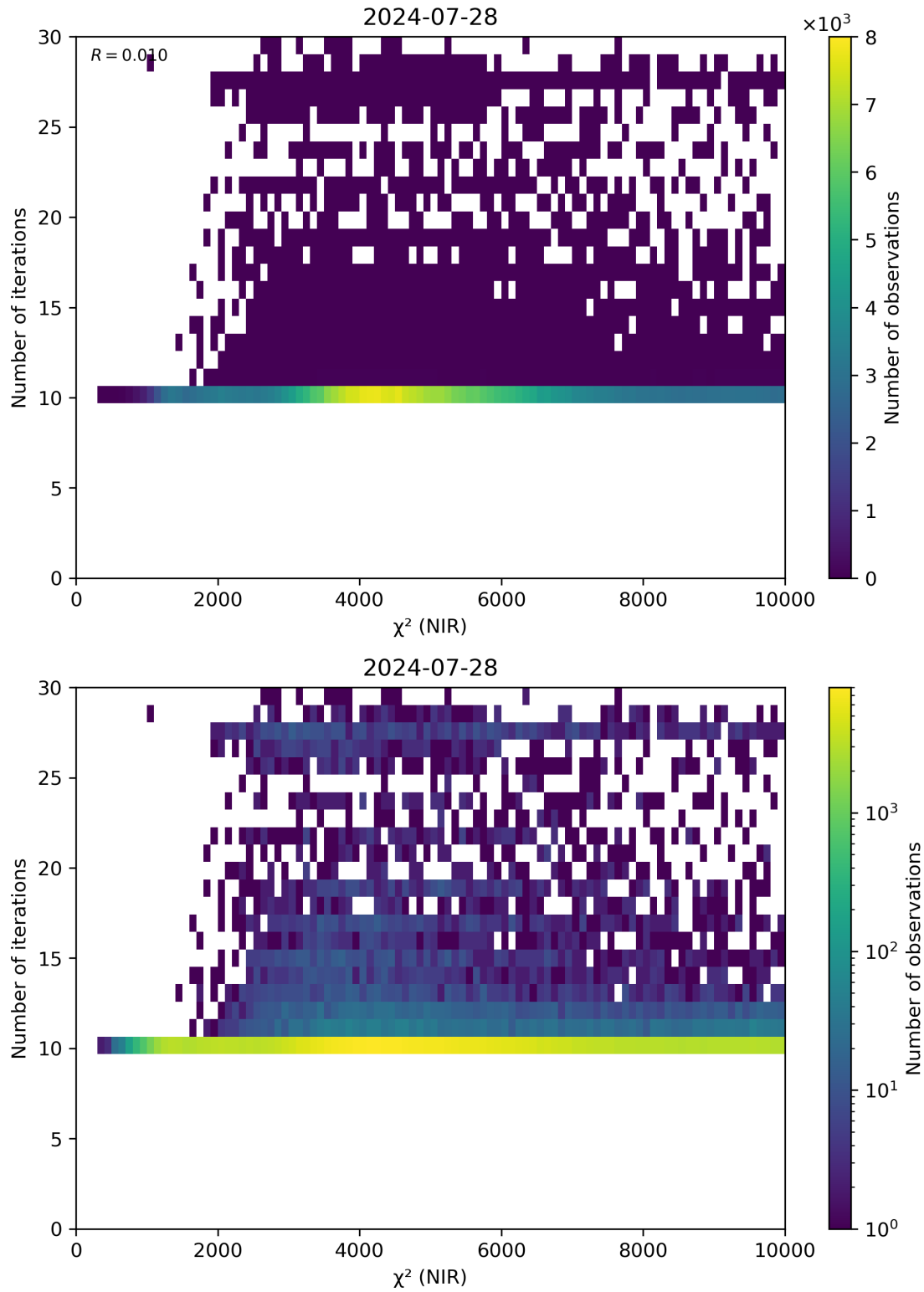
Figure 46: Scatter density plot of “ \chi^2 (NIR)” against “Number of iterations” for 2024-07-27 to 2024-07-29.
