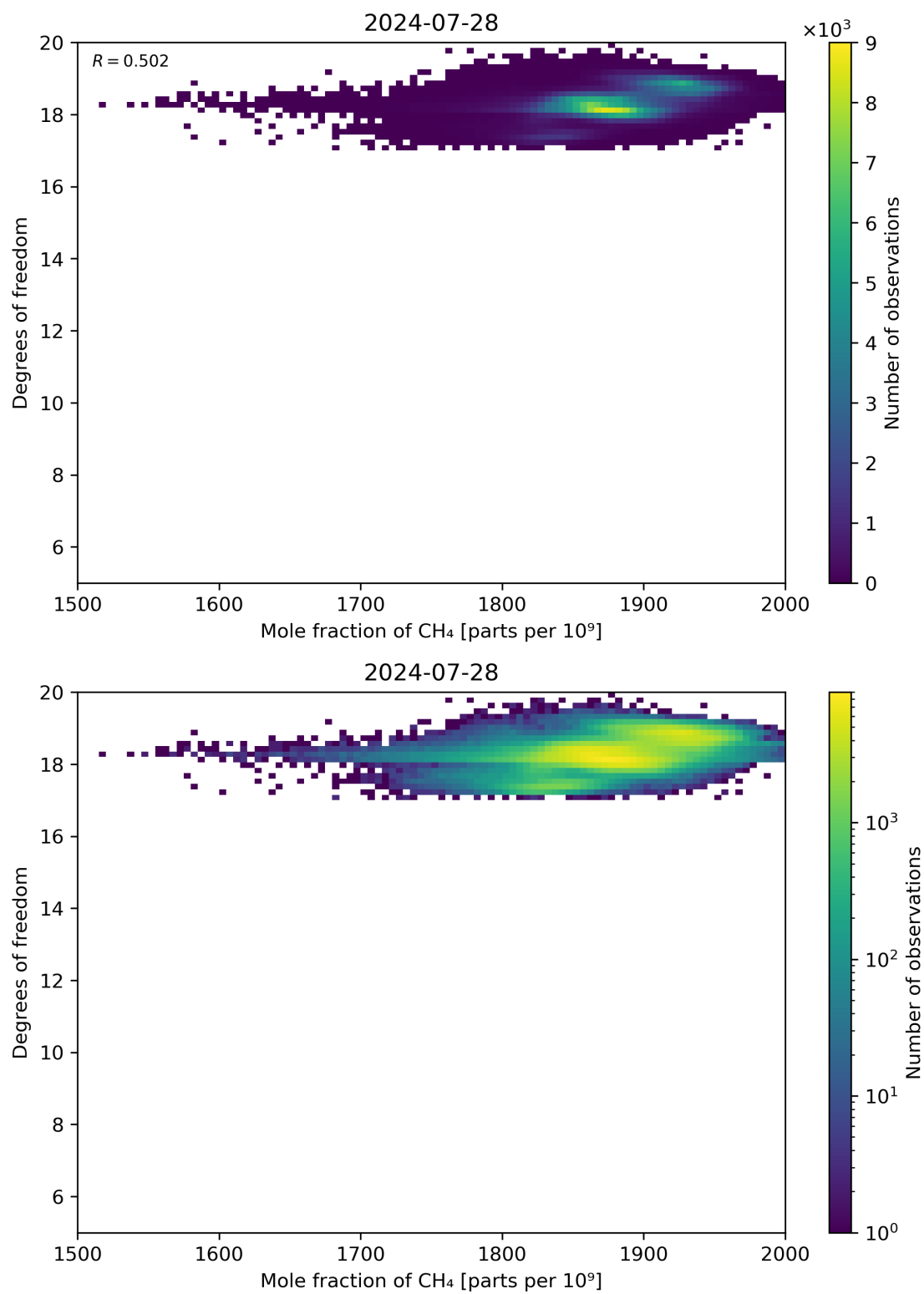
Figure 72: Scatter density plot of “Mole fraction of CH 4 ” against “Degrees of freedom” for 2024-07-27 to 2024-07-29.
