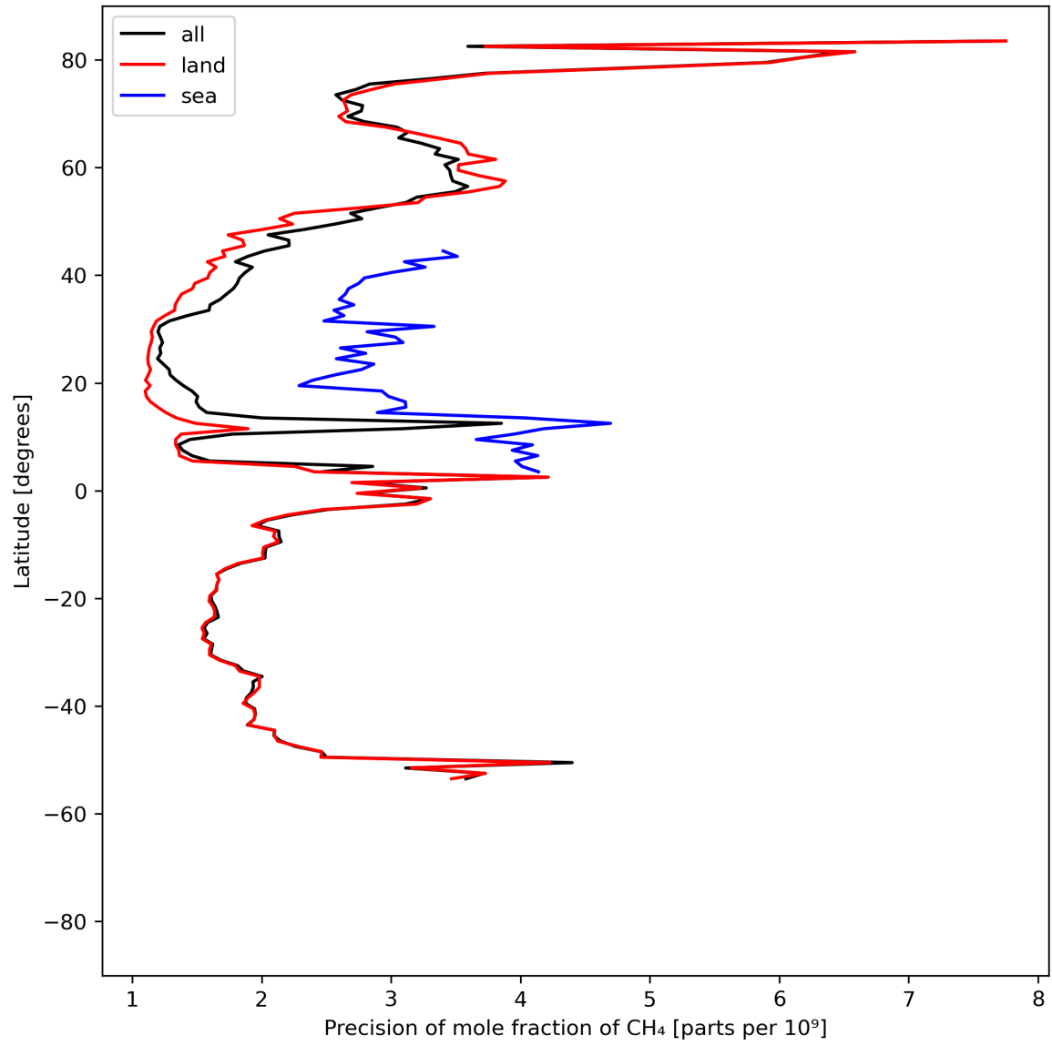
Figure 13: Zonal average of “Precision of mole fraction of CH 4 ” for 2024-07-27 to 2024-07-29.
