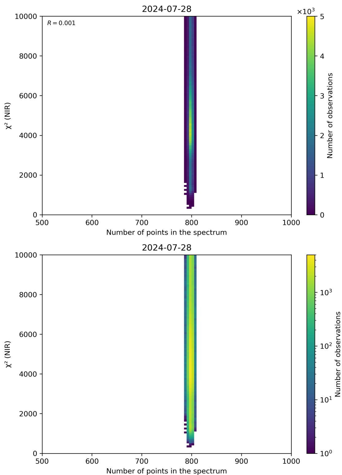
Figure 88: Scatter density plot of “Number of points in the spectrum” against “ \chi^2 (NIR)” for 2024-07-27 to 2024-07-29.
