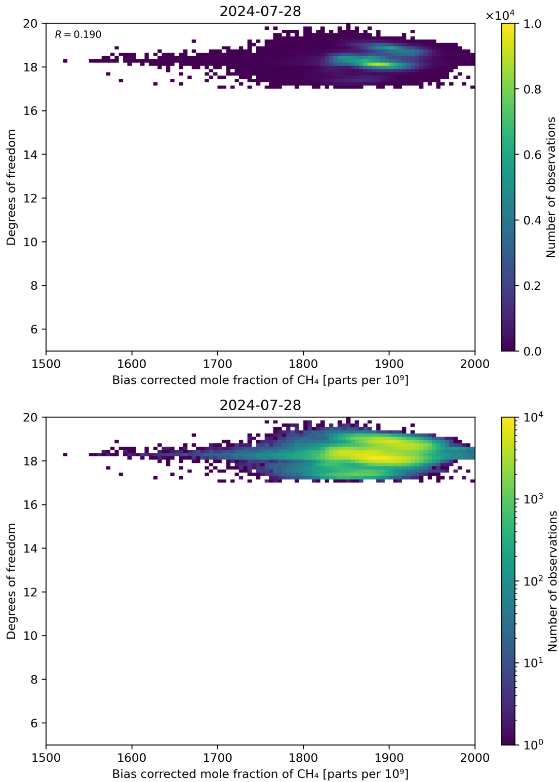
Figure 65: Scatter density plot of “Bias corrected mole fraction of CH 4 ” against “Degrees of freedom” for 2024-07-27 to 2024-07-29.
