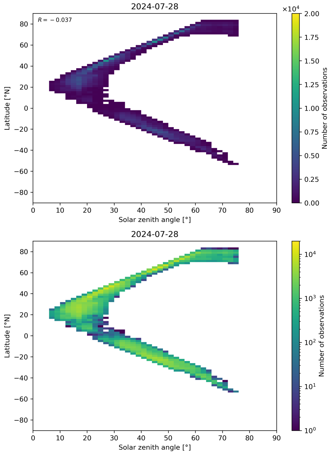
Figure 98: Scatter density plot of “Solar zenith angle” against “Latitude” for 2024-07-27 to 2024-07-29.
