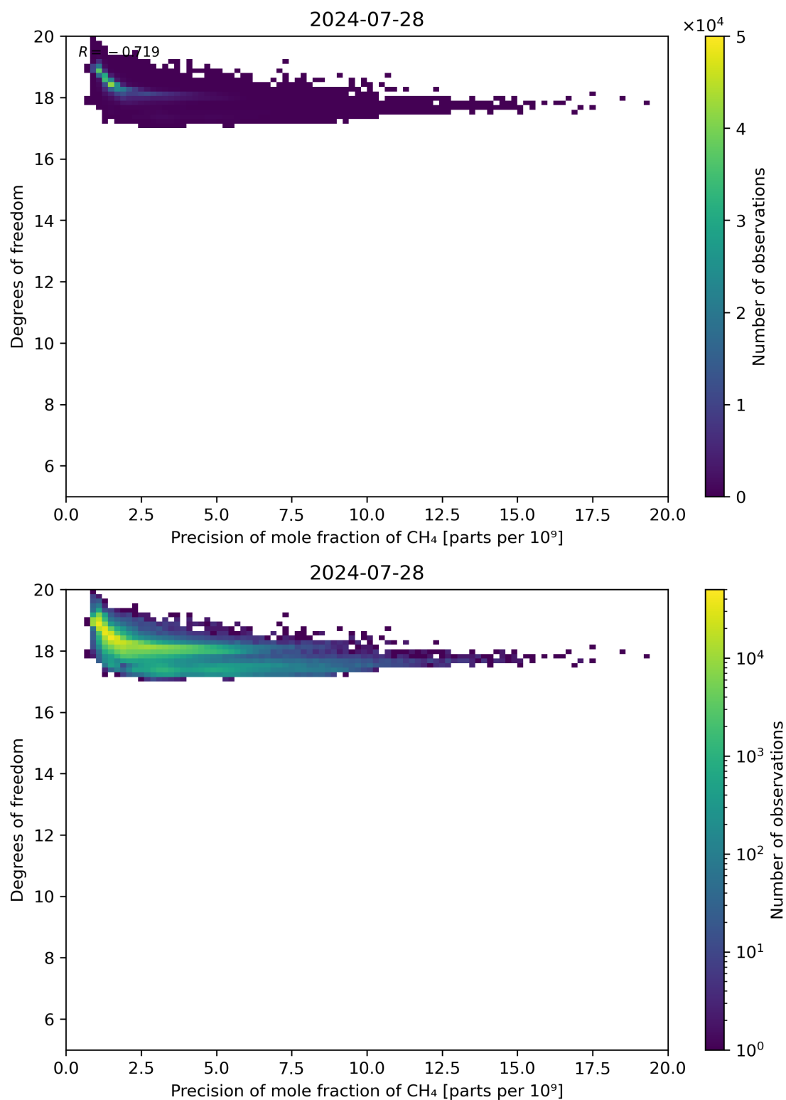
Figure 80: Scatter density plot of “Precision of mole fraction of CH 4 ” against “Degrees of freedom” for 2024-07-27 to 2024-07-29.
