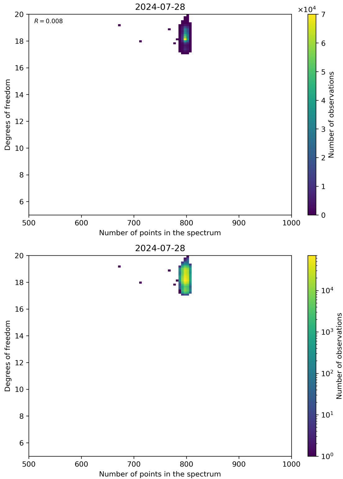
Figure 90: Scatter density plot of “Number of points in the spectrum” against “Degrees of freedom” for 2024-07-27 to 2024-07-29.
