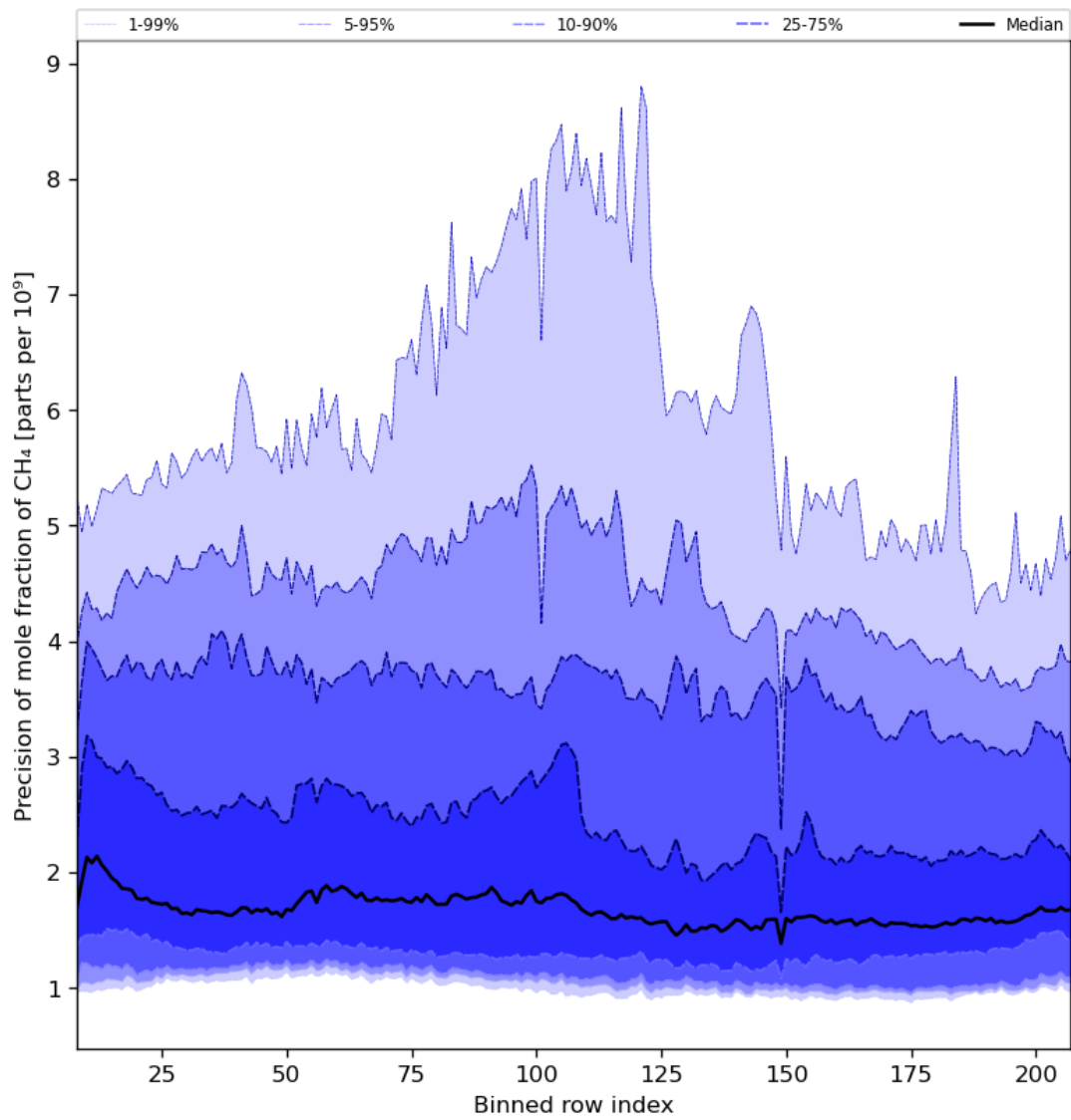
Figure 35: Along track statistics of “Precision of mole fraction of CH 4 ” for 2024-07-27 to 2024-07-29
