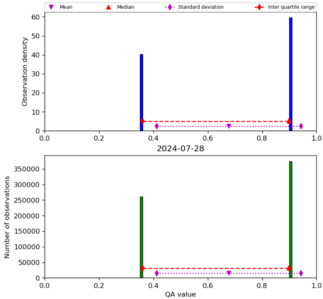
Figure 22: Histogram of “QA value” for 2024-07-27 to 2024-07-29
