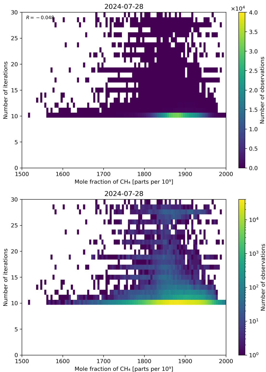
Figure 76: Scatter density plot of “Mole fraction of CH 4 ” against “Number of iterations” for 2024-07-27 to 2024-07-29.
