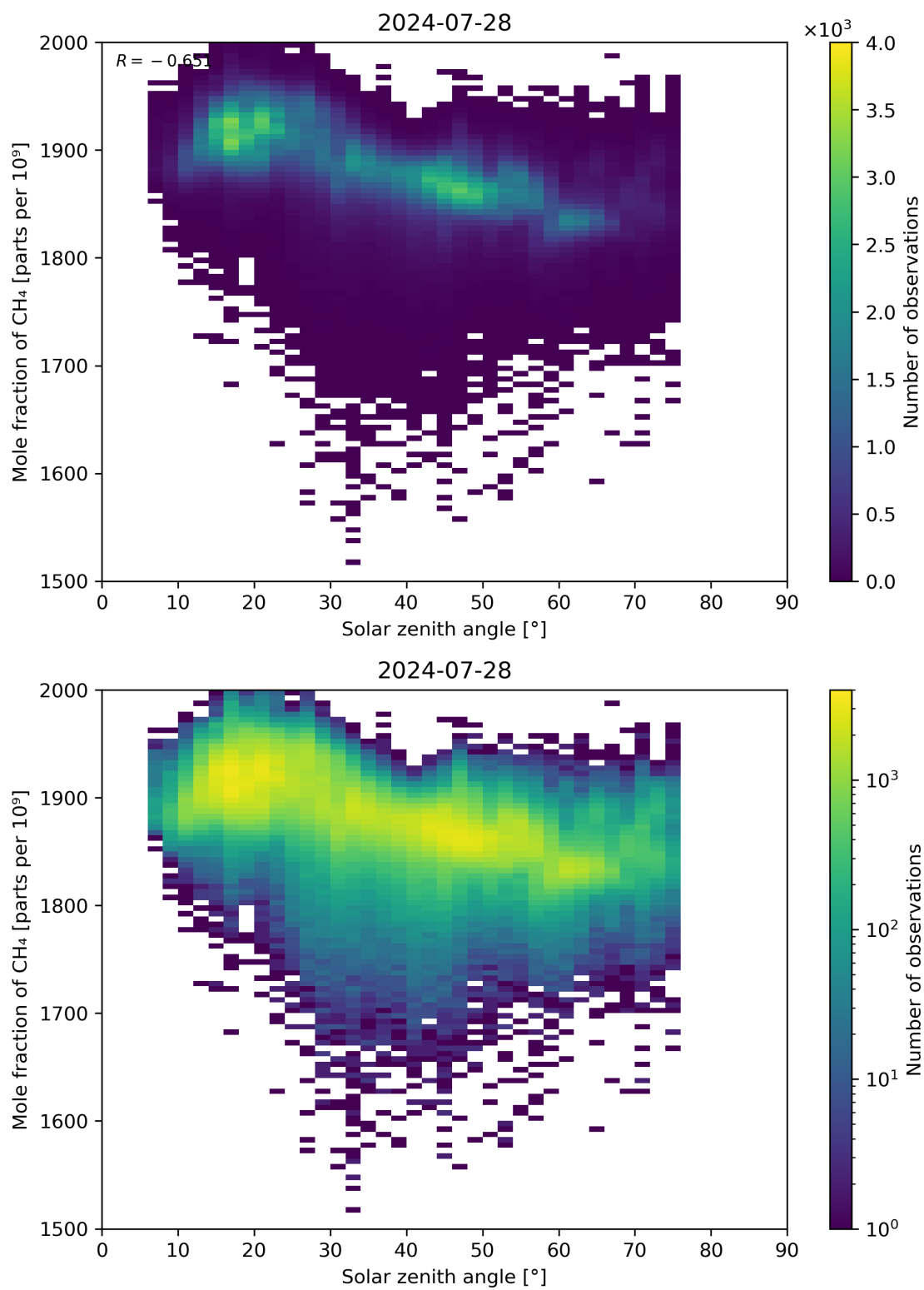
Figure 99: Scatter density plot of “Solar zenith angle” against “Mole fraction of \text{CH}_4 ” for 2024-07-27 to 2024-07-29.
