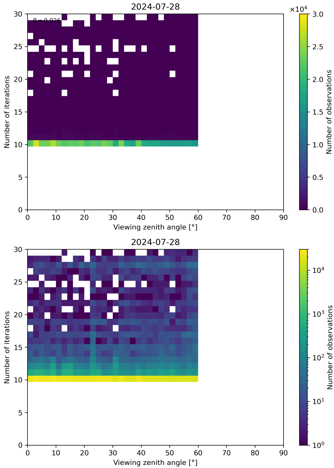
Figure 113: Scatter density plot of “Viewing zenith angle” against “Number of iterations” for 2024-07-27 to 2024-07-29.
