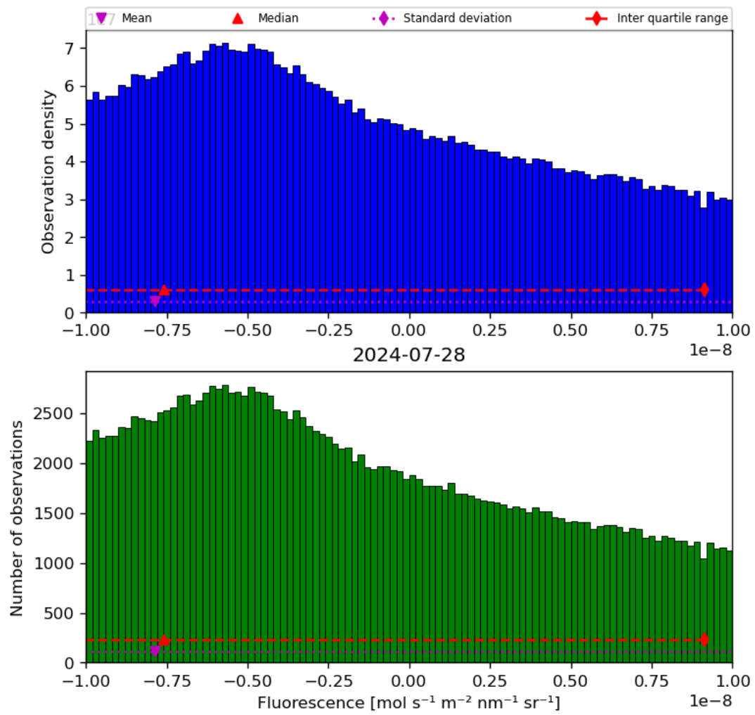
Figure 32: Histogram of “Fluorescence” for 2024-07-27 to 2024-07-29
