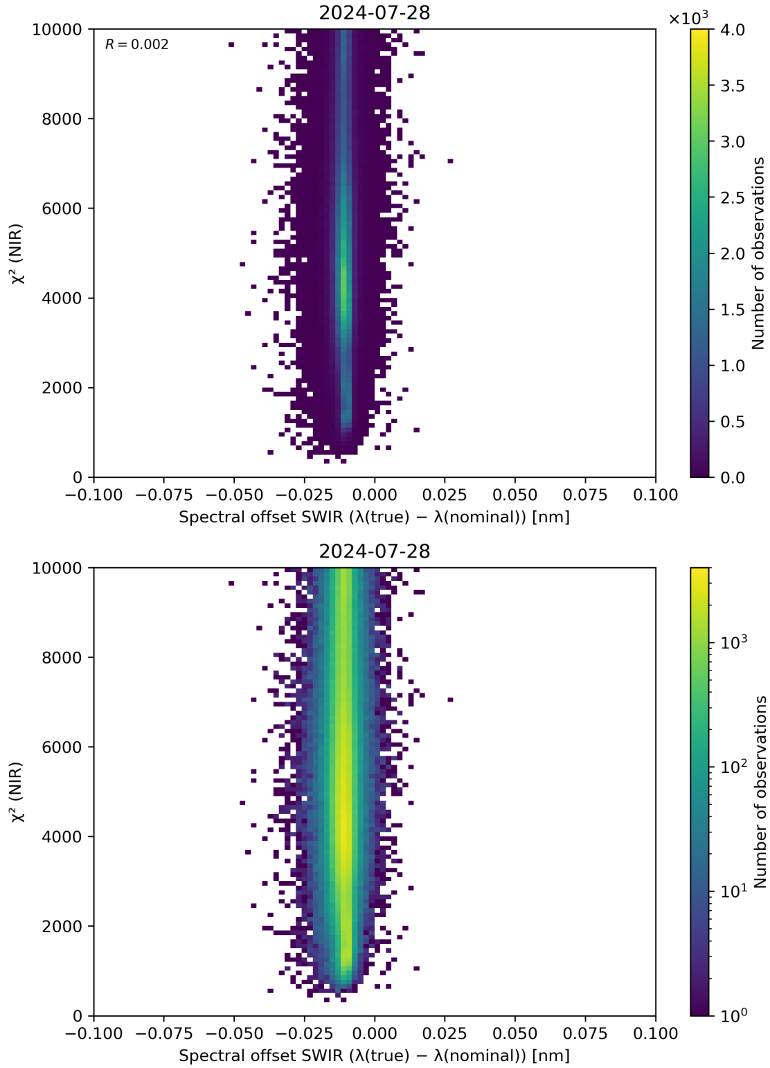
Figure 117: Scatter density plot of “Spectral offset SWIR ( \lambda(\text{true}) - \lambda(\text{nominal}) )” against “ \chi^2 (NIR)” for 2024-07-27 to 2024-07-29.
