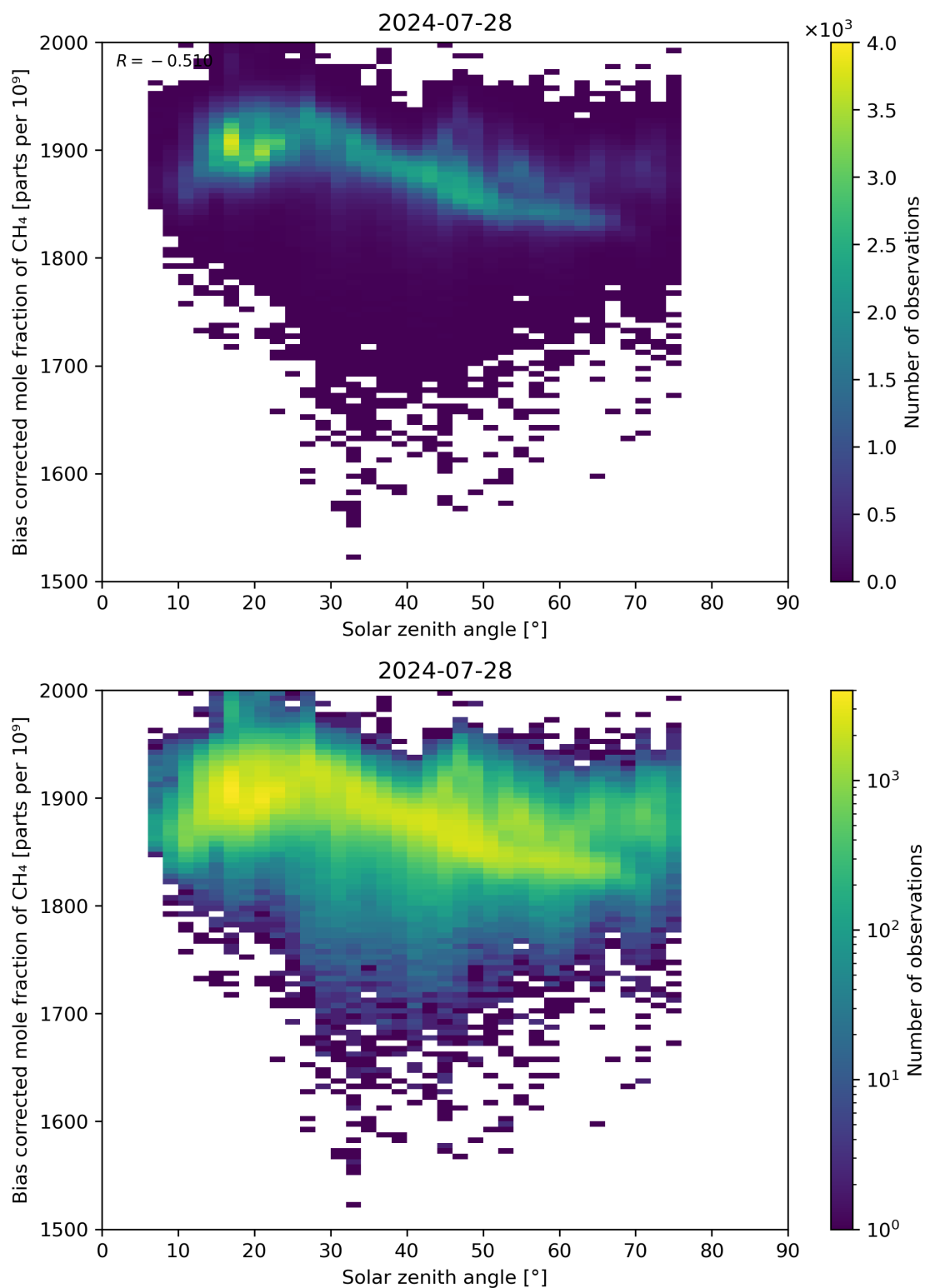
Figure 100: Scatter density plot of “Solar zenith angle” against “Bias corrected mole fraction of CH 4 ” for 2024-07-27 to 2024-07-29.
