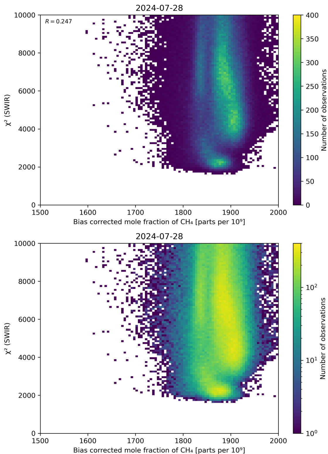
Figure 64: Scatter density plot of “Bias corrected mole fraction of \text{CH}_4 ” against “ \chi^2 (SWIR)” for 2024-07-27 to 2024-07-29.
