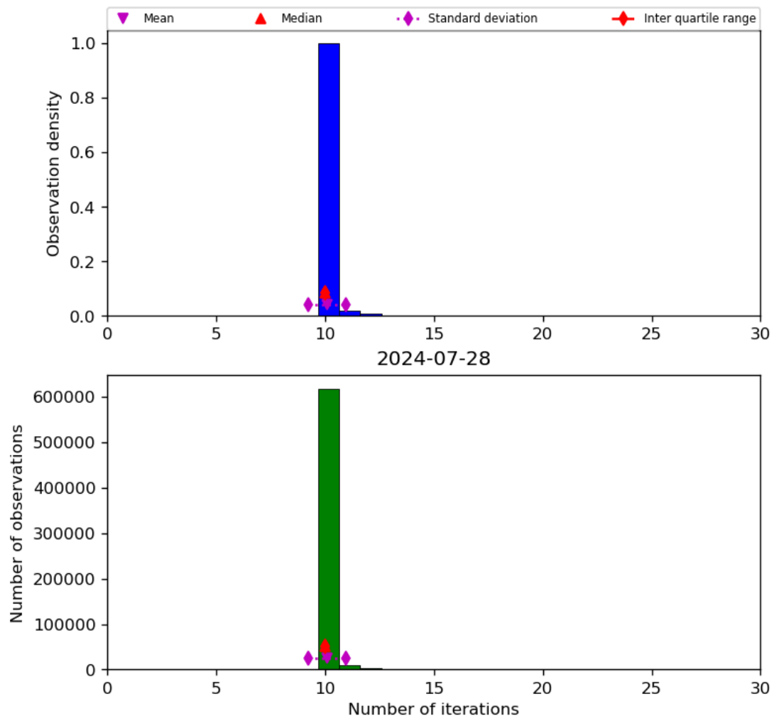
Figure 31: Histogram of “Number of iterations” for 2024-07-27 to 2024-07-29
