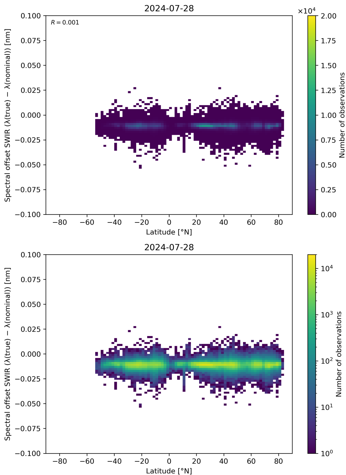
Figure 62: Scatter density plot of “Latitude” against “Spectral offset SWIR ( \lambda(\text{true}) - \lambda(\text{nominal}) )” for 2024-07-27 to 2024-07-29.
