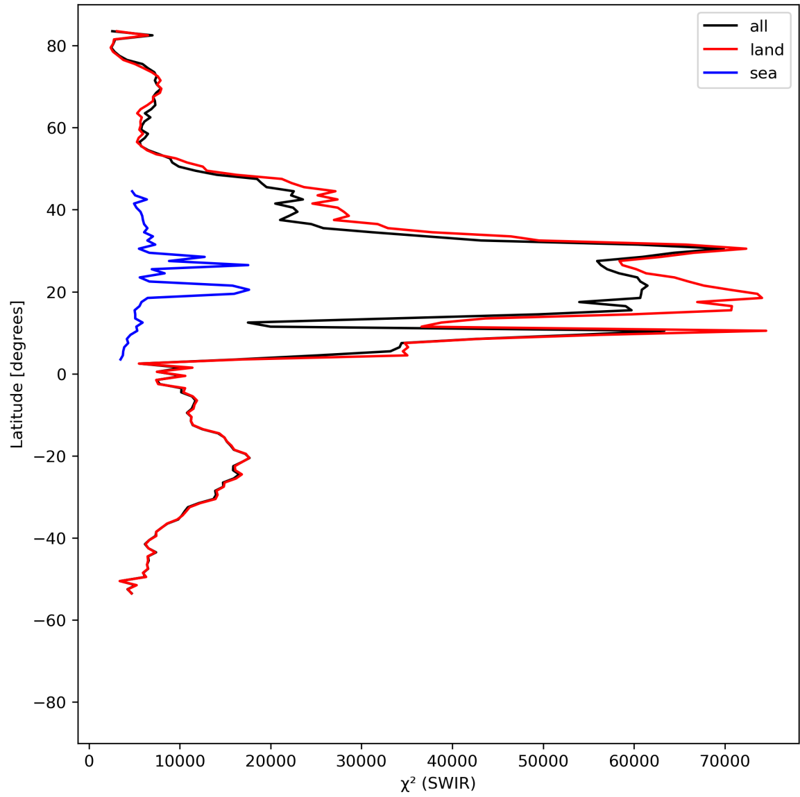
Figure 17: Zonal average of “ \chi^2 (SWIR)” for 2024-07-27 to 2024-07-29.
