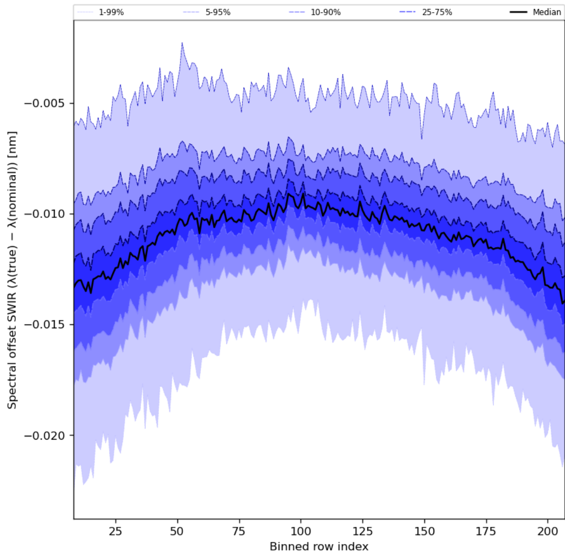
Figure 38: Along track statistics of “Spectral offset SWIR ( \lambda(\text{true}) - \lambda(\text{nominal}) )” for 2024-07-27 to 2024-07-29
