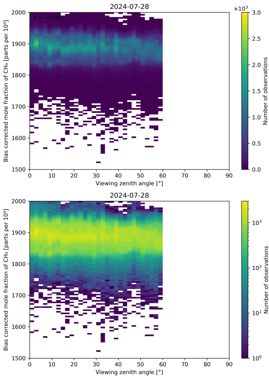
Figure 111: Scatter density plot of “Viewing zenith angle” against “Bias corrected mole fraction of CH 4 ” for 2024-07-27 to 2024-07-29.
