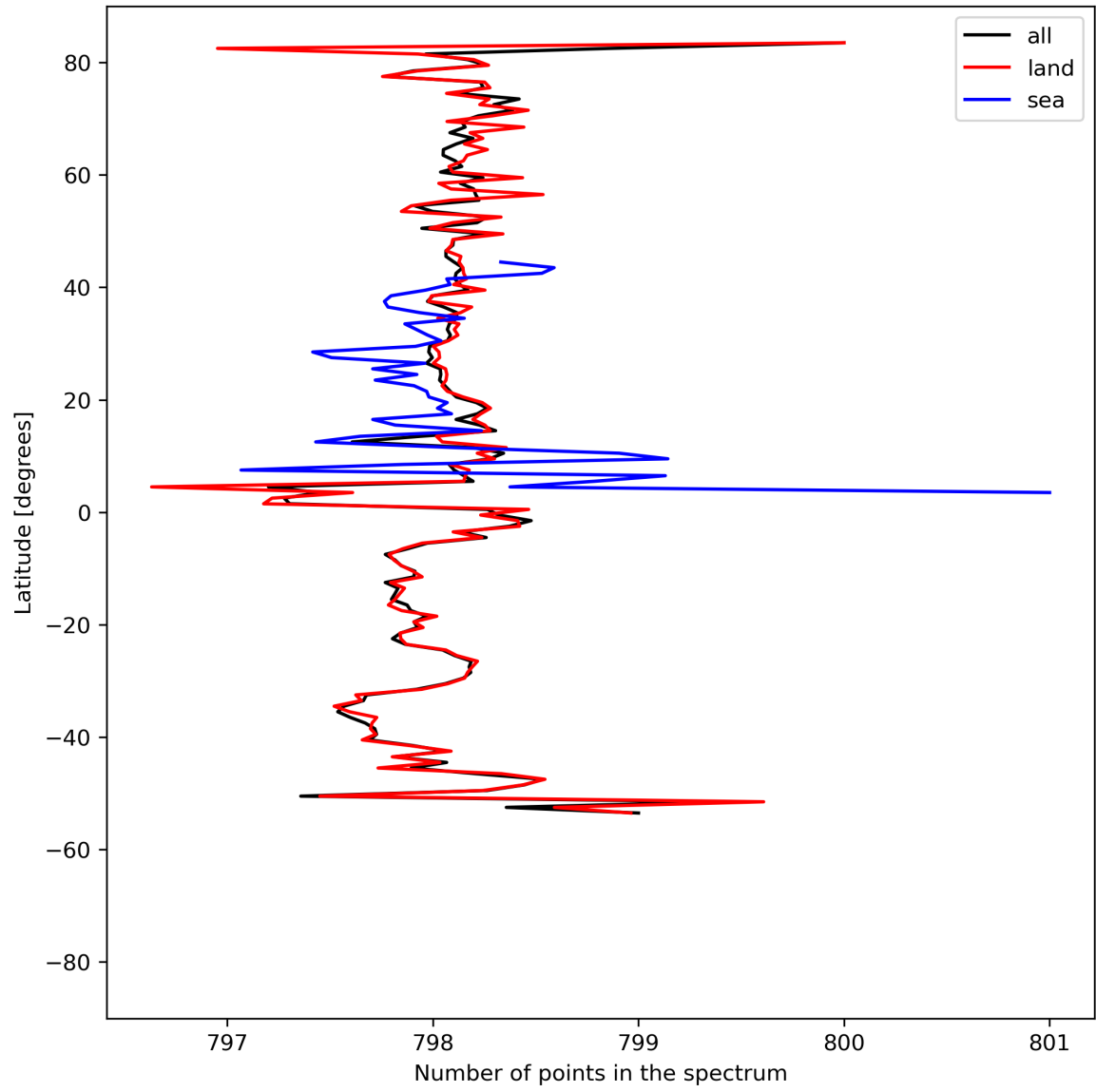
Figure 15: Zonal average of “Number of points in the spectrum” for 2024-07-27 to 2024-07-29.
