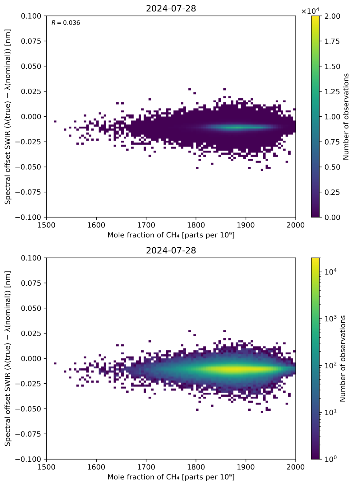
Figure 86: Scatter density plot of “Mole fraction of CH 4 ” against “Spectral offset SWIR ( \lambda(\text{true}) - \lambda(\text{nominal}) )” for 2024-07-27 to 2024-07-29.
