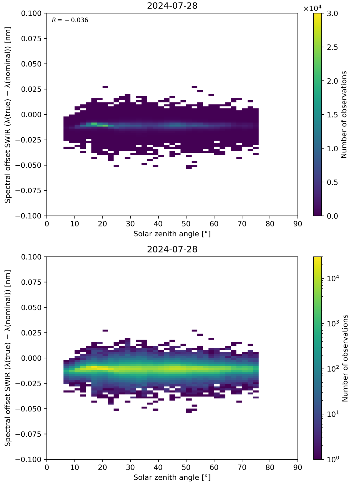
Figure 104: Scatter density plot of “Solar zenith angle” against “Spectral offset SWIR ( \lambda(\text{true}) - \lambda(\text{nominal}) )” for 2024-07-27 to 2024-07-29.
