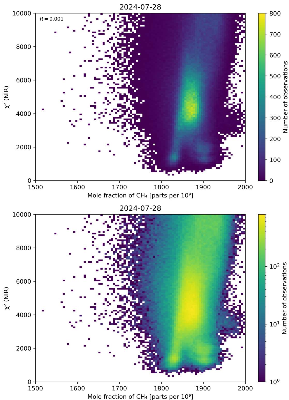
Figure 70: Scatter density plot of “Mole fraction of \text{CH}_4 ” against “ \chi^2 (NIR)” for 2024-07-27 to 2024-07-29.
