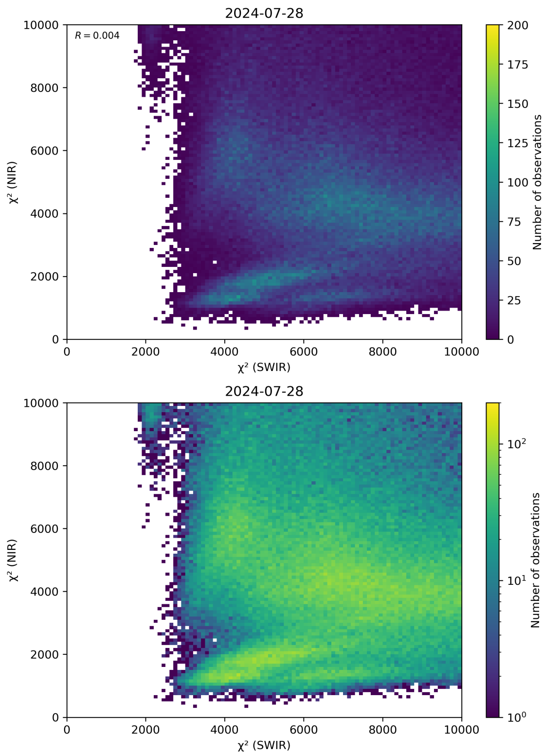
Figure 47: Scatter density plot of “ \chi^2 (SWIR)” against “ \chi^2 (NIR)” for 2024-07-27 to 2024-07-29.
