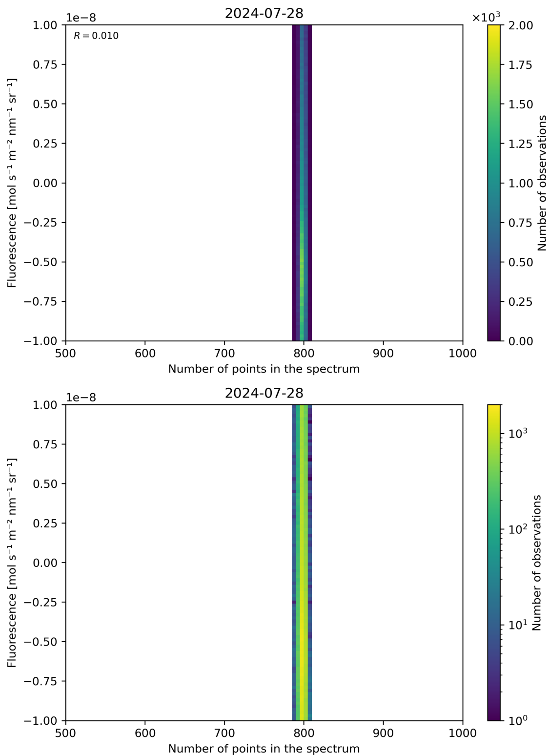
Figure 91: Scatter density plot of “Number of points in the spectrum” against “Fluorescence” for 2024-07-27 to 2024-07-29.
