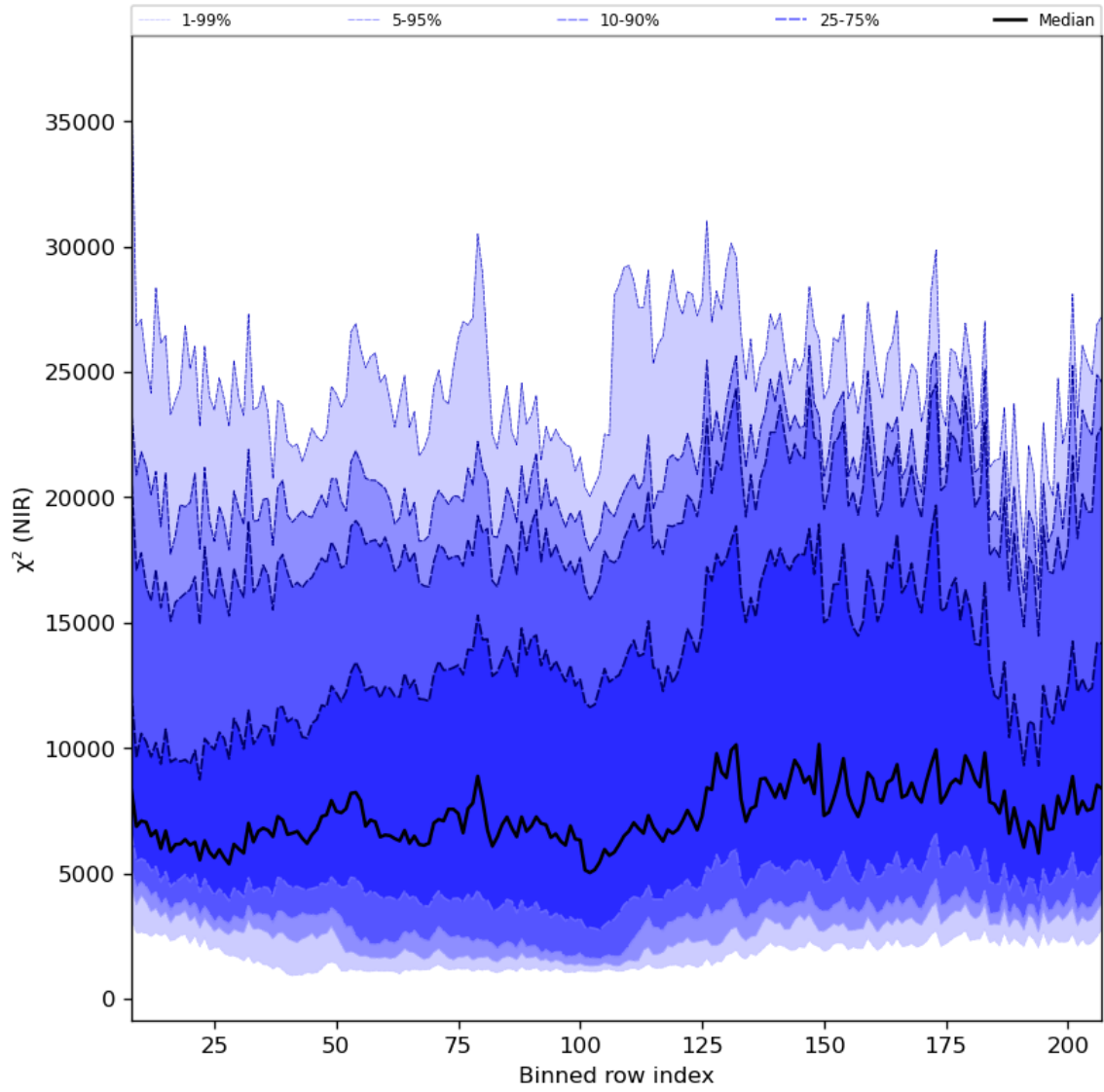
Figure 40: Along track statistics of “ \chi^2 (NIR)” for 2024-07-27 to 2024-07-29
