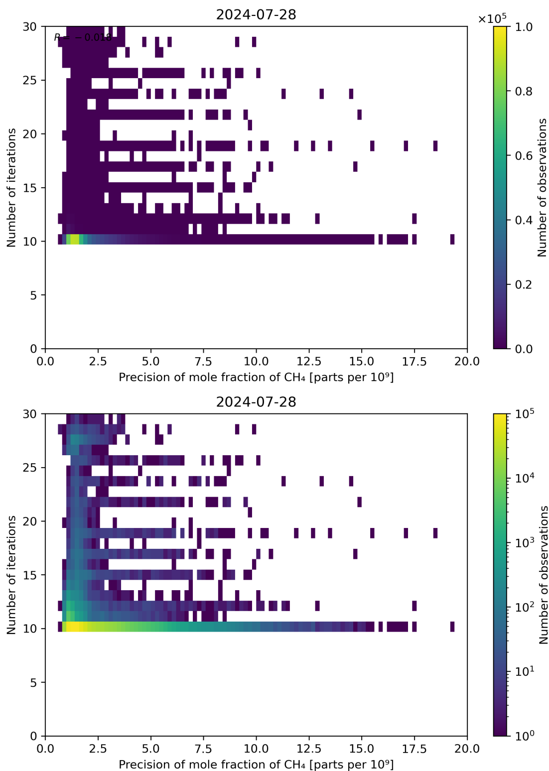
Figure 83: Scatter density plot of “Precision of mole fraction of CH 4 ” against “Number of iterations” for 2024-07-27 to 2024-07-29.
