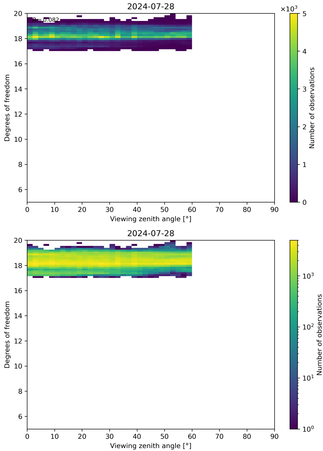
Figure 107: Scatter density plot of “Viewing zenith angle” against “Degrees of freedom” for 2024-07-27 to 2024-07-29.
