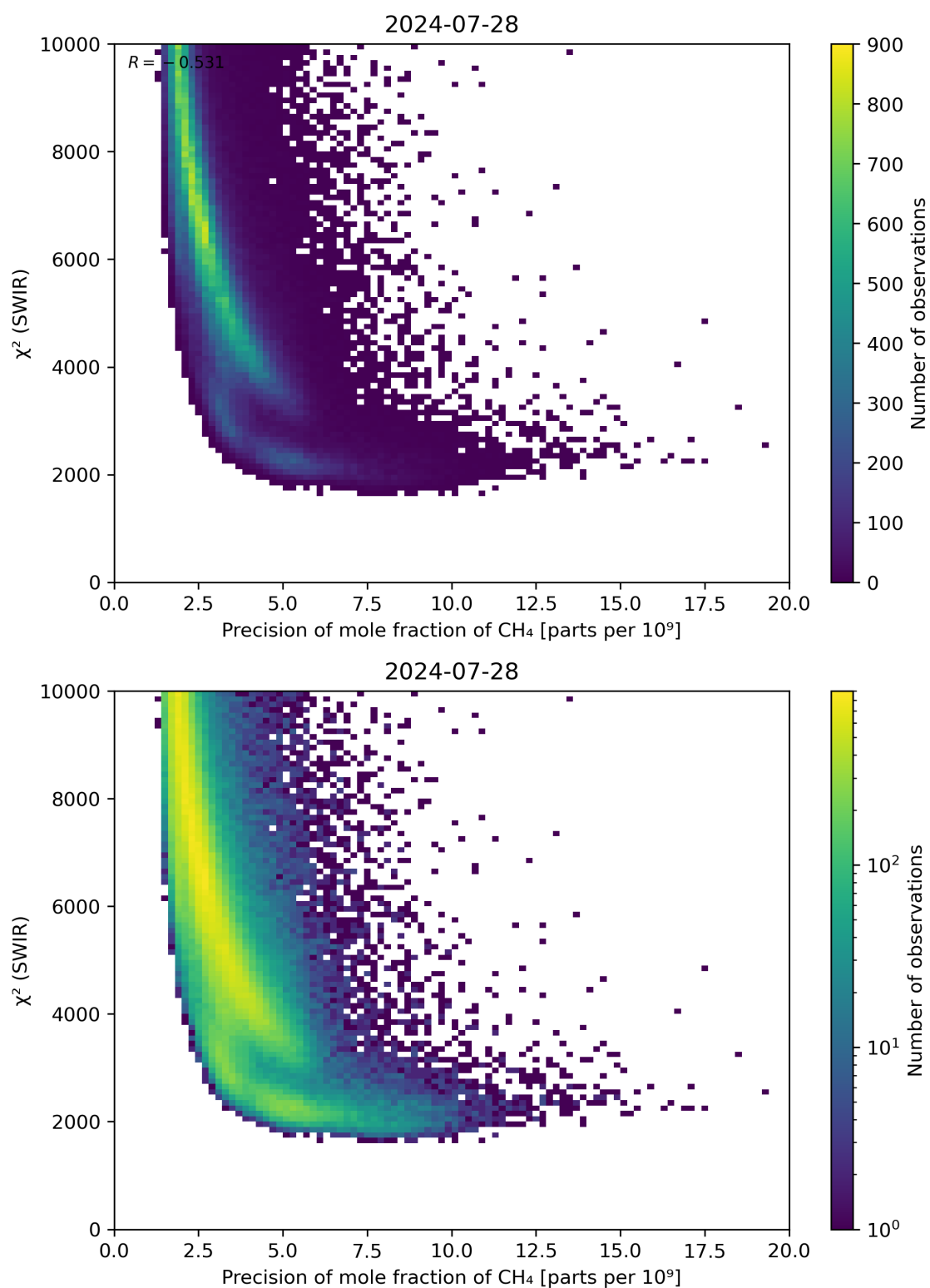
Figure 79: Scatter density plot of “Precision of mole fraction of \text{CH}_4 ” against “ \chi^2 (SWIR)” for 2024-07-27 to 2024-07-29.
