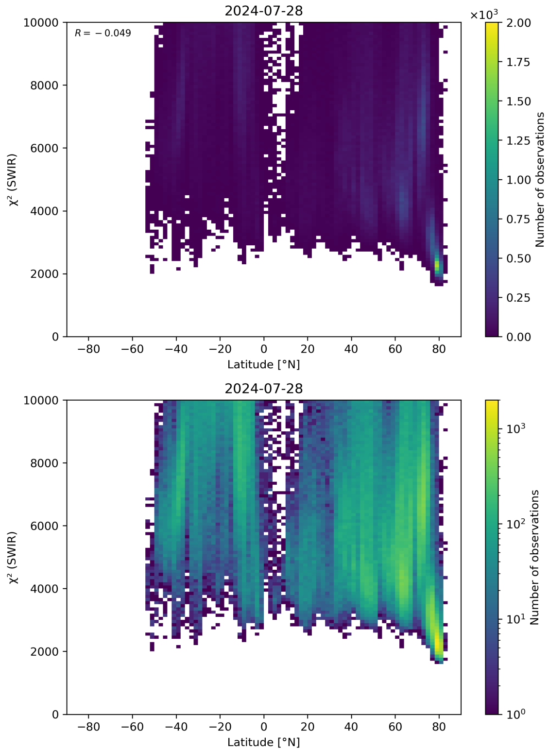
Figure 54: Scatter density plot of “Latitude” against “ \chi^2 (SWIR)” for 2024-07-27 to 2024-07-29.
