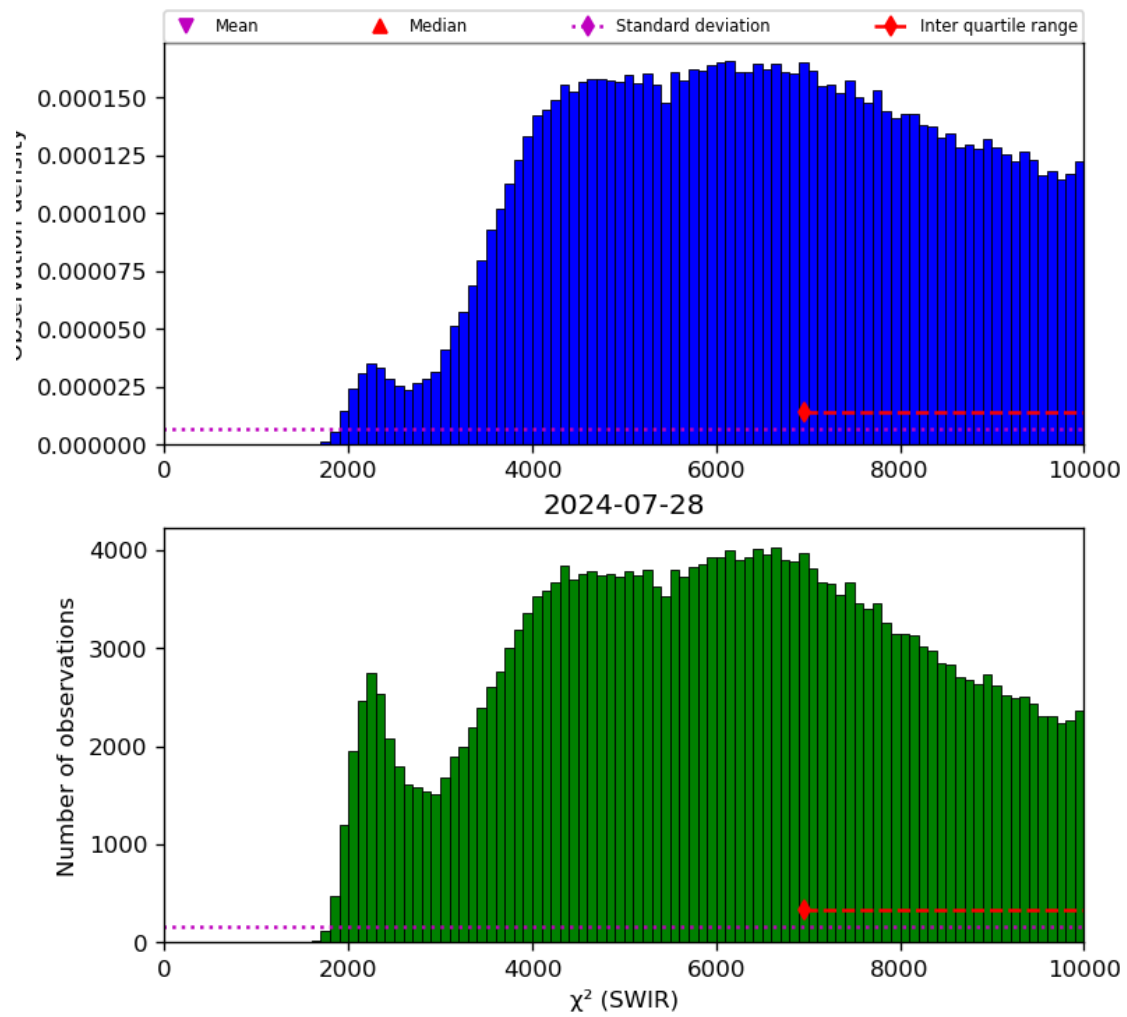
Figure 28: Histogram of “ \chi^2 (SWIR)” for 2024-07-27 to 2024-07-29
