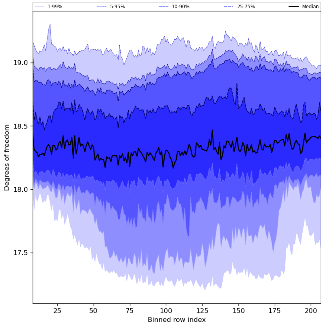
Figure 41: Along track statistics of “Degrees of freedom” for 2024-07-27 to 2024-07-29
