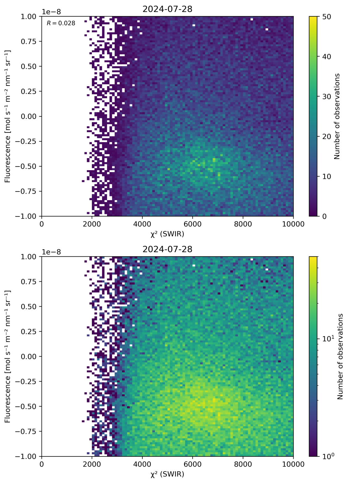
Figure 49: Scatter density plot of “ \chi^2 (SWIR)” against “Fluorescence” for 2024-07-27 to 2024-07-29.
