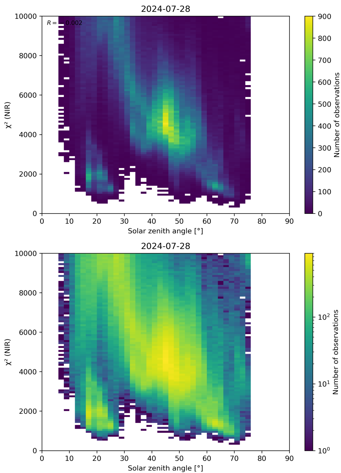
Figure 94: Scatter density plot of “Solar zenith angle” against “ \chi^2 (NIR)” for 2024-07-27 to 2024-07-29.
