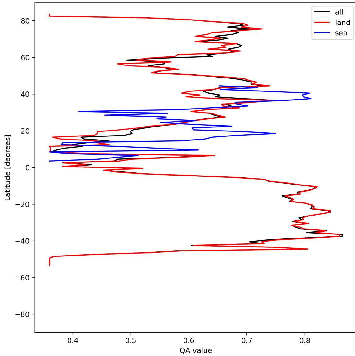
Figure 11: Zonal average of “QA value” for 2024-07-27 to 2024-07-29.
