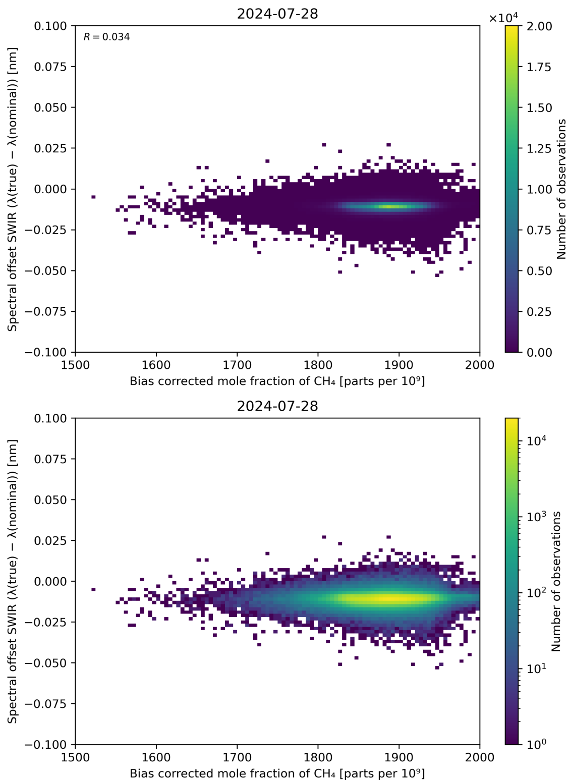
Figure 69: Scatter density plot of “Bias corrected mole fraction of \text{CH}_4 ” against “Spectral offset SWIR ( \lambda(\text{true}) - \lambda(\text{nominal}) )” for 2024-07-27 to 2024-07-29.
