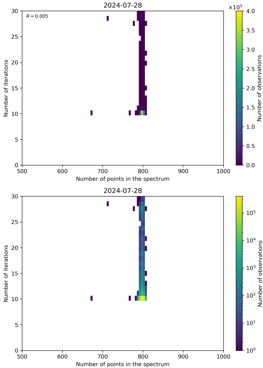
Figure 92: Scatter density plot of “Number of points in the spectrum” against “Number of iterations” for 2024-07-27 to 2024-07-29.
