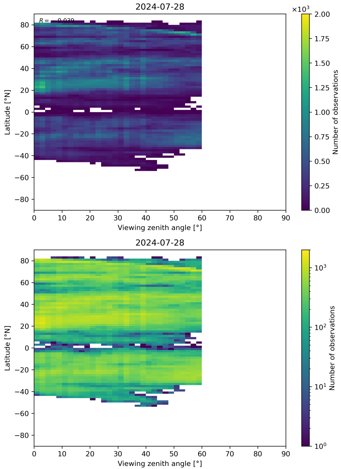
Figure 109: Scatter density plot of “Viewing zenith angle” against “Latitude” for 2024-07-27 to 2024-07-29.
