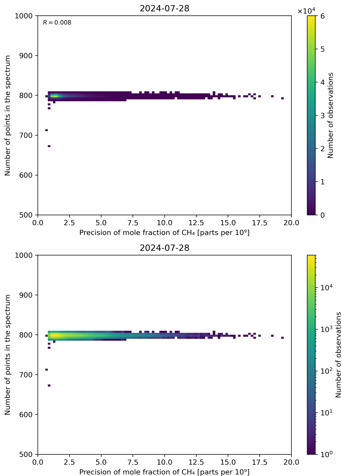
Figure 84: Scatter density plot of “Precision of mole fraction of CH 4 ” against “Number of points in the spectrum” for 2024-07-27 to 2024-07-29.
