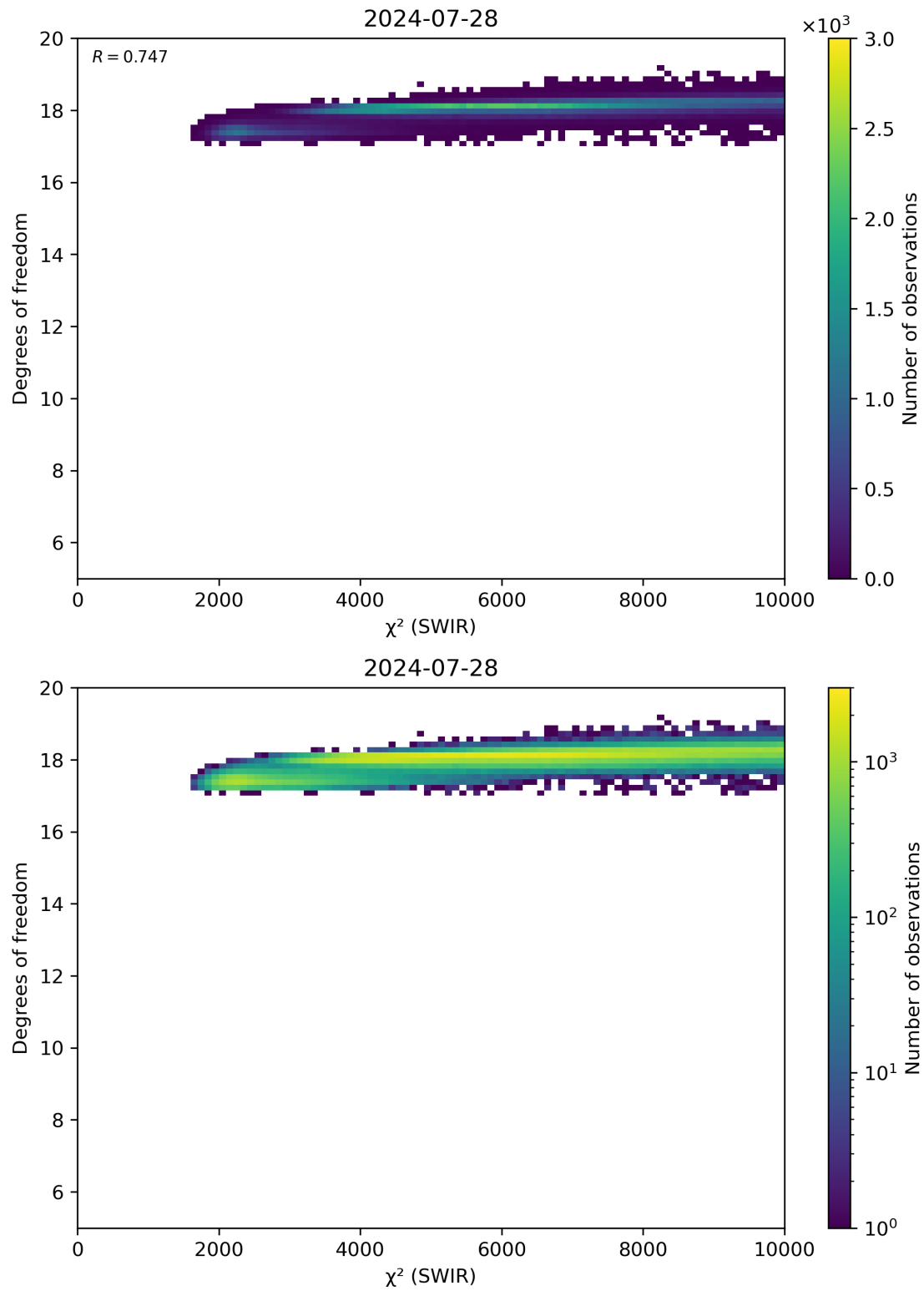
Figure 48: Scatter density plot of " \chi^2 (SWIR)" against "Degrees of freedom" for 2024-07-27 to 2024-07-29.
