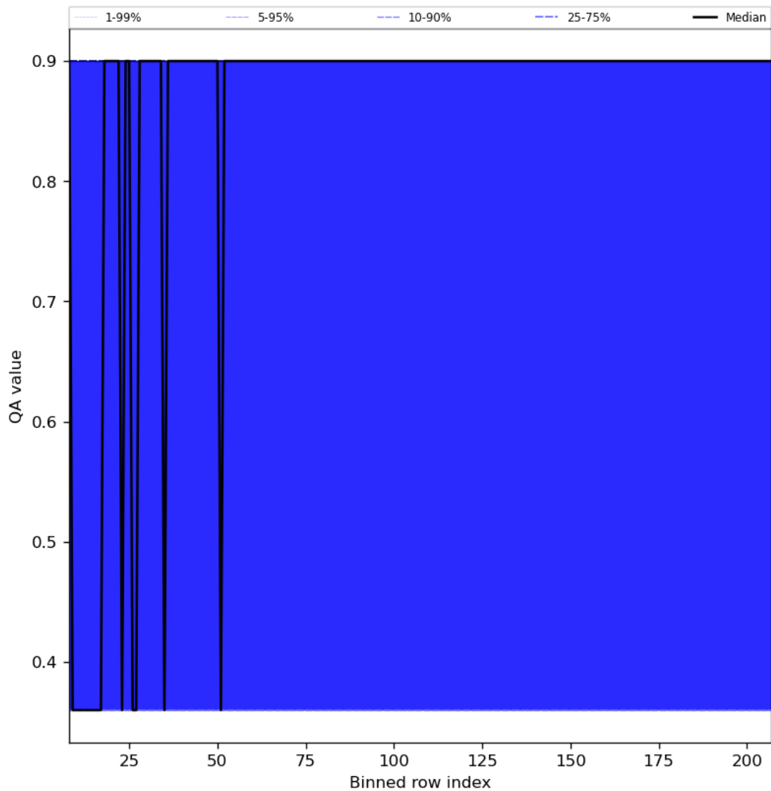
Figure 33: Along track statistics of “QA value” for 2024-07-27 to 2024-07-29
