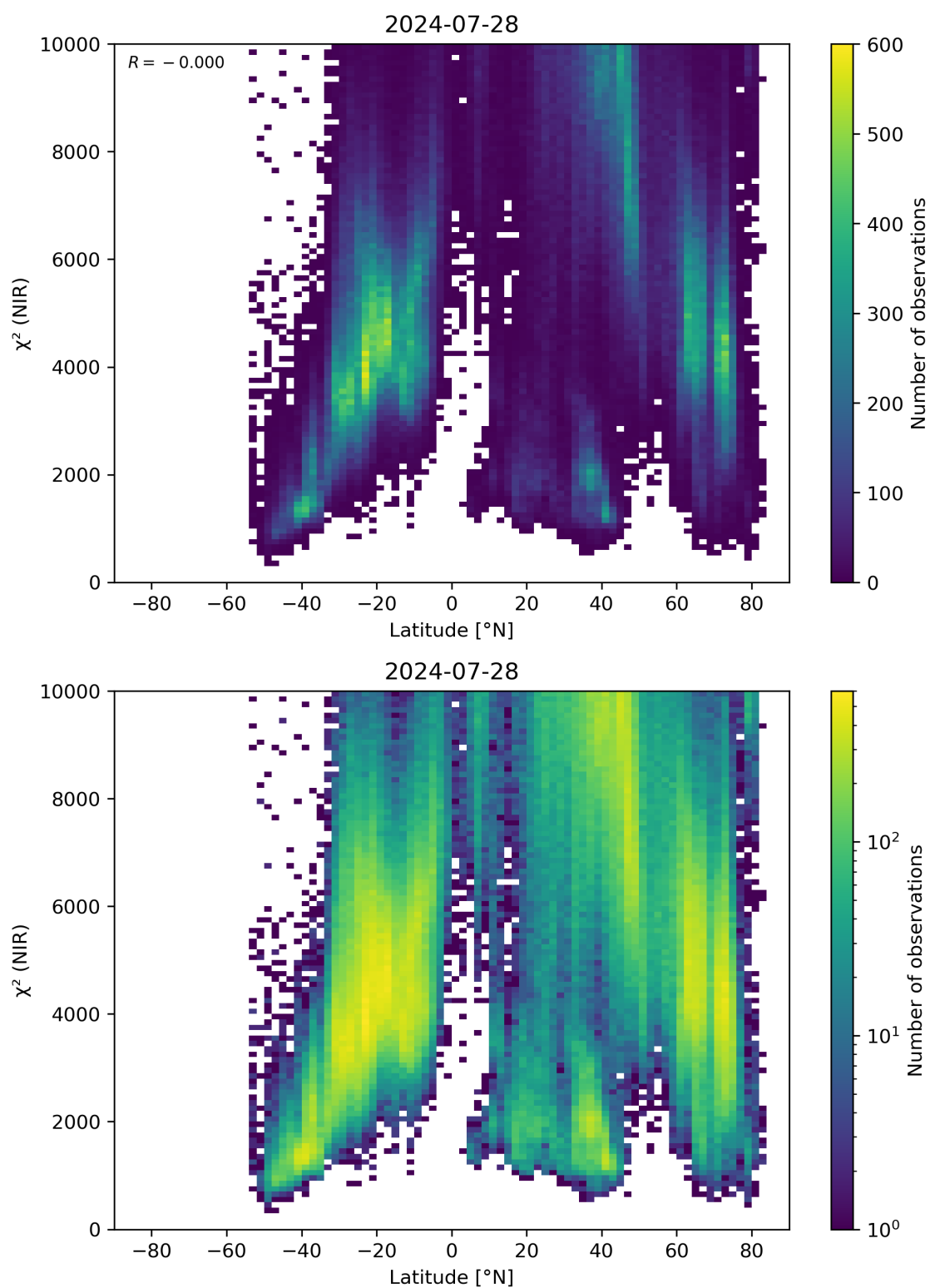
Figure 53: Scatter density plot of “Latitude” against “ \chi^2 (NIR)” for 2024-07-27 to 2024-07-29.
