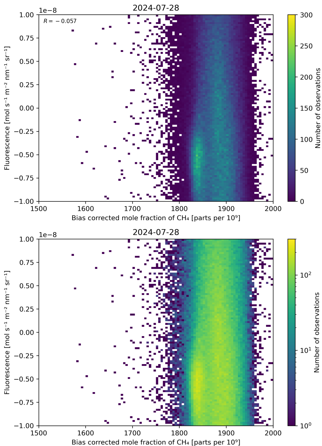
Figure 66: Scatter density plot of “Bias corrected mole fraction of \text{CH}_4 ” against “Fluorescence” for 2024-07-27 to 2024-07-29.
