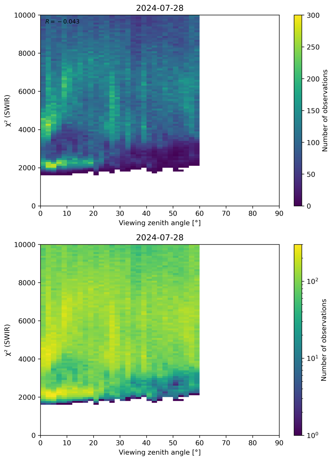
Figure 106: Scatter density plot of “Viewing zenith angle” against “ \chi^2 (SWIR)” for 2024-07-27 to 2024-07-29.
