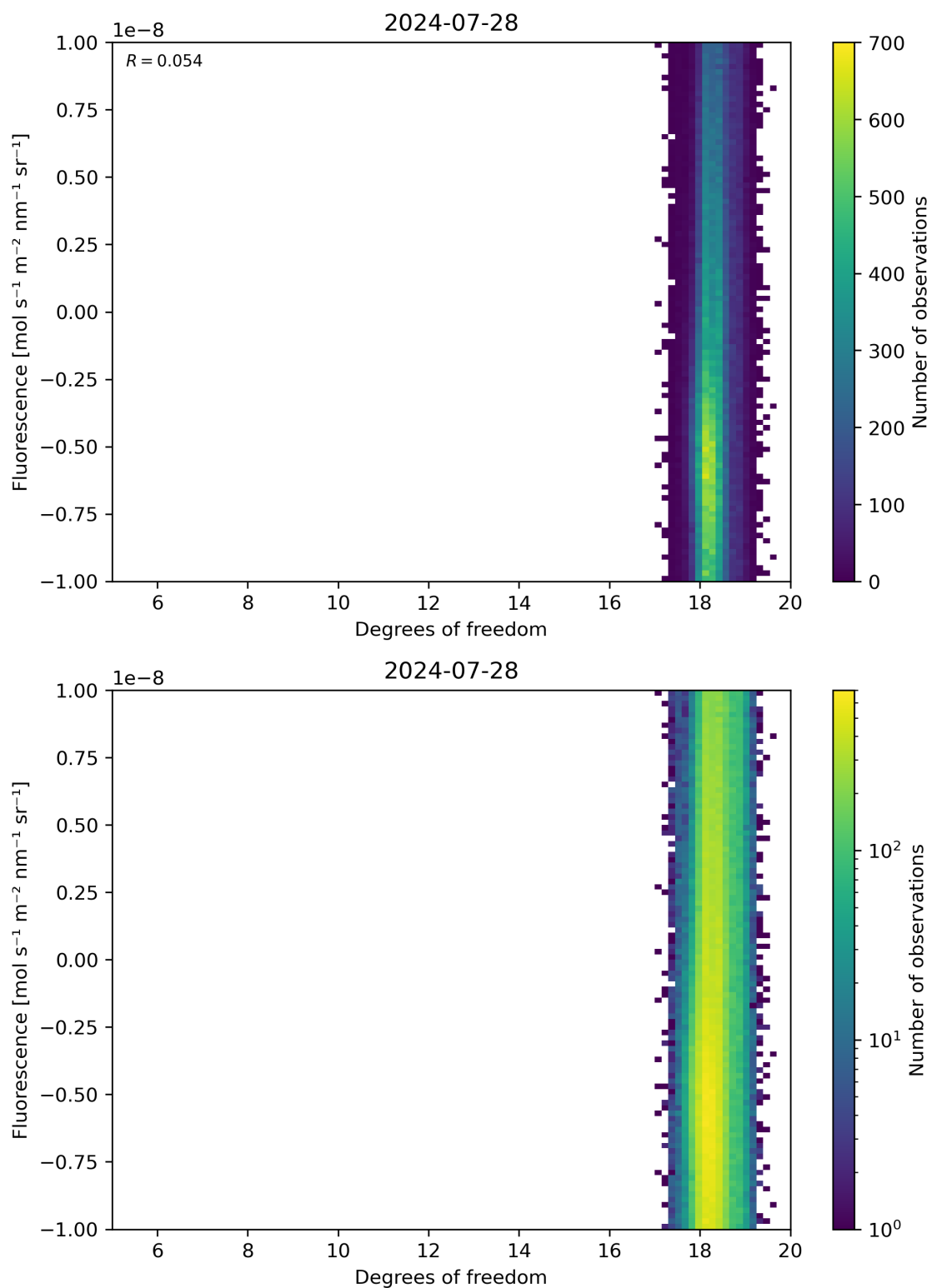
Figure 51: Scatter density plot of “Degrees of freedom” against “Fluorescence” for 2024-07-27 to 2024-07-29.
