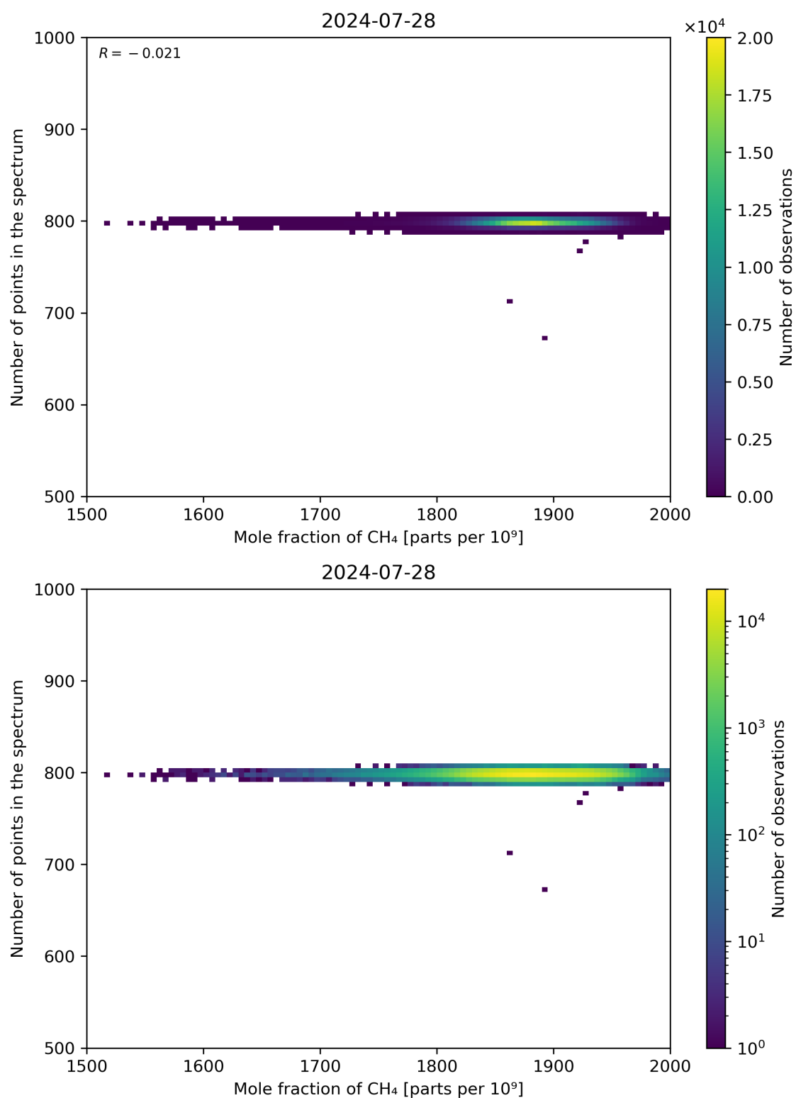
Figure 77: Scatter density plot of “Mole fraction of CH 4 ” against “Number of points in the spectrum” for 2024-07-27 to 2024-07-29.
