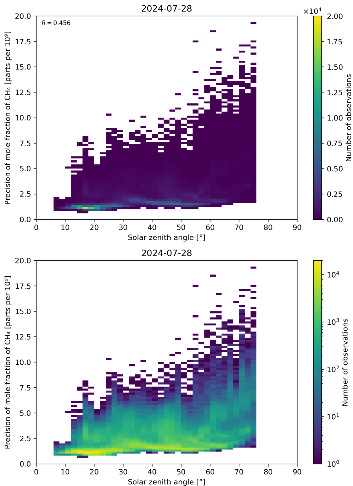
Figure 101: Scatter density plot of “Solar zenith angle” against “Precision of mole fraction of CH 4 ” for 2024-07-27 to 2024-07-29.
