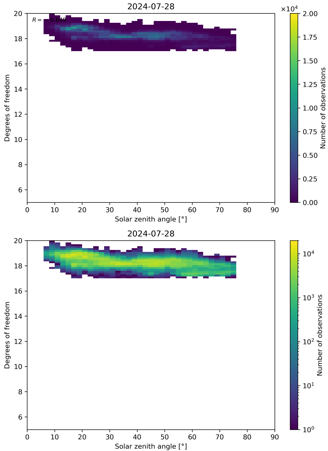
Figure 96: Scatter density plot of “Solar zenith angle” against “Degrees of freedom” for 2024-07-27 to 2024-07-29.
