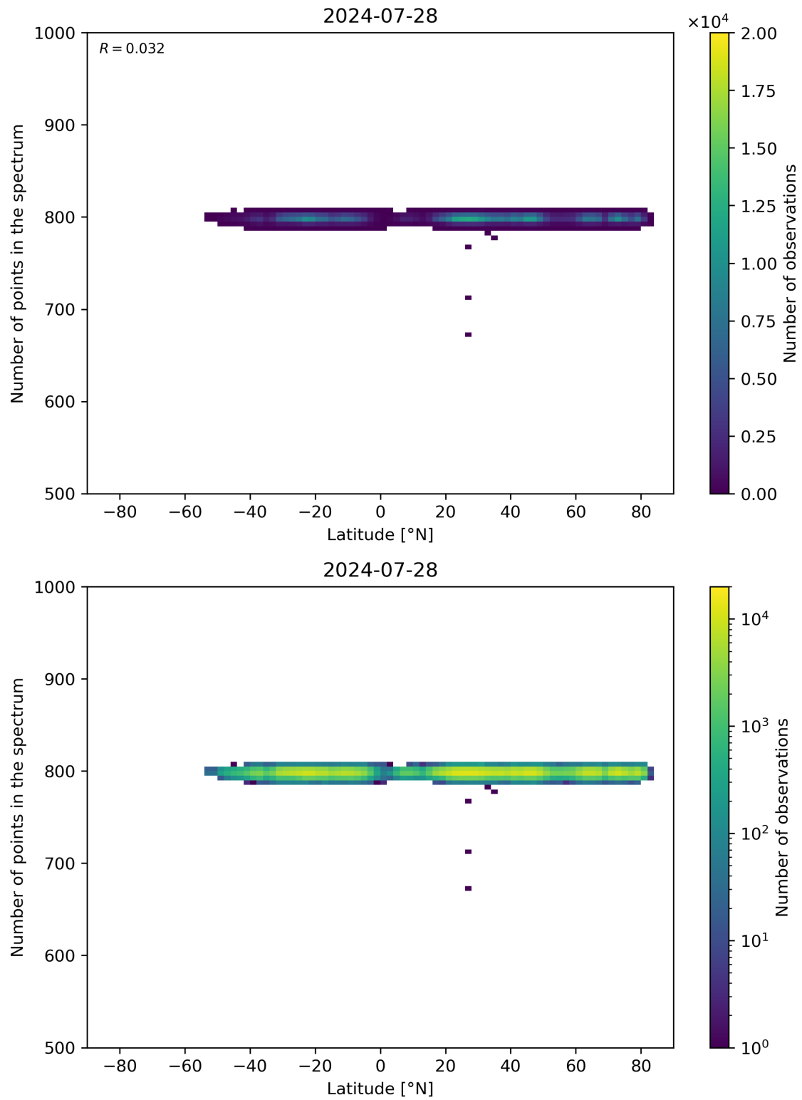
Figure 61: Scatter density plot of “Latitude” against “Number of points in the spectrum” for 2024-07-27 to 2024-07-29.
