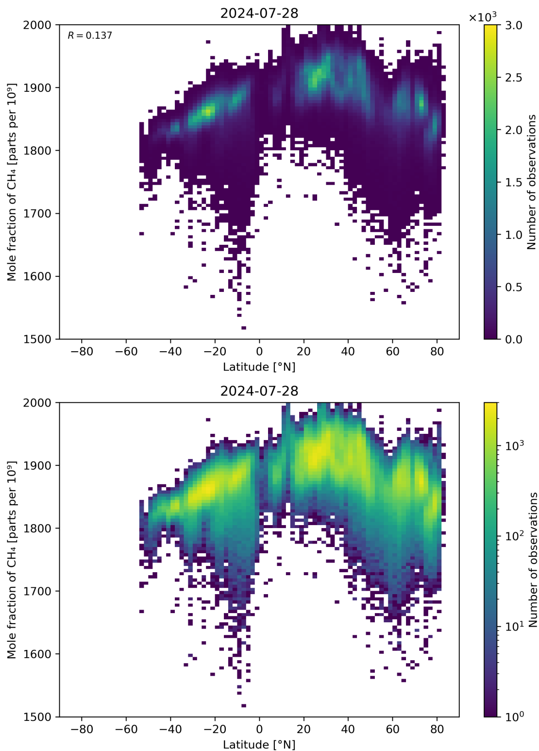
Figure 57: Scatter density plot of “Latitude” against “Mole fraction of \text{CH}_4 ” for 2024-07-27 to 2024-07-29.
