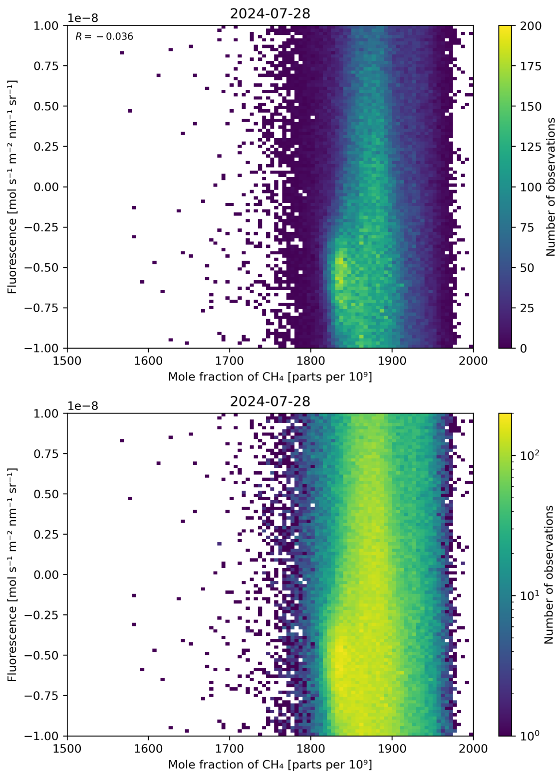
Figure 73: Scatter density plot of “Mole fraction of \text{CH}_4 ” against “Fluorescence” for 2024-07-27 to 2024-07-29.
