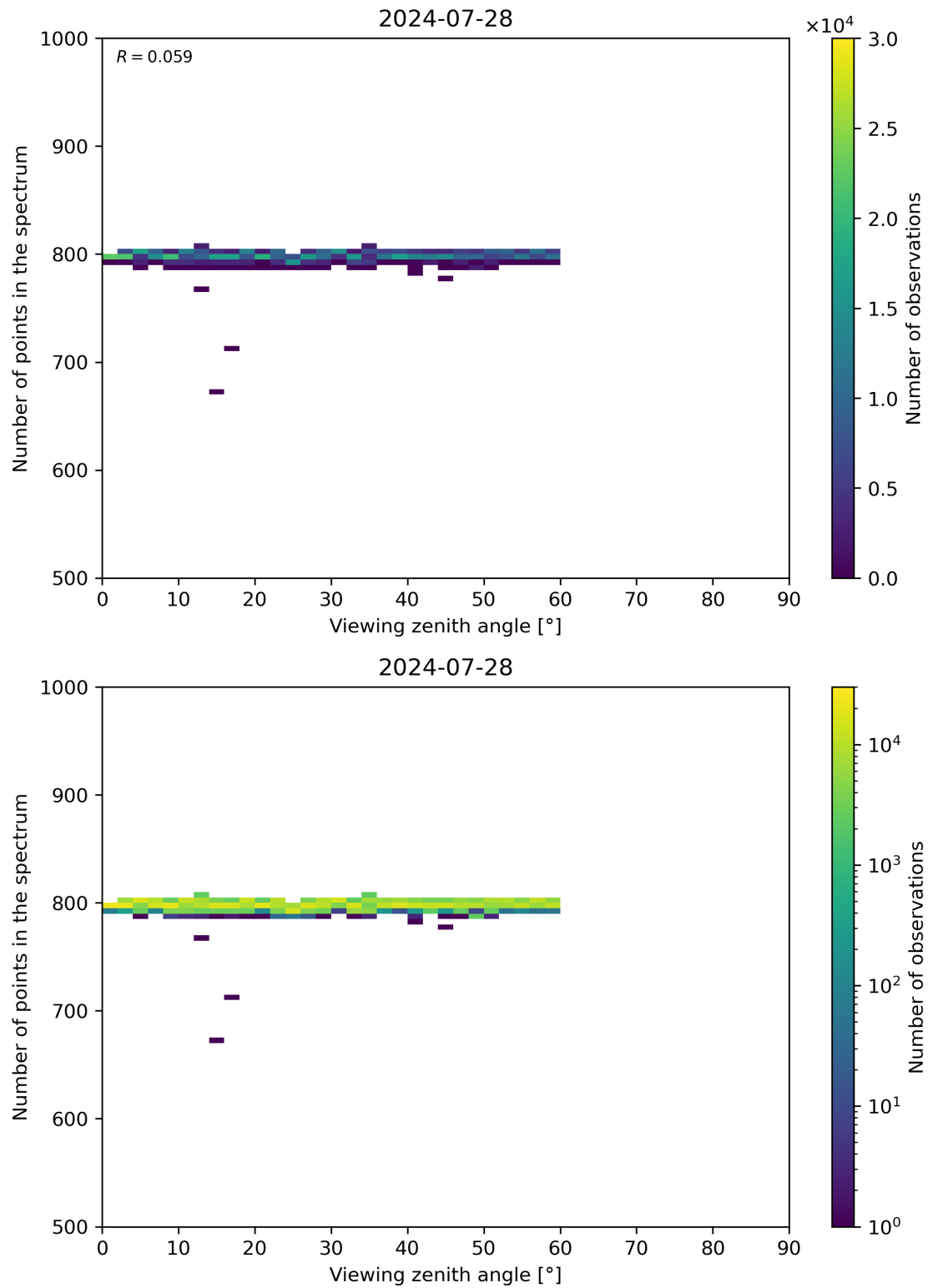
Figure 114: Scatter density plot of “Viewing zenith angle” against “Number of points in the spectrum” for 2024-07-27 to 2024-07-29.
